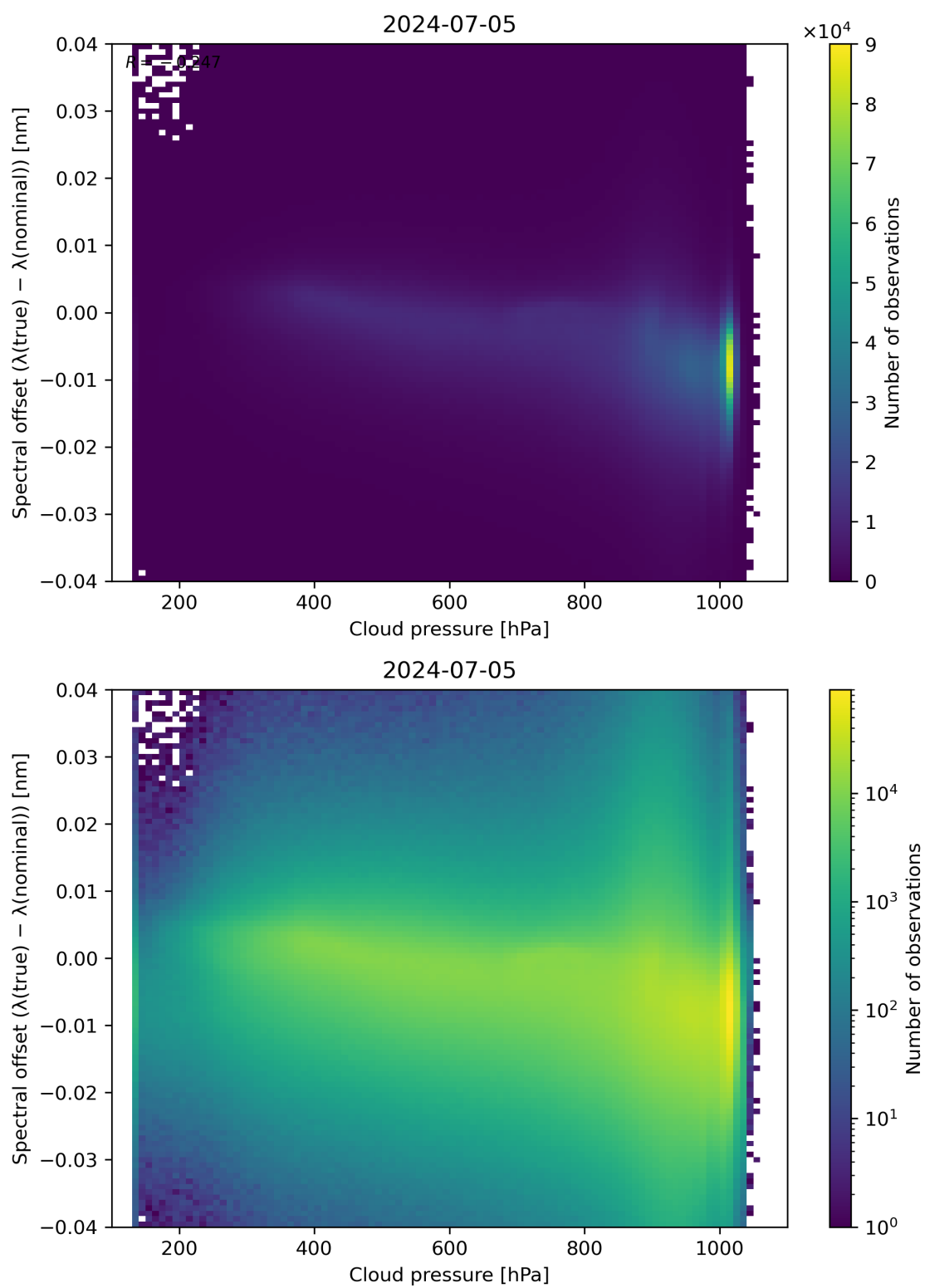
Figure 84: Scatter density plot of “Cloud pressure” against “Spectral offset ( \lambda(\text{true}) - \lambda(\text{nominal}) )” for 2024-07-05 to 2024-07-06.
