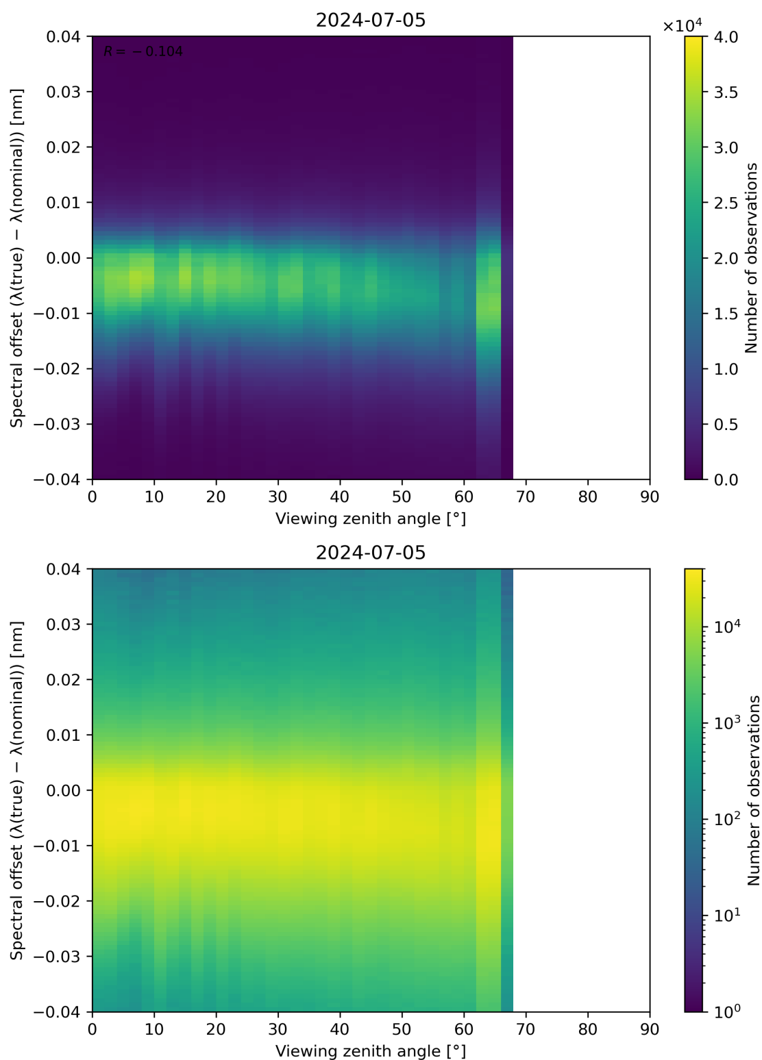
Figure 128: Scatter density plot of “Viewing zenith angle” against “Spectral offset ( \lambda(\text{true}) - \lambda(\text{nominal}) )” for 2024-07-05 to 2024-07-06.
