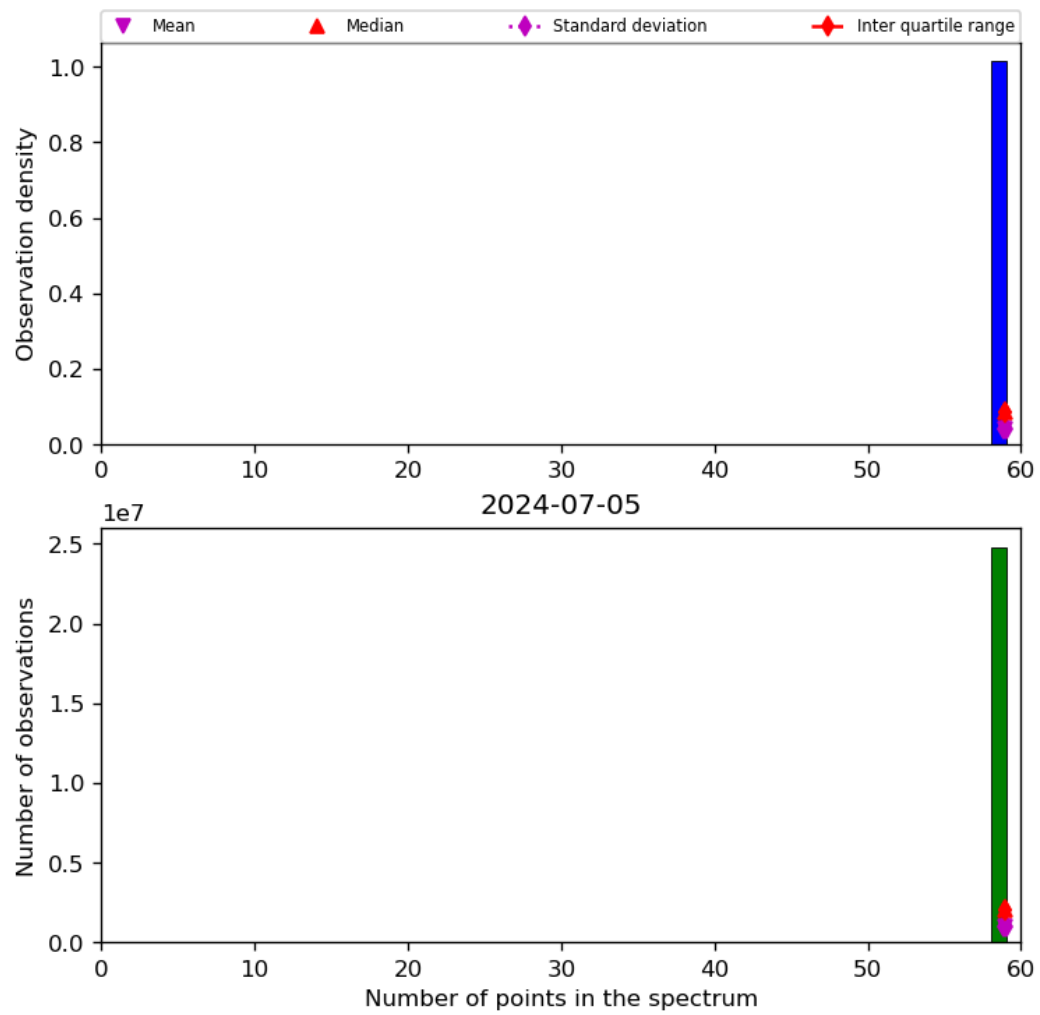
Figure 44: Histogram of “Number of points in the spectrum” for 2024-07-05 to 2024-07-06
