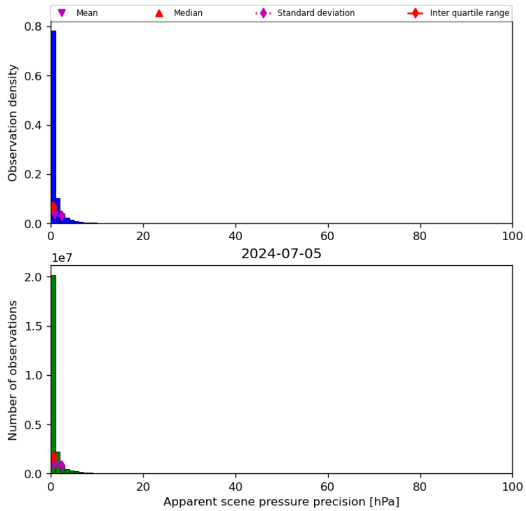
Figure 37: Histogram of “Apparent scene pressure precision” for 2024-07-05 to 2024-07-06
