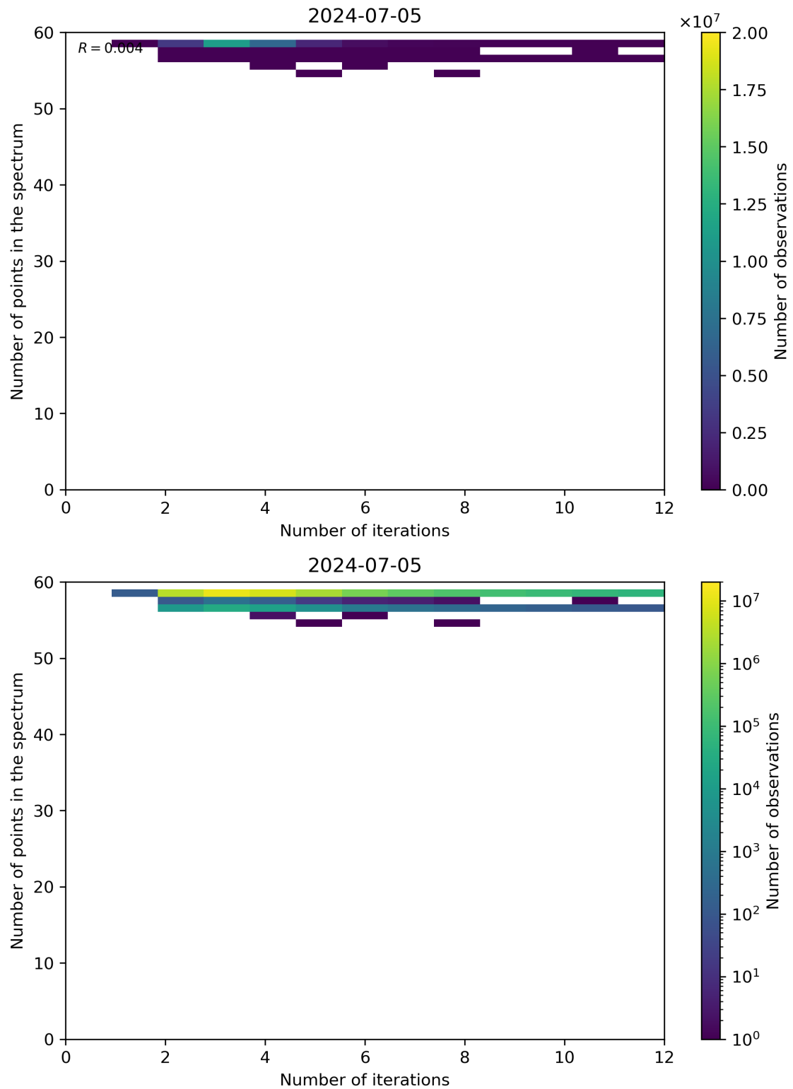
Figure 99: Scatter density plot of “Number of iterations” against “Number of points in the spectrum” for 2024-07-05 to 2024-07-06.
