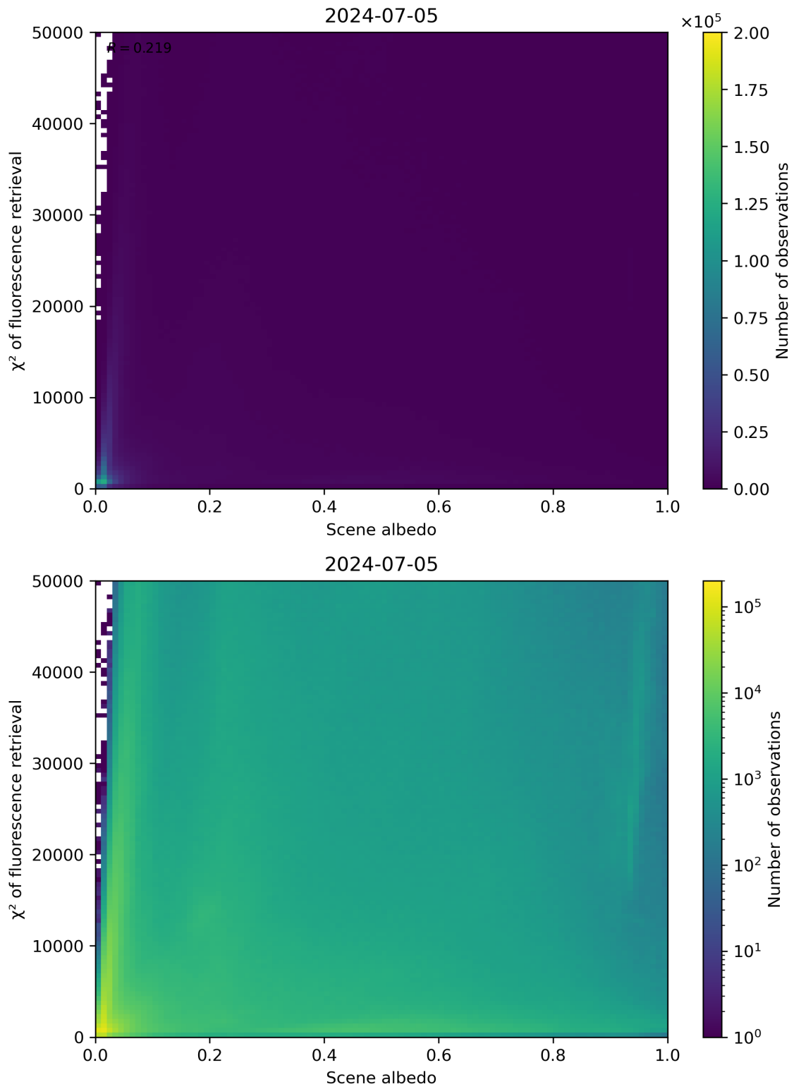
Figure 103: Scatter density plot of “Scene albedo” against “ \chi^2 of fluorescence retrieval” for 2024-07-05 to 2024-07-06.
