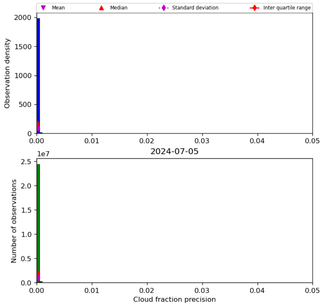
Figure 33: Histogram of “Cloud fraction precision” for 2024-07-05 to 2024-07-06
