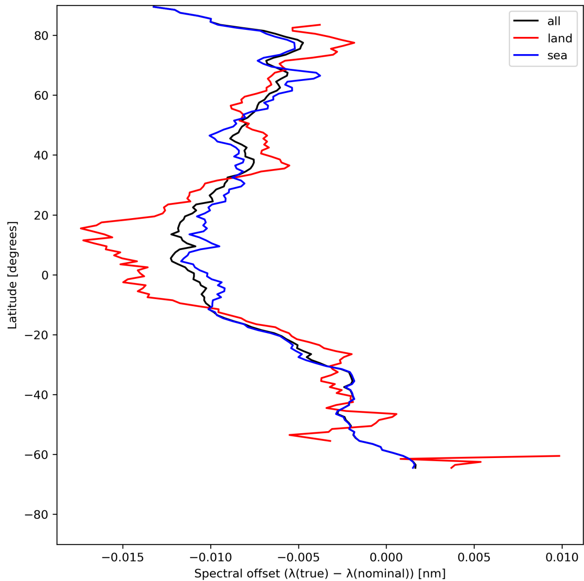
Figure 28: Zonal average of “Spectral offset ( \lambda(\text{true}) - \lambda(\text{nominal}) )” for 2024-07-05 to 2024-07-06.
