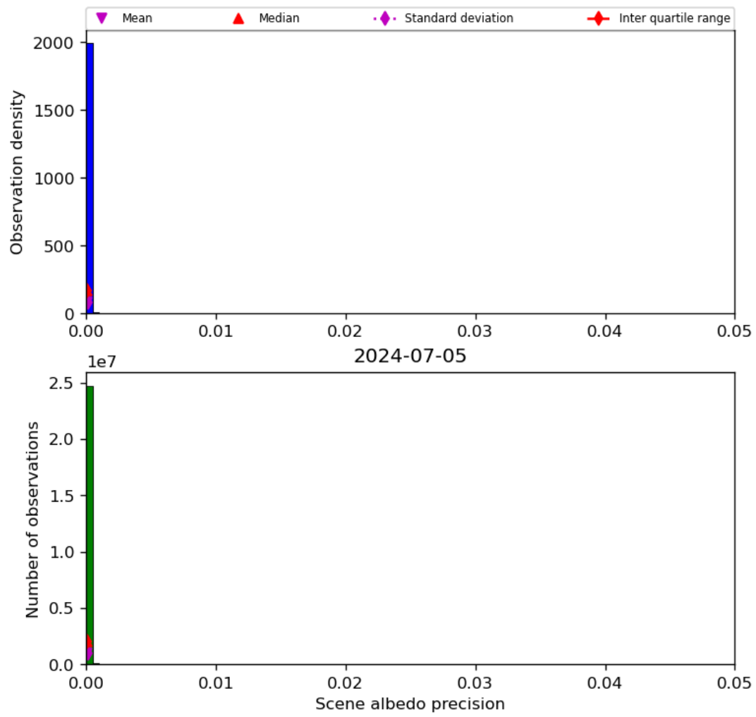
Figure 35: Histogram of “Scene albedo precision” for 2024-07-05 to 2024-07-06
