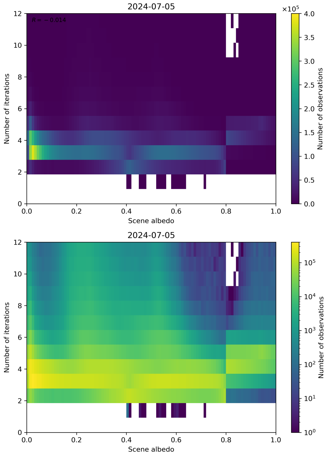
Figure 105: Scatter density plot of “Scene albedo” against “Number of iterations” for 2024-07-05 to 2024-07-06.
