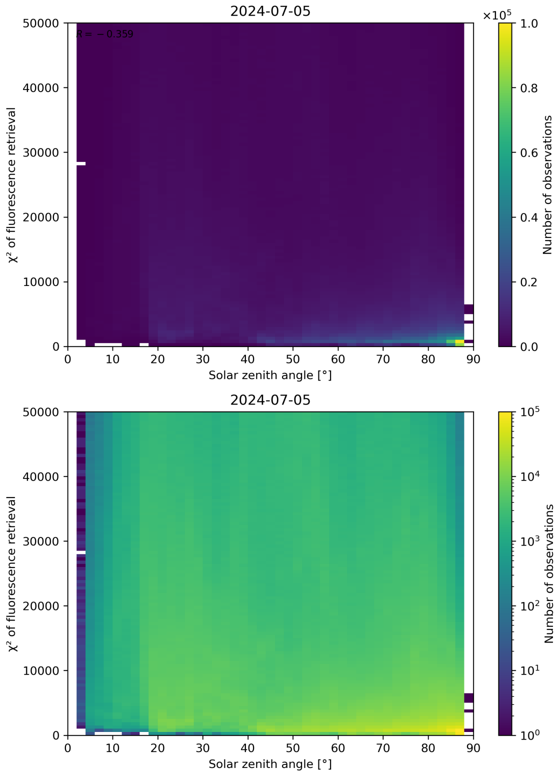
Figure 109: Scatter density plot of “Solar zenith angle” against “ \chi^2 of fluorescence retrieval” for 2024-07-05 to 2024-07-06.
