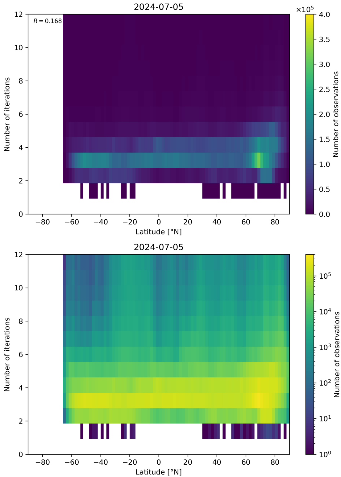
Figure 93: Scatter density plot of “Latitude” against “Number of iterations” for 2024-07-05 to 2024-07-06.
