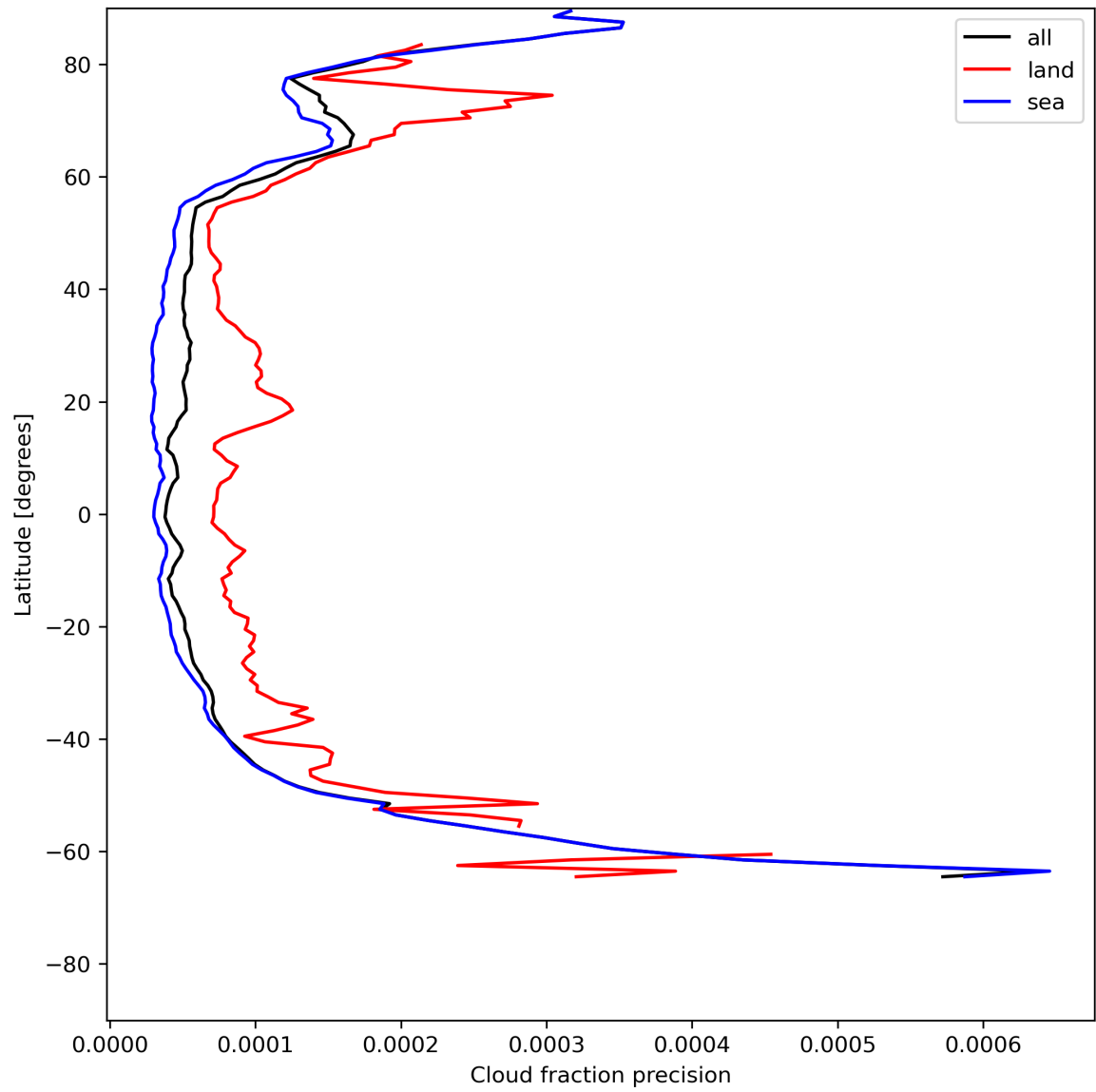
Figure 16: Zonal average of “Cloud fraction precision” for 2024-07-05 to 2024-07-06.
