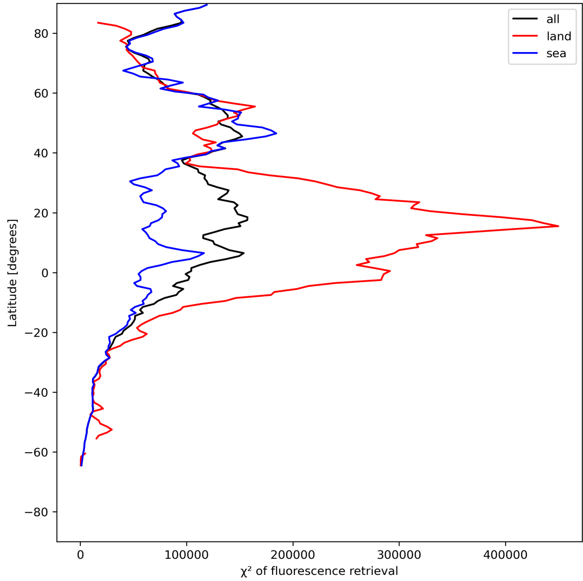
Figure 25: Zonal average of “ \chi^2 of fluorescence retrieval” for 2024-07-05 to 2024-07-06.
