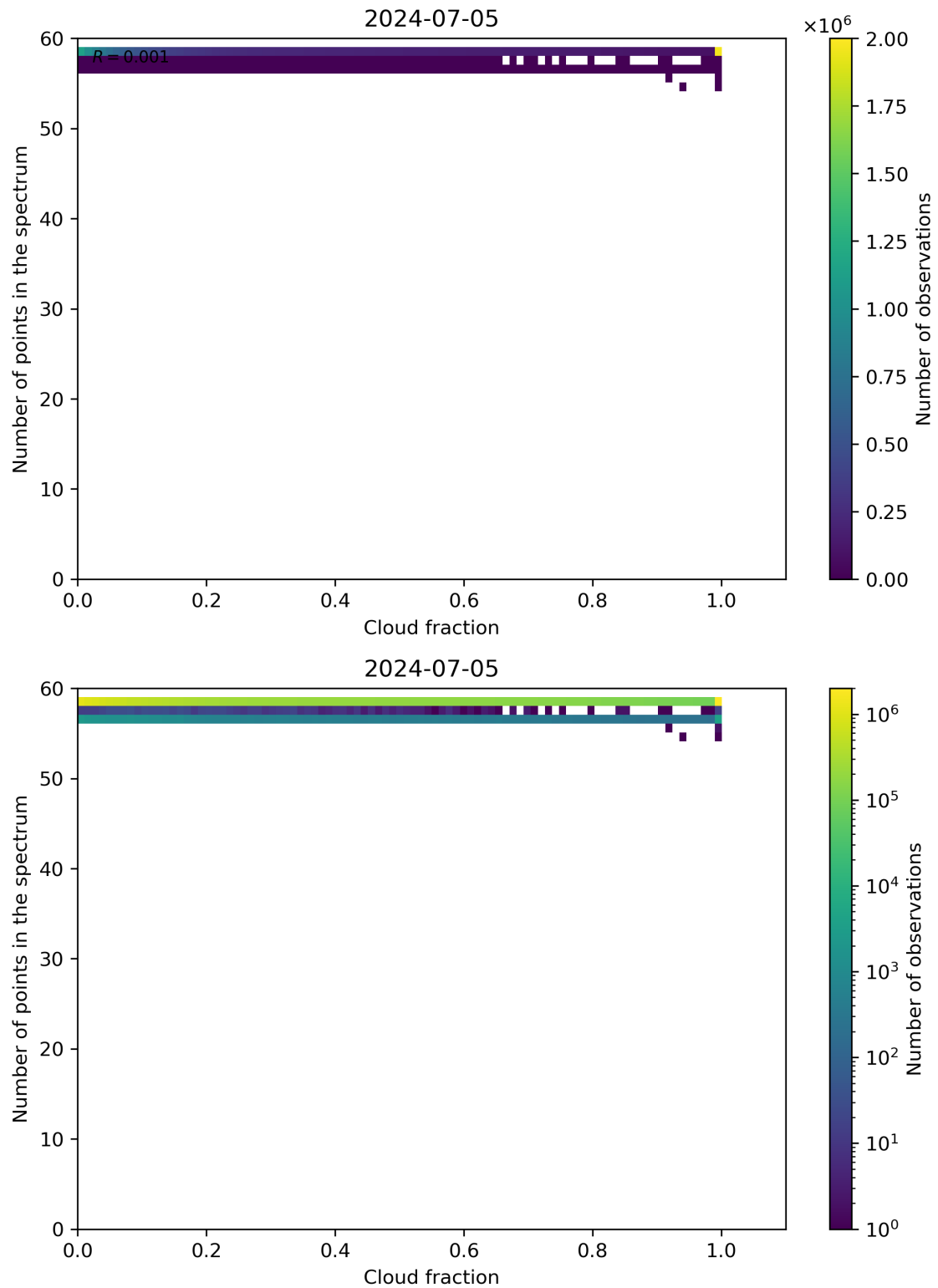
Figure 74: Scatter density plot of “Cloud fraction” against “Number of points in the spectrum” for 2024-07-05 to 2024-07-06.
