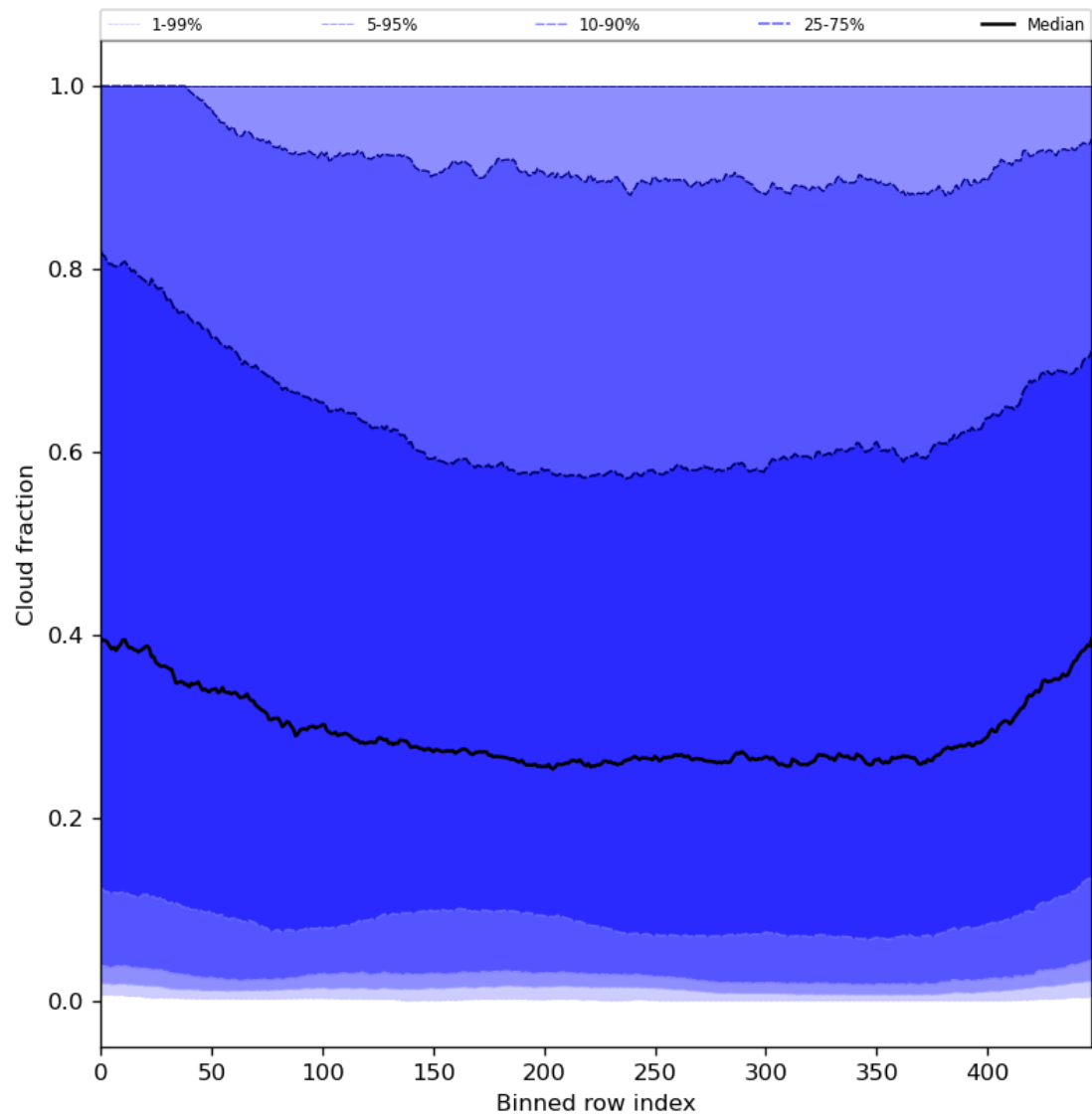
Figure 49: Along track statistics of “Cloud fraction” for 2024-07-05 to 2024-07-06
