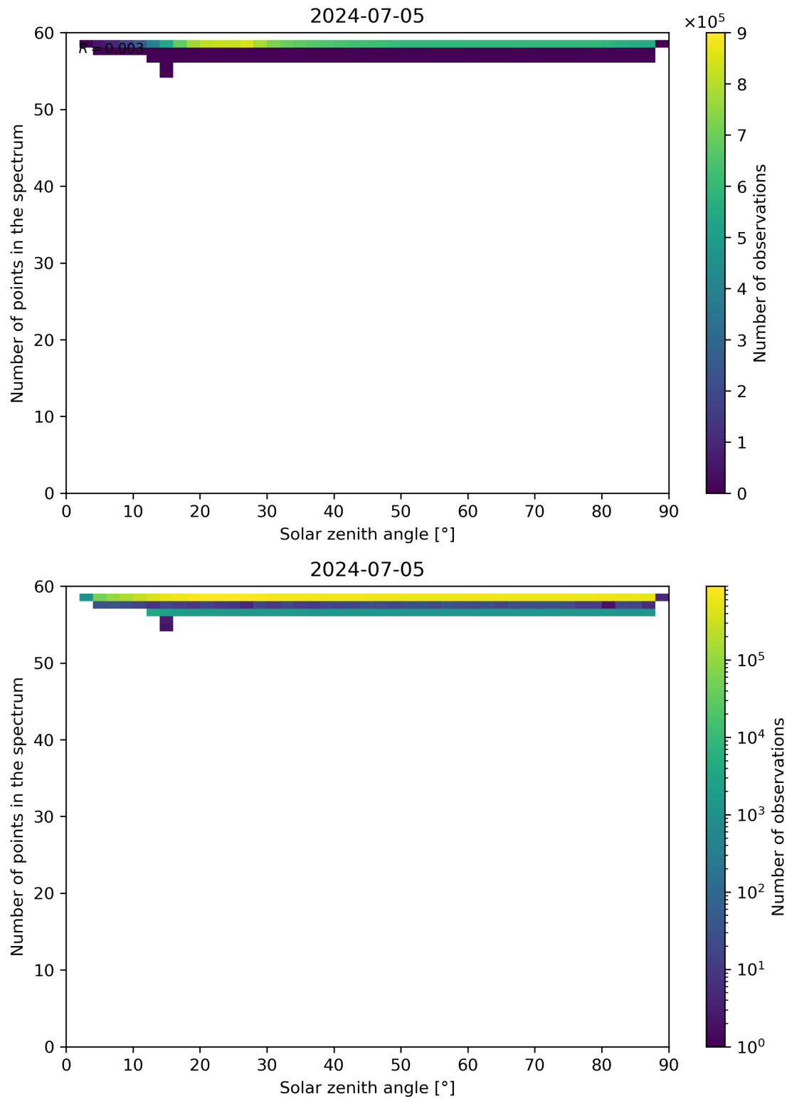
Figure 115: Scatter density plot of “Solar zenith angle” against “Number of points in the spectrum” for 2024-07-05 to 2024-07-06.
