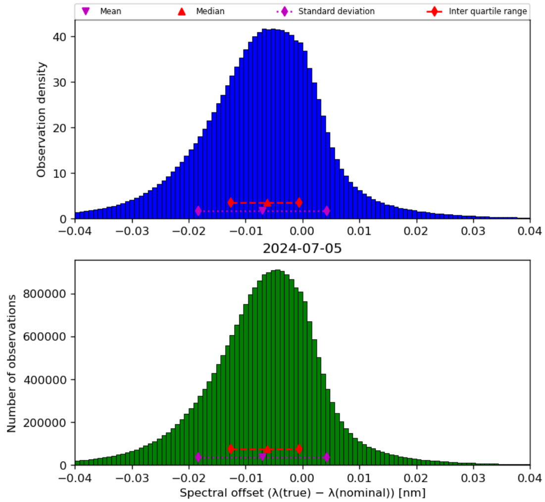
Figure 45: Histogram of “Spectral offset ( \lambda(\text{true}) - \lambda(\text{nominal}) )” for 2024-07-05 to 2024-07-06
