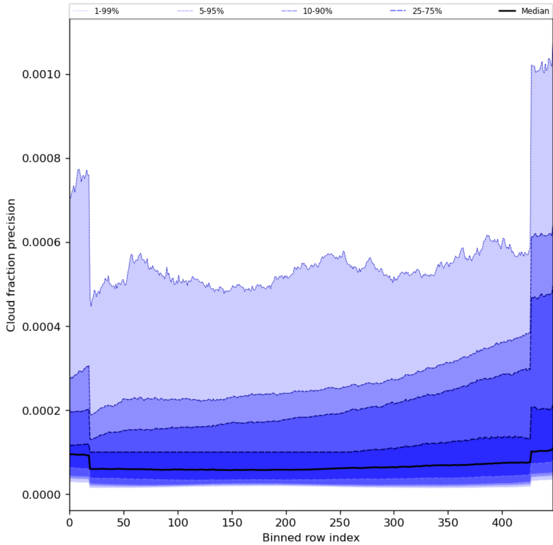
Figure 50: Along track statistics of “Cloud fraction precision” for 2024-07-05 to 2024-07-06
