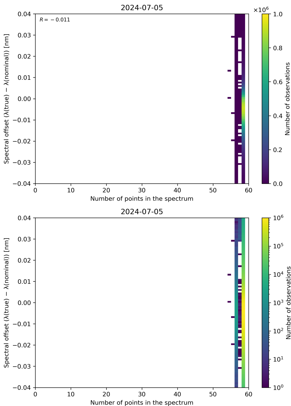
Figure 101: Scatter density plot of “Number of points in the spectrum” against “Spectral offset ( \lambda(\text{true}) - \lambda(\text{nominal}) )” for 2024-07-05 to 2024-07-06.
