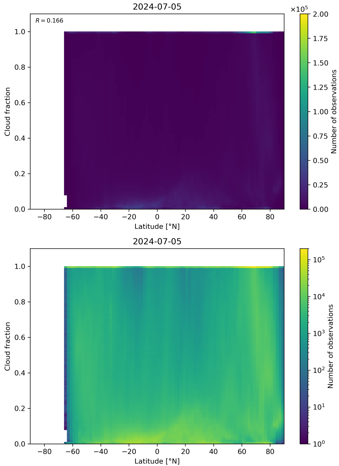
Figure 90: Scatter density plot of “Latitude” against “Cloud fraction” for 2024-07-05 to 2024-07-06.
