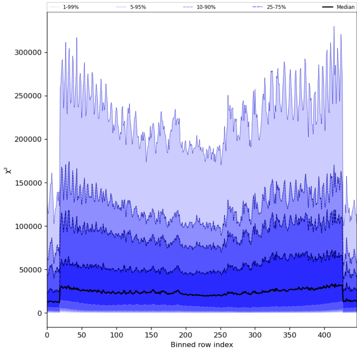
Figure 55: Along track statistics of “ \chi^2 ” for 2024-07-05 to 2024-07-06
