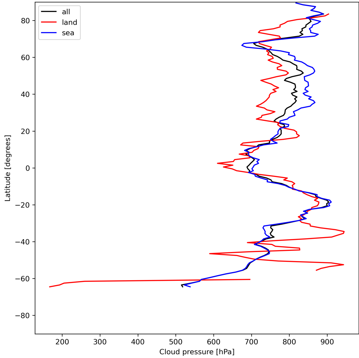
Figure 13: Zonal average of “Cloud pressure” for 2024-07-05 to 2024-07-06.
