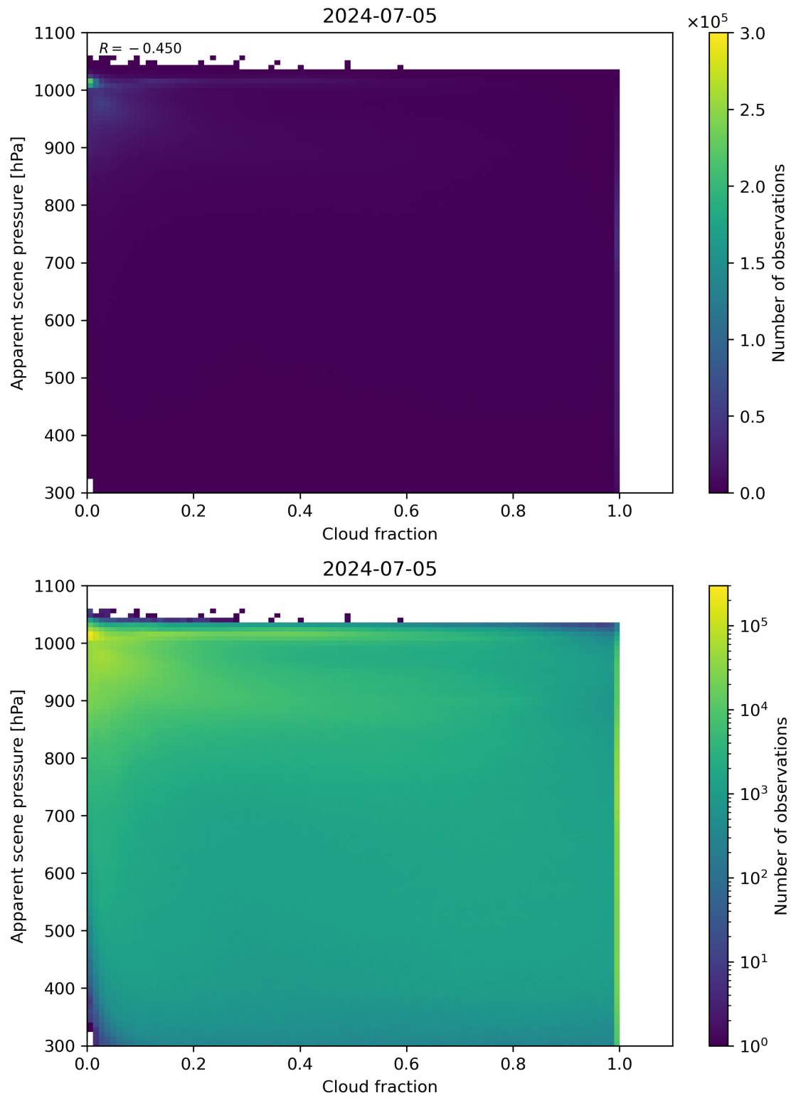
Figure 70: Scatter density plot of “Cloud fraction” against “Apparent scene pressure” for 2024-07-05 to 2024-07-06.
