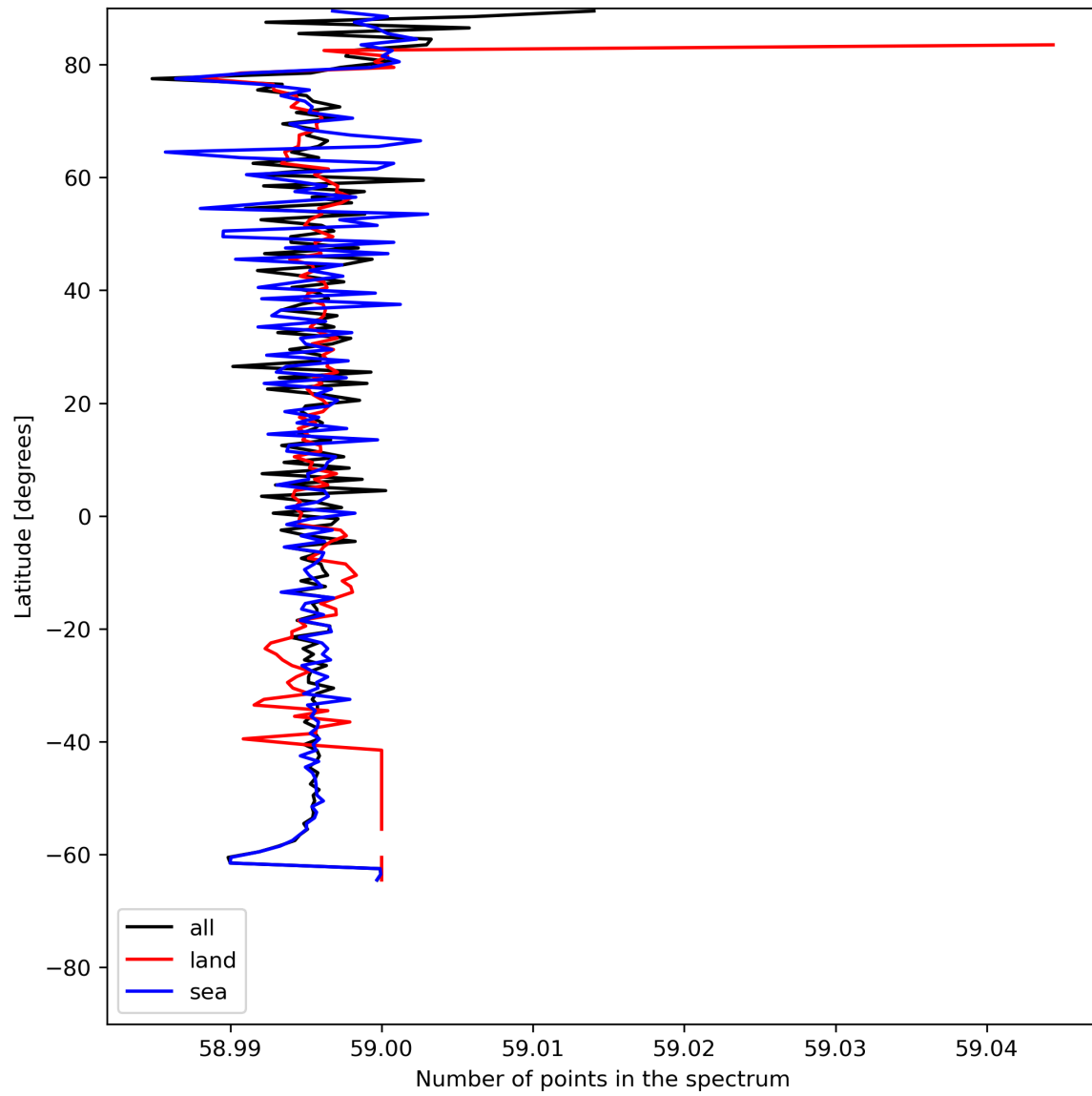
Figure 27: Zonal average of “Number of points in the spectrum” for 2024-07-05 to 2024-07-06.
