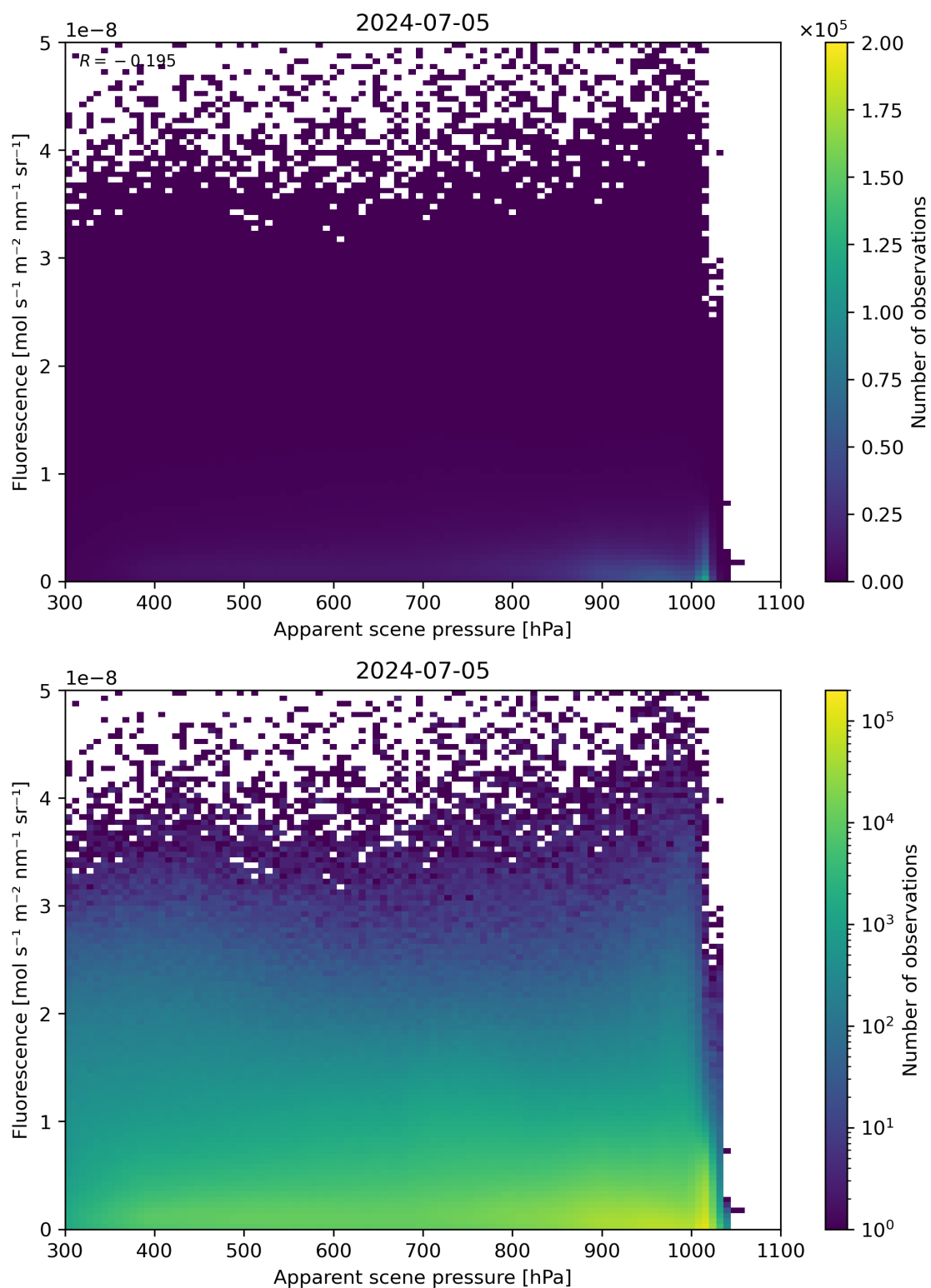
Figure 64: Scatter density plot of “Apparent scene pressure” against “Fluorescence” for 2024-07-05 to 2024-07-06.
