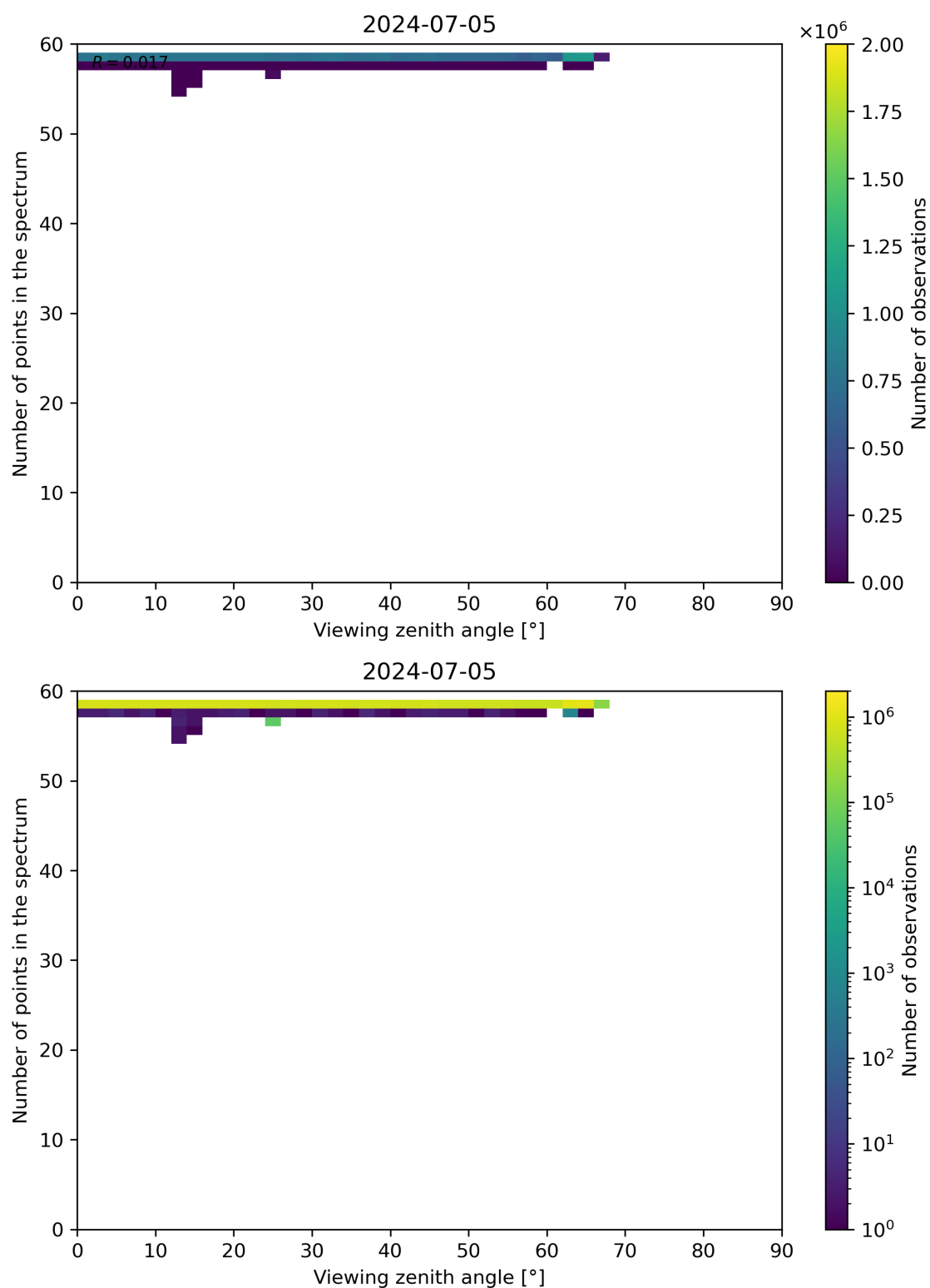
Figure 125: Scatter density plot of “Viewing zenith angle” against “Number of points in the spectrum” for 2024-07-05 to 2024-07-06.
