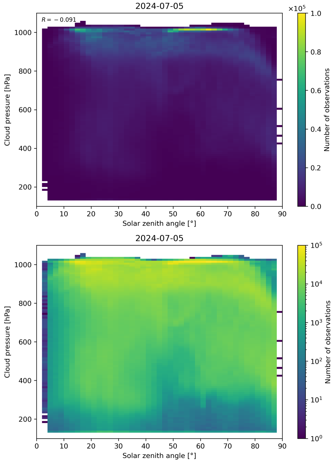
Figure 111: Scatter density plot of “Solar zenith angle” against “Cloud pressure” for 2024-07-05 to 2024-07-06.
