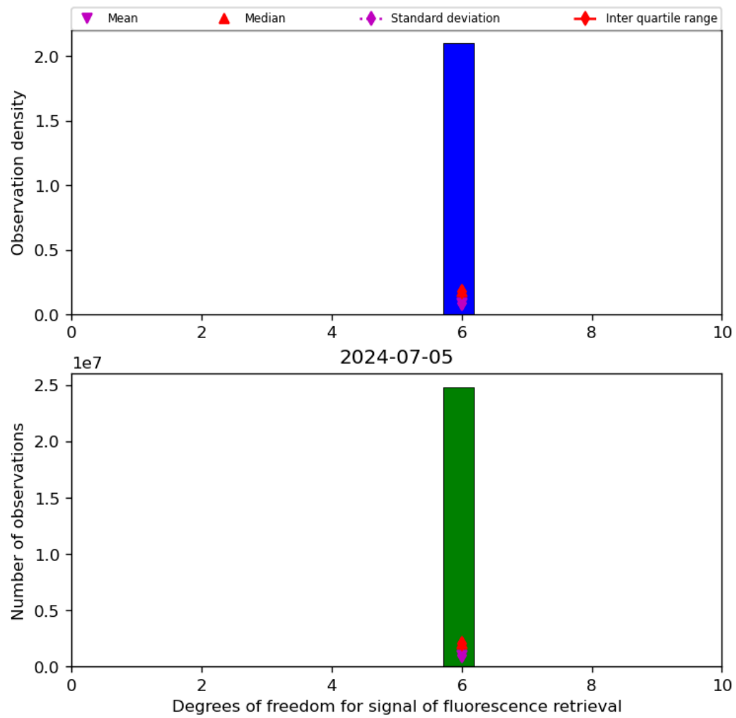
Figure 43: Histogram of “Degrees of freedom for signal of fluorescence retrieval” for 2024-07-05 to 2024-07-06
