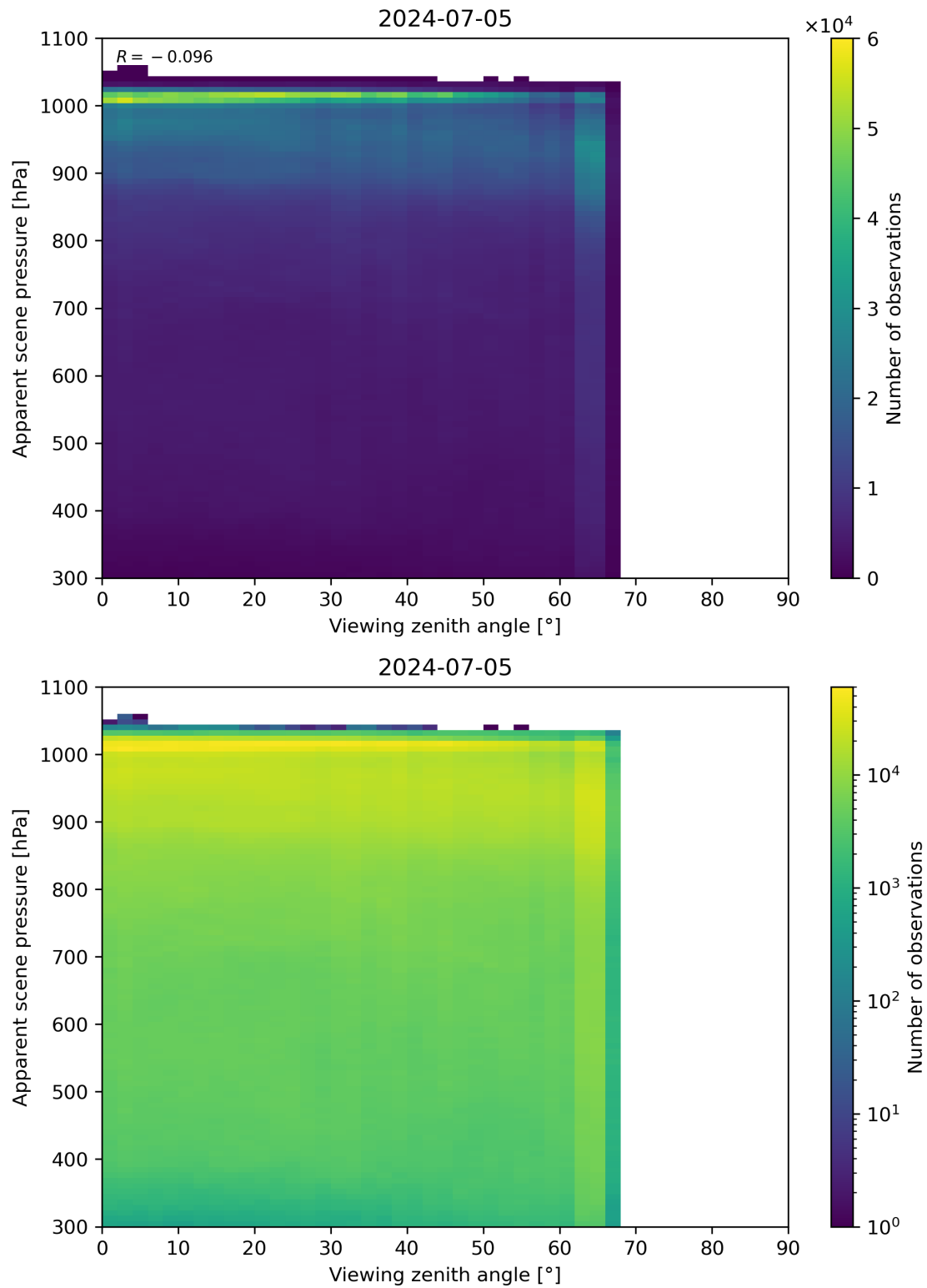
Figure 118: Scatter density plot of “Viewing zenith angle” against “Apparent scene pressure” for 2024-07-05 to 2024-07-06.
