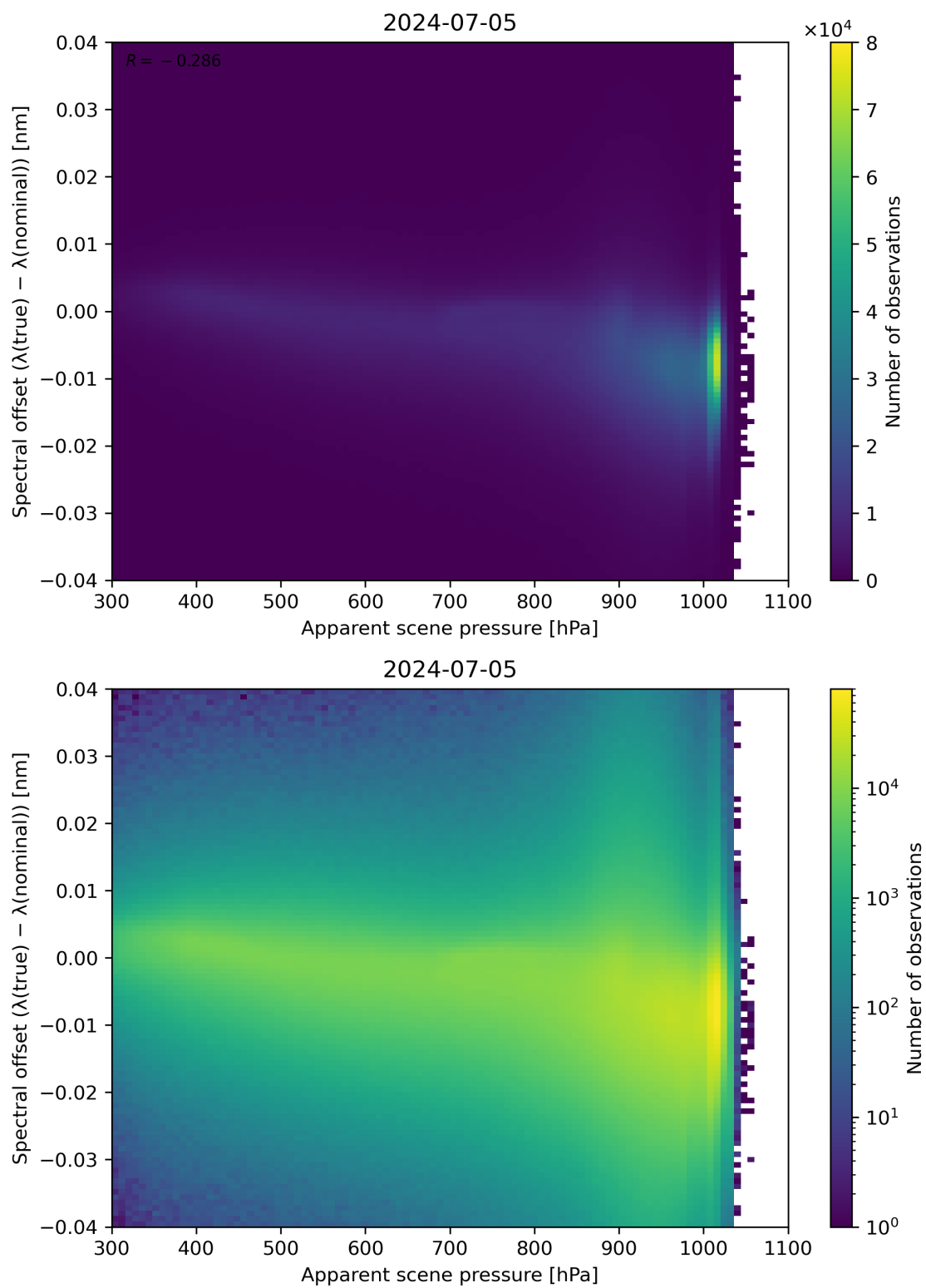
Figure 67: Scatter density plot of “Apparent scene pressure” against “Spectral offset ( \lambda(\text{true}) - \lambda(\text{nominal}) )” for 2024-07-05 to 2024-07-06.
