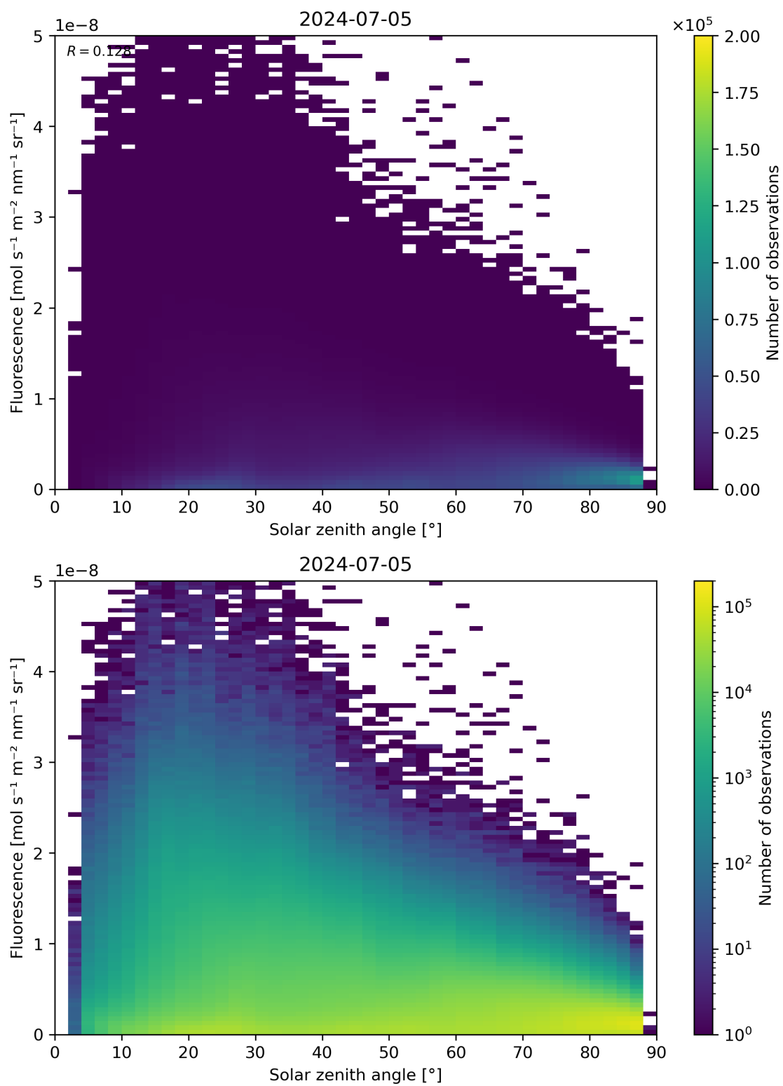
Figure 112: Scatter density plot of “Solar zenith angle” against “Fluorescence” for 2024-07-05 to 2024-07-06.
