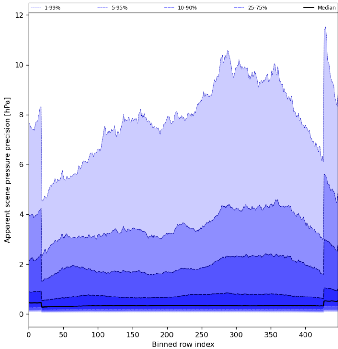
Figure 54: Along track statistics of “Apparent scene pressure precision” for 2024-07-05 to 2024-07-06
