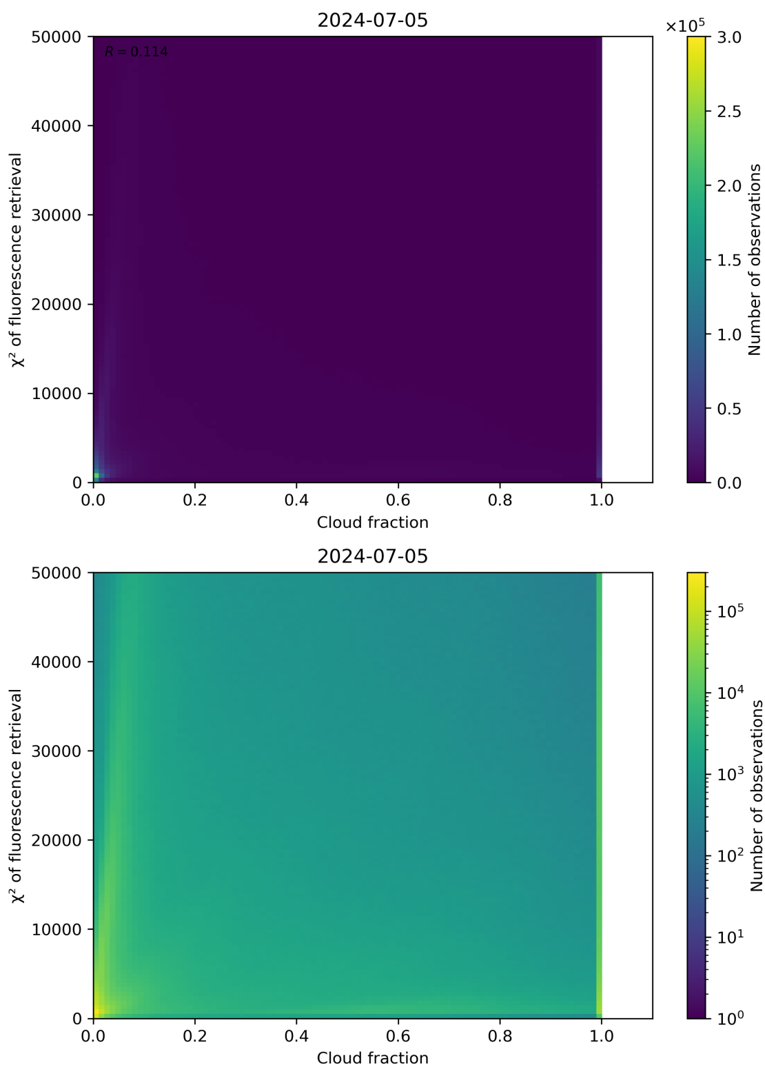
Figure 71: Scatter density plot of “Cloud fraction” against “ \chi^2 of fluorescence retrieval” for 2024-07-05 to 2024-07-06.
