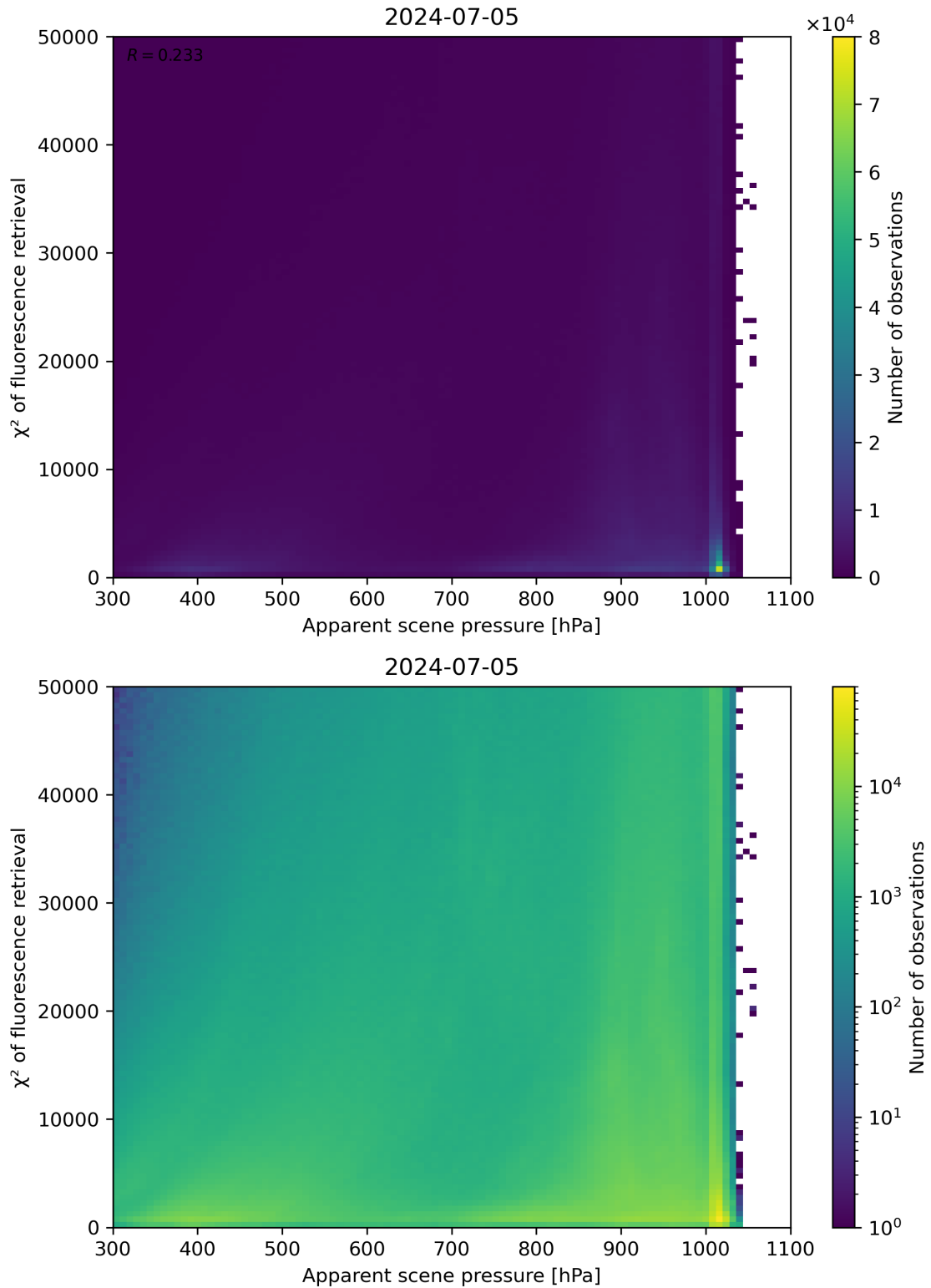
Figure 63: Scatter density plot of “Apparent scene pressure” against “ \chi^2 of fluorescence retrieval” for 2024-07-05 to 2024-07-06.
