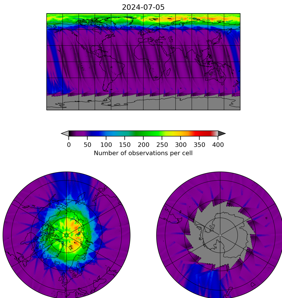
Figure 11: Map of the number of observations for 2024-07-05 to 2024-07-06
