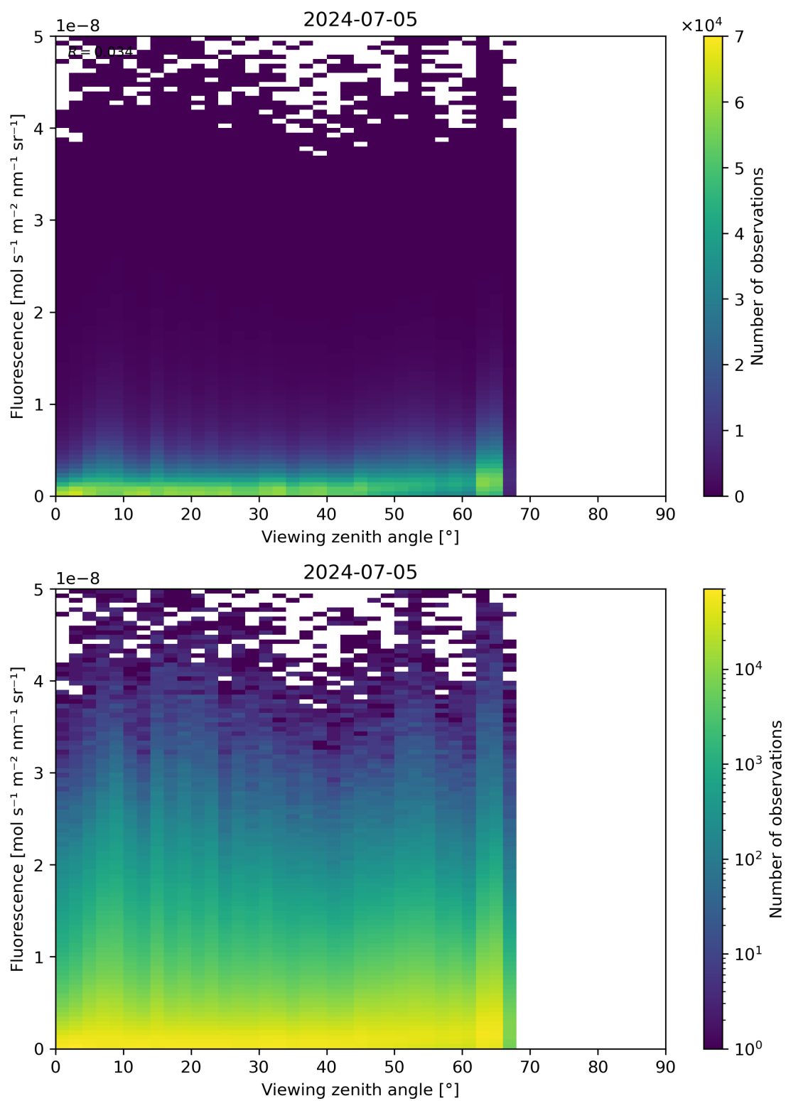
Figure 122: Scatter density plot of “Viewing zenith angle” against “Fluorescence” for 2024-07-05 to 2024-07-06.
