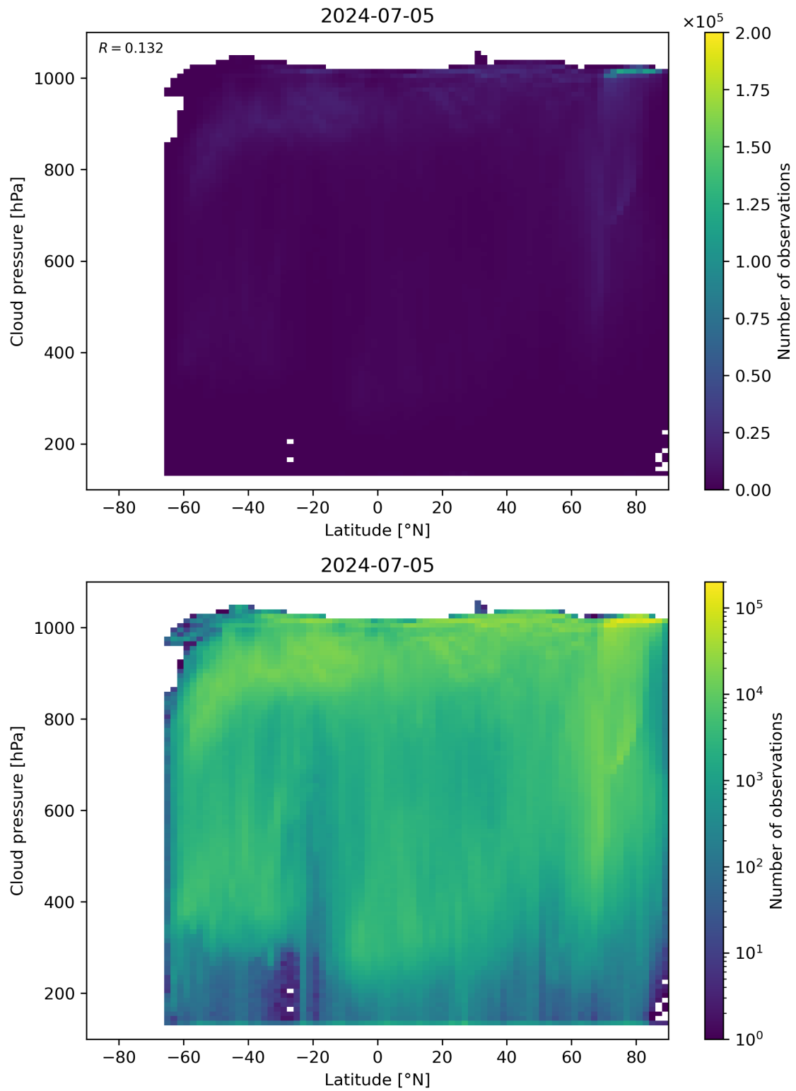
Figure 91: Scatter density plot of “Latitude” against “Cloud pressure” for 2024-07-05 to 2024-07-06.
