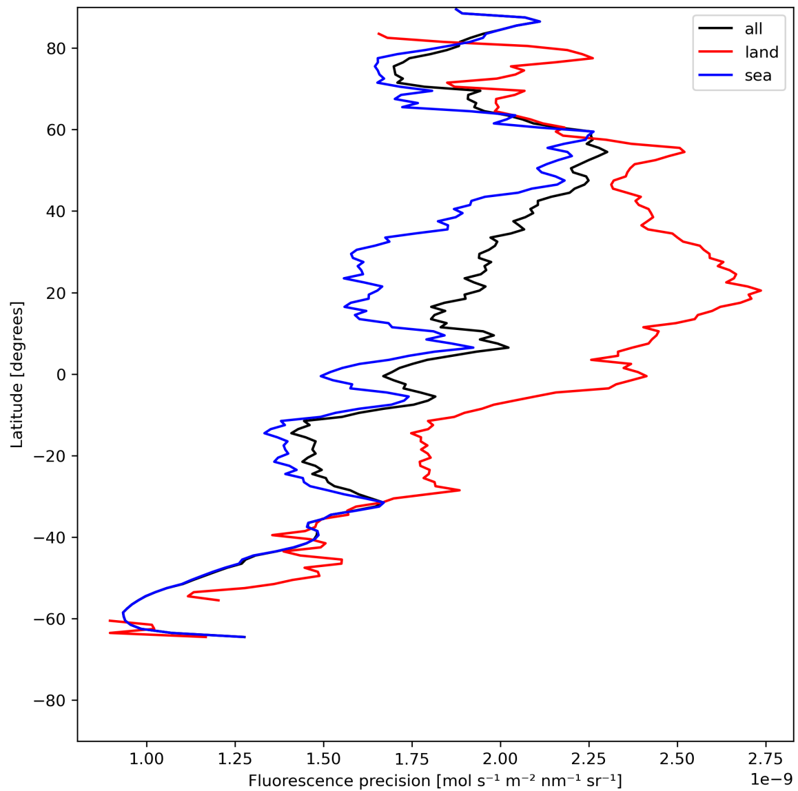
Figure 24: Zonal average of “Fluorescence precision” for 2024-07-05 to 2024-07-06.
