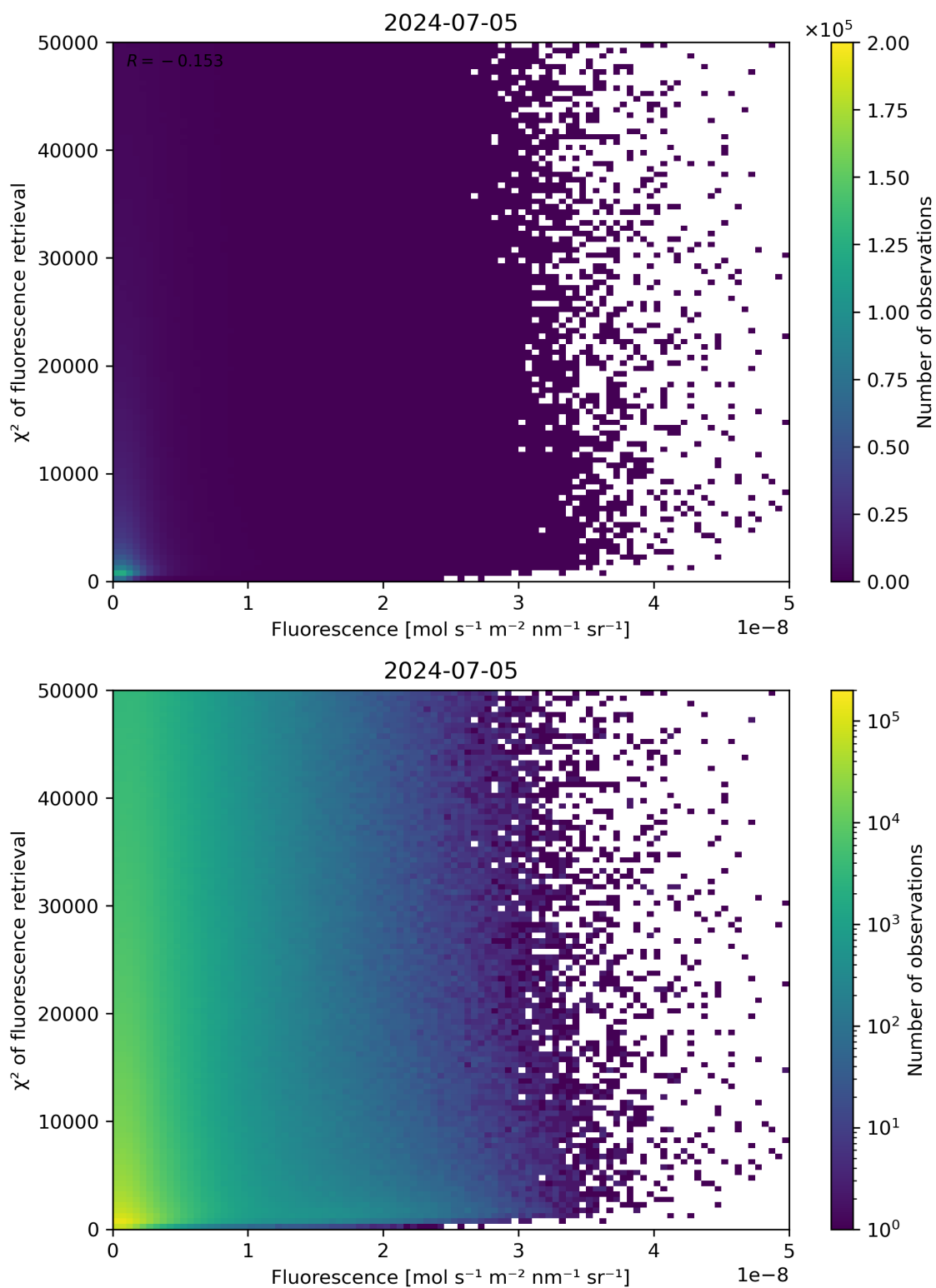
Figure 85: Scatter density plot of “Fluorescence” against “ \chi^2 of fluorescence retrieval” for 2024-07-05 to 2024-07-06.
