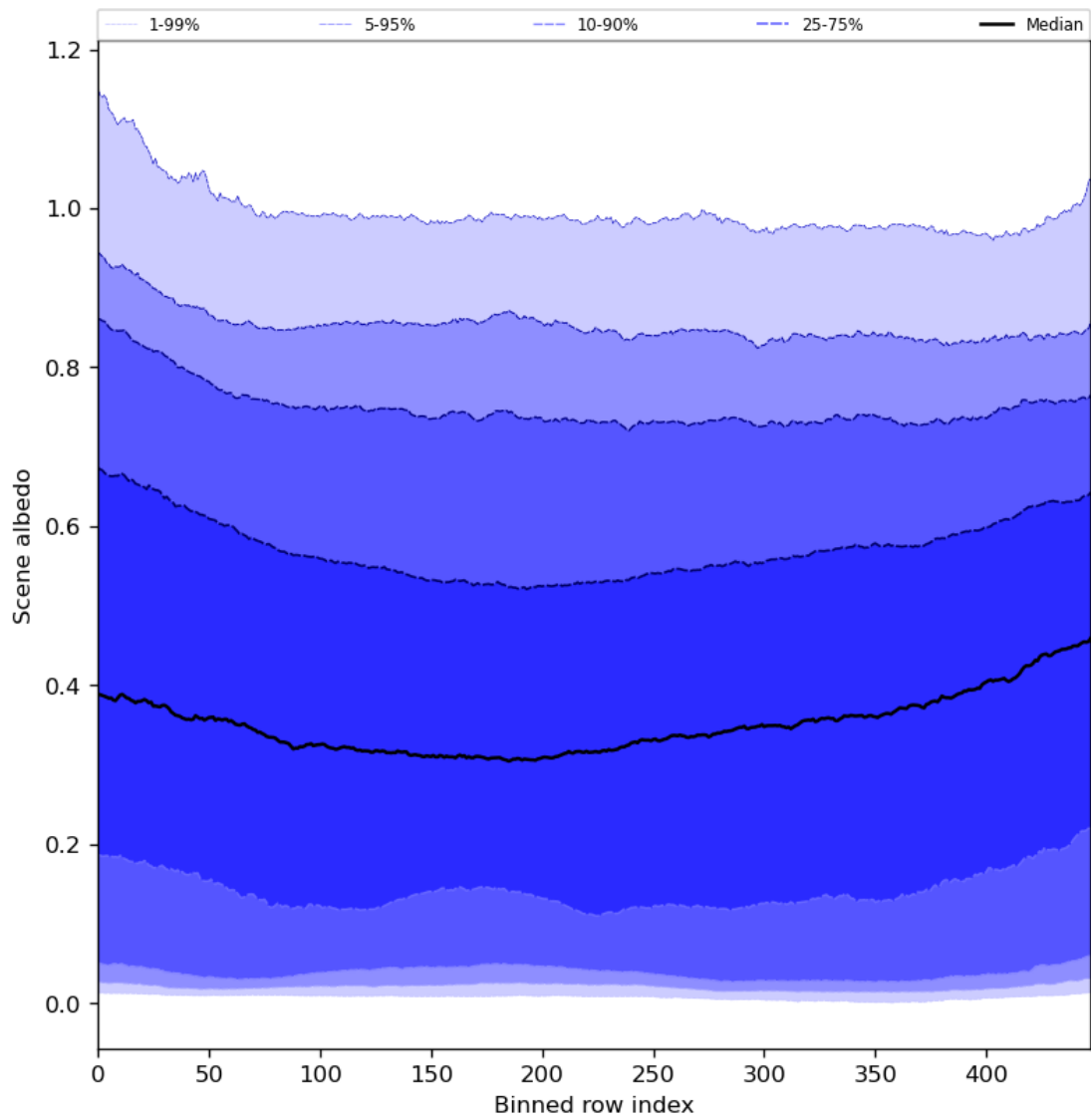
Figure 51: Along track statistics of “Scene albedo” for 2024-07-05 to 2024-07-06
