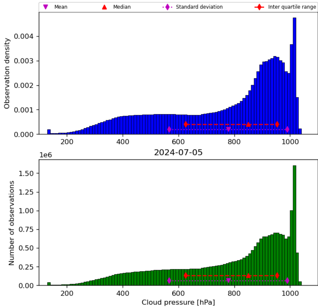
Figure 30: Histogram of “Cloud pressure” for 2024-07-05 to 2024-07-06
