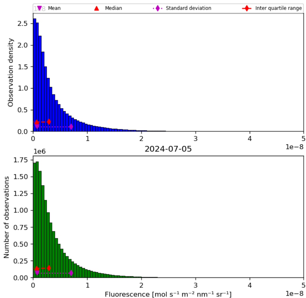
Figure 40: Histogram of “Fluorescence” for 2024-07-05 to 2024-07-06
