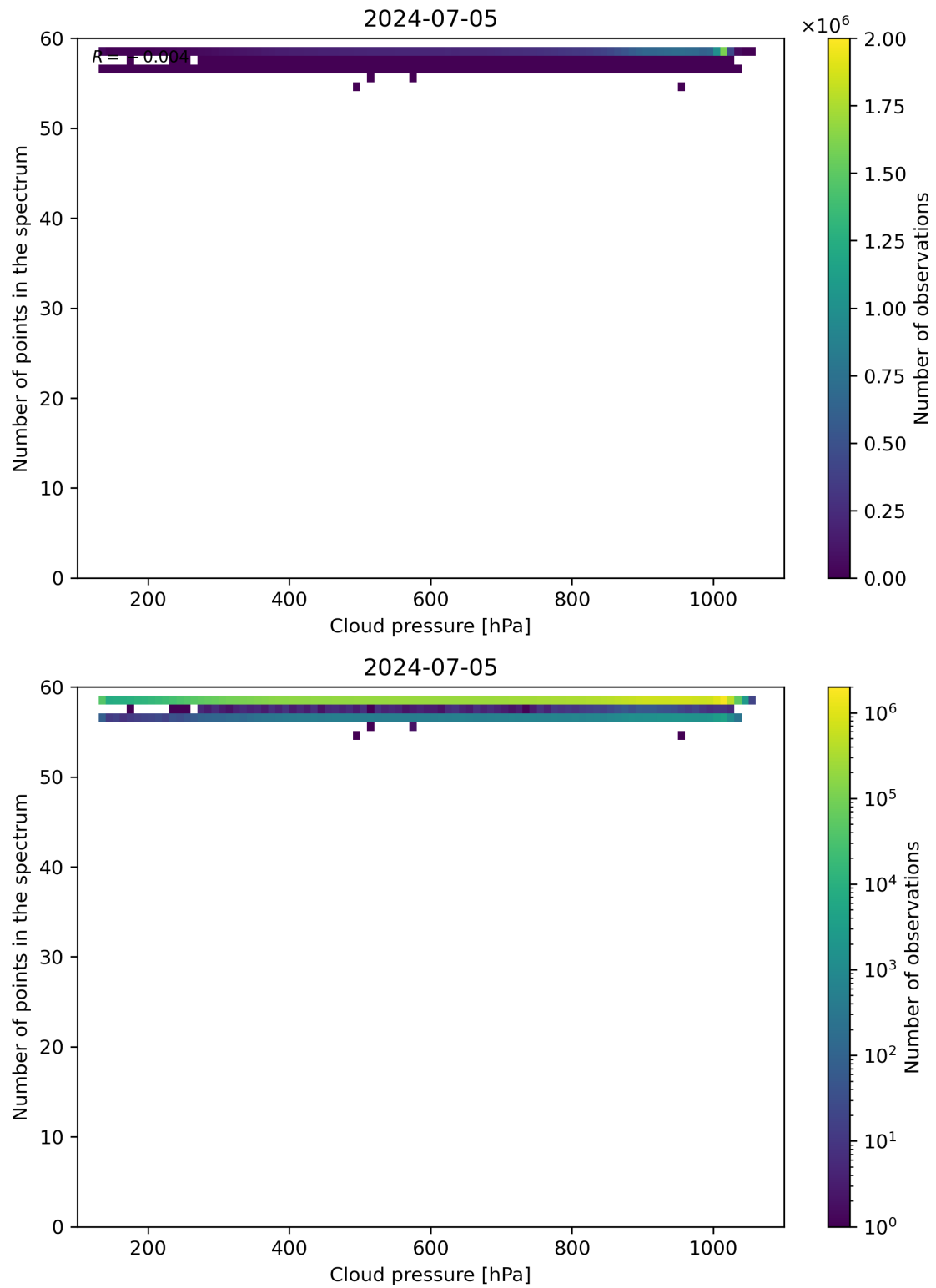
Figure 82: Scatter density plot of “Cloud pressure” against “Number of points in the spectrum” for 2024-07-05 to 2024-07-06.
