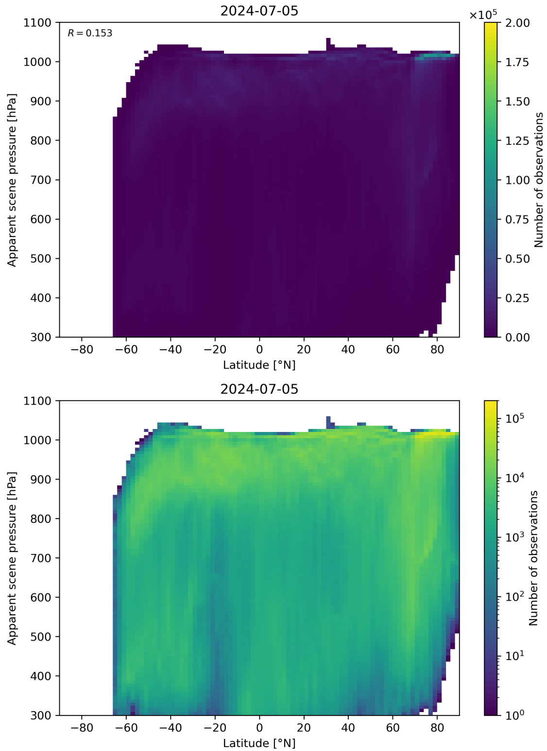
Figure 88: Scatter density plot of “Latitude” against “Apparent scene pressure” for 2024-07-05 to 2024-07-06.
