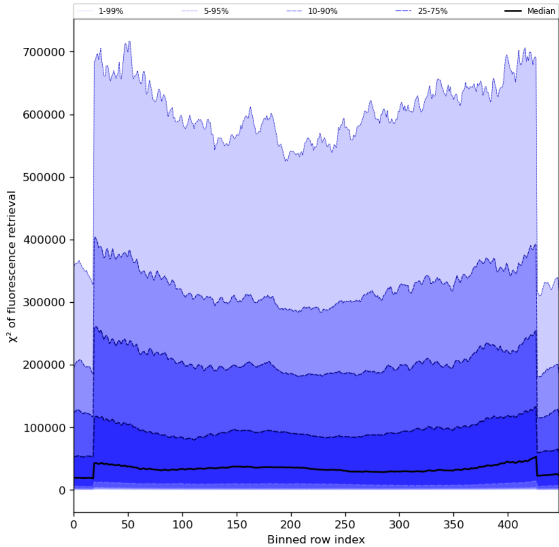
Figure 59: Along track statistics of “ \chi^2 of fluorescence retrieval” for 2024-07-05 to 2024-07-06
