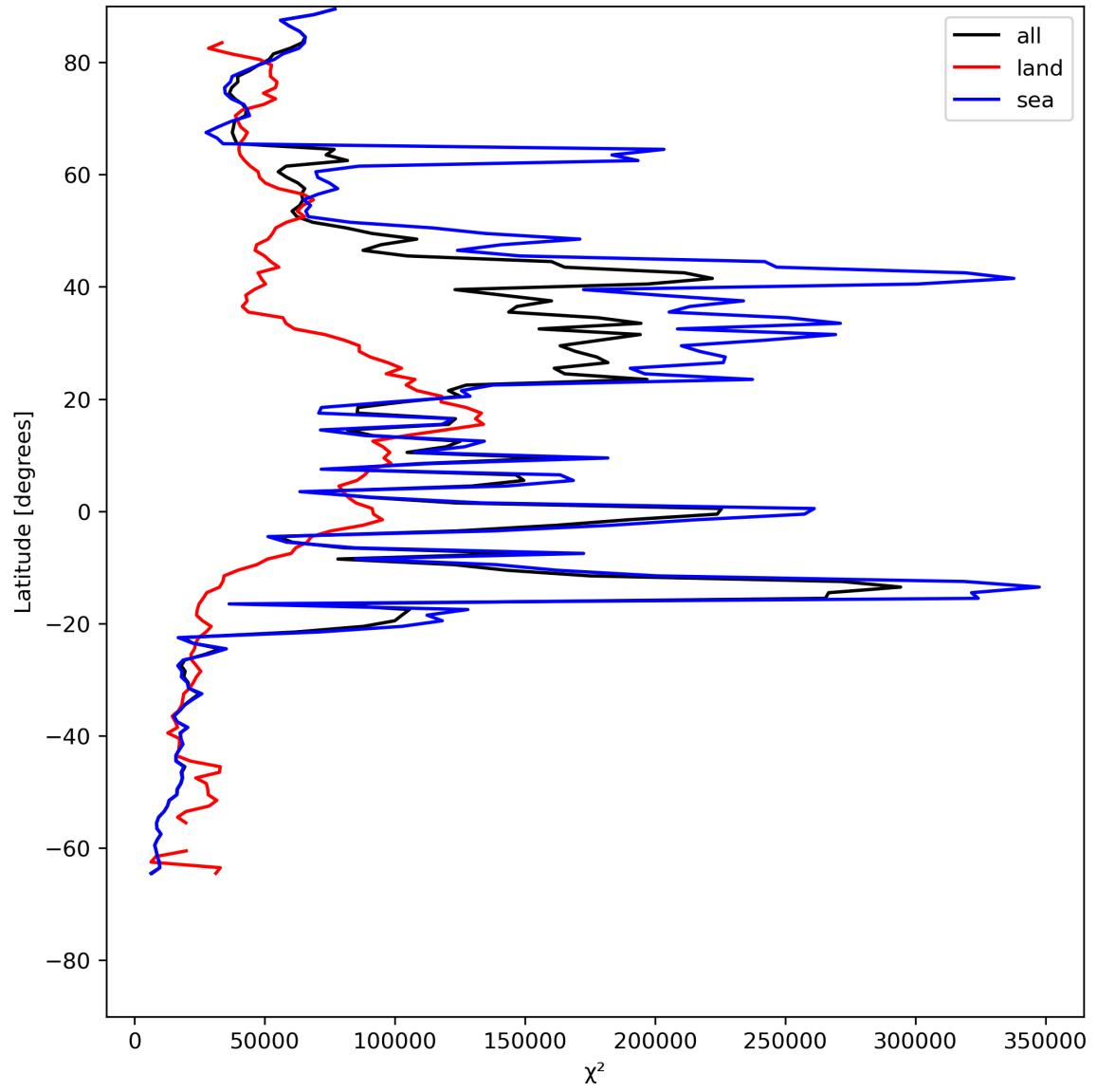
Figure 21: Zonal average of “ \chi^2 ” for 2024-07-05 to 2024-07-06.
