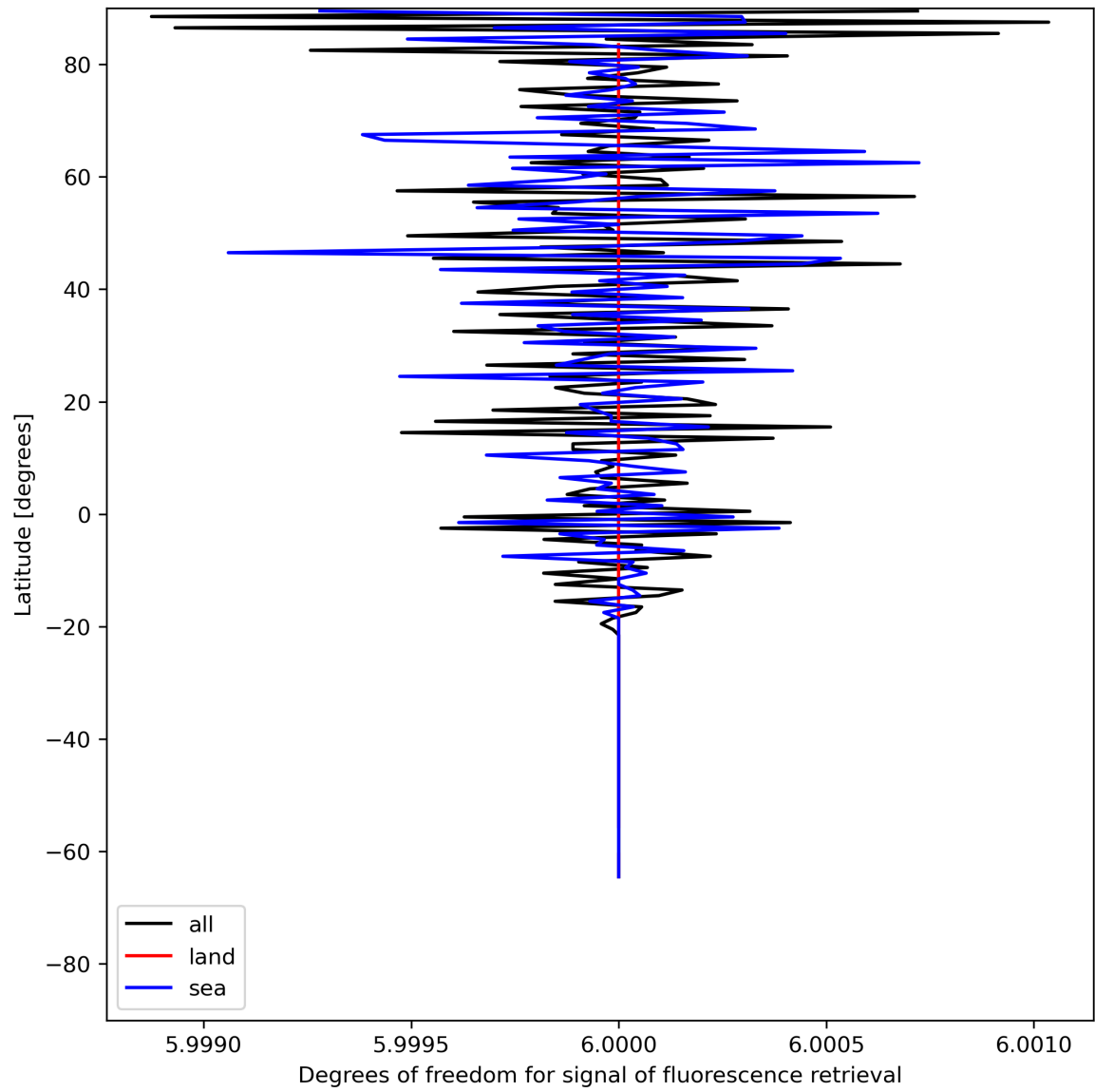
Figure 26: Zonal average of “Degrees of freedom for signal of fluorescence retrieval” for 2024-07-05 to 2024-07-06.
