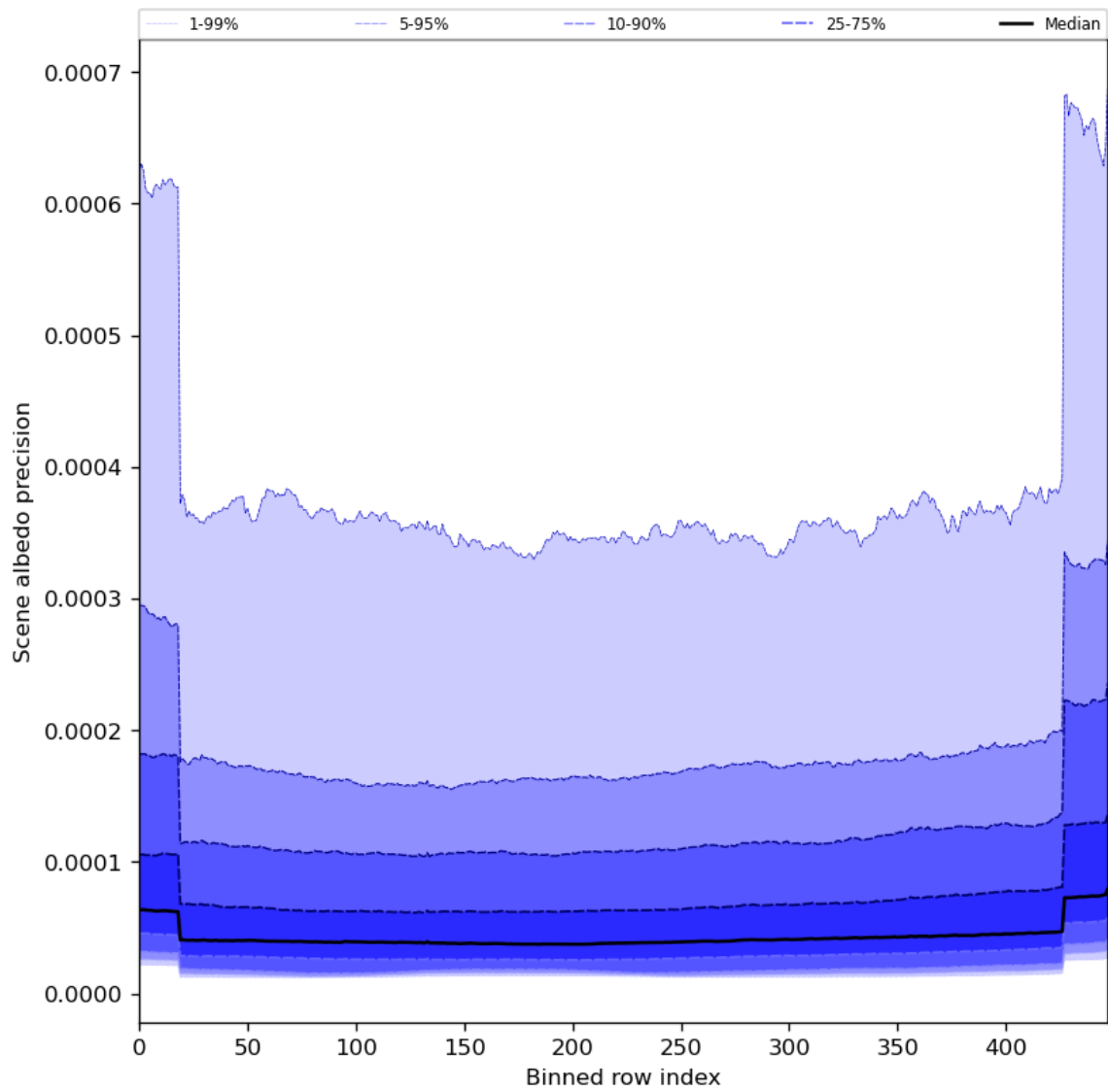
Figure 52: Along track statistics of “Scene albedo precision” for 2024-07-05 to 2024-07-06
