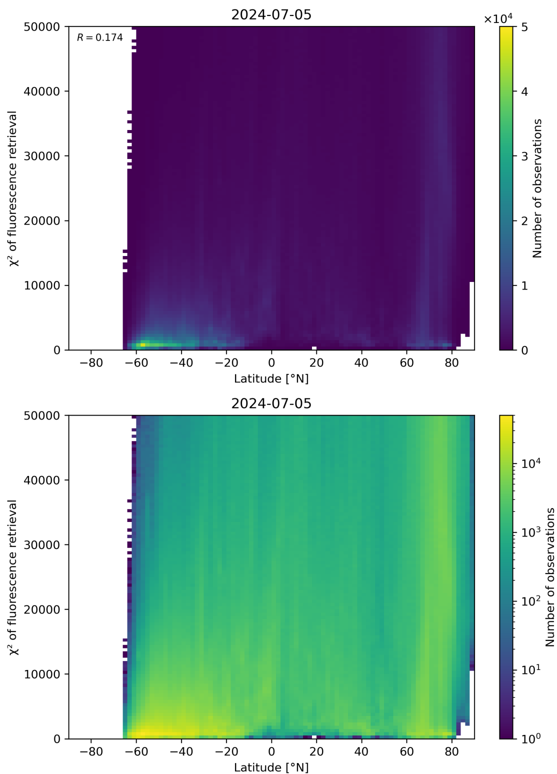
Figure 89: Scatter density plot of “Latitude” against “ \chi^2 of fluorescence retrieval” for 2024-07-05 to 2024-07-06.
