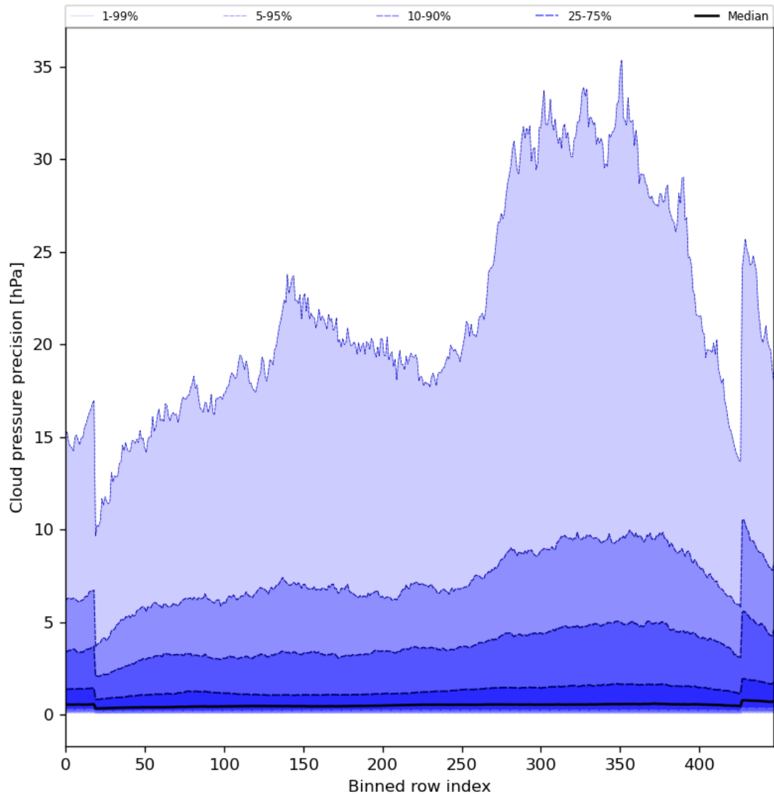
Figure 48: Along track statistics of “Cloud pressure precision” for 2024-07-05 to 2024-07-06
