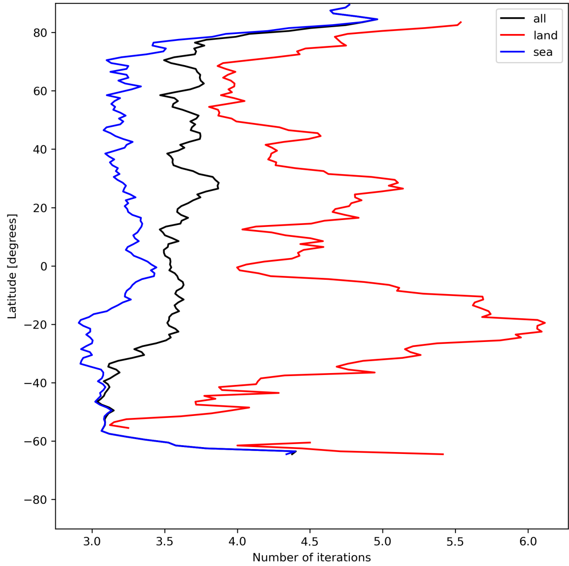
Figure 22: Zonal average of “Number of iterations” for 2024-07-05 to 2024-07-06.
