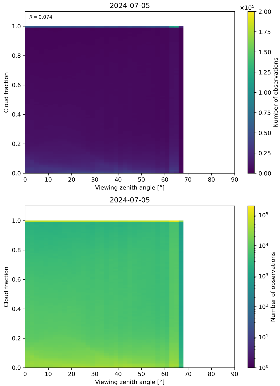
Figure 120: Scatter density plot of “Viewing zenith angle” against “Cloud fraction” for 2024-07-05 to 2024-07-06.
