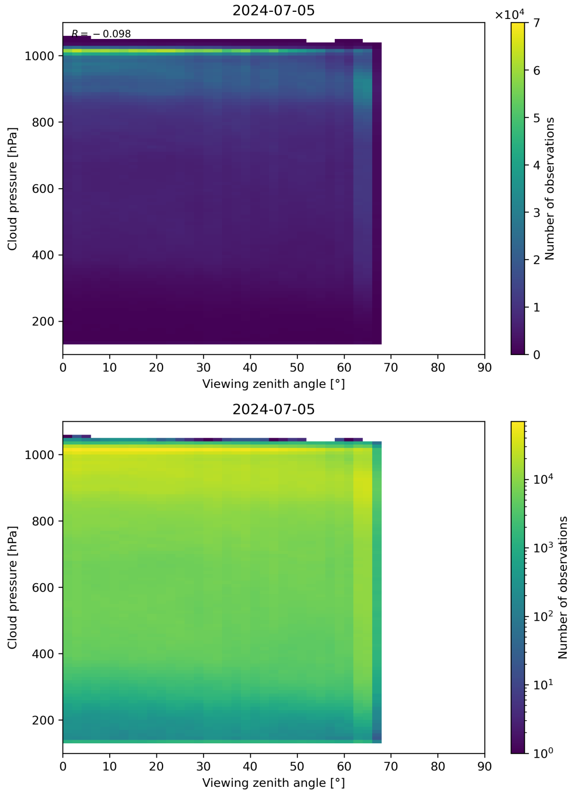
Figure 121: Scatter density plot of “Viewing zenith angle” against “Cloud pressure” for 2024-07-05 to 2024-07-06.
