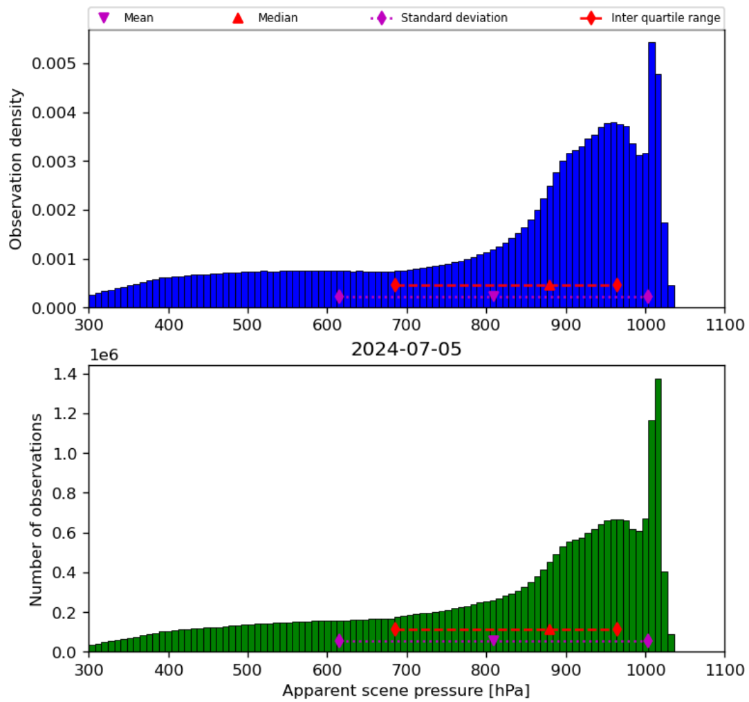
Figure 36: Histogram of “Apparent scene pressure” for 2024-07-05 to 2024-07-06
