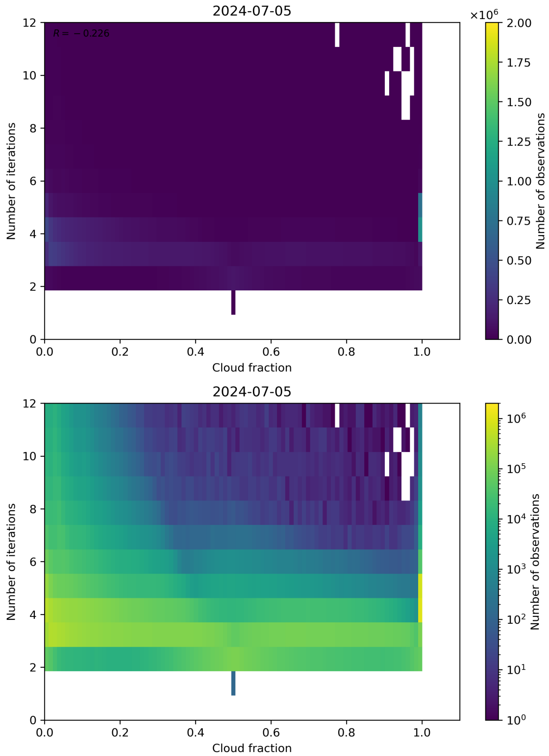
Figure 73: Scatter density plot of “Cloud fraction” against “Number of iterations” for 2024-07-05 to 2024-07-06.
