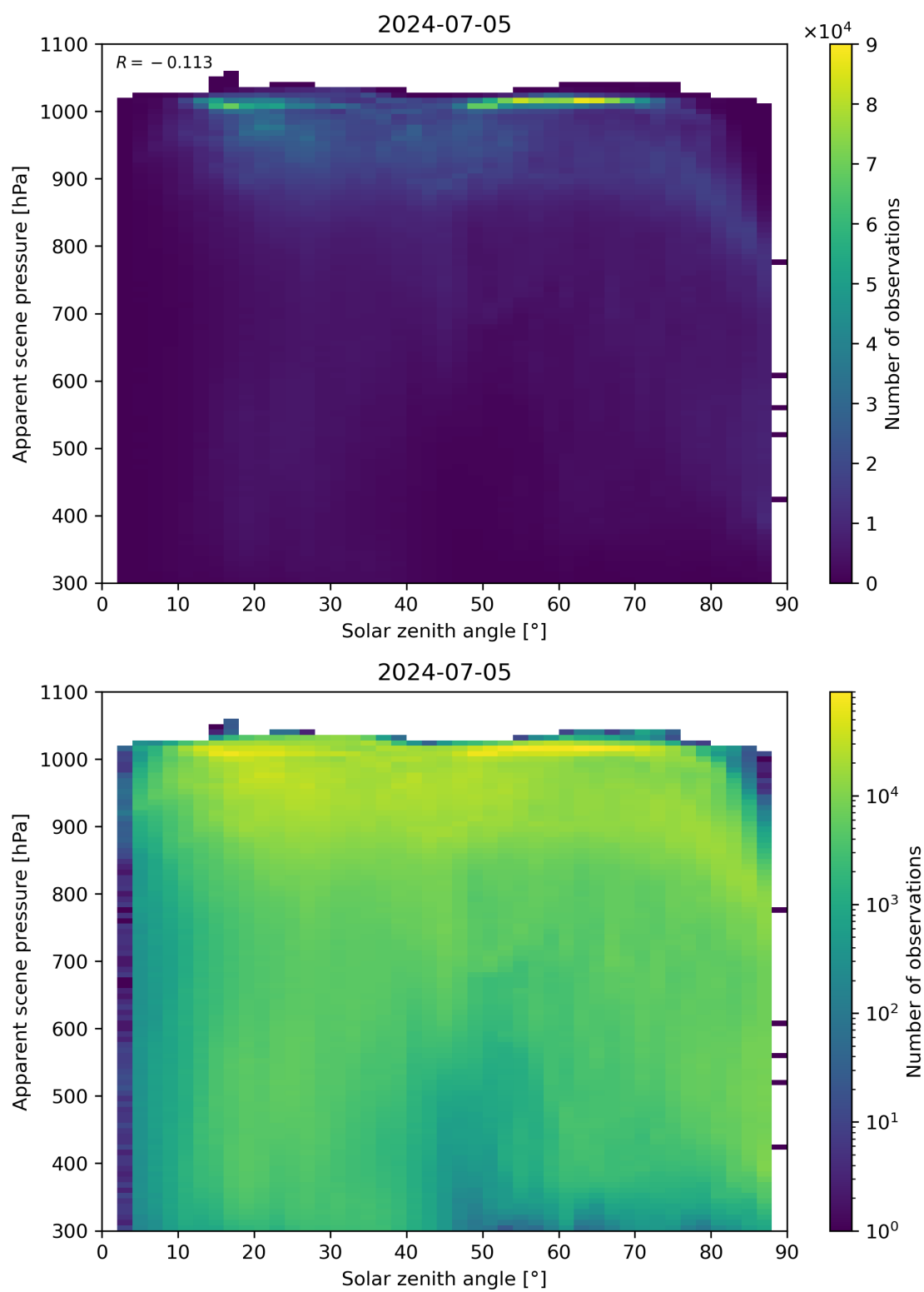
Figure 108: Scatter density plot of “Solar zenith angle” against “Apparent scene pressure” for 2024-07-05 to 2024-07-06.
