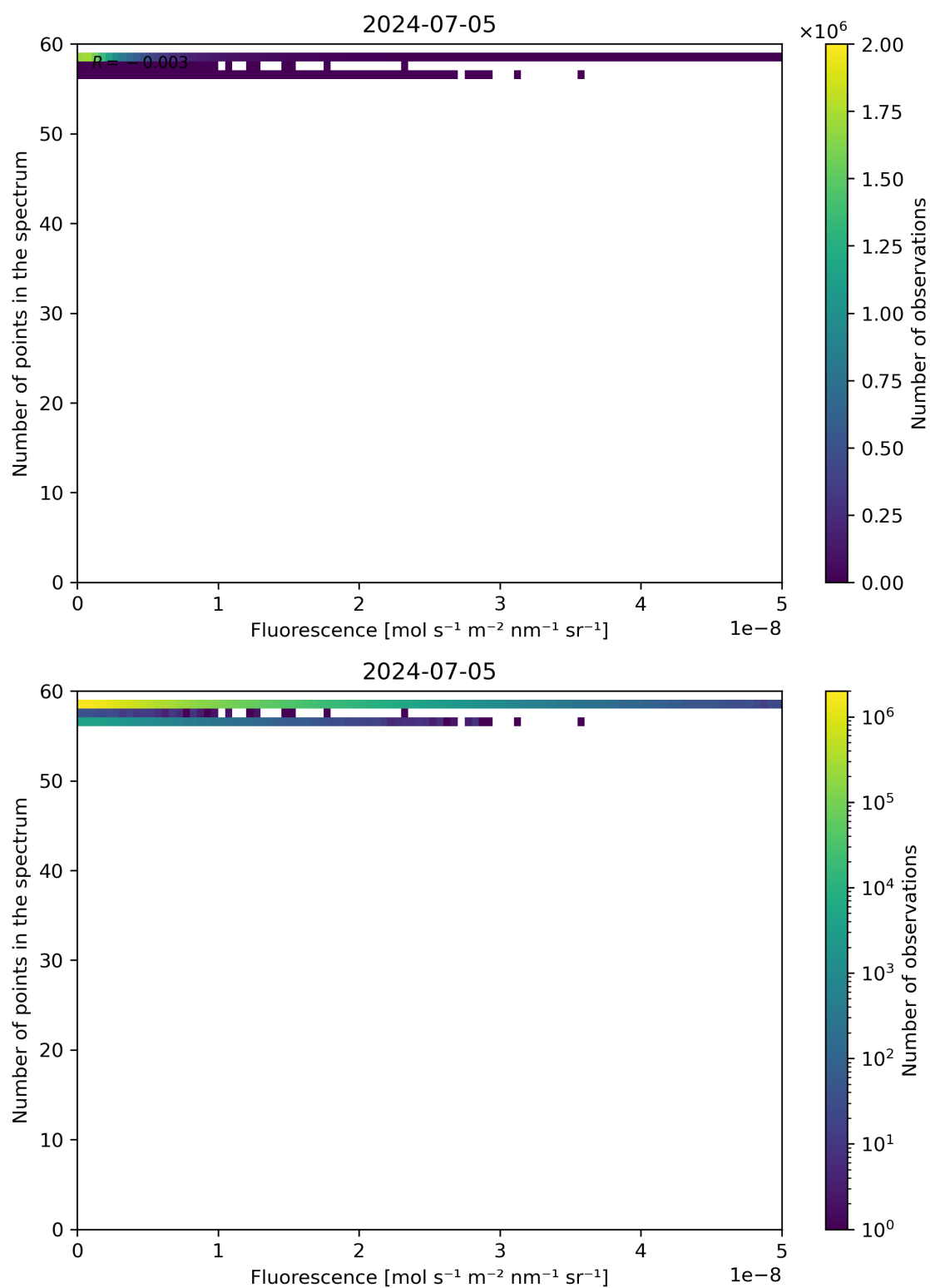
Figure 86: Scatter density plot of “Fluorescence” against “Number of points in the spectrum” for 2024-07-05 to 2024-07-06.
