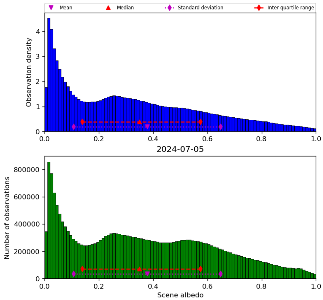
Figure 34: Histogram of “Scene albedo” for 2024-07-05 to 2024-07-06
