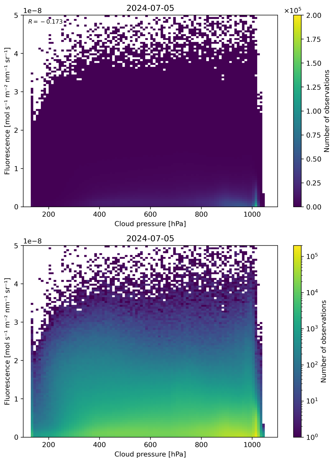
Figure 80: Scatter density plot of “Cloud pressure” against “Fluorescence” for 2024-07-05 to 2024-07-06.
