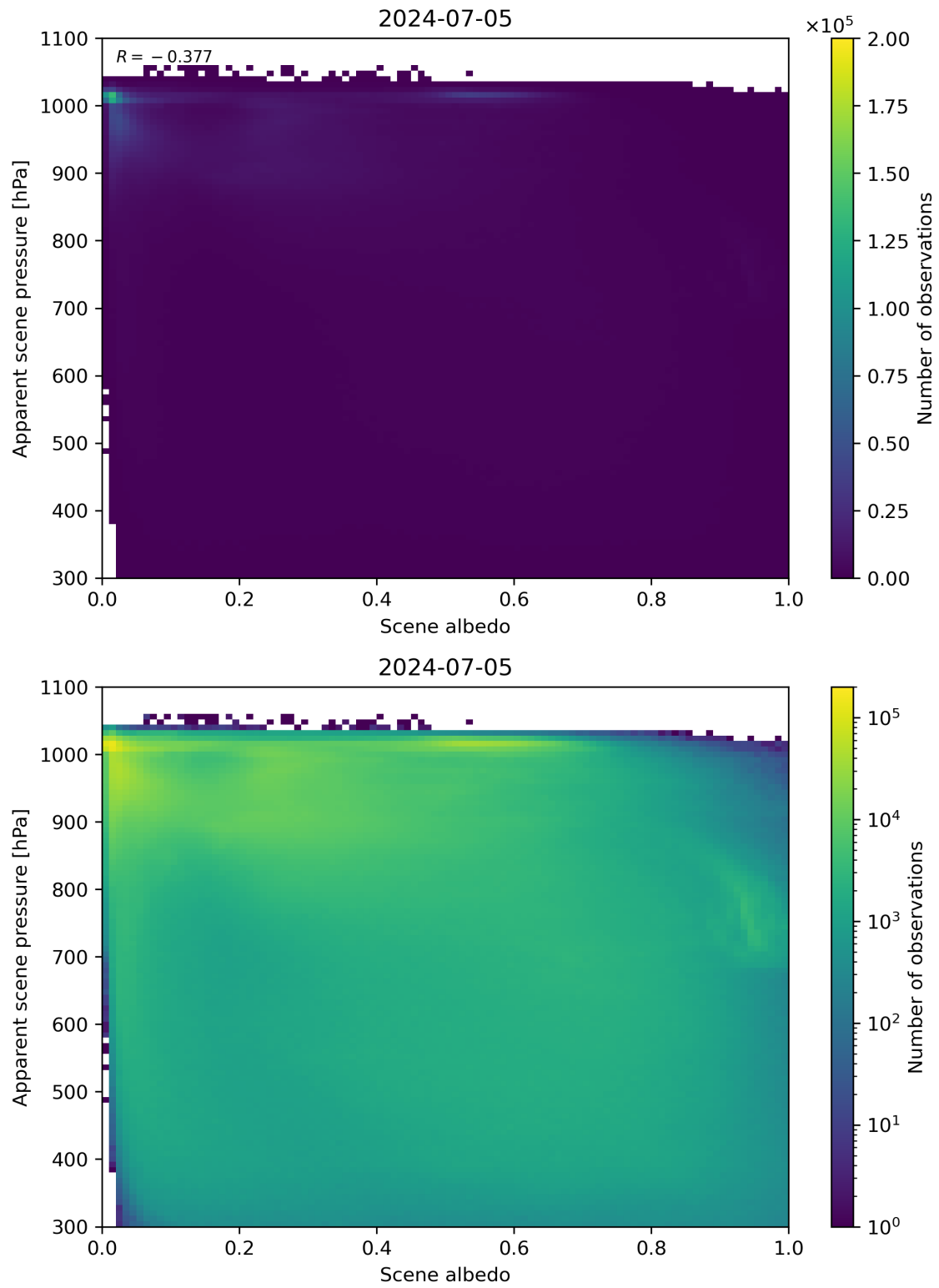
Figure 102: Scatter density plot of “Scene albedo” against “Apparent scene pressure” for 2024-07-05 to 2024-07-06.
