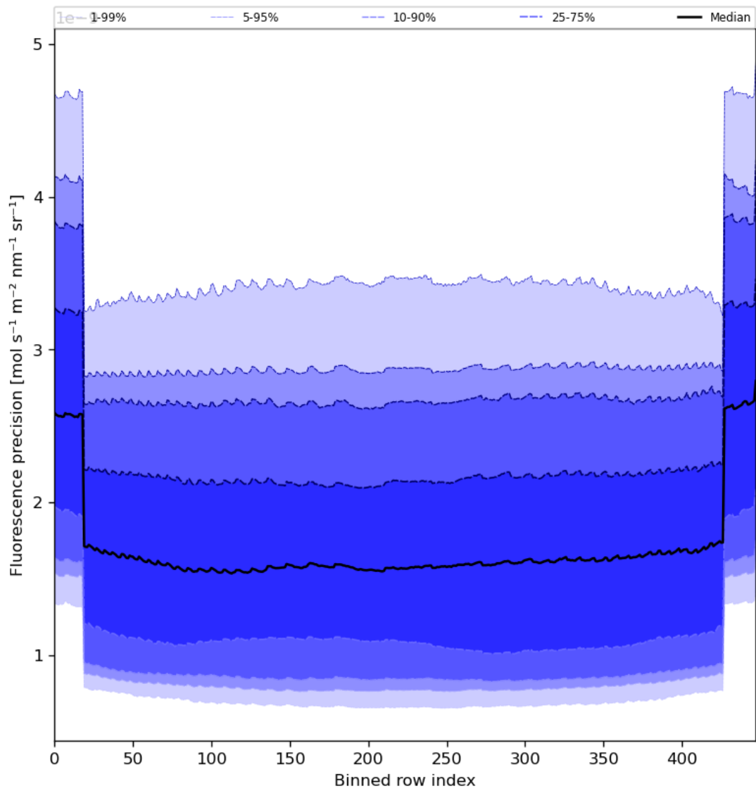
Figure 58: Along track statistics of “Fluorescence precision” for 2024-07-05 to 2024-07-06
