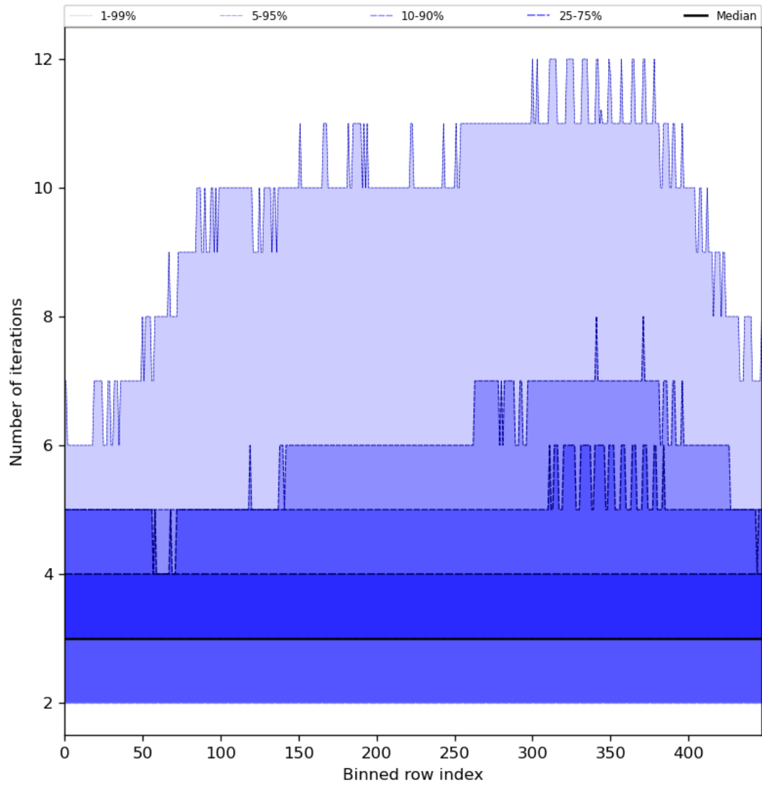
Figure 56: Along track statistics of “Number of iterations” for 2024-07-05 to 2024-07-06
