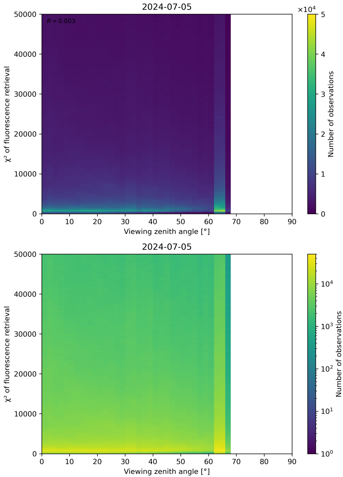
Figure 119: Scatter density plot of “Viewing zenith angle” against “ \chi^2 of fluorescence retrieval” for 2024-07-05 to 2024-07-06.
