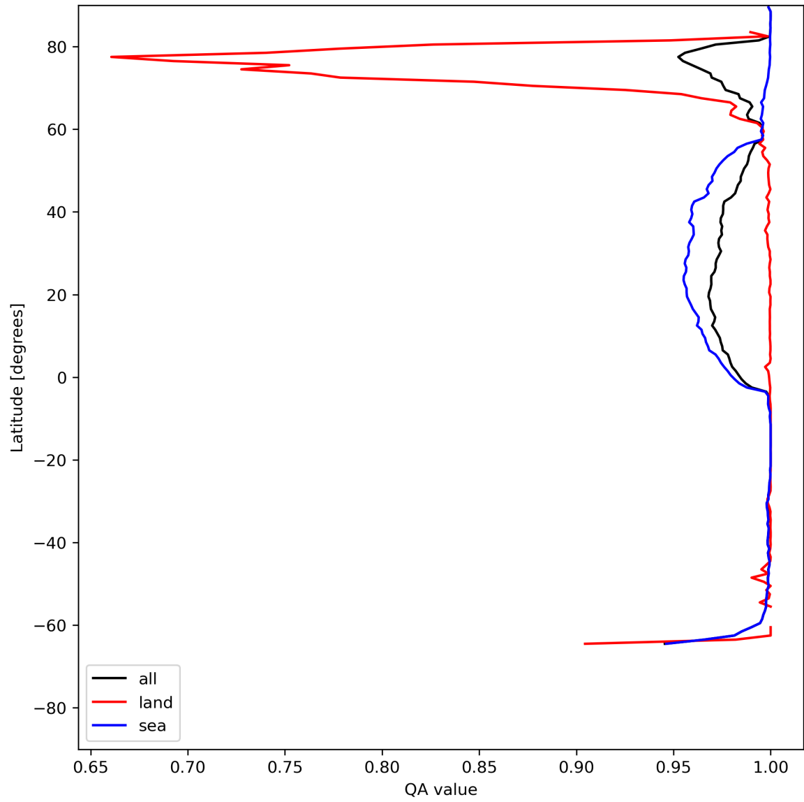
Figure 12: Zonal average of “QA value” for 2024-07-05 to 2024-07-06.
