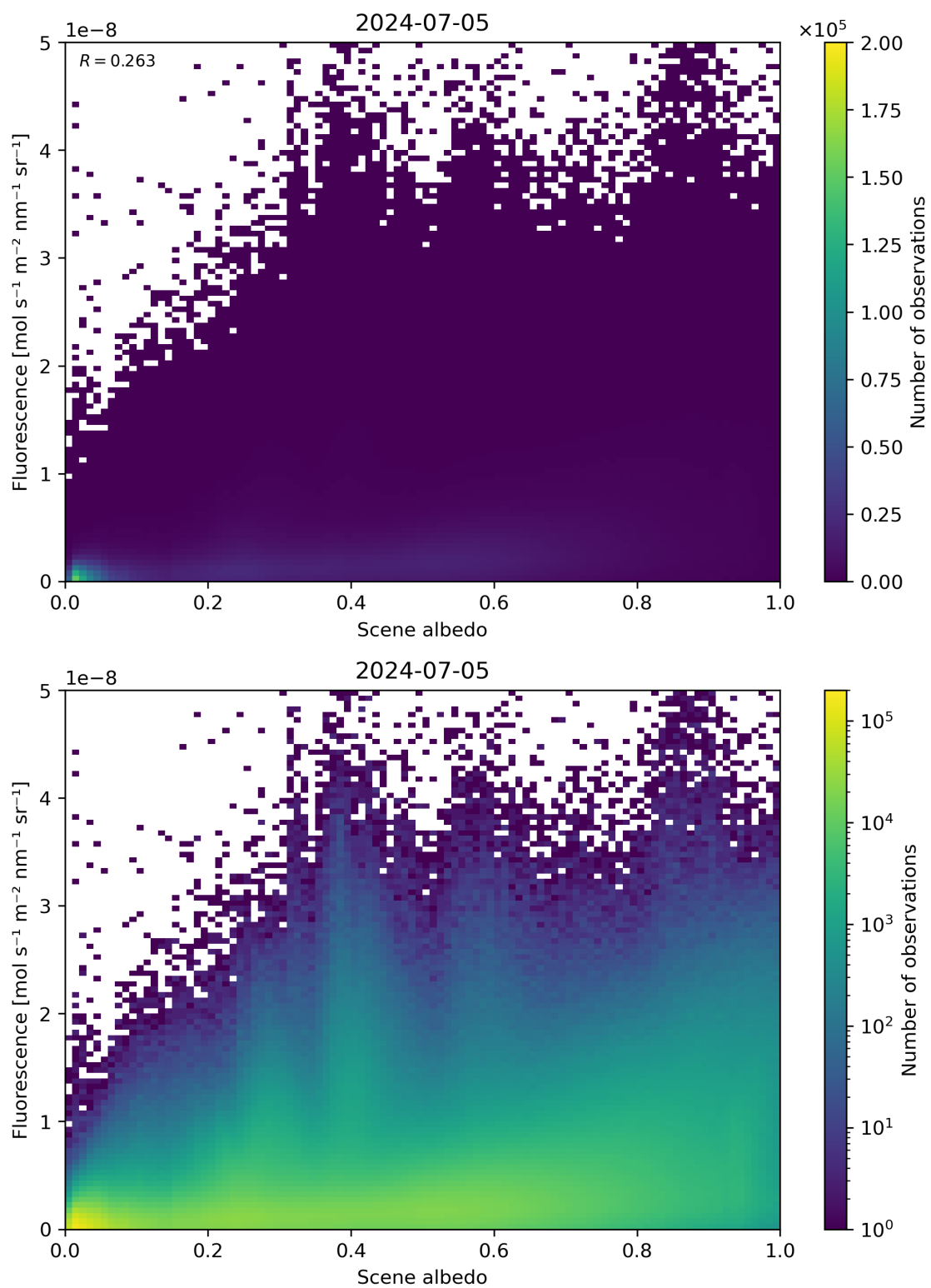
Figure 104: Scatter density plot of “Scene albedo” against “Fluorescence” for 2024-07-05 to 2024-07-06.
