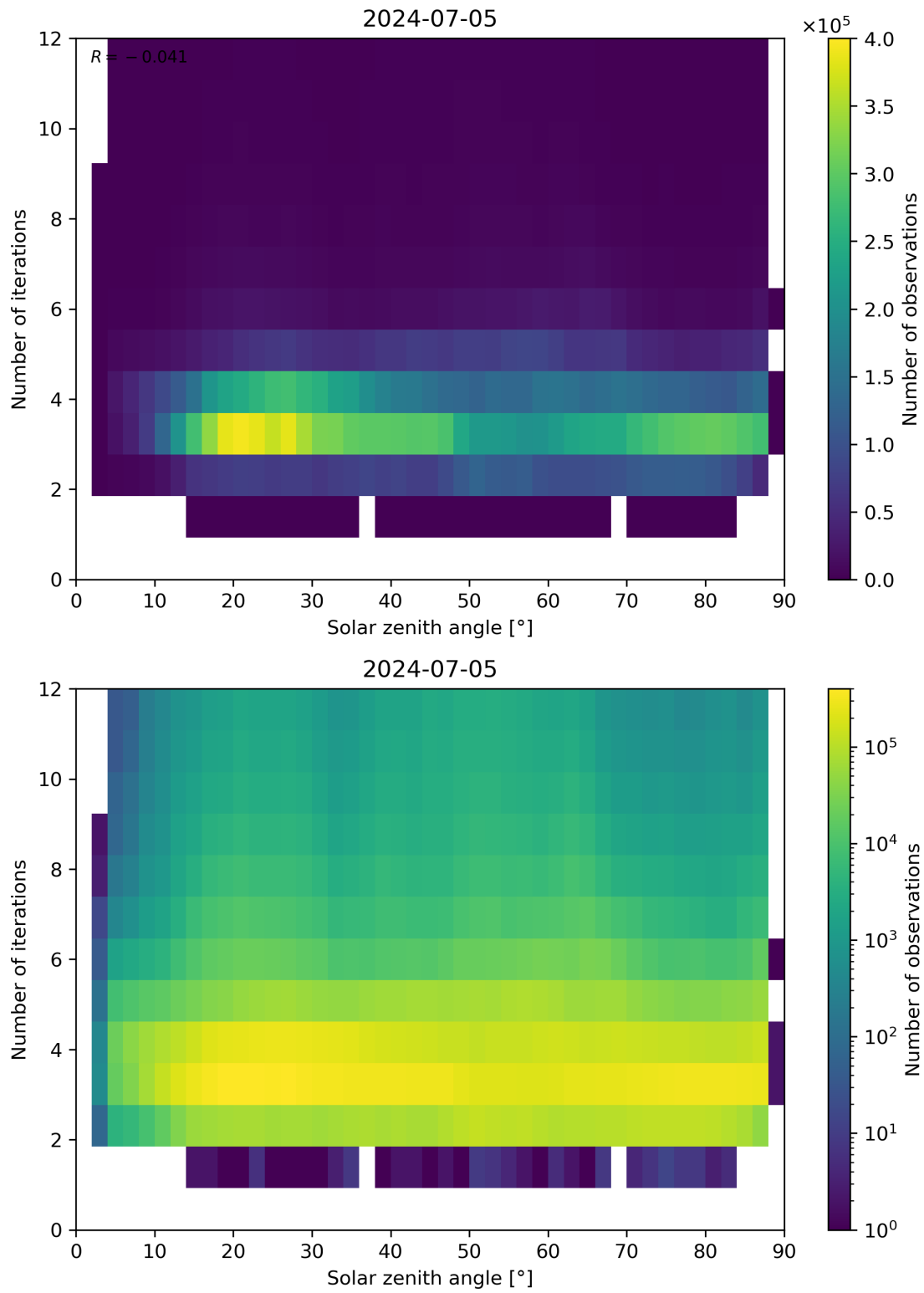
Figure 114: Scatter density plot of “Solar zenith angle” against “Number of iterations” for 2024-07-05 to 2024-07-06.
