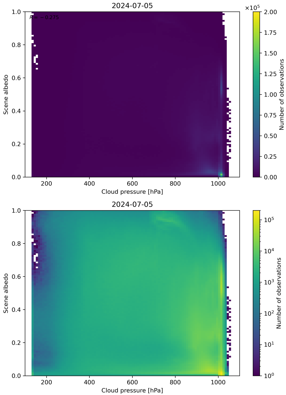
Figure 83: Scatter density plot of “Cloud pressure” against “Scene albedo” for 2024-07-05 to 2024-07-06.
