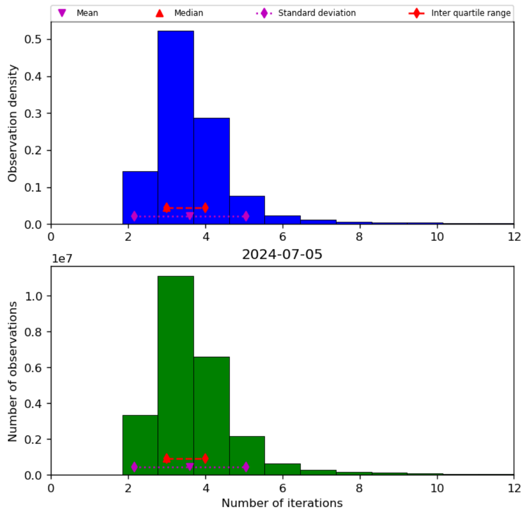
Figure 39: Histogram of “Number of iterations” for 2024-07-05 to 2024-07-06
