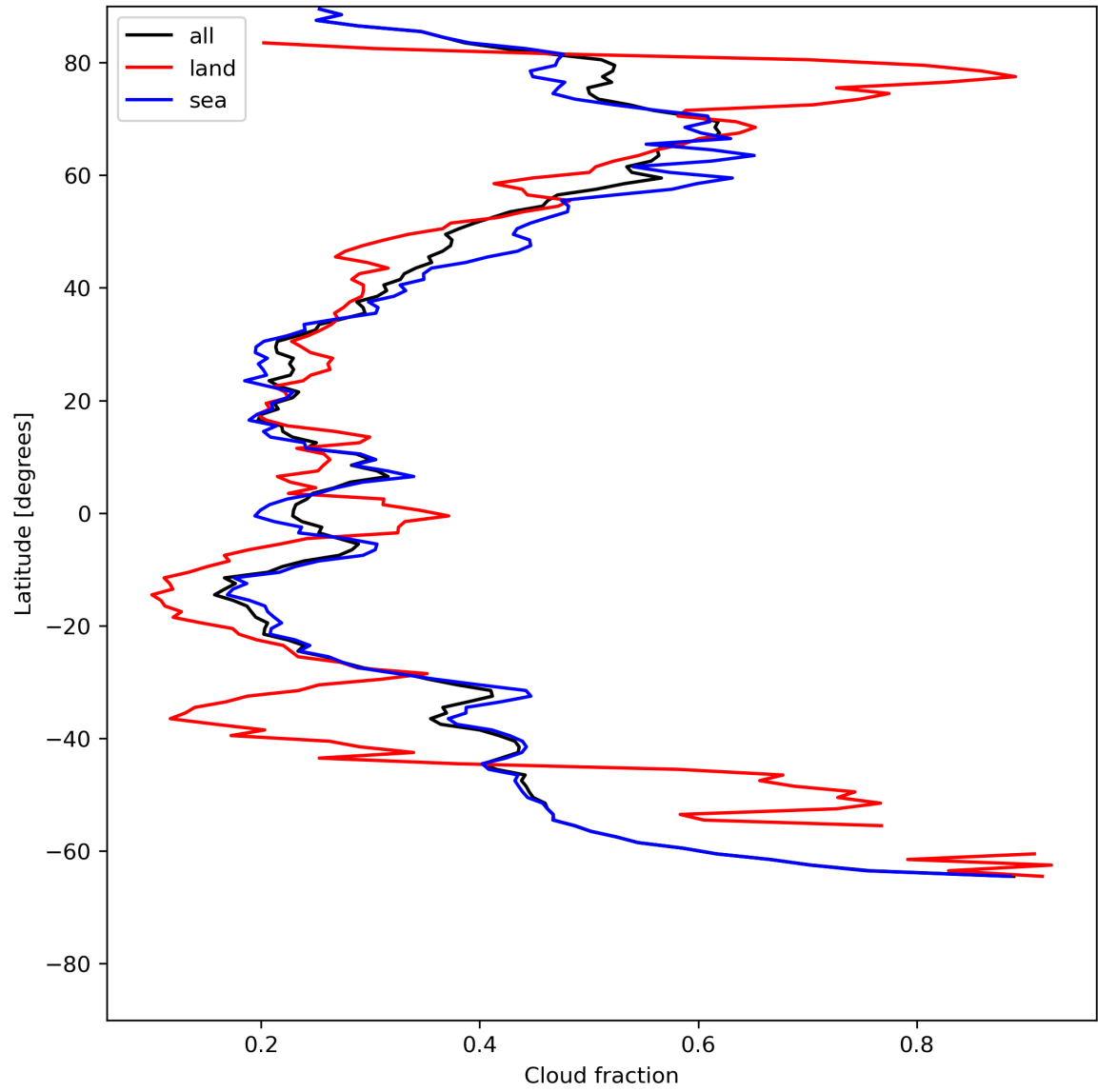
Figure 15: Zonal average of “Cloud fraction” for 2024-07-05 to 2024-07-06.
