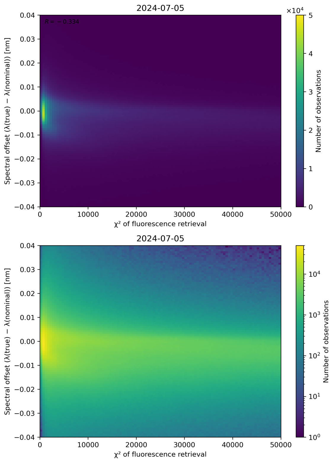
Figure 69: Scatter density plot of “ \chi^2 of fluorescence retrieval” against “Spectral offset ( \lambda(\text{true}) - \lambda(\text{nominal}) )” for 2024-07-05 to 2024-07-06.
