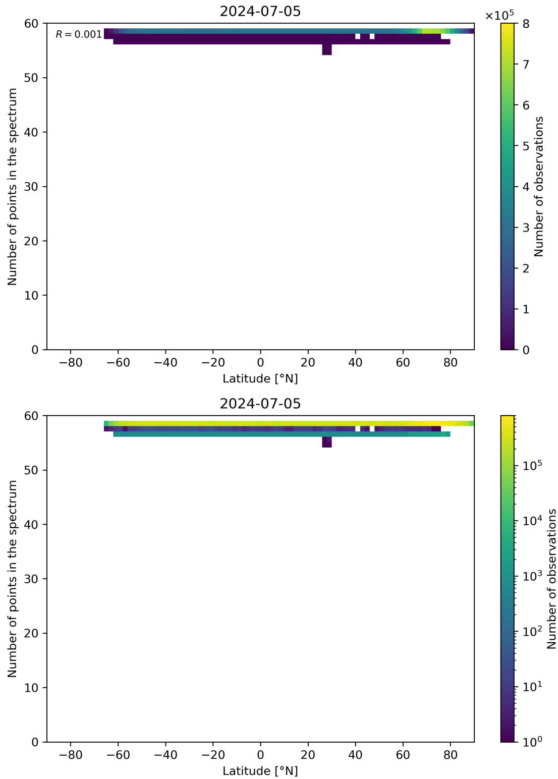
Figure 94: Scatter density plot of “Latitude” against “Number of points in the spectrum” for 2024-07-05 to 2024-07-06.
