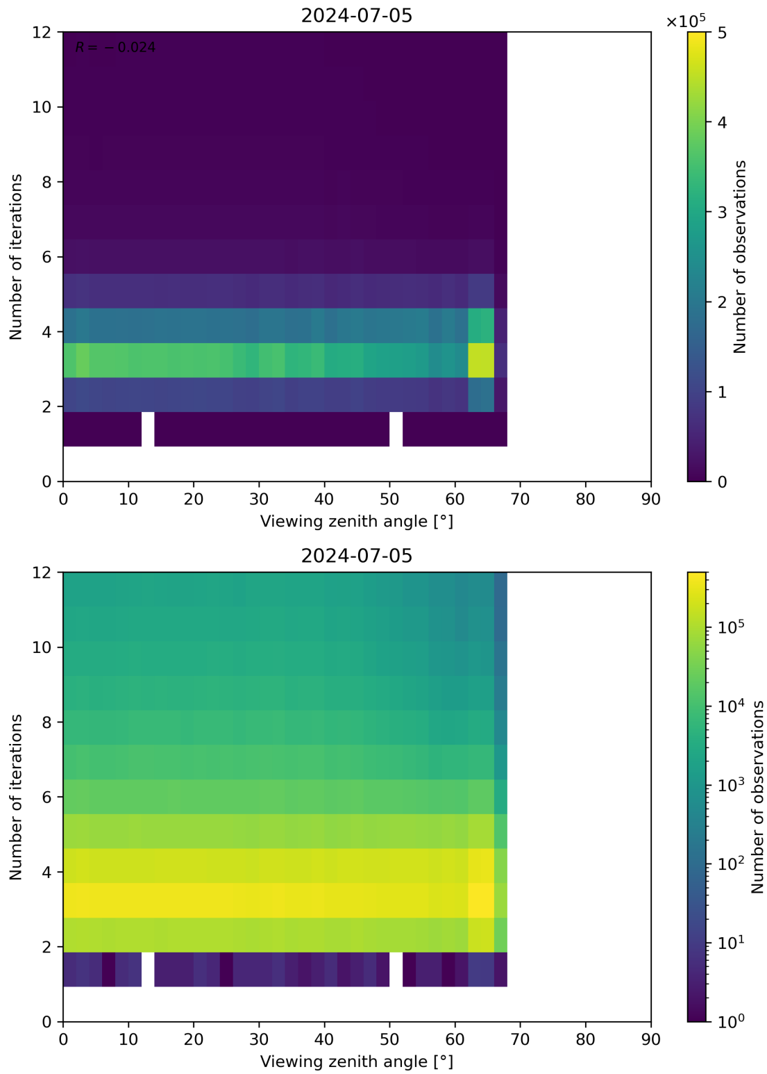
Figure 124: Scatter density plot of “Viewing zenith angle” against “Number of iterations” for 2024-07-05 to 2024-07-06.
