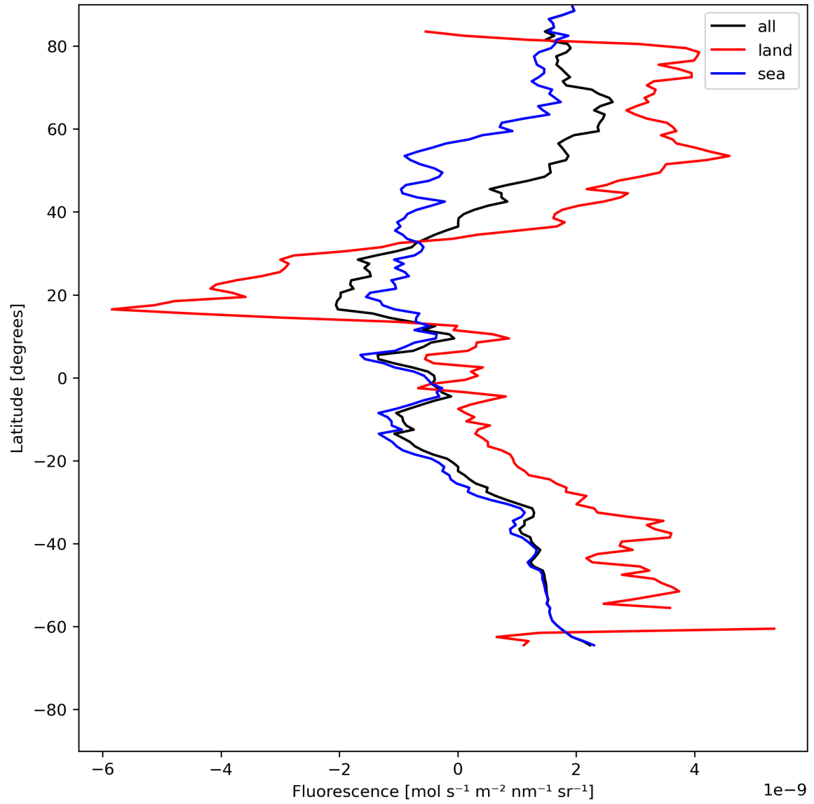
Figure 23: Zonal average of “Fluorescence” for 2024-07-05 to 2024-07-06.
