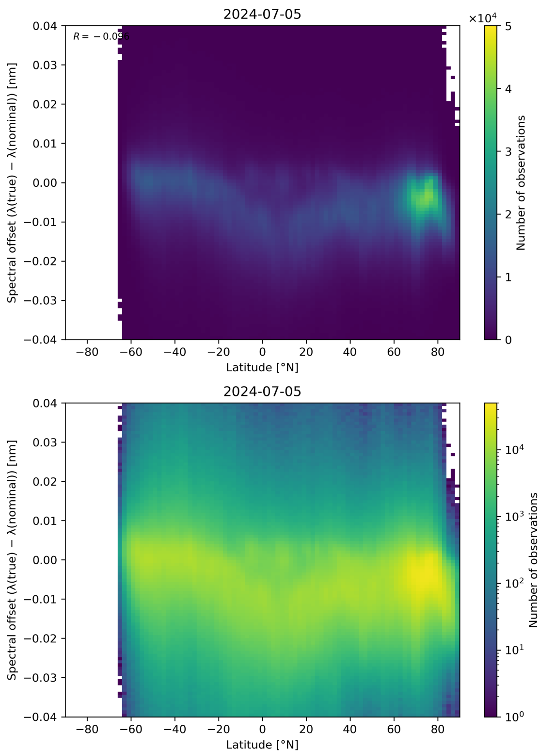
Figure 96: Scatter density plot of “Latitude” against “Spectral offset ( \lambda(\text{true}) - \lambda(\text{nominal}) )” for 2024-07-05 to 2024-07-06.
