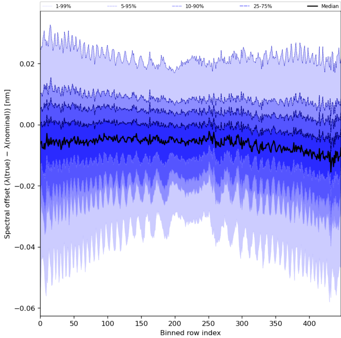
Figure 62: Along track statistics of “Spectral offset ( \lambda(\text{true}) - \lambda(\text{nominal}) )” for 2024-07-05 to 2024-07-06
