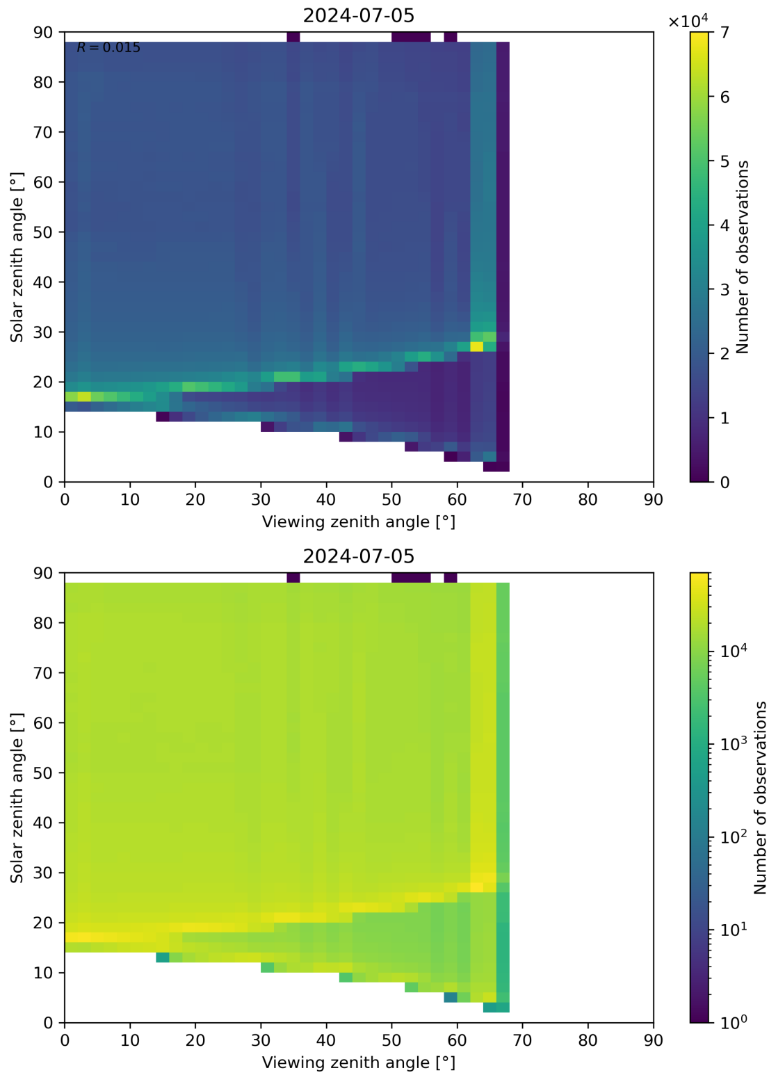
Figure 127: Scatter density plot of “Viewing zenith angle” against “Solar zenith angle” for 2024-07-05 to 2024-07-06.
