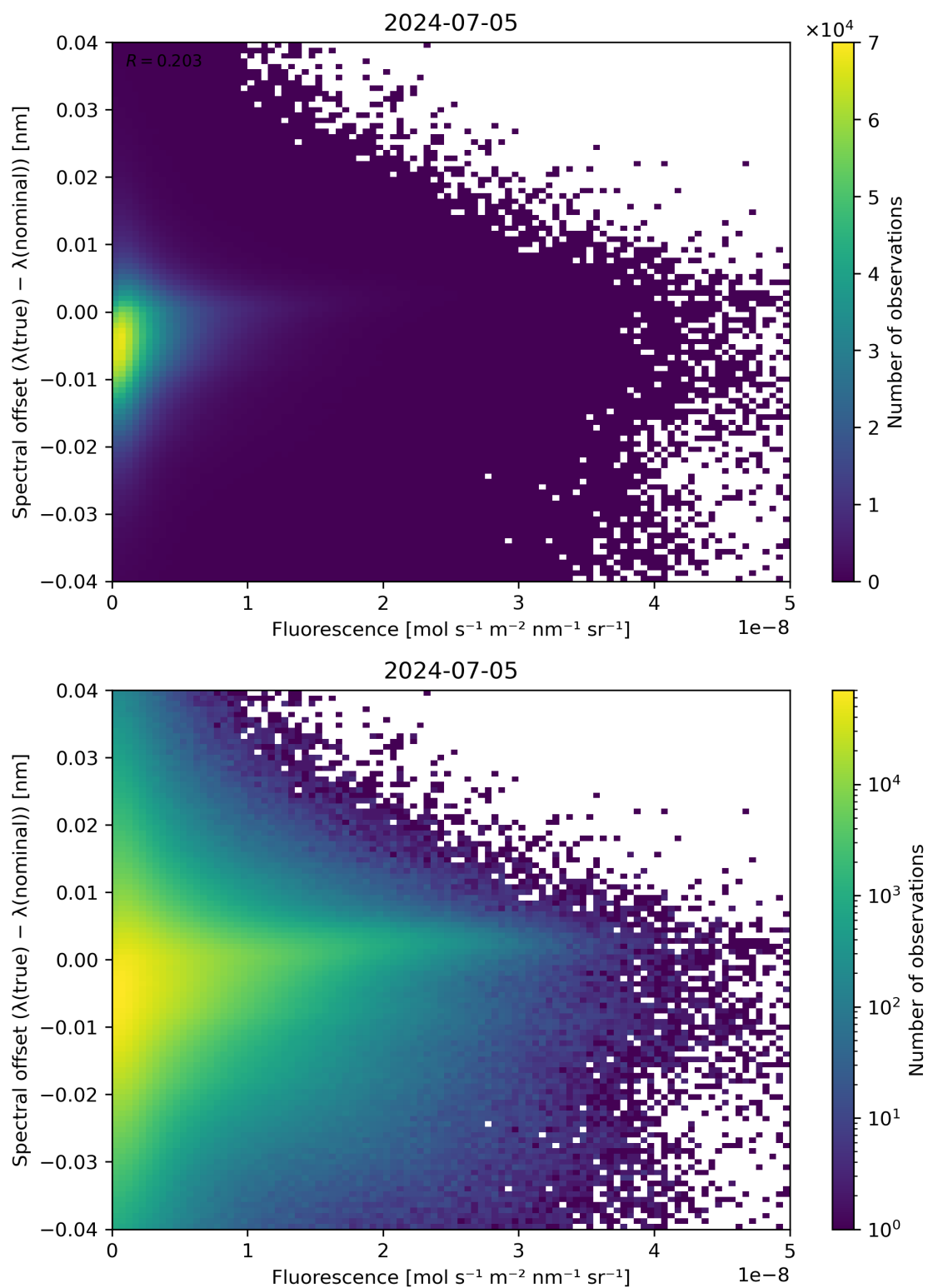
Figure 87: Scatter density plot of “Fluorescence” against “Spectral offset ( \lambda(\text{true}) - \lambda(\text{nominal}) )” for 2024-07-05 to 2024-07-06.
