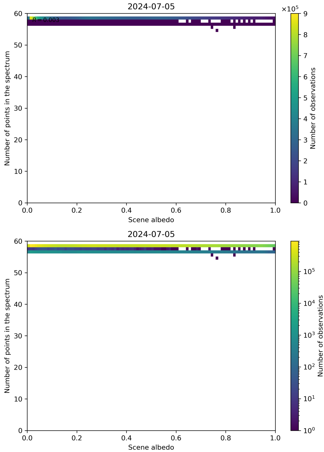
Figure 106: Scatter density plot of “Scene albedo” against “Number of points in the spectrum” for 2024-07-05 to 2024-07-06.
