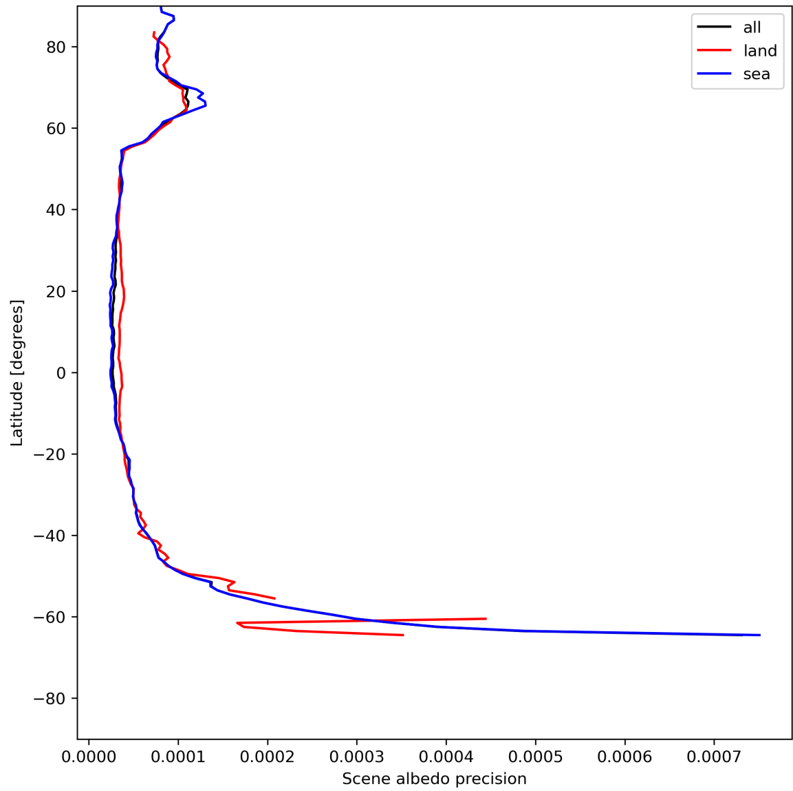
Figure 18: Zonal average of “Scene albedo precision” for 2024-07-05 to 2024-07-06.
