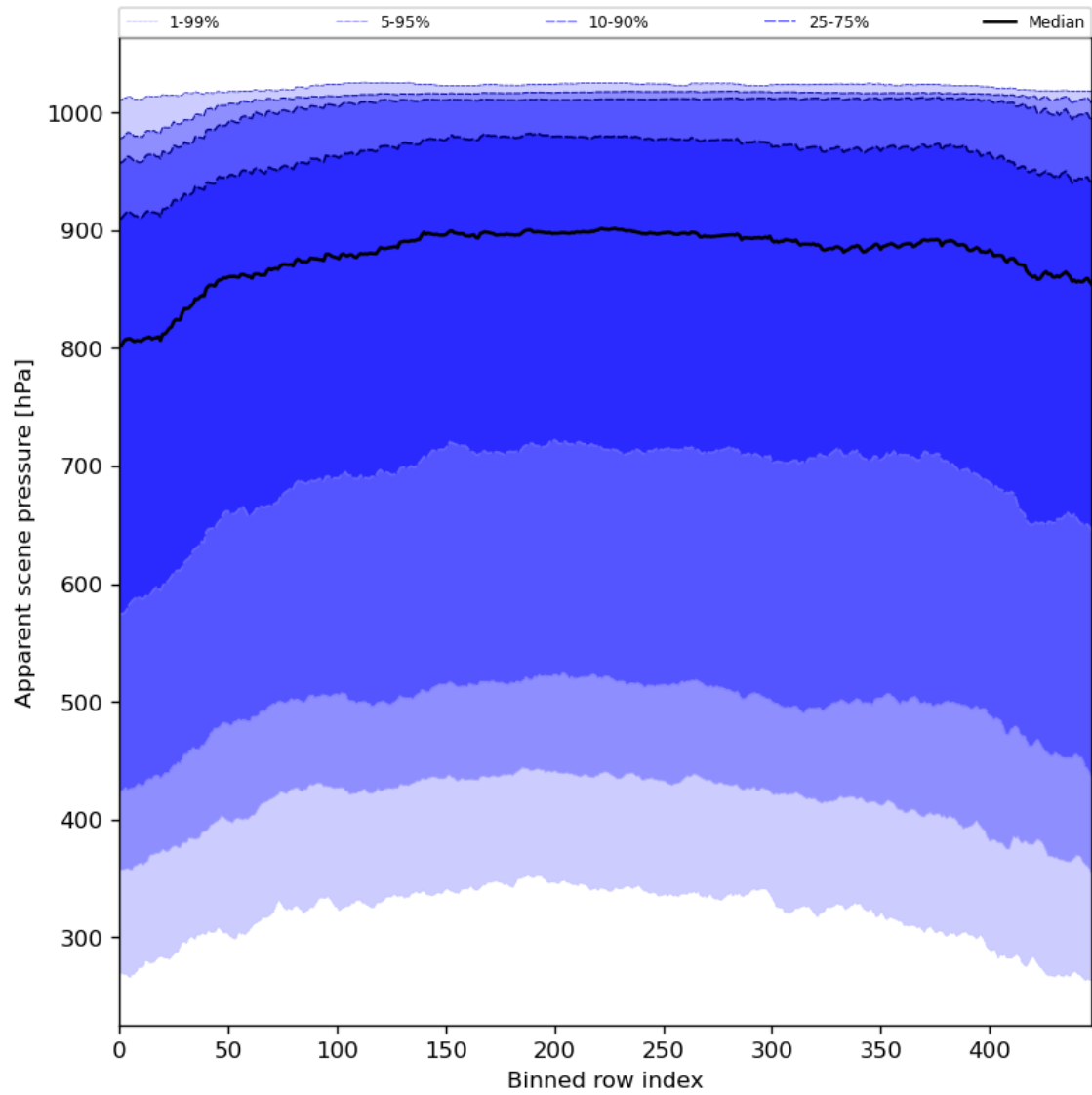
Figure 53: Along track statistics of “Apparent scene pressure” for 2024-07-05 to 2024-07-06
