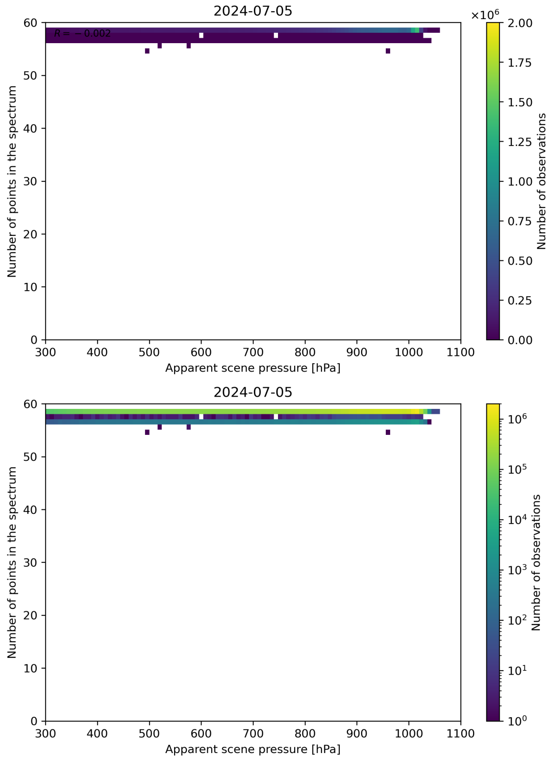
Figure 66: Scatter density plot of “Apparent scene pressure” against “Number of points in the spectrum” for 2024-07-05 to 2024-07-06.
