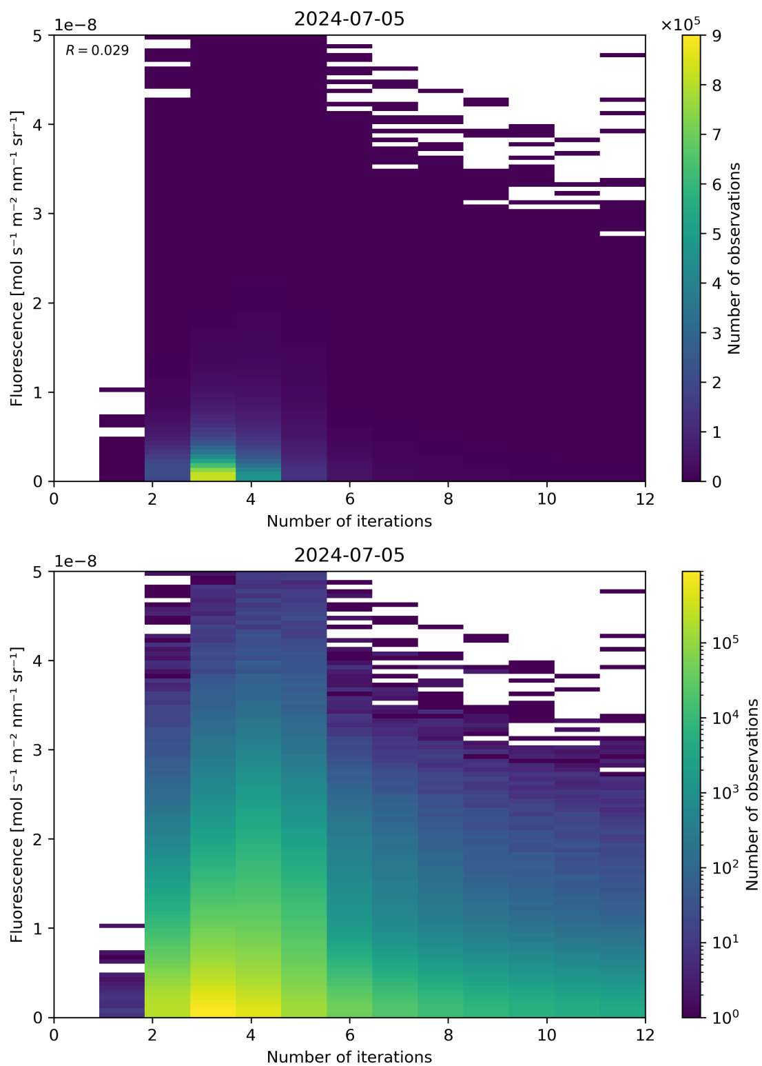
Figure 98: Scatter density plot of “Number of iterations” against “Fluorescence” for 2024-07-05 to 2024-07-06.
