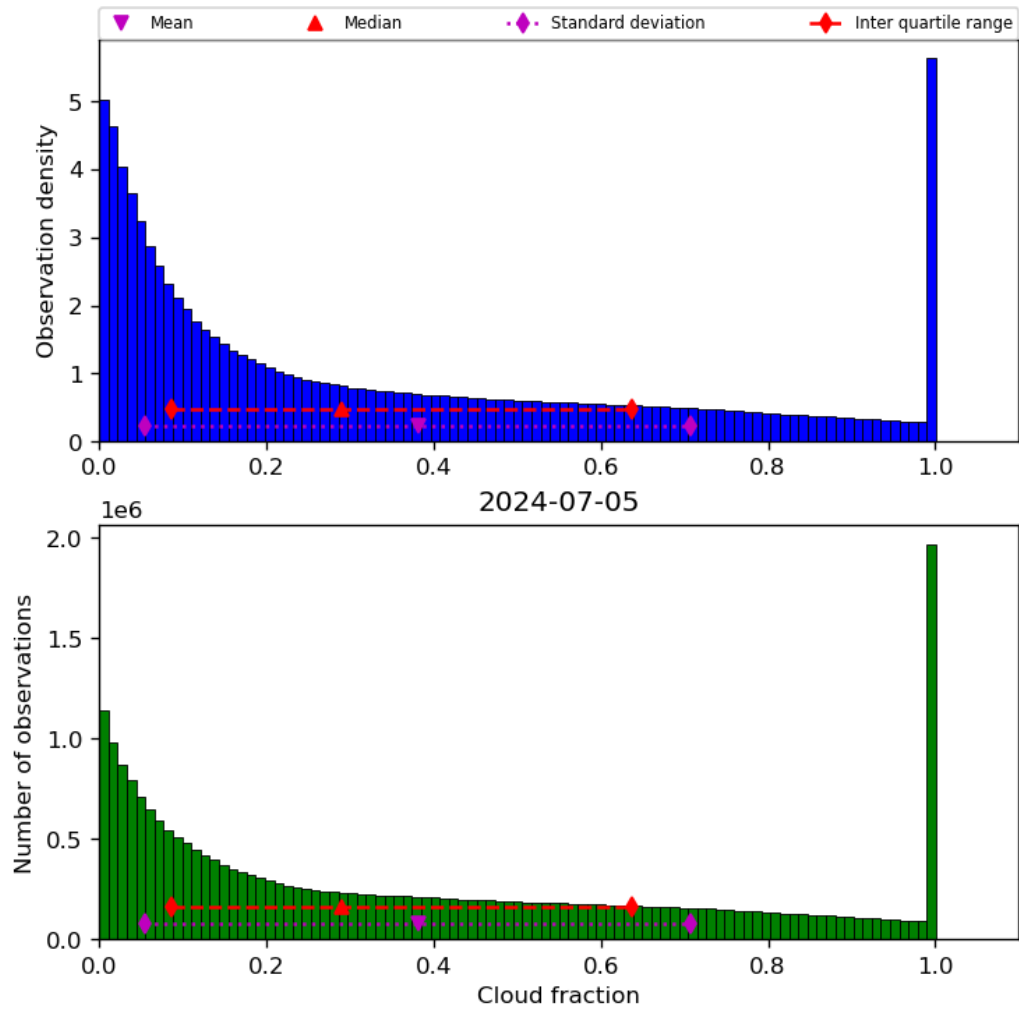
Figure 32: Histogram of “Cloud fraction” for 2024-07-05 to 2024-07-06
