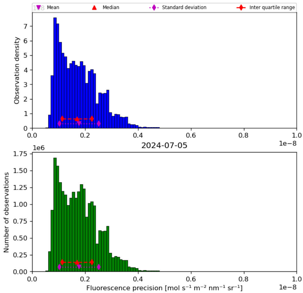
Figure 41: Histogram of “Fluorescence precision” for 2024-07-05 to 2024-07-06
