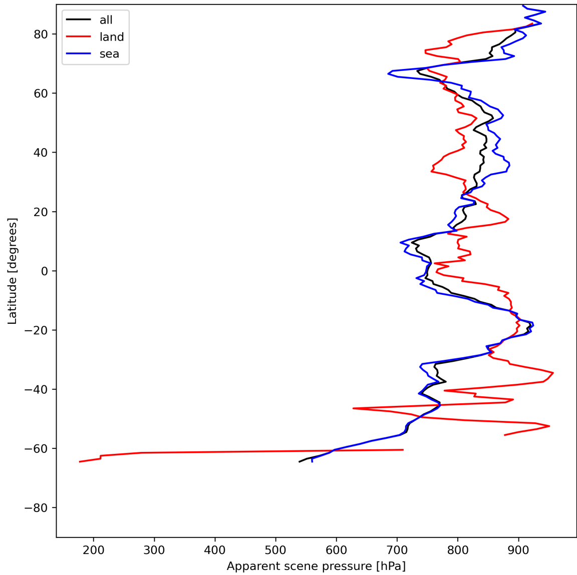
Figure 19: Zonal average of “Apparent scene pressure” for 2024-07-05 to 2024-07-06.
