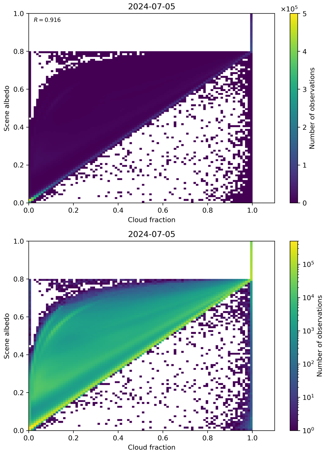
Figure 75: Scatter density plot of “Cloud fraction” against “Scene albedo” for 2024-07-05 to 2024-07-06.
