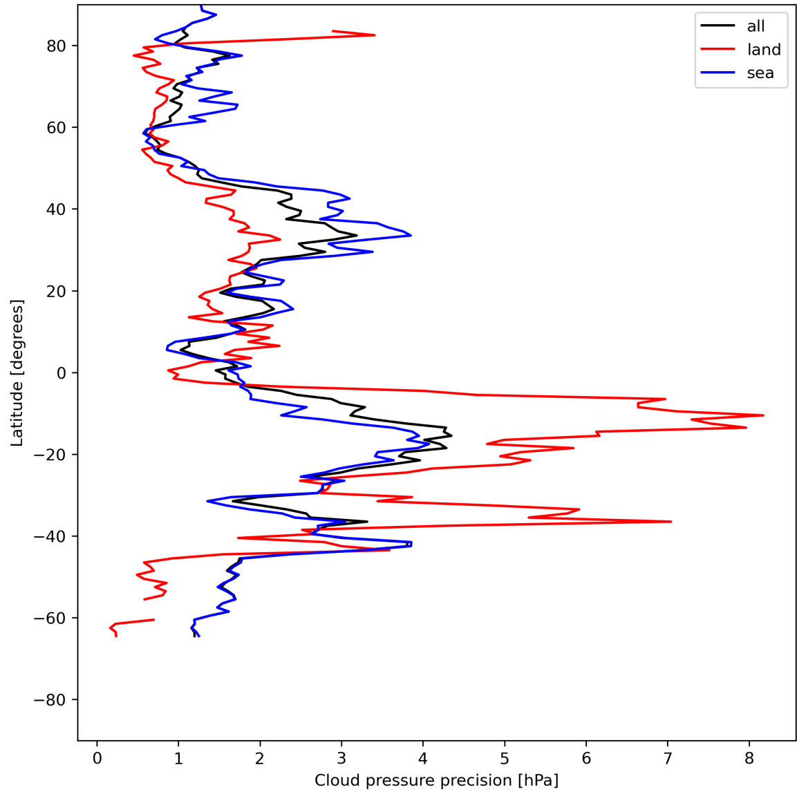
Figure 14: Zonal average of “Cloud pressure precision” for 2024-07-05 to 2024-07-06.
