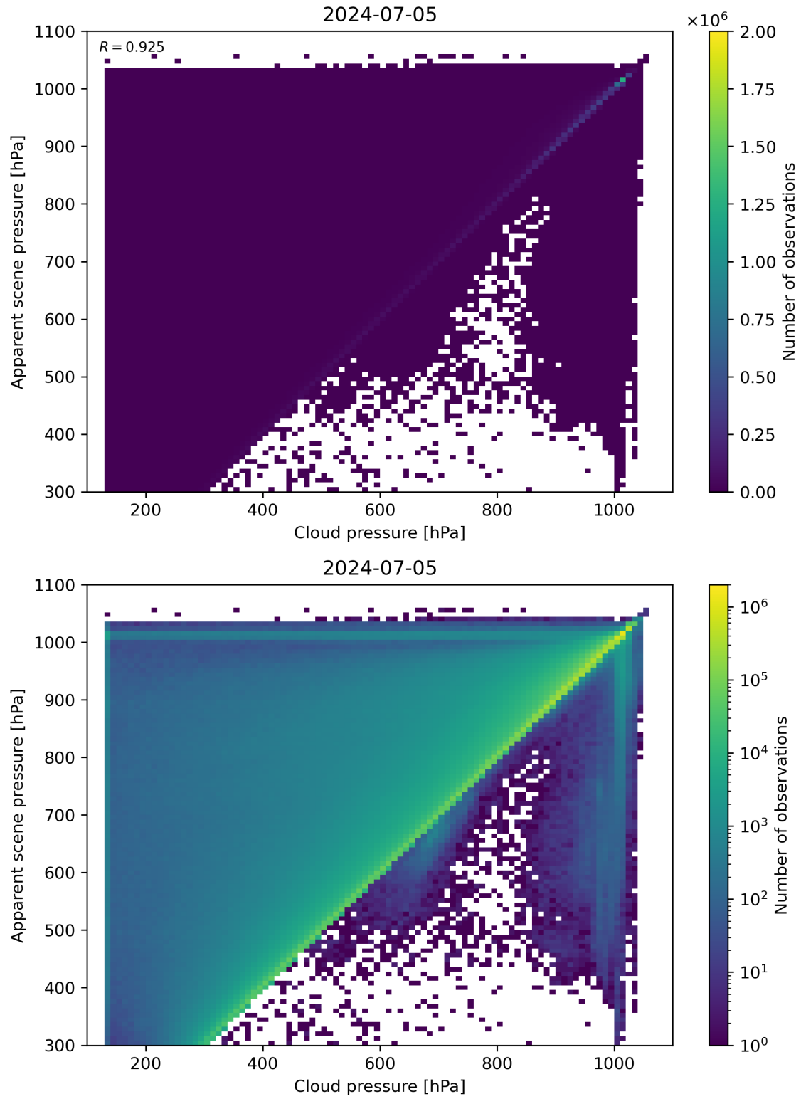
Figure 77: Scatter density plot of “Cloud pressure” against “Apparent scene pressure” for 2024-07-05 to 2024-07-06.
