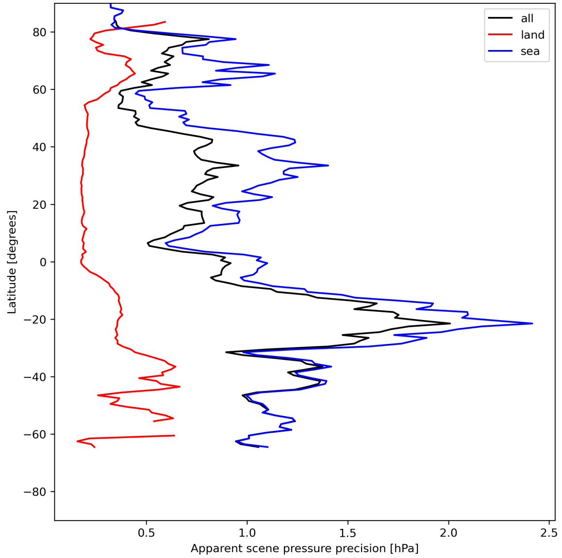
Figure 20: Zonal average of “Apparent scene pressure precision” for 2024-07-05 to 2024-07-06.
