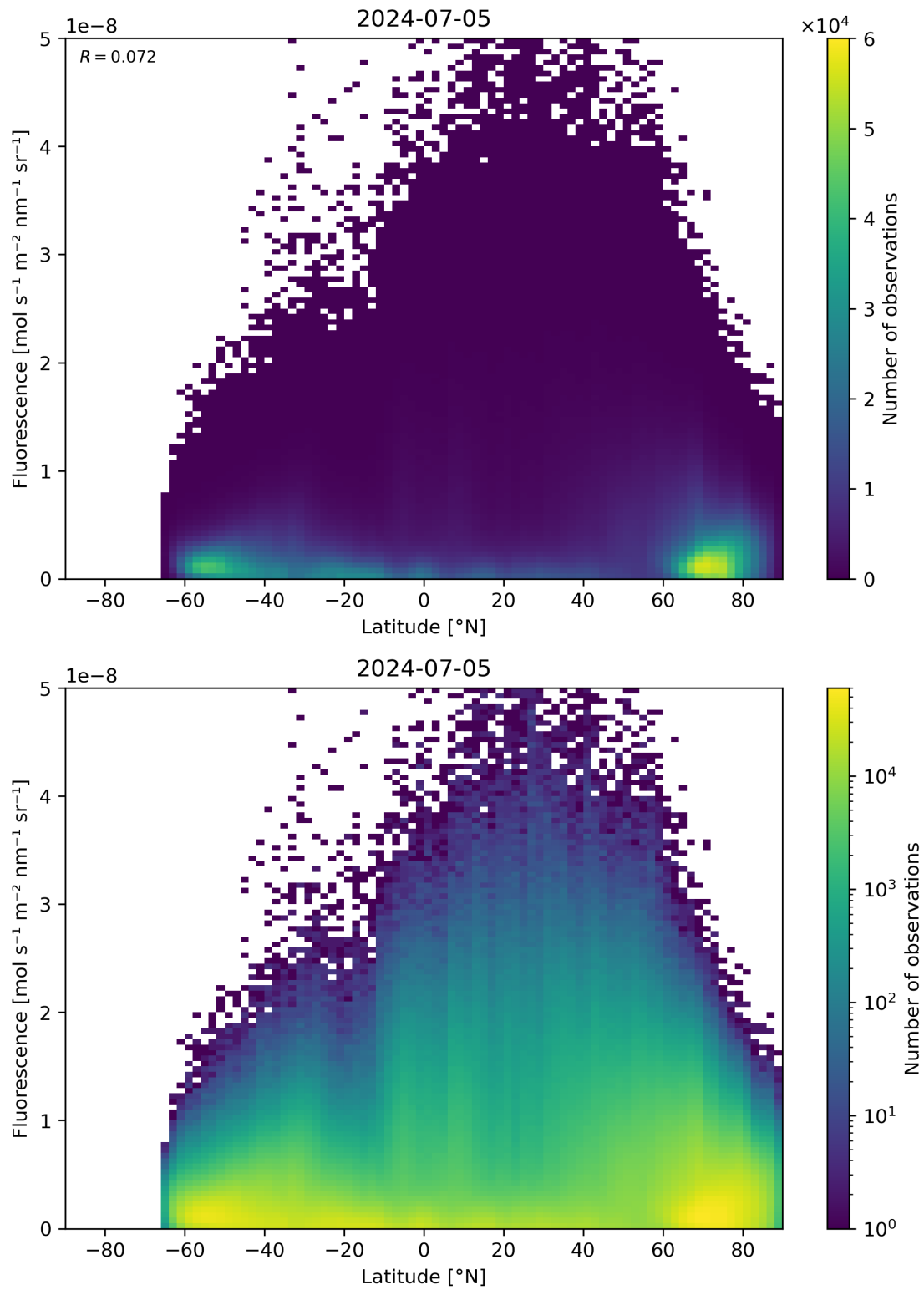
Figure 92: Scatter density plot of “Latitude” against “Fluorescence” for 2024-07-05 to 2024-07-06.
