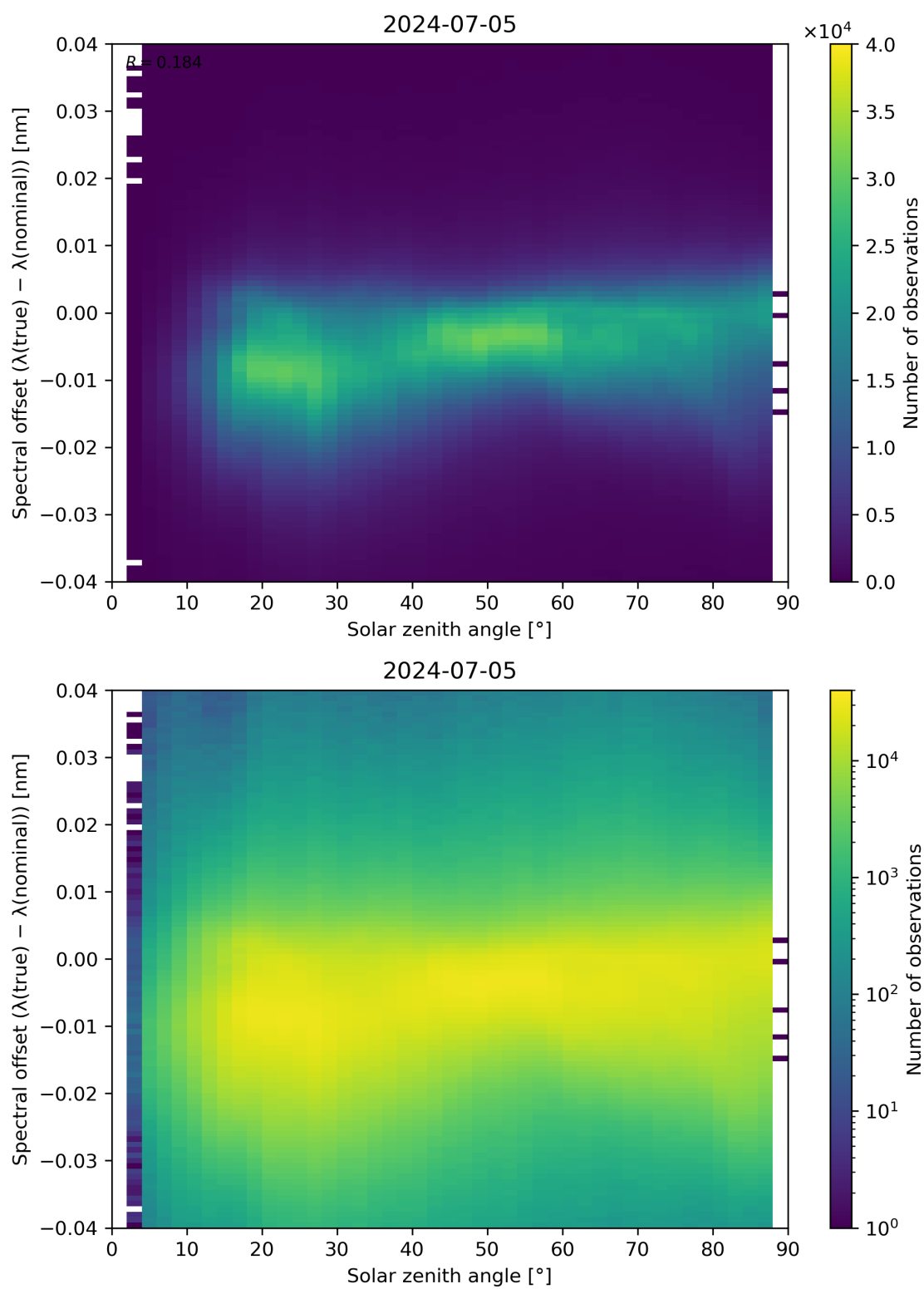
Figure 117: Scatter density plot of “Solar zenith angle” against “Spectral offset ( \lambda(\text{true}) - \lambda(\text{nominal}) )” for 2024-07-05 to 2024-07-06.
