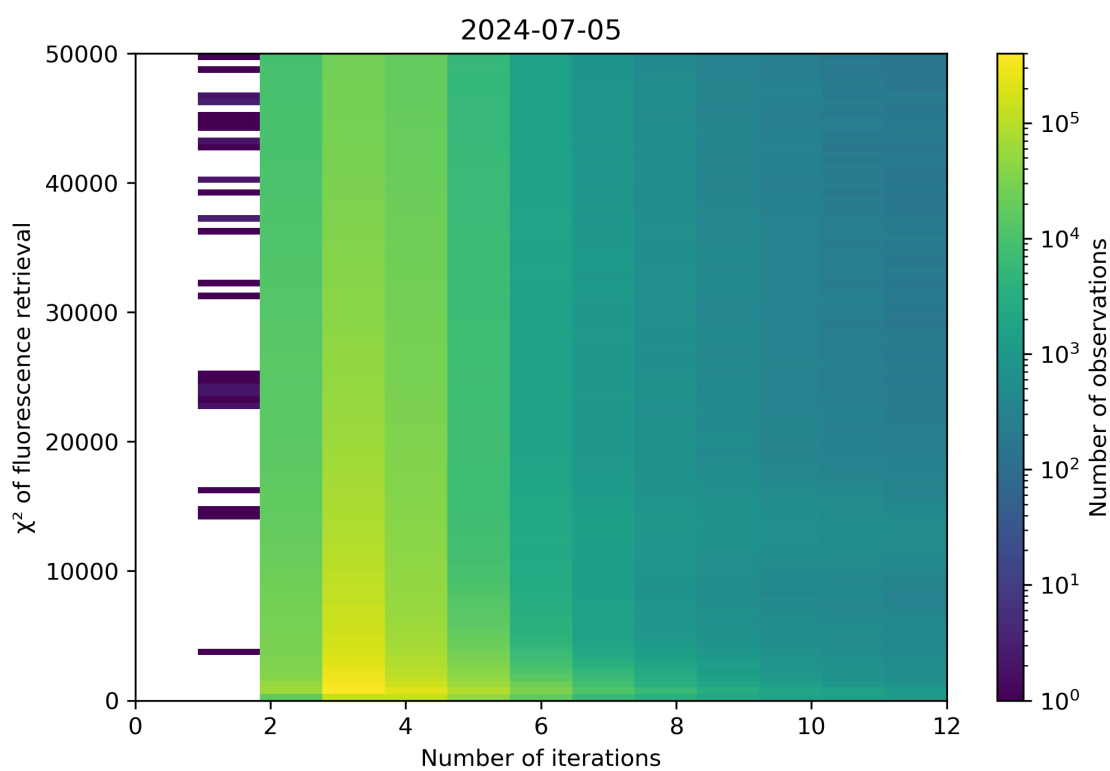
Figure 97: Scatter density plot of “Number of iterations” against “ \chi^2 of fluorescence retrieval” for 2024-07-05 to 2024-07-06.
