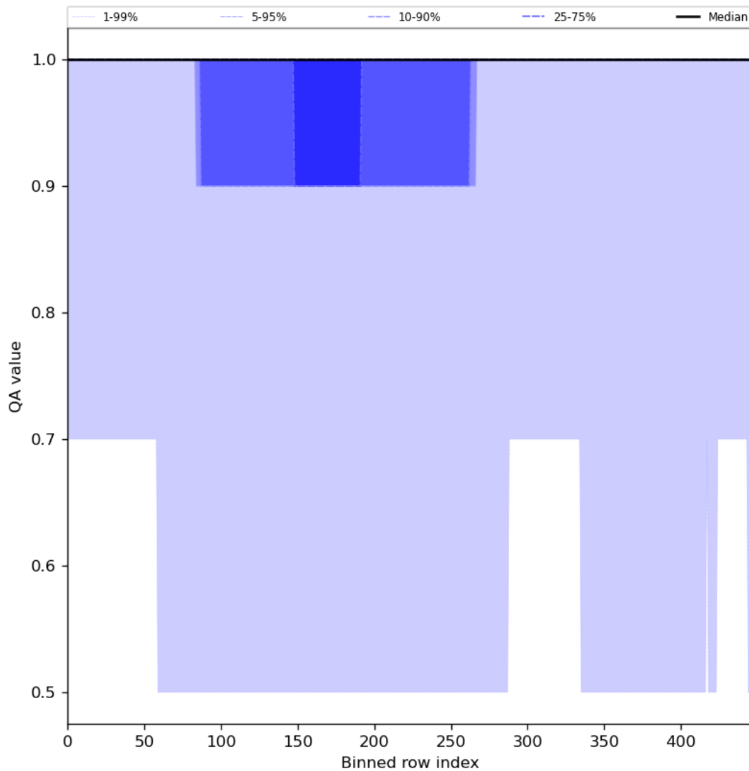
Figure 46: Along track statistics of “QA value” for 2024-07-05 to 2024-07-06
