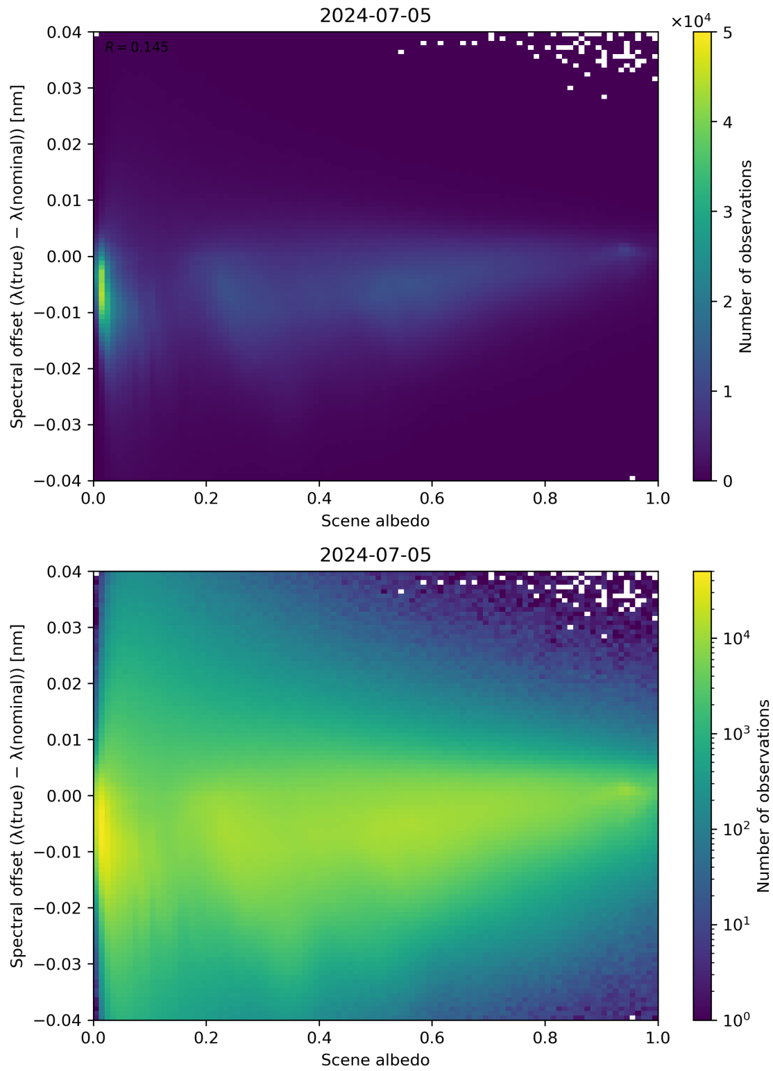
Figure 107: Scatter density plot of “Scene albedo” against “Spectral offset ( \lambda(\text{true}) - \lambda(\text{nominal}) )” for 2024-07-05 to 2024-07-06.
