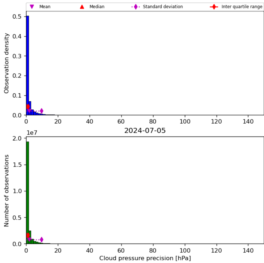
Figure 31: Histogram of “Cloud pressure precision” for 2024-07-05 to 2024-07-06
