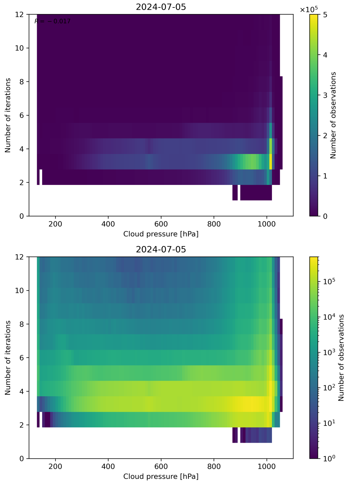
Figure 81: Scatter density plot of “Cloud pressure” against “Number of iterations” for 2024-07-05 to 2024-07-06.
