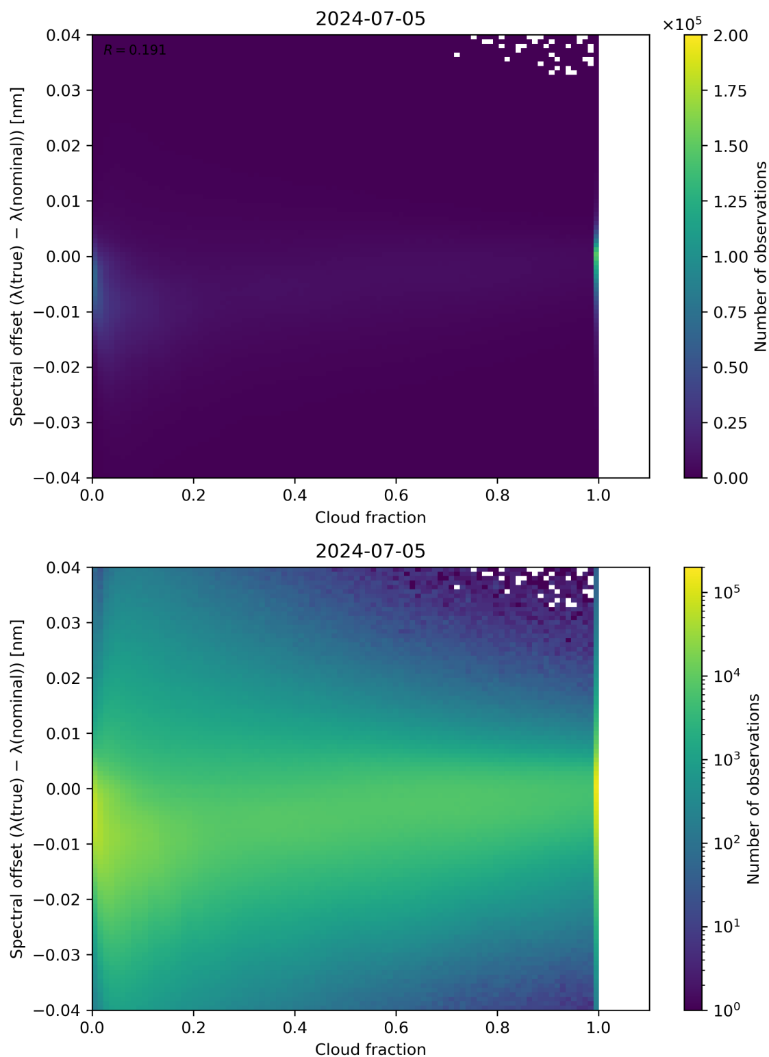
Figure 76: Scatter density plot of “Cloud fraction” against “Spectral offset ( \lambda(\text{true}) - \lambda(\text{nominal}) )” for 2024-07-05 to 2024-07-06.
