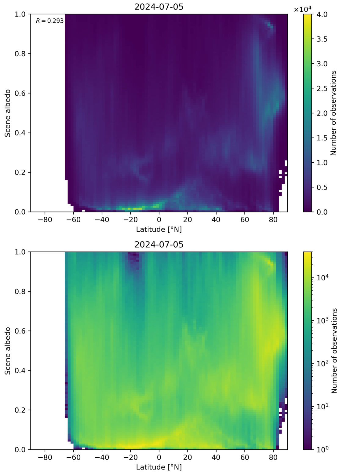
Figure 95: Scatter density plot of “Latitude” against “Scene albedo” for 2024-07-05 to 2024-07-06.
