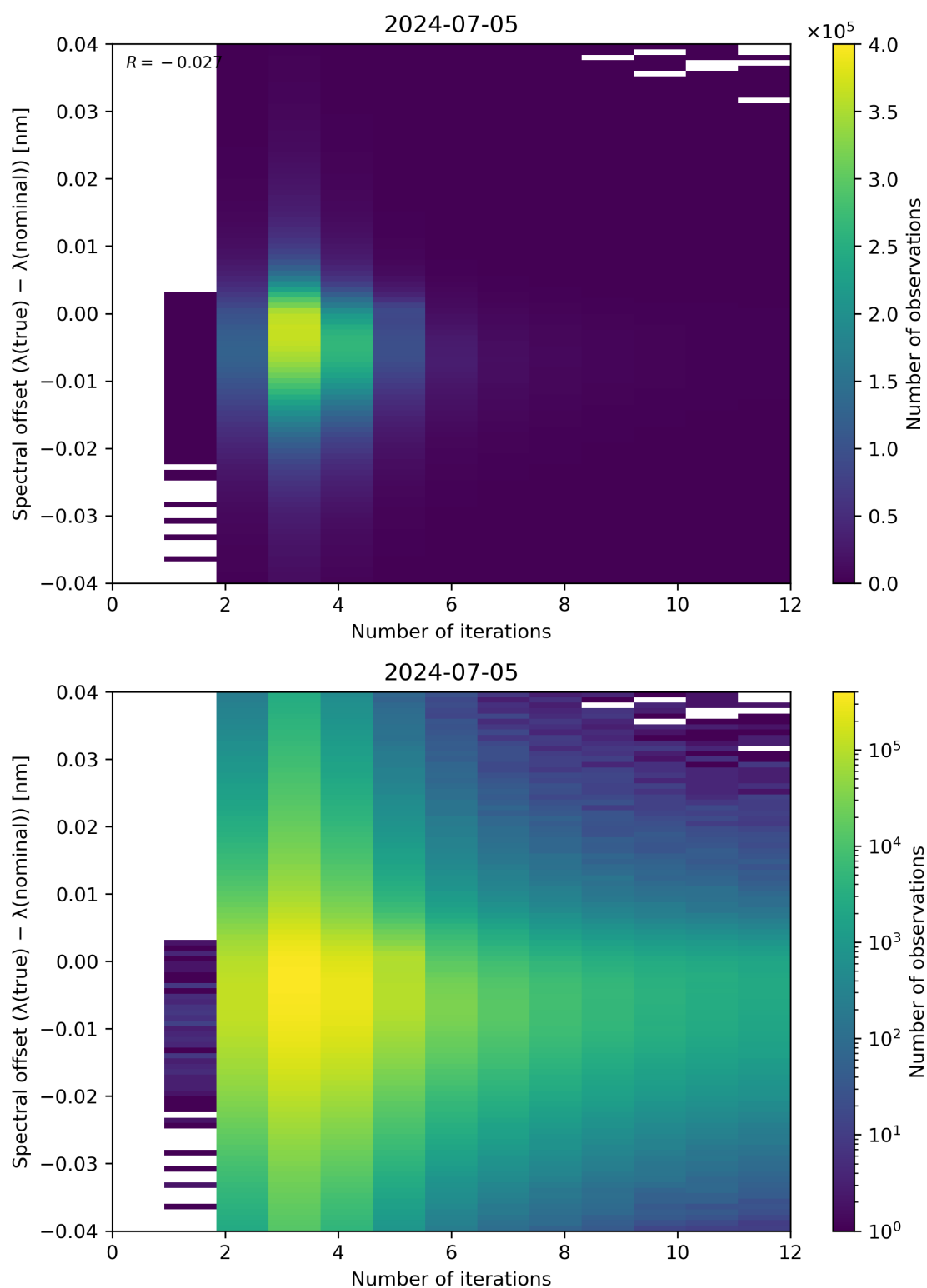
Figure 100: Scatter density plot of “Number of iterations” against “Spectral offset ( \lambda(\text{true}) - \lambda(\text{nominal}) )” for 2024-07-05 to 2024-07-06.
