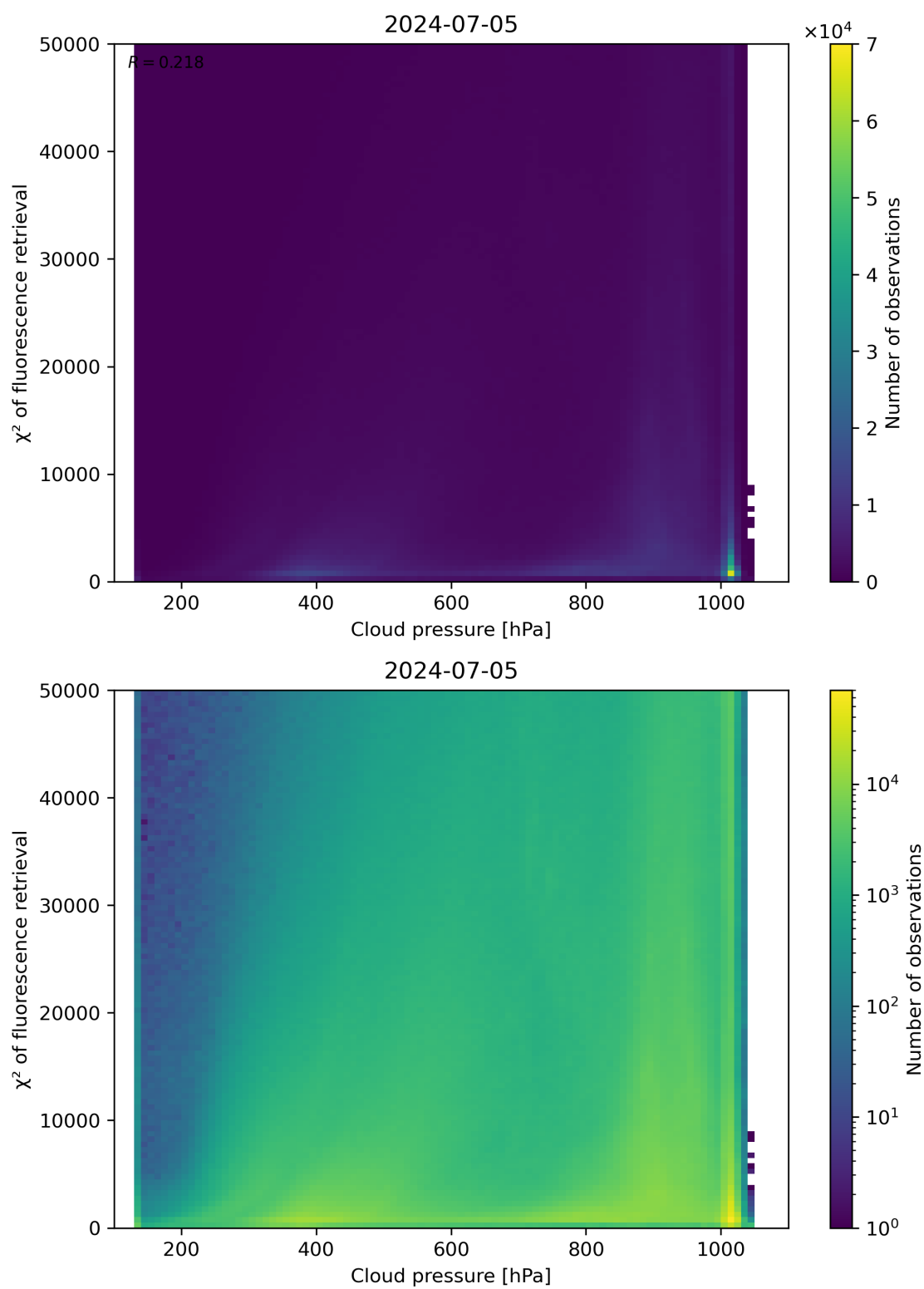
Figure 78: Scatter density plot of “Cloud pressure” against “ \chi^2 of fluorescence retrieval” for 2024-07-05 to 2024-07-06.
