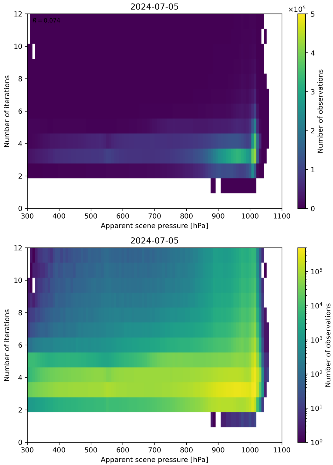
Figure 65: Scatter density plot of “Apparent scene pressure” against “Number of iterations” for 2024-07-05 to 2024-07-06.
