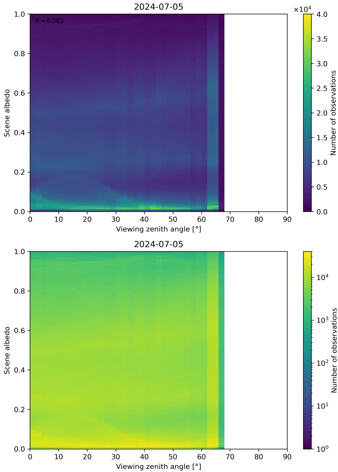
Figure 126: Scatter density plot of “Viewing zenith angle” against “Scene albedo” for 2024-07-05 to 2024-07-06.
