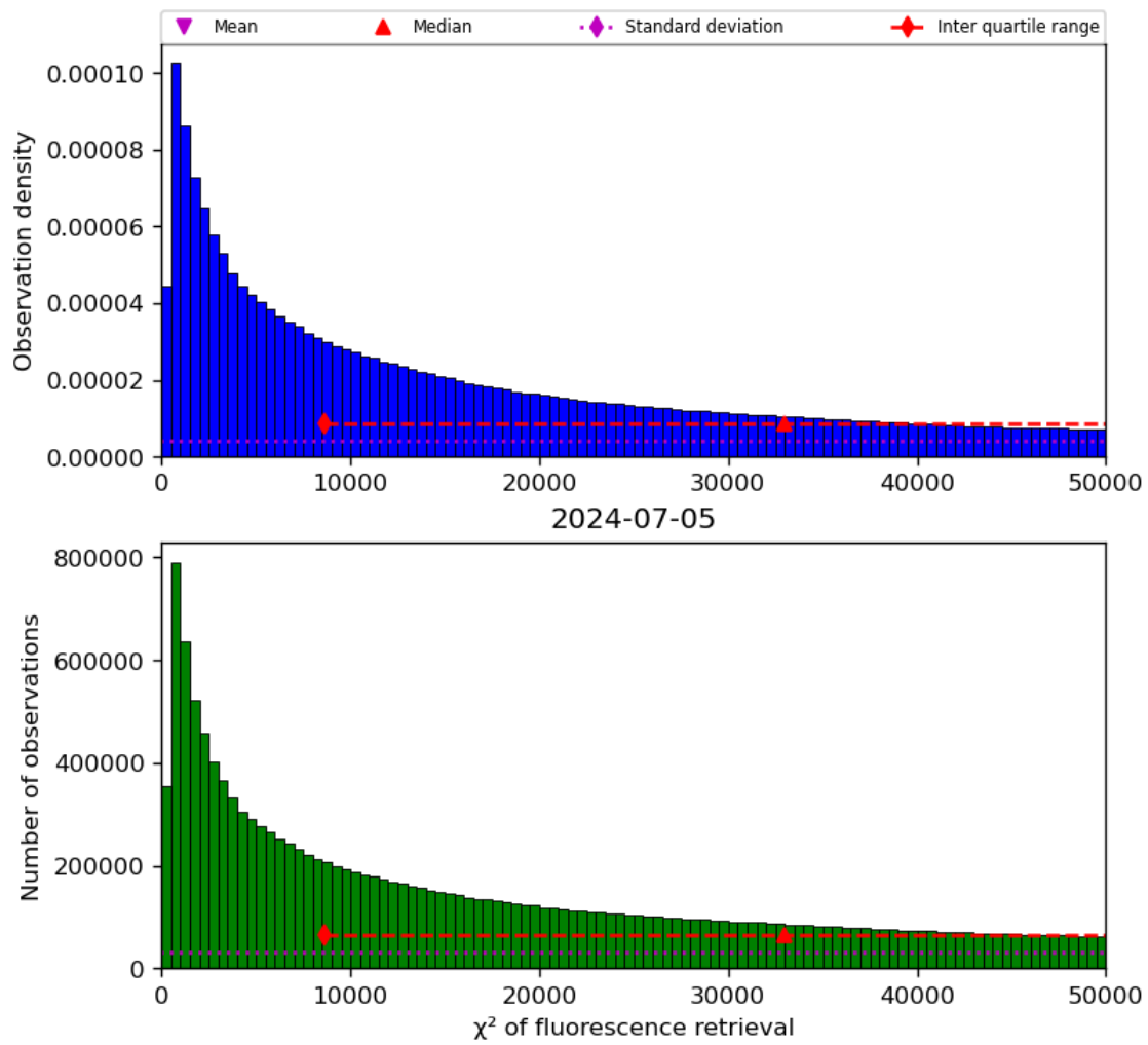
Figure 42: Histogram of “ \chi^2 of fluorescence retrieval” for 2024-07-05 to 2024-07-06
