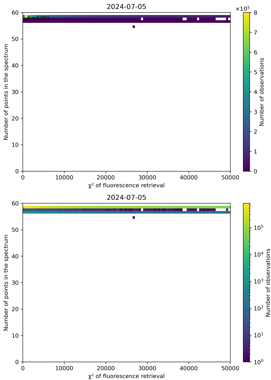
Figure 68: Scatter density plot of “ \chi^2 of fluorescence retrieval” against “Number of points in the spectrum” for 2024-07-05 to 2024-07-06.
