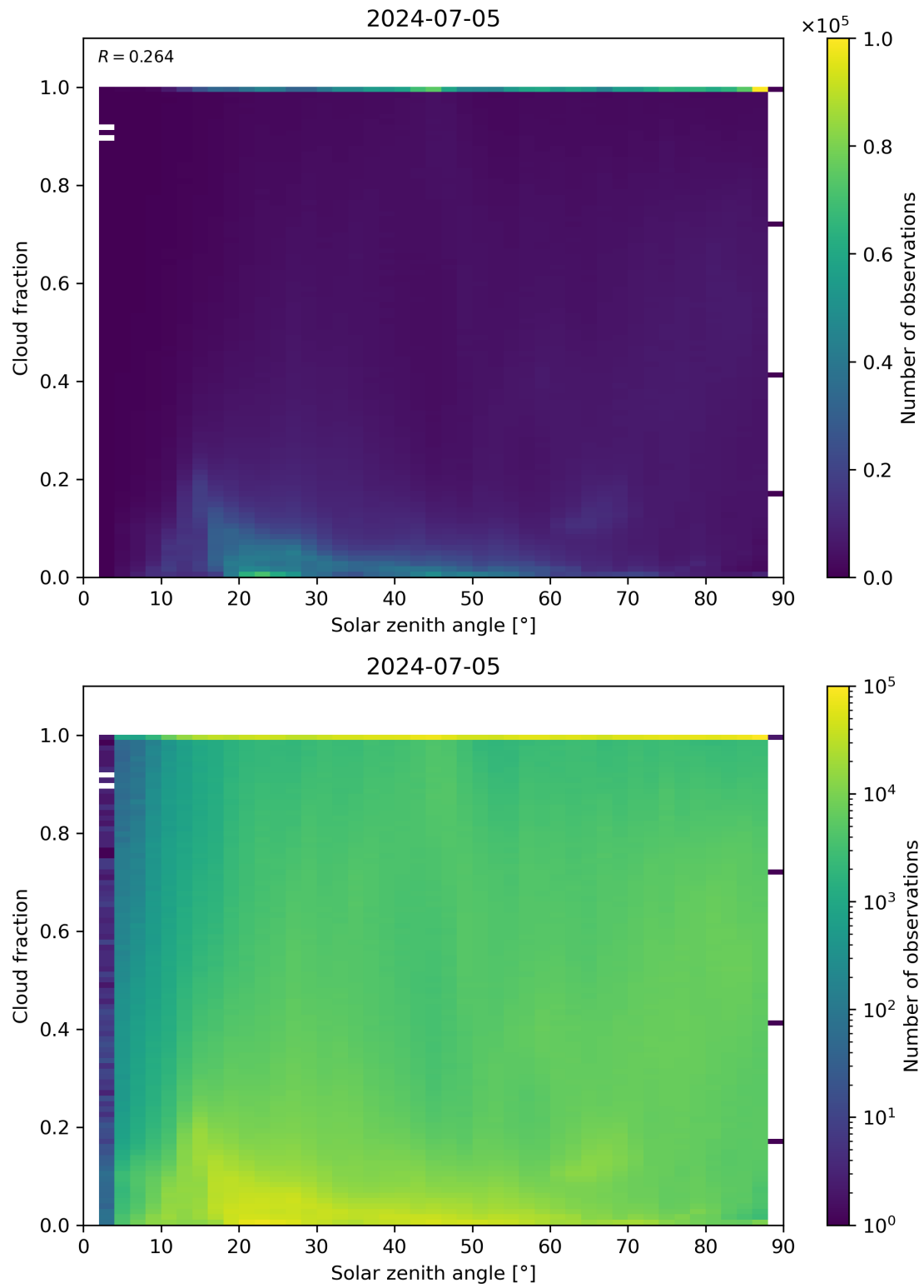
Figure 110: Scatter density plot of “Solar zenith angle” against “Cloud fraction” for 2024-07-05 to 2024-07-06.
