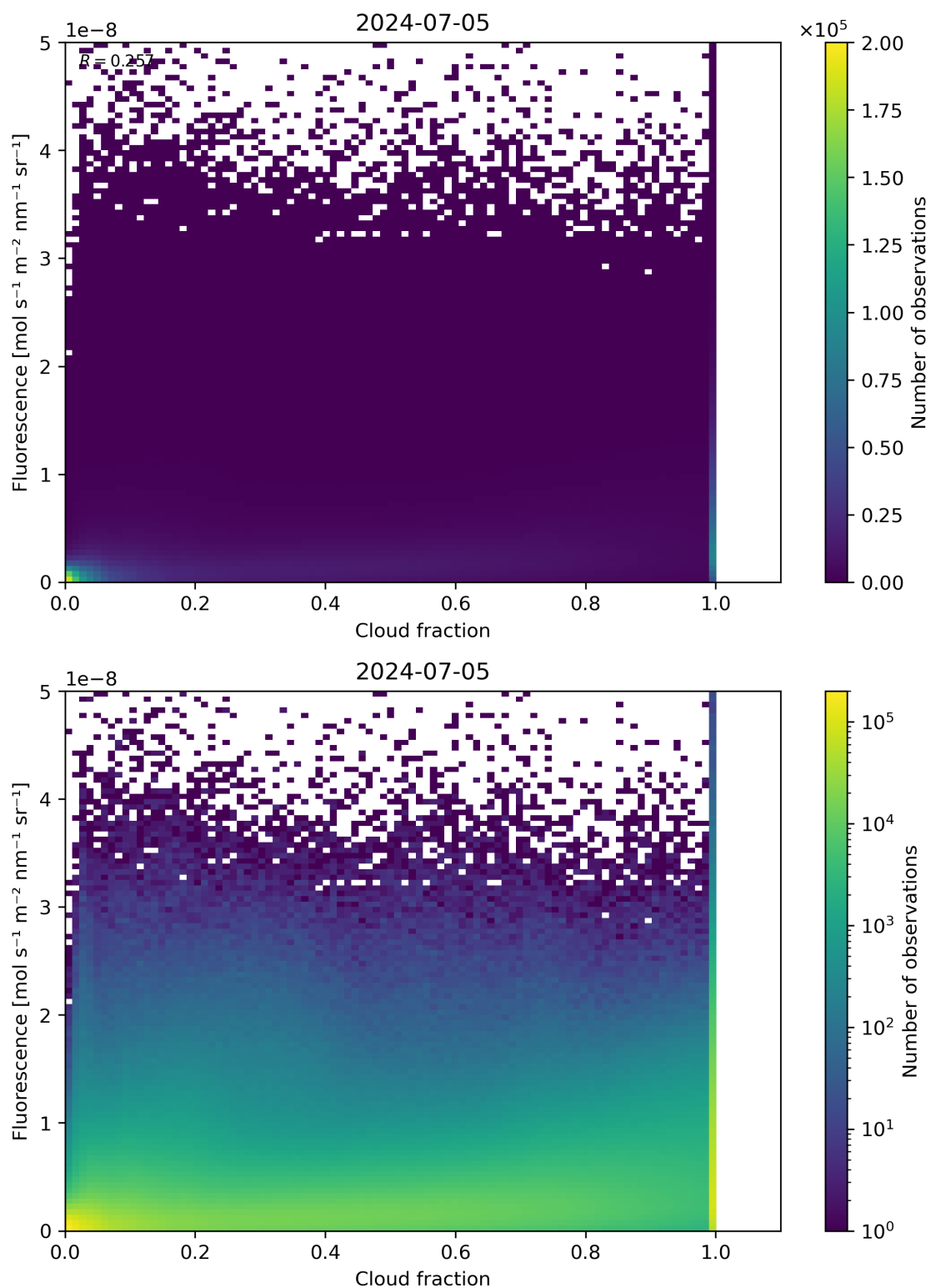
Figure 72: Scatter density plot of “Cloud fraction” against “Fluorescence” for 2024-07-05 to 2024-07-06.
