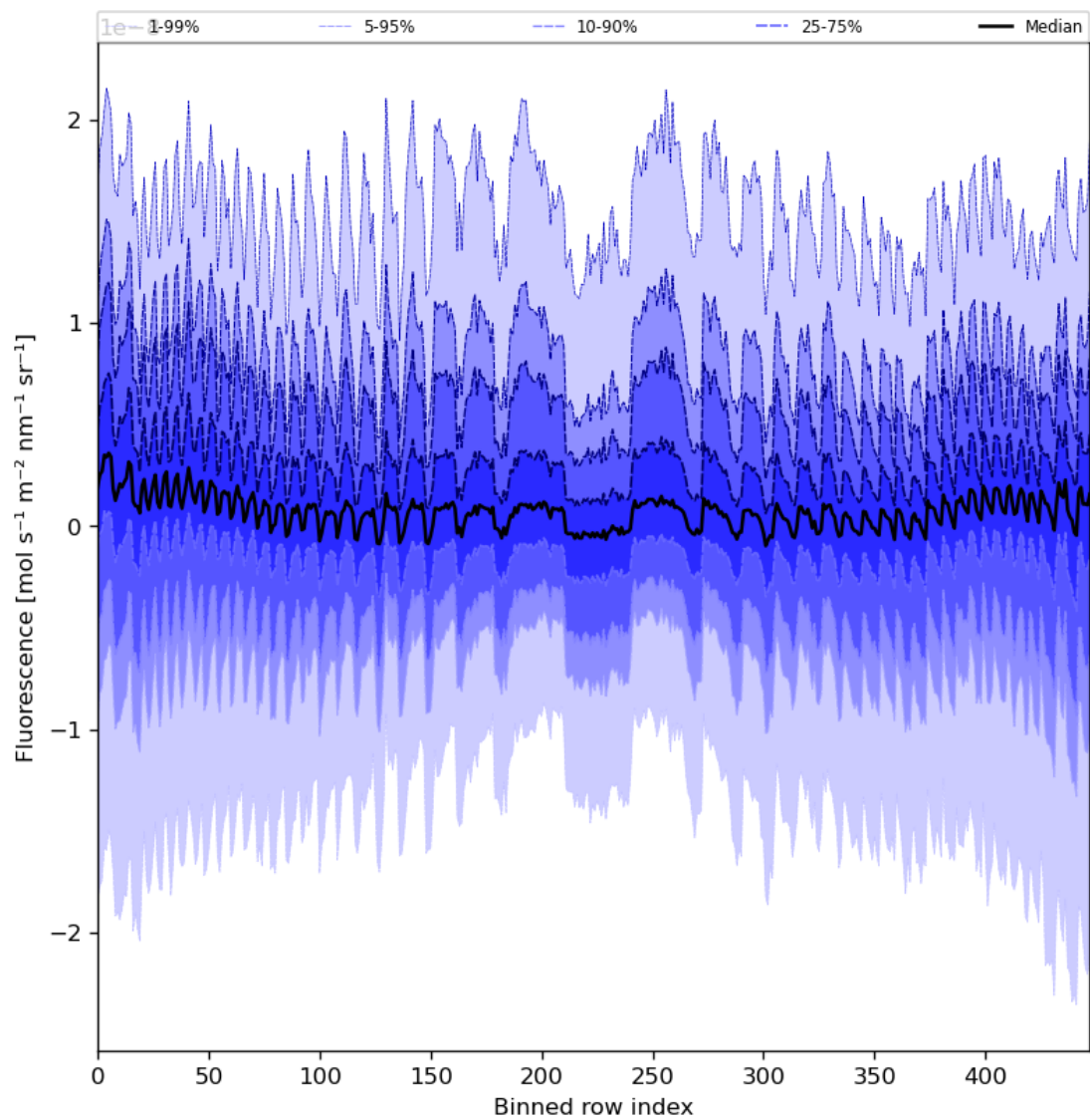
Figure 57: Along track statistics of “Fluorescence” for 2024-07-05 to 2024-07-06
