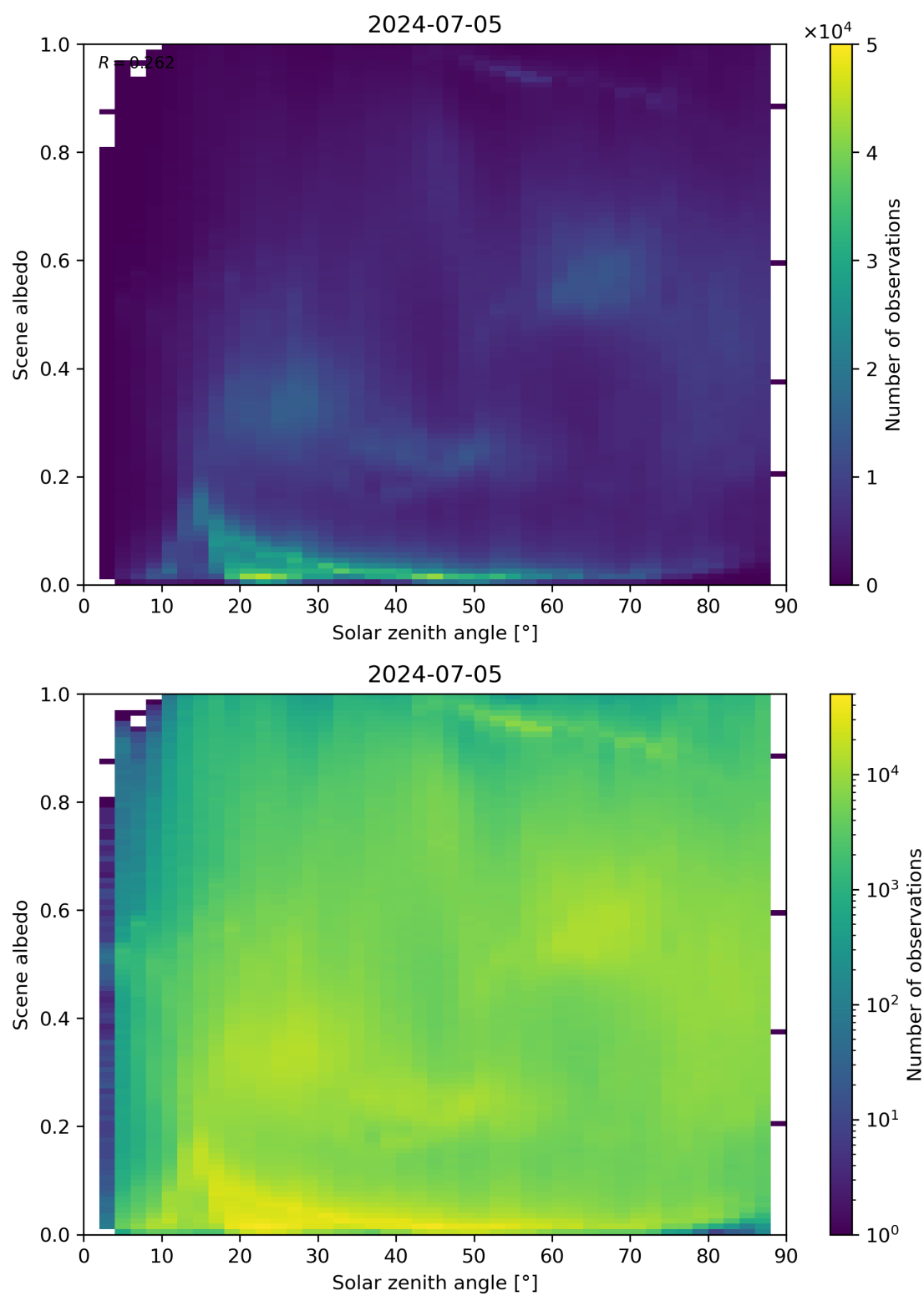
Figure 116: Scatter density plot of “Solar zenith angle” against “Scene albedo” for 2024-07-05 to 2024-07-06.
