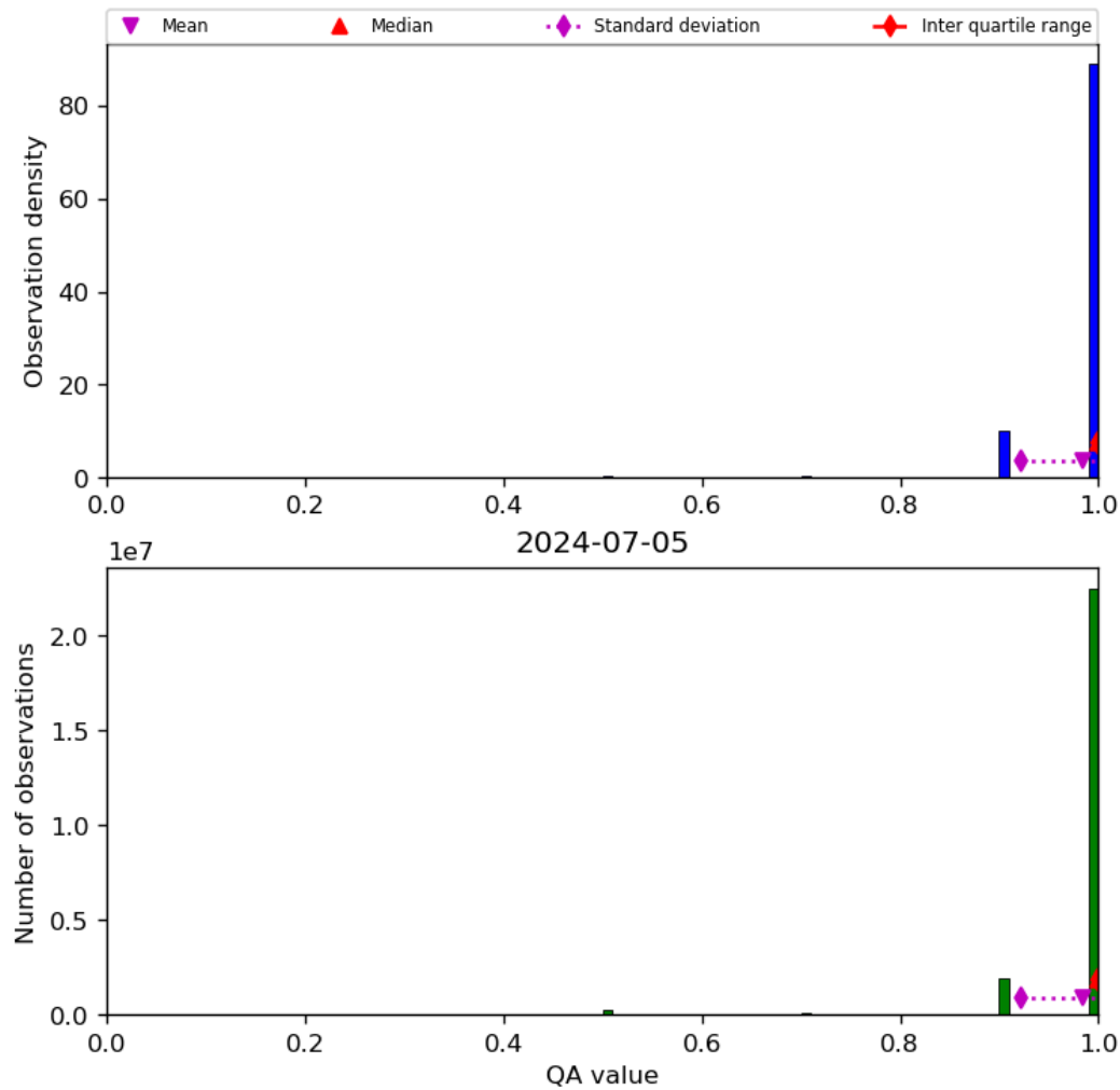
Figure 29: Histogram of “QA value” for 2024-07-05 to 2024-07-06
