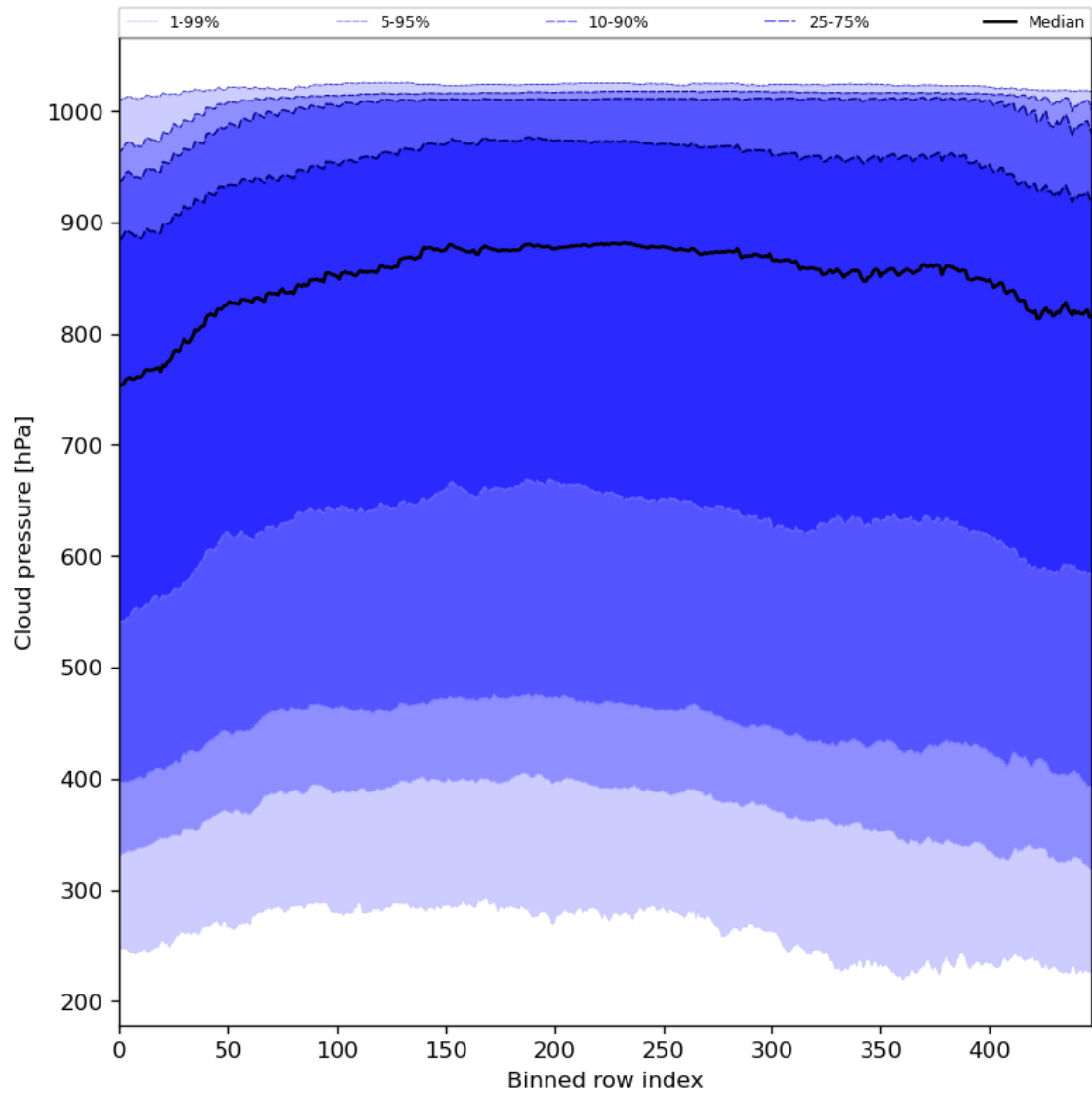
Figure 47: Along track statistics of “Cloud pressure” for 2024-07-05 to 2024-07-06
