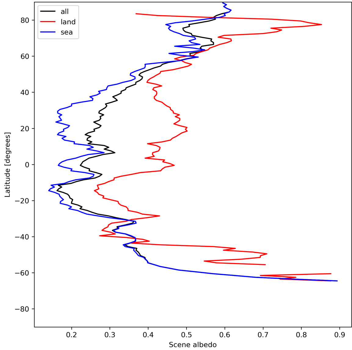
Figure 17: Zonal average of “Scene albedo” for 2024-07-05 to 2024-07-06.
