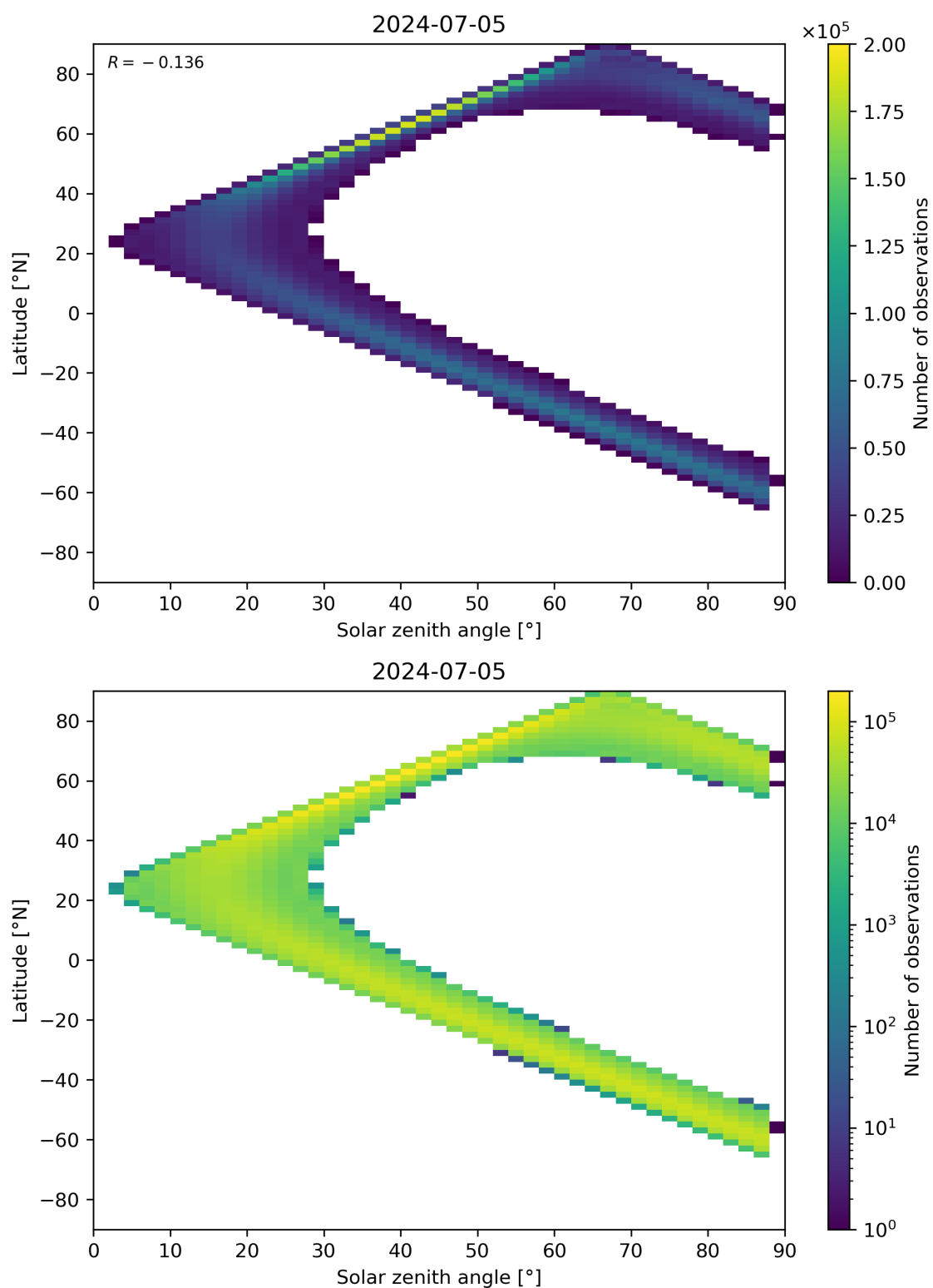
Figure 113: Scatter density plot of “Solar zenith angle” against “Latitude” for 2024-07-05 to 2024-07-06.
