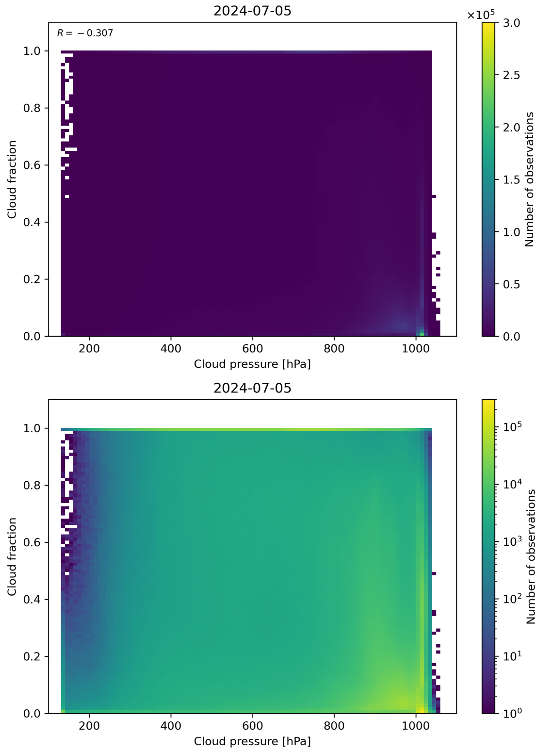
Figure 79: Scatter density plot of “Cloud pressure” against “Cloud fraction” for 2024-07-05 to 2024-07-06.
