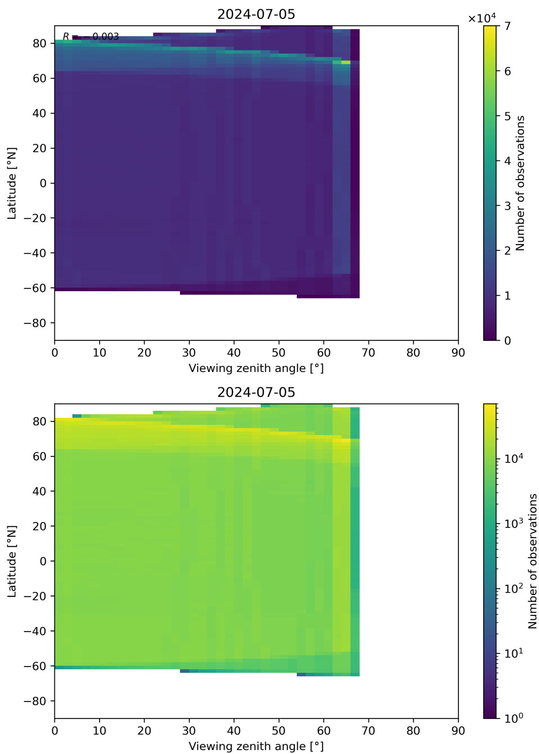
Figure 123: Scatter density plot of “Viewing zenith angle” against “Latitude” for 2024-07-05 to 2024-07-06.
