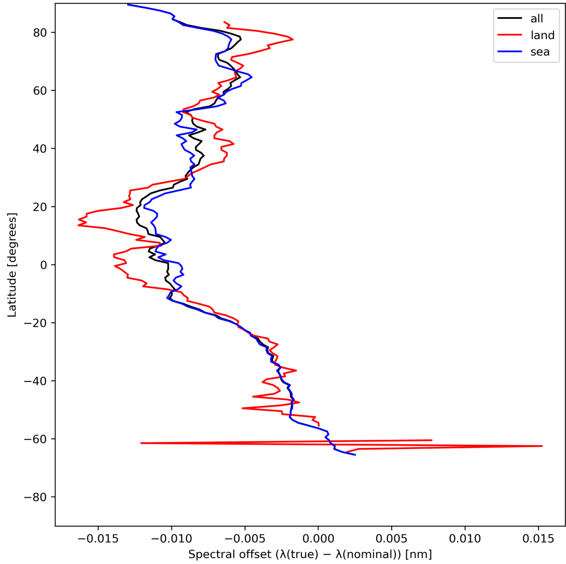
Figure 28: Zonal average of “Spectral offset ( \lambda(\text{true}) - \lambda(\text{nominal}) )” for 2024-07-05 to 2024-07-07.
