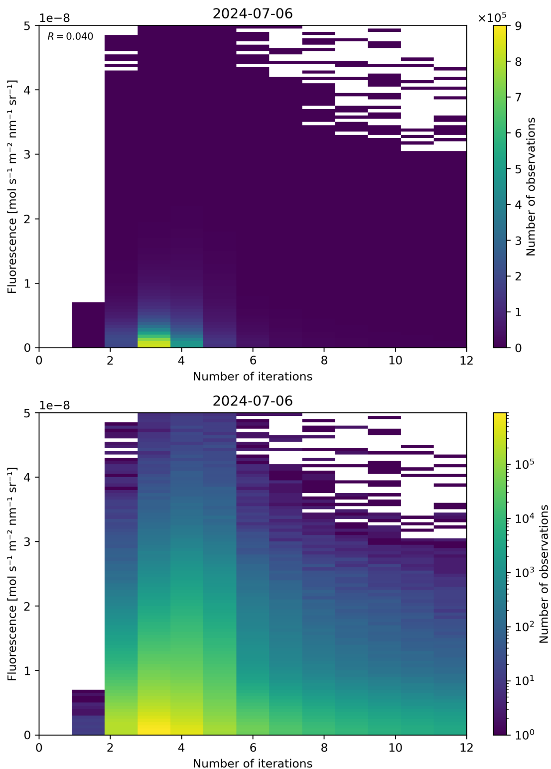
Figure 98: Scatter density plot of “Number of iterations” against “Fluorescence” for 2024-07-05 to 2024-07-07.
