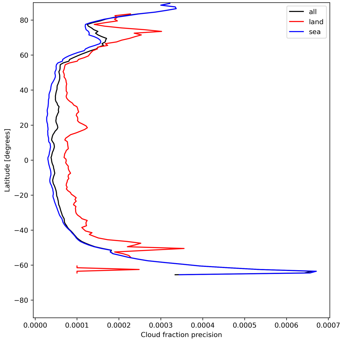
Figure 16: Zonal average of “Cloud fraction precision” for 2024-07-05 to 2024-07-07.
