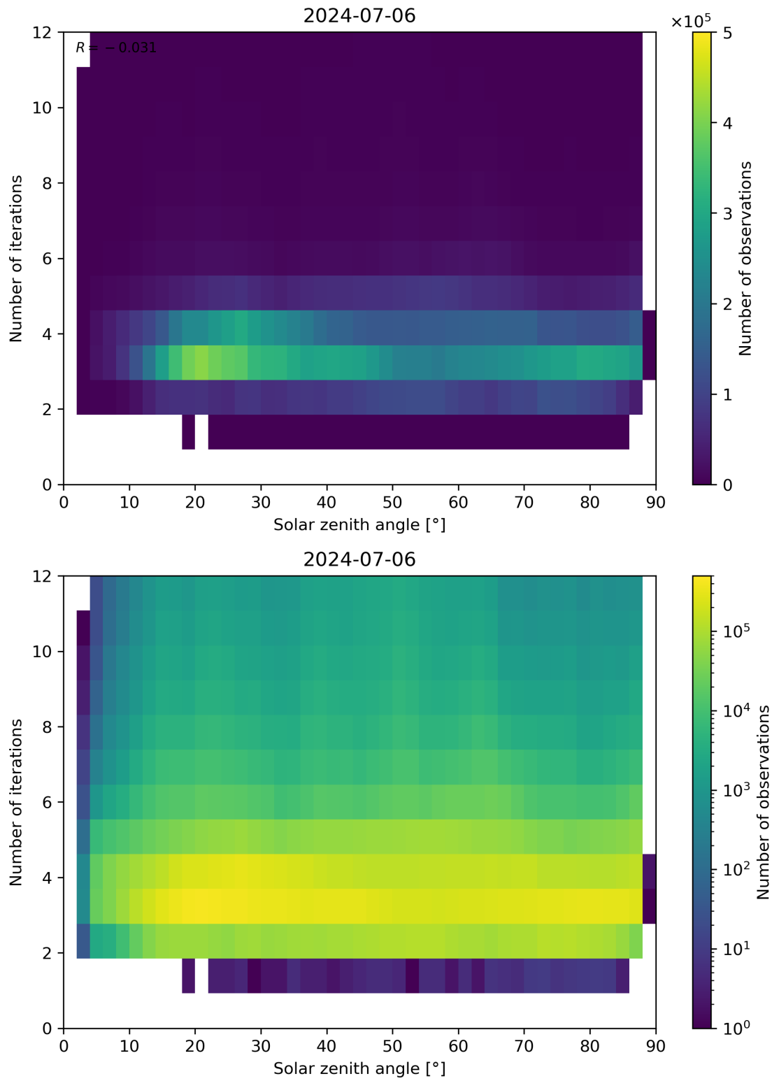
Figure 114: Scatter density plot of “Solar zenith angle” against “Number of iterations” for 2024-07-05 to 2024-07-07.
