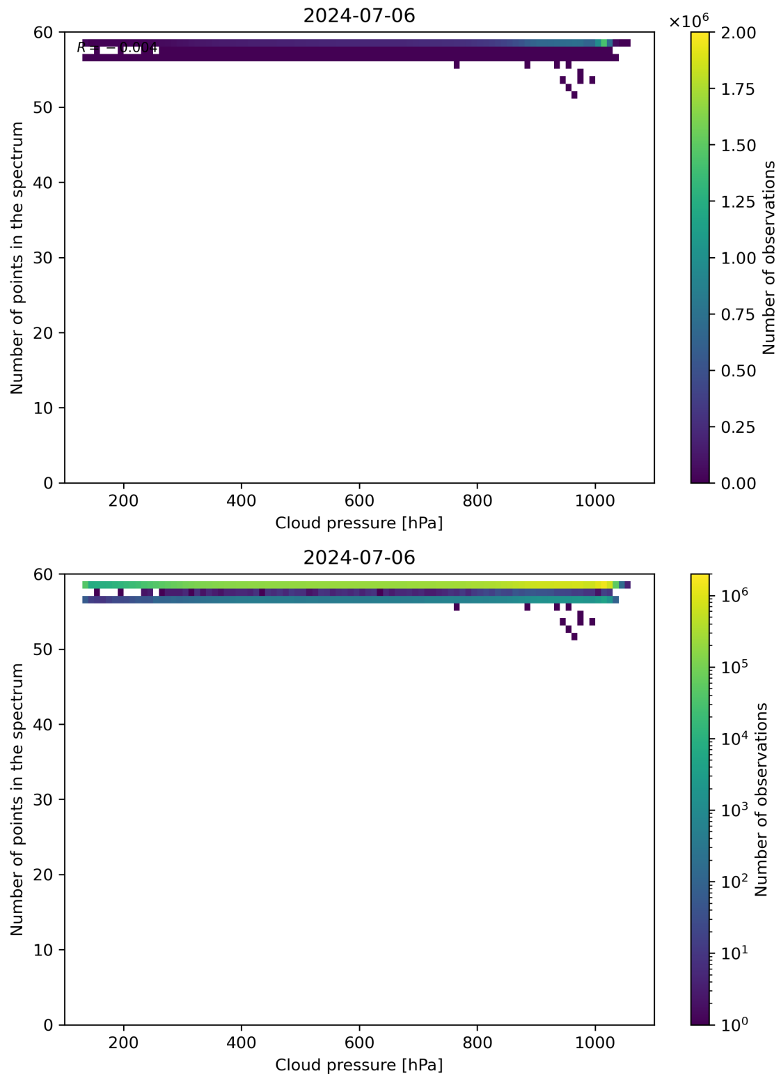
Figure 82: Scatter density plot of “Cloud pressure” against “Number of points in the spectrum” for 2024-07-05 to 2024-07-07.
