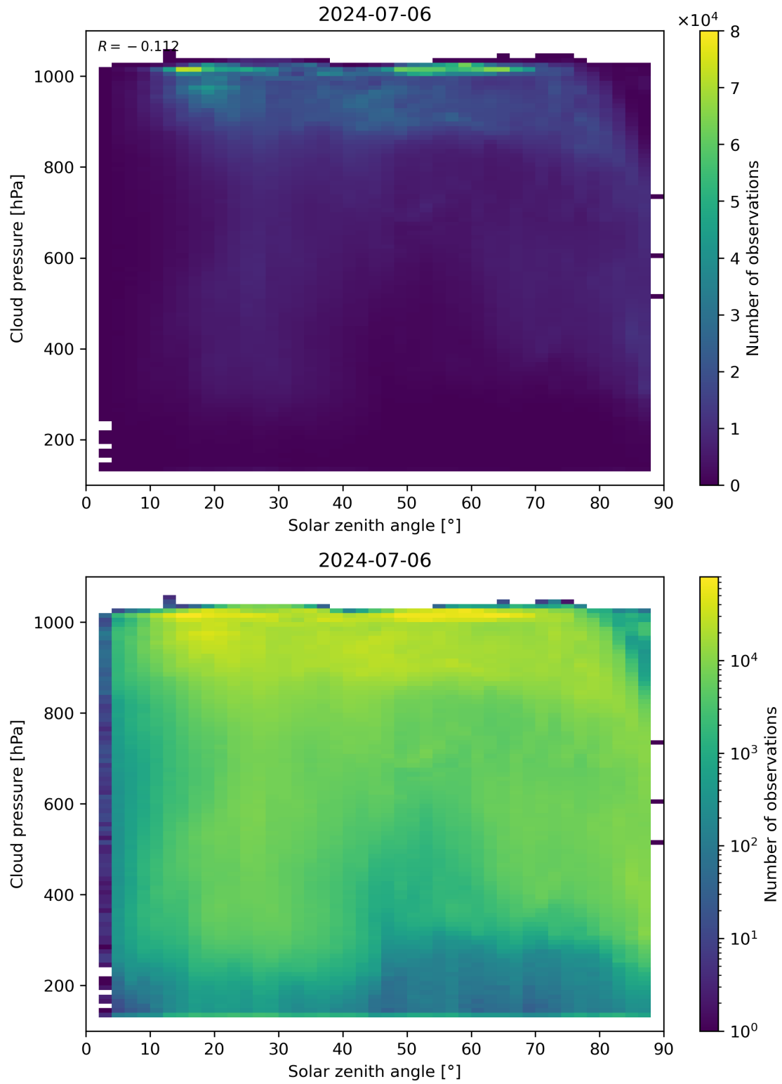
Figure 111: Scatter density plot of “Solar zenith angle” against “Cloud pressure” for 2024-07-05 to 2024-07-07.
