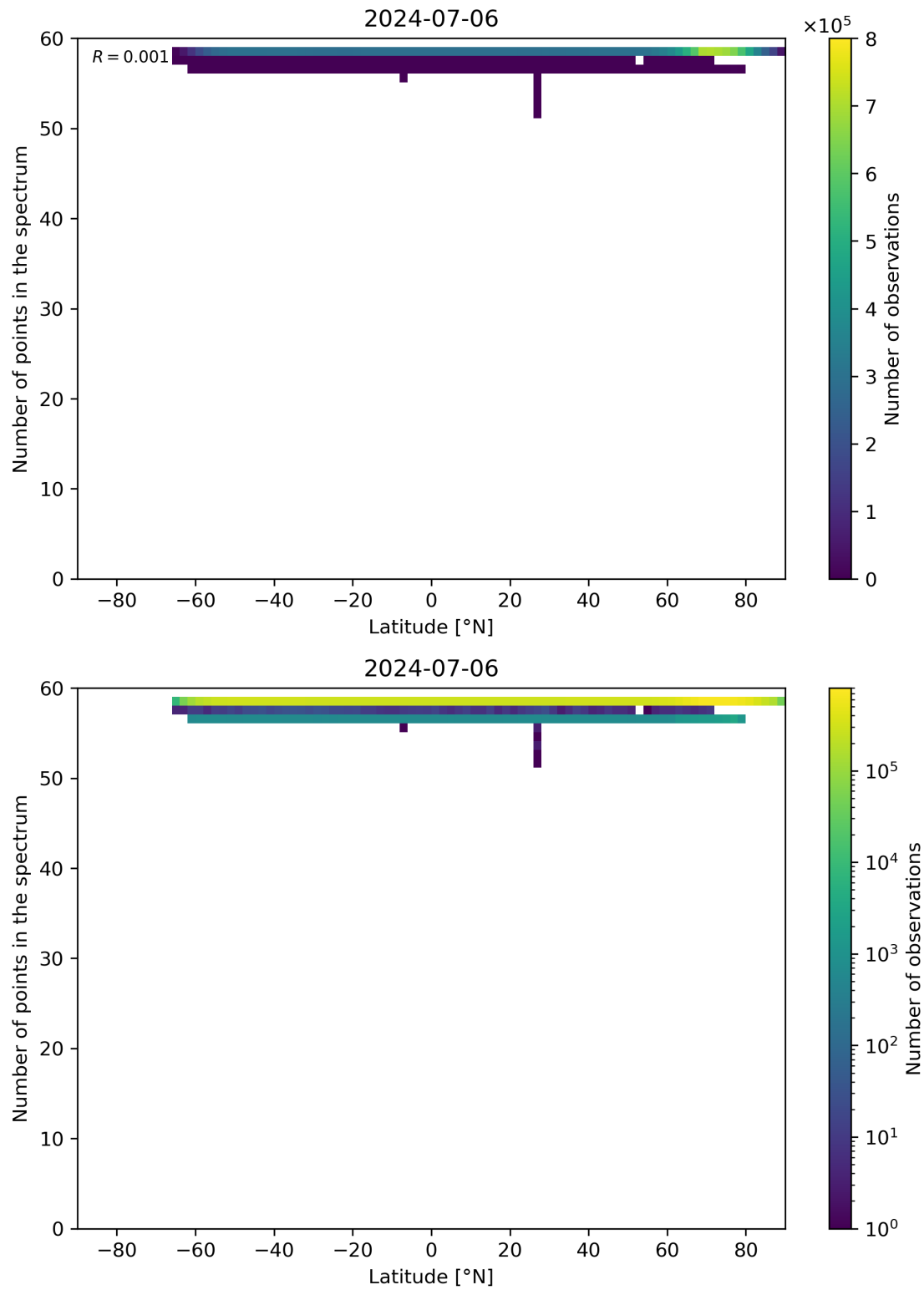
Figure 94: Scatter density plot of “Latitude” against “Number of points in the spectrum” for 2024-07-05 to 2024-07-07.
