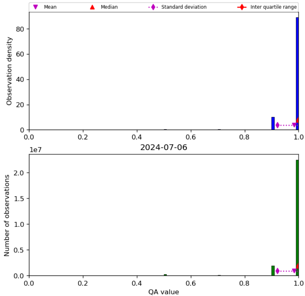
Figure 29: Histogram of “QA value” for 2024-07-05 to 2024-07-07
