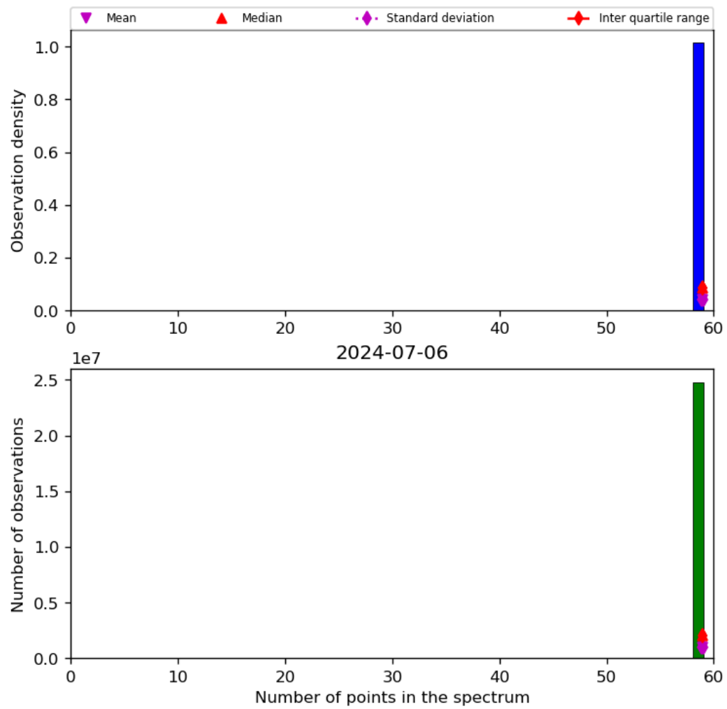
Figure 44: Histogram of “Number of points in the spectrum” for 2024-07-05 to 2024-07-07
