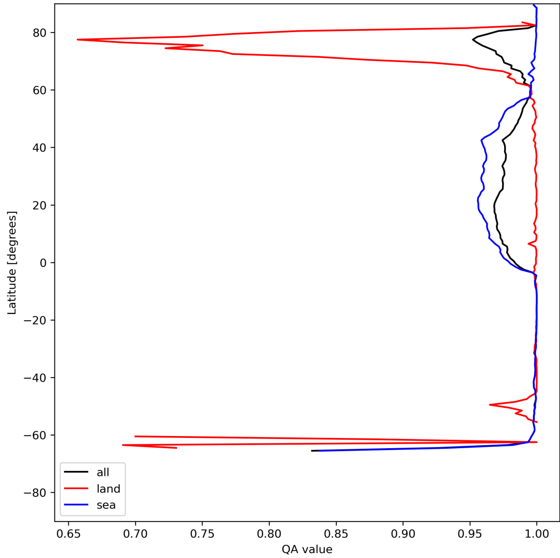
Figure 12: Zonal average of “QA value” for 2024-07-05 to 2024-07-07.
