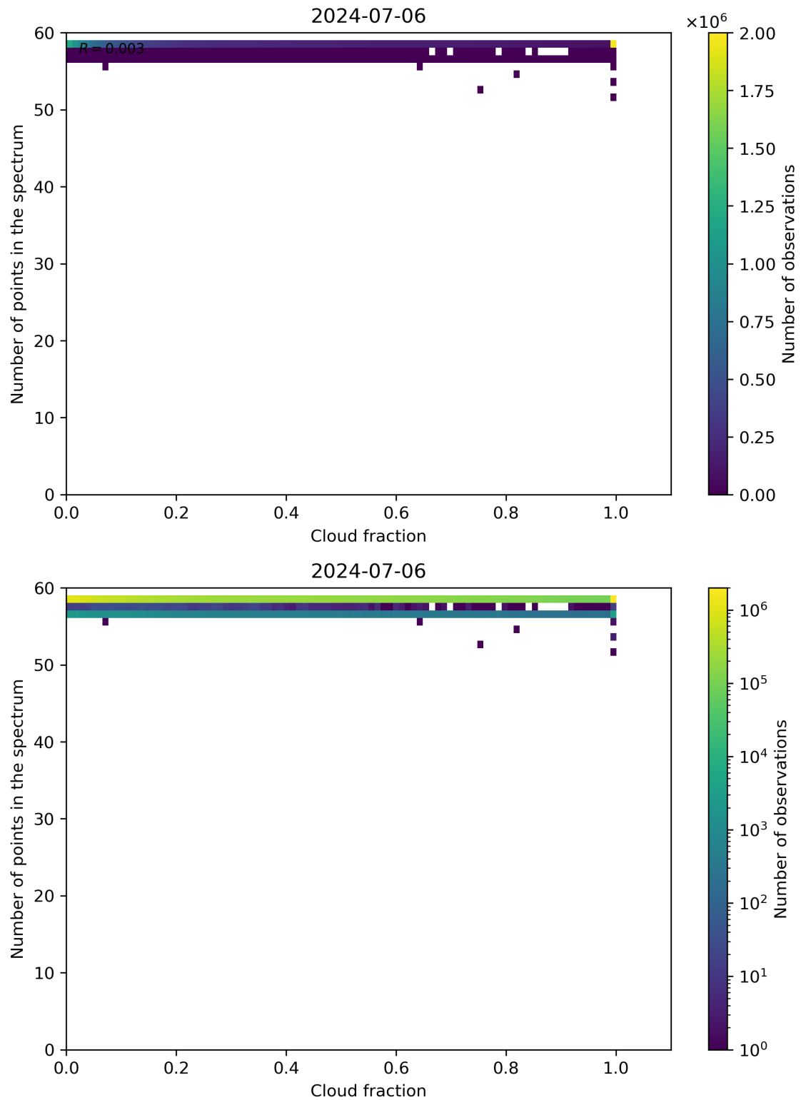
Figure 74: Scatter density plot of “Cloud fraction” against “Number of points in the spectrum” for 2024-07-05 to 2024-07-07.
