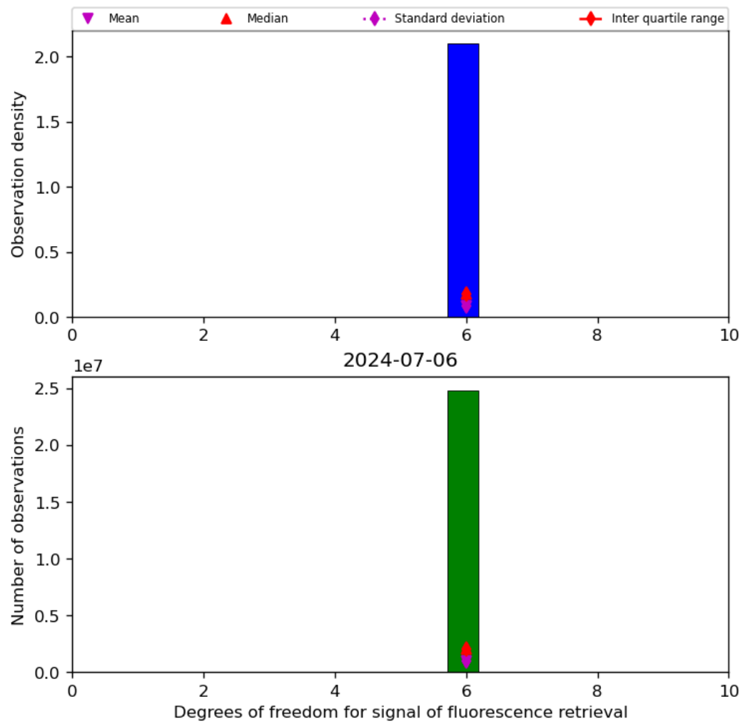
Figure 43: Histogram of “Degrees of freedom for signal of fluorescence retrieval” for 2024-07-05 to 2024-07-07
