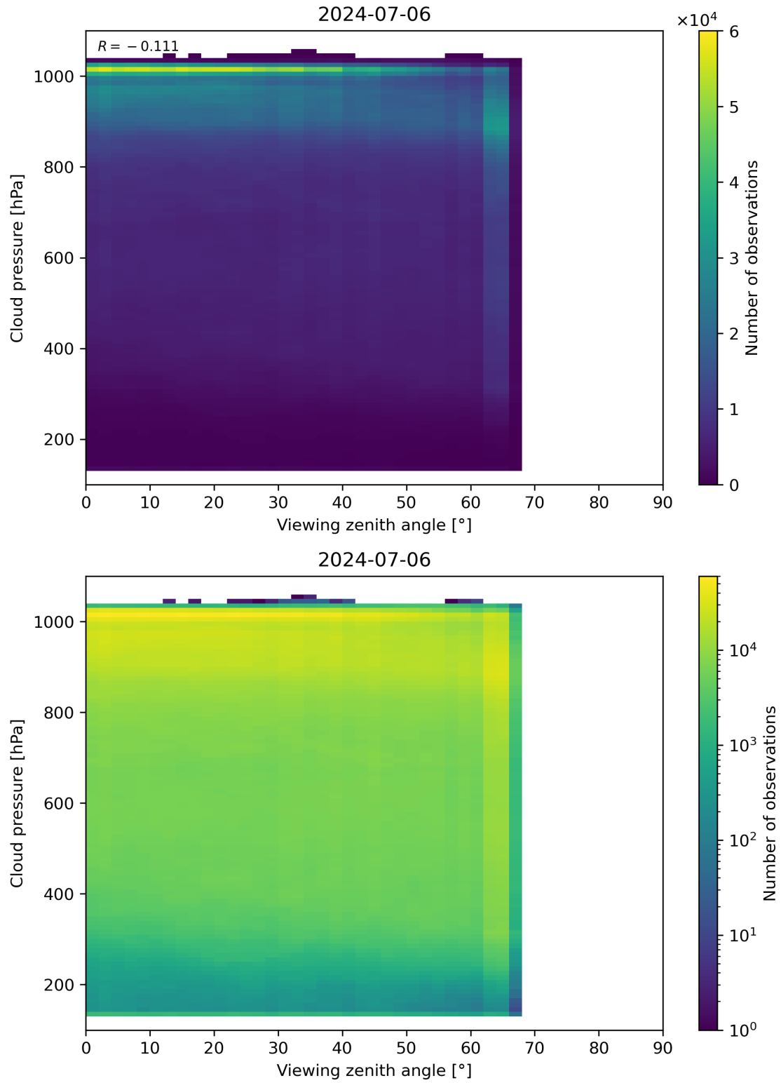
Figure 121: Scatter density plot of “Viewing zenith angle” against “Cloud pressure” for 2024-07-05 to 2024-07-07.
