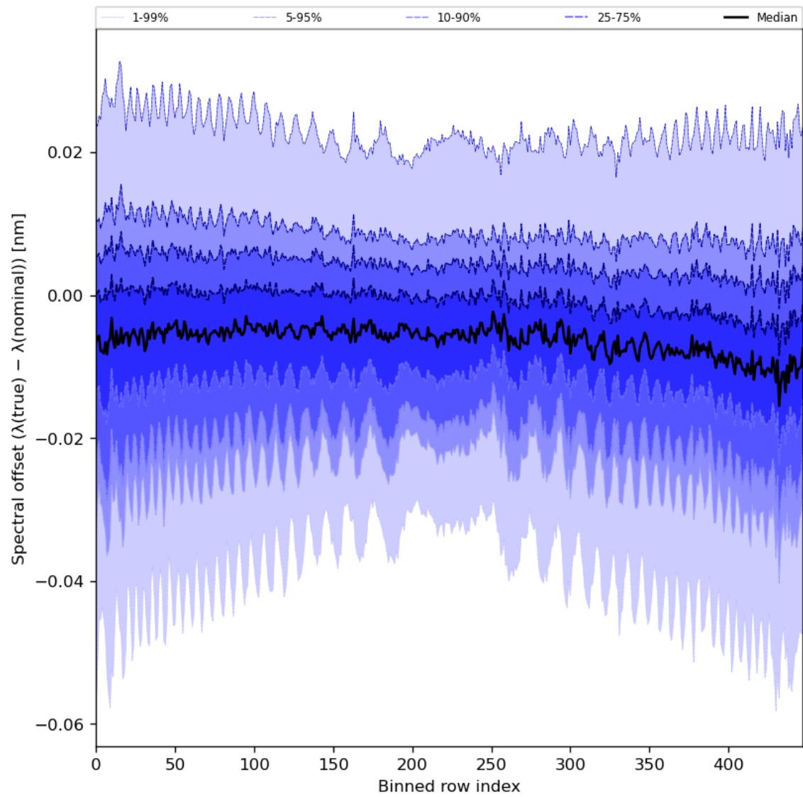
Figure 62: Along track statistics of “Spectral offset ( \lambda(\text{true}) - \lambda(\text{nominal}) )” for 2024-07-05 to 2024-07-07
