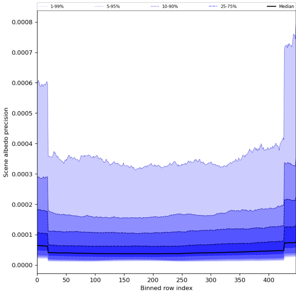
Figure 52: Along track statistics of “Scene albedo precision” for 2024-07-05 to 2024-07-07
