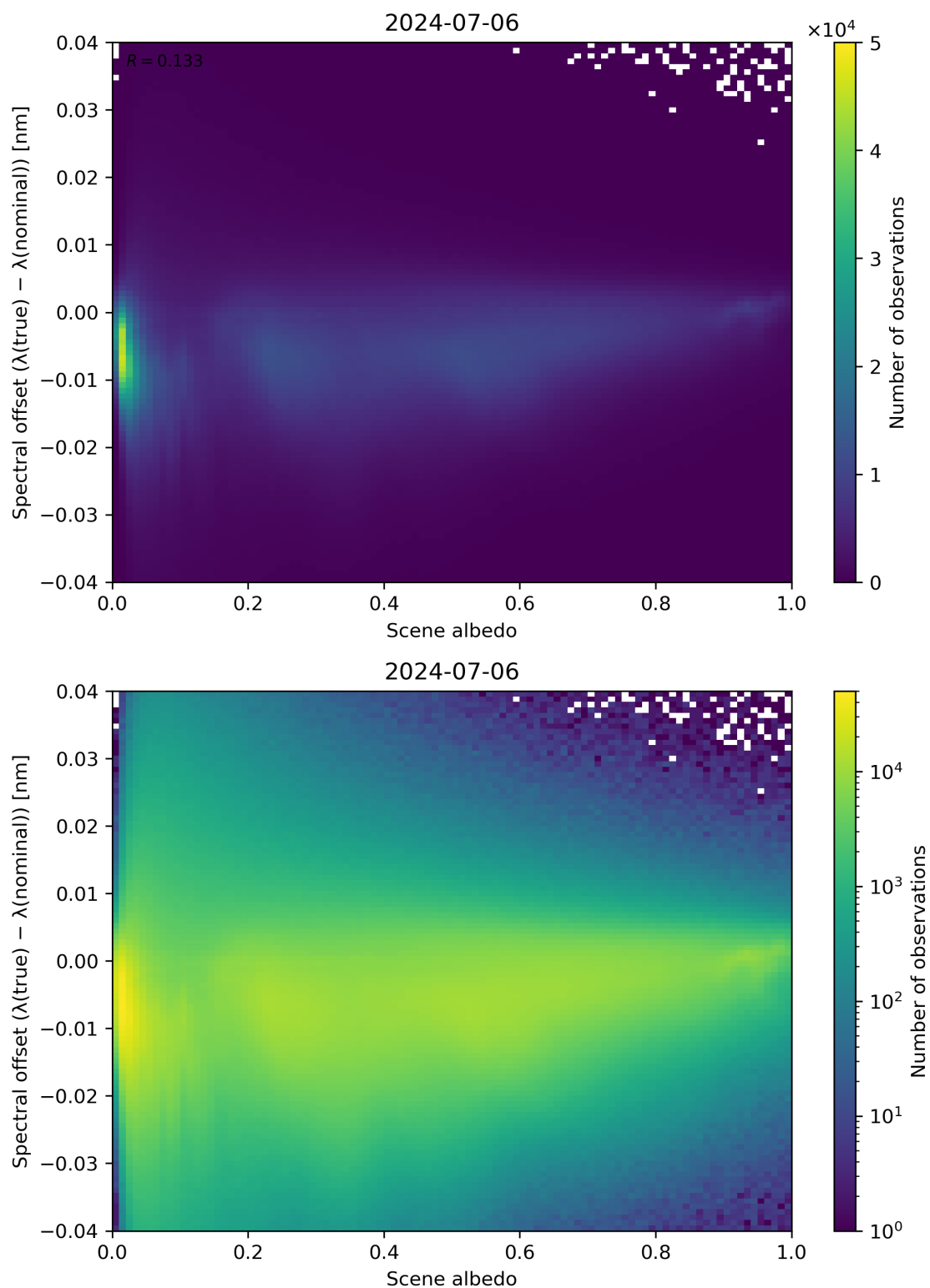
Figure 107: Scatter density plot of “Scene albedo” against “Spectral offset ( \lambda(\text{true}) - \lambda(\text{nominal}) )” for 2024-07-05 to 2024-07-07.
