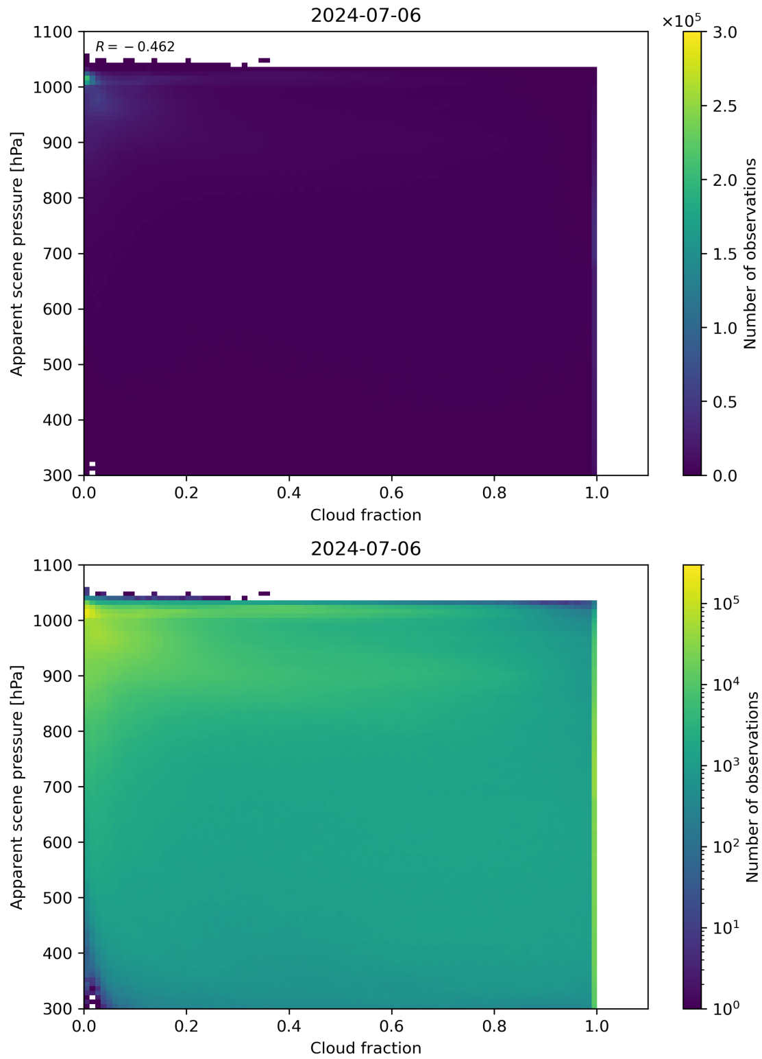
Figure 70: Scatter density plot of “Cloud fraction” against “Apparent scene pressure” for 2024-07-05 to 2024-07-07.
