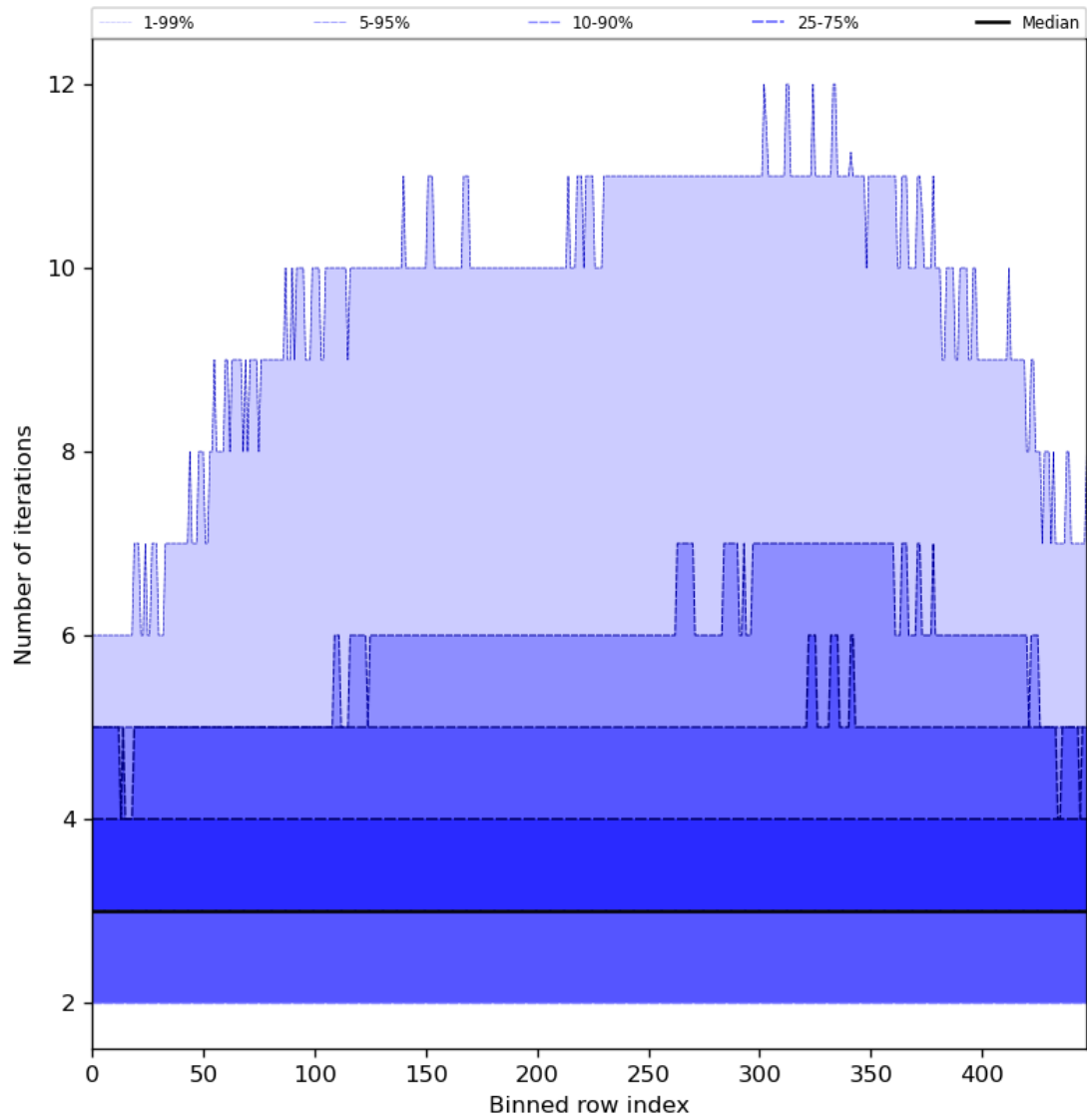
Figure 56: Along track statistics of “Number of iterations” for 2024-07-05 to 2024-07-07
