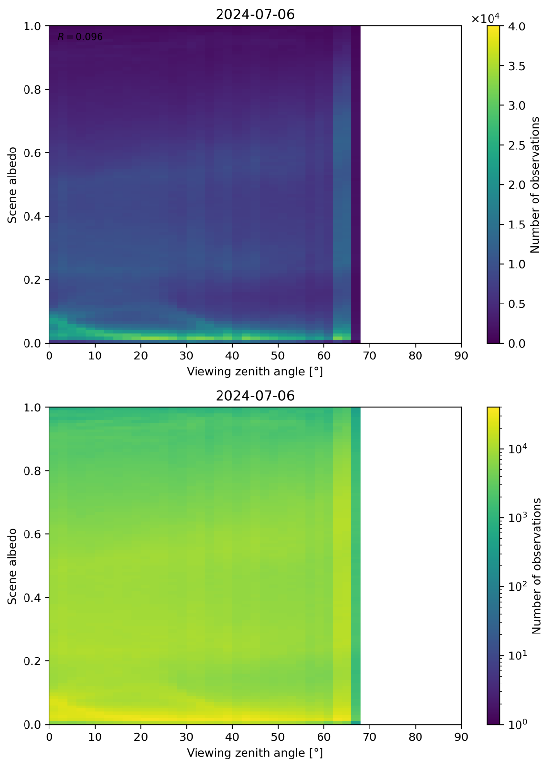
Figure 126: Scatter density plot of “Viewing zenith angle” against “Scene albedo” for 2024-07-05 to 2024-07-07.
