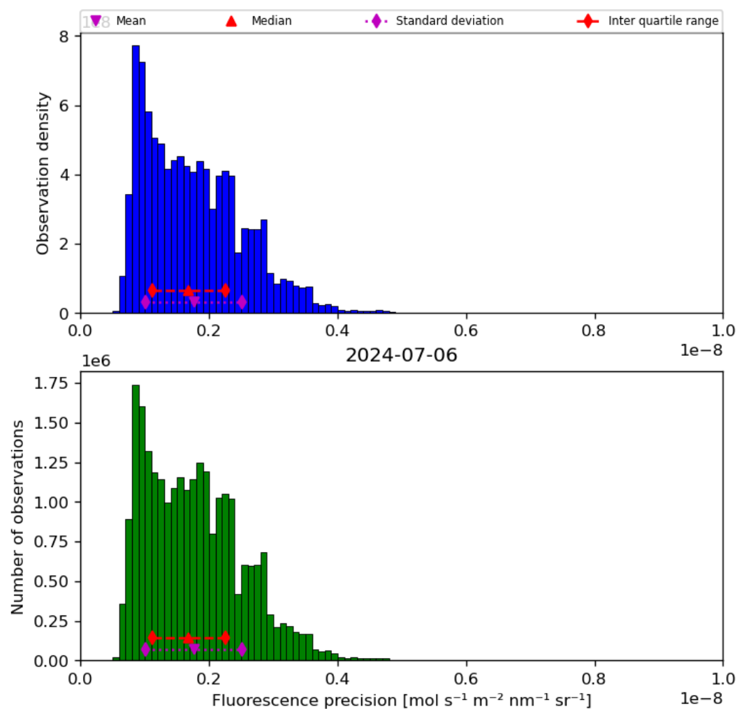
Figure 41: Histogram of “Fluorescence precision” for 2024-07-05 to 2024-07-07
