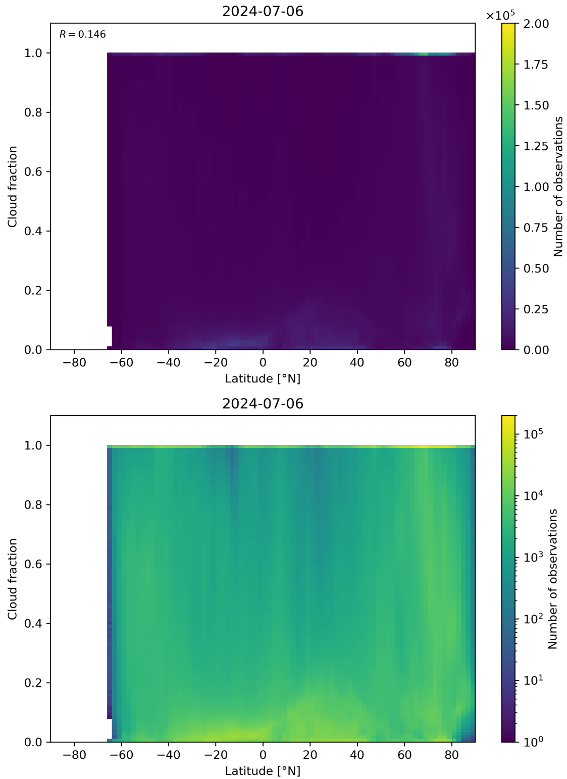
Figure 90: Scatter density plot of “Latitude” against “Cloud fraction” for 2024-07-05 to 2024-07-07.
