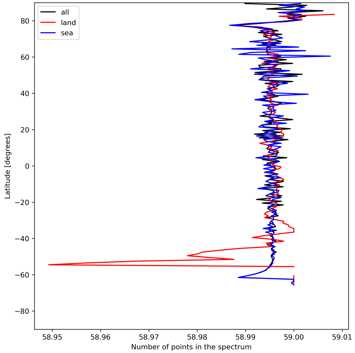
Figure 27: Zonal average of “Number of points in the spectrum” for 2024-07-05 to 2024-07-07.
