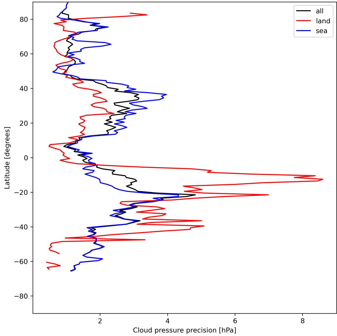
Figure 14: Zonal average of “Cloud pressure precision” for 2024-07-05 to 2024-07-07.
