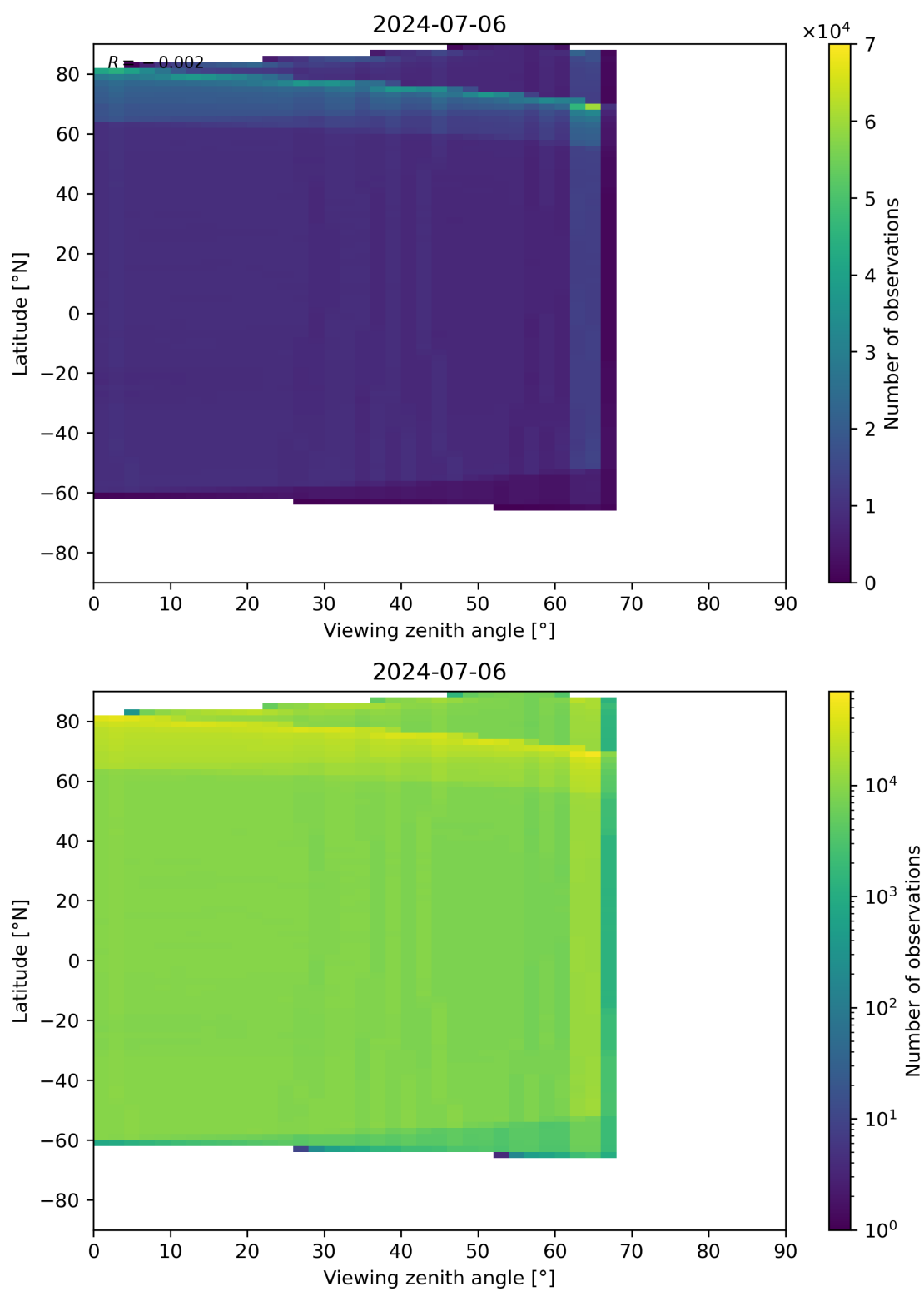
Figure 123: Scatter density plot of “Viewing zenith angle” against “Latitude” for 2024-07-05 to 2024-07-07.
