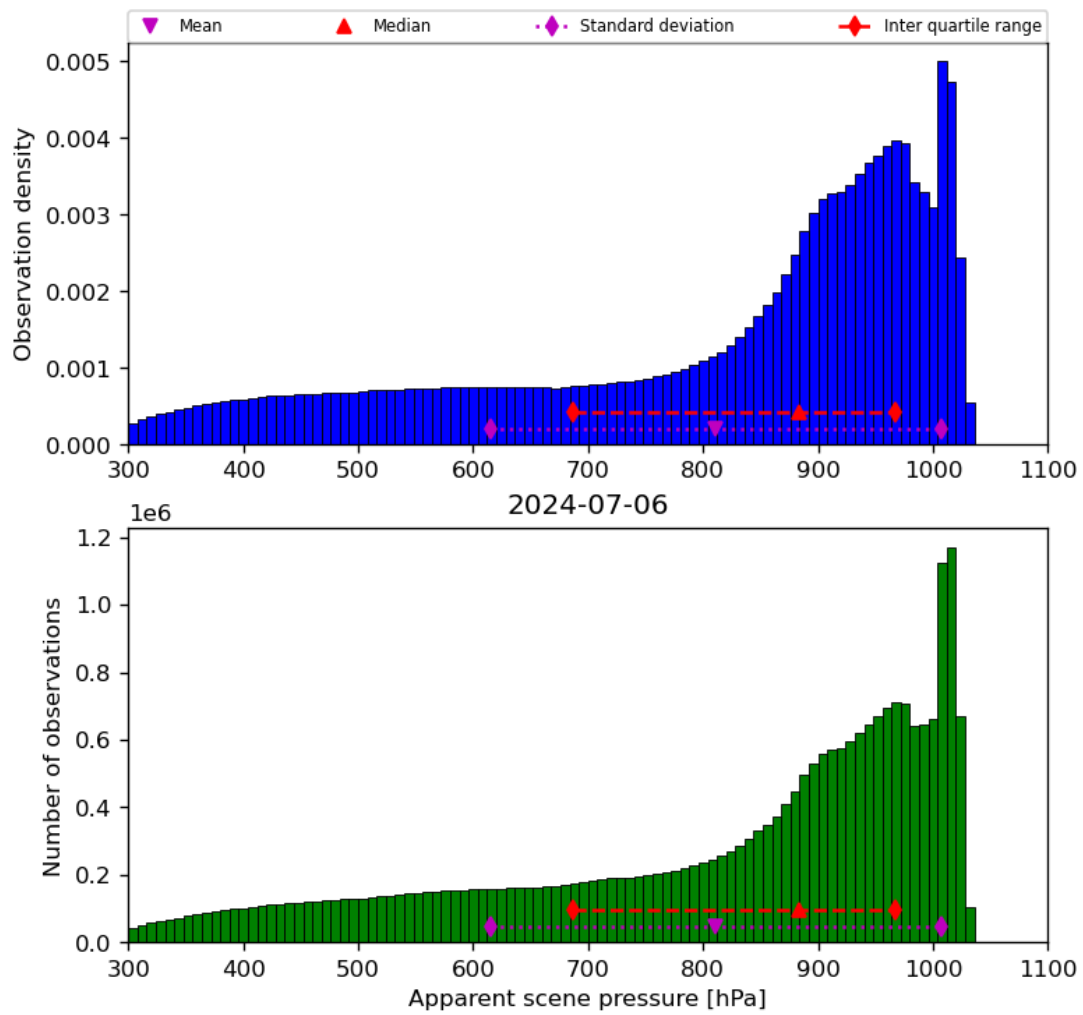
Figure 36: Histogram of “Apparent scene pressure” for 2024-07-05 to 2024-07-07
