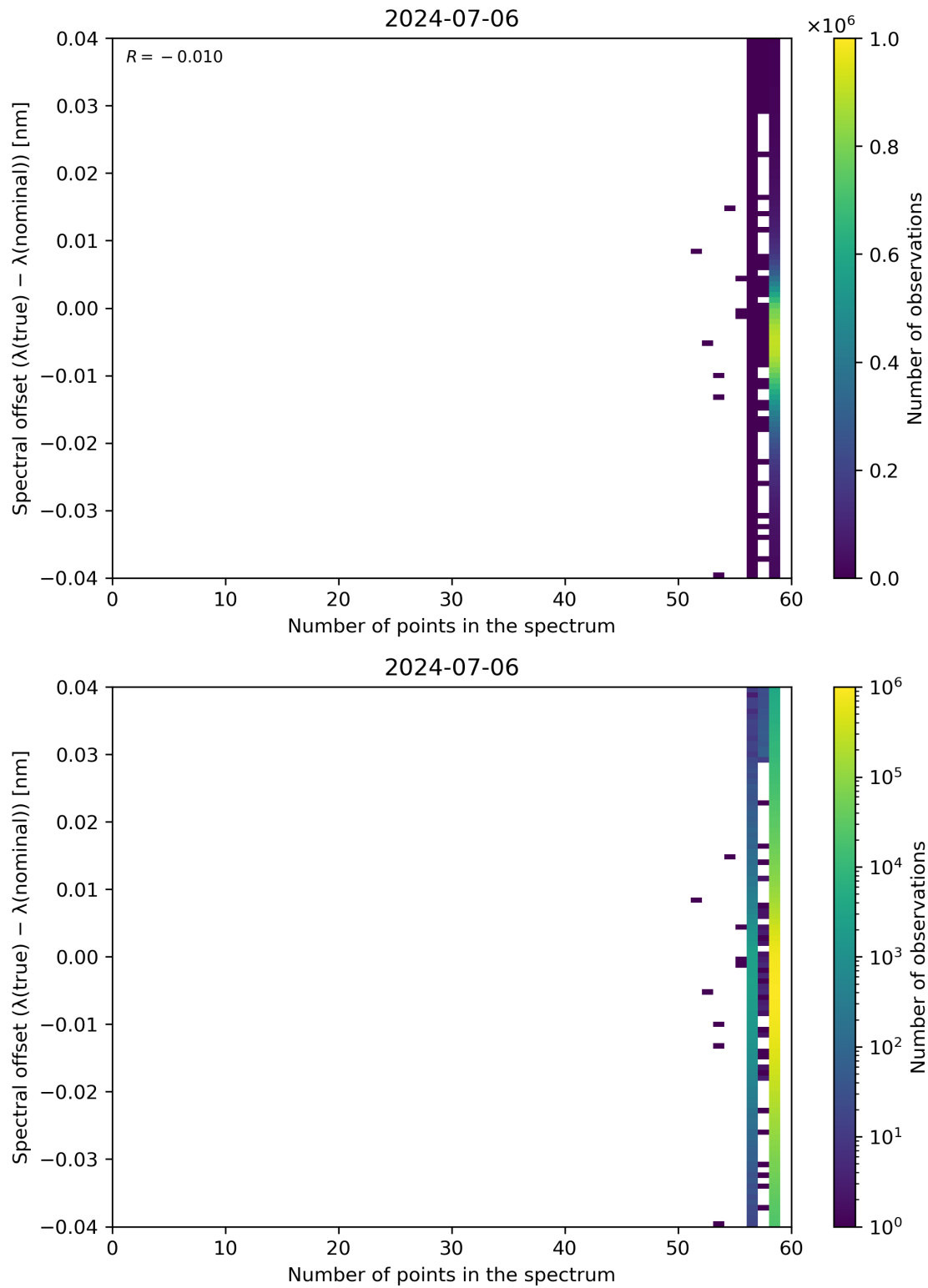
Figure 101: Scatter density plot of “Number of points in the spectrum” against “Spectral offset ( \lambda(\text{true}) - \lambda(\text{nominal}) )” for 2024-07-05 to 2024-07-07.
