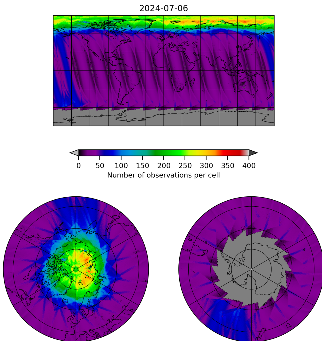
Figure 11: Map of the number of observations for 2024-07-05 to 2024-07-07
