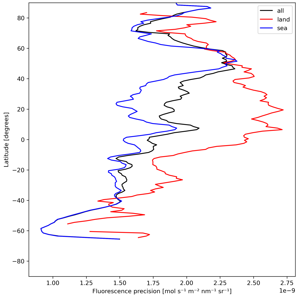
Figure 24: Zonal average of “Fluorescence precision” for 2024-07-05 to 2024-07-07.
