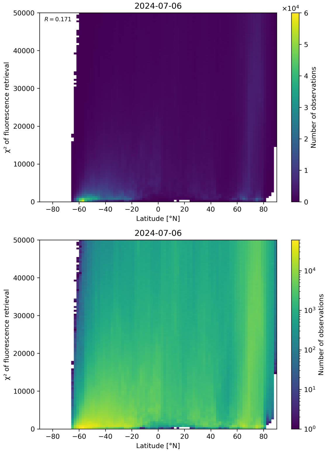
Figure 89: Scatter density plot of “Latitude” against “ \chi^2 of fluorescence retrieval” for 2024-07-05 to 2024-07-07.
