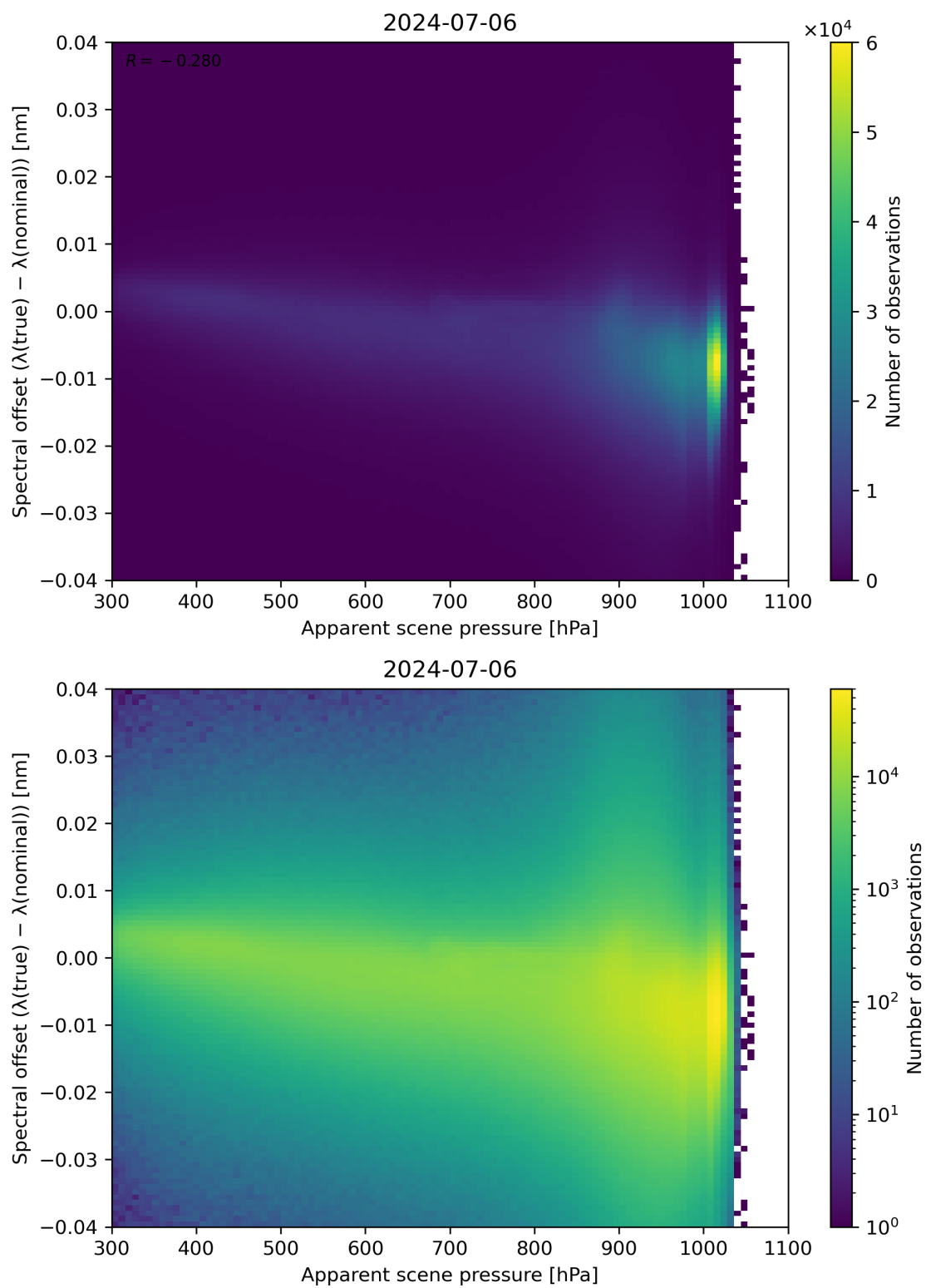
Figure 67: Scatter density plot of “Apparent scene pressure” against “Spectral offset ( \lambda(\text{true}) - \lambda(\text{nominal}) )” for 2024-07-05 to 2024-07-07.
