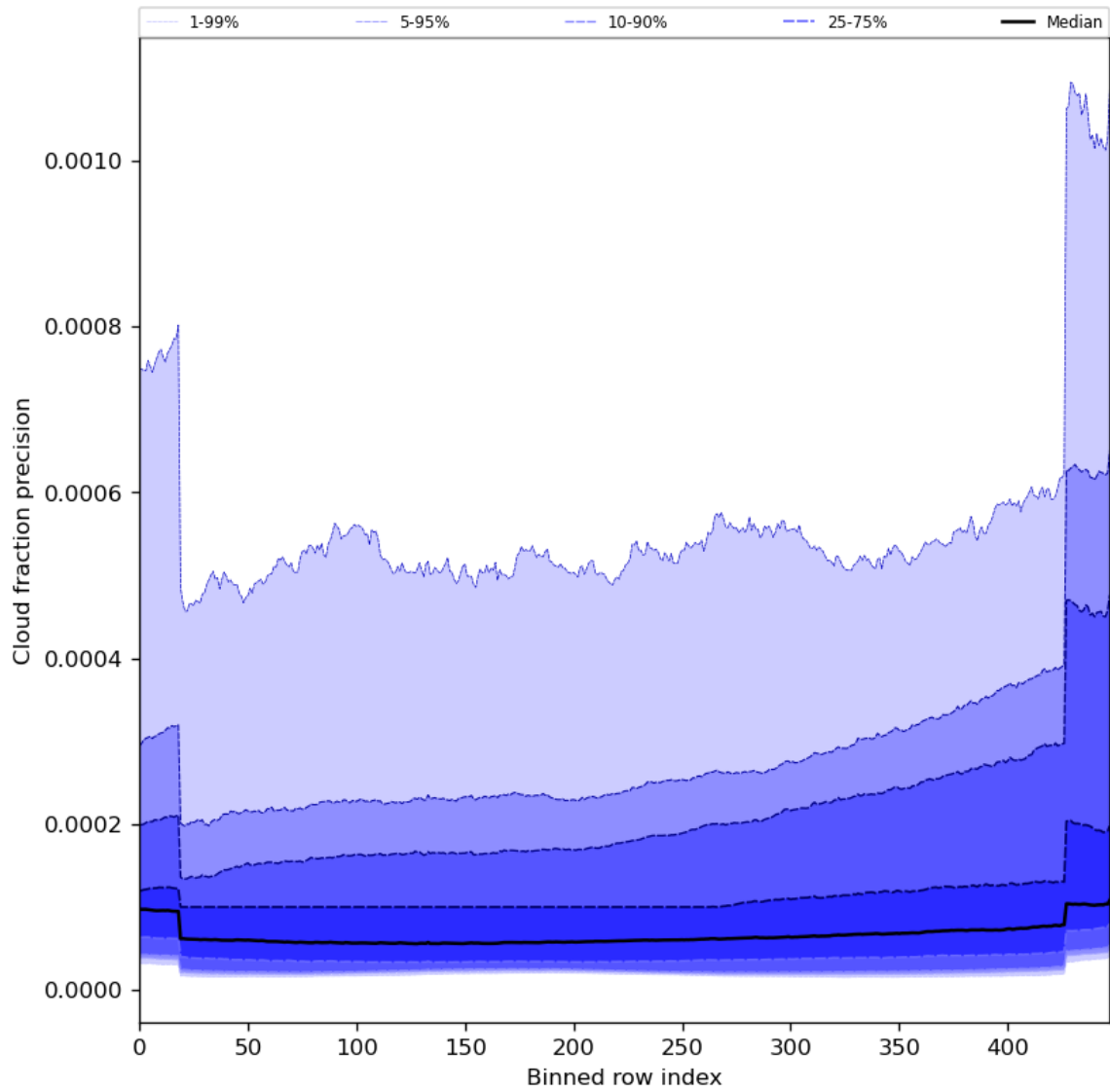
Figure 50: Along track statistics of “Cloud fraction precision” for 2024-07-05 to 2024-07-07
