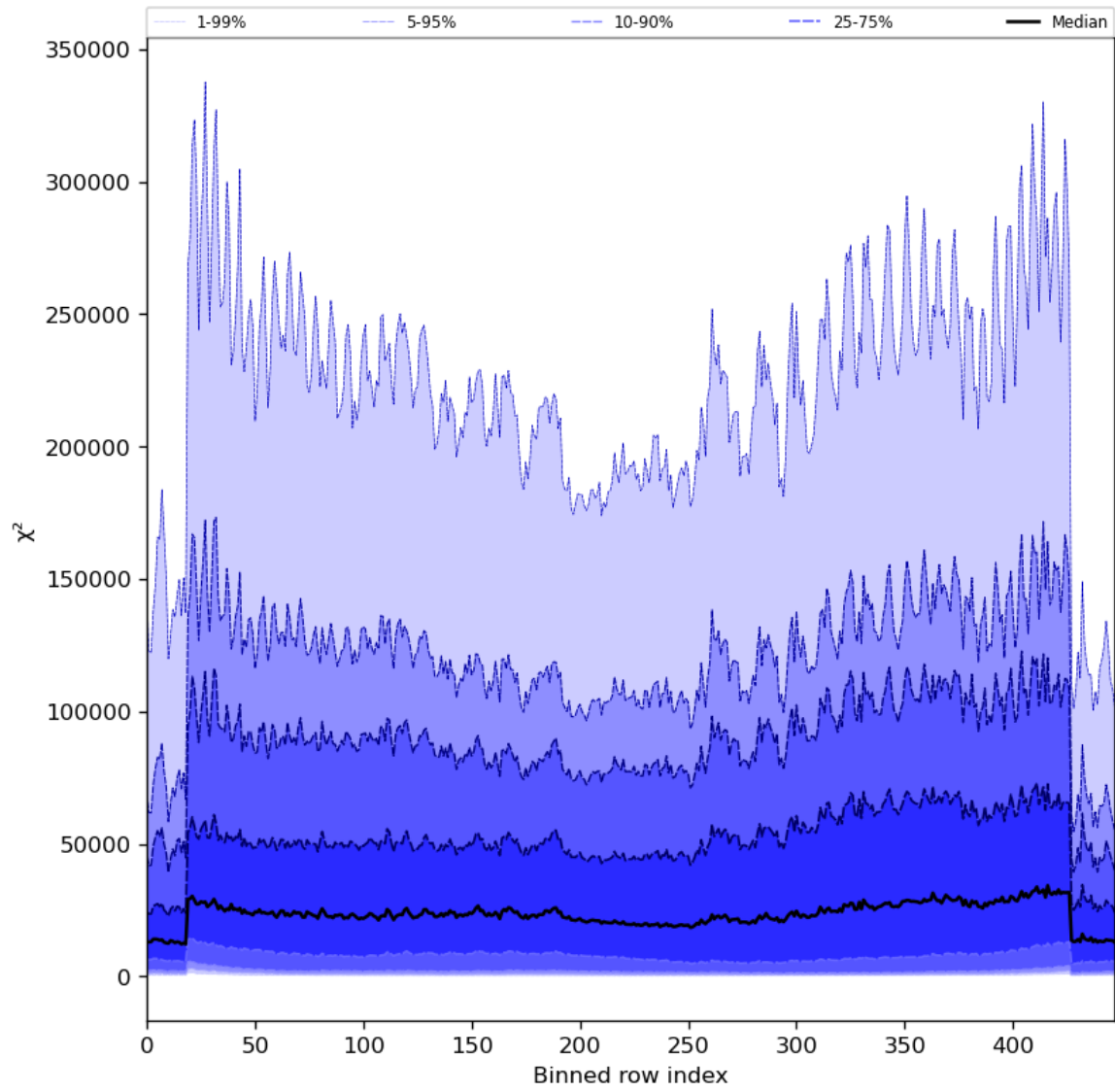
Figure 55: Along track statistics of “ \chi^2 ” for 2024-07-05 to 2024-07-07
