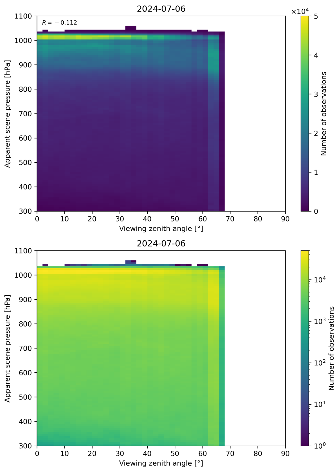
Figure 118: Scatter density plot of “Viewing zenith angle” against “Apparent scene pressure” for 2024-07-05 to 2024-07-07.
