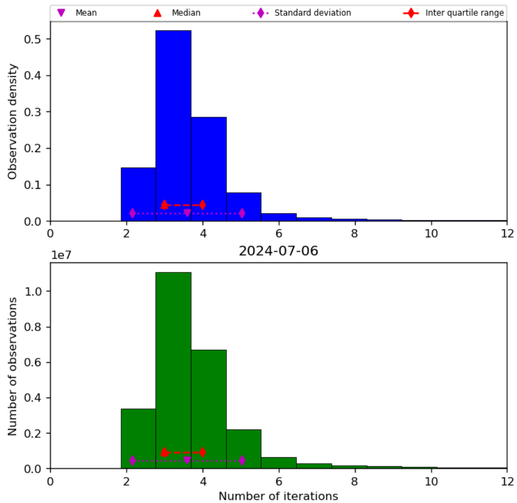
Figure 39: Histogram of “Number of iterations” for 2024-07-05 to 2024-07-07
