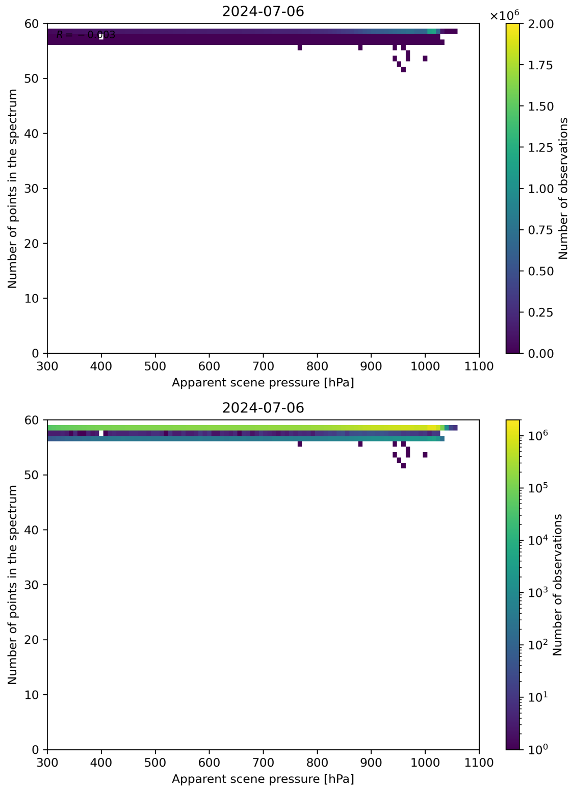
Figure 66: Scatter density plot of “Apparent scene pressure” against “Number of points in the spectrum” for 2024-07-05 to 2024-07-07.
