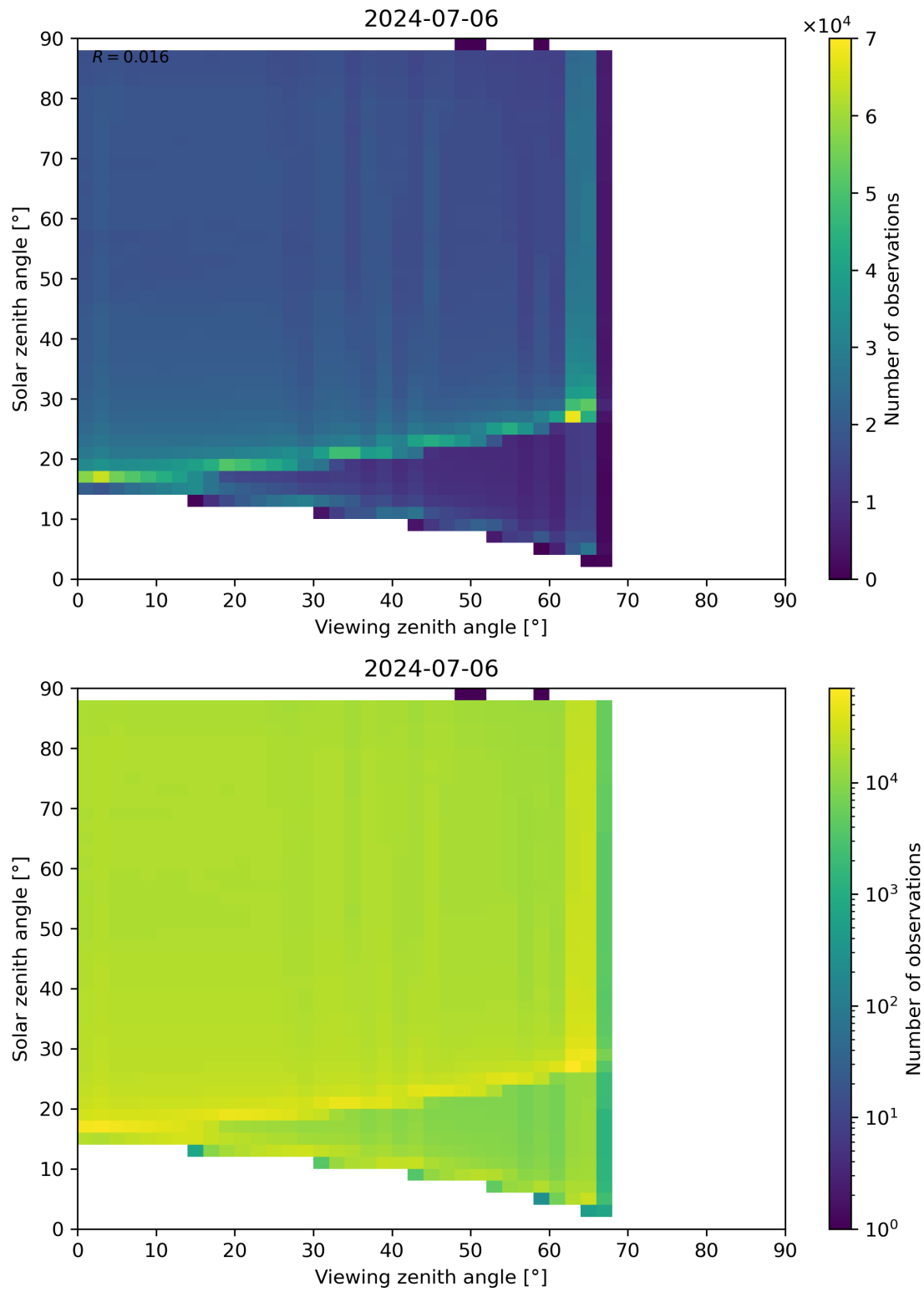
Figure 127: Scatter density plot of “Viewing zenith angle” against “Solar zenith angle” for 2024-07-05 to 2024-07-07.
