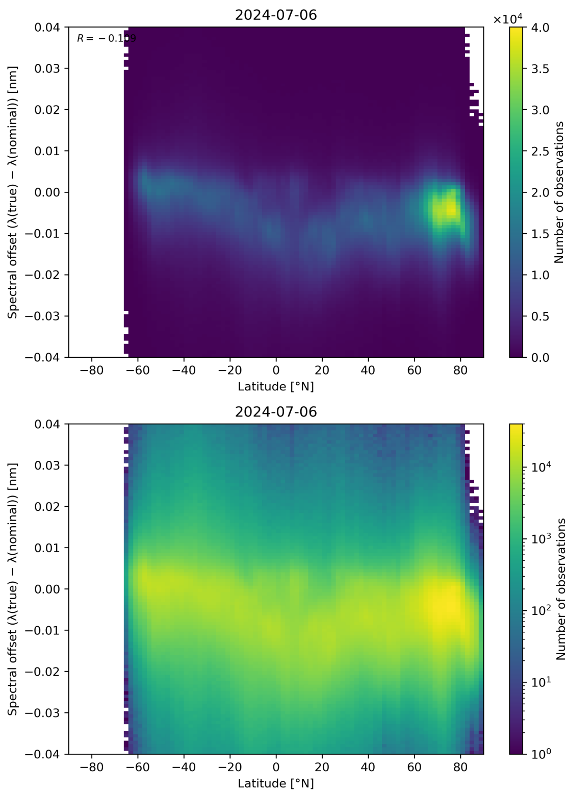
Figure 96: Scatter density plot of “Latitude” against “Spectral offset ( \lambda(\text{true}) - \lambda(\text{nominal}) )” for 2024-07-05 to 2024-07-07.
