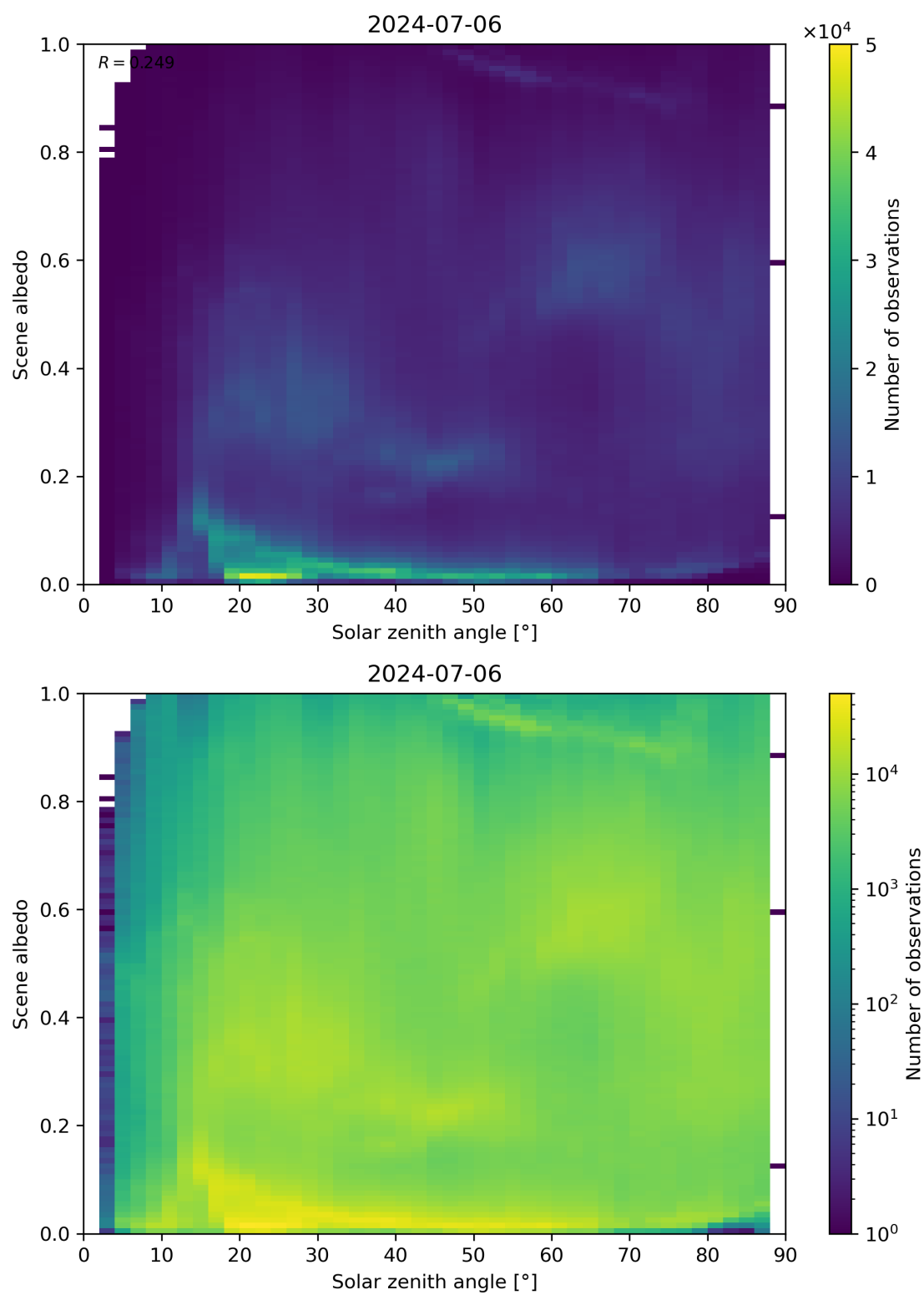
Figure 116: Scatter density plot of “Solar zenith angle” against “Scene albedo” for 2024-07-05 to 2024-07-07.
