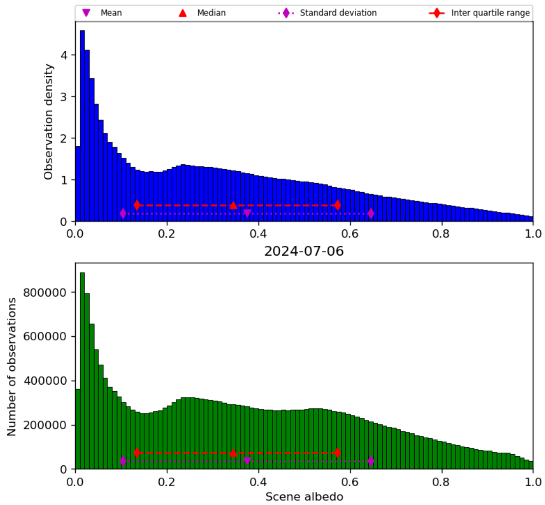
Figure 34: Histogram of “Scene albedo” for 2024-07-05 to 2024-07-07
