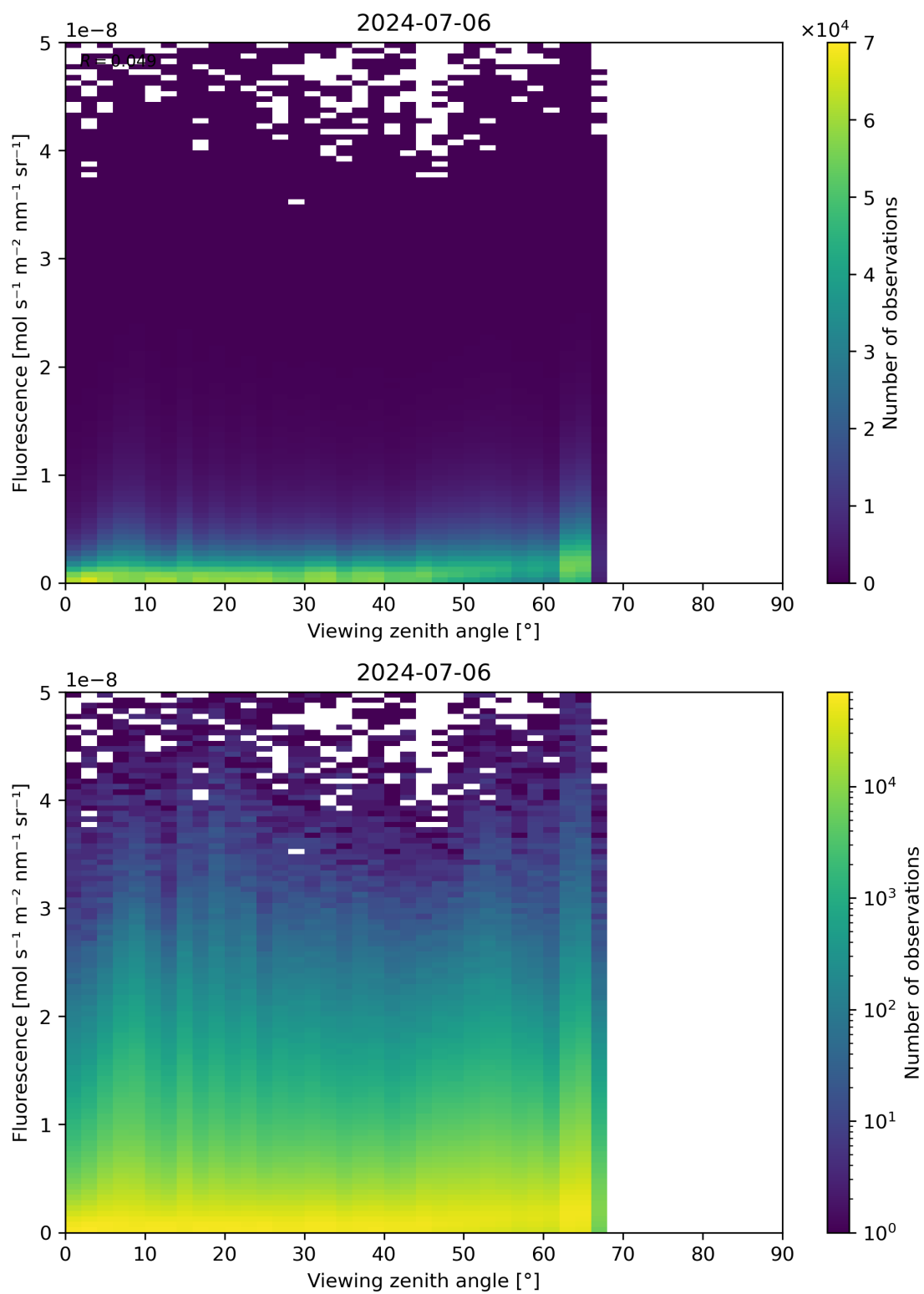
Figure 122: Scatter density plot of “Viewing zenith angle” against “Fluorescence” for 2024-07-05 to 2024-07-07.
