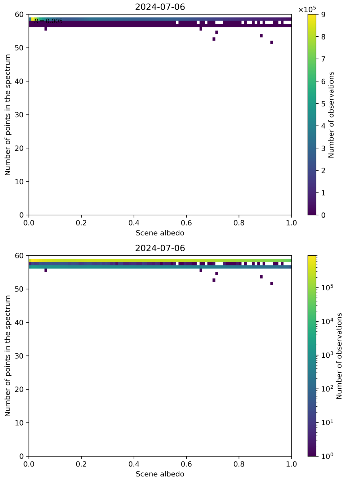
Figure 106: Scatter density plot of “Scene albedo” against “Number of points in the spectrum” for 2024-07-05 to 2024-07-07.
