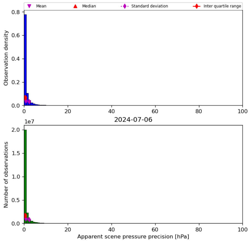
Figure 37: Histogram of "Apparent scene pressure precision" for 2024-07-05 to 2024-07-07
