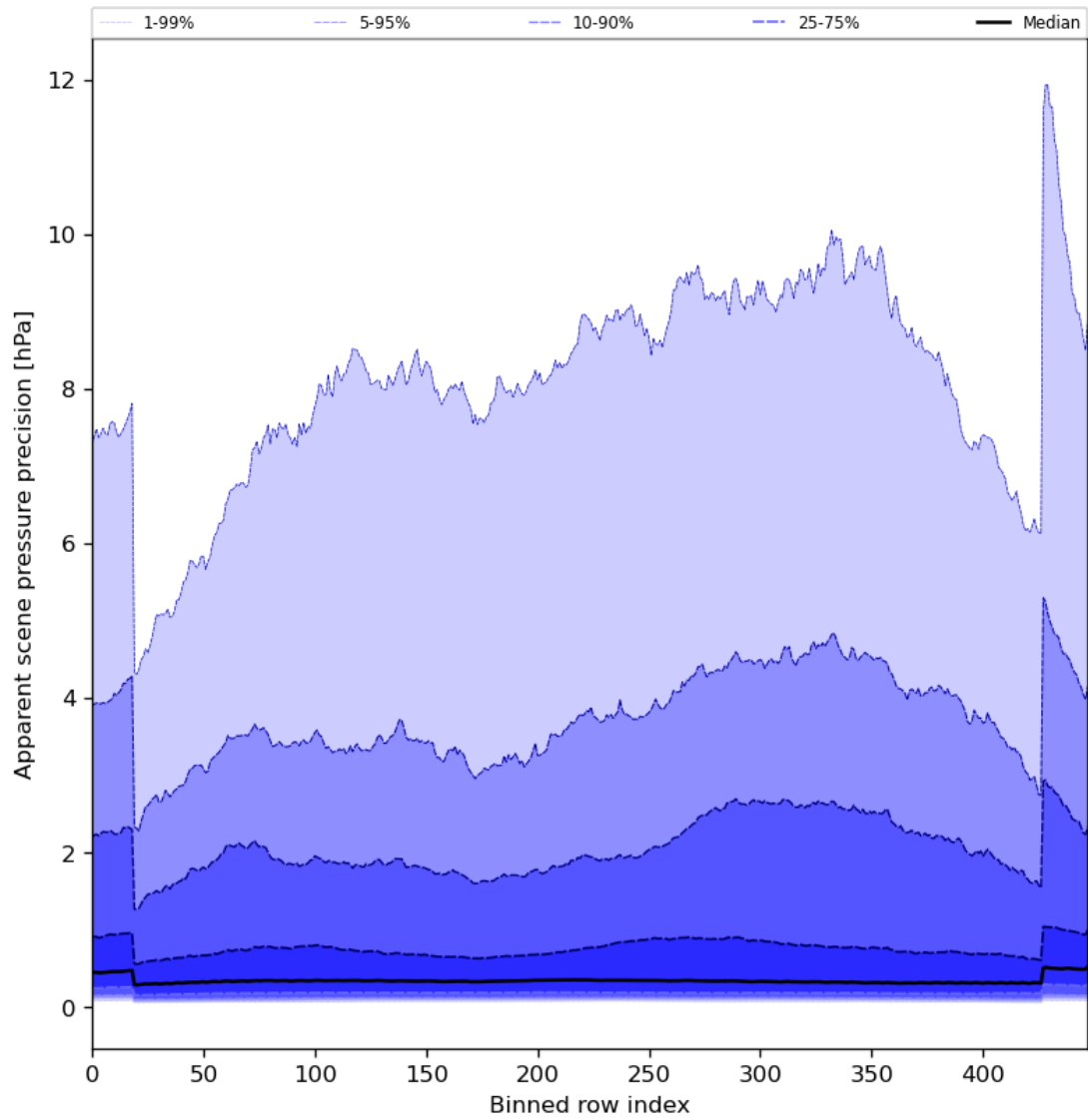
Figure 54: Along track statistics of “Apparent scene pressure precision” for 2024-07-05 to 2024-07-07
