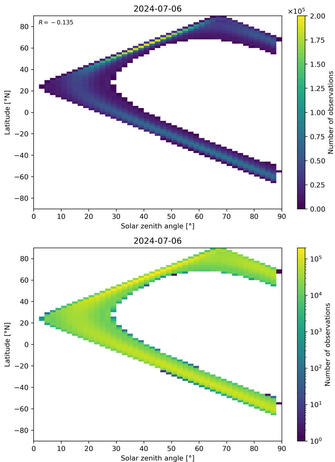
Figure 113: Scatter density plot of “Solar zenith angle” against “Latitude” for 2024-07-05 to 2024-07-07.
