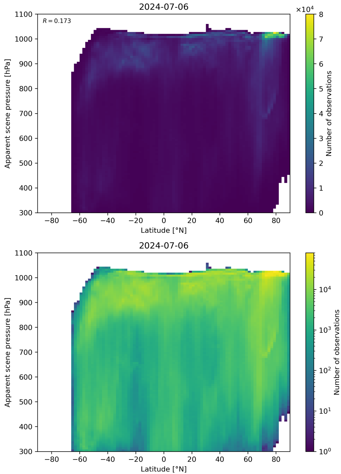
Figure 88: Scatter density plot of “Latitude” against “Apparent scene pressure” for 2024-07-05 to 2024-07-07.
