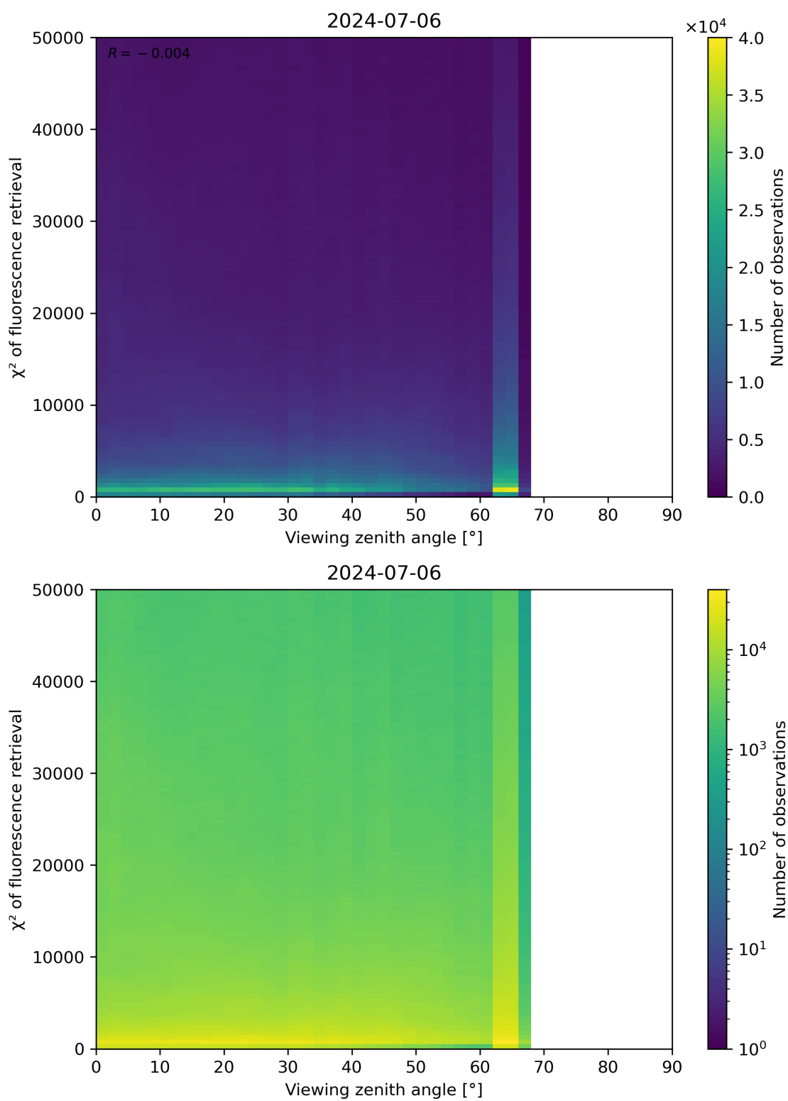
Figure 119: Scatter density plot of “Viewing zenith angle” against “ \chi^2 of fluorescence retrieval” for 2024-07-05 to 2024-07-07.
