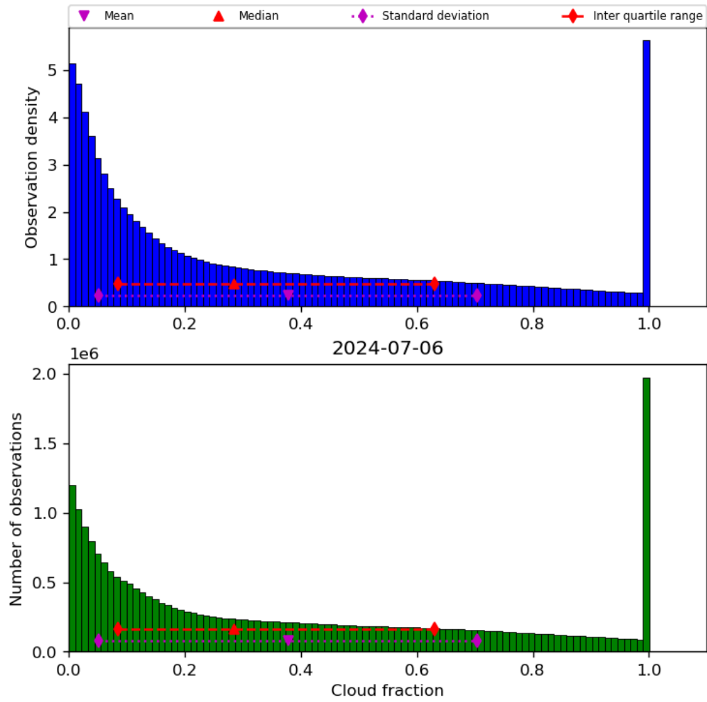
Figure 32: Histogram of “Cloud fraction” for 2024-07-05 to 2024-07-07
