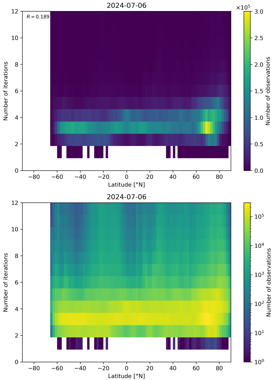
Figure 93: Scatter density plot of “Latitude” against “Number of iterations” for 2024-07-05 to 2024-07-07.
