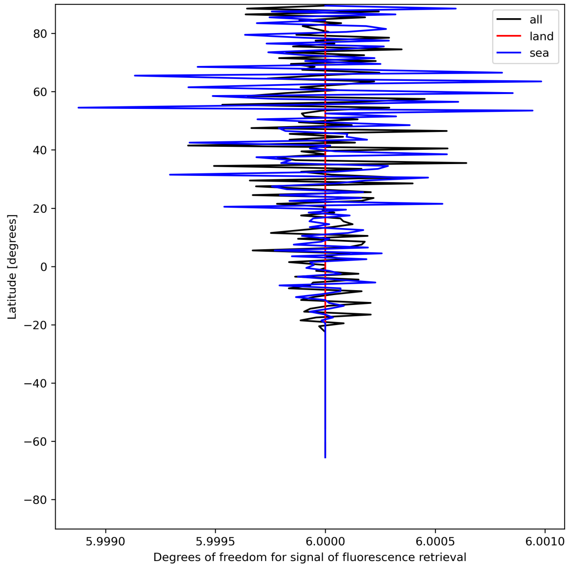
Figure 26: Zonal average of “Degrees of freedom for signal of fluorescence retrieval” for 2024-07-05 to 2024-07-07.
