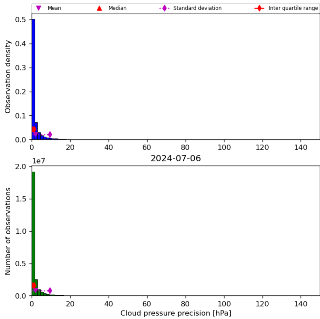
Figure 31: Histogram of “Cloud pressure precision” for 2024-07-05 to 2024-07-07
