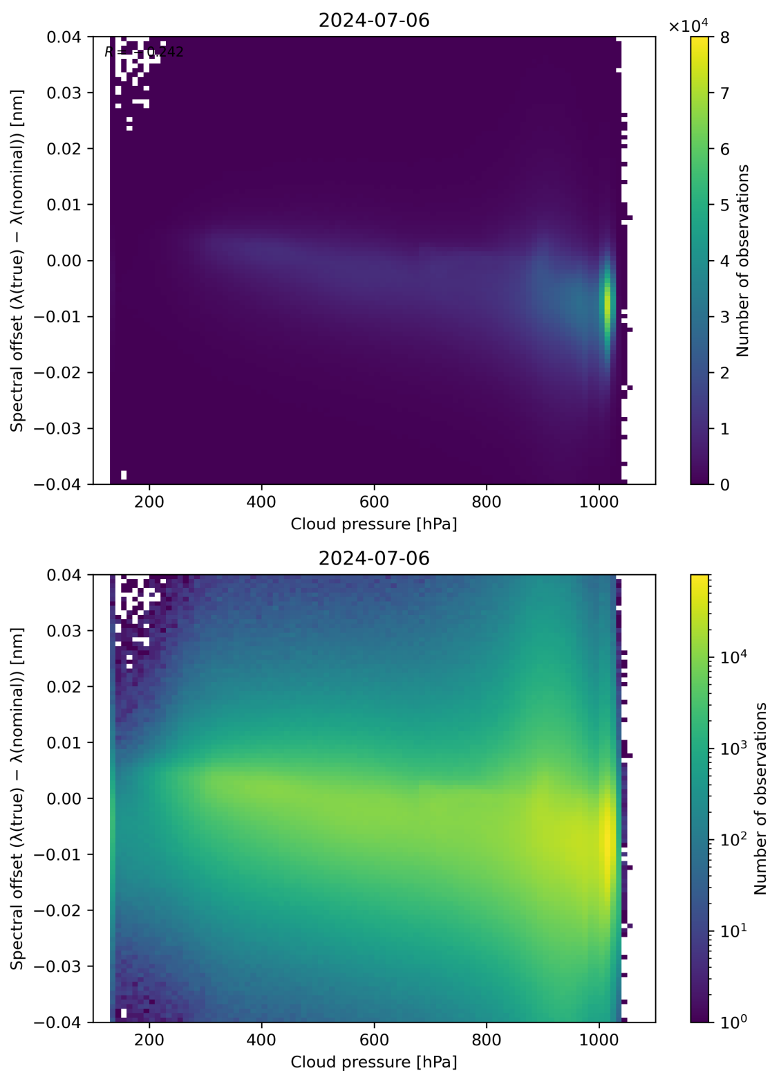
Figure 84: Scatter density plot of “Cloud pressure” against “Spectral offset ( \lambda(\text{true}) - \lambda(\text{nominal}) )” for 2024-07-05 to 2024-07-07.
