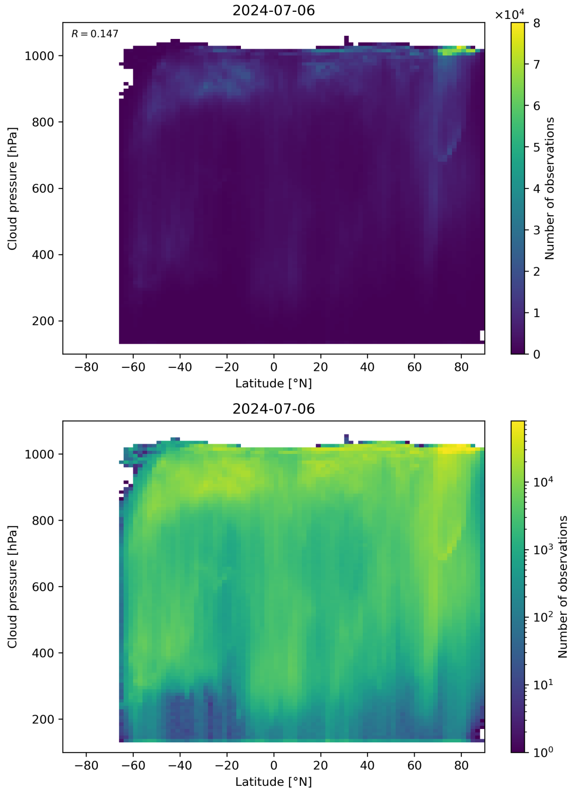
Figure 91: Scatter density plot of “Latitude” against “Cloud pressure” for 2024-07-05 to 2024-07-07.
