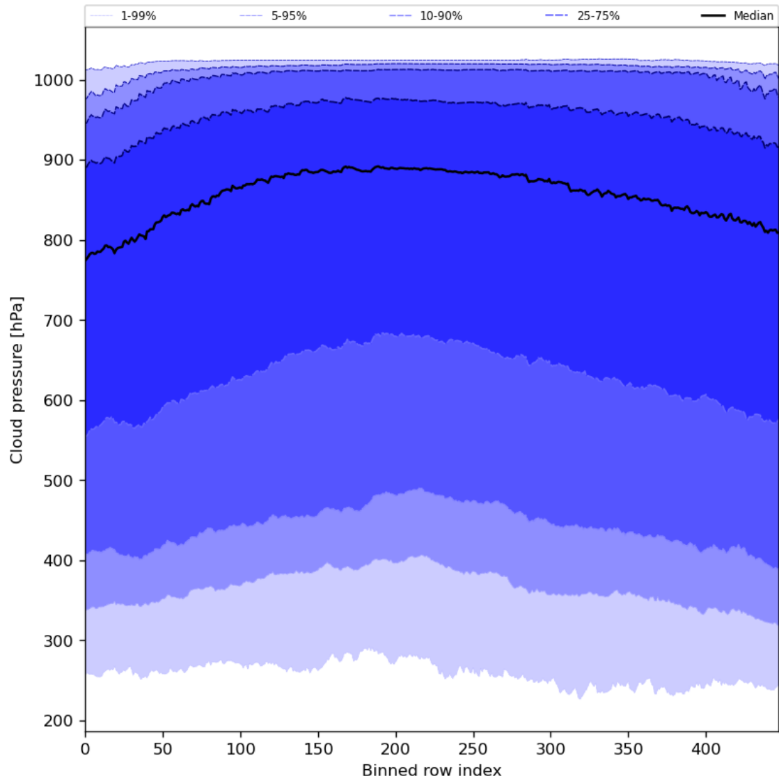
Figure 47: Along track statistics of “Cloud pressure” for 2024-07-05 to 2024-07-07
