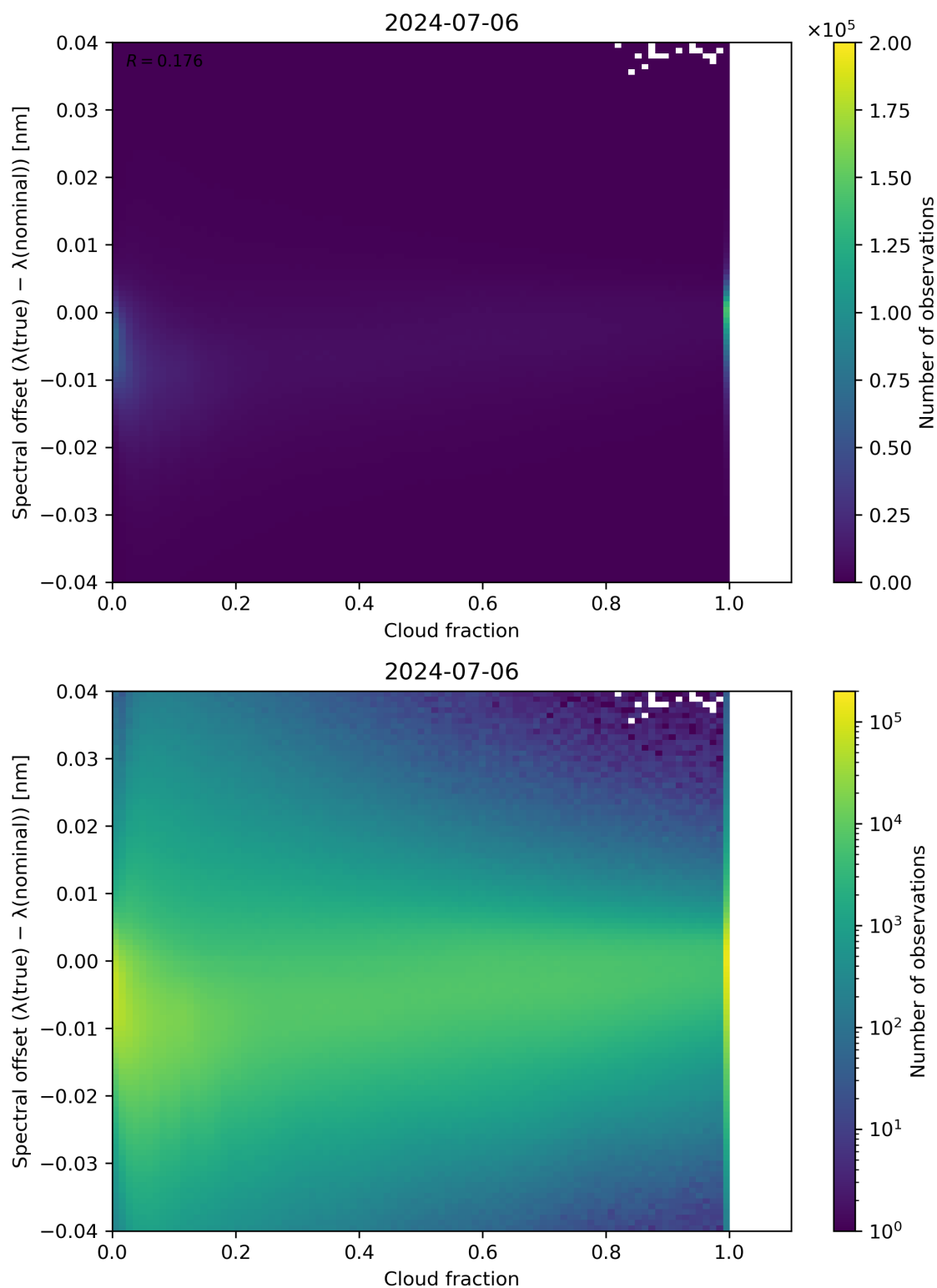
Figure 76: Scatter density plot of “Cloud fraction” against “Spectral offset ( \lambda(\text{true}) - \lambda(\text{nominal}) )” for 2024-07-05 to 2024-07-07.
