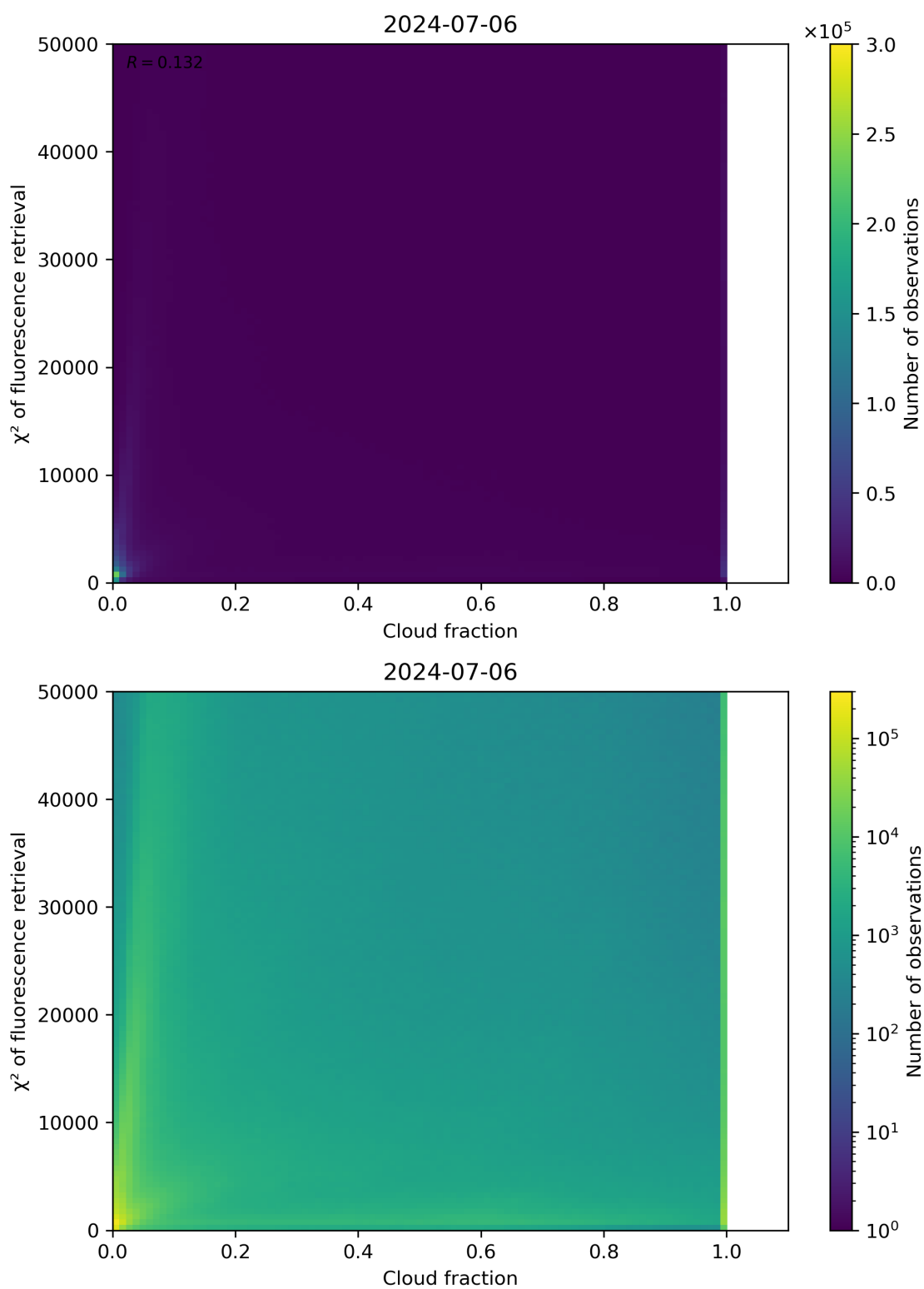
Figure 71: Scatter density plot of “Cloud fraction” against “ \chi^2 of fluorescence retrieval” for 2024-07-05 to 2024-07-07.
