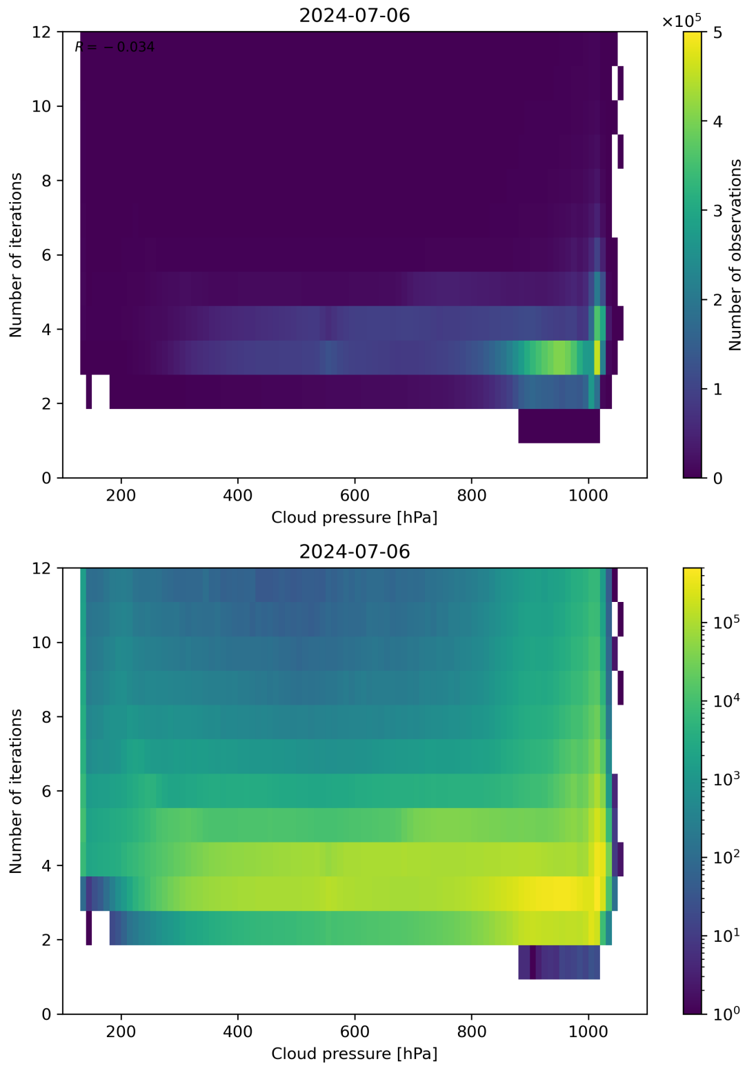
Figure 81: Scatter density plot of “Cloud pressure” against “Number of iterations” for 2024-07-05 to 2024-07-07.
