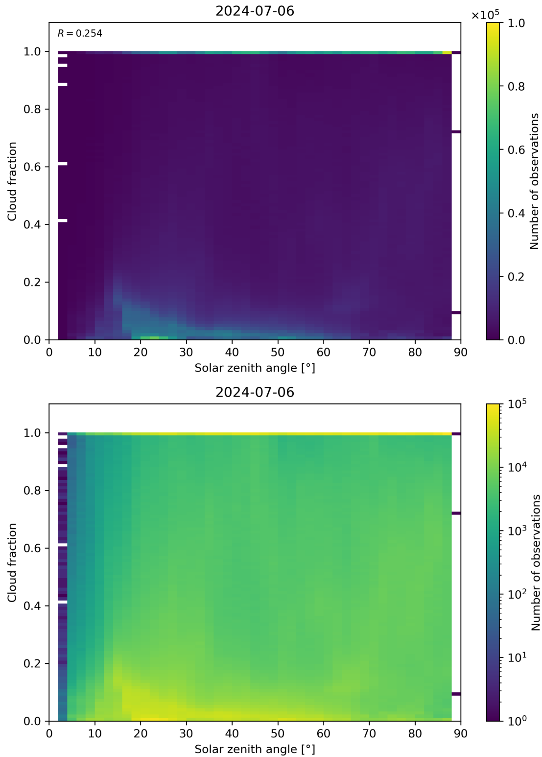
Figure 110: Scatter density plot of “Solar zenith angle” against “Cloud fraction” for 2024-07-05 to 2024-07-07.
