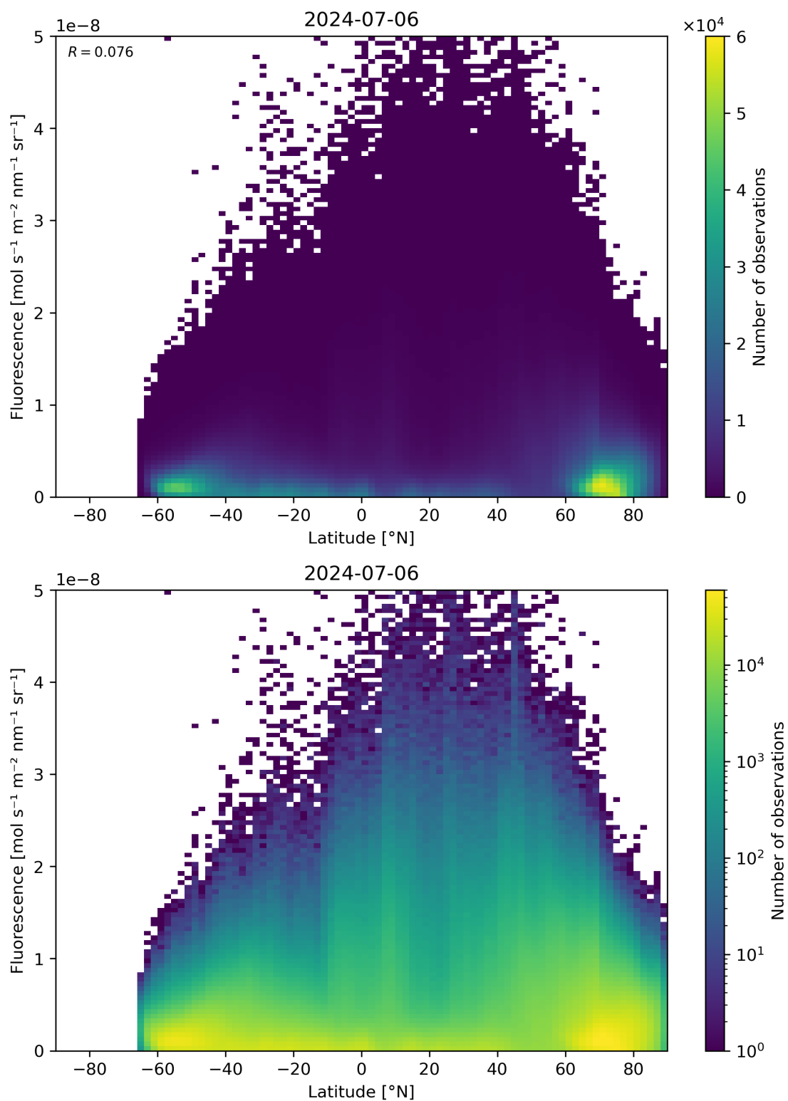
Figure 92: Scatter density plot of “Latitude” against “Fluorescence” for 2024-07-05 to 2024-07-07.
