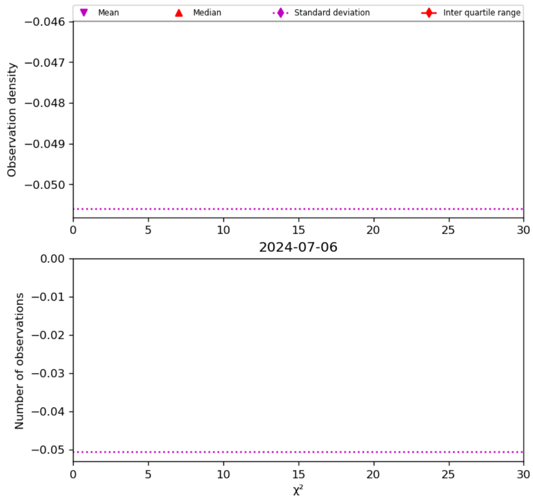
Figure 38: Histogram of “ \chi^2 ” for 2024-07-05 to 2024-07-07
