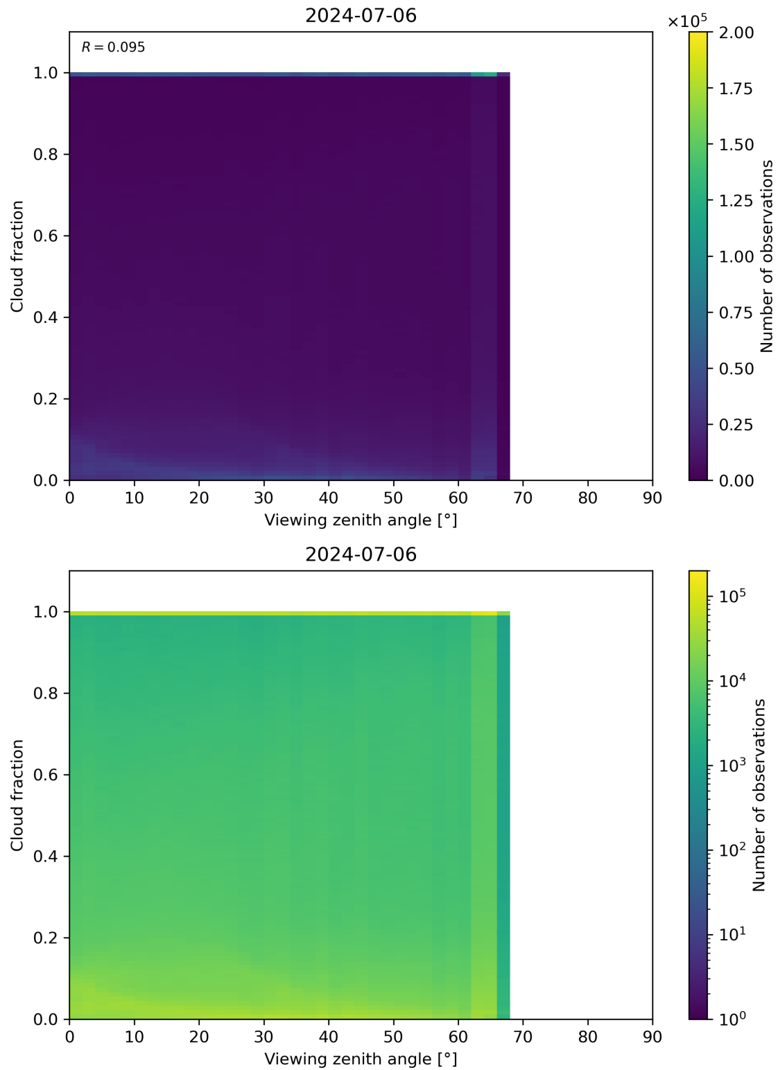
Figure 120: Scatter density plot of “Viewing zenith angle” against “Cloud fraction” for 2024-07-05 to 2024-07-07.
