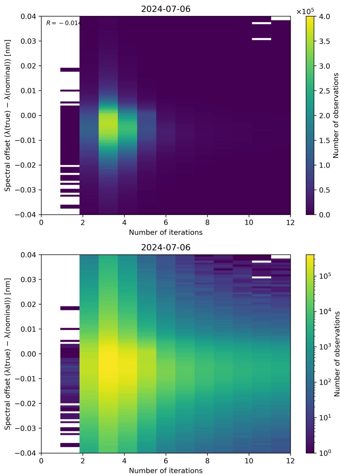
Figure 100: Scatter density plot of “Number of iterations” against “Spectral offset ( \lambda(\text{true}) - \lambda(\text{nominal}) )” for 2024-07-05 to 2024-07-07.
