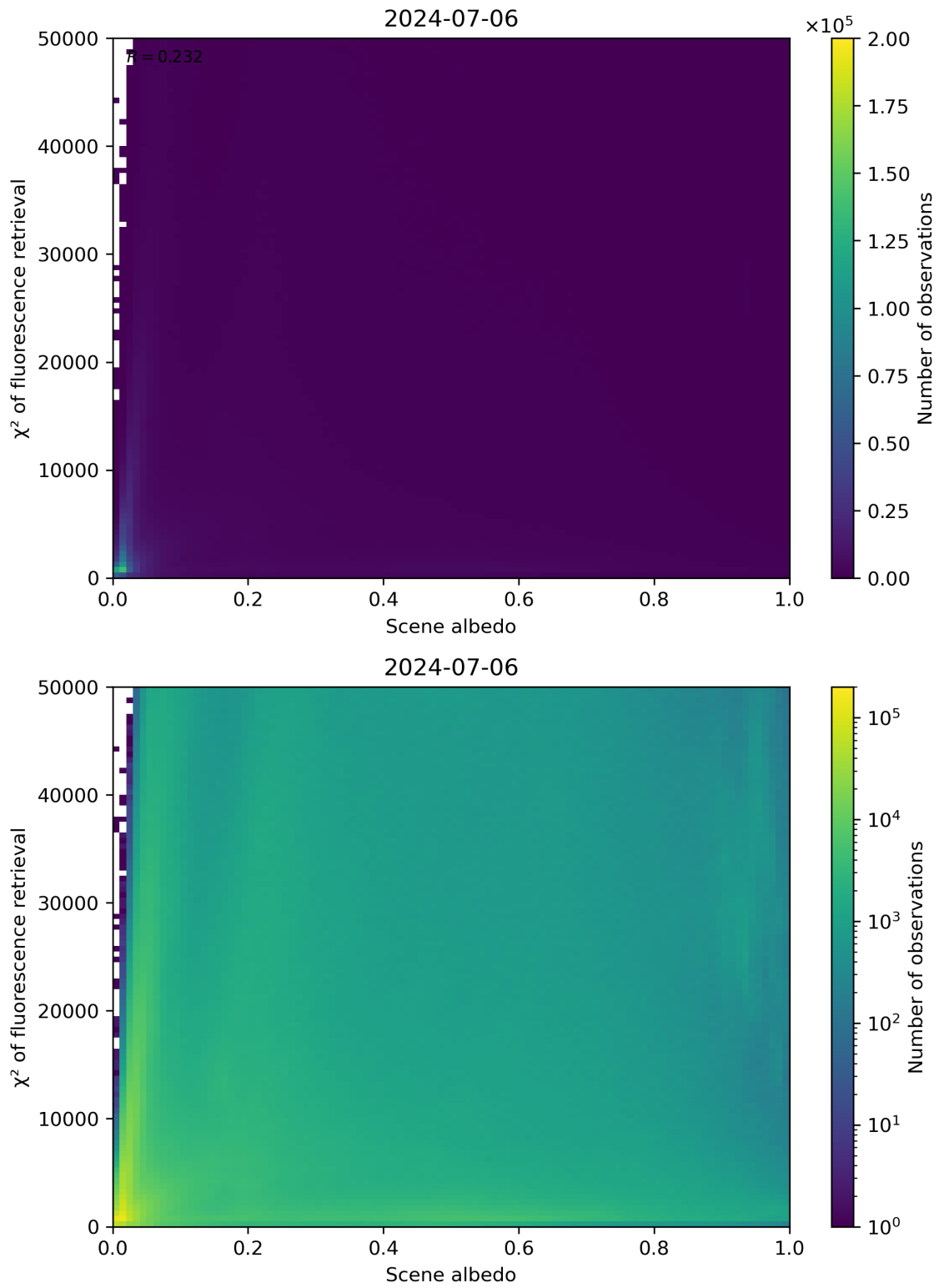
Figure 103: Scatter density plot of “Scene albedo” against “ \chi^2 of fluorescence retrieval” for 2024-07-05 to 2024-07-07.
