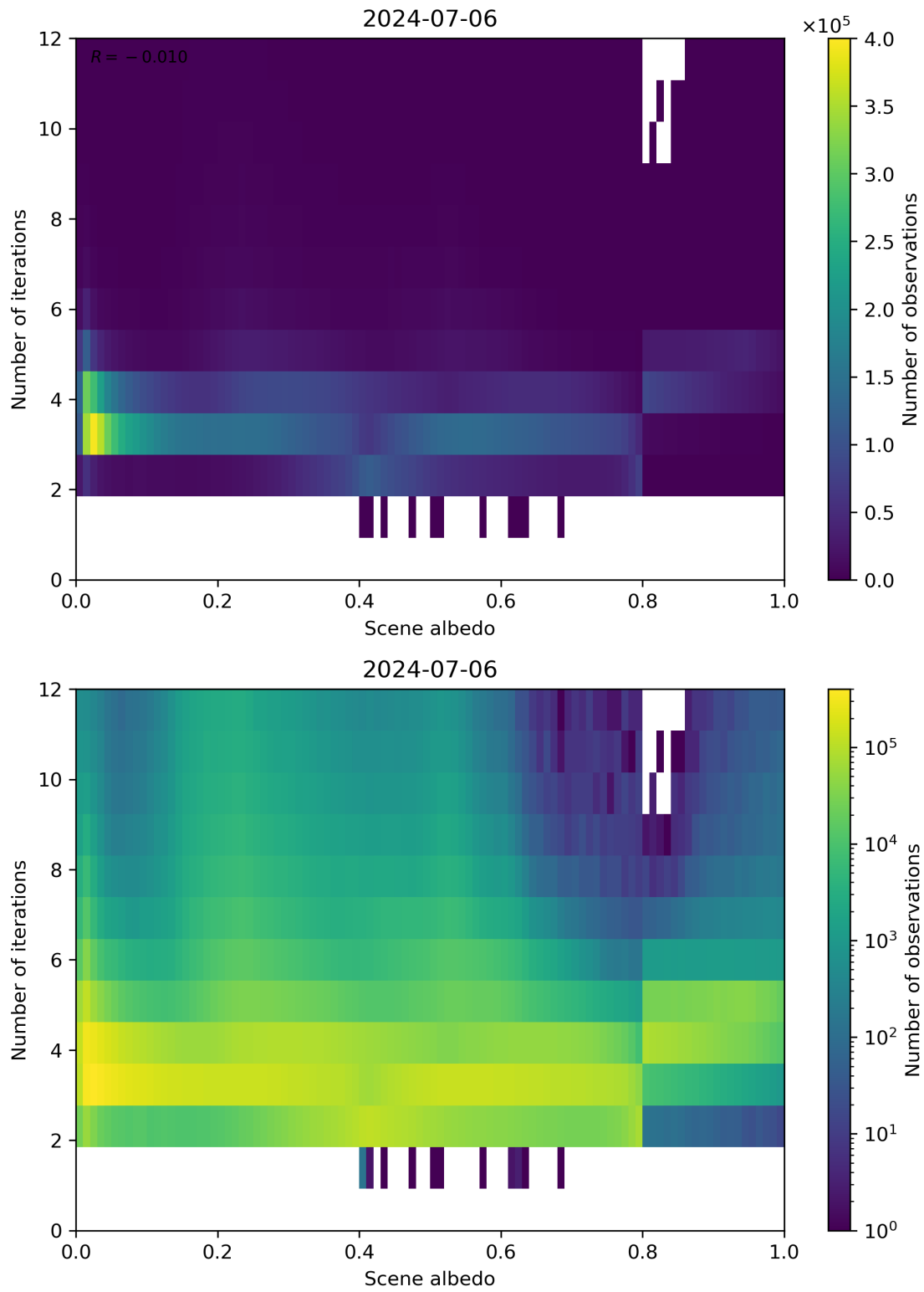
Figure 105: Scatter density plot of “Scene albedo” against “Number of iterations” for 2024-07-05 to 2024-07-07.
