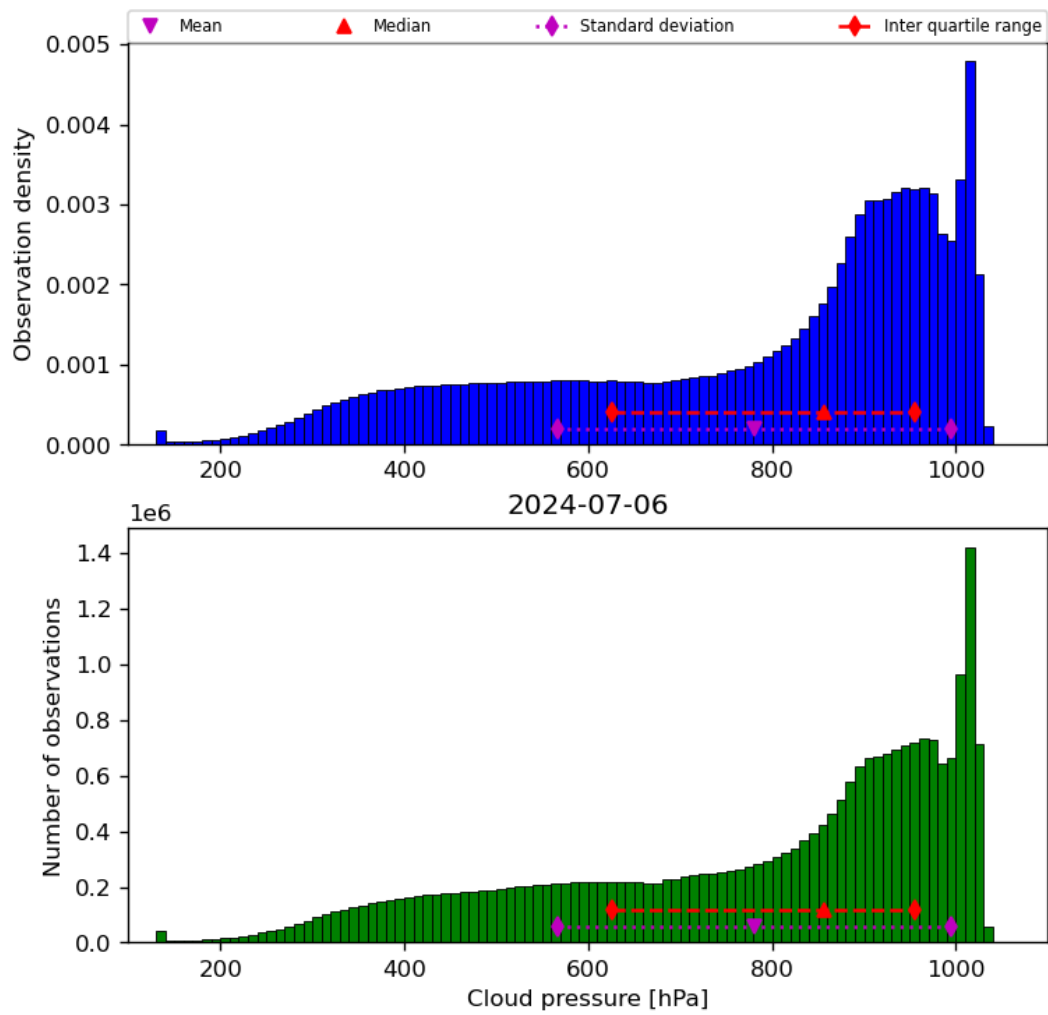
Figure 30: Histogram of “Cloud pressure” for 2024-07-05 to 2024-07-07
