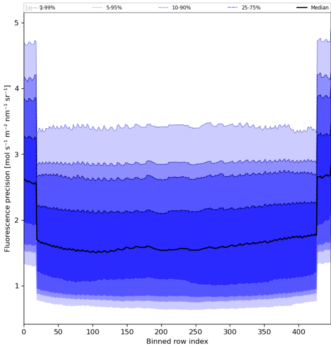
Figure 58: Along track statistics of “Fluorescence precision” for 2024-07-05 to 2024-07-07
