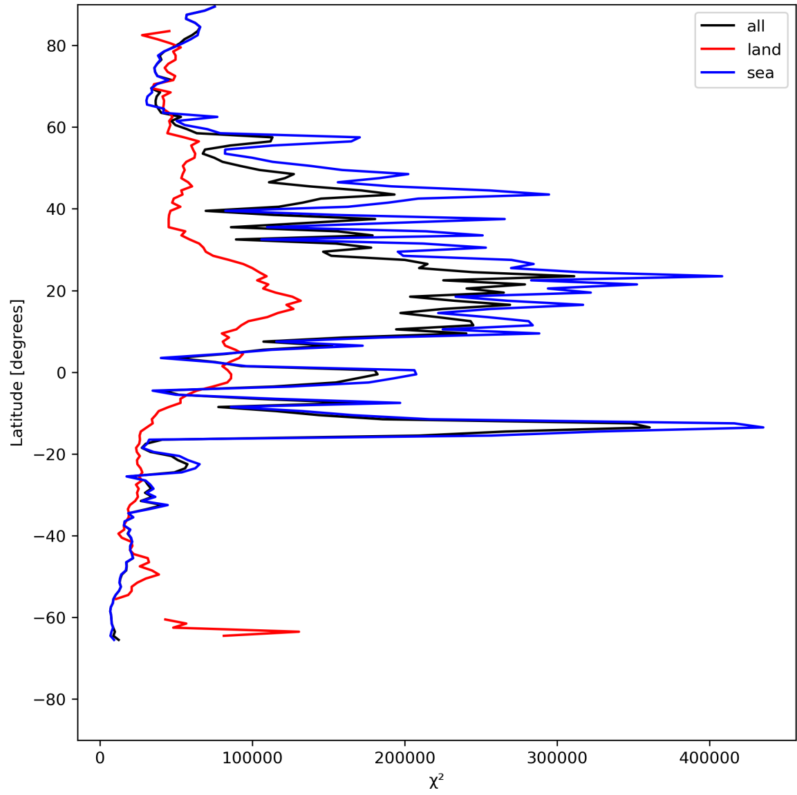
Figure 21: Zonal average of “ \chi^2 ” for 2024-07-05 to 2024-07-07.
