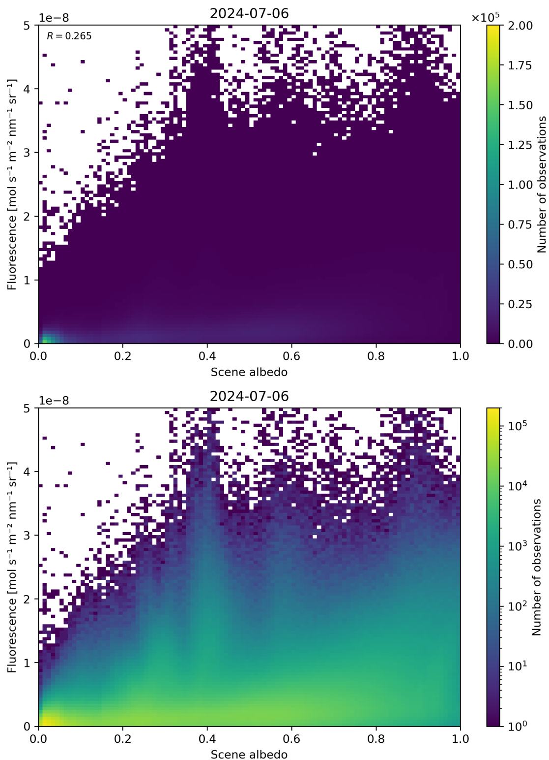
Figure 104: Scatter density plot of “Scene albedo” against “Fluorescence” for 2024-07-05 to 2024-07-07.
