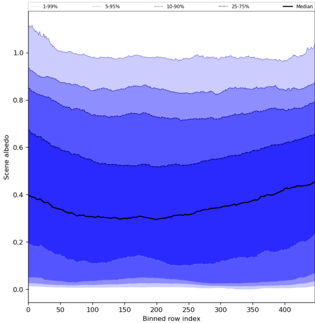
Figure 51: Along track statistics of “Scene albedo” for 2024-07-05 to 2024-07-07
