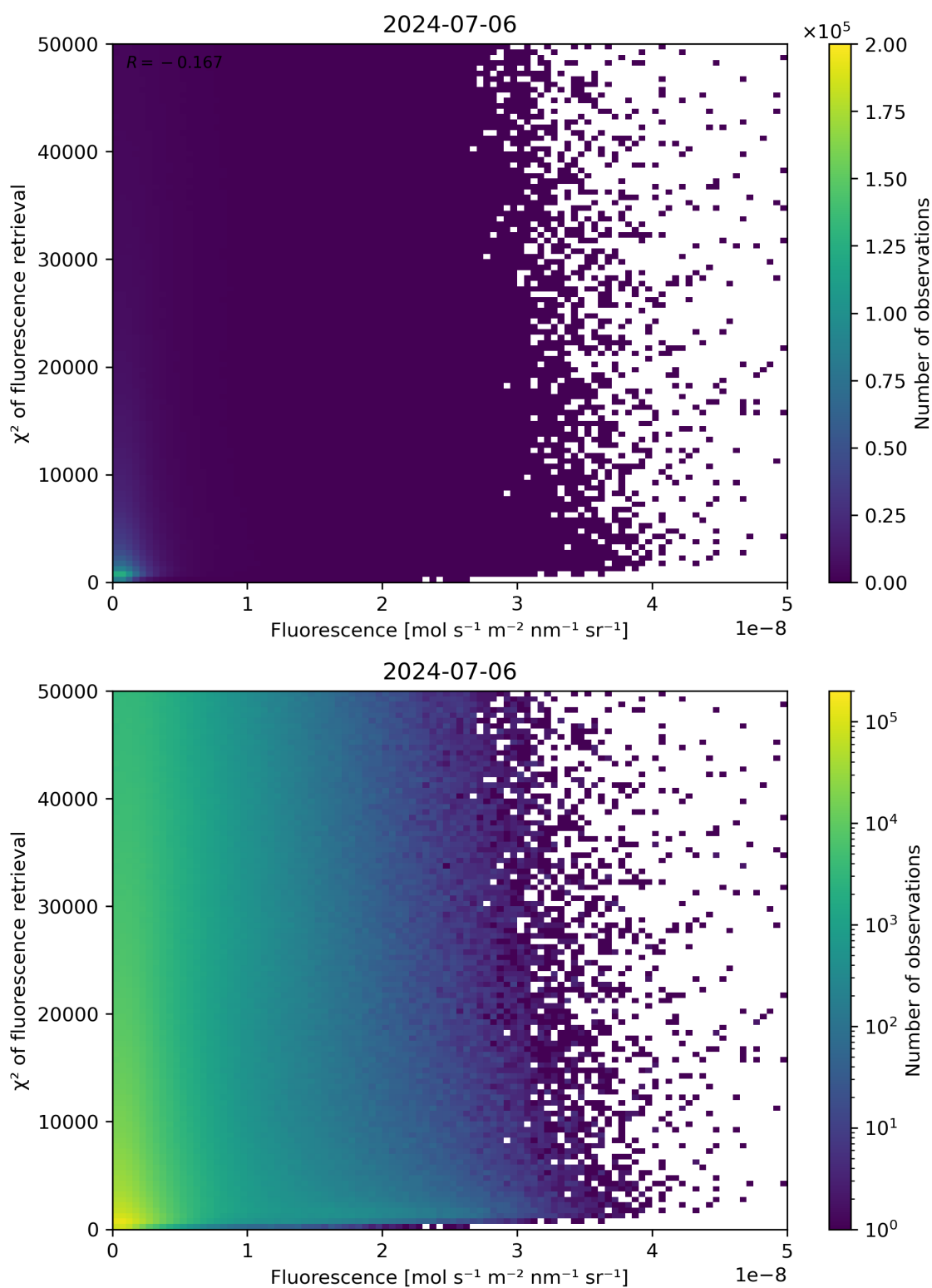
Figure 85: Scatter density plot of “Fluorescence” against “ \chi^2 of fluorescence retrieval” for 2024-07-05 to 2024-07-07.
