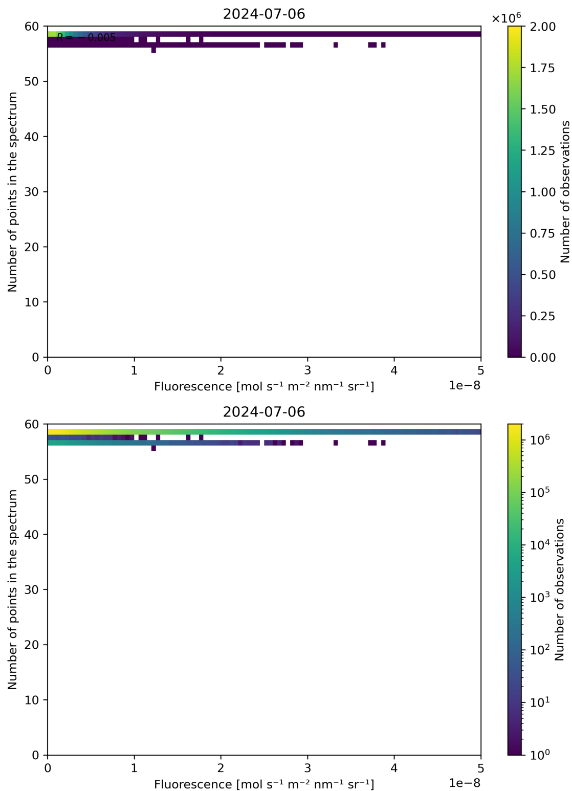
Figure 86: Scatter density plot of “Fluorescence” against “Number of points in the spectrum” for 2024-07-05 to 2024-07-07.
