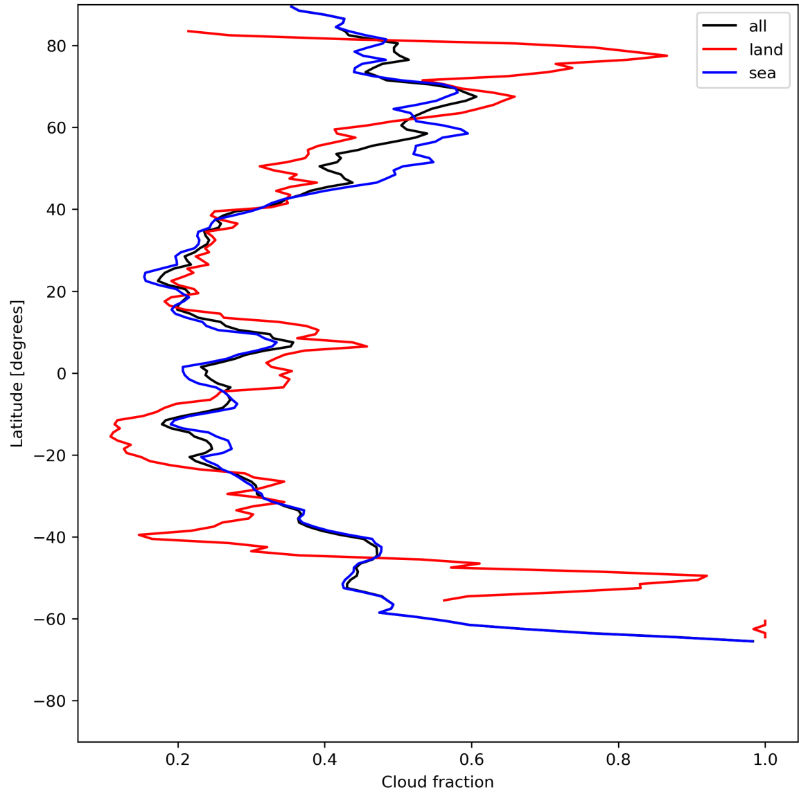
Figure 15: Zonal average of “Cloud fraction” for 2024-07-05 to 2024-07-07.
