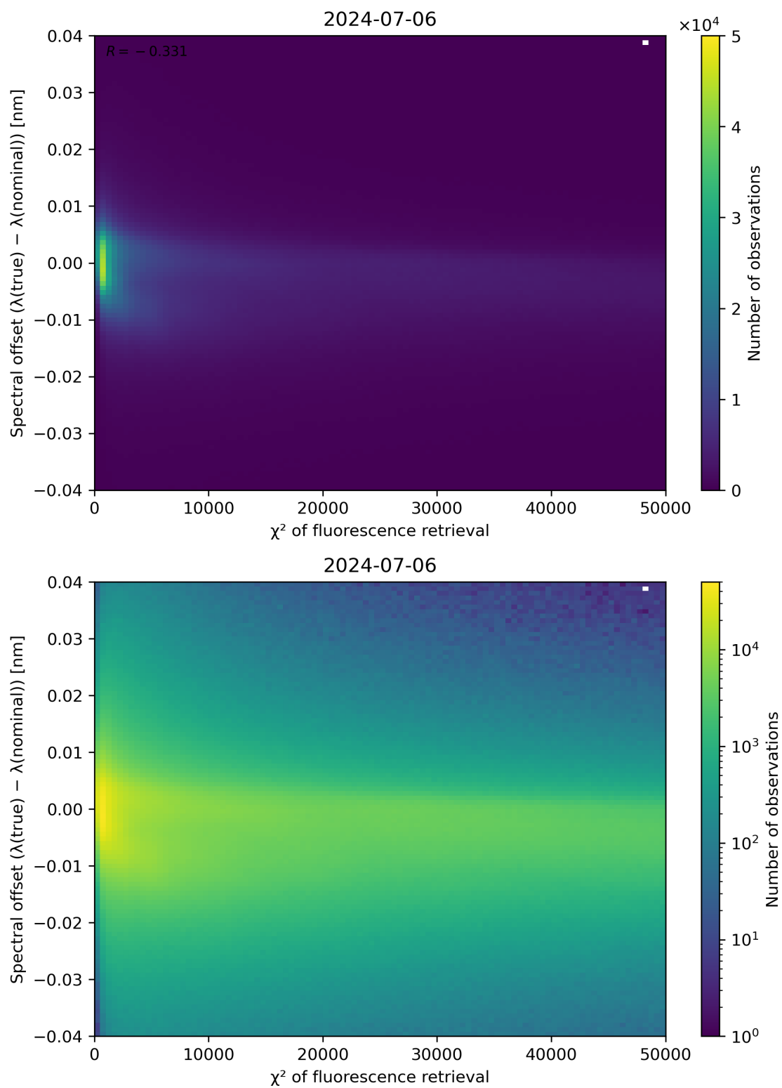
Figure 69: Scatter density plot of “ \chi^2 of fluorescence retrieval” against “Spectral offset ( \lambda(\text{true}) - \lambda(\text{nominal}) )” for 2024-07-05 to 2024-07-07.
