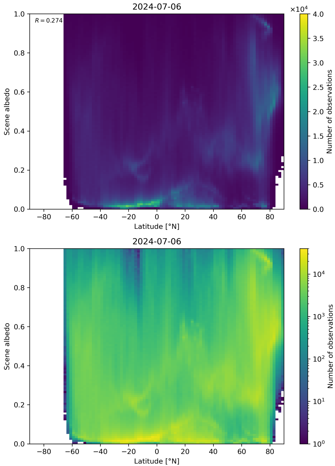
Figure 95: Scatter density plot of “Latitude” against “Scene albedo” for 2024-07-05 to 2024-07-07.
