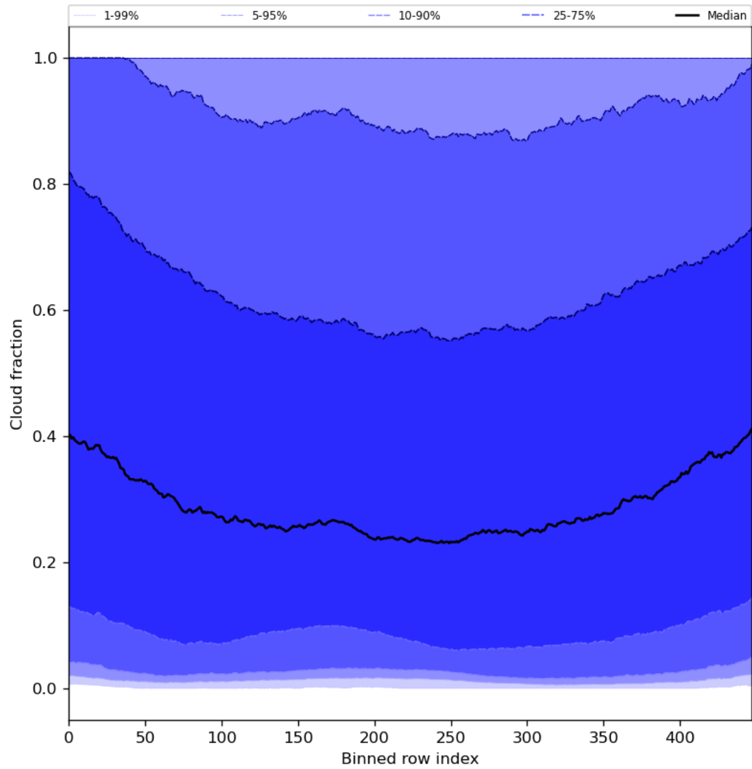
Figure 49: Along track statistics of “Cloud fraction” for 2024-07-05 to 2024-07-07
