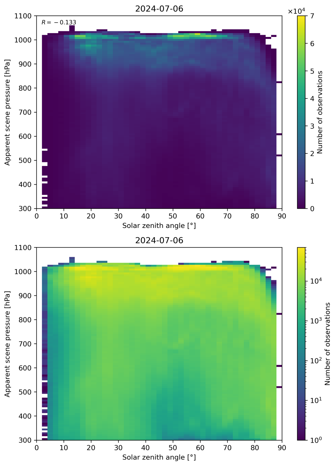
Figure 108: Scatter density plot of “Solar zenith angle” against “Apparent scene pressure” for 2024-07-05 to 2024-07-07.
