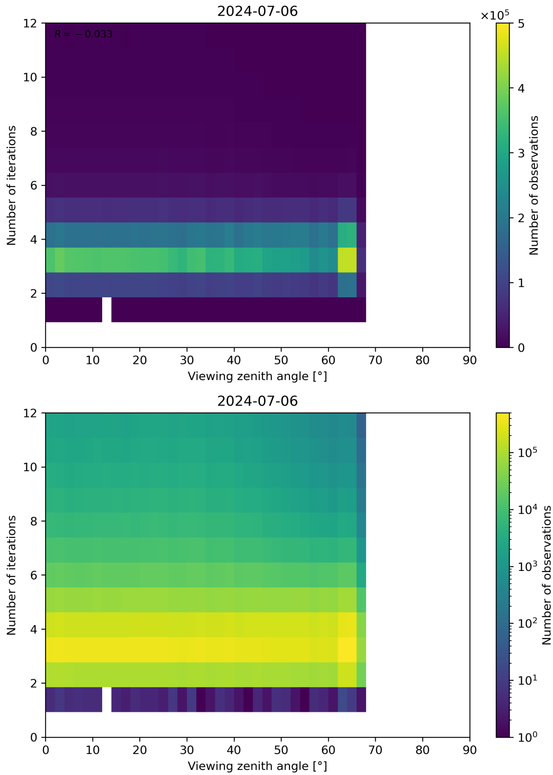
Figure 124: Scatter density plot of “Viewing zenith angle” against “Number of iterations” for 2024-07-05 to 2024-07-07.
