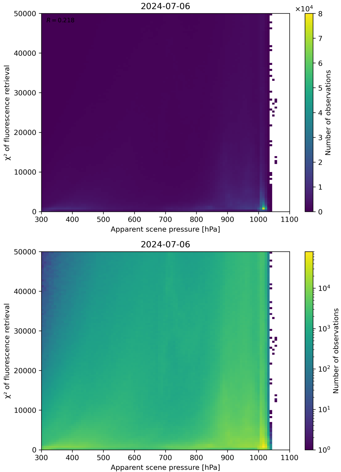
Figure 63: Scatter density plot of “Apparent scene pressure” against “ \chi^2 of fluorescence retrieval” for 2024-07-05 to 2024-07-07.
