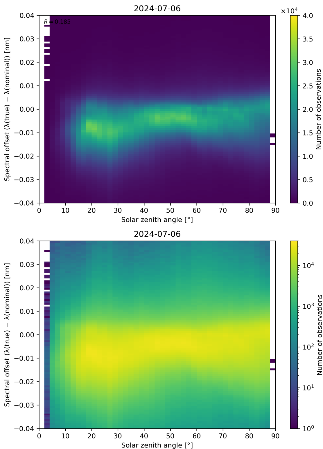
Figure 117: Scatter density plot of “Solar zenith angle” against “Spectral offset ( \lambda(\text{true}) - \lambda(\text{nominal}) )” for 2024-07-05 to 2024-07-07.
