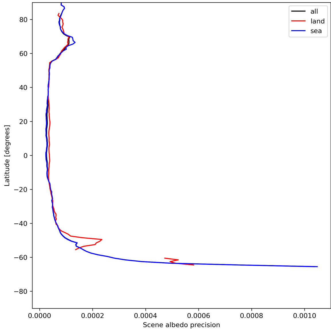
Figure 18: Zonal average of “Scene albedo precision” for 2024-07-05 to 2024-07-07.
