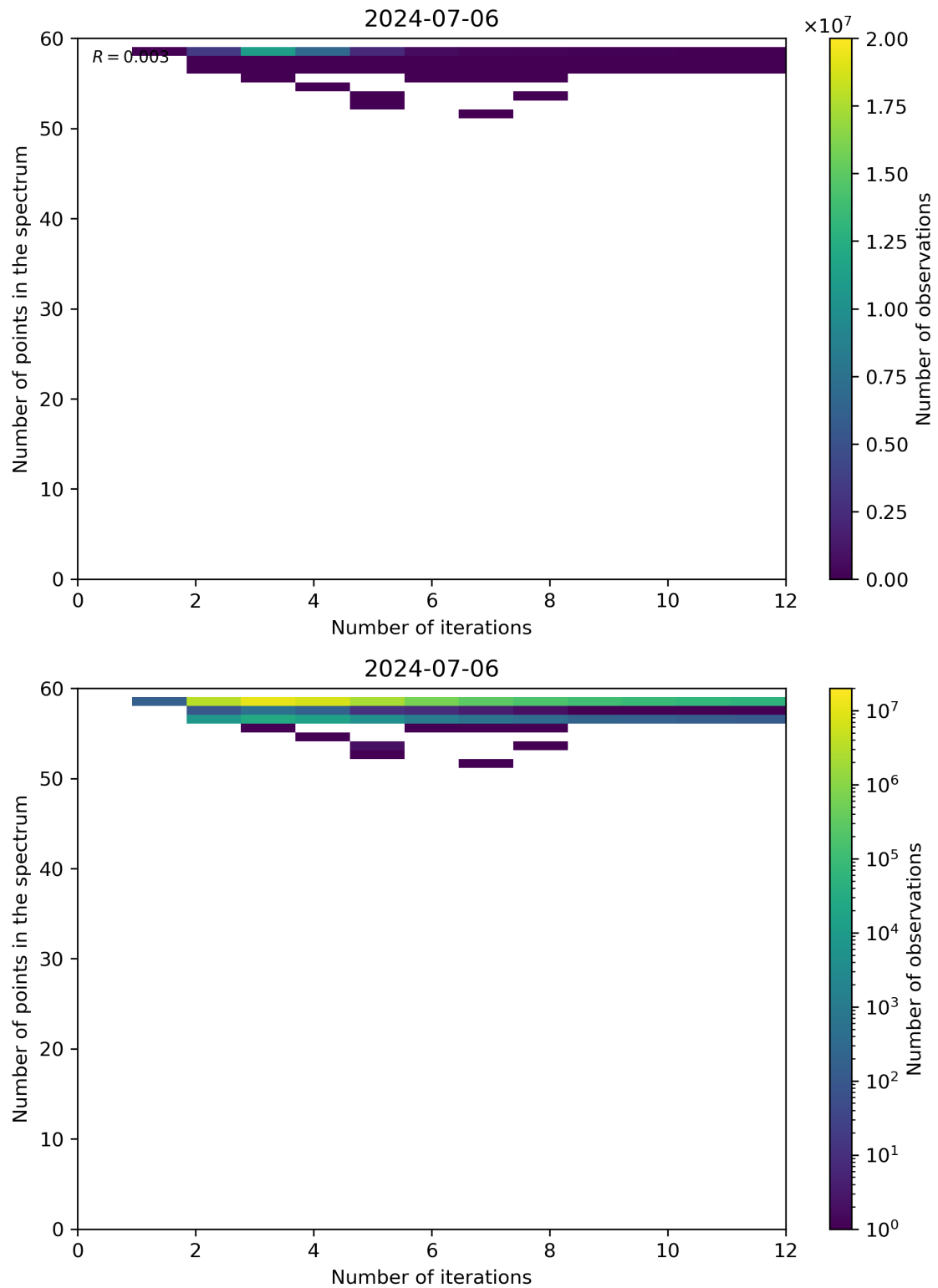
Figure 99: Scatter density plot of “Number of iterations” against “Number of points in the spectrum” for 2024-07-05 to 2024-07-07.
