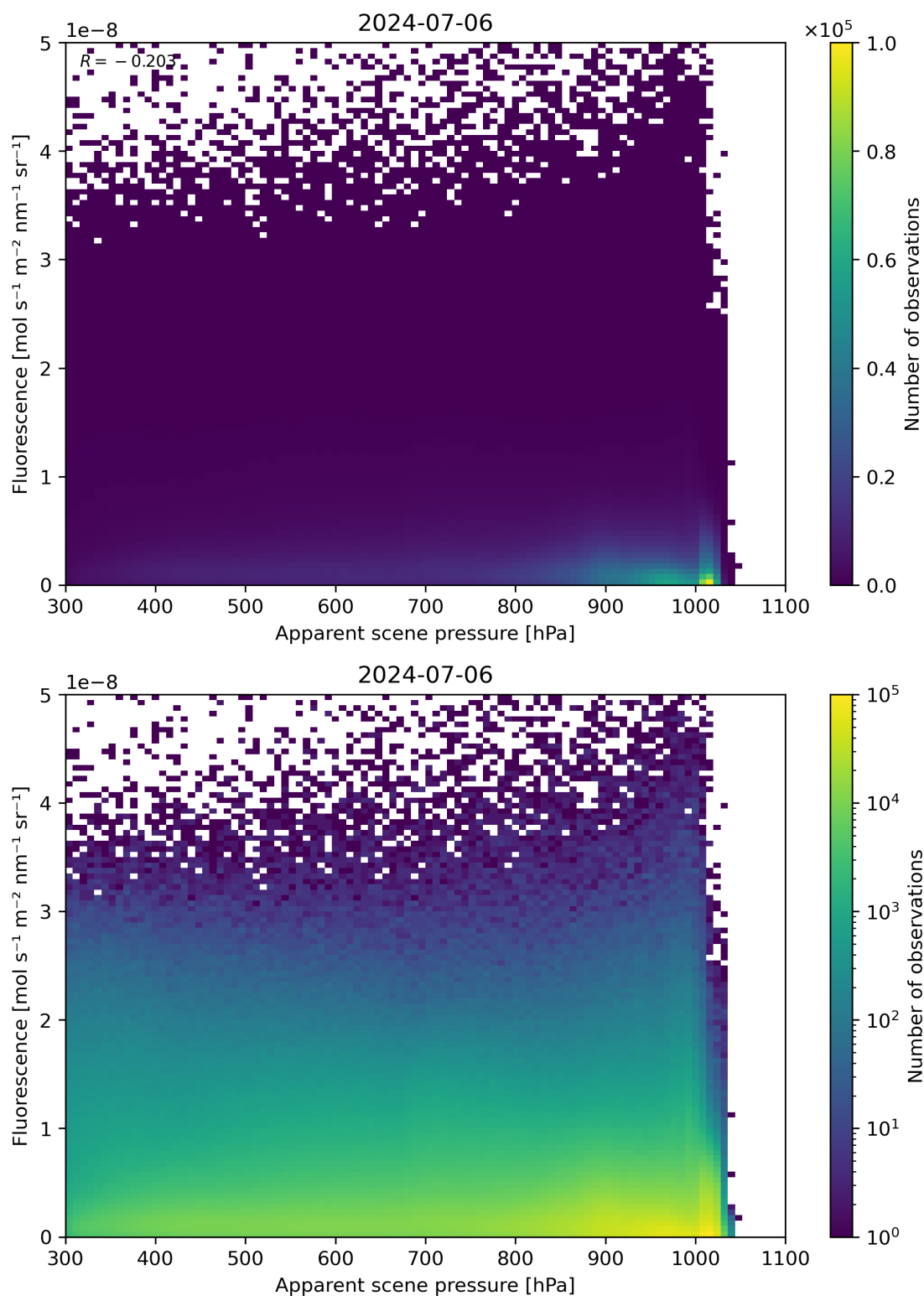
Figure 64: Scatter density plot of “Apparent scene pressure” against “Fluorescence” for 2024-07-05 to 2024-07-07.
