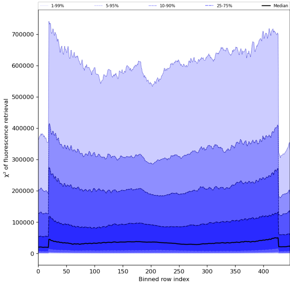
Figure 59: Along track statistics of “ \chi^2 of fluorescence retrieval” for 2024-07-05 to 2024-07-07
