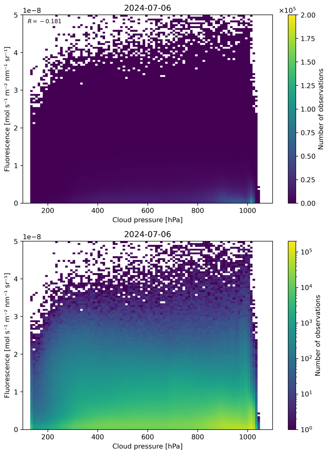
Figure 80: Scatter density plot of “Cloud pressure” against “Fluorescence” for 2024-07-05 to 2024-07-07.
