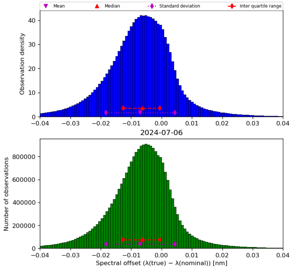
Figure 45: Histogram of “Spectral offset ( \lambda(\text{true}) - \lambda(\text{nominal}) )” for 2024-07-05 to 2024-07-07
