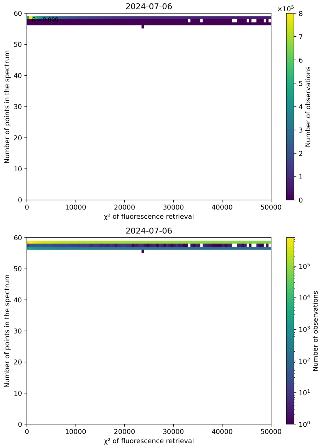
Figure 68: Scatter density plot of “ \chi^2 of fluorescence retrieval” against “Number of points in the spectrum” for 2024-07-05 to 2024-07-07.
