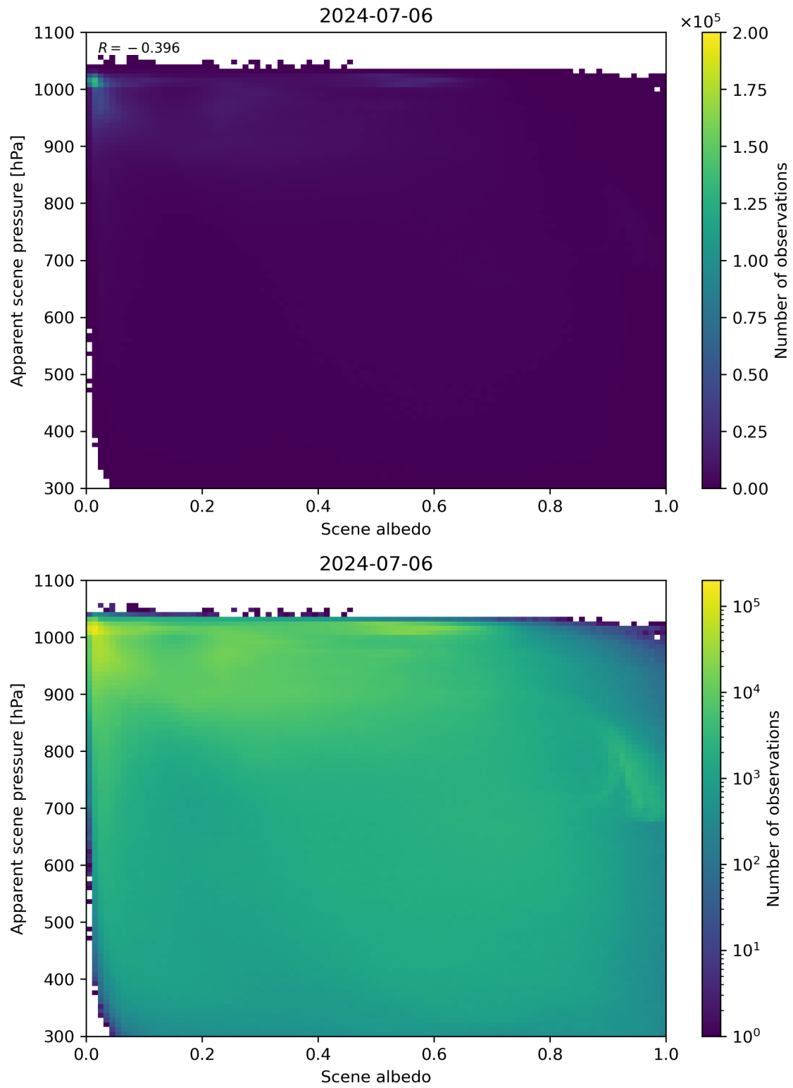
Figure 102: Scatter density plot of “Scene albedo” against “Apparent scene pressure” for 2024-07-05 to 2024-07-07.
