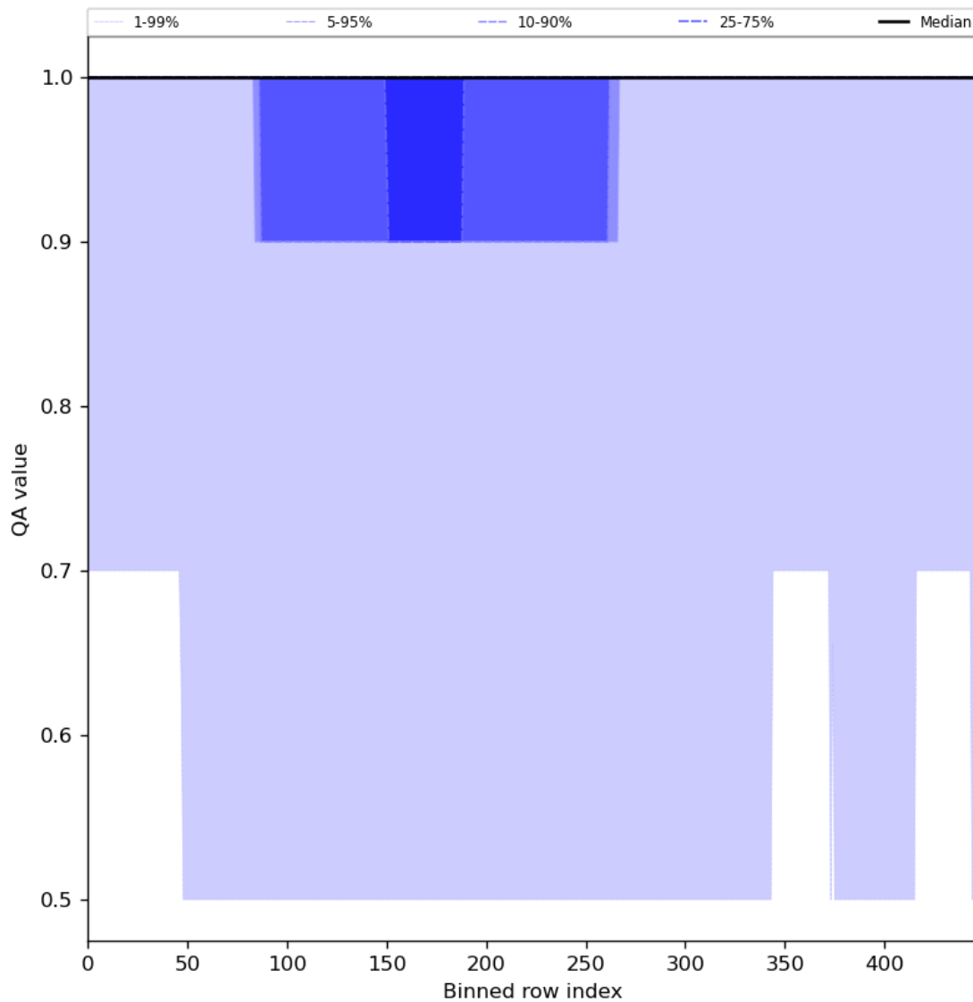
Figure 46: Along track statistics of “QA value” for 2024-07-05 to 2024-07-07
