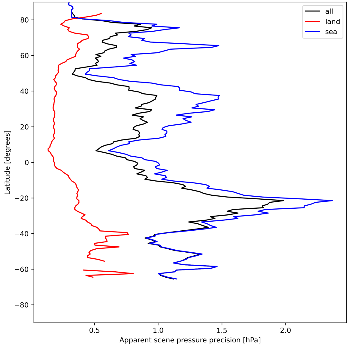
Figure 20: Zonal average of “Apparent scene pressure precision” for 2024-07-05 to 2024-07-07.
