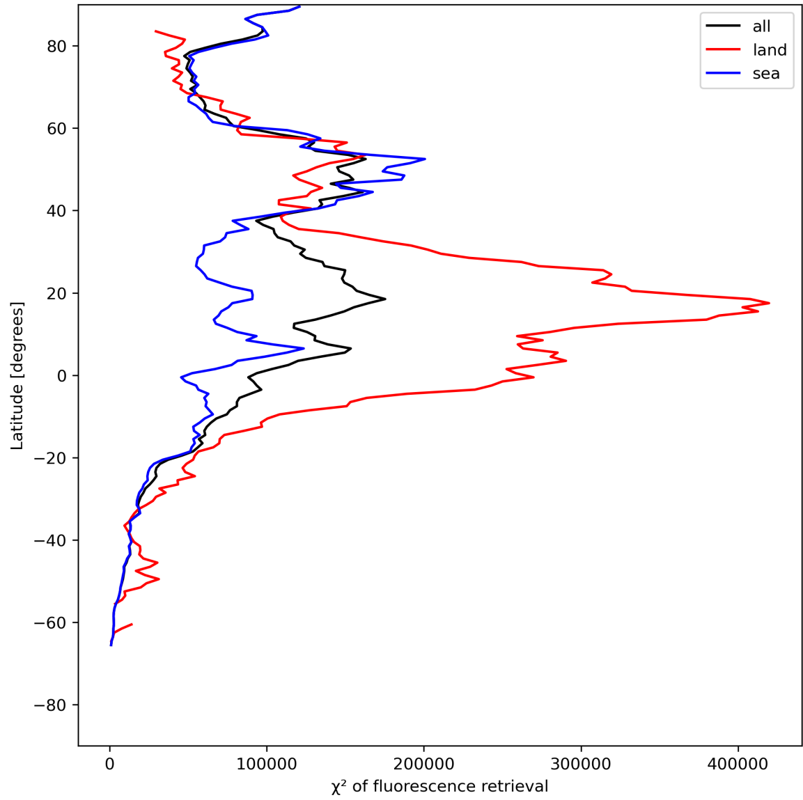
Figure 25: Zonal average of “ \chi^2 of fluorescence retrieval” for 2024-07-05 to 2024-07-07.
