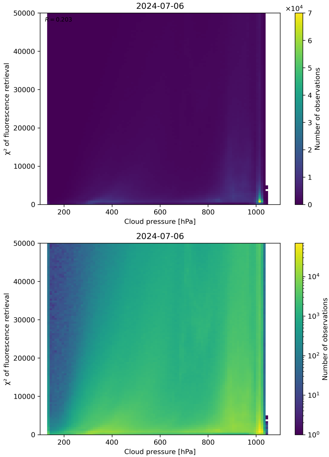
Figure 78: Scatter density plot of “Cloud pressure” against “ \chi^2 of fluorescence retrieval” for 2024-07-05 to 2024-07-07.
