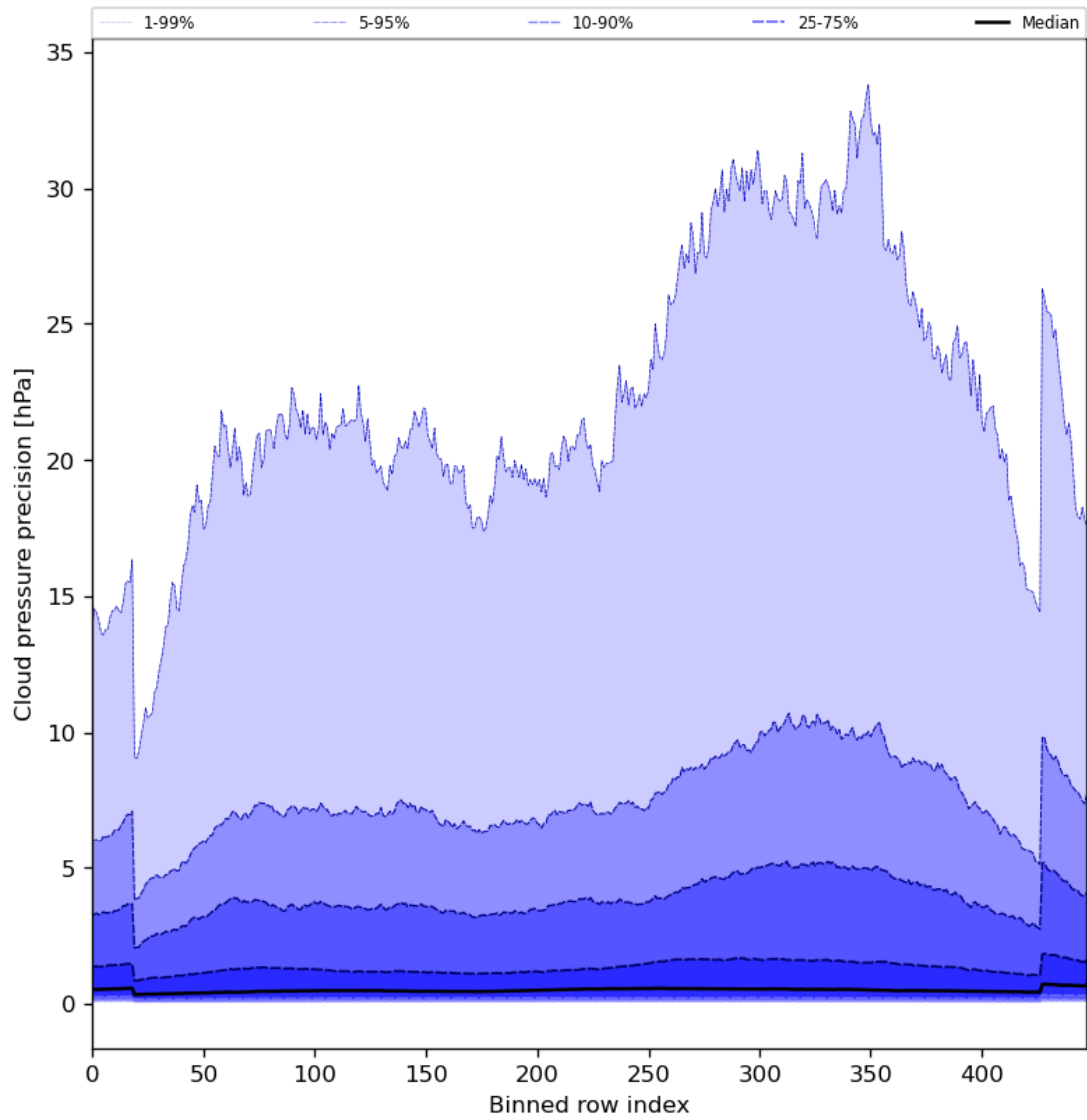
Figure 48: Along track statistics of “Cloud pressure precision” for 2024-07-05 to 2024-07-07
