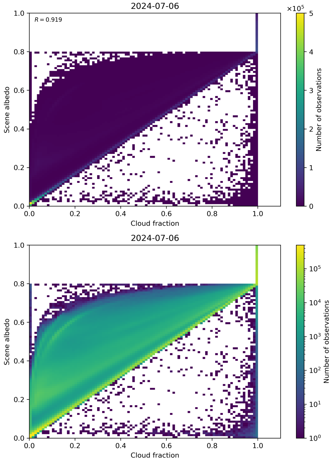
Figure 75: Scatter density plot of “Cloud fraction” against “Scene albedo” for 2024-07-05 to 2024-07-07.
