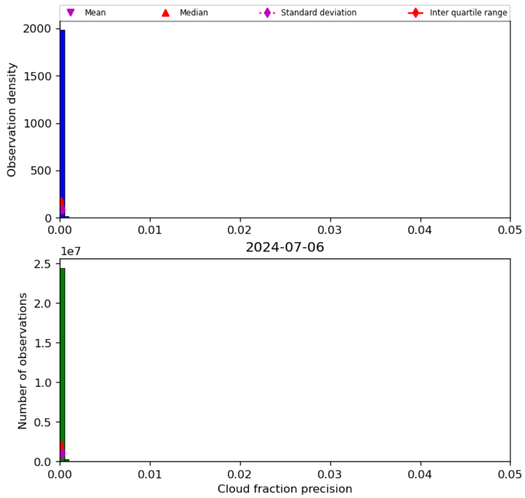
Figure 33: Histogram of “Cloud fraction precision” for 2024-07-05 to 2024-07-07
