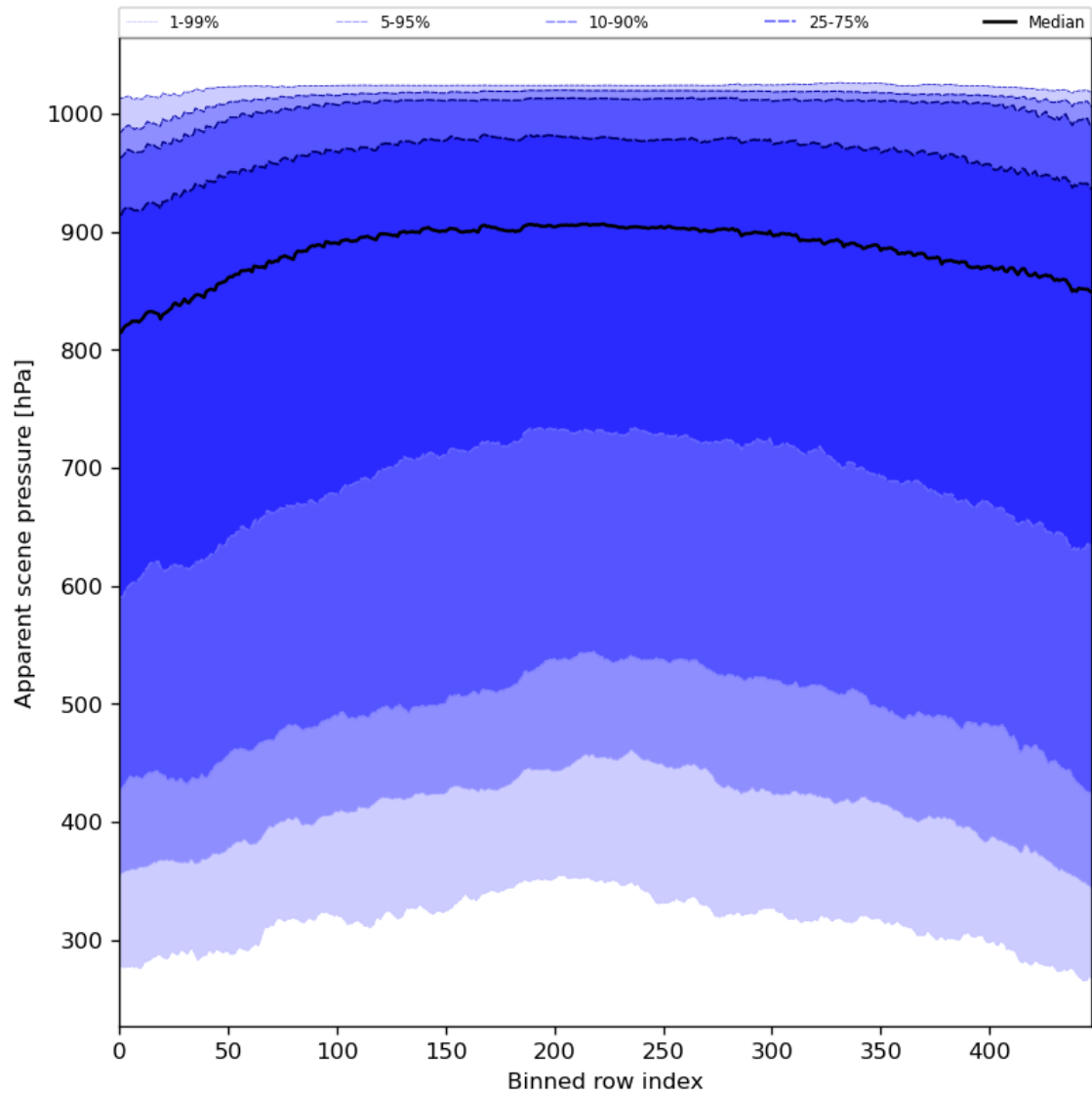
Figure 53: Along track statistics of “Apparent scene pressure” for 2024-07-05 to 2024-07-07
