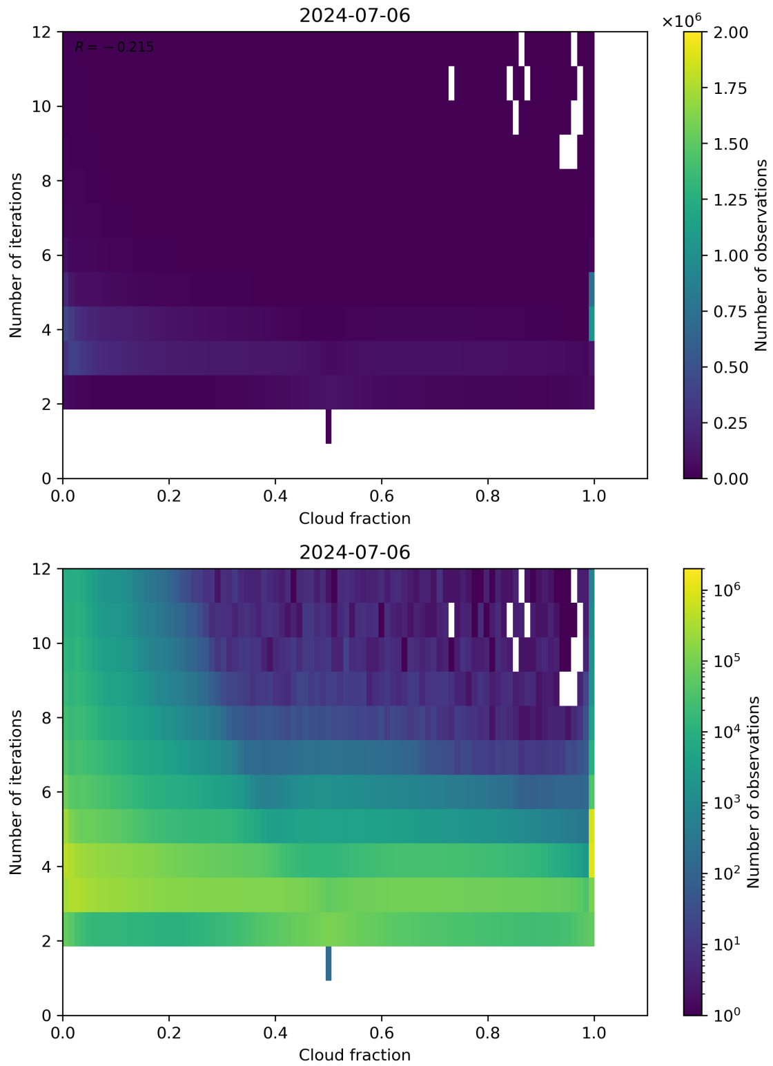
Figure 73: Scatter density plot of “Cloud fraction” against “Number of iterations” for 2024-07-05 to 2024-07-07.
