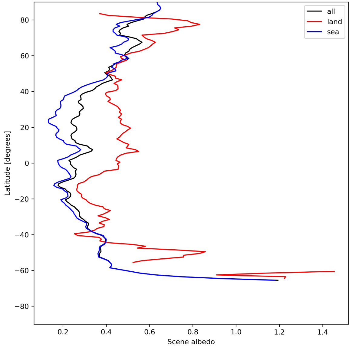
Figure 17: Zonal average of “Scene albedo” for 2024-07-05 to 2024-07-07.
