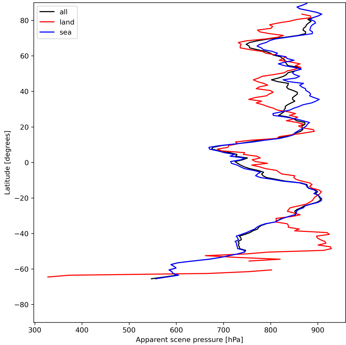
Figure 19: Zonal average of “Apparent scene pressure” for 2024-07-05 to 2024-07-07.
