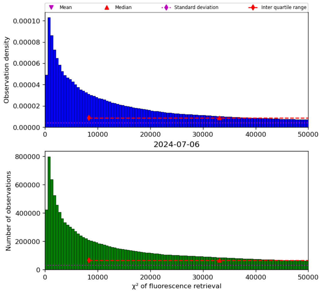
Figure 42: Histogram of “ \chi^2 of fluorescence retrieval” for 2024-07-05 to 2024-07-07
