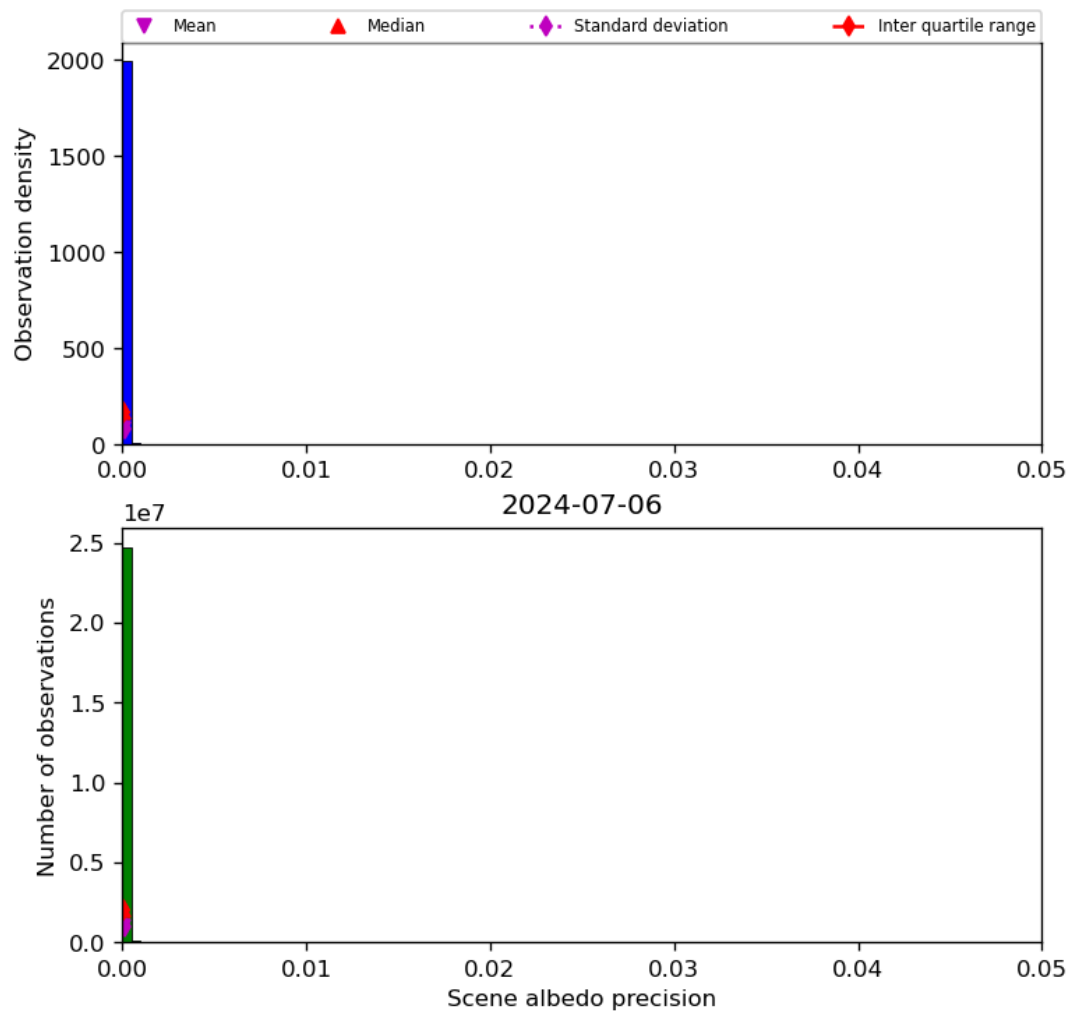
Figure 35: Histogram of “Scene albedo precision” for 2024-07-05 to 2024-07-07
