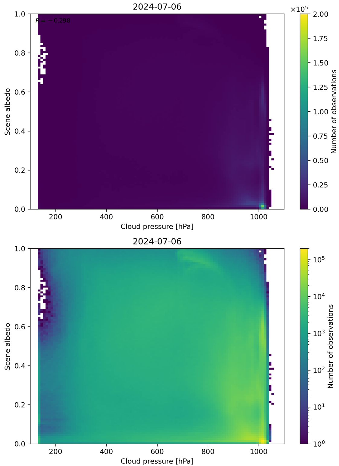
Figure 83: Scatter density plot of “Cloud pressure” against “Scene albedo” for 2024-07-05 to 2024-07-07.
