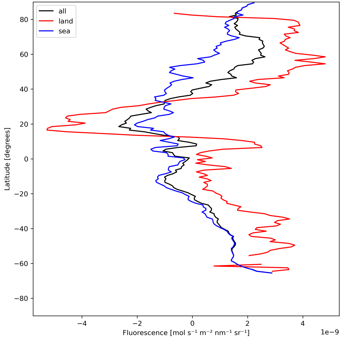
Figure 23: Zonal average of “Fluorescence” for 2024-07-05 to 2024-07-07.
