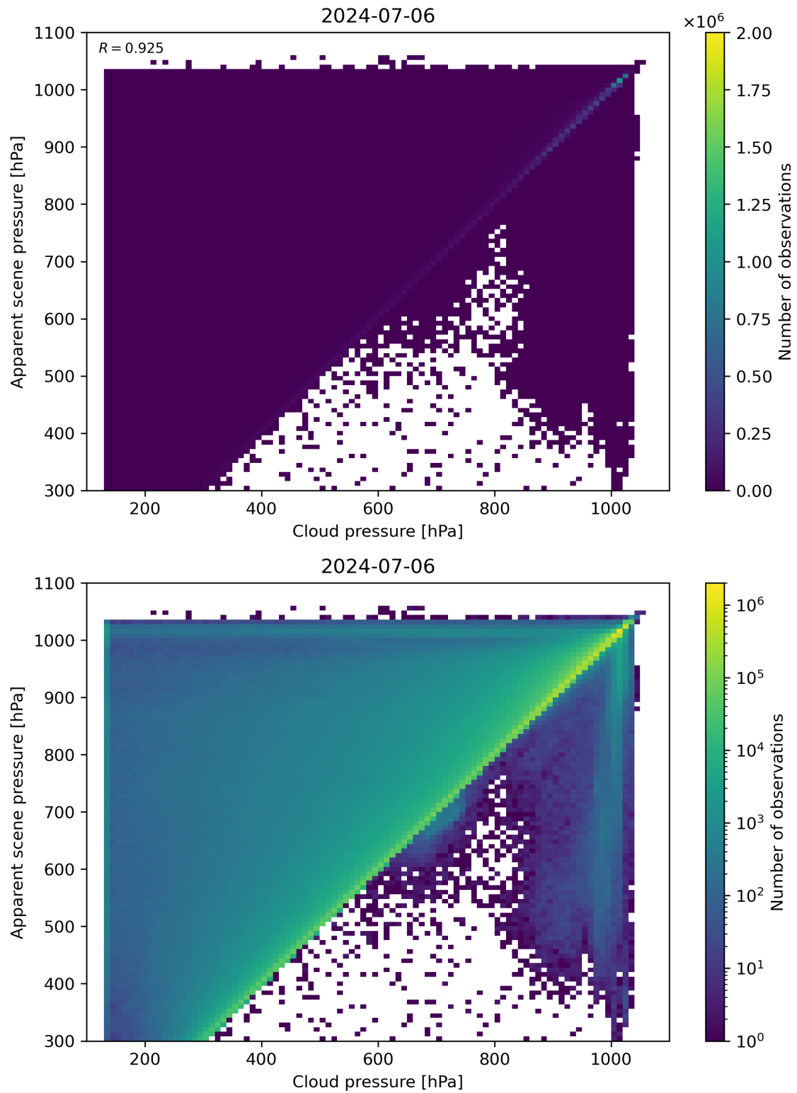
Figure 77: Scatter density plot of “Cloud pressure” against “Apparent scene pressure” for 2024-07-05 to 2024-07-07.
