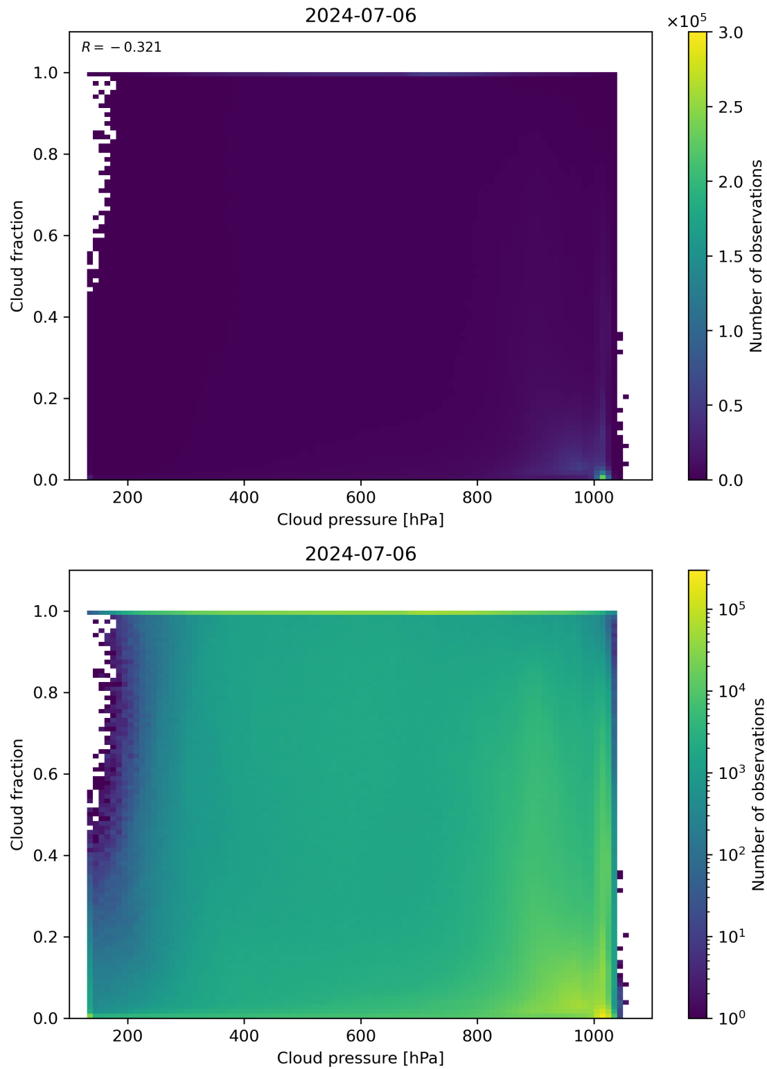
Figure 79: Scatter density plot of “Cloud pressure” against “Cloud fraction” for 2024-07-05 to 2024-07-07.
