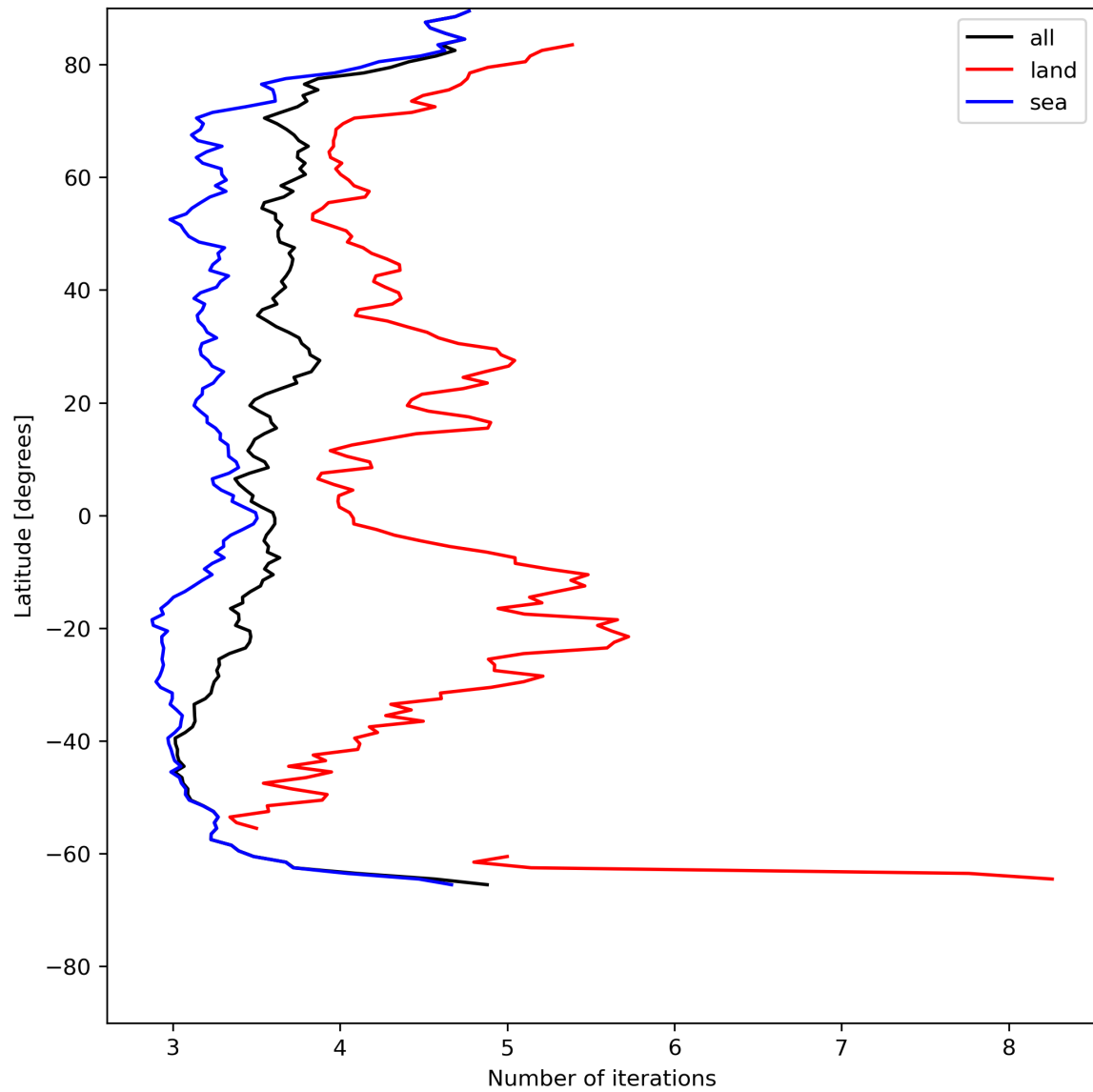
Figure 22: Zonal average of “Number of iterations” for 2024-07-05 to 2024-07-07.
