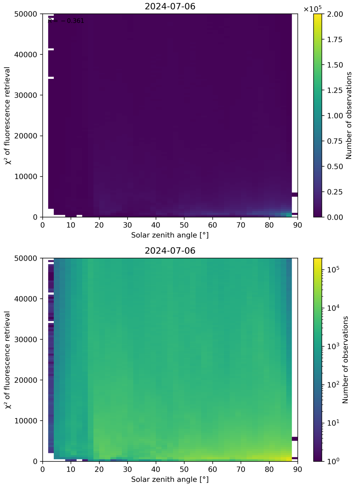
Figure 109: Scatter density plot of “Solar zenith angle” against “ \chi^2 of fluorescence retrieval” for 2024-07-05 to 2024-07-07.
