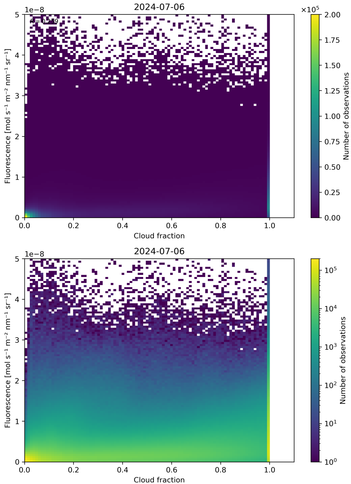
Figure 72: Scatter density plot of “Cloud fraction” against “Fluorescence” for 2024-07-05 to 2024-07-07.
