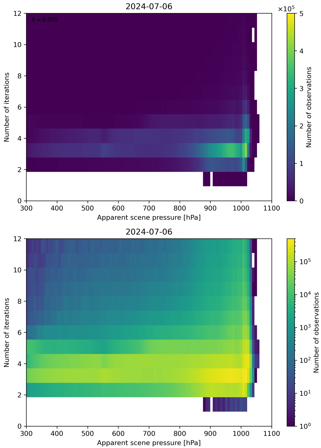
Figure 65: Scatter density plot of “Apparent scene pressure” against “Number of iterations” for 2024-07-05 to 2024-07-07.
