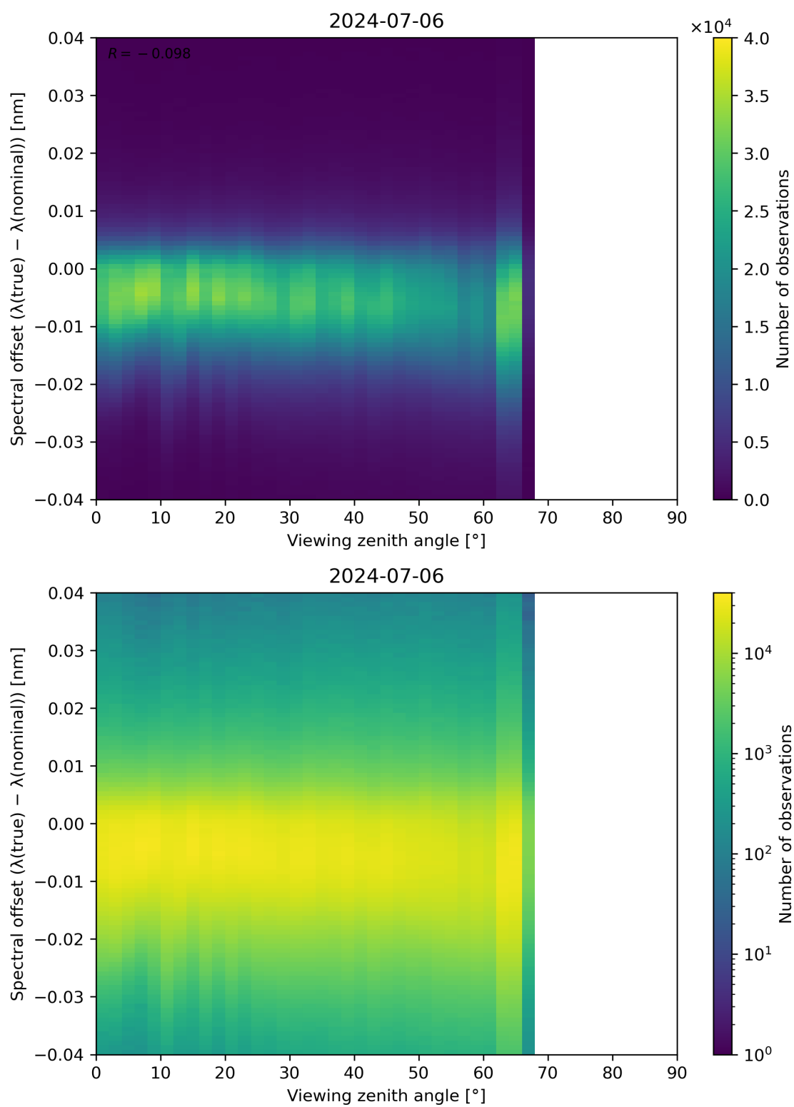
Figure 128: Scatter density plot of “Viewing zenith angle” against “Spectral offset ( \lambda(\text{true}) - \lambda(\text{nominal}) )” for 2024-07-05 to 2024-07-07.
