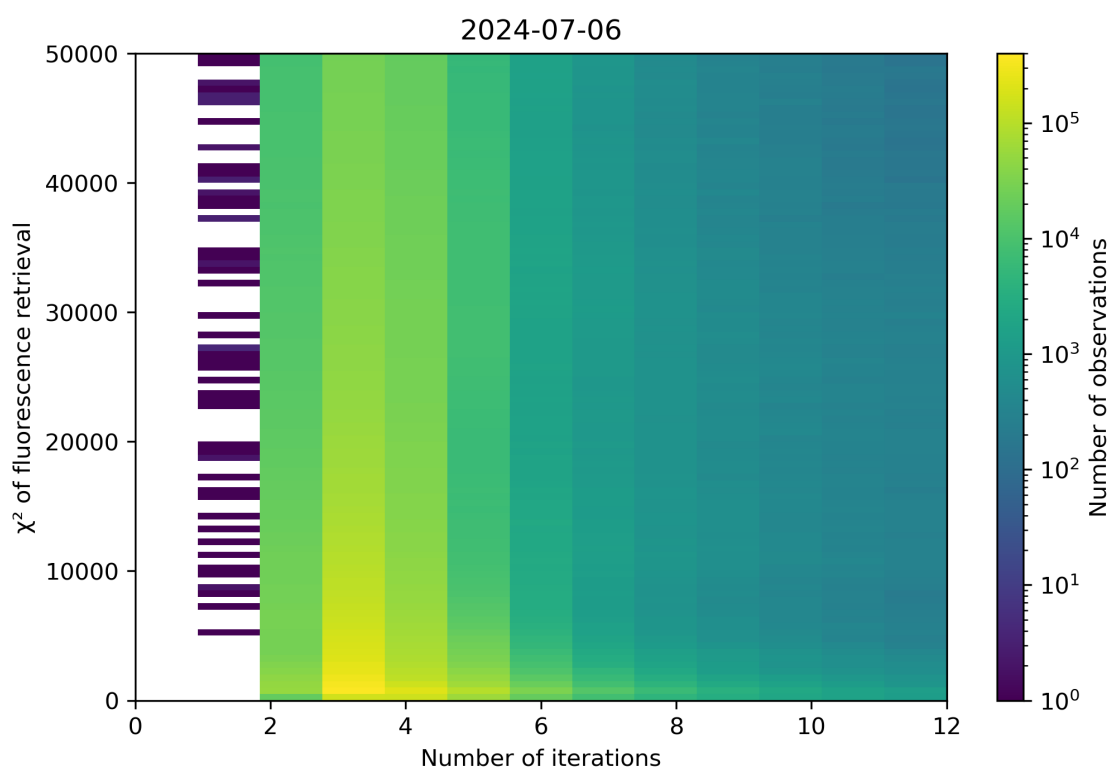
Figure 97: Scatter density plot of “Number of iterations” against “ \chi^2 of fluorescence retrieval” for 2024-07-05 to 2024-07-07.
