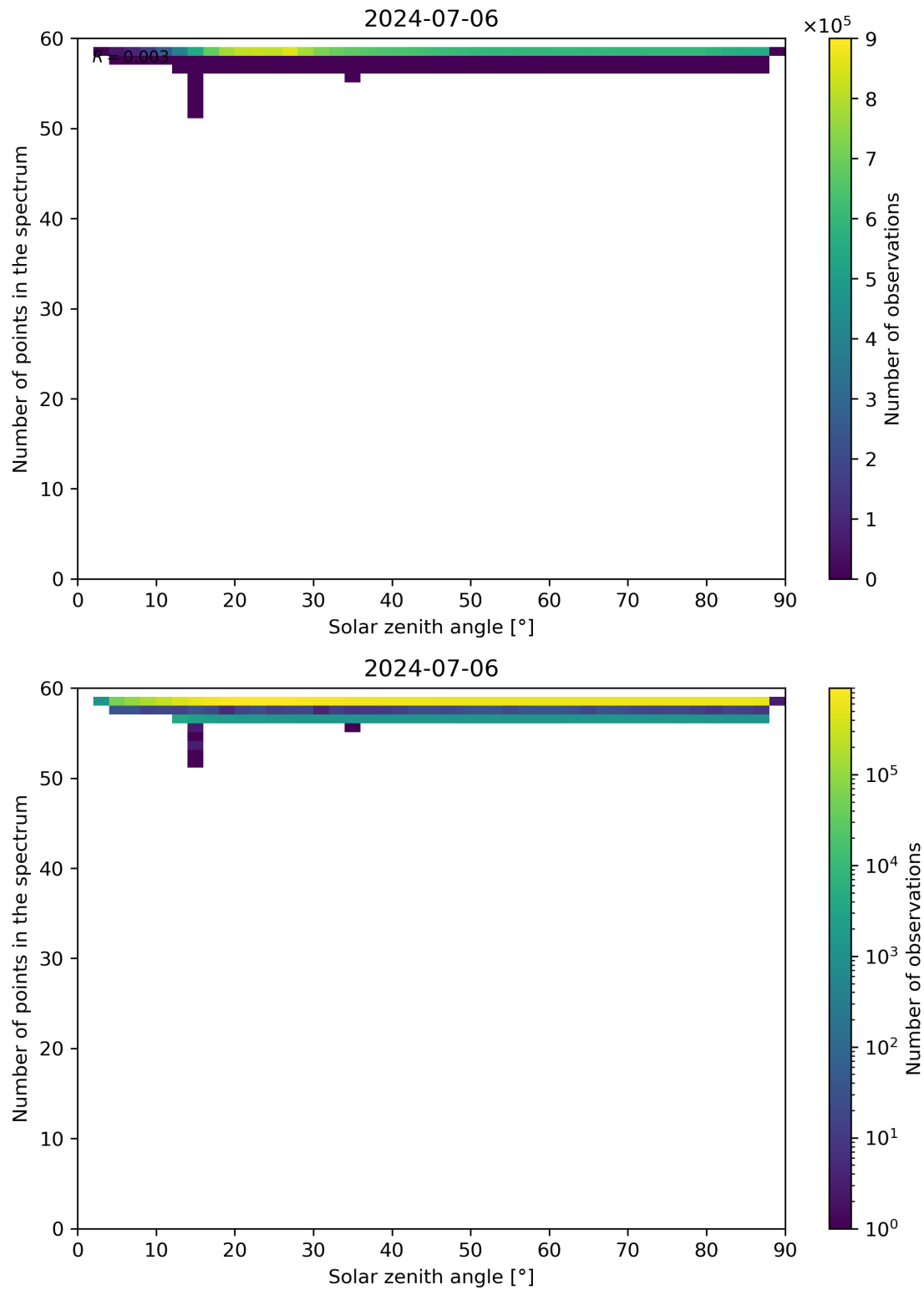
Figure 115: Scatter density plot of “Solar zenith angle” against “Number of points in the spectrum” for 2024-07-05 to 2024-07-07.
