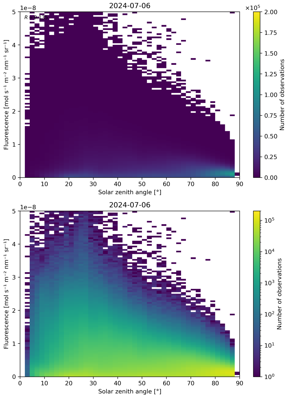
Figure 112: Scatter density plot of “Solar zenith angle” against “Fluorescence” for 2024-07-05 to 2024-07-07.
