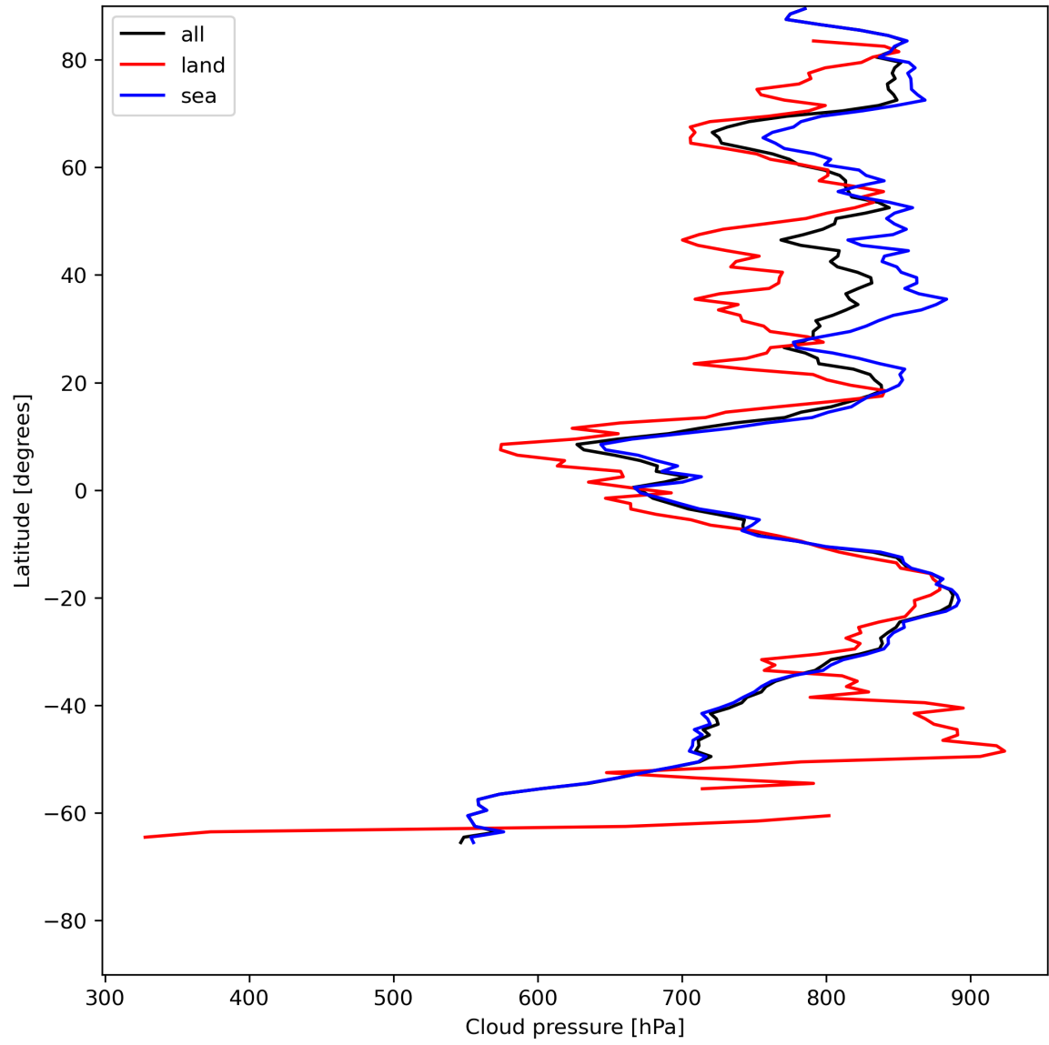
Figure 13: Zonal average of “Cloud pressure” for 2024-07-05 to 2024-07-07.
