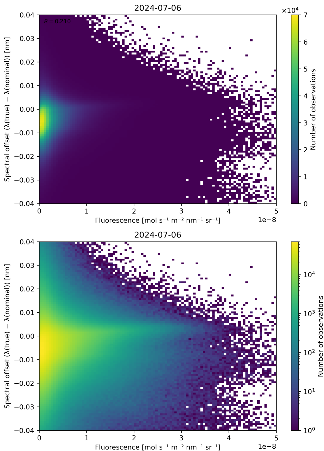
Figure 87: Scatter density plot of “Fluorescence” against “Spectral offset ( \lambda(\text{true}) - \lambda(\text{nominal}) )” for 2024-07-05 to 2024-07-07.
