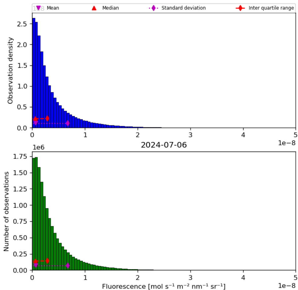
Figure 40: Histogram of “Fluorescence” for 2024-07-05 to 2024-07-07
