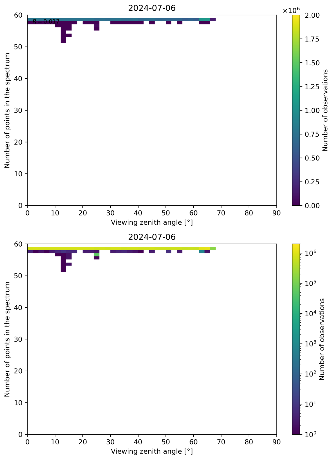
Figure 125: Scatter density plot of “Viewing zenith angle” against “Number of points in the spectrum” for 2024-07-05 to 2024-07-07.
