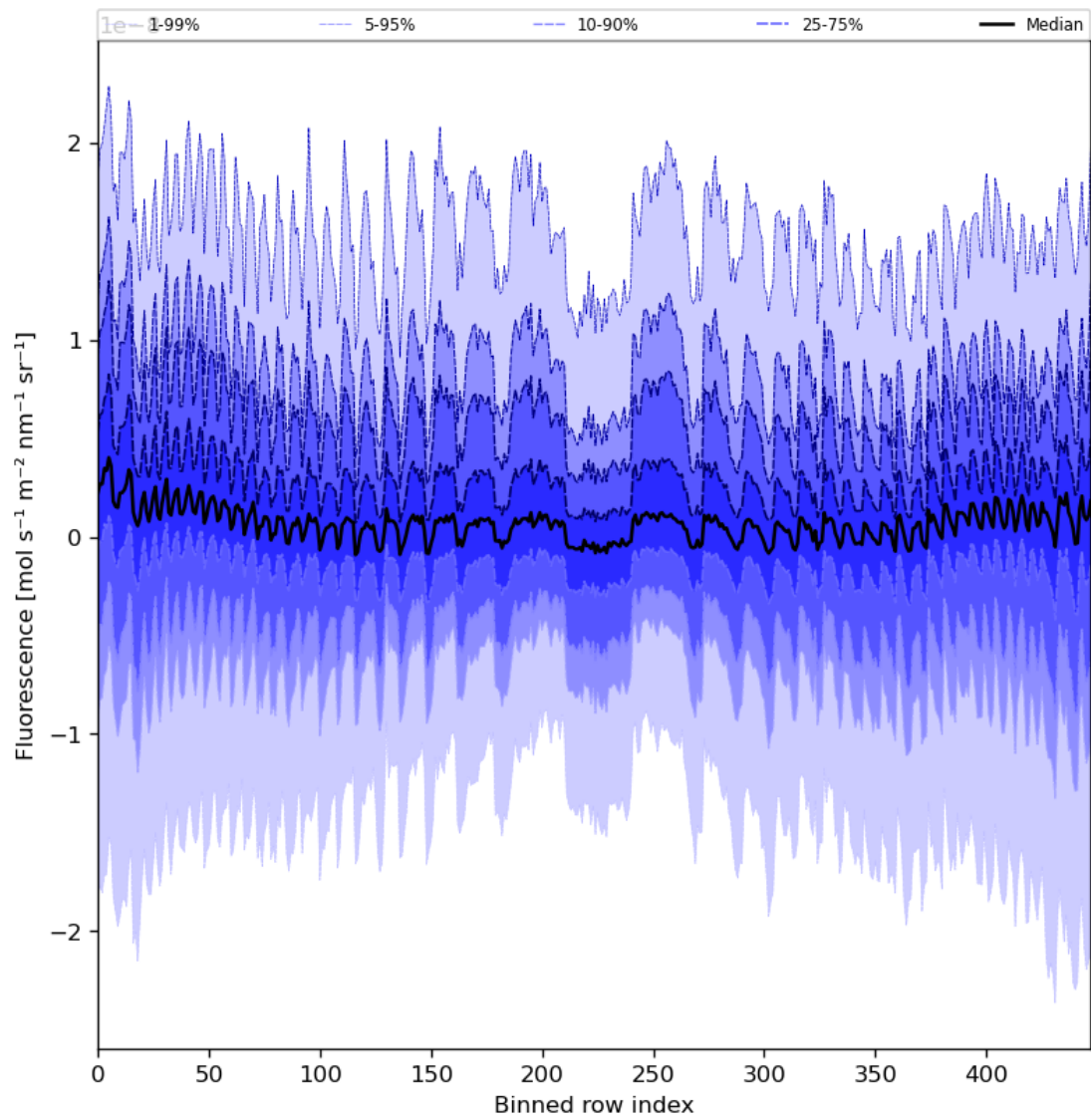
Figure 57: Along track statistics of “Fluorescence” for 2024-07-05 to 2024-07-07
