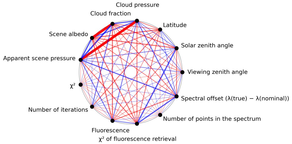
Figure 1: Map of correlation graph for 2024-07-05 to 2024-07-07.
