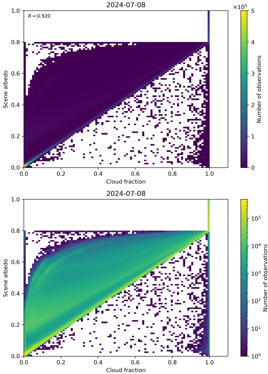
Figure 75: Scatter density plot of “Cloud fraction” against “Scene albedo” for 2024-07-07 to 2024-07-09.
