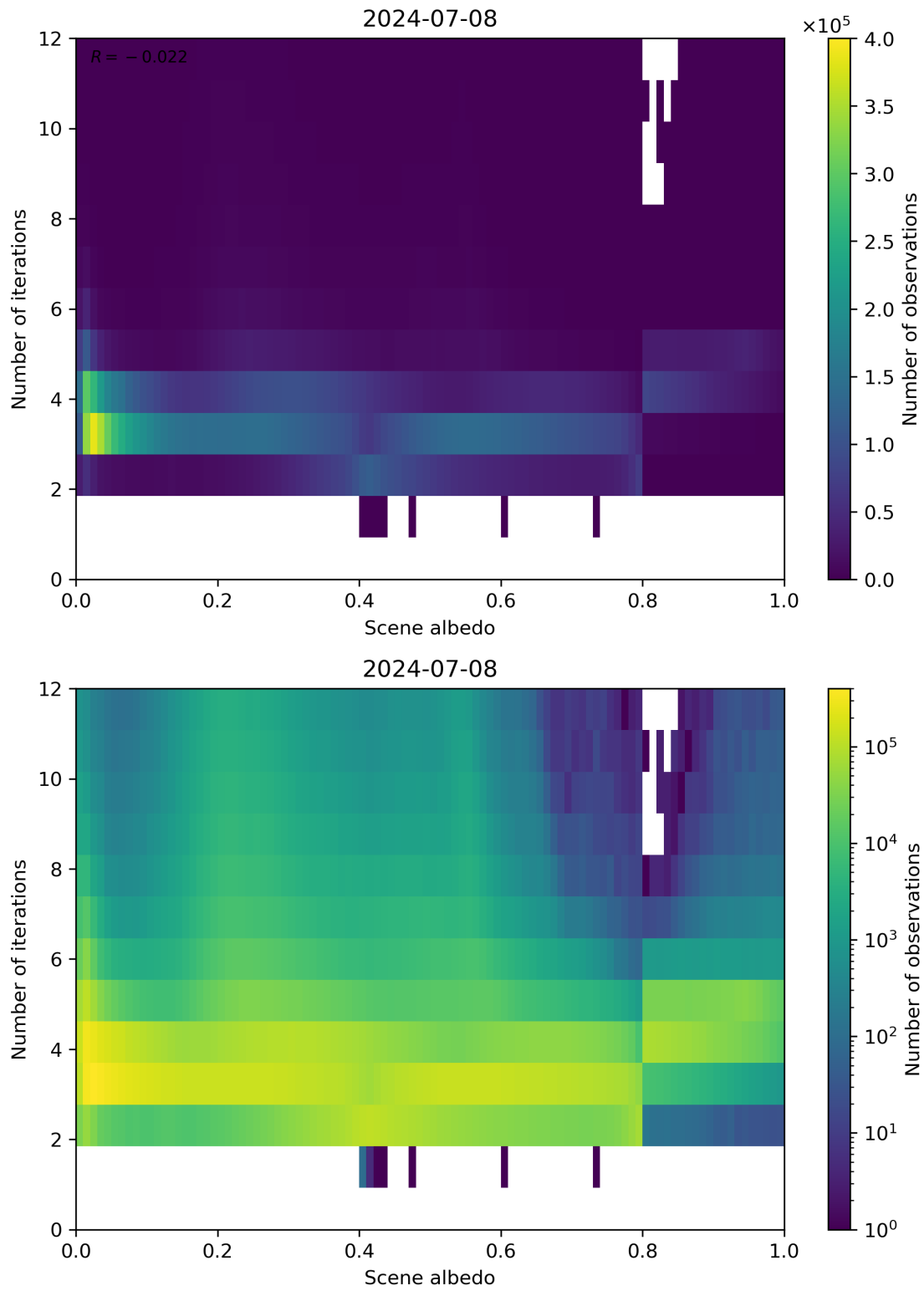
Figure 105: Scatter density plot of “Scene albedo” against “Number of iterations” for 2024-07-07 to 2024-07-09.
