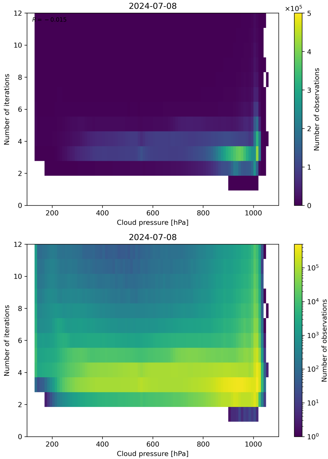
Figure 81: Scatter density plot of “Cloud pressure” against “Number of iterations” for 2024-07-07 to 2024-07-09.
