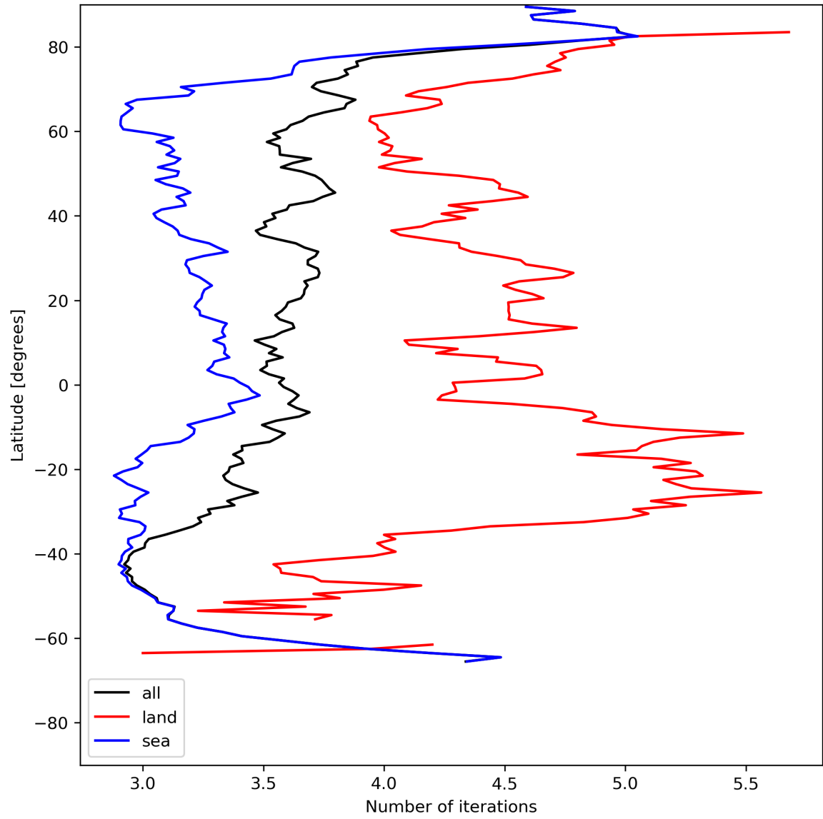
Figure 22: Zonal average of “Number of iterations” for 2024-07-07 to 2024-07-09.
