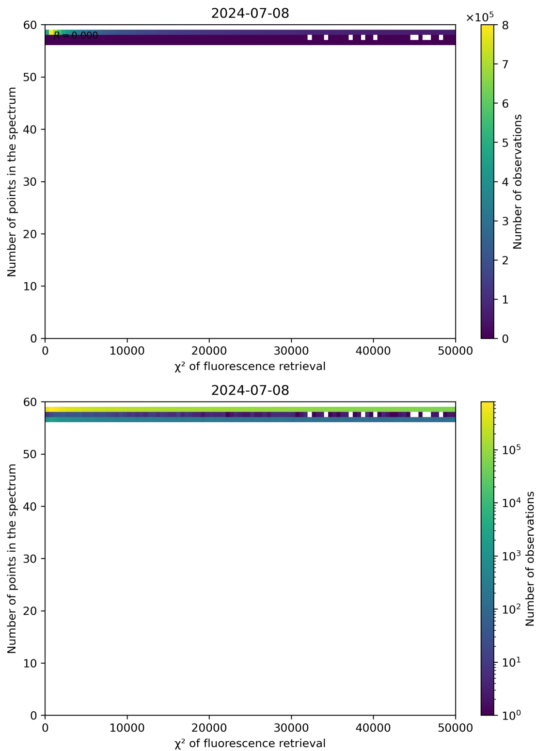
Figure 68: Scatter density plot of " \chi^2 of fluorescence retrieval" against "Number of points in the spectrum" for 2024-07-07 to 2024-07-09.
