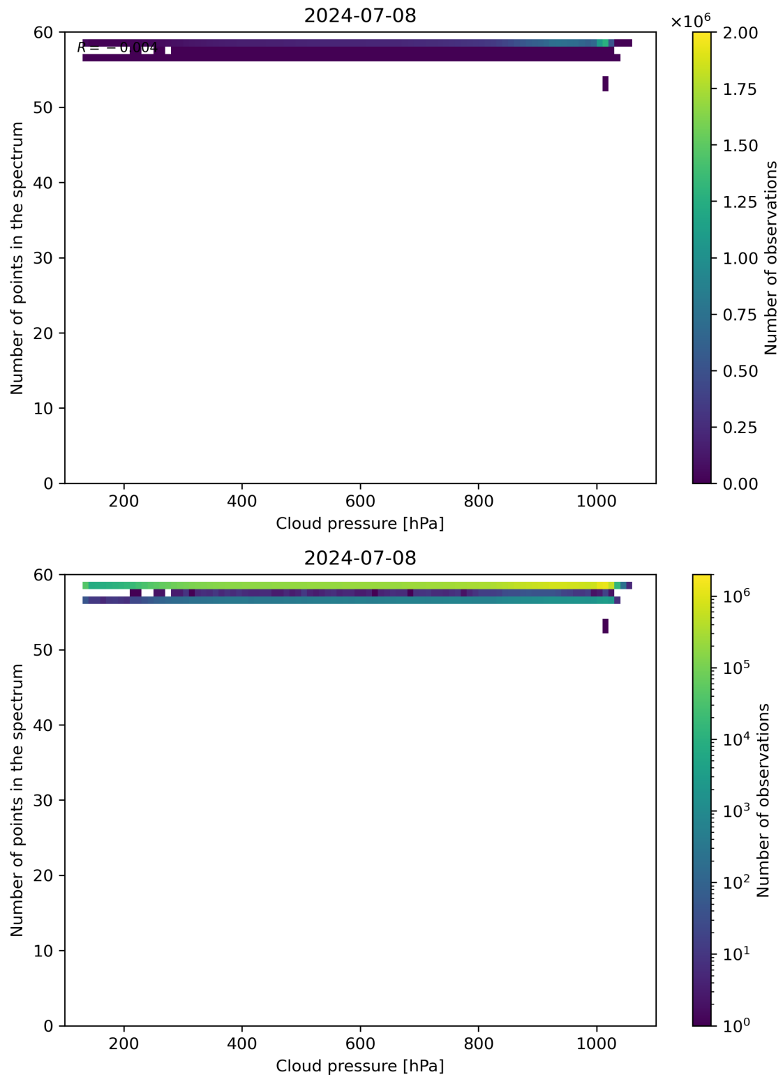
Figure 82: Scatter density plot of “Cloud pressure” against “Number of points in the spectrum” for 2024-07-07 to 2024-07-09.
