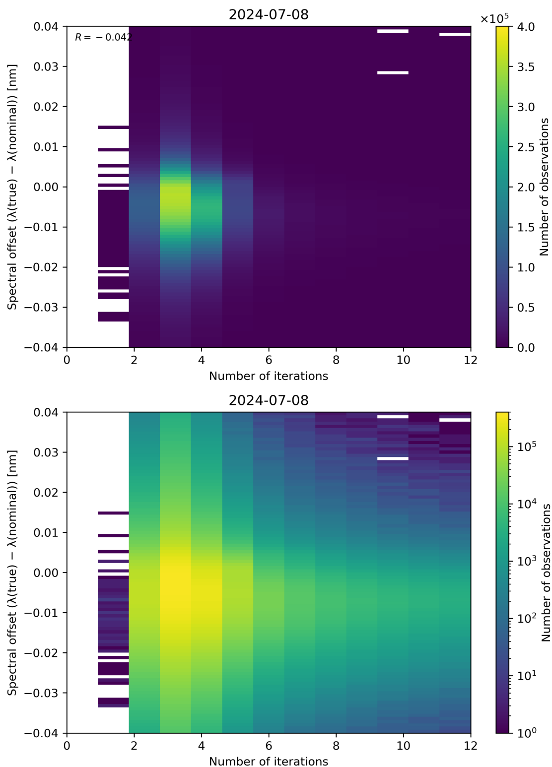
Figure 100: Scatter density plot of “Number of iterations” against “Spectral offset ( \lambda(\text{true}) - \lambda(\text{nominal}) )” for 2024-07-07 to 2024-07-09.
