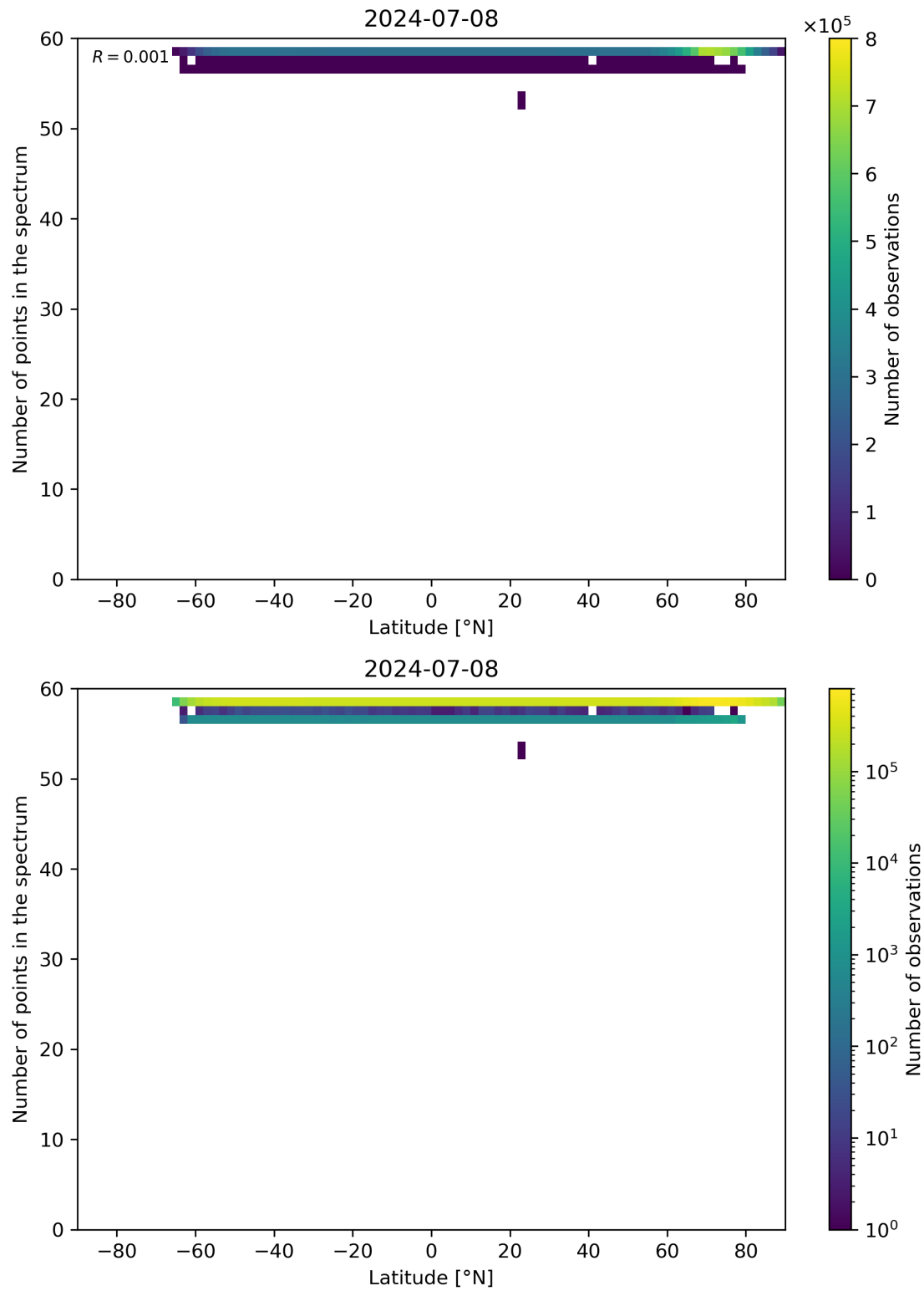
Figure 94: Scatter density plot of “Latitude” against “Number of points in the spectrum” for 2024-07-07 to 2024-07-09.
