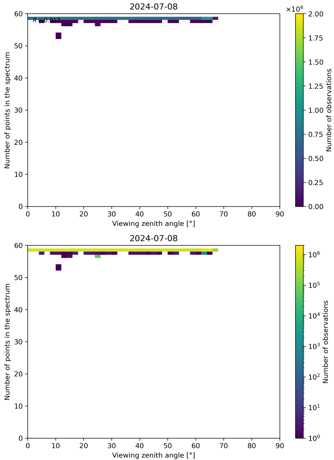
Figure 125: Scatter density plot of “Viewing zenith angle” against “Number of points in the spectrum” for 2024-07-07 to 2024-07-09.
