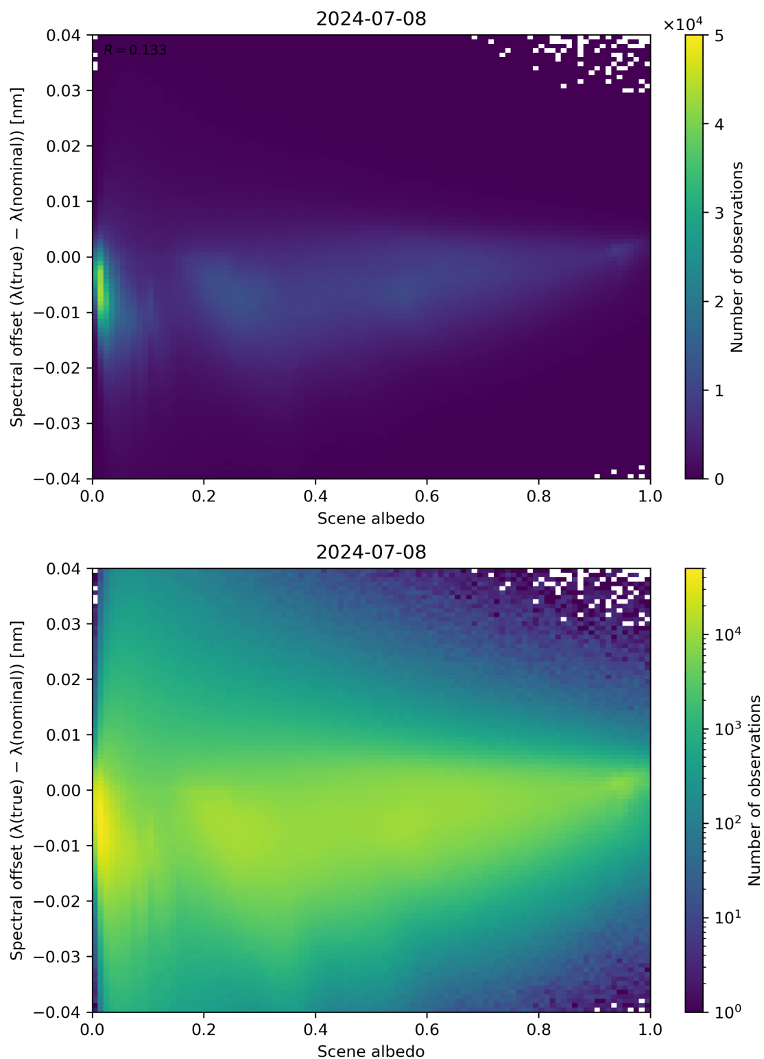
Figure 107: Scatter density plot of “Scene albedo” against “Spectral offset ( \lambda(\text{true}) - \lambda(\text{nominal}) )” for 2024-07-07 to 2024-07-09.
