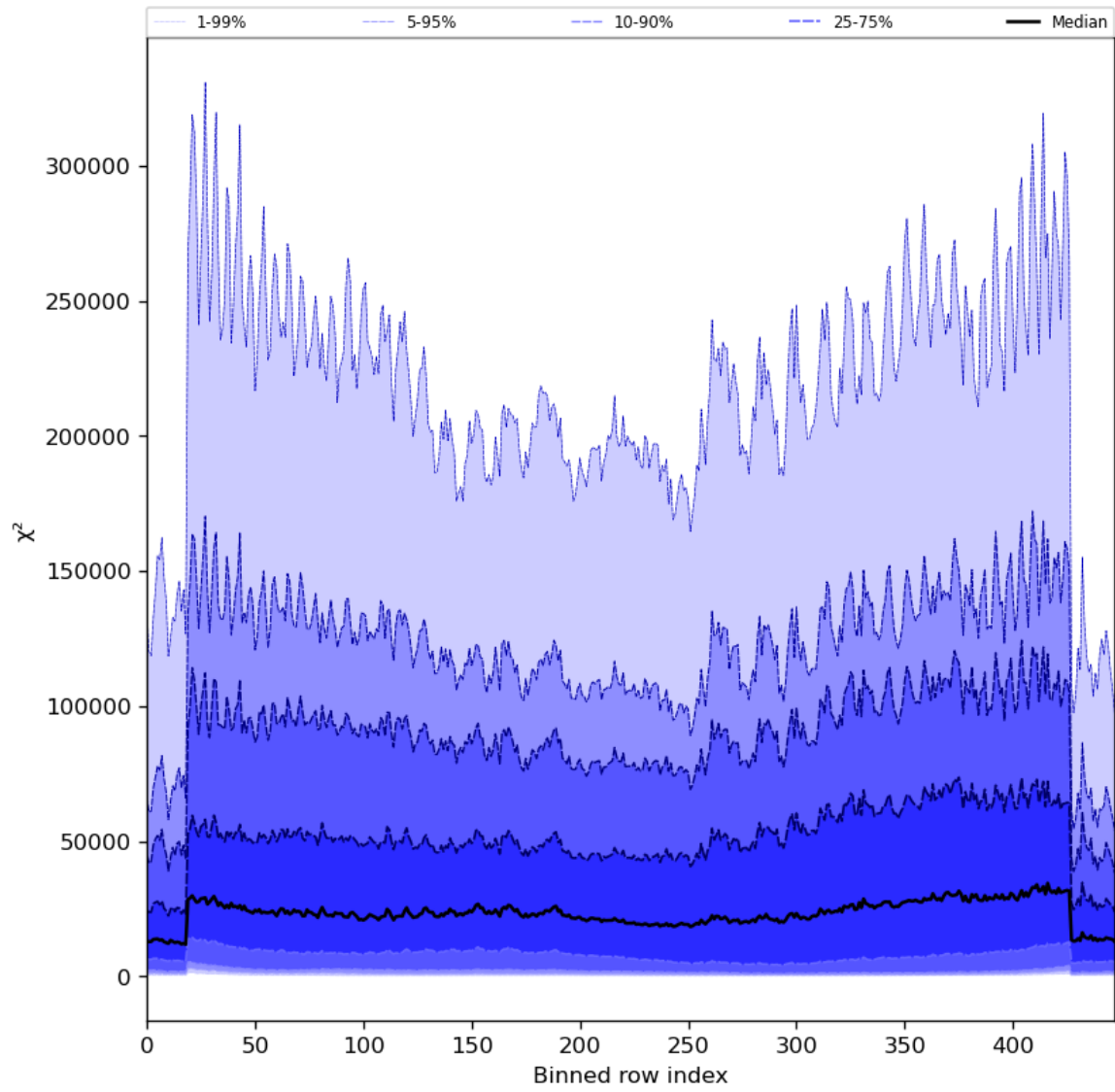
Figure 55: Along track statistics of “ \chi^2 ” for 2024-07-07 to 2024-07-09
