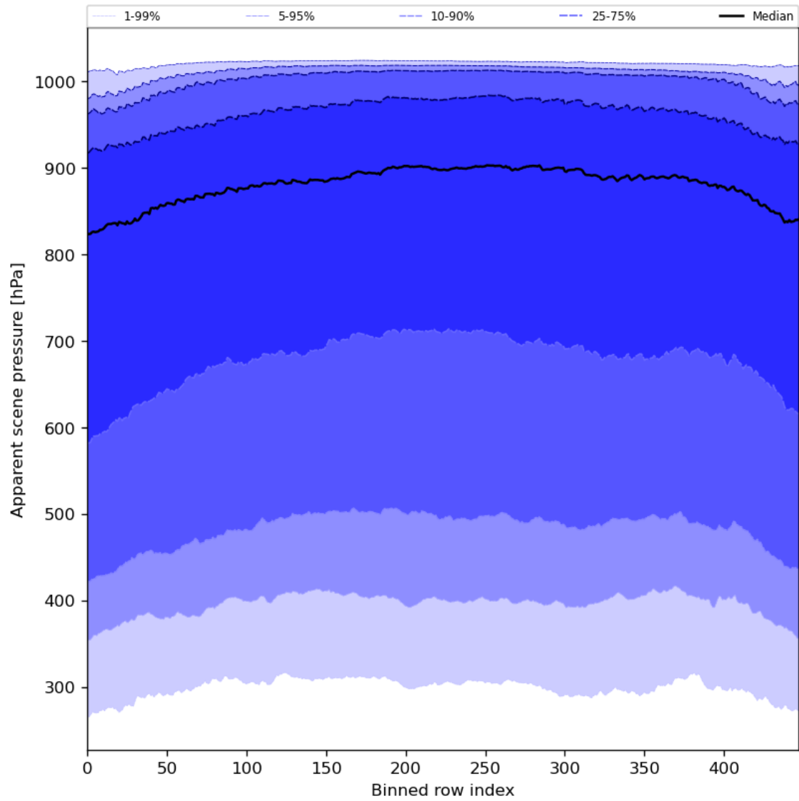
Figure 53: Along track statistics of “Apparent scene pressure” for 2024-07-07 to 2024-07-09
