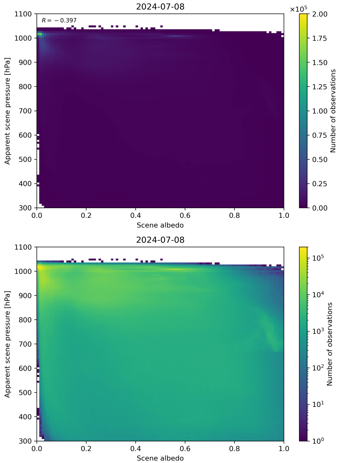
Figure 102: Scatter density plot of “Scene albedo” against “Apparent scene pressure” for 2024-07-07 to 2024-07-09.
