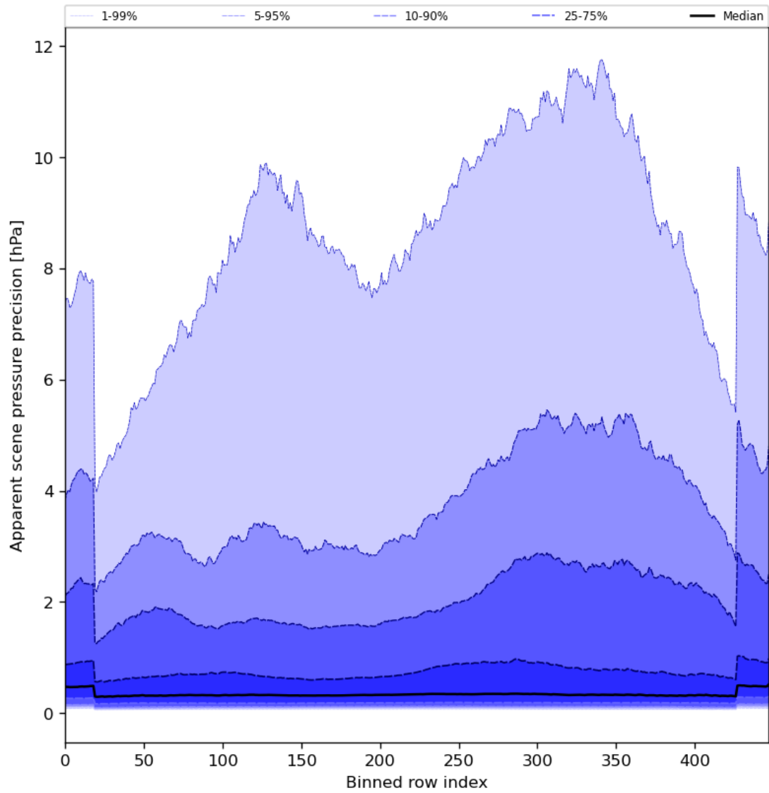
Figure 54: Along track statistics of “Apparent scene pressure precision” for 2024-07-07 to 2024-07-09
