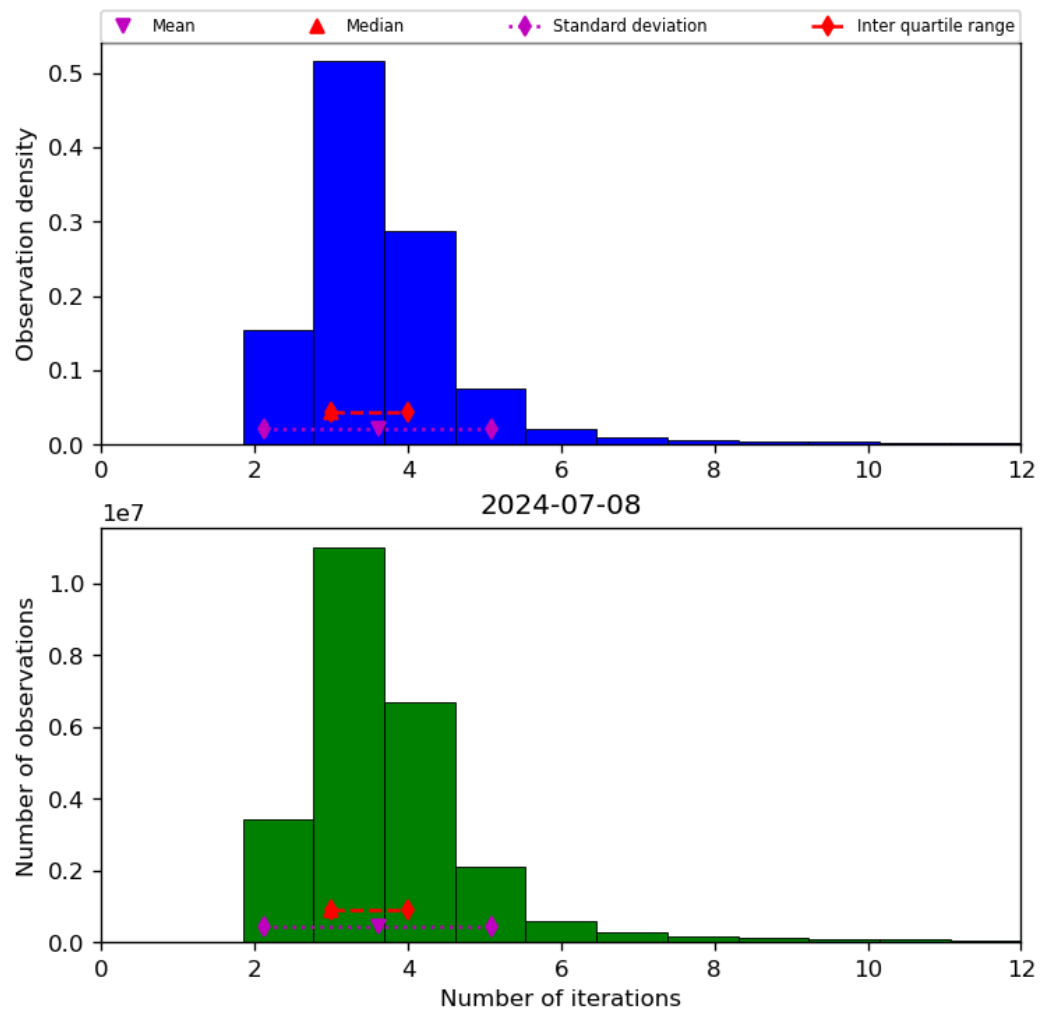
Figure 39: Histogram of “Number of iterations” for 2024-07-07 to 2024-07-09
