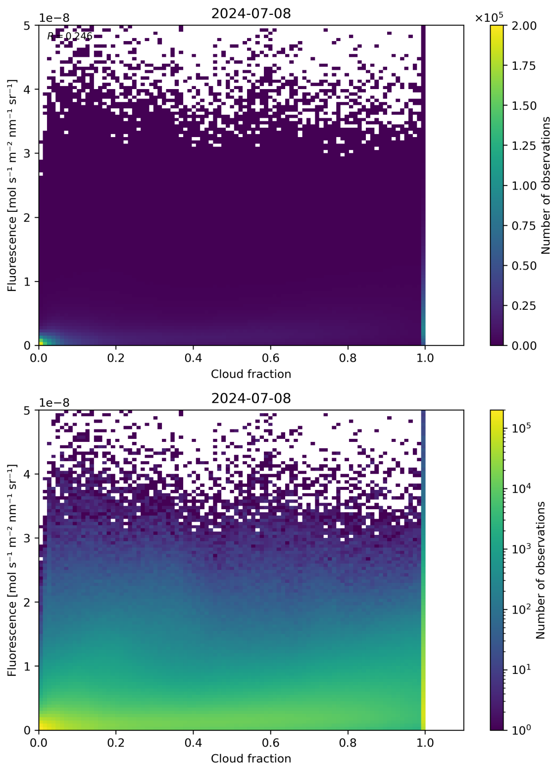
Figure 72: Scatter density plot of “Cloud fraction” against “Fluorescence” for 2024-07-07 to 2024-07-09.
