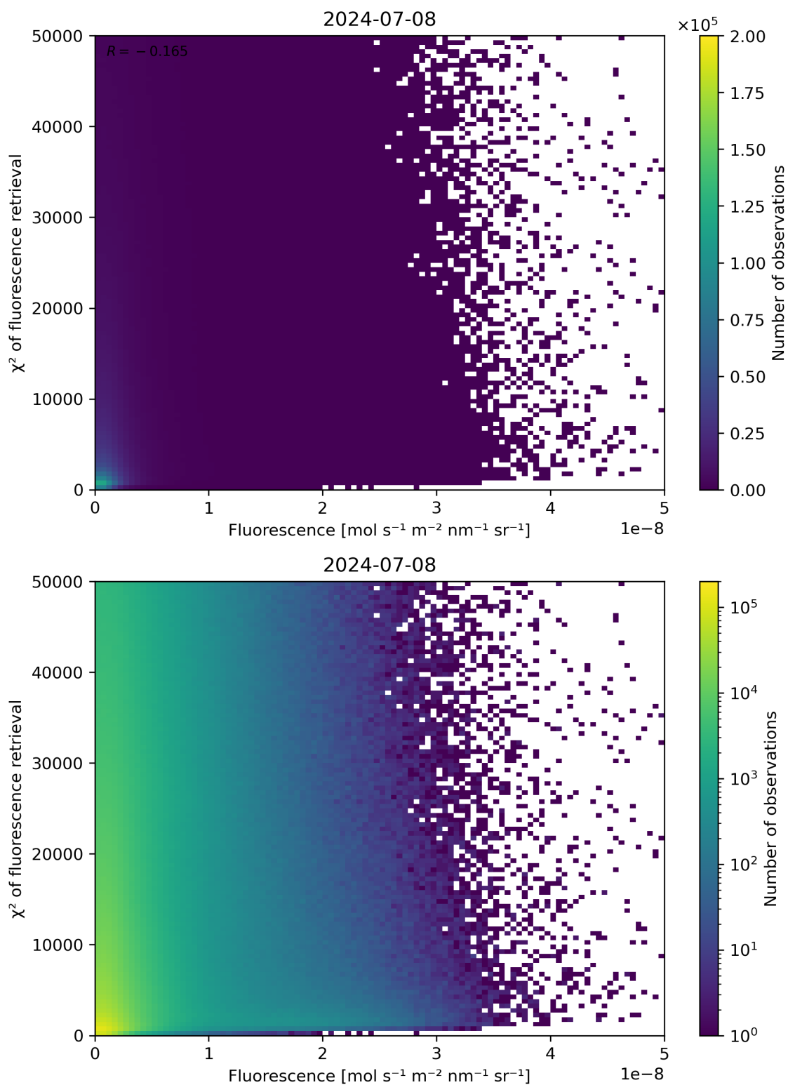
Figure 85: Scatter density plot of “Fluorescence” against “ \chi^2 of fluorescence retrieval” for 2024-07-07 to 2024-07-09.
