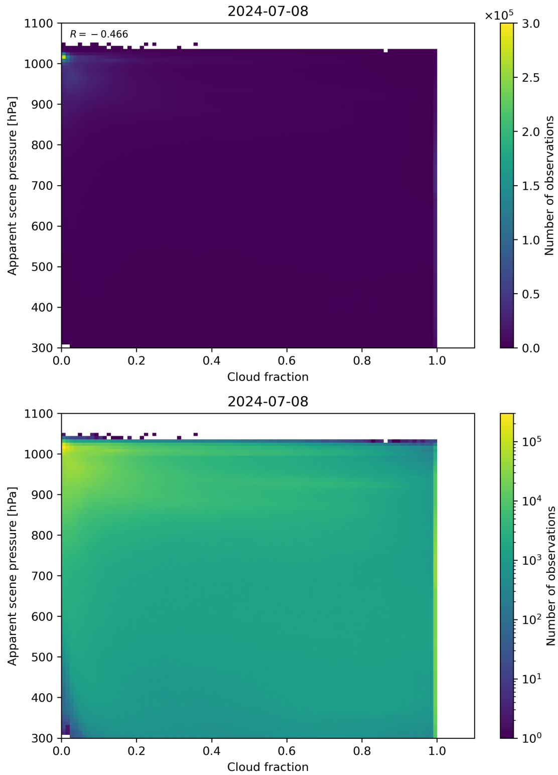
Figure 70: Scatter density plot of “Cloud fraction” against “Apparent scene pressure” for 2024-07-07 to 2024-07-09.
