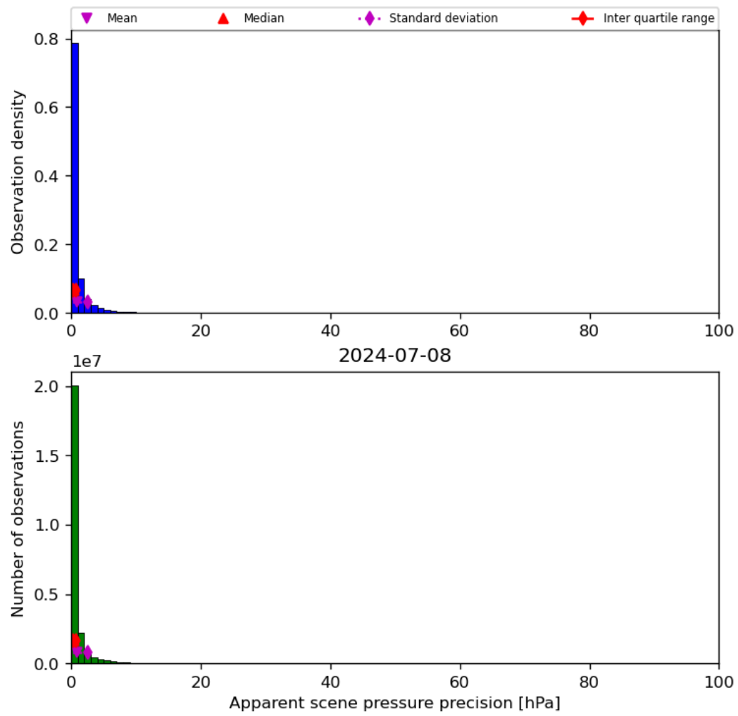
Figure 37: Histogram of “Apparent scene pressure precision” for 2024-07-07 to 2024-07-09
