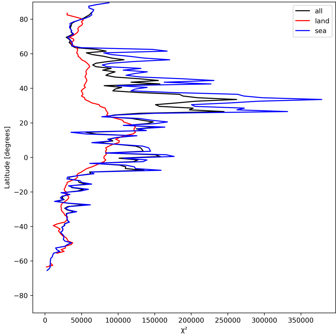
Figure 21: Zonal average of “ \chi^2 ” for 2024-07-07 to 2024-07-09.
