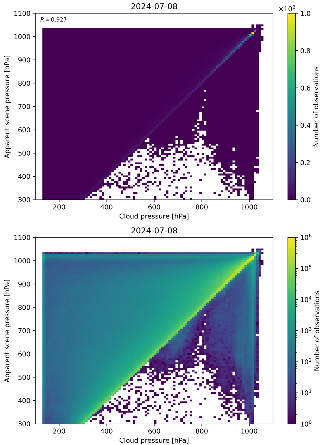
Figure 77: Scatter density plot of “Cloud pressure” against “Apparent scene pressure” for 2024-07-07 to 2024-07-09.
