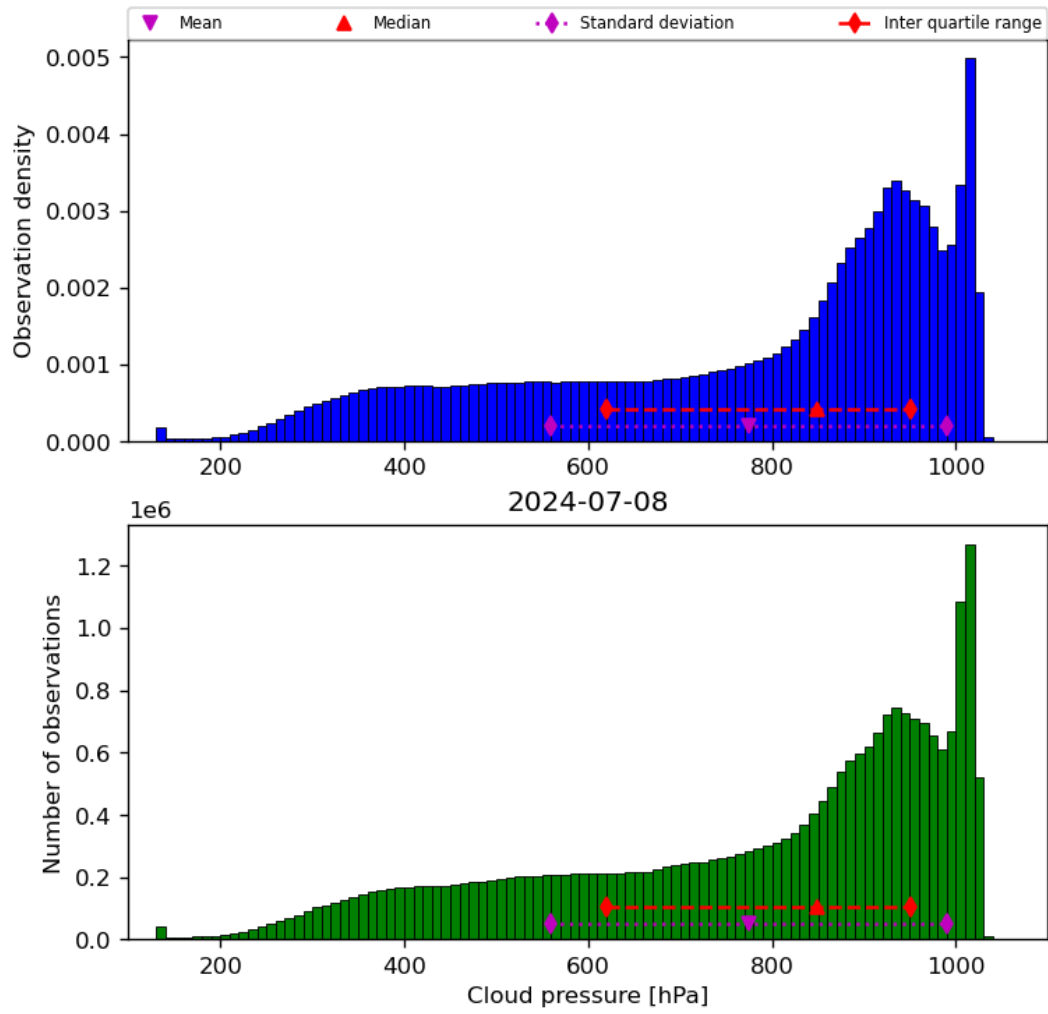
Figure 30: Histogram of “Cloud pressure” for 2024-07-07 to 2024-07-09
