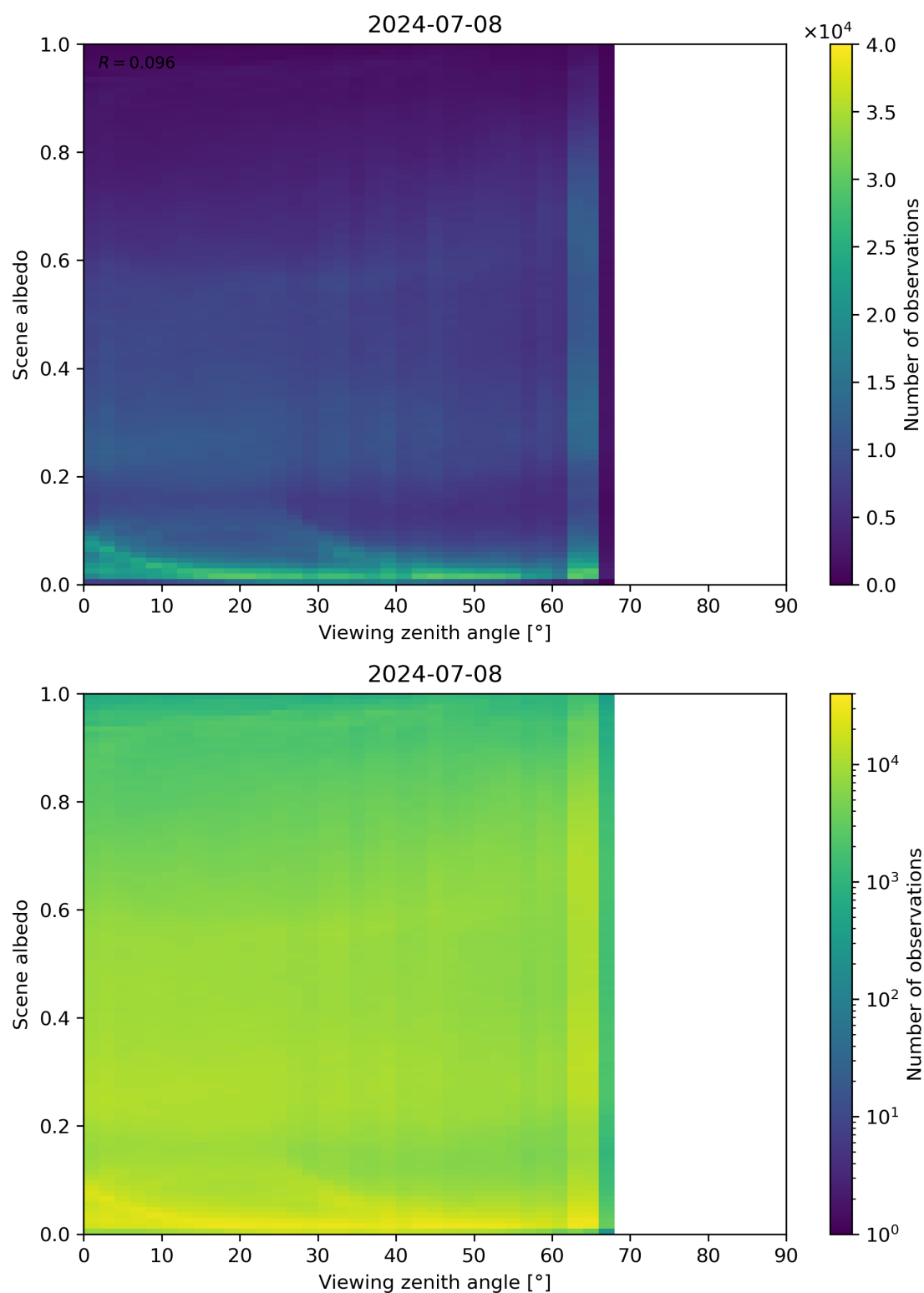
Figure 126: Scatter density plot of “Viewing zenith angle” against “Scene albedo” for 2024-07-07 to 2024-07-09.
