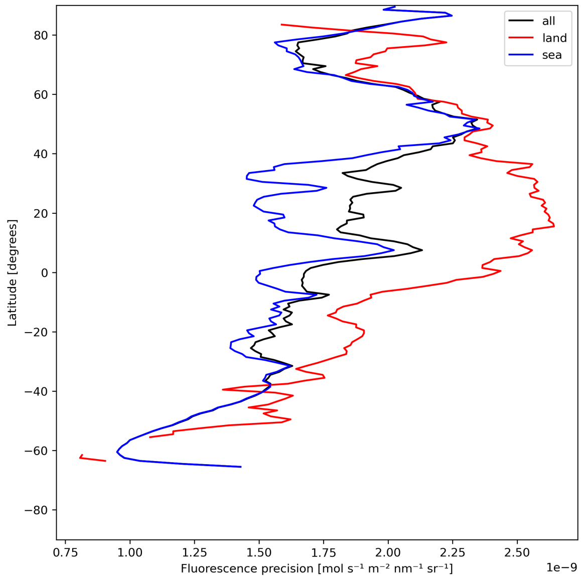
Figure 24: Zonal average of “Fluorescence precision” for 2024-07-07 to 2024-07-09.
