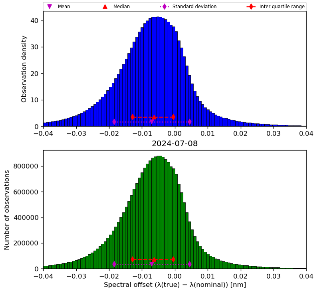
Figure 45: Histogram of “Spectral offset ( \lambda(\text{true}) - \lambda(\text{nominal}) )” for 2024-07-07 to 2024-07-09
