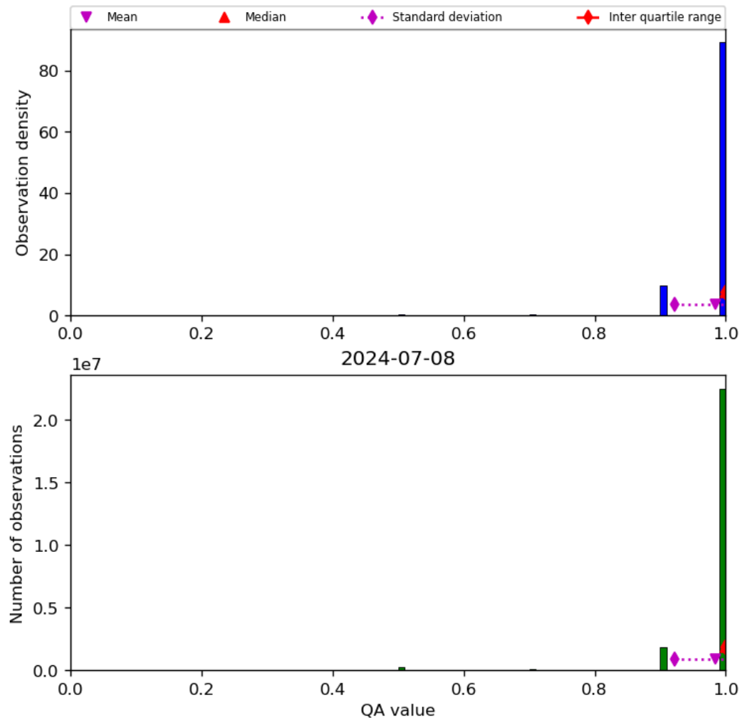
Figure 29: Histogram of “QA value” for 2024-07-07 to 2024-07-09
