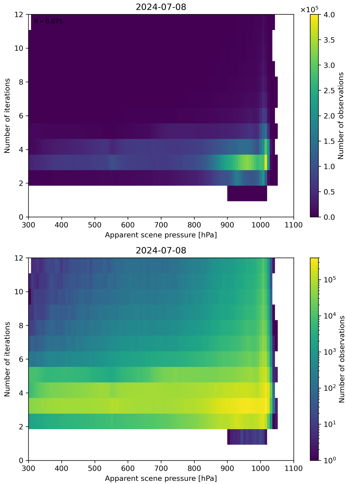
Figure 65: Scatter density plot of “Apparent scene pressure” against “Number of iterations” for 2024-07-07 to 2024-07-09.
