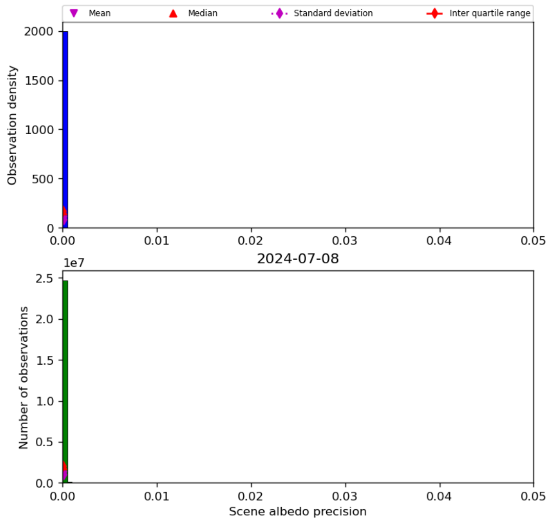
Figure 35: Histogram of “Scene albedo precision” for 2024-07-07 to 2024-07-09
