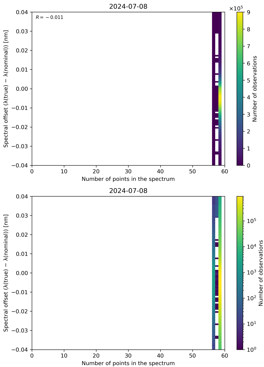
Figure 101: Scatter density plot of “Number of points in the spectrum” against “Spectral offset ( \lambda(\text{true}) - \lambda(\text{nominal}) )” for 2024-07-07 to 2024-07-09.
