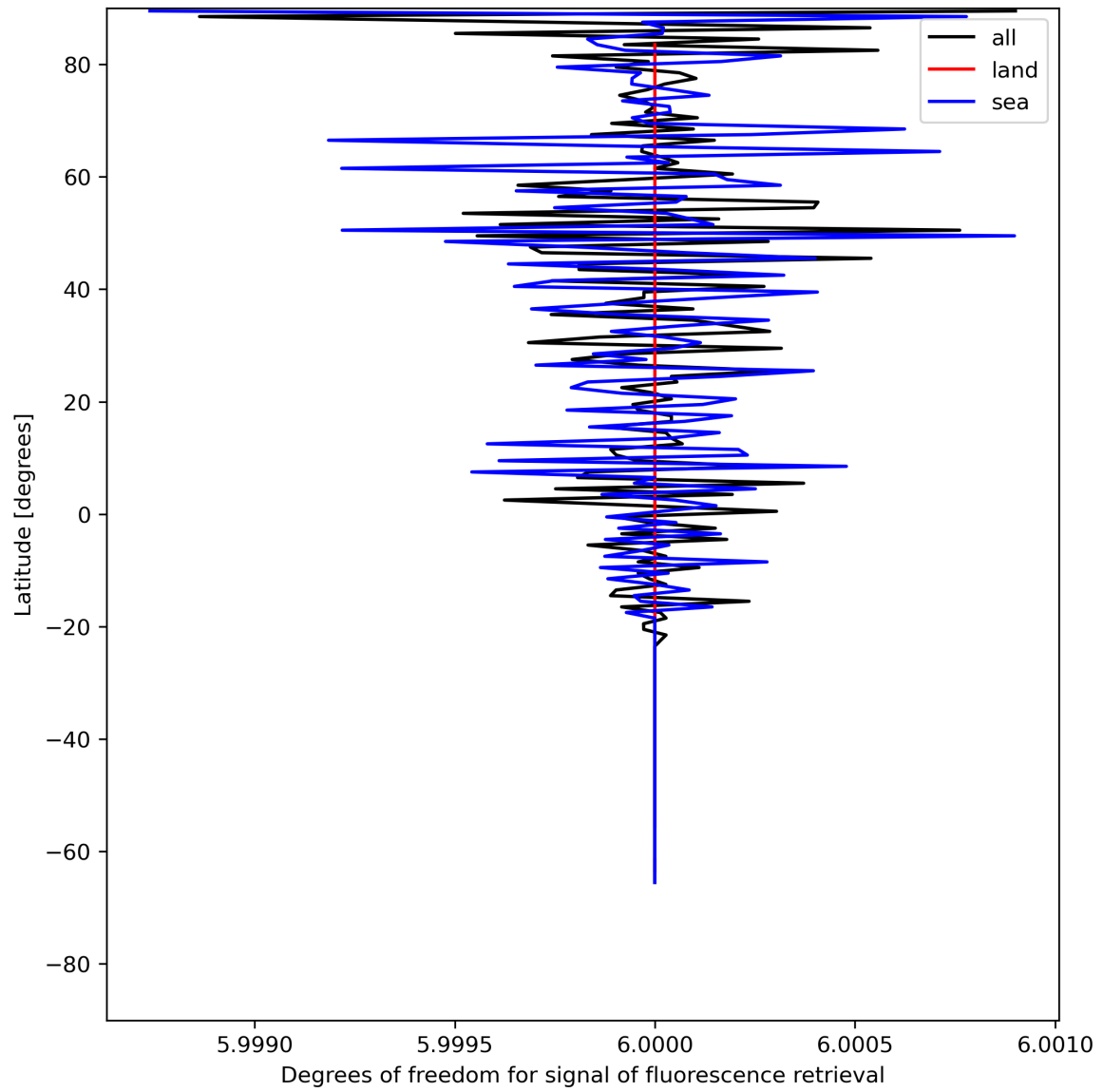
Figure 26: Zonal average of “Degrees of freedom for signal of fluorescence retrieval” for 2024-07-07 to 2024-07-09.
