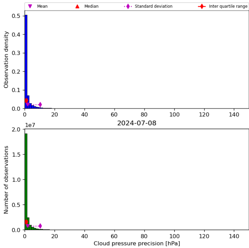
Figure 31: Histogram of “Cloud pressure precision” for 2024-07-07 to 2024-07-09
