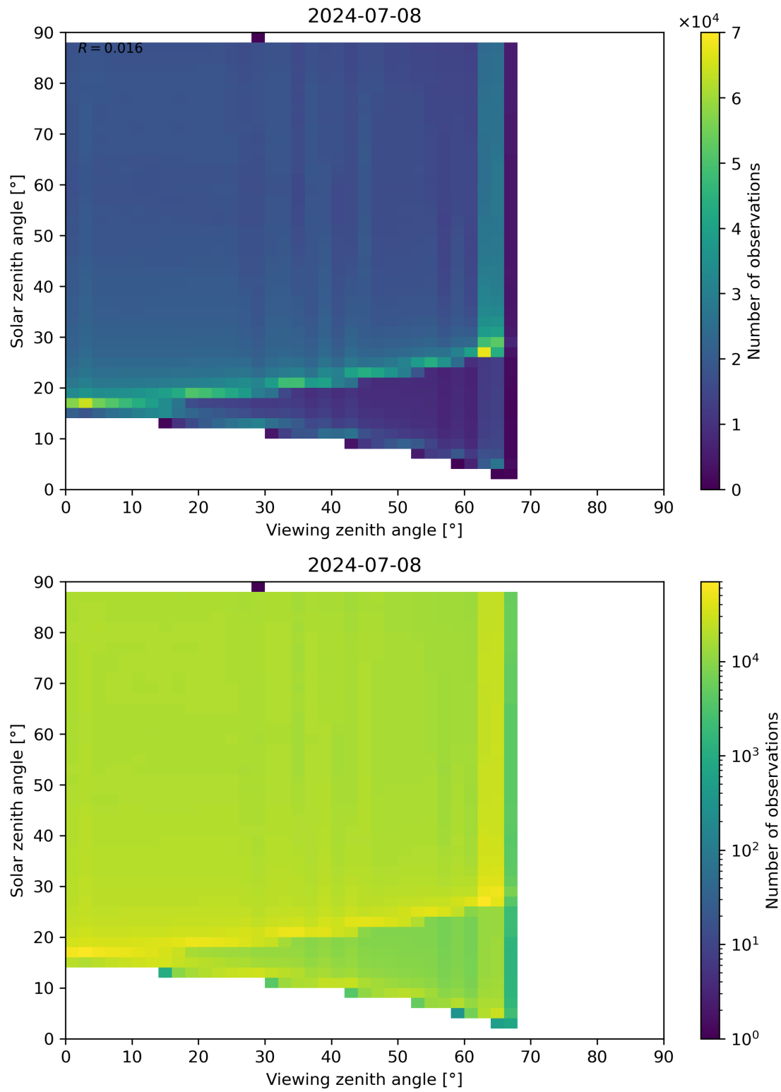
Figure 127: Scatter density plot of “Viewing zenith angle” against “Solar zenith angle” for 2024-07-07 to 2024-07-09.
