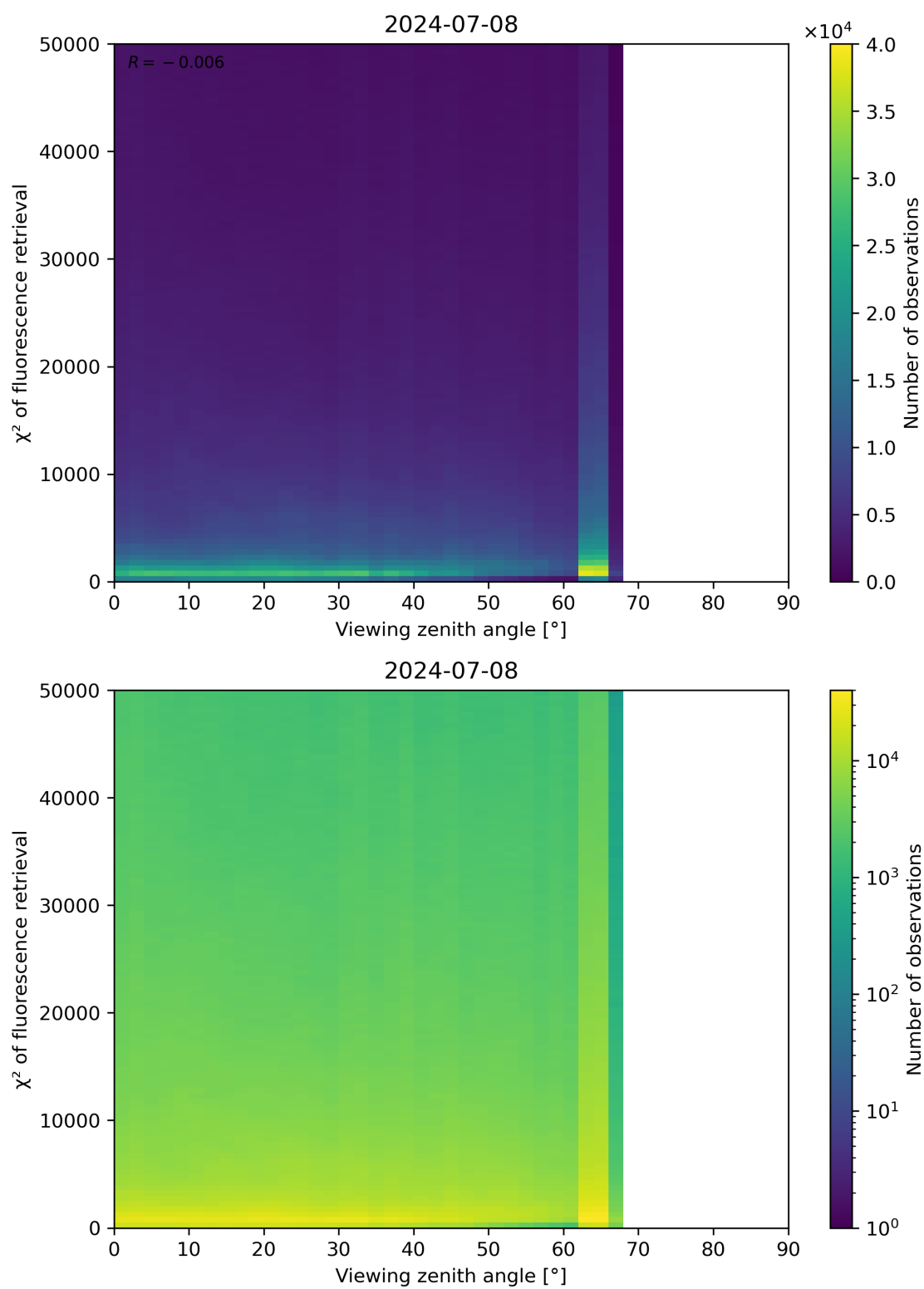
Figure 119: Scatter density plot of “Viewing zenith angle” against “ \chi^2 of fluorescence retrieval” for 2024-07-07 to 2024-07-09.
