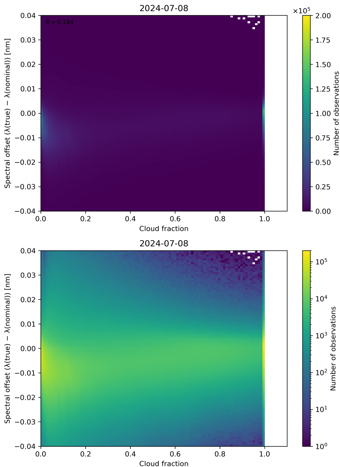
Figure 76: Scatter density plot of “Cloud fraction” against “Spectral offset ( \lambda(\text{true}) - \lambda(\text{nominal}) )” for 2024-07-07 to 2024-07-09.
