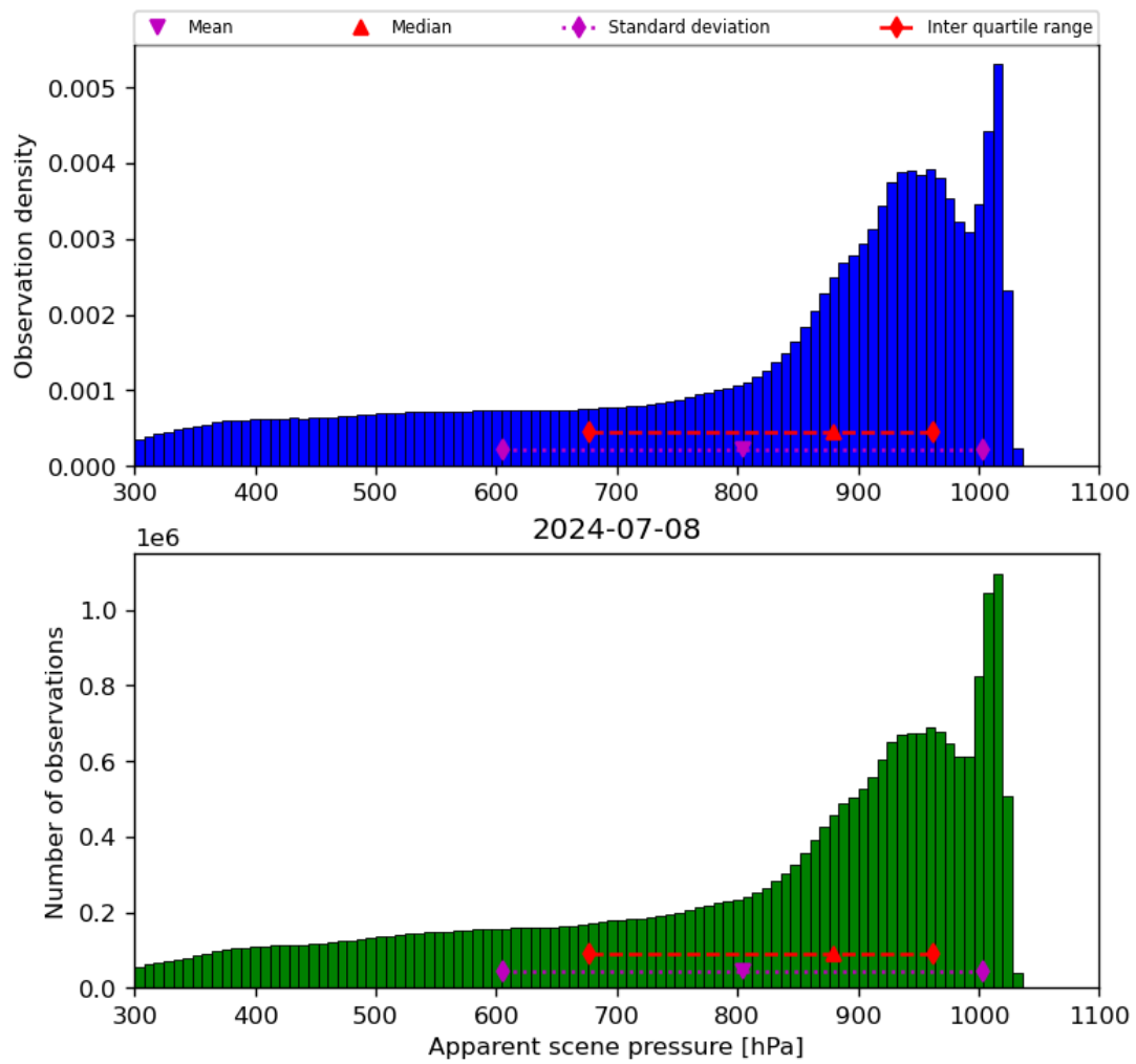
Figure 36: Histogram of “Apparent scene pressure” for 2024-07-07 to 2024-07-09
