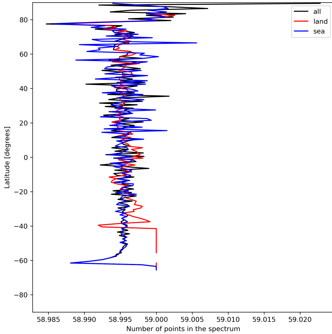
Figure 27: Zonal average of “Number of points in the spectrum” for 2024-07-07 to 2024-07-09.
