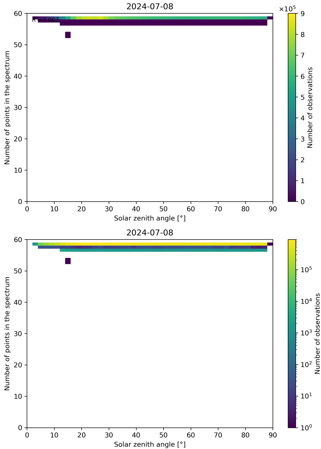
Figure 115: Scatter density plot of “Solar zenith angle” against “Number of points in the spectrum” for 2024-07-07 to 2024-07-09.
