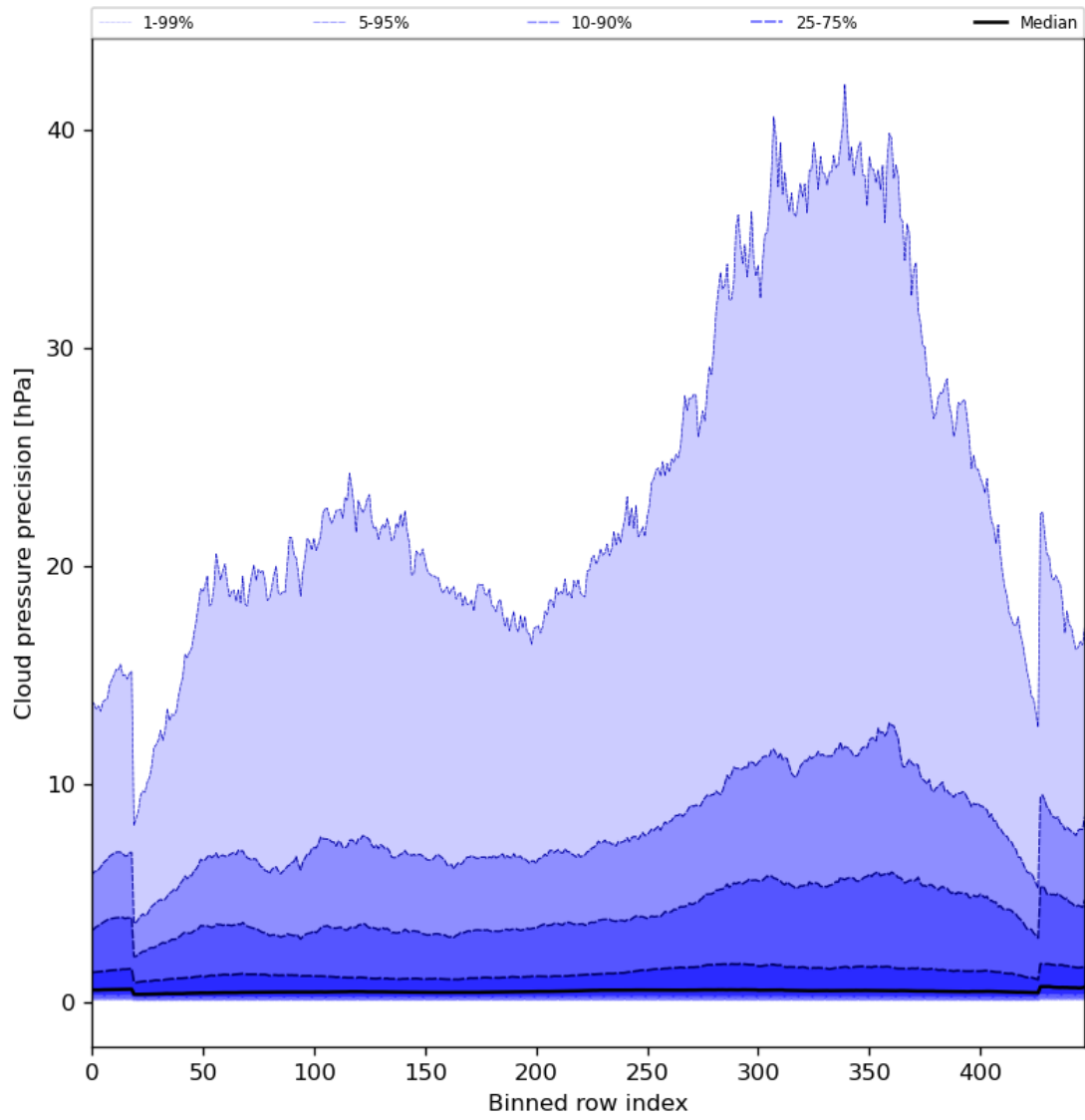
Figure 48: Along track statistics of “Cloud pressure precision” for 2024-07-07 to 2024-07-09
