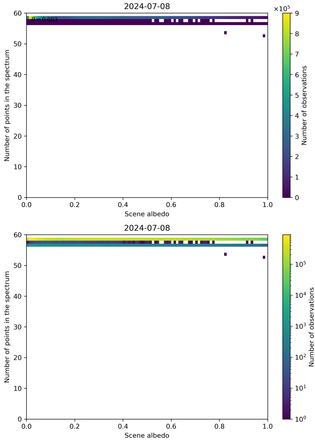
Figure 106: Scatter density plot of “Scene albedo” against “Number of points in the spectrum” for 2024-07-07 to 2024-07-09.
