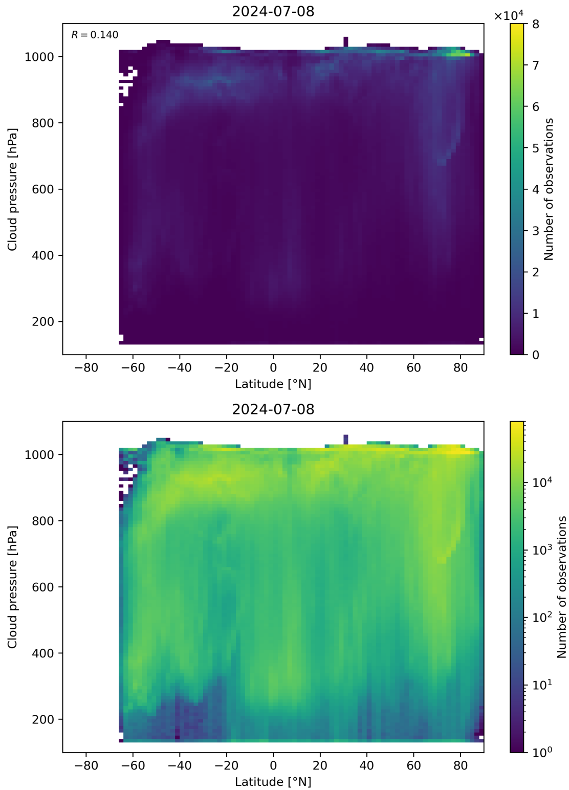
Figure 91: Scatter density plot of “Latitude” against “Cloud pressure” for 2024-07-07 to 2024-07-09.
