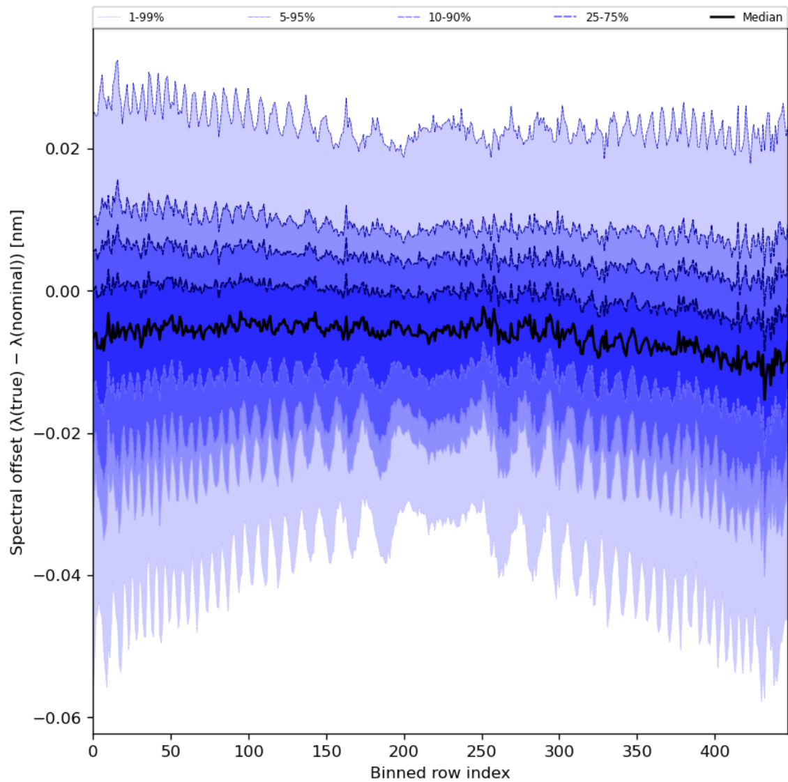
Figure 62: Along track statistics of “Spectral offset ( \lambda(\text{true}) - \lambda(\text{nominal}) )” for 2024-07-07 to 2024-07-09
