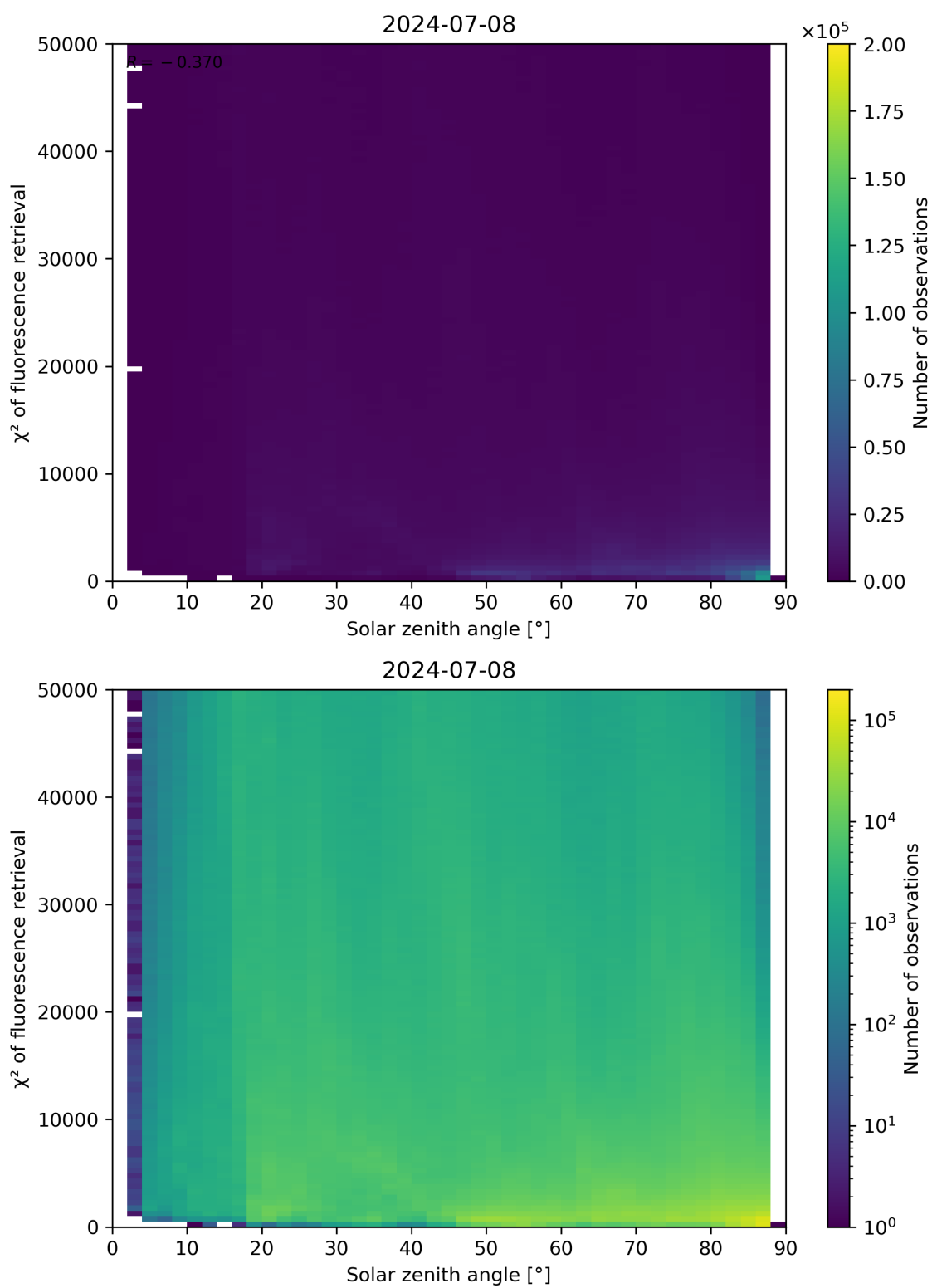
Figure 109: Scatter density plot of “Solar zenith angle” against “ \chi^2 of fluorescence retrieval” for 2024-07-07 to 2024-07-09.
