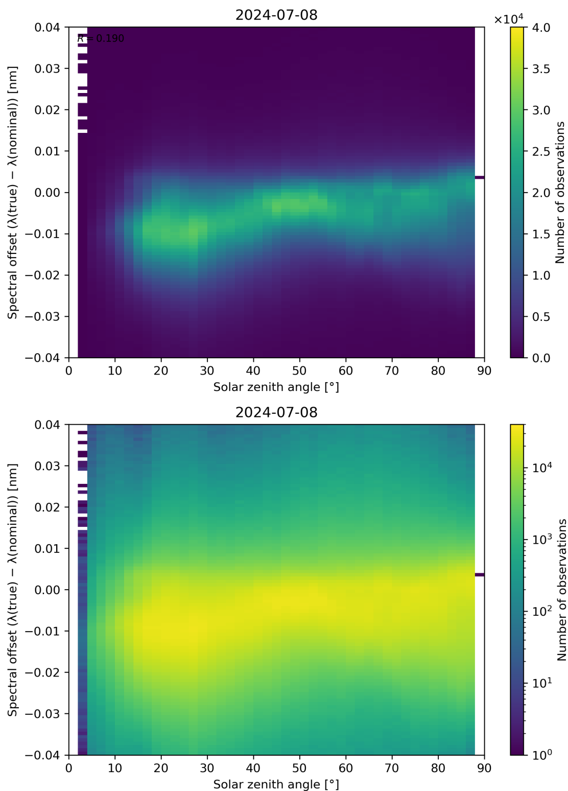
Figure 117: Scatter density plot of “Solar zenith angle” against “Spectral offset ( \lambda(\text{true}) - \lambda(\text{nominal}) )” for 2024-07-07 to 2024-07-09.
