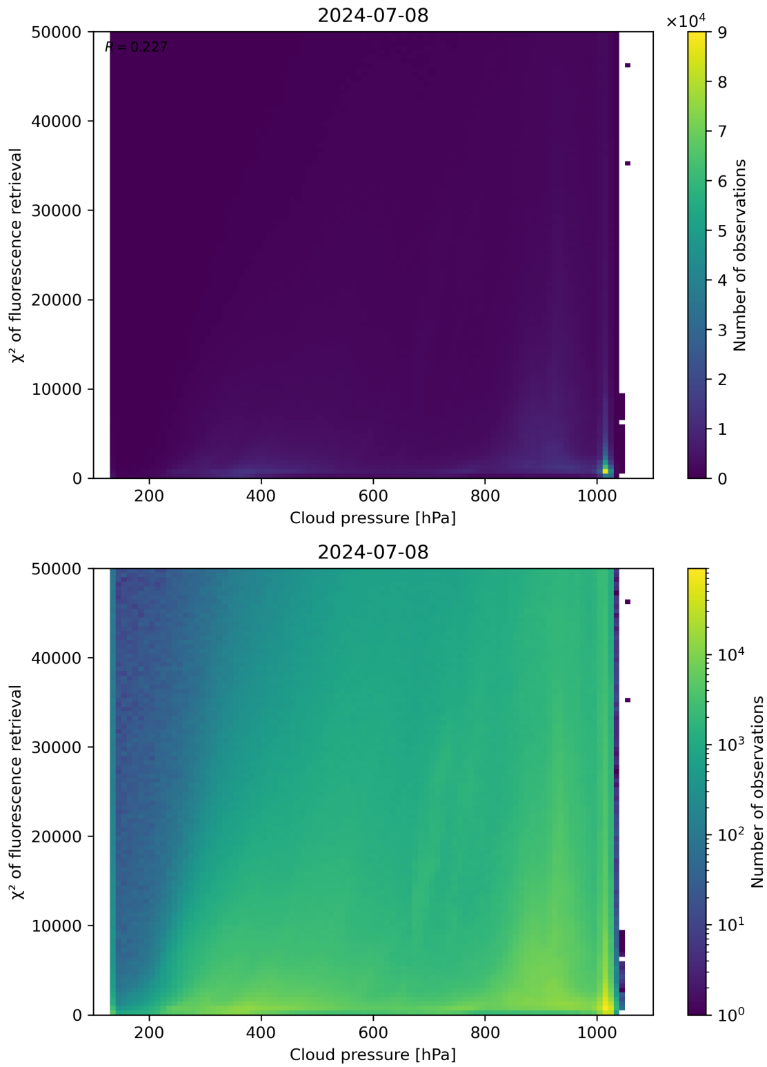
Figure 78: Scatter density plot of “Cloud pressure” against “ \chi^2 of fluorescence retrieval” for 2024-07-07 to 2024-07-09.
