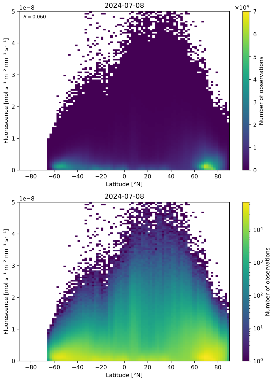
Figure 92: Scatter density plot of “Latitude” against “Fluorescence” for 2024-07-07 to 2024-07-09.
