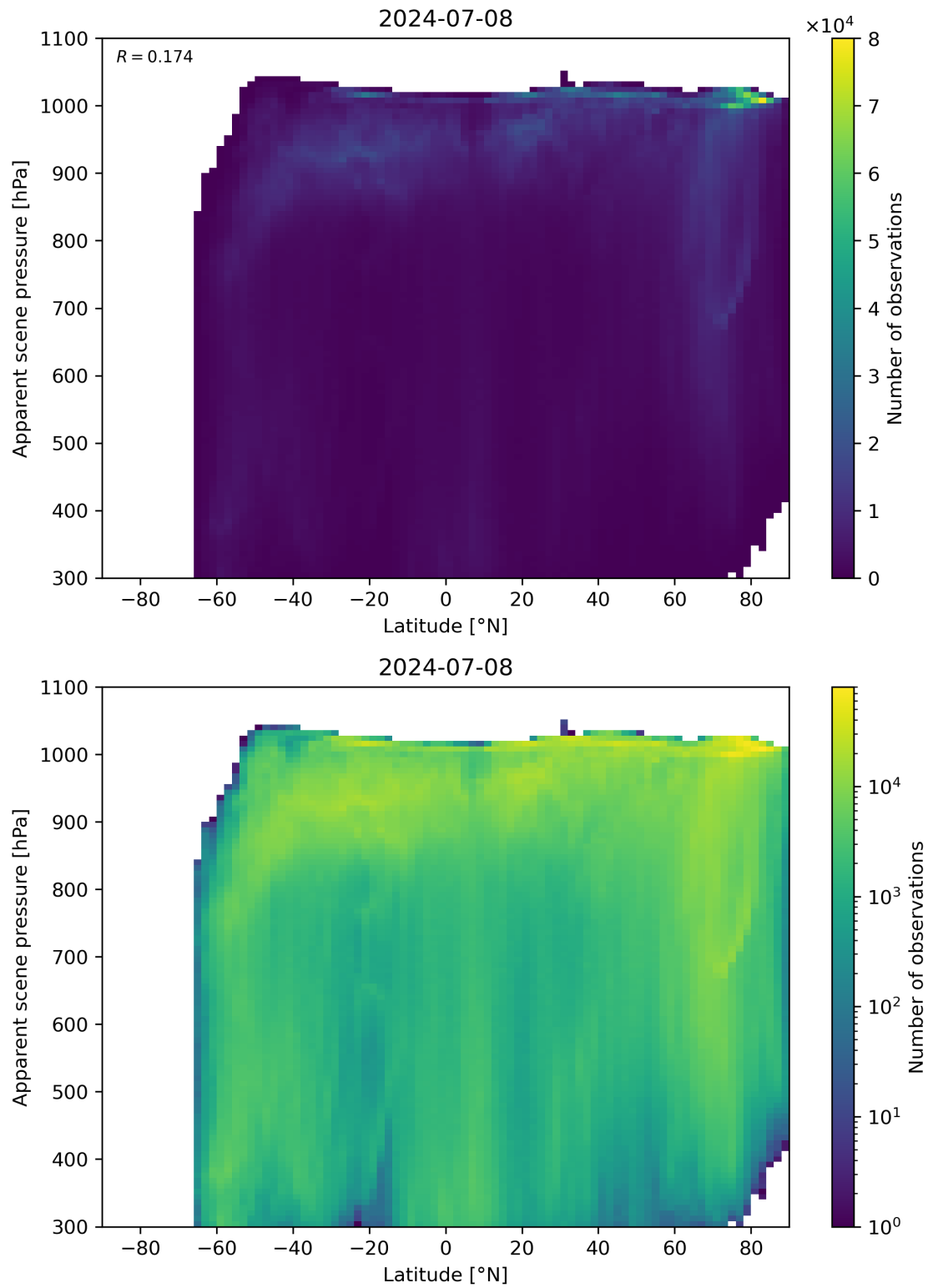
Figure 88: Scatter density plot of “Latitude” against “Apparent scene pressure” for 2024-07-07 to 2024-07-09.
