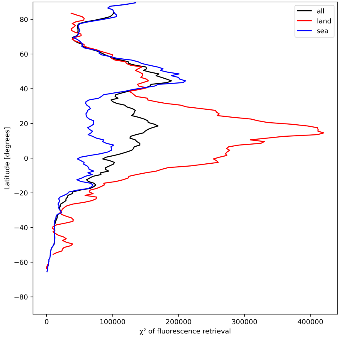
Figure 25: Zonal average of “ \chi^2 of fluorescence retrieval” for 2024-07-07 to 2024-07-09.
