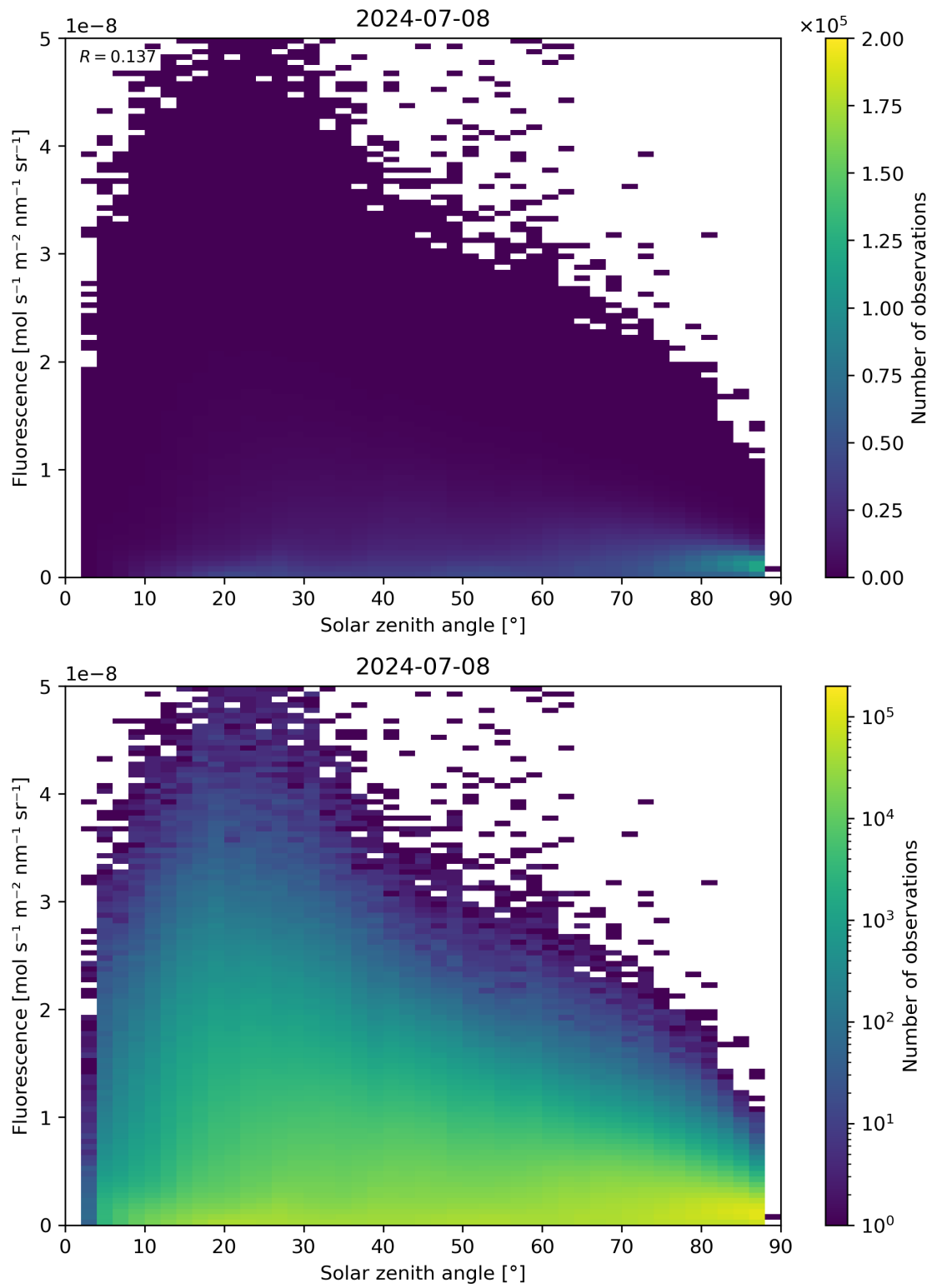
Figure 112: Scatter density plot of “Solar zenith angle” against “Fluorescence” for 2024-07-07 to 2024-07-09.
