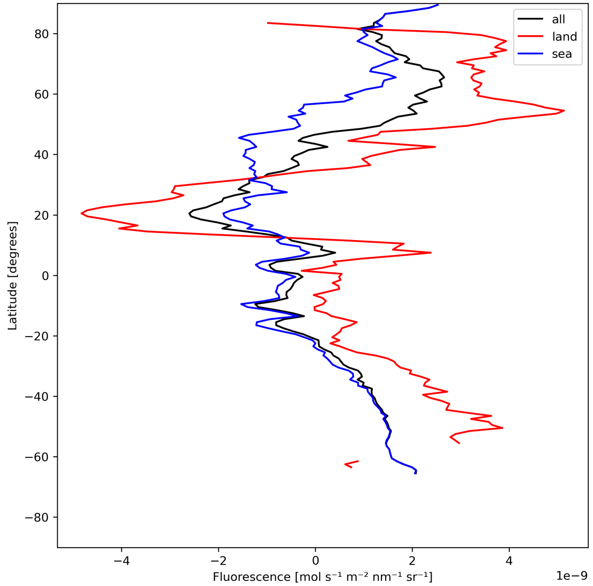
Figure 23: Zonal average of “Fluorescence” for 2024-07-07 to 2024-07-09.
