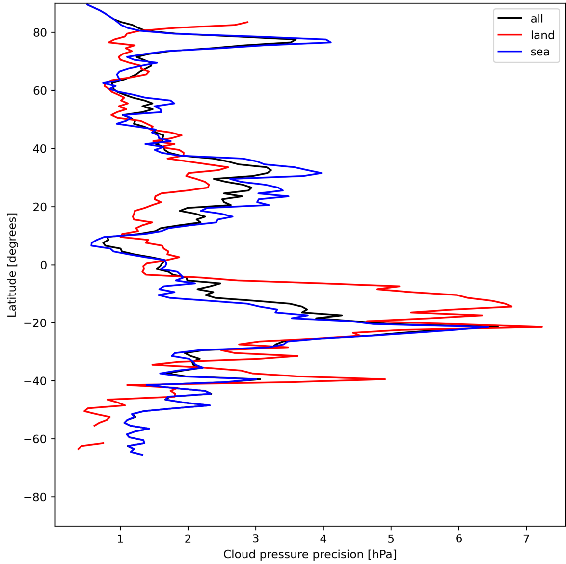
Figure 14: Zonal average of “Cloud pressure precision” for 2024-07-07 to 2024-07-09.
