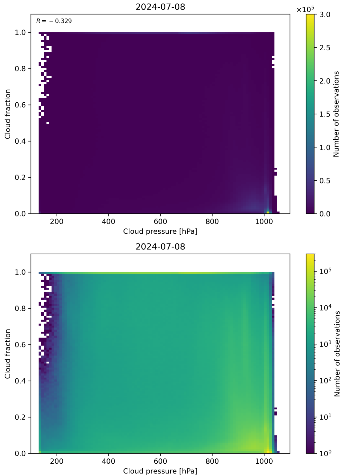
Figure 79: Scatter density plot of “Cloud pressure” against “Cloud fraction” for 2024-07-07 to 2024-07-09.
