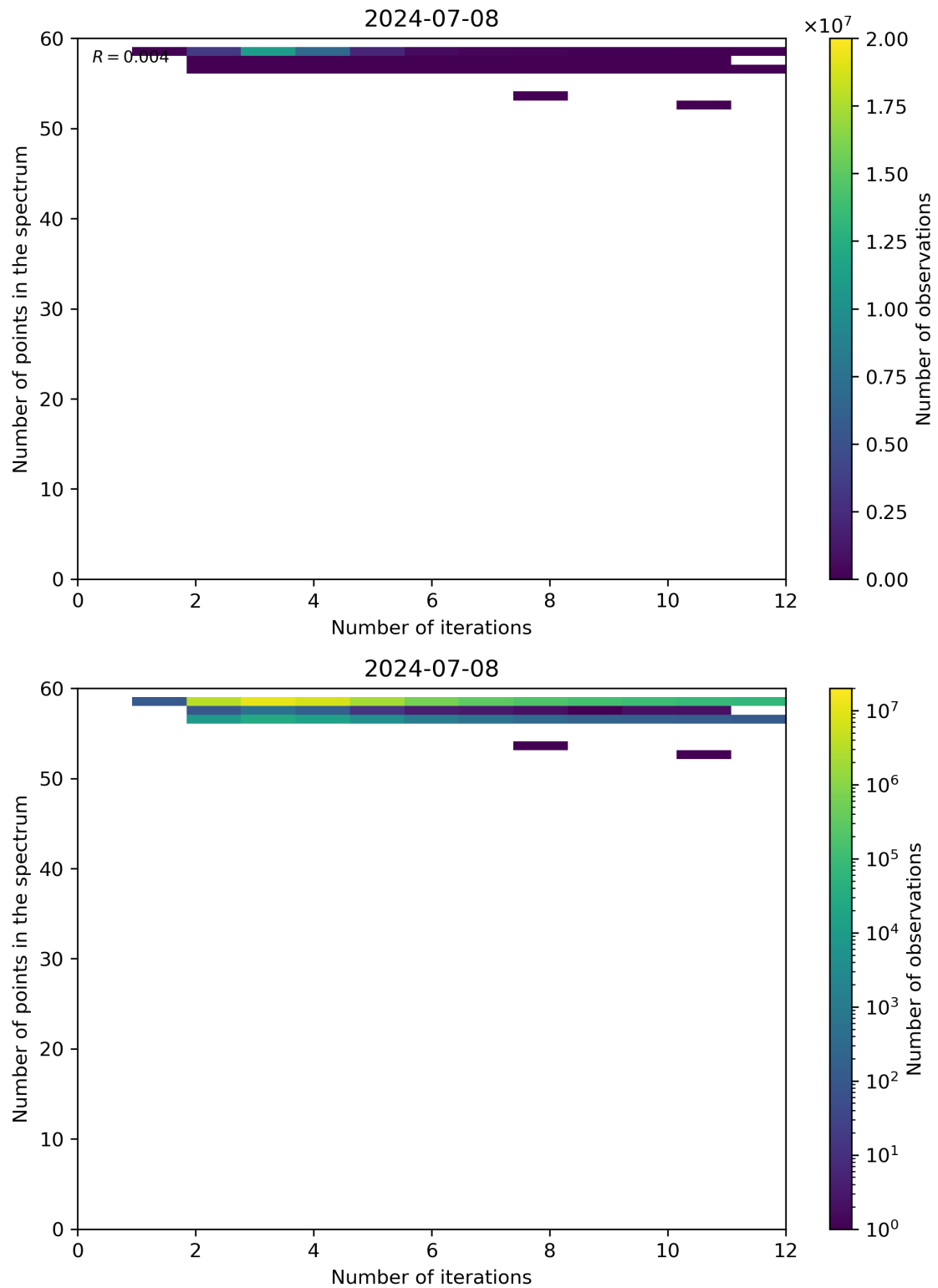
Figure 99: Scatter density plot of “Number of iterations” against “Number of points in the spectrum” for 2024-07-07 to 2024-07-09.
