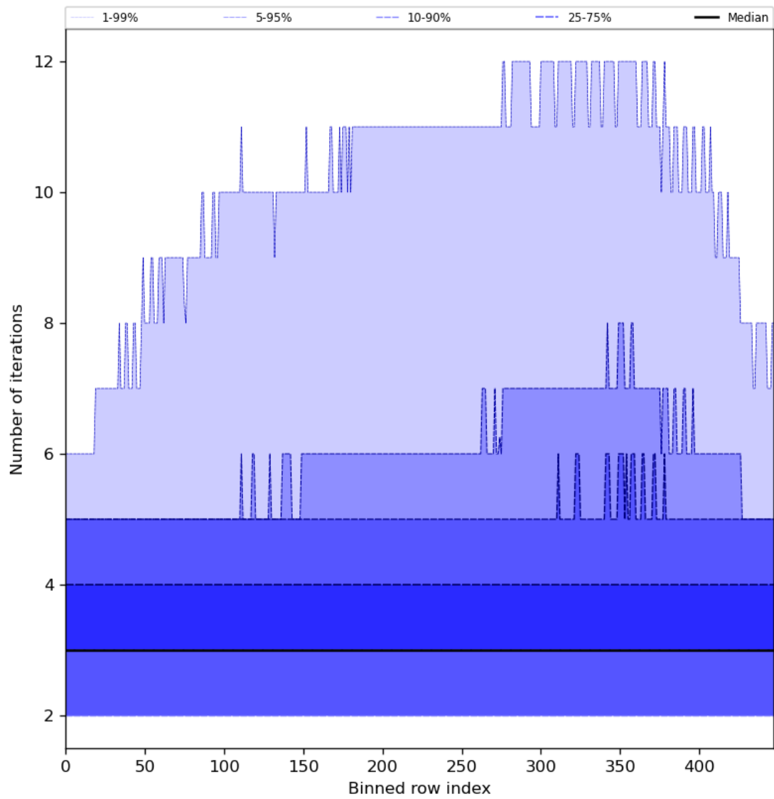
Figure 56: Along track statistics of “Number of iterations” for 2024-07-07 to 2024-07-09
