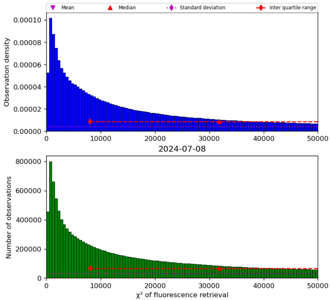
Figure 42: Histogram of “ \chi^2 of fluorescence retrieval” for 2024-07-07 to 2024-07-09
