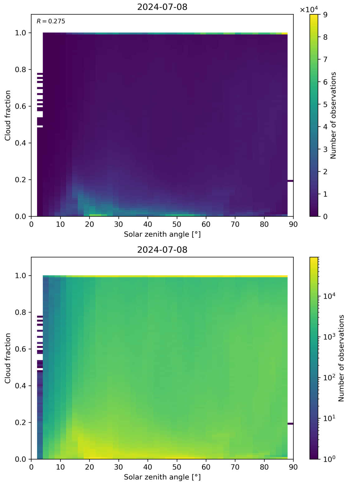
Figure 110: Scatter density plot of “Solar zenith angle” against “Cloud fraction” for 2024-07-07 to 2024-07-09.
