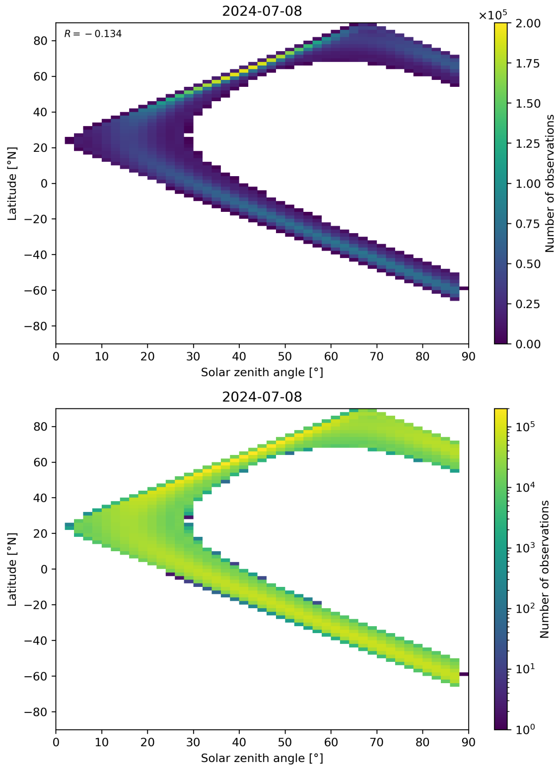
Figure 113: Scatter density plot of “Solar zenith angle” against “Latitude” for 2024-07-07 to 2024-07-09.
