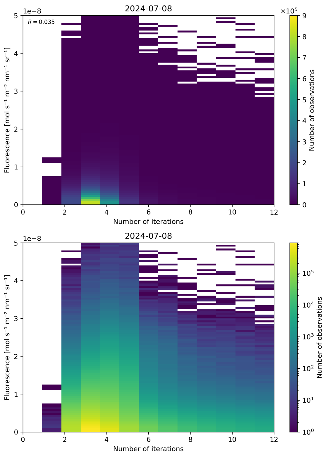
Figure 98: Scatter density plot of “Number of iterations” against “Fluorescence” for 2024-07-07 to 2024-07-09.
