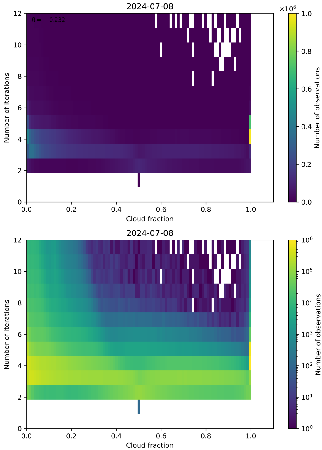
Figure 73: Scatter density plot of “Cloud fraction” against “Number of iterations” for 2024-07-07 to 2024-07-09.
