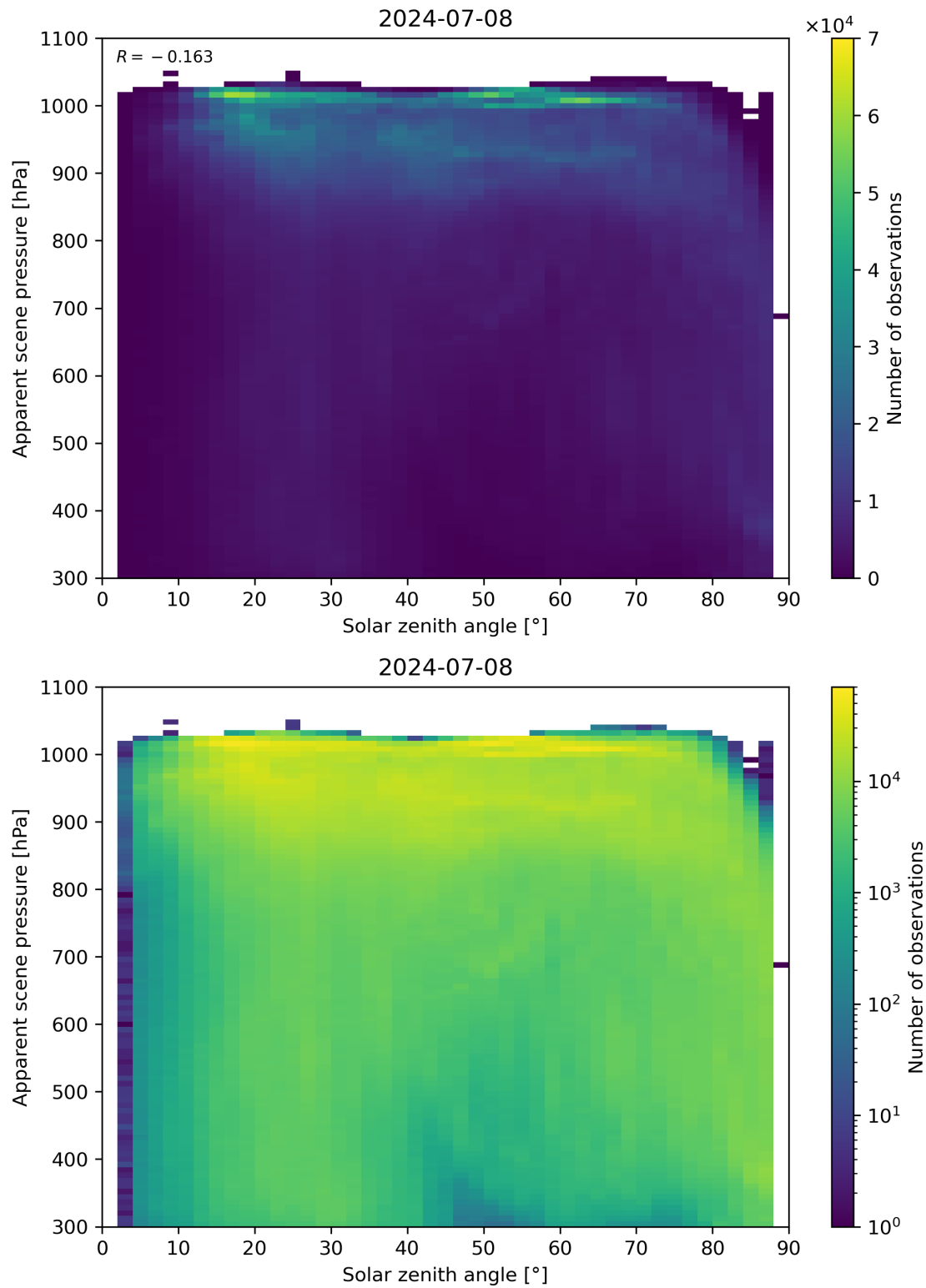
Figure 108: Scatter density plot of “Solar zenith angle” against “Apparent scene pressure” for 2024-07-07 to 2024-07-09.
