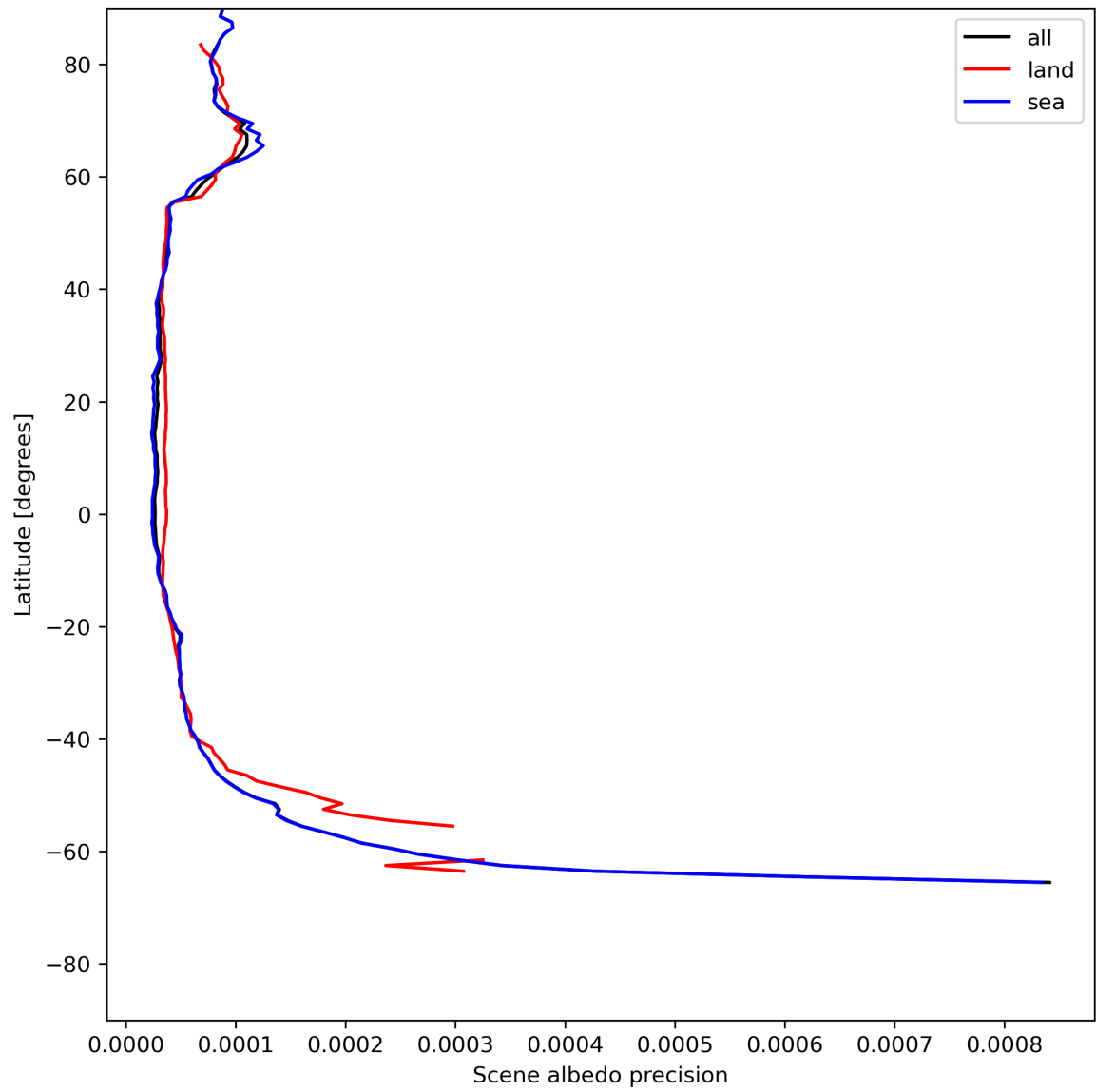
Figure 18: Zonal average of “Scene albedo precision” for 2024-07-07 to 2024-07-09.
