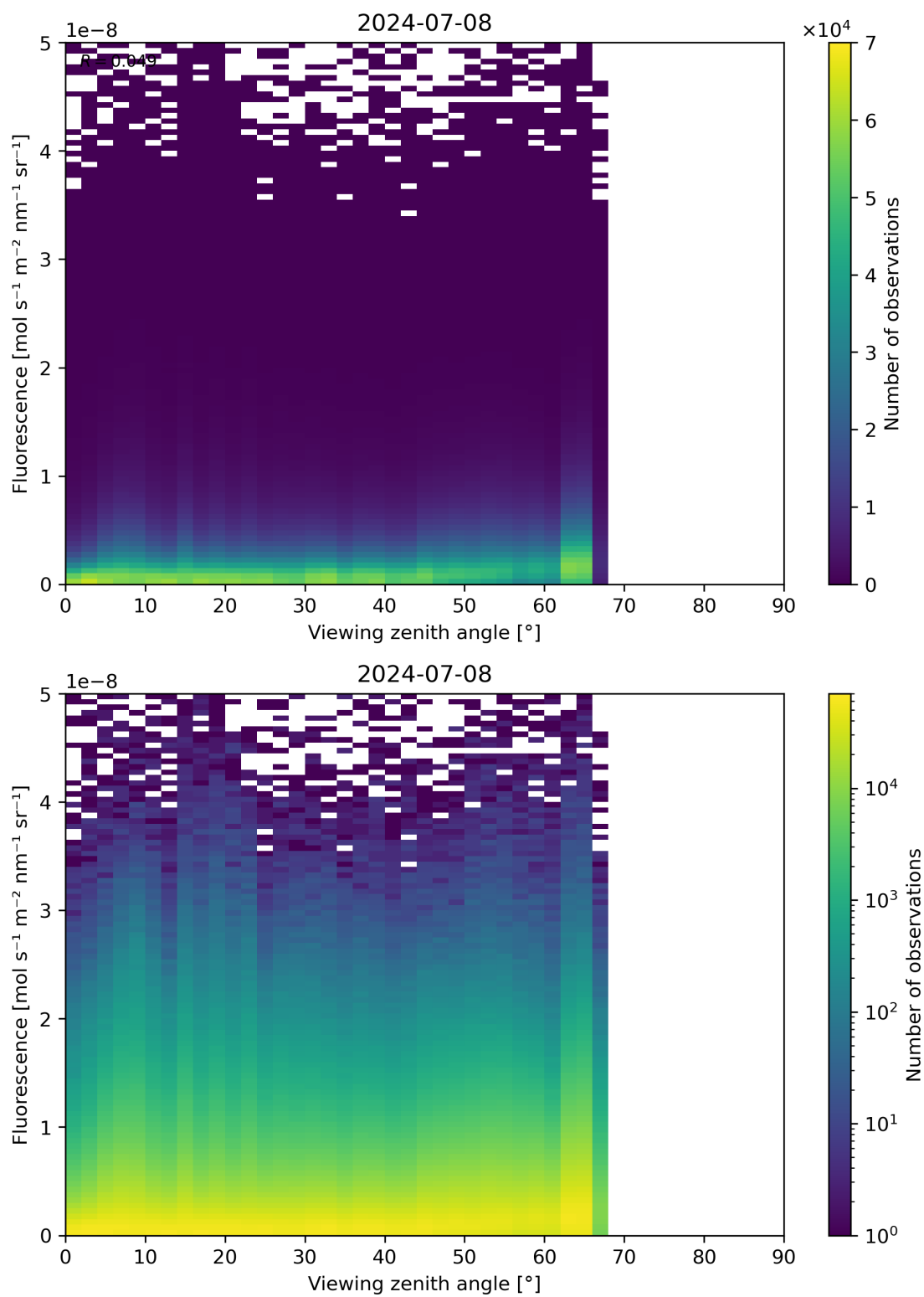
Figure 122: Scatter density plot of “Viewing zenith angle” against “Fluorescence” for 2024-07-07 to 2024-07-09.
