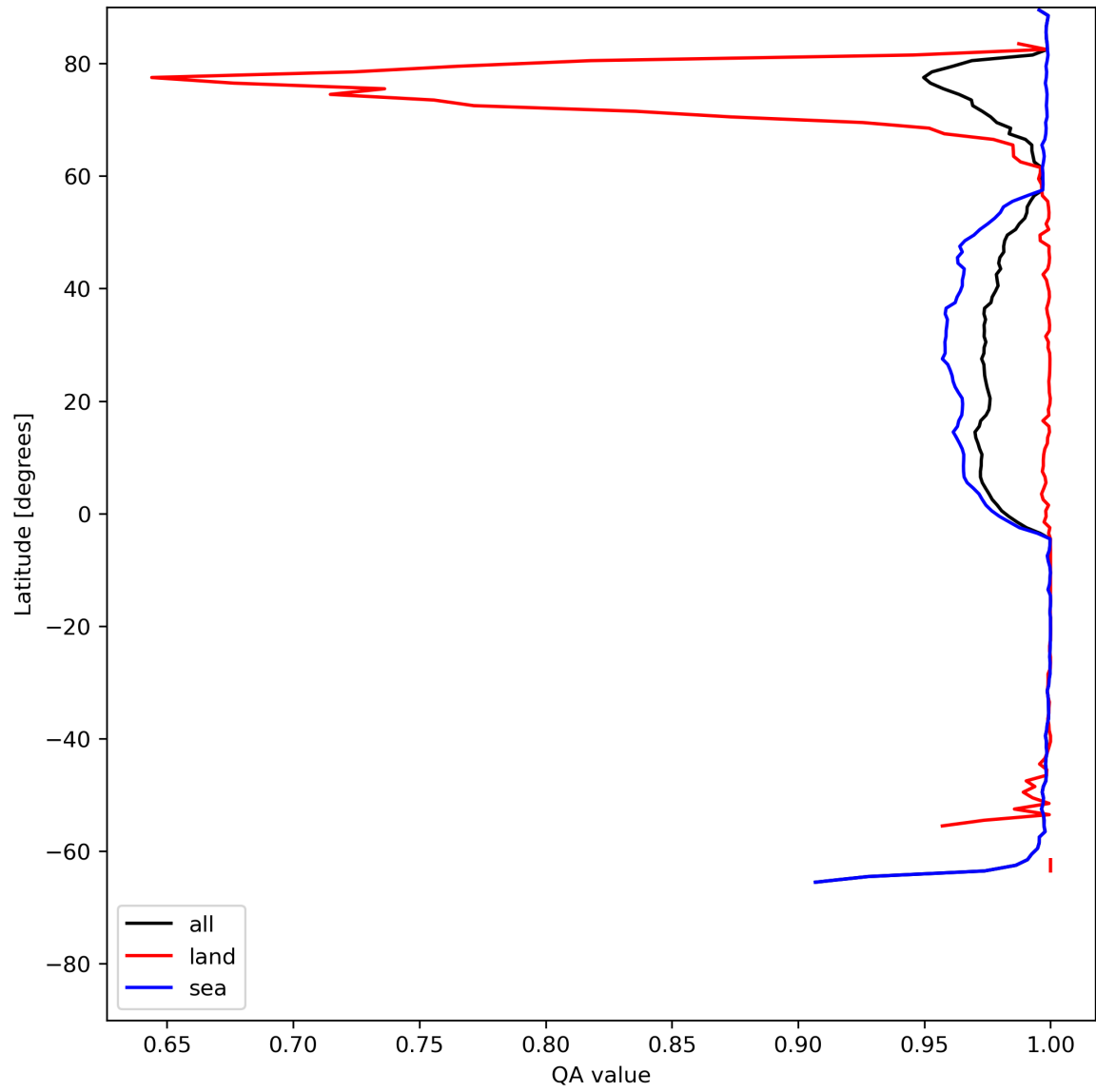
Figure 12: Zonal average of “QA value” for 2024-07-07 to 2024-07-09.
