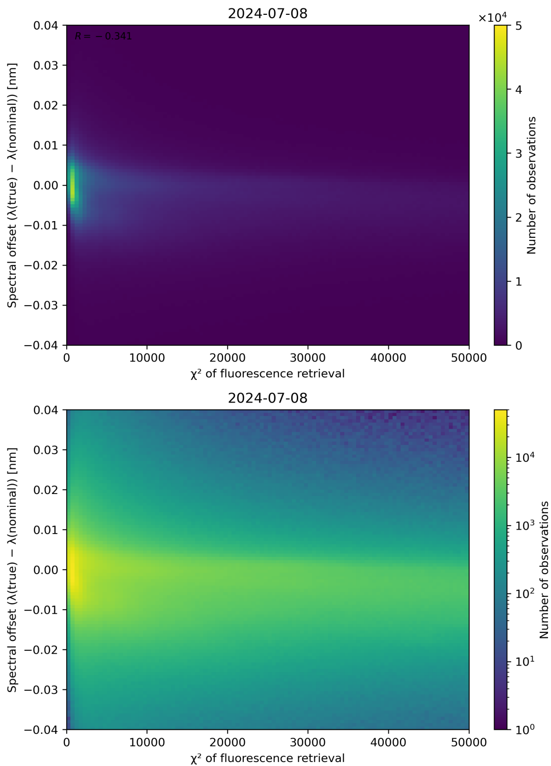
Figure 69: Scatter density plot of “ \chi^2 of fluorescence retrieval” against “Spectral offset ( \lambda(\text{true}) - \lambda(\text{nominal}) )” for 2024-07-07 to 2024-07-09.
