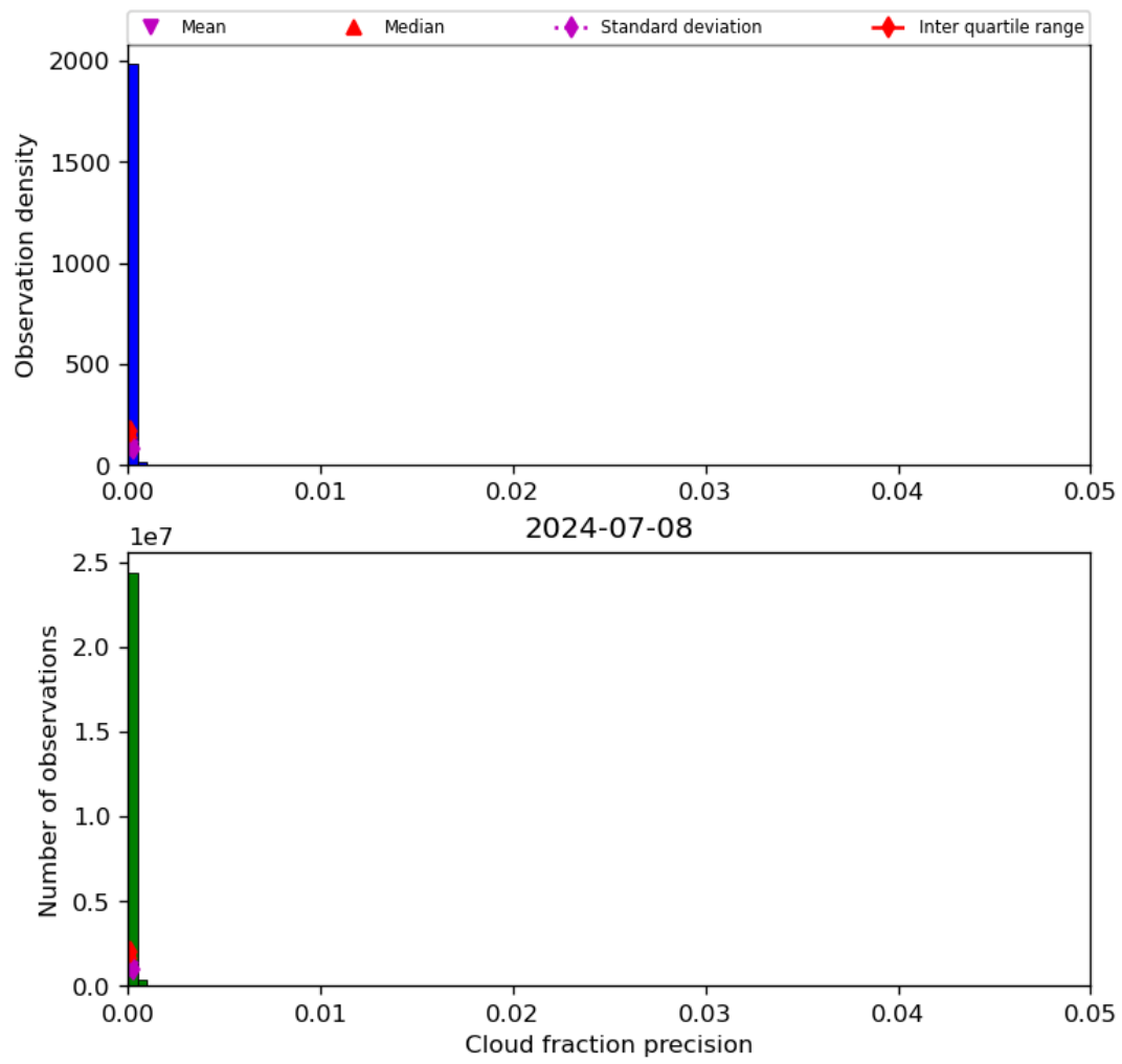
Figure 33: Histogram of “Cloud fraction precision” for 2024-07-07 to 2024-07-09
