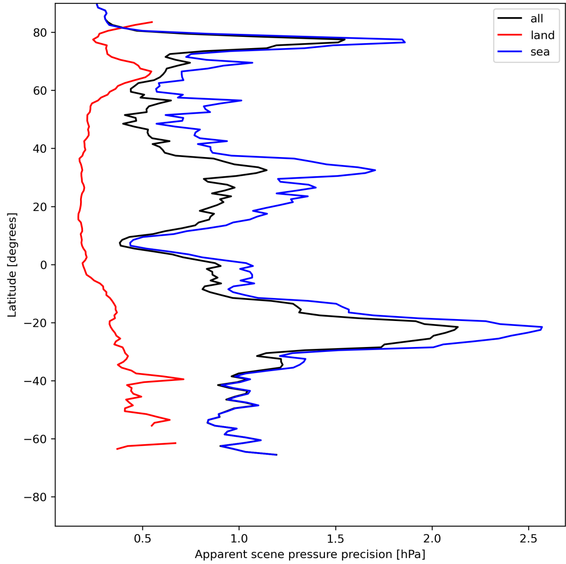
Figure 20: Zonal average of “Apparent scene pressure precision” for 2024-07-07 to 2024-07-09.
