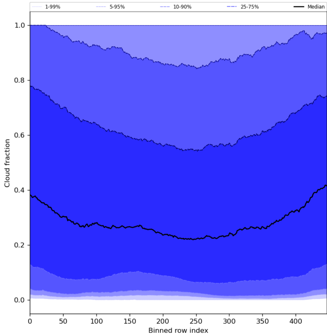
Figure 49: Along track statistics of “Cloud fraction” for 2024-07-07 to 2024-07-09
