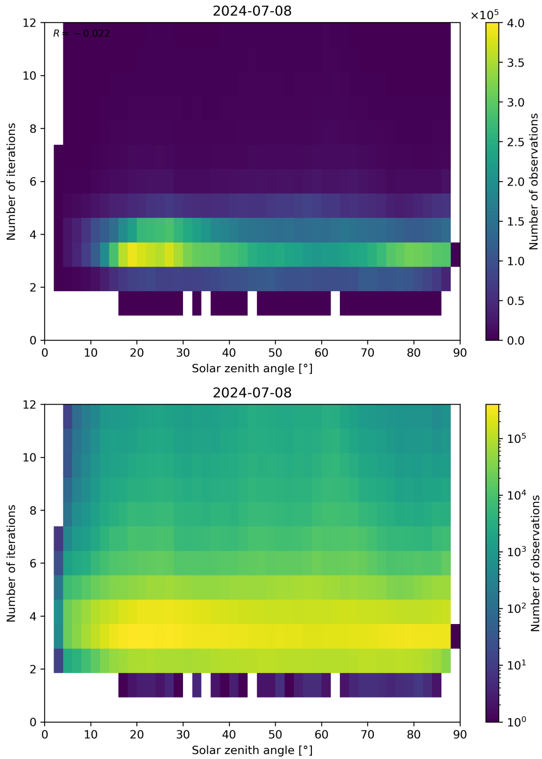
Figure 114: Scatter density plot of “Solar zenith angle” against “Number of iterations” for 2024-07-07 to 2024-07-09.
