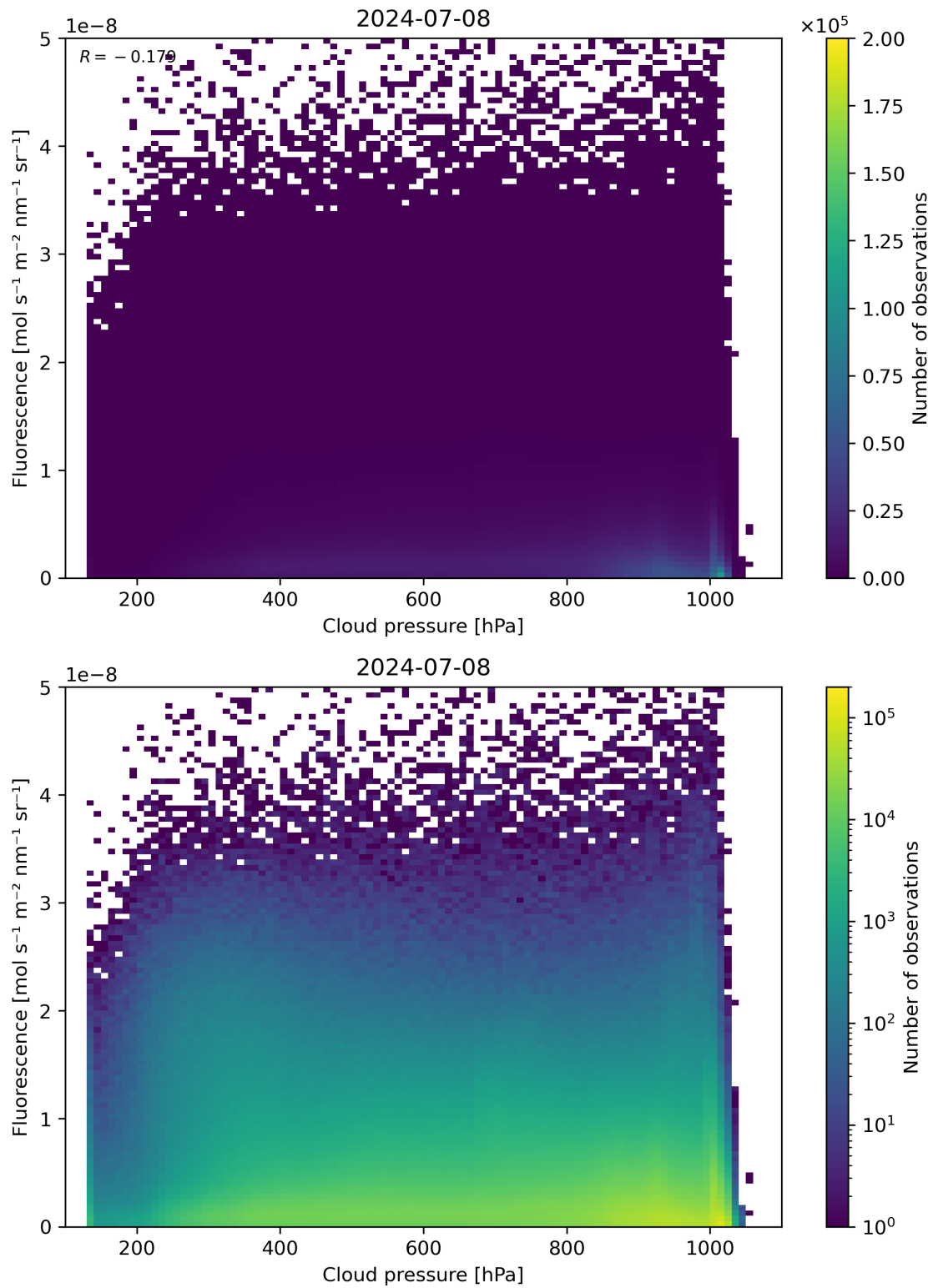
Figure 80: Scatter density plot of “Cloud pressure” against “Fluorescence” for 2024-07-07 to 2024-07-09.
