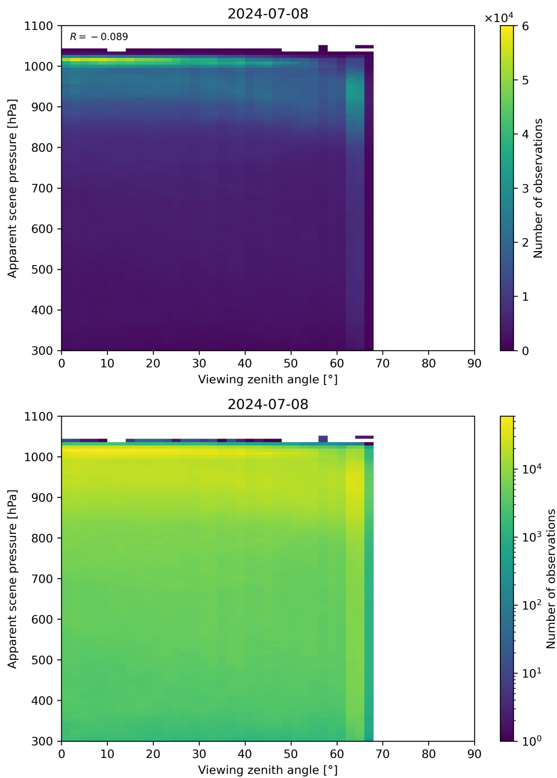
Figure 118: Scatter density plot of “Viewing zenith angle” against “Apparent scene pressure” for 2024-07-07 to 2024-07-09.
