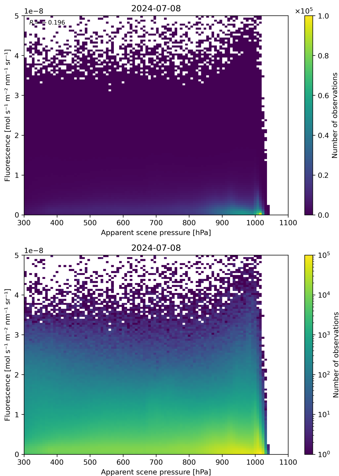
Figure 64: Scatter density plot of “Apparent scene pressure” against “Fluorescence” for 2024-07-07 to 2024-07-09.
