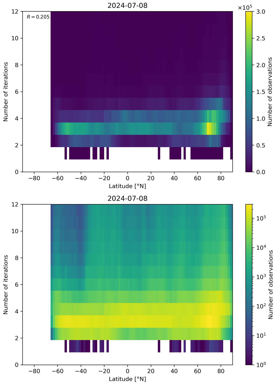
Figure 93: Scatter density plot of “Latitude” against “Number of iterations” for 2024-07-07 to 2024-07-09.
