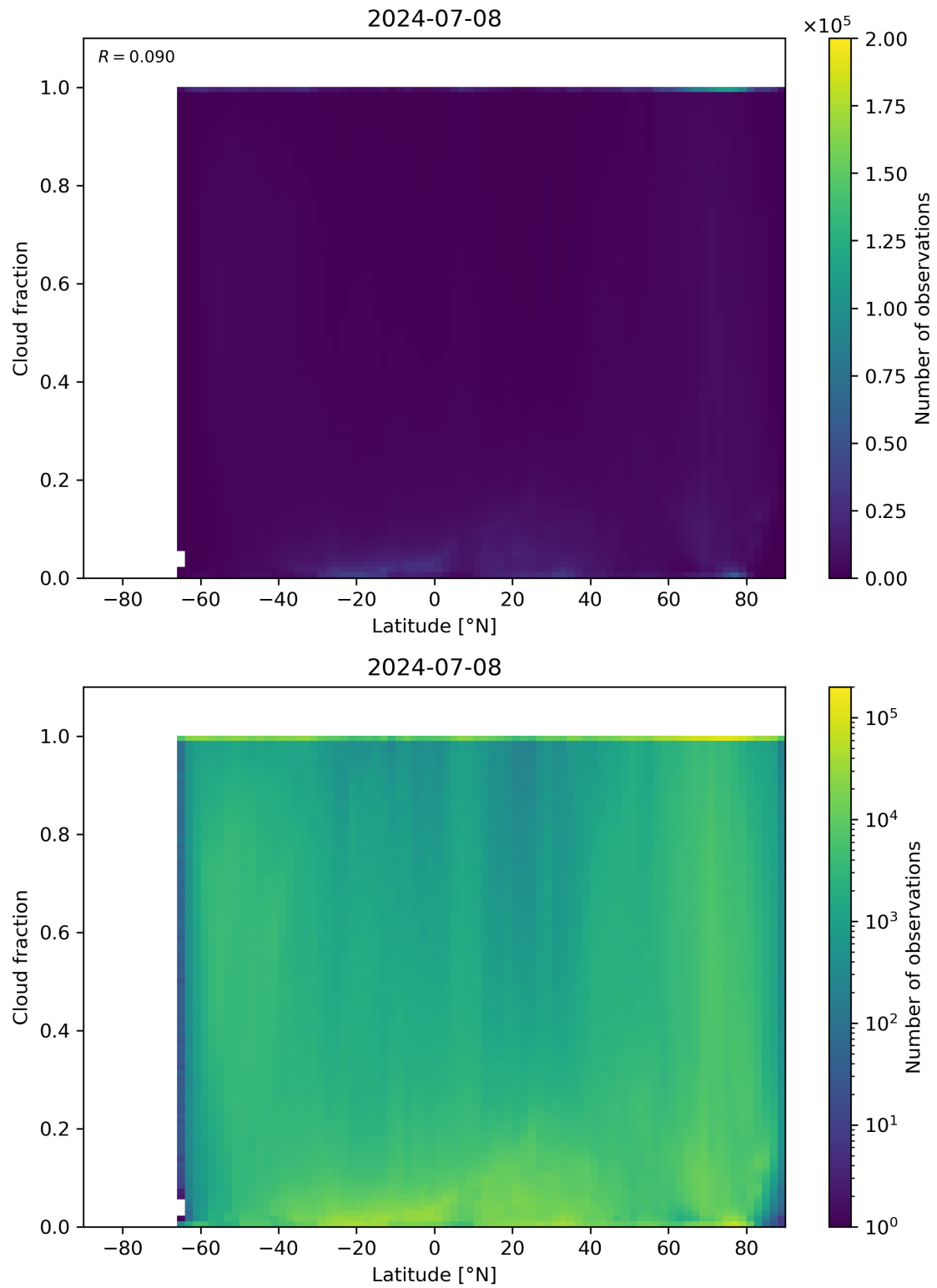
Figure 90: Scatter density plot of “Latitude” against “Cloud fraction” for 2024-07-07 to 2024-07-09.
