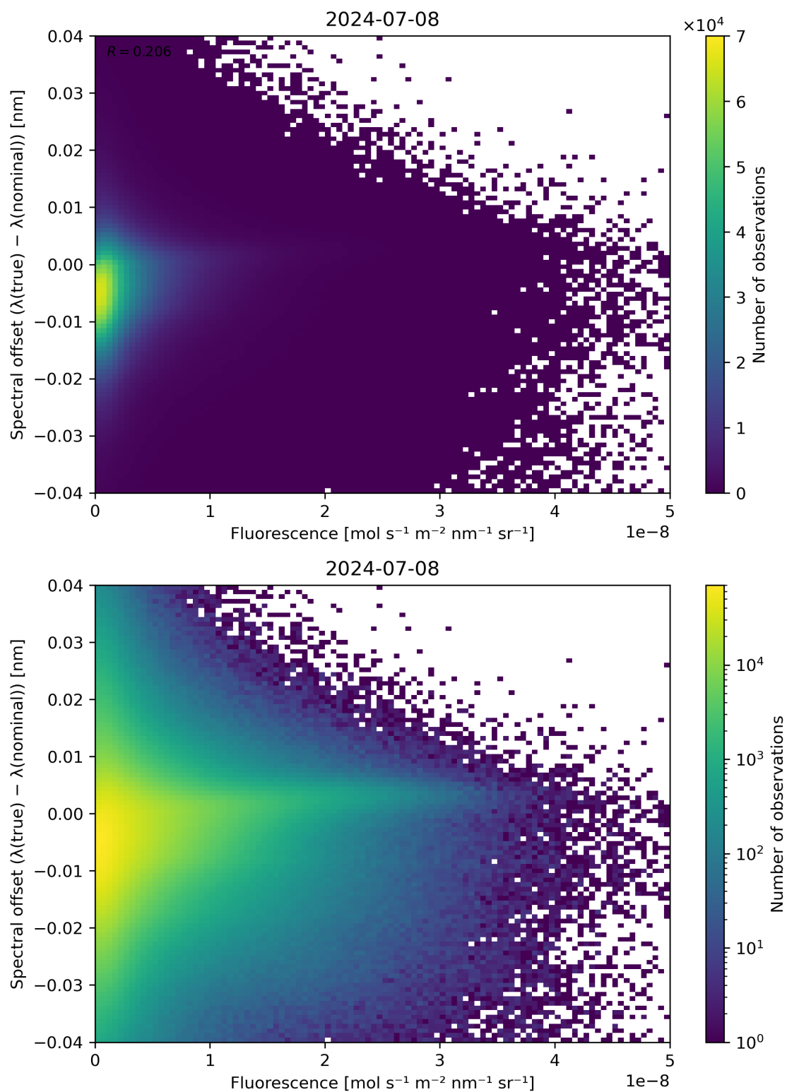
Figure 87: Scatter density plot of “Fluorescence” against “Spectral offset ( \lambda(\text{true}) - \lambda(\text{nominal}) )” for 2024-07-07 to 2024-07-09.
