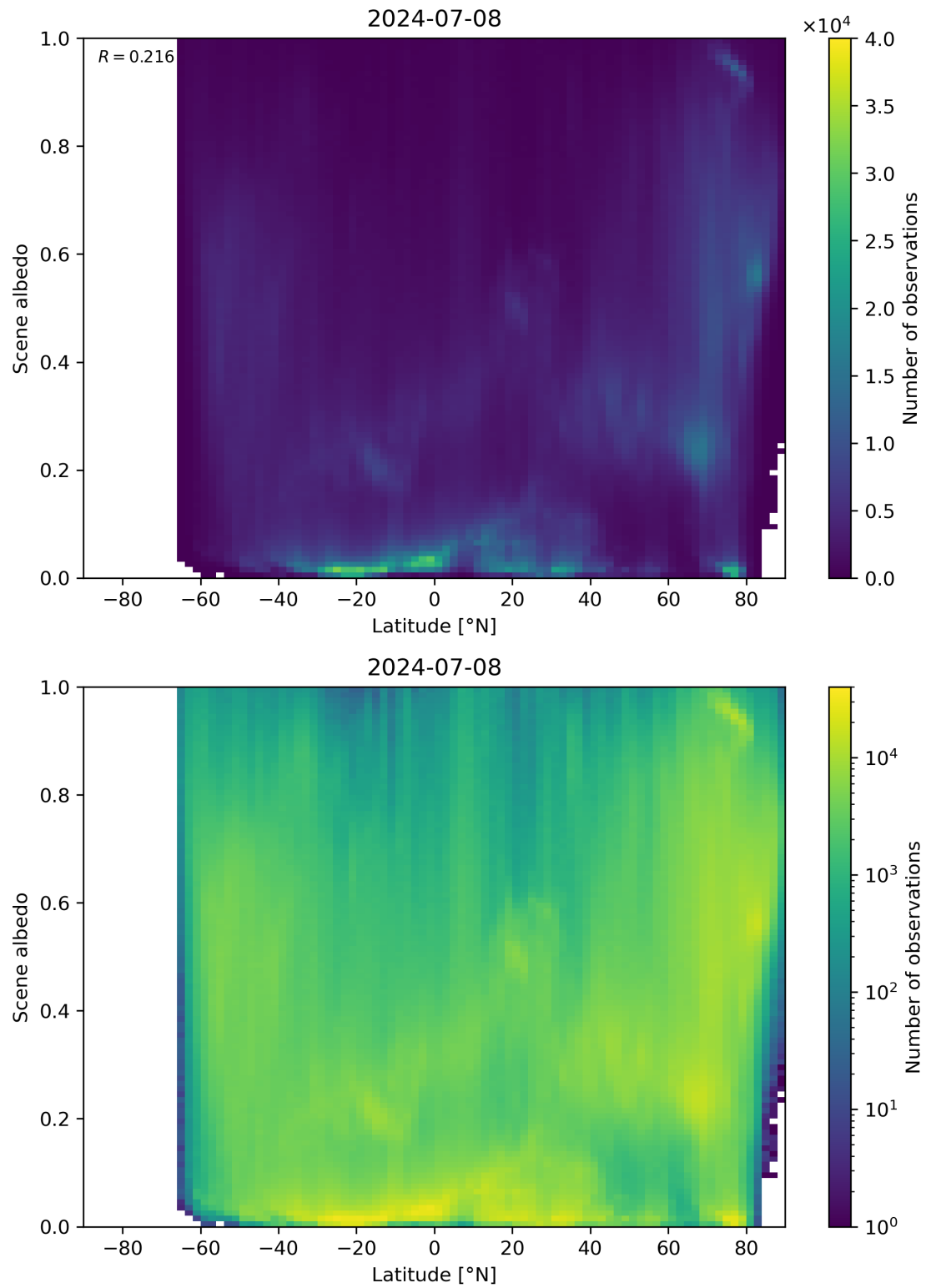
Figure 95: Scatter density plot of “Latitude” against “Scene albedo” for 2024-07-07 to 2024-07-09.
