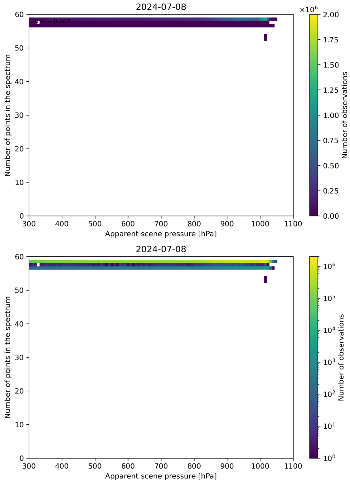
Figure 66: Scatter density plot of “Apparent scene pressure” against “Number of points in the spectrum” for 2024-07-07 to 2024-07-09.
