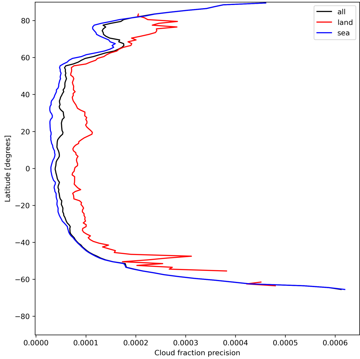
Figure 16: Zonal average of “Cloud fraction precision” for 2024-07-07 to 2024-07-09.
