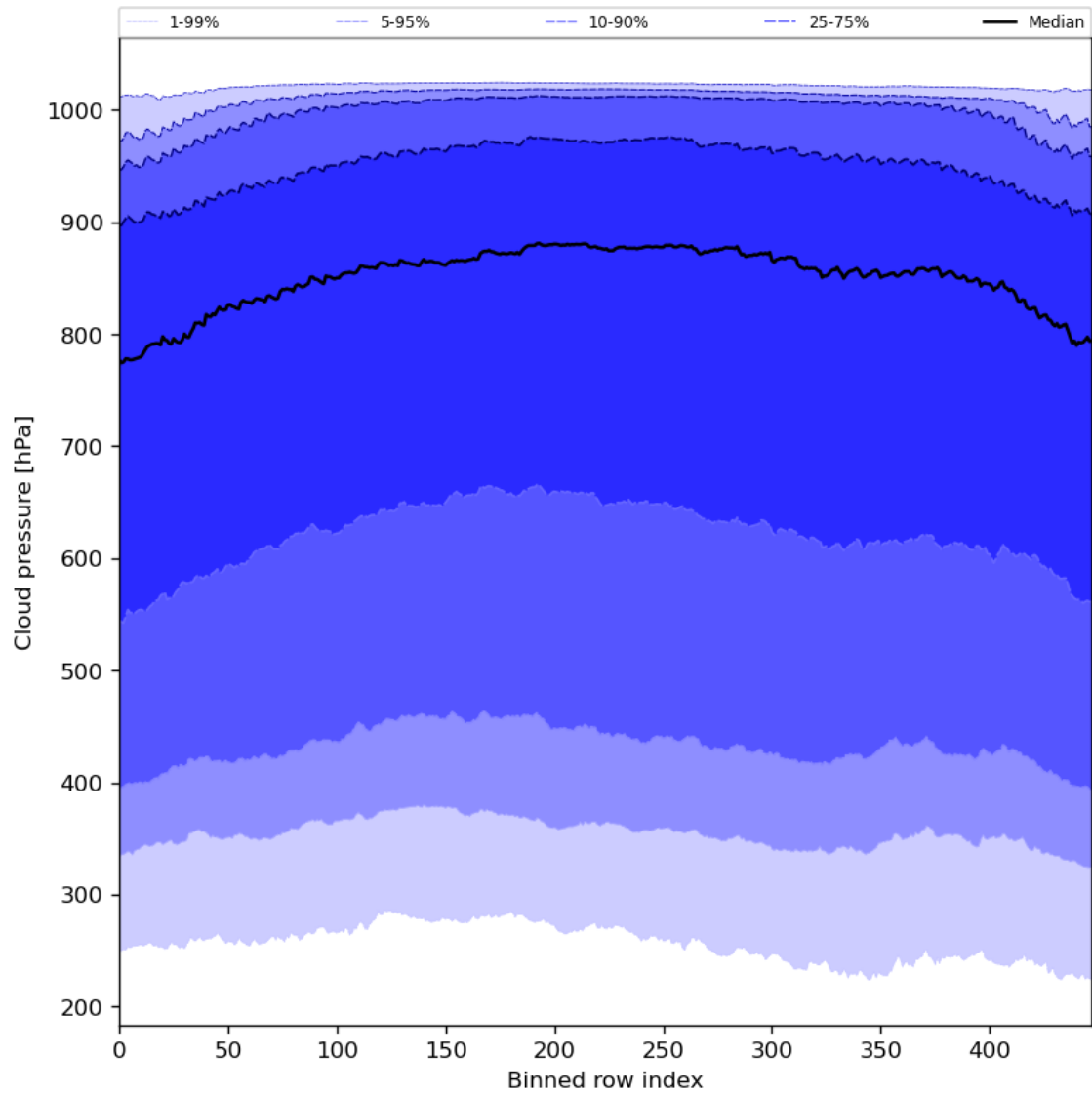
Figure 47: Along track statistics of “Cloud pressure” for 2024-07-07 to 2024-07-09
