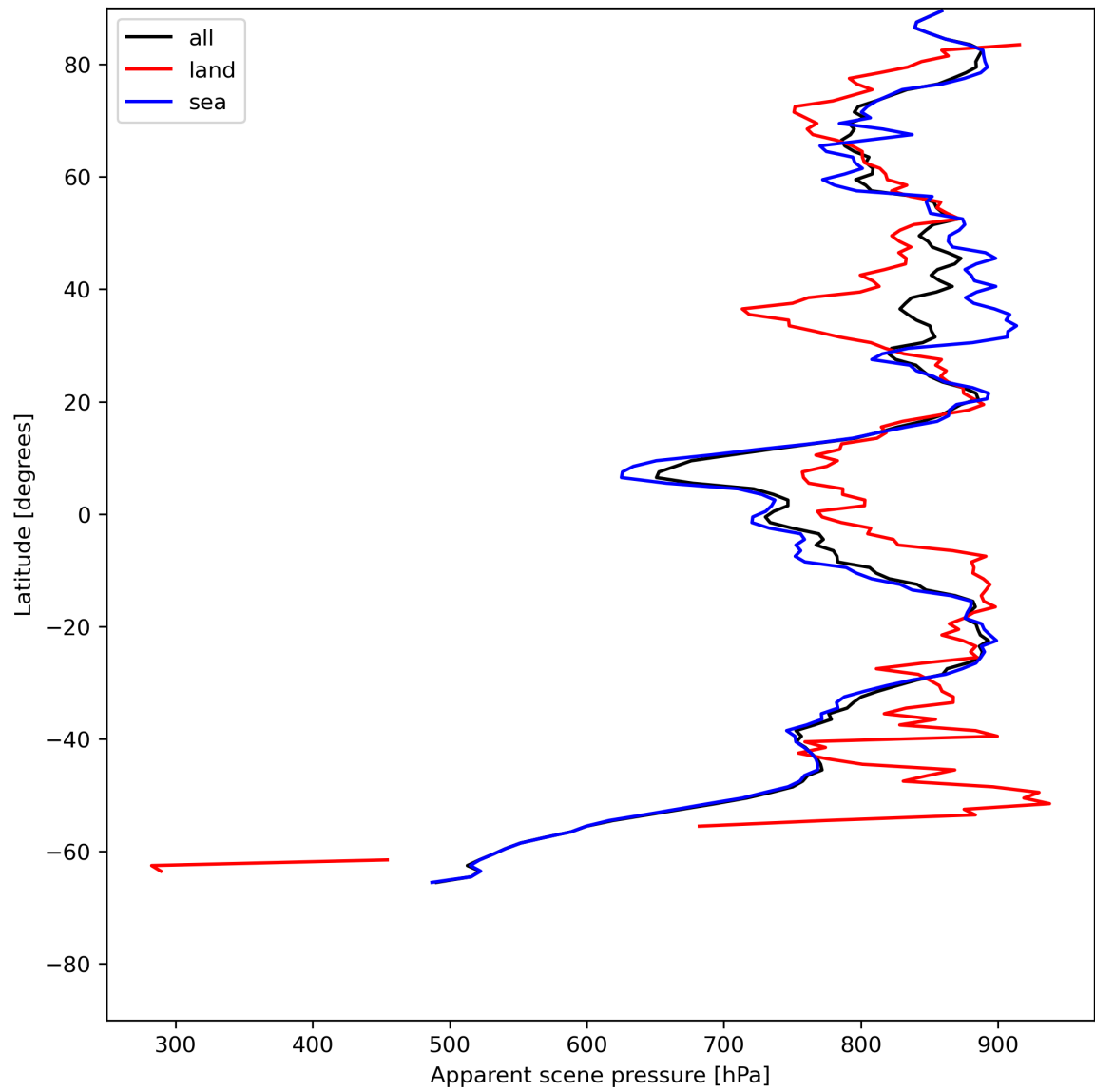
Figure 19: Zonal average of “Apparent scene pressure” for 2024-07-07 to 2024-07-09.
