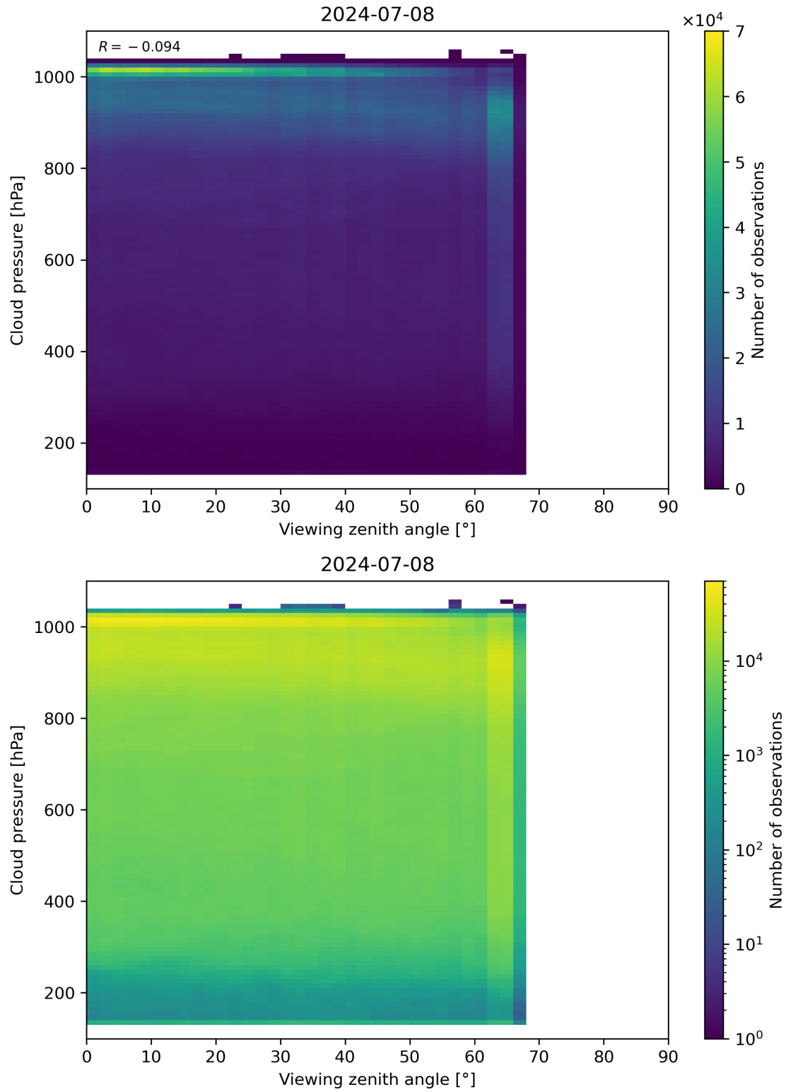
Figure 121: Scatter density plot of “Viewing zenith angle” against “Cloud pressure” for 2024-07-07 to 2024-07-09.
