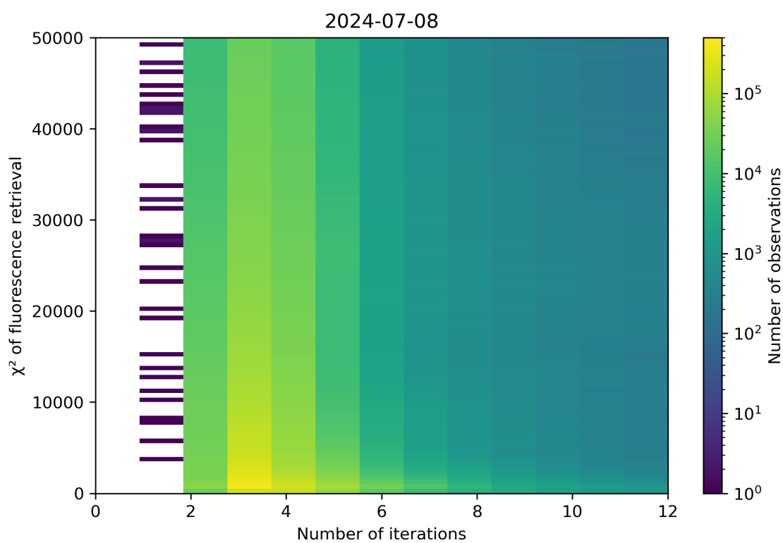
Figure 97: Scatter density plot of “Number of iterations” against “ \chi^2 of fluorescence retrieval” for 2024-07-07 to 2024-07-09.
