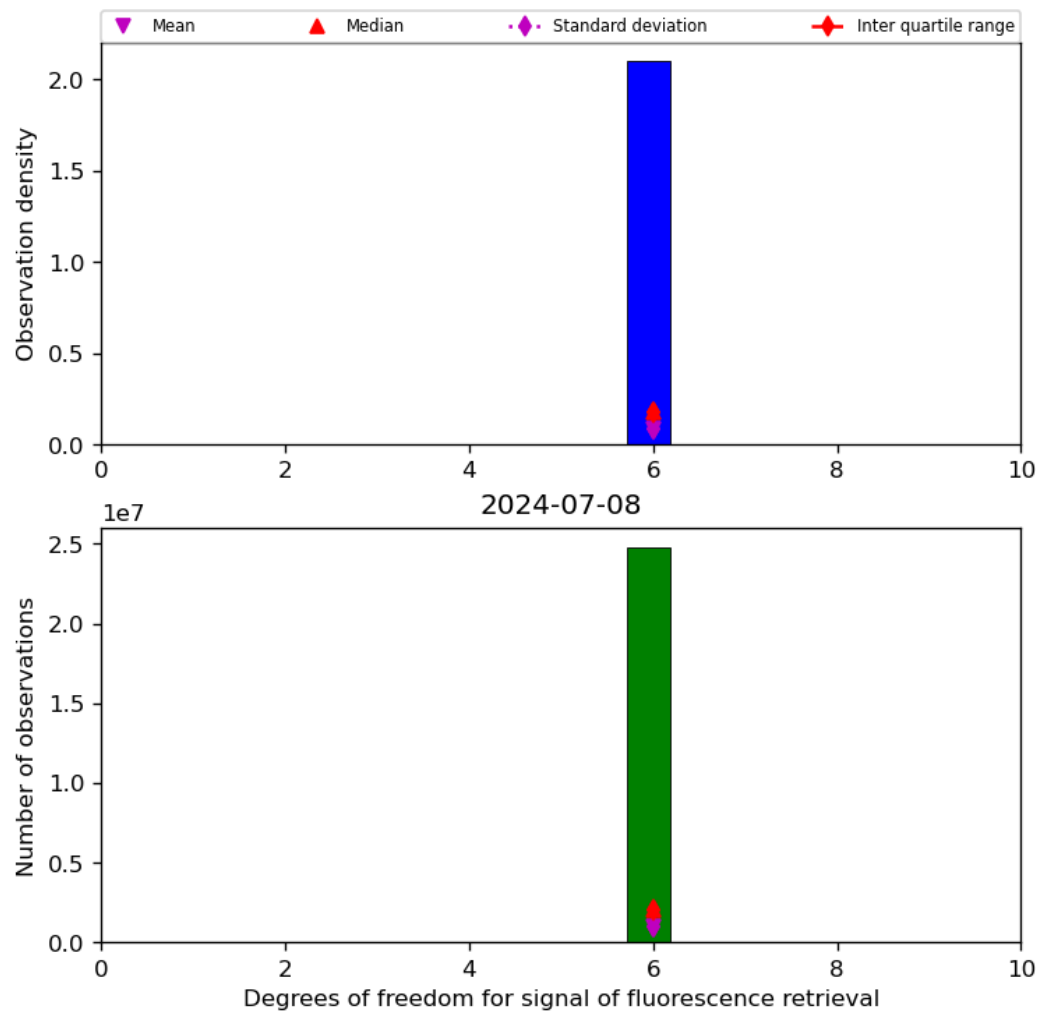
Figure 43: Histogram of “Degrees of freedom for signal of fluorescence retrieval” for 2024-07-07 to 2024-07-09
