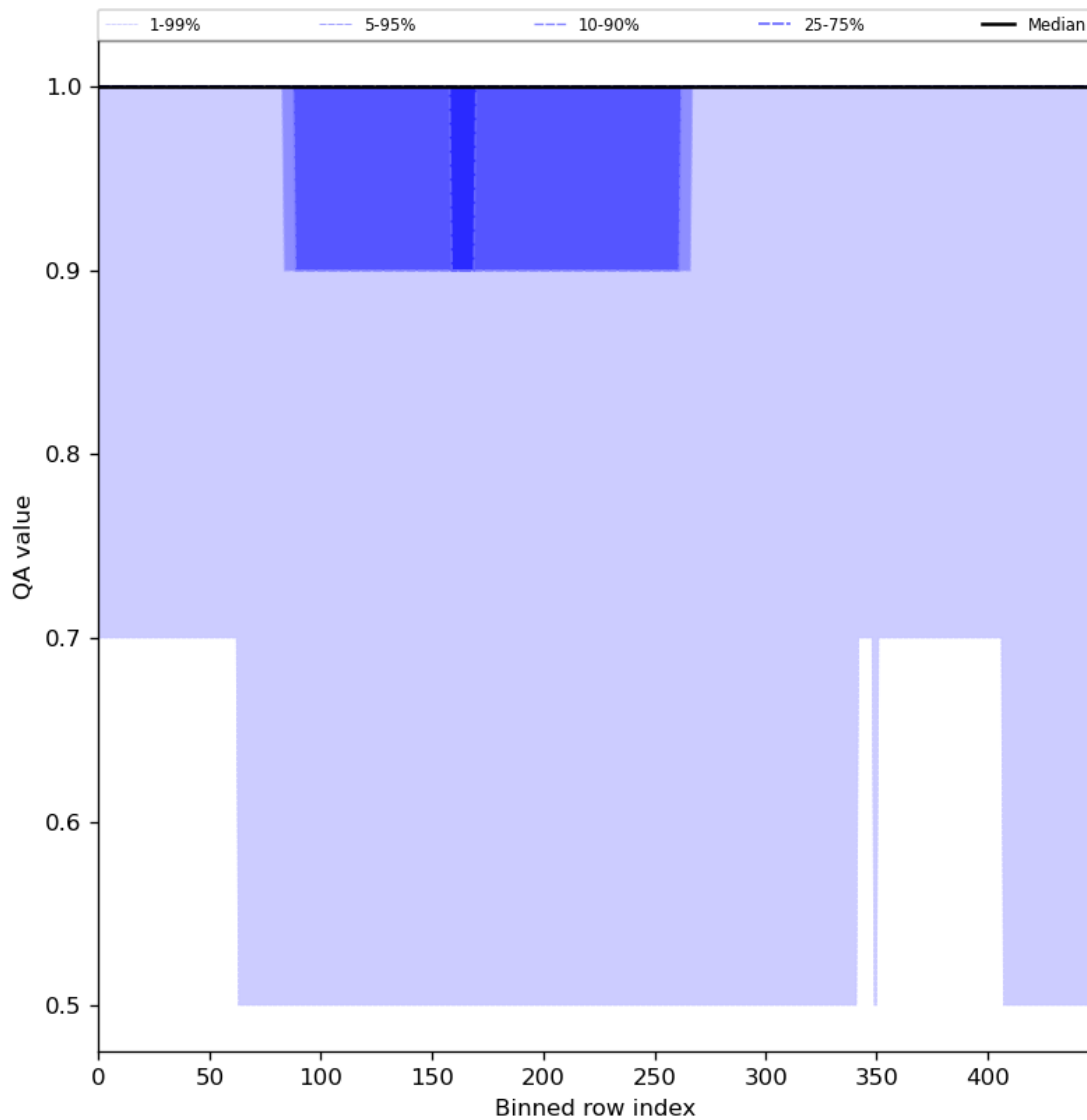
Figure 46: Along track statistics of “QA value” for 2024-07-07 to 2024-07-09
