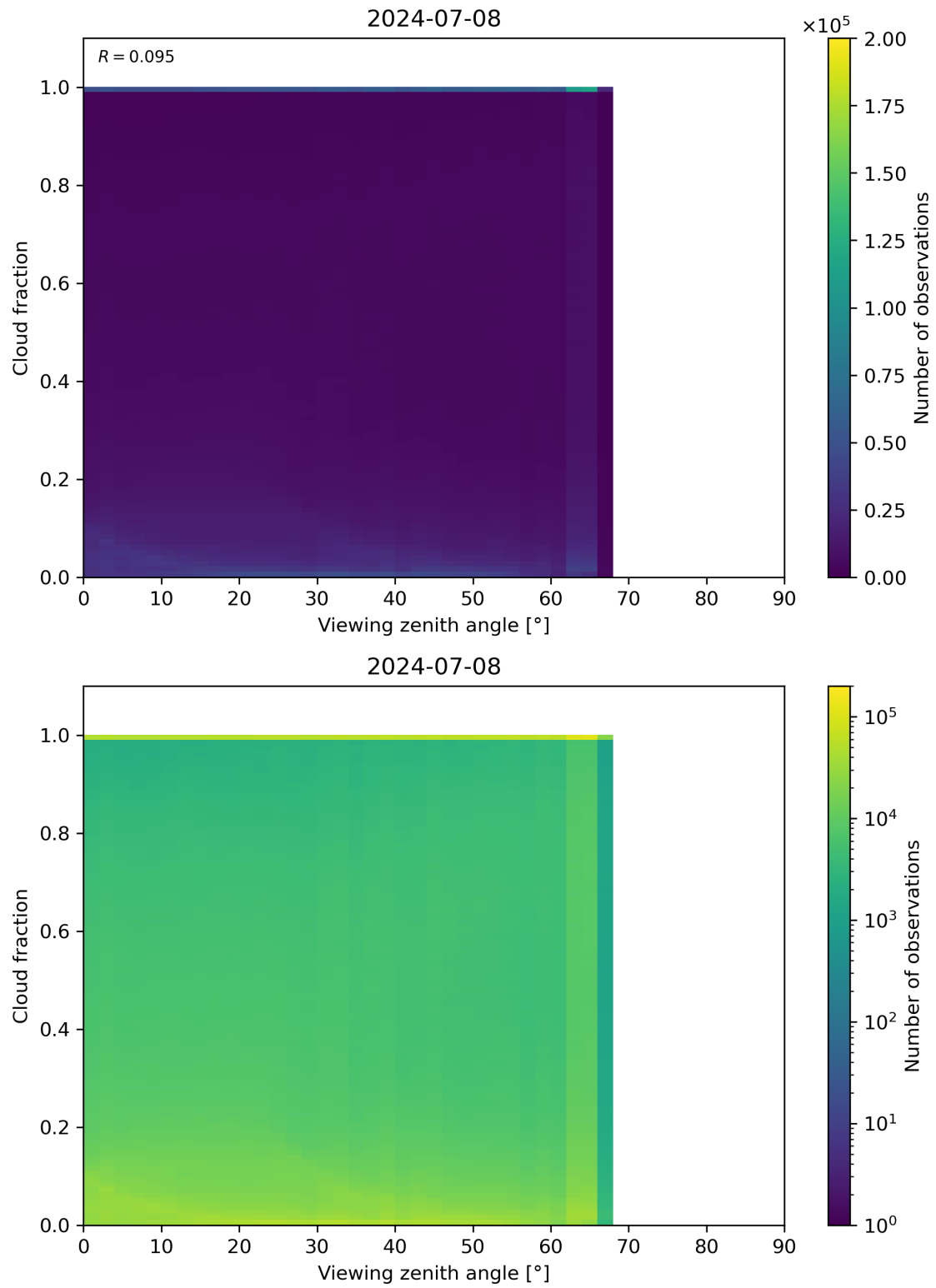
Figure 120: Scatter density plot of “Viewing zenith angle” against “Cloud fraction” for 2024-07-07 to 2024-07-09.
