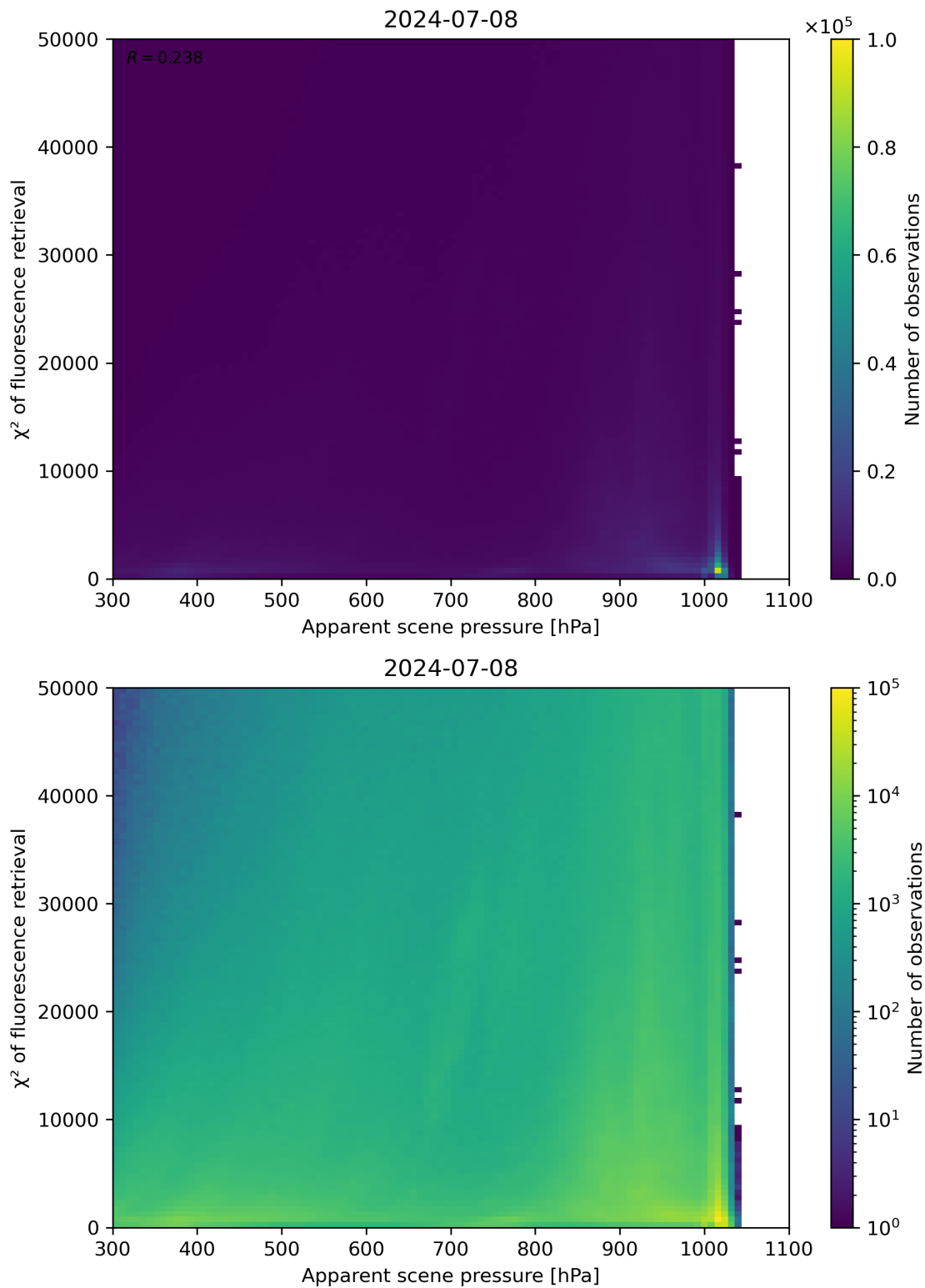
Figure 63: Scatter density plot of “Apparent scene pressure” against “ \chi^2 of fluorescence retrieval” for 2024-07-07 to 2024-07-09.
