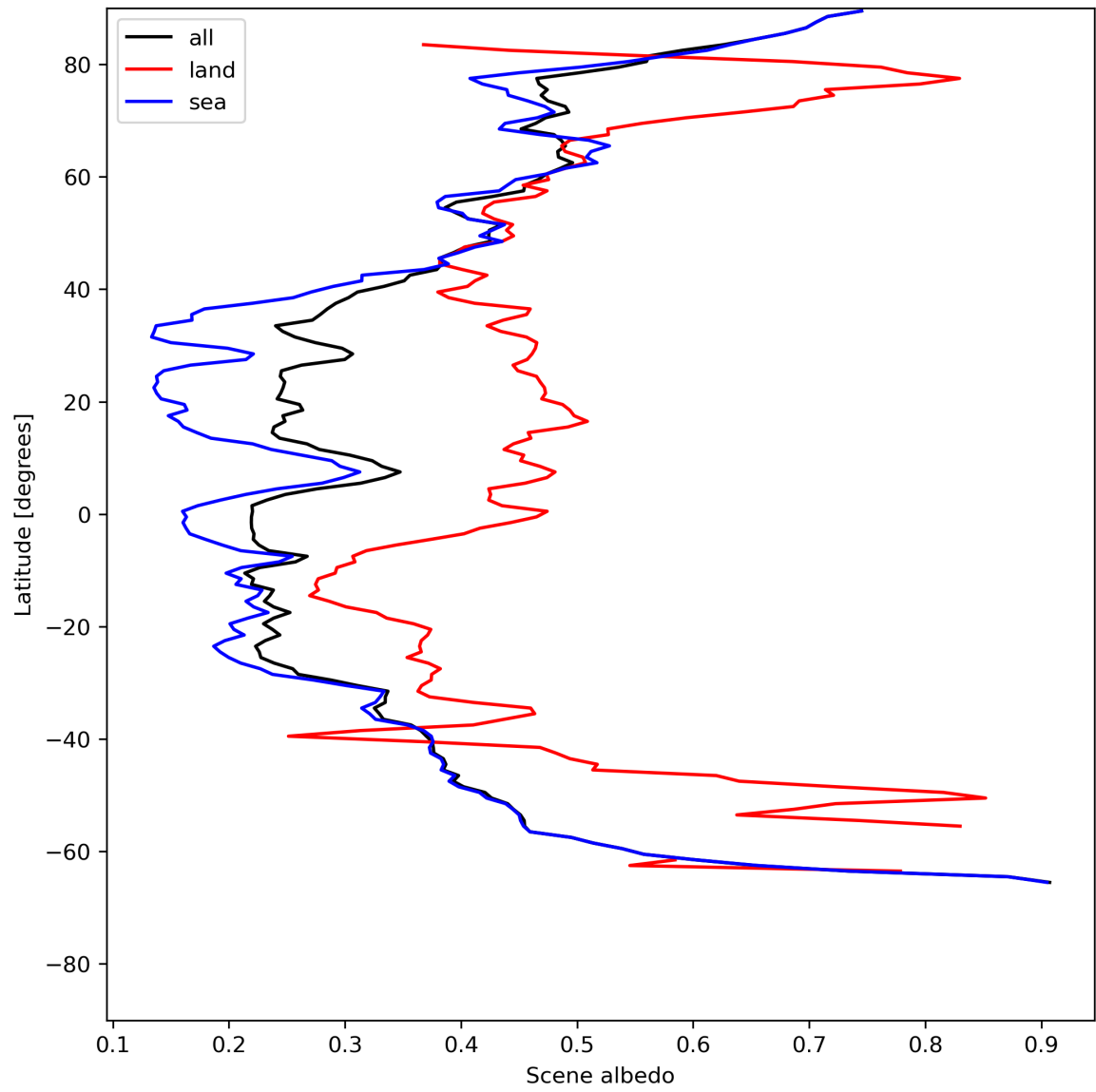
Figure 17: Zonal average of “Scene albedo” for 2024-07-07 to 2024-07-09.
