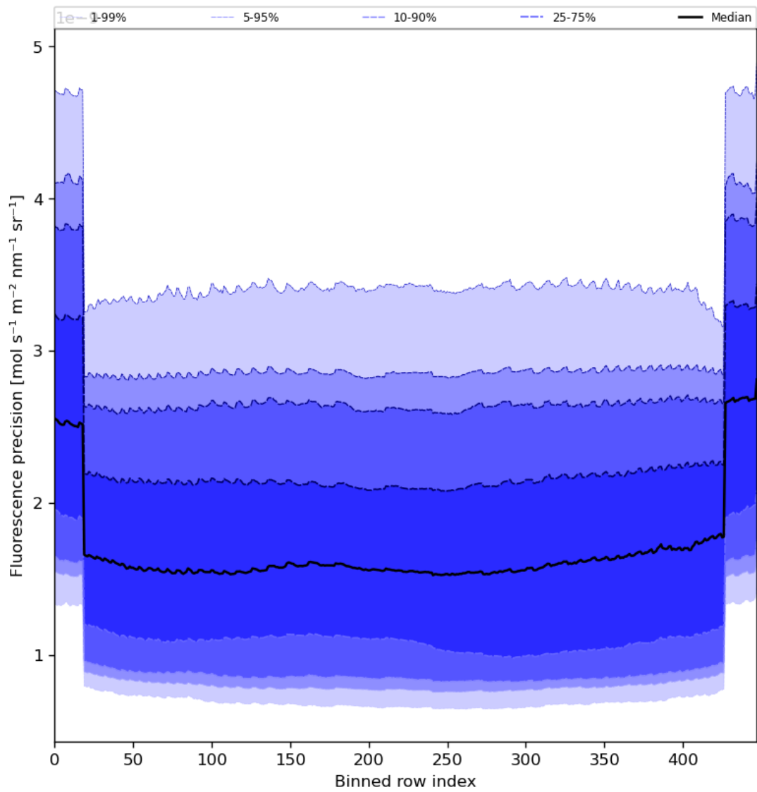
Figure 58: Along track statistics of “Fluorescence precision” for 2024-07-07 to 2024-07-09
