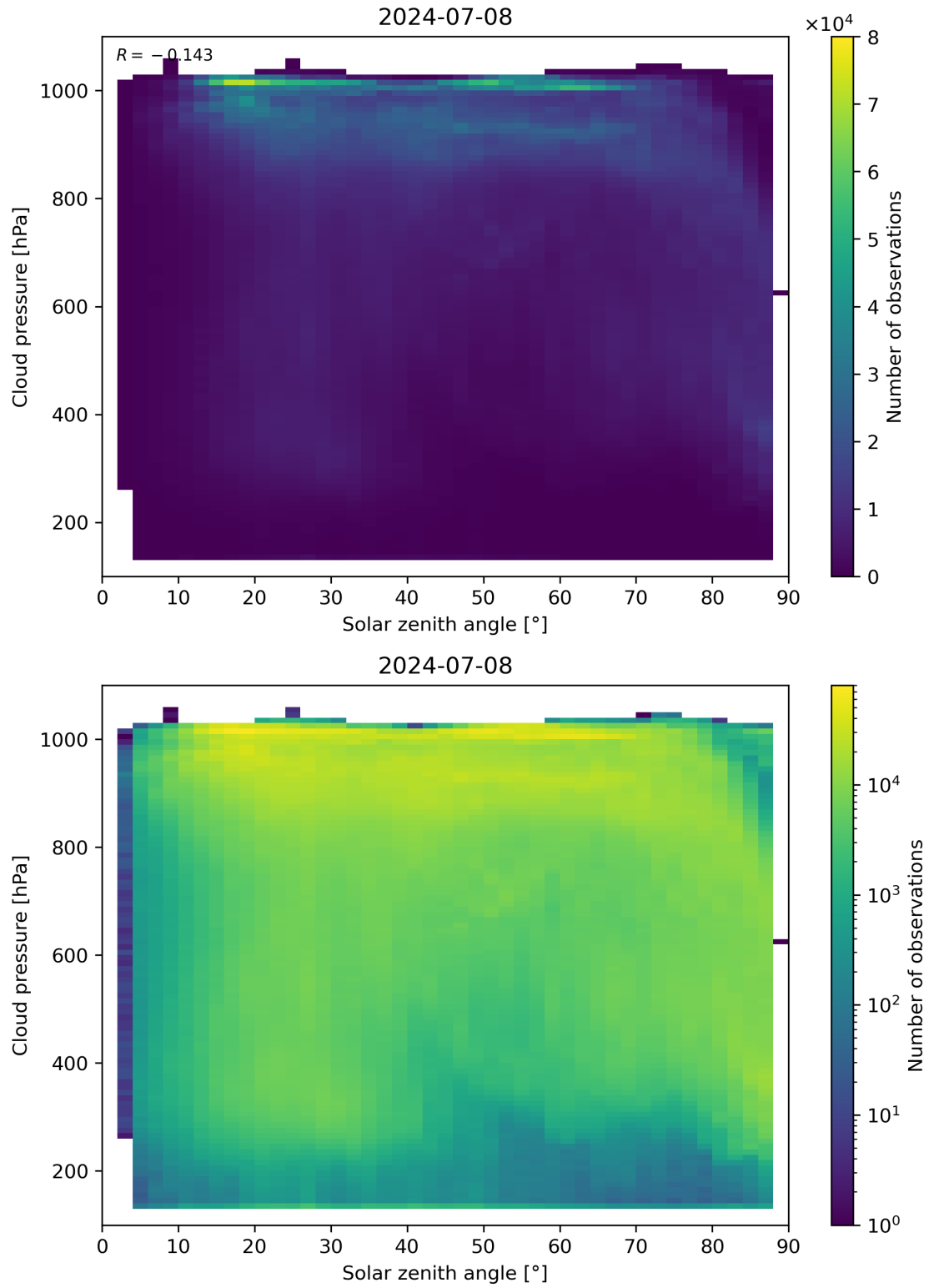
Figure 111: Scatter density plot of “Solar zenith angle” against “Cloud pressure” for 2024-07-07 to 2024-07-09.
