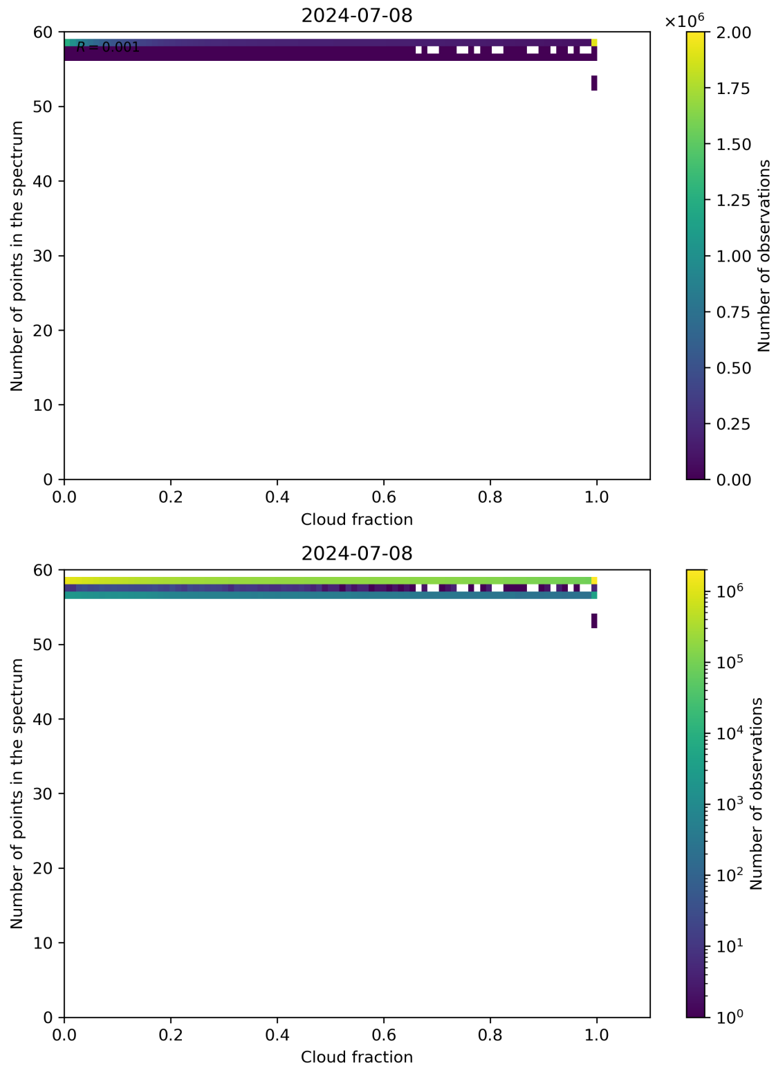
Figure 74: Scatter density plot of “Cloud fraction” against “Number of points in the spectrum” for 2024-07-07 to 2024-07-09.
