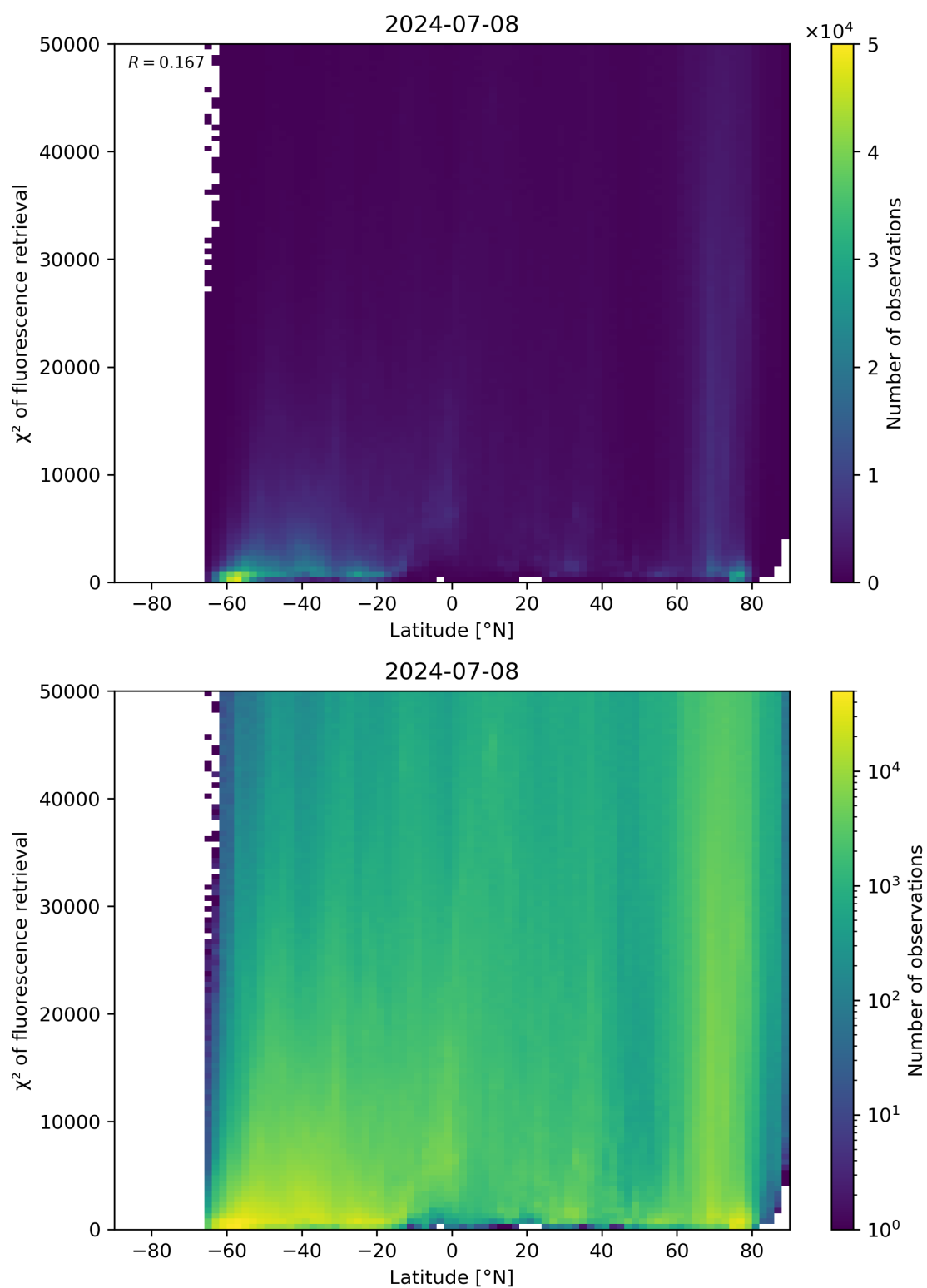
Figure 89: Scatter density plot of “Latitude” against “ \chi^2 of fluorescence retrieval” for 2024-07-07 to 2024-07-09.
