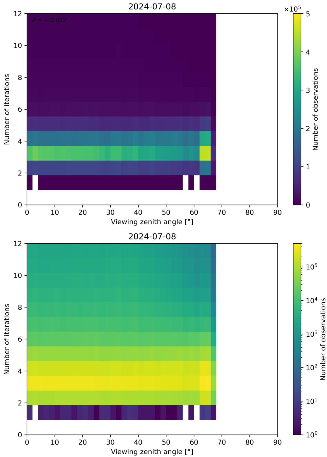
Figure 124: Scatter density plot of “Viewing zenith angle” against “Number of iterations” for 2024-07-07 to 2024-07-09.
