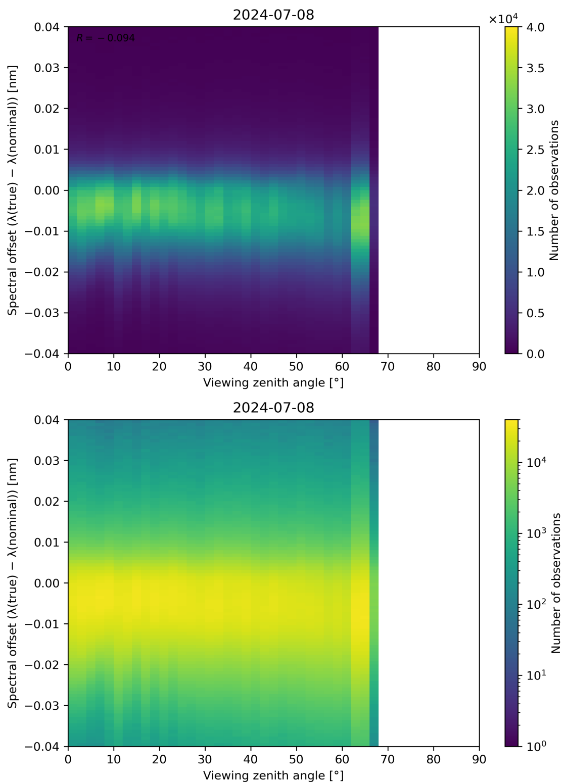
Figure 128: Scatter density plot of “Viewing zenith angle” against “Spectral offset ( \lambda(\text{true}) - \lambda(\text{nominal}) )” for 2024-07-07 to 2024-07-09.
