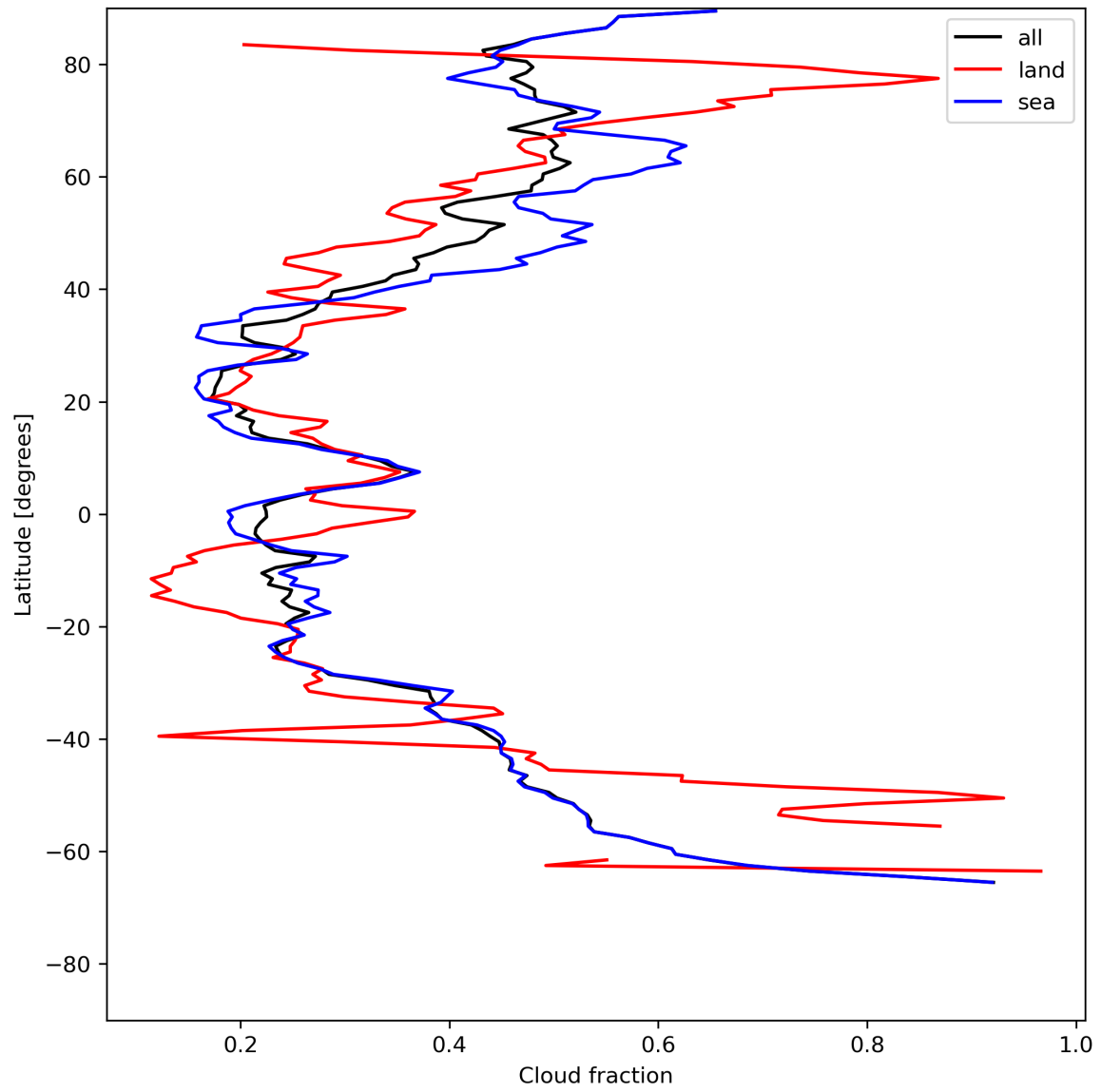
Figure 15: Zonal average of “Cloud fraction” for 2024-07-07 to 2024-07-09.
