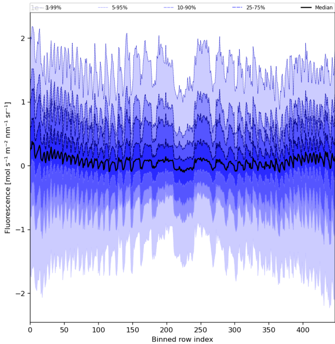
Figure 57: Along track statistics of “Fluorescence” for 2024-07-07 to 2024-07-09
