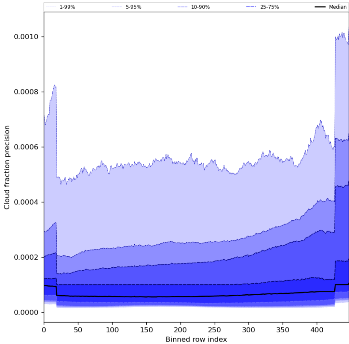
Figure 50: Along track statistics of “Cloud fraction precision” for 2024-07-07 to 2024-07-09
