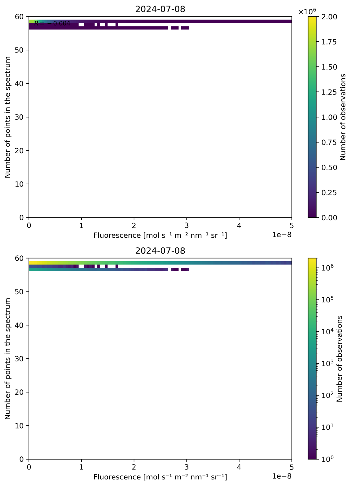
Figure 86: Scatter density plot of “Fluorescence” against “Number of points in the spectrum” for 2024-07-07 to 2024-07-09.
