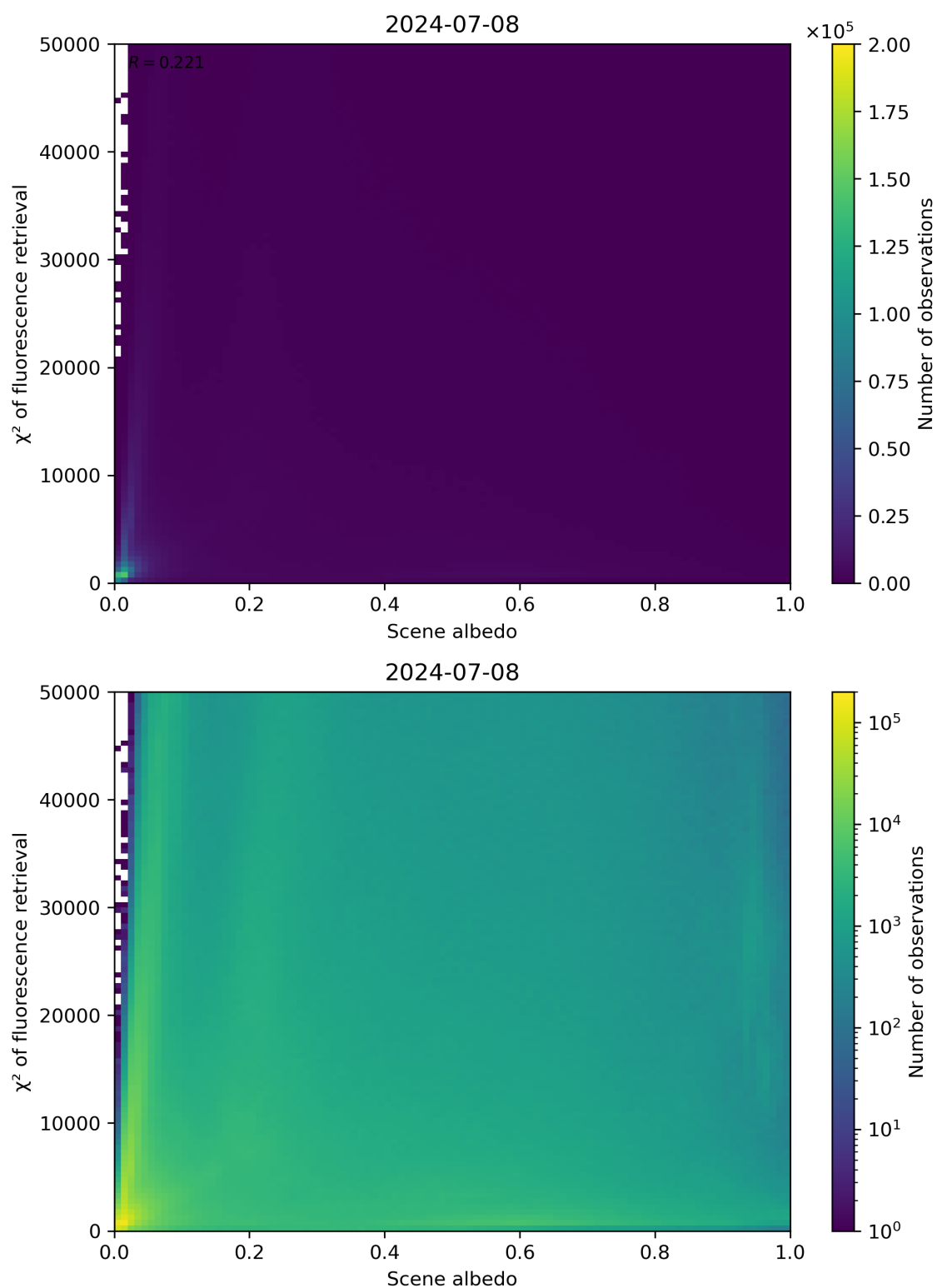
Figure 103: Scatter density plot of “Scene albedo” against “ \chi^2 of fluorescence retrieval” for 2024-07-07 to 2024-07-09.
