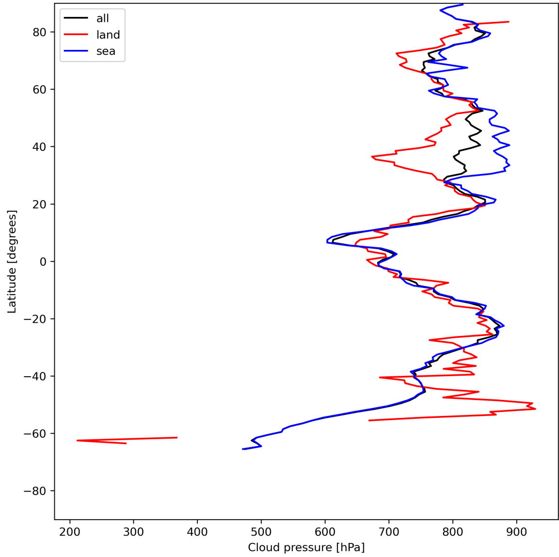
Figure 13: Zonal average of “Cloud pressure” for 2024-07-07 to 2024-07-09.
