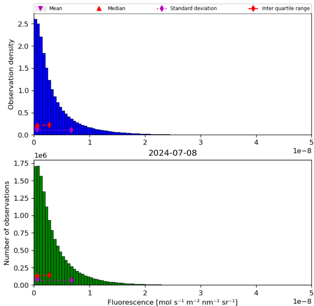
Figure 40: Histogram of “Fluorescence” for 2024-07-07 to 2024-07-09
