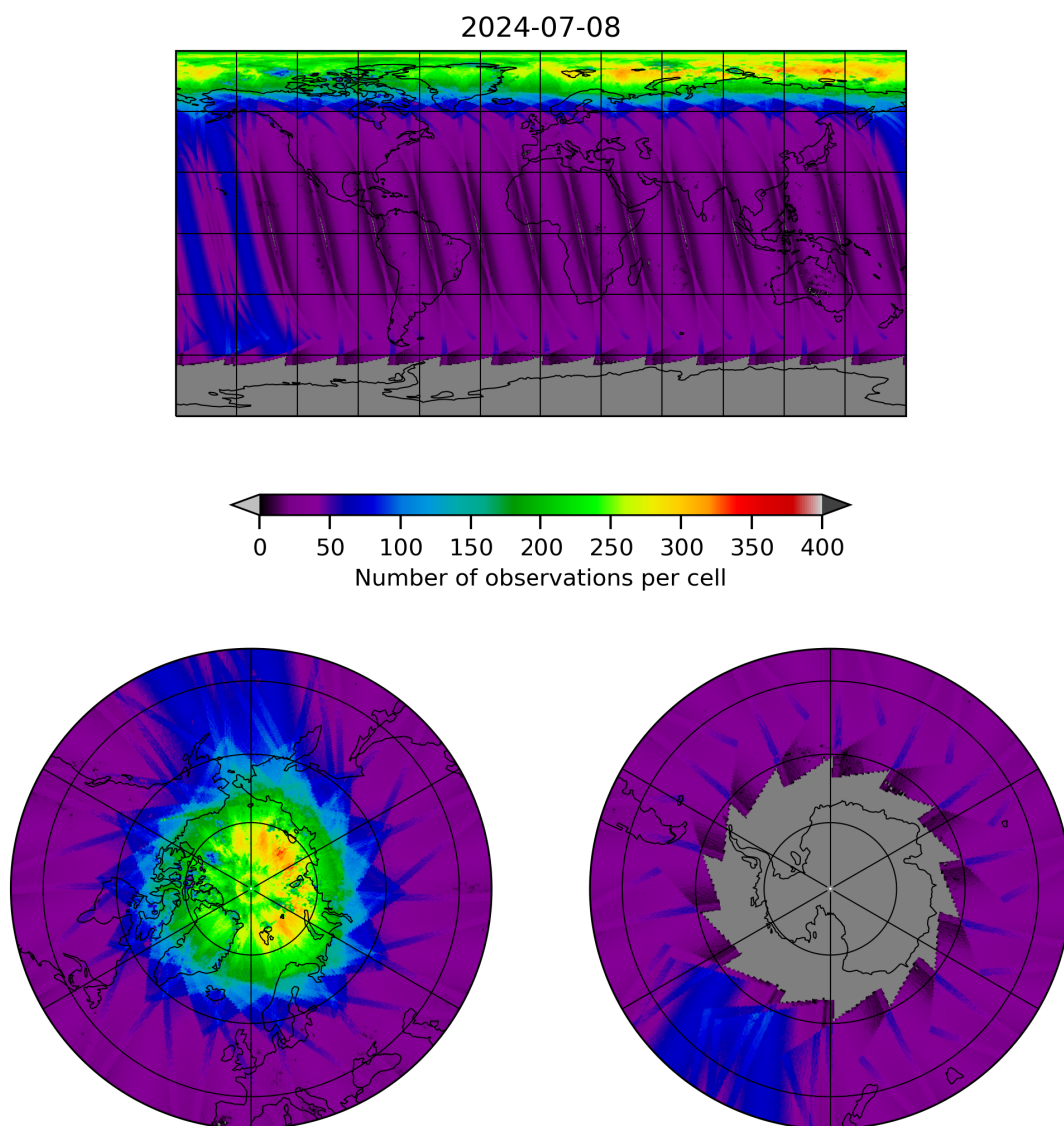
Figure 11: Map of the number of observations for 2024-07-07 to 2024-07-09
