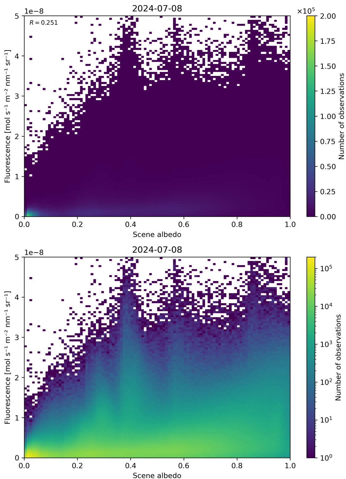
Figure 104: Scatter density plot of “Scene albedo” against “Fluorescence” for 2024-07-07 to 2024-07-09.
