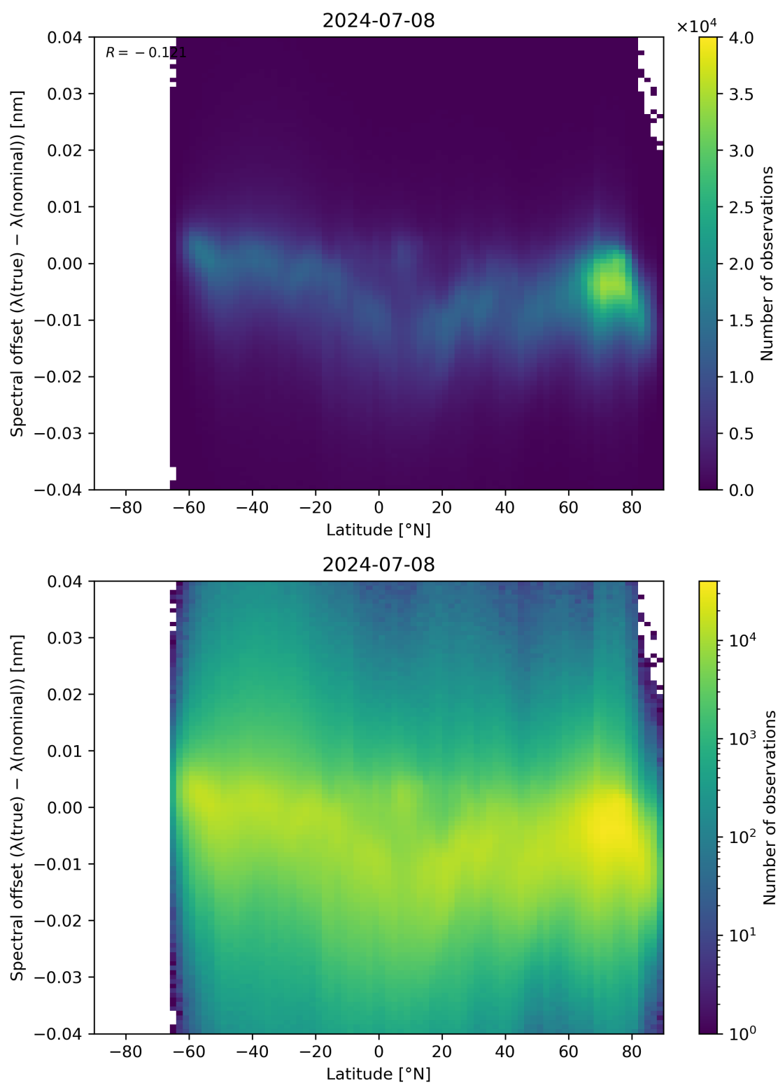
Figure 96: Scatter density plot of “Latitude” against “Spectral offset ( \lambda(\text{true}) - \lambda(\text{nominal}) )” for 2024-07-07 to 2024-07-09.
