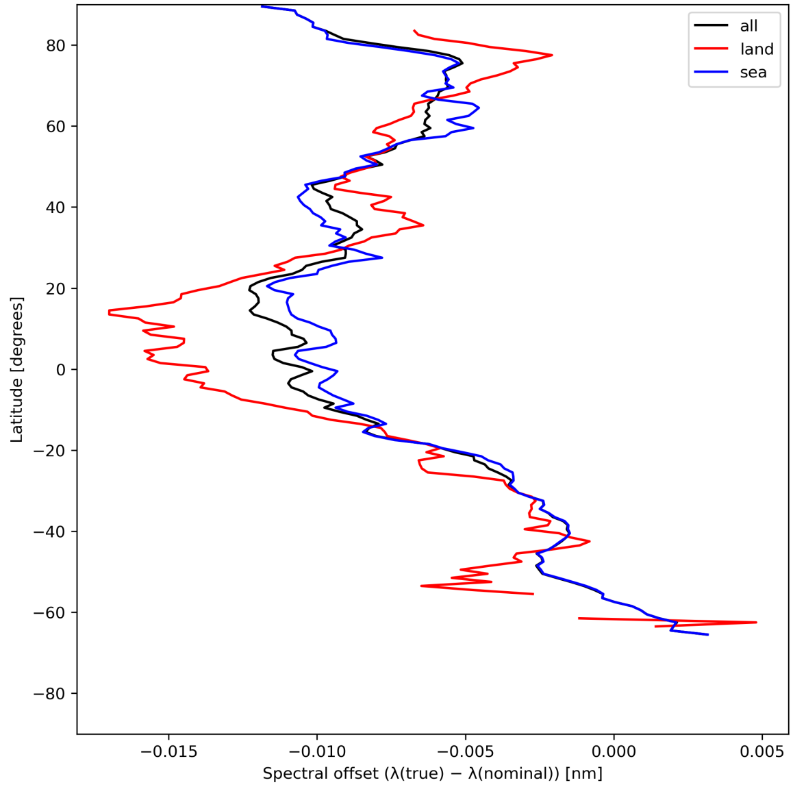
Figure 28: Zonal average of “Spectral offset ( \lambda(\text{true}) - \lambda(\text{nominal}) )” for 2024-07-07 to 2024-07-09.
