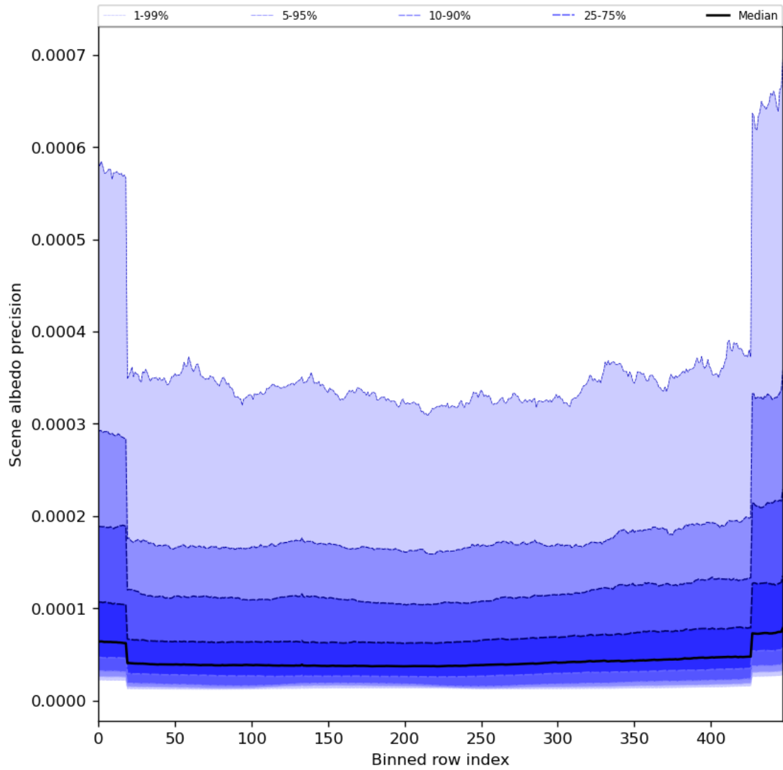
Figure 52: Along track statistics of “Scene albedo precision” for 2024-07-07 to 2024-07-09
