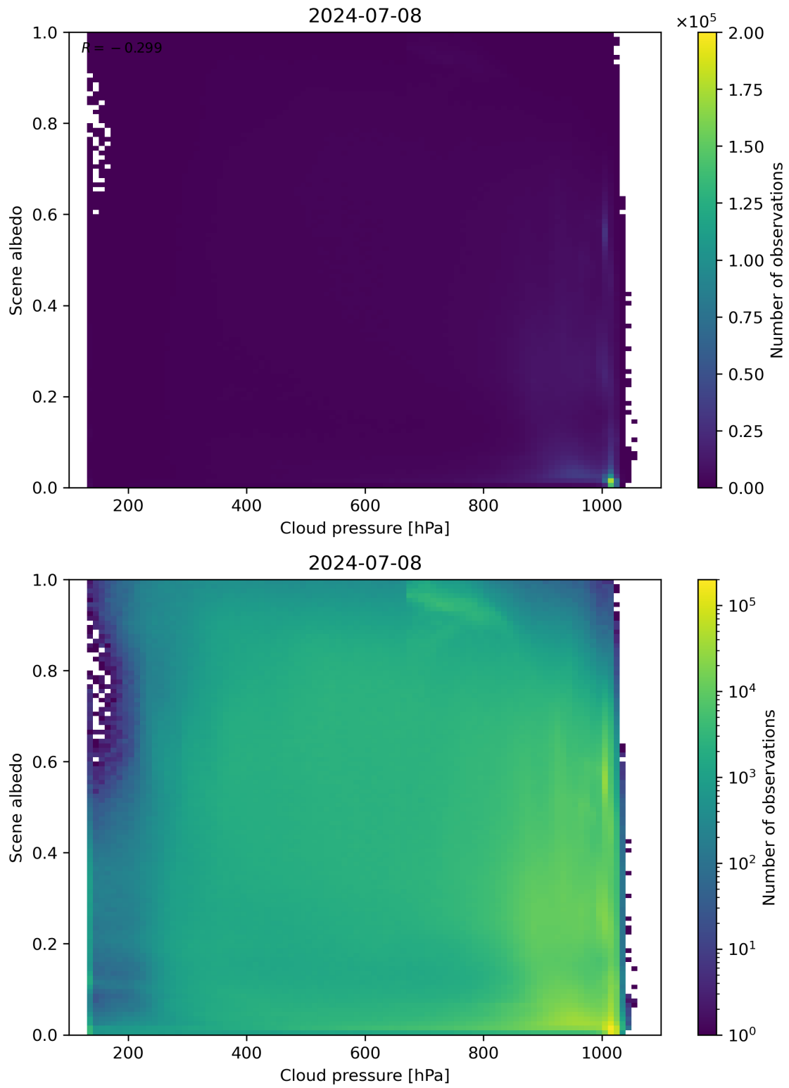
Figure 83: Scatter density plot of “Cloud pressure” against “Scene albedo” for 2024-07-07 to 2024-07-09.
