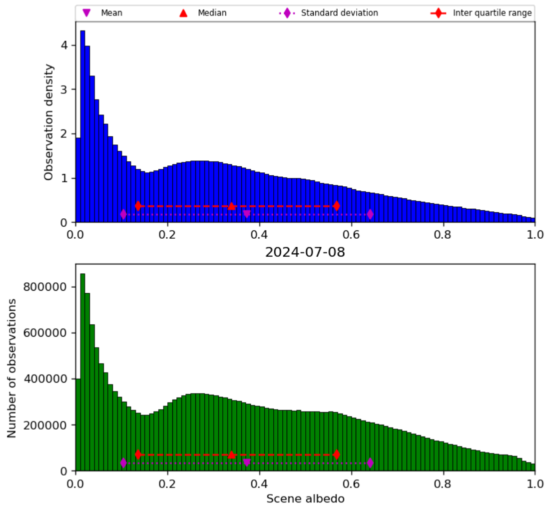
Figure 34: Histogram of “Scene albedo” for 2024-07-07 to 2024-07-09
