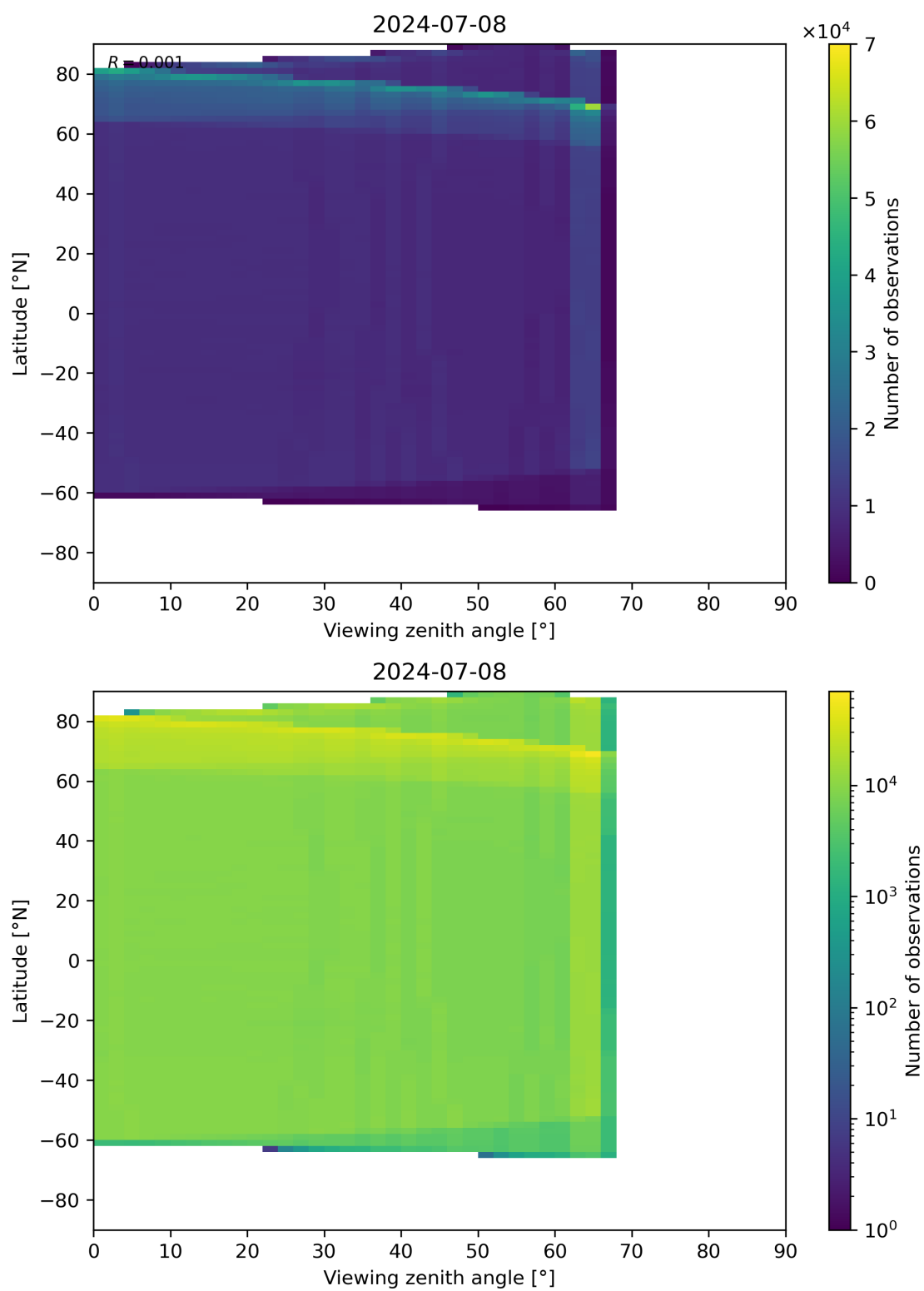
Figure 123: Scatter density plot of “Viewing zenith angle” against “Latitude” for 2024-07-07 to 2024-07-09.
