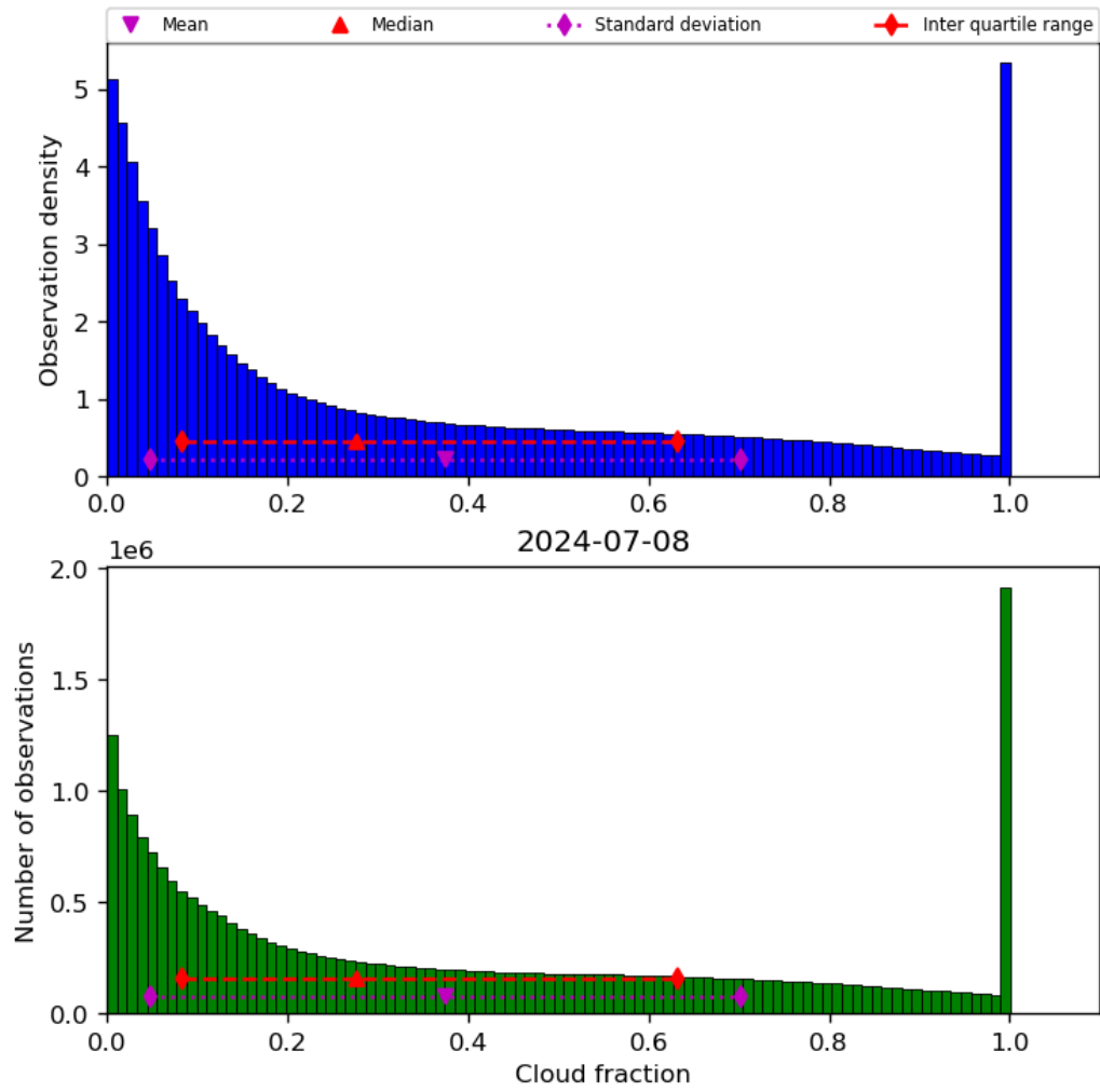
Figure 32: Histogram of “Cloud fraction” for 2024-07-07 to 2024-07-09
