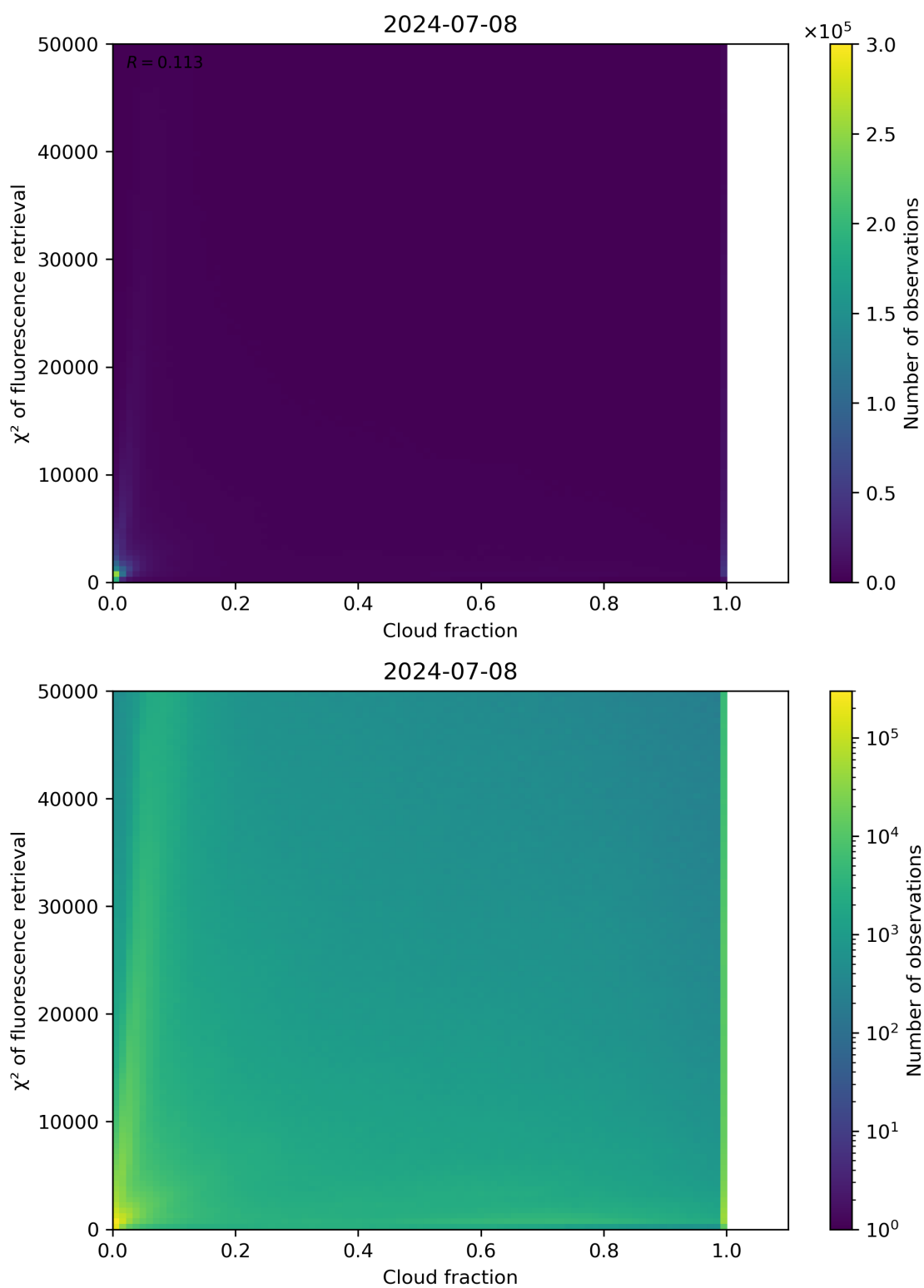
Figure 71: Scatter density plot of “Cloud fraction” against “ \chi^2 of fluorescence retrieval” for 2024-07-07 to 2024-07-09.
