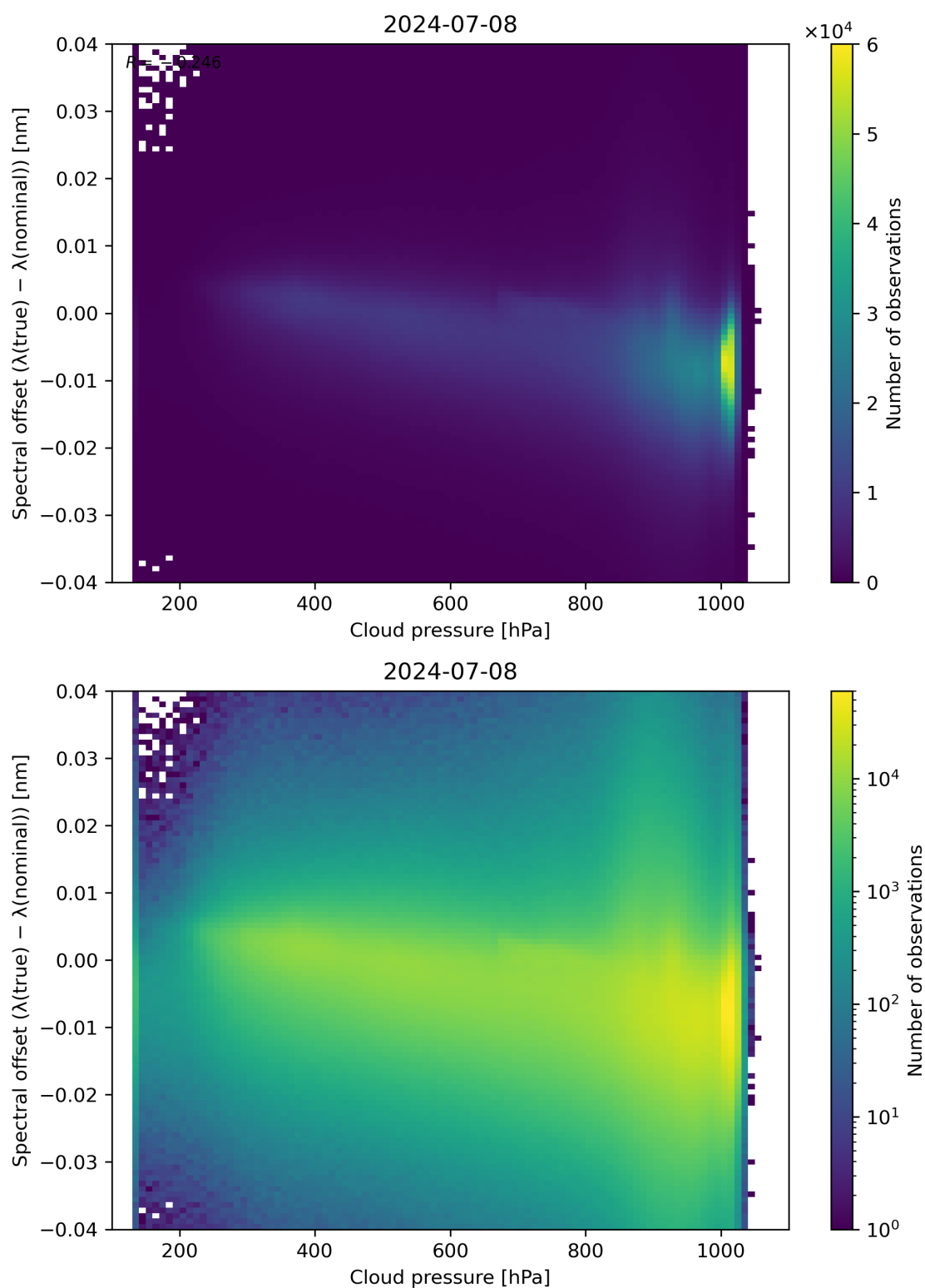
Figure 84: Scatter density plot of “Cloud pressure” against “Spectral offset ( \lambda(\text{true}) - \lambda(\text{nominal}) )” for 2024-07-07 to 2024-07-09.
