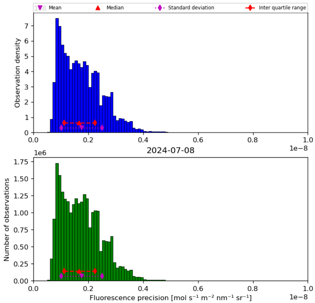
Figure 41: Histogram of “Fluorescence precision” for 2024-07-07 to 2024-07-09
