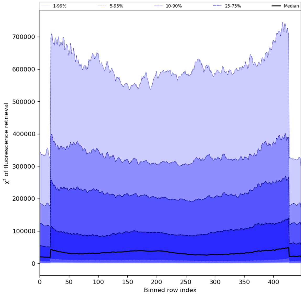
Figure 59: Along track statistics of “ \chi^2 of fluorescence retrieval” for 2024-07-07 to 2024-07-09
