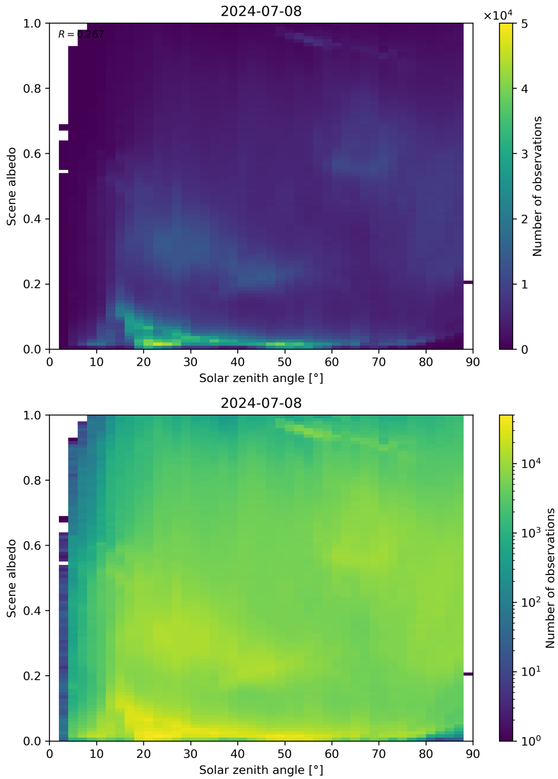
Figure 116: Scatter density plot of “Solar zenith angle” against “Scene albedo” for 2024-07-07 to 2024-07-09.
