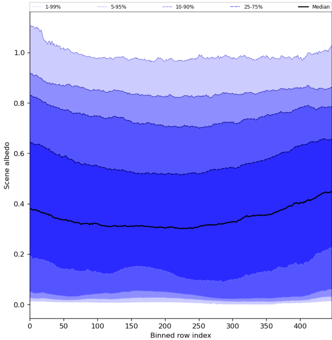
Figure 51: Along track statistics of “Scene albedo” for 2024-07-07 to 2024-07-09
