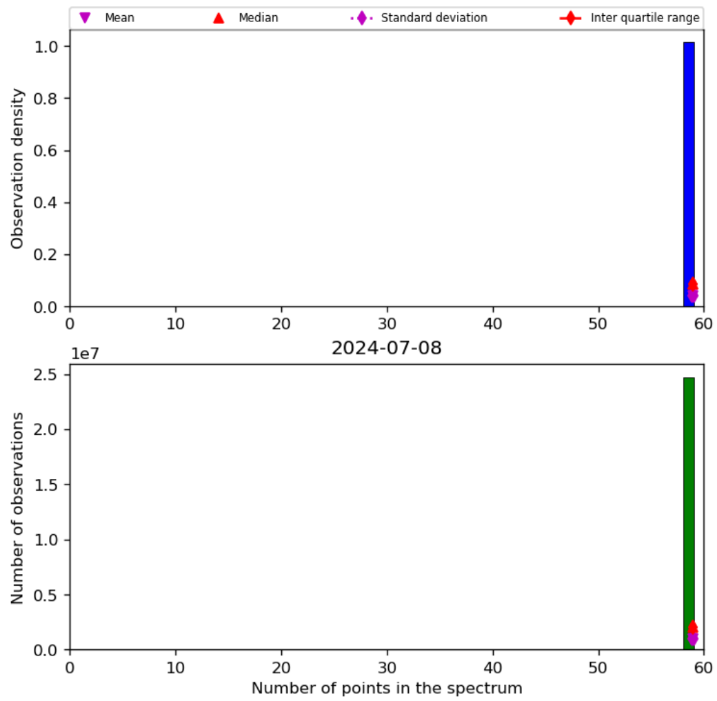
Figure 44: Histogram of “Number of points in the spectrum” for 2024-07-07 to 2024-07-09
