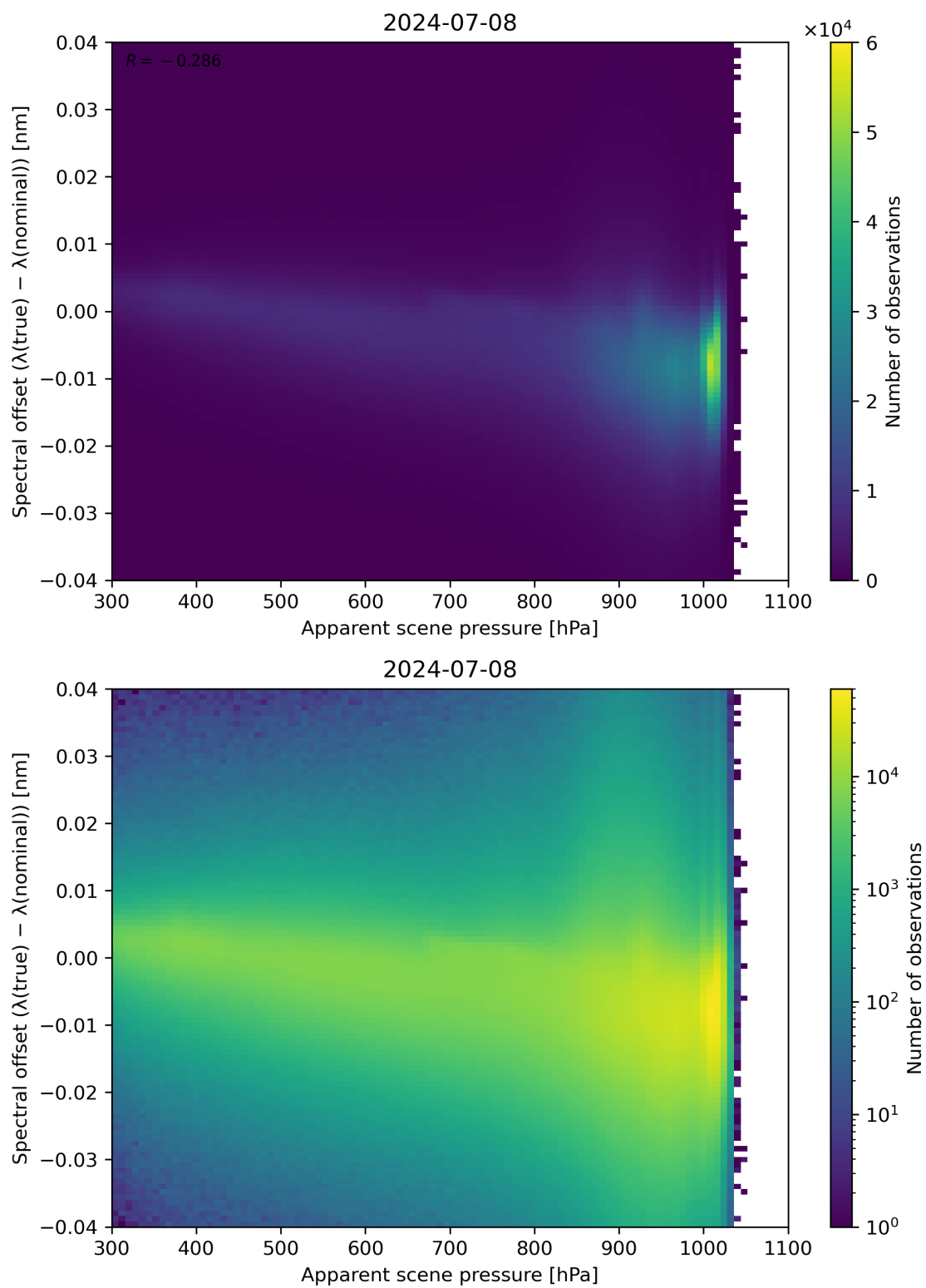
Figure 67: Scatter density plot of “Apparent scene pressure” against “Spectral offset ( \lambda(\text{true}) - \lambda(\text{nominal}) )” for 2024-07-07 to 2024-07-09.
