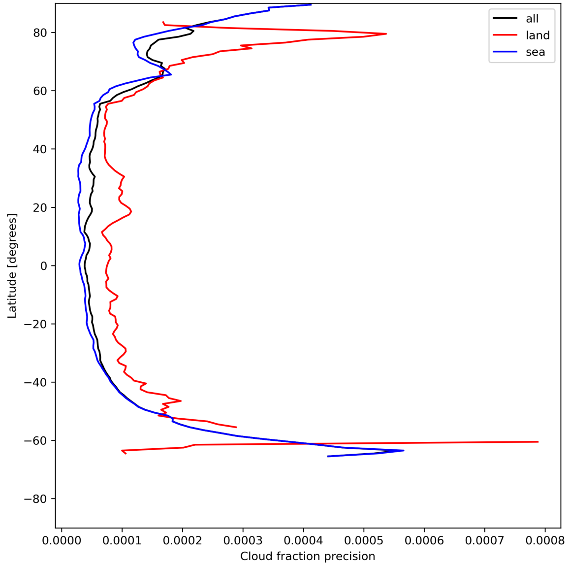
Figure 16: Zonal average of “Cloud fraction precision” for 2024-07-08 to 2024-07-10.
