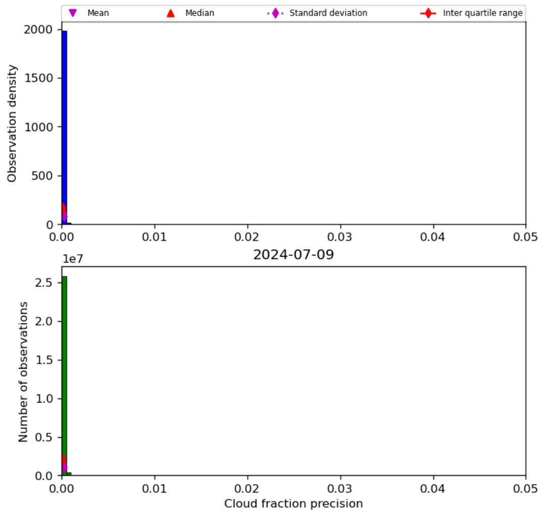
Figure 33: Histogram of “Cloud fraction precision” for 2024-07-08 to 2024-07-10
