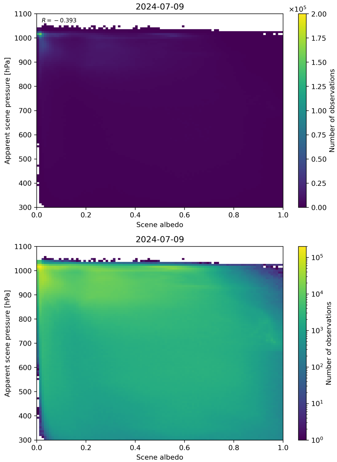
Figure 102: Scatter density plot of “Scene albedo” against “Apparent scene pressure” for 2024-07-08 to 2024-07-10.
