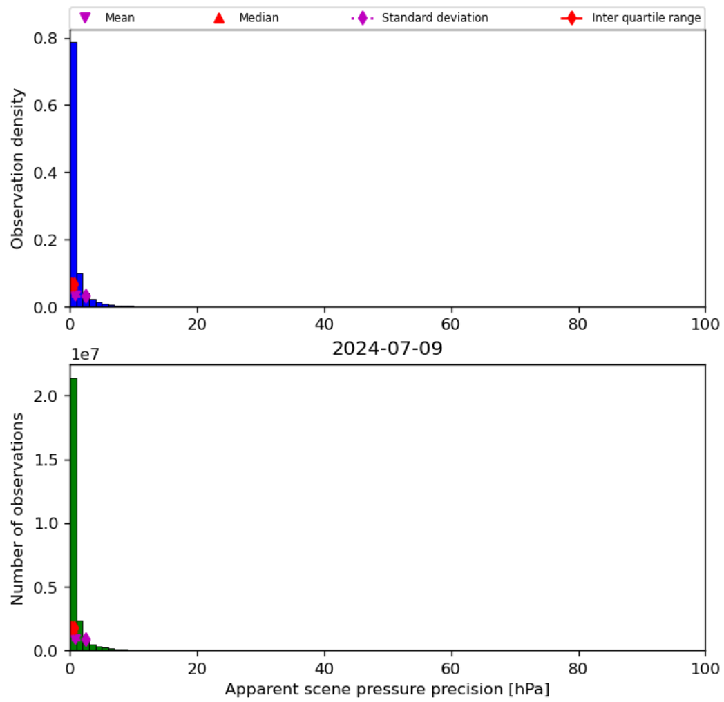
Figure 37: Histogram of “Apparent scene pressure precision” for 2024-07-08 to 2024-07-10
