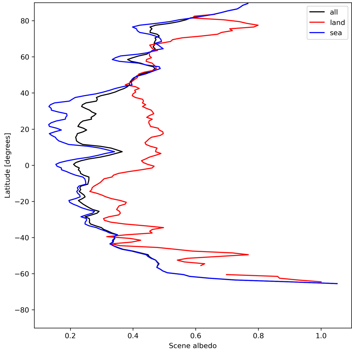
Figure 17: Zonal average of “Scene albedo” for 2024-07-08 to 2024-07-10.
