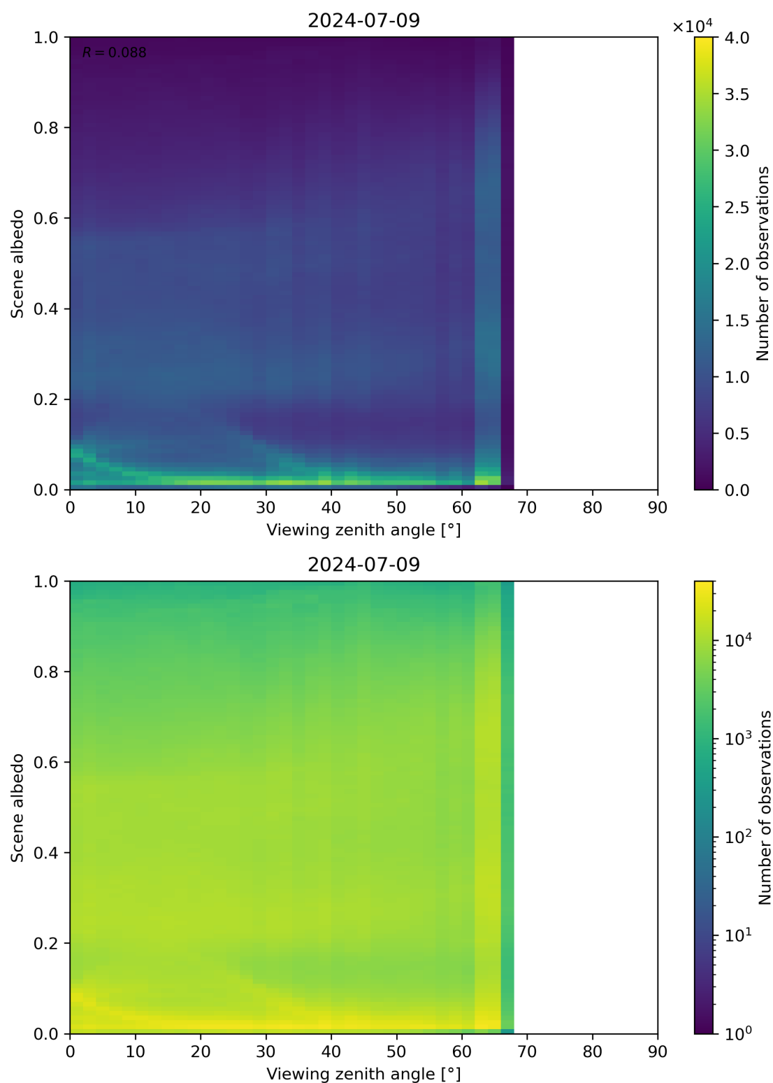
Figure 126: Scatter density plot of “Viewing zenith angle” against “Scene albedo” for 2024-07-08 to 2024-07-10.
