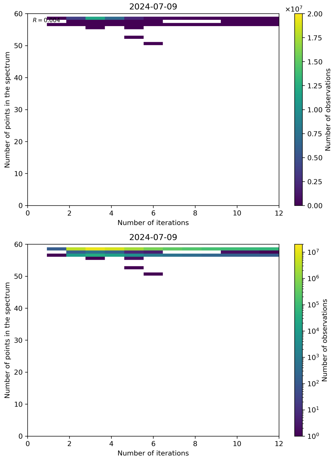
Figure 99: Scatter density plot of “Number of iterations” against “Number of points in the spectrum” for 2024-07-08 to 2024-07-10.
