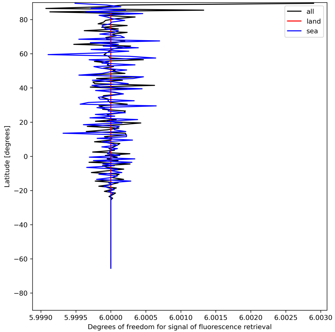
Figure 26: Zonal average of “Degrees of freedom for signal of fluorescence retrieval” for 2024-07-08 to 2024-07-10.
