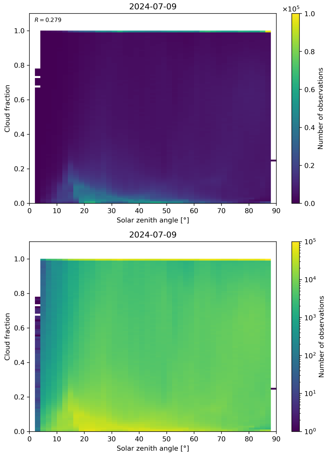
Figure 110: Scatter density plot of “Solar zenith angle” against “Cloud fraction” for 2024-07-08 to 2024-07-10.
