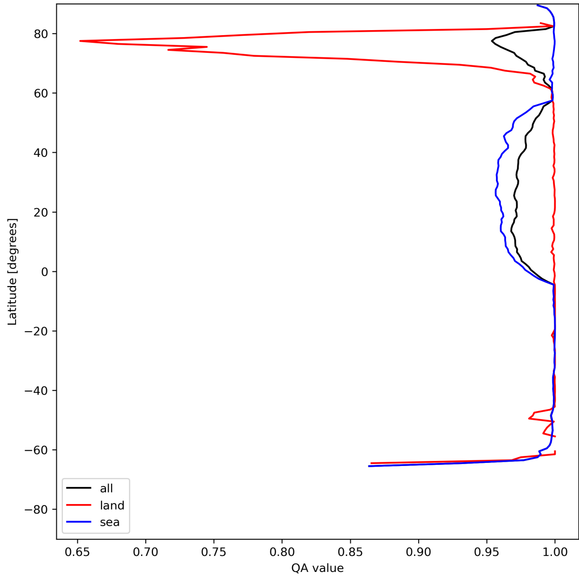
Figure 12: Zonal average of “QA value” for 2024-07-08 to 2024-07-10.
