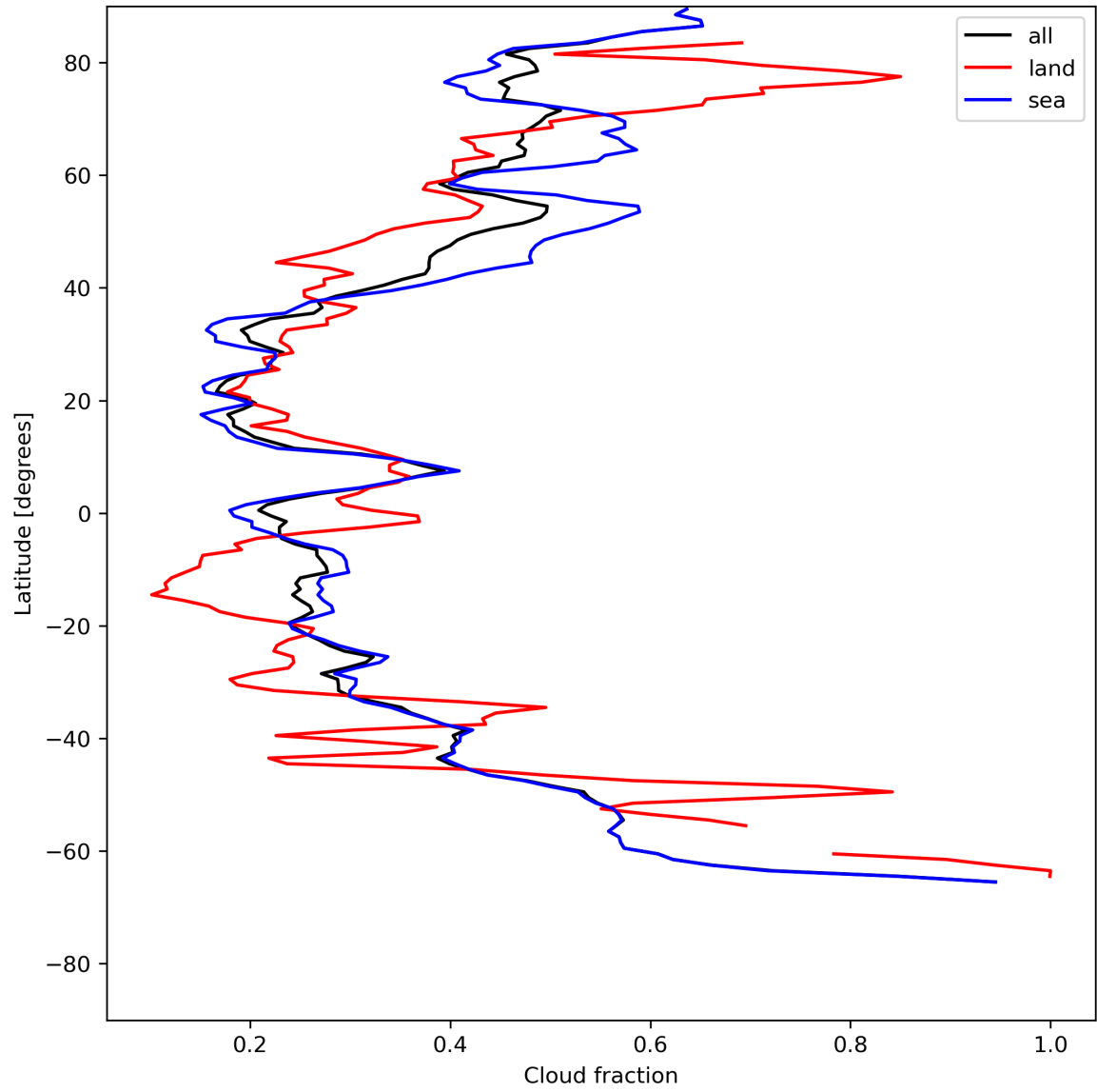
Figure 15: Zonal average of “Cloud fraction” for 2024-07-08 to 2024-07-10.
