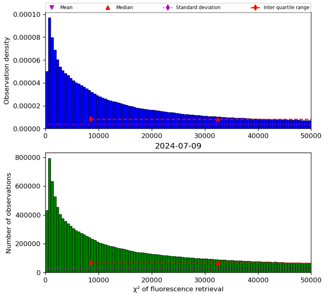
Figure 42: Histogram of “ \chi^2 of fluorescence retrieval” for 2024-07-08 to 2024-07-10
