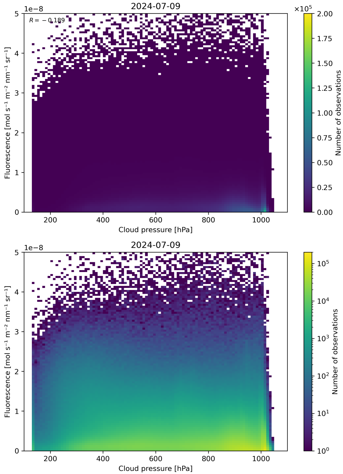
Figure 80: Scatter density plot of “Cloud pressure” against “Fluorescence” for 2024-07-08 to 2024-07-10.
