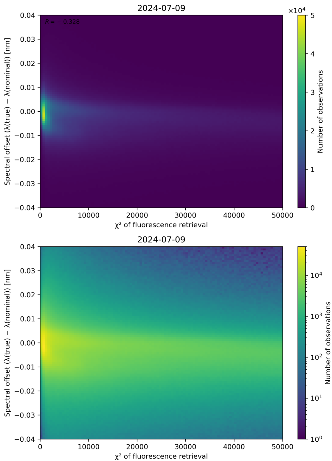
Figure 69: Scatter density plot of “ \chi^2 of fluorescence retrieval” against “Spectral offset ( \lambda(\text{true}) - \lambda(\text{nominal}) )” for 2024-07-08 to 2024-07-10.
