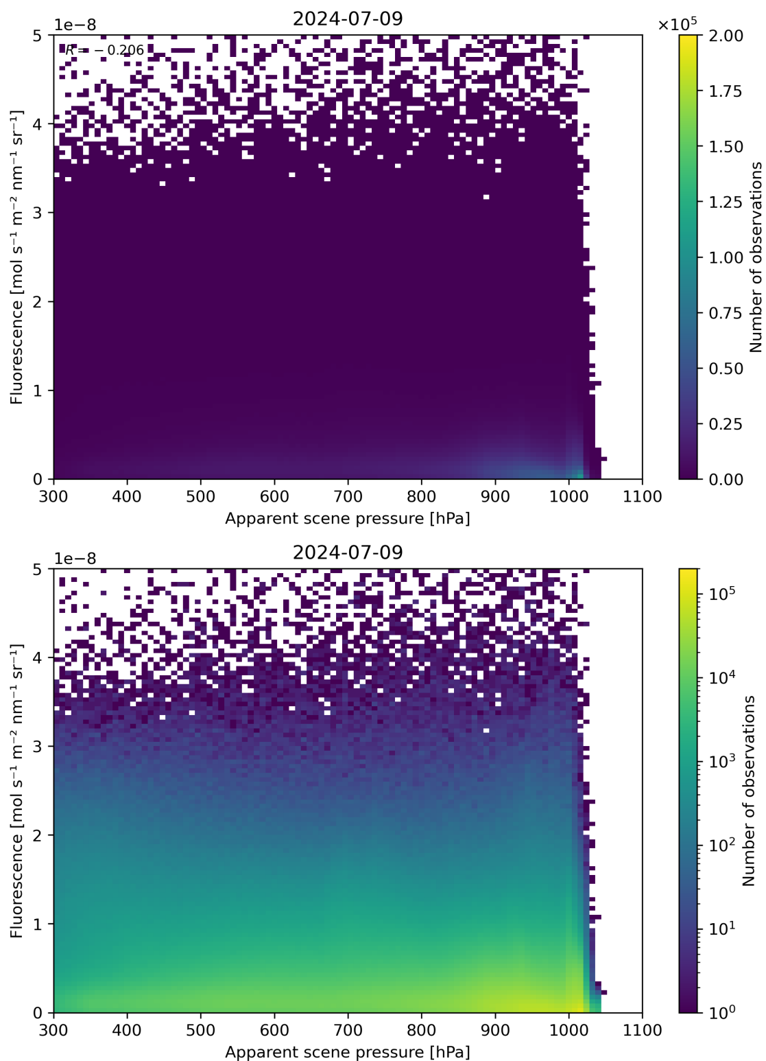
Figure 64: Scatter density plot of “Apparent scene pressure” against “Fluorescence” for 2024-07-08 to 2024-07-10.
