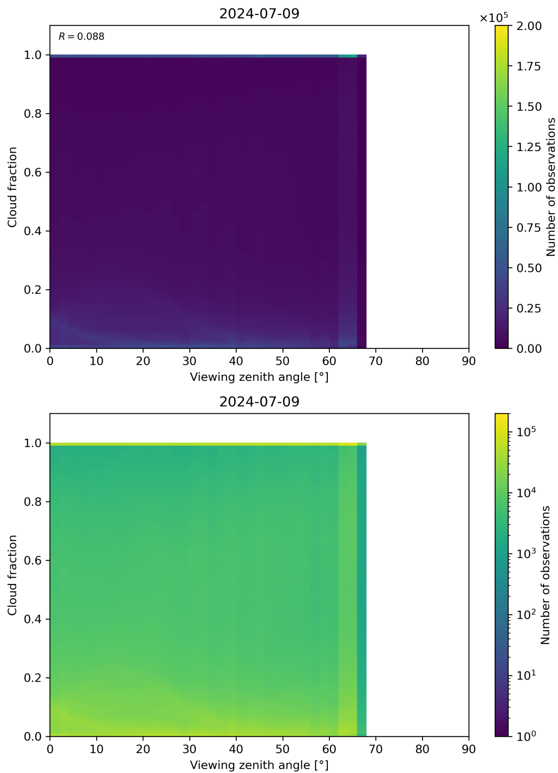
Figure 120: Scatter density plot of “Viewing zenith angle” against “Cloud fraction” for 2024-07-08 to 2024-07-10.
