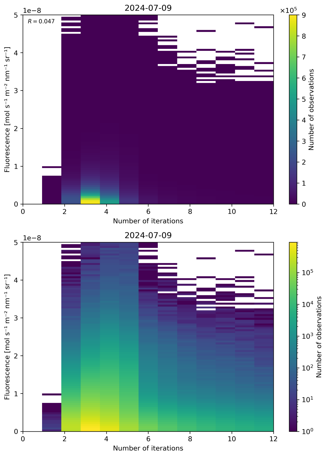
Figure 98: Scatter density plot of “Number of iterations” against “Fluorescence” for 2024-07-08 to 2024-07-10.
