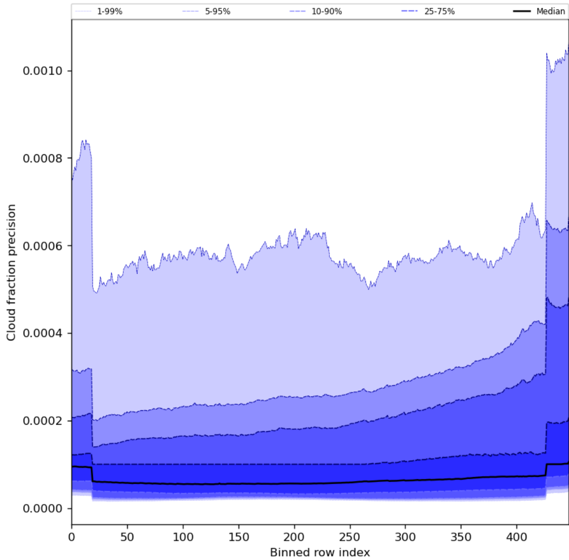
Figure 50: Along track statistics of “Cloud fraction precision” for 2024-07-08 to 2024-07-10
