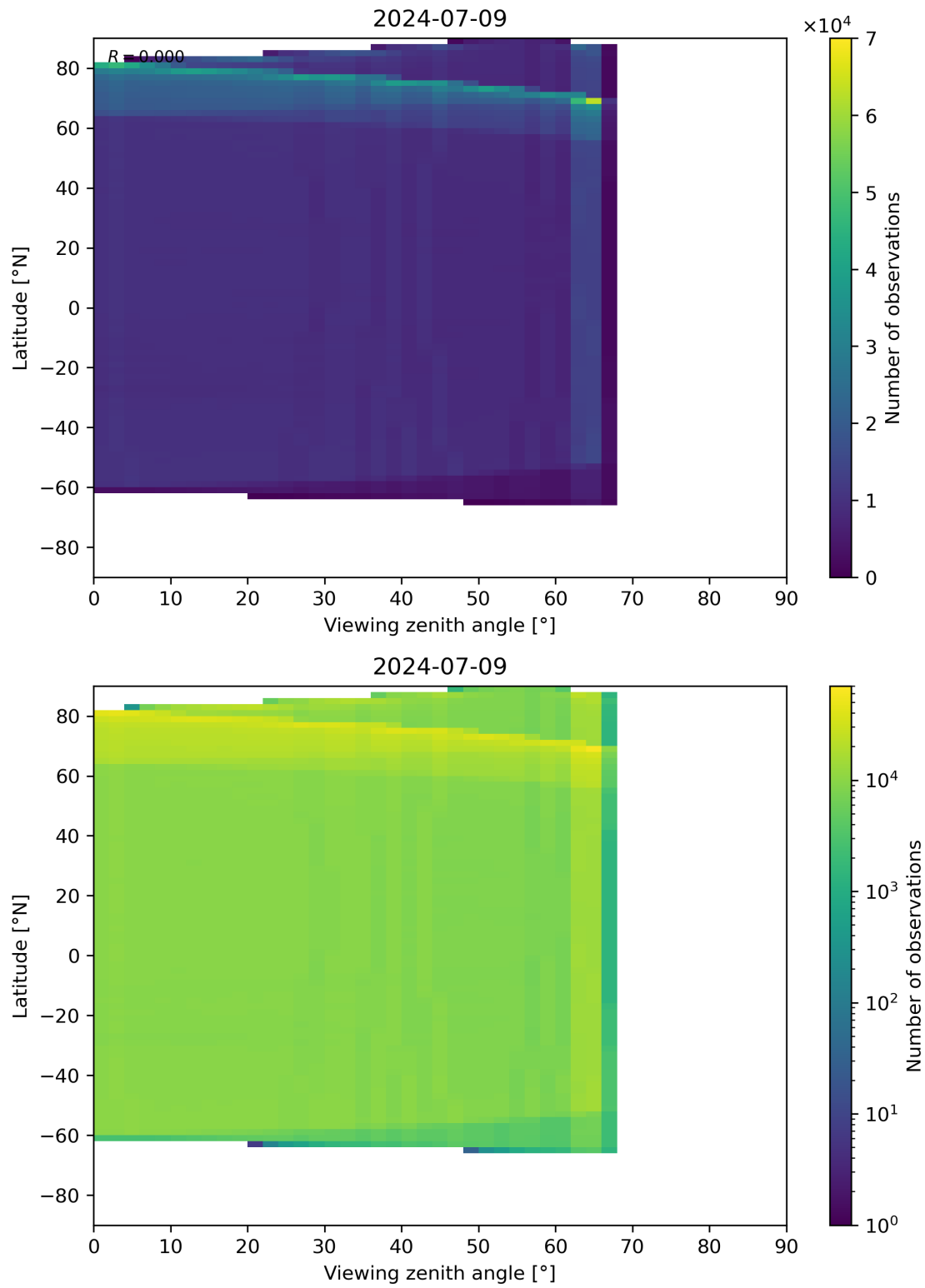
Figure 123: Scatter density plot of “Viewing zenith angle” against “Latitude” for 2024-07-08 to 2024-07-10.
