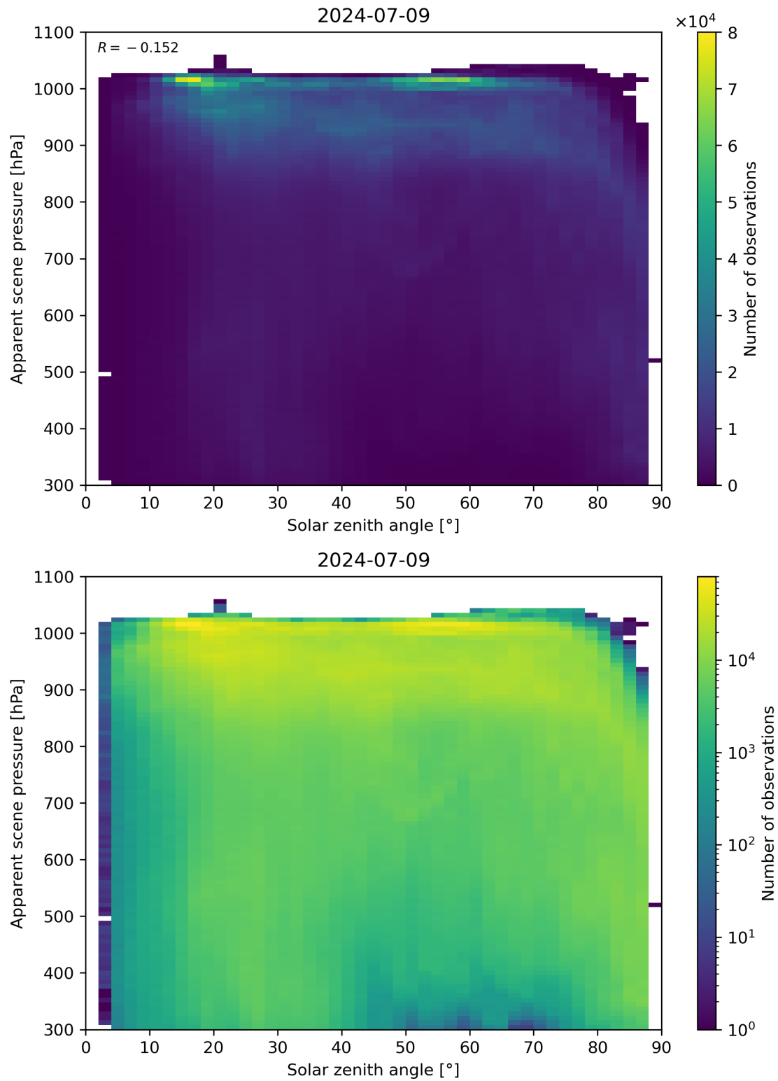
Figure 108: Scatter density plot of “Solar zenith angle” against “Apparent scene pressure” for 2024-07-08 to 2024-07-10.
