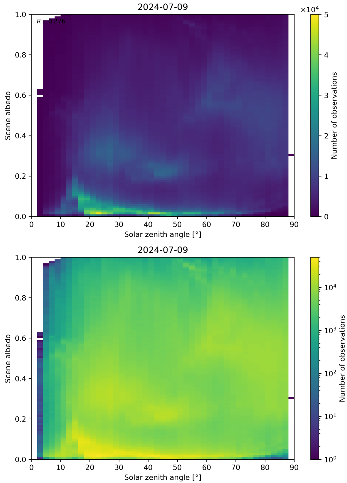
Figure 116: Scatter density plot of “Solar zenith angle” against “Scene albedo” for 2024-07-08 to 2024-07-10.
