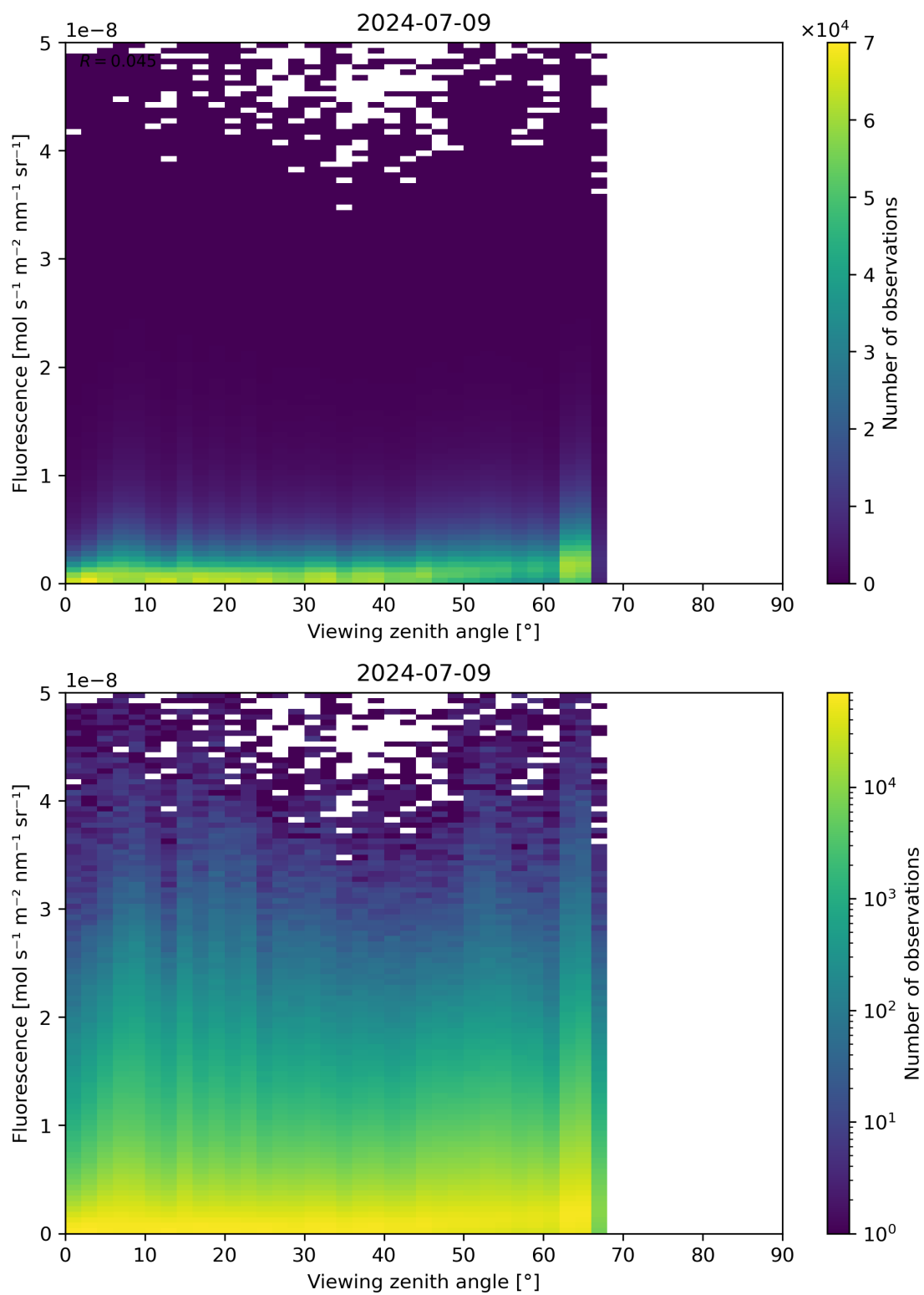
Figure 122: Scatter density plot of “Viewing zenith angle” against “Fluorescence” for 2024-07-08 to 2024-07-10.
