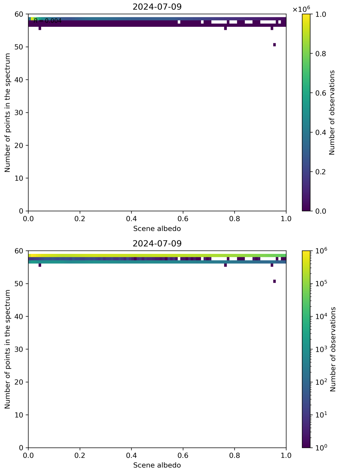
Figure 106: Scatter density plot of “Scene albedo” against “Number of points in the spectrum” for 2024-07-08 to 2024-07-10.
