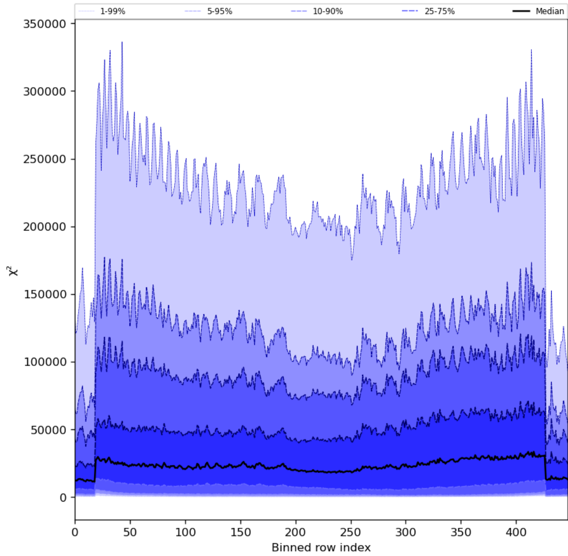
Figure 55: Along track statistics of “ \chi^2 ” for 2024-07-08 to 2024-07-10
