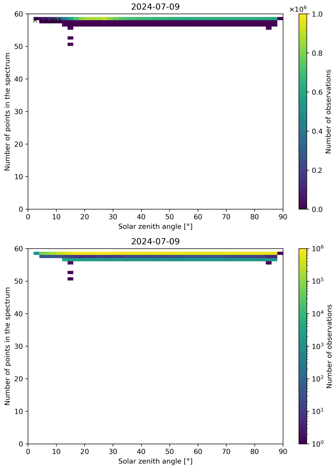
Figure 115: Scatter density plot of “Solar zenith angle” against “Number of points in the spectrum” for 2024-07-08 to 2024-07-10.
