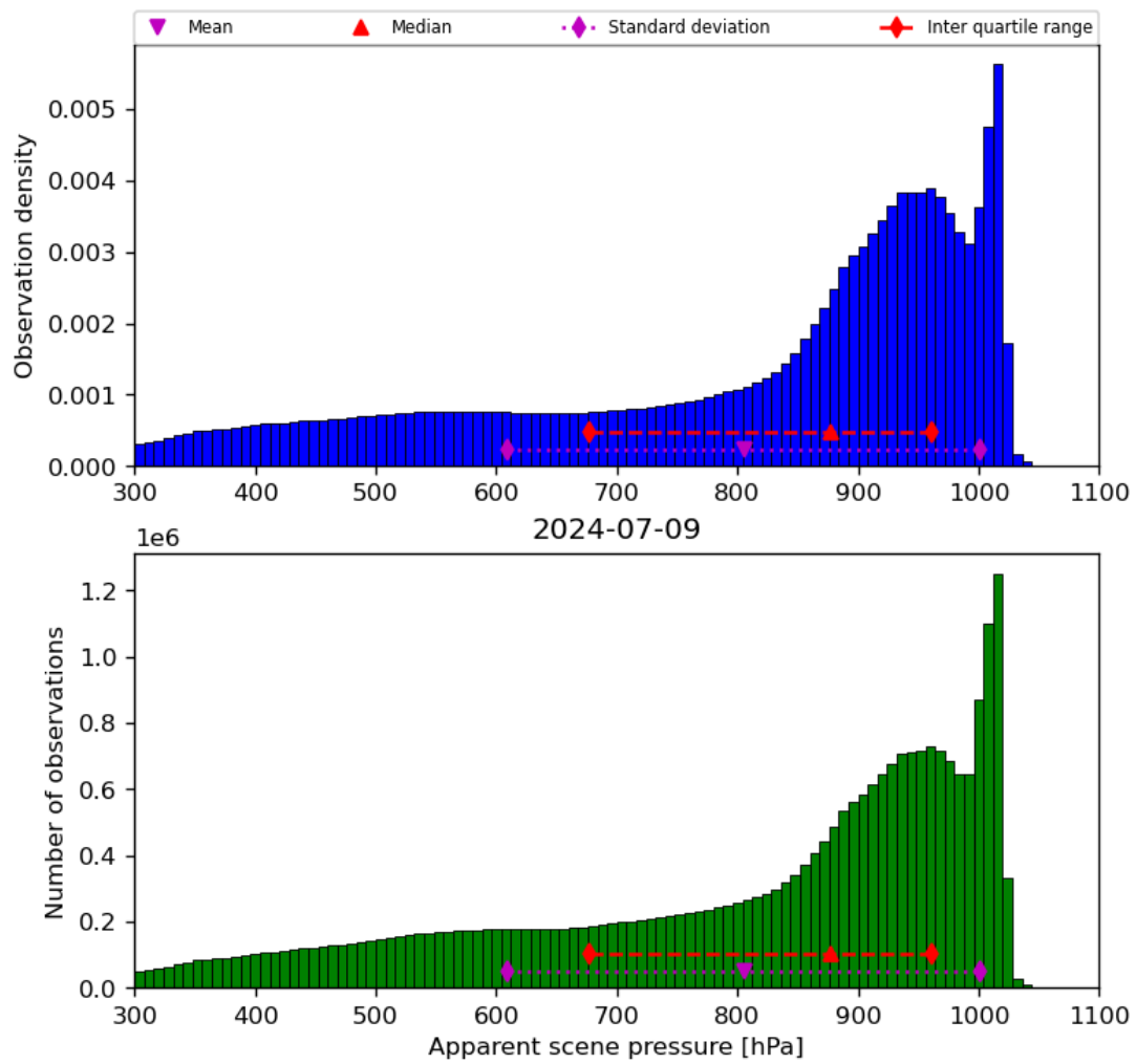
Figure 36: Histogram of “Apparent scene pressure” for 2024-07-08 to 2024-07-10
