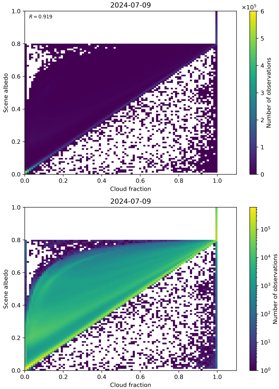
Figure 75: Scatter density plot of “Cloud fraction” against “Scene albedo” for 2024-07-08 to 2024-07-10.
