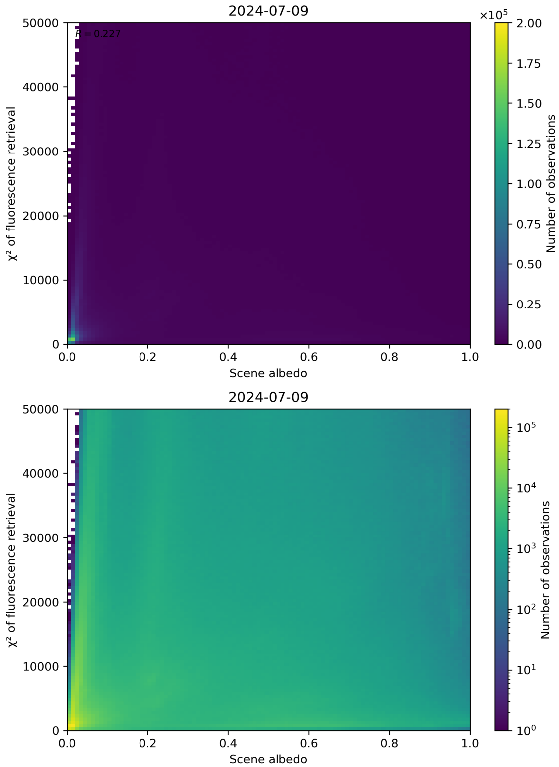
Figure 103: Scatter density plot of “Scene albedo” against “ \chi^2 of fluorescence retrieval” for 2024-07-08 to 2024-07-10.
