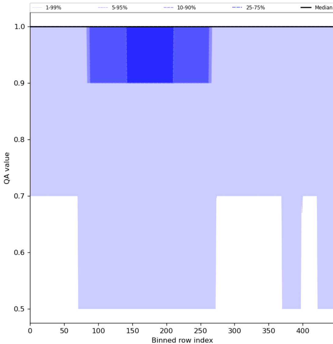
Figure 46: Along track statistics of “QA value” for 2024-07-08 to 2024-07-10
