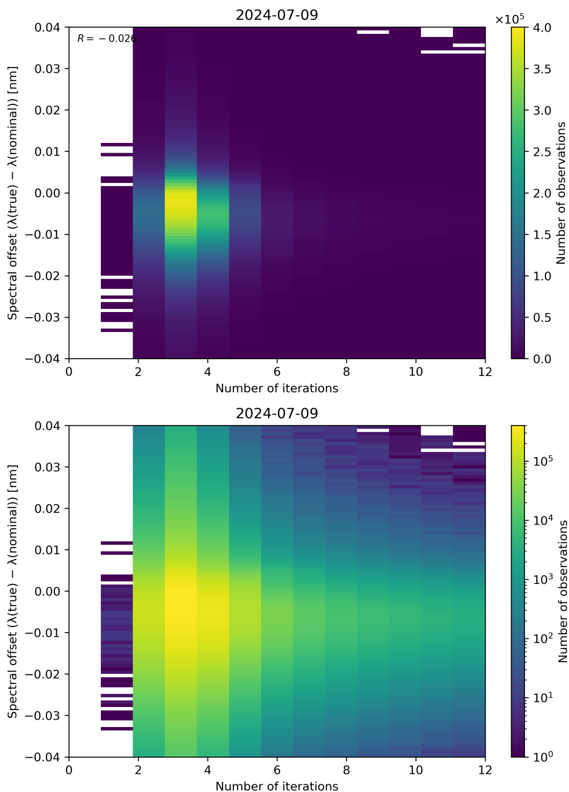
Figure 100: Scatter density plot of “Number of iterations” against “Spectral offset ( \lambda(\text{true}) - \lambda(\text{nominal}) )” for 2024-07-08 to 2024-07-10.
