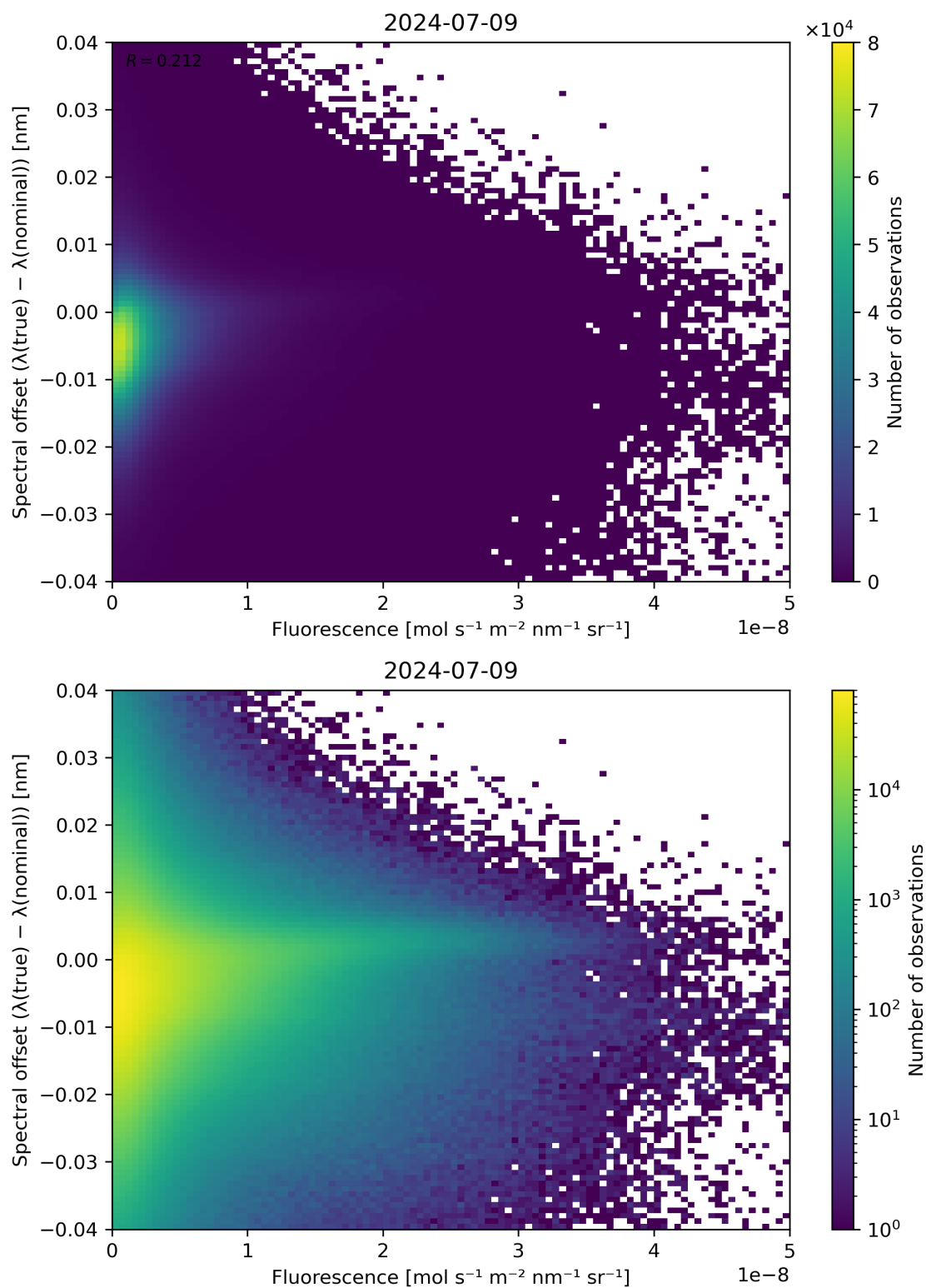
Figure 87: Scatter density plot of “Fluorescence” against “Spectral offset ( \lambda(\text{true}) - \lambda(\text{nominal}) )” for 2024-07-08 to 2024-07-10.
