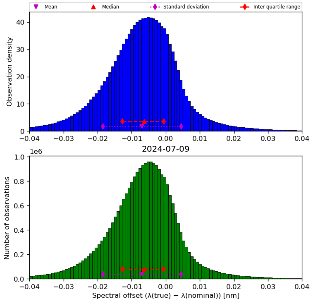
Figure 45: Histogram of “Spectral offset ( \lambda(\text{true}) - \lambda(\text{nominal}) )” for 2024-07-08 to 2024-07-10
