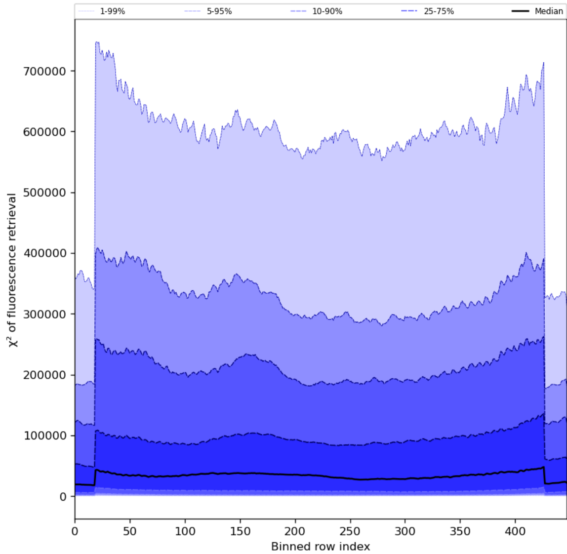
Figure 59: Along track statistics of “ \chi^2 of fluorescence retrieval” for 2024-07-08 to 2024-07-10
