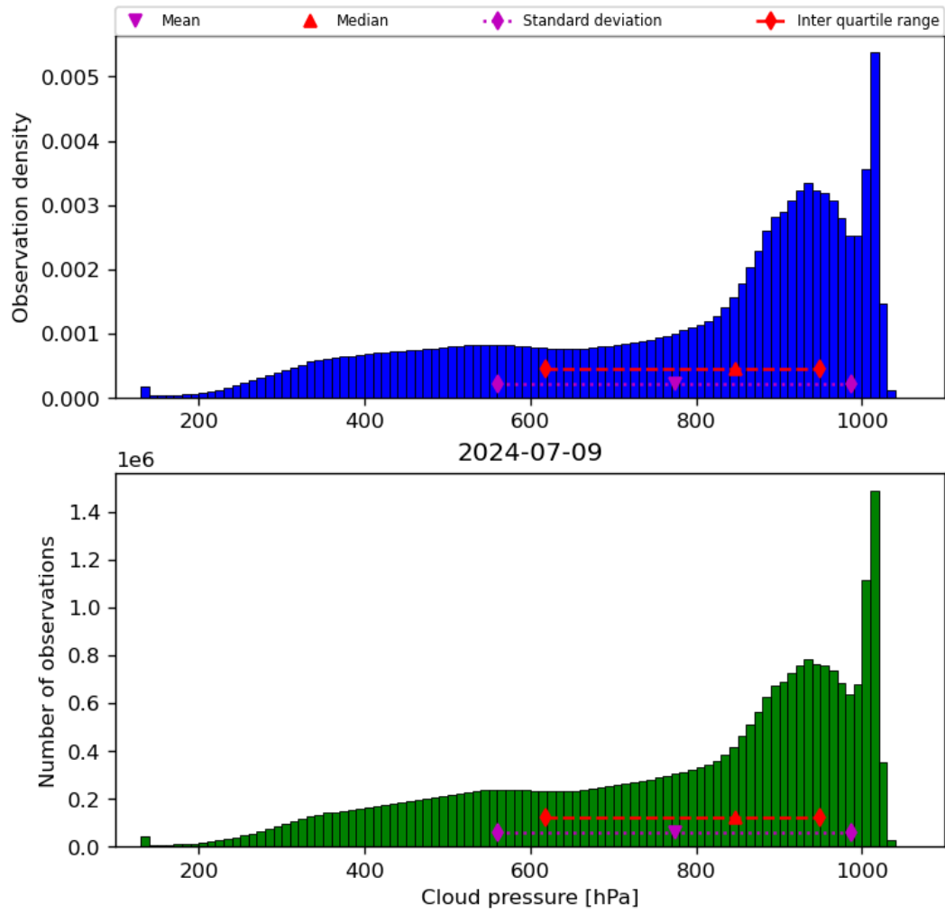
Figure 30: Histogram of “Cloud pressure” for 2024-07-08 to 2024-07-10
