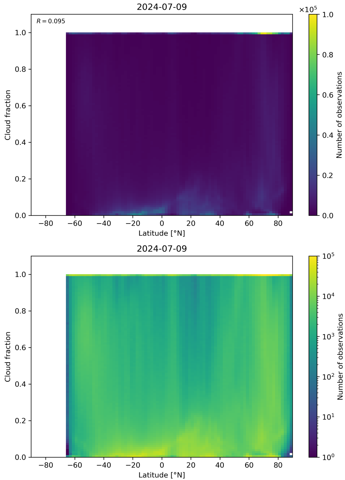
Figure 90: Scatter density plot of “Latitude” against “Cloud fraction” for 2024-07-08 to 2024-07-10.
