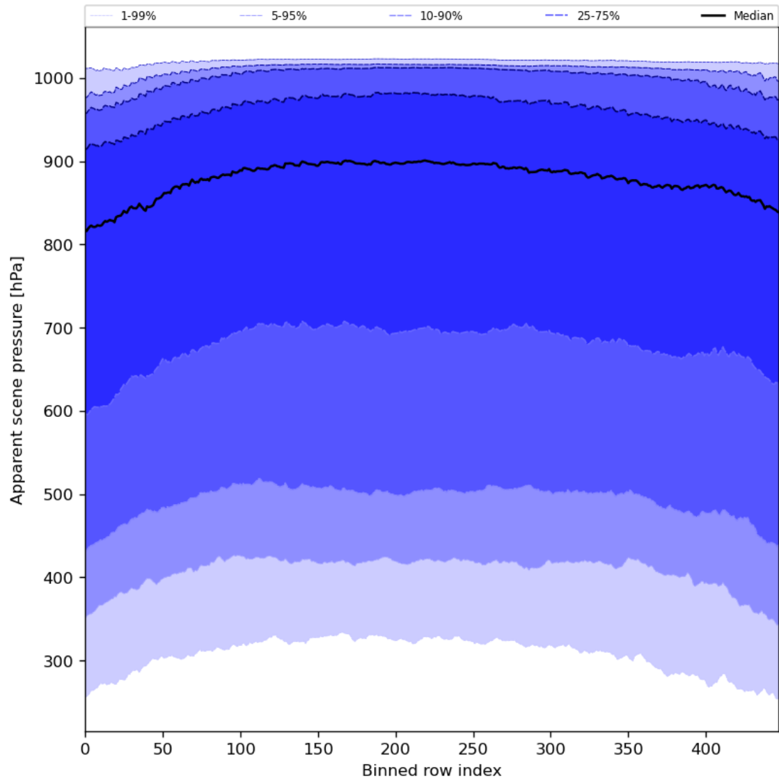
Figure 53: Along track statistics of “Apparent scene pressure” for 2024-07-08 to 2024-07-10
