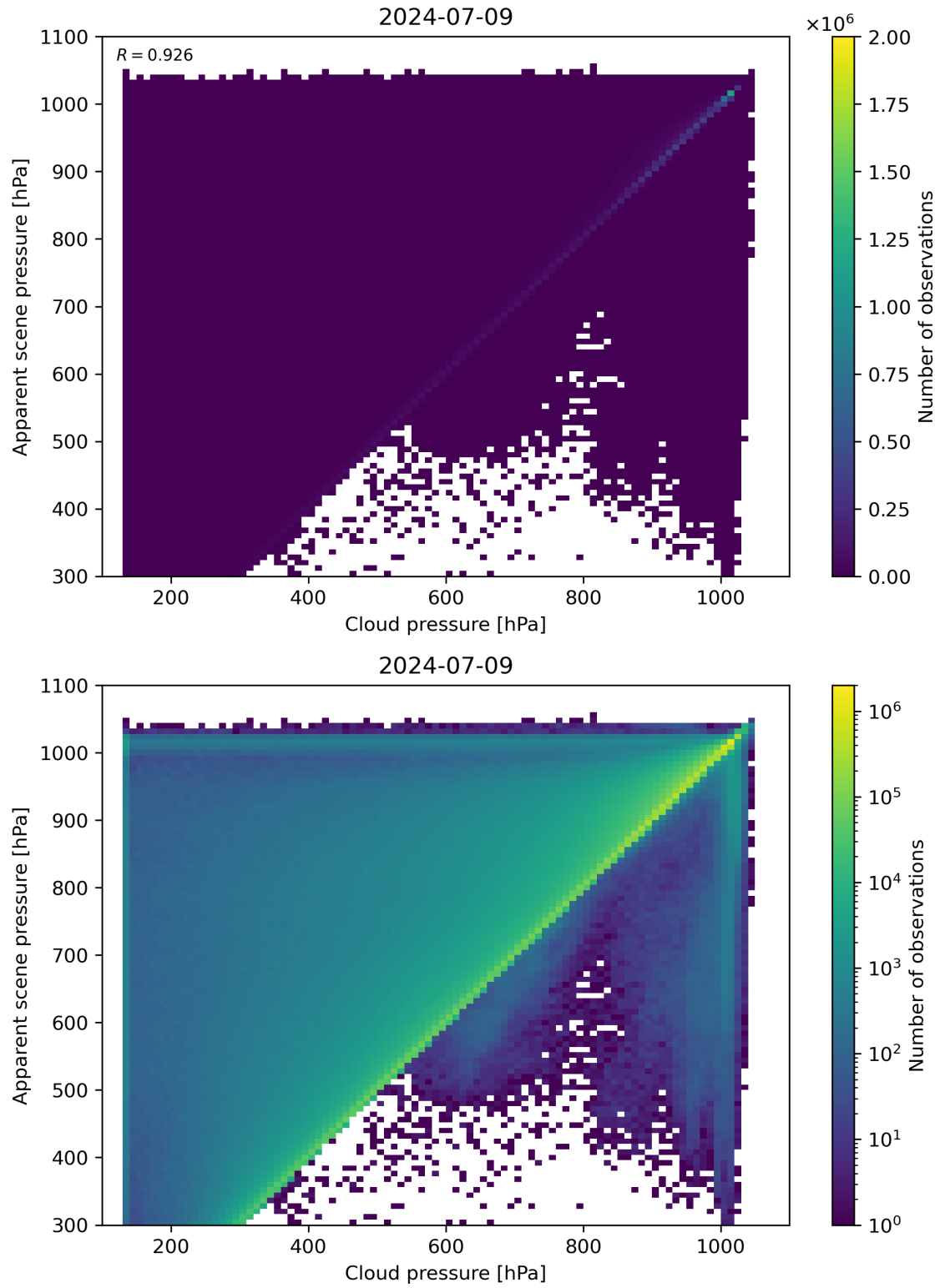
Figure 77: Scatter density plot of “Cloud pressure” against “Apparent scene pressure” for 2024-07-08 to 2024-07-10.
