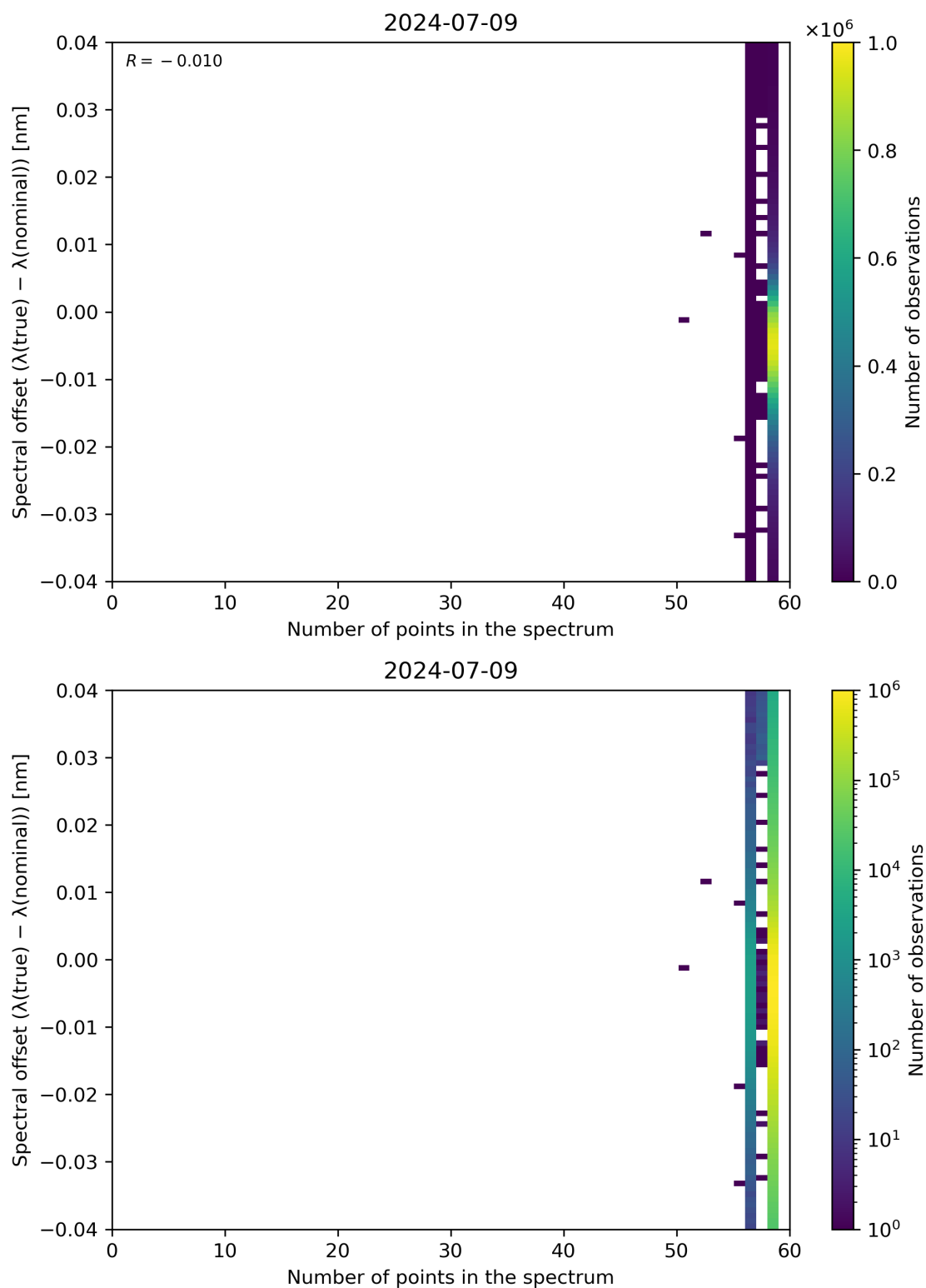
Figure 101: Scatter density plot of “Number of points in the spectrum” against “Spectral offset ( \lambda(\text{true}) - \lambda(\text{nominal}) )” for 2024-07-08 to 2024-07-10.
