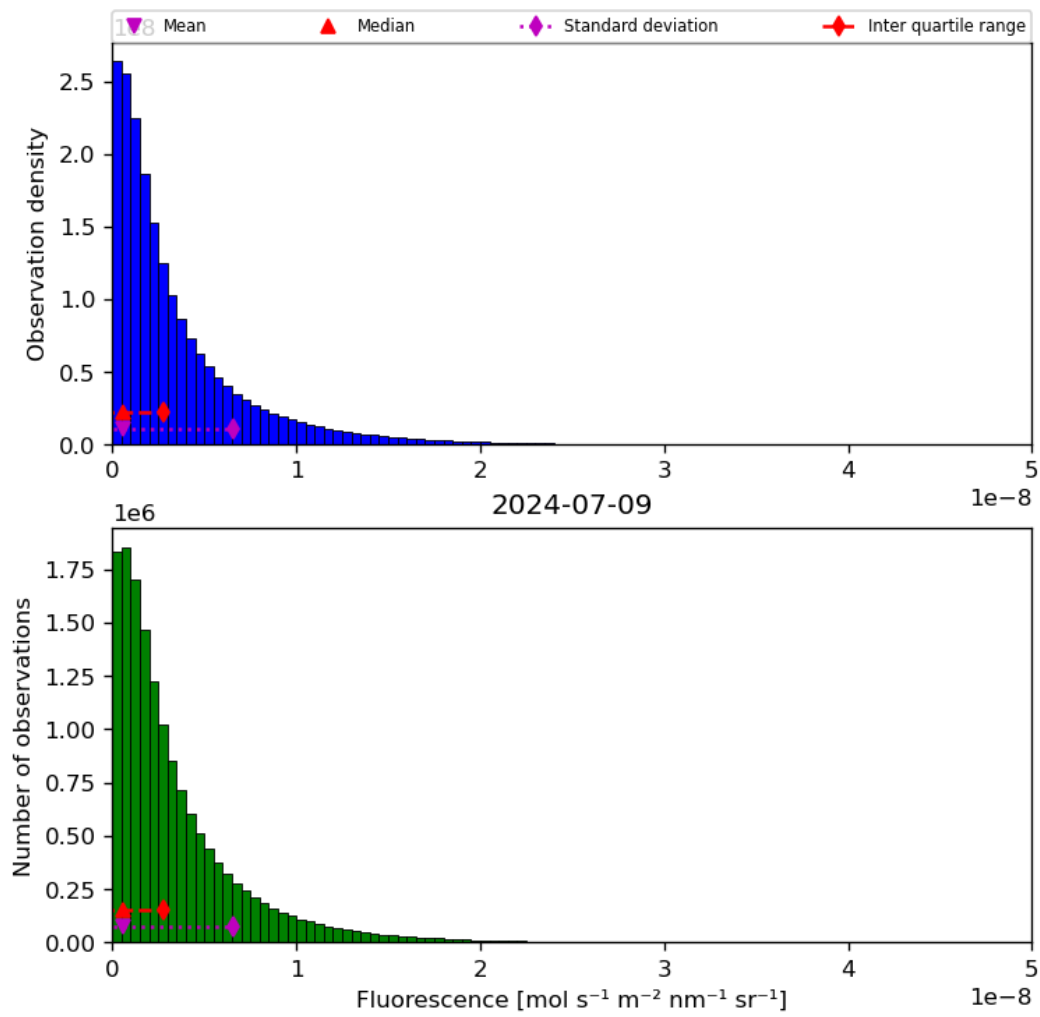
Figure 40: Histogram of “Fluorescence” for 2024-07-08 to 2024-07-10
