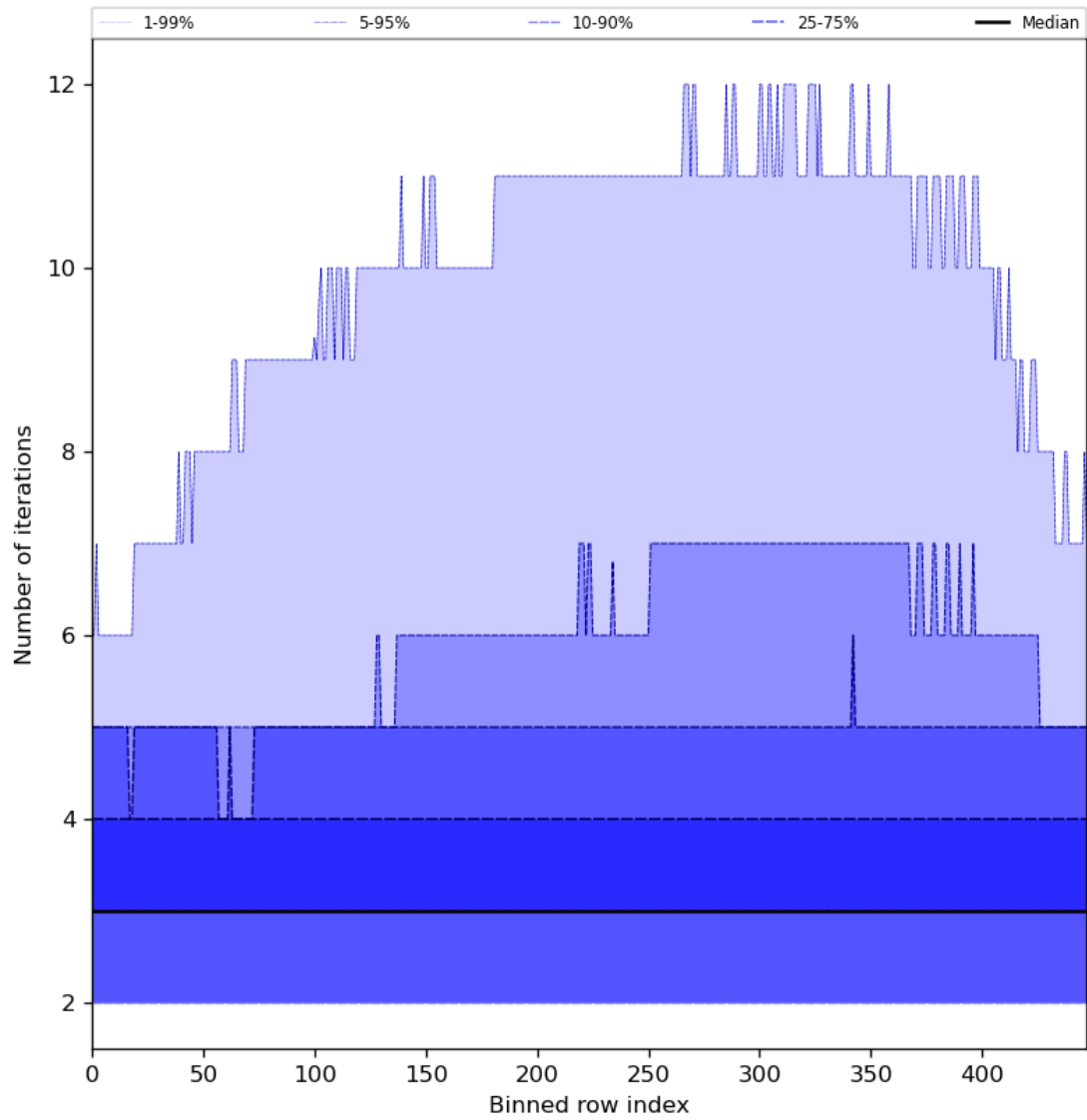
Figure 56: Along track statistics of “Number of iterations” for 2024-07-08 to 2024-07-10
