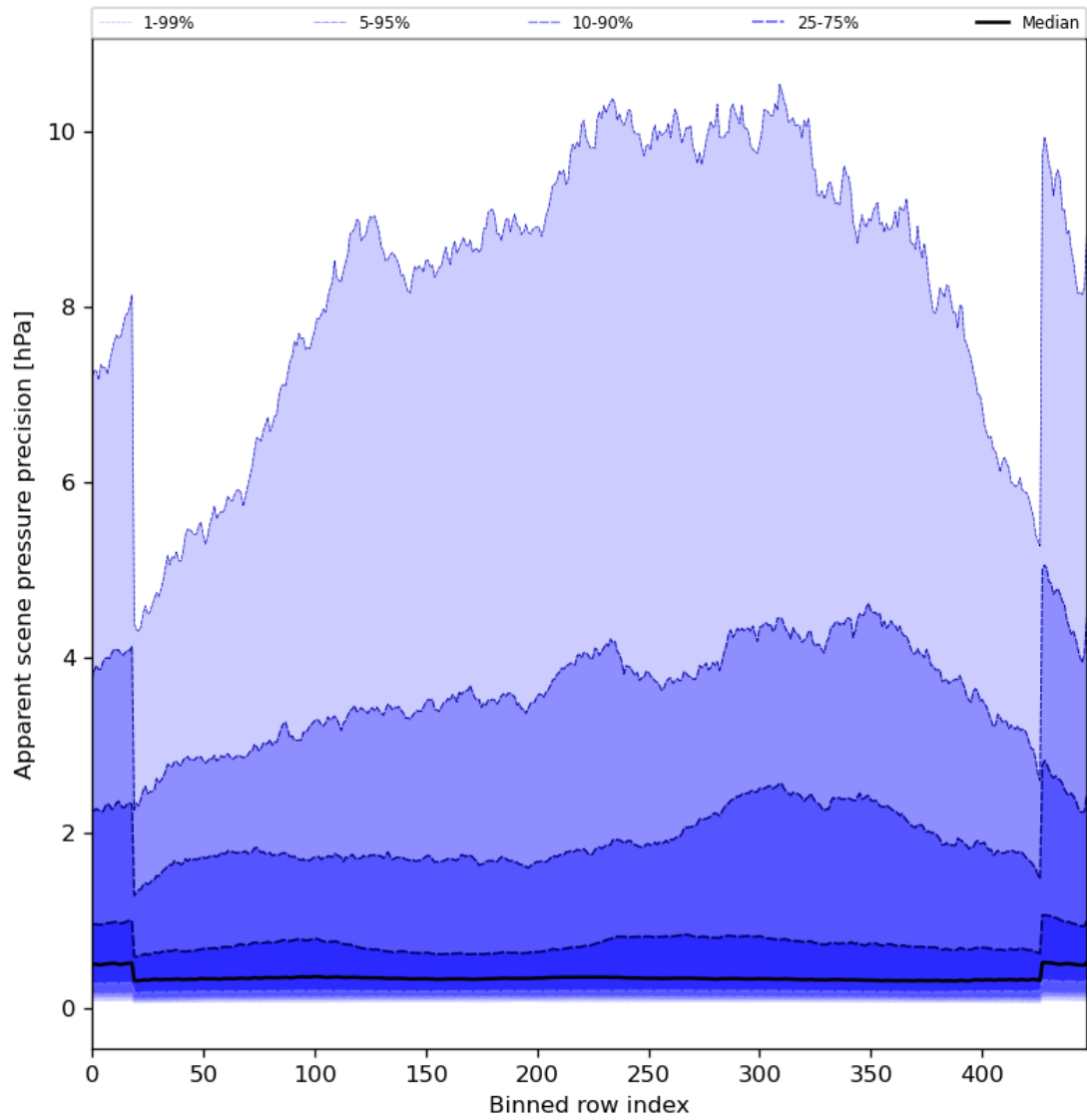
Figure 54: Along track statistics of “Apparent scene pressure precision” for 2024-07-08 to 2024-07-10
