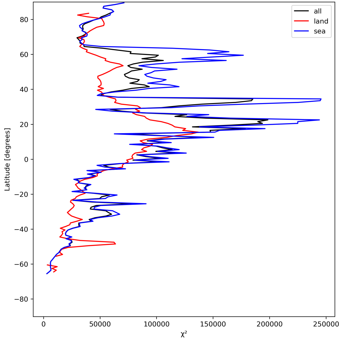
Figure 21: Zonal average of “ \chi^2 ” for 2024-07-08 to 2024-07-10.
