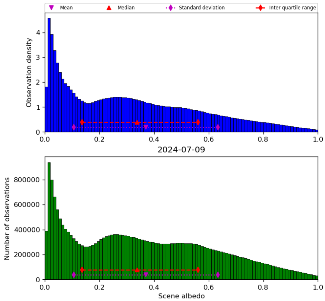
Figure 34: Histogram of “Scene albedo” for 2024-07-08 to 2024-07-10
