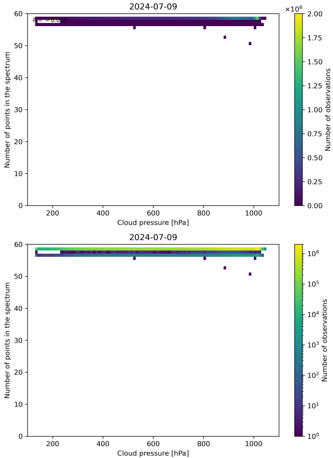
Figure 82: Scatter density plot of “Cloud pressure” against “Number of points in the spectrum” for 2024-07-08 to 2024-07-10.
