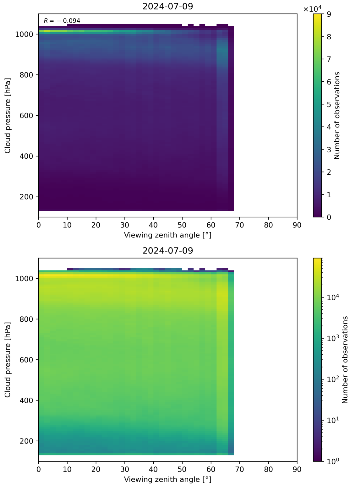
Figure 121: Scatter density plot of “Viewing zenith angle” against “Cloud pressure” for 2024-07-08 to 2024-07-10.
