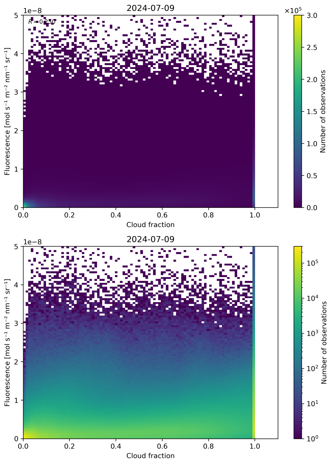
Figure 72: Scatter density plot of "Cloud fraction" against "Fluorescence" for 2024-07-08 to 2024-07-10.
