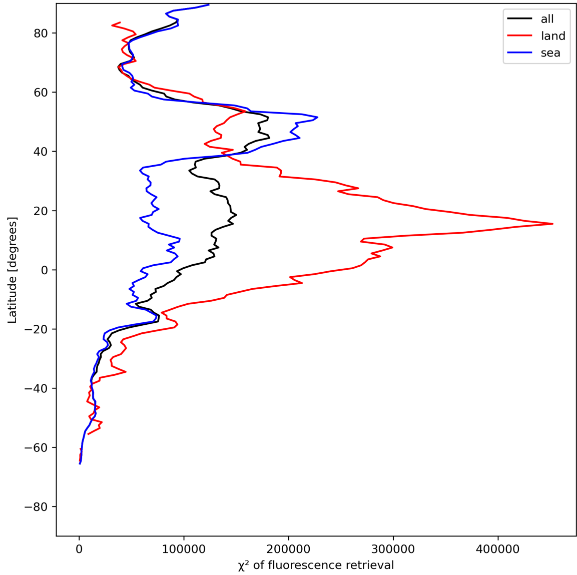
Figure 25: Zonal average of “ \chi^2 of fluorescence retrieval” for 2024-07-08 to 2024-07-10.
