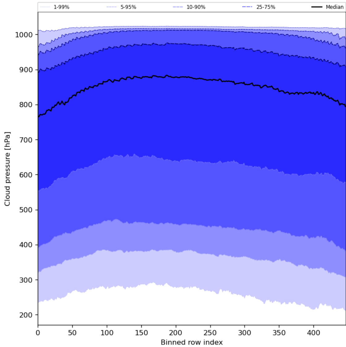
Figure 47: Along track statistics of “Cloud pressure” for 2024-07-08 to 2024-07-10
