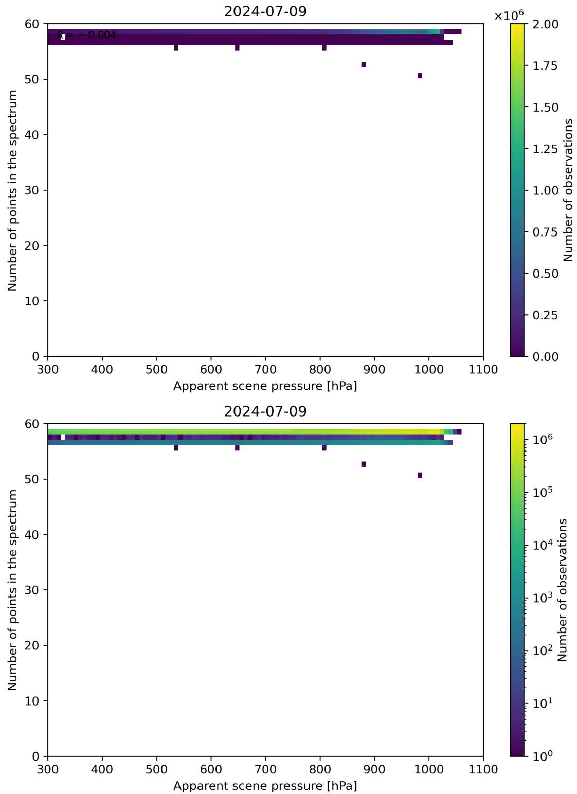
Figure 66: Scatter density plot of “Apparent scene pressure” against “Number of points in the spectrum” for 2024-07-08 to 2024-07-10.
