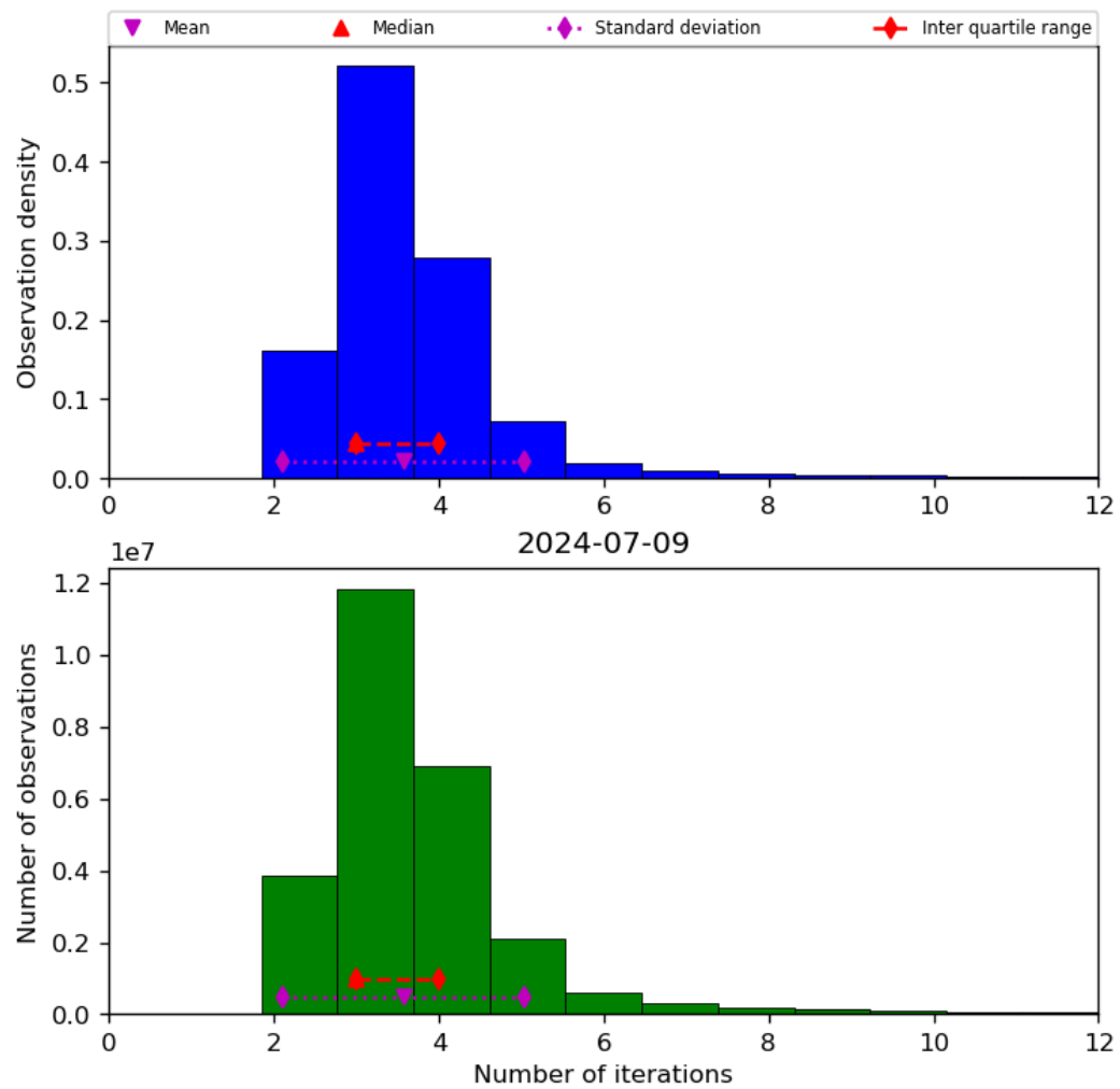
Figure 39: Histogram of “Number of iterations” for 2024-07-08 to 2024-07-10
