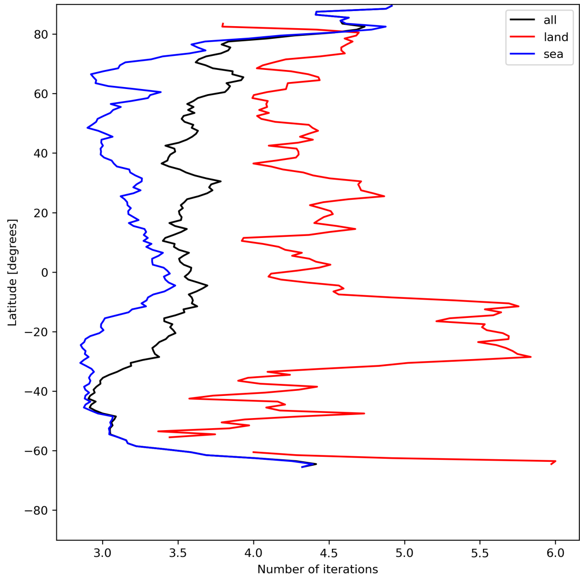
Figure 22: Zonal average of “Number of iterations” for 2024-07-08 to 2024-07-10.
