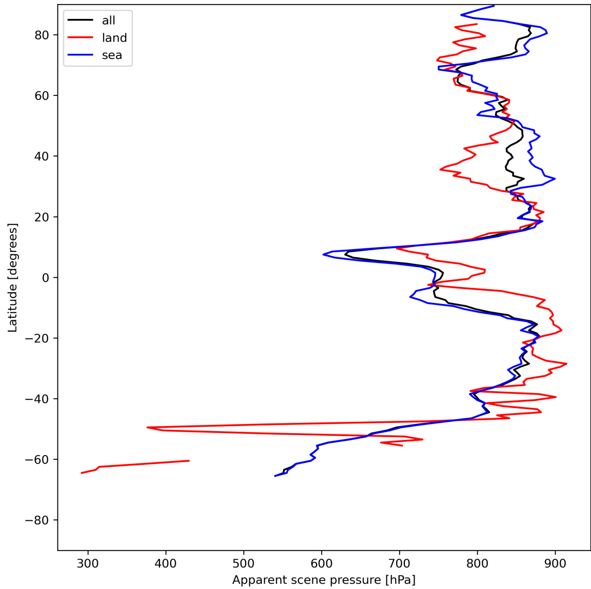
Figure 19: Zonal average of “Apparent scene pressure” for 2024-07-08 to 2024-07-10.
