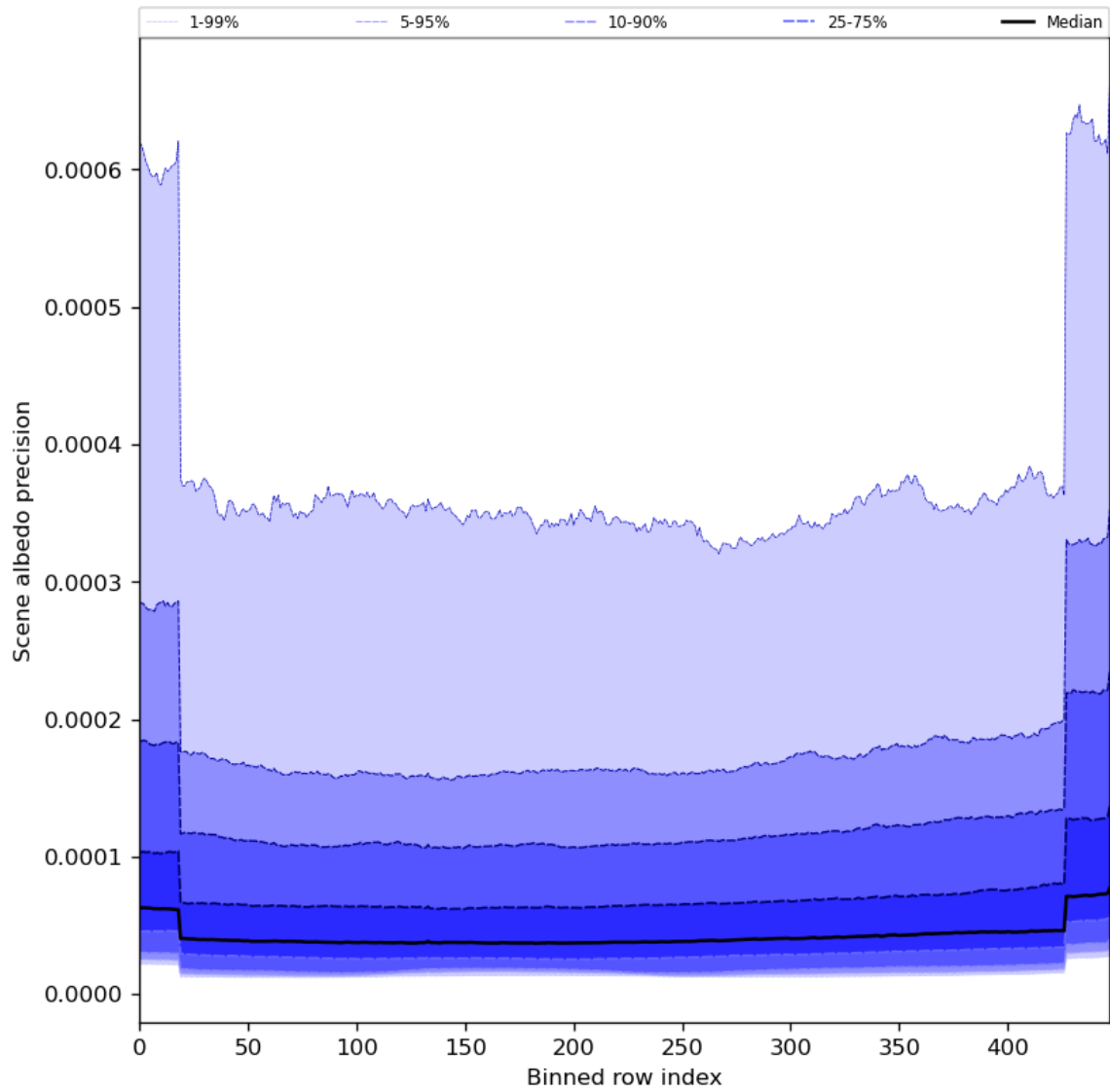
Figure 52: Along track statistics of “Scene albedo precision” for 2024-07-08 to 2024-07-10
