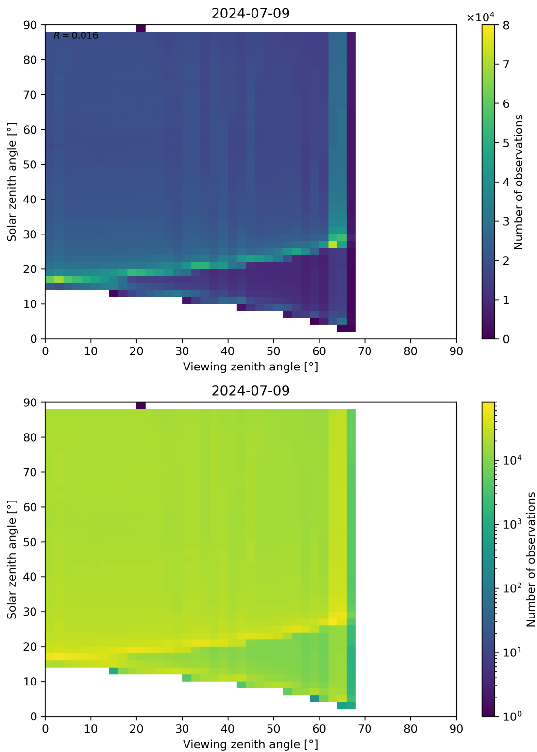
Figure 127: Scatter density plot of “Viewing zenith angle” against “Solar zenith angle” for 2024-07-08 to 2024-07-10.
