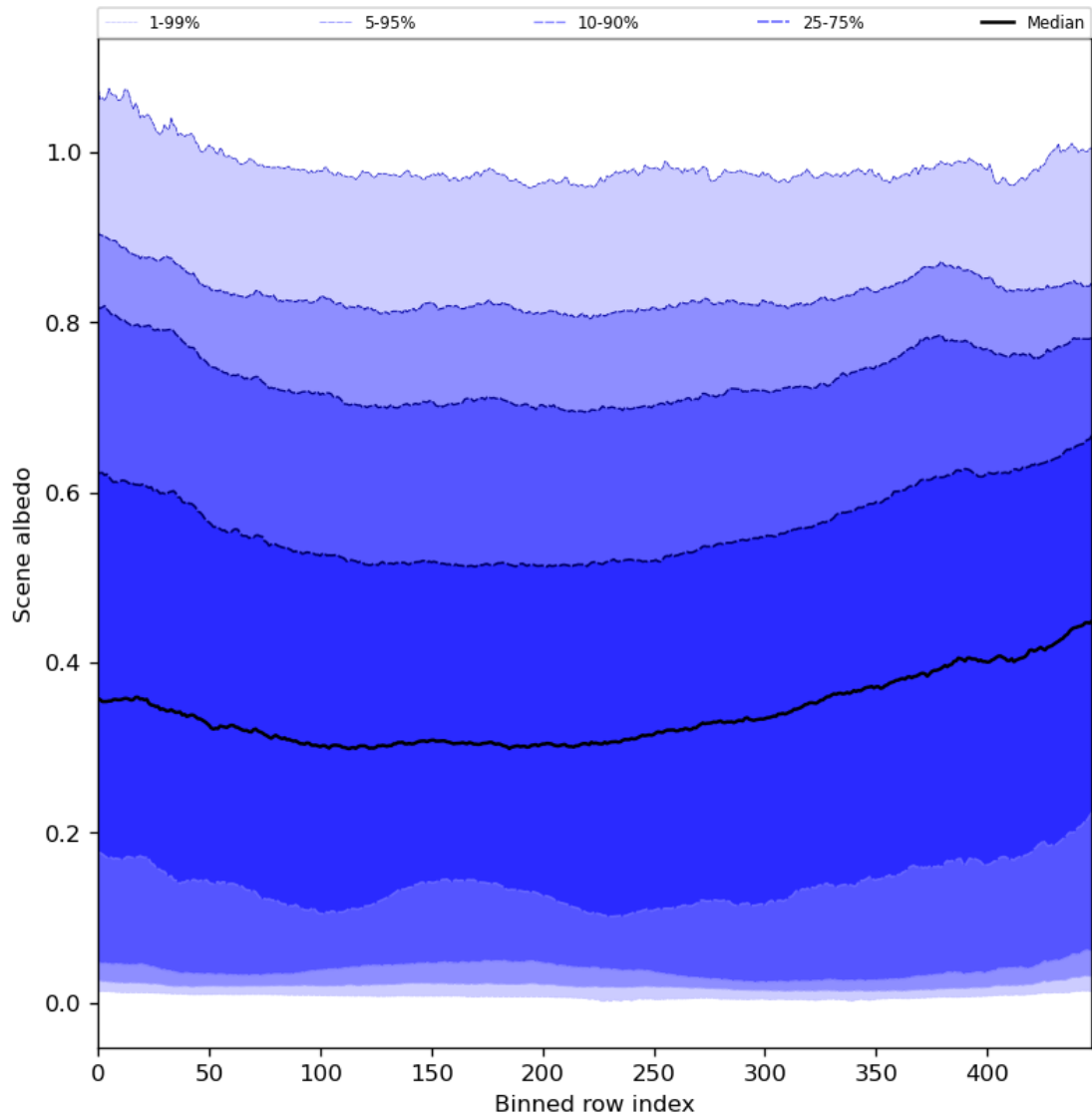
Figure 51: Along track statistics of “Scene albedo” for 2024-07-08 to 2024-07-10
