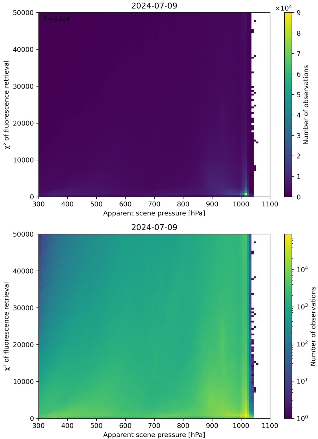
Figure 63: Scatter density plot of “Apparent scene pressure” against “ \chi^2 of fluorescence retrieval” for 2024-07-08 to 2024-07-10.
