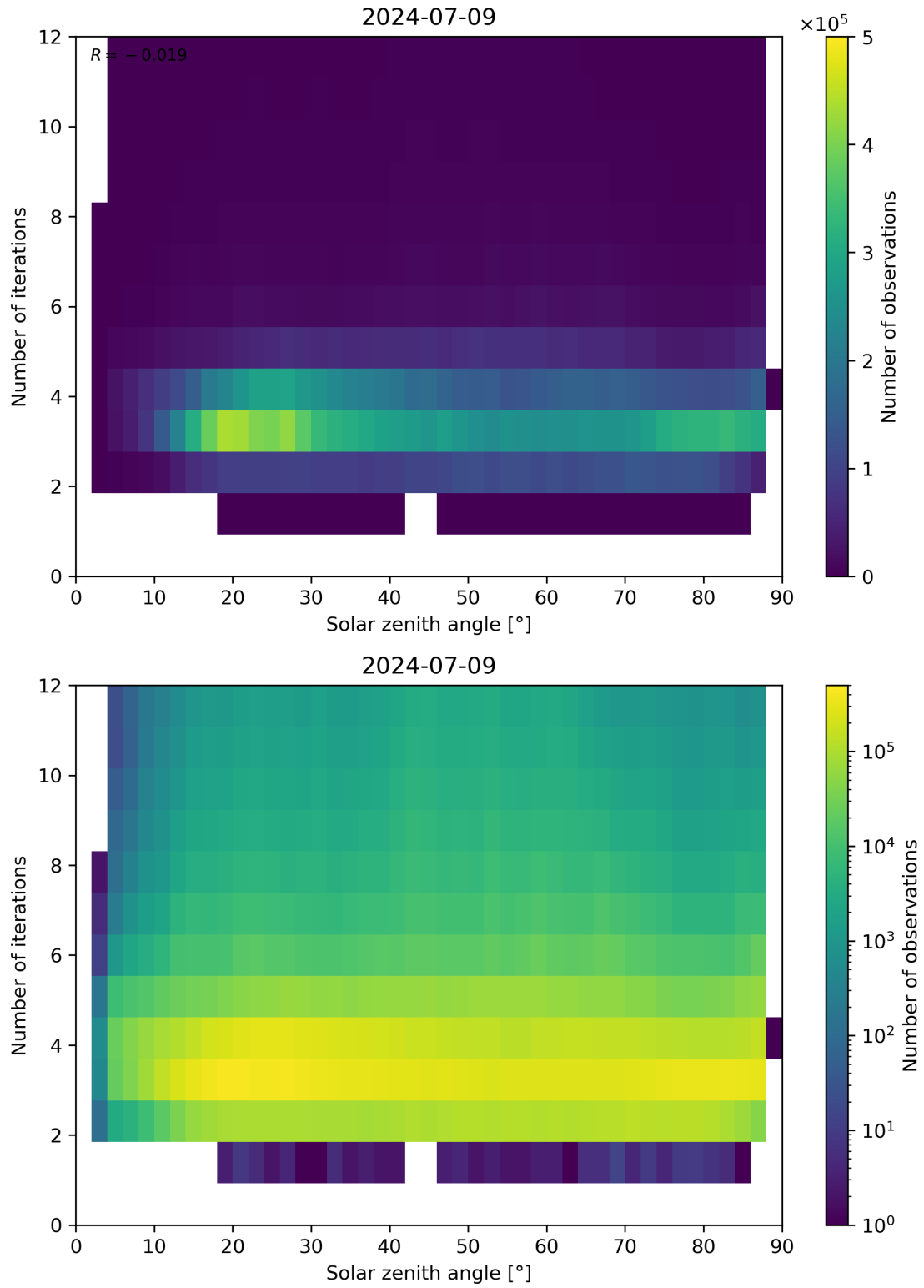
Figure 114: Scatter density plot of “Solar zenith angle” against “Number of iterations” for 2024-07-08 to 2024-07-10.
