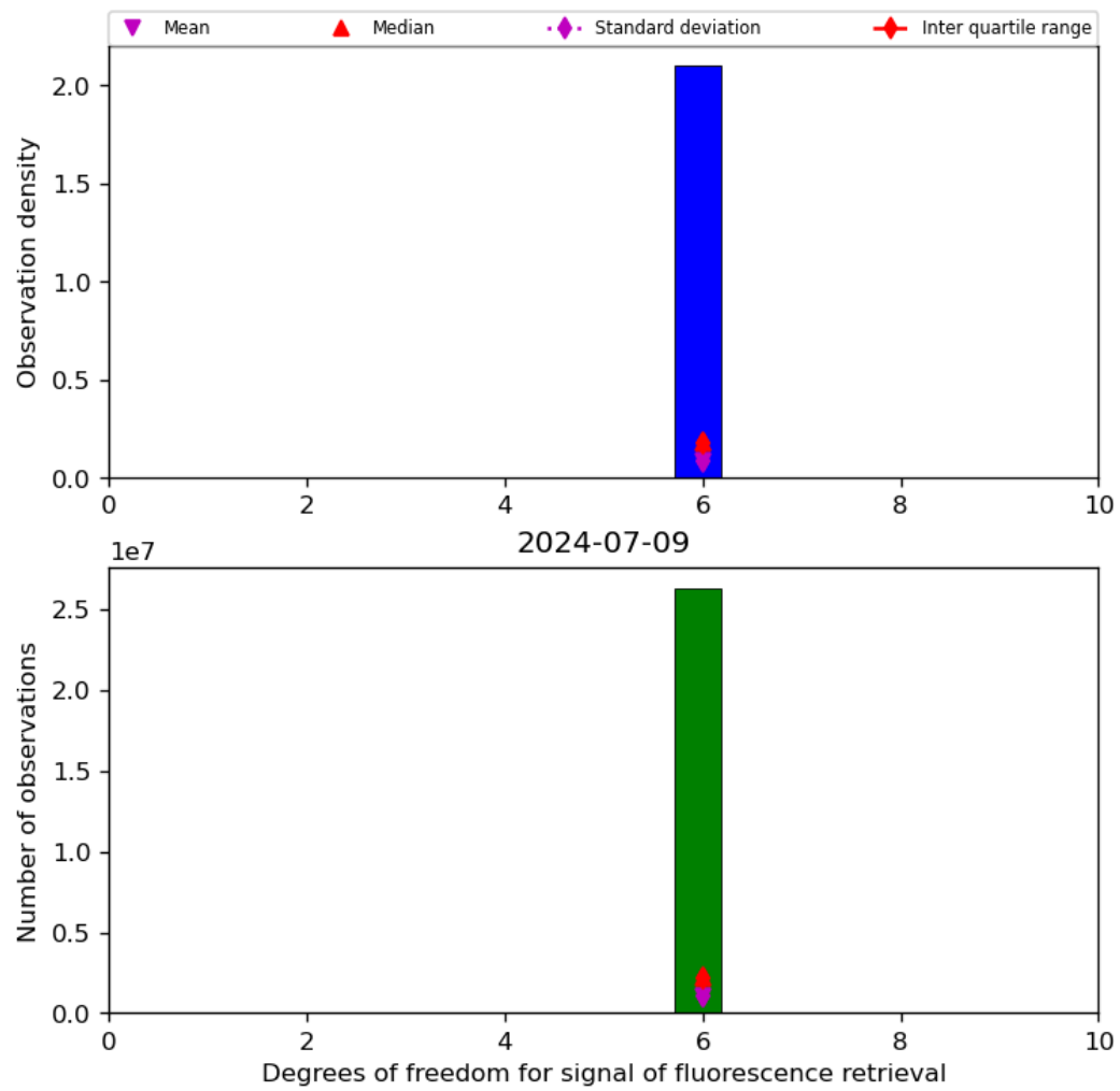
Figure 43: Histogram of “Degrees of freedom for signal of fluorescence retrieval” for 2024-07-08 to 2024-07-10
