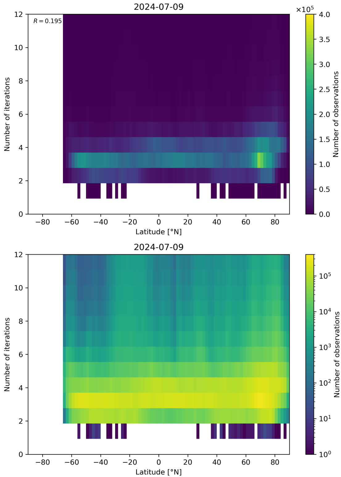
Figure 93: Scatter density plot of “Latitude” against “Number of iterations” for 2024-07-08 to 2024-07-10.
