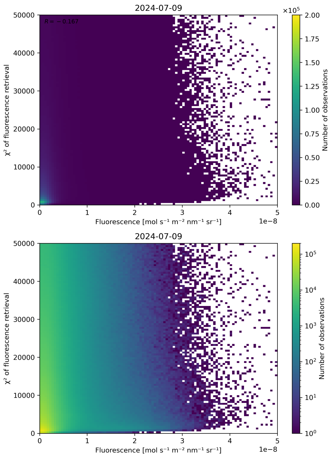
Figure 85: Scatter density plot of “Fluorescence” against “ \chi^2 of fluorescence retrieval” for 2024-07-08 to 2024-07-10.
