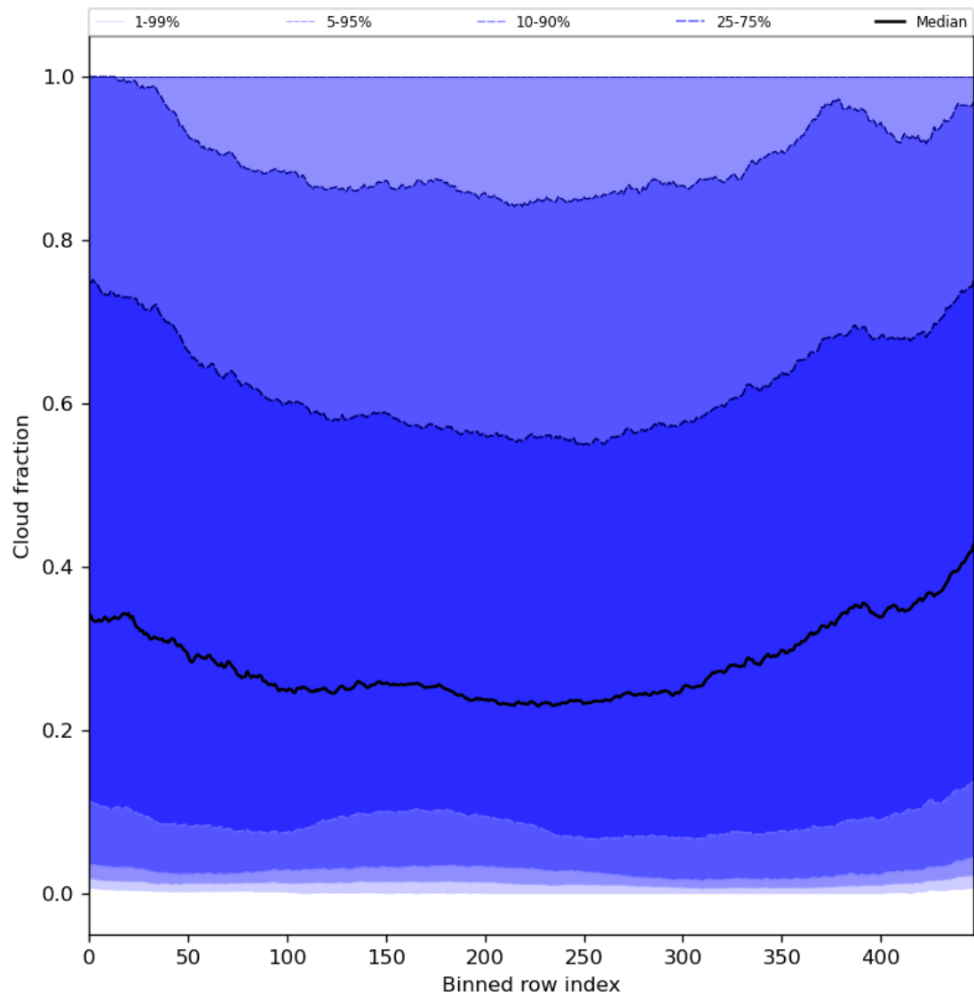
Figure 49: Along track statistics of “Cloud fraction” for 2024-07-08 to 2024-07-10
