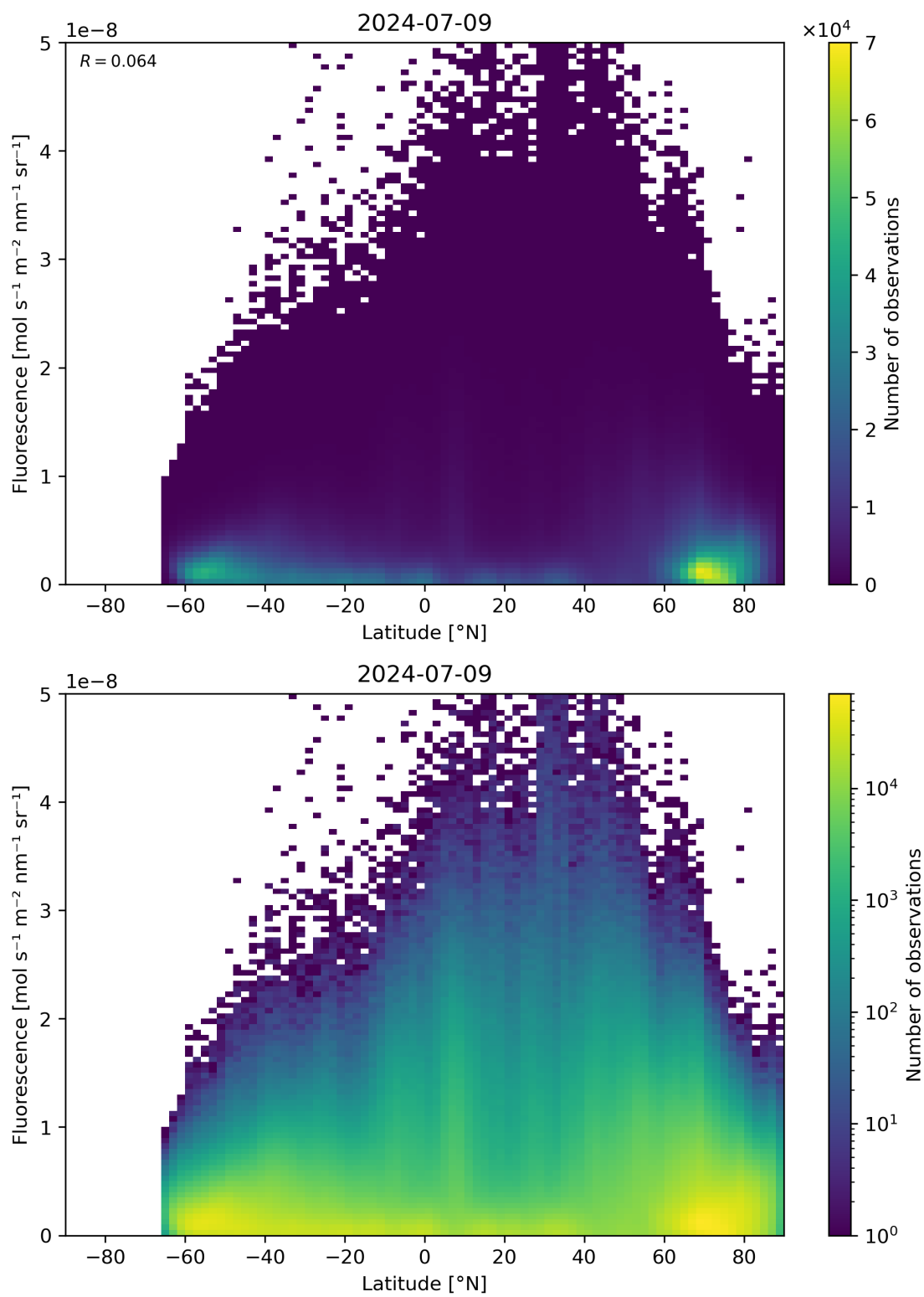
Figure 92: Scatter density plot of “Latitude” against “Fluorescence” for 2024-07-08 to 2024-07-10.
