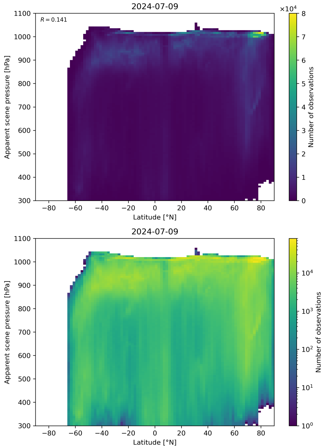
Figure 88: Scatter density plot of “Latitude” against “Apparent scene pressure” for 2024-07-08 to 2024-07-10.
