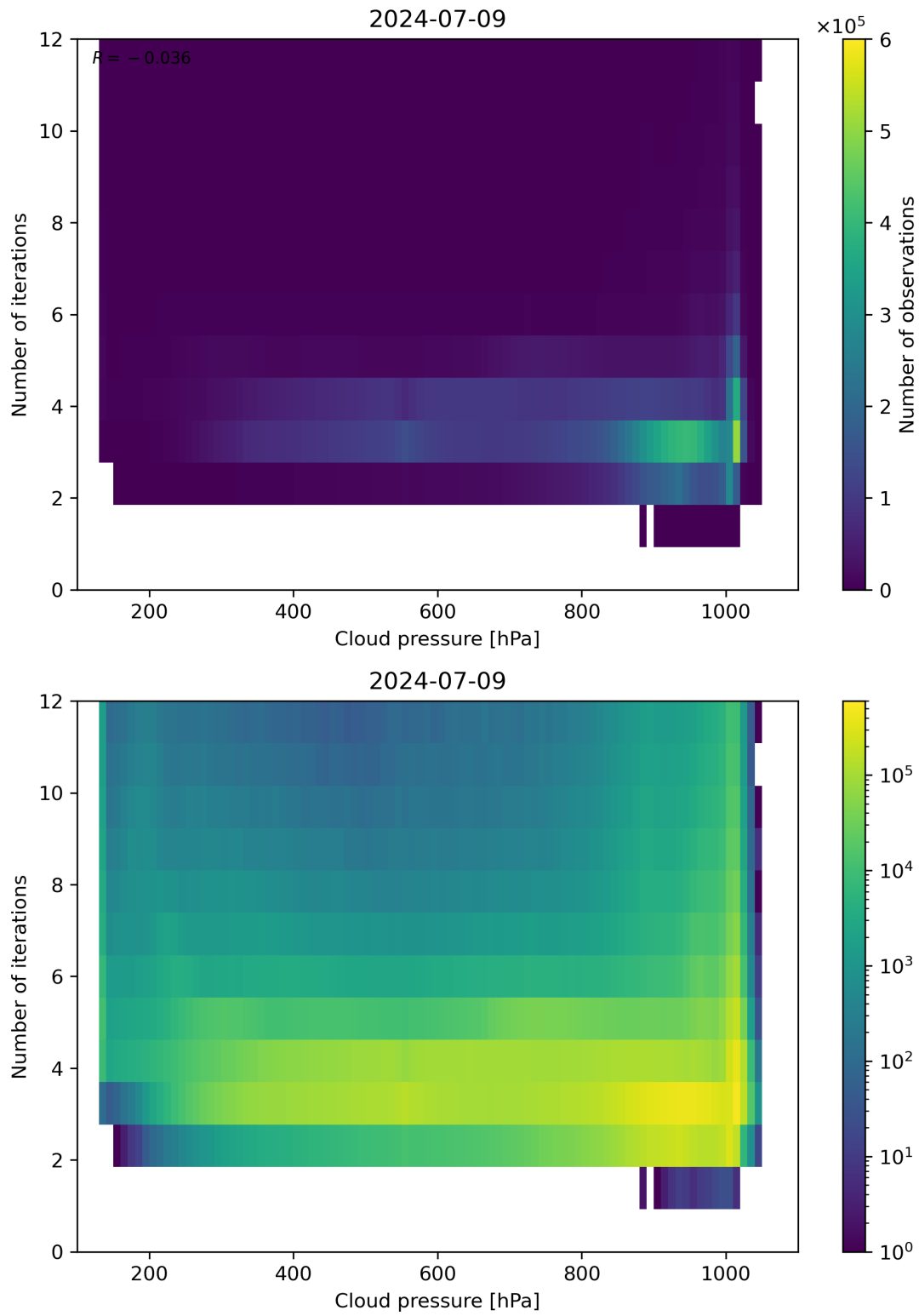
Figure 81: Scatter density plot of “Cloud pressure” against “Number of iterations” for 2024-07-08 to 2024-07-10.
