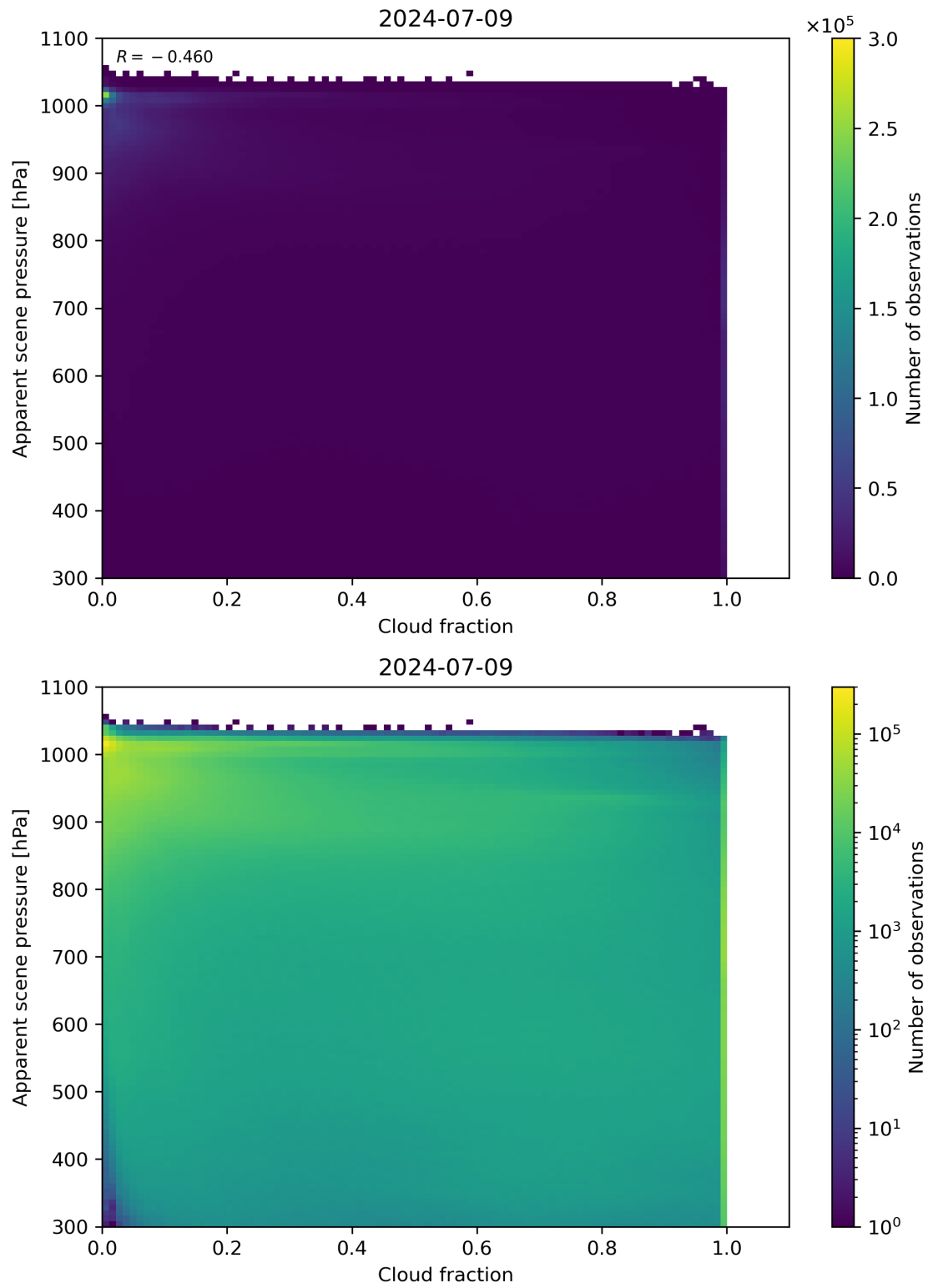
Figure 70: Scatter density plot of “Cloud fraction” against “Apparent scene pressure” for 2024-07-08 to 2024-07-10.
