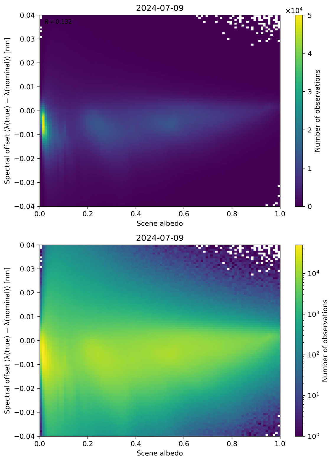
Figure 107: Scatter density plot of “Scene albedo” against “Spectral offset ( \lambda(\text{true}) - \lambda(\text{nominal}) )” for 2024-07-08 to 2024-07-10.
