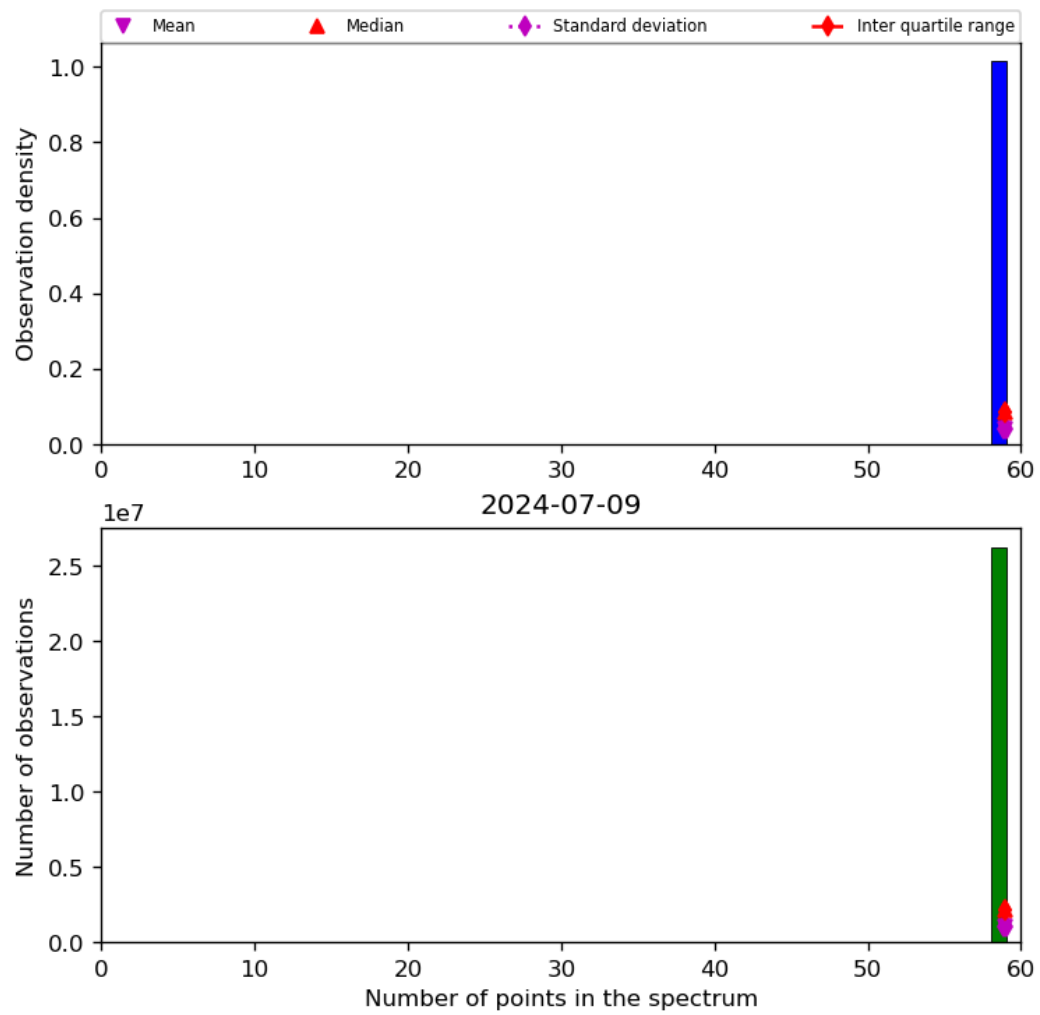
Figure 44: Histogram of “Number of points in the spectrum” for 2024-07-08 to 2024-07-10
