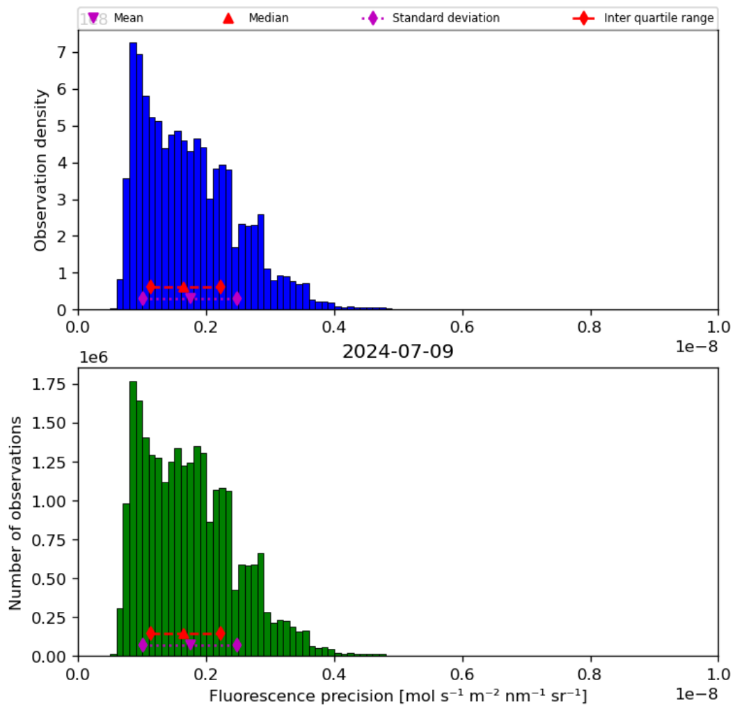
Figure 41: Histogram of “Fluorescence precision” for 2024-07-08 to 2024-07-10
