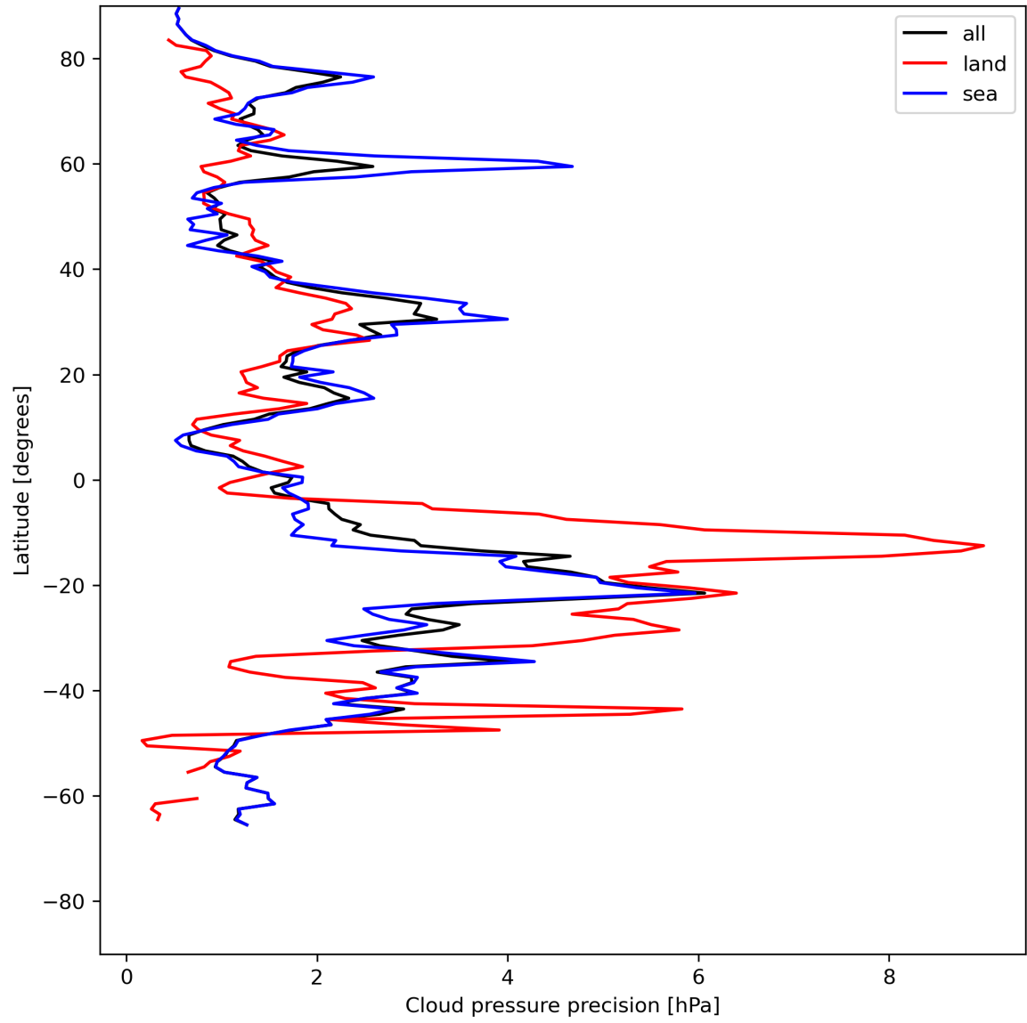
Figure 14: Zonal average of “Cloud pressure precision” for 2024-07-08 to 2024-07-10.
