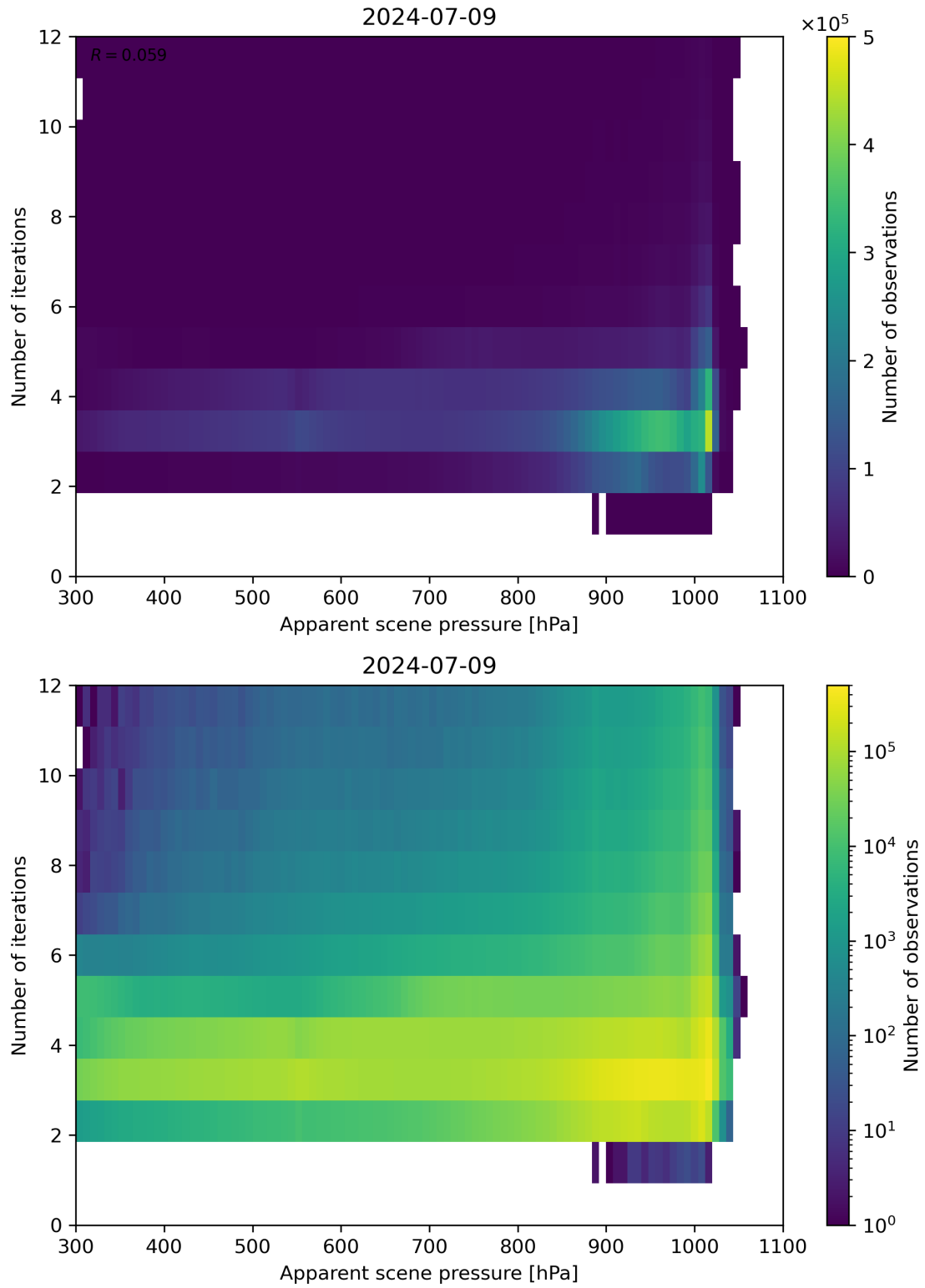
Figure 65: Scatter density plot of “Apparent scene pressure” against “Number of iterations” for 2024-07-08 to 2024-07-10.
