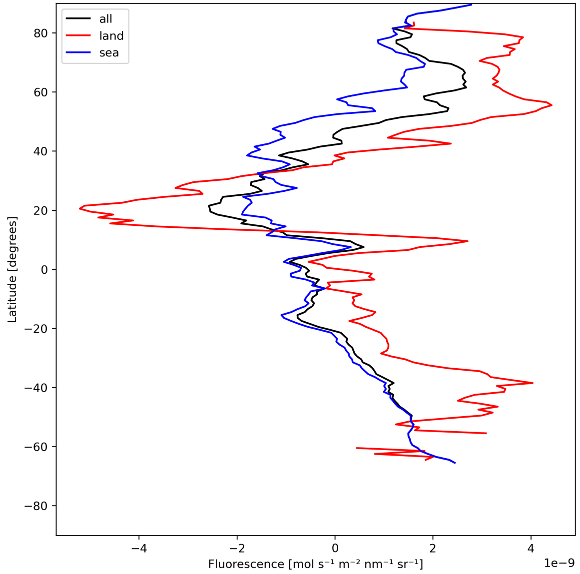
Figure 23: Zonal average of “Fluorescence” for 2024-07-08 to 2024-07-10.
