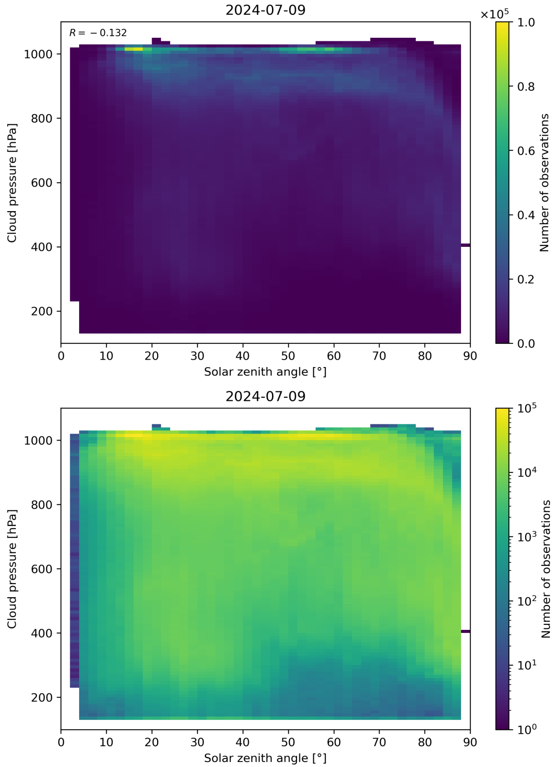
Figure 111: Scatter density plot of “Solar zenith angle” against “Cloud pressure” for 2024-07-08 to 2024-07-10.
