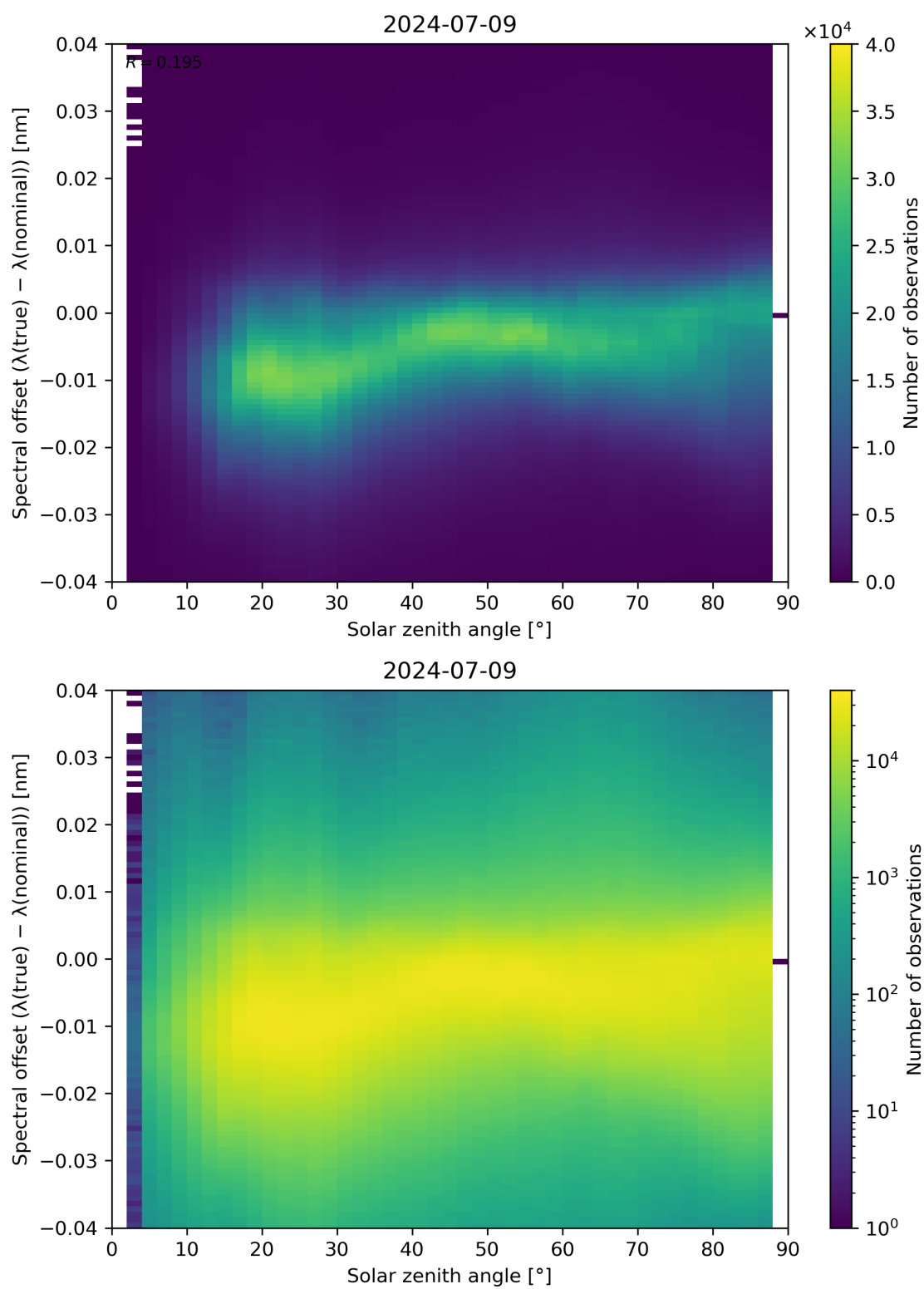
Figure 117: Scatter density plot of “Solar zenith angle” against “Spectral offset ( \lambda(\text{true}) - \lambda(\text{nominal}) )” for 2024-07-08 to 2024-07-10.
