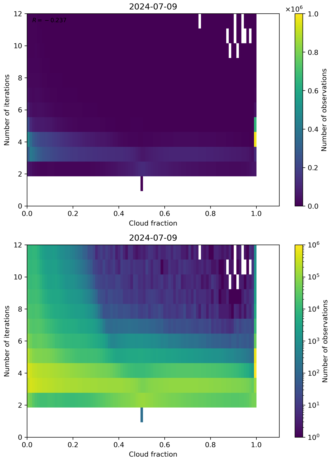
Figure 73: Scatter density plot of “Cloud fraction” against “Number of iterations” for 2024-07-08 to 2024-07-10.
