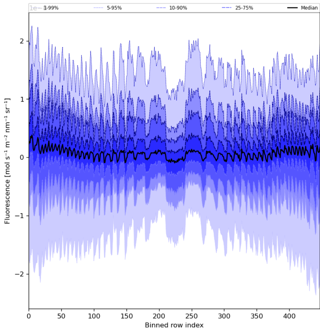
Figure 57: Along track statistics of “Fluorescence” for 2024-07-08 to 2024-07-10
