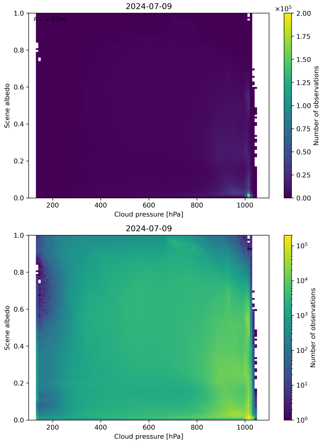
Figure 83: Scatter density plot of “Cloud pressure” against “Scene albedo” for 2024-07-08 to 2024-07-10.
