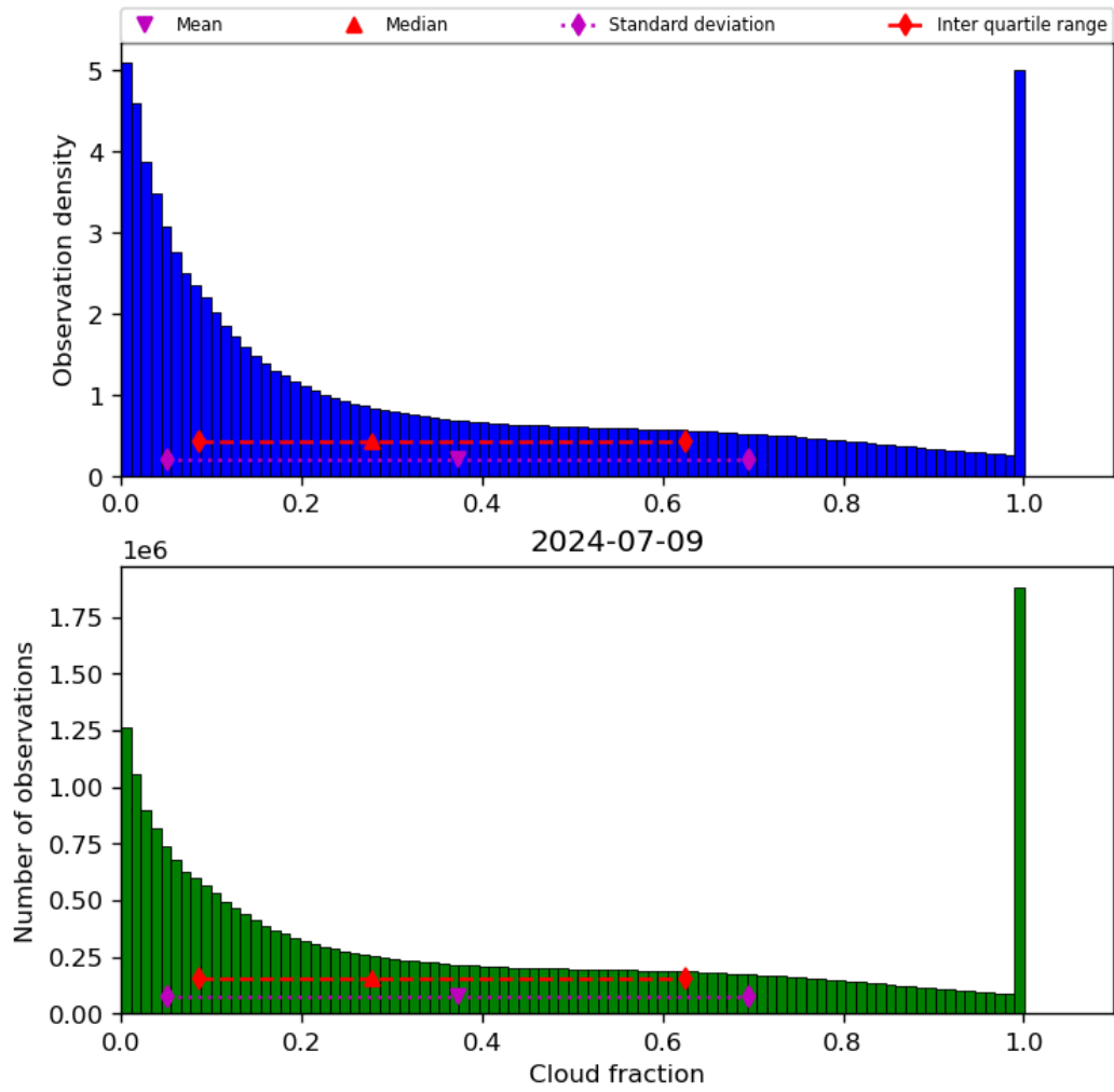
Figure 32: Histogram of “Cloud fraction” for 2024-07-08 to 2024-07-10
