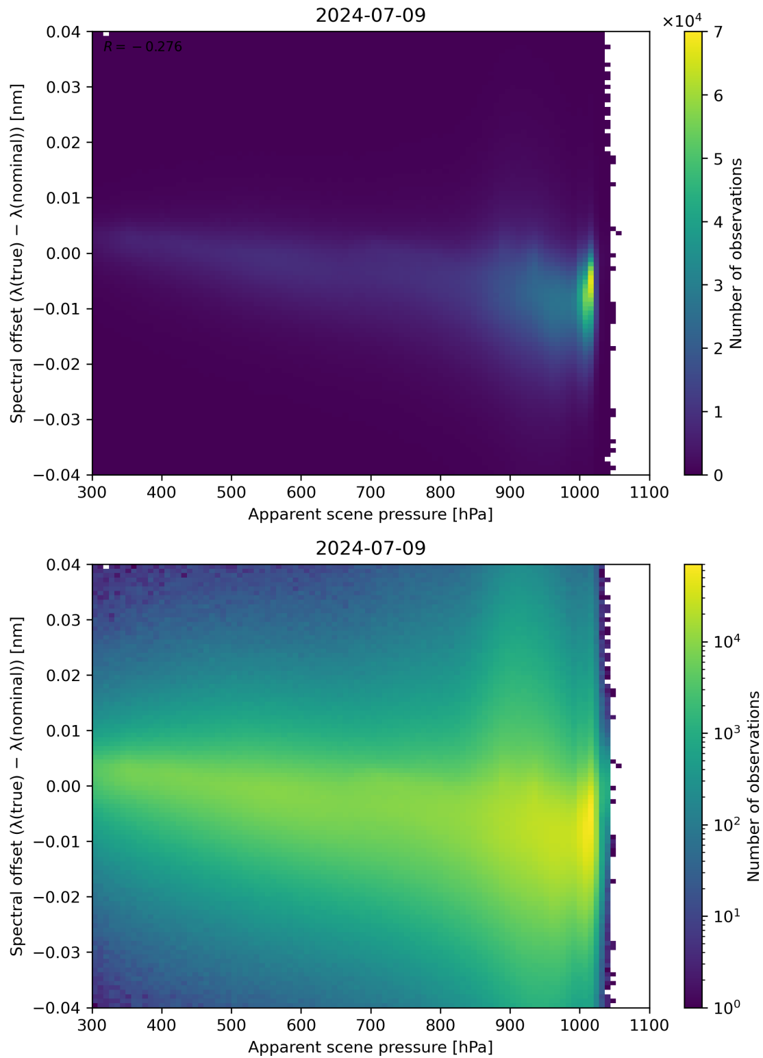
Figure 67: Scatter density plot of “Apparent scene pressure” against “Spectral offset ( \lambda(\text{true}) - \lambda(\text{nominal}) )” for 2024-07-08 to 2024-07-10.
