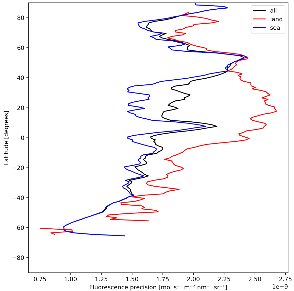
Figure 24: Zonal average of “Fluorescence precision” for 2024-07-08 to 2024-07-10.
