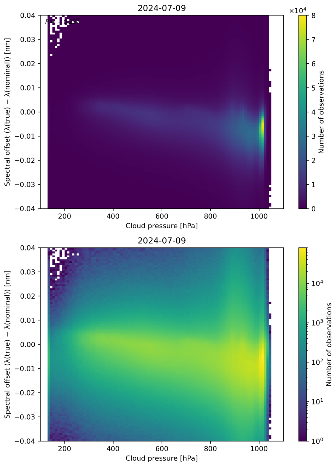
Figure 84: Scatter density plot of “Cloud pressure” against “Spectral offset ( \lambda(\text{true}) - \lambda(\text{nominal}) )” for 2024-07-08 to 2024-07-10.
