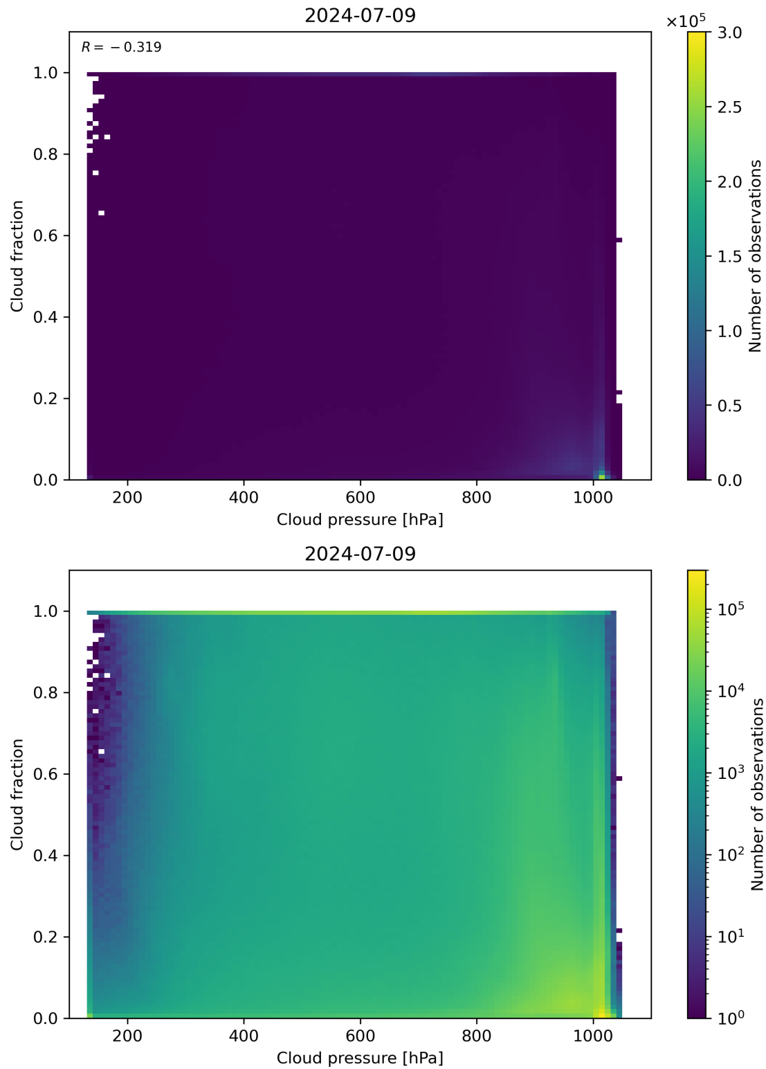
Figure 79: Scatter density plot of “Cloud pressure” against “Cloud fraction” for 2024-07-08 to 2024-07-10.
