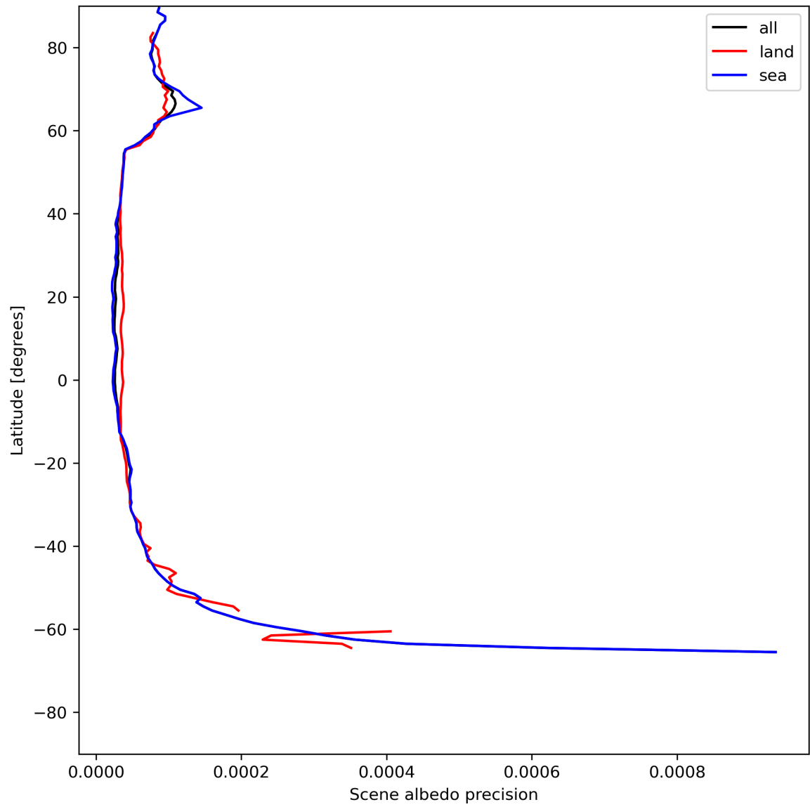
Figure 18: Zonal average of “Scene albedo precision” for 2024-07-08 to 2024-07-10.
