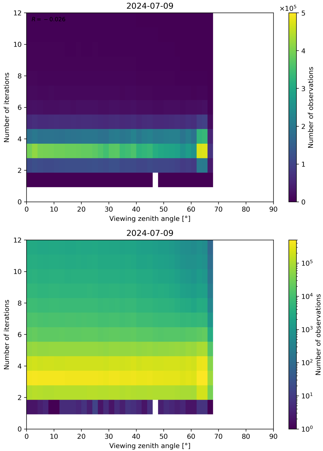
Figure 124: Scatter density plot of “Viewing zenith angle” against “Number of iterations” for 2024-07-08 to 2024-07-10.
