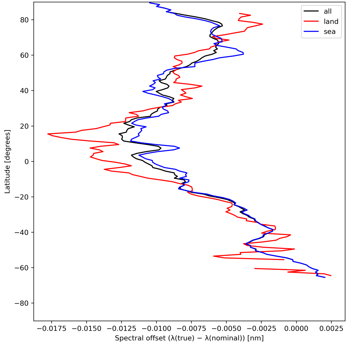
Figure 28: Zonal average of “Spectral offset ( \lambda(\text{true}) - \lambda(\text{nominal}) )” for 2024-07-08 to 2024-07-10.
