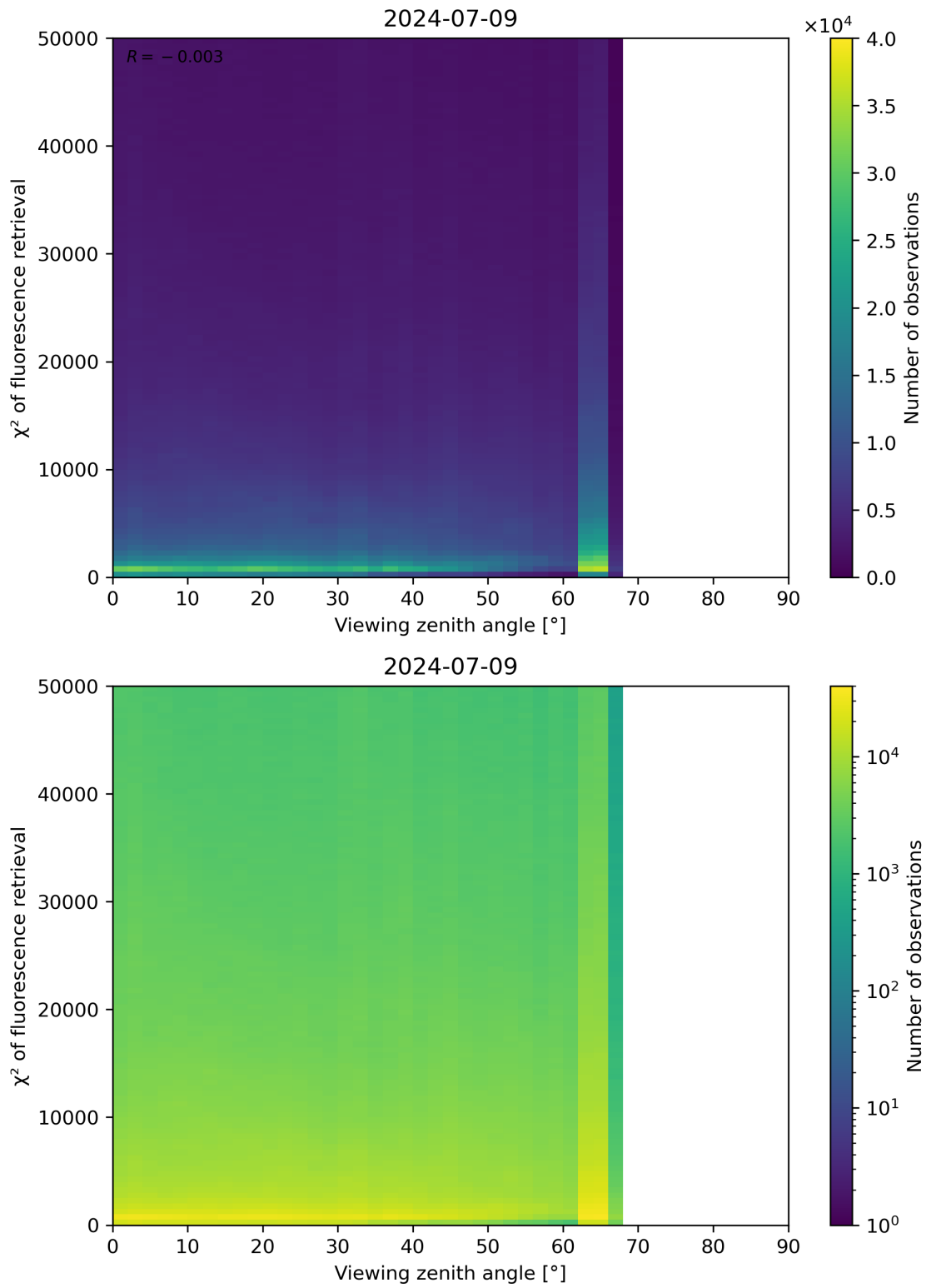
Figure 119: Scatter density plot of “Viewing zenith angle” against “ \chi^2 of fluorescence retrieval” for 2024-07-08 to 2024-07-10.
