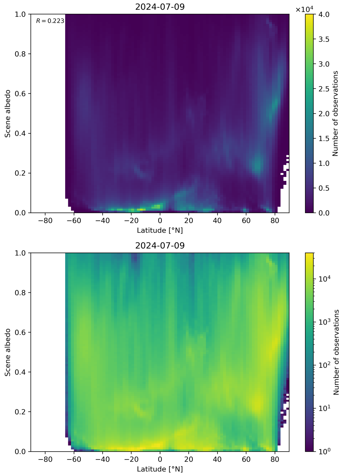
Figure 95: Scatter density plot of “Latitude” against “Scene albedo” for 2024-07-08 to 2024-07-10.
