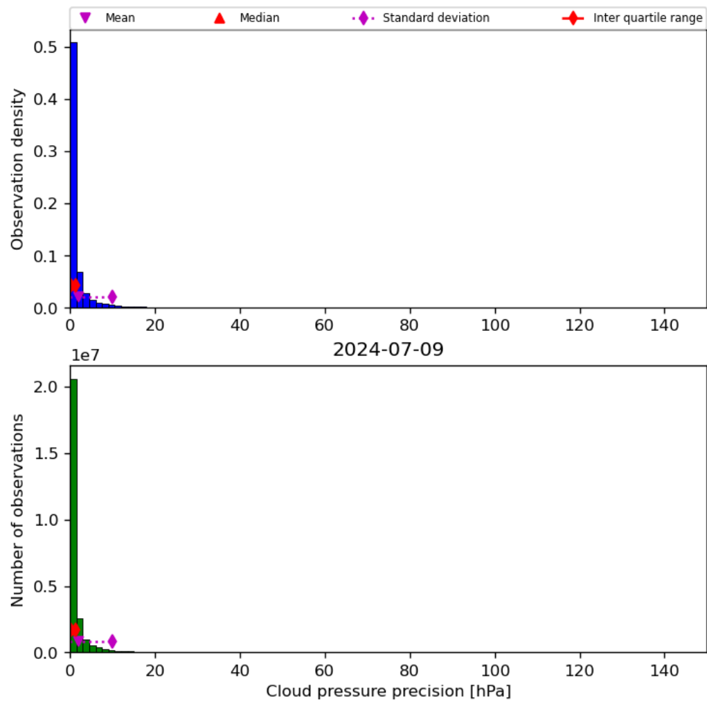
Figure 31: Histogram of “Cloud pressure precision” for 2024-07-08 to 2024-07-10
