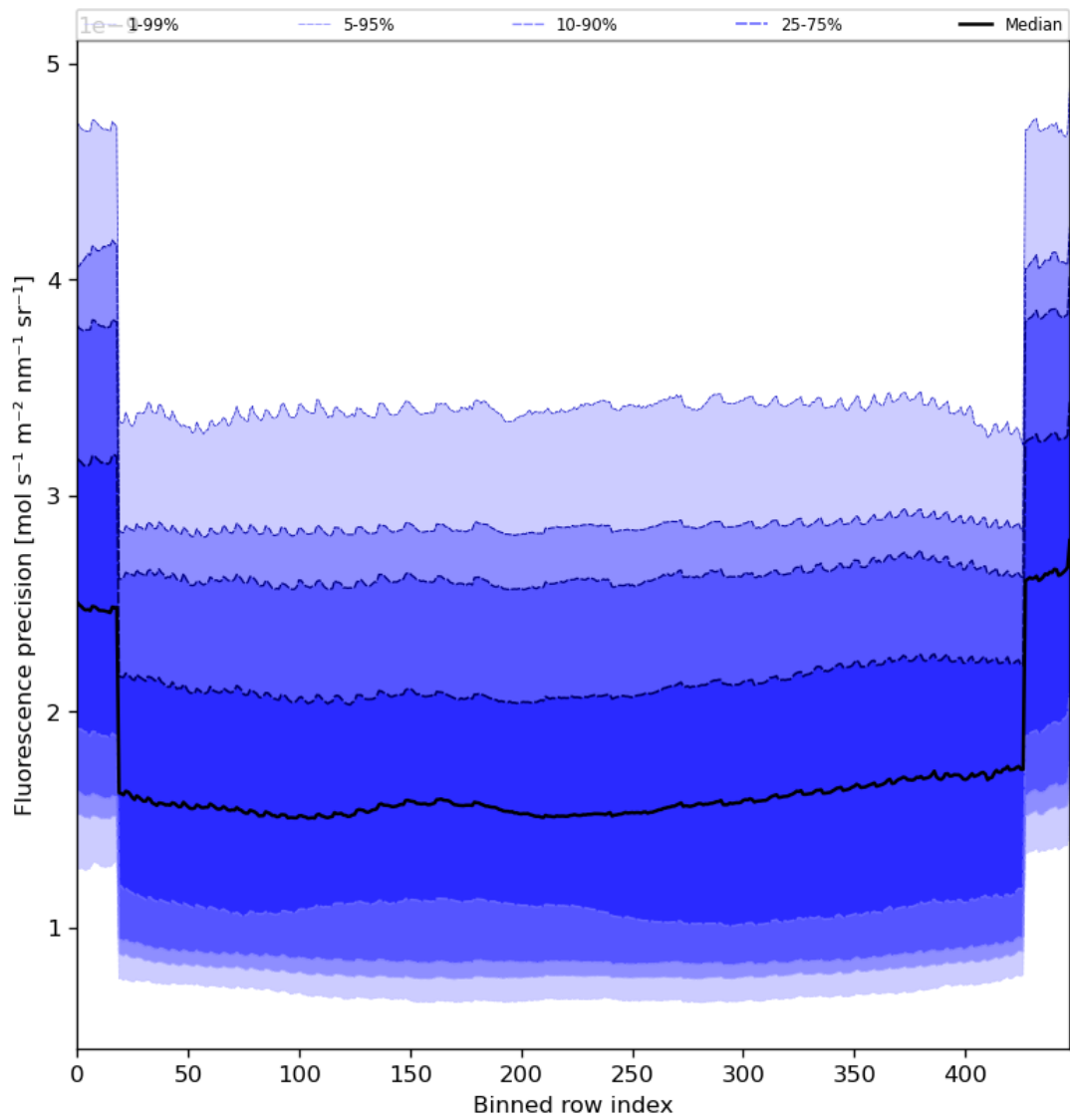
Figure 58: Along track statistics of “Fluorescence precision” for 2024-07-08 to 2024-07-10
