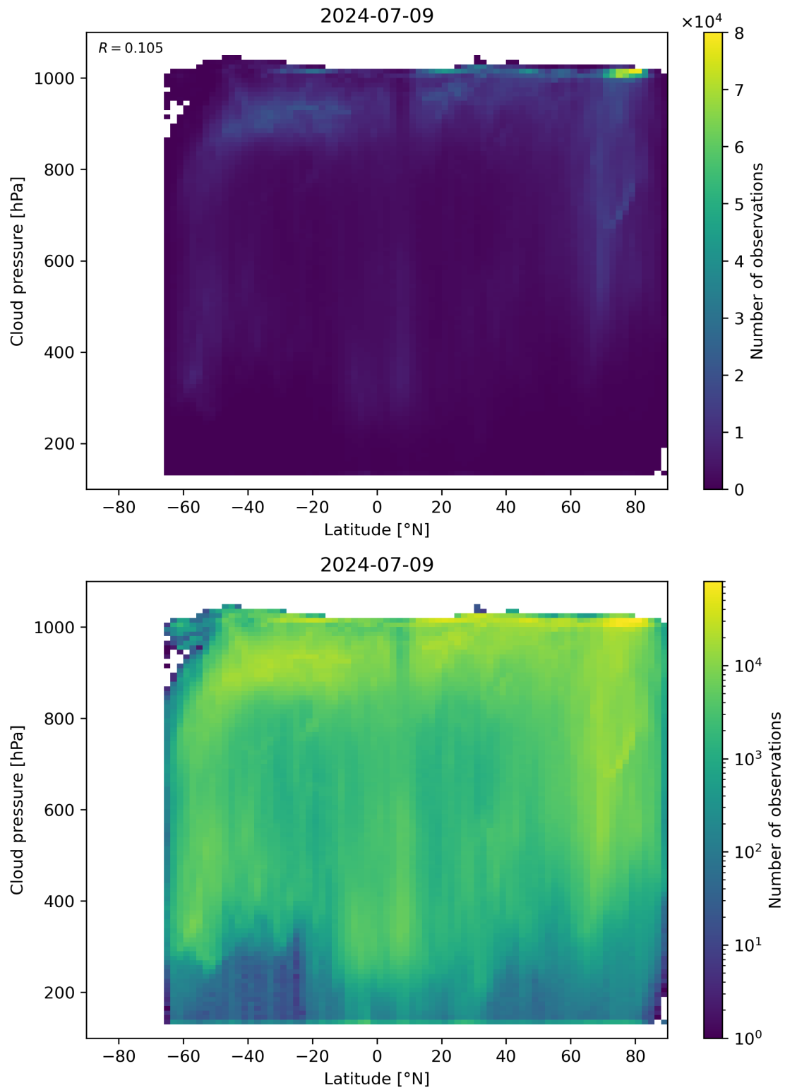
Figure 91: Scatter density plot of “Latitude” against “Cloud pressure” for 2024-07-08 to 2024-07-10.
