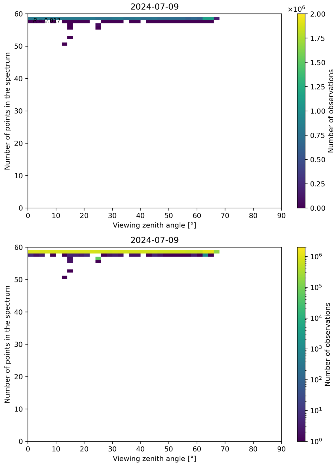
Figure 125: Scatter density plot of “Viewing zenith angle” against “Number of points in the spectrum” for 2024-07-08 to 2024-07-10.
