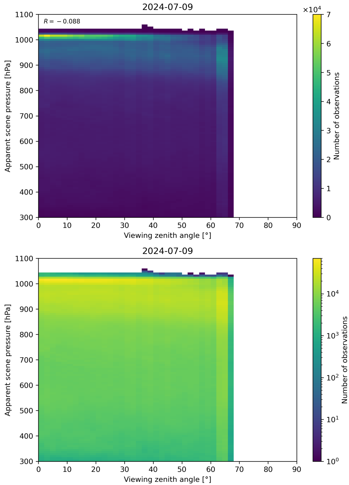
Figure 118: Scatter density plot of “Viewing zenith angle” against “Apparent scene pressure” for 2024-07-08 to 2024-07-10.
