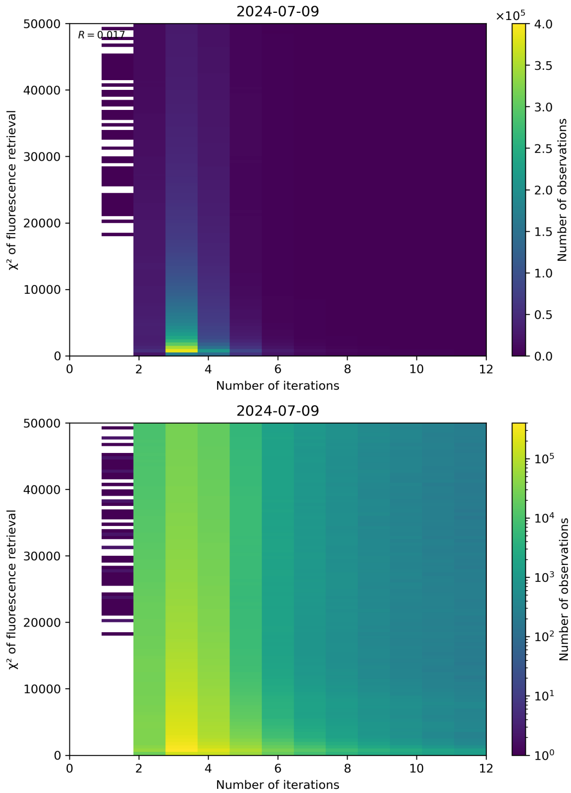
Figure 97: Scatter density plot of “Number of iterations” against “ \chi^2 of fluorescence retrieval” for 2024-07-08 to 2024-07-10.
