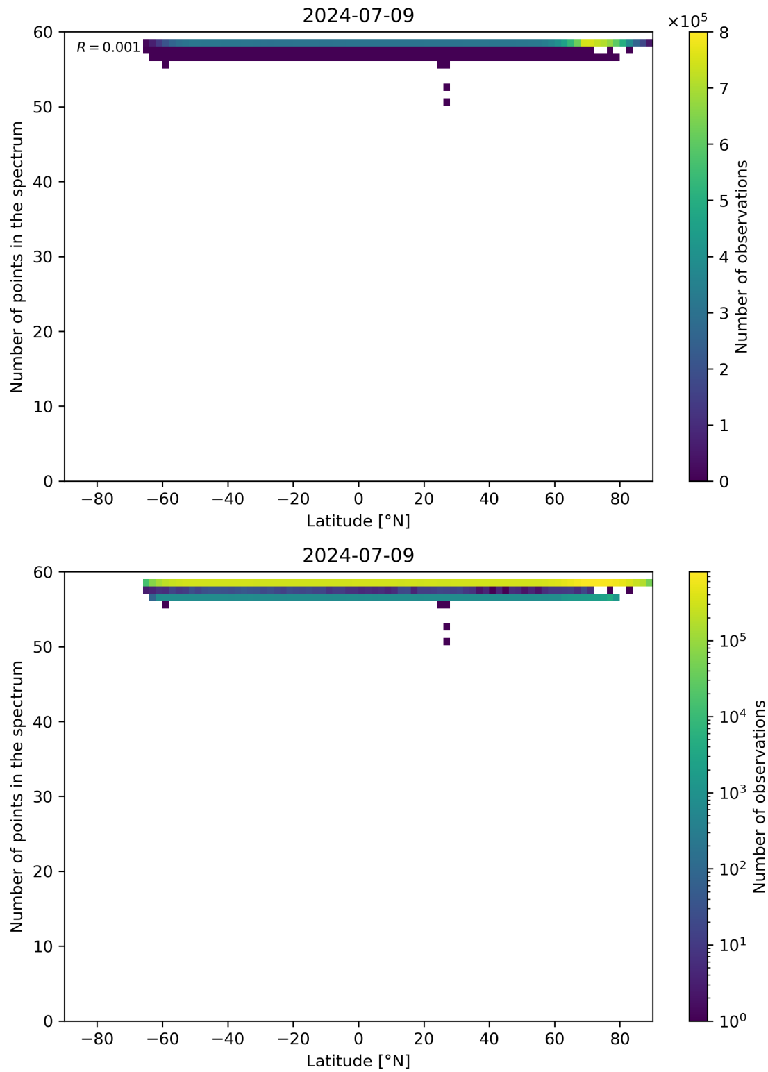
Figure 94: Scatter density plot of “Latitude” against “Number of points in the spectrum” for 2024-07-08 to 2024-07-10.
