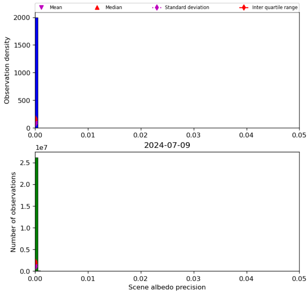
Figure 35: Histogram of “Scene albedo precision” for 2024-07-08 to 2024-07-10
