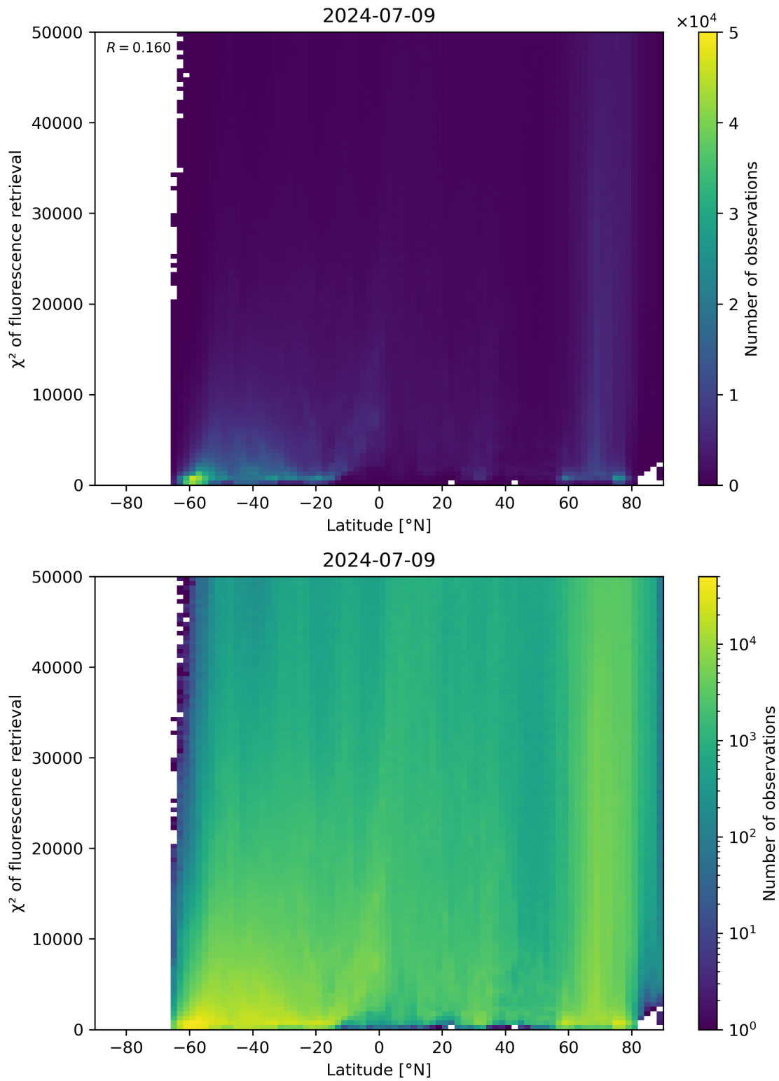
Figure 89: Scatter density plot of “Latitude” against “ \chi^2 of fluorescence retrieval” for 2024-07-08 to 2024-07-10.
