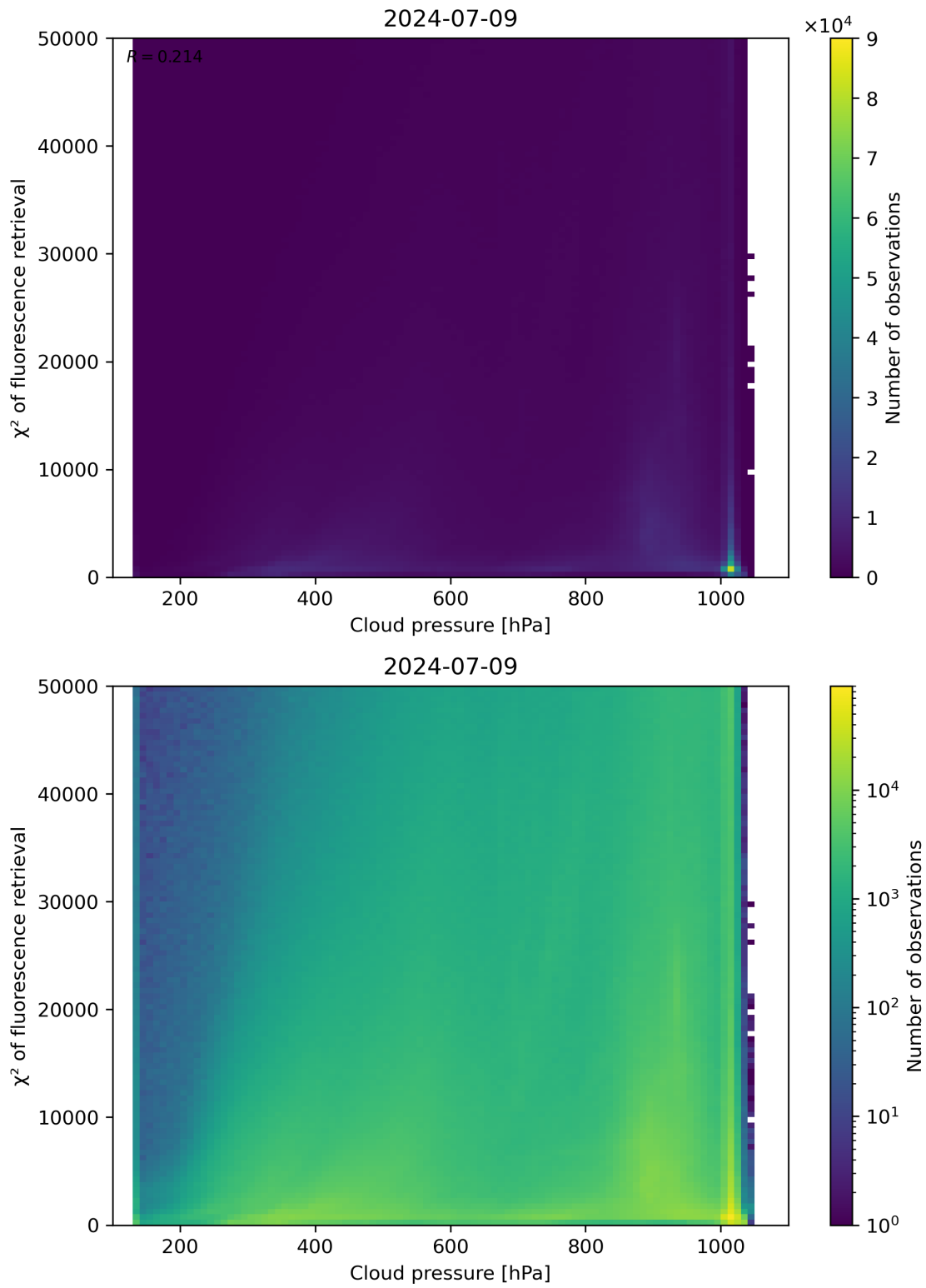
Figure 78: Scatter density plot of “Cloud pressure” against “ \chi^2 of fluorescence retrieval” for 2024-07-08 to 2024-07-10.
