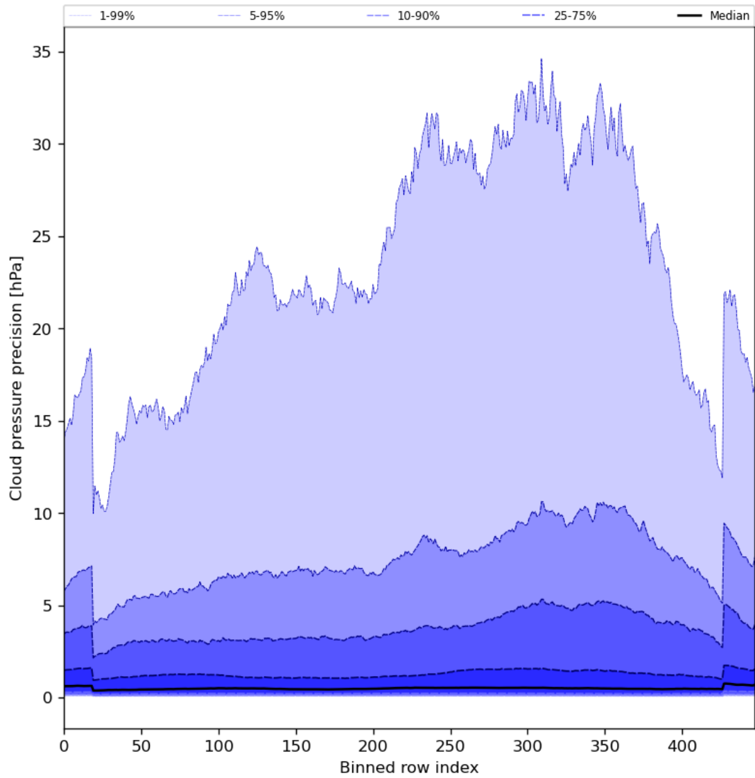
Figure 48: Along track statistics of “Cloud pressure precision” for 2024-07-08 to 2024-07-10
