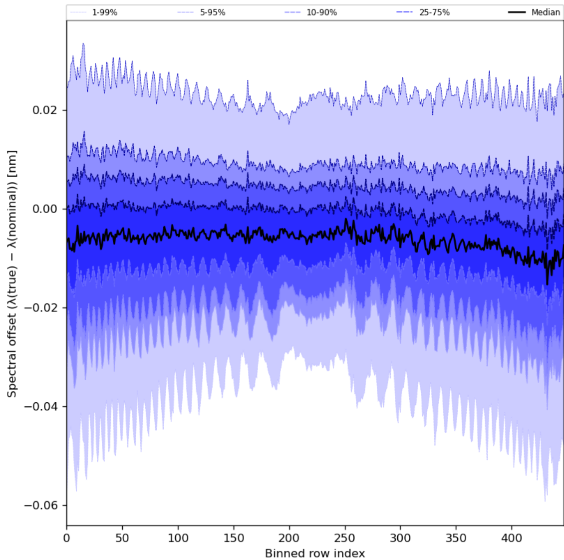
Figure 62: Along track statistics of “Spectral offset ( \lambda(\text{true}) - \lambda(\text{nominal}) )” for 2024-07-08 to 2024-07-10
