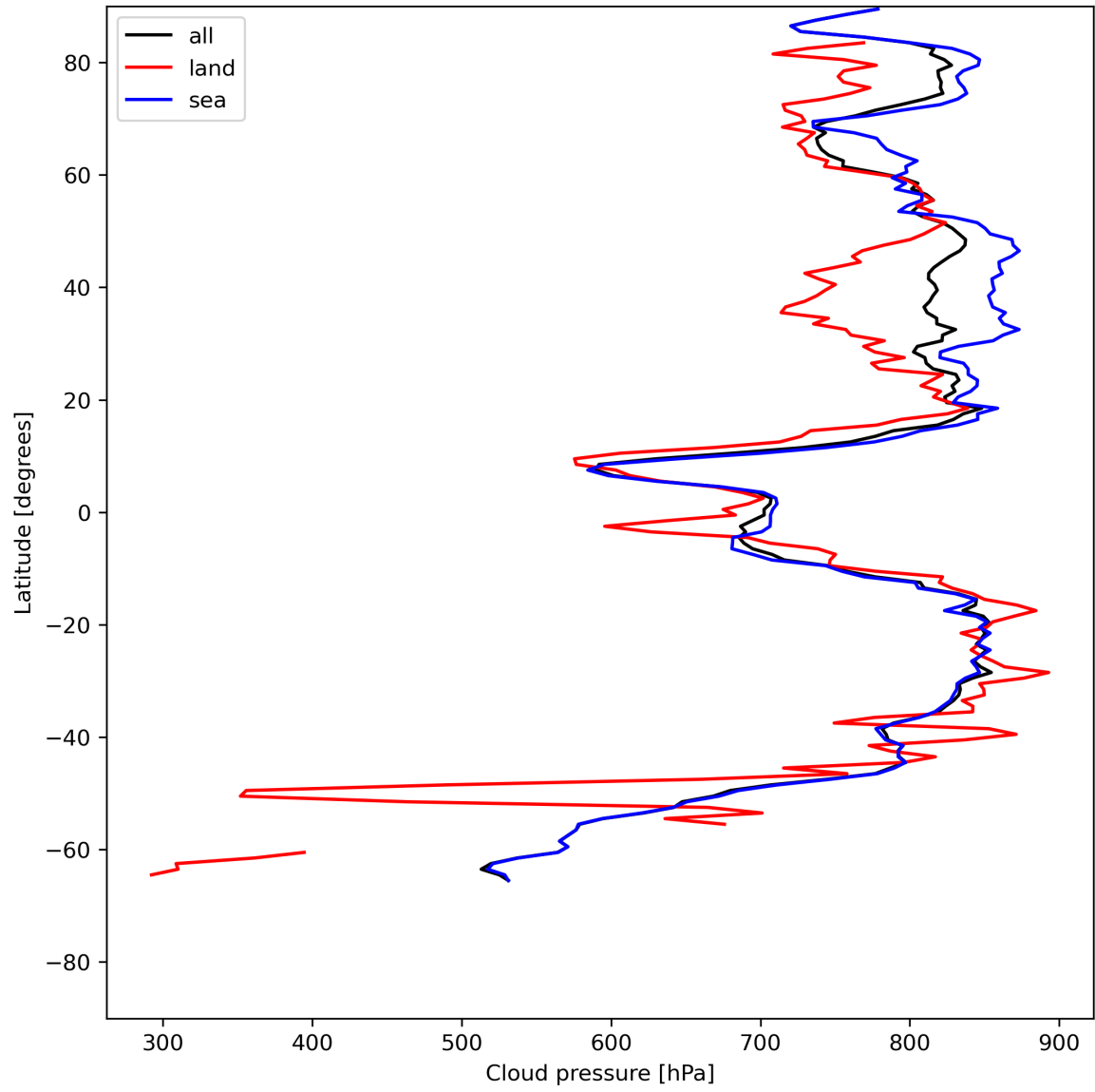
Figure 13: Zonal average of “Cloud pressure” for 2024-07-08 to 2024-07-10.
