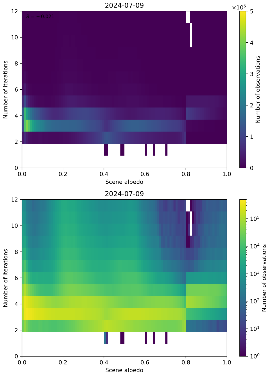
Figure 105: Scatter density plot of “Scene albedo” against “Number of iterations” for 2024-07-08 to 2024-07-10.
