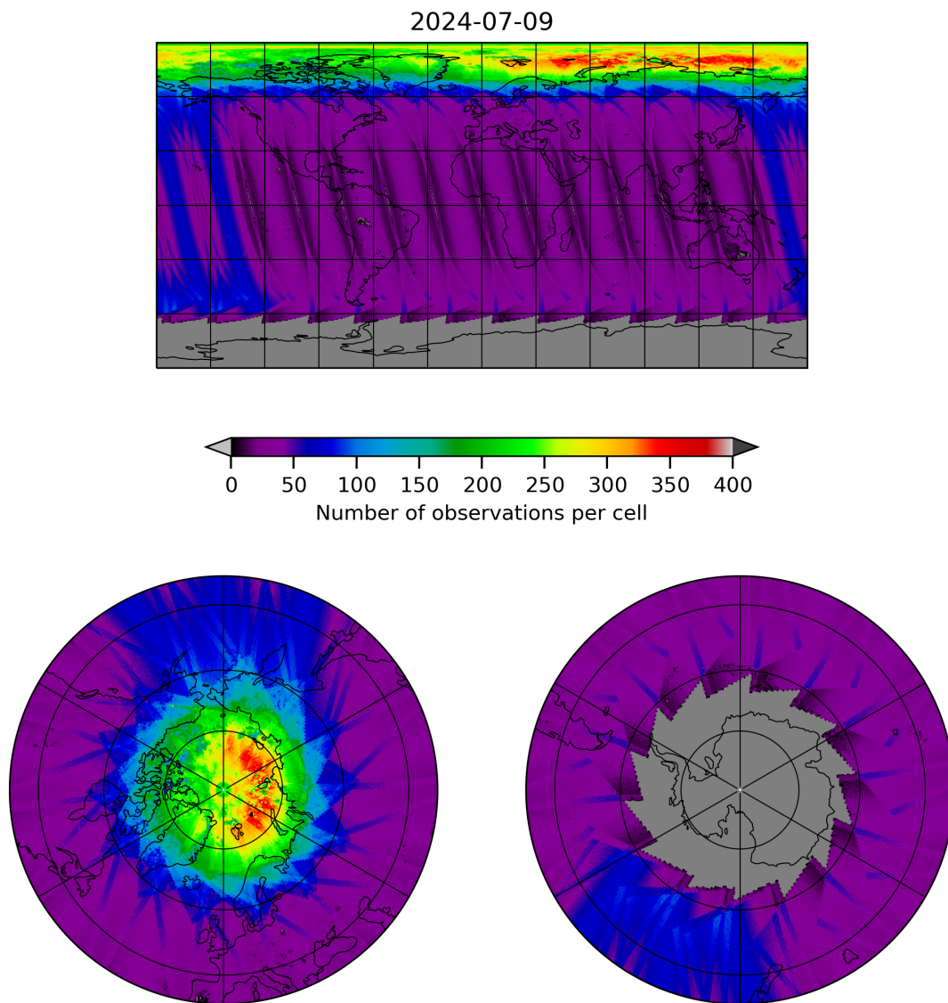
Figure 11: Map of the number of observations for 2024-07-08 to 2024-07-10
