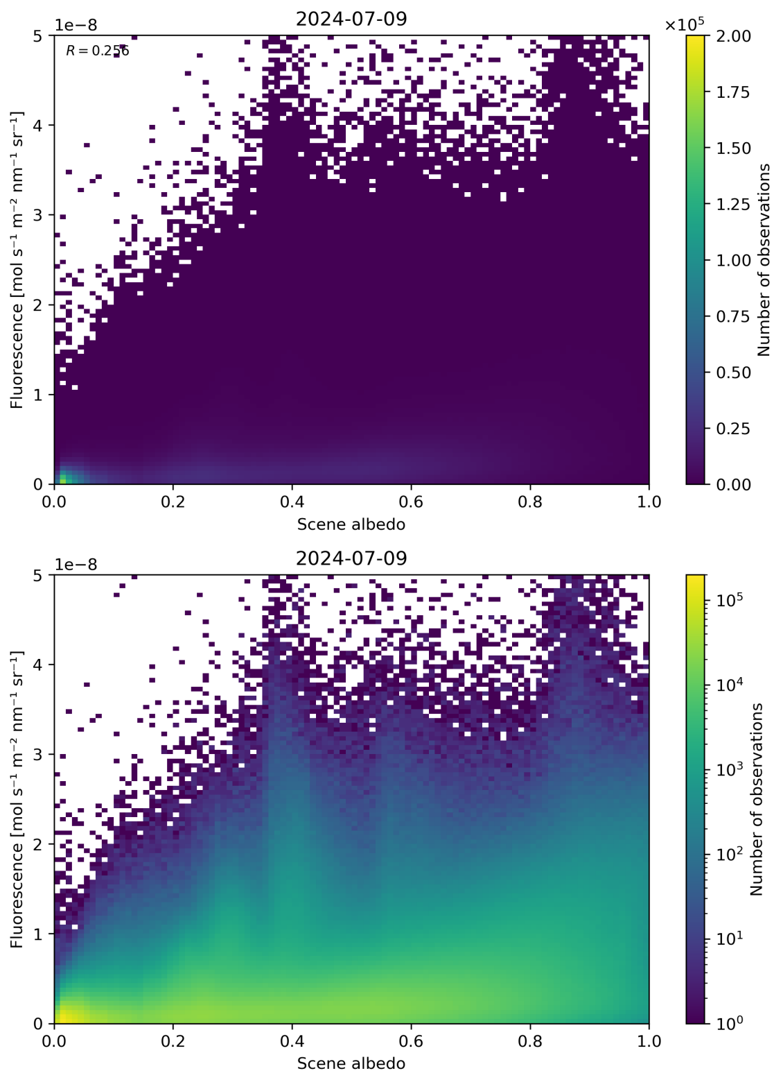
Figure 104: Scatter density plot of “Scene albedo” against “Fluorescence” for 2024-07-08 to 2024-07-10.
