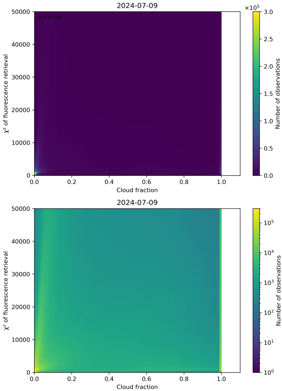
Figure 71: Scatter density plot of “Cloud fraction” against “ \chi^2 of fluorescence retrieval” for 2024-07-08 to 2024-07-10.
