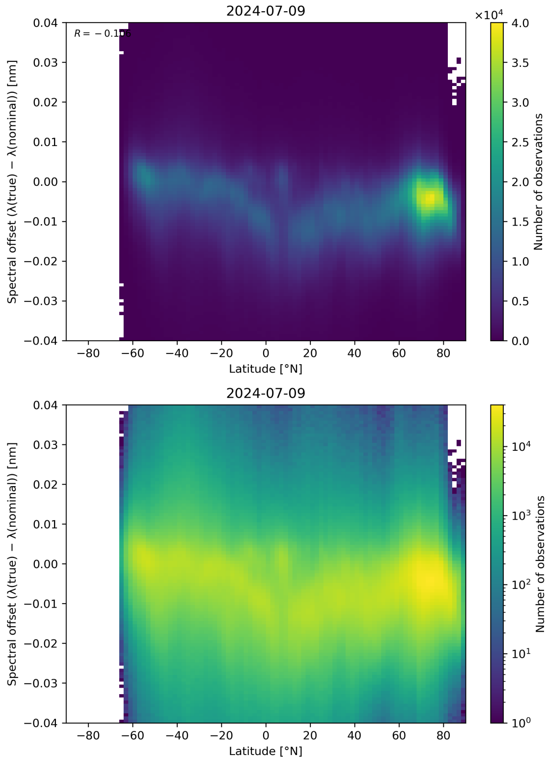
Figure 96: Scatter density plot of “Latitude” against “Spectral offset ( \lambda(\text{true}) - \lambda(\text{nominal}) )” for 2024-07-08 to 2024-07-10.
