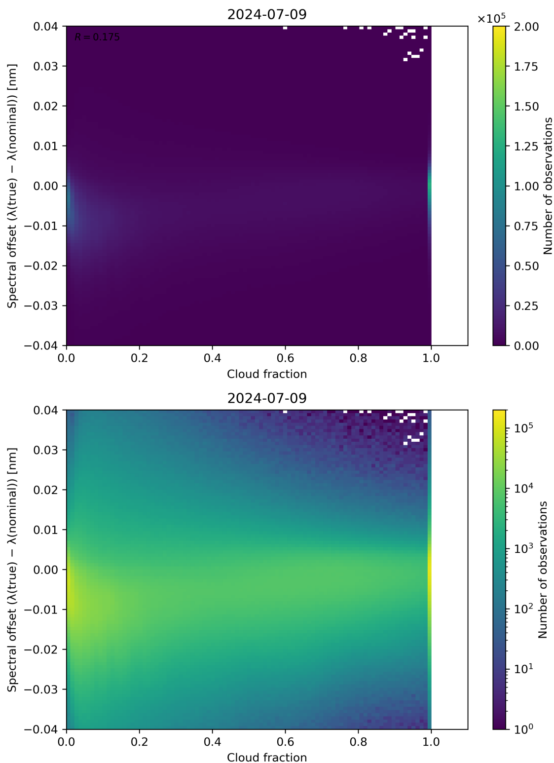
Figure 76: Scatter density plot of “Cloud fraction” against “Spectral offset ( \lambda(\text{true}) - \lambda(\text{nominal}) )” for 2024-07-08 to 2024-07-10.
