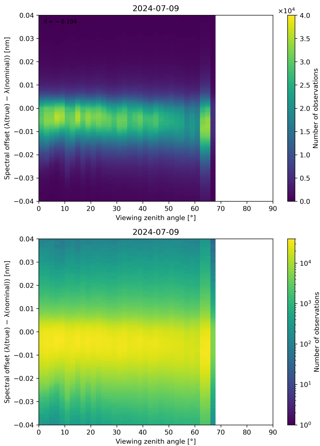
Figure 128: Scatter density plot of “Viewing zenith angle” against “Spectral offset ( \lambda(\text{true}) - \lambda(\text{nominal}) )” for 2024-07-08 to 2024-07-10.
