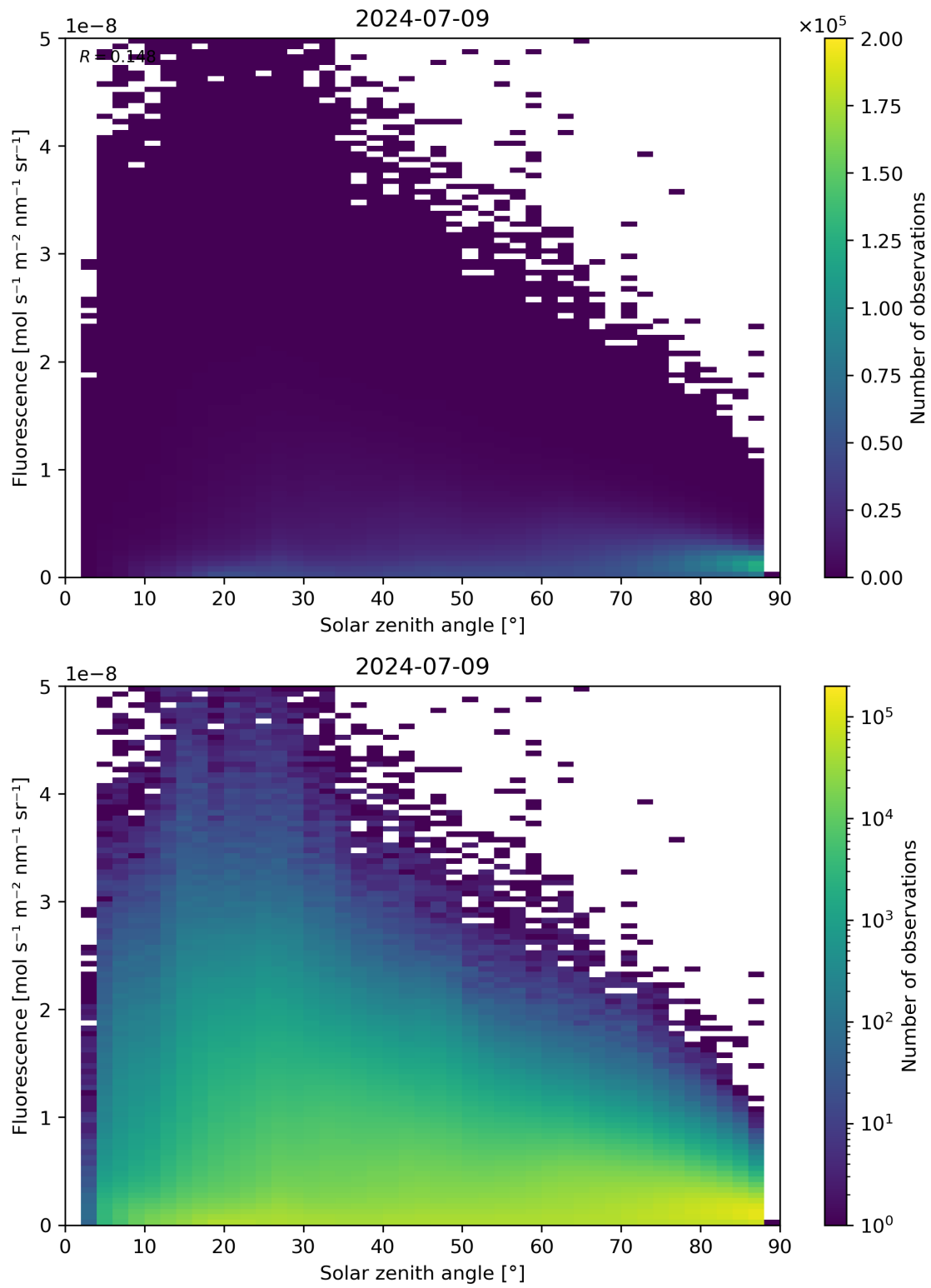
Figure 112: Scatter density plot of “Solar zenith angle” against “Fluorescence” for 2024-07-08 to 2024-07-10.
