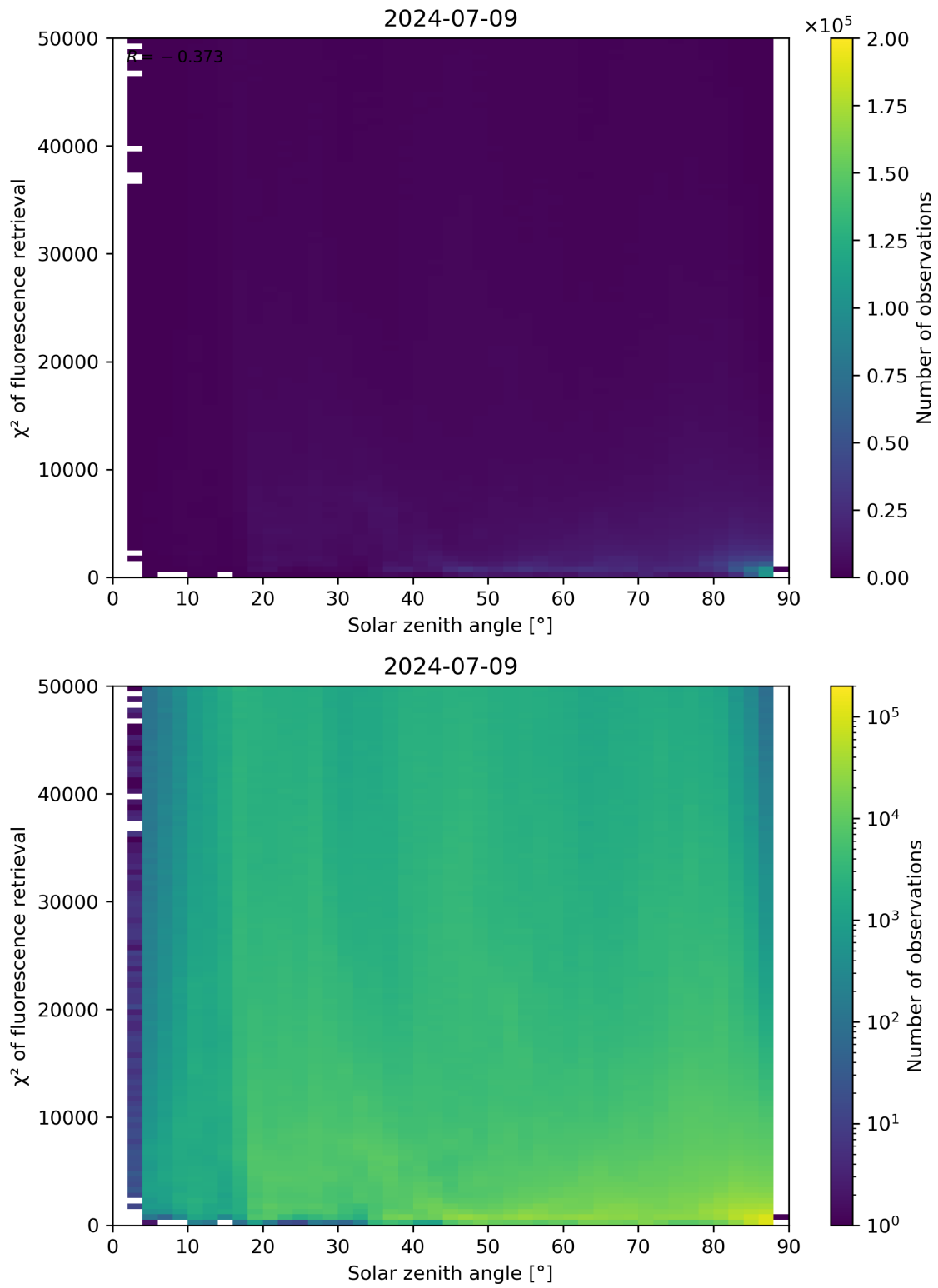
Figure 109: Scatter density plot of “Solar zenith angle” against “ \chi^2 of fluorescence retrieval” for 2024-07-08 to 2024-07-10.
