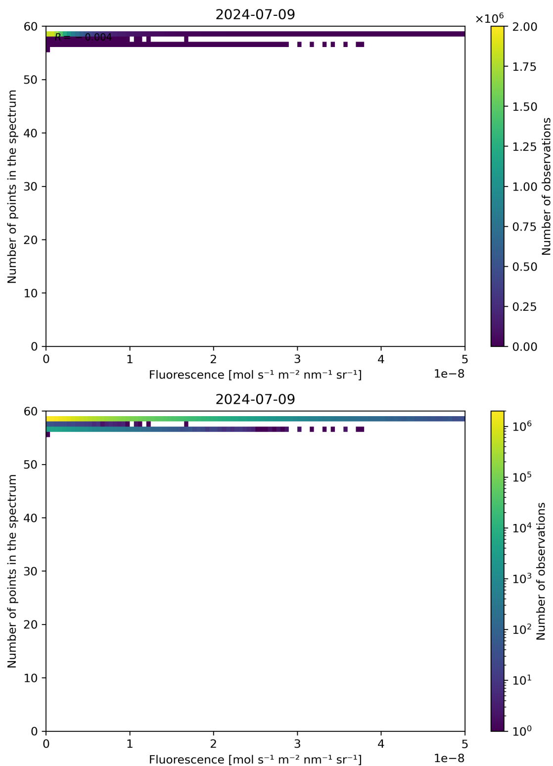
Figure 86: Scatter density plot of “Fluorescence” against “Number of points in the spectrum” for 2024-07-08 to 2024-07-10.
