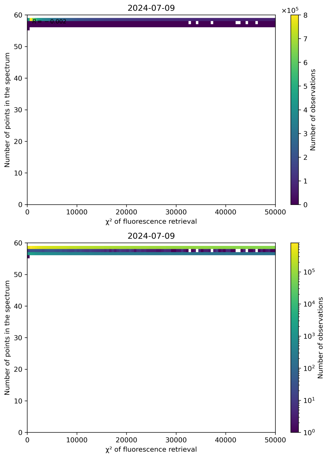
Figure 68: Scatter density plot of " \chi^2 of fluorescence retrieval" against "Number of points in the spectrum" for 2024-07-08 to 2024-07-10.
