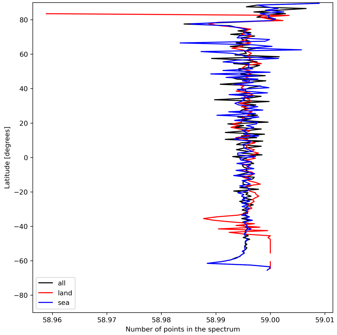
Figure 27: Zonal average of “Number of points in the spectrum” for 2024-07-08 to 2024-07-10.
