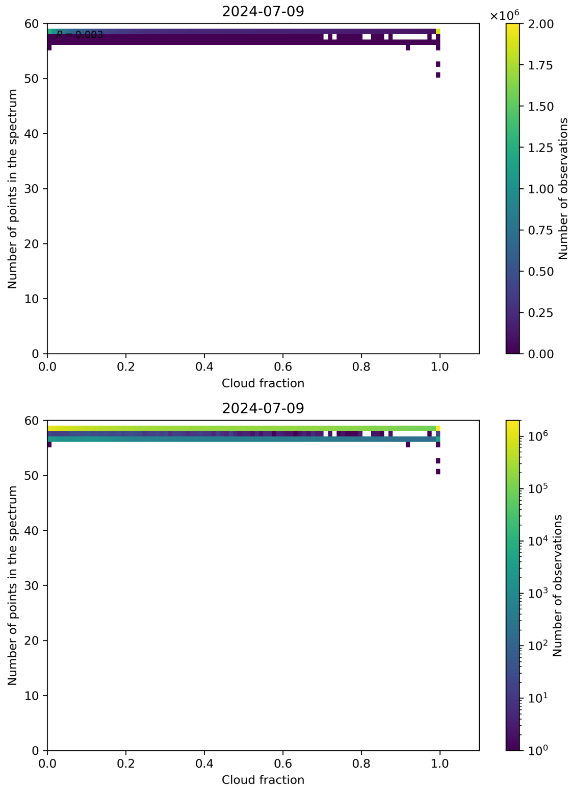
Figure 74: Scatter density plot of “Cloud fraction” against “Number of points in the spectrum” for 2024-07-08 to 2024-07-10.
