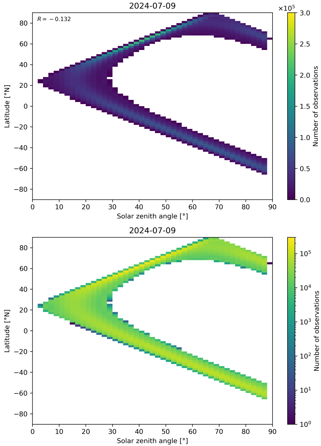
Figure 113: Scatter density plot of “Solar zenith angle” against “Latitude” for 2024-07-08 to 2024-07-10.
