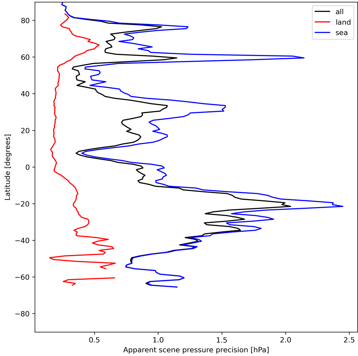
Figure 20: Zonal average of “Apparent scene pressure precision” for 2024-07-08 to 2024-07-10.
