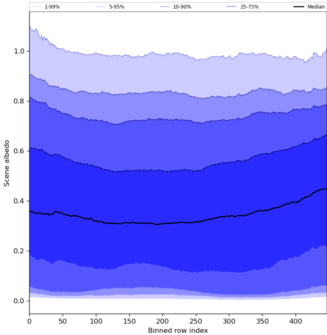
Figure 51: Along track statistics of “Scene albedo” for 2024-07-10 to 2024-07-11
