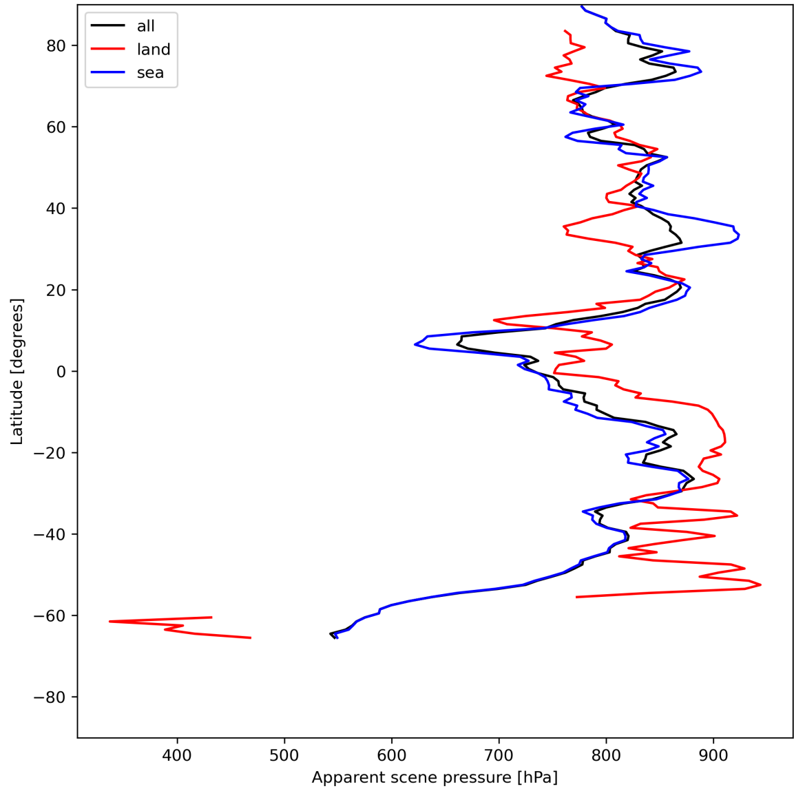
Figure 19: Zonal average of “Apparent scene pressure” for 2024-07-10 to 2024-07-11.
