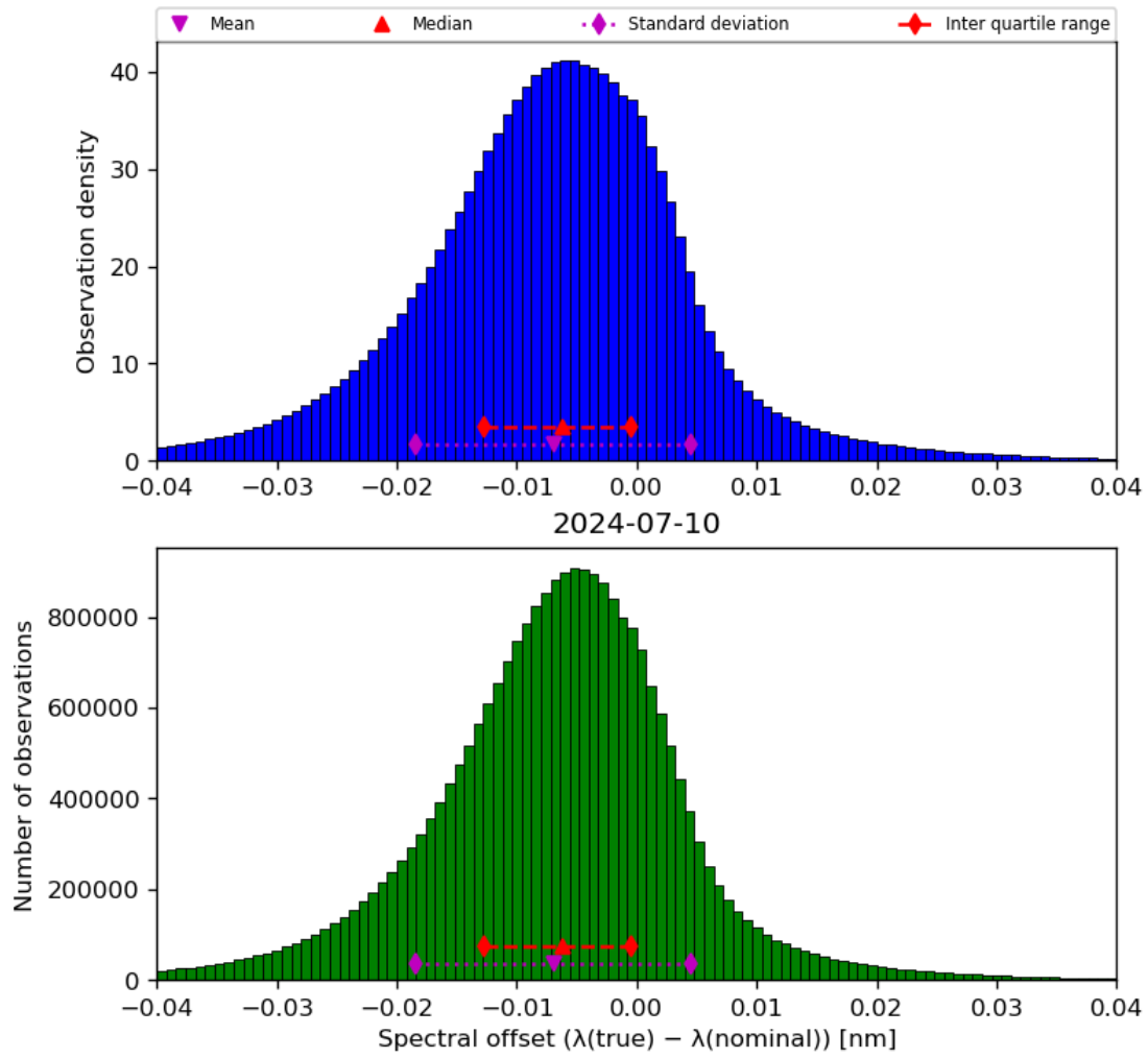
Figure 45: Histogram of “Spectral offset ( \lambda(\text{true}) - \lambda(\text{nominal}) )” for 2024-07-10 to 2024-07-11
