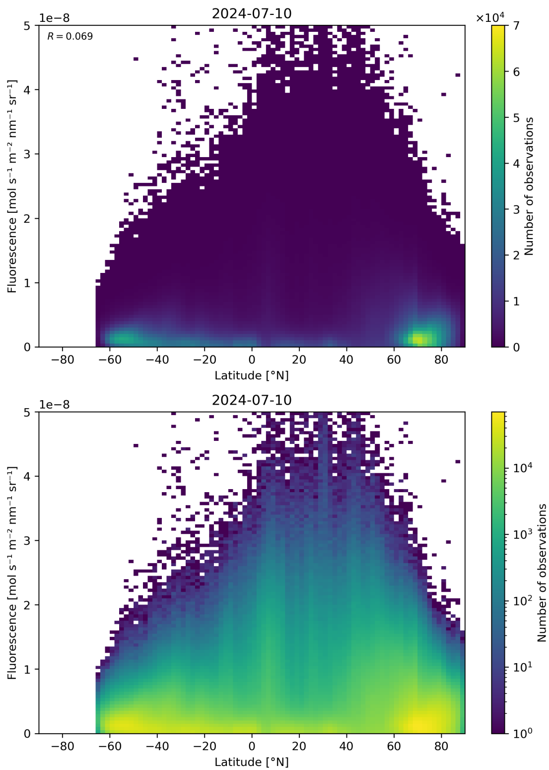
Figure 92: Scatter density plot of “Latitude” against “Fluorescence” for 2024-07-10 to 2024-07-11.
