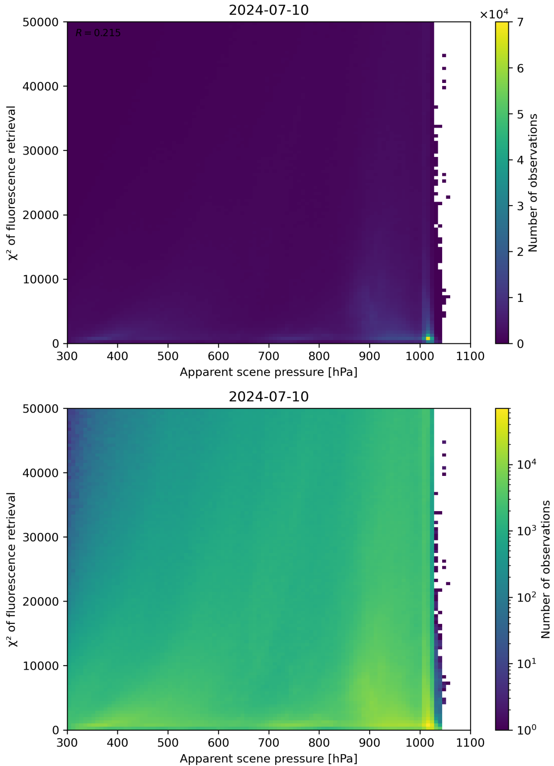
Figure 63: Scatter density plot of “Apparent scene pressure” against “ \chi^2 of fluorescence retrieval” for 2024-07-10 to 2024-07-11.
