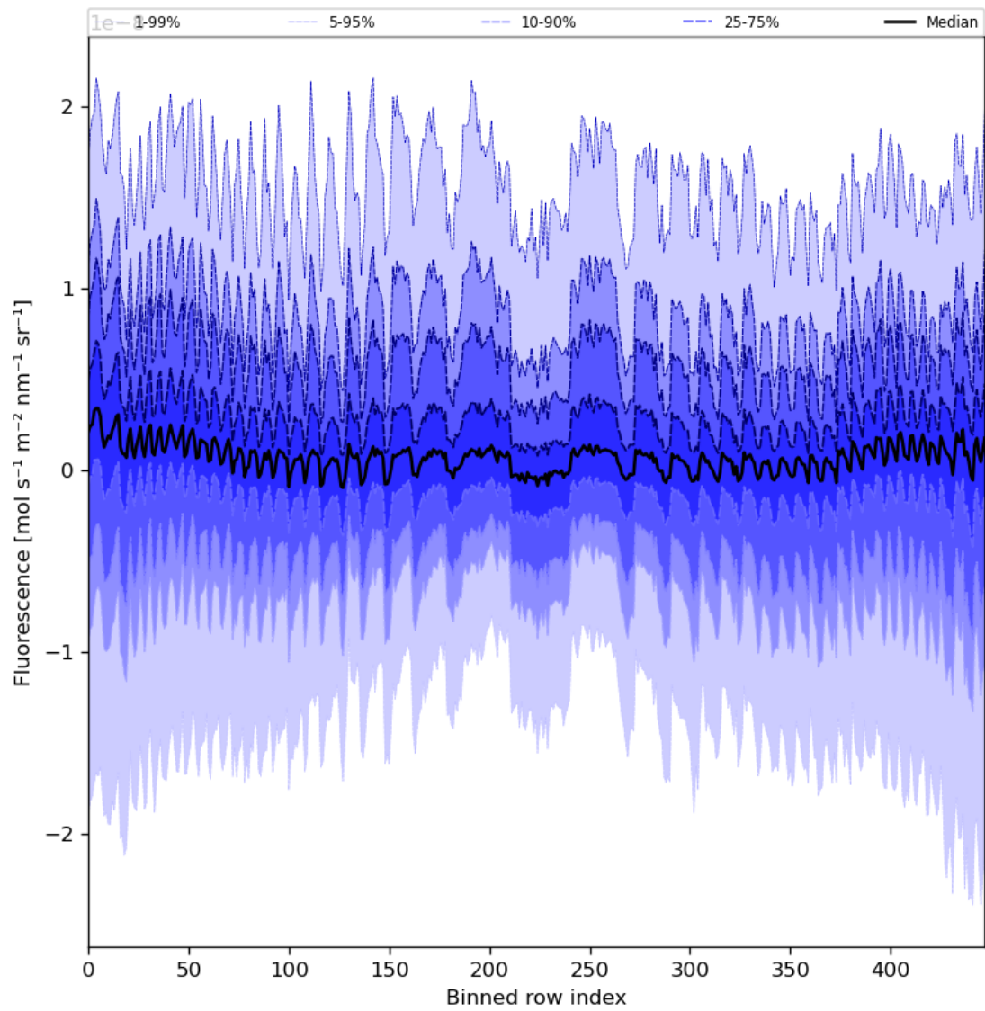
Figure 57: Along track statistics of “Fluorescence” for 2024-07-10 to 2024-07-11
