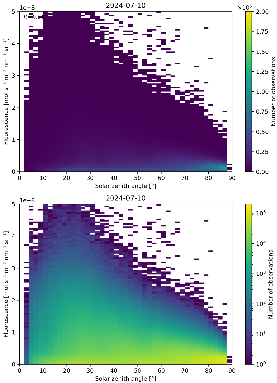
Figure 112: Scatter density plot of “Solar zenith angle” against “Fluorescence” for 2024-07-10 to 2024-07-11.
