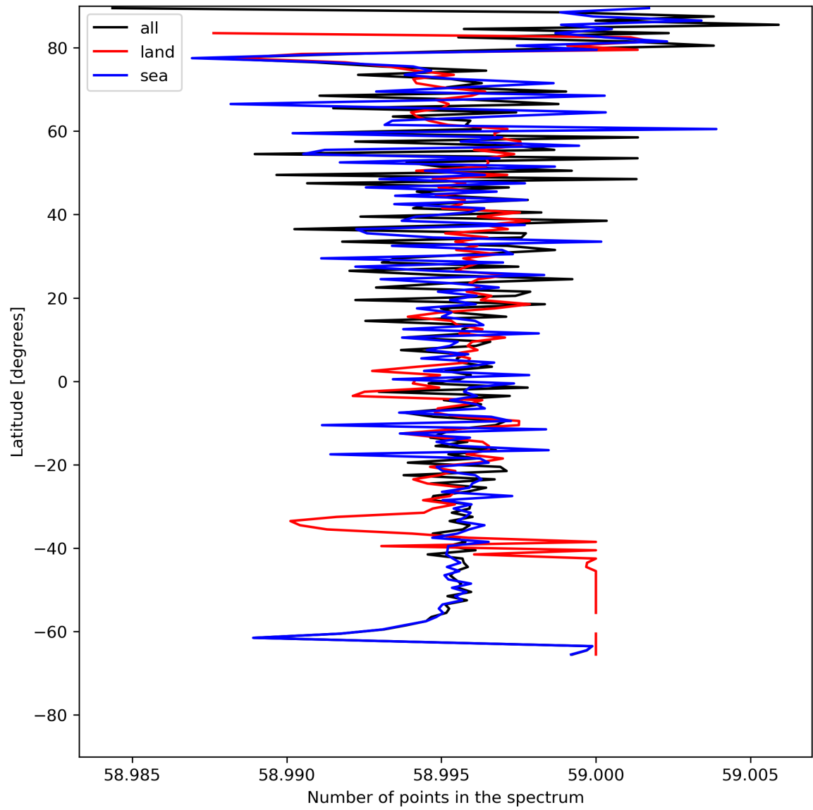
Figure 27: Zonal average of “Number of points in the spectrum” for 2024-07-10 to 2024-07-11.
