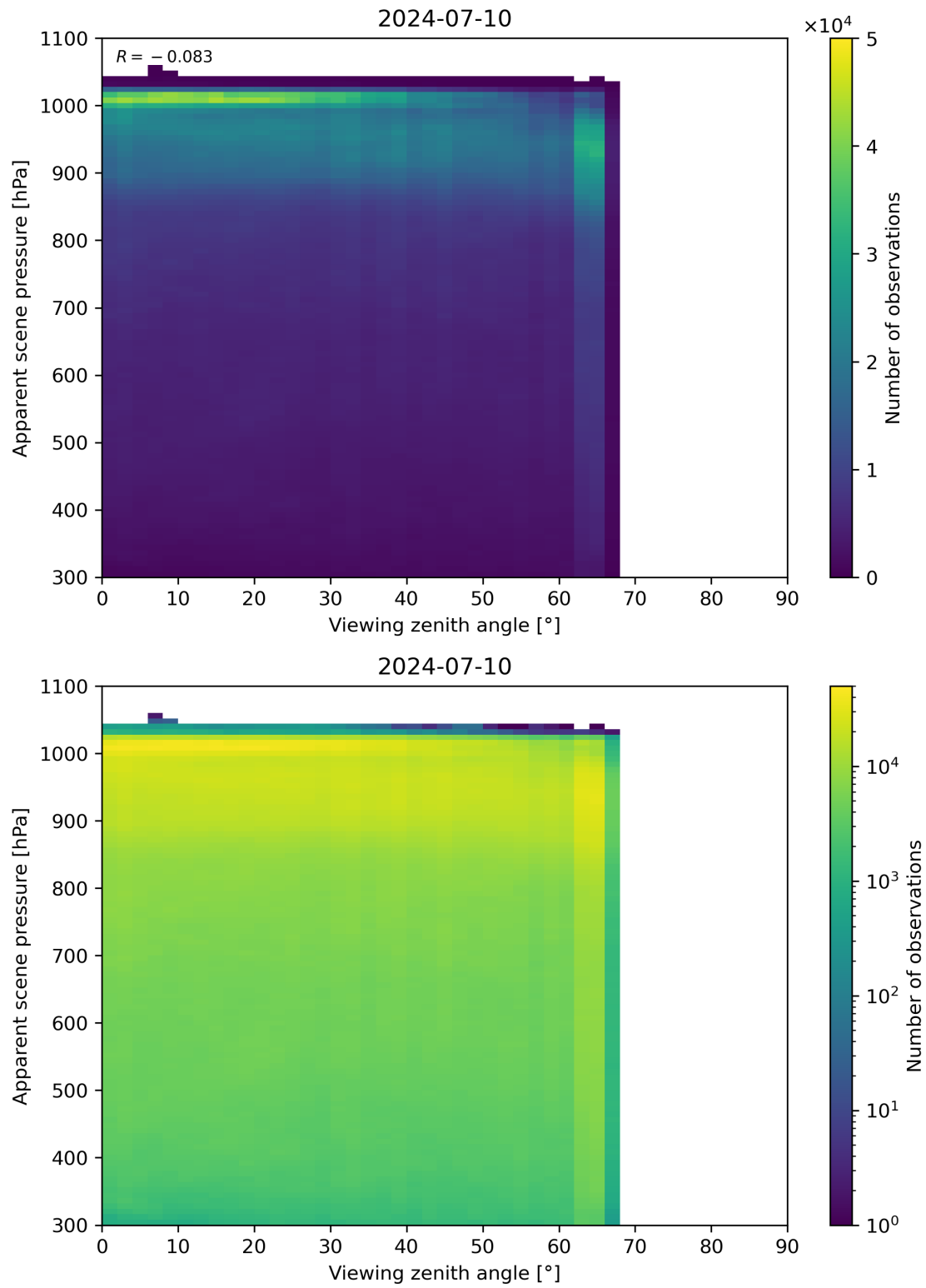
Figure 118: Scatter density plot of “Viewing zenith angle” against “Apparent scene pressure” for 2024-07-10 to 2024-07-11.
