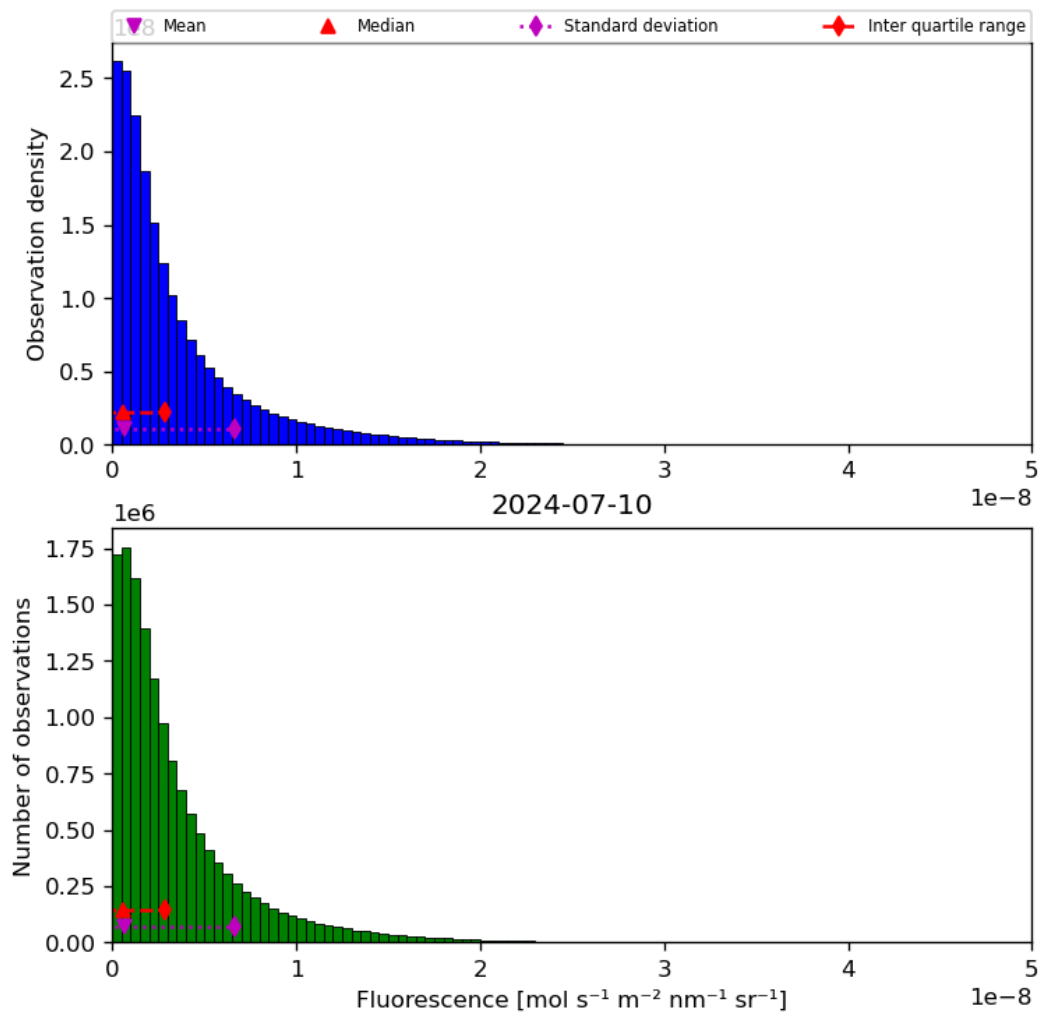
Figure 40: Histogram of “Fluorescence” for 2024-07-10 to 2024-07-11
