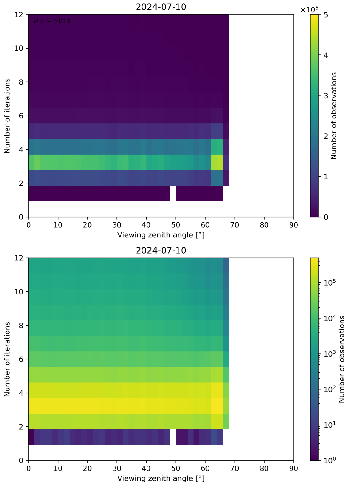
Figure 124: Scatter density plot of “Viewing zenith angle” against “Number of iterations” for 2024-07-10 to 2024-07-11.
