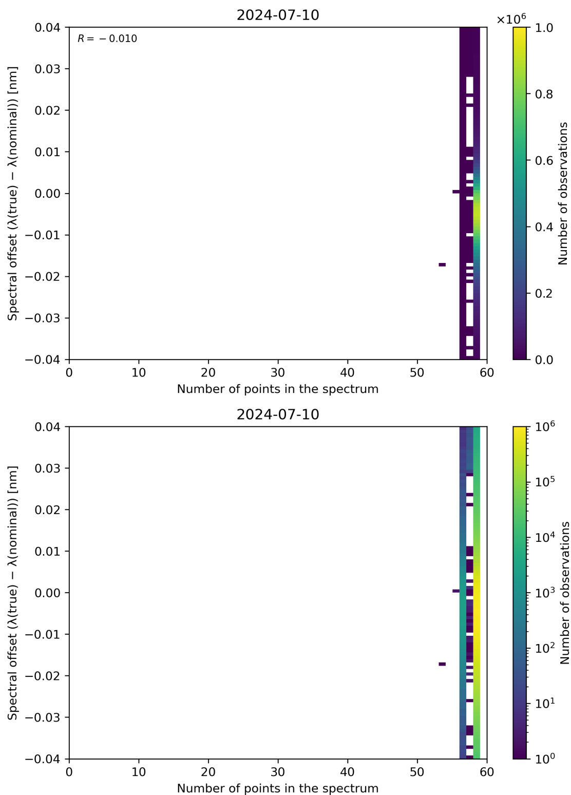
Figure 101: Scatter density plot of “Number of points in the spectrum” against “Spectral offset ( \lambda(\text{true}) - \lambda(\text{nominal}) )” for 2024-07-10 to 2024-07-11.
