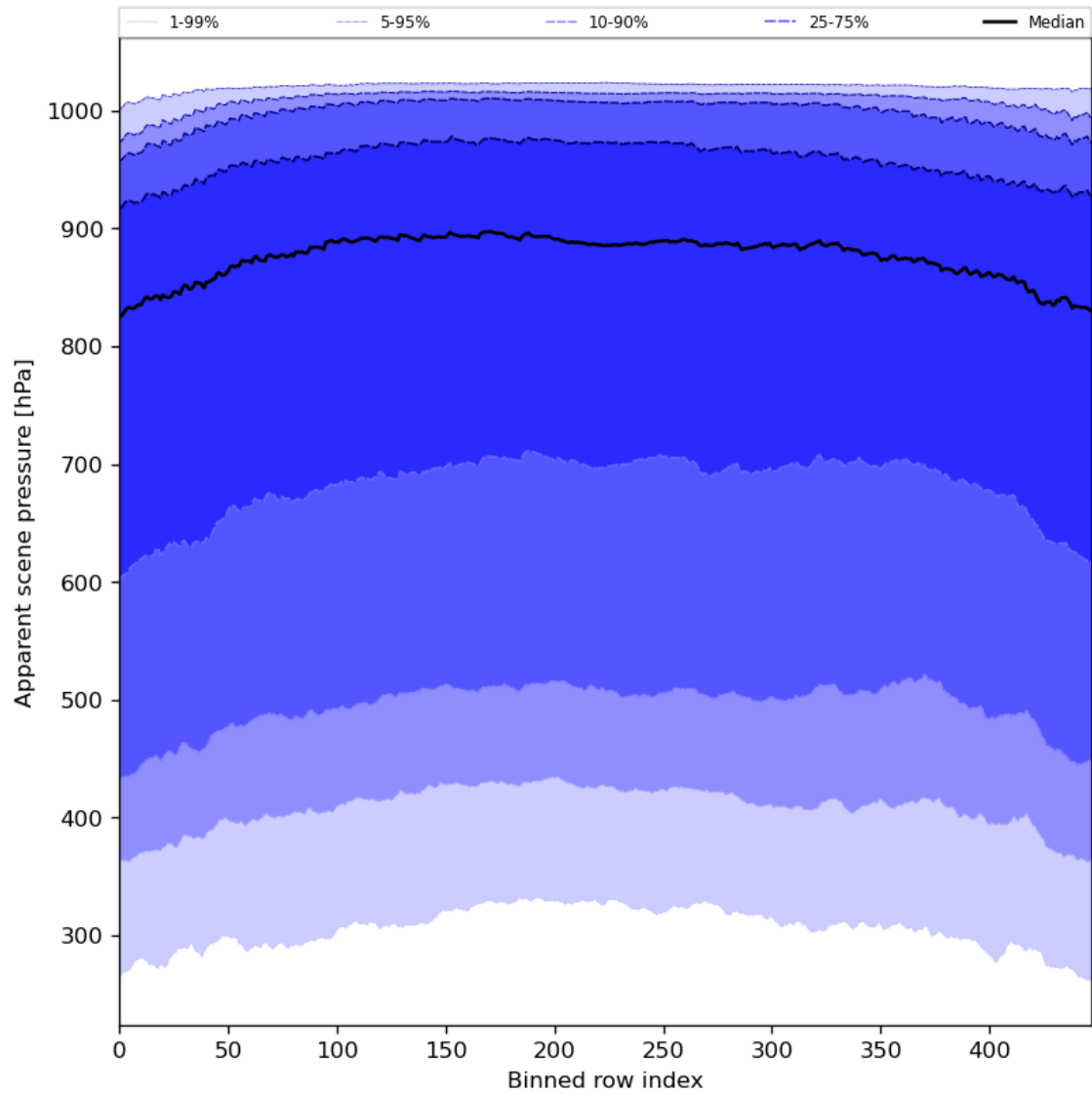
Figure 53: Along track statistics of “Apparent scene pressure” for 2024-07-10 to 2024-07-11
