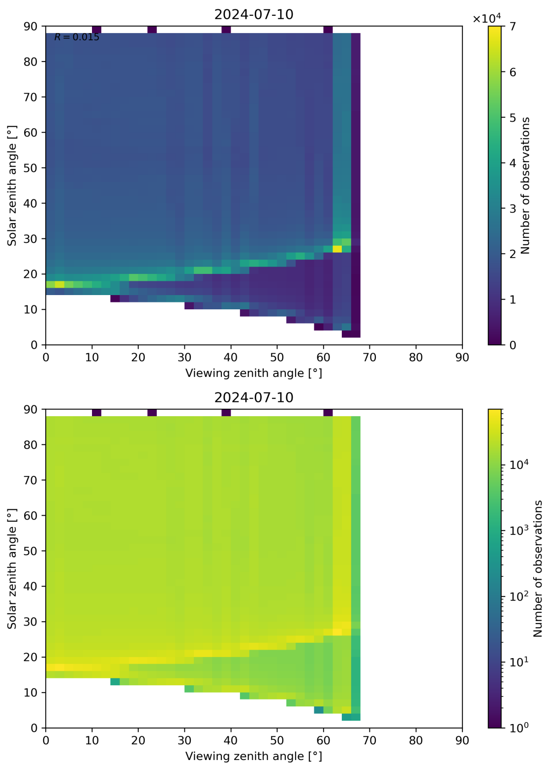
Figure 127: Scatter density plot of “Viewing zenith angle” against “Solar zenith angle” for 2024-07-10 to 2024-07-11.
