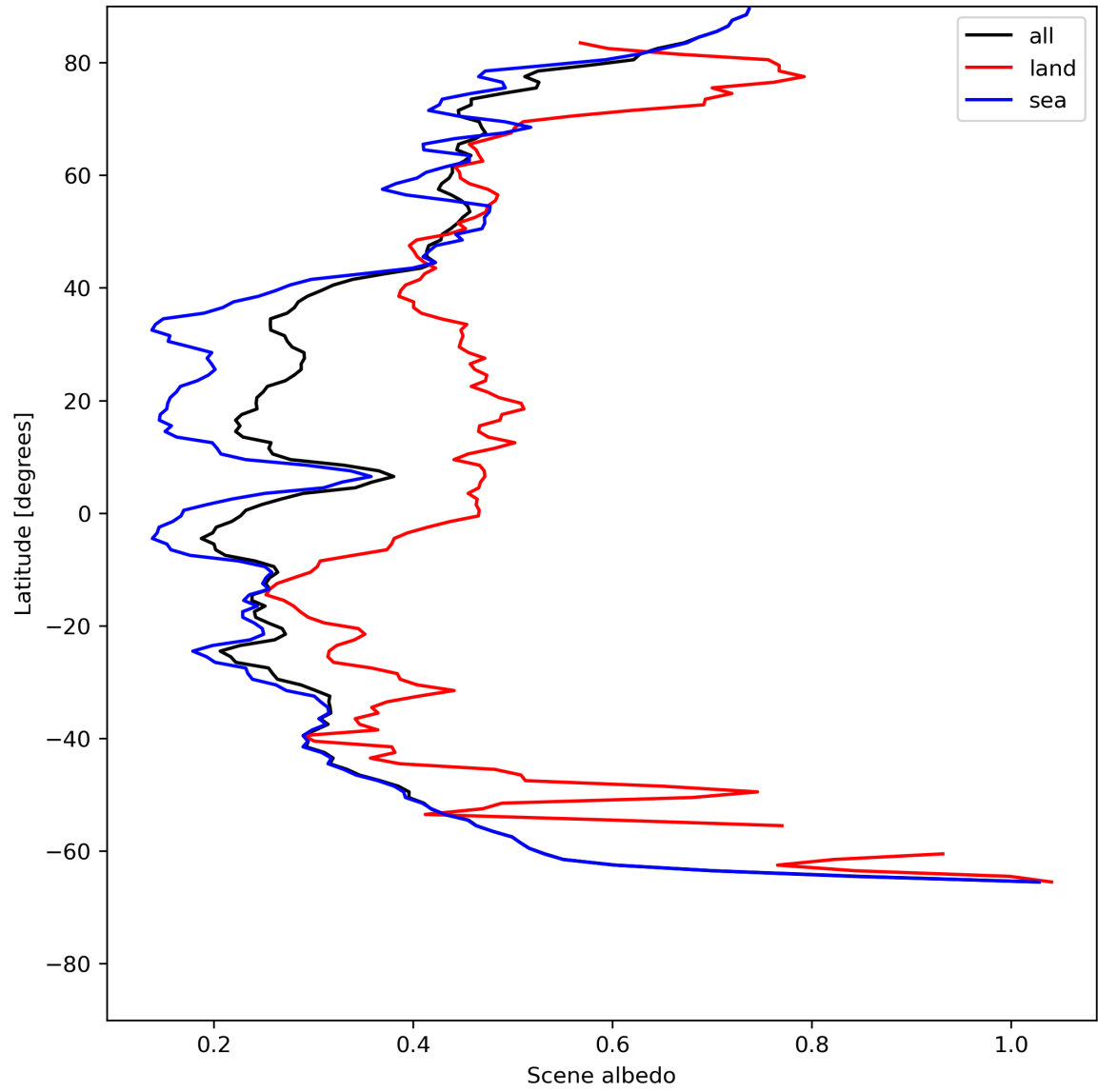
Figure 17: Zonal average of “Scene albedo” for 2024-07-10 to 2024-07-11.
