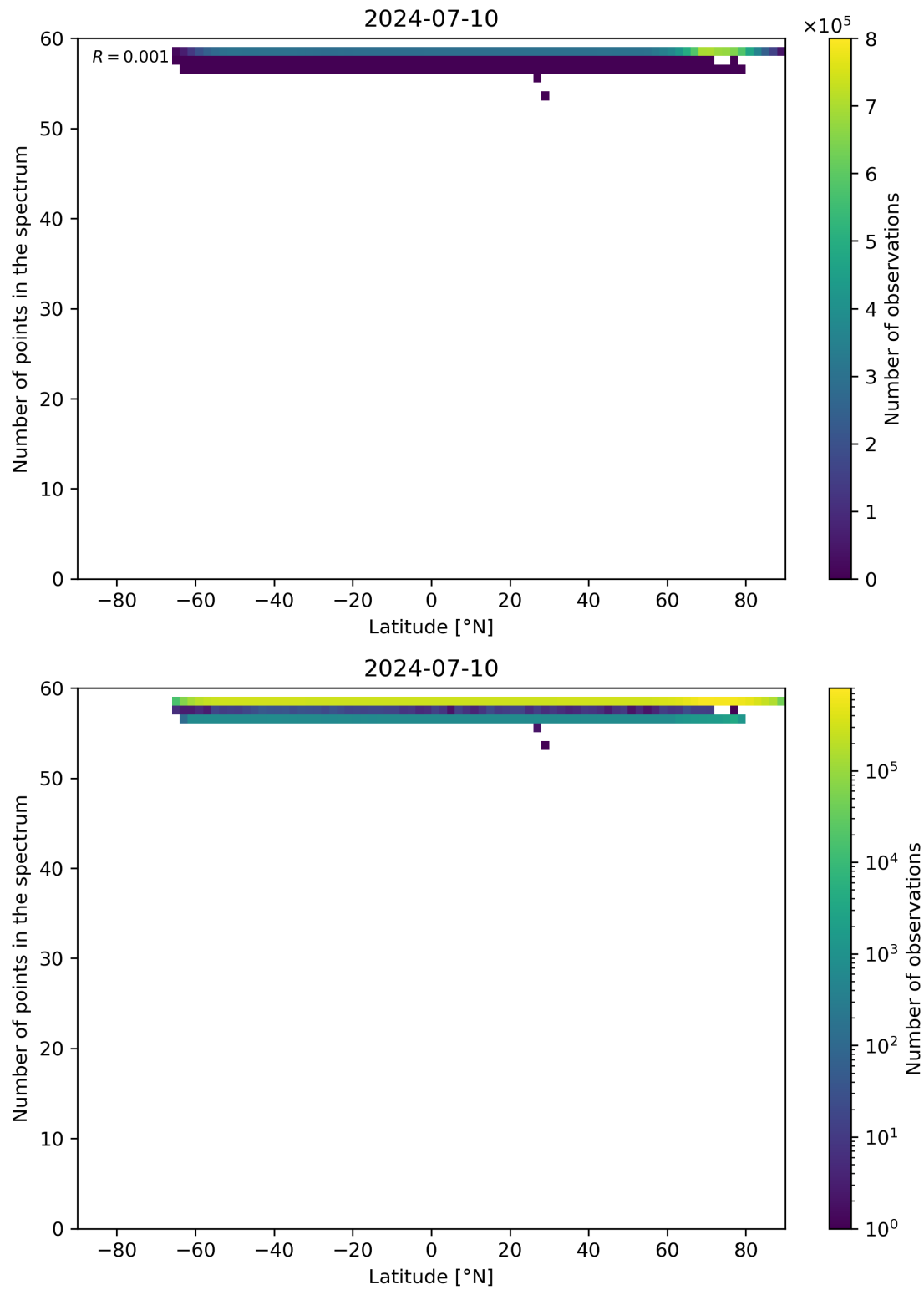
Figure 94: Scatter density plot of “Latitude” against “Number of points in the spectrum” for 2024-07-10 to 2024-07-11.
