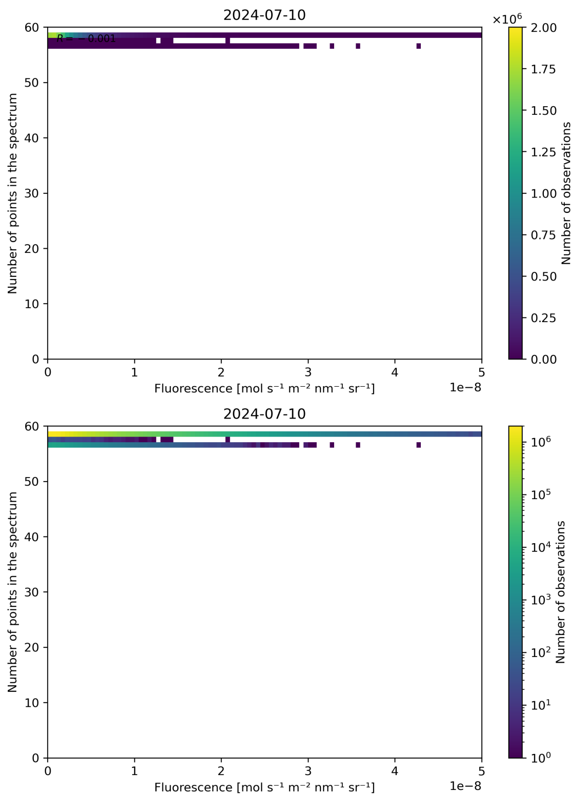
Figure 86: Scatter density plot of “Fluorescence” against “Number of points in the spectrum” for 2024-07-10 to 2024-07-11.
