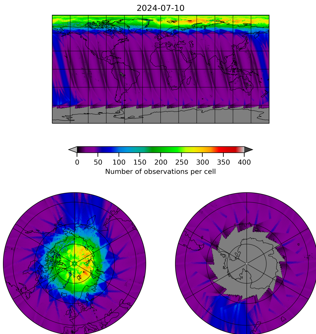
Figure 11: Map of the number of observations for 2024-07-10 to 2024-07-11
