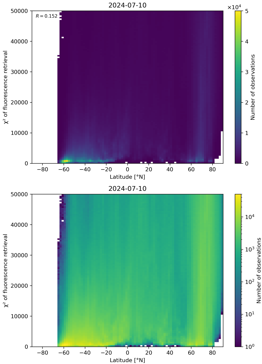
Figure 89: Scatter density plot of “Latitude” against “ \chi^2 of fluorescence retrieval” for 2024-07-10 to 2024-07-11.
