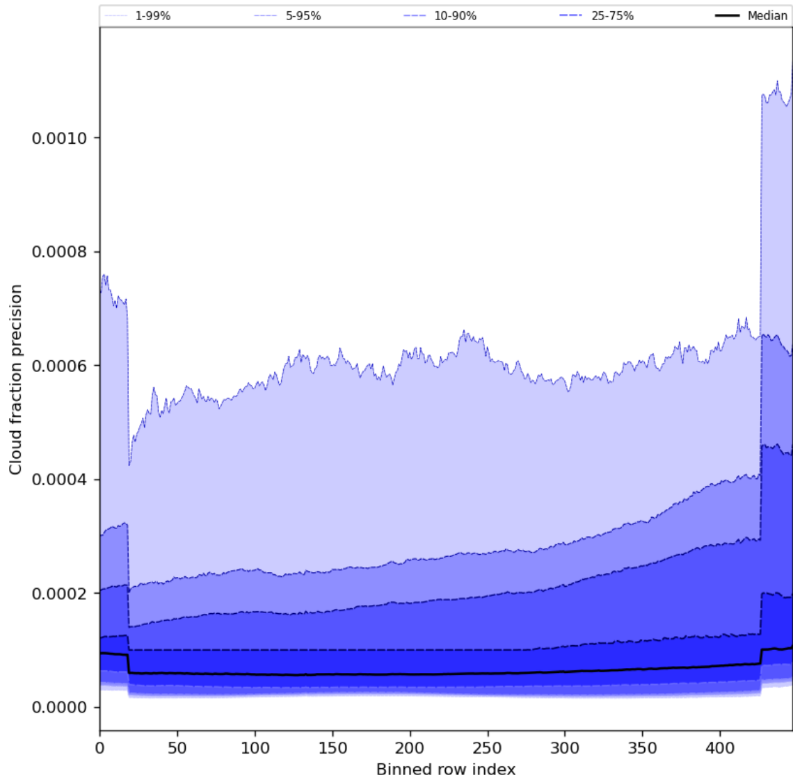
Figure 50: Along track statistics of “Cloud fraction precision” for 2024-07-10 to 2024-07-11
