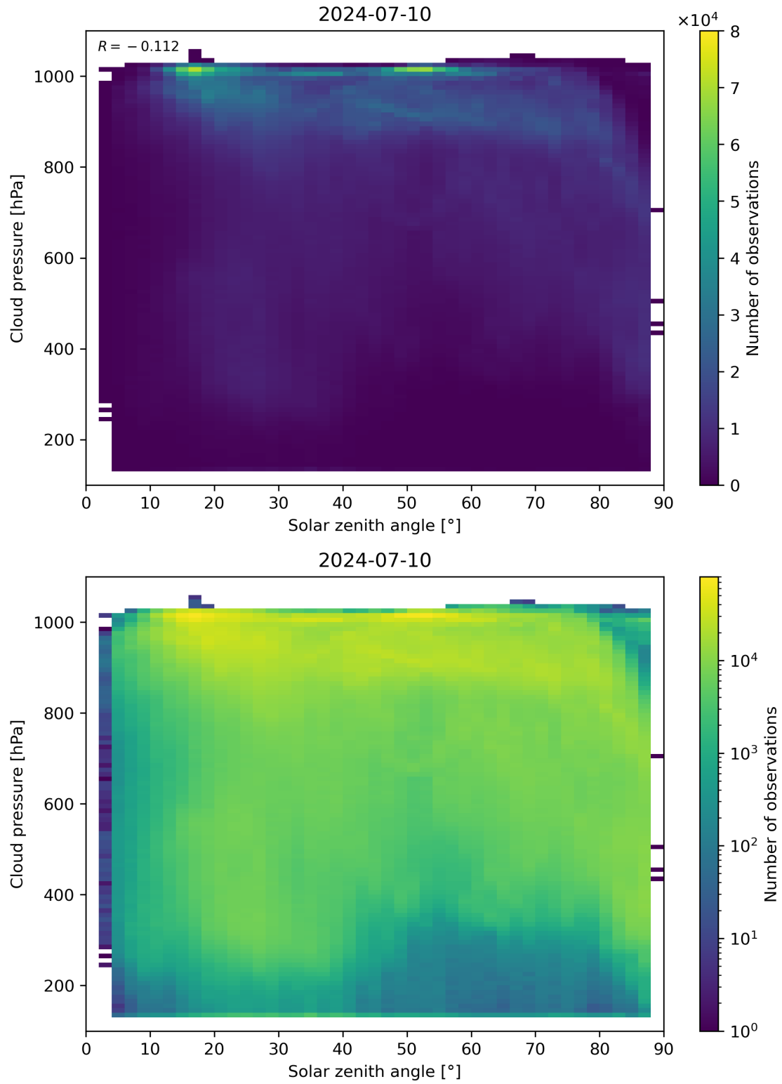
Figure 111: Scatter density plot of “Solar zenith angle” against “Cloud pressure” for 2024-07-10 to 2024-07-11.
