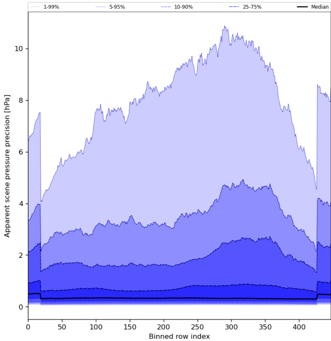
Figure 54: Along track statistics of “Apparent scene pressure precision” for 2024-07-10 to 2024-07-11
