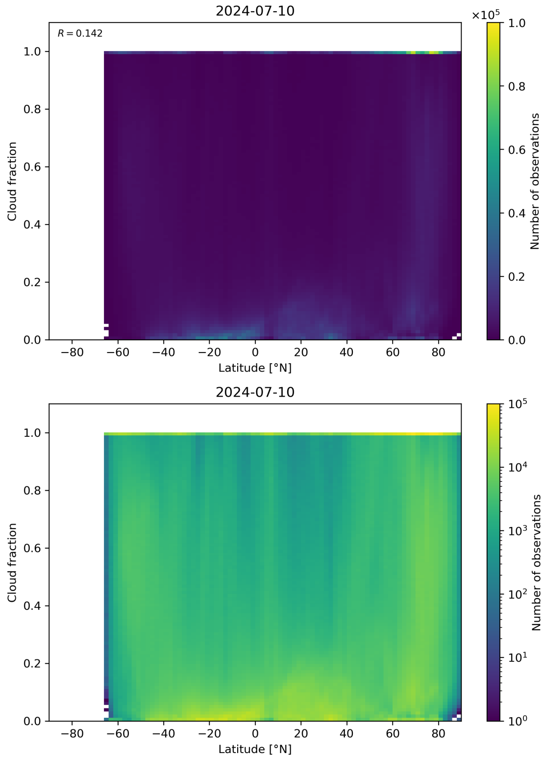
Figure 90: Scatter density plot of “Latitude” against “Cloud fraction” for 2024-07-10 to 2024-07-11.
