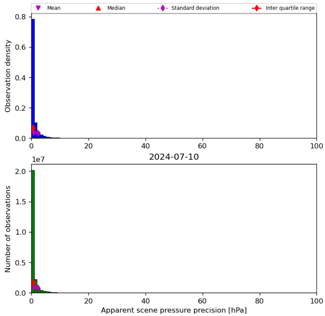
Figure 37: Histogram of “Apparent scene pressure precision” for 2024-07-10 to 2024-07-11
