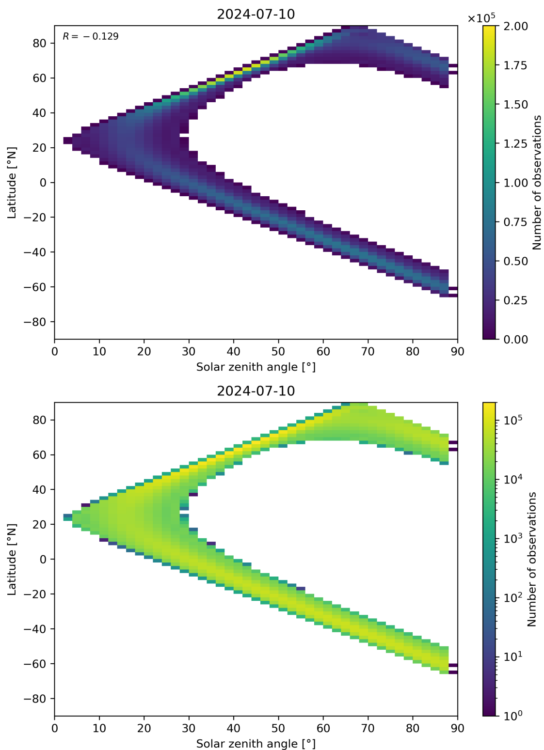
Figure 113: Scatter density plot of “Solar zenith angle” against “Latitude” for 2024-07-10 to 2024-07-11.
