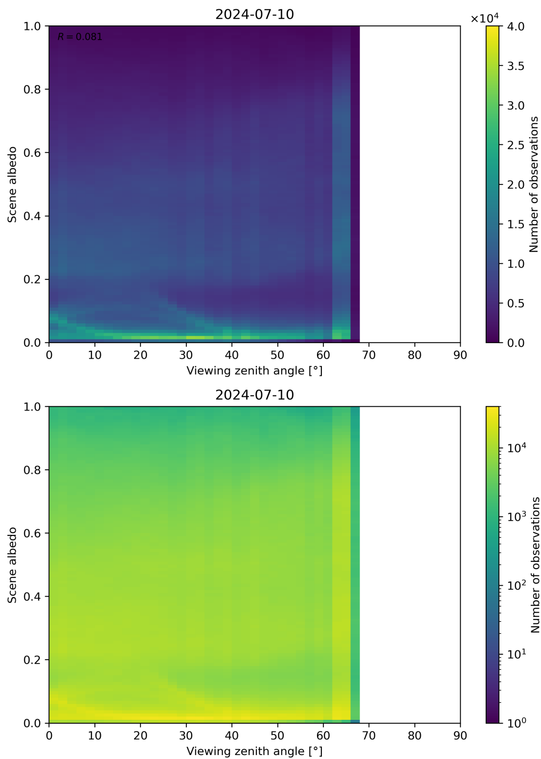
Figure 126: Scatter density plot of “Viewing zenith angle” against “Scene albedo” for 2024-07-10 to 2024-07-11.
