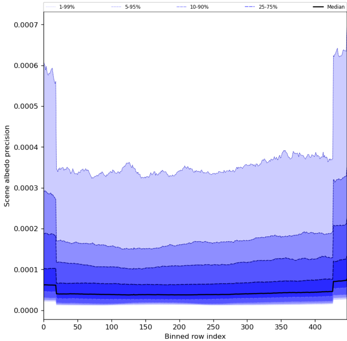
Figure 52: Along track statistics of “Scene albedo precision” for 2024-07-10 to 2024-07-11
