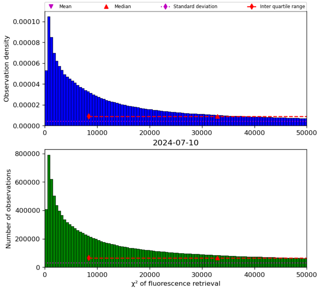
Figure 42: Histogram of “ \chi^2 of fluorescence retrieval” for 2024-07-10 to 2024-07-11
