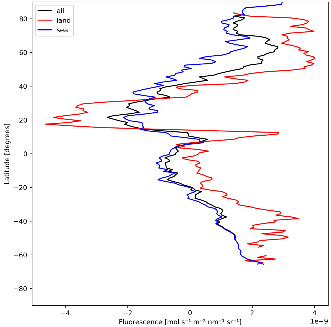
Figure 23: Zonal average of “Fluorescence” for 2024-07-10 to 2024-07-11.
