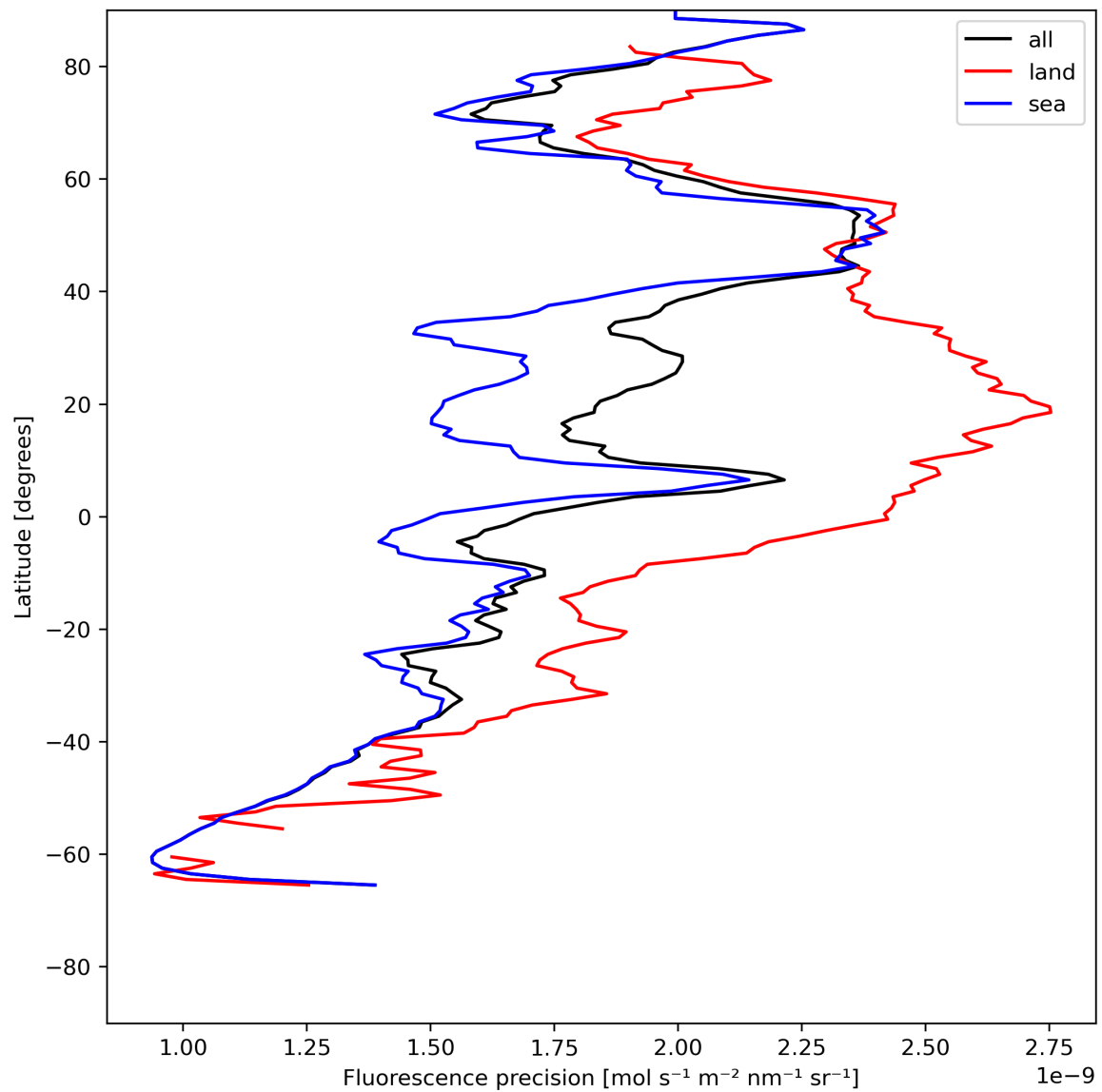
Figure 24: Zonal average of “Fluorescence precision” for 2024-07-10 to 2024-07-11.
