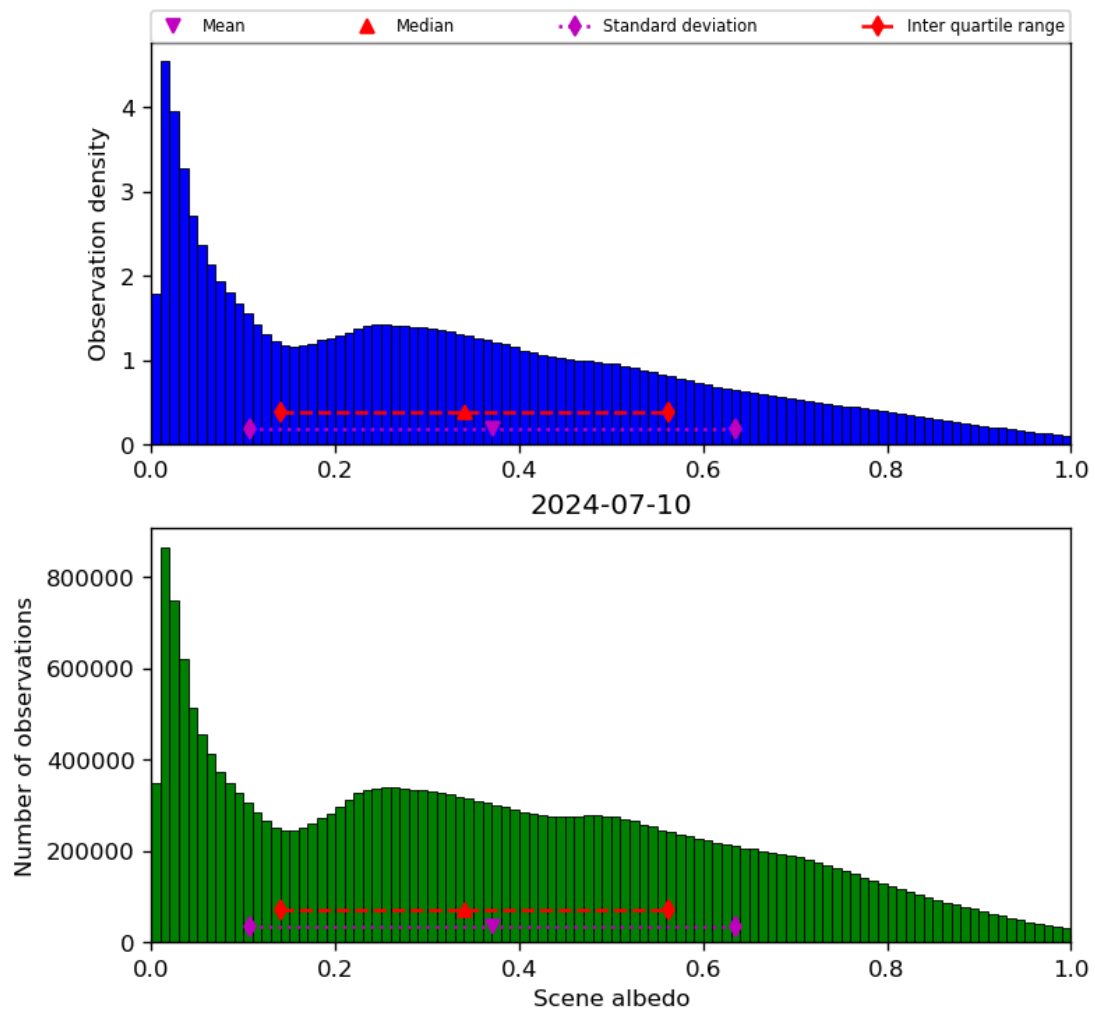
Figure 34: Histogram of “Scene albedo” for 2024-07-10 to 2024-07-11
