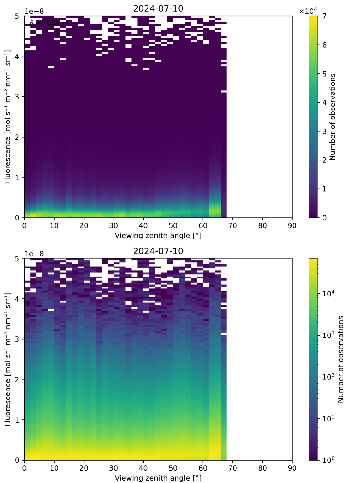
Figure 122: Scatter density plot of “Viewing zenith angle” against “Fluorescence” for 2024-07-10 to 2024-07-11.
