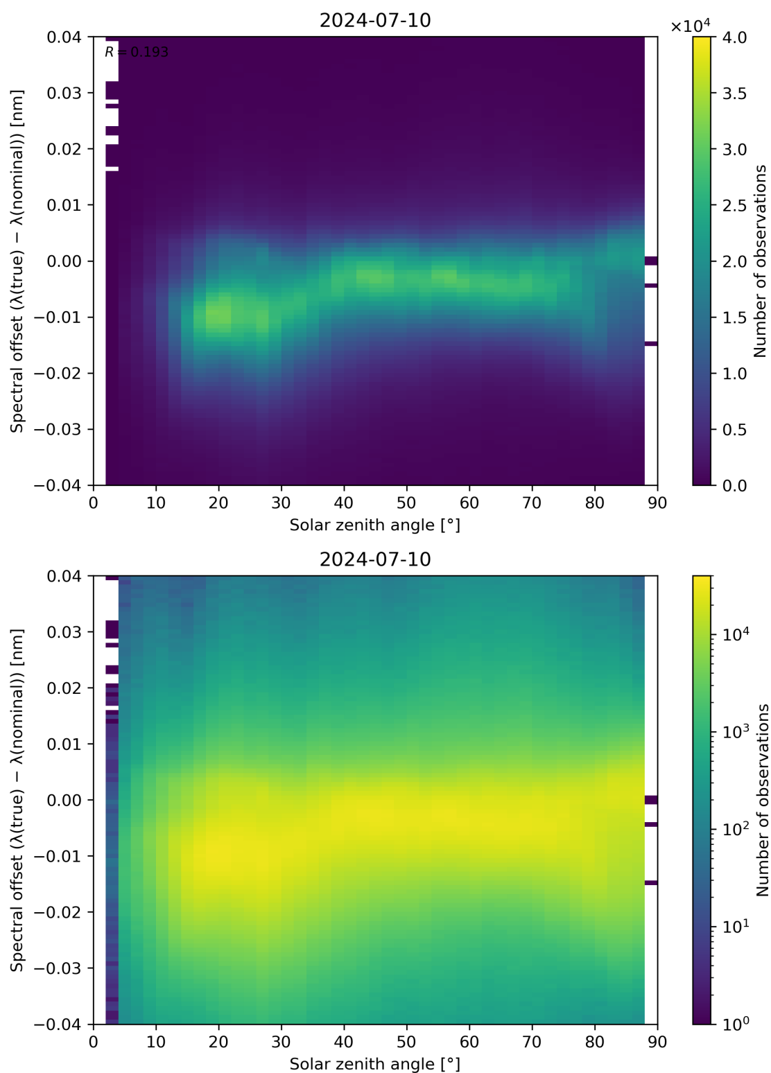
Figure 117: Scatter density plot of “Solar zenith angle” against “Spectral offset ( \lambda(\text{true}) - \lambda(\text{nominal}) )” for 2024-07-10 to 2024-07-11.
