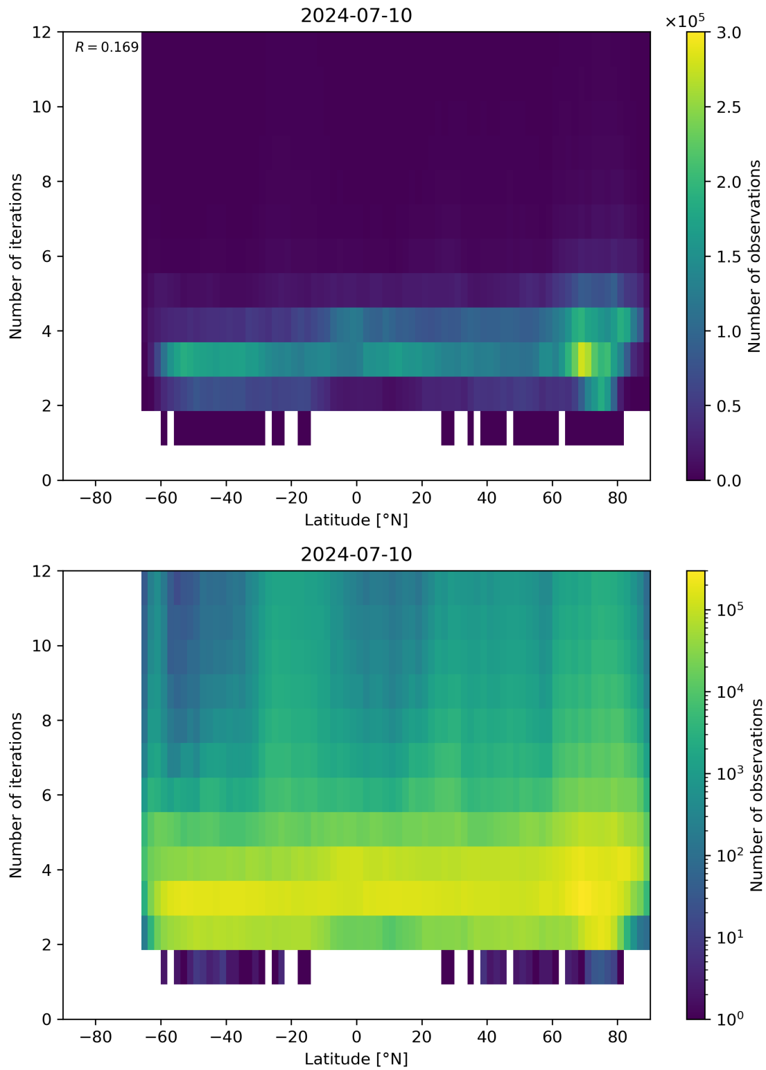
Figure 93: Scatter density plot of “Latitude” against “Number of iterations” for 2024-07-10 to 2024-07-11.
