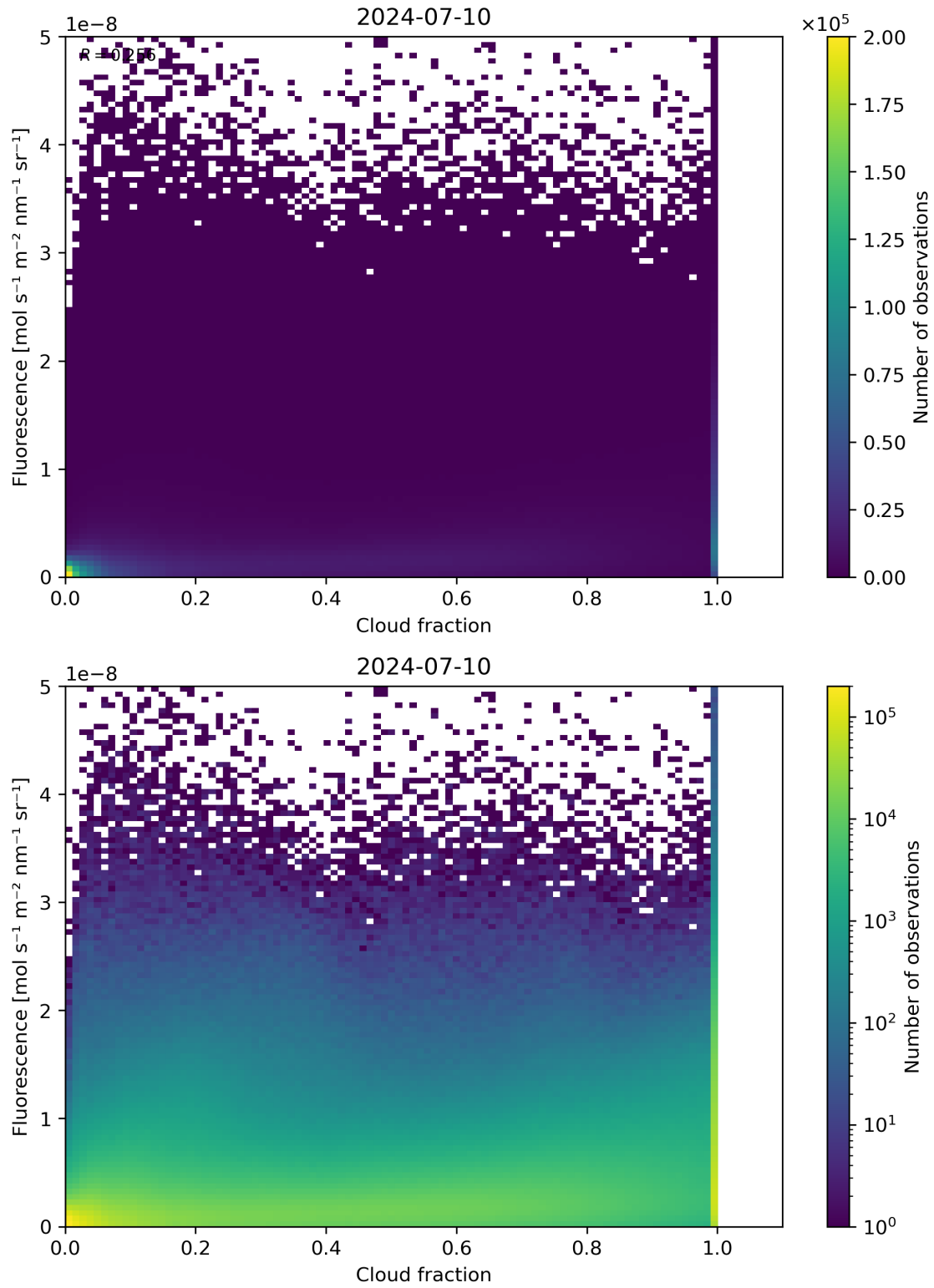
Figure 72: Scatter density plot of “Cloud fraction” against “Fluorescence” for 2024-07-10 to 2024-07-11.
