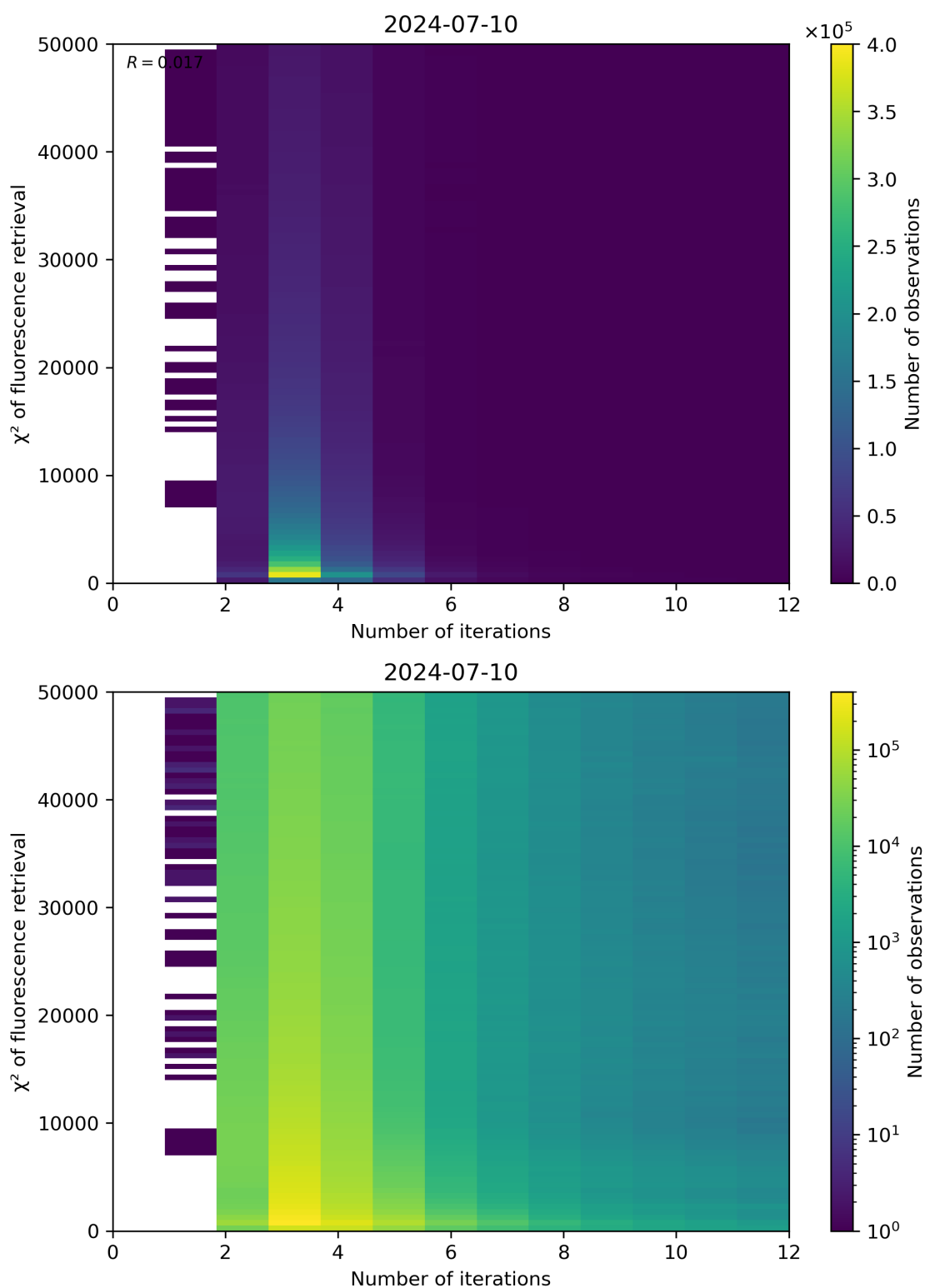
Figure 97: Scatter density plot of “Number of iterations” against “ \chi^2 of fluorescence retrieval” for 2024-07-10 to 2024-07-11.
