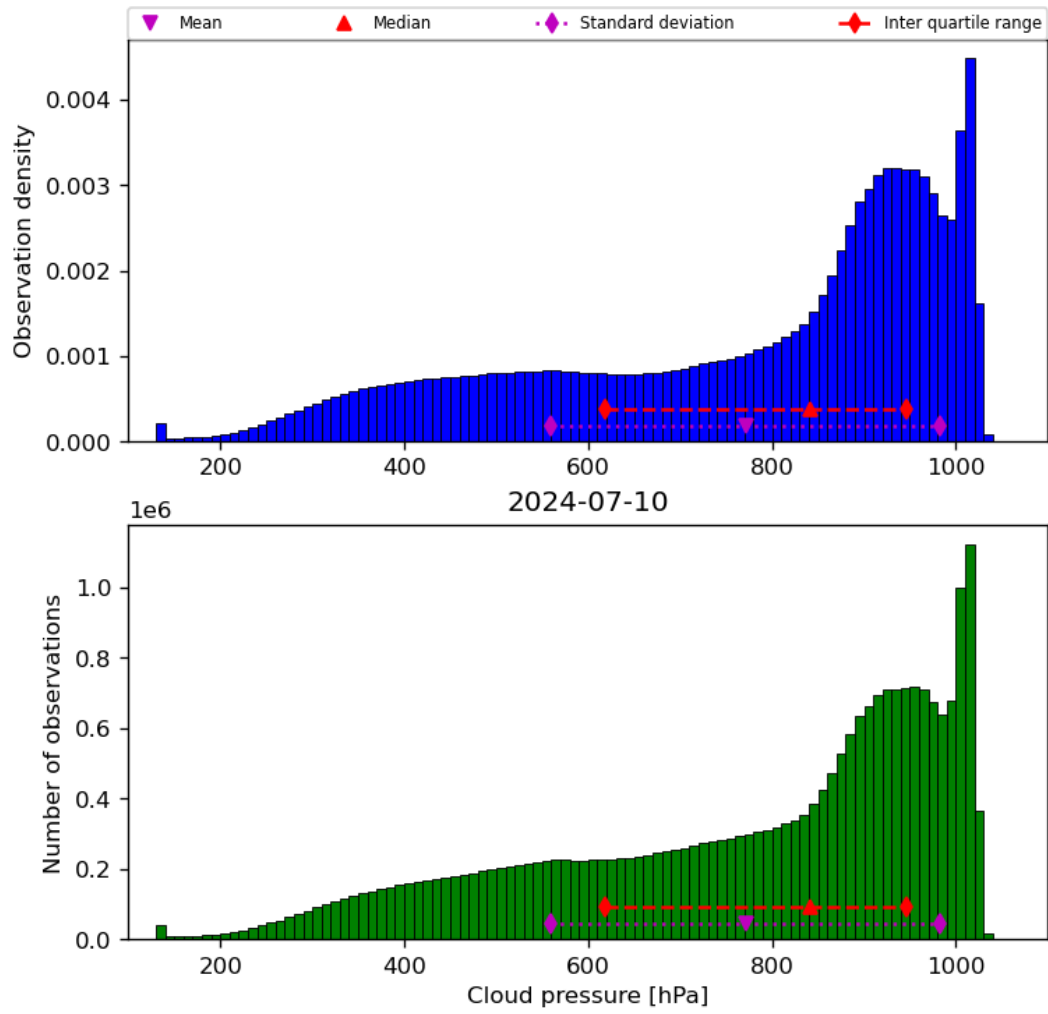
Figure 30: Histogram of “Cloud pressure” for 2024-07-10 to 2024-07-11
