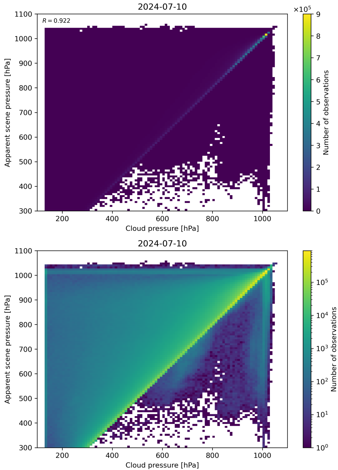
Figure 77: Scatter density plot of “Cloud pressure” against “Apparent scene pressure” for 2024-07-10 to 2024-07-11.
