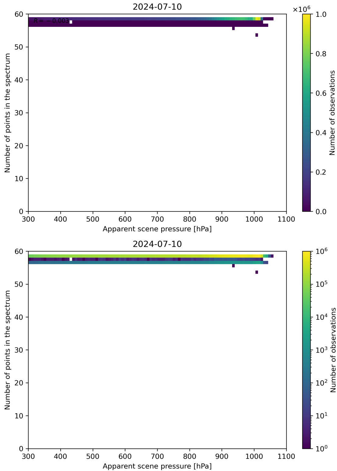
Figure 66: Scatter density plot of “Apparent scene pressure” against “Number of points in the spectrum” for 2024-07-10 to 2024-07-11.
