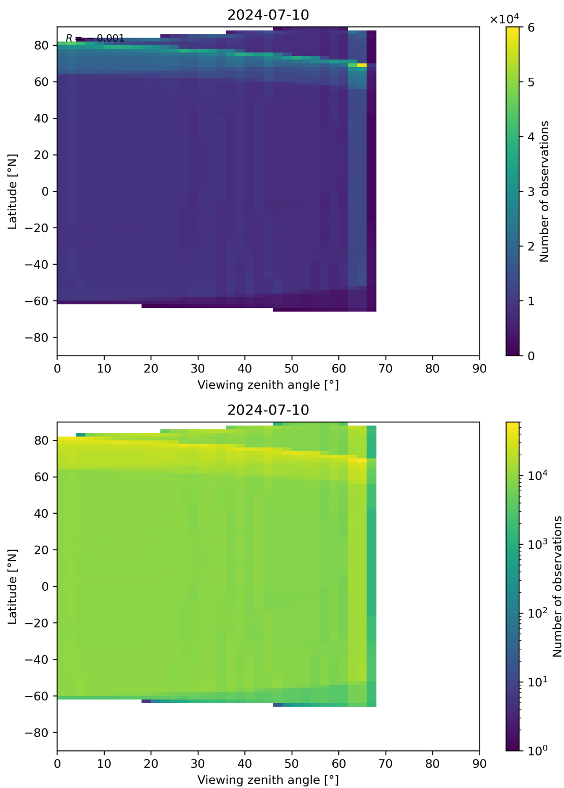
Figure 123: Scatter density plot of “Viewing zenith angle” against “Latitude” for 2024-07-10 to 2024-07-11.
