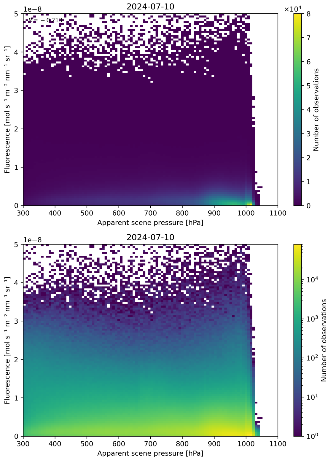
Figure 64: Scatter density plot of “Apparent scene pressure” against “Fluorescence” for 2024-07-10 to 2024-07-11.
