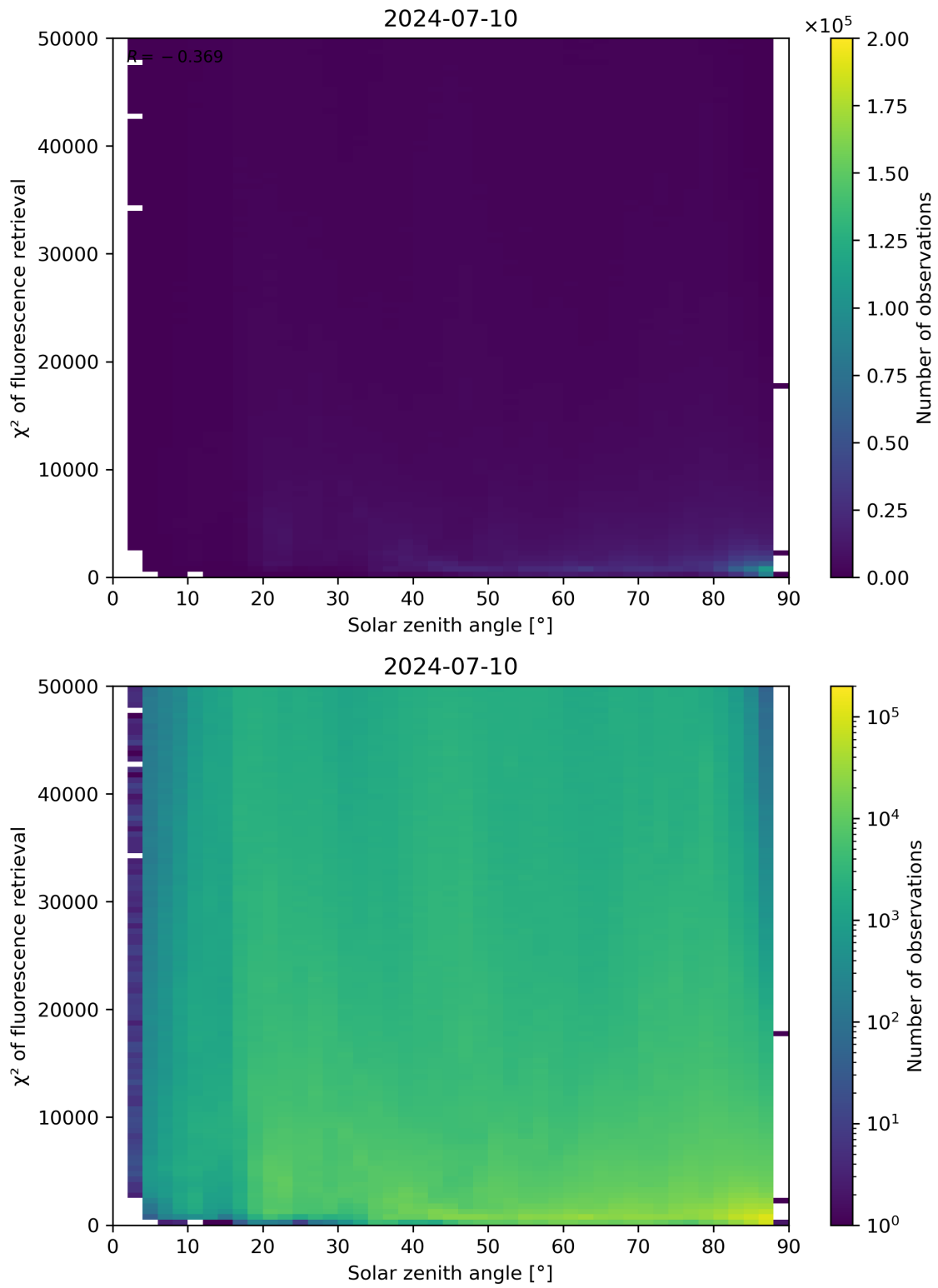
Figure 109: Scatter density plot of “Solar zenith angle” against “ \chi^2 of fluorescence retrieval” for 2024-07-10 to 2024-07-11.
