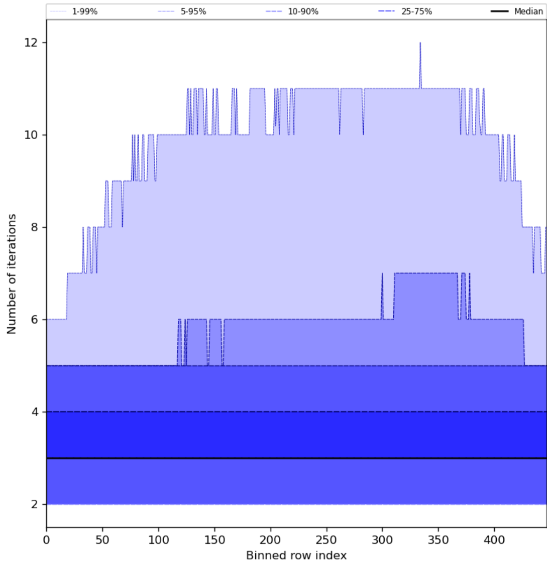
Figure 56: Along track statistics of “Number of iterations” for 2024-07-10 to 2024-07-11
