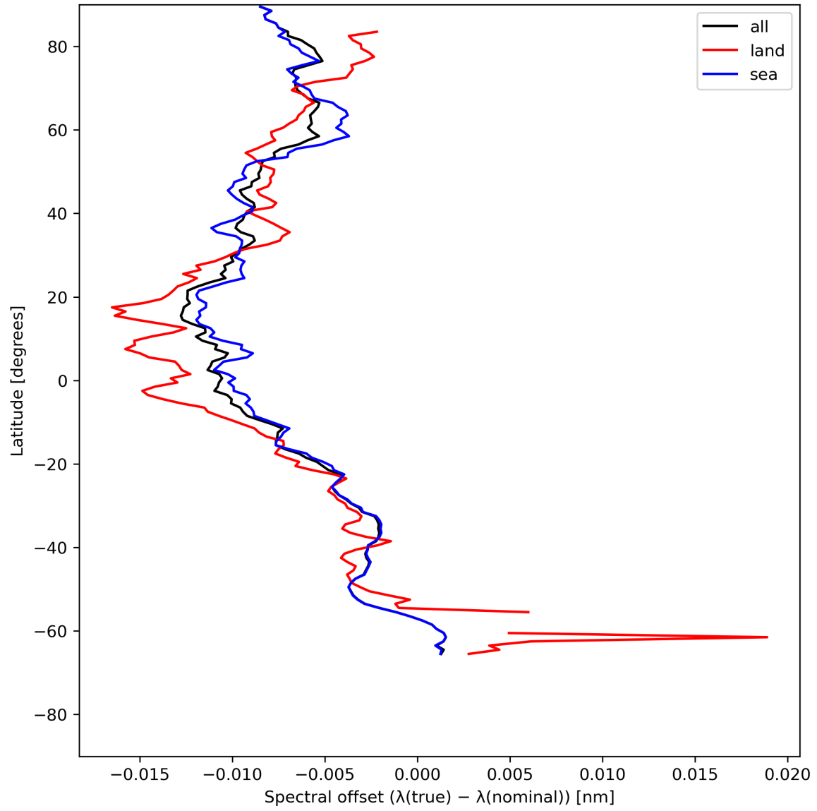
Figure 28: Zonal average of “Spectral offset ( \lambda(\text{true}) - \lambda(\text{nominal}) )” for 2024-07-10 to 2024-07-11.
