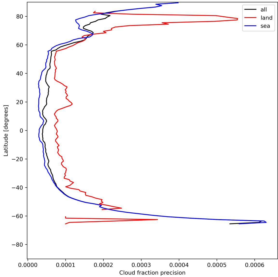
Figure 16: Zonal average of “Cloud fraction precision” for 2024-07-10 to 2024-07-11.
