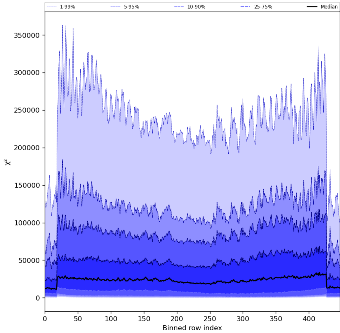
Figure 55: Along track statistics of “ \chi^2 ” for 2024-07-10 to 2024-07-11
