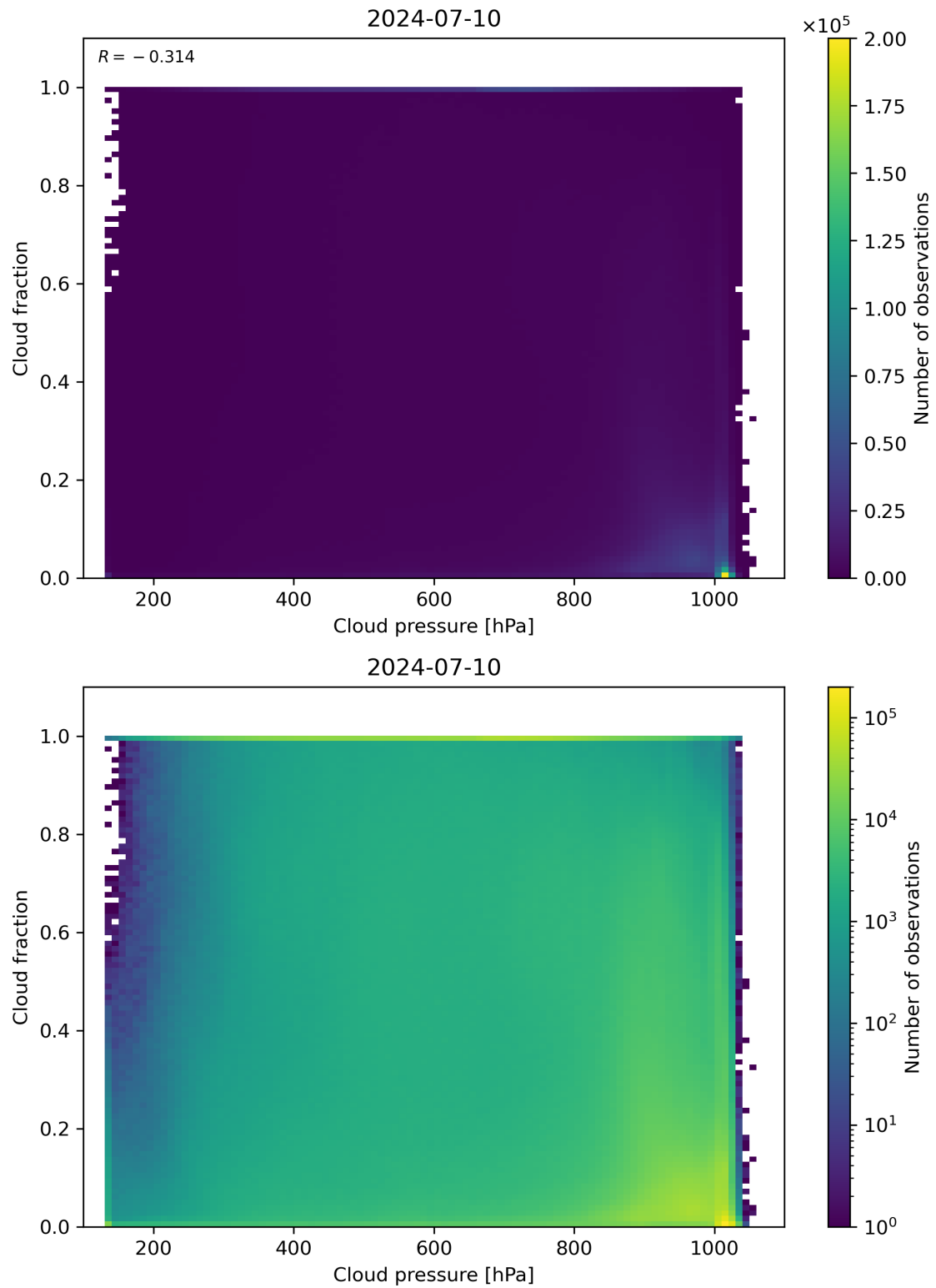
Figure 79: Scatter density plot of “Cloud pressure” against “Cloud fraction” for 2024-07-10 to 2024-07-11.
