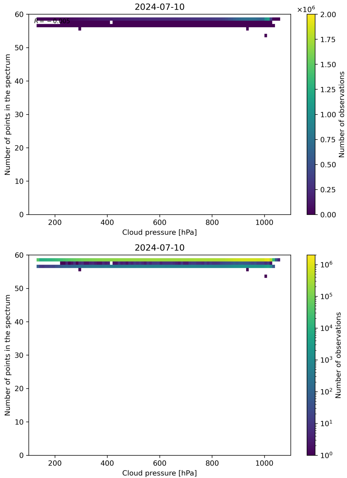
Figure 82: Scatter density plot of “Cloud pressure” against “Number of points in the spectrum” for 2024-07-10 to 2024-07-11.
