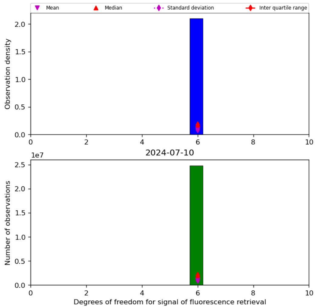
Figure 43: Histogram of "Degrees of freedom for signal of fluorescence retrieval" for 2024-07-10 to 2024-07-11
