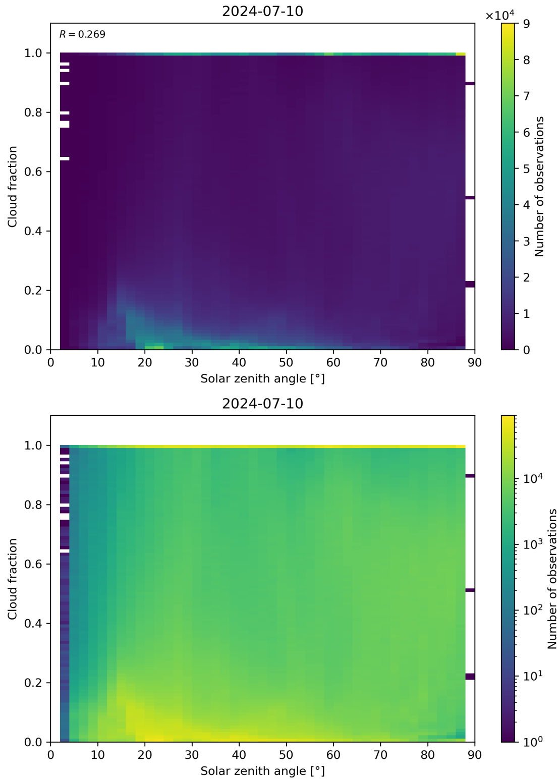
Figure 110: Scatter density plot of “Solar zenith angle” against “Cloud fraction” for 2024-07-10 to 2024-07-11.
