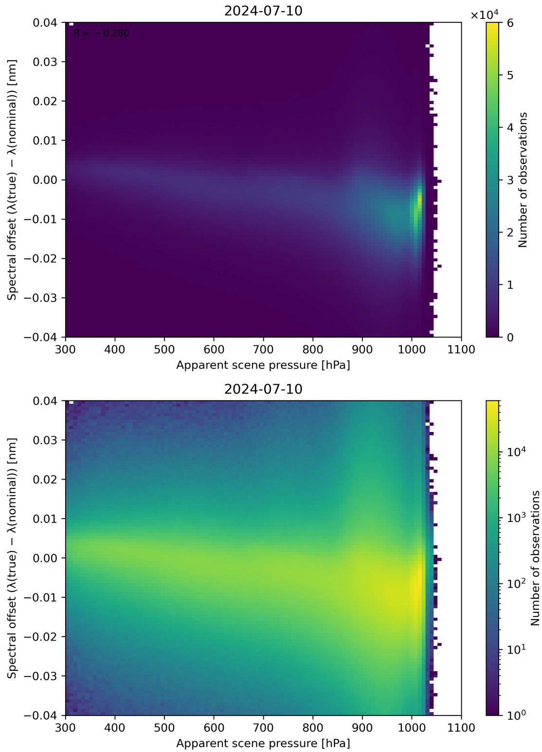
Figure 67: Scatter density plot of “Apparent scene pressure” against “Spectral offset ( \lambda(\text{true}) - \lambda(\text{nominal}) )” for 2024-07-10 to 2024-07-11.
