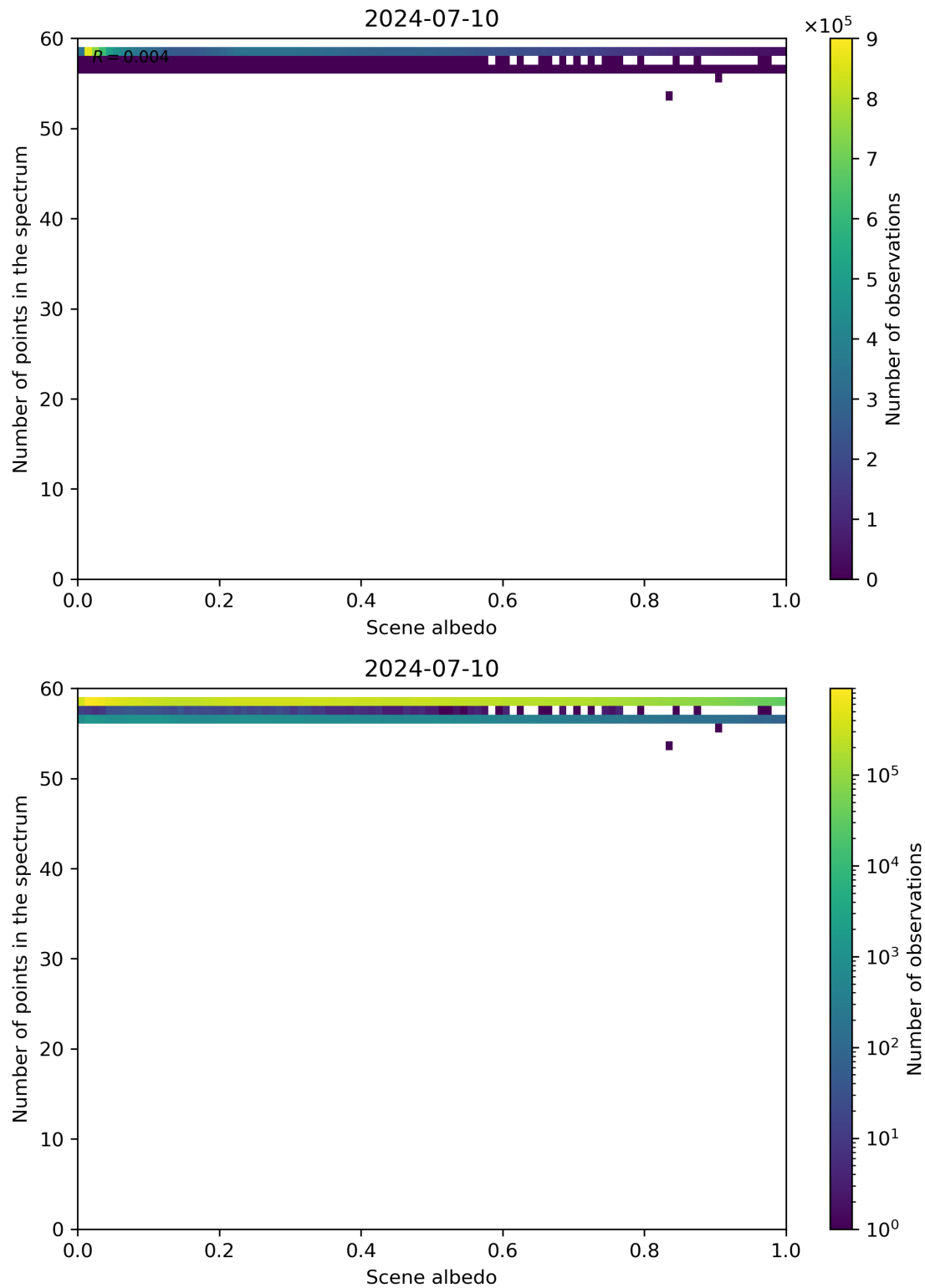
Figure 106: Scatter density plot of “Scene albedo” against “Number of points in the spectrum” for 2024-07-10 to 2024-07-11.
