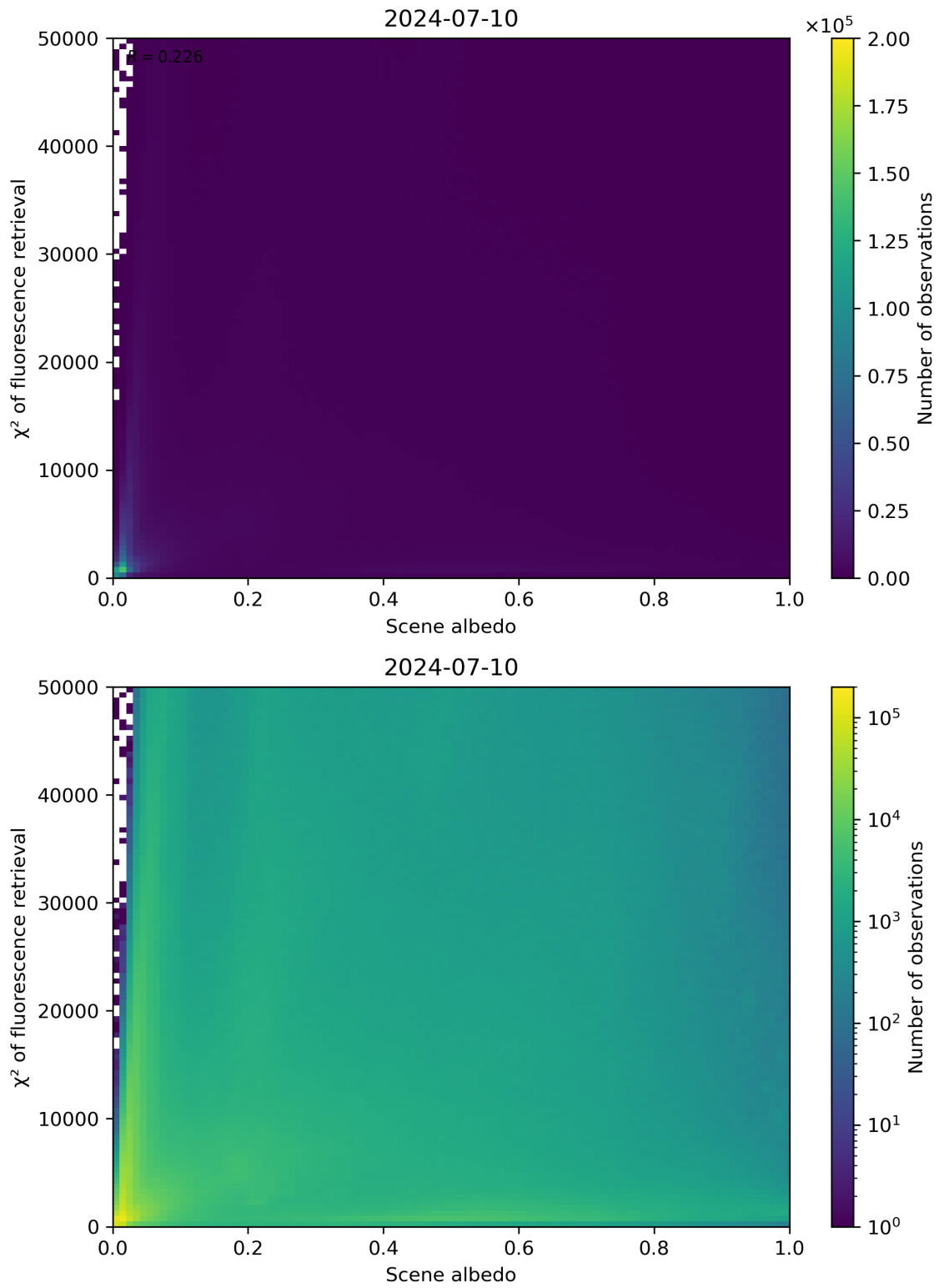
Figure 103: Scatter density plot of “Scene albedo” against “ \chi^2 of fluorescence retrieval” for 2024-07-10 to 2024-07-11.
