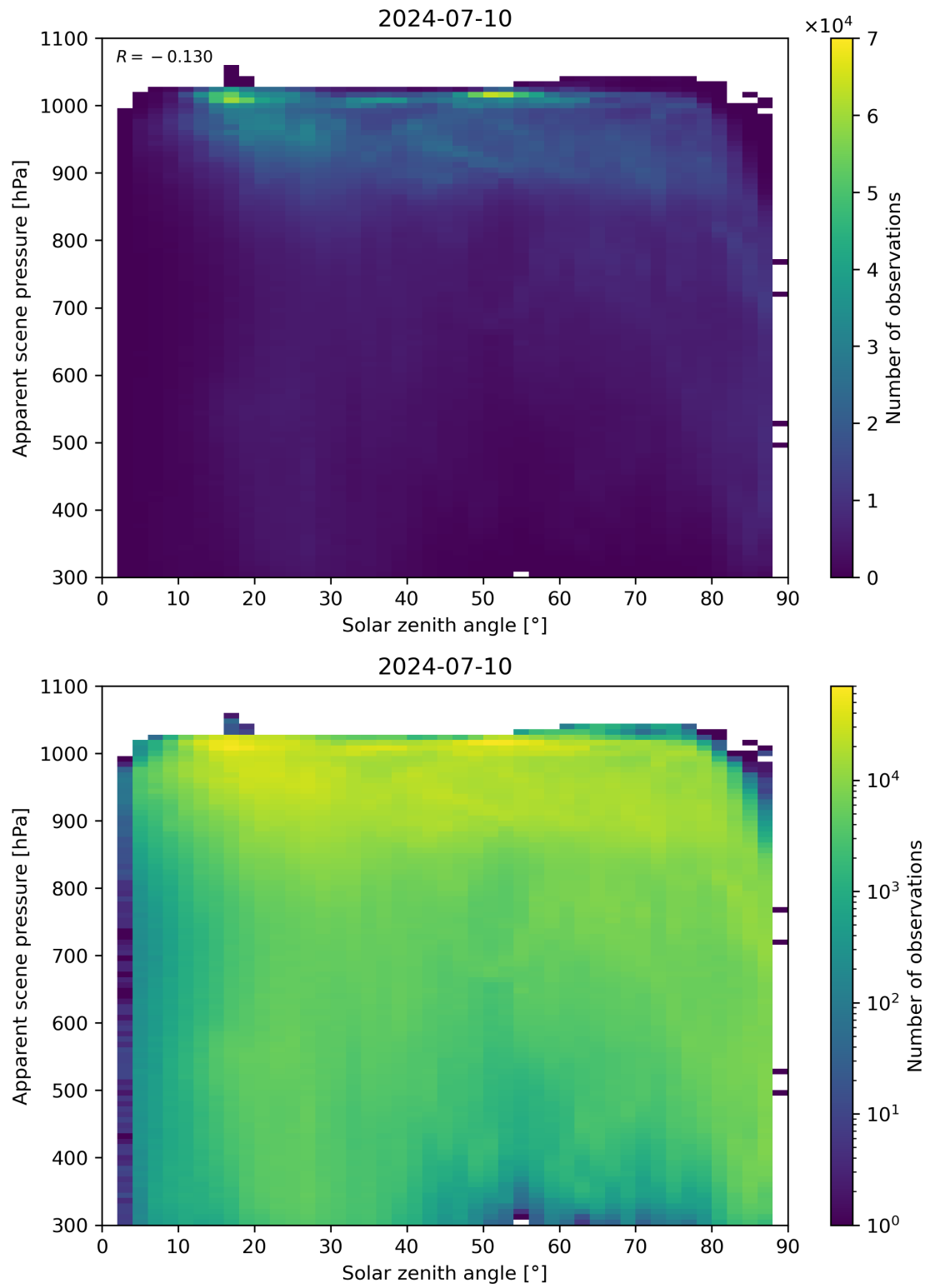
Figure 108: Scatter density plot of “Solar zenith angle” against “Apparent scene pressure” for 2024-07-10 to 2024-07-11.
