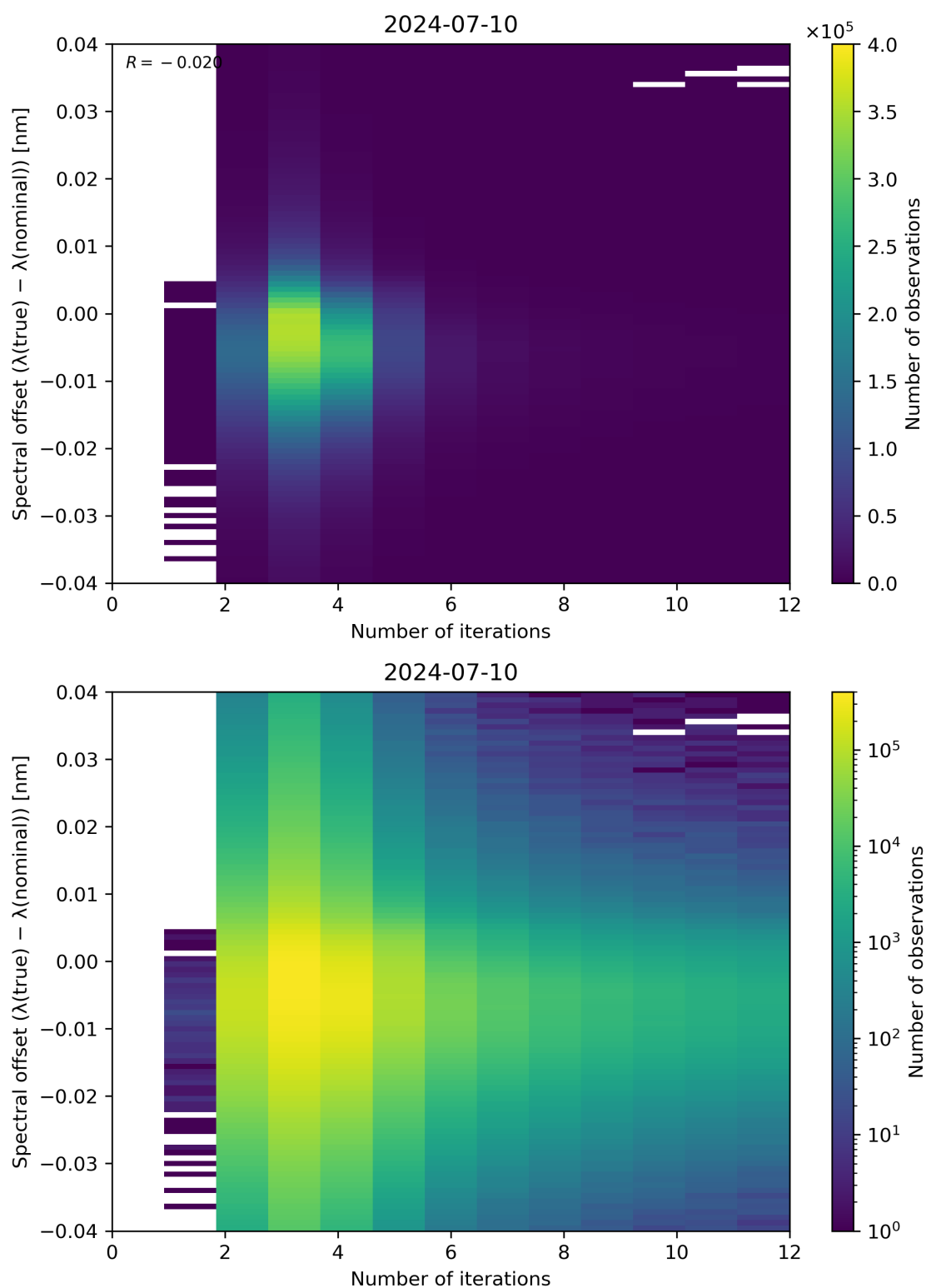
Figure 100: Scatter density plot of “Number of iterations” against “Spectral offset ( \lambda(\text{true}) - \lambda(\text{nominal}) )” for 2024-07-10 to 2024-07-11.
