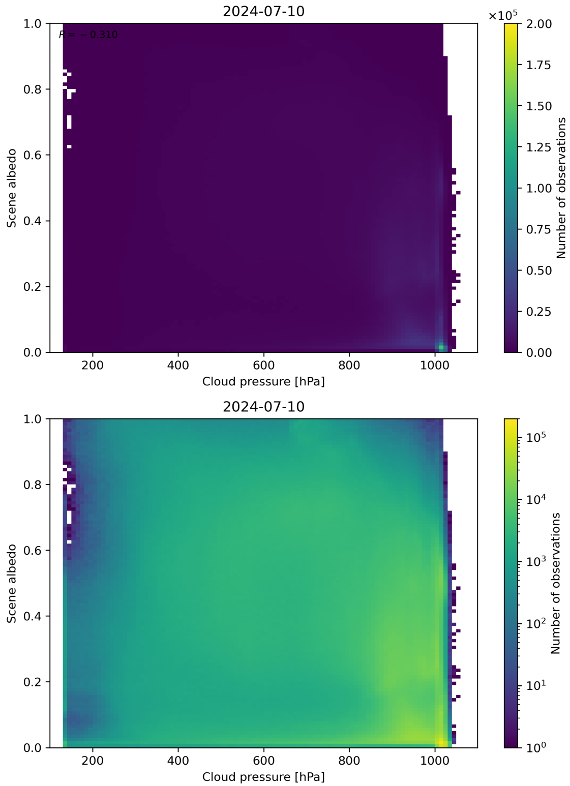
Figure 83: Scatter density plot of “Cloud pressure” against “Scene albedo” for 2024-07-10 to 2024-07-11.
