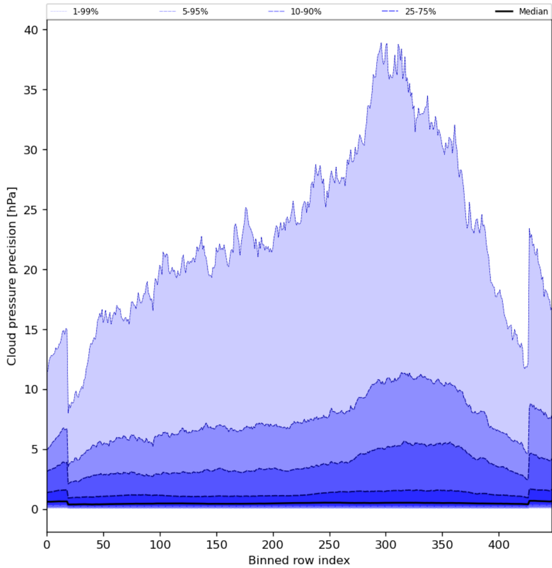
Figure 48: Along track statistics of “Cloud pressure precision” for 2024-07-10 to 2024-07-11
