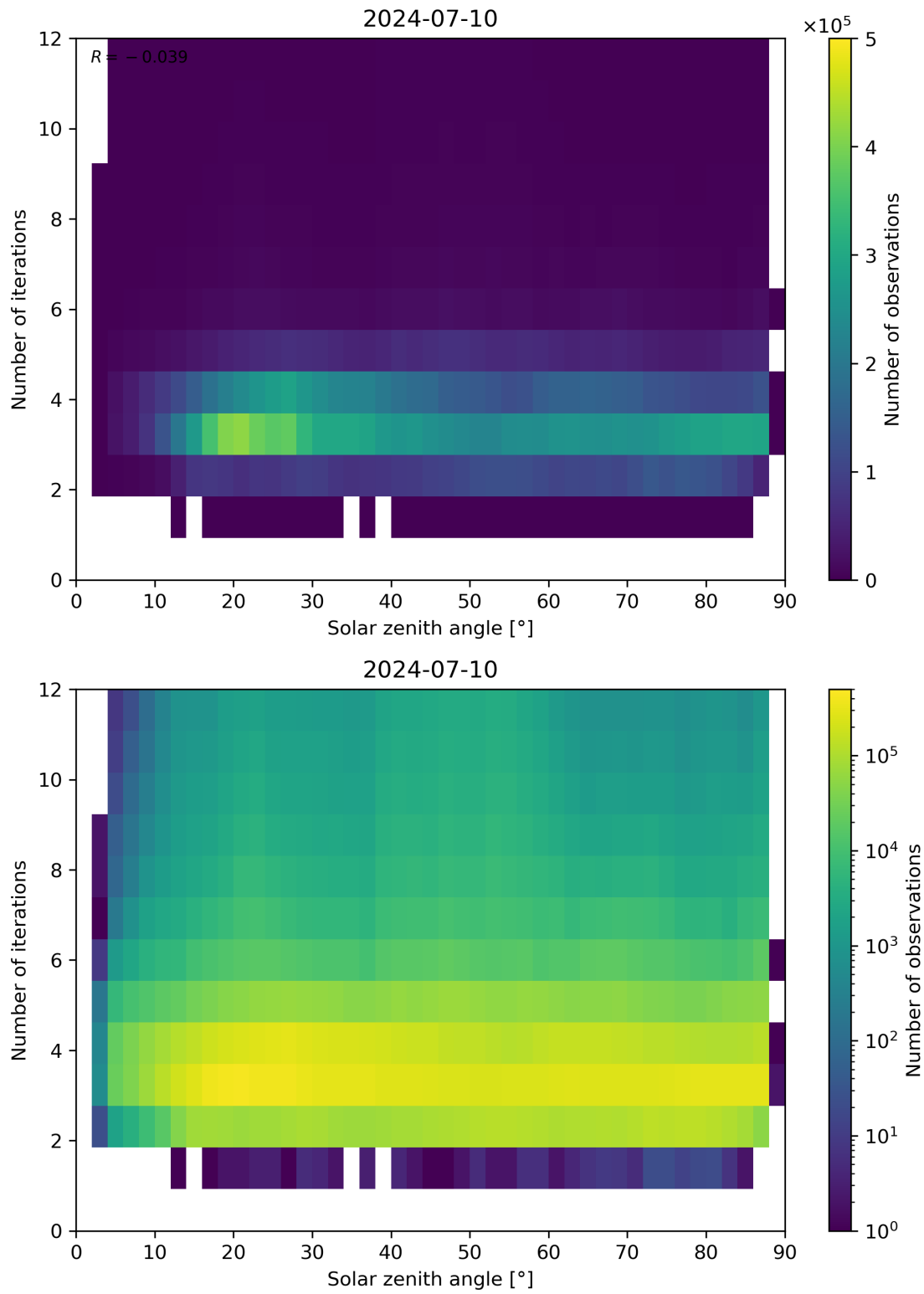
Figure 114: Scatter density plot of “Solar zenith angle” against “Number of iterations” for 2024-07-10 to 2024-07-11.
