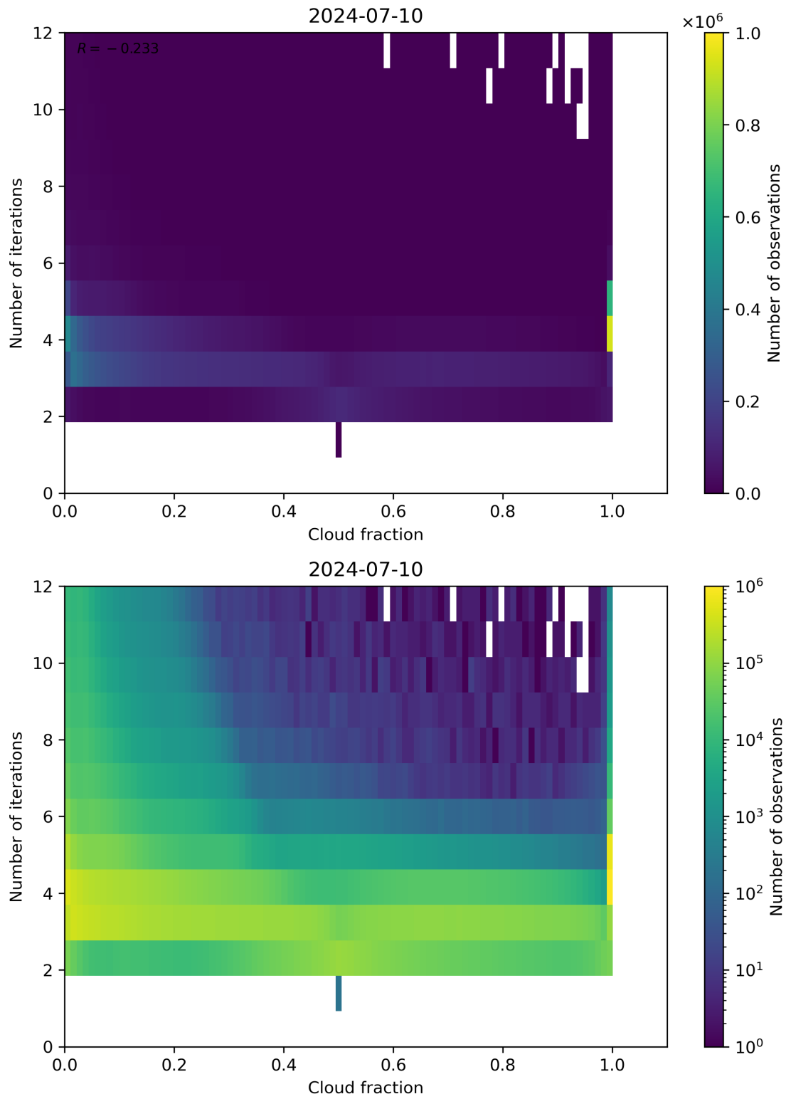
Figure 73: Scatter density plot of “Cloud fraction” against “Number of iterations” for 2024-07-10 to 2024-07-11.
