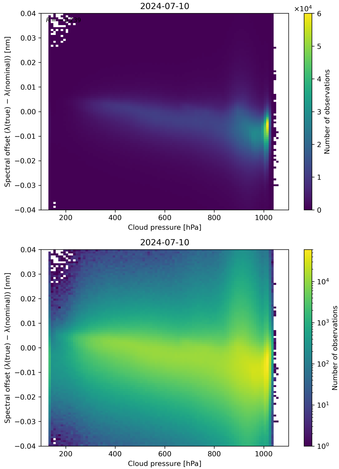
Figure 84: Scatter density plot of “Cloud pressure” against “Spectral offset ( \lambda(\text{true}) - \lambda(\text{nominal}) )” for 2024-07-10 to 2024-07-11.
