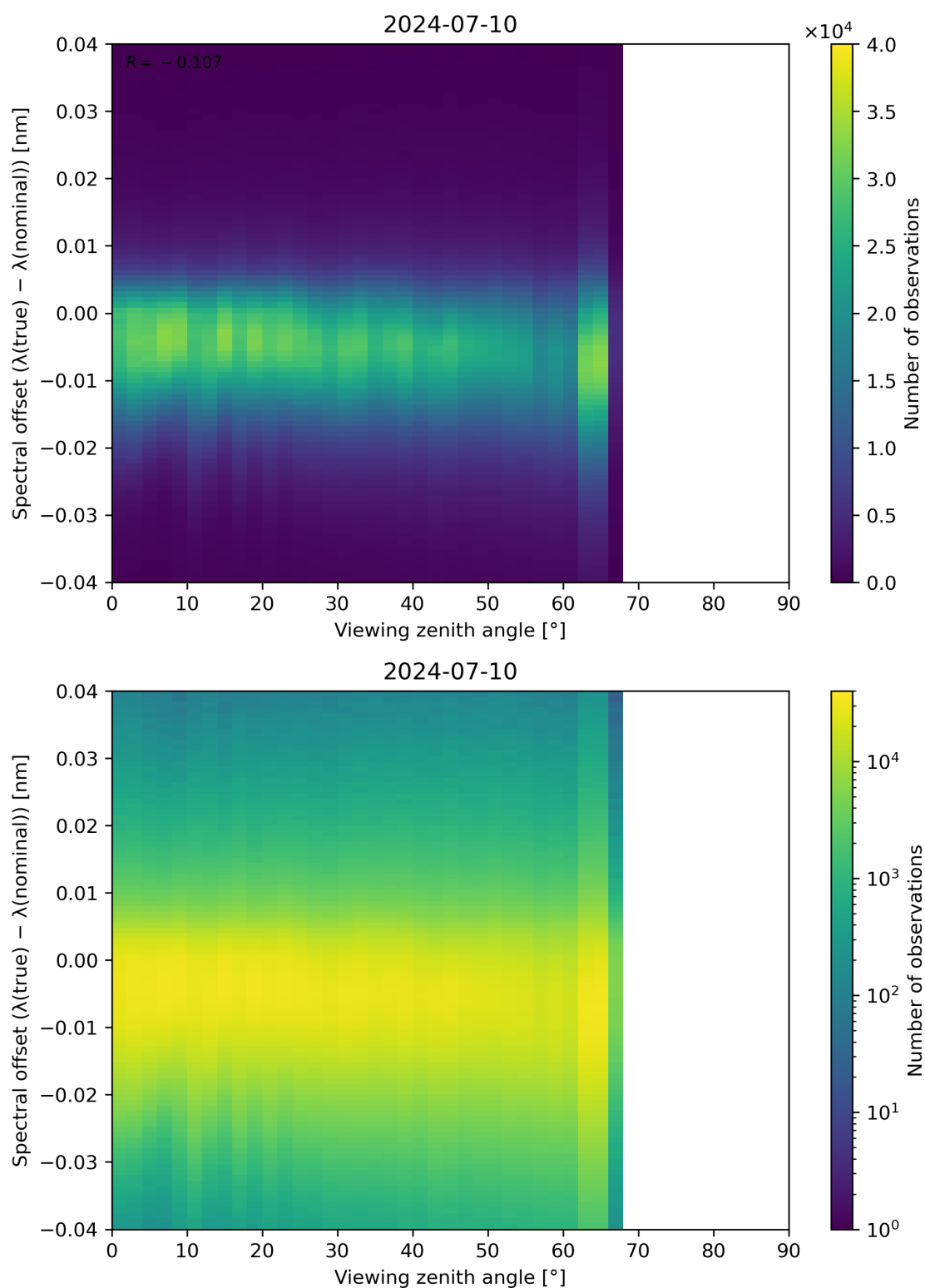
Figure 128: Scatter density plot of “Viewing zenith angle” against “Spectral offset ( \lambda(\text{true}) - \lambda(\text{nominal}) )” for 2024-07-10 to 2024-07-11.
