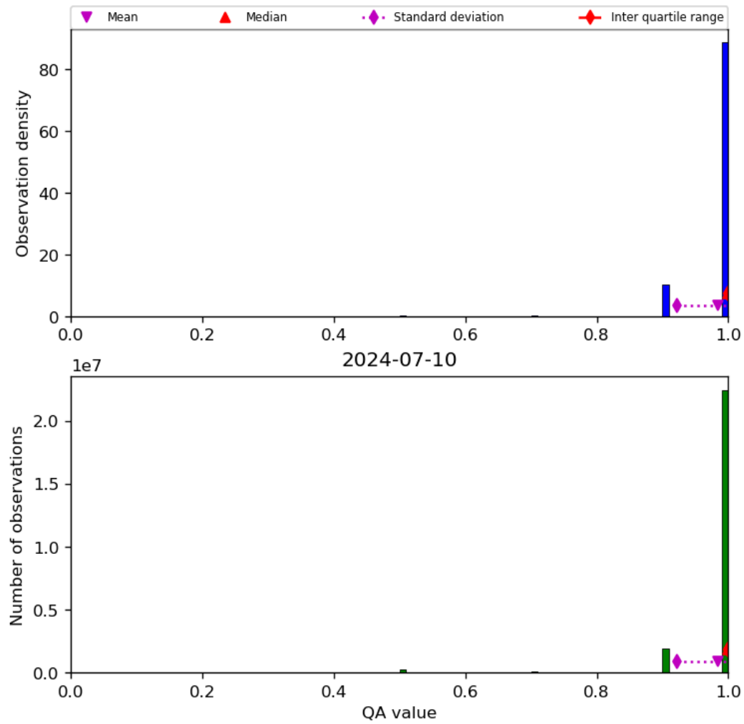
Figure 29: Histogram of “QA value” for 2024-07-10 to 2024-07-11
