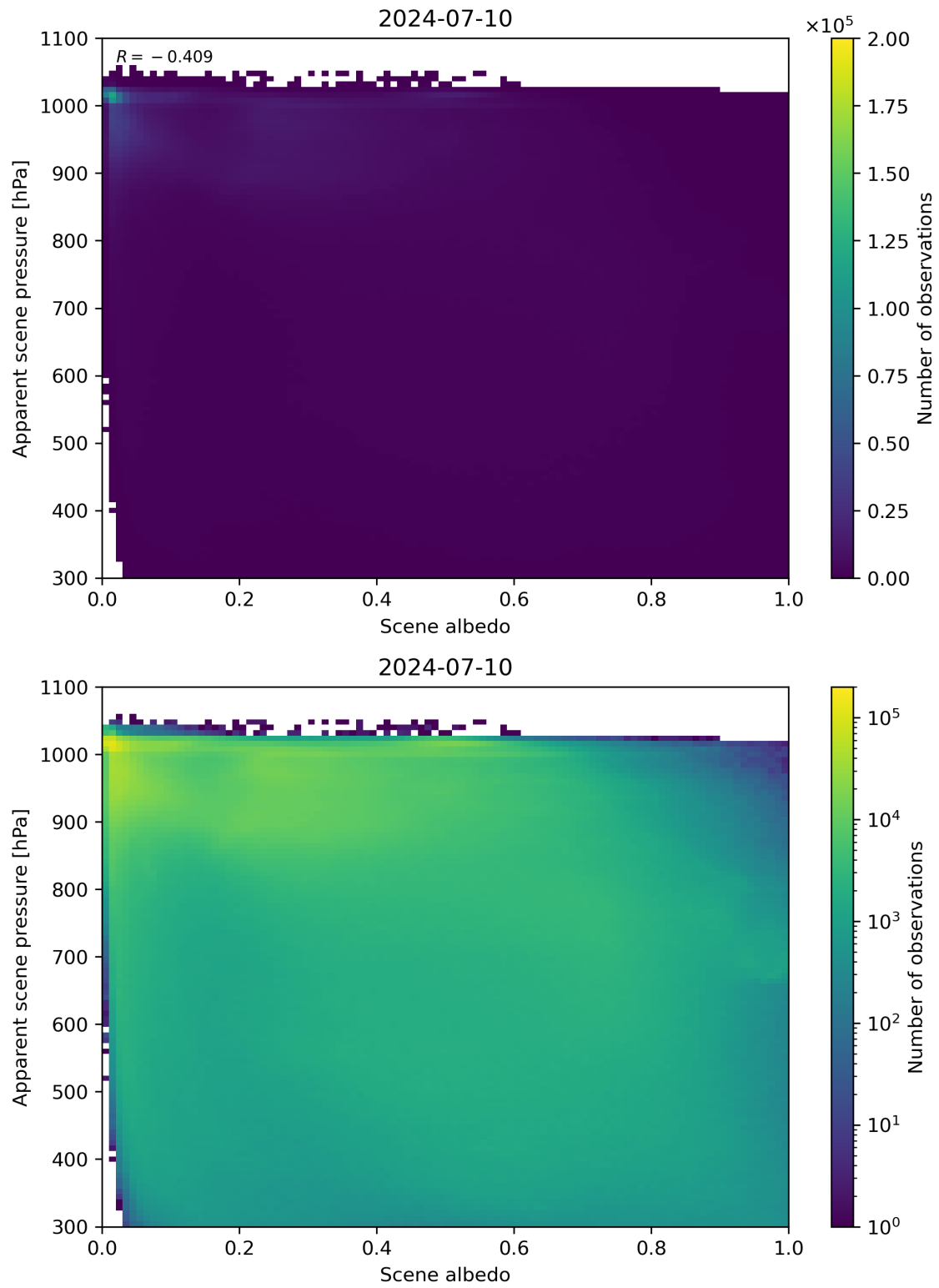
Figure 102: Scatter density plot of “Scene albedo” against “Apparent scene pressure” for 2024-07-10 to 2024-07-11.
