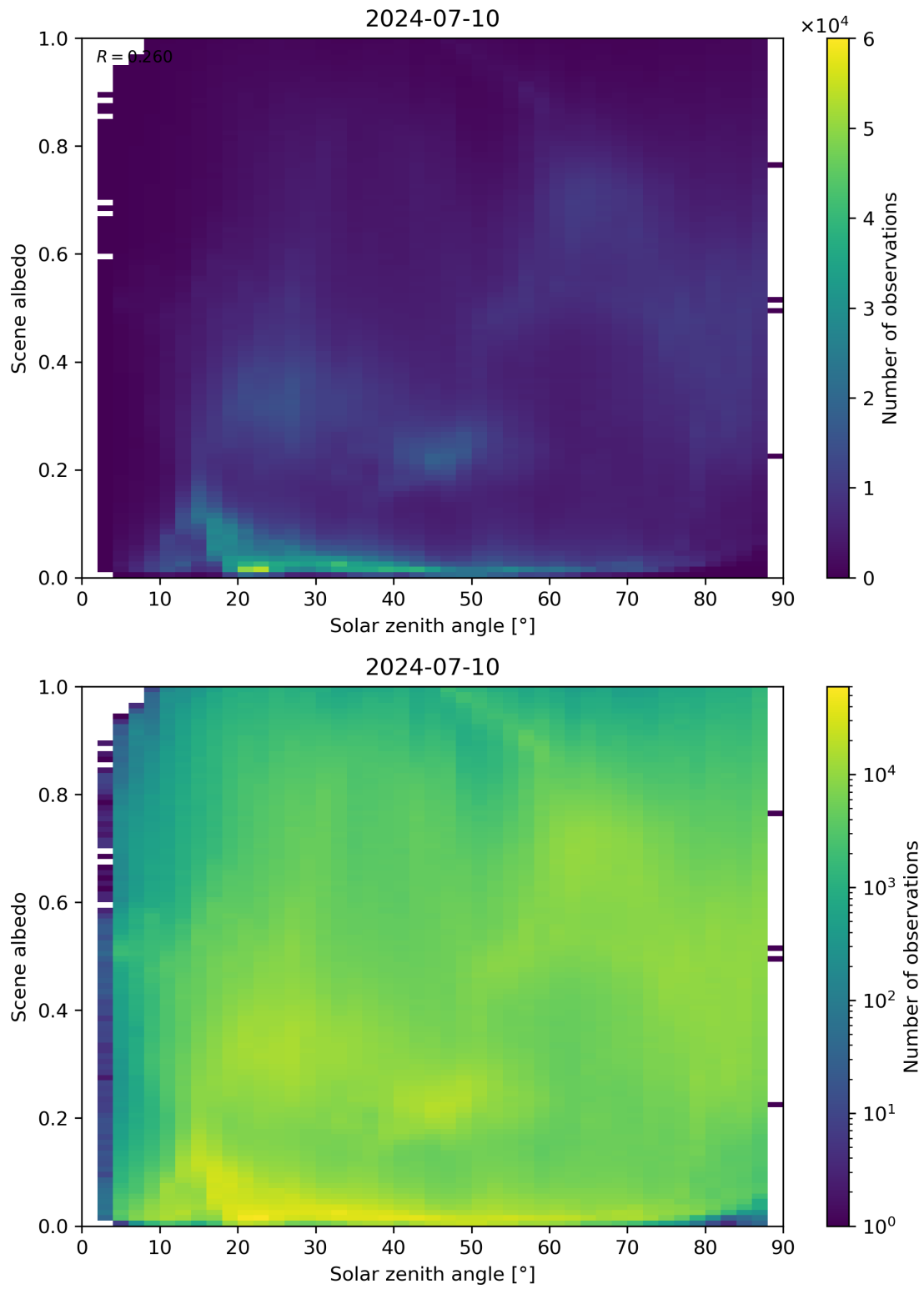
Figure 116: Scatter density plot of “Solar zenith angle” against “Scene albedo” for 2024-07-10 to 2024-07-11.
