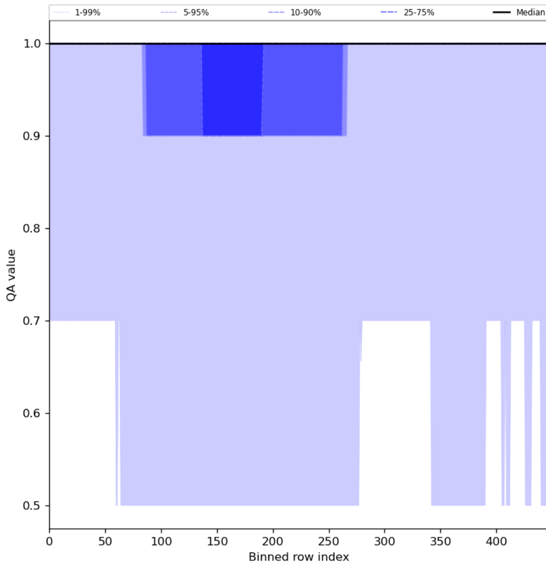
Figure 46: Along track statistics of “QA value” for 2024-07-10 to 2024-07-11
