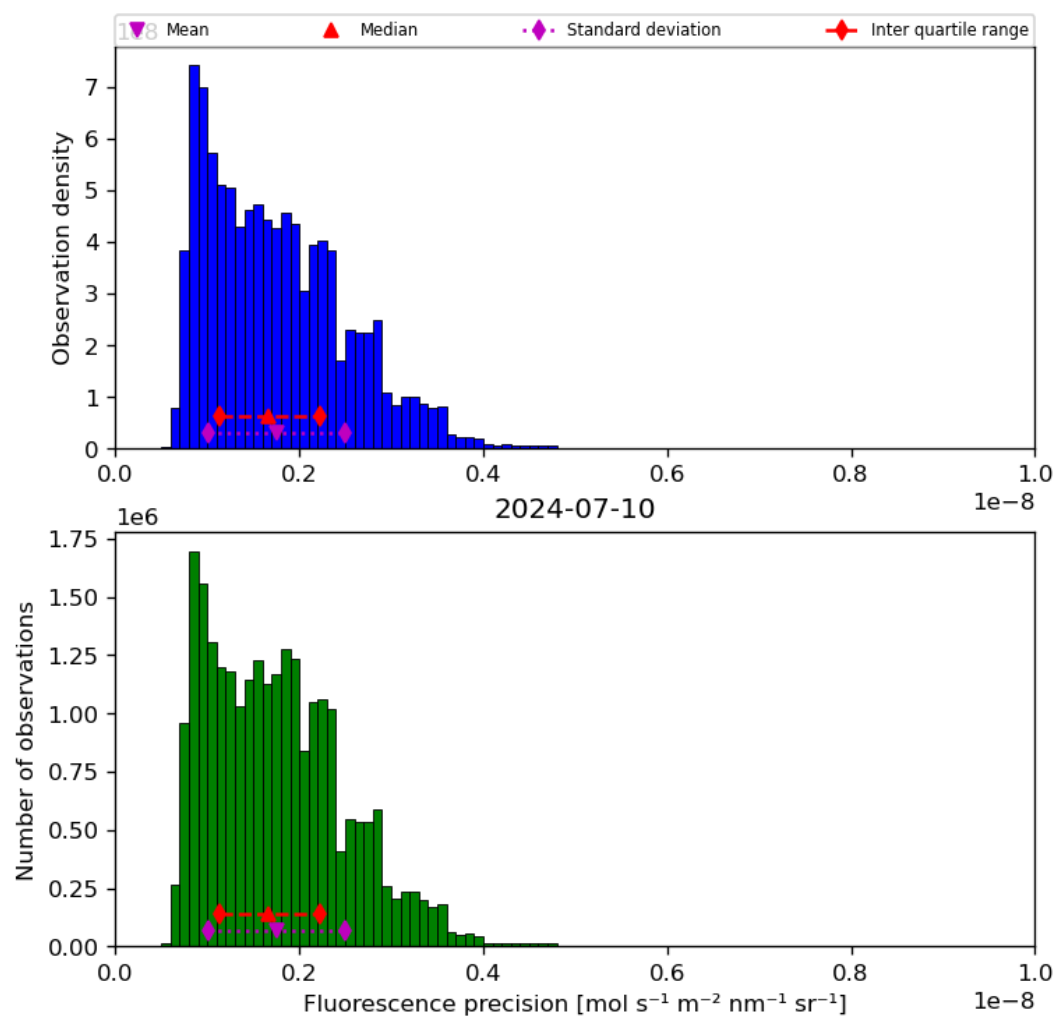
Figure 41: Histogram of “Fluorescence precision” for 2024-07-10 to 2024-07-11
