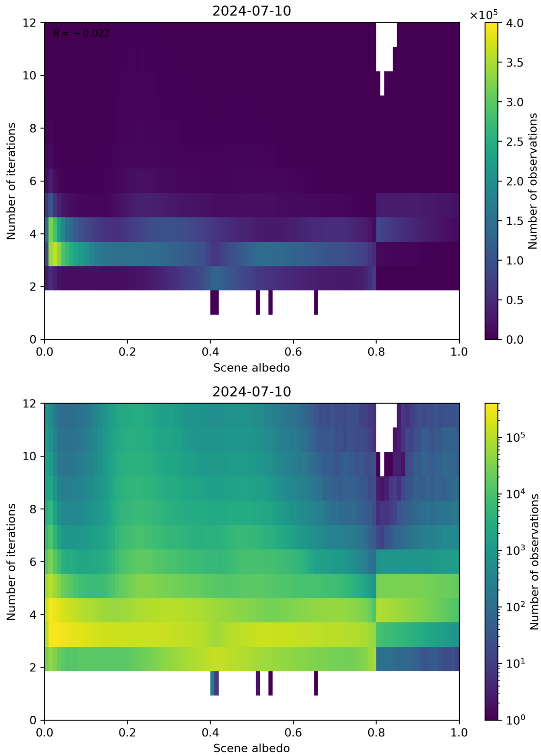
Figure 105: Scatter density plot of “Scene albedo” against “Number of iterations” for 2024-07-10 to 2024-07-11.
