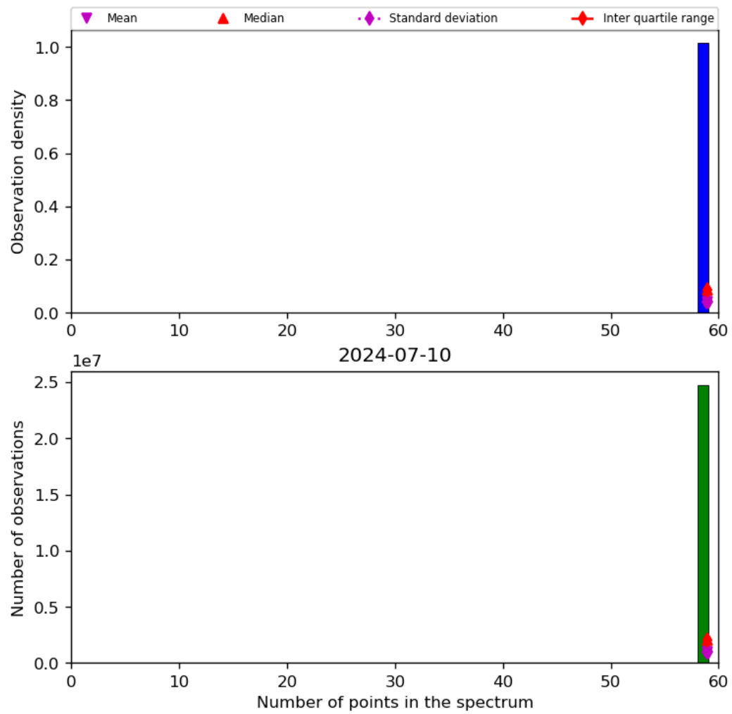
Figure 44: Histogram of “Number of points in the spectrum” for 2024-07-10 to 2024-07-11
