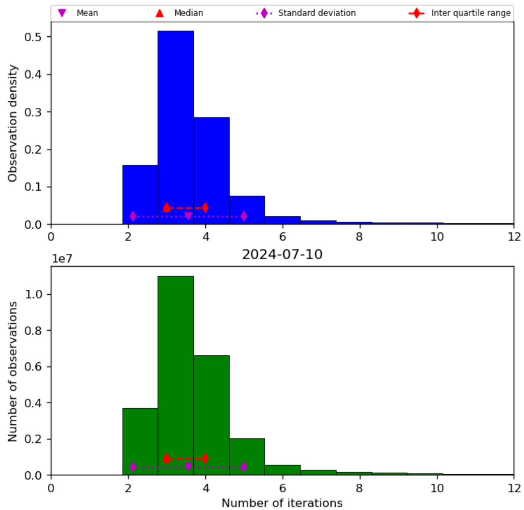
Figure 39: Histogram of “Number of iterations” for 2024-07-10 to 2024-07-11
