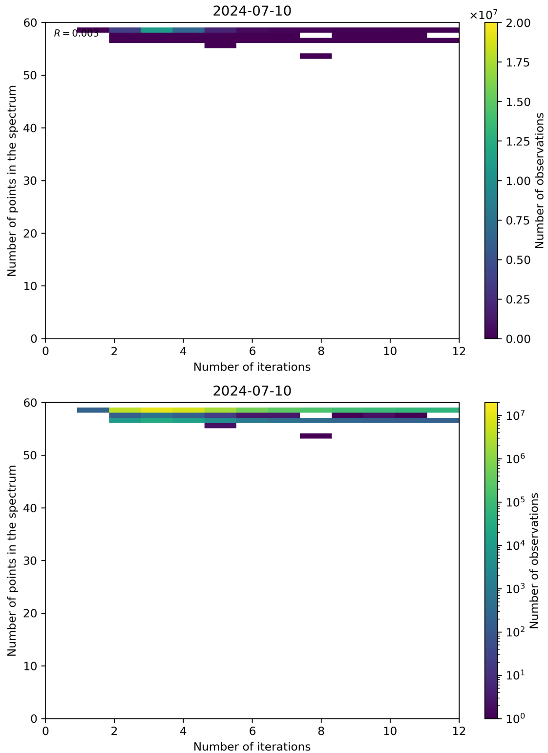
Figure 99: Scatter density plot of “Number of iterations” against “Number of points in the spectrum” for 2024-07-10 to 2024-07-11.
