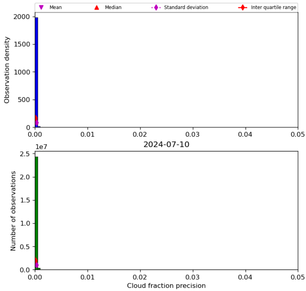
Figure 33: Histogram of “Cloud fraction precision” for 2024-07-10 to 2024-07-11
