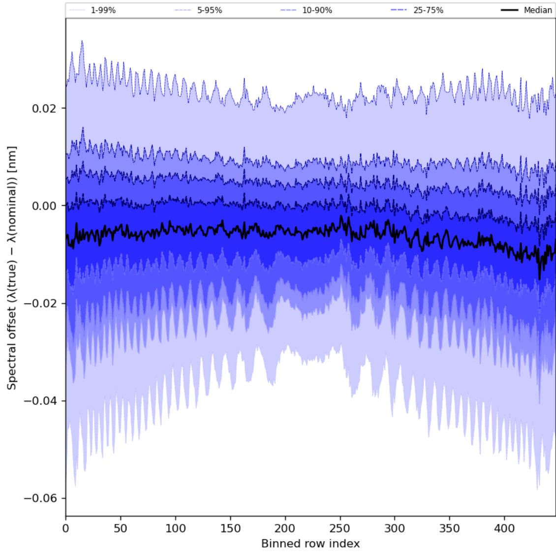
Figure 62: Along track statistics of “Spectral offset ( \lambda(\text{true}) - \lambda(\text{nominal}) )” for 2024-07-10 to 2024-07-11
