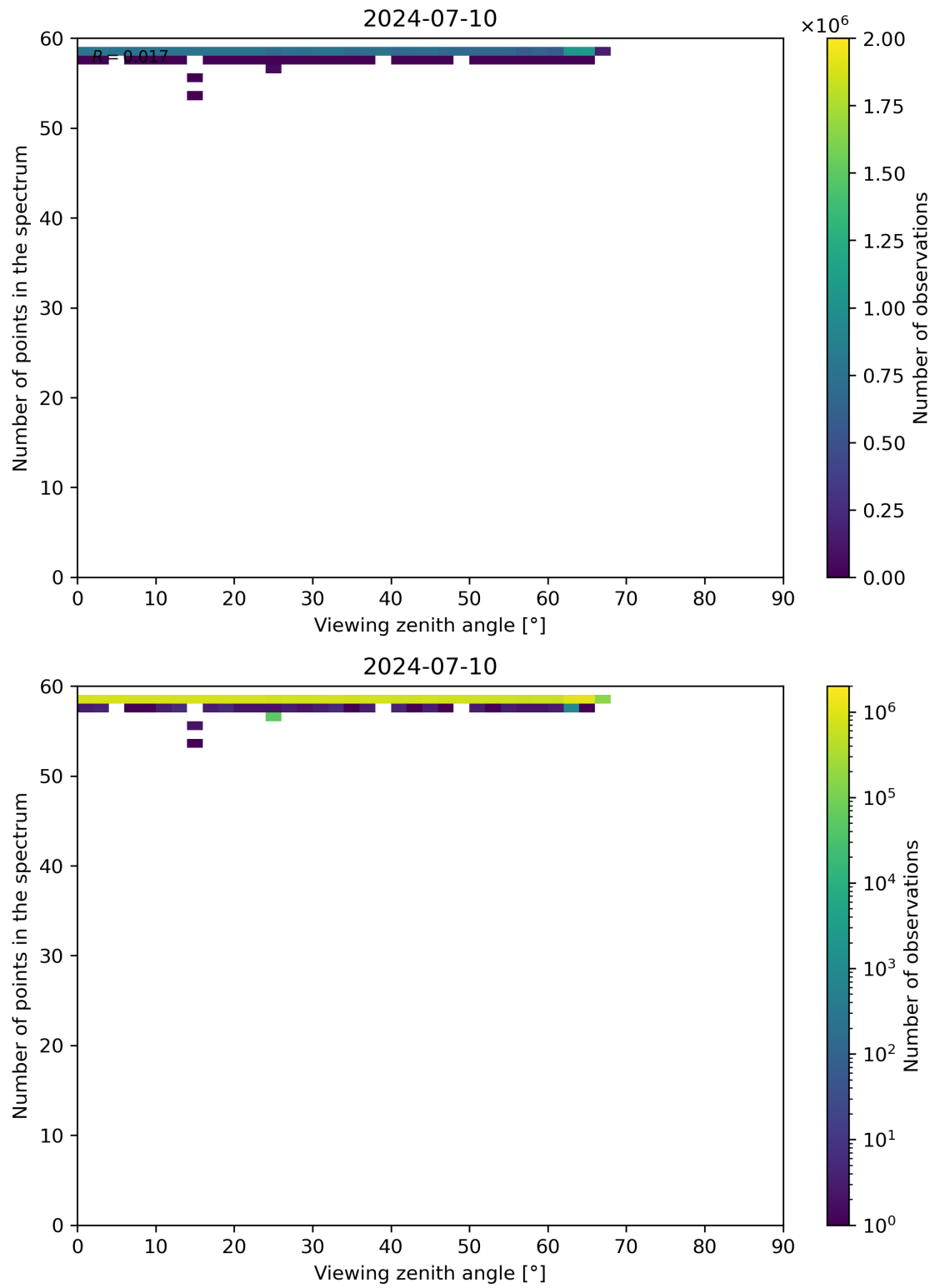
Figure 125: Scatter density plot of “Viewing zenith angle” against “Number of points in the spectrum” for 2024-07-10 to 2024-07-11.
