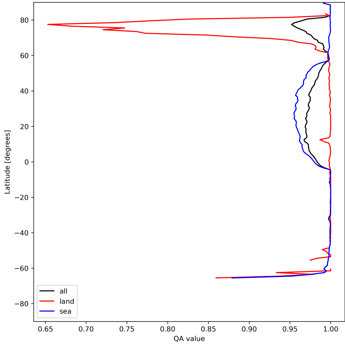
Figure 12: Zonal average of “QA value” for 2024-07-10 to 2024-07-11.
