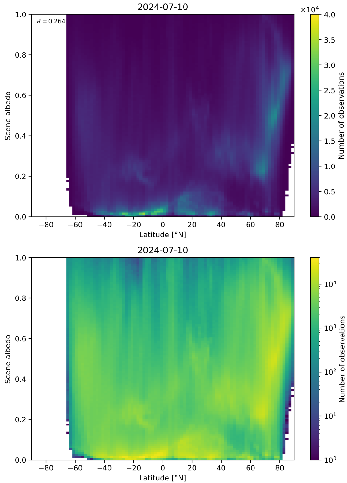
Figure 95: Scatter density plot of “Latitude” against “Scene albedo” for 2024-07-10 to 2024-07-11.
