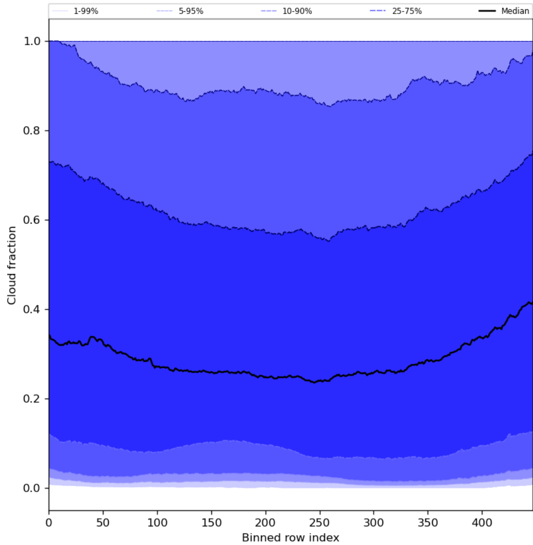
Figure 49: Along track statistics of “Cloud fraction” for 2024-07-10 to 2024-07-11
