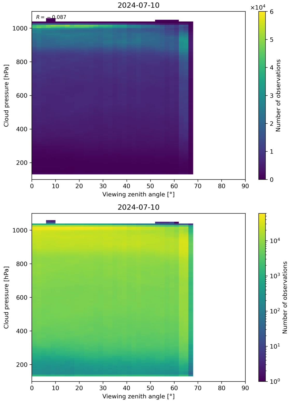
Figure 121: Scatter density plot of “Viewing zenith angle” against “Cloud pressure” for 2024-07-10 to 2024-07-11.
