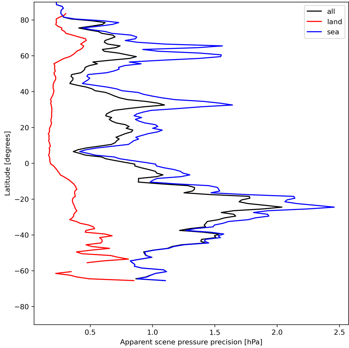
Figure 20: Zonal average of “Apparent scene pressure precision” for 2024-07-10 to 2024-07-11.
