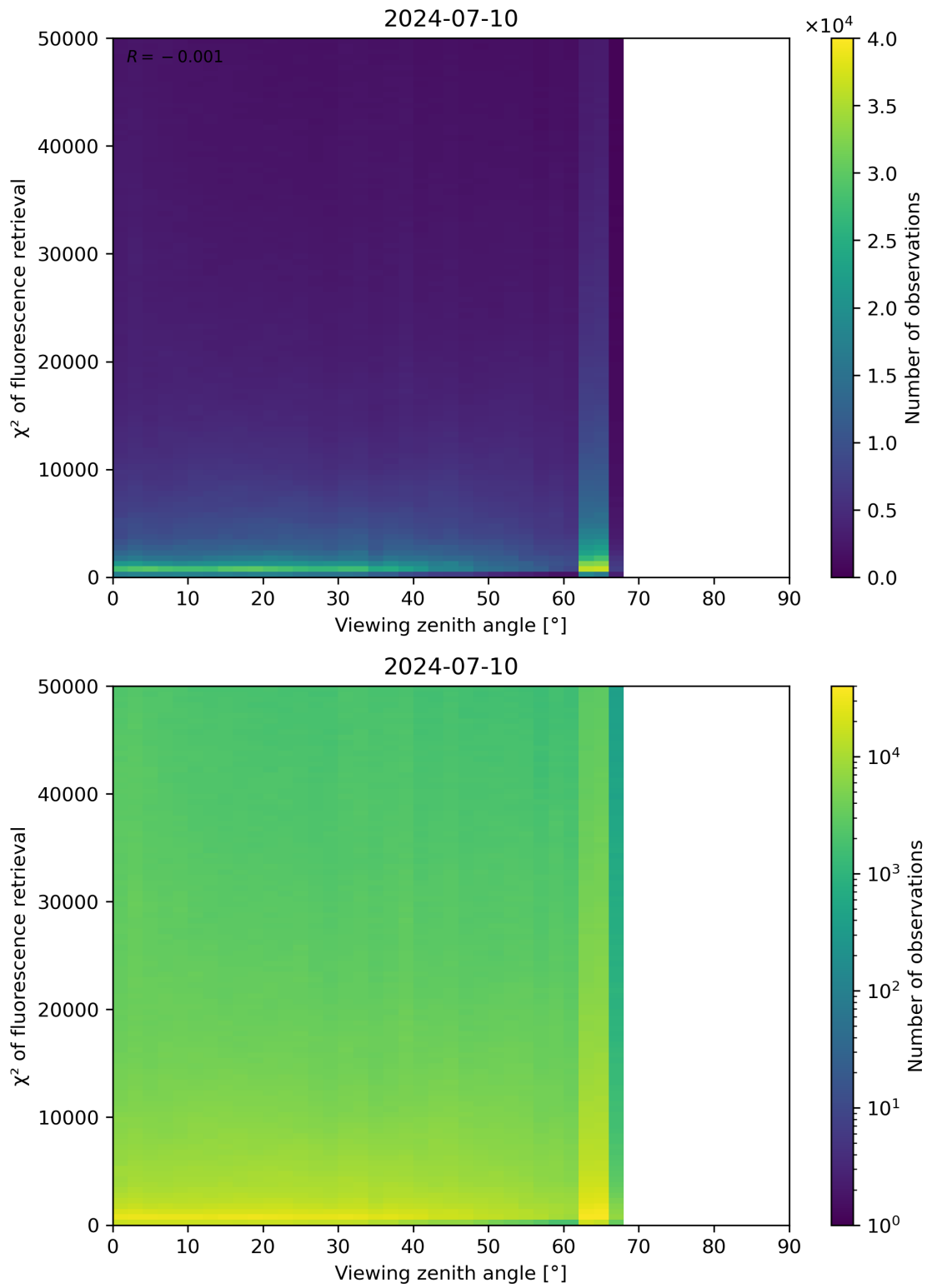
Figure 119: Scatter density plot of “Viewing zenith angle” against “ \chi^2 of fluorescence retrieval” for 2024-07-10 to 2024-07-11.
