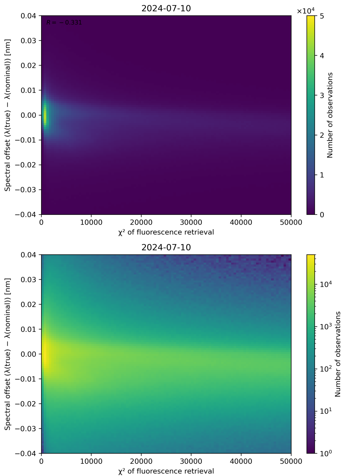
Figure 69: Scatter density plot of “ \chi^2 of fluorescence retrieval” against “Spectral offset ( \lambda(\text{true}) - \lambda(\text{nominal}) )” for 2024-07-10 to 2024-07-11.
