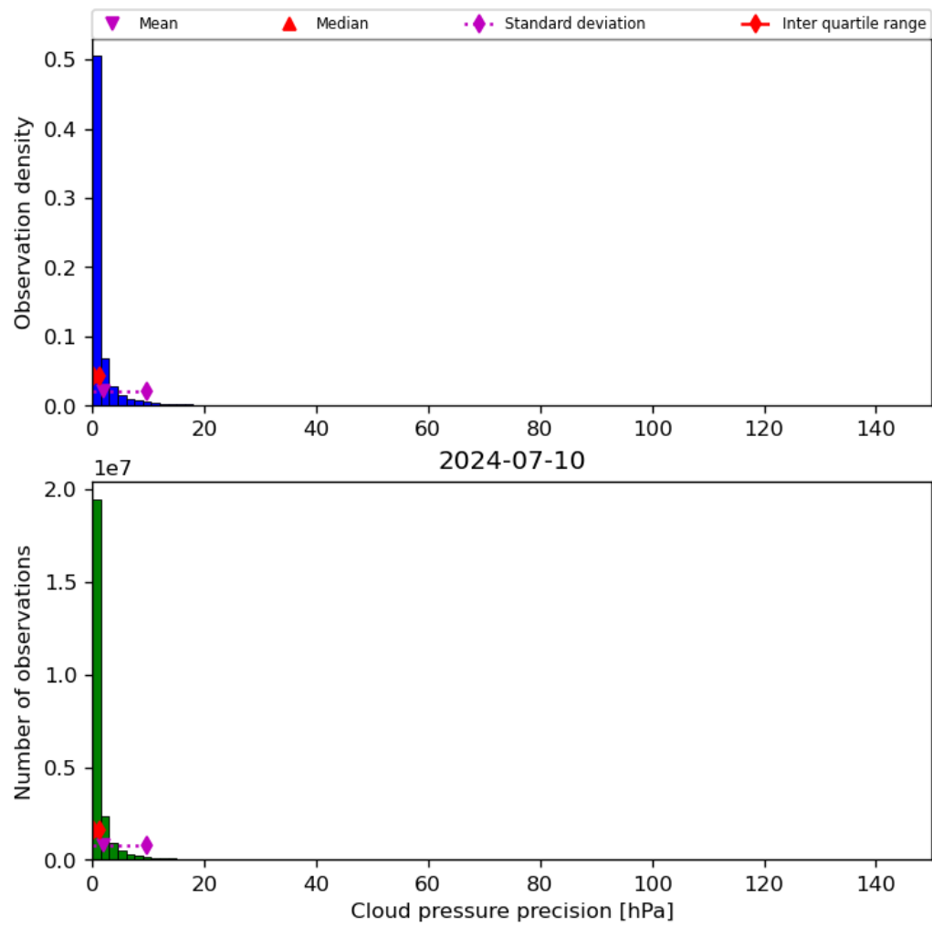
Figure 31: Histogram of “Cloud pressure precision” for 2024-07-10 to 2024-07-11
