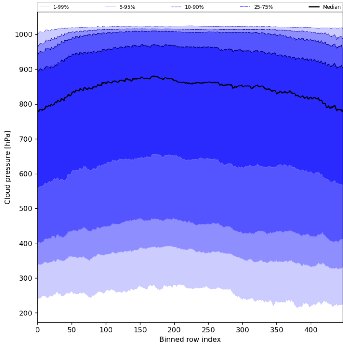
Figure 47: Along track statistics of “Cloud pressure” for 2024-07-10 to 2024-07-11
