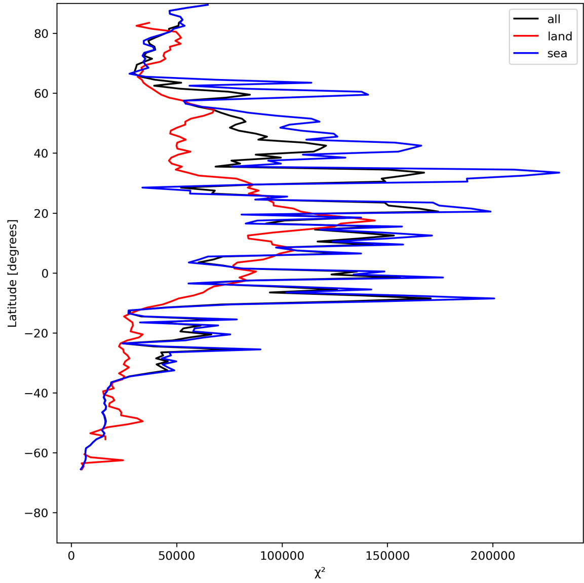
Figure 21: Zonal average of “ \chi^2 ” for 2024-07-10 to 2024-07-11.
