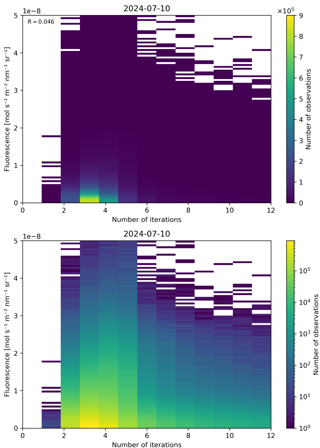
Figure 98: Scatter density plot of “Number of iterations” against “Fluorescence” for 2024-07-10 to 2024-07-11.
