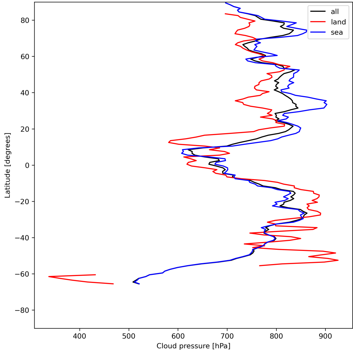
Figure 13: Zonal average of “Cloud pressure” for 2024-07-10 to 2024-07-11.
