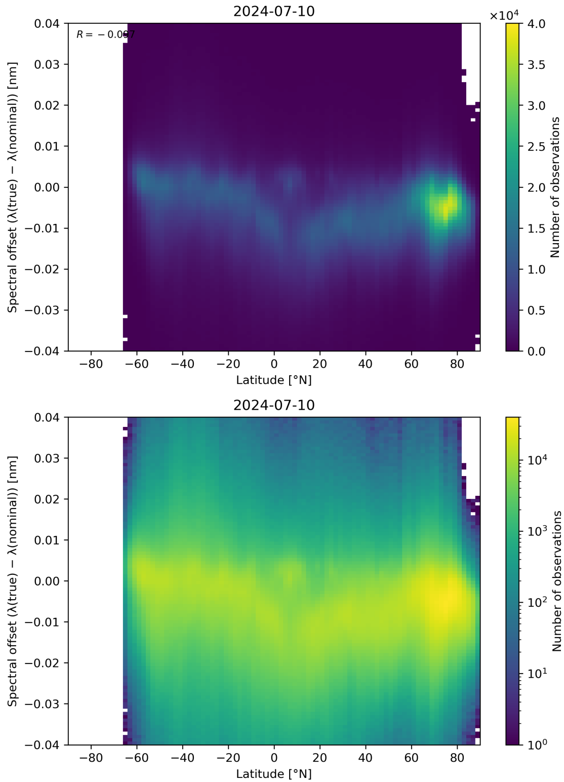
Figure 96: Scatter density plot of “Latitude” against “Spectral offset ( \lambda(\text{true}) - \lambda(\text{nominal}) )” for 2024-07-10 to 2024-07-11.
