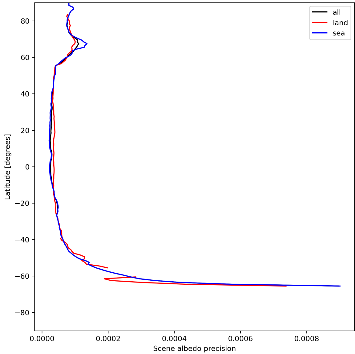
Figure 18: Zonal average of “Scene albedo precision” for 2024-07-10 to 2024-07-11.
