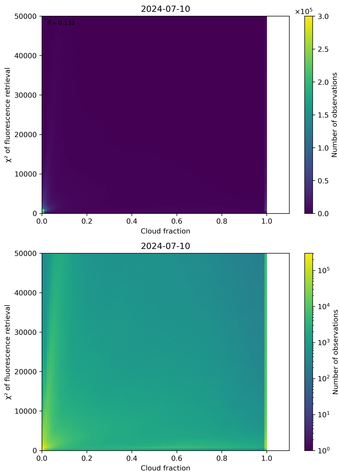
Figure 71: Scatter density plot of “Cloud fraction” against “ \chi^2 of fluorescence retrieval” for 2024-07-10 to 2024-07-11.
