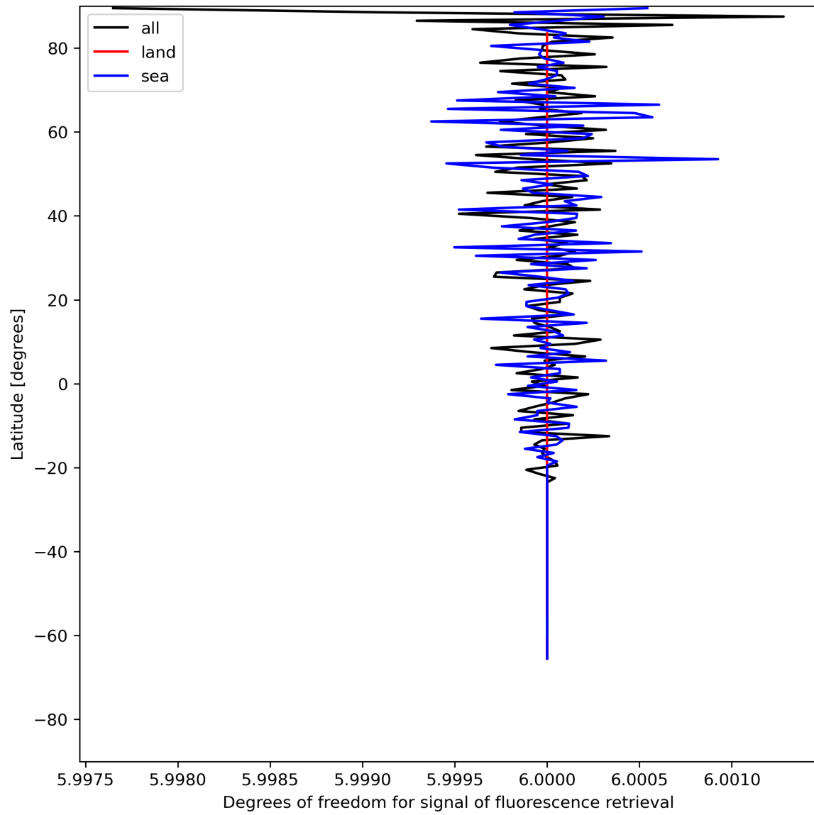
Figure 26: Zonal average of “Degrees of freedom for signal of fluorescence retrieval” for 2024-07-10 to 2024-07-11.
