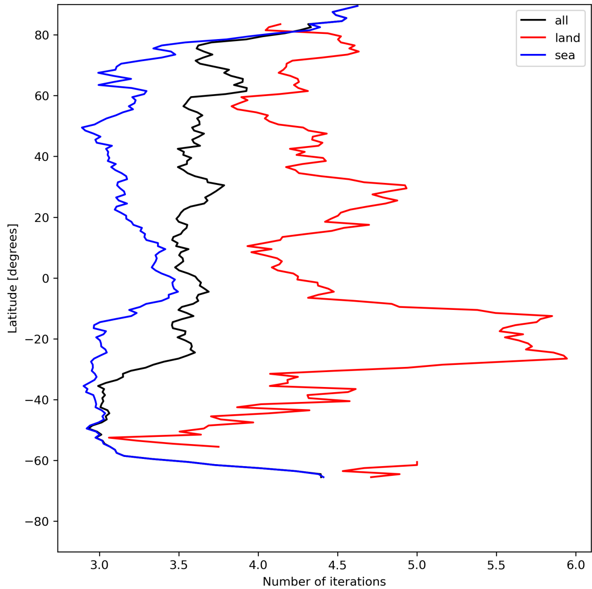
Figure 22: Zonal average of “Number of iterations” for 2024-07-10 to 2024-07-11.
