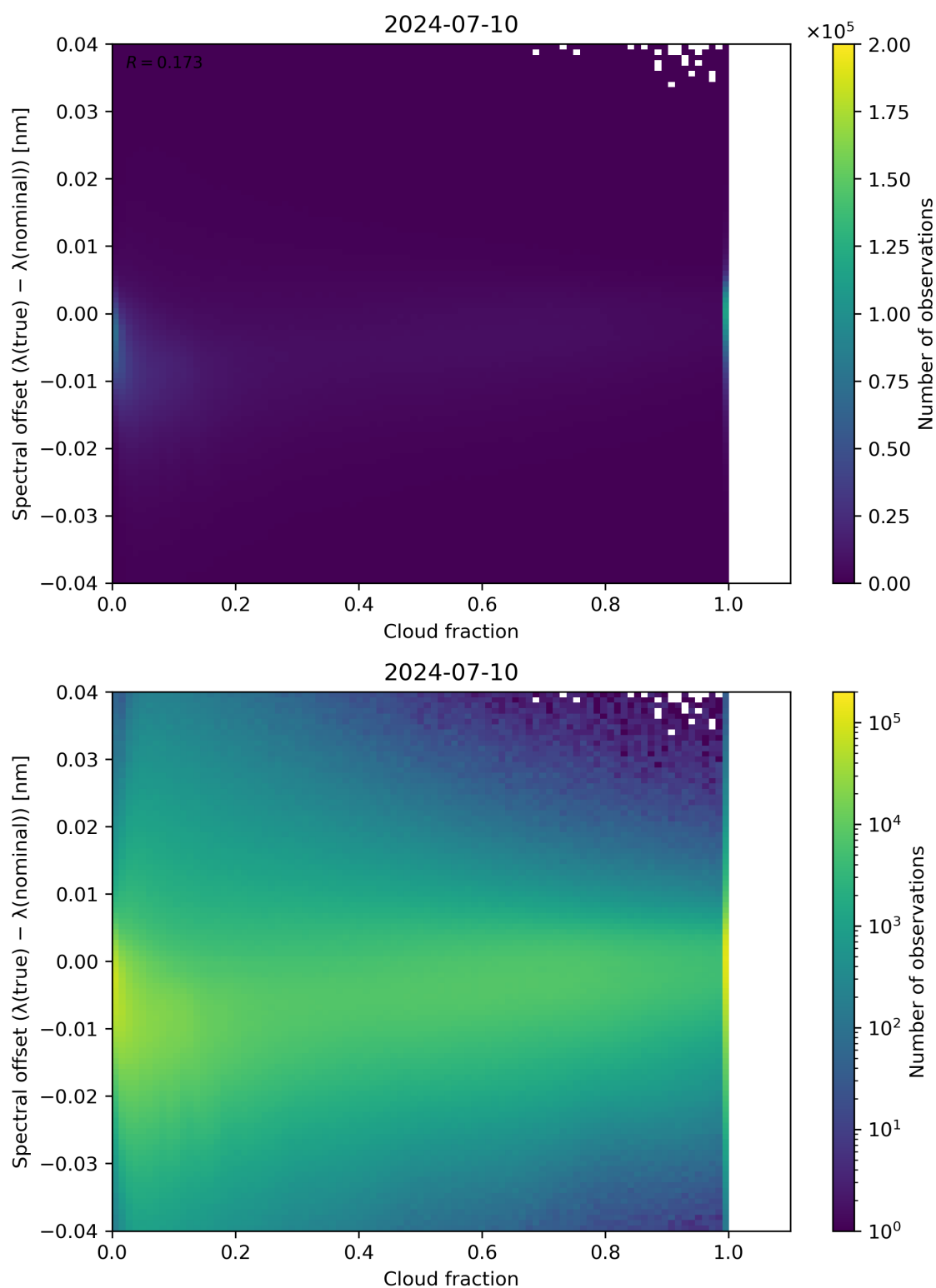
Figure 76: Scatter density plot of “Cloud fraction” against “Spectral offset ( \lambda(\text{true}) - \lambda(\text{nominal}) )” for 2024-07-10 to 2024-07-11.
