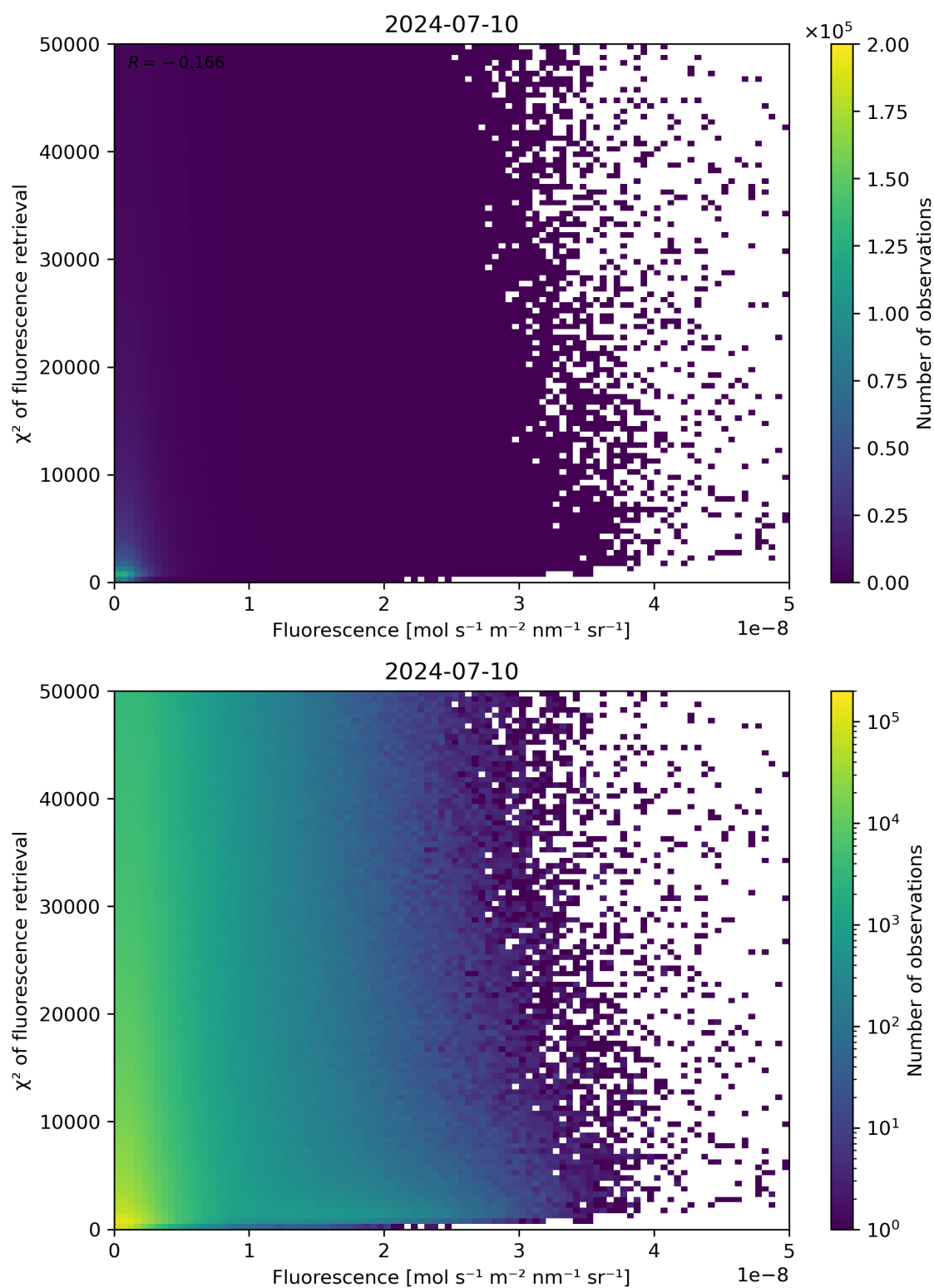
Figure 85: Scatter density plot of “Fluorescence” against “ \chi^2 of fluorescence retrieval” for 2024-07-10 to 2024-07-11.
