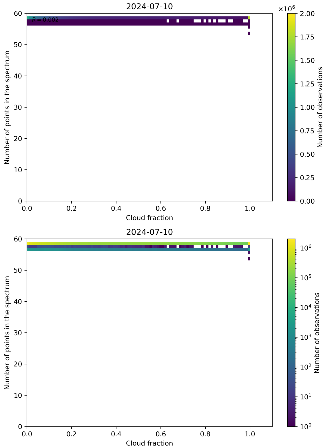
Figure 74: Scatter density plot of “Cloud fraction” against “Number of points in the spectrum” for 2024-07-10 to 2024-07-11.
