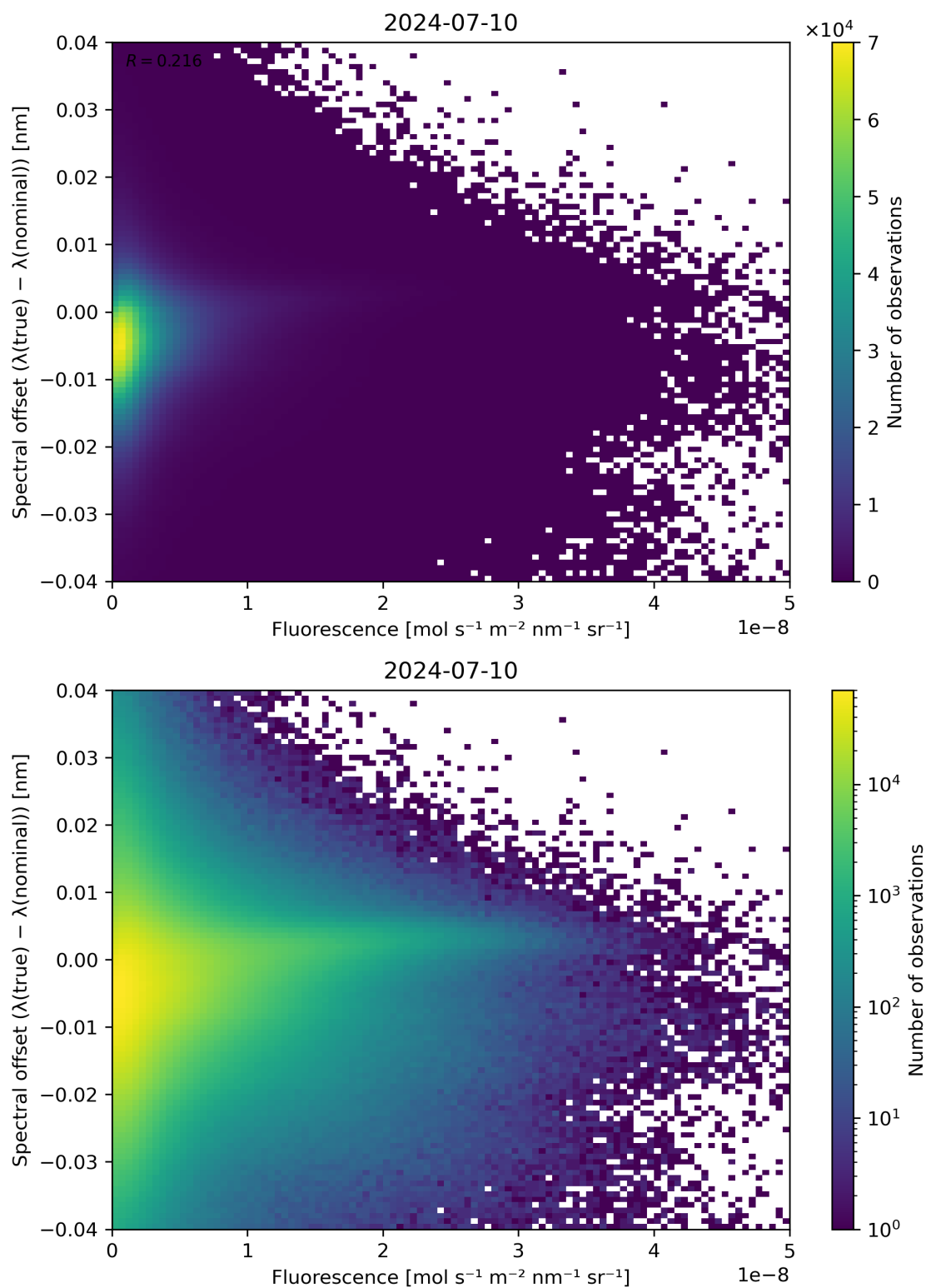
Figure 87: Scatter density plot of “Fluorescence” against “Spectral offset ( \lambda(\text{true}) - \lambda(\text{nominal}) )” for 2024-07-10 to 2024-07-11.
