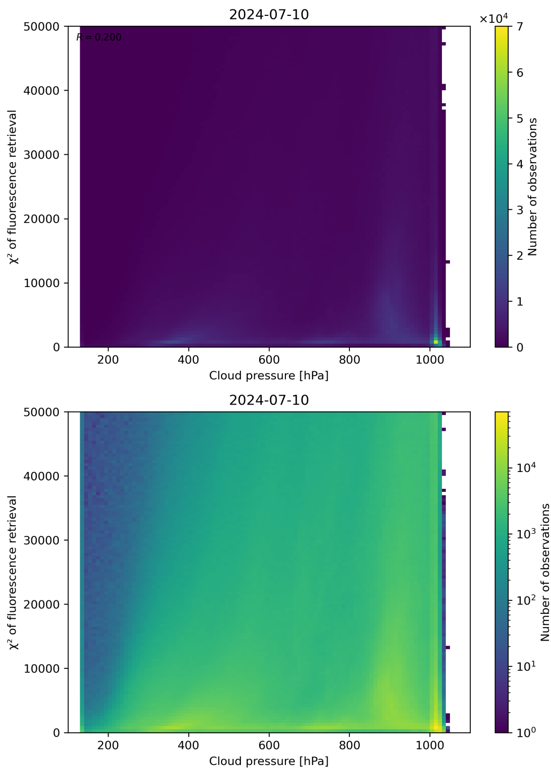
Figure 78: Scatter density plot of “Cloud pressure” against “ \chi^2 of fluorescence retrieval” for 2024-07-10 to 2024-07-11.
