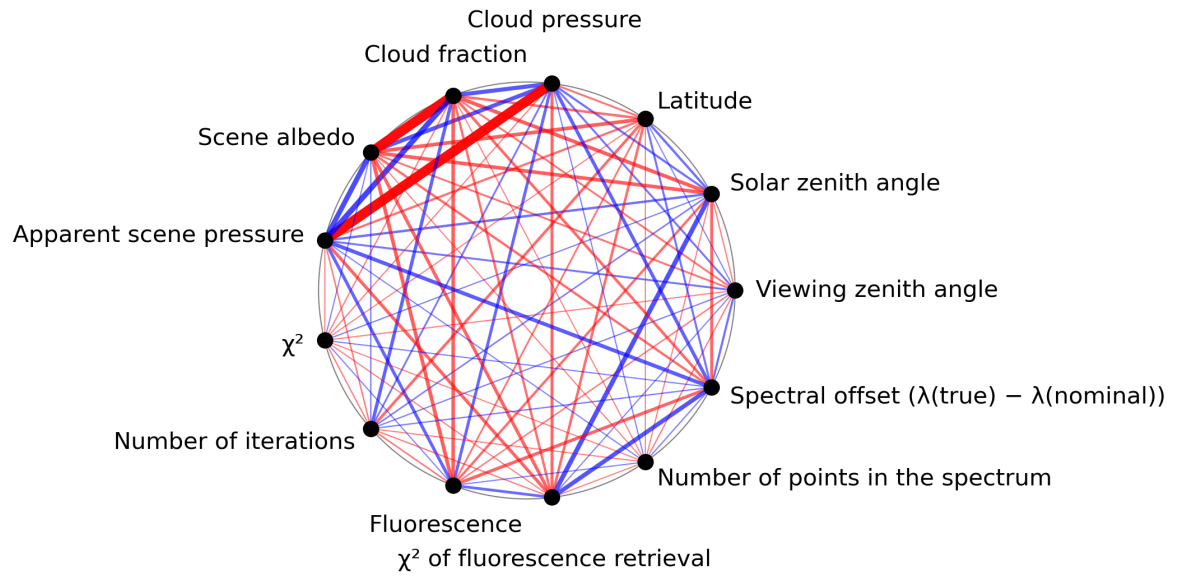
Figure 1: Map of correlation graph for 2024-07-10 to 2024-07-11.
