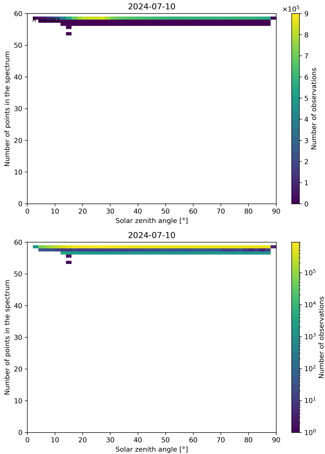
Figure 115: Scatter density plot of “Solar zenith angle” against “Number of points in the spectrum” for 2024-07-10 to 2024-07-11.
