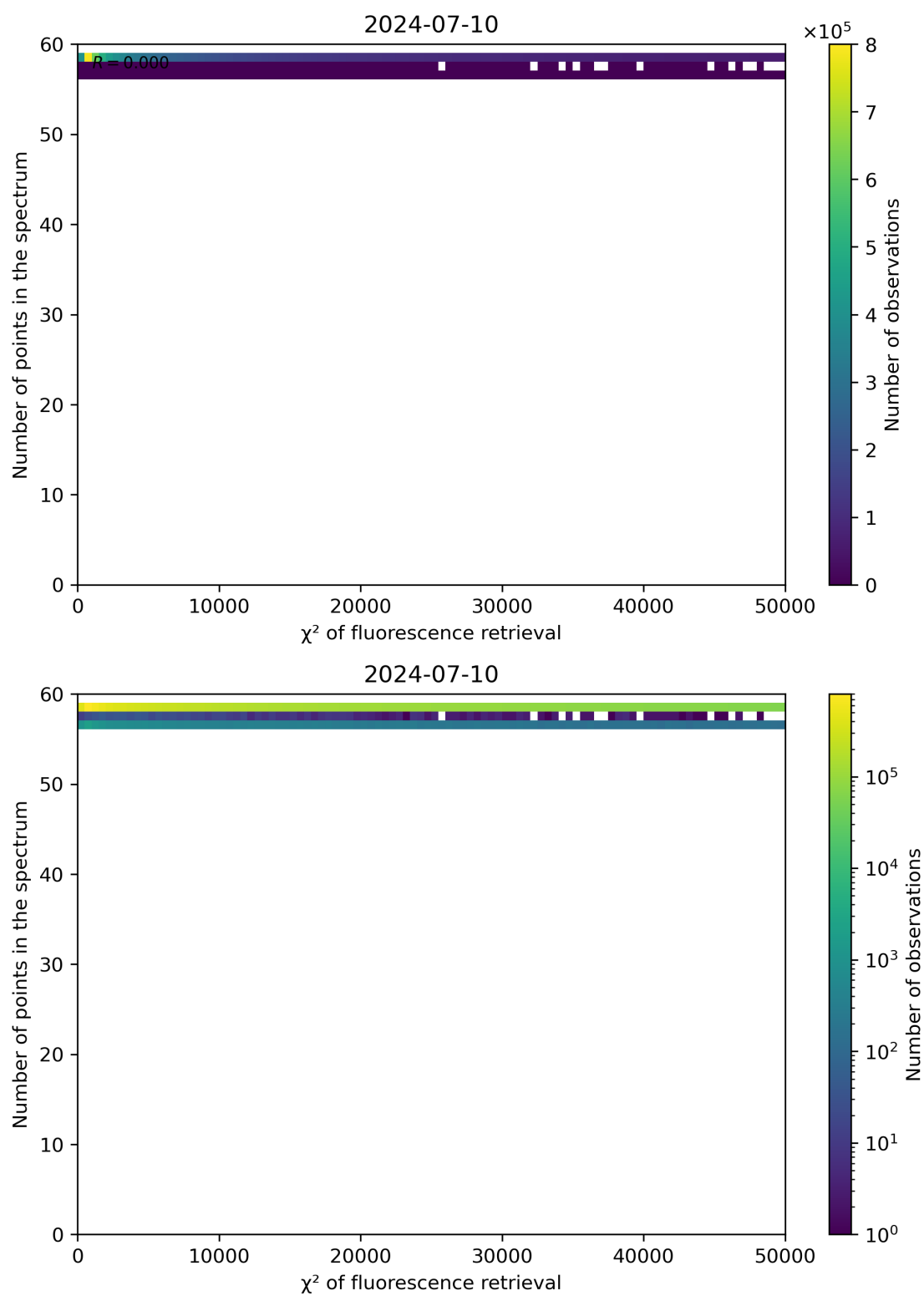
Figure 68: Scatter density plot of " \chi^2 of fluorescence retrieval" against "Number of points in the spectrum" for 2024-07-10 to 2024-07-11.
