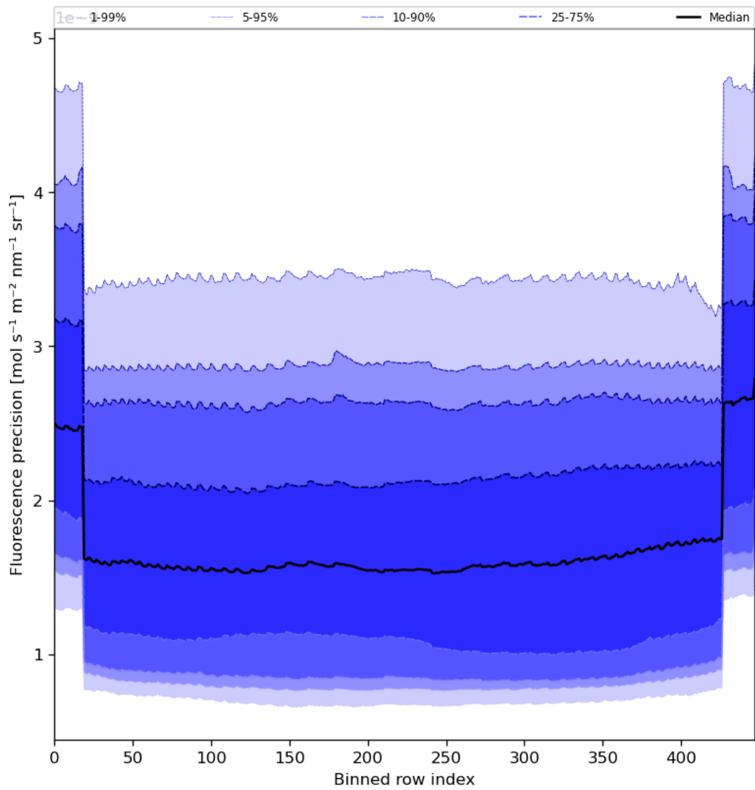
Figure 58: Along track statistics of “Fluorescence precision” for 2024-07-10 to 2024-07-11
