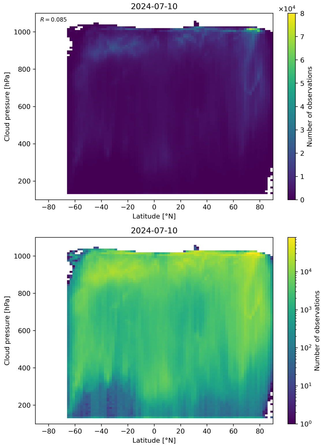
Figure 91: Scatter density plot of “Latitude” against “Cloud pressure” for 2024-07-10 to 2024-07-11.
