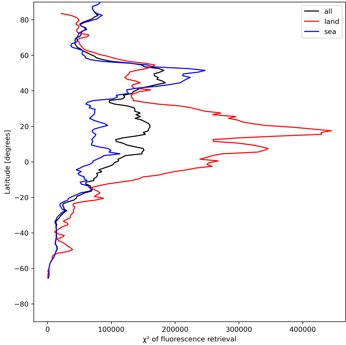
Figure 25: Zonal average of “ \chi^2 of fluorescence retrieval” for 2024-07-10 to 2024-07-11.
