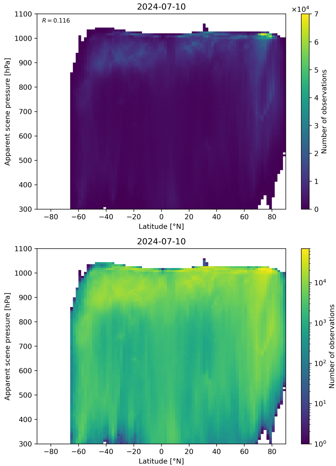
Figure 88: Scatter density plot of “Latitude” against “Apparent scene pressure” for 2024-07-10 to 2024-07-11.
