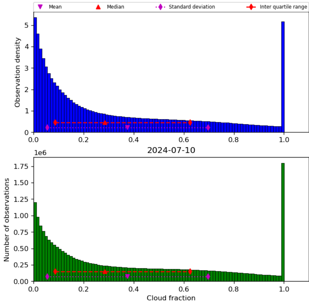
Figure 32: Histogram of “Cloud fraction” for 2024-07-10 to 2024-07-11
