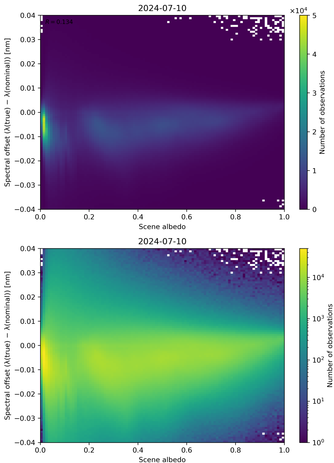
Figure 107: Scatter density plot of “Scene albedo” against “Spectral offset ( \lambda(\text{true}) - \lambda(\text{nominal}) )” for 2024-07-10 to 2024-07-11.
