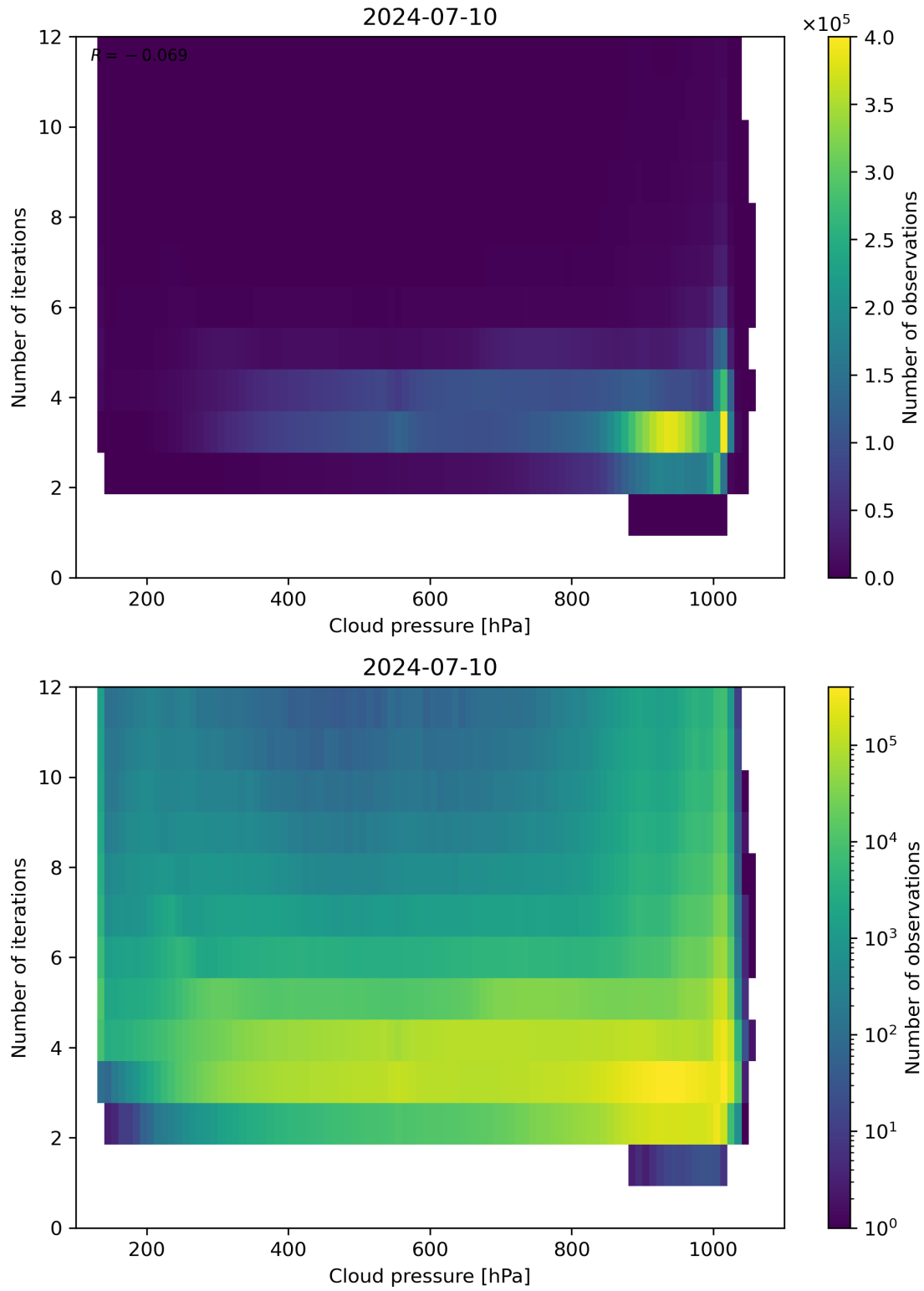
Figure 81: Scatter density plot of “Cloud pressure” against “Number of iterations” for 2024-07-10 to 2024-07-11.
