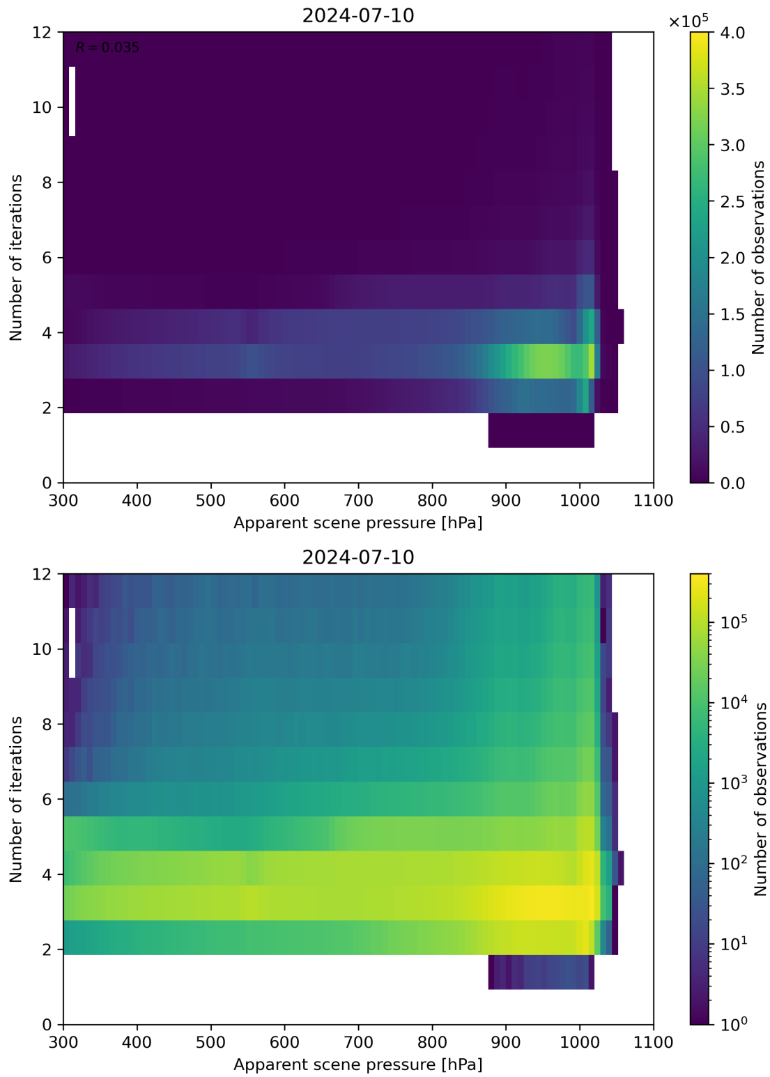
Figure 65: Scatter density plot of “Apparent scene pressure” against “Number of iterations” for 2024-07-10 to 2024-07-11.
