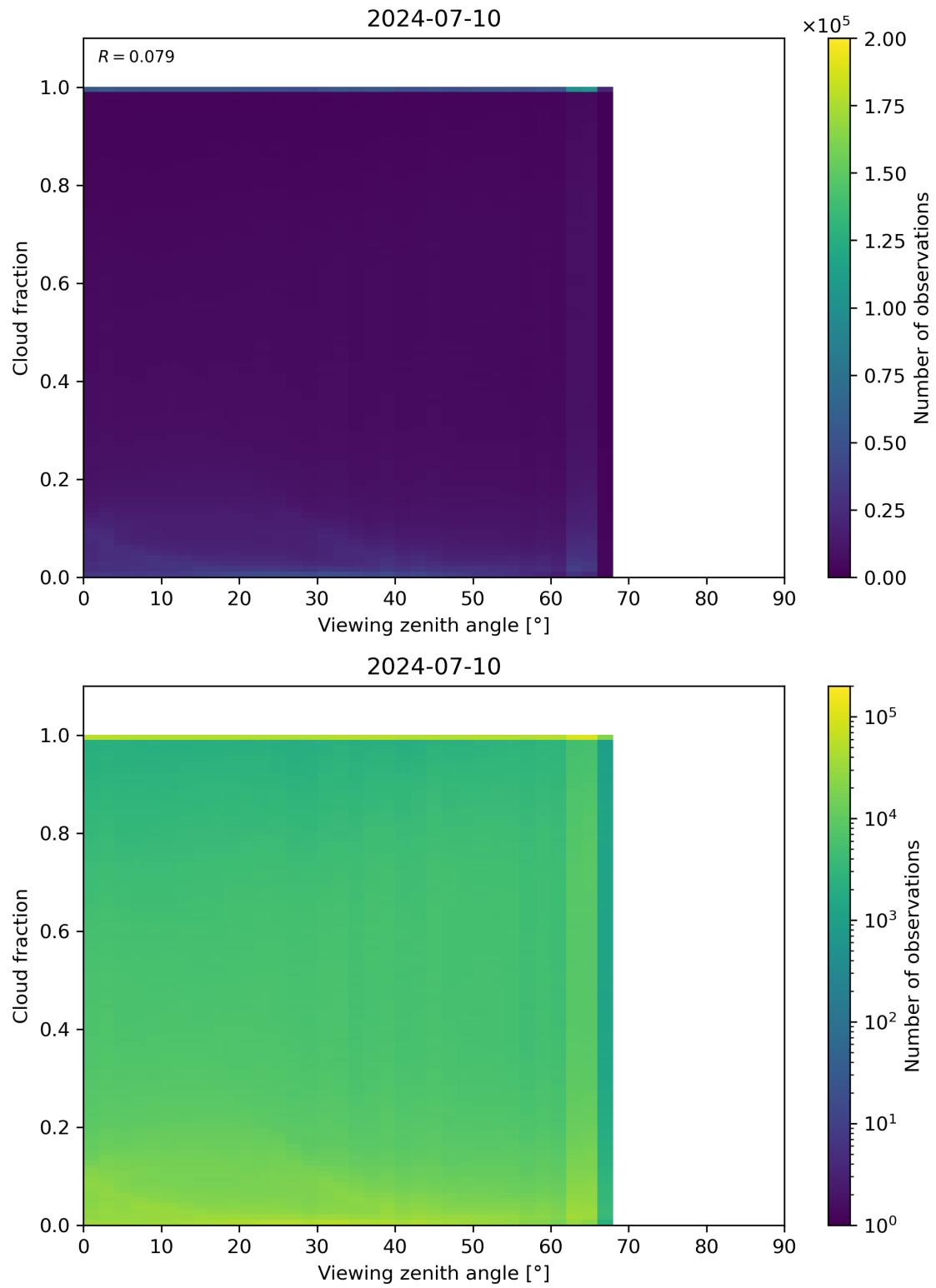
Figure 120: Scatter density plot of “Viewing zenith angle” against “Cloud fraction” for 2024-07-10 to 2024-07-11.
