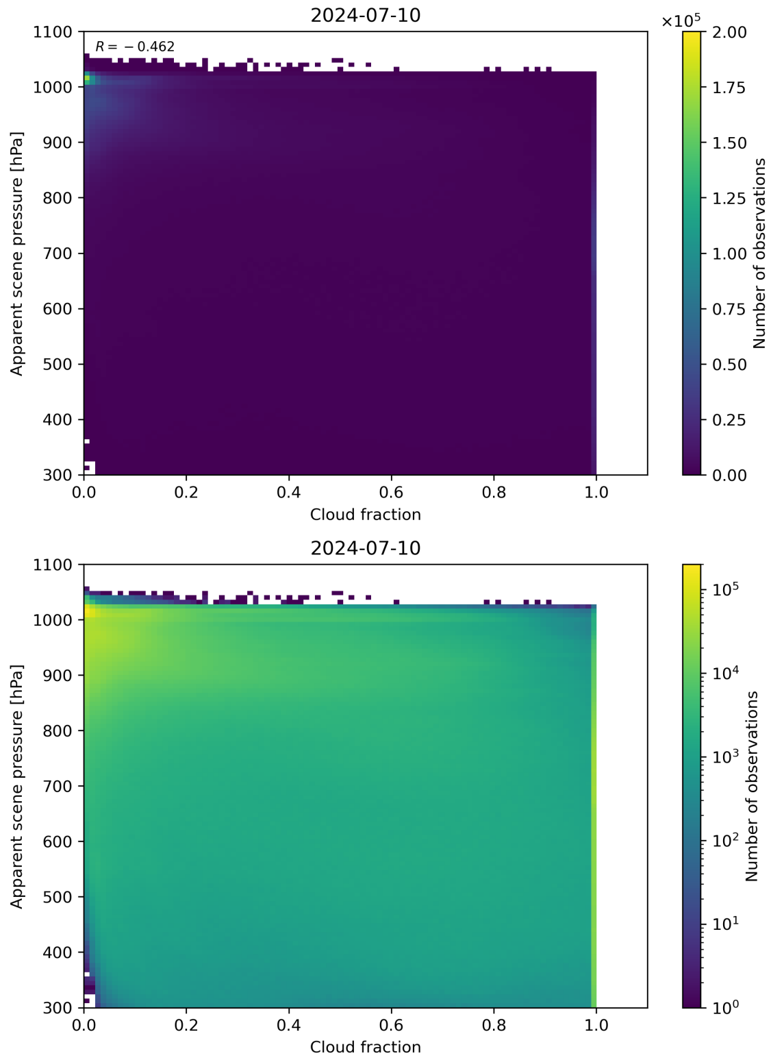
Figure 70: Scatter density plot of “Cloud fraction” against “Apparent scene pressure” for 2024-07-10 to 2024-07-11.
