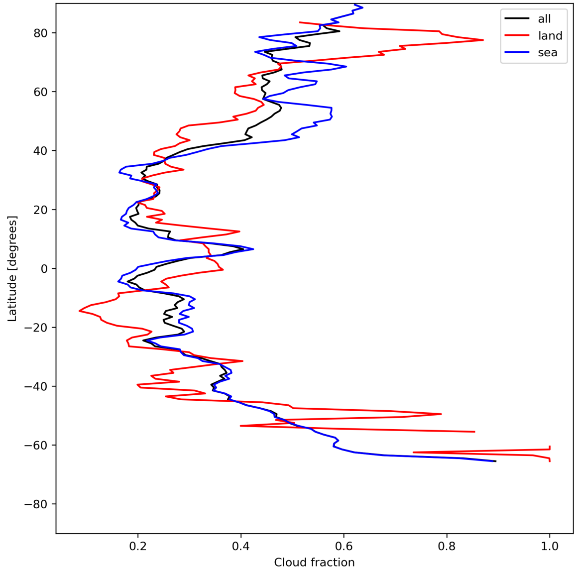
Figure 15: Zonal average of “Cloud fraction” for 2024-07-10 to 2024-07-11.
