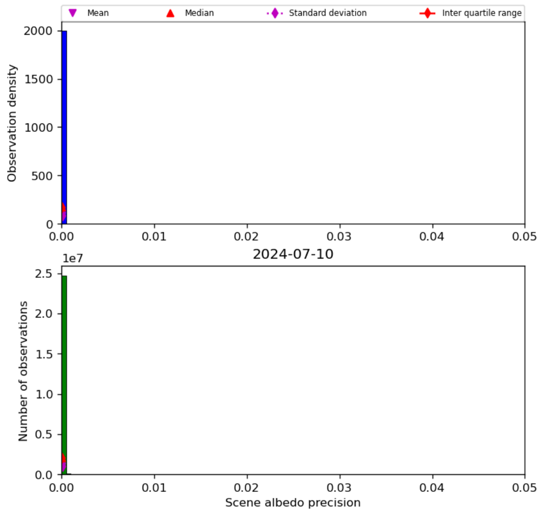
Figure 35: Histogram of “Scene albedo precision” for 2024-07-10 to 2024-07-11
