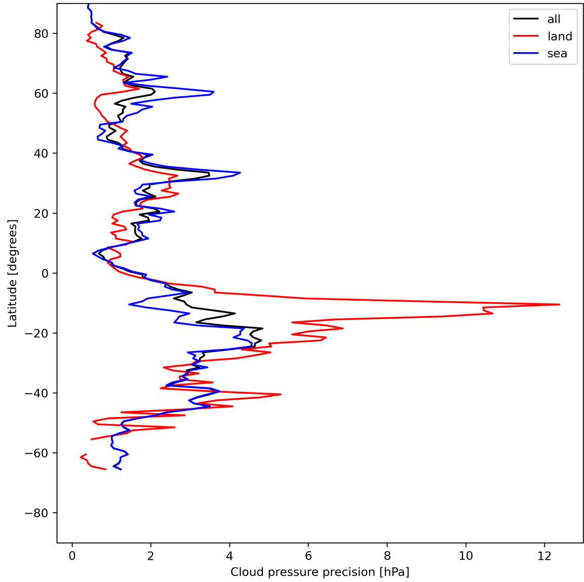
Figure 14: Zonal average of “Cloud pressure precision” for 2024-07-10 to 2024-07-11.
