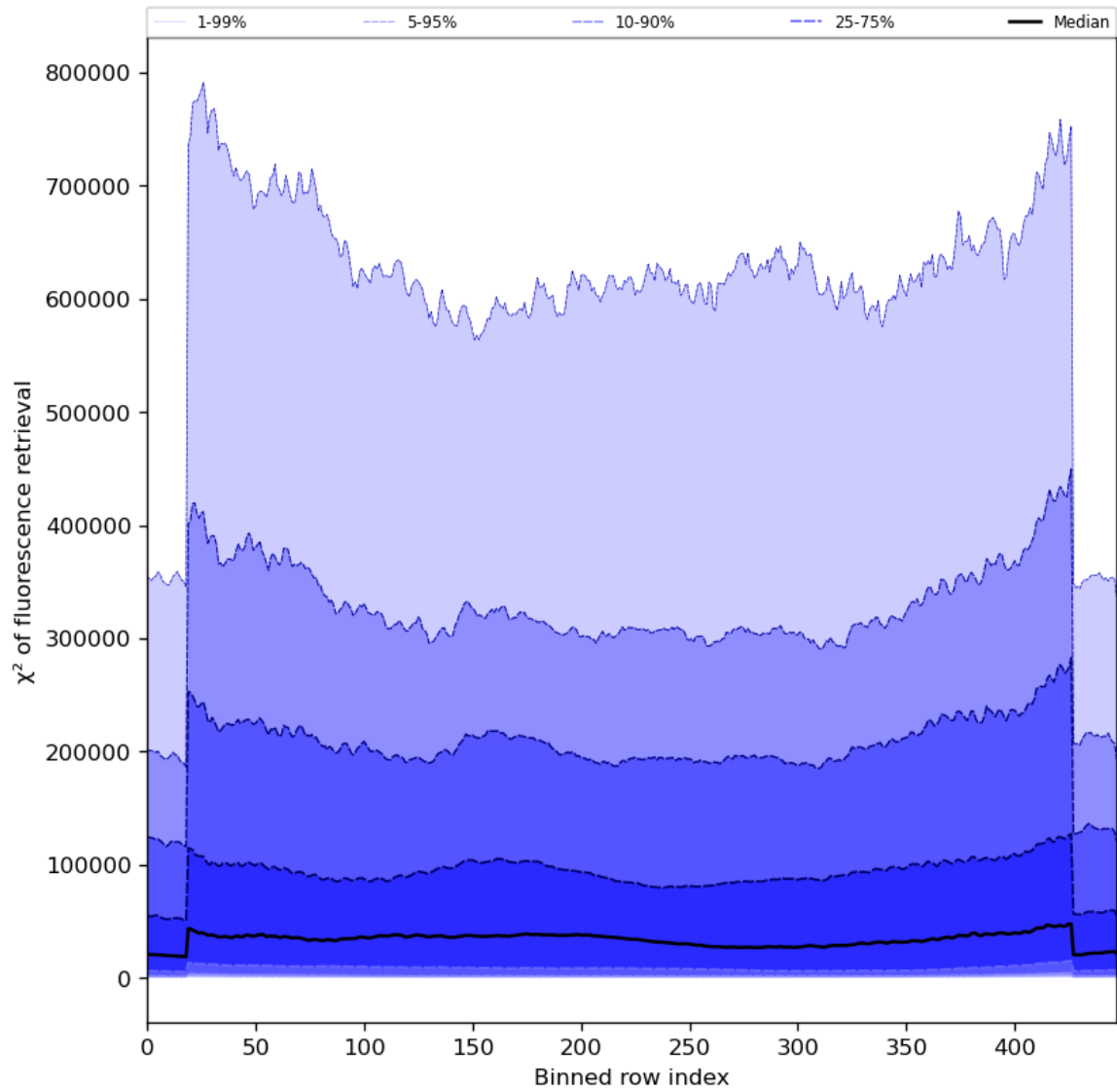
Figure 59: Along track statistics of “ \chi^2 of fluorescence retrieval” for 2024-07-10 to 2024-07-11
