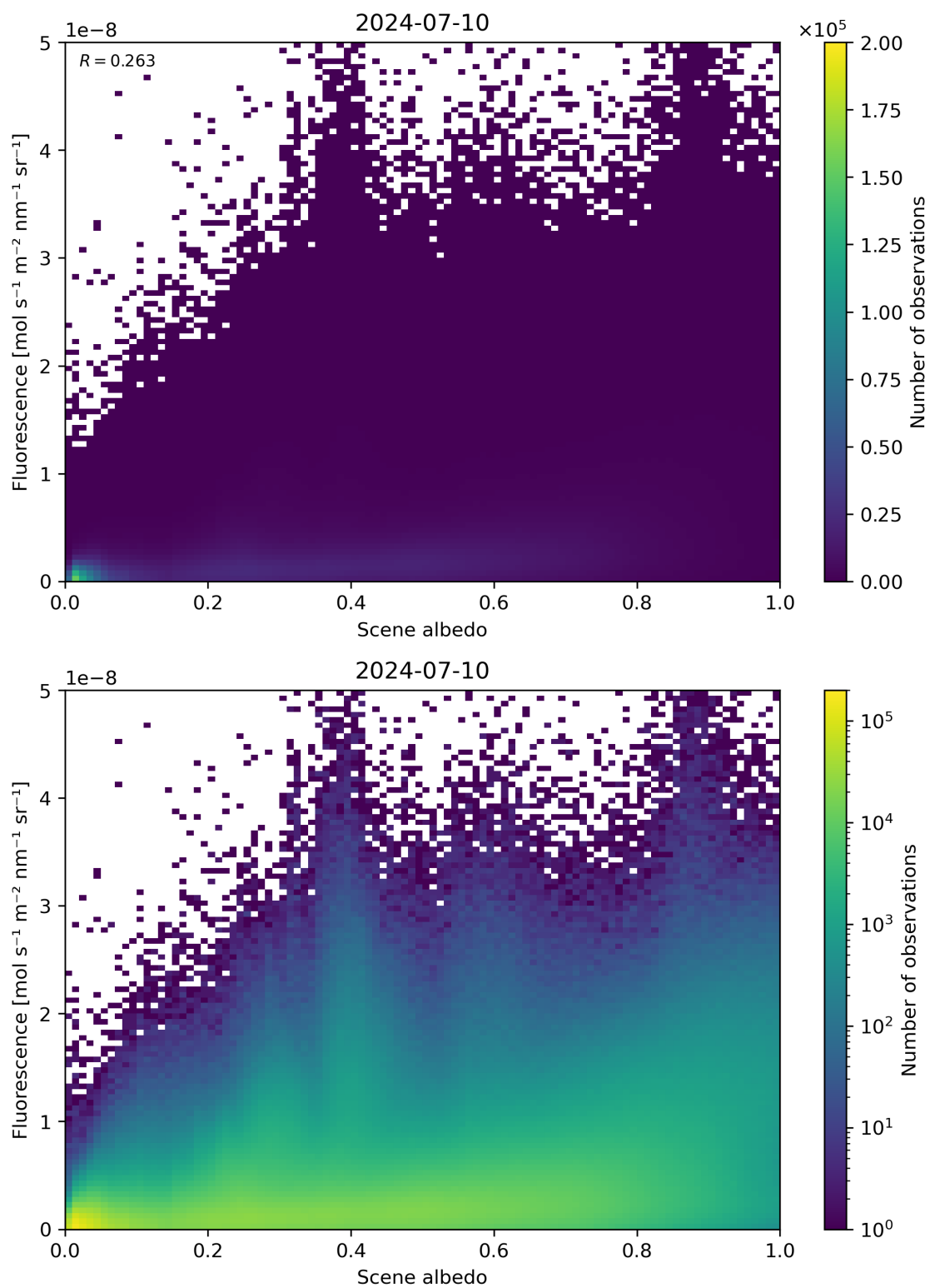
Figure 104: Scatter density plot of “Scene albedo” against “Fluorescence” for 2024-07-10 to 2024-07-11.
