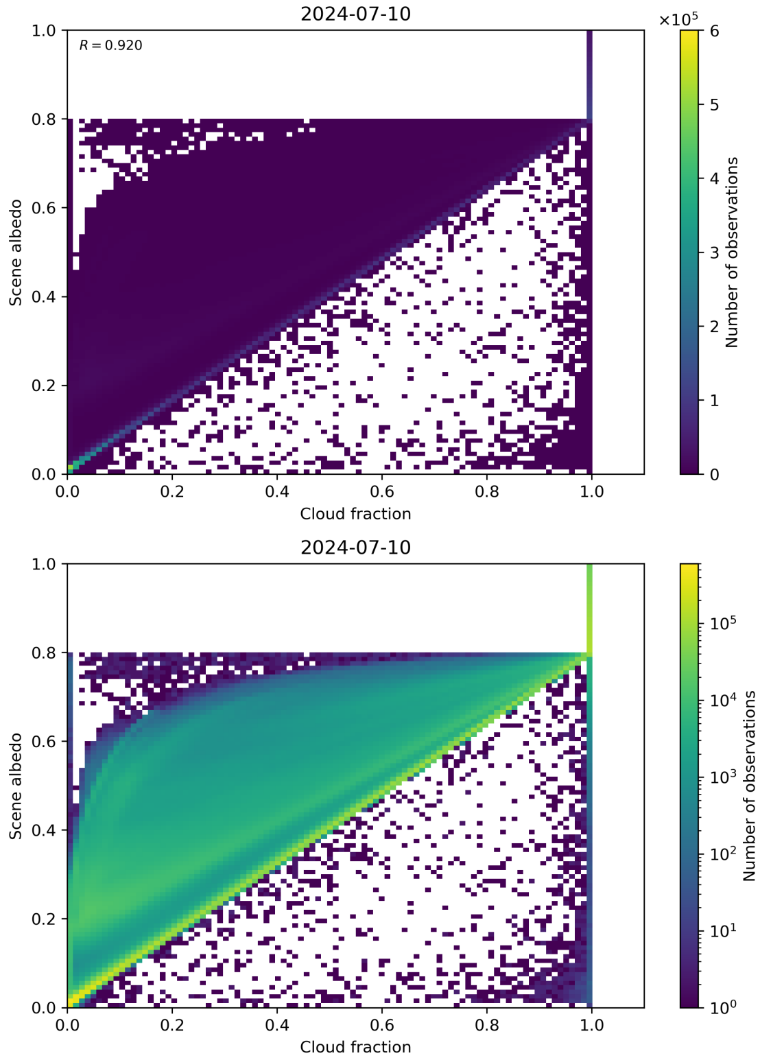
Figure 75: Scatter density plot of “Cloud fraction” against “Scene albedo” for 2024-07-10 to 2024-07-11.
