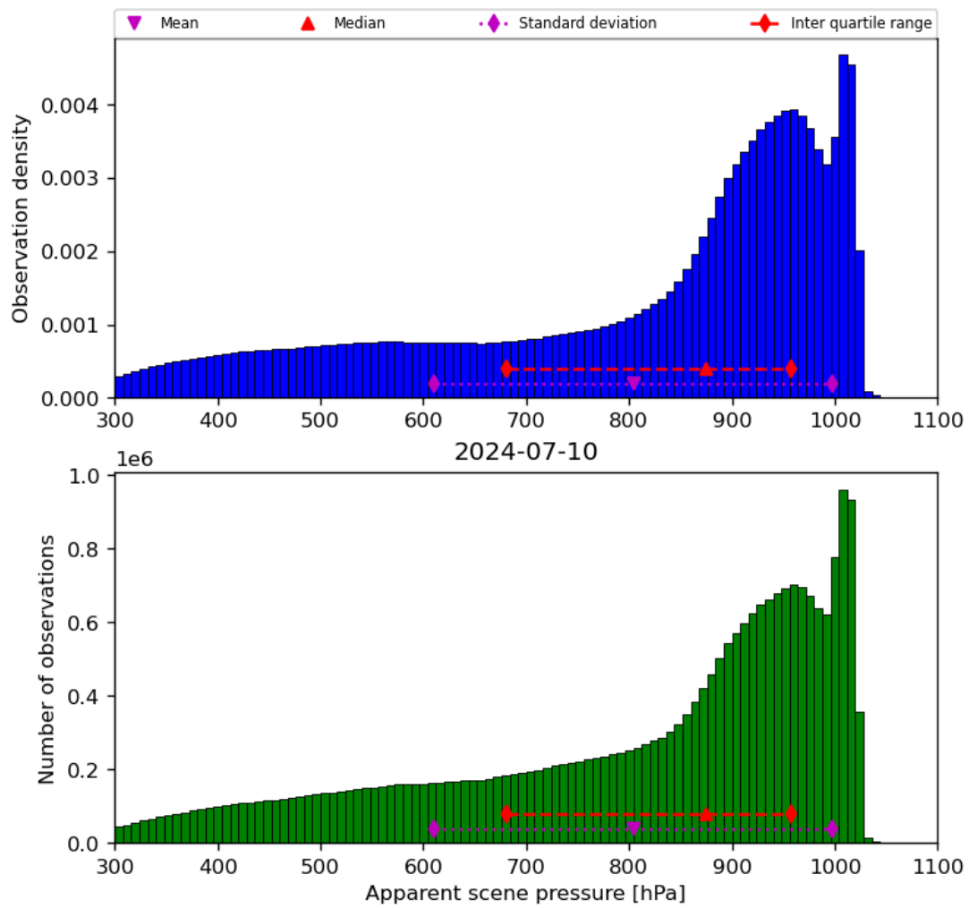
Figure 36: Histogram of “Apparent scene pressure” for 2024-07-10 to 2024-07-11
