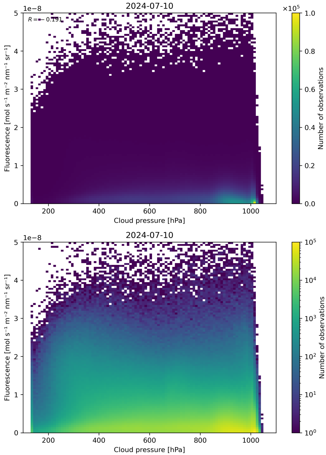
Figure 80: Scatter density plot of “Cloud pressure” against “Fluorescence” for 2024-07-10 to 2024-07-11.
