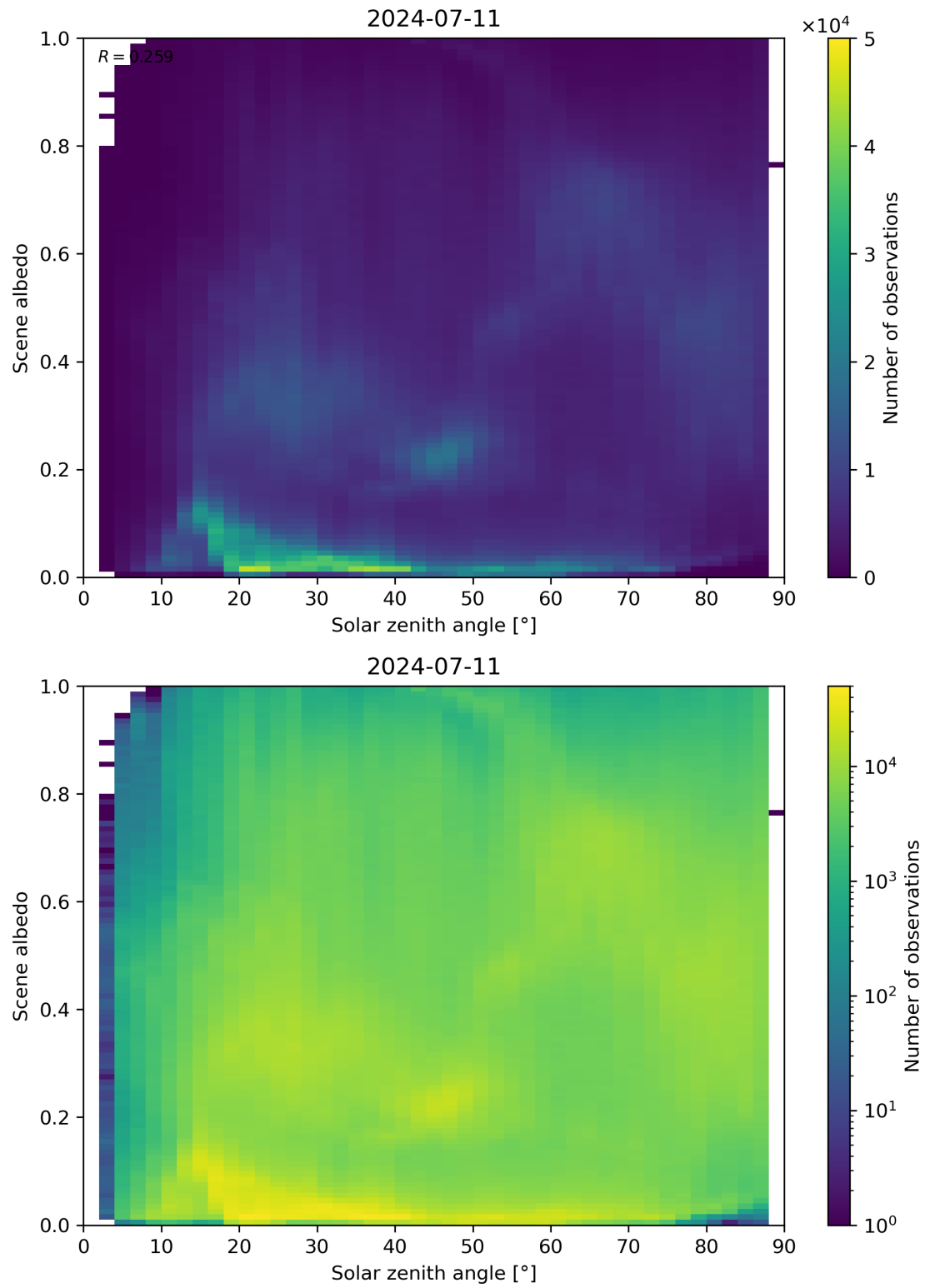
Figure 116: Scatter density plot of “Solar zenith angle” against “Scene albedo” for 2024-07-10 to 2024-07-12.
