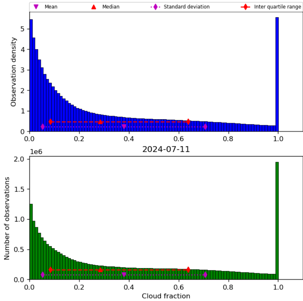
Figure 32: Histogram of “Cloud fraction” for 2024-07-10 to 2024-07-12
