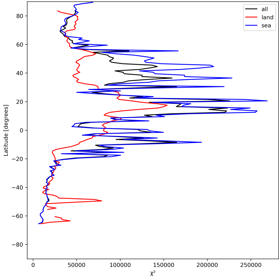
Figure 21: Zonal average of “ \chi^2 ” for 2024-07-10 to 2024-07-12.
