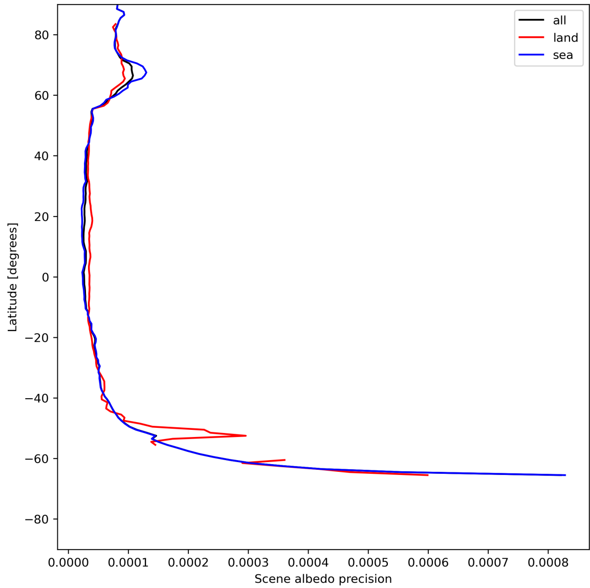
Figure 18: Zonal average of “Scene albedo precision” for 2024-07-10 to 2024-07-12.
