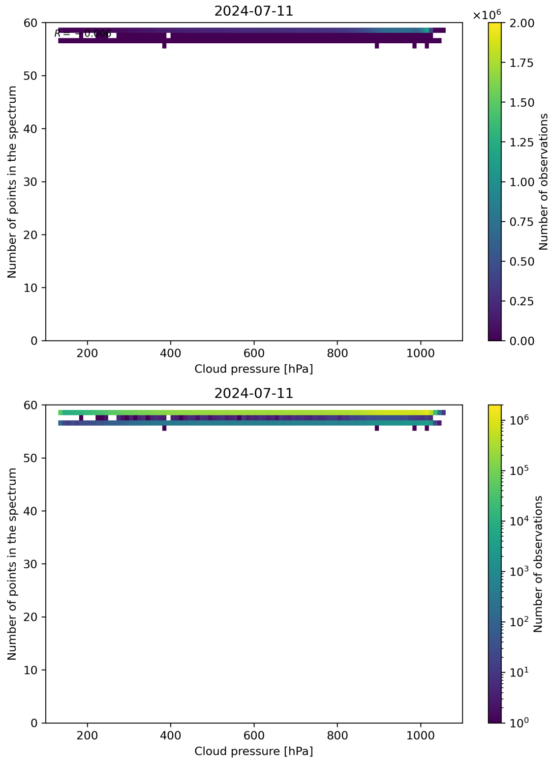
Figure 82: Scatter density plot of “Cloud pressure” against “Number of points in the spectrum” for 2024-07-10 to 2024-07-12.
