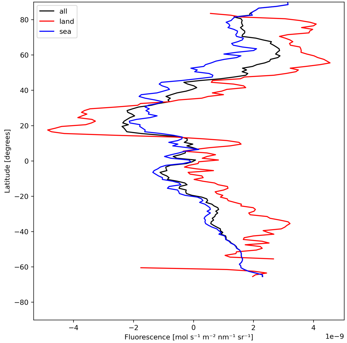
Figure 23: Zonal average of “Fluorescence” for 2024-07-10 to 2024-07-12.
