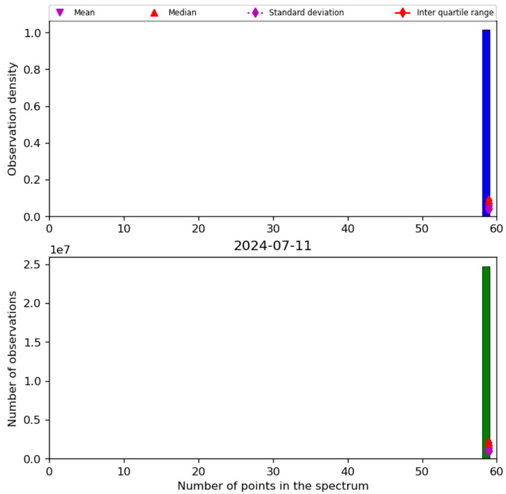
Figure 44: Histogram of “Number of points in the spectrum” for 2024-07-10 to 2024-07-12
