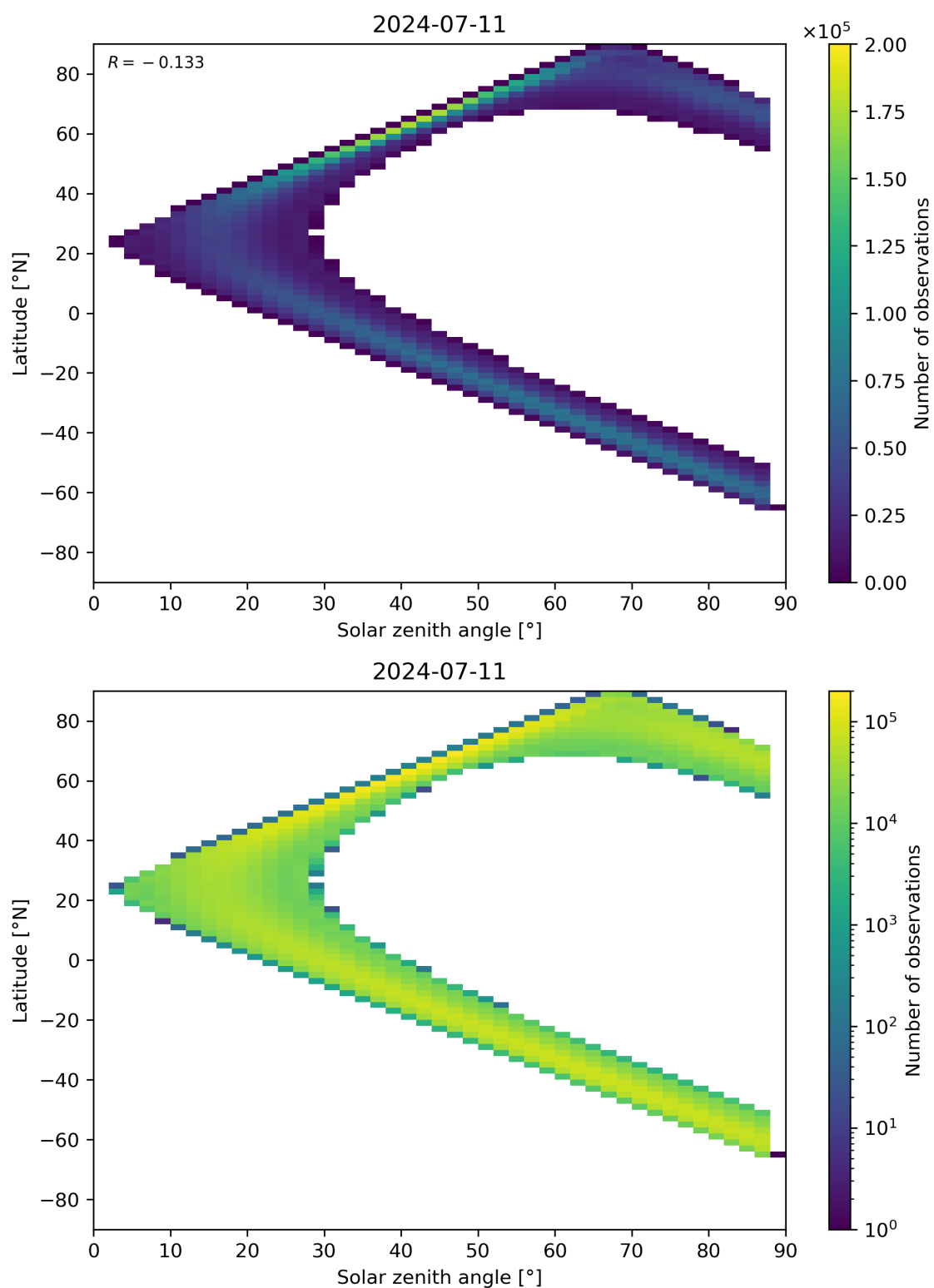
Figure 113: Scatter density plot of “Solar zenith angle” against “Latitude” for 2024-07-10 to 2024-07-12.
