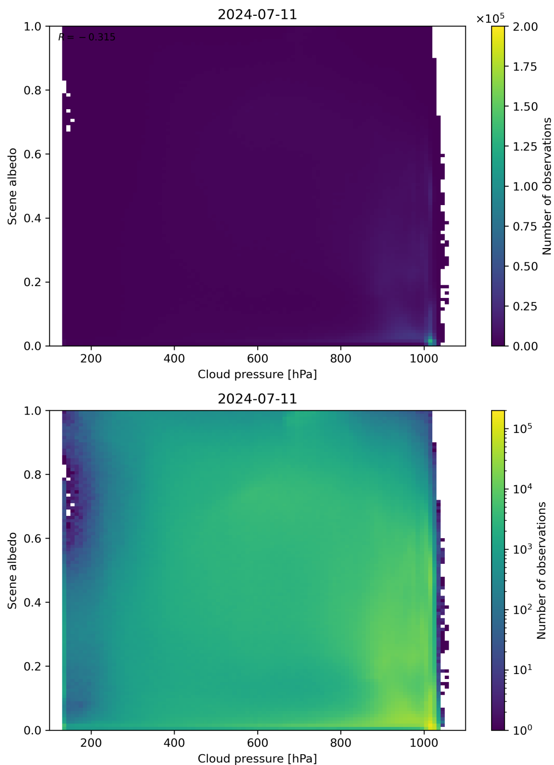
Figure 83: Scatter density plot of “Cloud pressure” against “Scene albedo” for 2024-07-10 to 2024-07-12.
