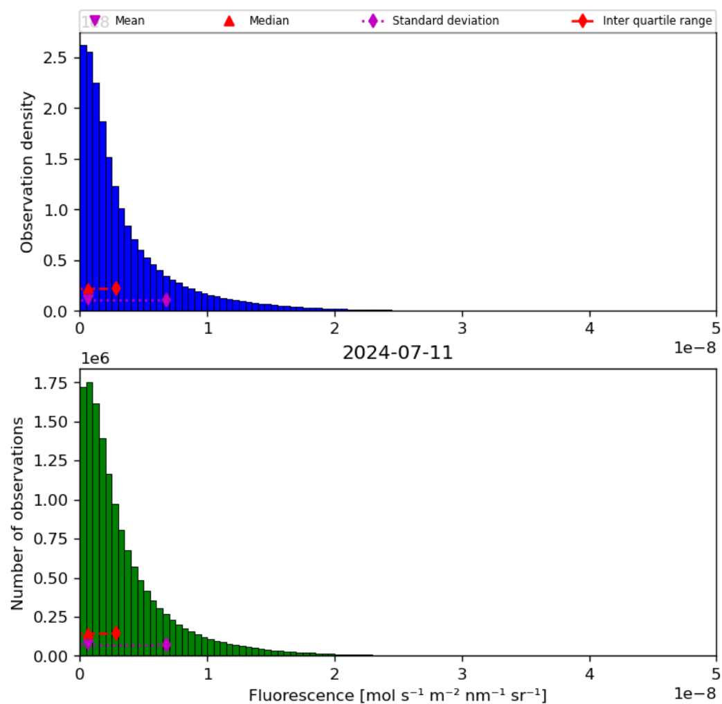
Figure 40: Histogram of “Fluorescence” for 2024-07-10 to 2024-07-12
