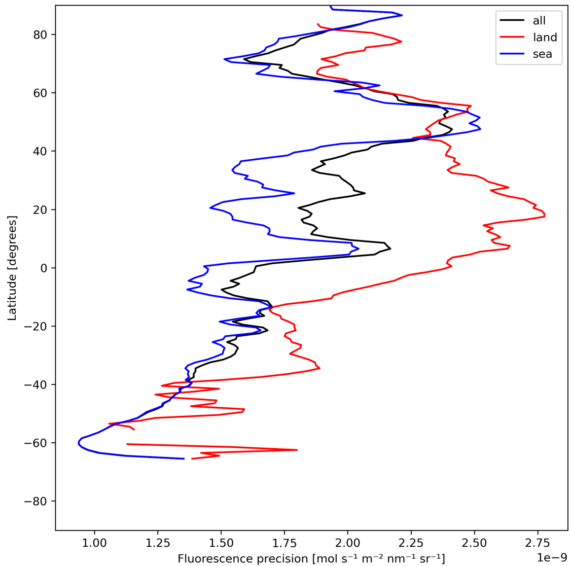
Figure 24: Zonal average of “Fluorescence precision” for 2024-07-10 to 2024-07-12.
