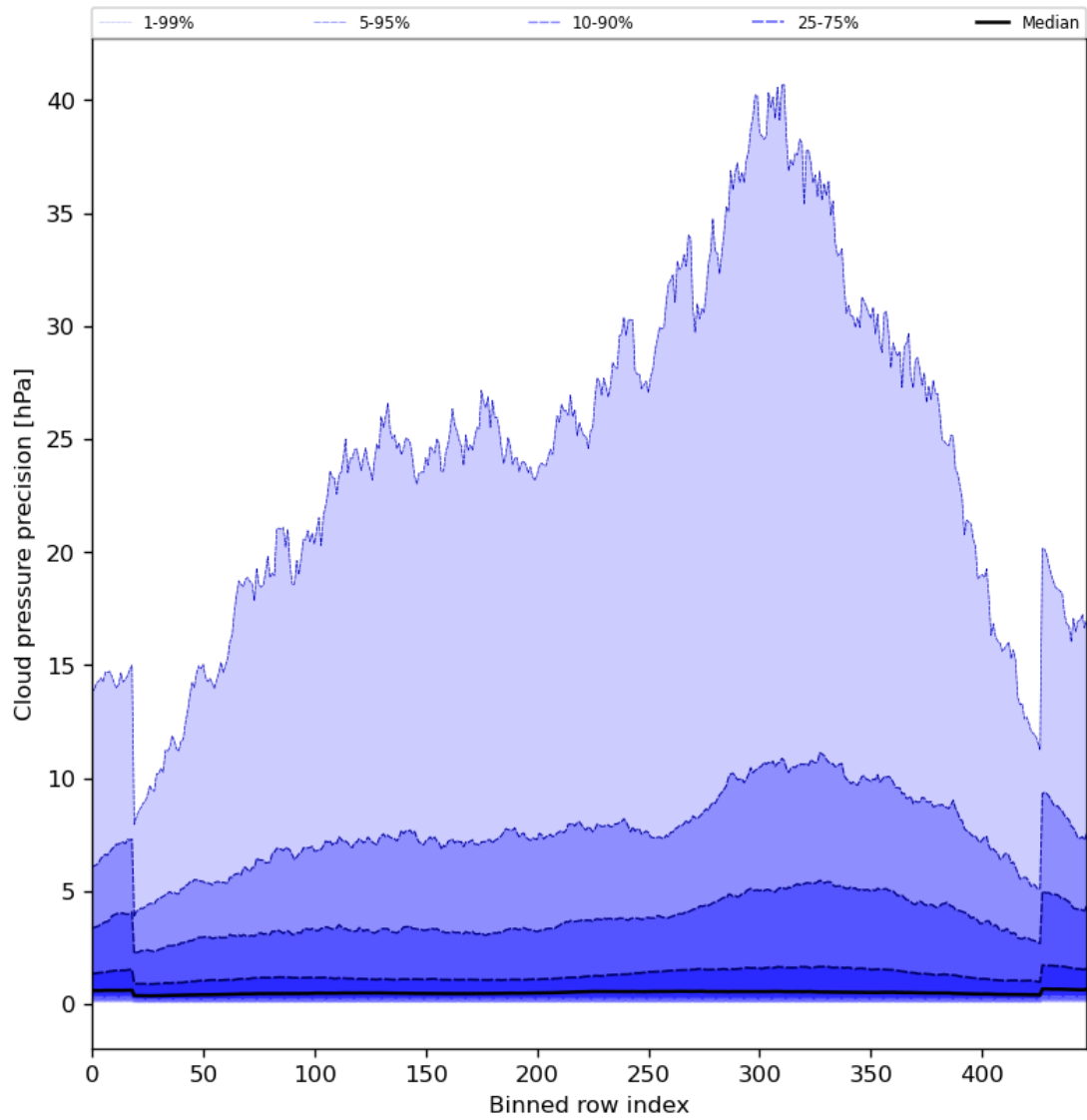
Figure 48: Along track statistics of “Cloud pressure precision” for 2024-07-10 to 2024-07-12
