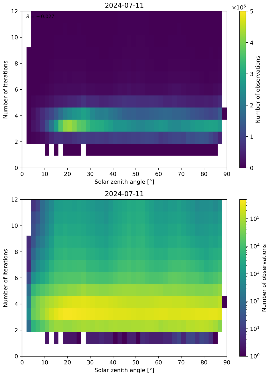
Figure 114: Scatter density plot of “Solar zenith angle” against “Number of iterations” for 2024-07-10 to 2024-07-12.
