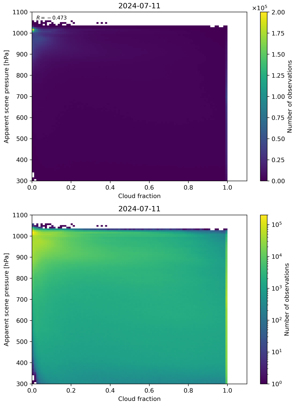
Figure 70: Scatter density plot of “Cloud fraction” against “Apparent scene pressure” for 2024-07-10 to 2024-07-12.
