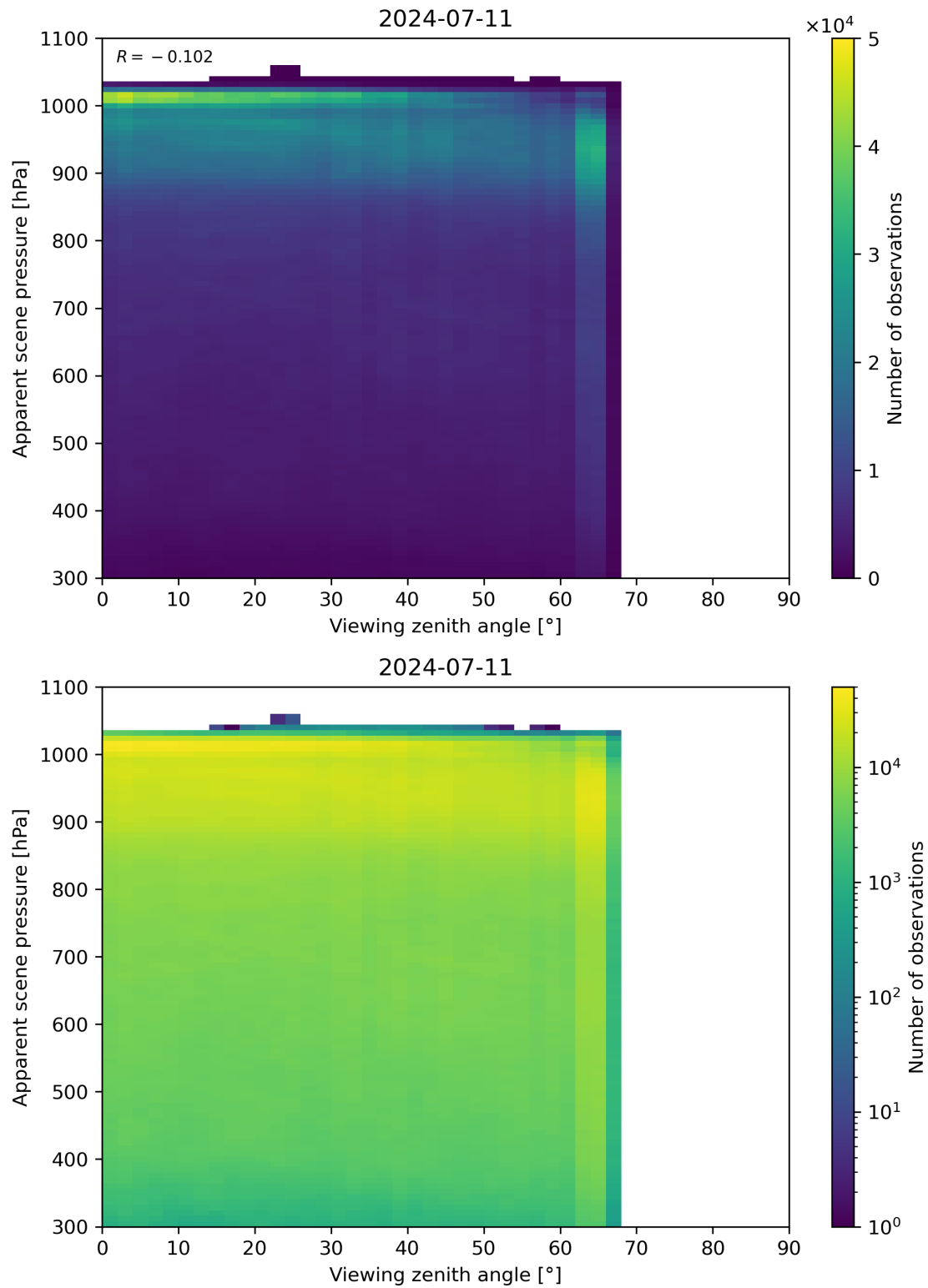
Figure 118: Scatter density plot of “Viewing zenith angle” against “Apparent scene pressure” for 2024-07-10 to 2024-07-12.
