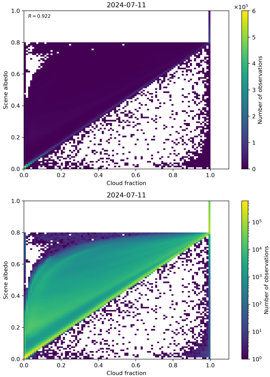
Figure 75: Scatter density plot of “Cloud fraction” against “Scene albedo” for 2024-07-10 to 2024-07-12.
