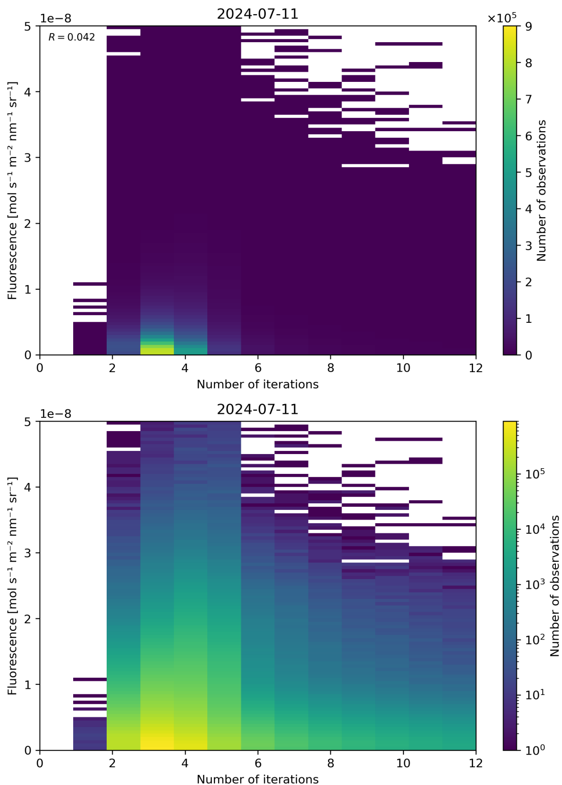
Figure 98: Scatter density plot of “Number of iterations” against “Fluorescence” for 2024-07-10 to 2024-07-12.
