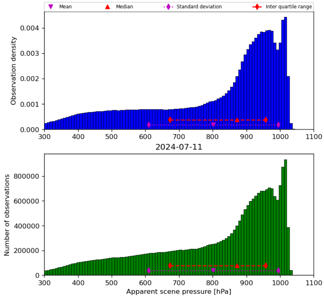
Figure 36: Histogram of “Apparent scene pressure” for 2024-07-10 to 2024-07-12
