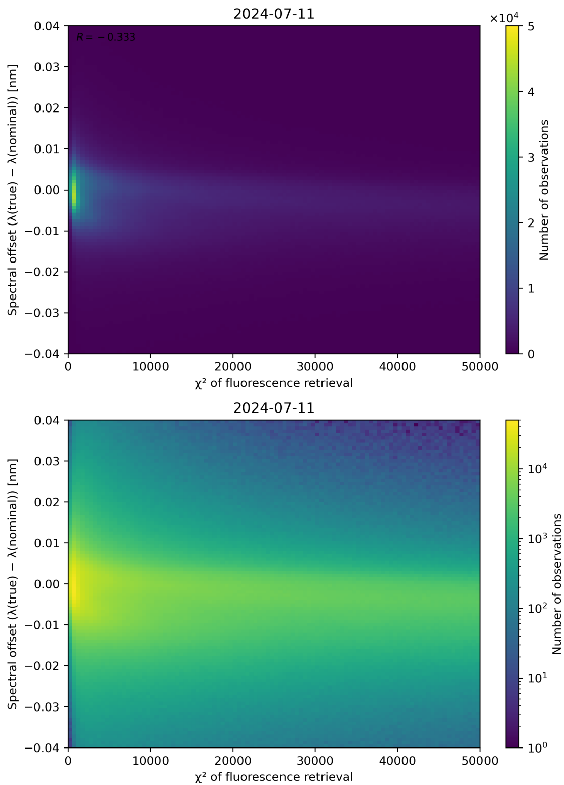
Figure 69: Scatter density plot of “ \chi^2 of fluorescence retrieval” against “Spectral offset ( \lambda(\text{true}) - \lambda(\text{nominal}) )” for 2024-07-10 to 2024-07-12.
