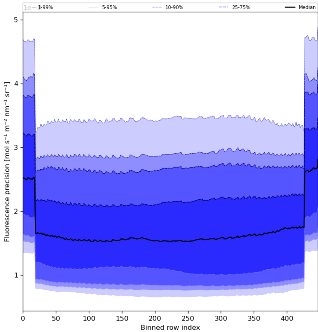
Figure 58: Along track statistics of “Fluorescence precision” for 2024-07-10 to 2024-07-12
