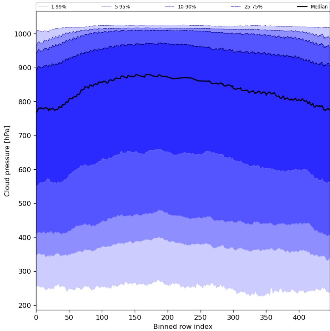
Figure 47: Along track statistics of “Cloud pressure” for 2024-07-10 to 2024-07-12
