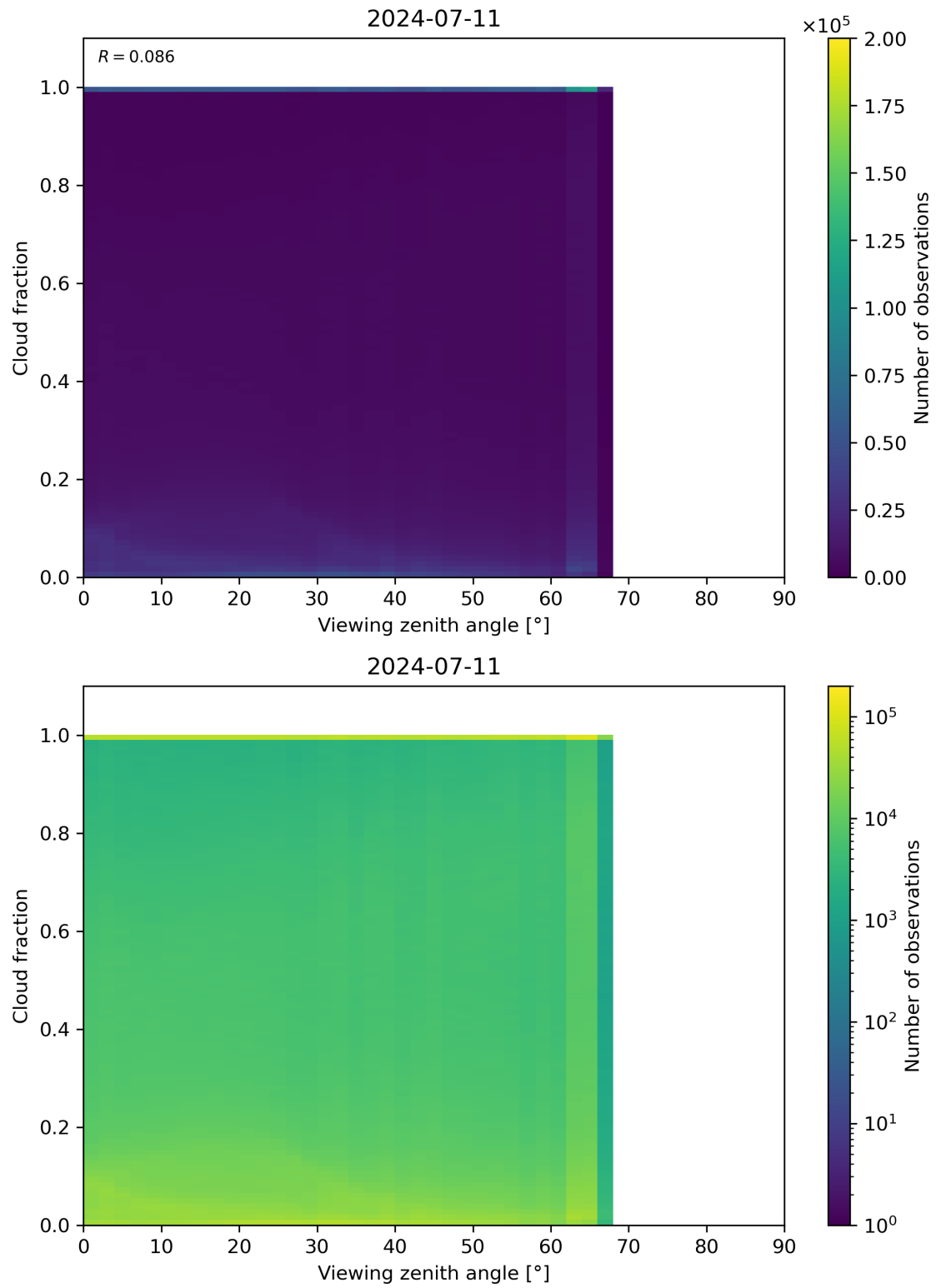
Figure 120: Scatter density plot of “Viewing zenith angle” against “Cloud fraction” for 2024-07-10 to 2024-07-12.
