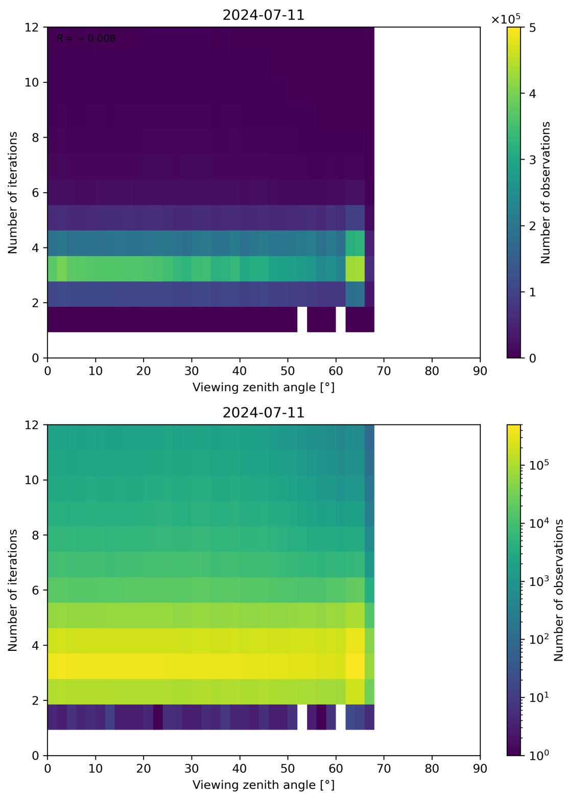
Figure 124: Scatter density plot of “Viewing zenith angle” against “Number of iterations” for 2024-07-10 to 2024-07-12.
