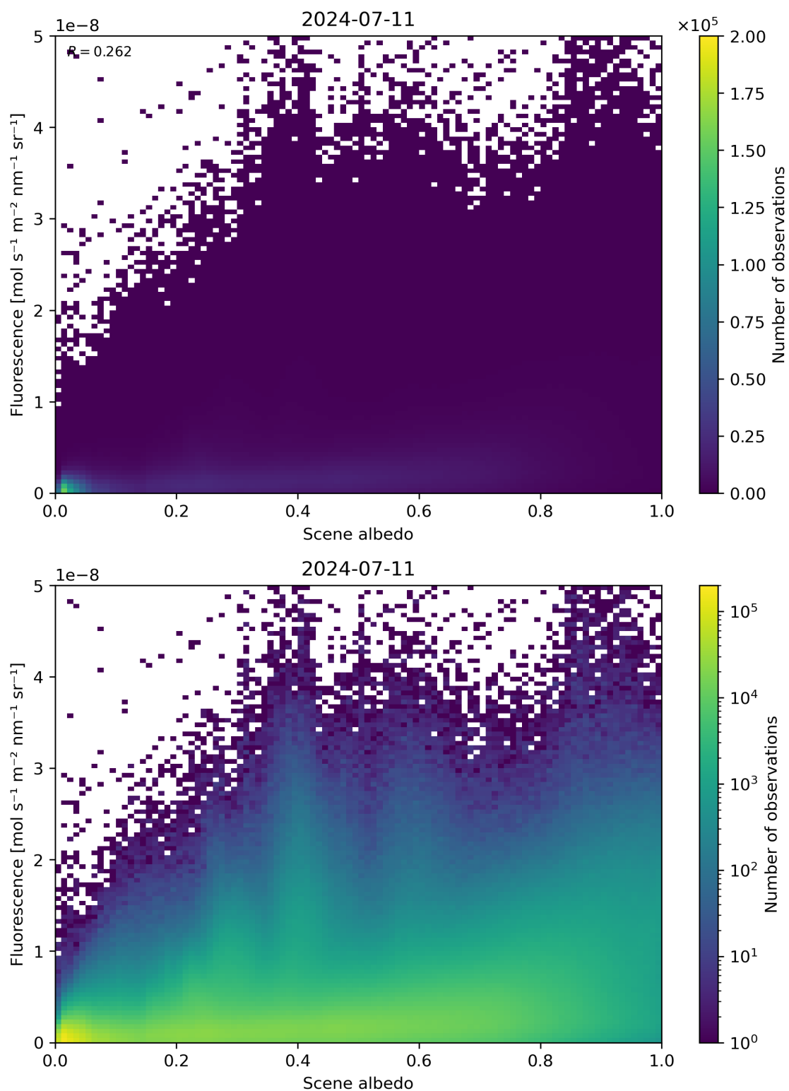
Figure 104: Scatter density plot of “Scene albedo” against “Fluorescence” for 2024-07-10 to 2024-07-12.
