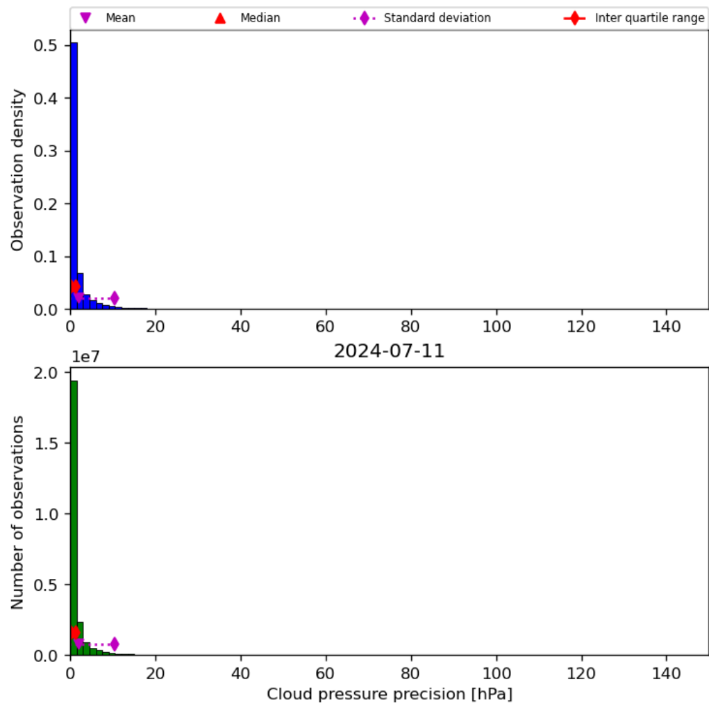
Figure 31: Histogram of “Cloud pressure precision” for 2024-07-10 to 2024-07-12
