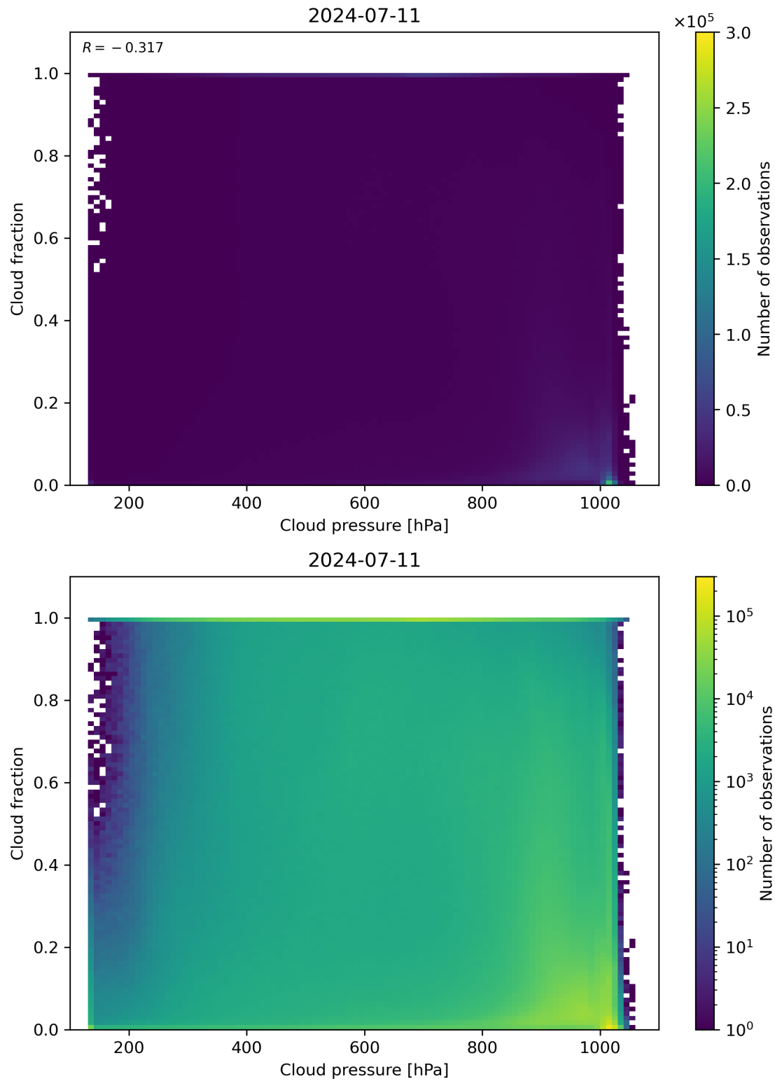
Figure 79: Scatter density plot of “Cloud pressure” against “Cloud fraction” for 2024-07-10 to 2024-07-12.
