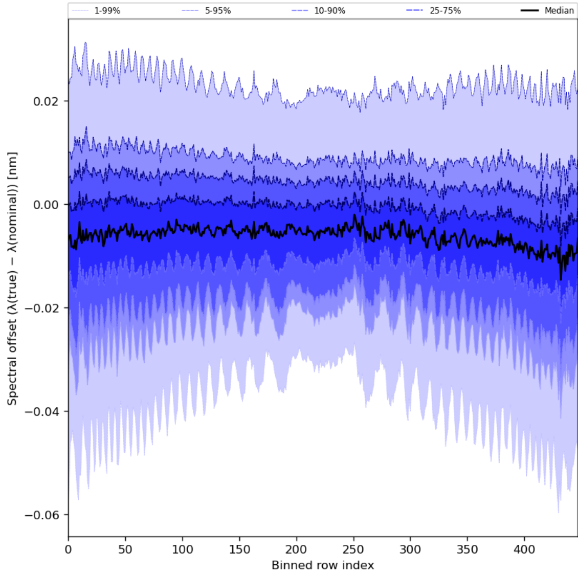
Figure 62: Along track statistics of “Spectral offset ( \lambda(\text{true}) - \lambda(\text{nominal}) )” for 2024-07-10 to 2024-07-12
