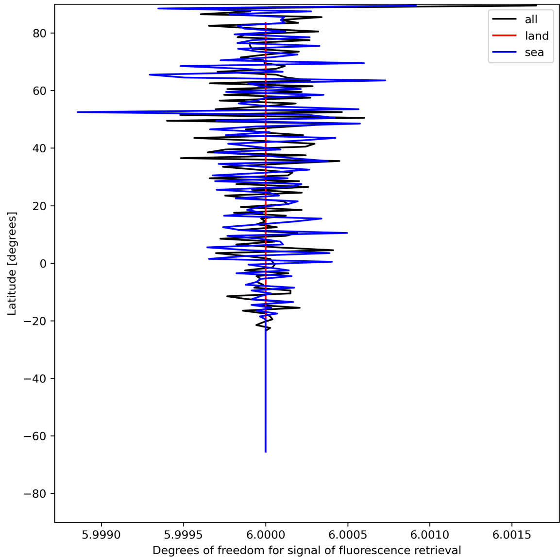
Figure 26: Zonal average of “Degrees of freedom for signal of fluorescence retrieval” for 2024-07-10 to 2024-07-12.
