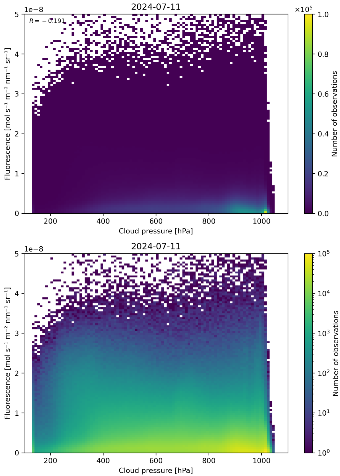
Figure 80: Scatter density plot of “Cloud pressure” against “Fluorescence” for 2024-07-10 to 2024-07-12.
