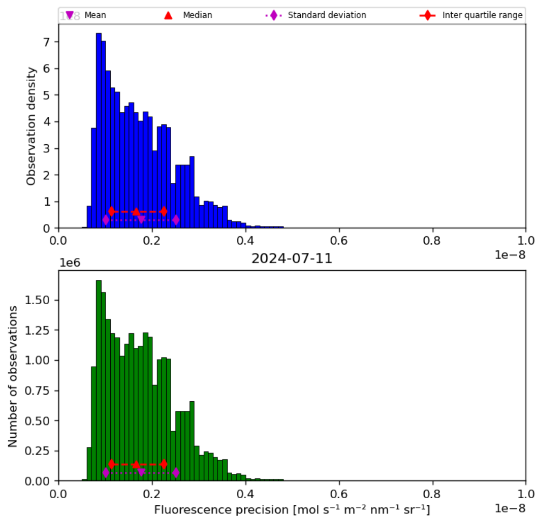
Figure 41: Histogram of “Fluorescence precision” for 2024-07-10 to 2024-07-12
