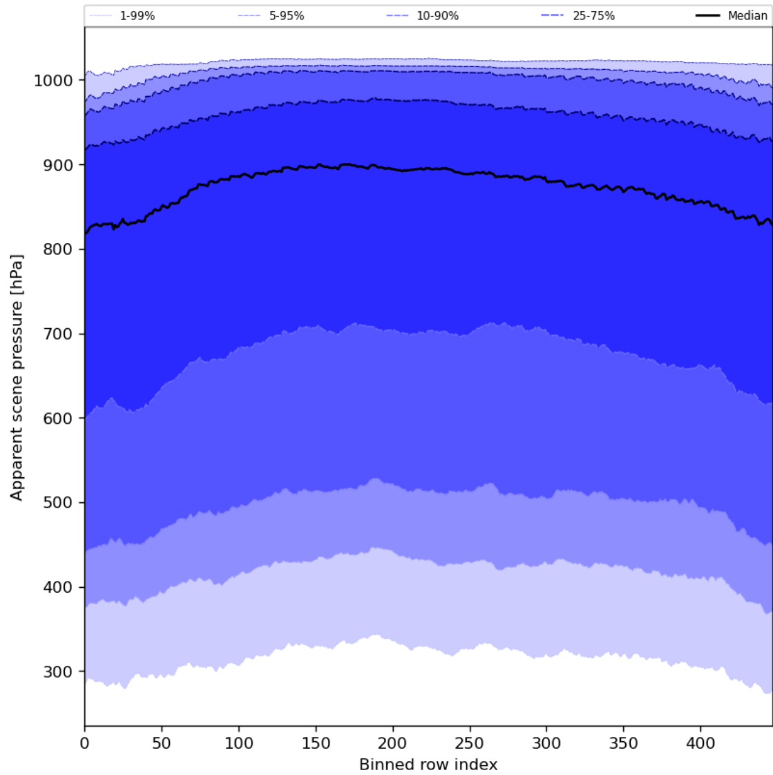
Figure 53: Along track statistics of “Apparent scene pressure” for 2024-07-10 to 2024-07-12
