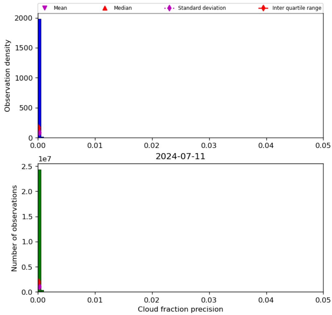
Figure 33: Histogram of “Cloud fraction precision” for 2024-07-10 to 2024-07-12
