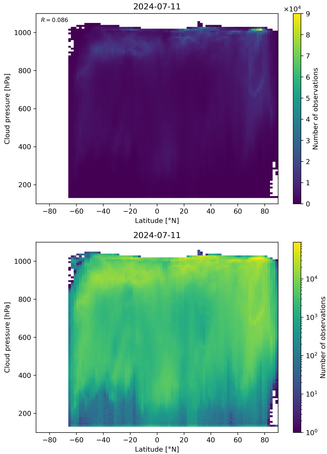
Figure 91: Scatter density plot of “Latitude” against “Cloud pressure” for 2024-07-10 to 2024-07-12.
