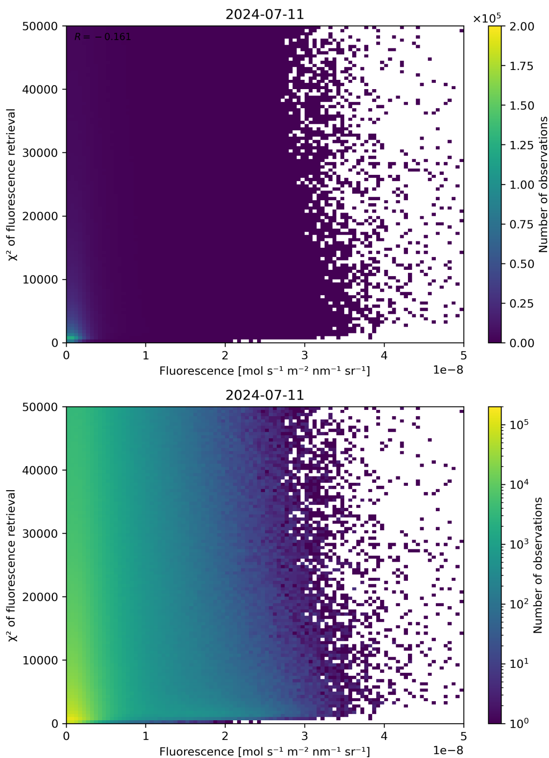
Figure 85: Scatter density plot of “Fluorescence” against “ \chi^2 of fluorescence retrieval” for 2024-07-10 to 2024-07-12.
