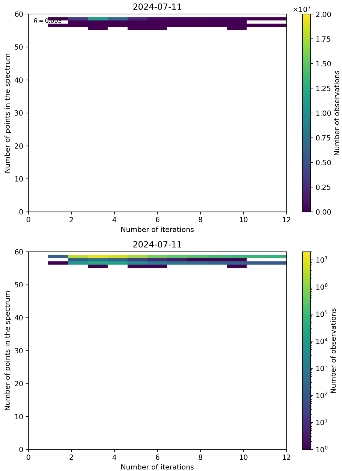
Figure 99: Scatter density plot of “Number of iterations” against “Number of points in the spectrum” for 2024-07-10 to 2024-07-12.
