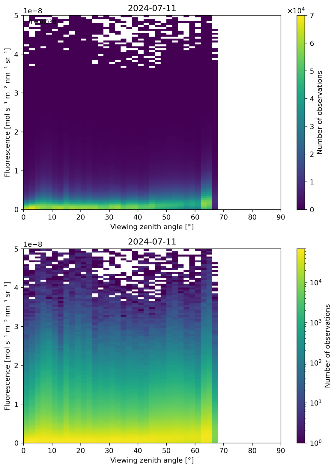
Figure 122: Scatter density plot of “Viewing zenith angle” against “Fluorescence” for 2024-07-10 to 2024-07-12.
