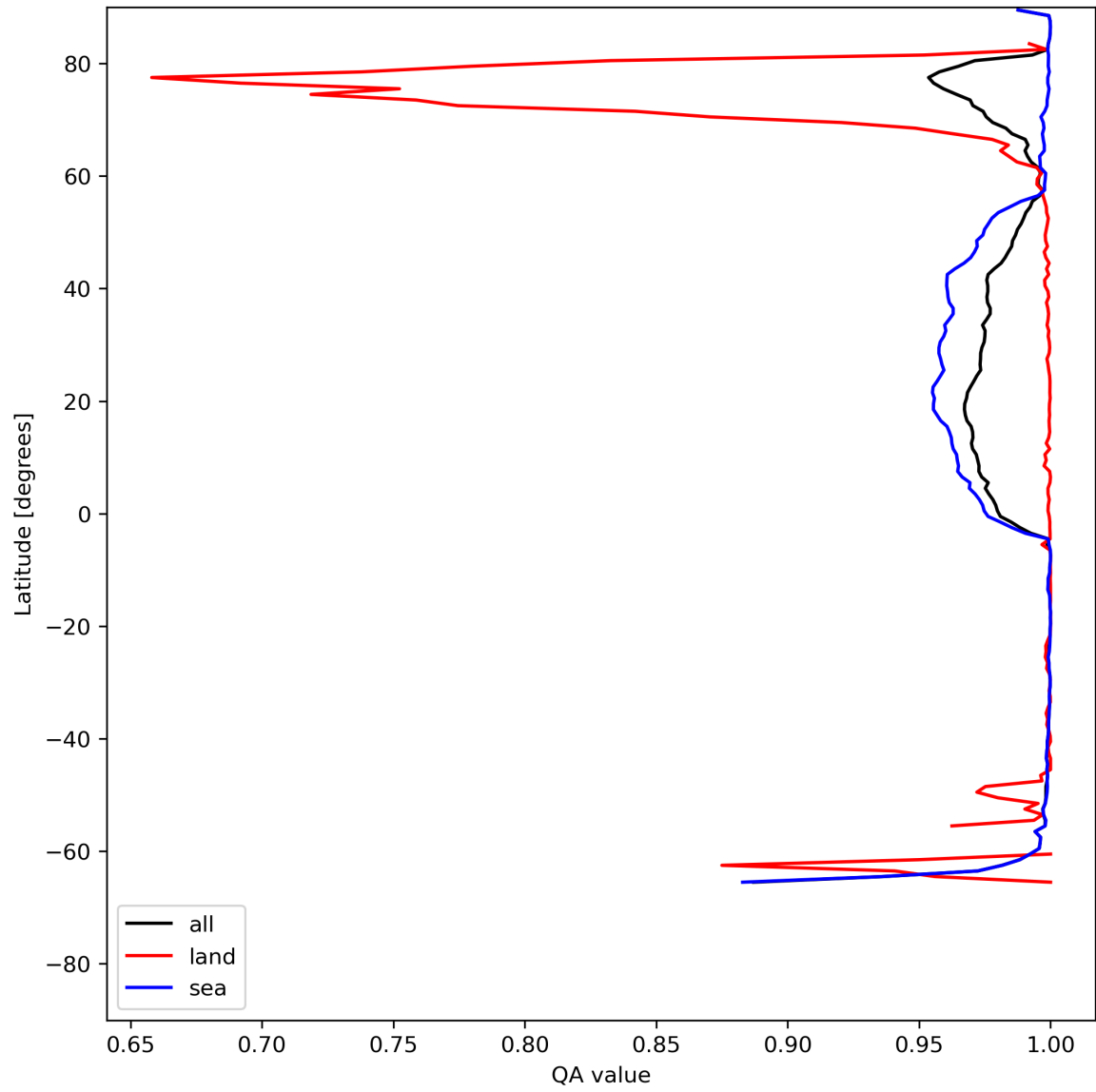
Figure 12: Zonal average of “QA value” for 2024-07-10 to 2024-07-12.
