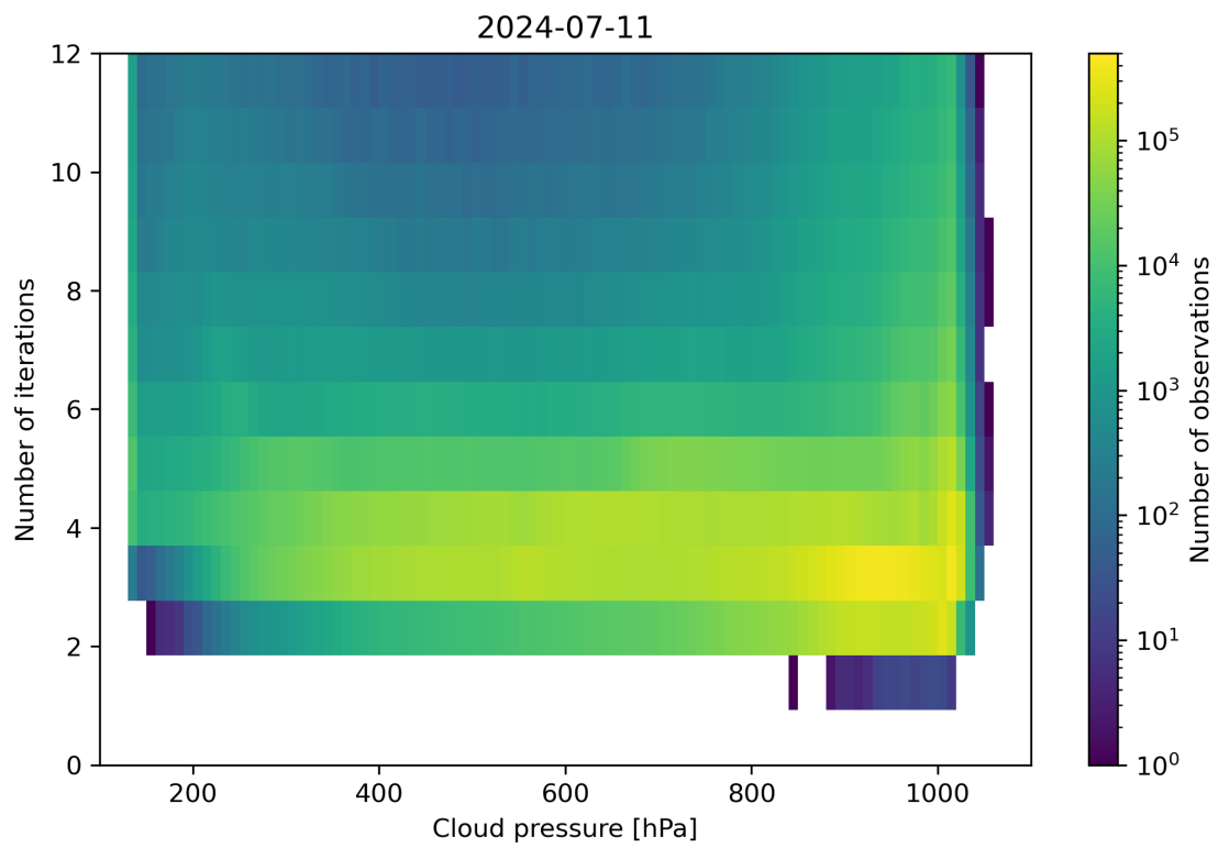
Figure 81: Scatter density plot of “Cloud pressure” against “Number of iterations” for 2024-07-10 to 2024-07-12.
