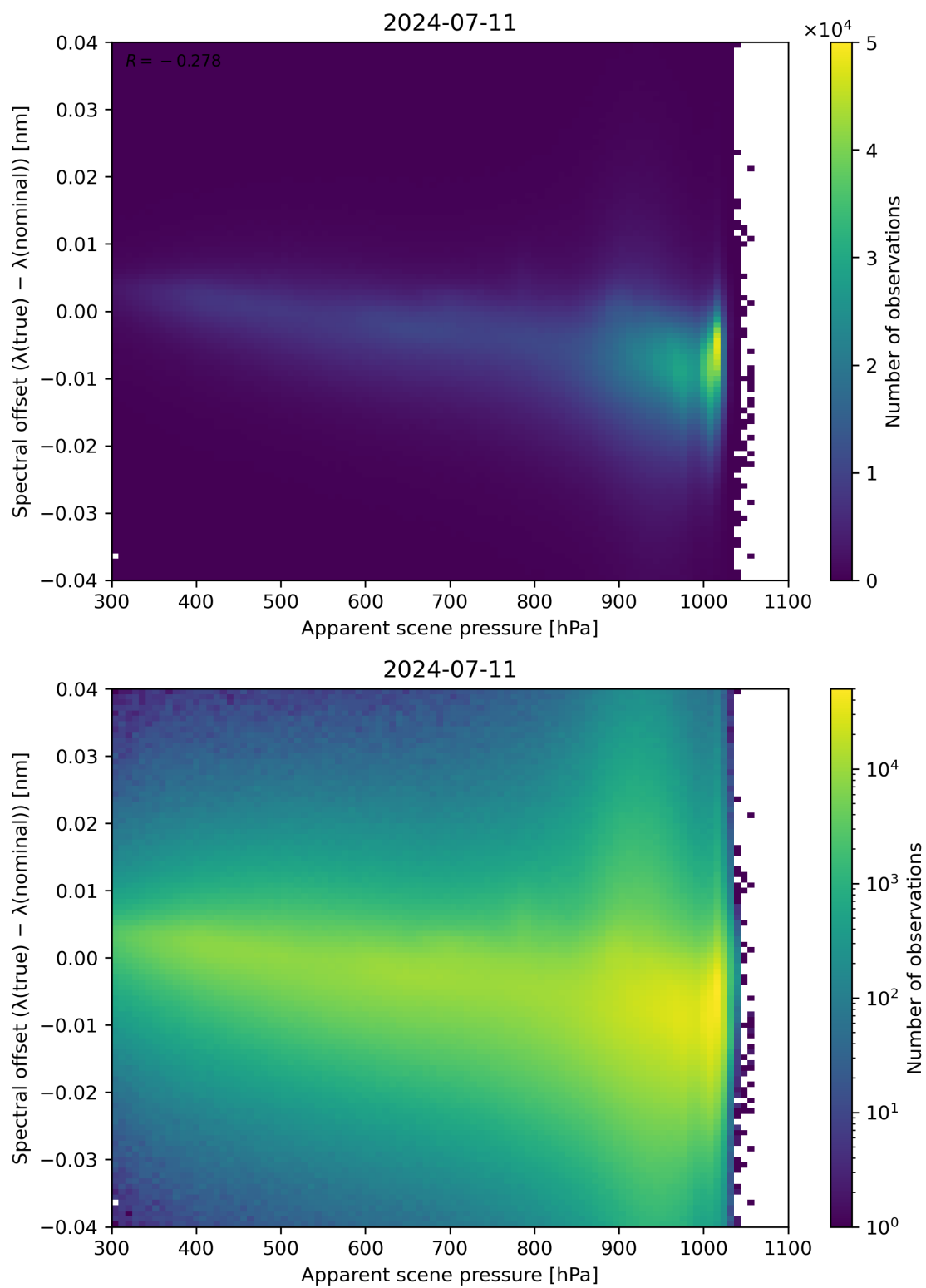
Figure 67: Scatter density plot of “Apparent scene pressure” against “Spectral offset ( \lambda(\text{true}) - \lambda(\text{nominal}) )” for 2024-07-10 to 2024-07-12.
