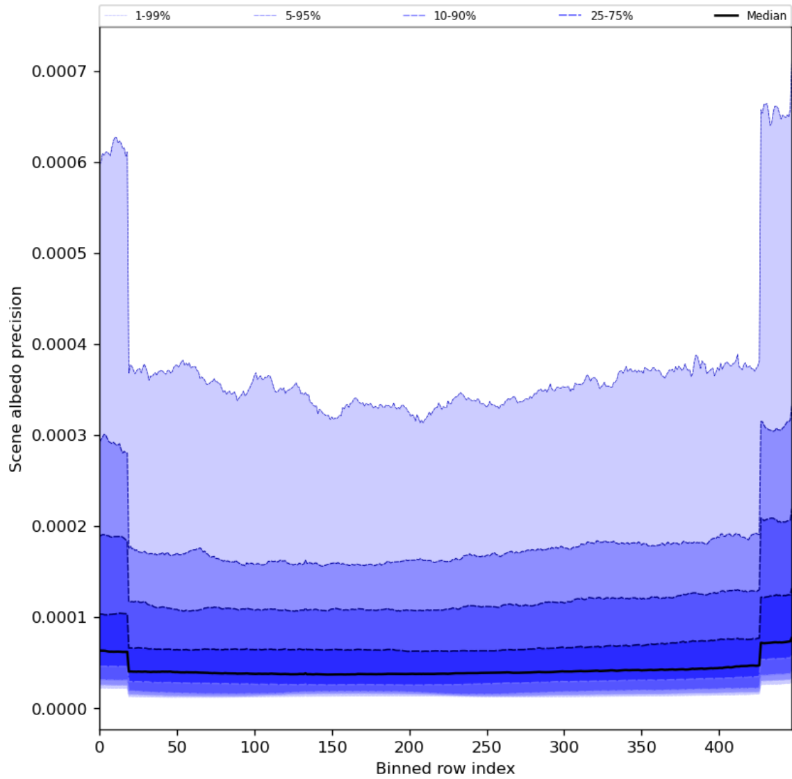
Figure 52: Along track statistics of “Scene albedo precision” for 2024-07-10 to 2024-07-12
