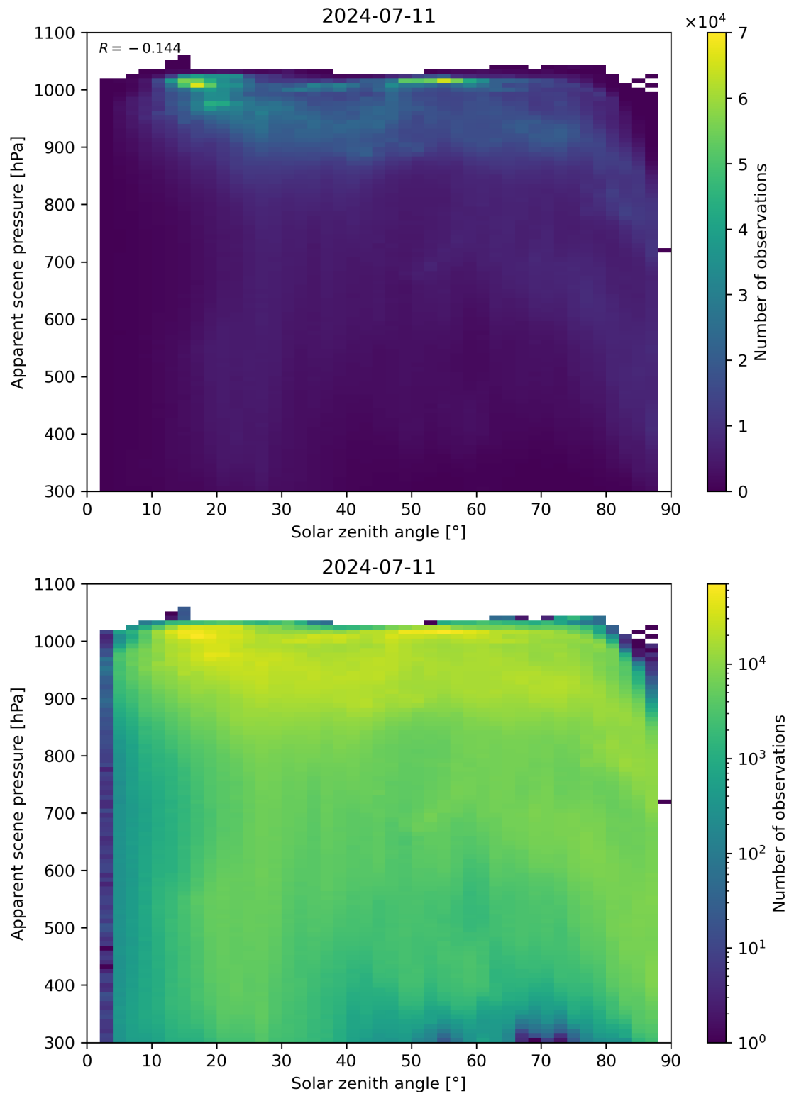
Figure 108: Scatter density plot of “Solar zenith angle” against “Apparent scene pressure” for 2024-07-10 to 2024-07-12.
