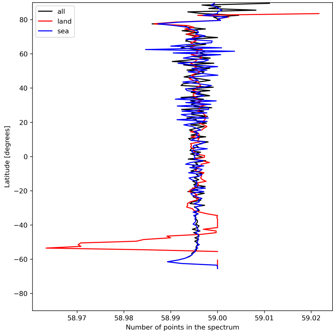
Figure 27: Zonal average of “Number of points in the spectrum” for 2024-07-10 to 2024-07-12.
