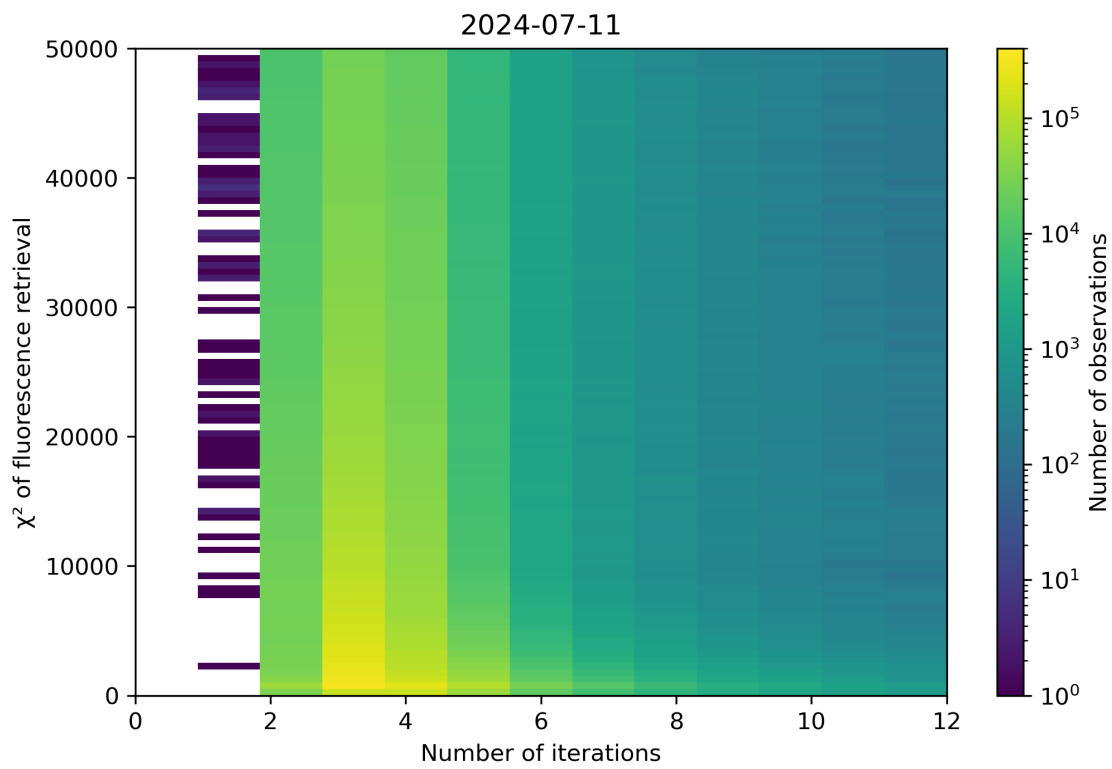
Figure 97: Scatter density plot of “Number of iterations” against “ \chi^2 of fluorescence retrieval” for 2024-07-10 to 2024-07-12.
