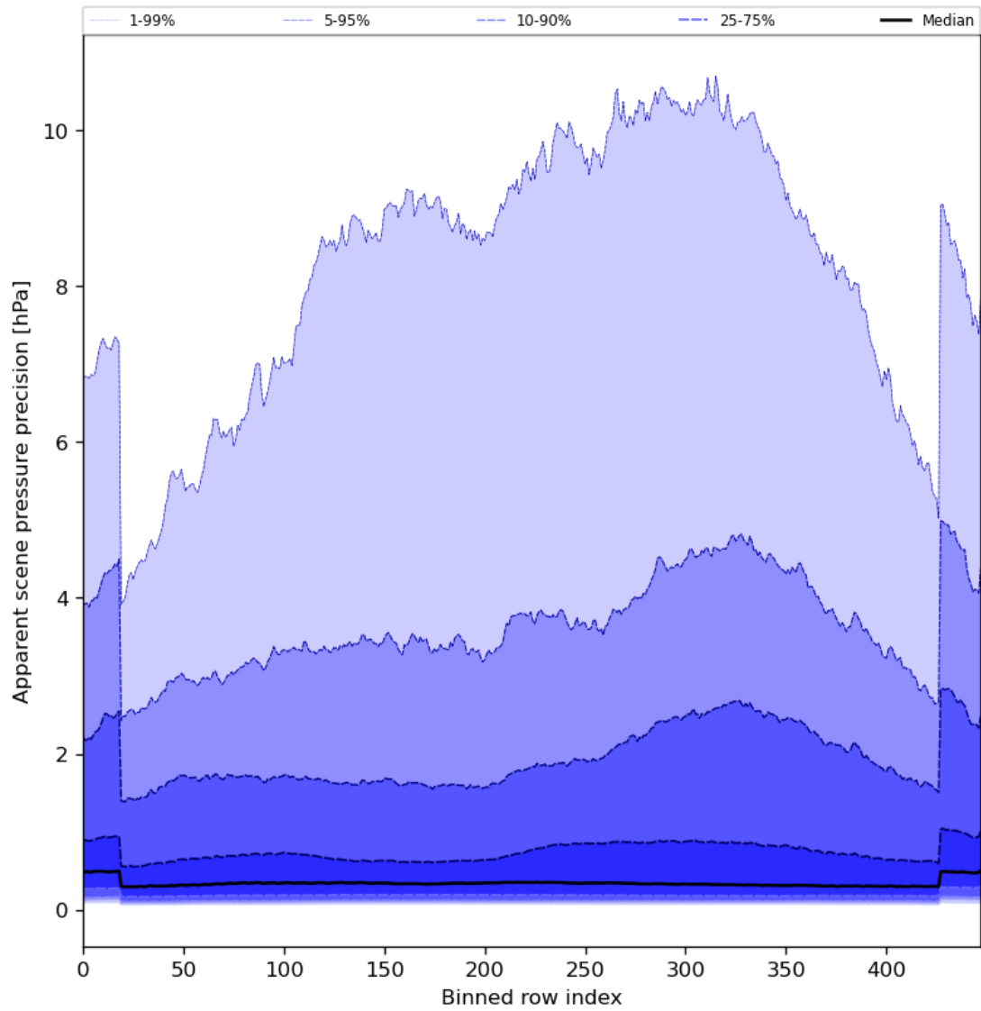
Figure 54: Along track statistics of “Apparent scene pressure precision” for 2024-07-10 to 2024-07-12
