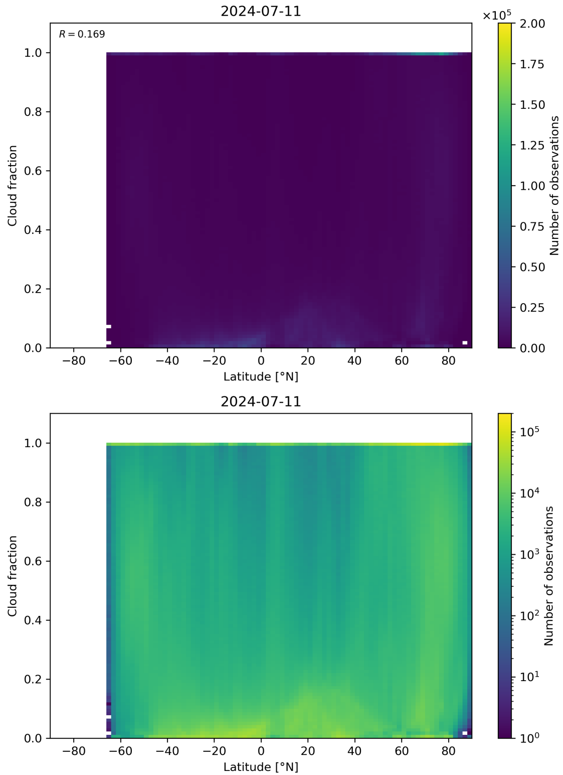
Figure 90: Scatter density plot of “Latitude” against “Cloud fraction” for 2024-07-10 to 2024-07-12.
