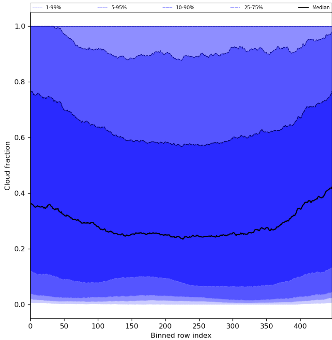
Figure 49: Along track statistics of “Cloud fraction” for 2024-07-10 to 2024-07-12
