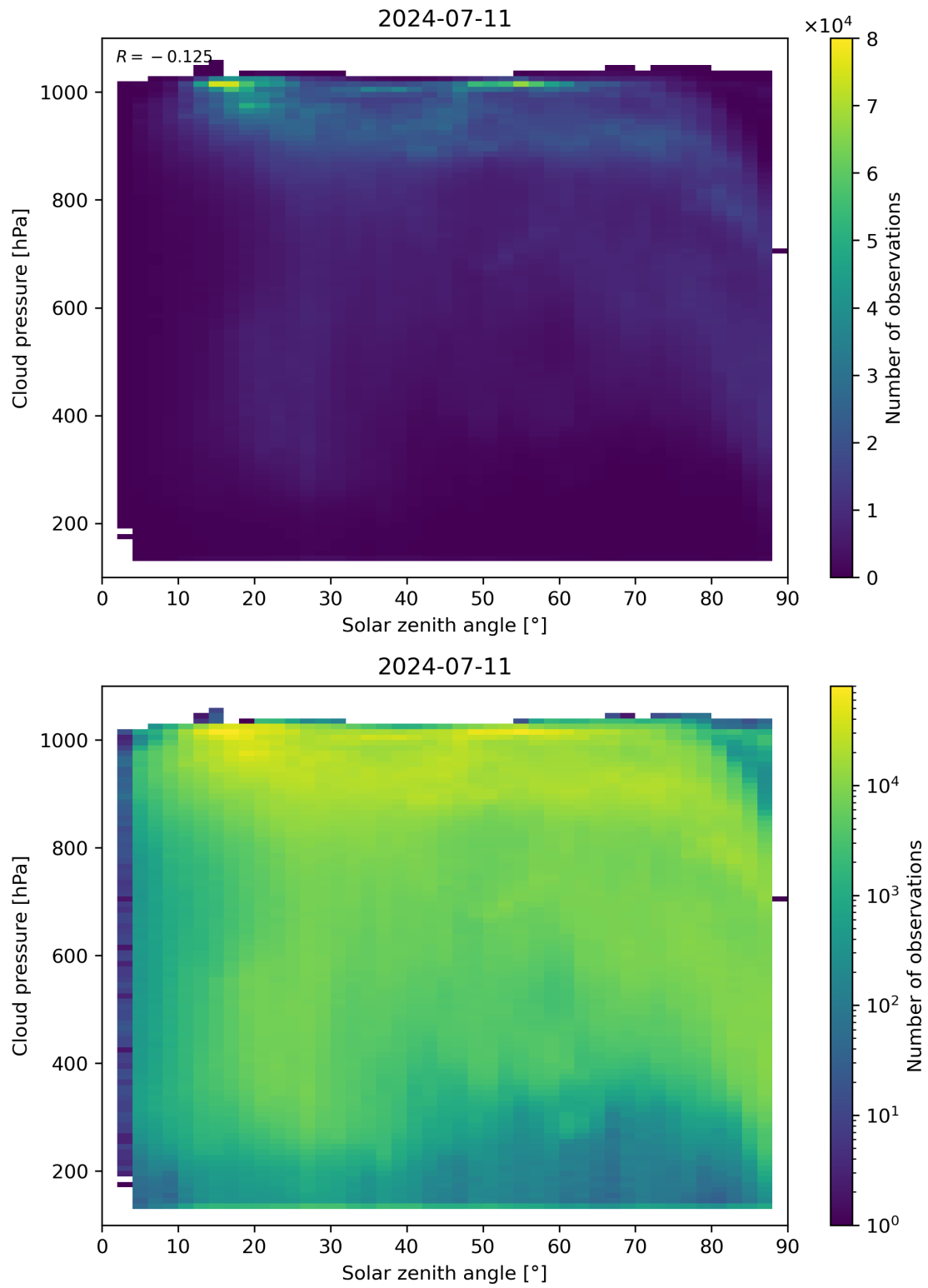
Figure 111: Scatter density plot of “Solar zenith angle” against “Cloud pressure” for 2024-07-10 to 2024-07-12.
