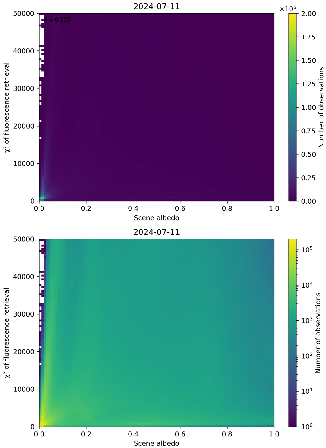
Figure 103: Scatter density plot of “Scene albedo” against “ \chi^2 of fluorescence retrieval” for 2024-07-10 to 2024-07-12.
