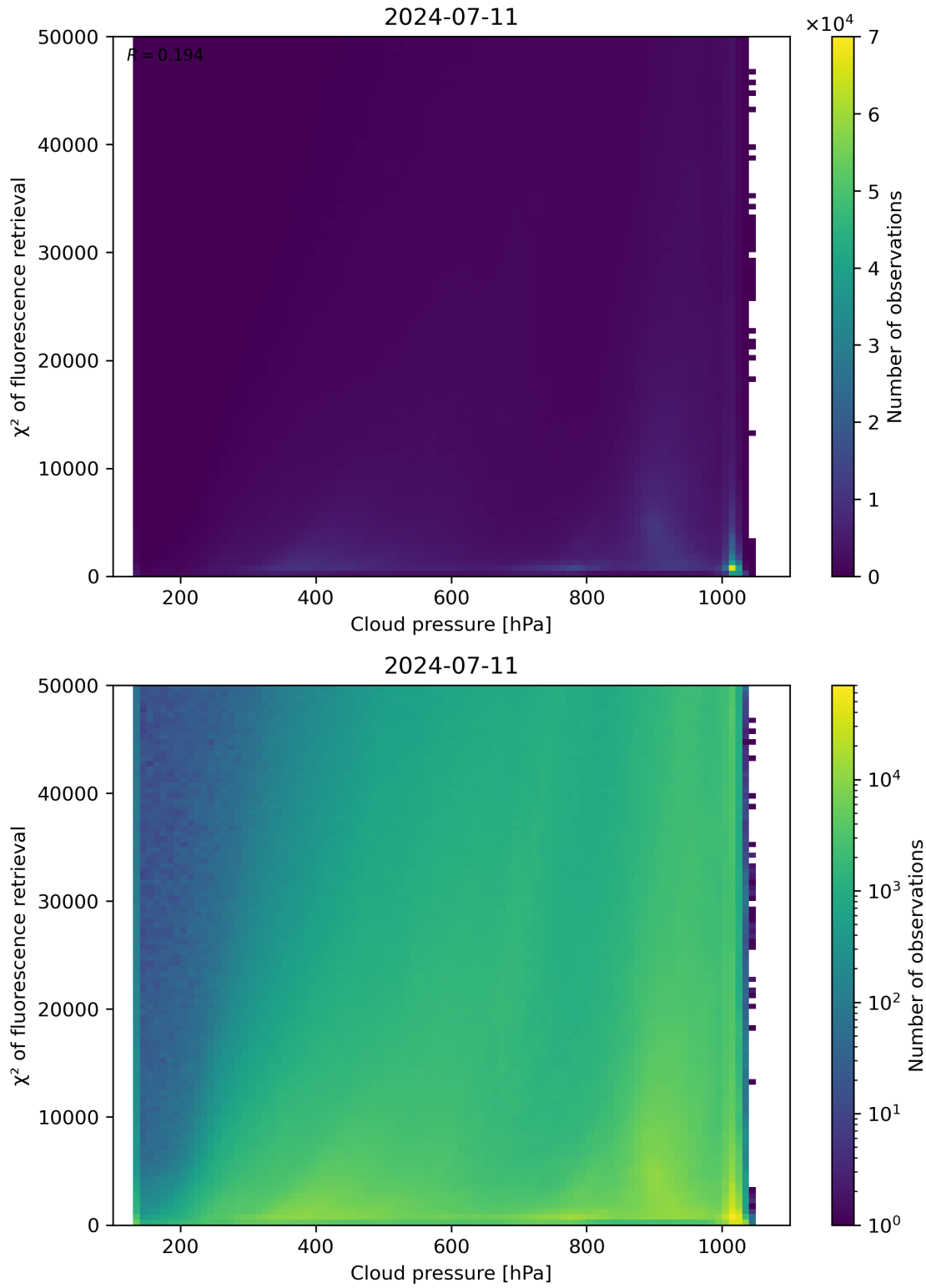
Figure 78: Scatter density plot of “Cloud pressure” against “ \chi^2 of fluorescence retrieval” for 2024-07-10 to 2024-07-12.
