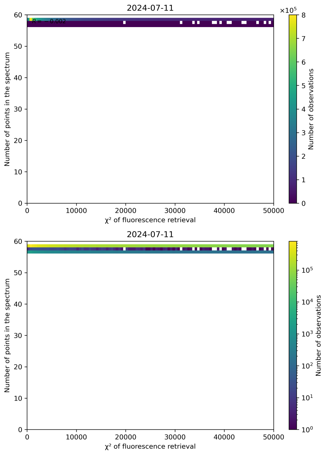
Figure 68: Scatter density plot of " \chi^2 of fluorescence retrieval" against "Number of points in the spectrum" for 2024-07-10 to 2024-07-12.
