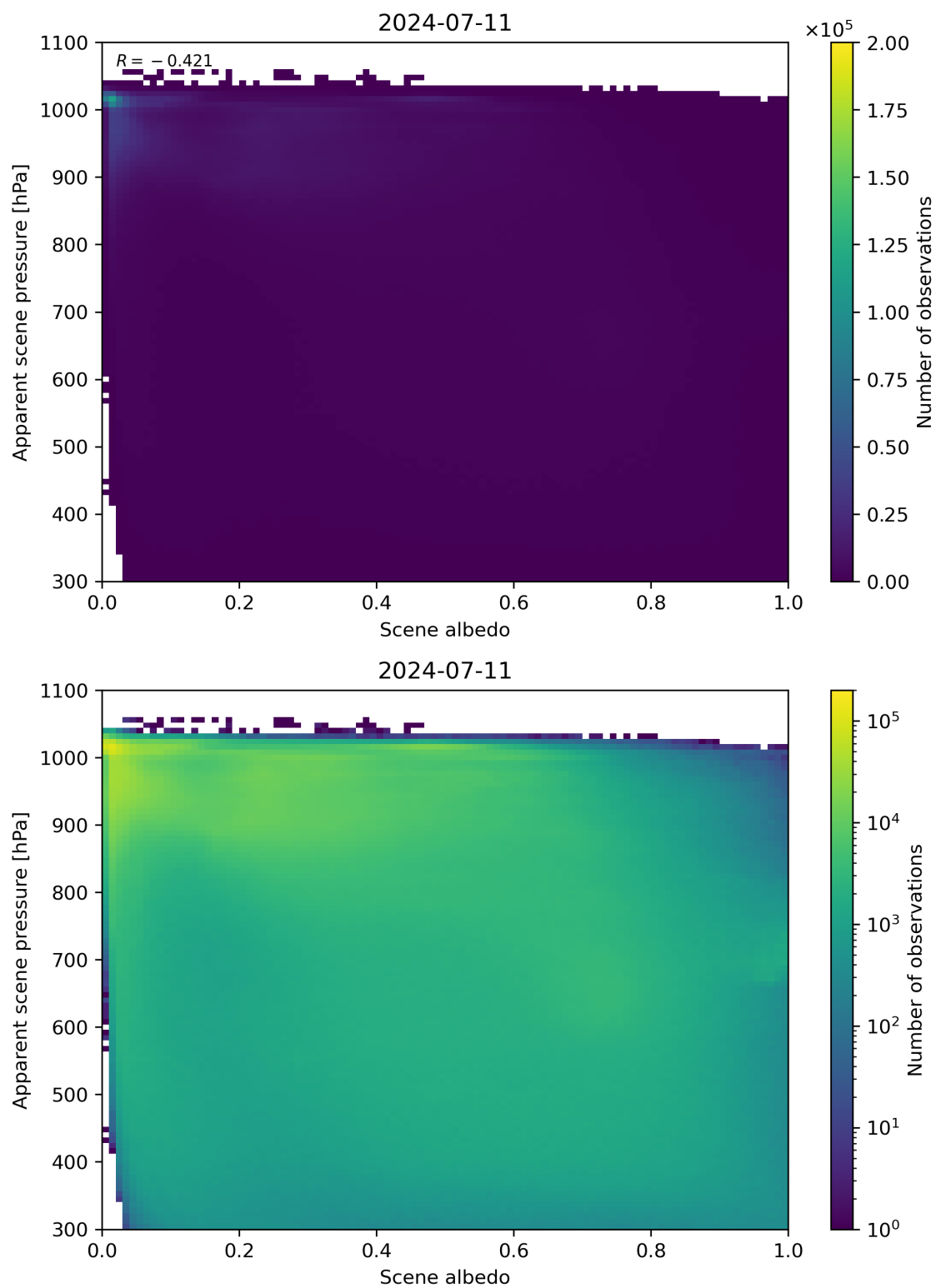
Figure 102: Scatter density plot of “Scene albedo” against “Apparent scene pressure” for 2024-07-10 to 2024-07-12.
