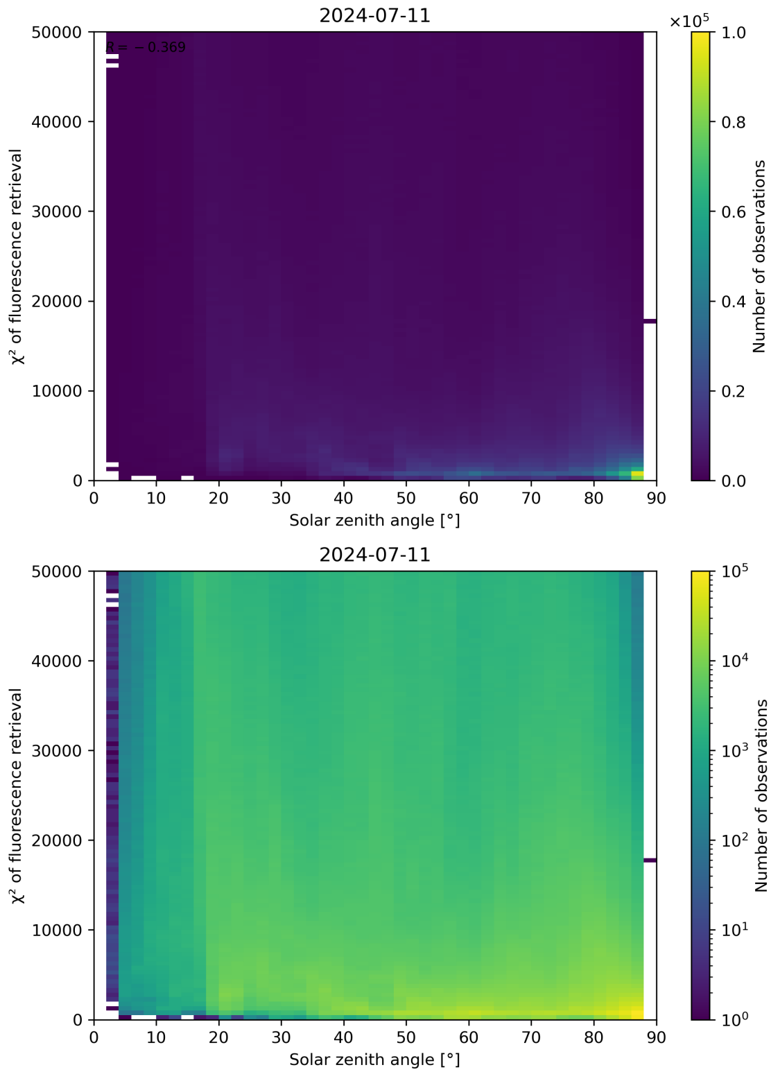
Figure 109: Scatter density plot of “Solar zenith angle” against “ \chi^2 of fluorescence retrieval” for 2024-07-10 to 2024-07-12.
