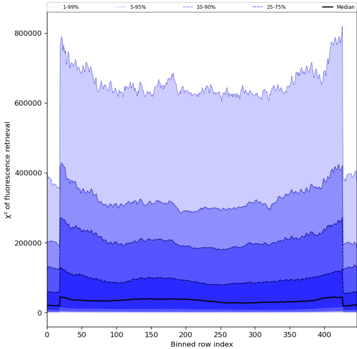
Figure 59: Along track statistics of “ \chi^2 of fluorescence retrieval” for 2024-07-10 to 2024-07-12
