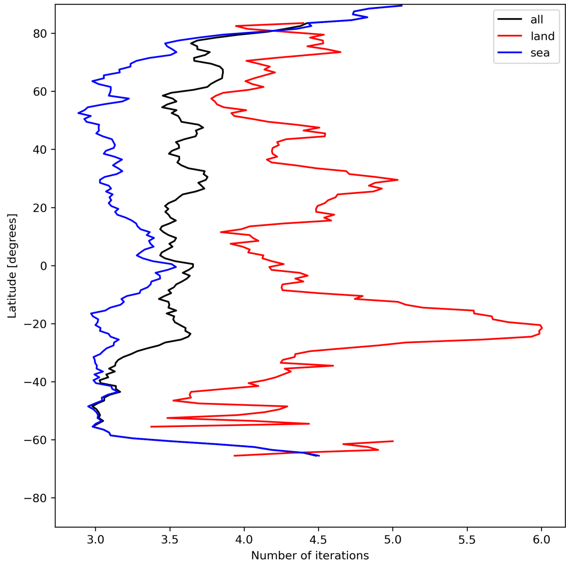
Figure 22: Zonal average of “Number of iterations” for 2024-07-10 to 2024-07-12.
