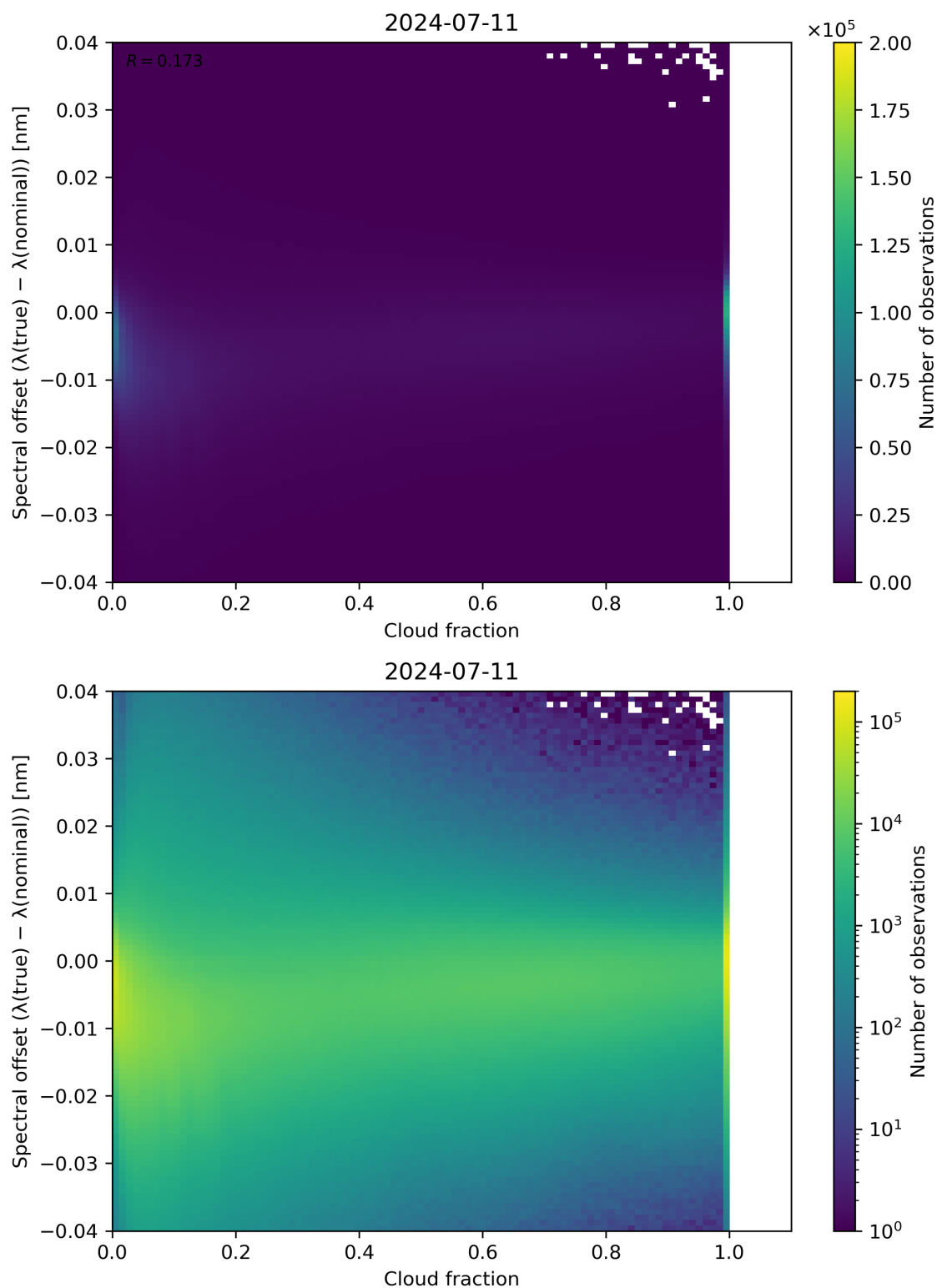
Figure 76: Scatter density plot of “Cloud fraction” against “Spectral offset ( \lambda(\text{true}) - \lambda(\text{nominal}) )” for 2024-07-10 to 2024-07-12.
