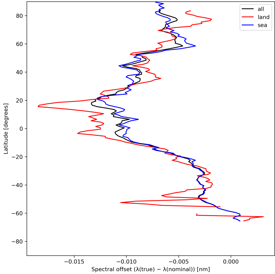
Figure 28: Zonal average of “Spectral offset ( \lambda(\text{true}) - \lambda(\text{nominal}) )” for 2024-07-10 to 2024-07-12.
