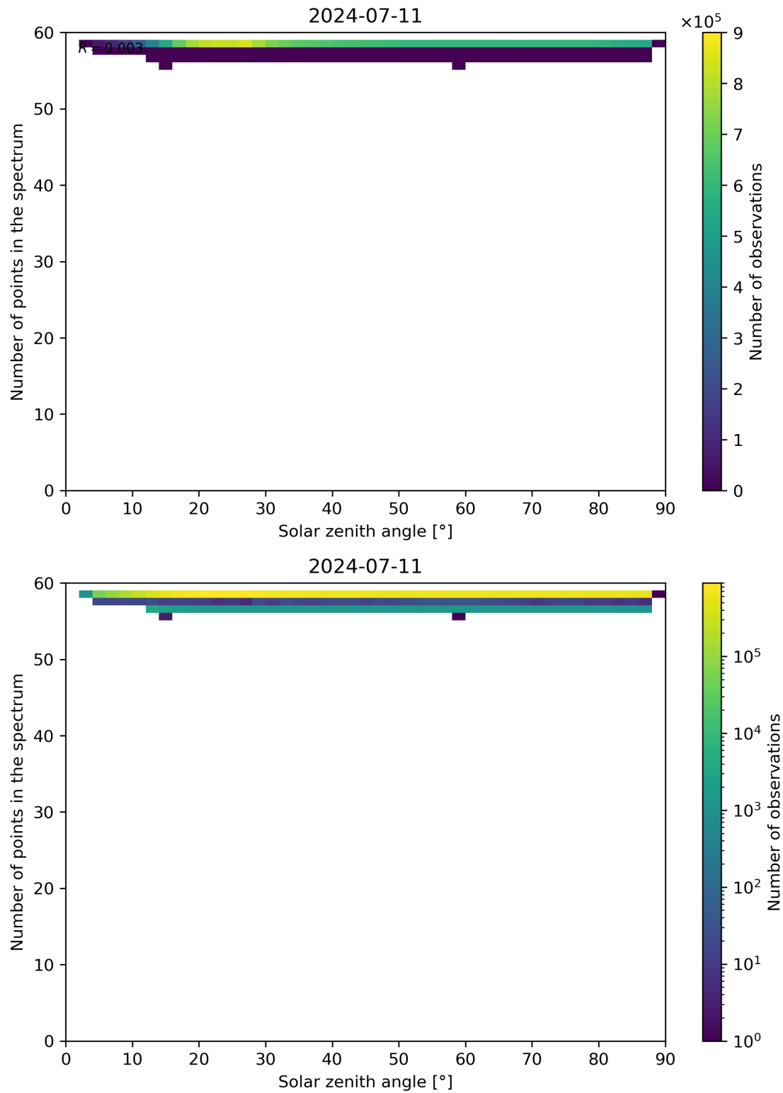
Figure 115: Scatter density plot of “Solar zenith angle” against “Number of points in the spectrum” for 2024-07-10 to 2024-07-12.
