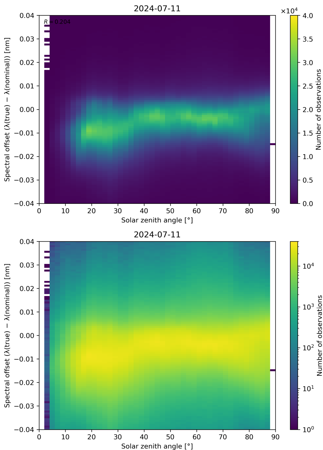
Figure 117: Scatter density plot of “Solar zenith angle” against “Spectral offset ( \lambda(\text{true}) - \lambda(\text{nominal}) )” for 2024-07-10 to 2024-07-12.
