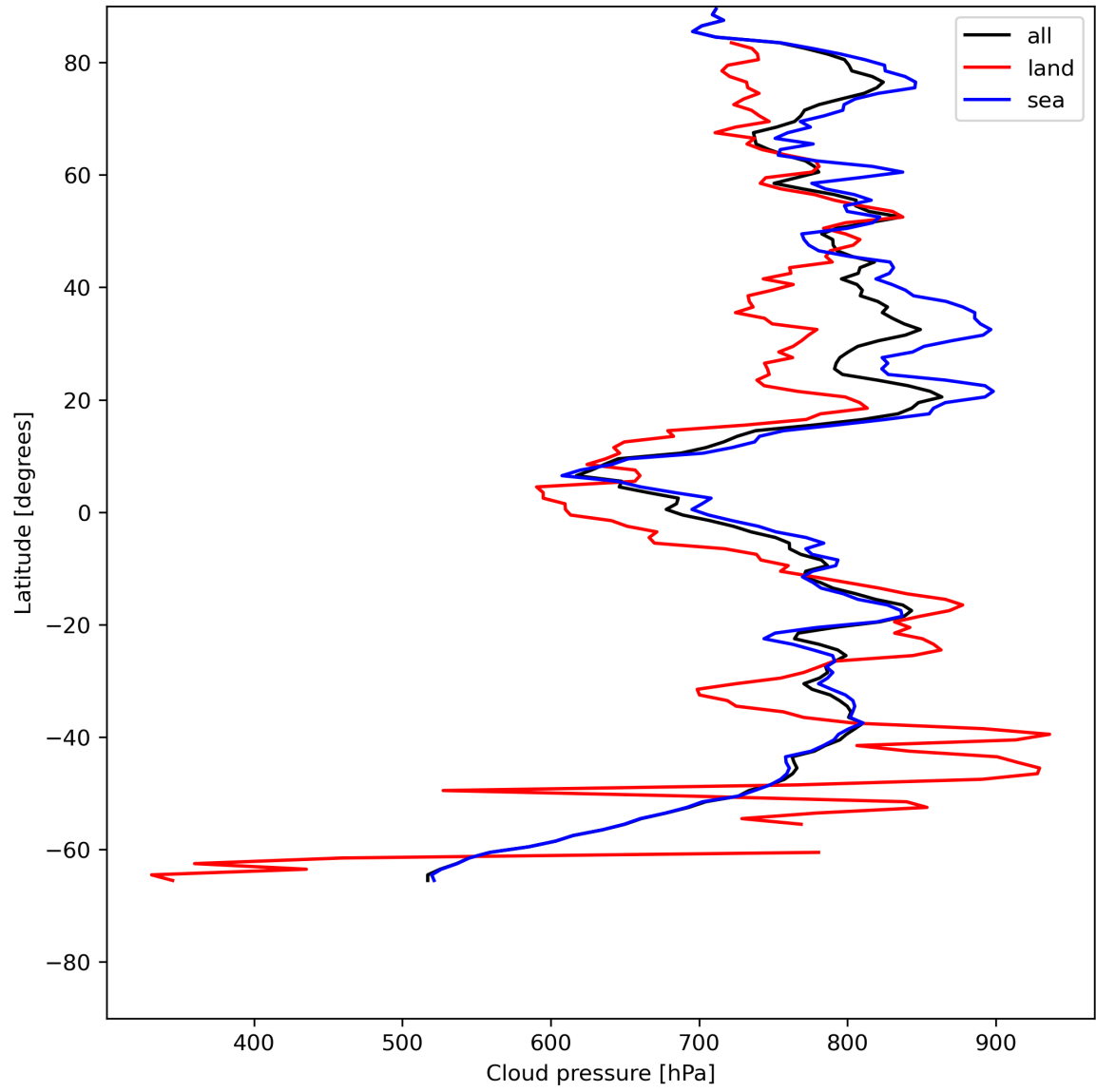
Figure 13: Zonal average of “Cloud pressure” for 2024-07-10 to 2024-07-12.
