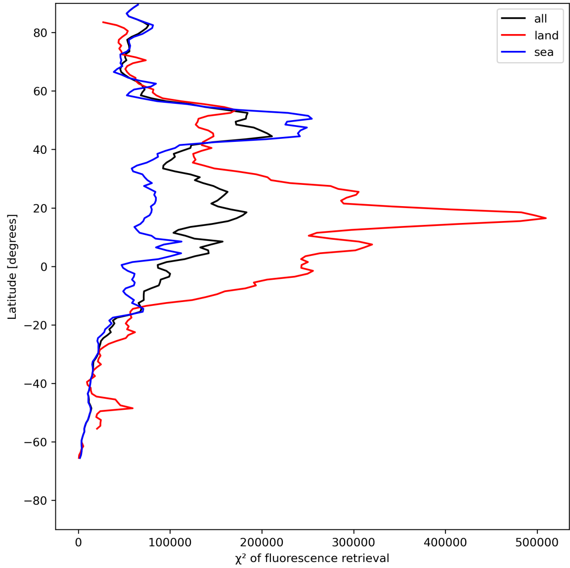
Figure 25: Zonal average of “ \chi^2 of fluorescence retrieval” for 2024-07-10 to 2024-07-12.
