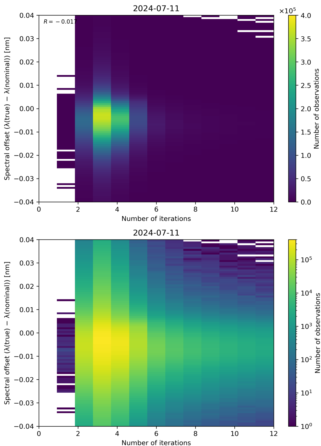
Figure 100: Scatter density plot of “Number of iterations” against “Spectral offset ( \lambda(\text{true}) - \lambda(\text{nominal}) )” for 2024-07-10 to 2024-07-12.
