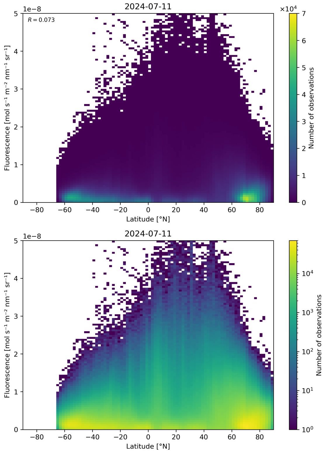
Figure 92: Scatter density plot of “Latitude” against “Fluorescence” for 2024-07-10 to 2024-07-12.
