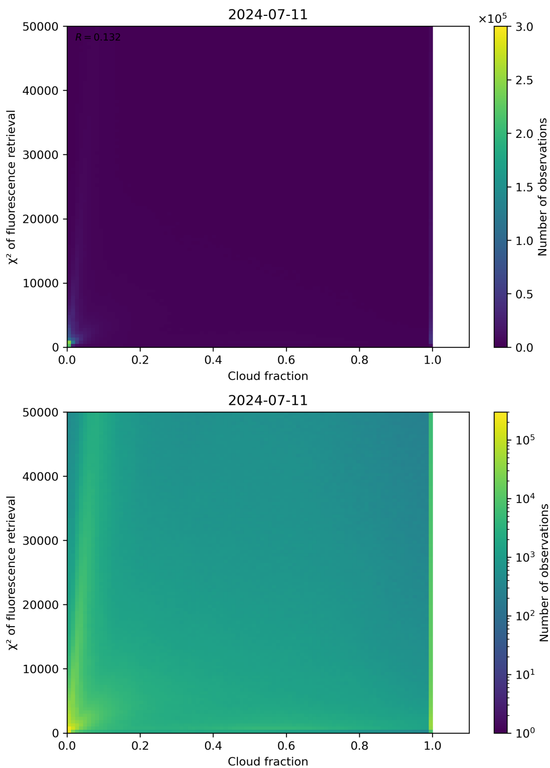
Figure 71: Scatter density plot of “Cloud fraction” against “ \chi^2 of fluorescence retrieval” for 2024-07-10 to 2024-07-12.
