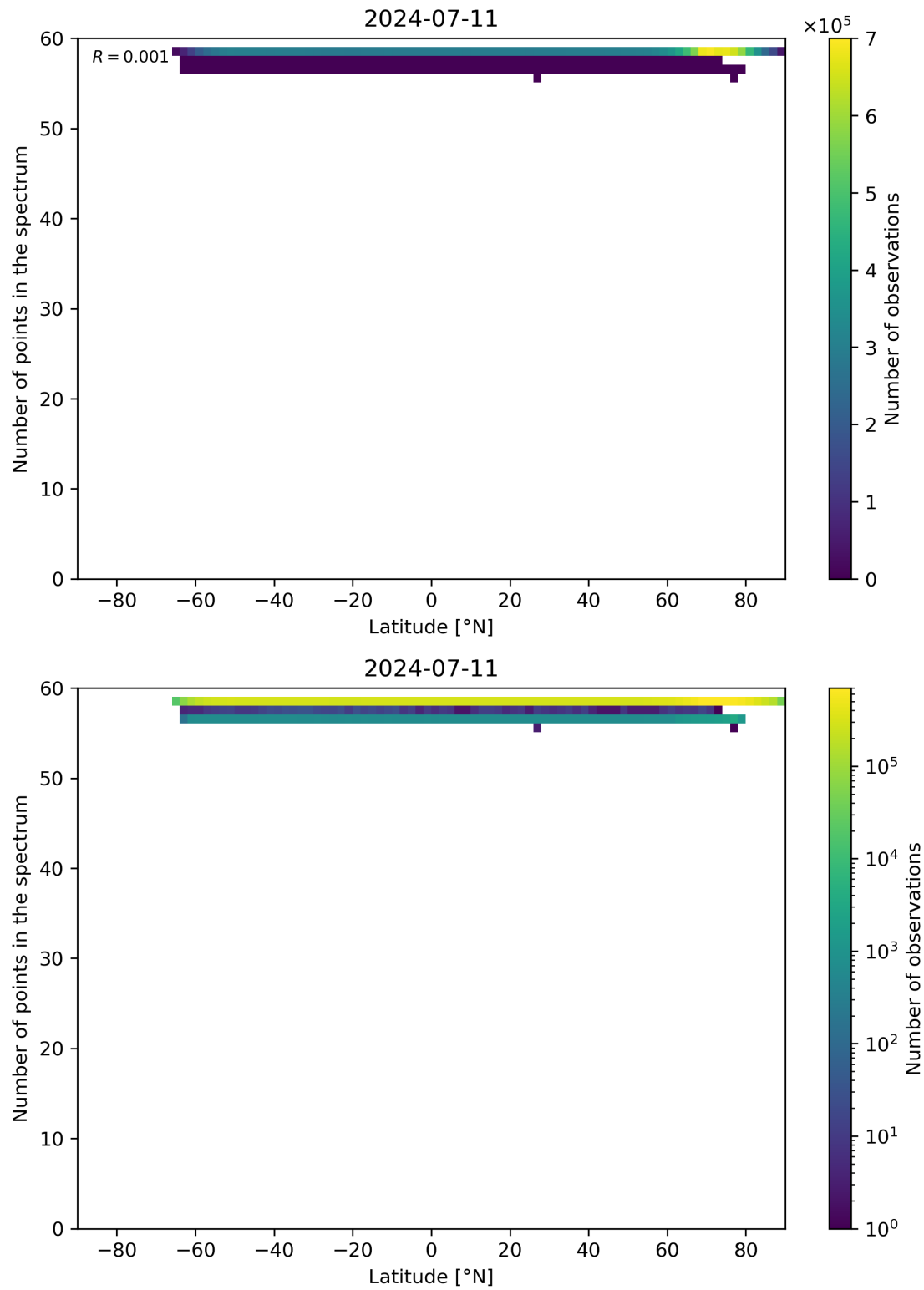
Figure 94: Scatter density plot of “Latitude” against “Number of points in the spectrum” for 2024-07-10 to 2024-07-12.
