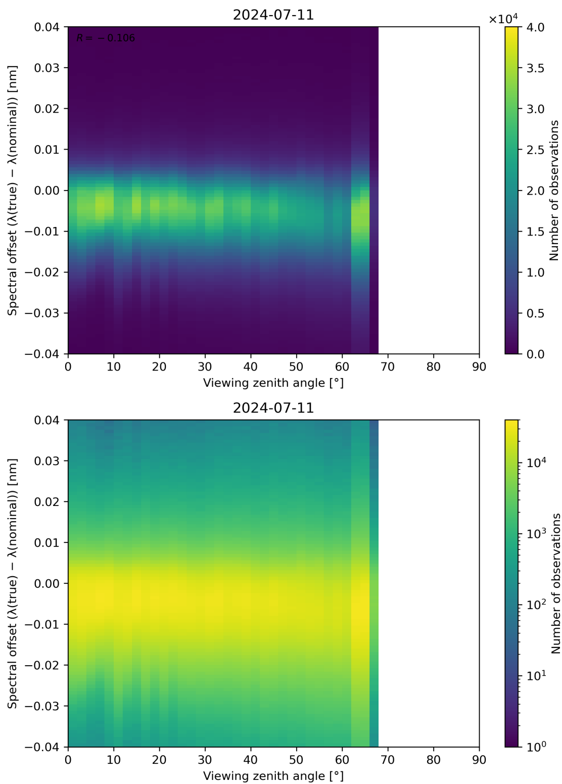
Figure 128: Scatter density plot of “Viewing zenith angle” against “Spectral offset ( \lambda(\text{true}) - \lambda(\text{nominal}) )” for 2024-07-10 to 2024-07-12.
