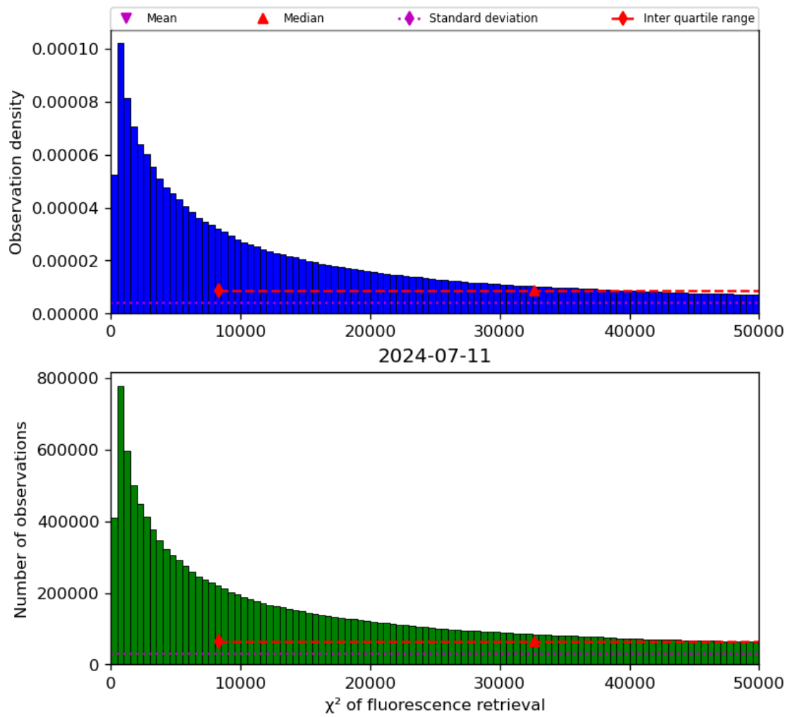
Figure 42: Histogram of “ \chi^2 of fluorescence retrieval” for 2024-07-10 to 2024-07-12
