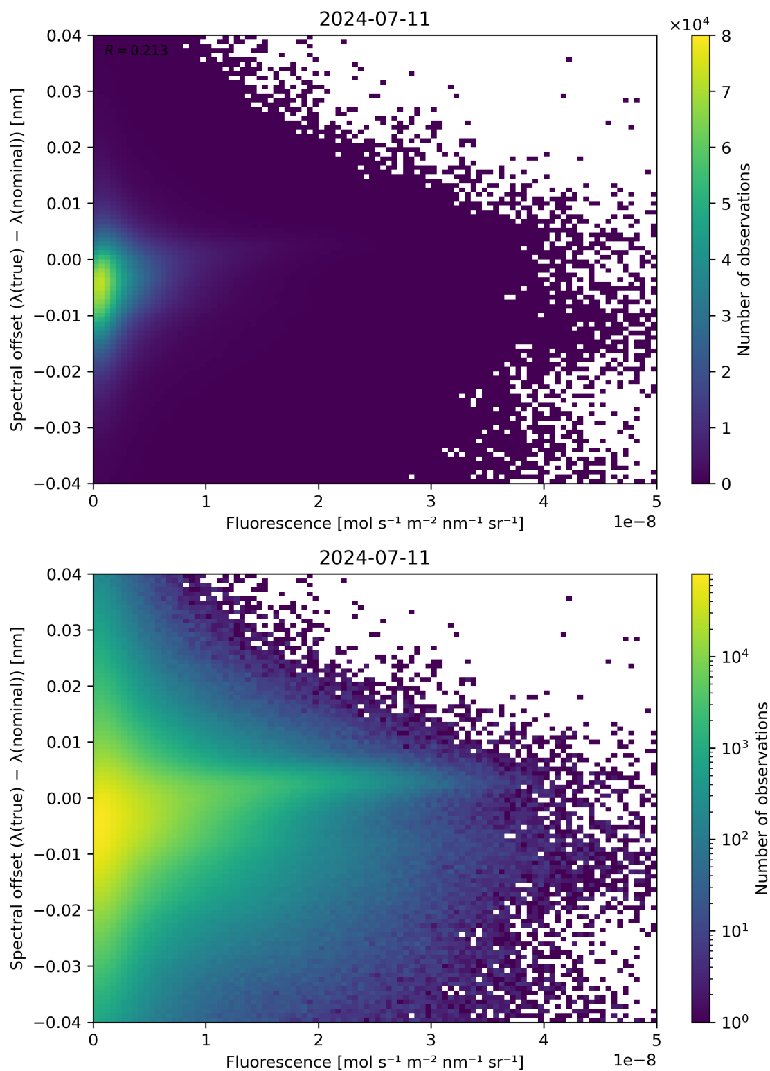
Figure 87: Scatter density plot of “Fluorescence” against “Spectral offset ( \lambda(\text{true}) - \lambda(\text{nominal}) )” for 2024-07-10 to 2024-07-12.
