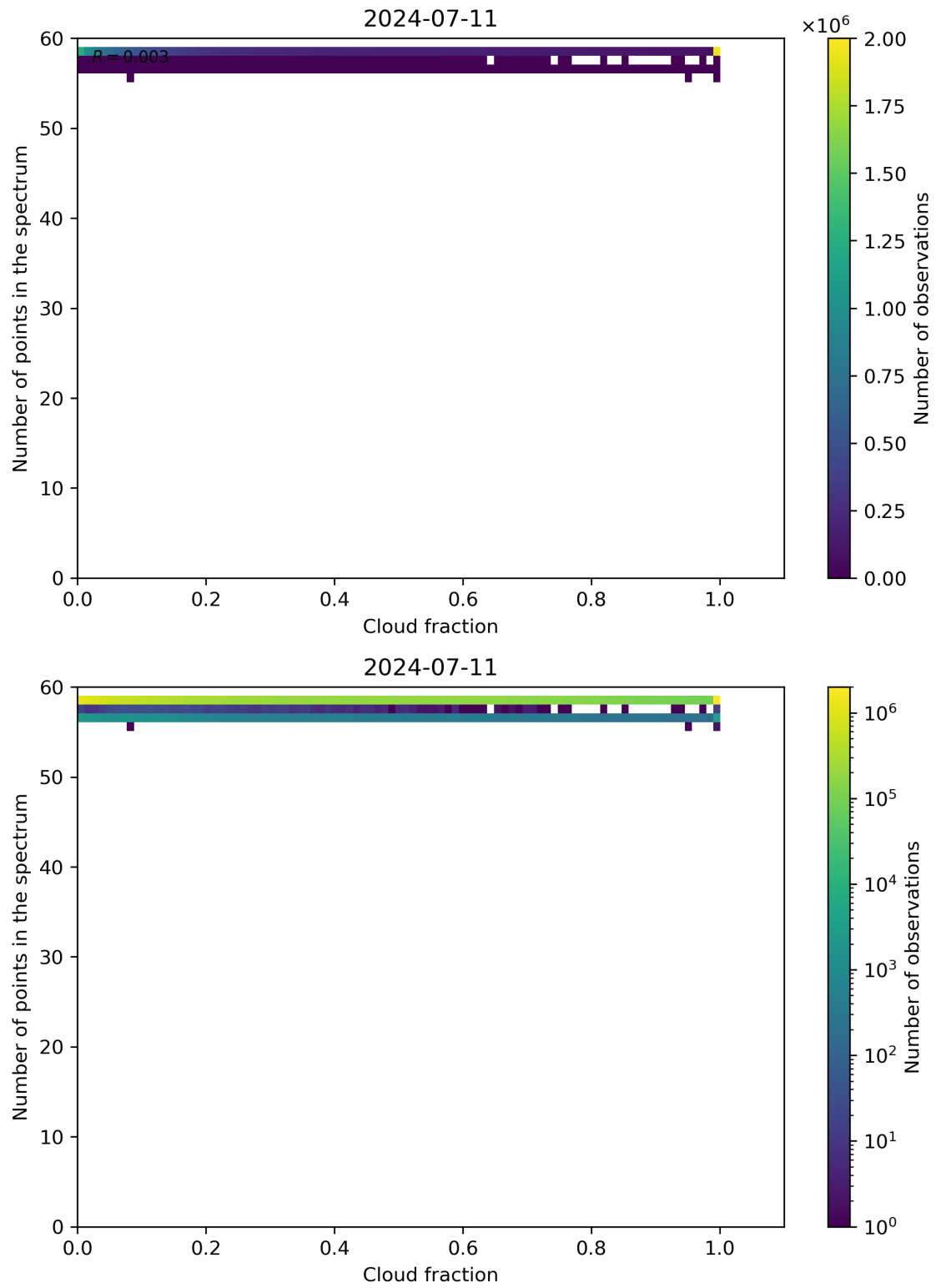
Figure 74: Scatter density plot of “Cloud fraction” against “Number of points in the spectrum” for 2024-07-10 to 2024-07-12.
