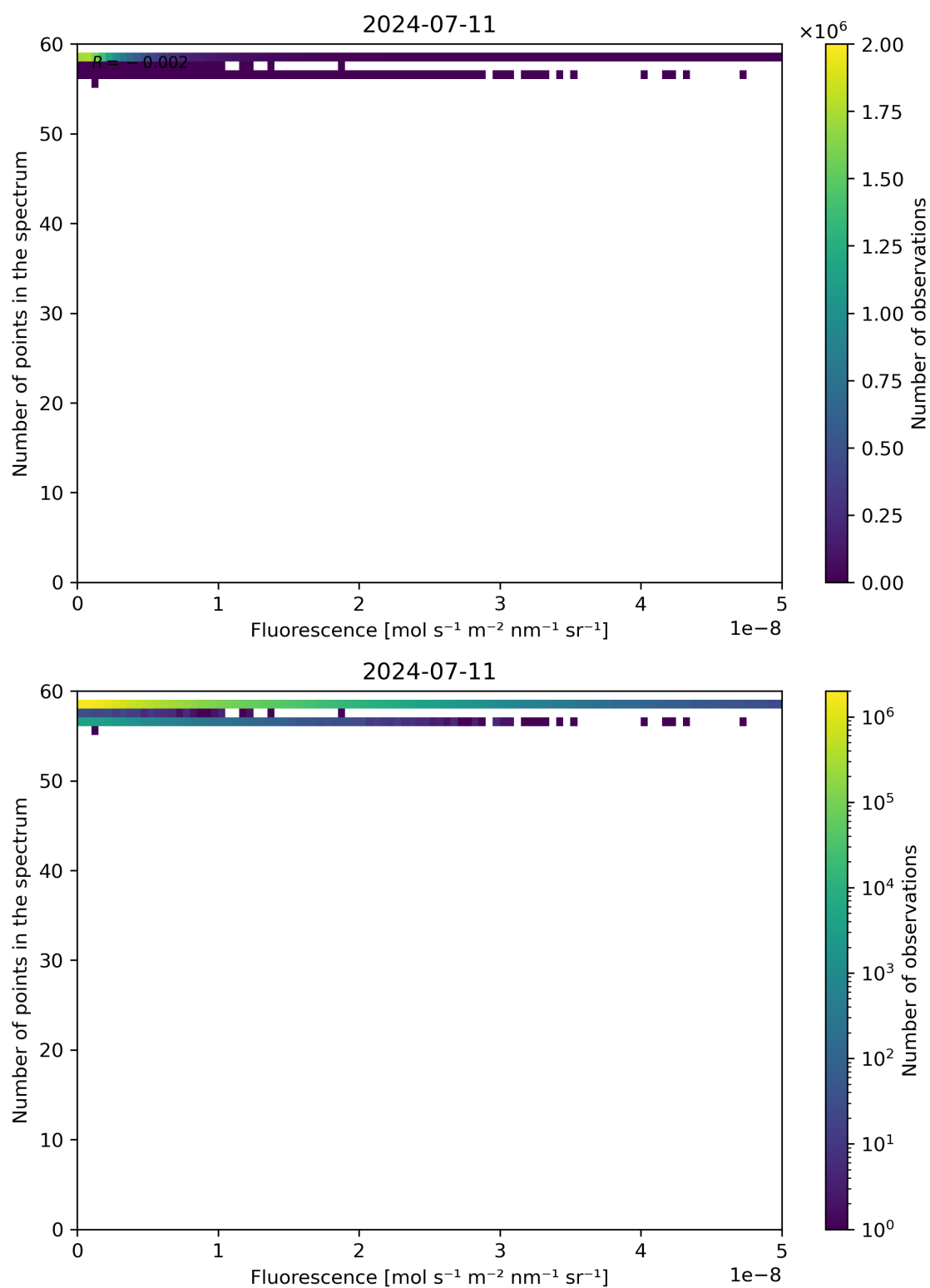
Figure 86: Scatter density plot of “Fluorescence” against “Number of points in the spectrum” for 2024-07-10 to 2024-07-12.
