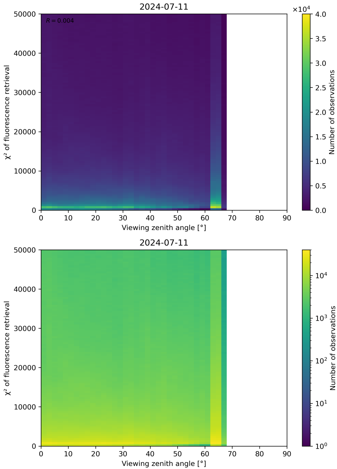
Figure 119: Scatter density plot of “Viewing zenith angle” against “ \chi^2 of fluorescence retrieval” for 2024-07-10 to 2024-07-12.
