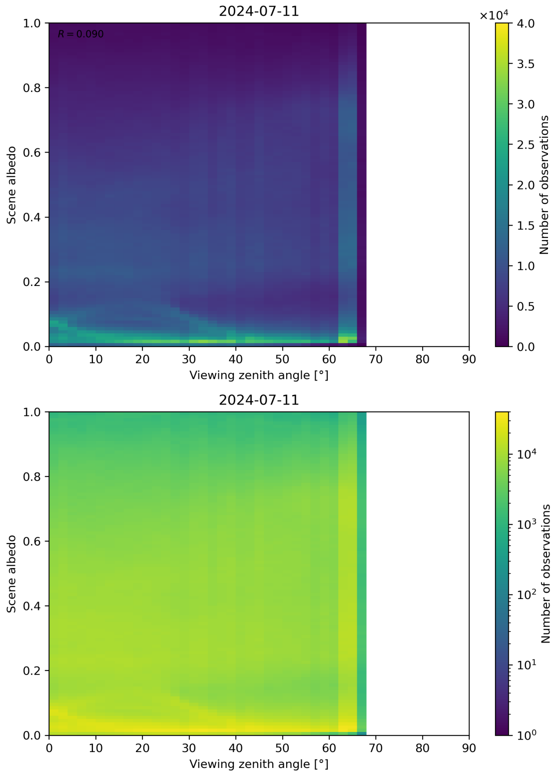
Figure 126: Scatter density plot of “Viewing zenith angle” against “Scene albedo” for 2024-07-10 to 2024-07-12.
