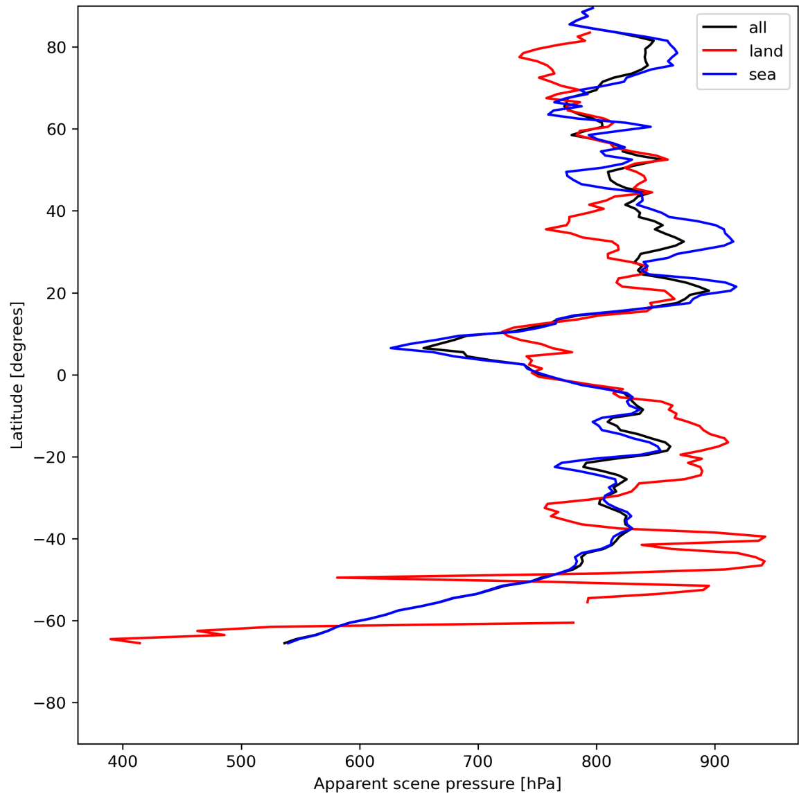
Figure 19: Zonal average of “Apparent scene pressure” for 2024-07-10 to 2024-07-12.
