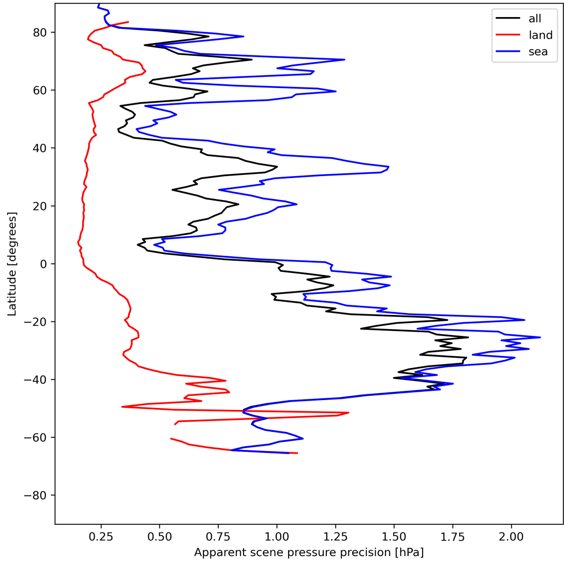
Figure 20: Zonal average of “Apparent scene pressure precision” for 2024-07-10 to 2024-07-12.
