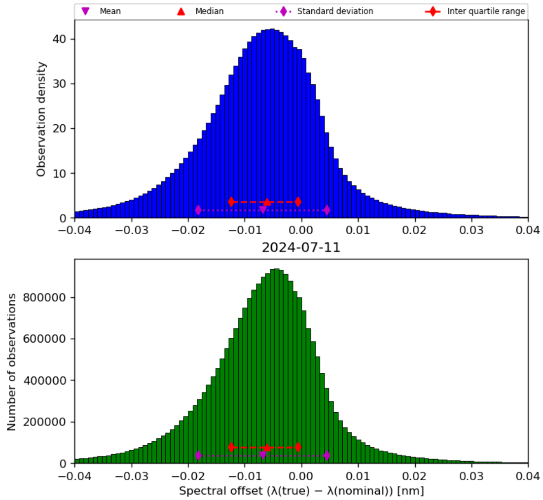
Figure 45: Histogram of “Spectral offset ( \lambda(\text{true}) - \lambda(\text{nominal}) )” for 2024-07-10 to 2024-07-12
