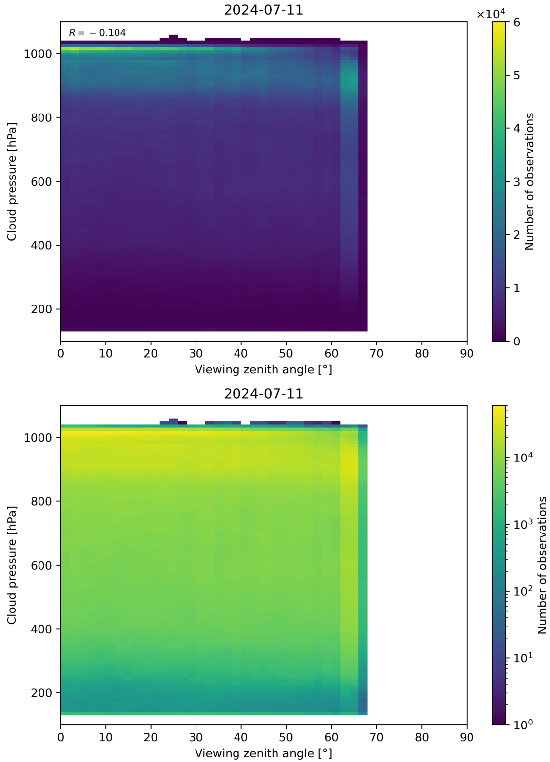
Figure 121: Scatter density plot of “Viewing zenith angle” against “Cloud pressure” for 2024-07-10 to 2024-07-12.
