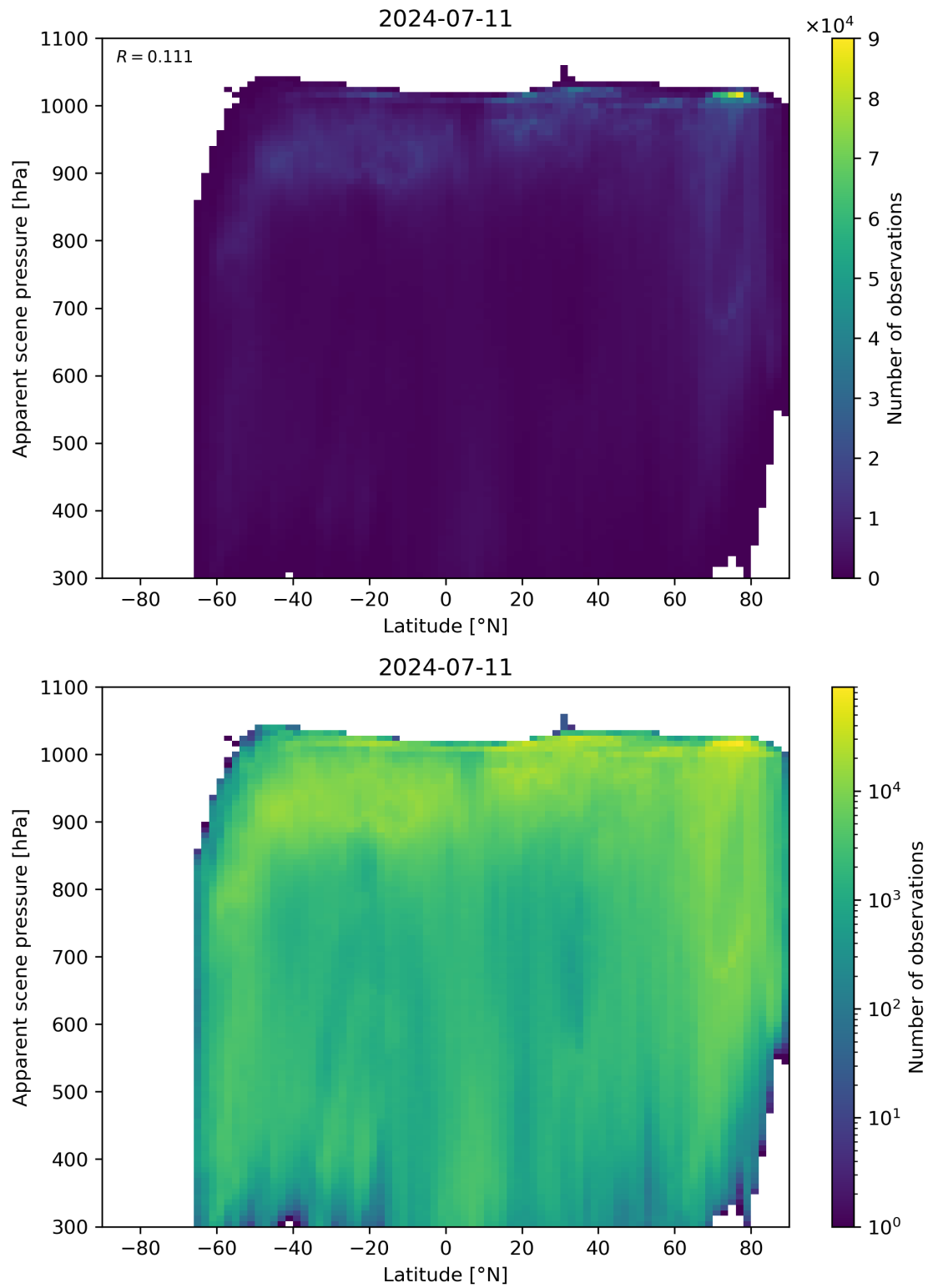
Figure 88: Scatter density plot of “Latitude” against “Apparent scene pressure” for 2024-07-10 to 2024-07-12.
