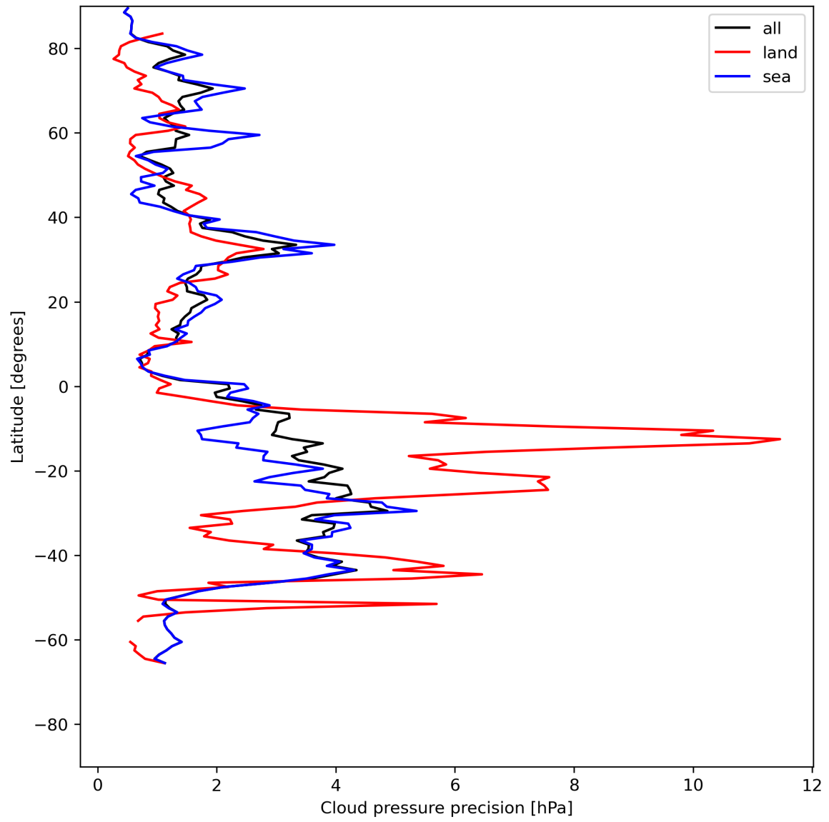
Figure 14: Zonal average of “Cloud pressure precision” for 2024-07-10 to 2024-07-12.
