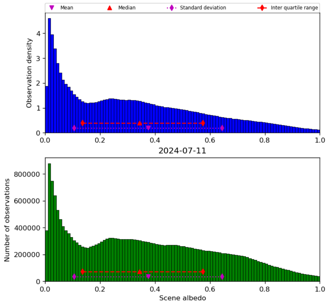
Figure 34: Histogram of “Scene albedo” for 2024-07-10 to 2024-07-12
