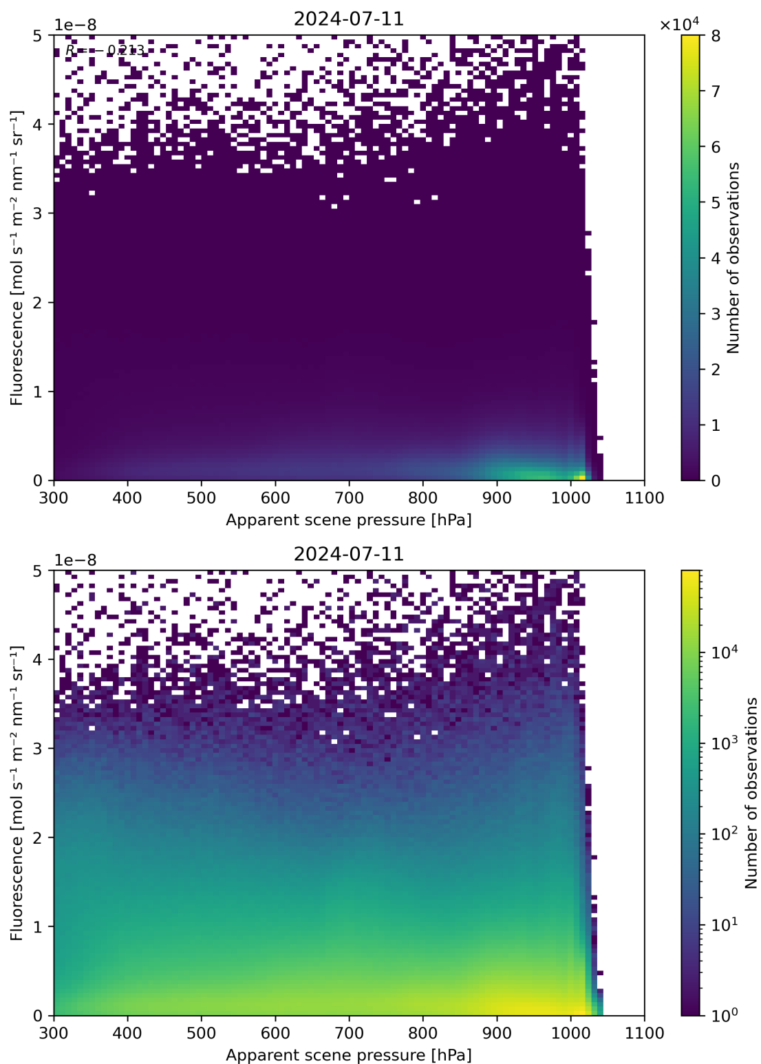
Figure 64: Scatter density plot of “Apparent scene pressure” against “Fluorescence” for 2024-07-10 to 2024-07-12.
