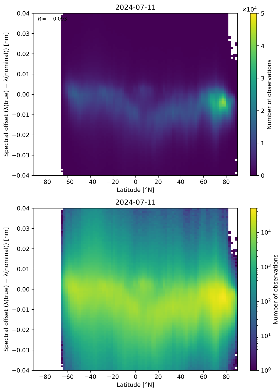
Figure 96: Scatter density plot of “Latitude” against “Spectral offset ( \lambda(\text{true}) - \lambda(\text{nominal}) )” for 2024-07-10 to 2024-07-12.
