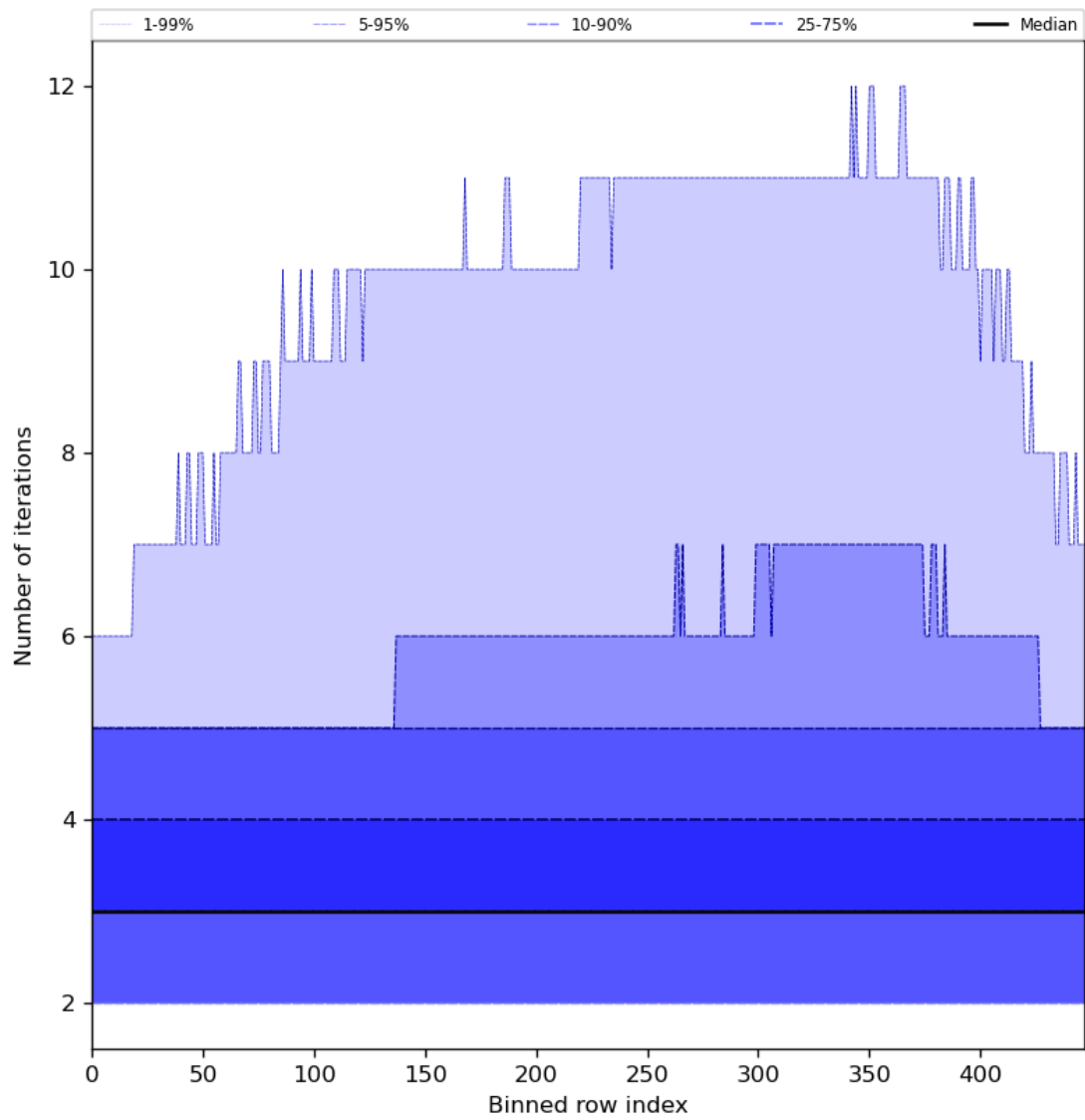
Figure 56: Along track statistics of “Number of iterations” for 2024-07-11 to 2024-07-13
