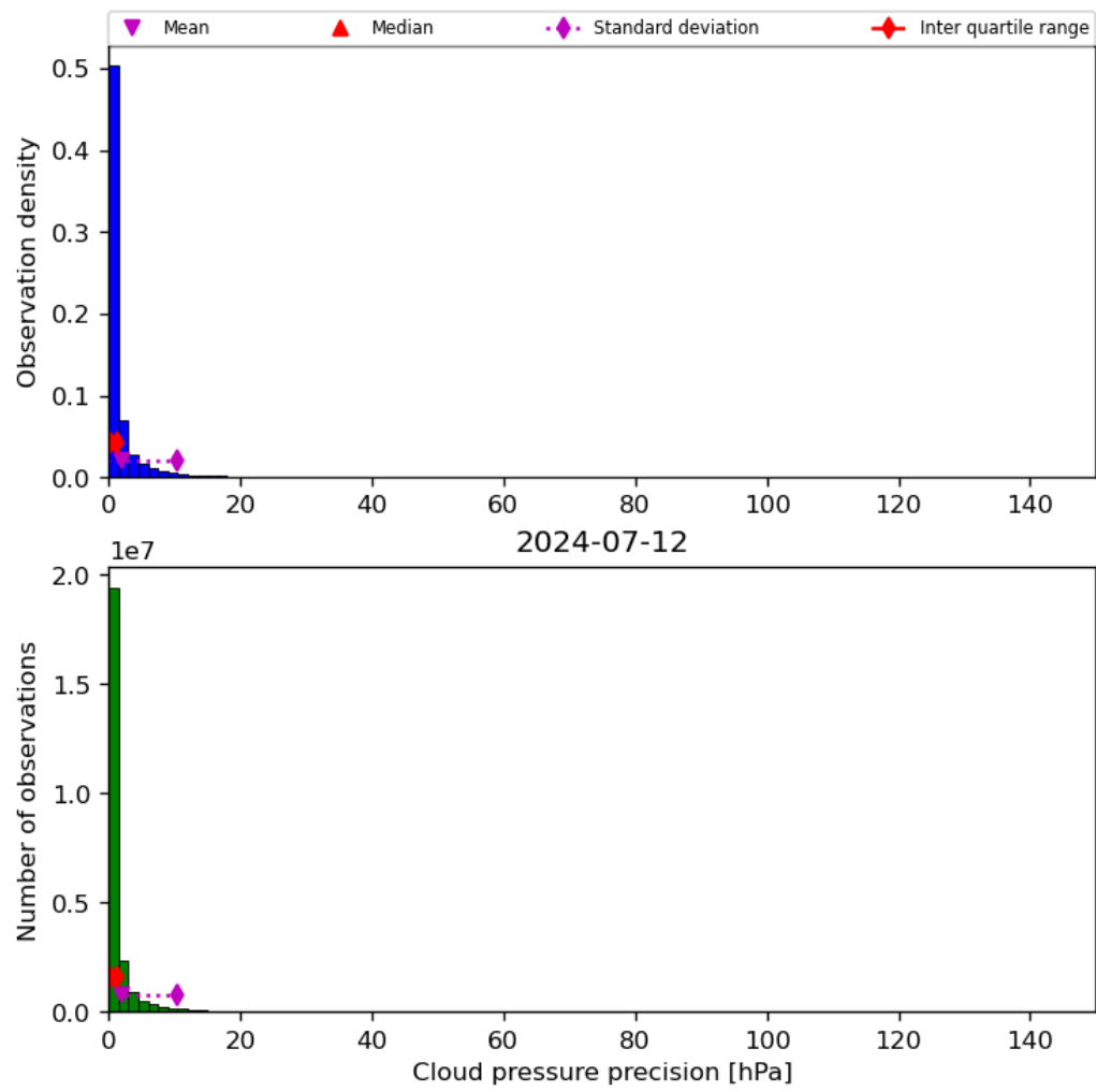
Figure 31: Histogram of “Cloud pressure precision” for 2024-07-11 to 2024-07-13
