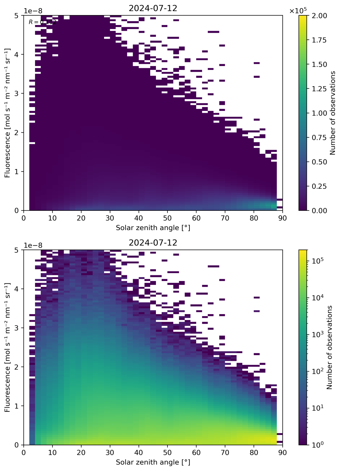
Figure 112: Scatter density plot of “Solar zenith angle” against “Fluorescence” for 2024-07-11 to 2024-07-13.
