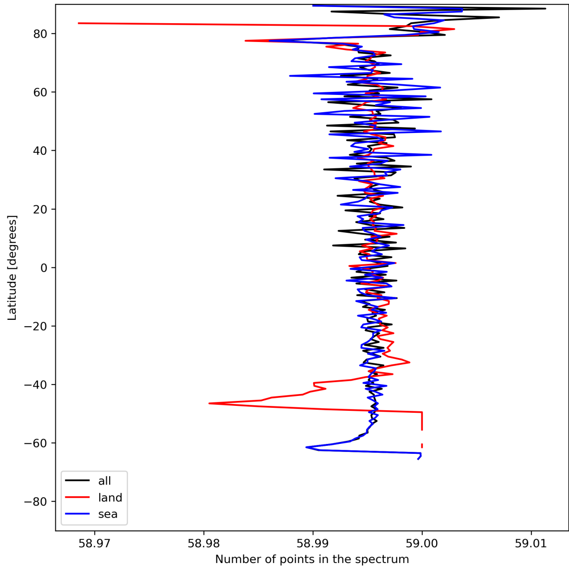
Figure 27: Zonal average of “Number of points in the spectrum” for 2024-07-11 to 2024-07-13.
