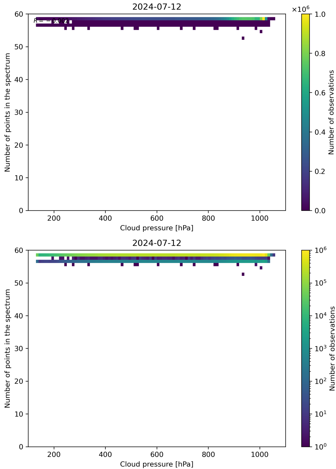
Figure 82: Scatter density plot of “Cloud pressure” against “Number of points in the spectrum” for 2024-07-11 to 2024-07-13.
