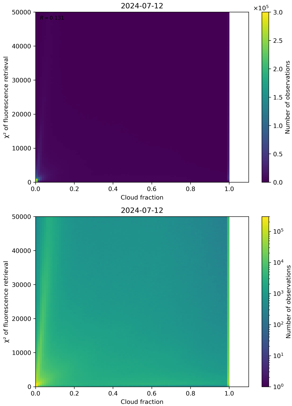
Figure 71: Scatter density plot of “Cloud fraction” against “ \chi^2 of fluorescence retrieval” for 2024-07-11 to 2024-07-13.
