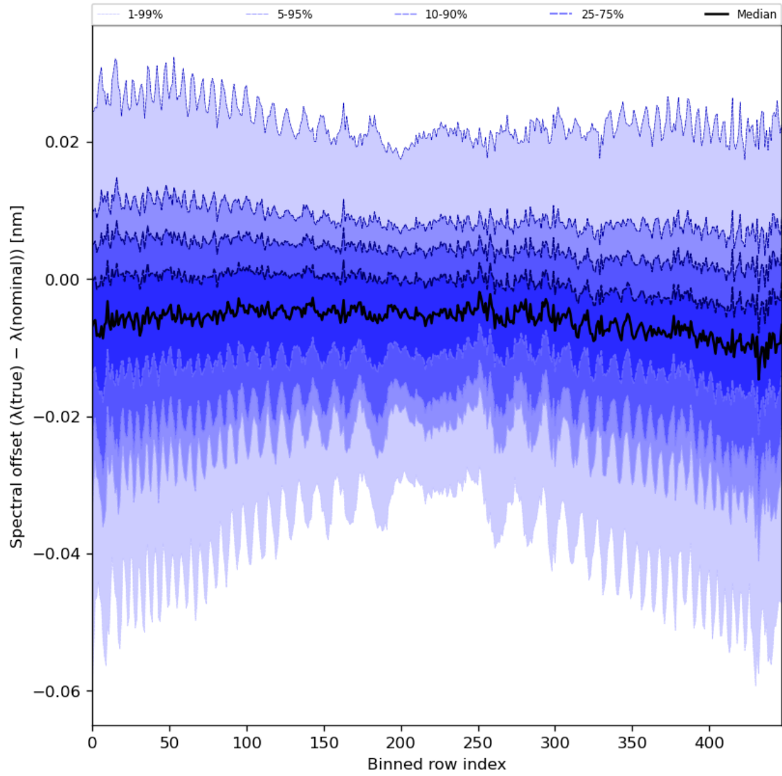
Figure 62: Along track statistics of “Spectral offset ( \lambda(\text{true}) - \lambda(\text{nominal}) )” for 2024-07-11 to 2024-07-13
