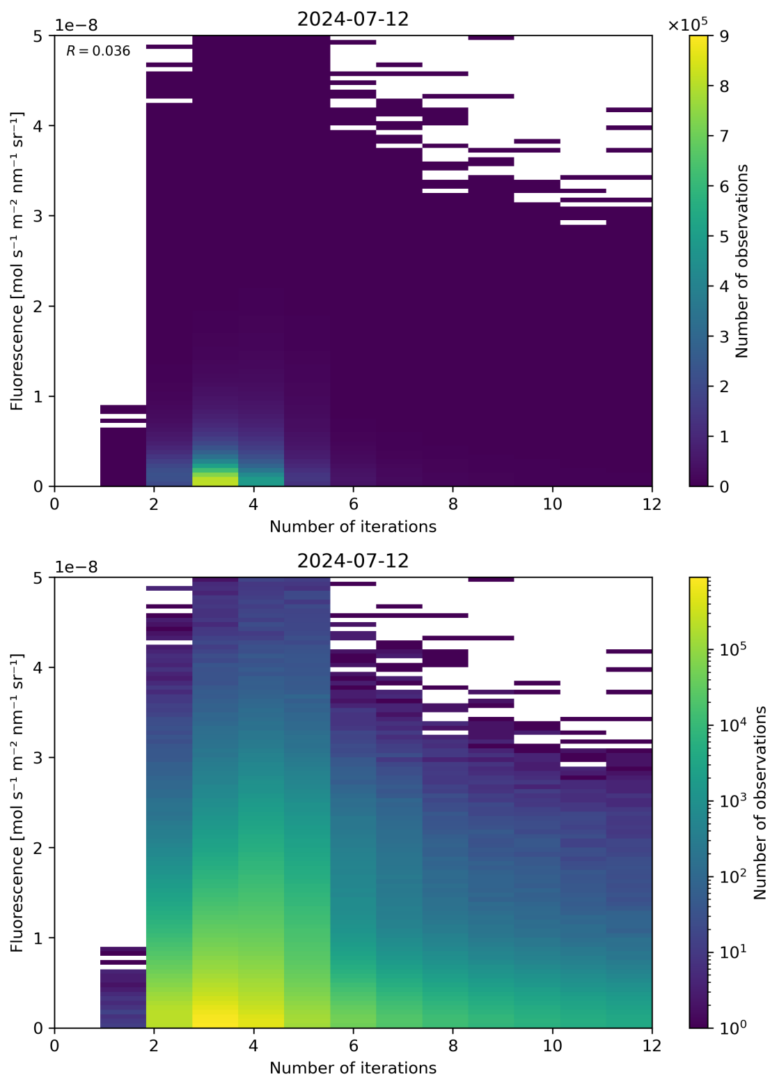
Figure 98: Scatter density plot of “Number of iterations” against “Fluorescence” for 2024-07-11 to 2024-07-13.
