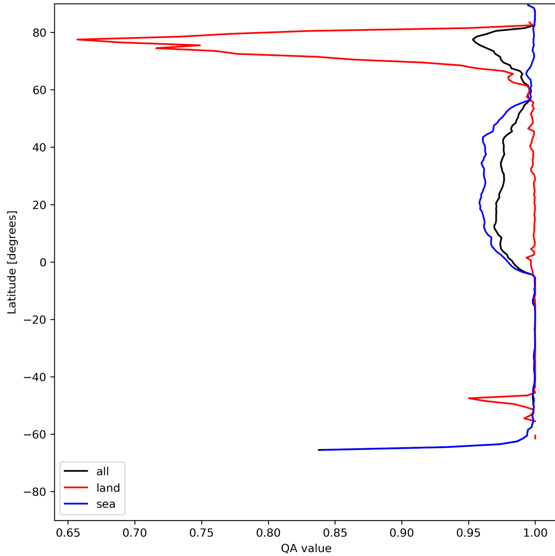
Figure 12: Zonal average of “QA value” for 2024-07-11 to 2024-07-13.
