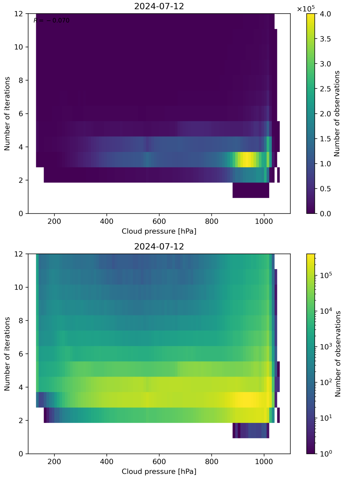
Figure 81: Scatter density plot of “Cloud pressure” against “Number of iterations” for 2024-07-11 to 2024-07-13.
