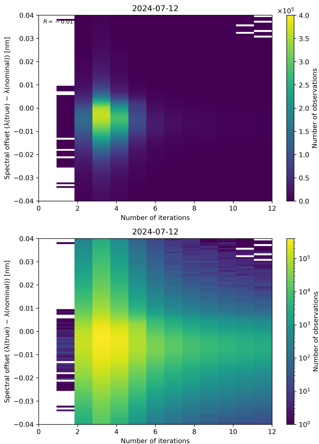
Figure 100: Scatter density plot of “Number of iterations” against “Spectral offset ( \lambda(\text{true}) - \lambda(\text{nominal}) )” for 2024-07-11 to 2024-07-13.
