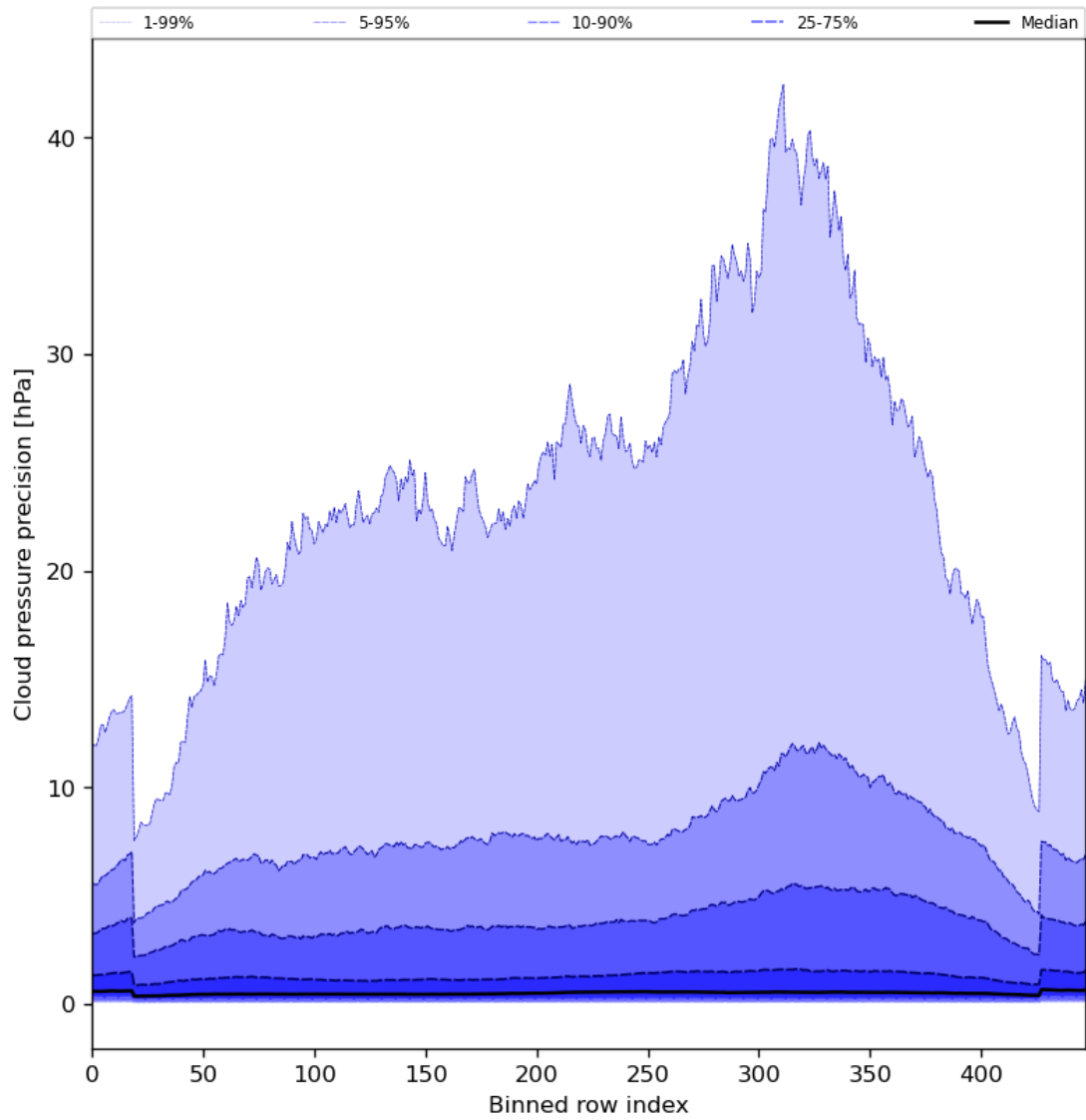
Figure 48: Along track statistics of “Cloud pressure precision” for 2024-07-11 to 2024-07-13
