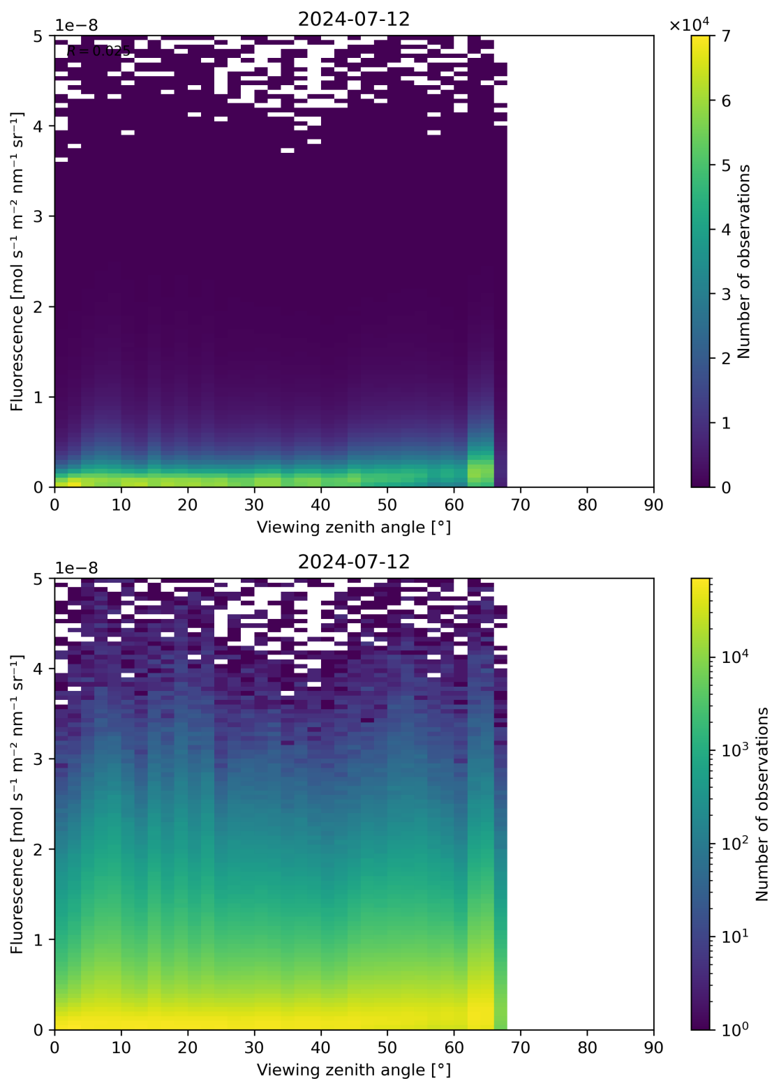
Figure 122: Scatter density plot of “Viewing zenith angle” against “Fluorescence” for 2024-07-11 to 2024-07-13.
