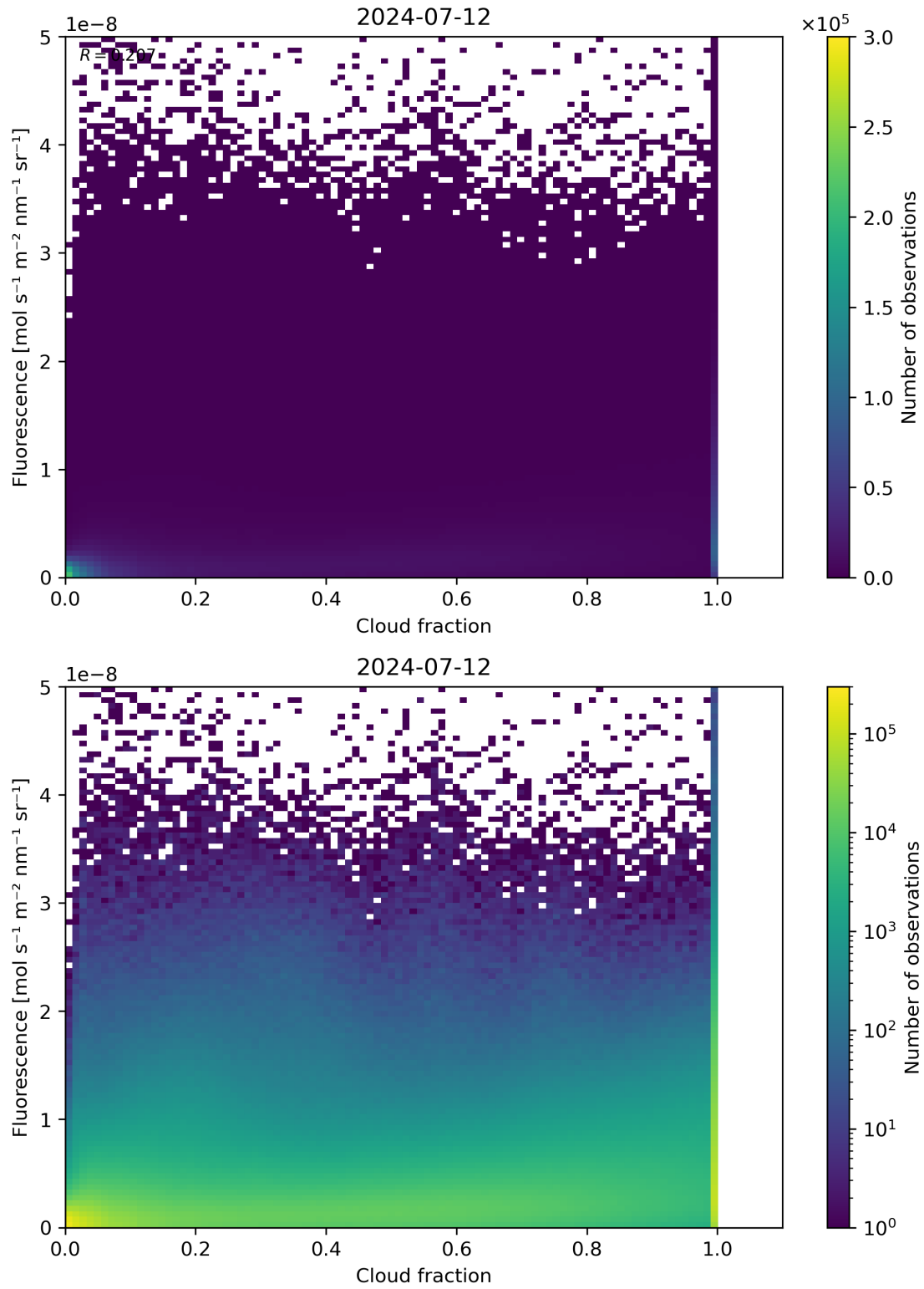
Figure 72: Scatter density plot of “Cloud fraction” against “Fluorescence” for 2024-07-11 to 2024-07-13.
