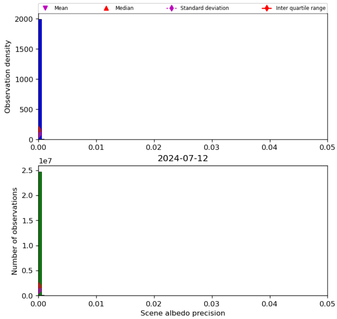
Figure 35: Histogram of “Scene albedo precision” for 2024-07-11 to 2024-07-13
