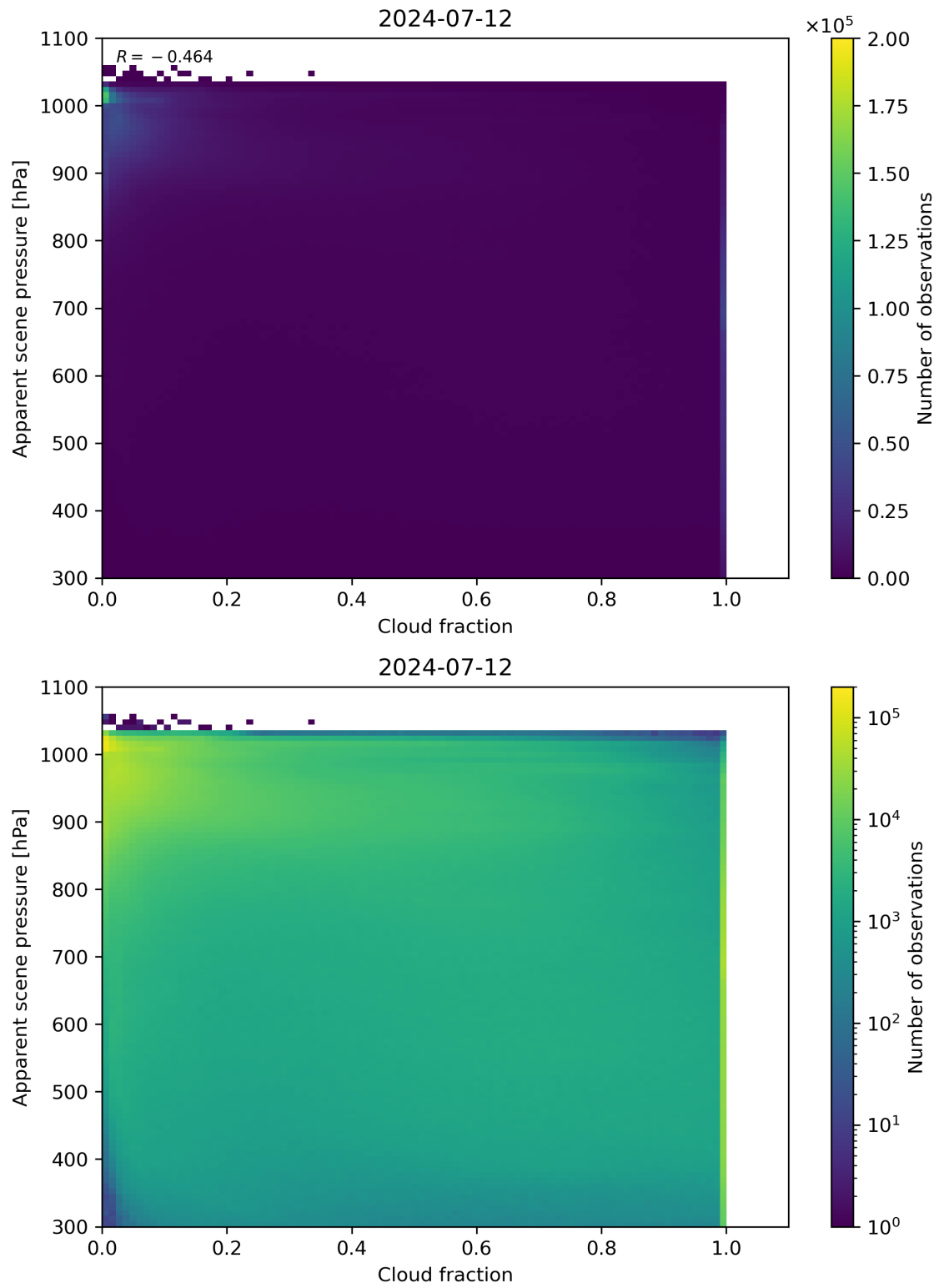
Figure 70: Scatter density plot of “Cloud fraction” against “Apparent scene pressure” for 2024-07-11 to 2024-07-13.
