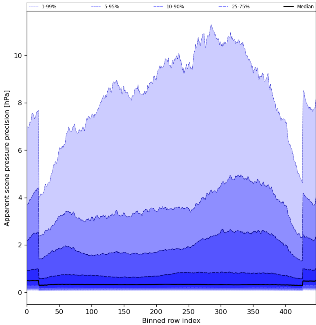
Figure 54: Along track statistics of “Apparent scene pressure precision” for 2024-07-11 to 2024-07-13
