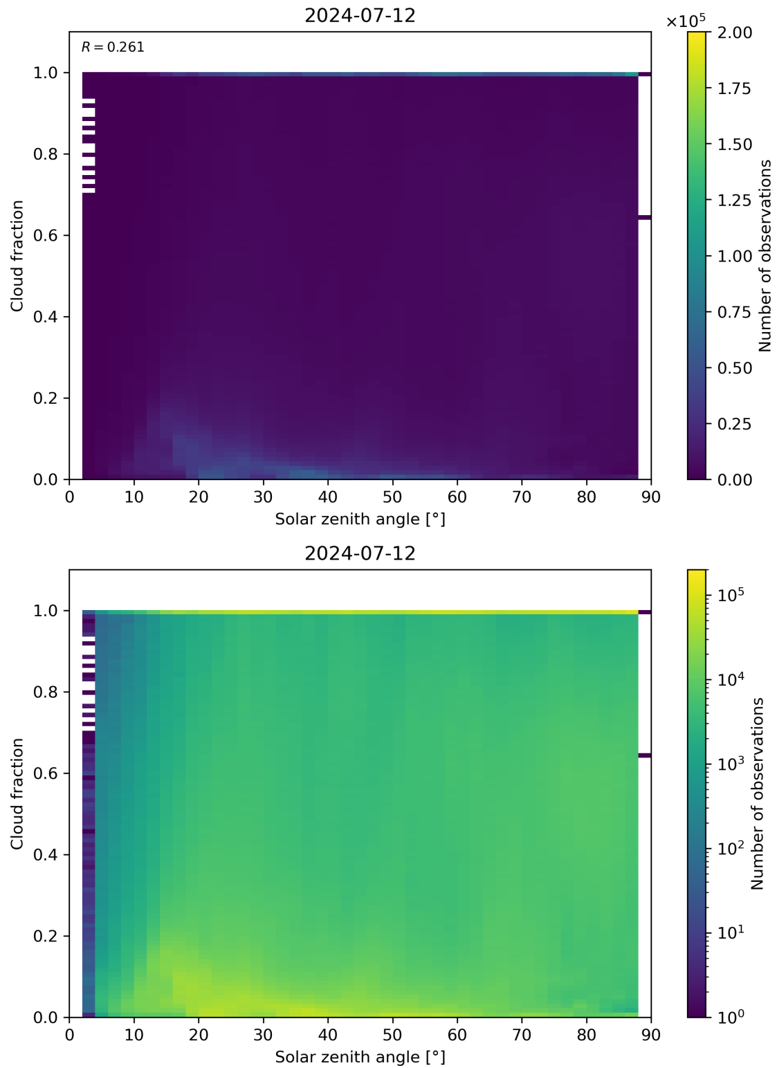
Figure 110: Scatter density plot of “Solar zenith angle” against “Cloud fraction” for 2024-07-11 to 2024-07-13.
