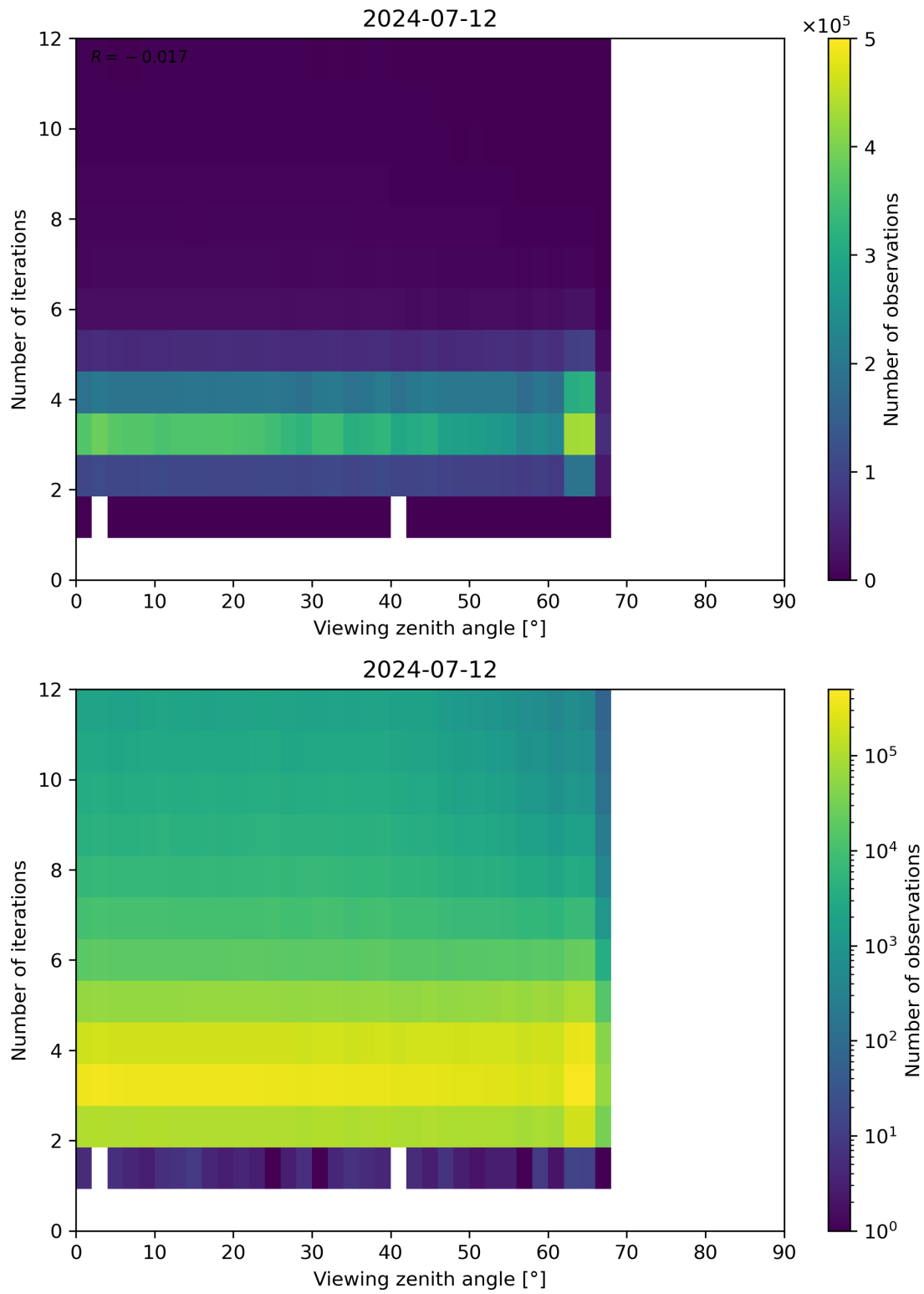
Figure 124: Scatter density plot of “Viewing zenith angle” against “Number of iterations” for 2024-07-11 to 2024-07-13.
