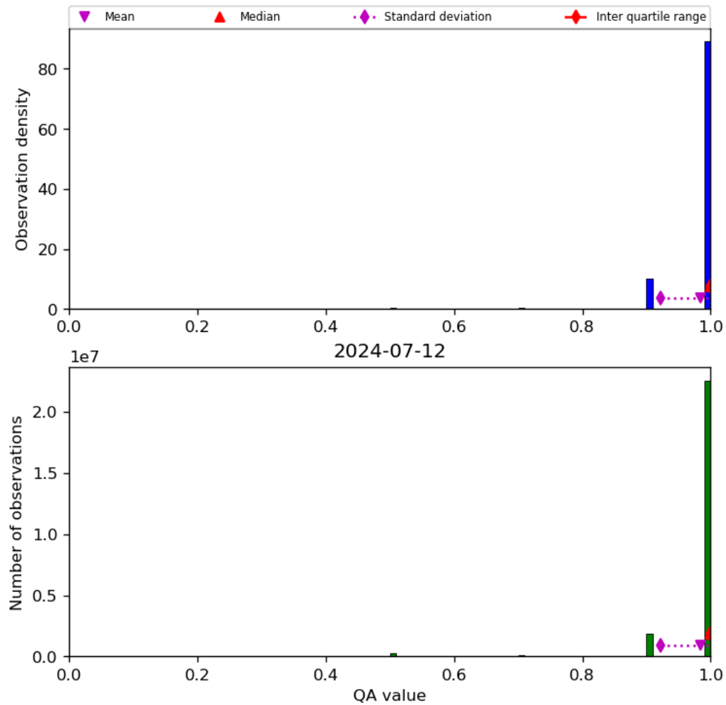
Figure 29: Histogram of “QA value” for 2024-07-11 to 2024-07-13
