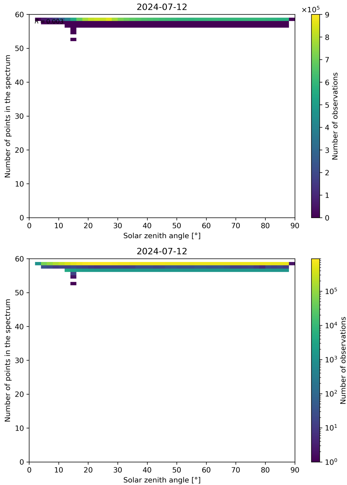
Figure 115: Scatter density plot of “Solar zenith angle” against “Number of points in the spectrum” for 2024-07-11 to 2024-07-13.
