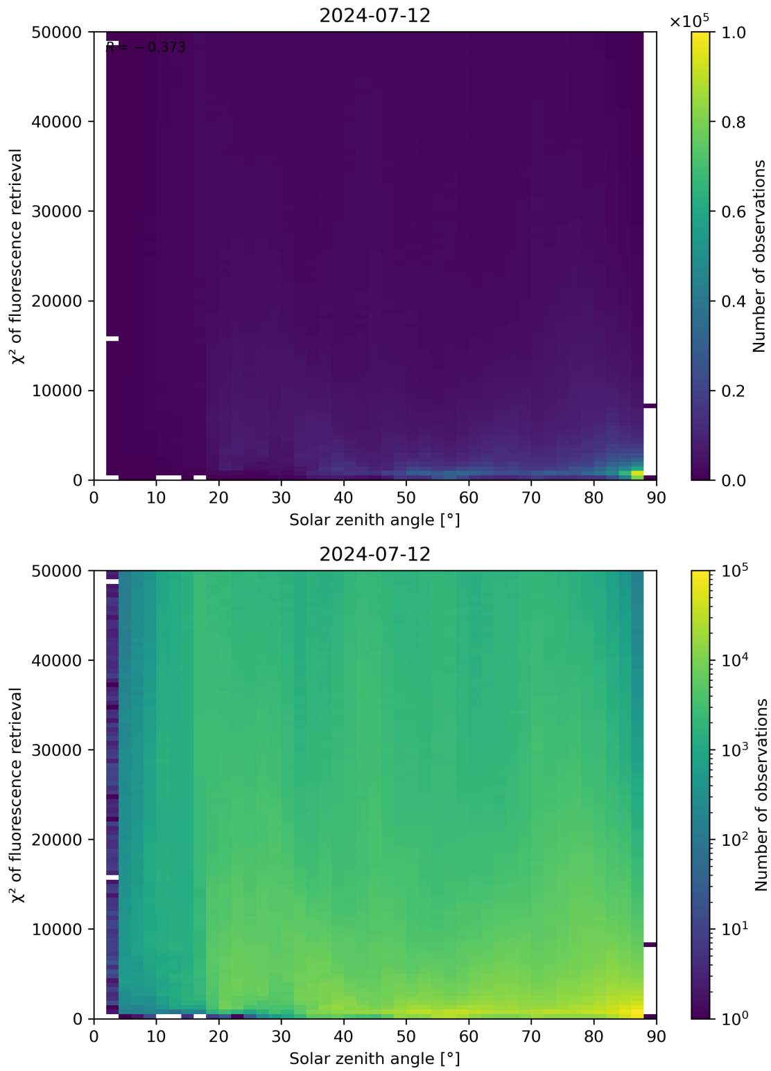
Figure 109: Scatter density plot of “Solar zenith angle” against “ \chi^2 of fluorescence retrieval” for 2024-07-11 to 2024-07-13.
