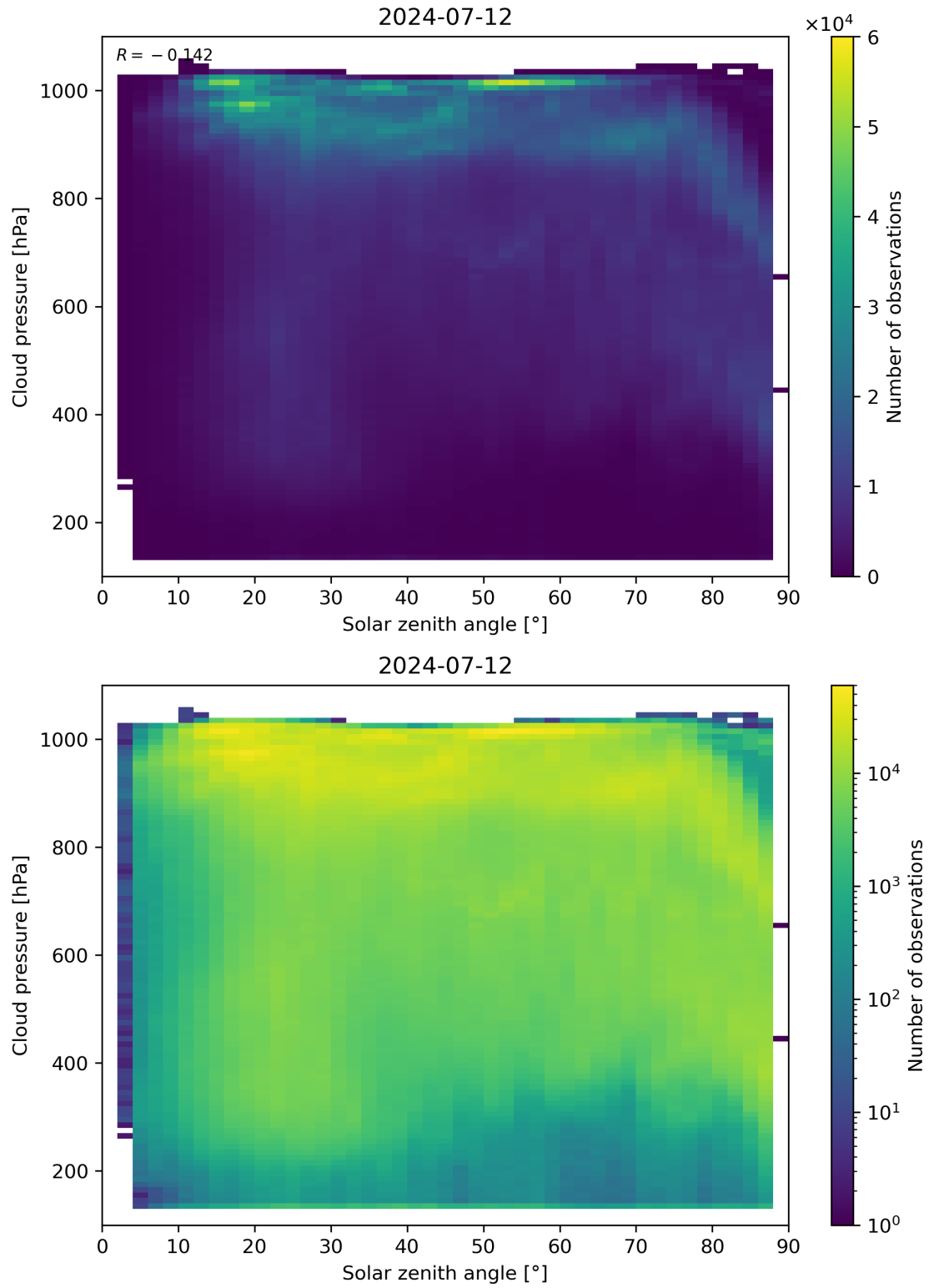
Figure 111: Scatter density plot of “Solar zenith angle” against “Cloud pressure” for 2024-07-11 to 2024-07-13.
