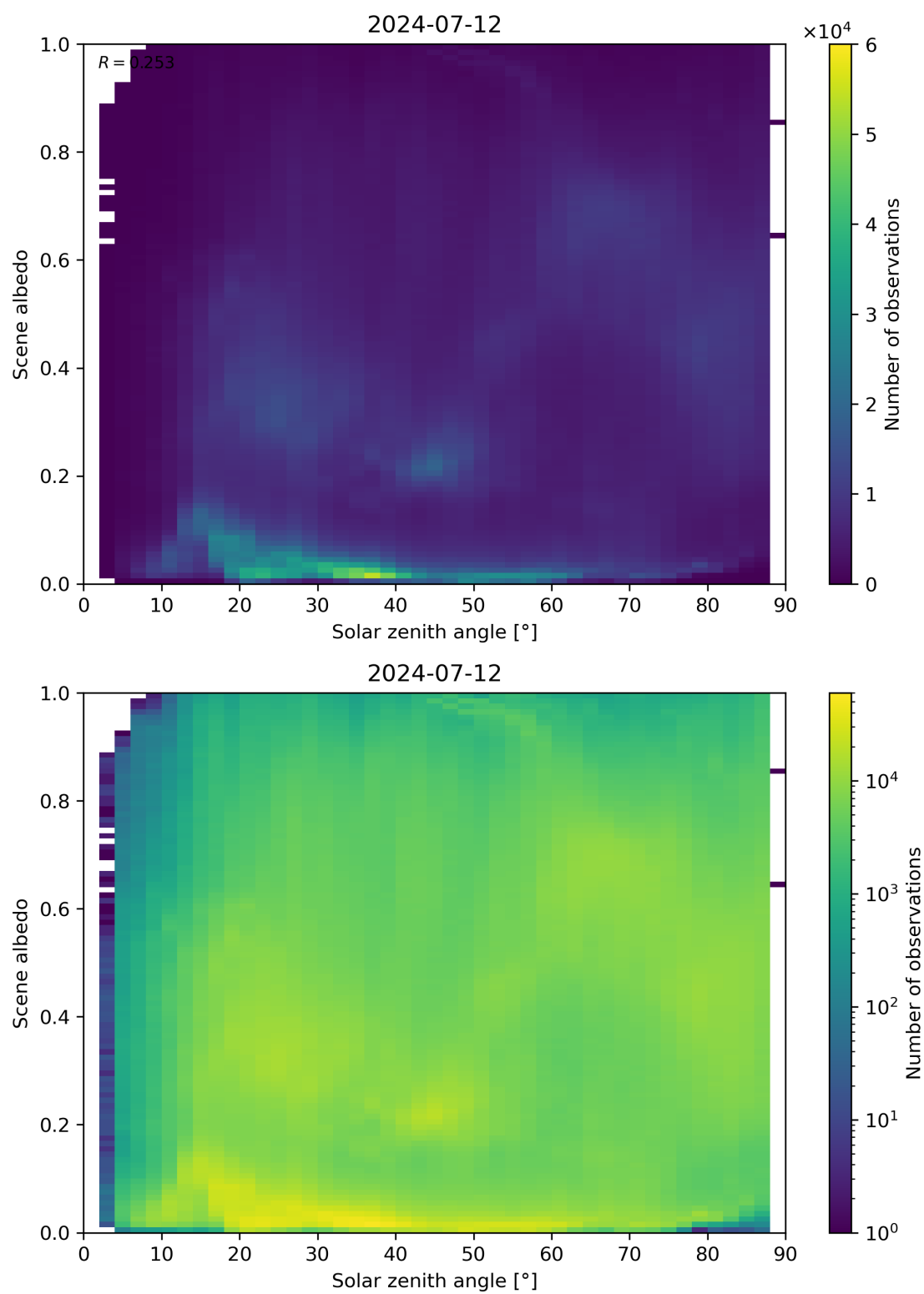
Figure 116: Scatter density plot of “Solar zenith angle” against “Scene albedo” for 2024-07-11 to 2024-07-13.
