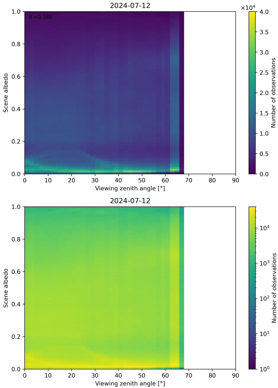
Figure 126: Scatter density plot of “Viewing zenith angle” against “Scene albedo” for 2024-07-11 to 2024-07-13.
