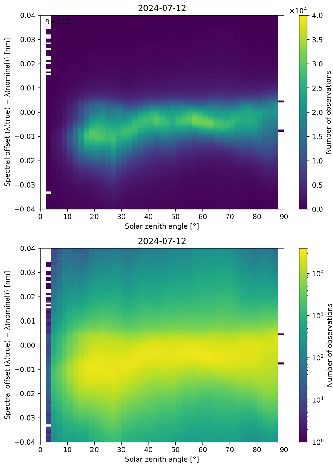
Figure 117: Scatter density plot of “Solar zenith angle” against “Spectral offset ( \lambda(\text{true}) - \lambda(\text{nominal}) )” for 2024-07-11 to 2024-07-13.
