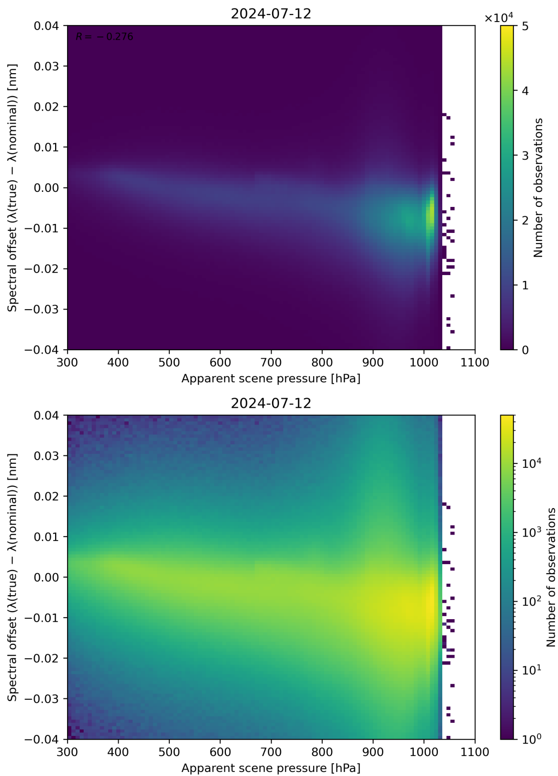
Figure 67: Scatter density plot of “Apparent scene pressure” against “Spectral offset ( \lambda(\text{true}) - \lambda(\text{nominal}) )” for 2024-07-11 to 2024-07-13.
