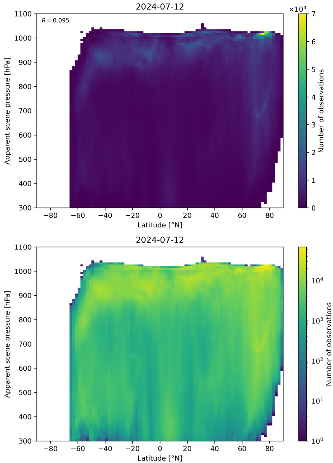
Figure 88: Scatter density plot of “Latitude” against “Apparent scene pressure” for 2024-07-11 to 2024-07-13.
