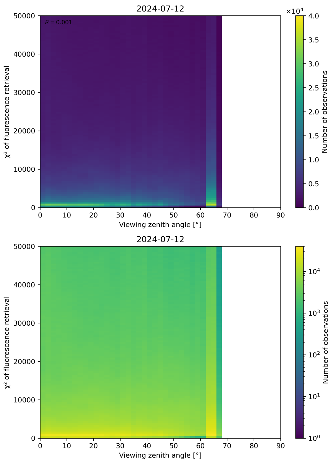
Figure 119: Scatter density plot of “Viewing zenith angle” against “ \chi^2 of fluorescence retrieval” for 2024-07-11 to 2024-07-13.
