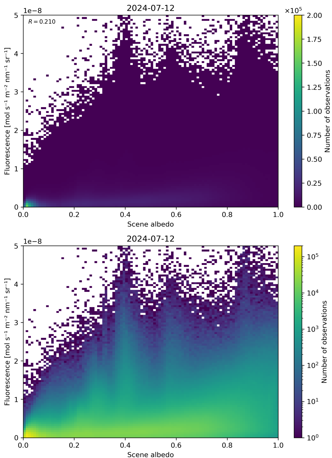
Figure 104: Scatter density plot of “Scene albedo” against “Fluorescence” for 2024-07-11 to 2024-07-13.
