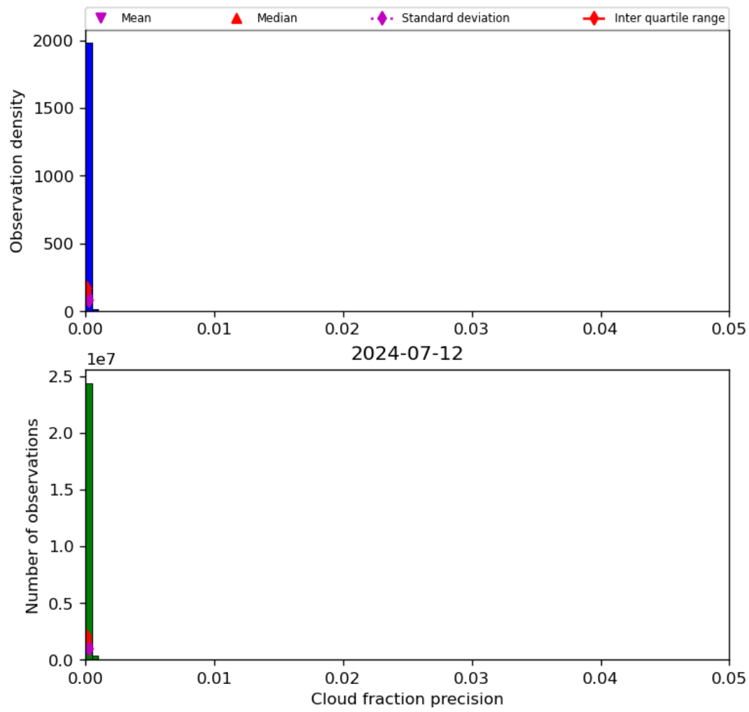
Figure 33: Histogram of “Cloud fraction precision” for 2024-07-11 to 2024-07-13
