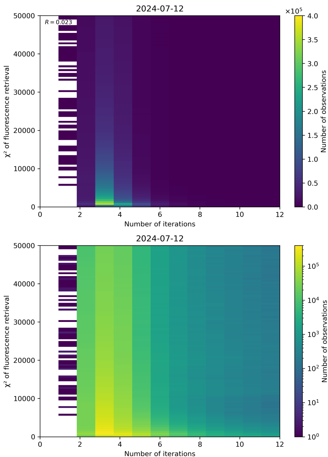
Figure 97: Scatter density plot of “Number of iterations” against “ \chi^2 of fluorescence retrieval” for 2024-07-11 to 2024-07-13.
