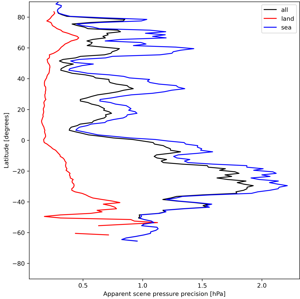
Figure 20: Zonal average of “Apparent scene pressure precision” for 2024-07-11 to 2024-07-13.
