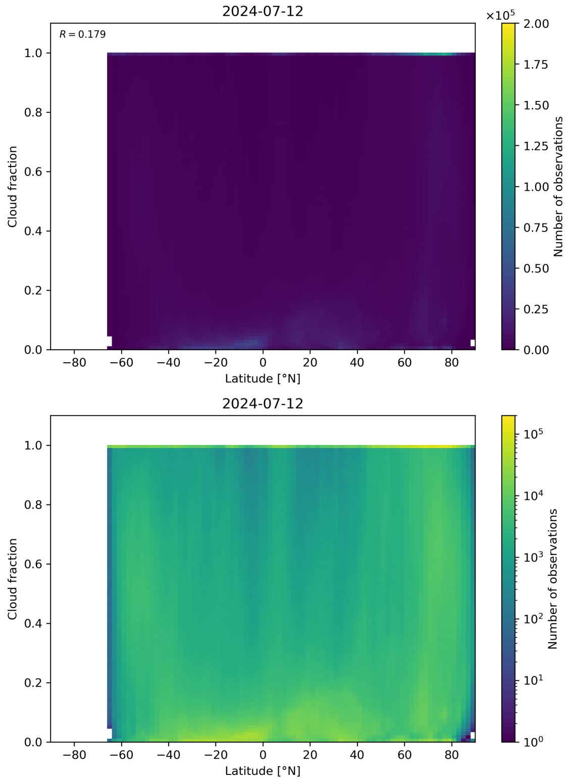
Figure 90: Scatter density plot of “Latitude” against “Cloud fraction” for 2024-07-11 to 2024-07-13.
