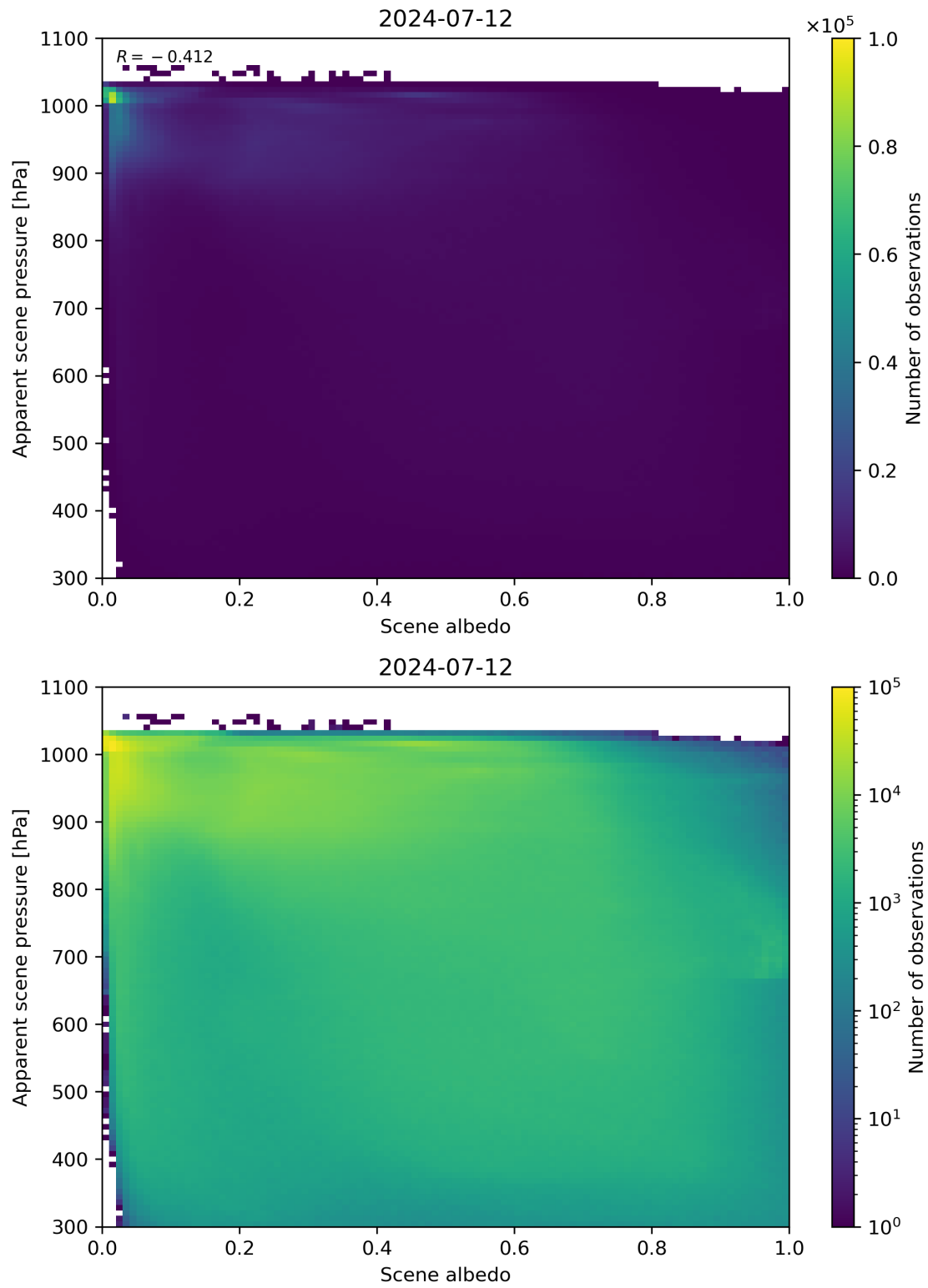
Figure 102: Scatter density plot of “Scene albedo” against “Apparent scene pressure” for 2024-07-11 to 2024-07-13.
