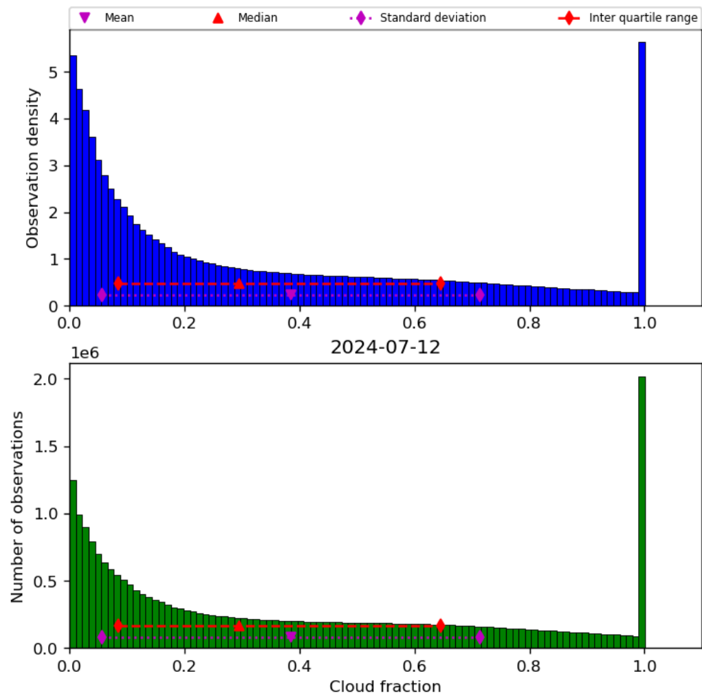
Figure 32: Histogram of “Cloud fraction” for 2024-07-11 to 2024-07-13
