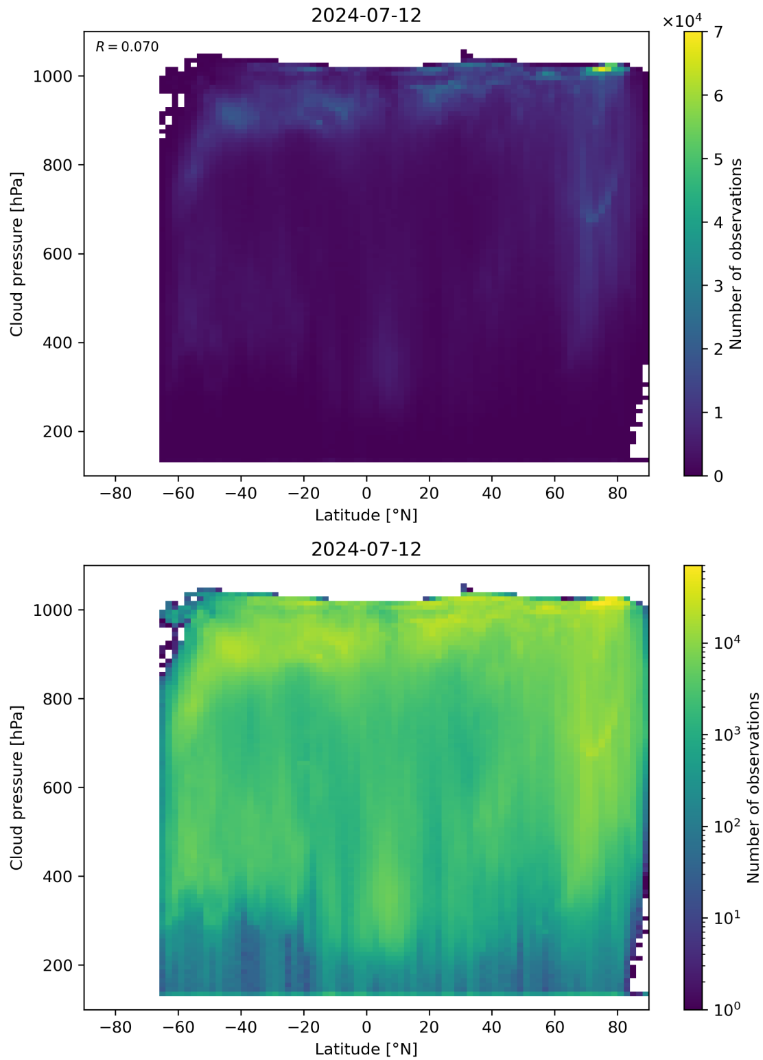
Figure 91: Scatter density plot of “Latitude” against “Cloud pressure” for 2024-07-11 to 2024-07-13.
