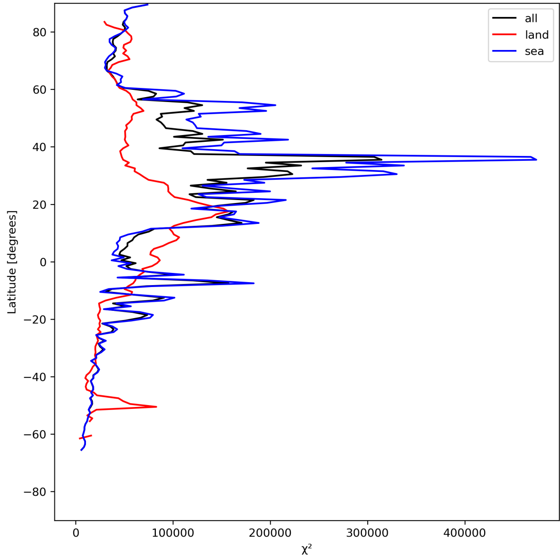
Figure 21: Zonal average of “ \chi^2 ” for 2024-07-11 to 2024-07-13.
