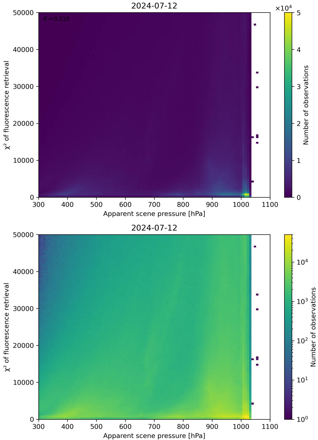
Figure 63: Scatter density plot of “Apparent scene pressure” against “ \chi^2 of fluorescence retrieval” for 2024-07-11 to 2024-07-13.
