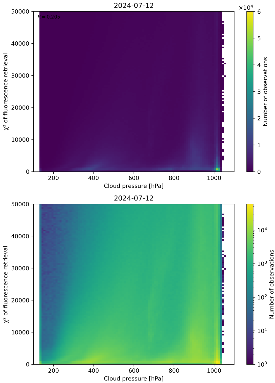
Figure 78: Scatter density plot of “Cloud pressure” against “ \chi^2 of fluorescence retrieval” for 2024-07-11 to 2024-07-13.
