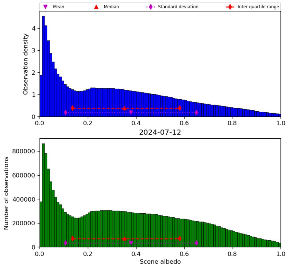
Figure 34: Histogram of “Scene albedo” for 2024-07-11 to 2024-07-13
