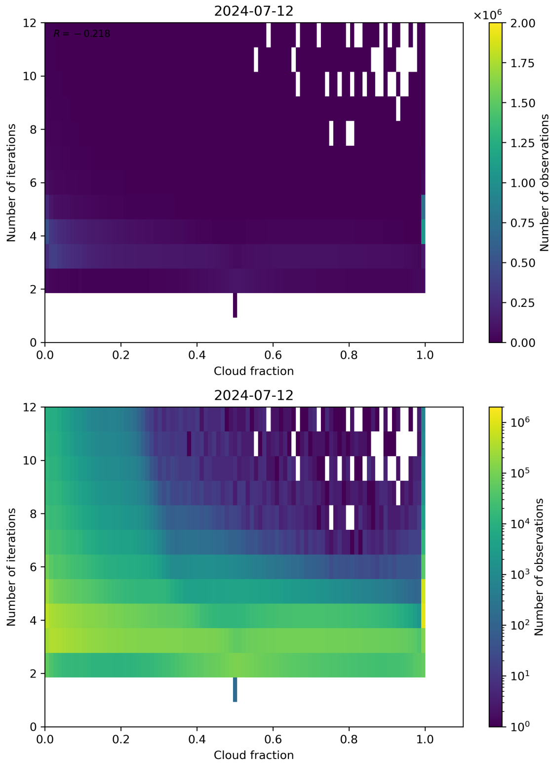
Figure 73: Scatter density plot of “Cloud fraction” against “Number of iterations” for 2024-07-11 to 2024-07-13.
