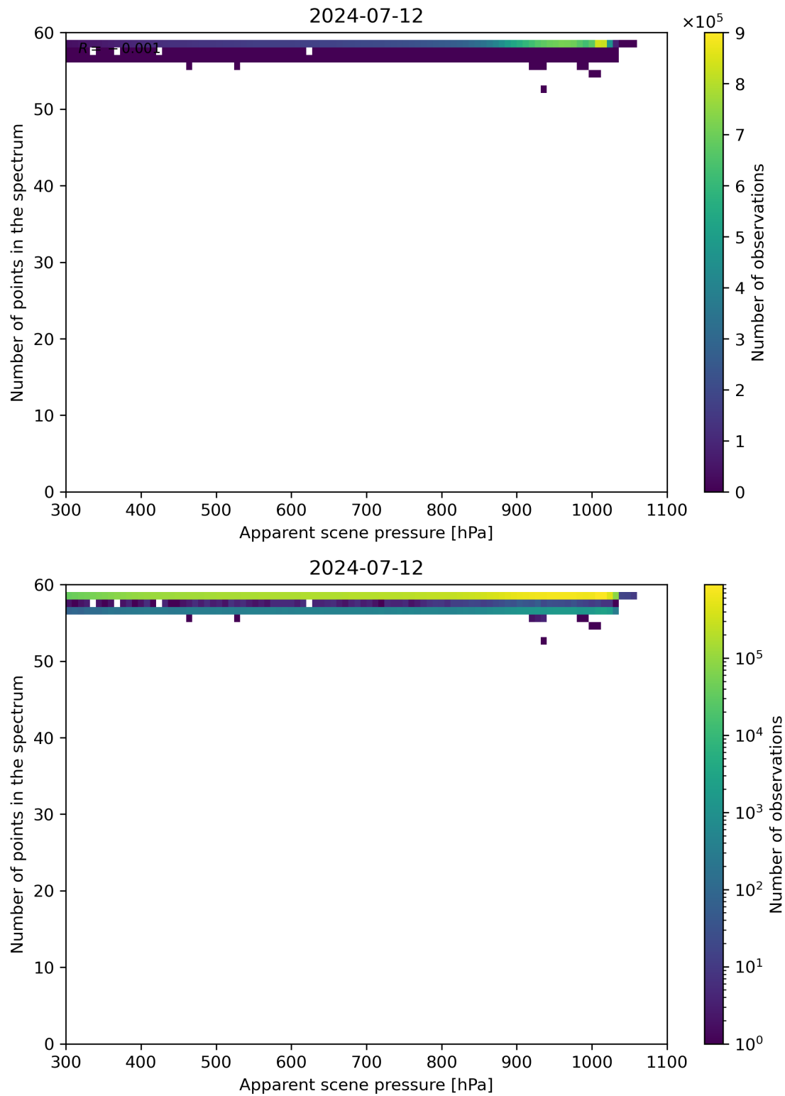
Figure 66: Scatter density plot of “Apparent scene pressure” against “Number of points in the spectrum” for 2024-07-11 to 2024-07-13.
