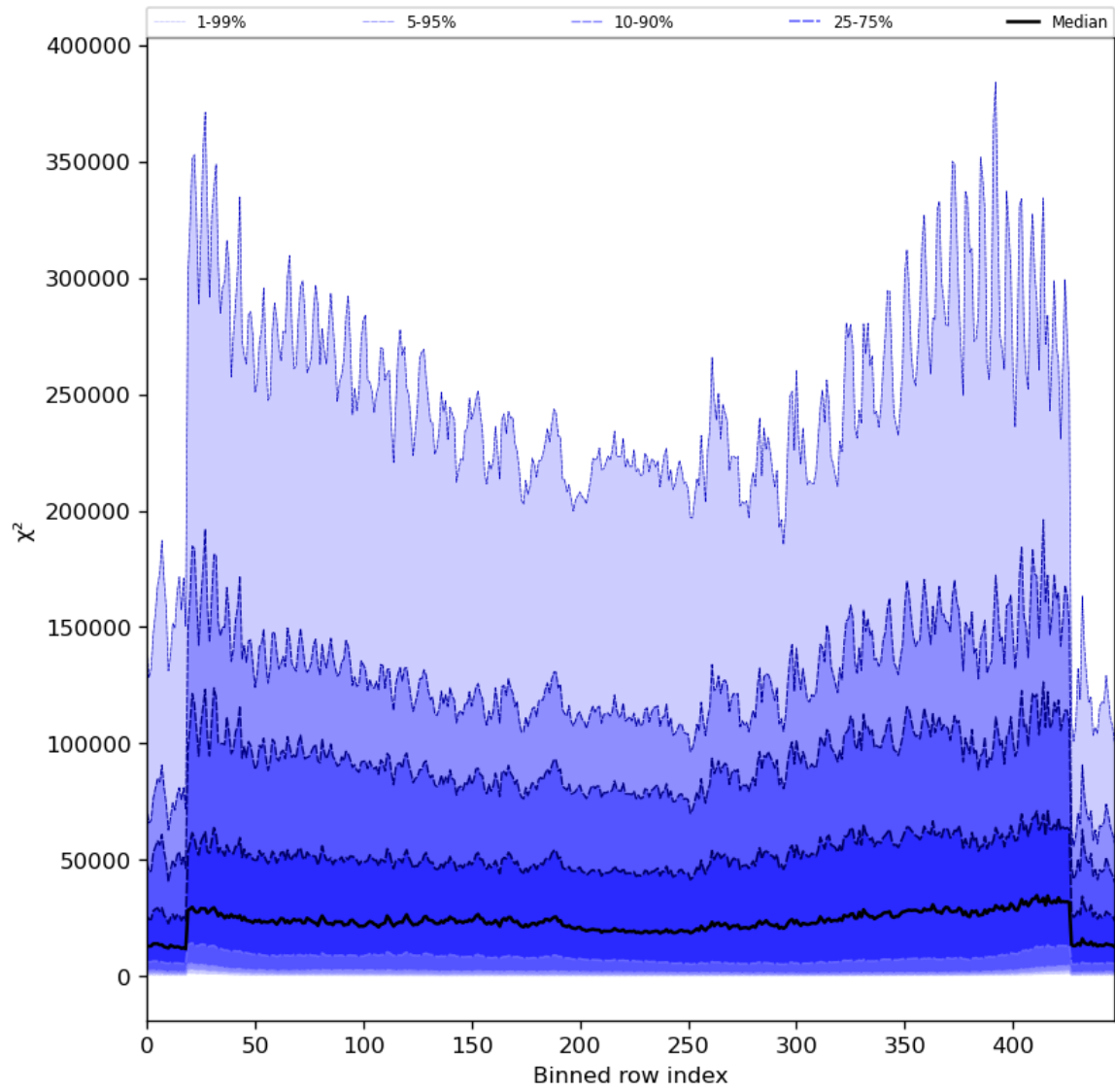
Figure 55: Along track statistics of “ \chi^2 ” for 2024-07-11 to 2024-07-13
