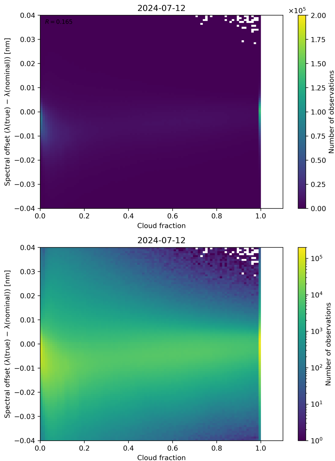
Figure 76: Scatter density plot of “Cloud fraction” against “Spectral offset ( \lambda(\text{true}) - \lambda(\text{nominal}) )” for 2024-07-11 to 2024-07-13.
