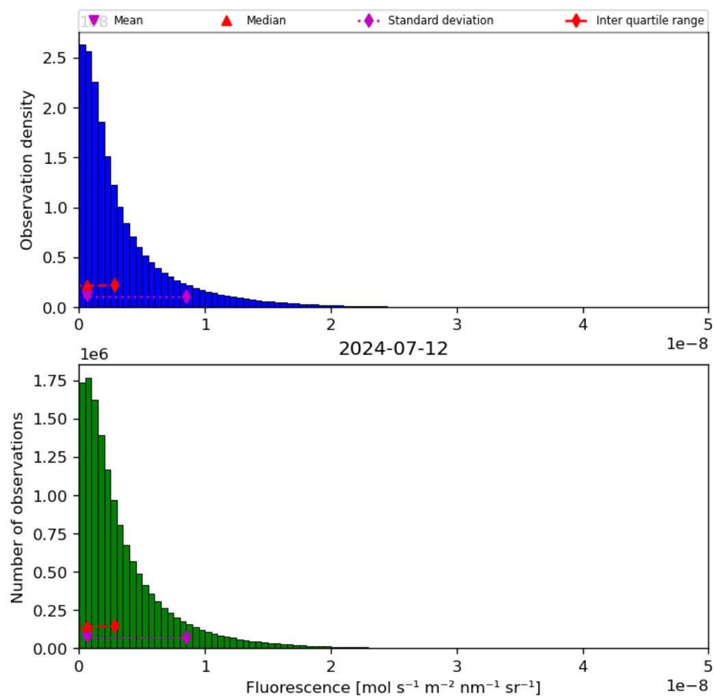
Figure 40: Histogram of “Fluorescence” for 2024-07-11 to 2024-07-13
