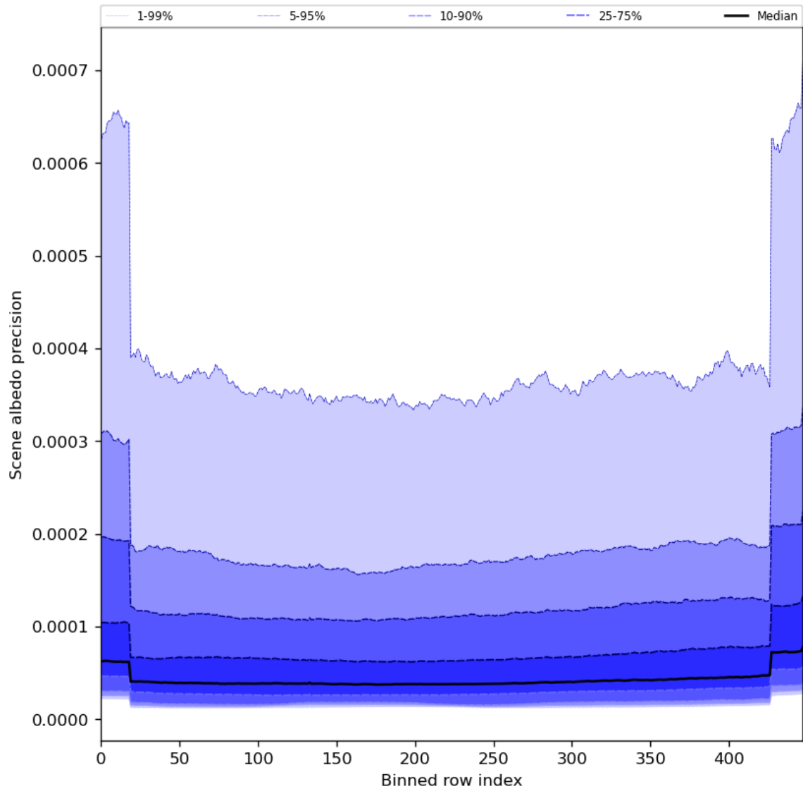
Figure 52: Along track statistics of “Scene albedo precision” for 2024-07-11 to 2024-07-13
