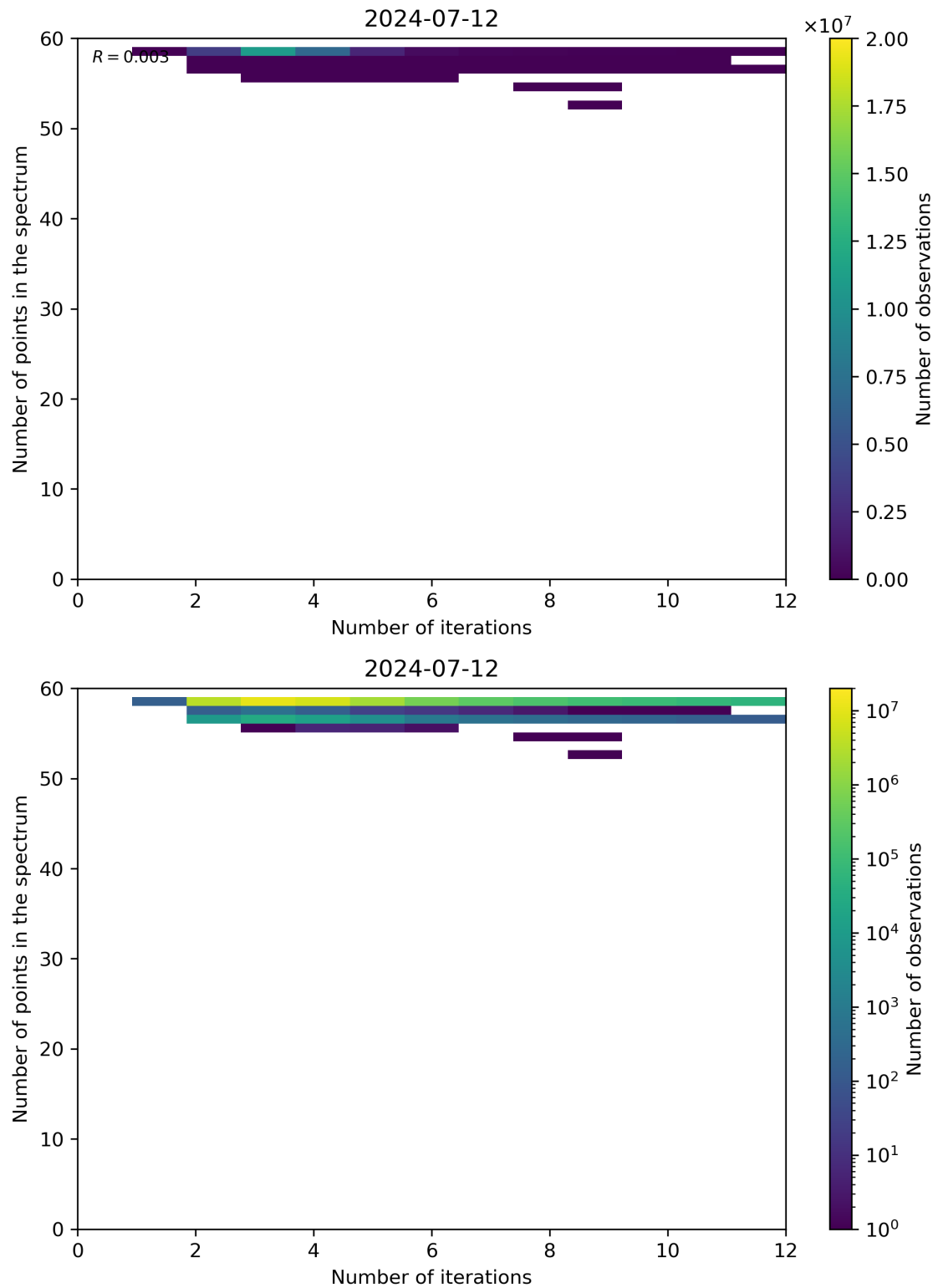
Figure 99: Scatter density plot of “Number of iterations” against “Number of points in the spectrum” for 2024-07-11 to 2024-07-13.
