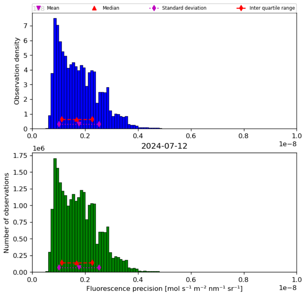
Figure 41: Histogram of “Fluorescence precision” for 2024-07-11 to 2024-07-13
