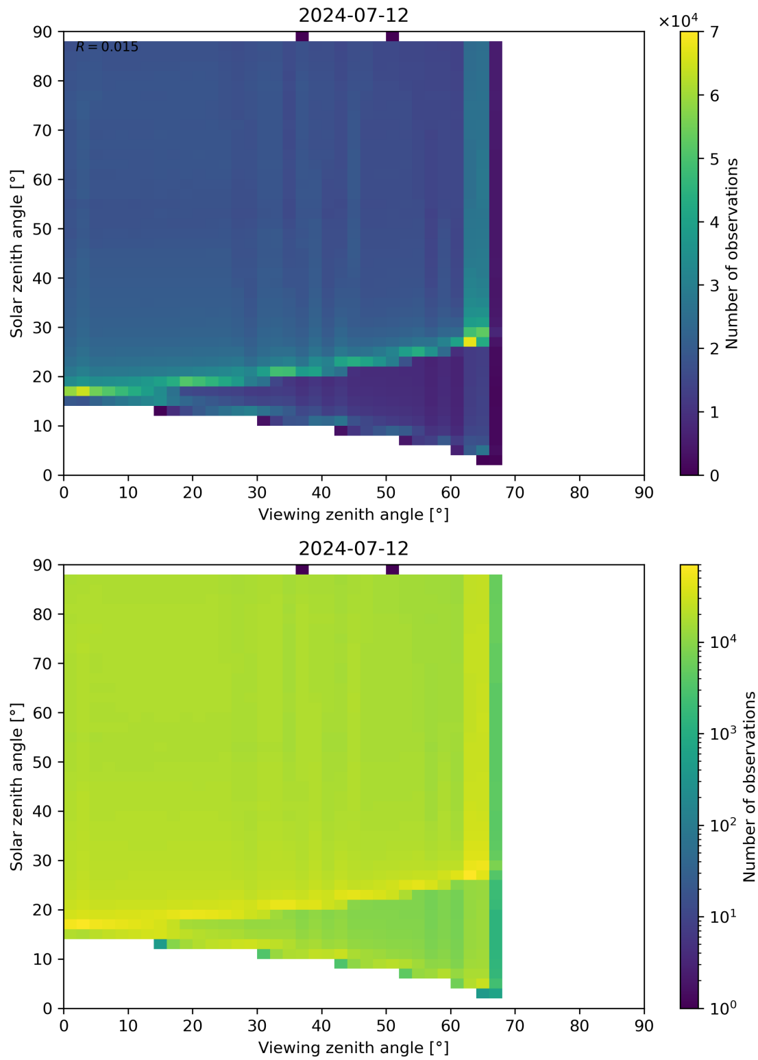
Figure 127: Scatter density plot of “Viewing zenith angle” against “Solar zenith angle” for 2024-07-11 to 2024-07-13.
