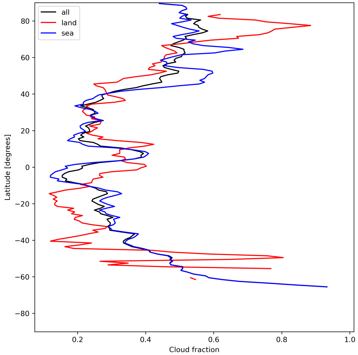
Figure 15: Zonal average of “Cloud fraction” for 2024-07-11 to 2024-07-13.
