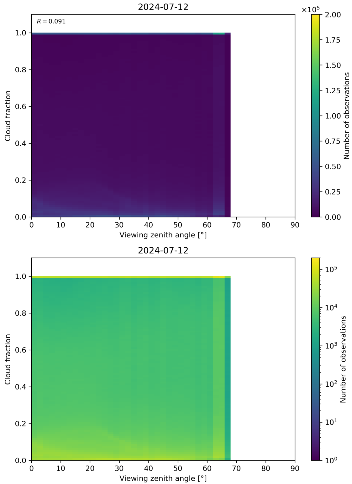
Figure 120: Scatter density plot of “Viewing zenith angle” against “Cloud fraction” for 2024-07-11 to 2024-07-13.
