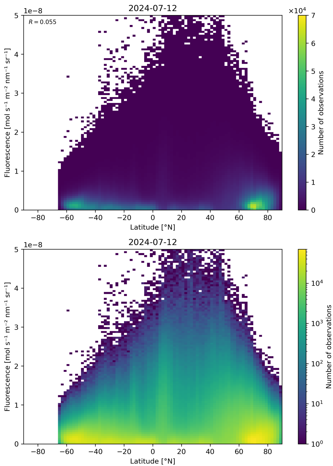
Figure 92: Scatter density plot of “Latitude” against “Fluorescence” for 2024-07-11 to 2024-07-13.
