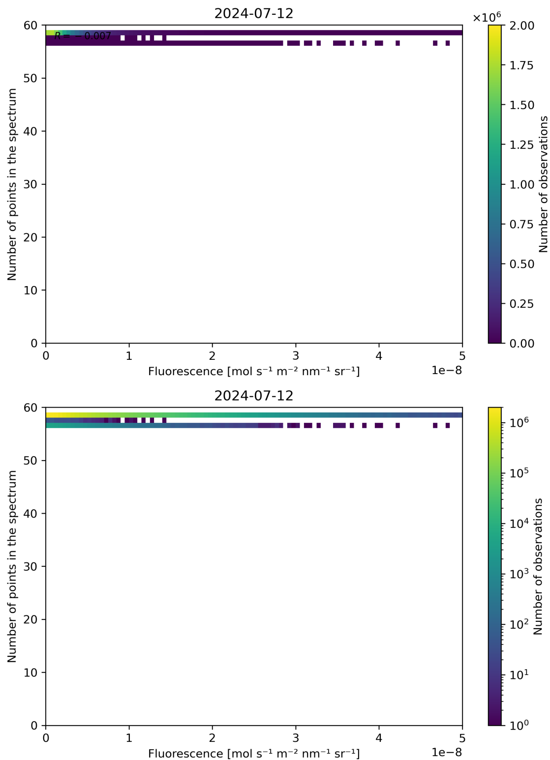
Figure 86: Scatter density plot of “Fluorescence” against “Number of points in the spectrum” for 2024-07-11 to 2024-07-13.
