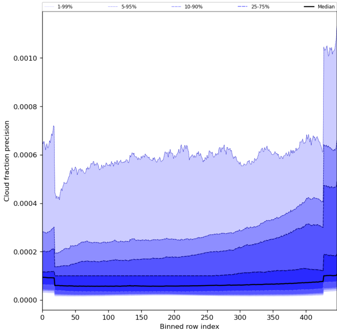
Figure 50: Along track statistics of “Cloud fraction precision” for 2024-07-11 to 2024-07-13
