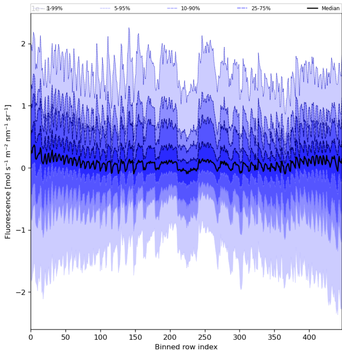
Figure 57: Along track statistics of “Fluorescence” for 2024-07-11 to 2024-07-13
