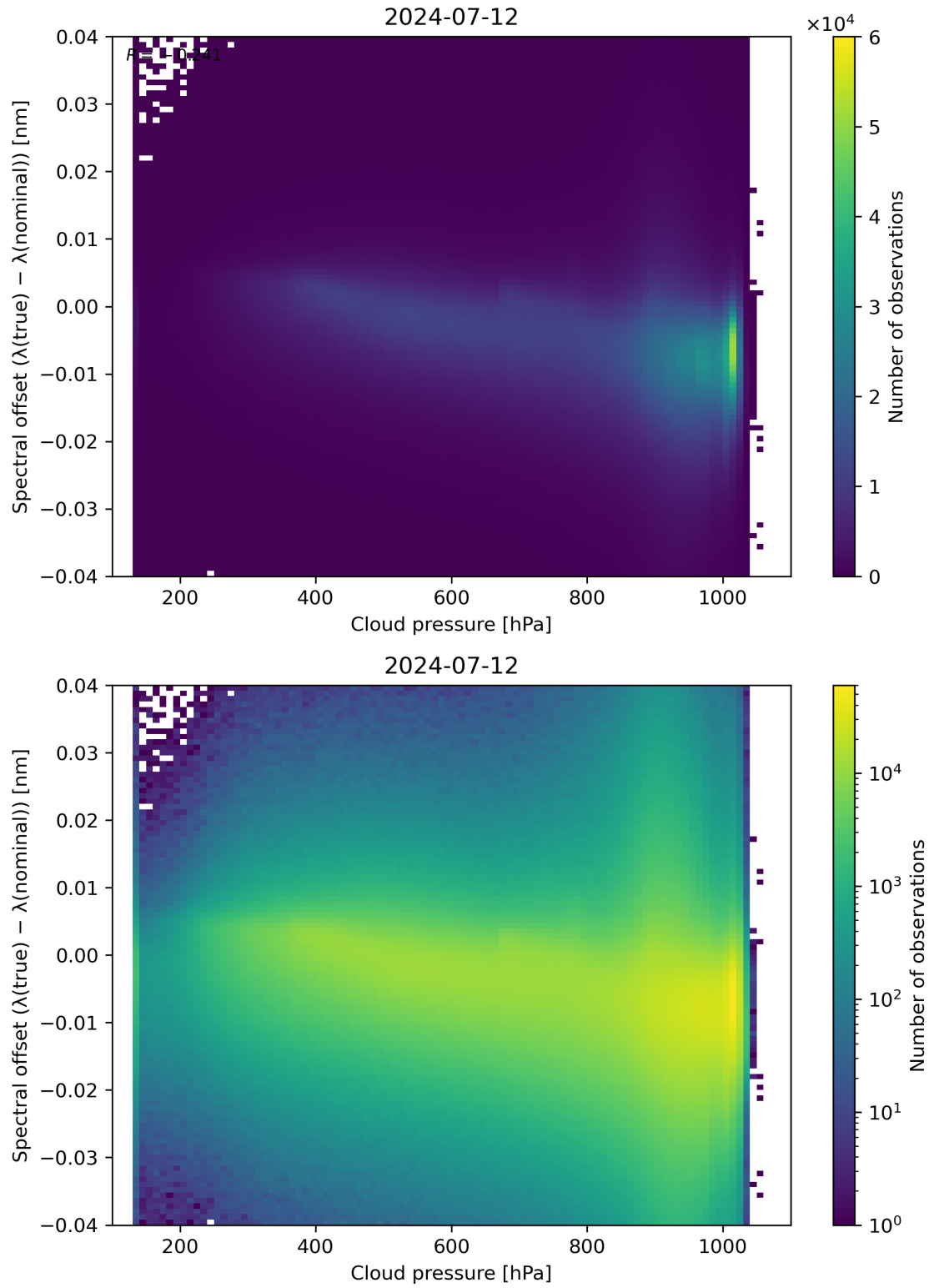
Figure 84: Scatter density plot of “Cloud pressure” against “Spectral offset ( \lambda(\text{true}) - \lambda(\text{nominal}) )” for 2024-07-11 to 2024-07-13.
