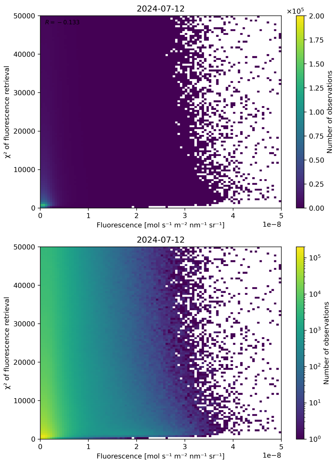
Figure 85: Scatter density plot of “Fluorescence” against “ \chi^2 of fluorescence retrieval” for 2024-07-11 to 2024-07-13.
