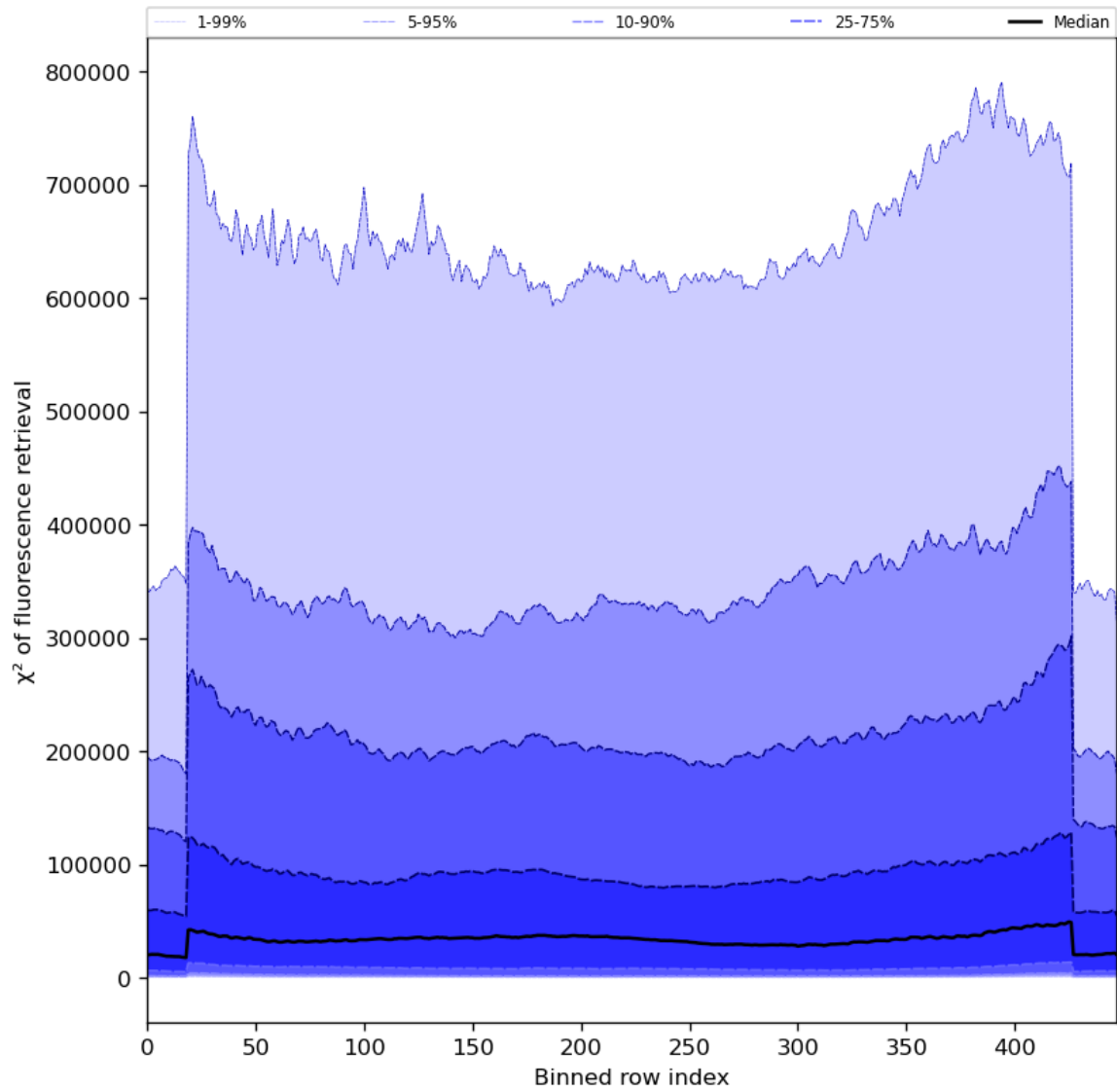
Figure 59: Along track statistics of “ \chi^2 of fluorescence retrieval” for 2024-07-11 to 2024-07-13
