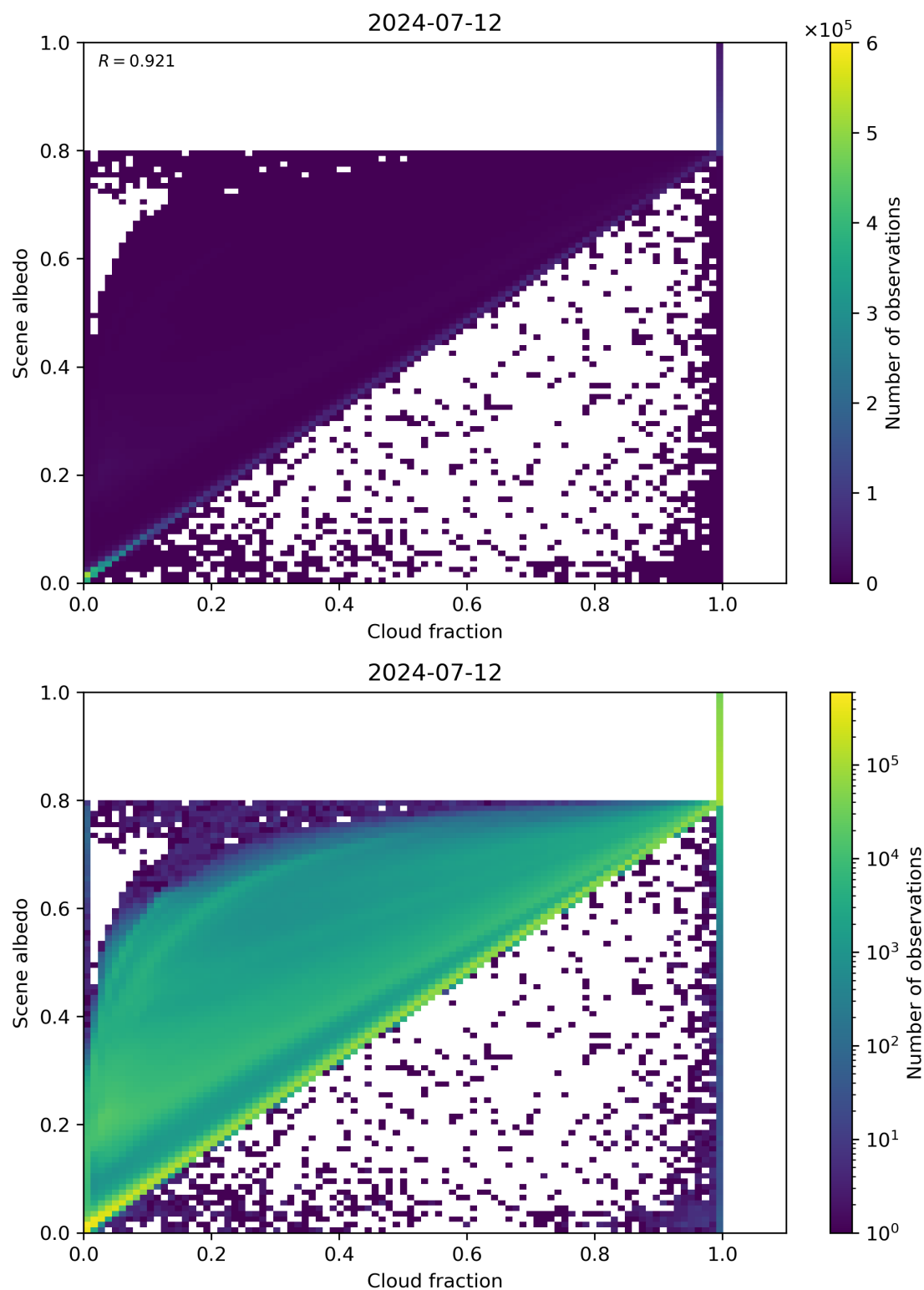
Figure 75: Scatter density plot of “Cloud fraction” against “Scene albedo” for 2024-07-11 to 2024-07-13.
