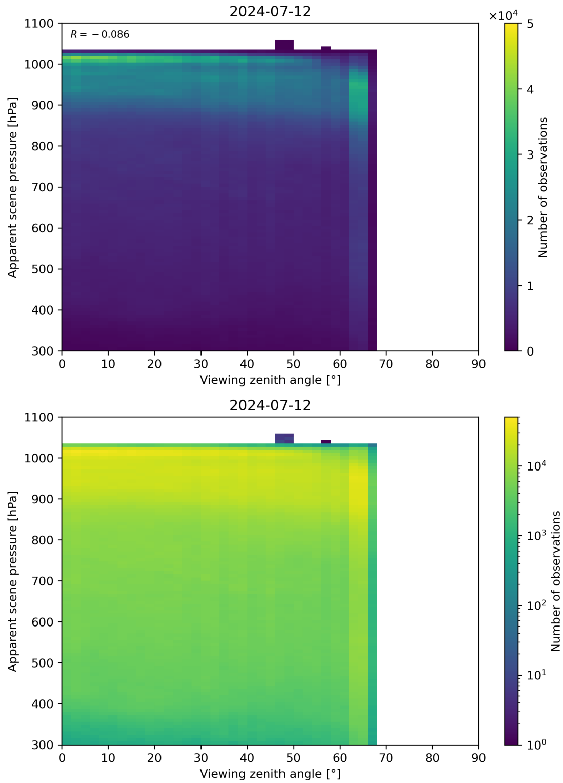
Figure 118: Scatter density plot of “Viewing zenith angle” against “Apparent scene pressure” for 2024-07-11 to 2024-07-13.
