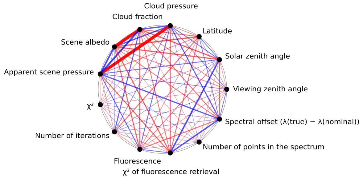
Figure 1: Map of correlation graph for 2024-07-11 to 2024-07-13.
