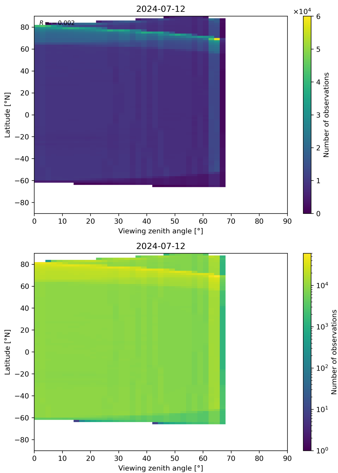
Figure 123: Scatter density plot of “Viewing zenith angle” against “Latitude” for 2024-07-11 to 2024-07-13.
