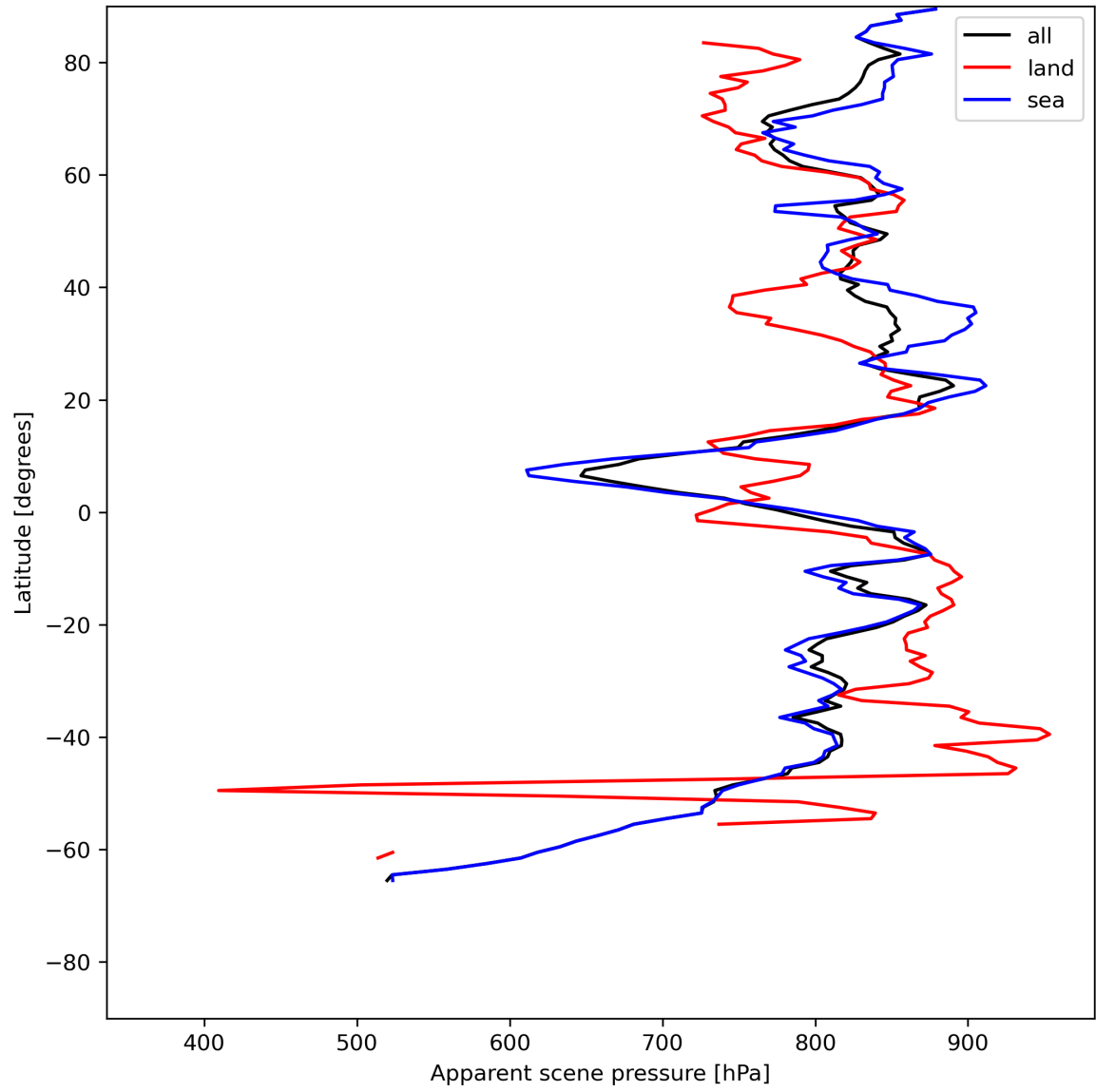
Figure 19: Zonal average of “Apparent scene pressure” for 2024-07-11 to 2024-07-13.
