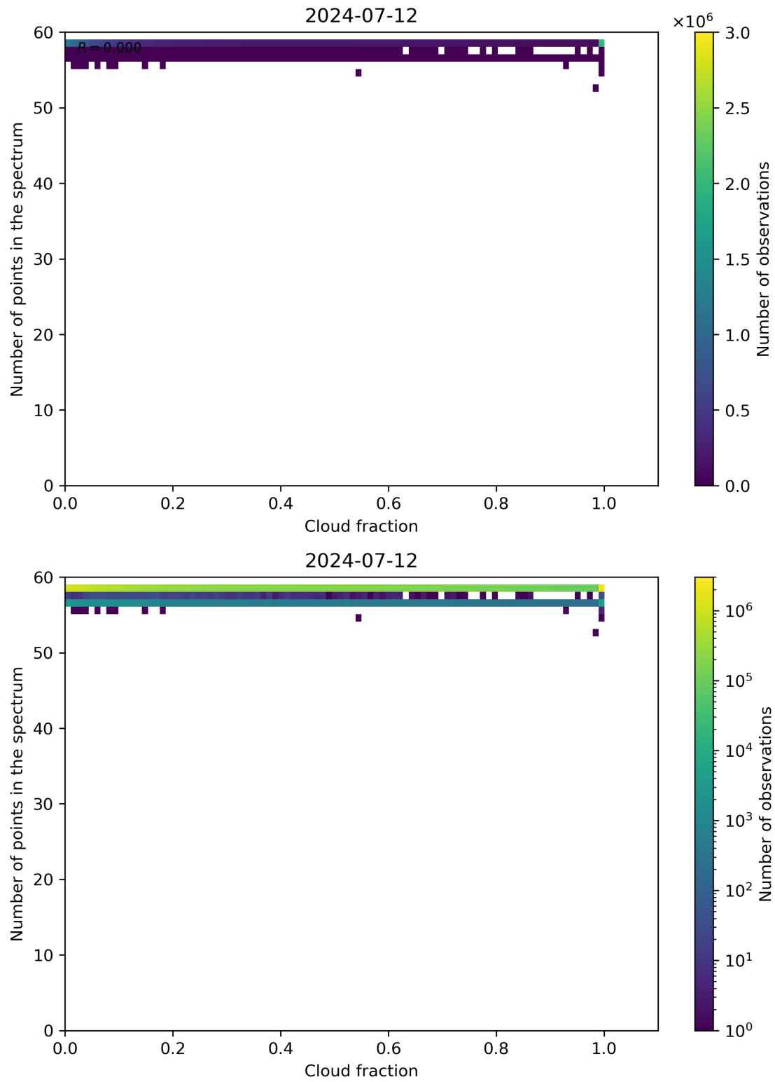
Figure 74: Scatter density plot of “Cloud fraction” against “Number of points in the spectrum” for 2024-07-11 to 2024-07-13.
