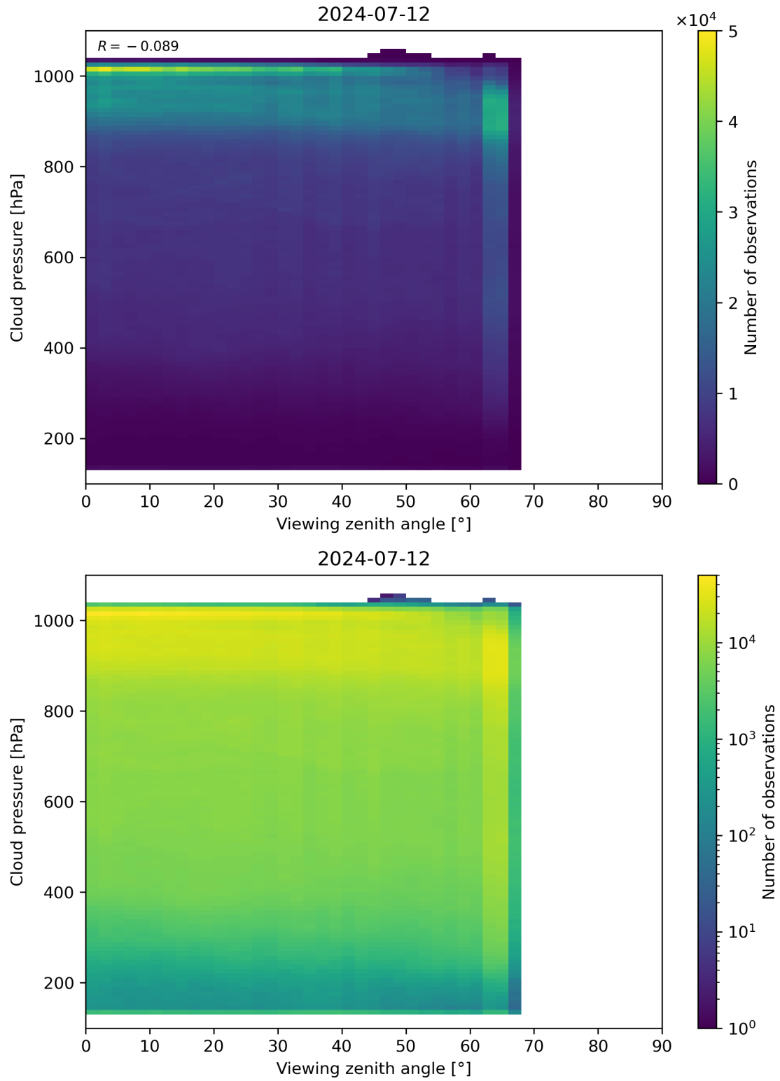
Figure 121: Scatter density plot of “Viewing zenith angle” against “Cloud pressure” for 2024-07-11 to 2024-07-13.
