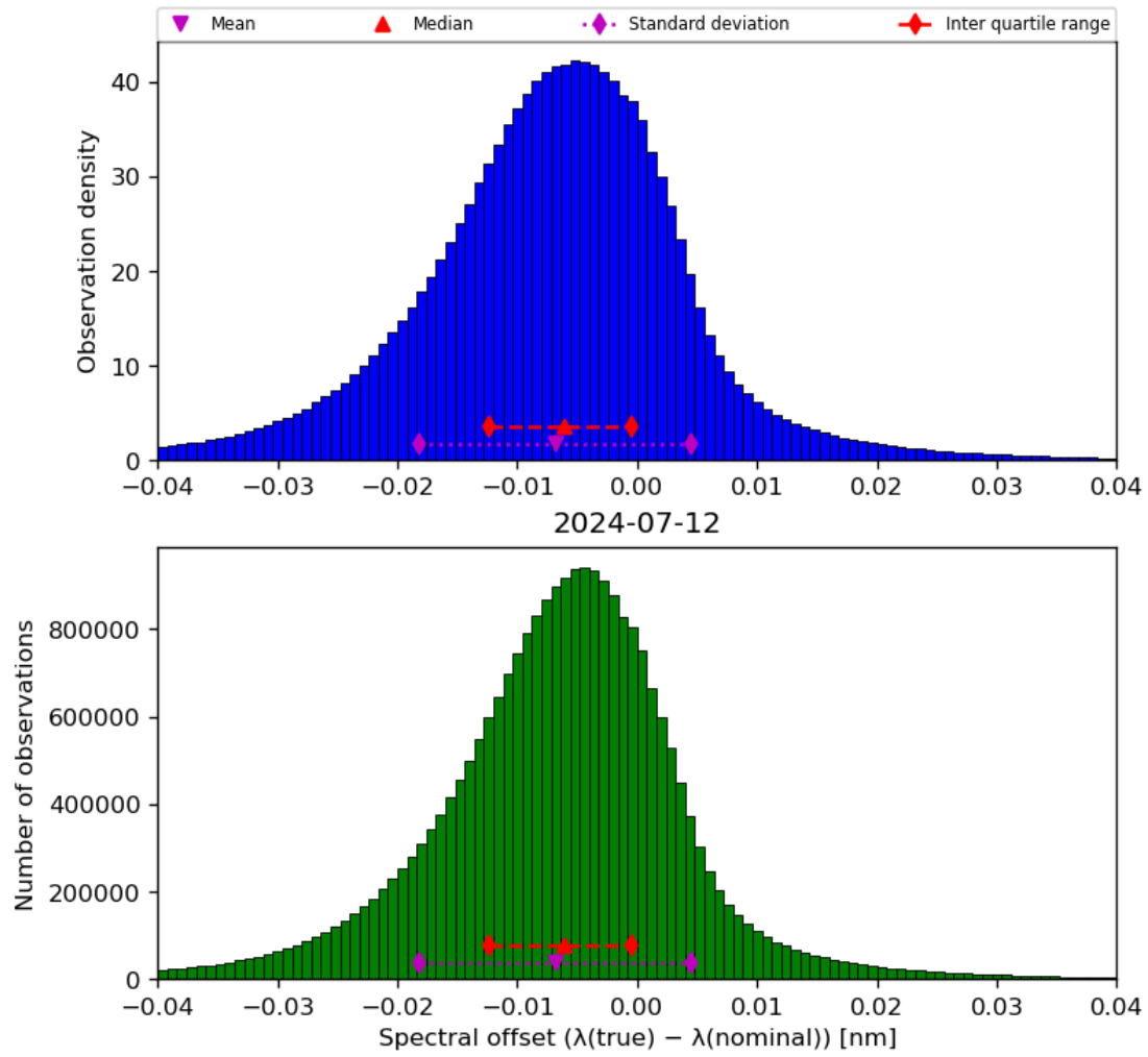
Figure 45: Histogram of “Spectral offset ( \lambda(\text{true}) - \lambda(\text{nominal}) )” for 2024-07-11 to 2024-07-13
