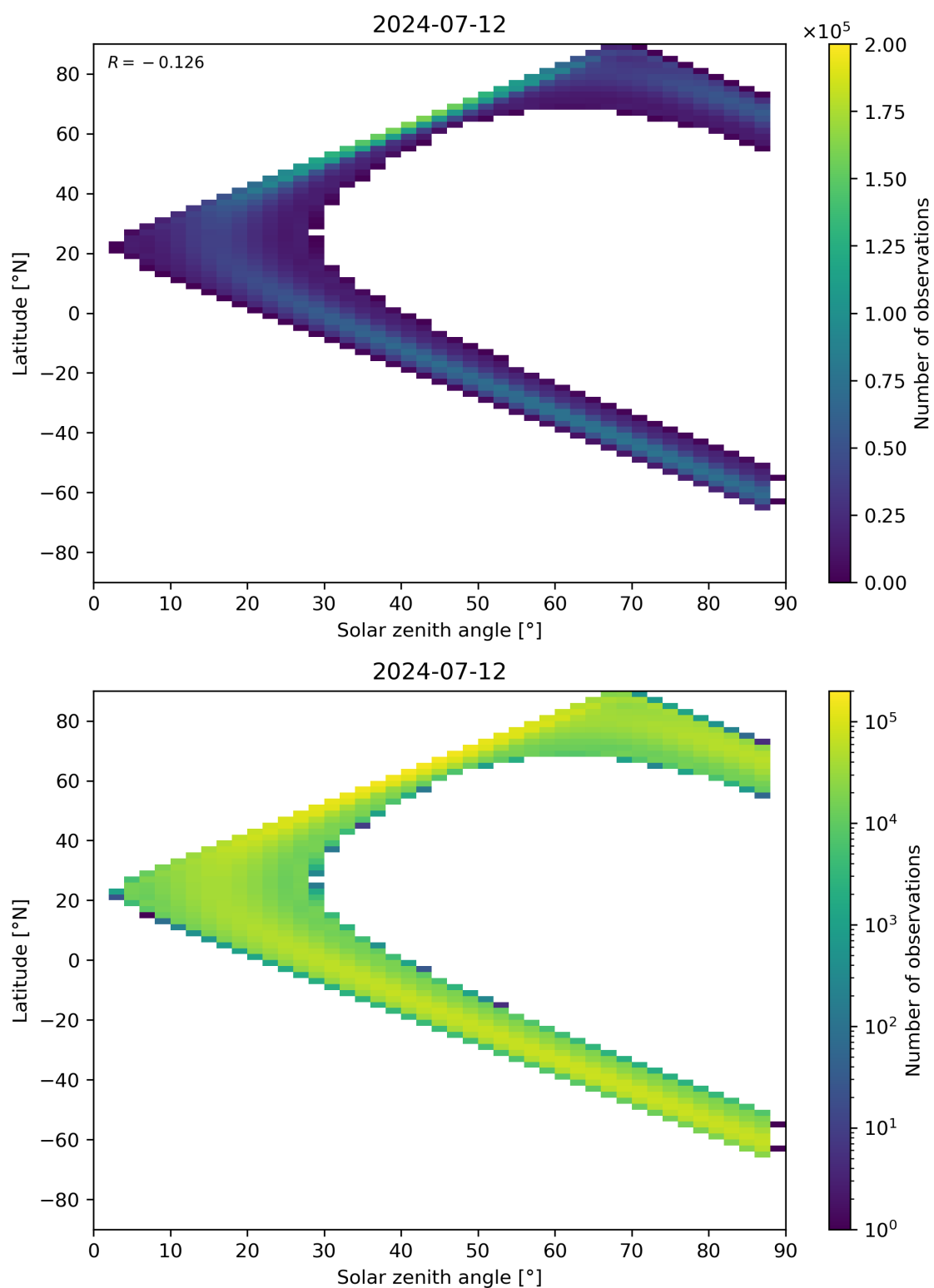
Figure 113: Scatter density plot of “Solar zenith angle” against “Latitude” for 2024-07-11 to 2024-07-13.
