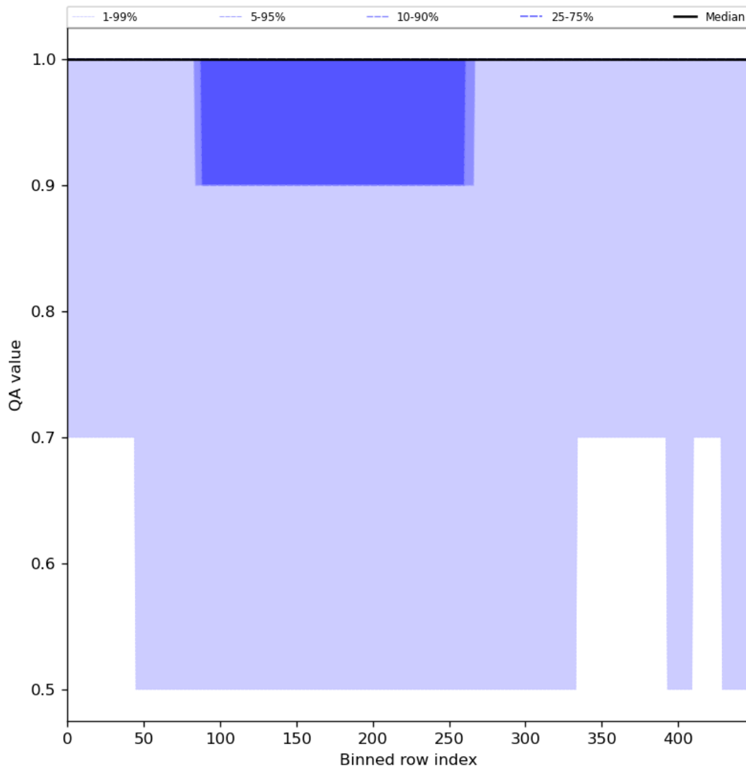
Figure 46: Along track statistics of “QA value” for 2024-07-11 to 2024-07-13
