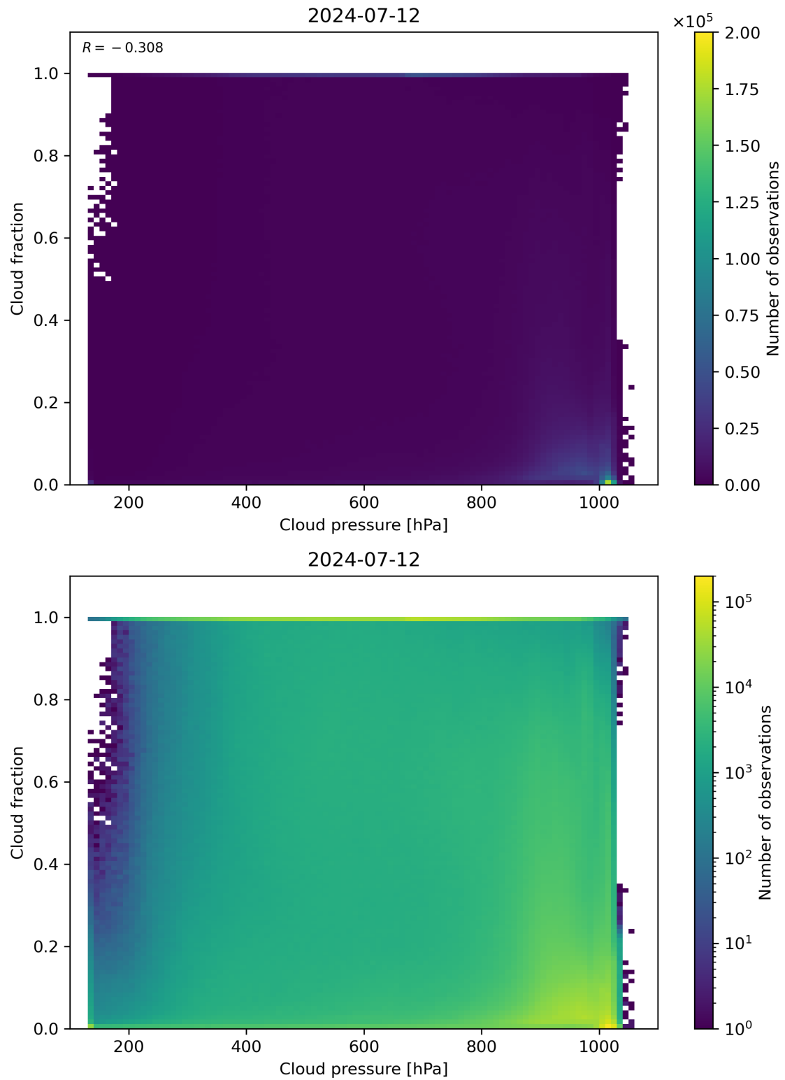
Figure 79: Scatter density plot of “Cloud pressure” against “Cloud fraction” for 2024-07-11 to 2024-07-13.
