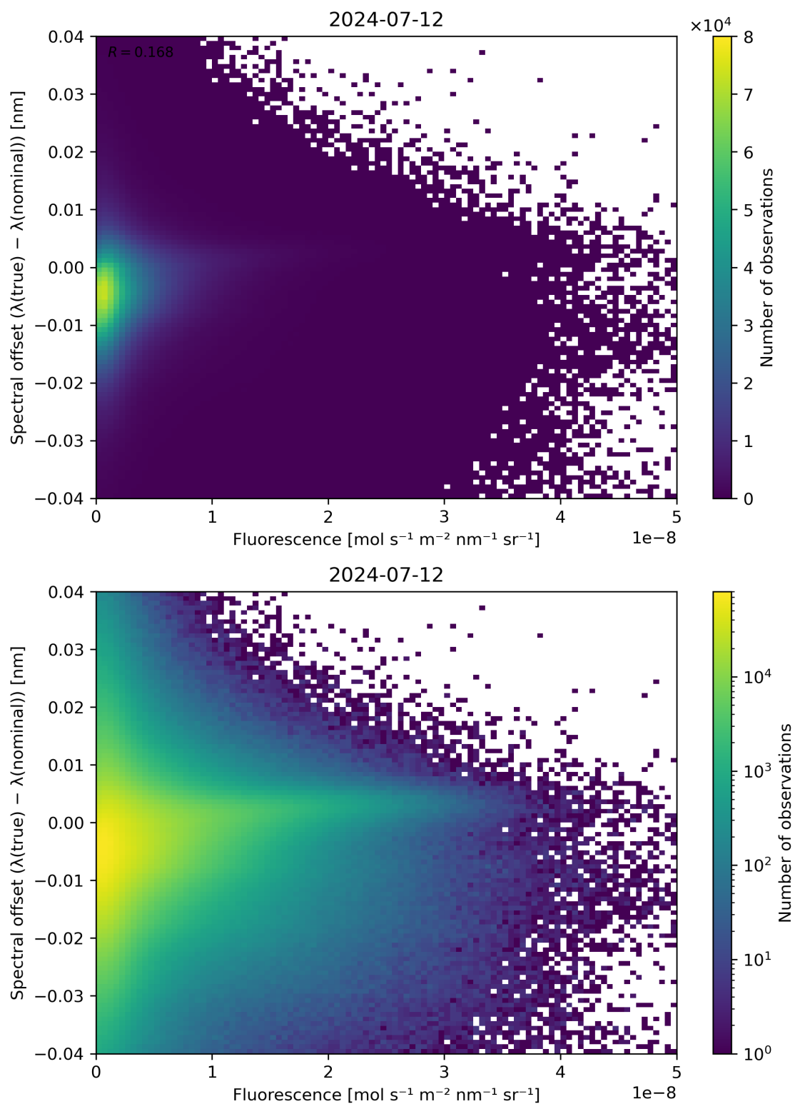
Figure 87: Scatter density plot of “Fluorescence” against “Spectral offset ( \lambda(\text{true}) - \lambda(\text{nominal}) )” for 2024-07-11 to 2024-07-13.
