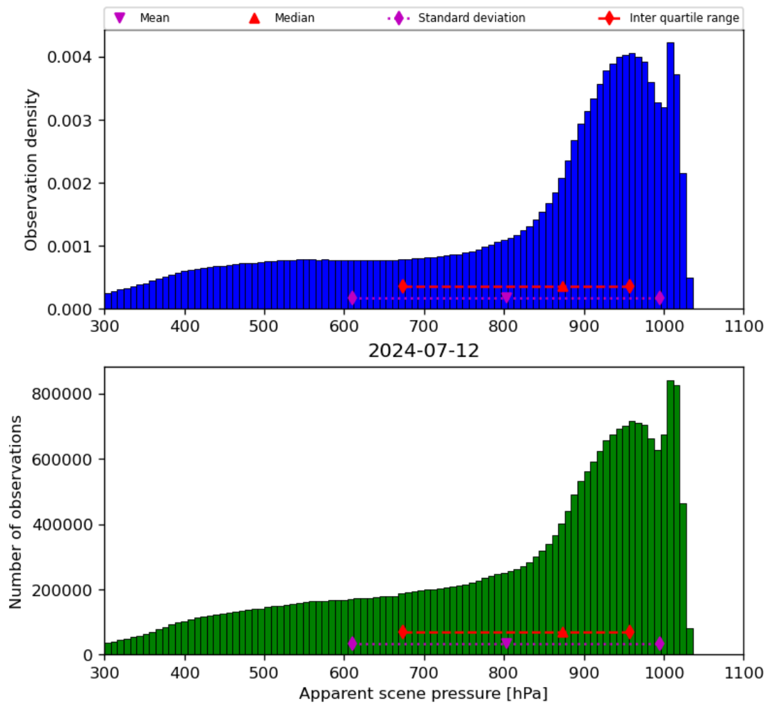
Figure 36: Histogram of “Apparent scene pressure” for 2024-07-11 to 2024-07-13
