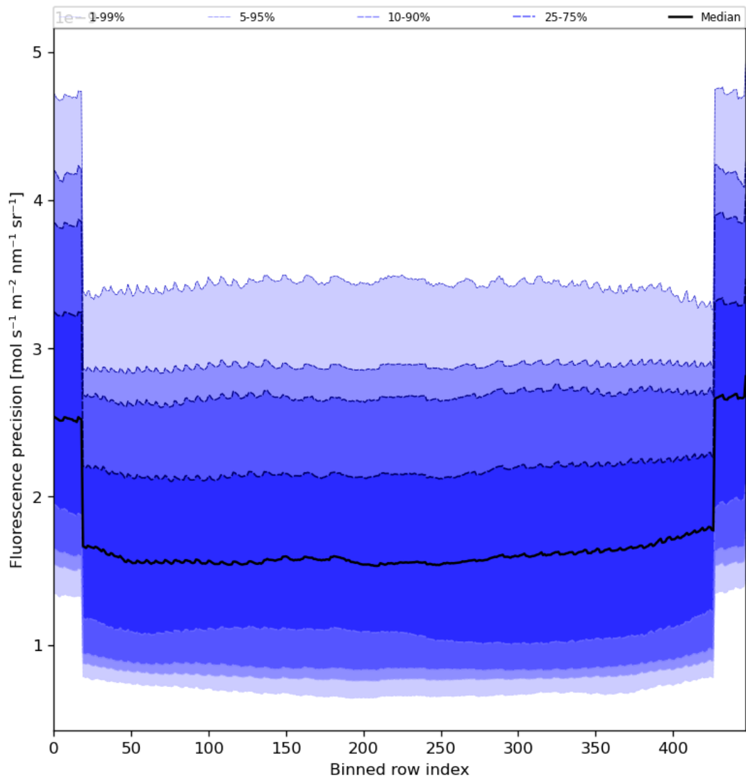
Figure 58: Along track statistics of “Fluorescence precision” for 2024-07-11 to 2024-07-13
