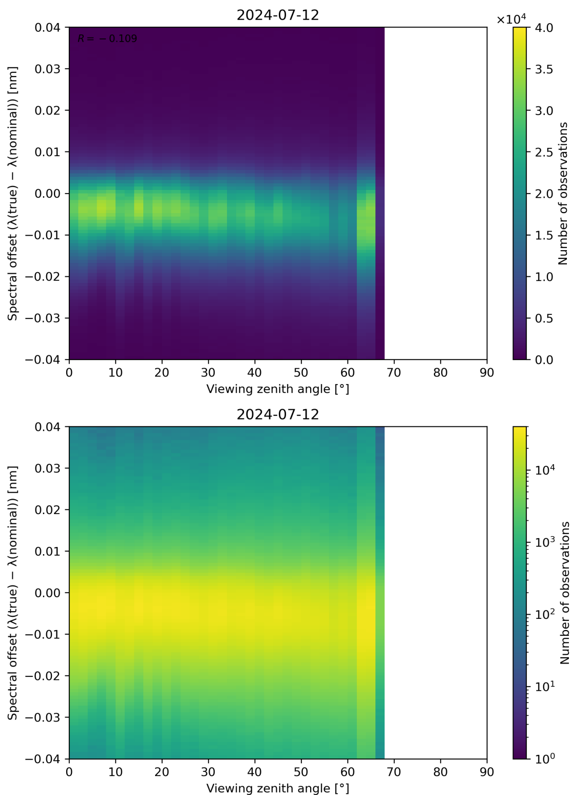
Figure 128: Scatter density plot of “Viewing zenith angle” against “Spectral offset ( \lambda(\text{true}) - \lambda(\text{nominal}) )” for 2024-07-11 to 2024-07-13.
