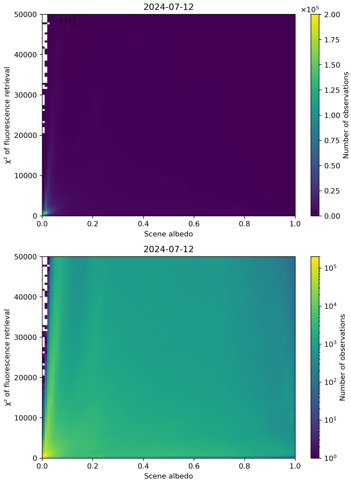
Figure 103: Scatter density plot of “Scene albedo” against “ \chi^2 of fluorescence retrieval” for 2024-07-11 to 2024-07-13.
