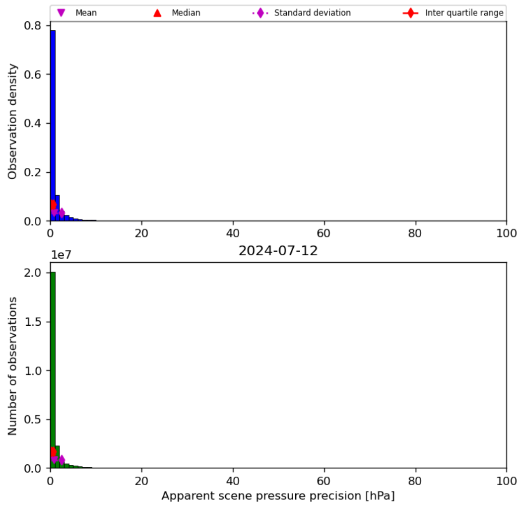
Figure 37: Histogram of “Apparent scene pressure precision” for 2024-07-11 to 2024-07-13
