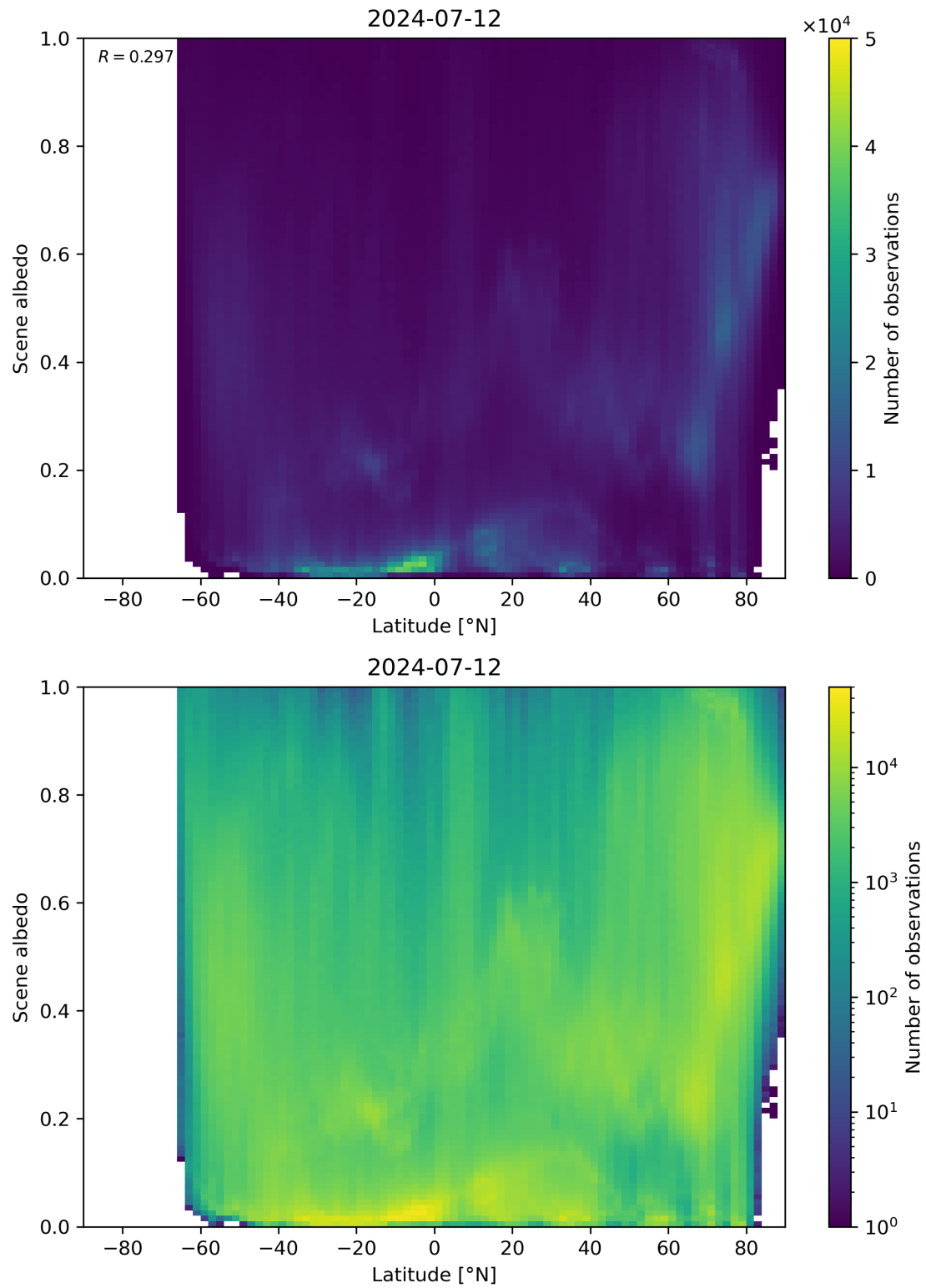
Figure 95: Scatter density plot of “Latitude” against “Scene albedo” for 2024-07-11 to 2024-07-13.
