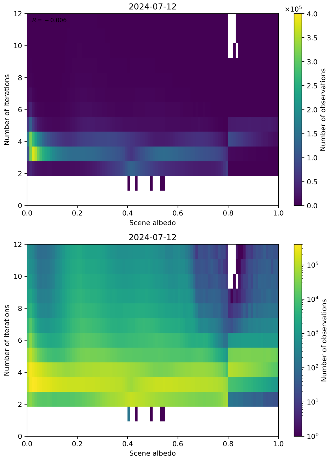
Figure 105: Scatter density plot of “Scene albedo” against “Number of iterations” for 2024-07-11 to 2024-07-13.
