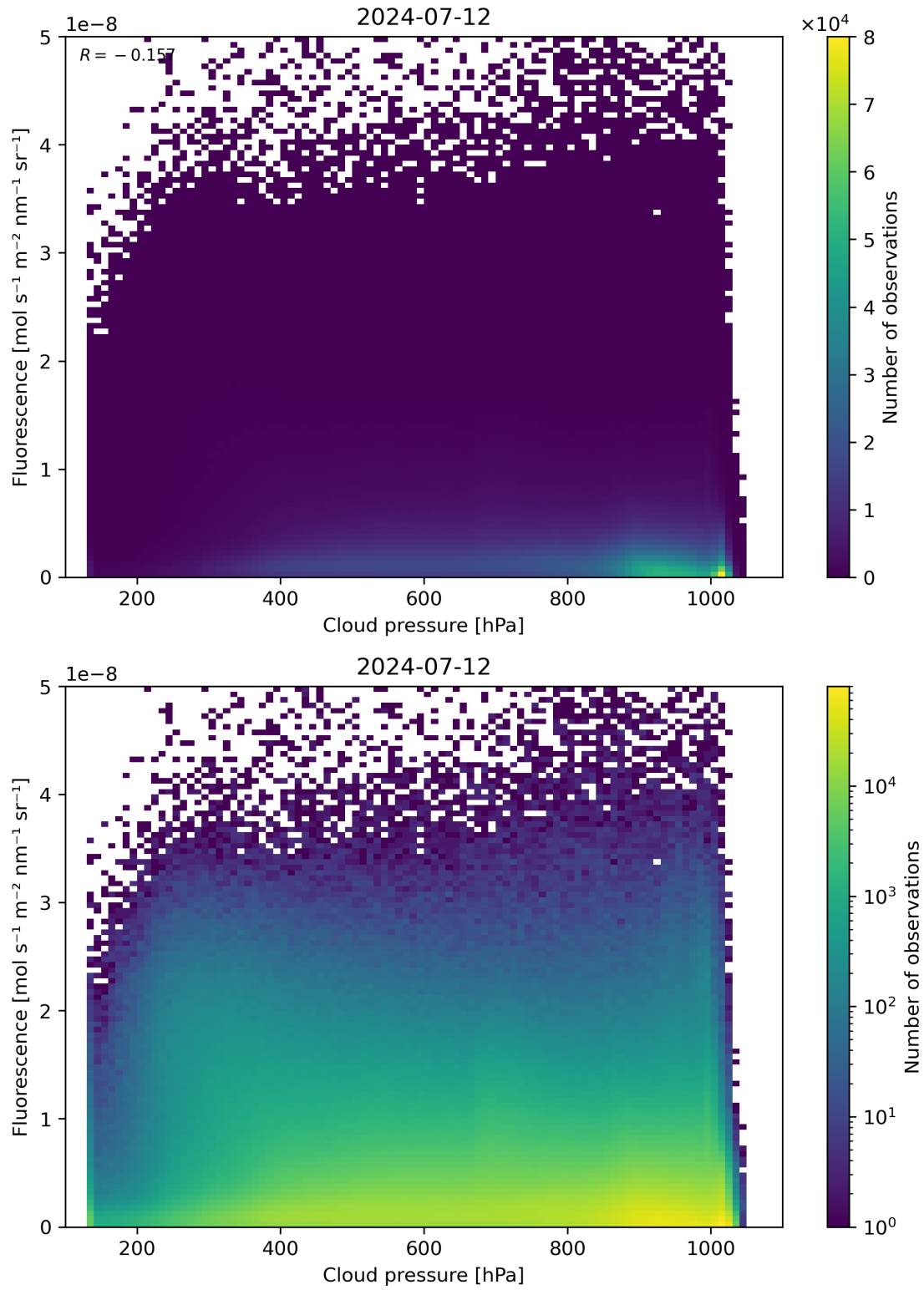
Figure 80: Scatter density plot of “Cloud pressure” against “Fluorescence” for 2024-07-11 to 2024-07-13.
