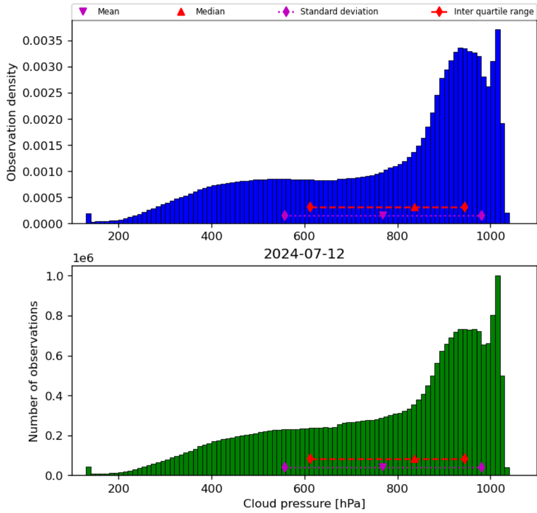
Figure 30: Histogram of “Cloud pressure” for 2024-07-11 to 2024-07-13
