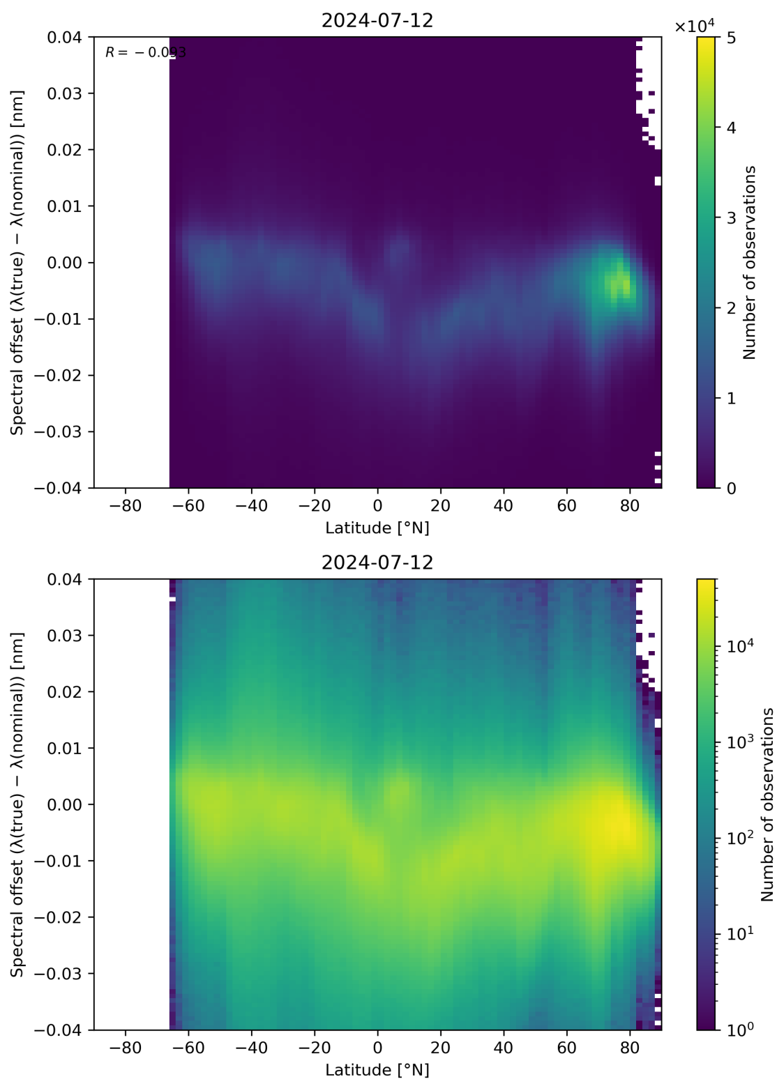
Figure 96: Scatter density plot of “Latitude” against “Spectral offset ( \lambda(\text{true}) - \lambda(\text{nominal}) )” for 2024-07-11 to 2024-07-13.
