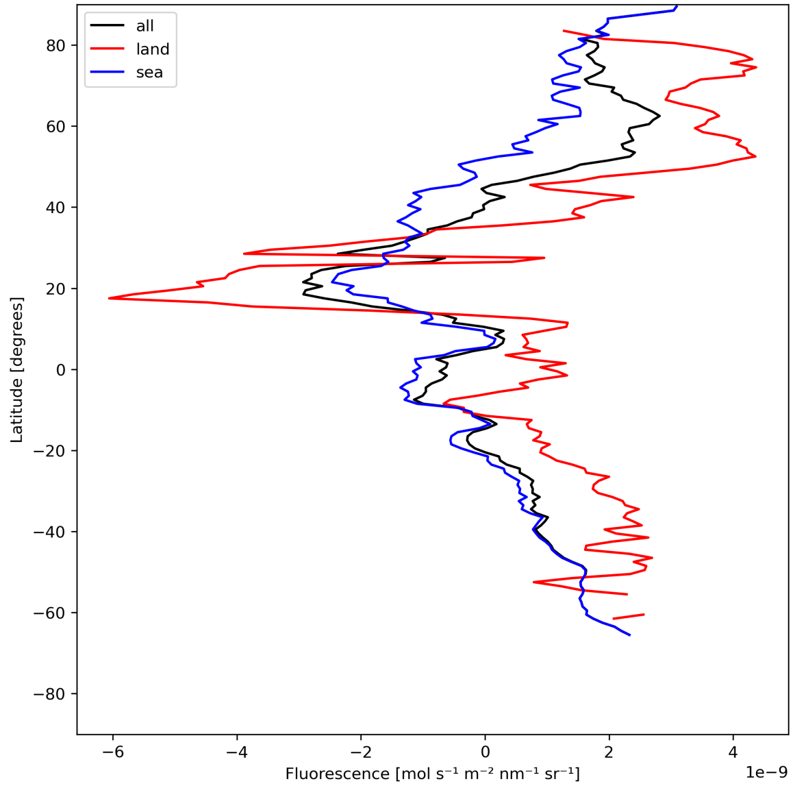
Figure 23: Zonal average of “Fluorescence” for 2024-07-11 to 2024-07-13.
