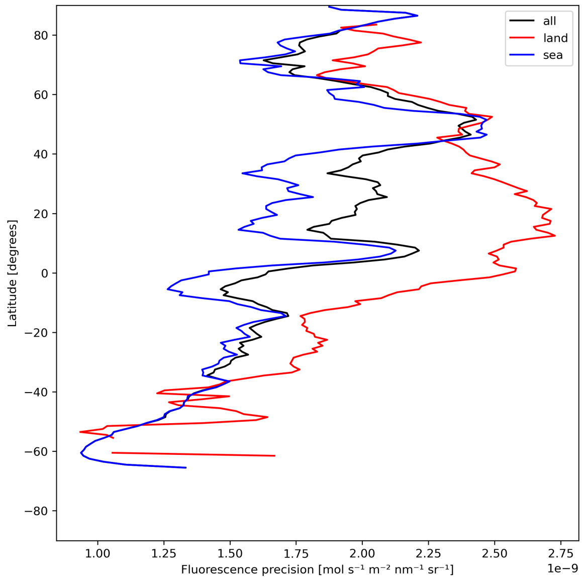
Figure 24: Zonal average of “Fluorescence precision” for 2024-07-11 to 2024-07-13.
