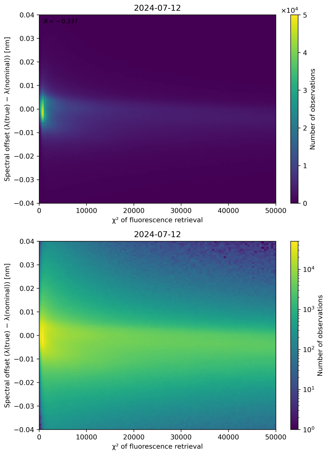
Figure 69: Scatter density plot of “ \chi^2 of fluorescence retrieval” against “Spectral offset ( \lambda(\text{true}) - \lambda(\text{nominal}) )” for 2024-07-11 to 2024-07-13.
