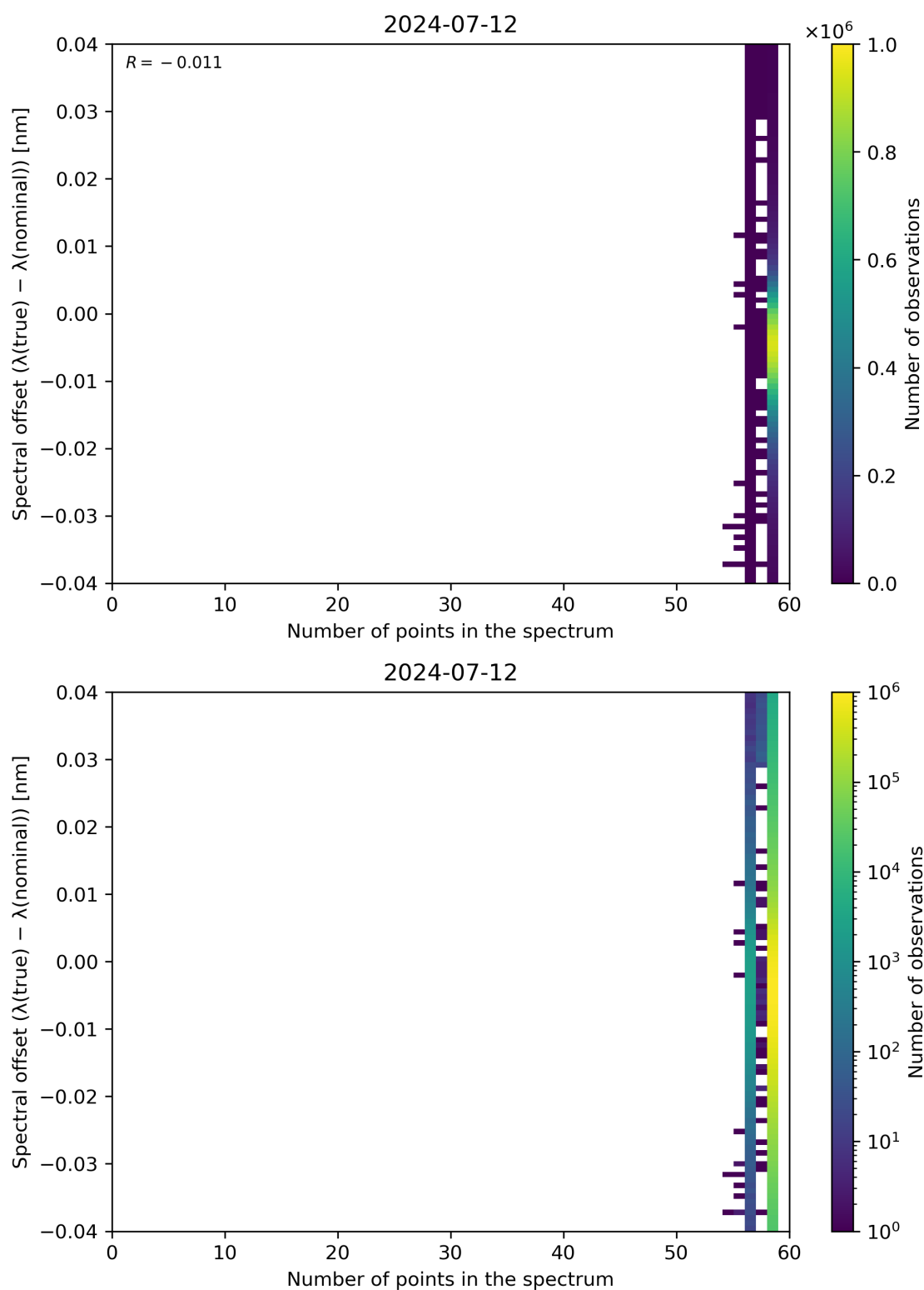
Figure 101: Scatter density plot of “Number of points in the spectrum” against “Spectral offset ( \lambda(\text{true}) - \lambda(\text{nominal}) )” for 2024-07-11 to 2024-07-13.
