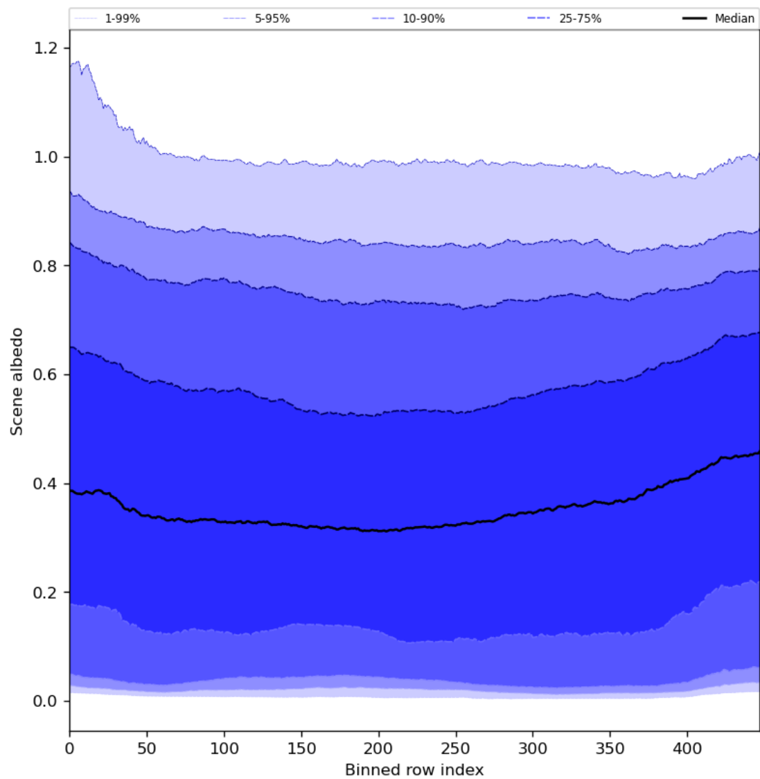
Figure 51: Along track statistics of “Scene albedo” for 2024-07-11 to 2024-07-13
