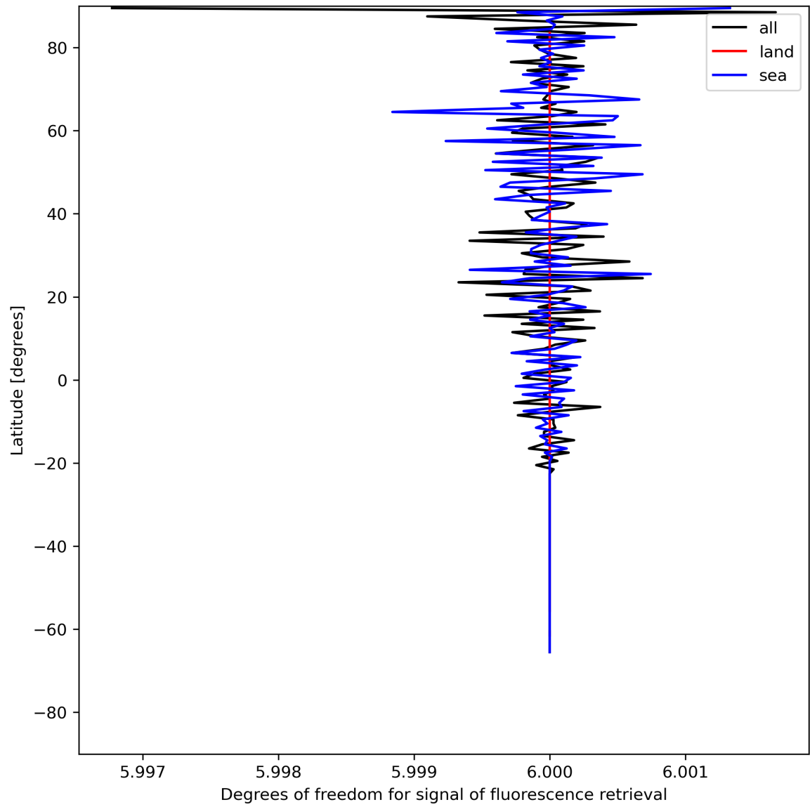
Figure 26: Zonal average of “Degrees of freedom for signal of fluorescence retrieval” for 2024-07-11 to 2024-07-13.
