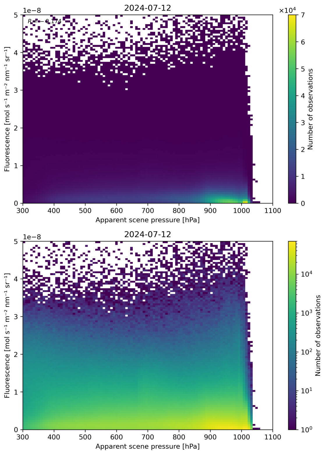
Figure 64: Scatter density plot of “Apparent scene pressure” against “Fluorescence” for 2024-07-11 to 2024-07-13.
