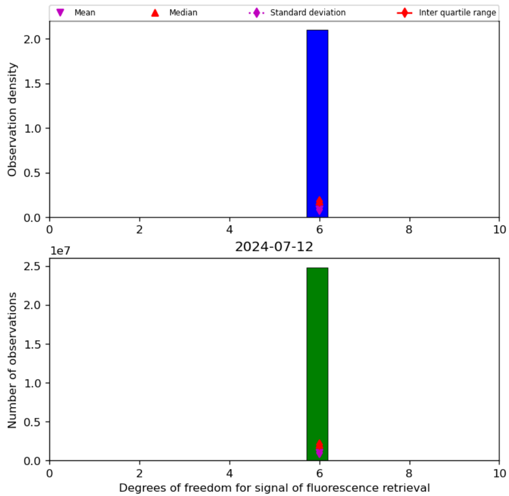
Figure 43: Histogram of “Degrees of freedom for signal of fluorescence retrieval” for 2024-07-11 to 2024-07-13
