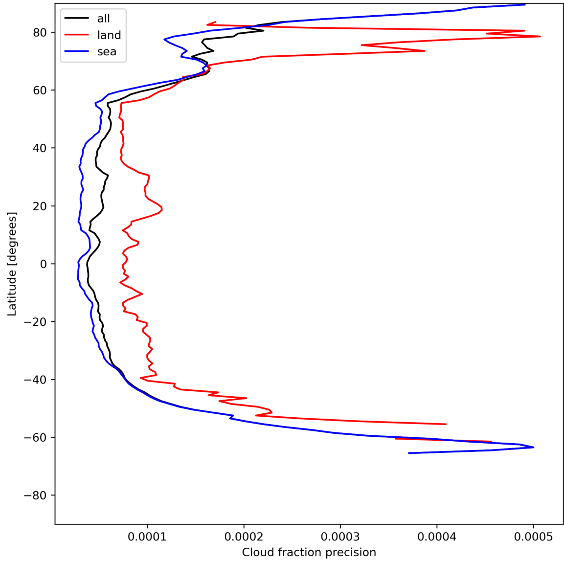
Figure 16: Zonal average of “Cloud fraction precision” for 2024-07-11 to 2024-07-13.
