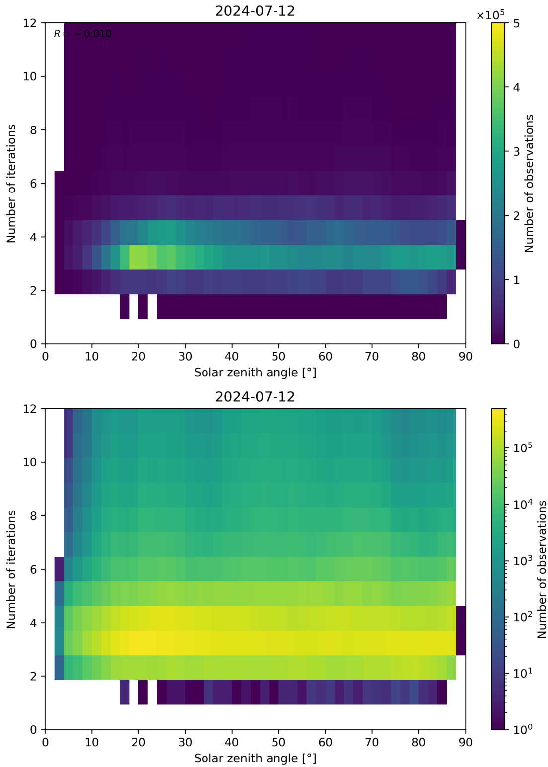
Figure 114: Scatter density plot of “Solar zenith angle” against “Number of iterations” for 2024-07-11 to 2024-07-13.
