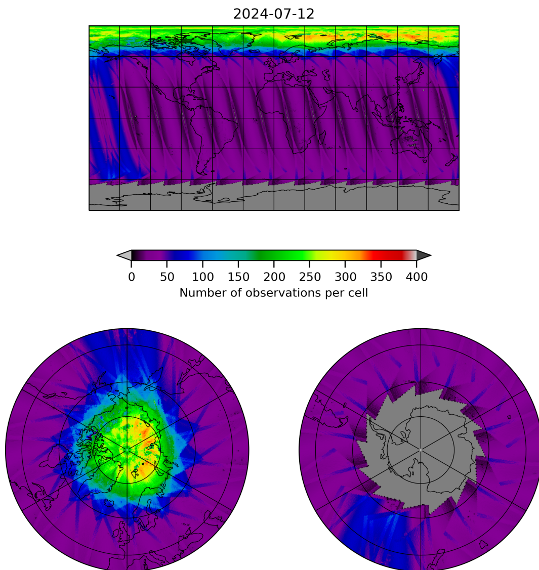
Figure 11: Map of the number of observations for 2024-07-11 to 2024-07-13
