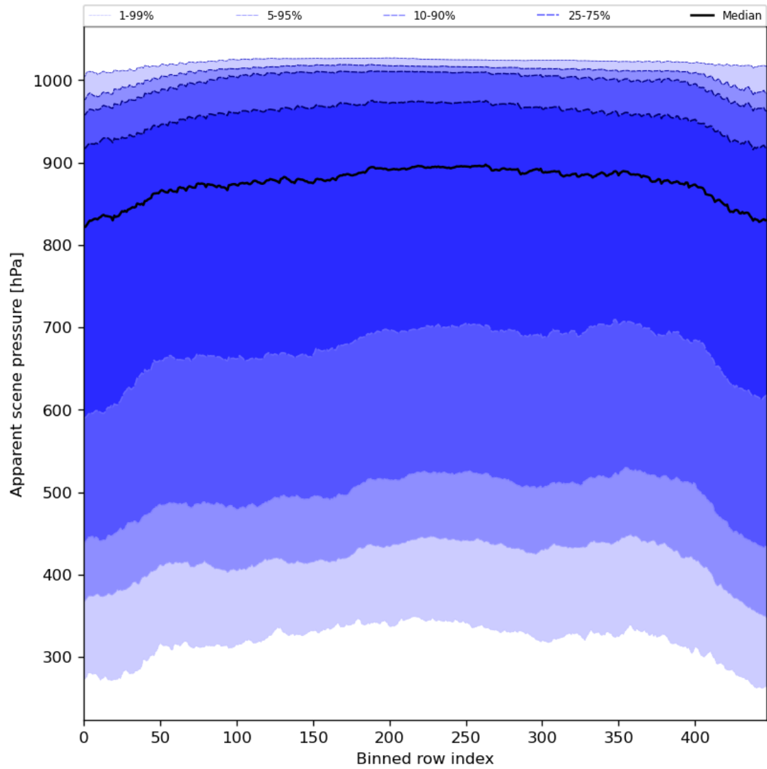
Figure 53: Along track statistics of “Apparent scene pressure” for 2024-07-11 to 2024-07-13
