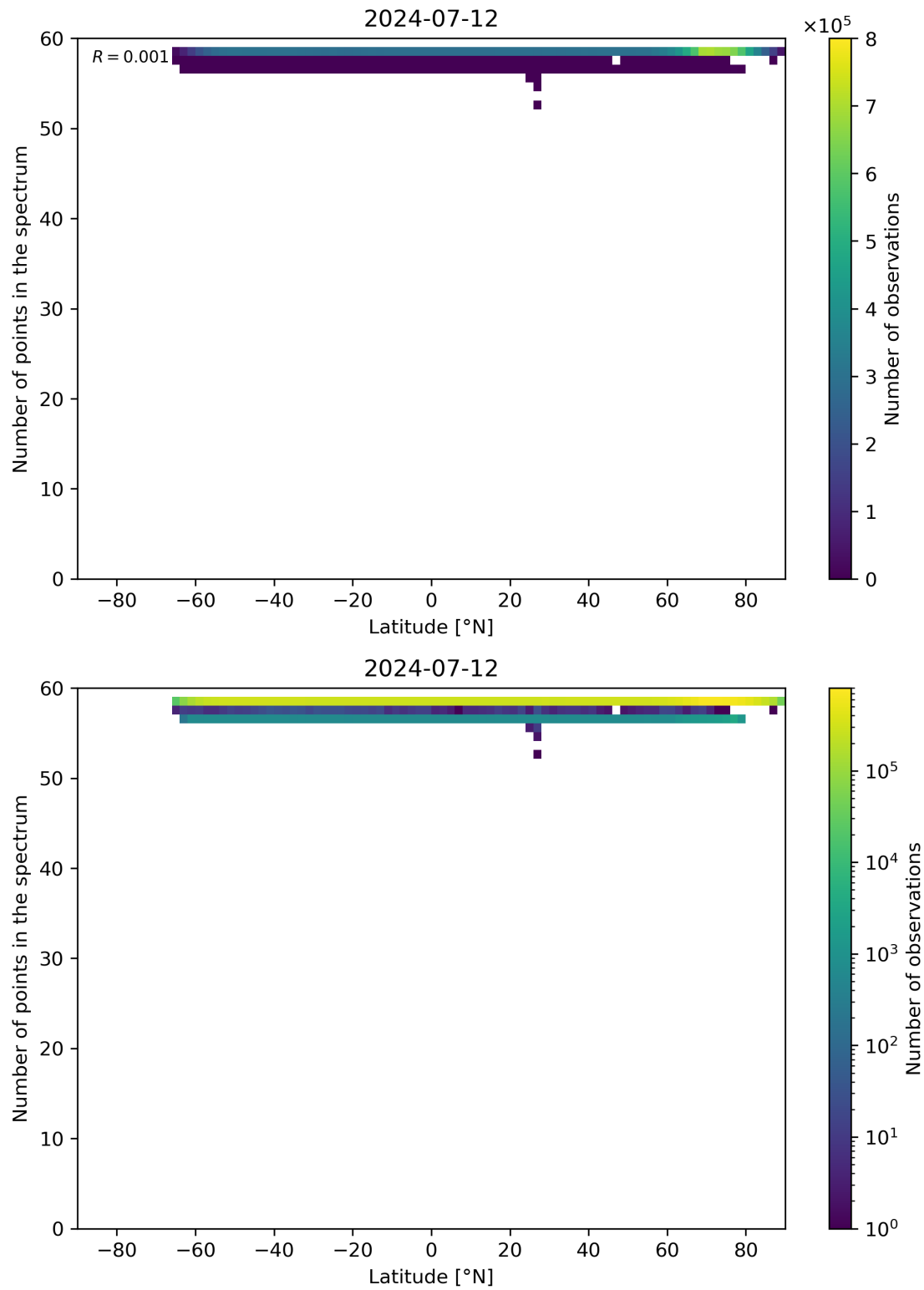
Figure 94: Scatter density plot of “Latitude” against “Number of points in the spectrum” for 2024-07-11 to 2024-07-13.
