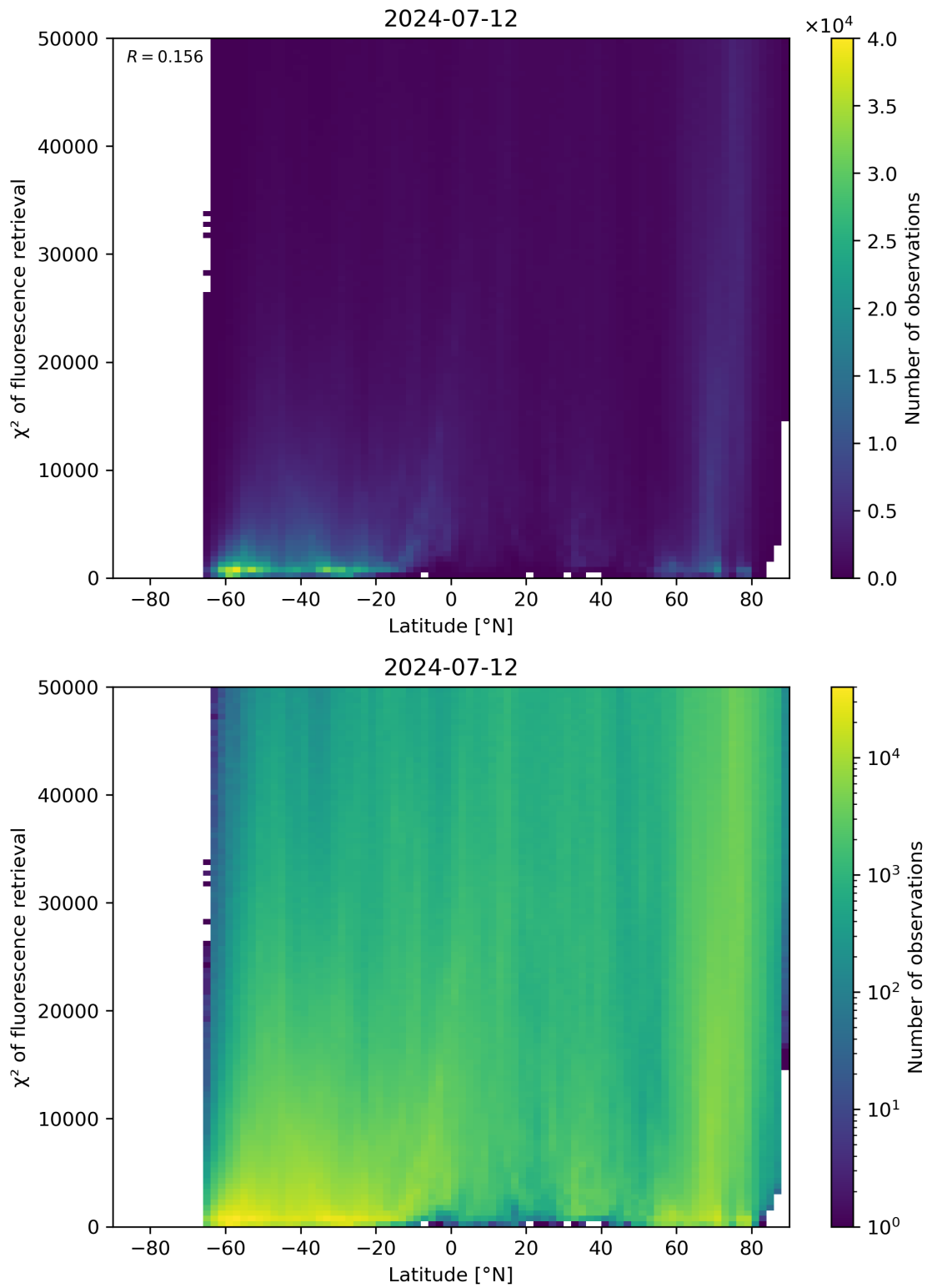
Figure 89: Scatter density plot of “Latitude” against “ \chi^2 of fluorescence retrieval” for 2024-07-11 to 2024-07-13.
