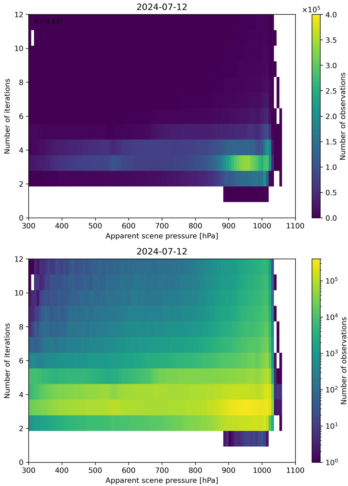
Figure 65: Scatter density plot of “Apparent scene pressure” against “Number of iterations” for 2024-07-11 to 2024-07-13.
