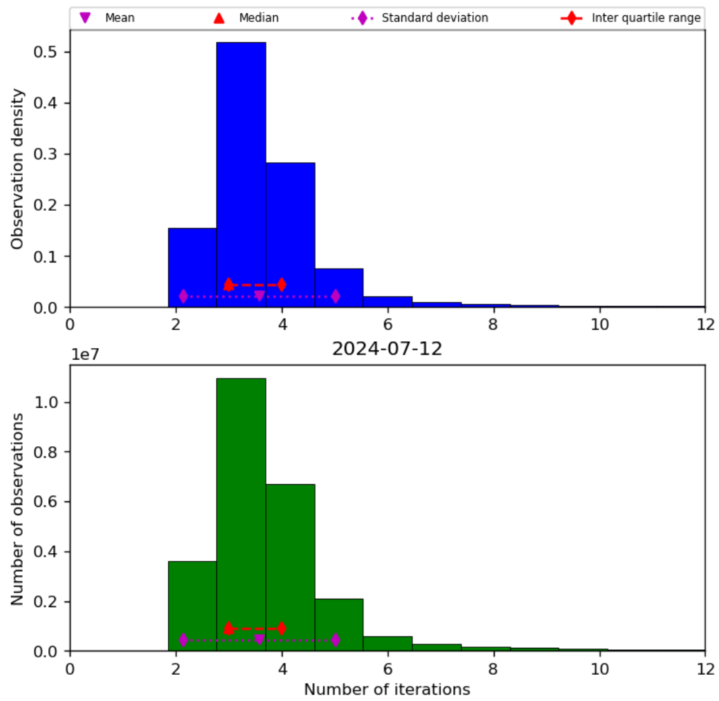
Figure 39: Histogram of “Number of iterations” for 2024-07-11 to 2024-07-13
