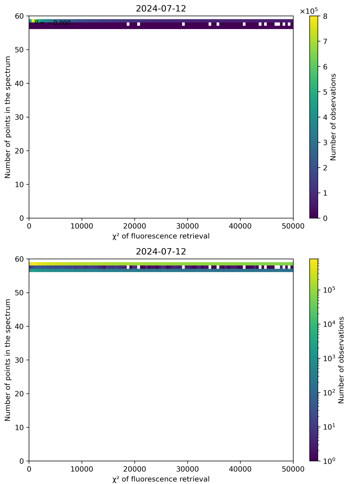
Figure 68: Scatter density plot of “ \chi^2 of fluorescence retrieval” against “Number of points in the spectrum” for 2024-07-11 to 2024-07-13.
