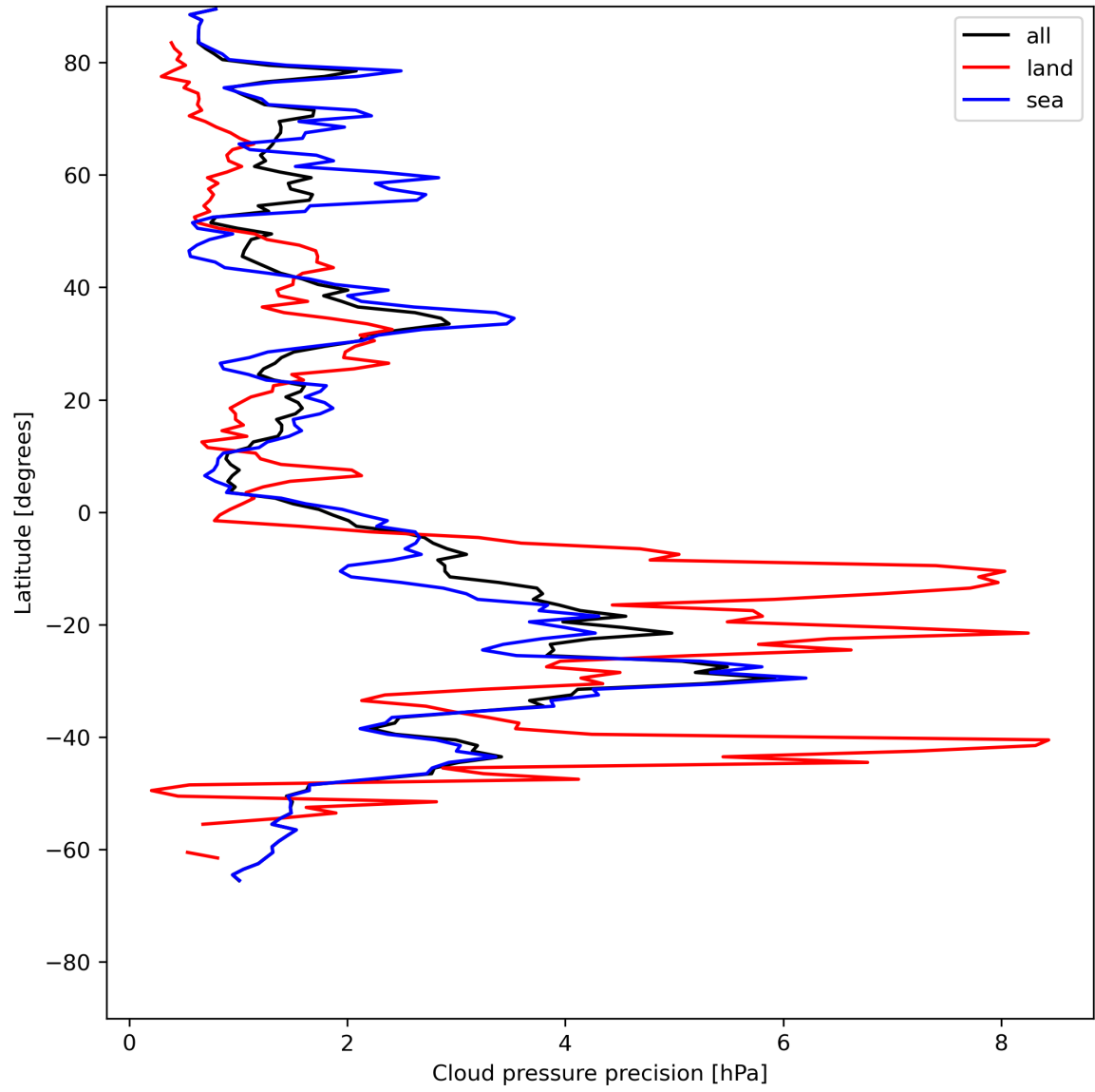
Figure 14: Zonal average of “Cloud pressure precision” for 2024-07-11 to 2024-07-13.
