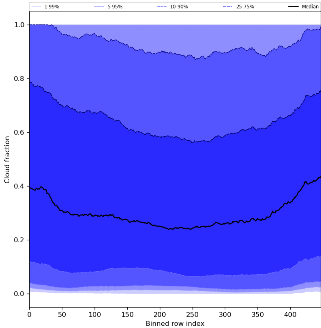
Figure 49: Along track statistics of “Cloud fraction” for 2024-07-11 to 2024-07-13
