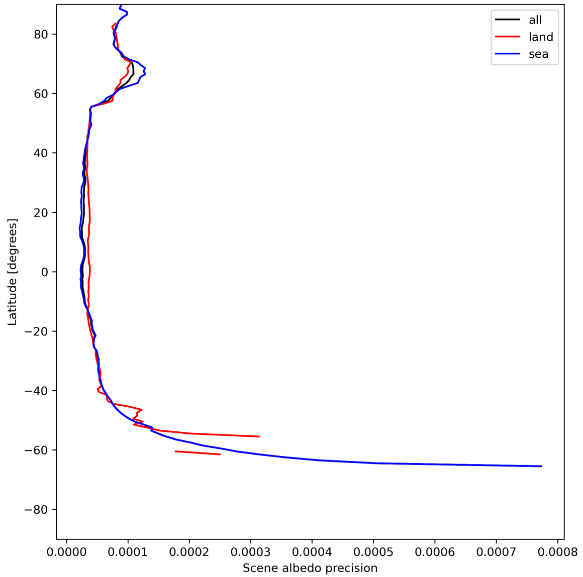
Figure 18: Zonal average of “Scene albedo precision” for 2024-07-11 to 2024-07-13.
