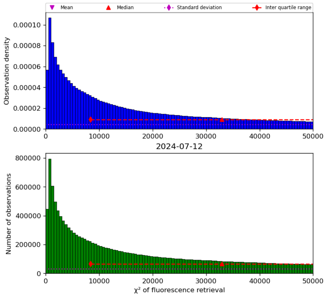
Figure 42: Histogram of “ \chi^2 of fluorescence retrieval” for 2024-07-11 to 2024-07-13
