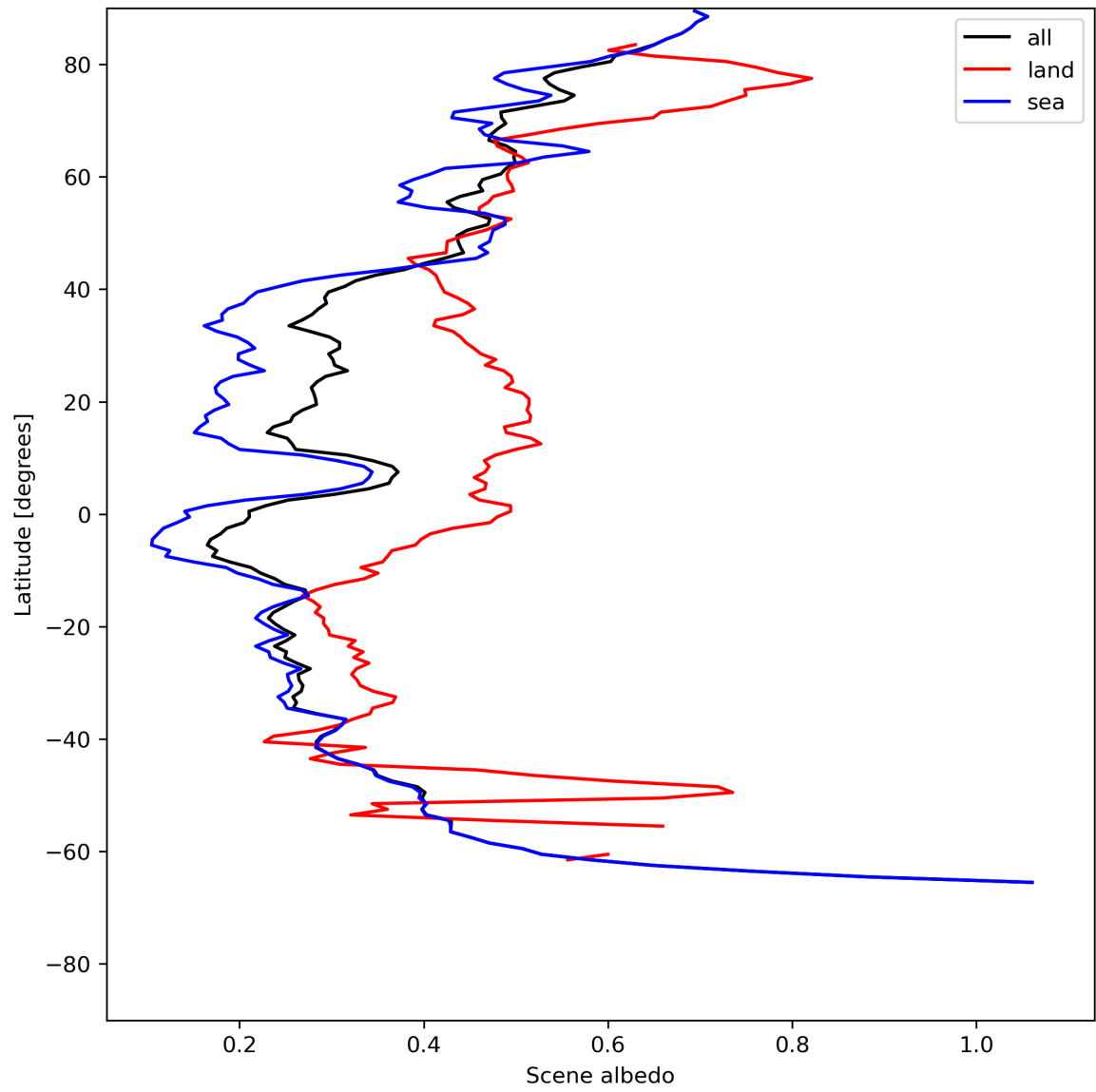
Figure 17: Zonal average of “Scene albedo” for 2024-07-11 to 2024-07-13.
