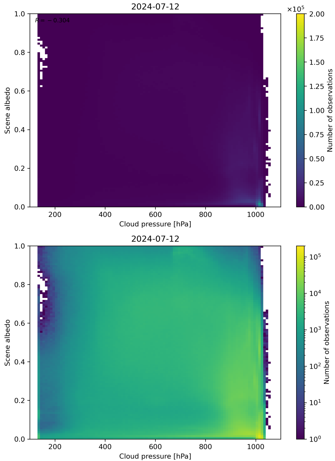
Figure 83: Scatter density plot of “Cloud pressure” against “Scene albedo” for 2024-07-11 to 2024-07-13.
