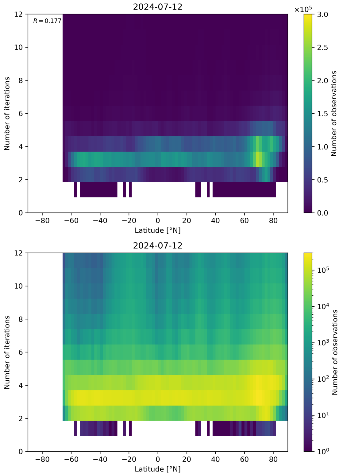
Figure 93: Scatter density plot of “Latitude” against “Number of iterations” for 2024-07-11 to 2024-07-13.
