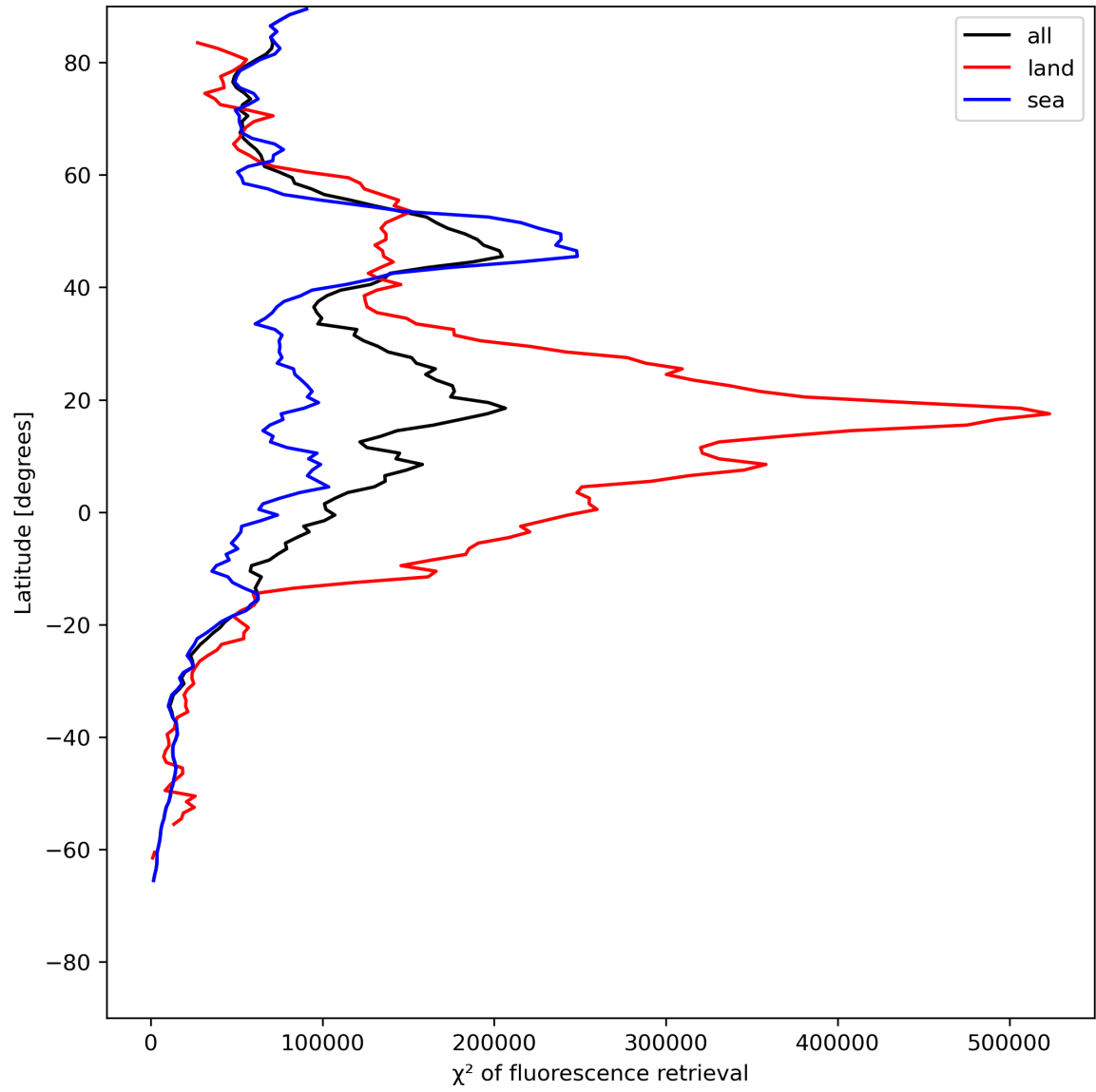
Figure 25: Zonal average of “ \chi^2 of fluorescence retrieval” for 2024-07-11 to 2024-07-13.
