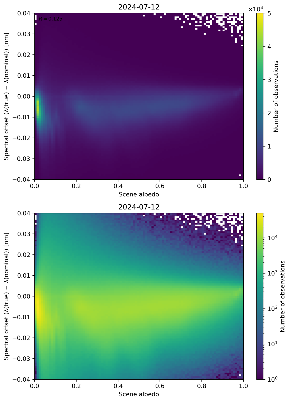
Figure 107: Scatter density plot of “Scene albedo” against “Spectral offset ( \lambda(\text{true}) - \lambda(\text{nominal}) )” for 2024-07-11 to 2024-07-13.
