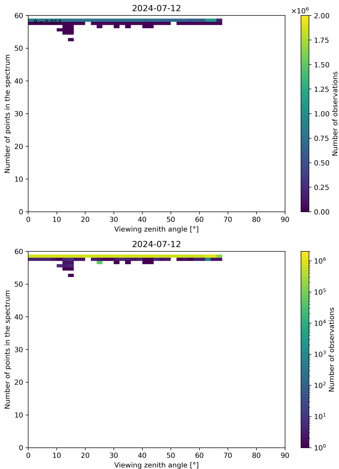
Figure 125: Scatter density plot of “Viewing zenith angle” against “Number of points in the spectrum” for 2024-07-11 to 2024-07-13.
