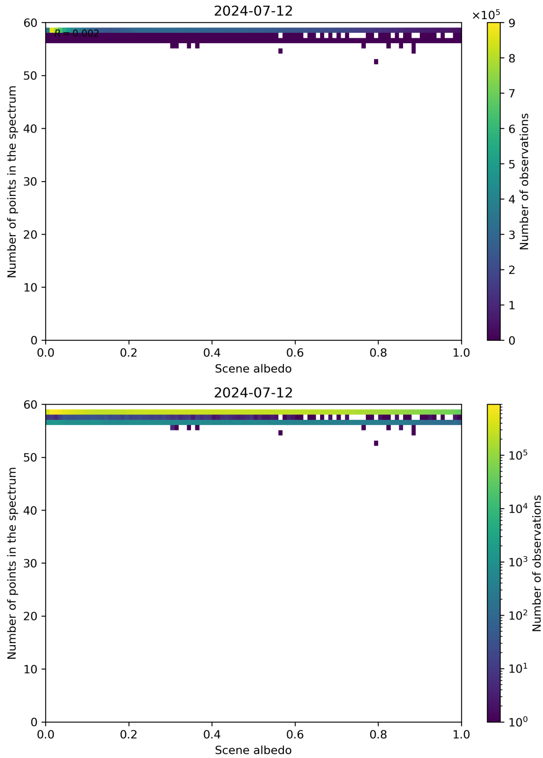
Figure 106: Scatter density plot of “Scene albedo” against “Number of points in the spectrum” for 2024-07-11 to 2024-07-13.
