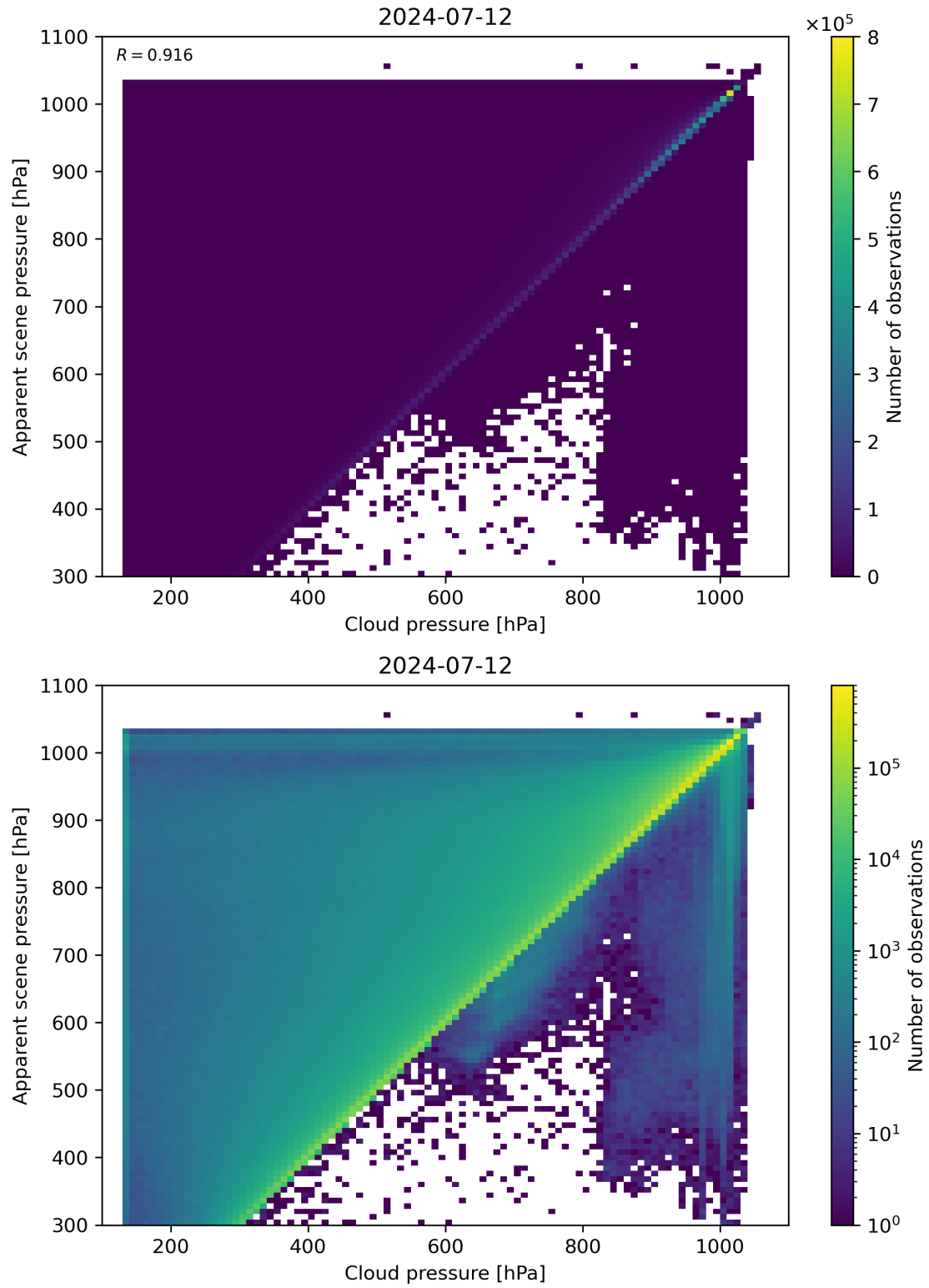
Figure 77: Scatter density plot of “Cloud pressure” against “Apparent scene pressure” for 2024-07-11 to 2024-07-13.
