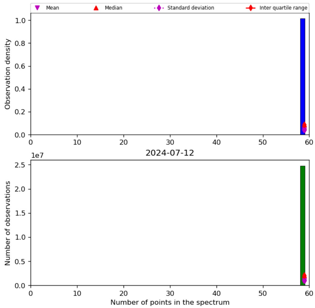
Figure 44: Histogram of “Number of points in the spectrum” for 2024-07-11 to 2024-07-13
