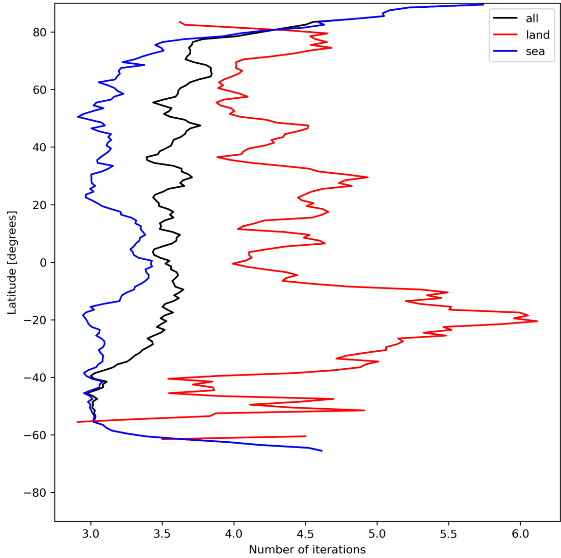
Figure 22: Zonal average of “Number of iterations” for 2024-07-11 to 2024-07-13.
