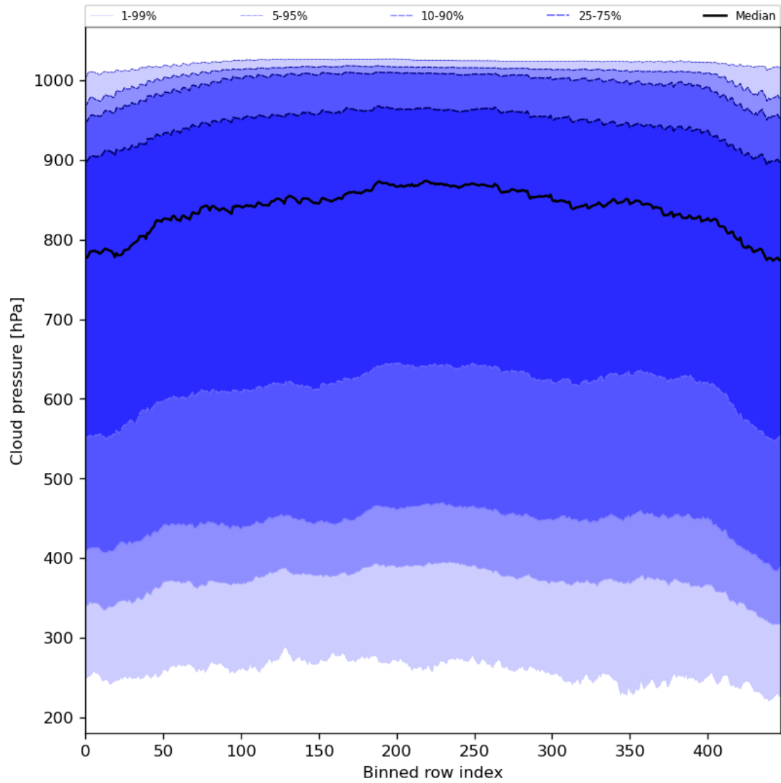
Figure 47: Along track statistics of “Cloud pressure” for 2024-07-11 to 2024-07-13
