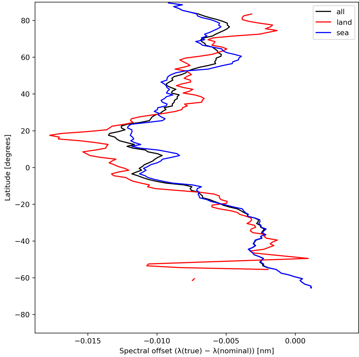
Figure 28: Zonal average of “Spectral offset ( \lambda(\text{true}) - \lambda(\text{nominal}) )” for 2024-07-11 to 2024-07-13.
