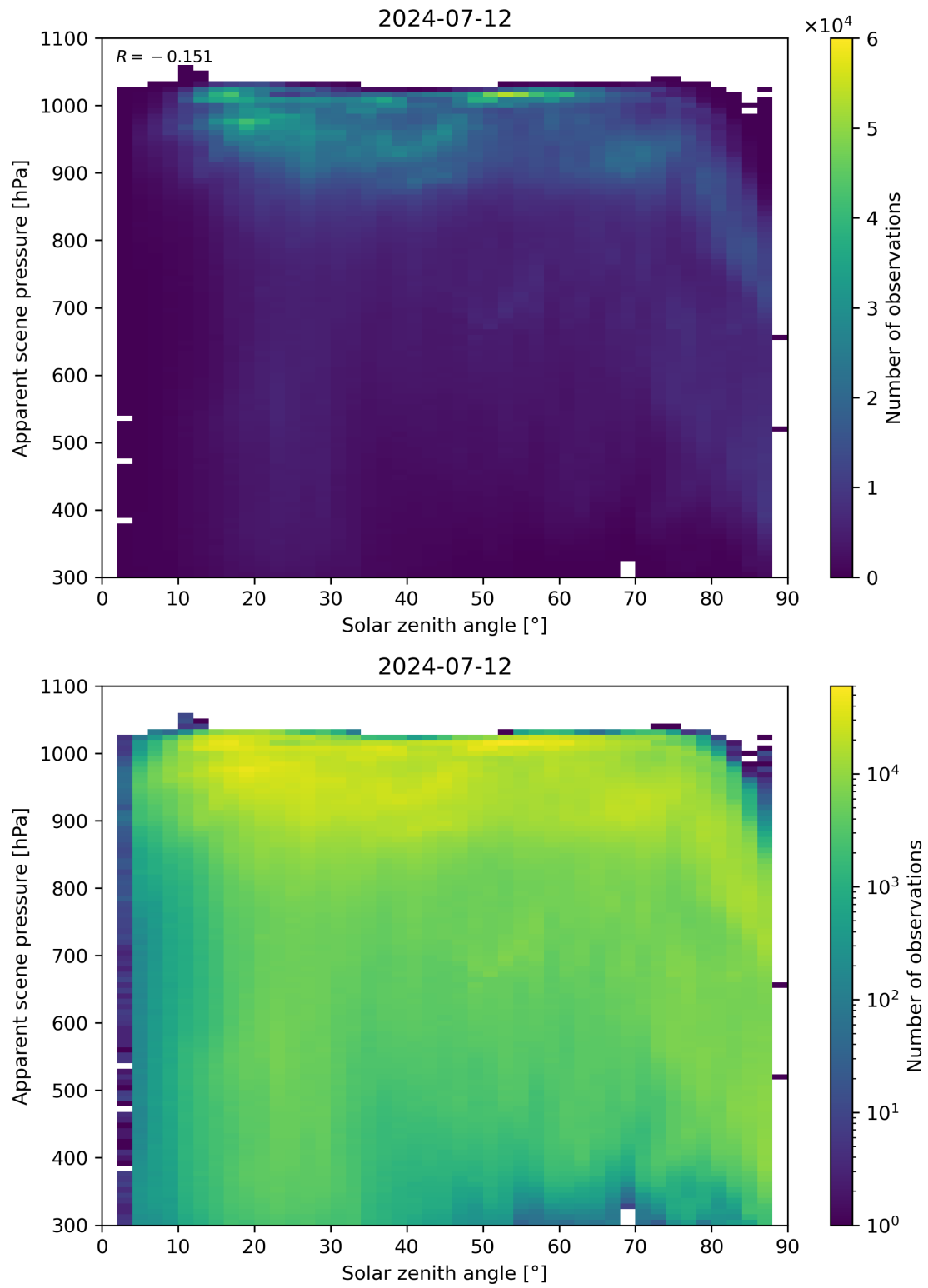
Figure 108: Scatter density plot of “Solar zenith angle” against “Apparent scene pressure” for 2024-07-11 to 2024-07-13.
