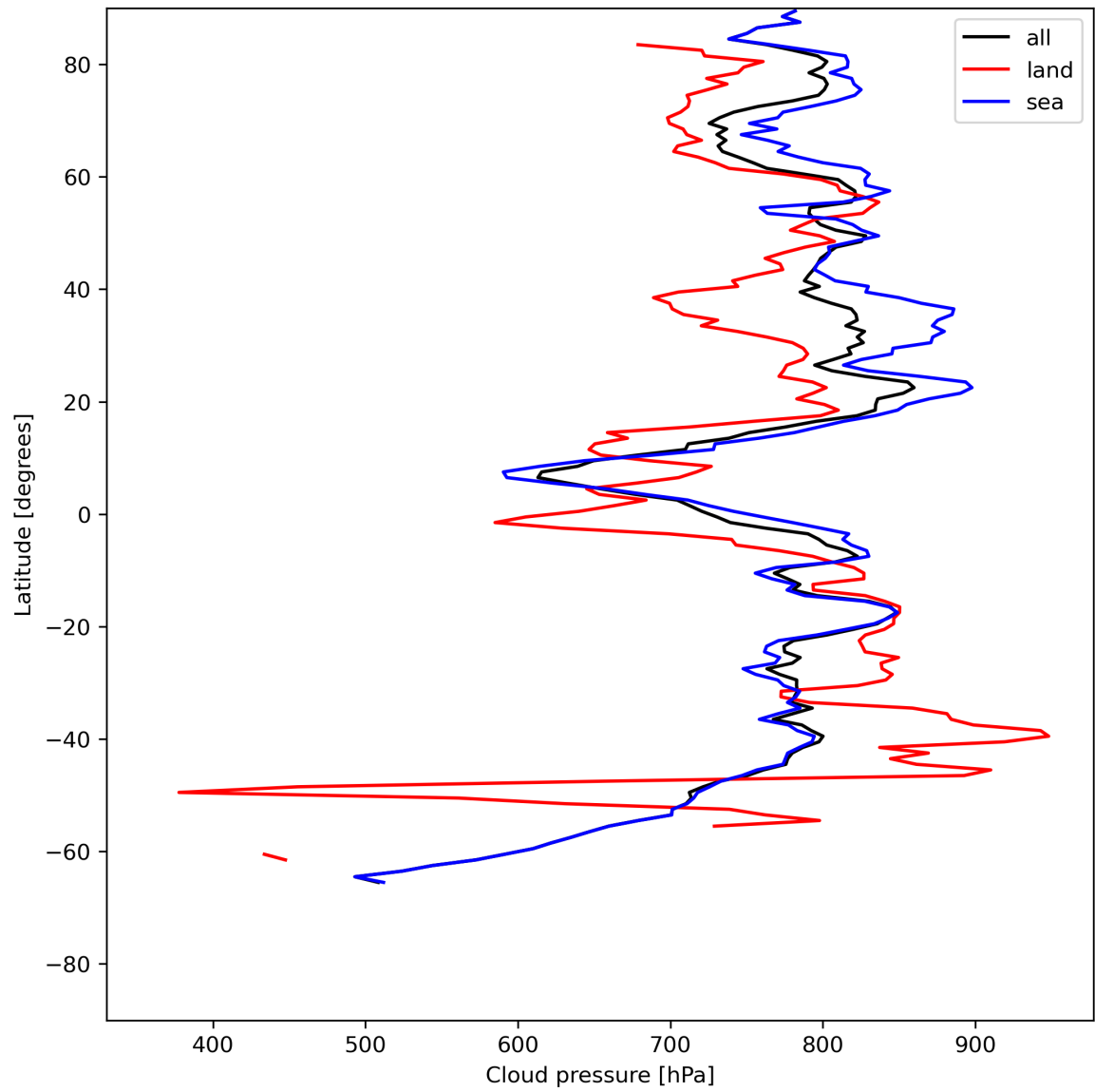
Figure 13: Zonal average of “Cloud pressure” for 2024-07-11 to 2024-07-13.
