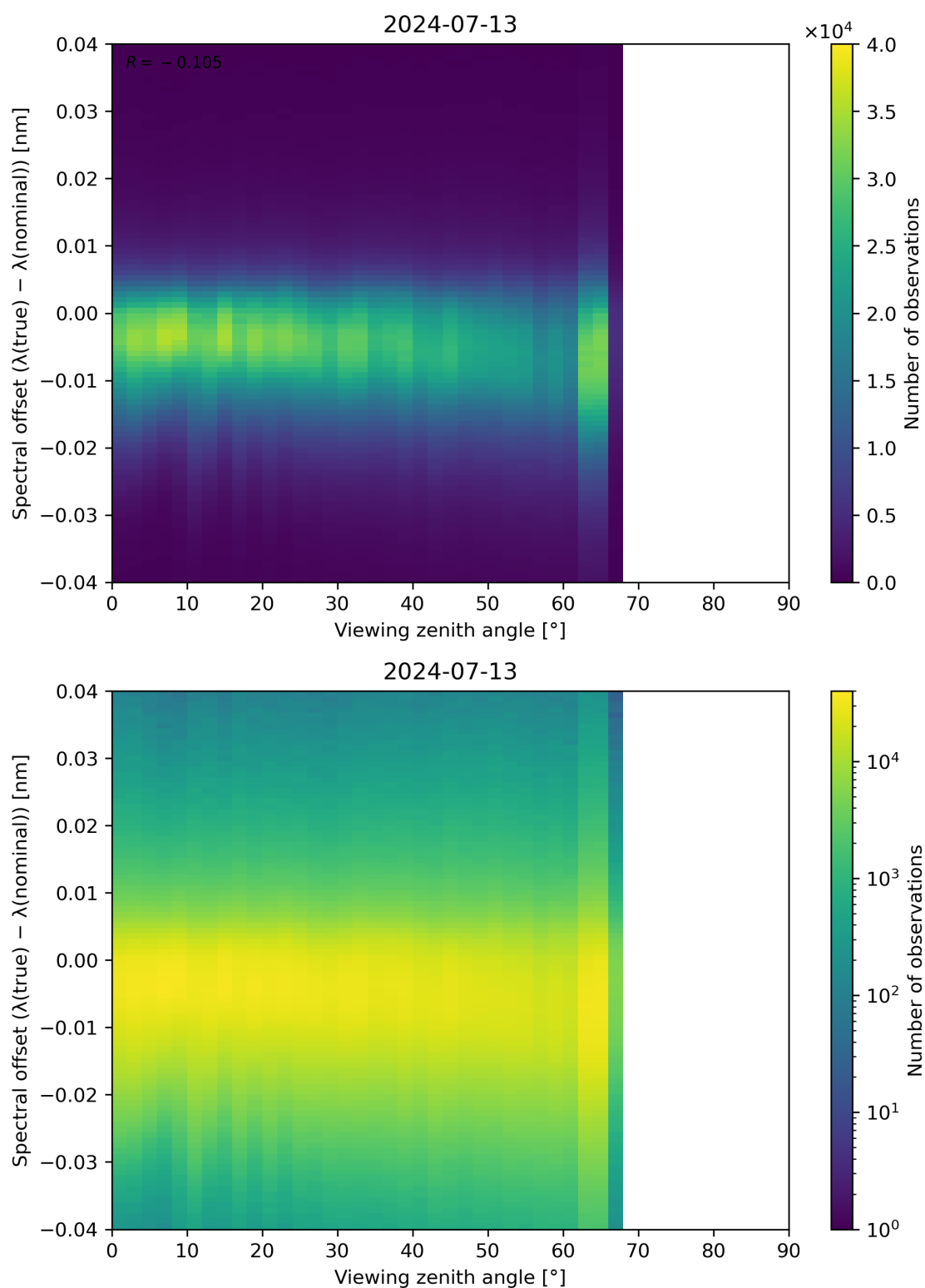
Figure 128: Scatter density plot of “Viewing zenith angle” against “Spectral offset ( \lambda(\text{true}) - \lambda(\text{nominal}) )” for 2024-07-12 to 2024-07-14.
