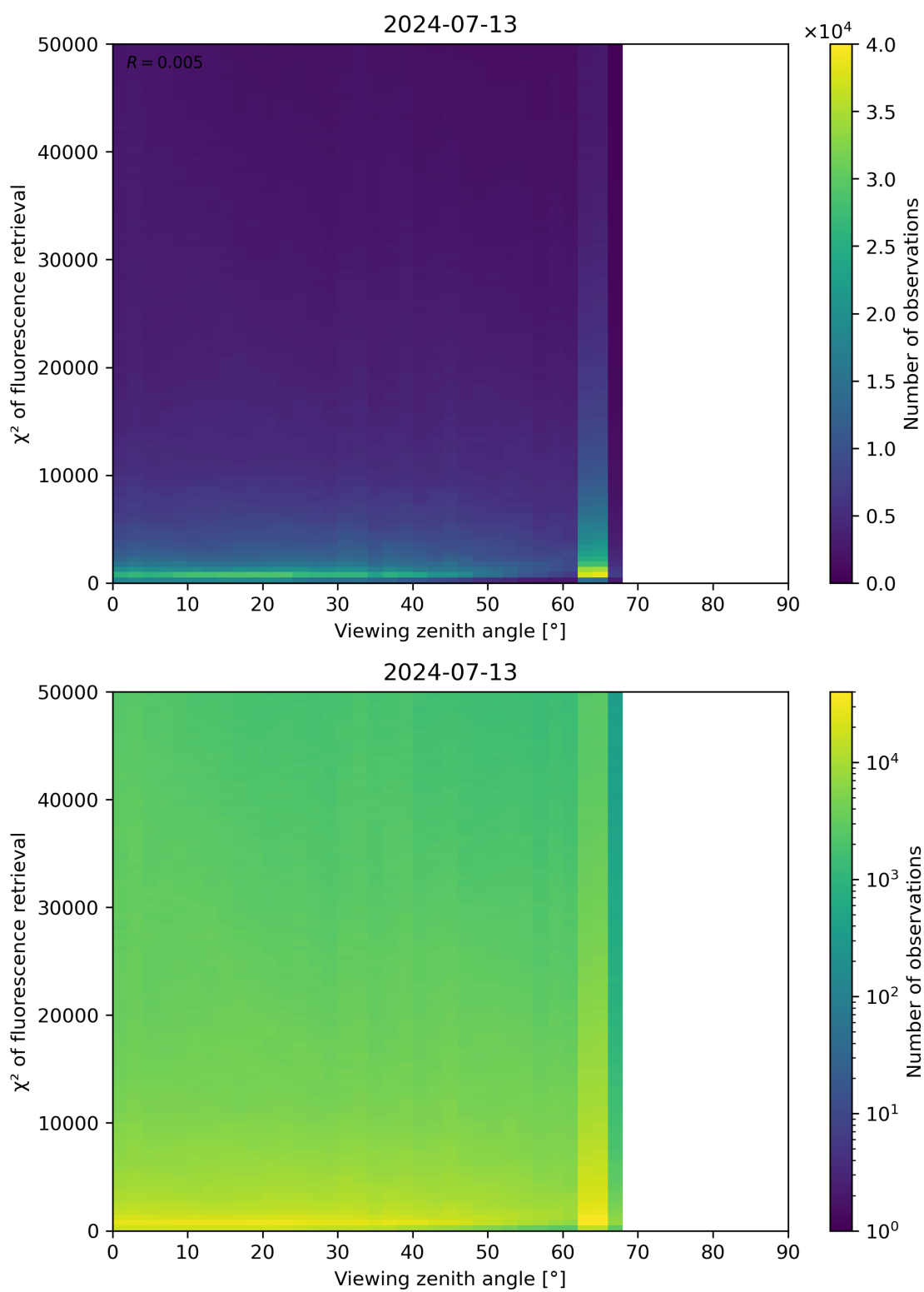
Figure 119: Scatter density plot of “Viewing zenith angle” against “ \chi^2 of fluorescence retrieval” for 2024-07-12 to 2024-07-14.
