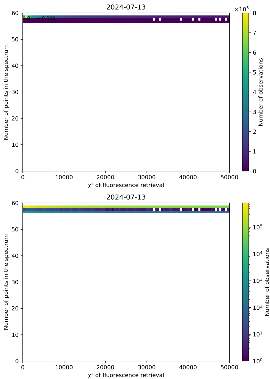
Figure 68: Scatter density plot of " \chi^2 of fluorescence retrieval" against "Number of points in the spectrum" for 2024-07-12 to 2024-07-14.
