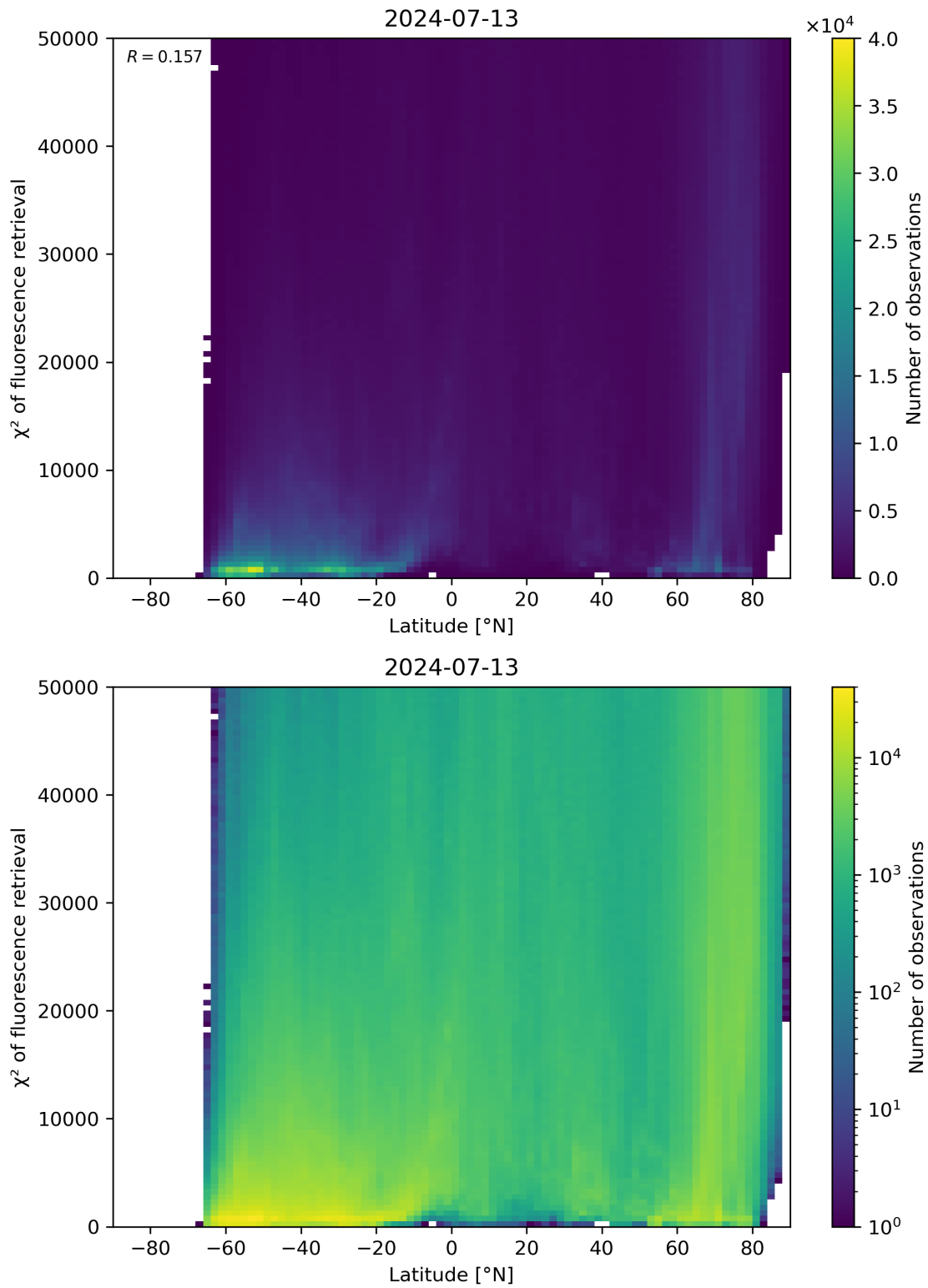
Figure 89: Scatter density plot of “Latitude” against “ \chi^2 of fluorescence retrieval” for 2024-07-12 to 2024-07-14.
