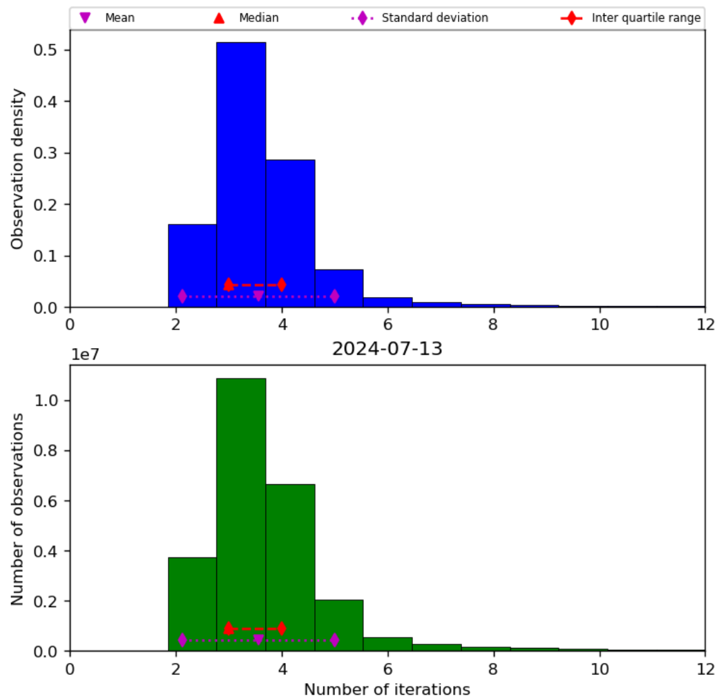
Figure 39: Histogram of “Number of iterations” for 2024-07-12 to 2024-07-14
