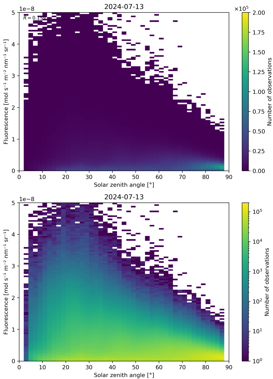
Figure 112: Scatter density plot of “Solar zenith angle” against “Fluorescence” for 2024-07-12 to 2024-07-14.
