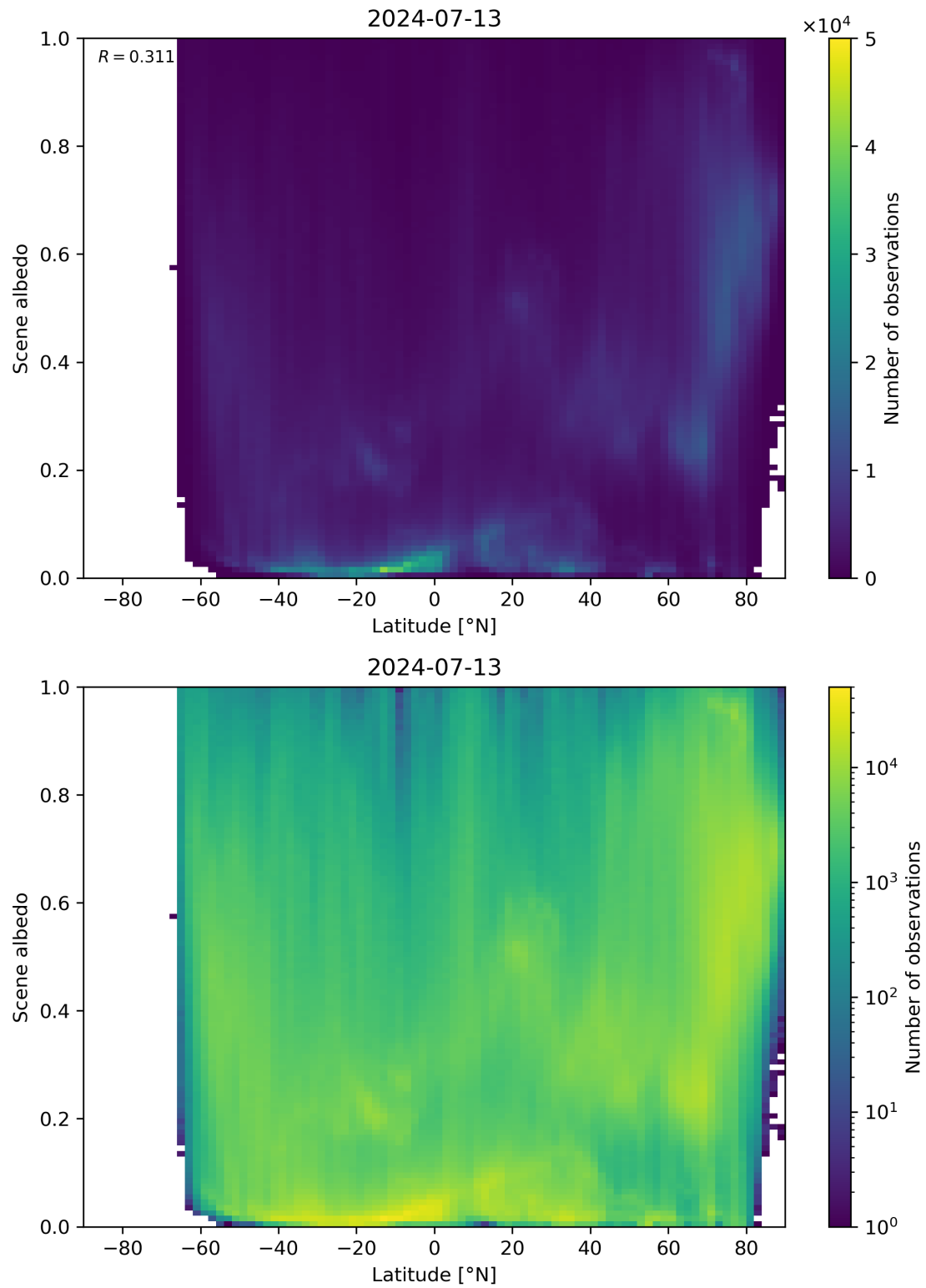
Figure 95: Scatter density plot of “Latitude” against “Scene albedo” for 2024-07-12 to 2024-07-14.
