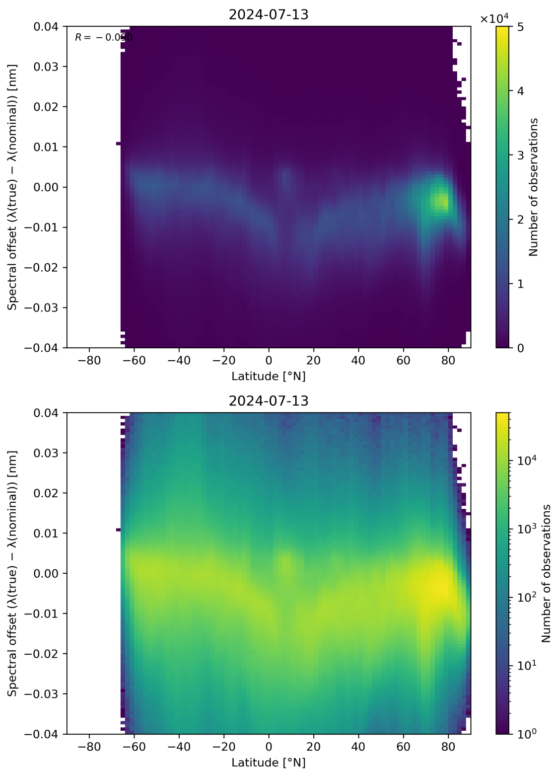
Figure 96: Scatter density plot of “Latitude” against “Spectral offset ( \lambda(\text{true}) - \lambda(\text{nominal}) )” for 2024-07-12 to 2024-07-14.
