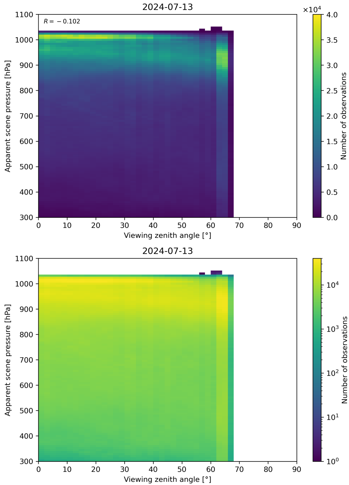
Figure 118: Scatter density plot of “Viewing zenith angle” against “Apparent scene pressure” for 2024-07-12 to 2024-07-14.
