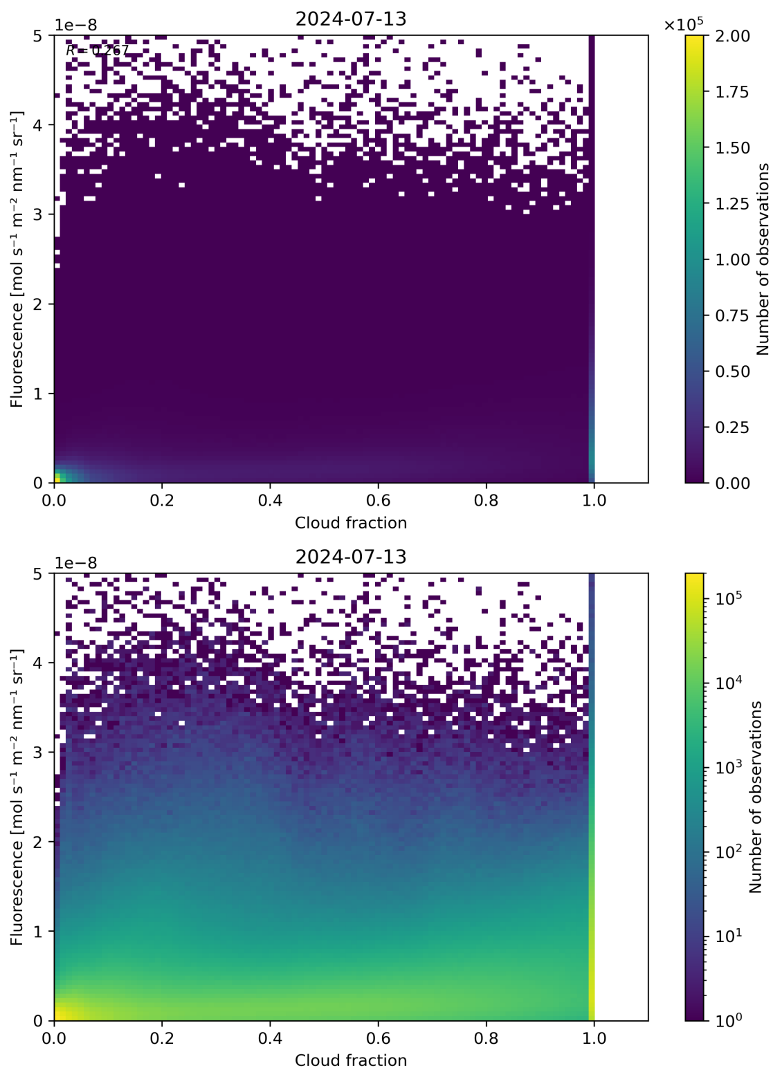
Figure 72: Scatter density plot of “Cloud fraction” against “Fluorescence” for 2024-07-12 to 2024-07-14.
