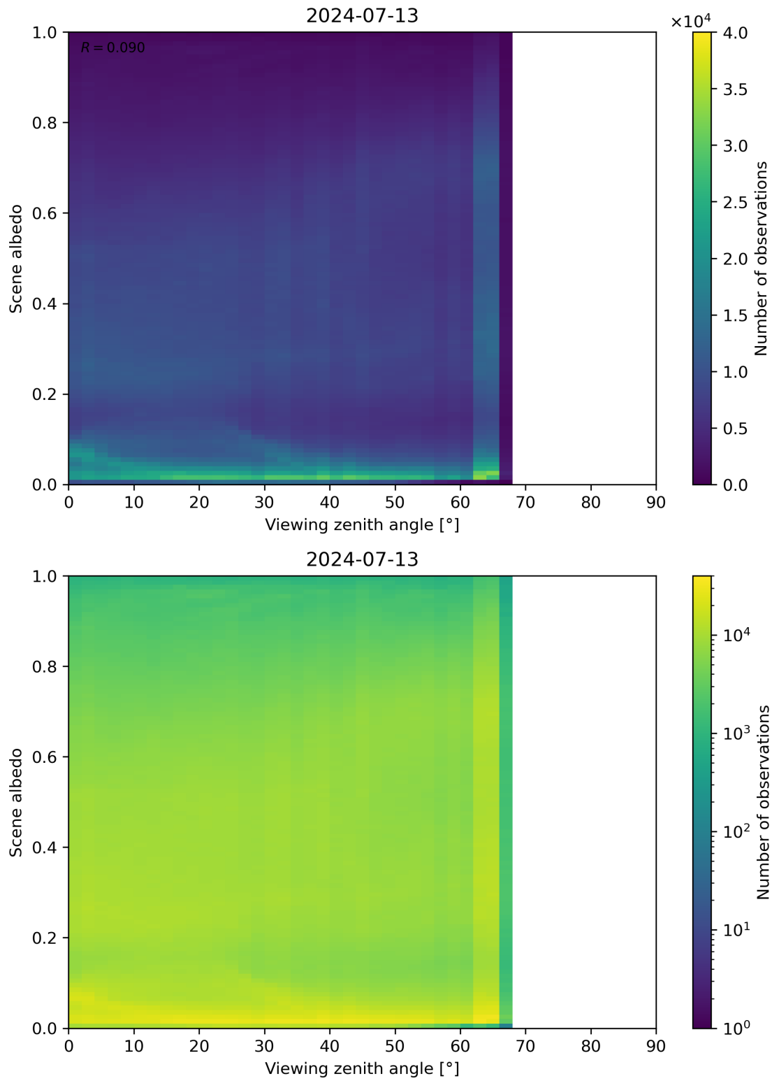
Figure 126: Scatter density plot of “Viewing zenith angle” against “Scene albedo” for 2024-07-12 to 2024-07-14.
