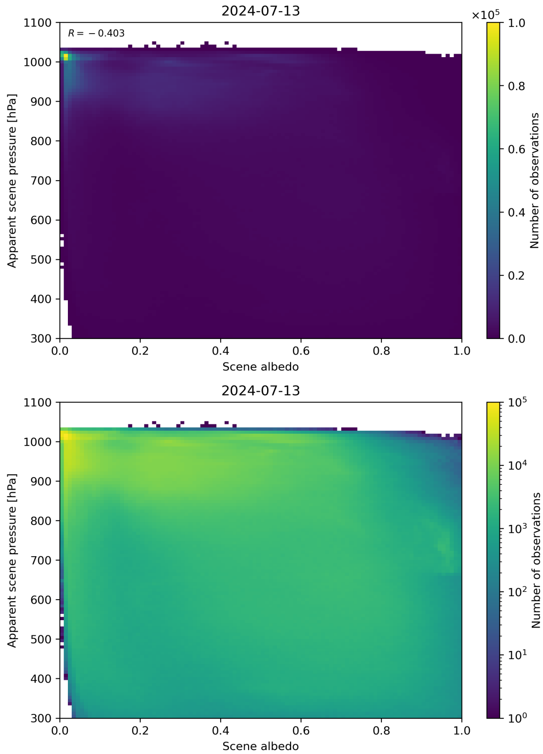
Figure 102: Scatter density plot of “Scene albedo” against “Apparent scene pressure” for 2024-07-12 to 2024-07-14.
