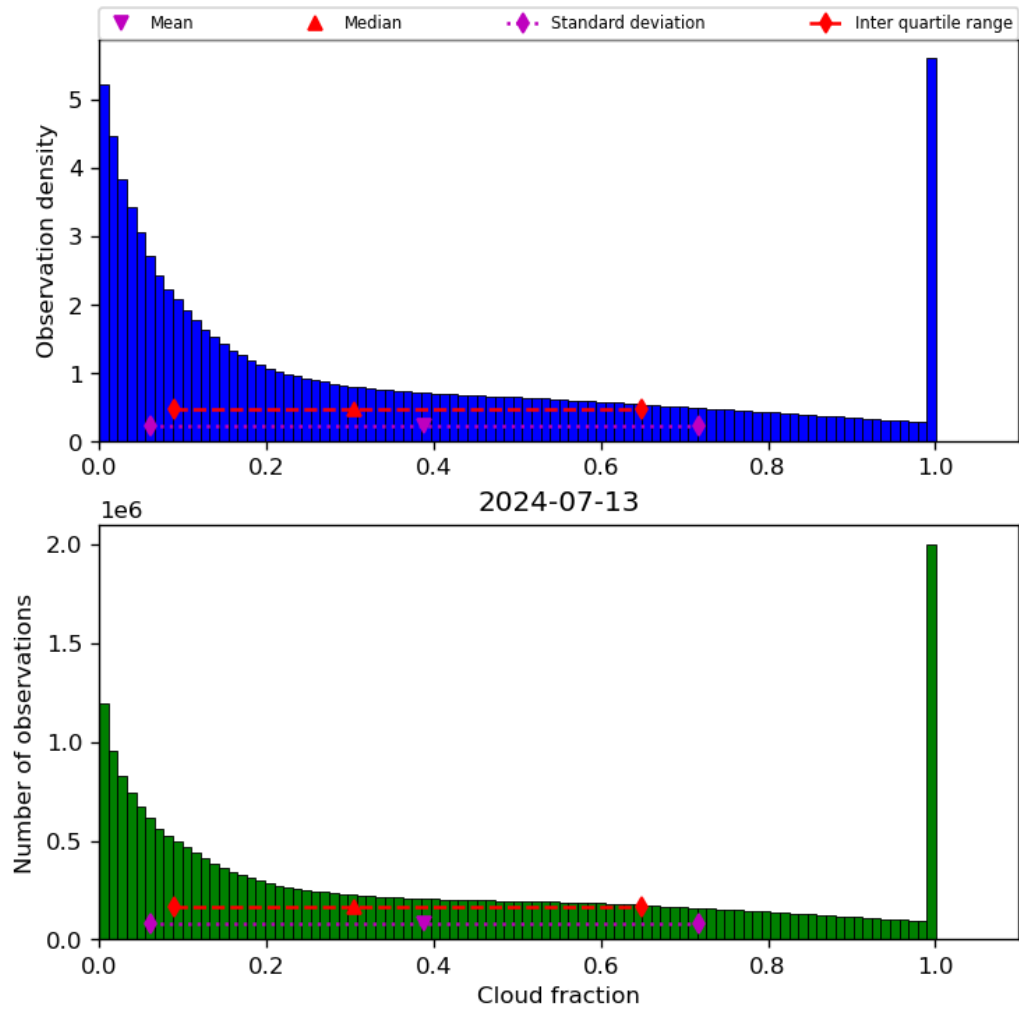
Figure 32: Histogram of “Cloud fraction” for 2024-07-12 to 2024-07-14
