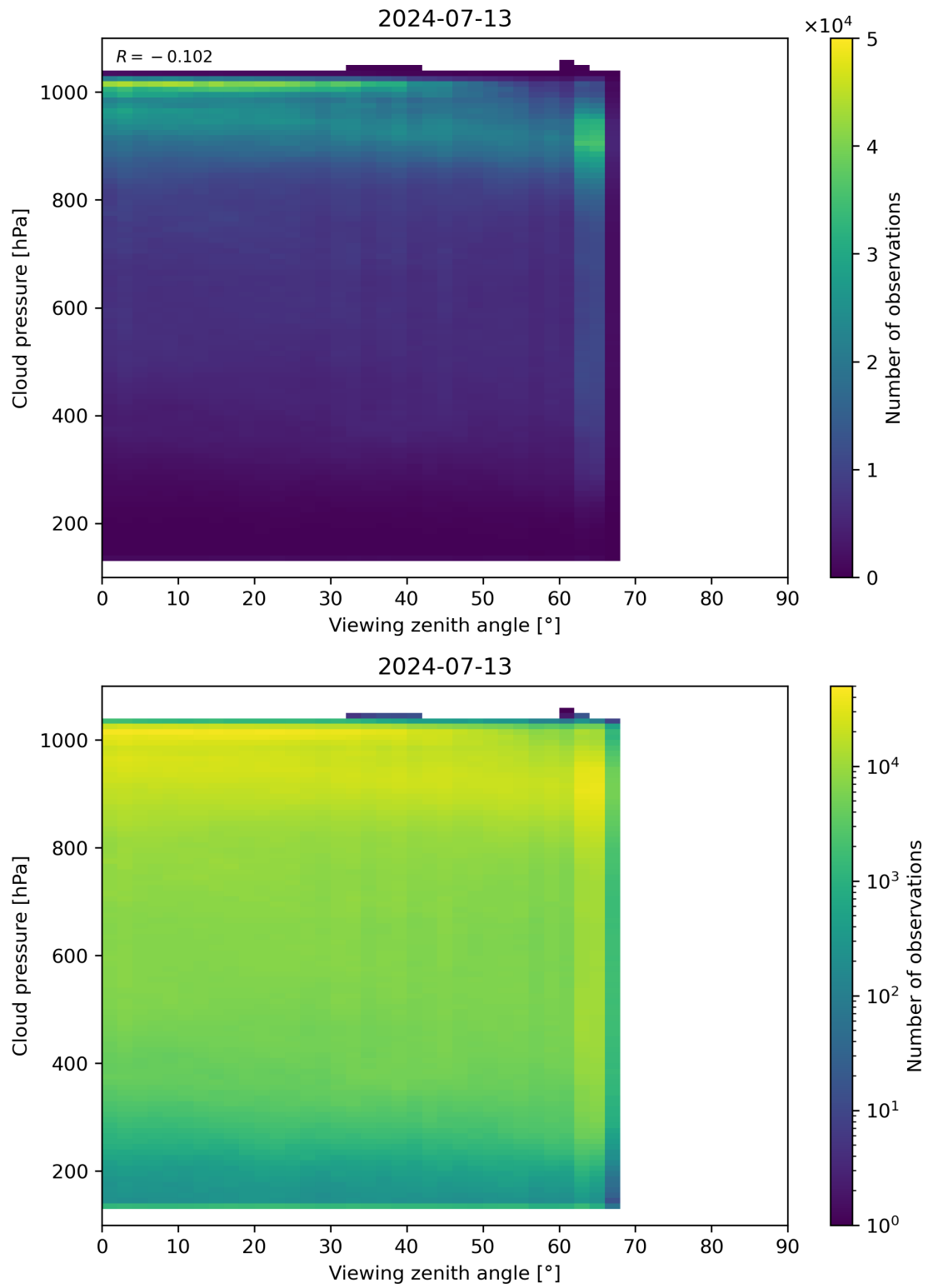
Figure 121: Scatter density plot of “Viewing zenith angle” against “Cloud pressure” for 2024-07-12 to 2024-07-14.
