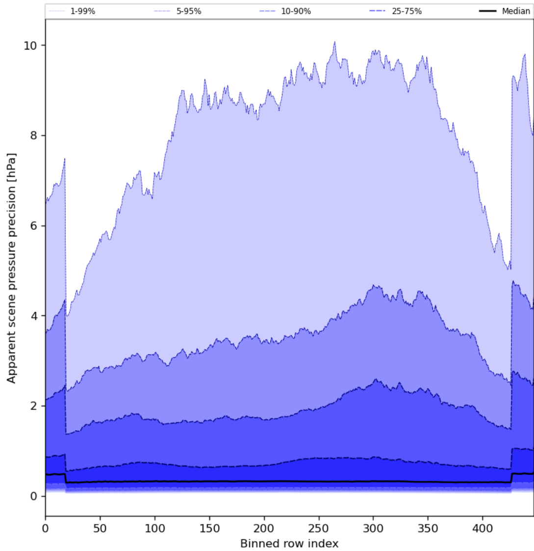
Figure 54: Along track statistics of “Apparent scene pressure precision” for 2024-07-12 to 2024-07-14
