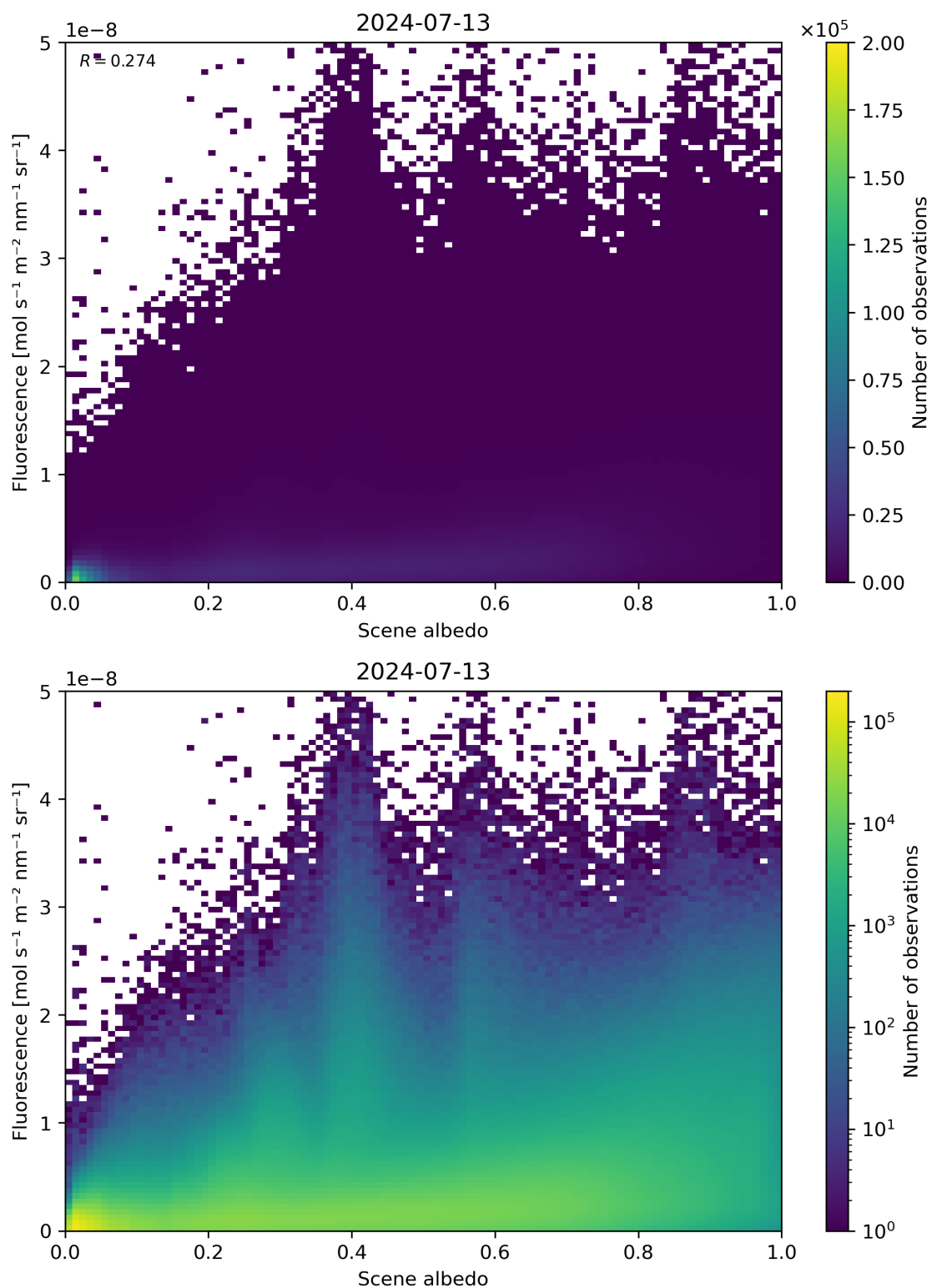
Figure 104: Scatter density plot of “Scene albedo” against “Fluorescence” for 2024-07-12 to 2024-07-14.
