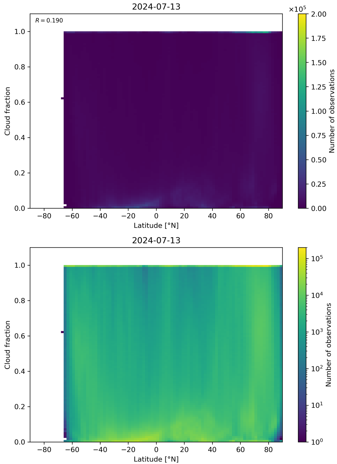
Figure 90: Scatter density plot of “Latitude” against “Cloud fraction” for 2024-07-12 to 2024-07-14.
