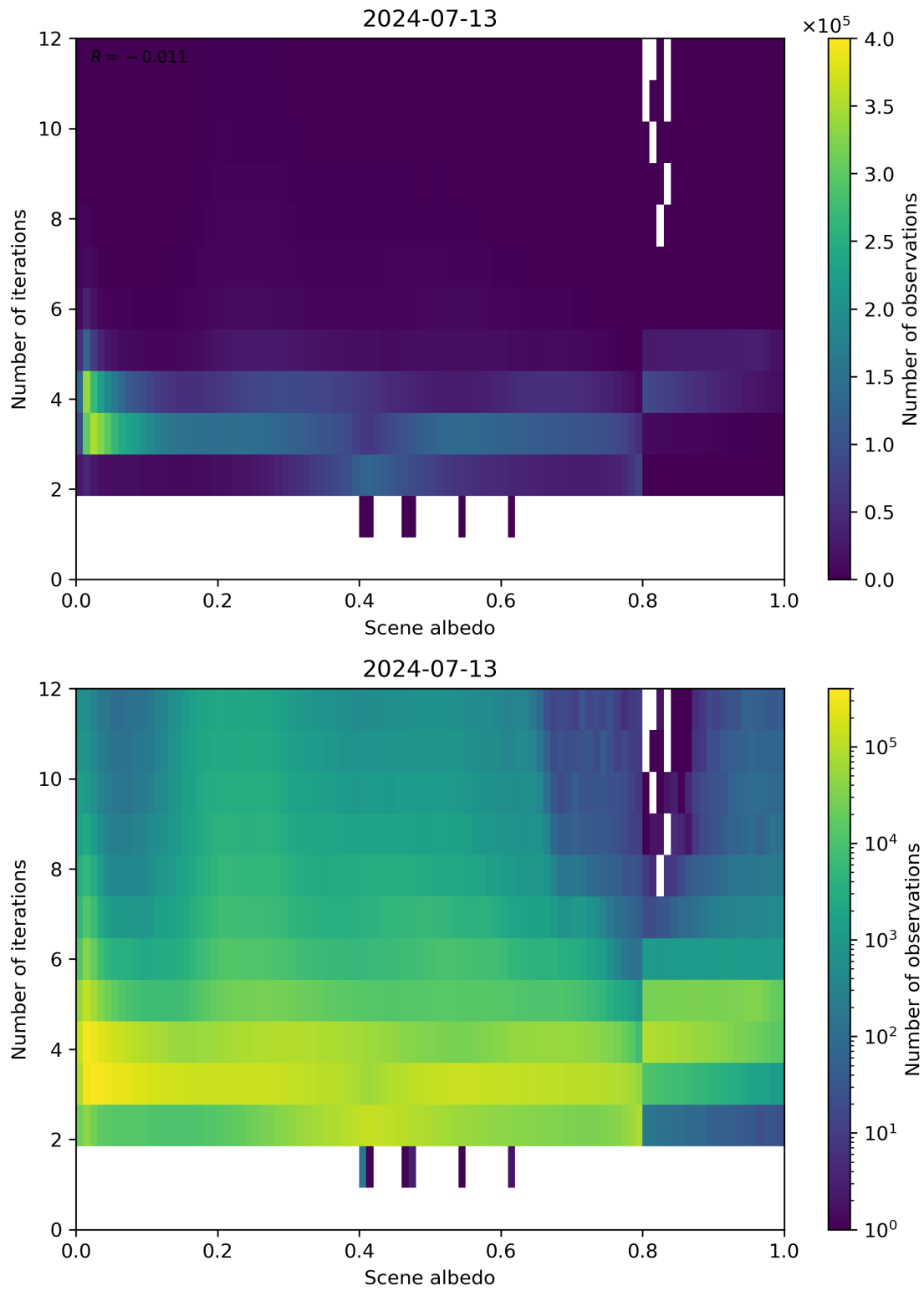
Figure 105: Scatter density plot of “Scene albedo” against “Number of iterations” for 2024-07-12 to 2024-07-14.
