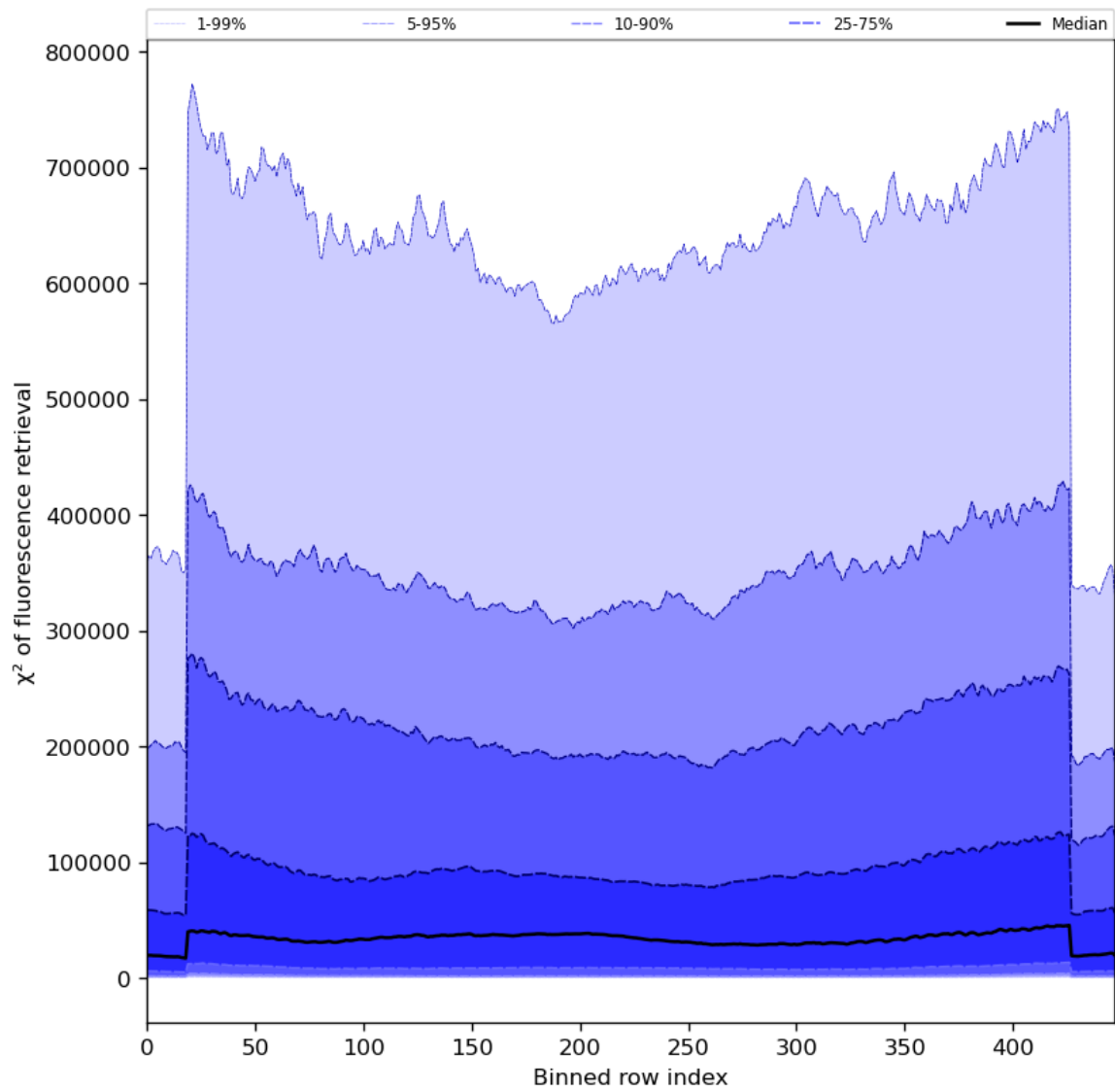
Figure 59: Along track statistics of “ \chi^2 of fluorescence retrieval” for 2024-07-12 to 2024-07-14
