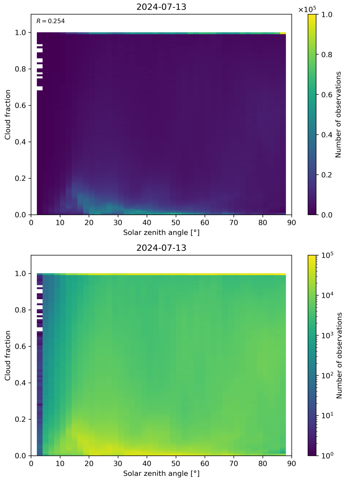
Figure 110: Scatter density plot of “Solar zenith angle” against “Cloud fraction” for 2024-07-12 to 2024-07-14.
