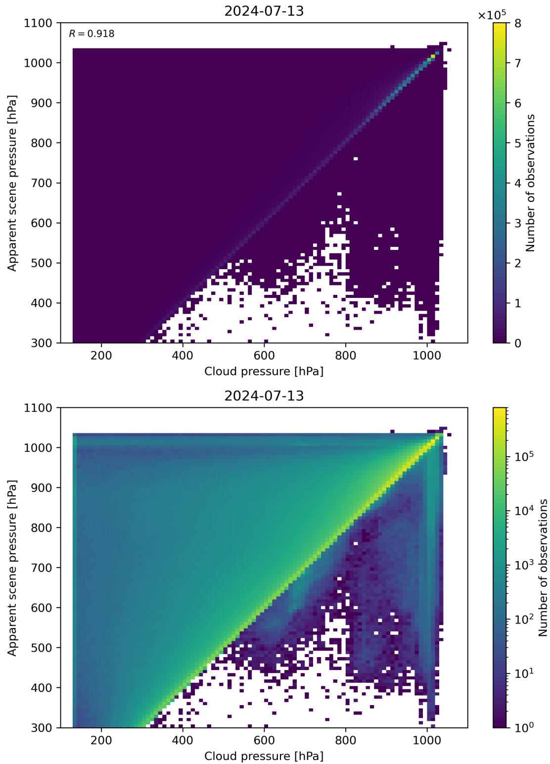
Figure 77: Scatter density plot of “Cloud pressure” against “Apparent scene pressure” for 2024-07-12 to 2024-07-14.
