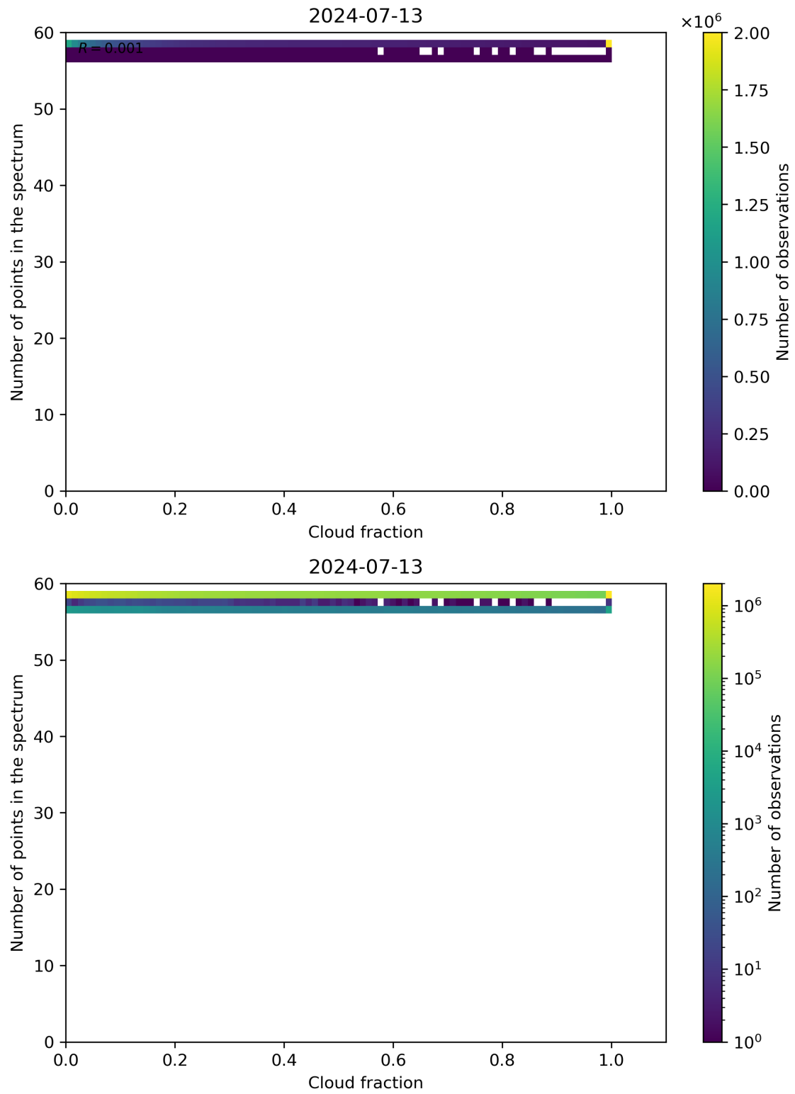
Figure 74: Scatter density plot of “Cloud fraction” against “Number of points in the spectrum” for 2024-07-12 to 2024-07-14.
