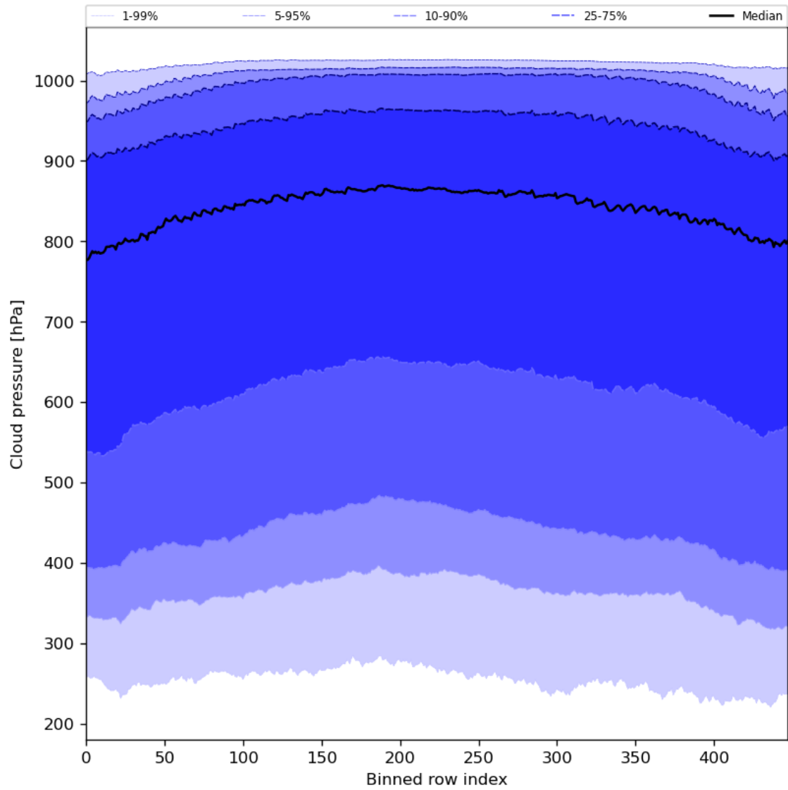
Figure 47: Along track statistics of “Cloud pressure” for 2024-07-12 to 2024-07-14
