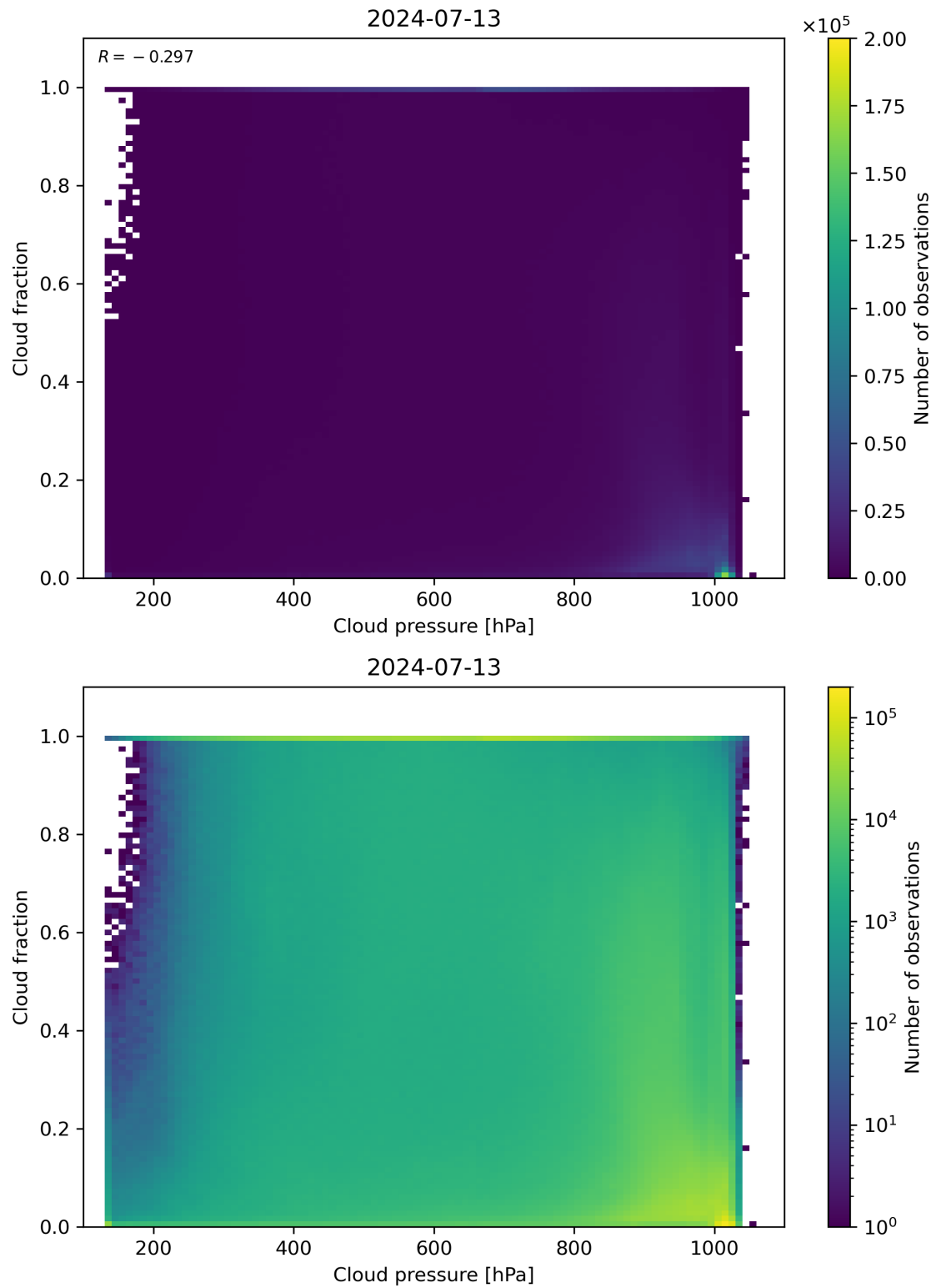
Figure 79: Scatter density plot of “Cloud pressure” against “Cloud fraction” for 2024-07-12 to 2024-07-14.
