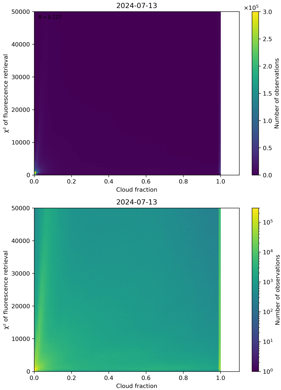
Figure 71: Scatter density plot of “Cloud fraction” against “ \chi^2 of fluorescence retrieval” for 2024-07-12 to 2024-07-14.
