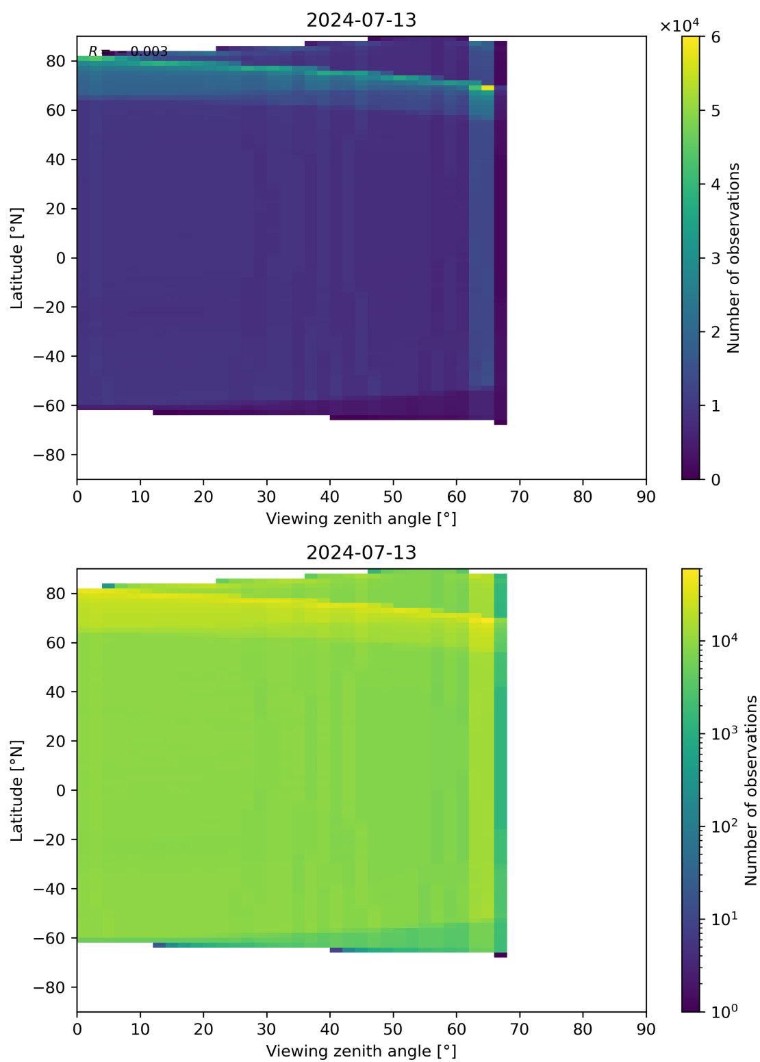
Figure 123: Scatter density plot of “Viewing zenith angle” against “Latitude” for 2024-07-12 to 2024-07-14.
