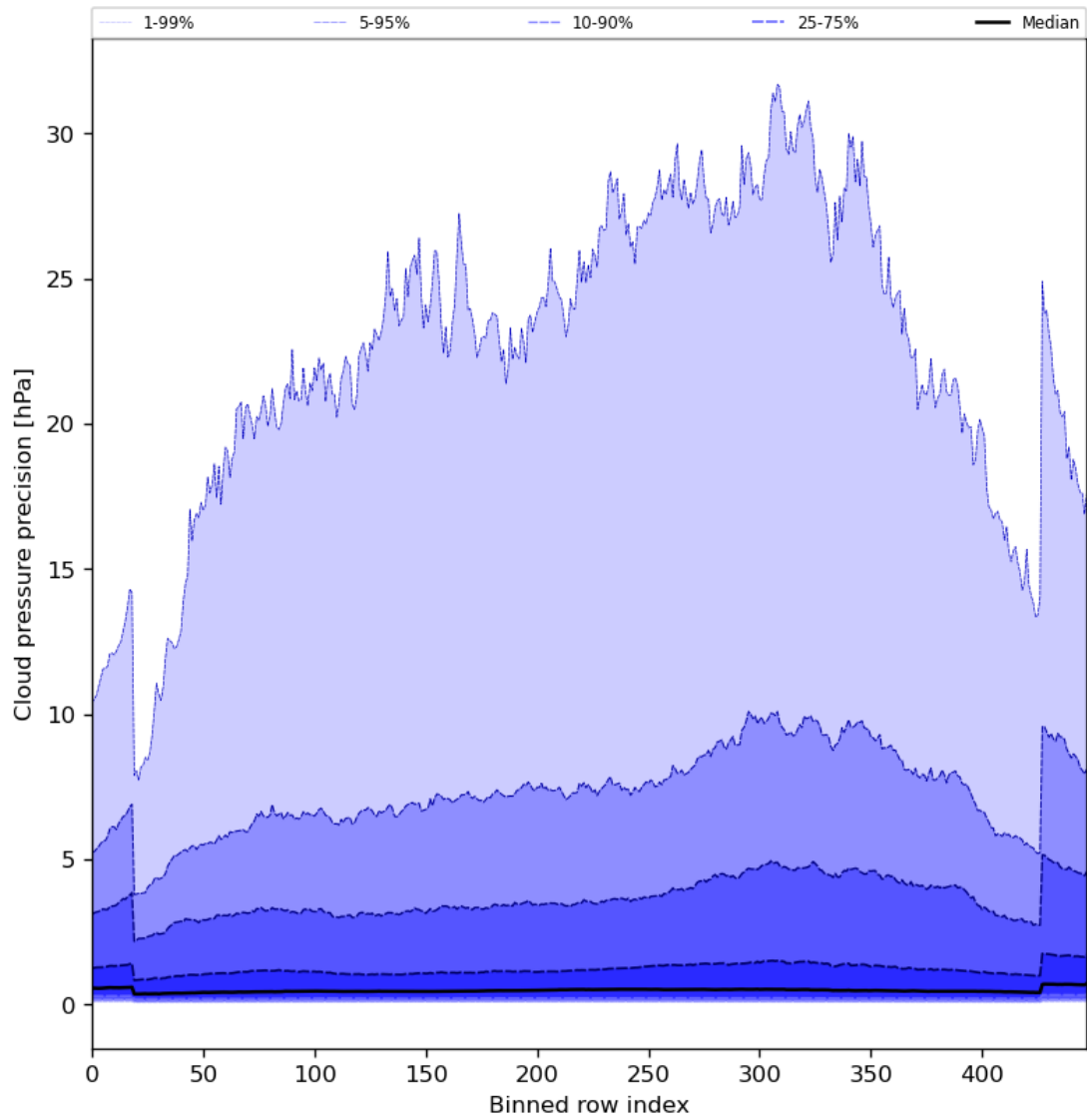
Figure 48: Along track statistics of “Cloud pressure precision” for 2024-07-12 to 2024-07-14
