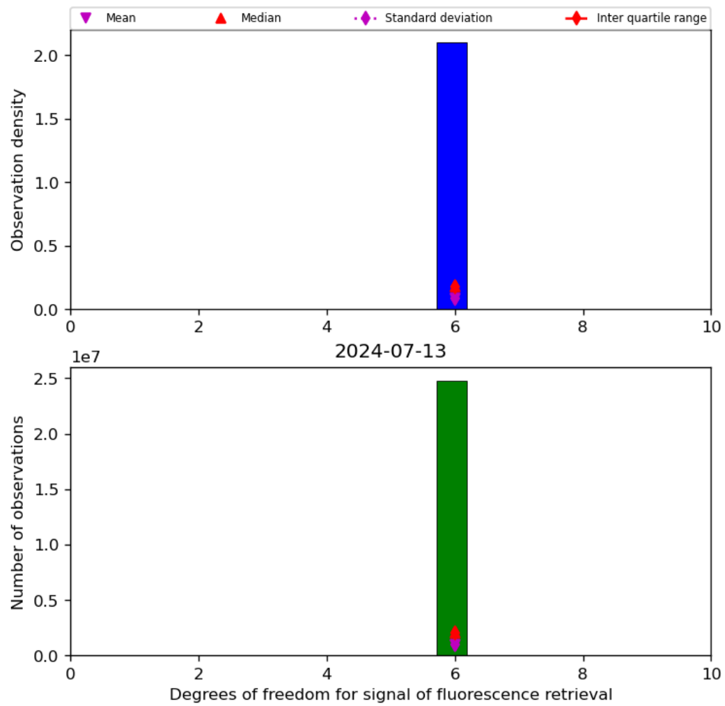
Figure 43: Histogram of “Degrees of freedom for signal of fluorescence retrieval” for 2024-07-12 to 2024-07-14
