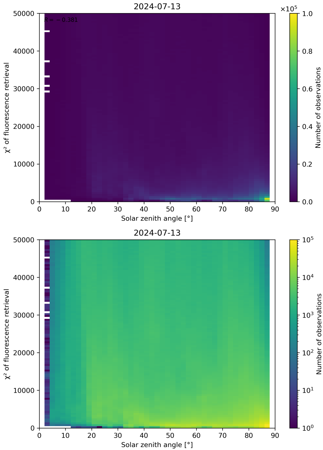
Figure 109: Scatter density plot of “Solar zenith angle” against “ \chi^2 of fluorescence retrieval” for 2024-07-12 to 2024-07-14.
