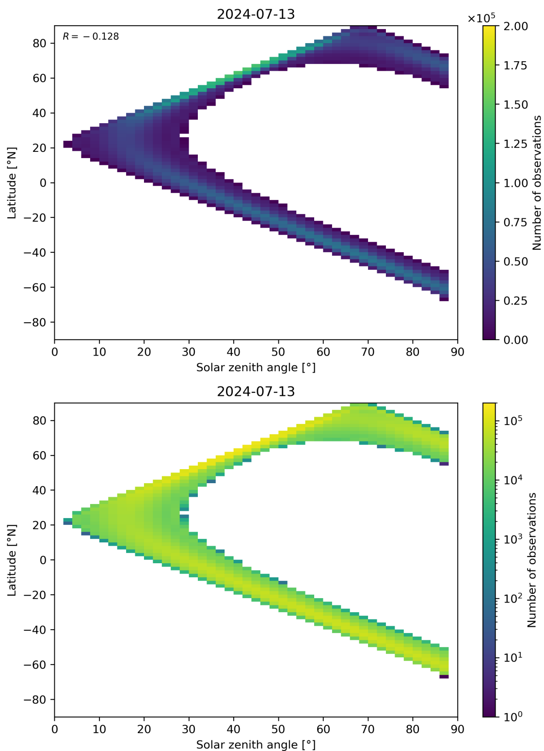
Figure 113: Scatter density plot of “Solar zenith angle” against “Latitude” for 2024-07-12 to 2024-07-14.
