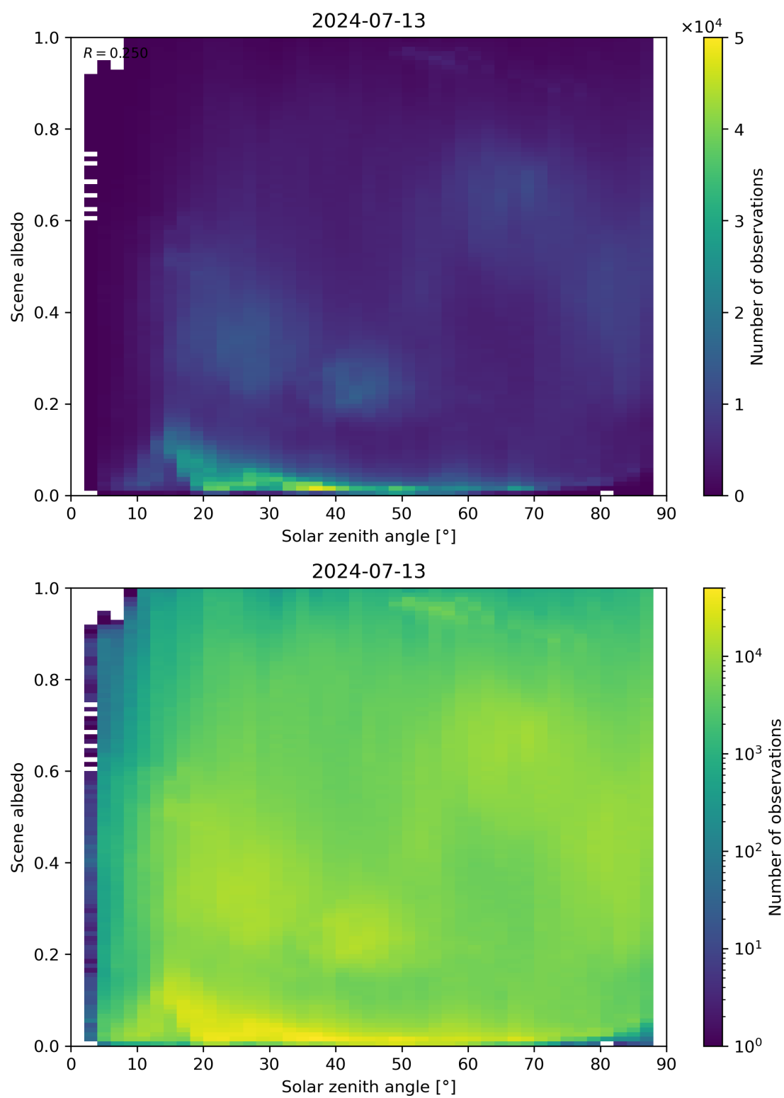
Figure 116: Scatter density plot of “Solar zenith angle” against “Scene albedo” for 2024-07-12 to 2024-07-14.
