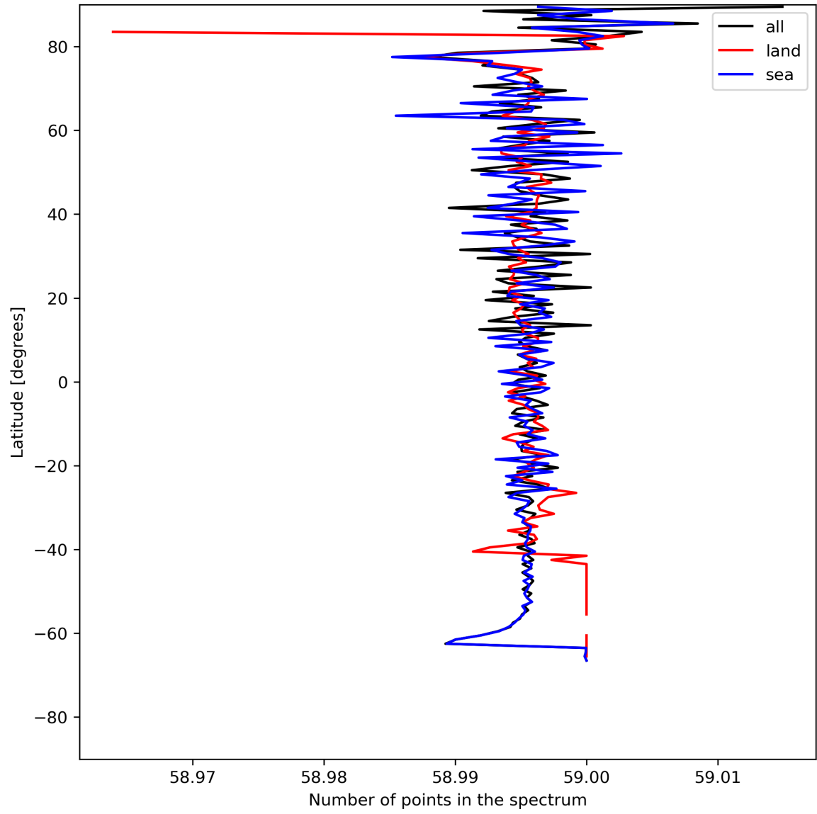
Figure 27: Zonal average of “Number of points in the spectrum” for 2024-07-12 to 2024-07-14.
