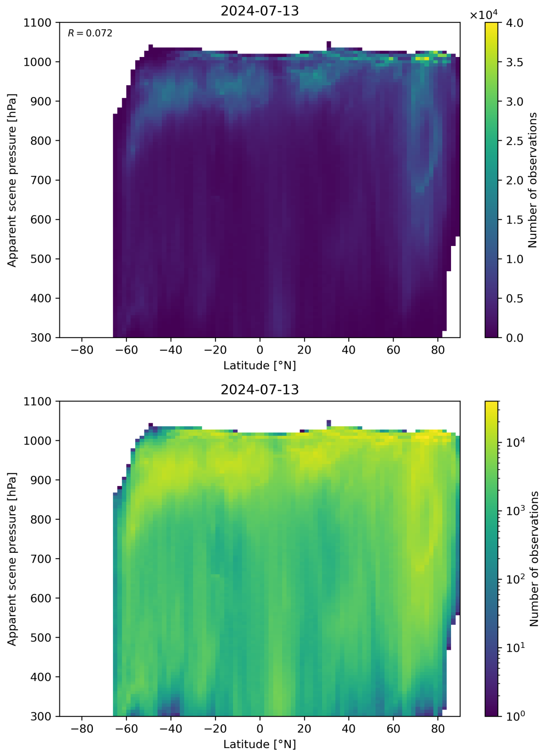
Figure 88: Scatter density plot of “Latitude” against “Apparent scene pressure” for 2024-07-12 to 2024-07-14.
