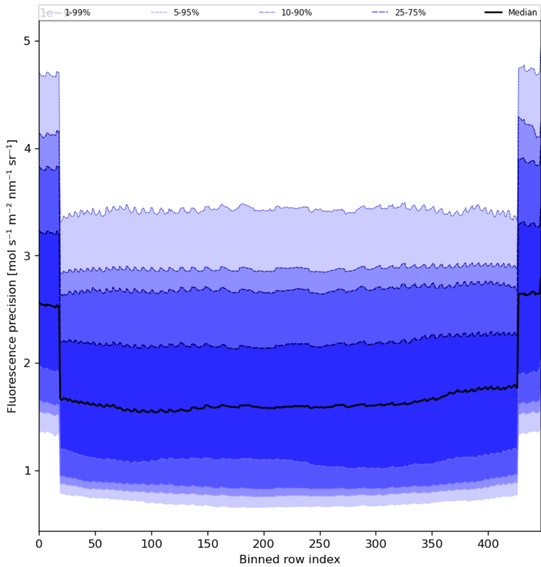
Figure 58: Along track statistics of “Fluorescence precision” for 2024-07-12 to 2024-07-14
