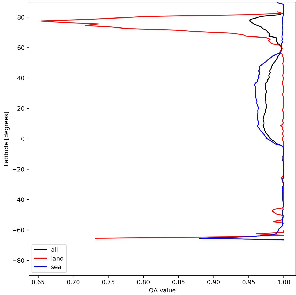
Figure 12: Zonal average of “QA value” for 2024-07-12 to 2024-07-14.
