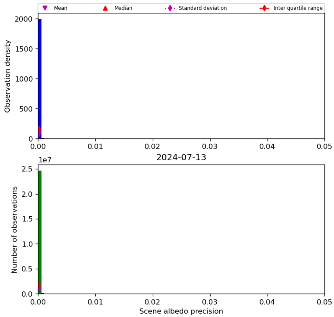
Figure 35: Histogram of “Scene albedo precision” for 2024-07-12 to 2024-07-14
