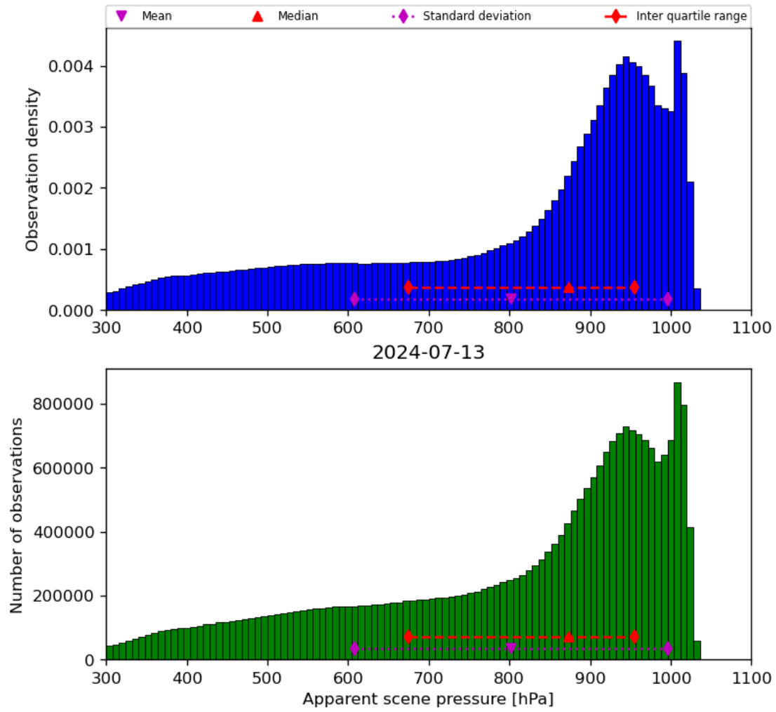
Figure 36: Histogram of “Apparent scene pressure” for 2024-07-12 to 2024-07-14
