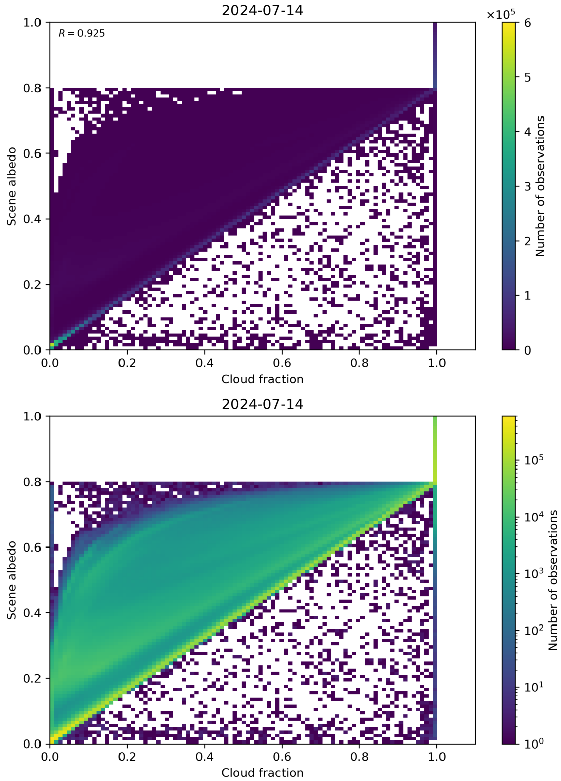
Figure 75: Scatter density plot of “Cloud fraction” against “Scene albedo” for 2024-07-13 to 2024-07-15.
