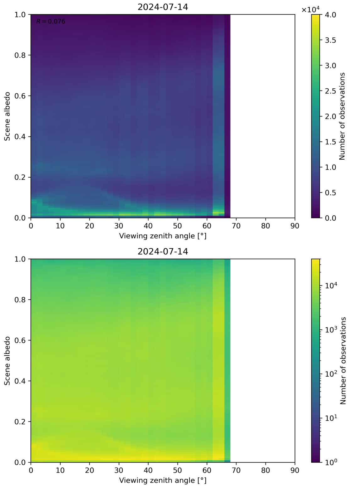
Figure 126: Scatter density plot of “Viewing zenith angle” against “Scene albedo” for 2024-07-13 to 2024-07-15.
