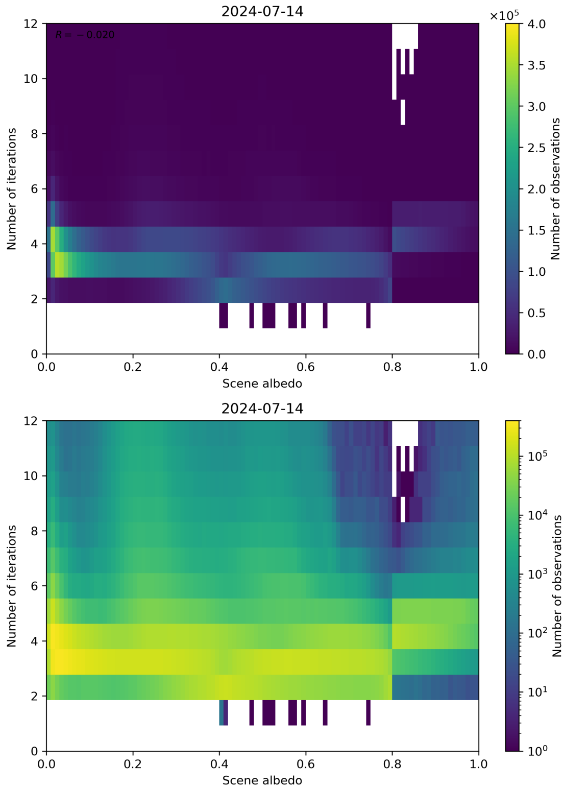
Figure 105: Scatter density plot of “Scene albedo” against “Number of iterations” for 2024-07-13 to 2024-07-15.
