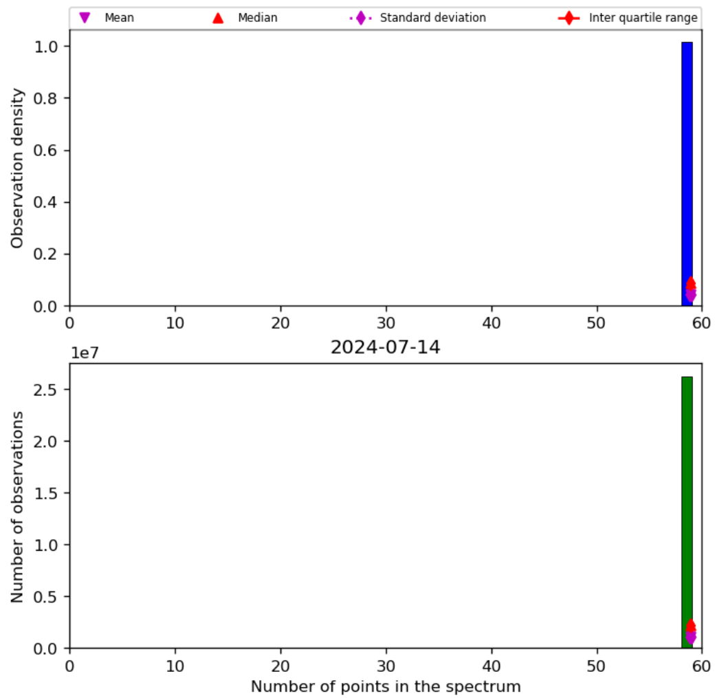
Figure 44: Histogram of “Number of points in the spectrum” for 2024-07-13 to 2024-07-15
