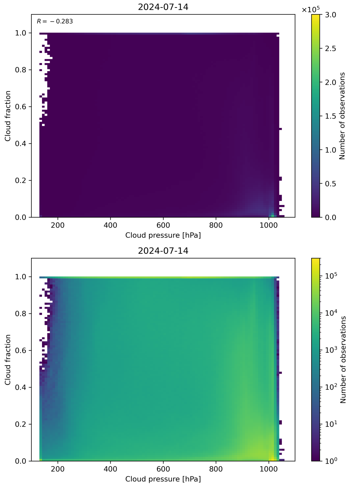
Figure 79: Scatter density plot of “Cloud pressure” against “Cloud fraction” for 2024-07-13 to 2024-07-15.
