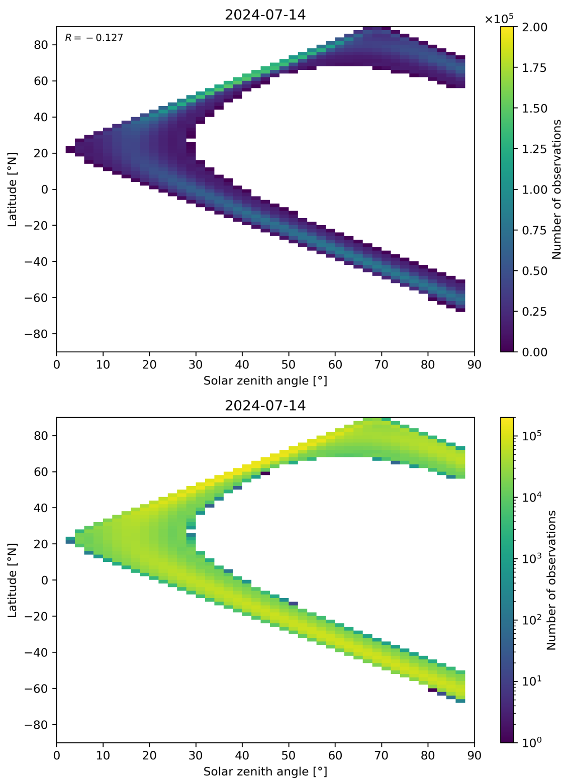
Figure 113: Scatter density plot of “Solar zenith angle” against “Latitude” for 2024-07-13 to 2024-07-15.
