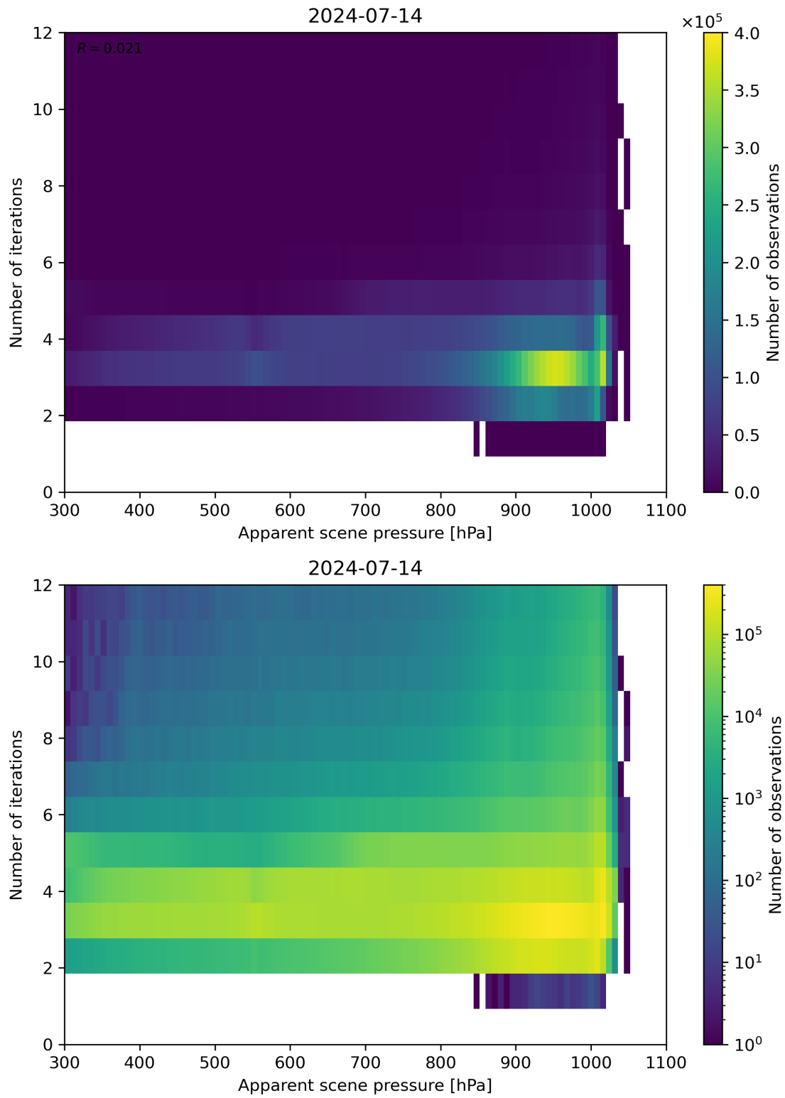
Figure 65: Scatter density plot of “Apparent scene pressure” against “Number of iterations” for 2024-07-13 to 2024-07-15.
