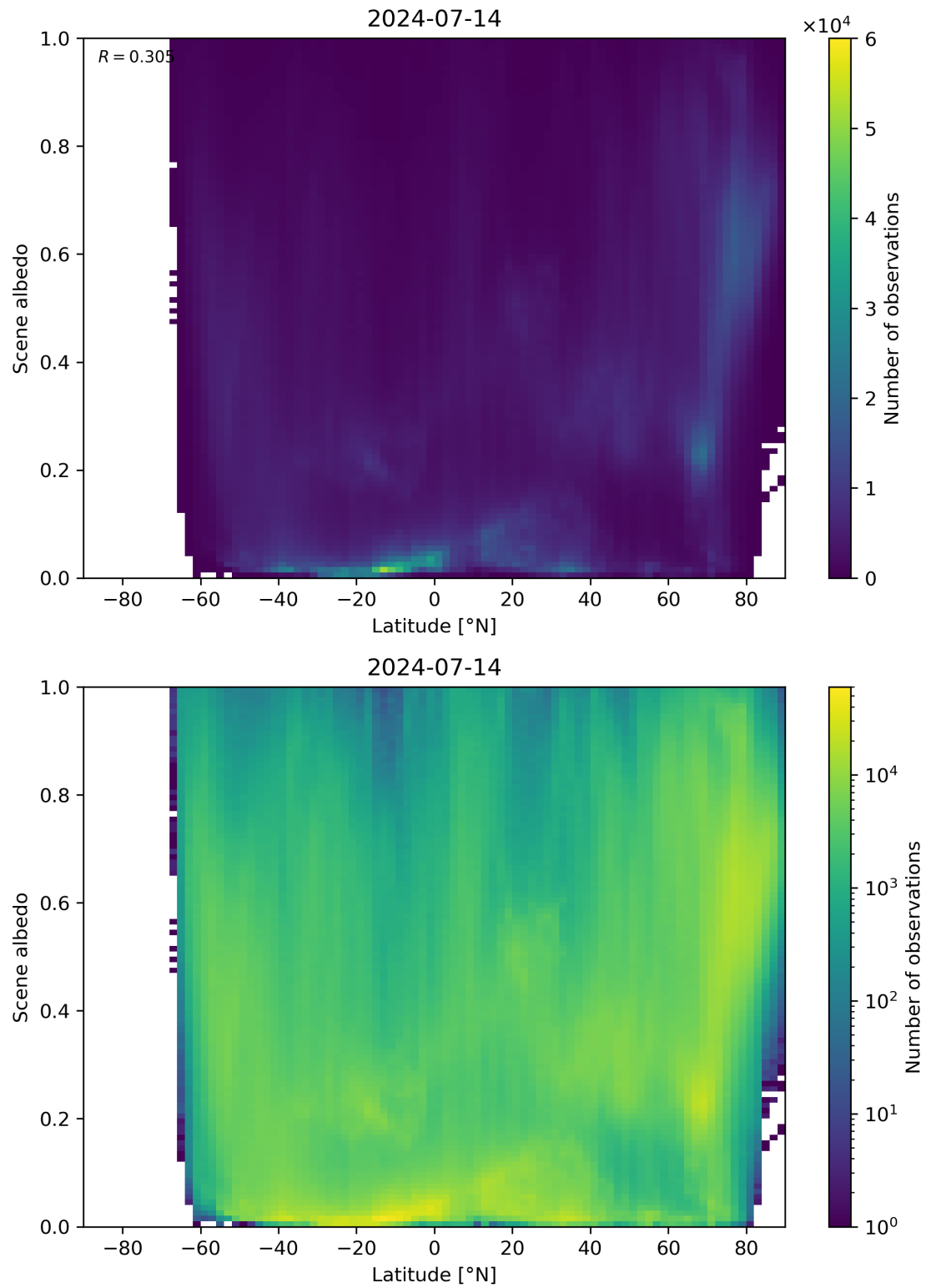
Figure 95: Scatter density plot of “Latitude” against “Scene albedo” for 2024-07-13 to 2024-07-15.
