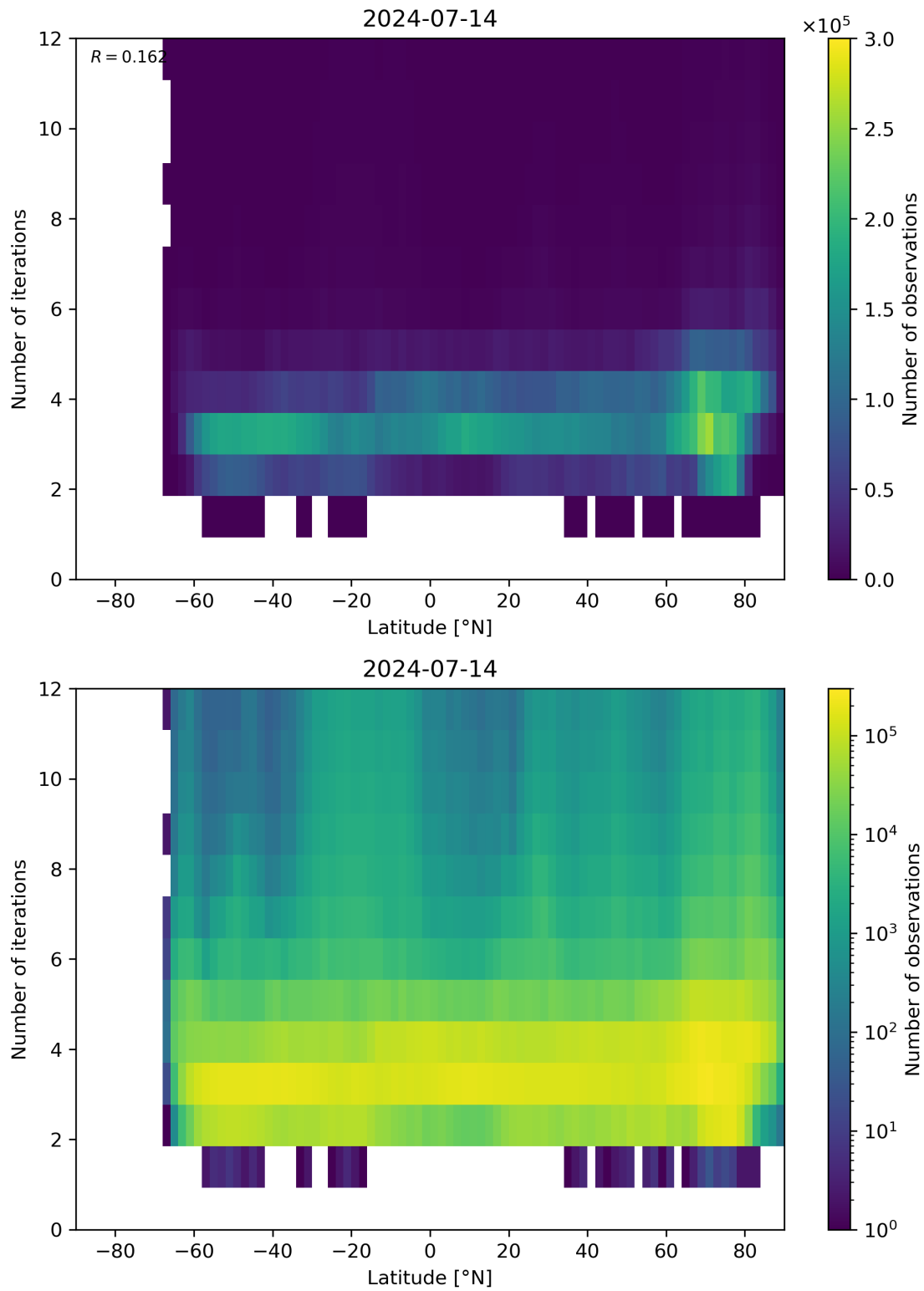
Figure 93: Scatter density plot of “Latitude” against “Number of iterations” for 2024-07-13 to 2024-07-15.
