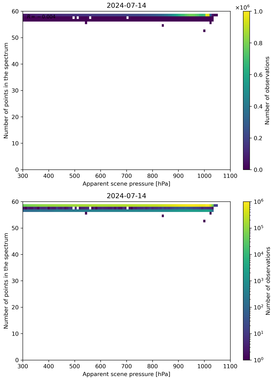
Figure 66: Scatter density plot of “Apparent scene pressure” against “Number of points in the spectrum” for 2024-07-13 to 2024-07-15.
