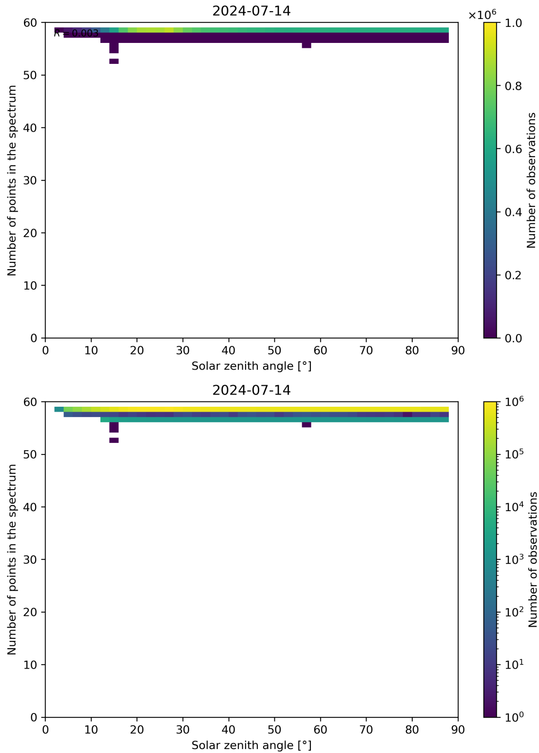
Figure 115: Scatter density plot of “Solar zenith angle” against “Number of points in the spectrum” for 2024-07-13 to 2024-07-15.
