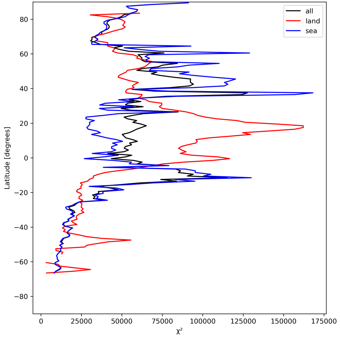
Figure 21: Zonal average of “ \chi^2 ” for 2024-07-13 to 2024-07-15.
