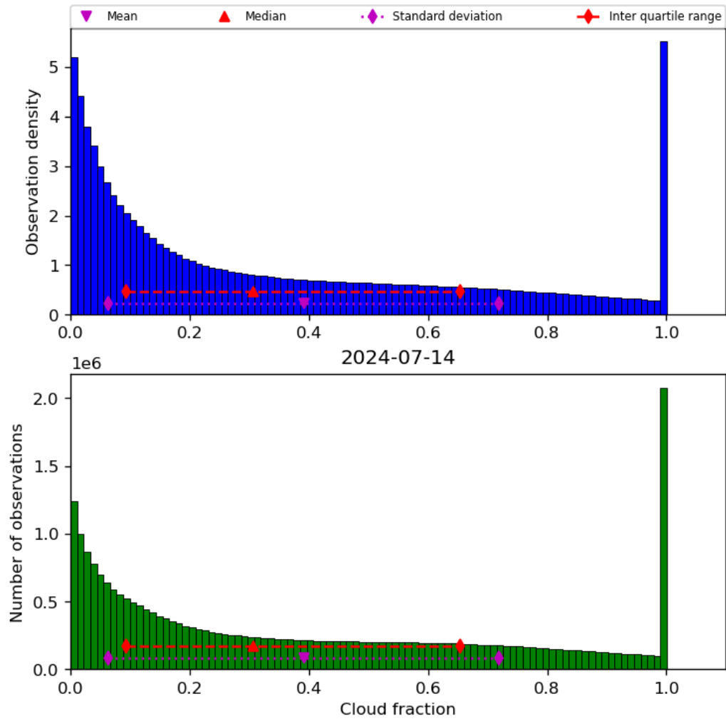
Figure 32: Histogram of “Cloud fraction” for 2024-07-13 to 2024-07-15
