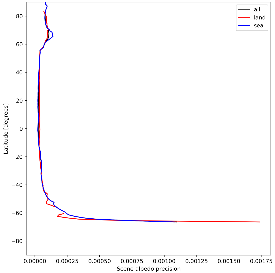
Figure 18: Zonal average of “Scene albedo precision” for 2024-07-13 to 2024-07-15.
