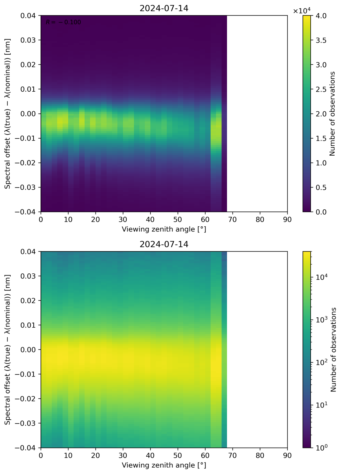
Figure 128: Scatter density plot of “Viewing zenith angle” against “Spectral offset ( \lambda(\text{true}) - \lambda(\text{nominal}) )” for 2024-07-13 to 2024-07-15.
