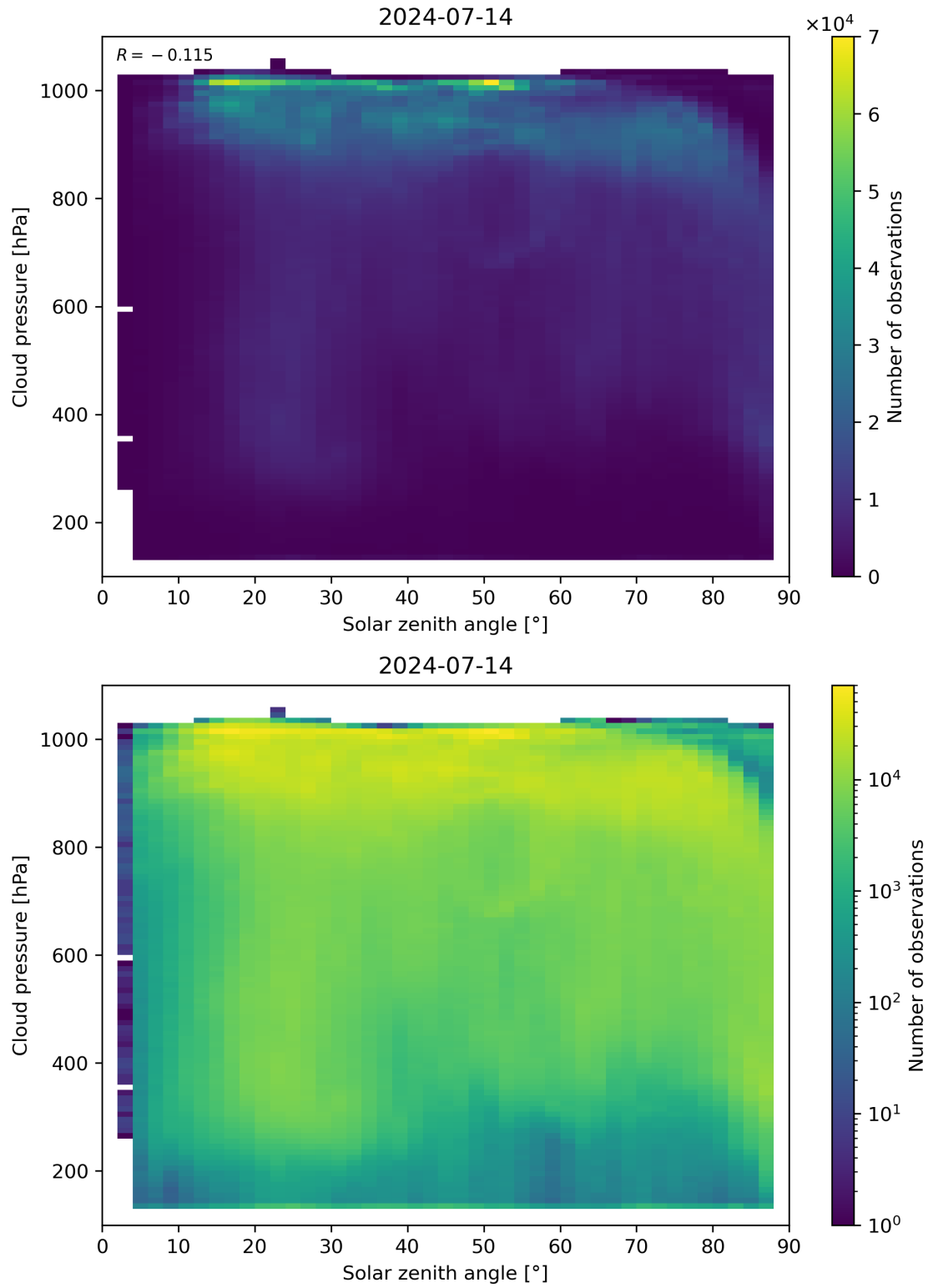
Figure 111: Scatter density plot of “Solar zenith angle” against “Cloud pressure” for 2024-07-13 to 2024-07-15.
