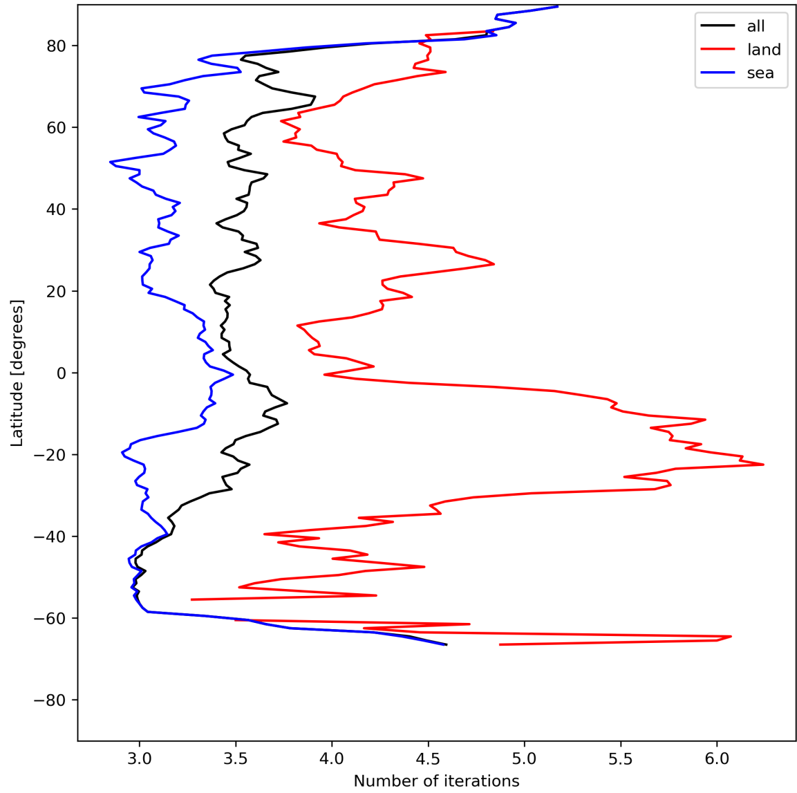
Figure 22: Zonal average of “Number of iterations” for 2024-07-13 to 2024-07-15.
