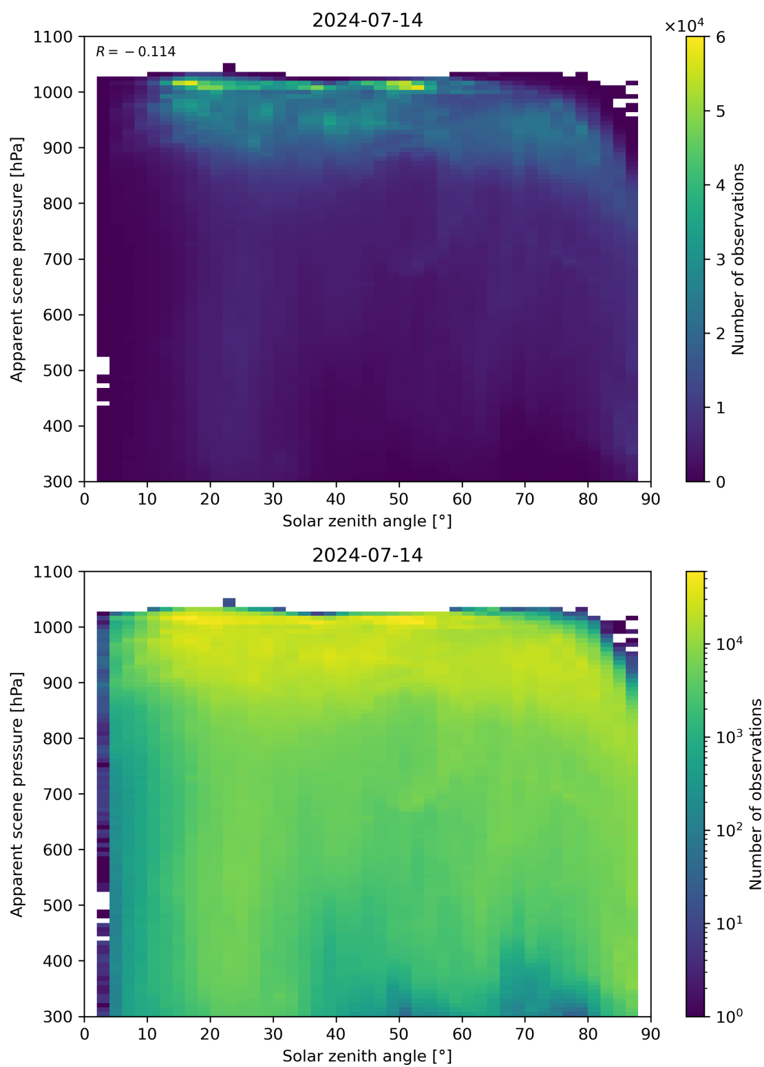
Figure 108: Scatter density plot of “Solar zenith angle” against “Apparent scene pressure” for 2024-07-13 to 2024-07-15.
