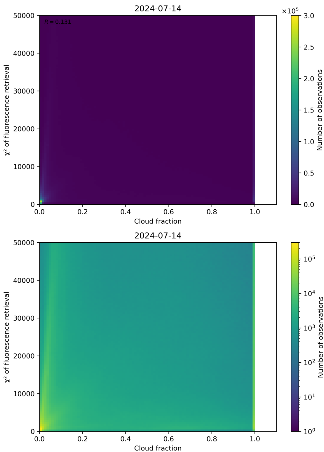
Figure 71: Scatter density plot of “Cloud fraction” against “ \chi^2 of fluorescence retrieval” for 2024-07-13 to 2024-07-15.
