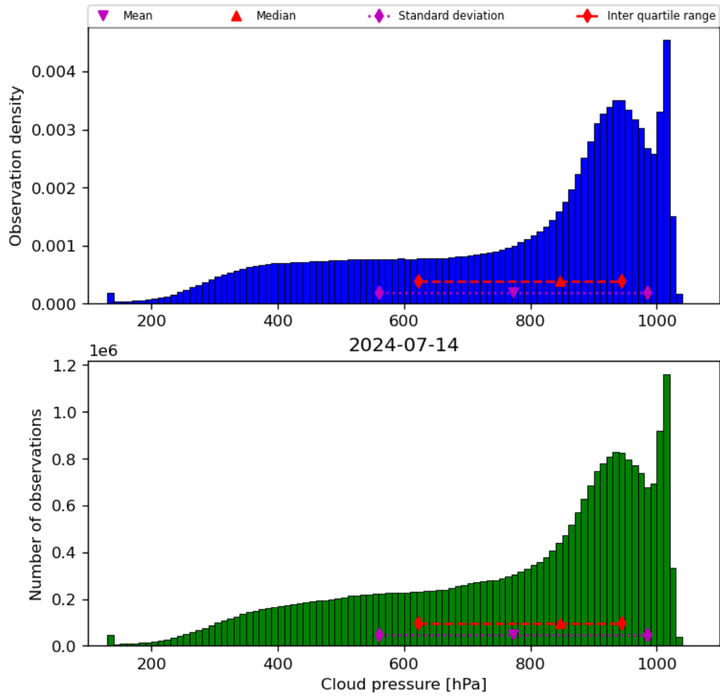
Figure 30: Histogram of “Cloud pressure” for 2024-07-13 to 2024-07-15
