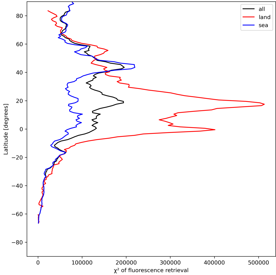
Figure 25: Zonal average of “ \chi^2 of fluorescence retrieval” for 2024-07-13 to 2024-07-15.
