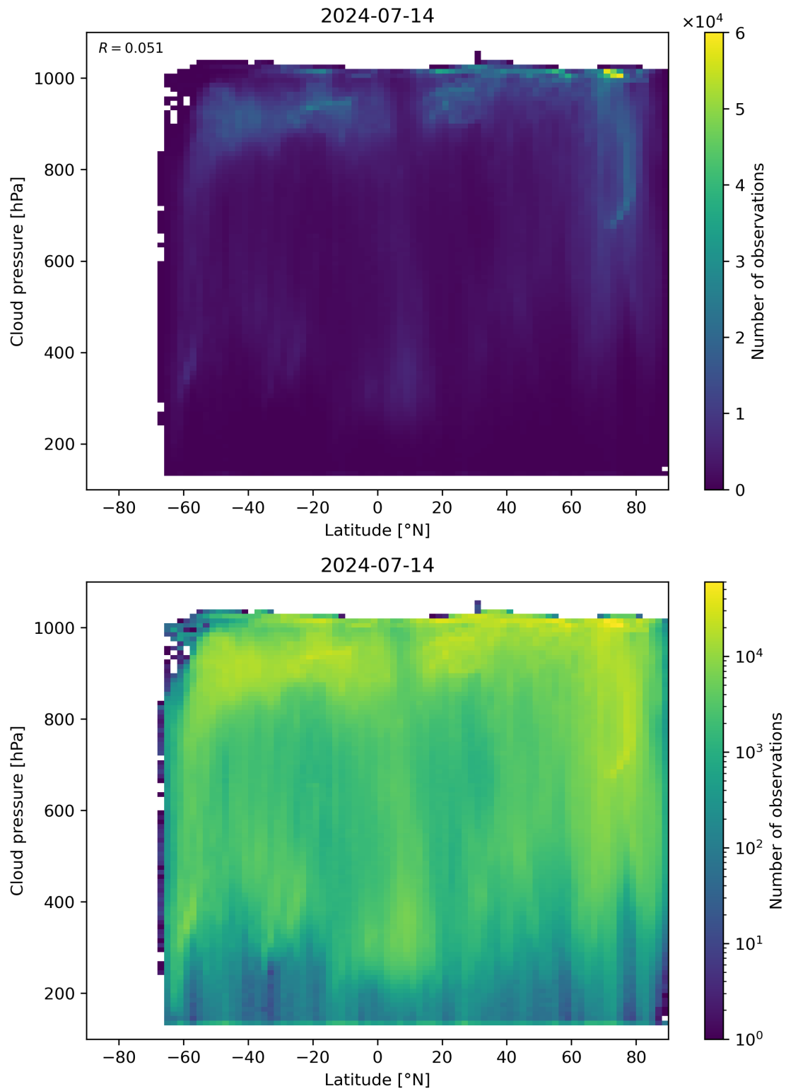
Figure 91: Scatter density plot of “Latitude” against “Cloud pressure” for 2024-07-13 to 2024-07-15.
