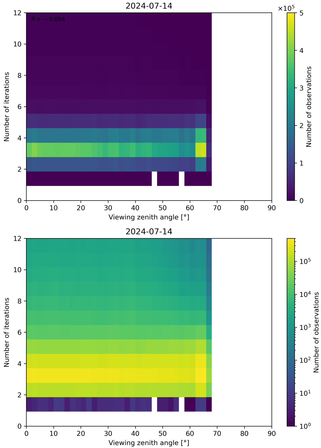
Figure 124: Scatter density plot of “Viewing zenith angle” against “Number of iterations” for 2024-07-13 to 2024-07-15.
