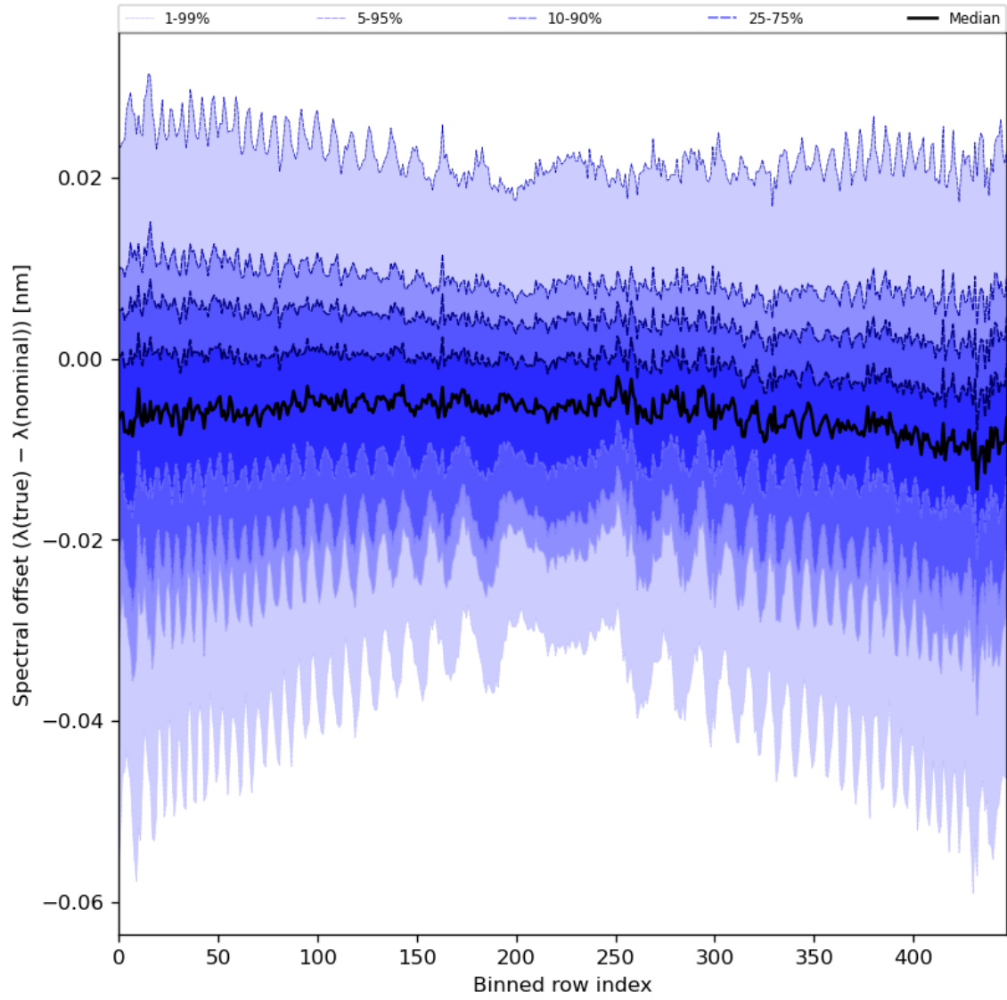
Figure 62: Along track statistics of “Spectral offset ( \lambda(\text{true}) - \lambda(\text{nominal}) )” for 2024-07-13 to 2024-07-15
