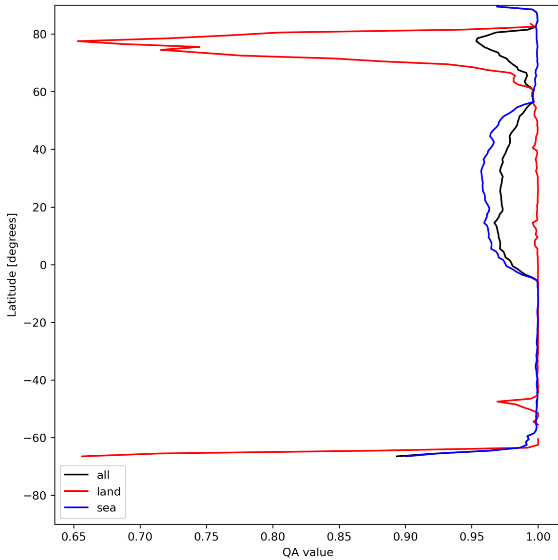
Figure 12: Zonal average of “QA value” for 2024-07-13 to 2024-07-15.
