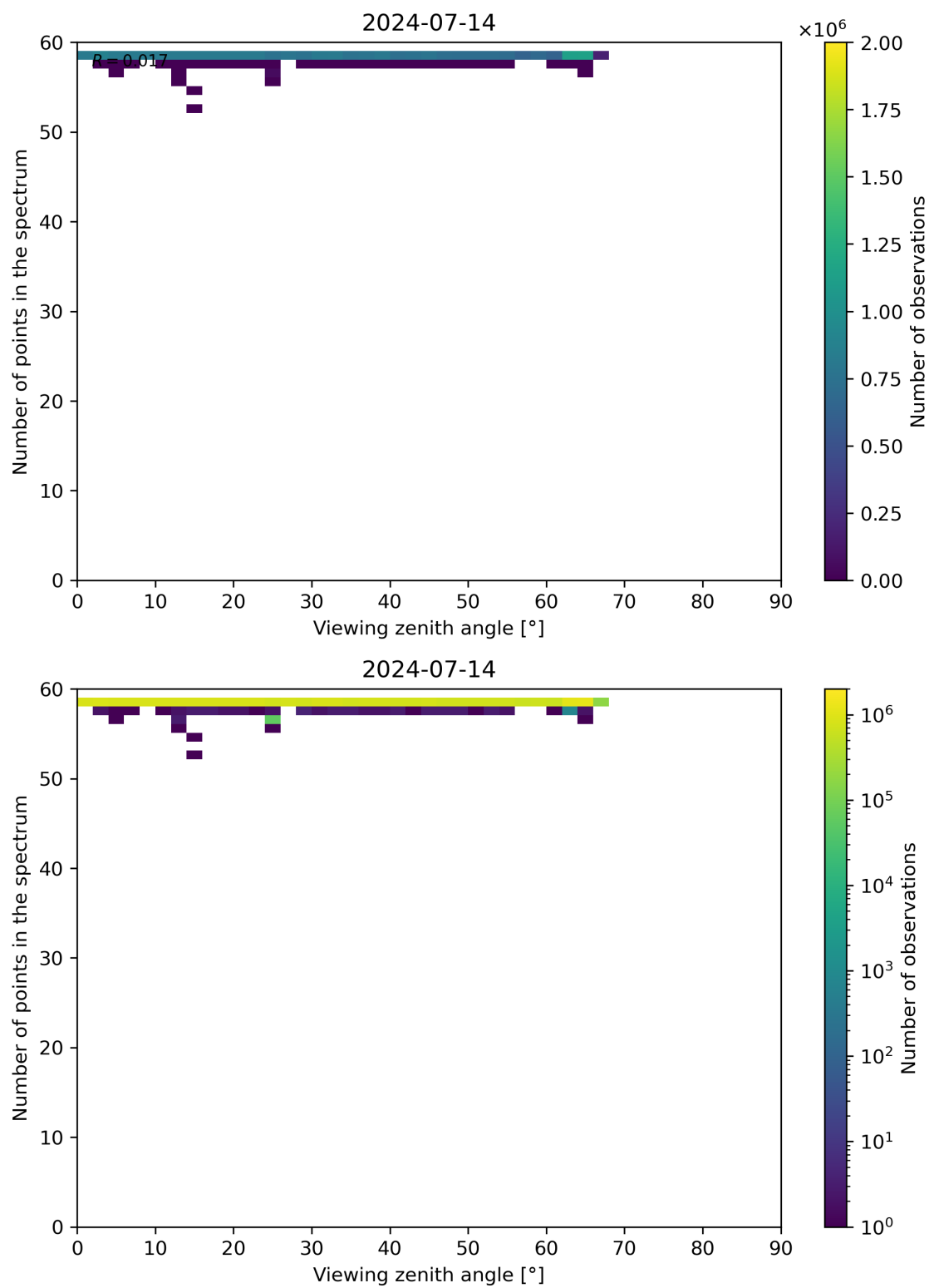
Figure 125: Scatter density plot of “Viewing zenith angle” against “Number of points in the spectrum” for 2024-07-13 to 2024-07-15.
