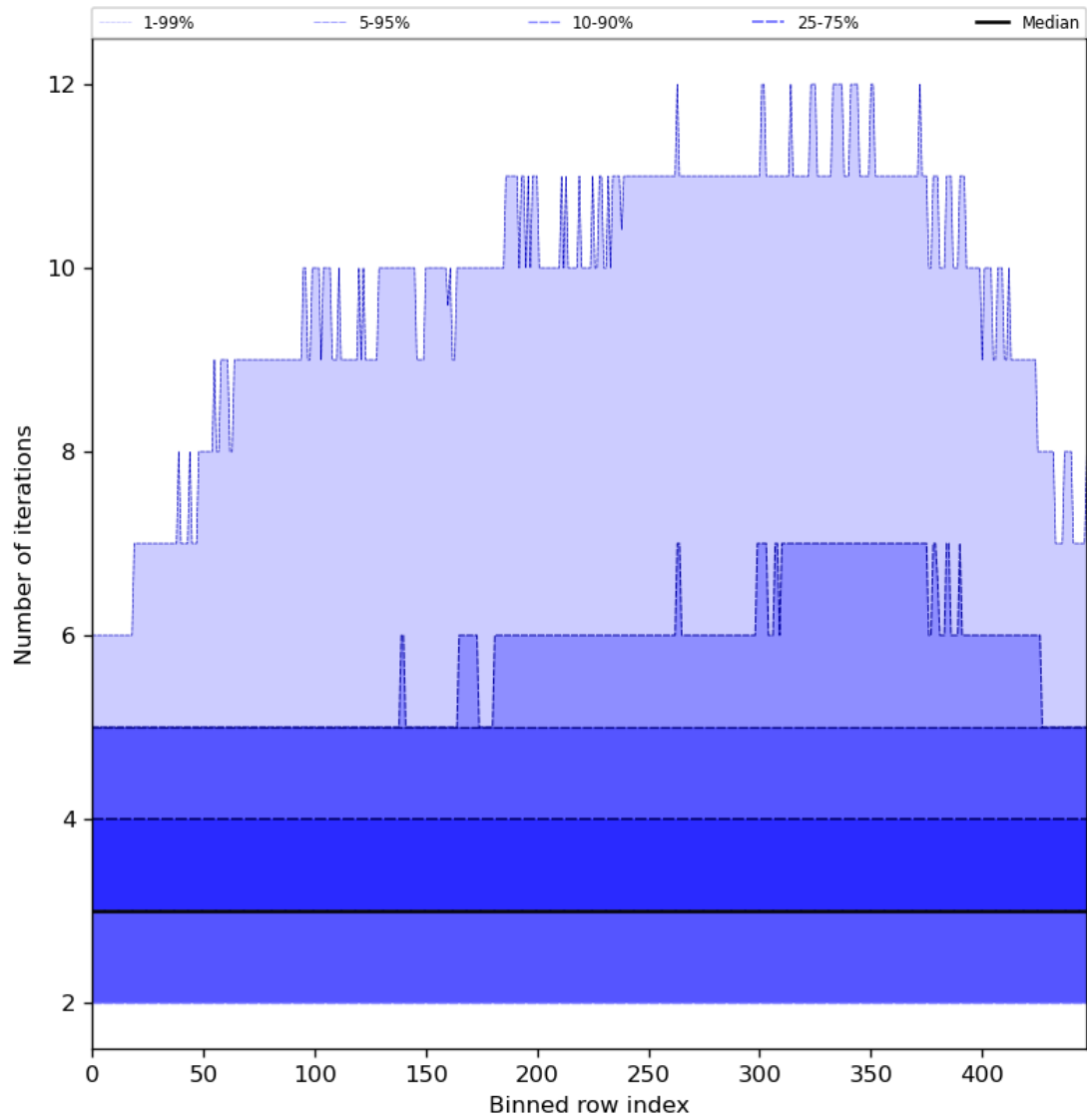
Figure 56: Along track statistics of “Number of iterations” for 2024-07-13 to 2024-07-15
