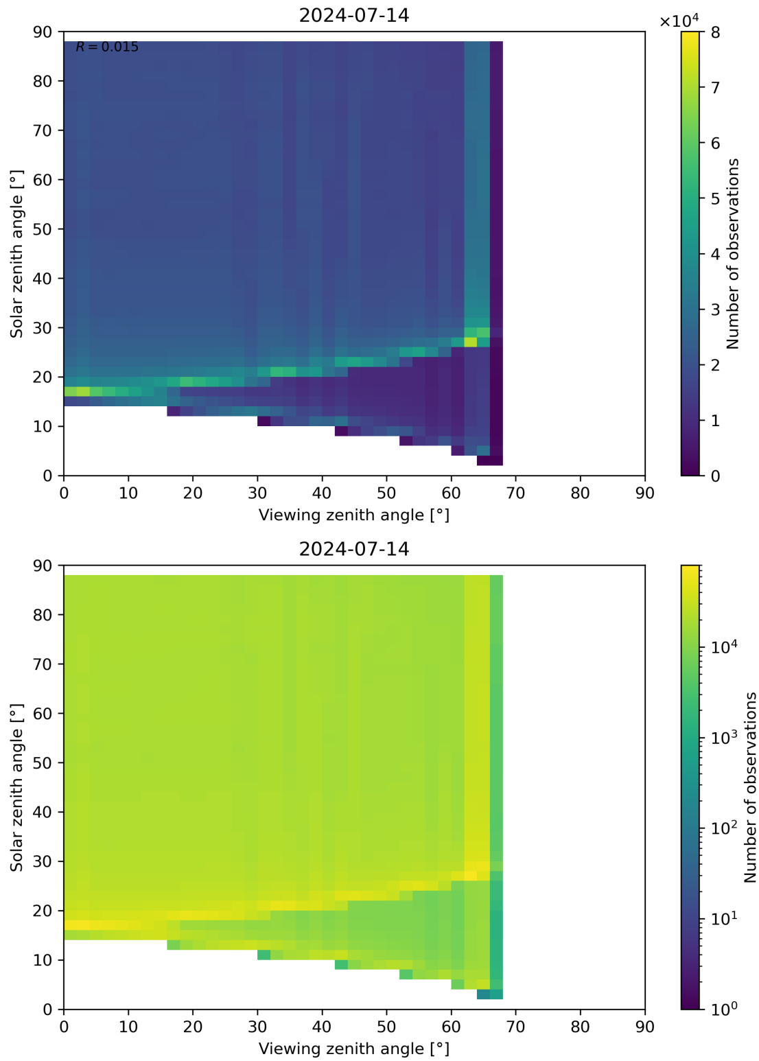
Figure 127: Scatter density plot of “Viewing zenith angle” against “Solar zenith angle” for 2024-07-13 to 2024-07-15.
