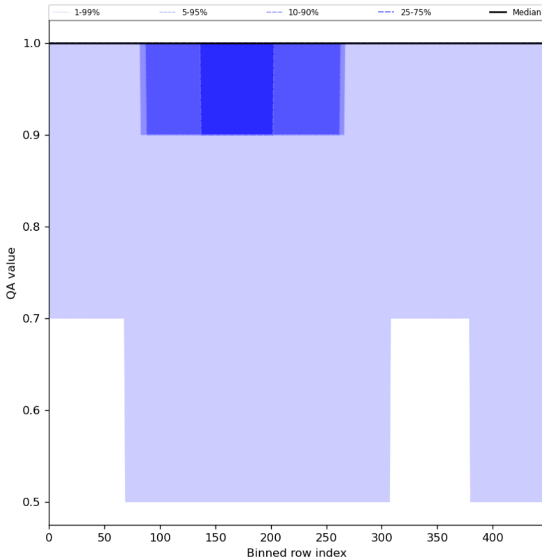
Figure 46: Along track statistics of “QA value” for 2024-07-13 to 2024-07-15
