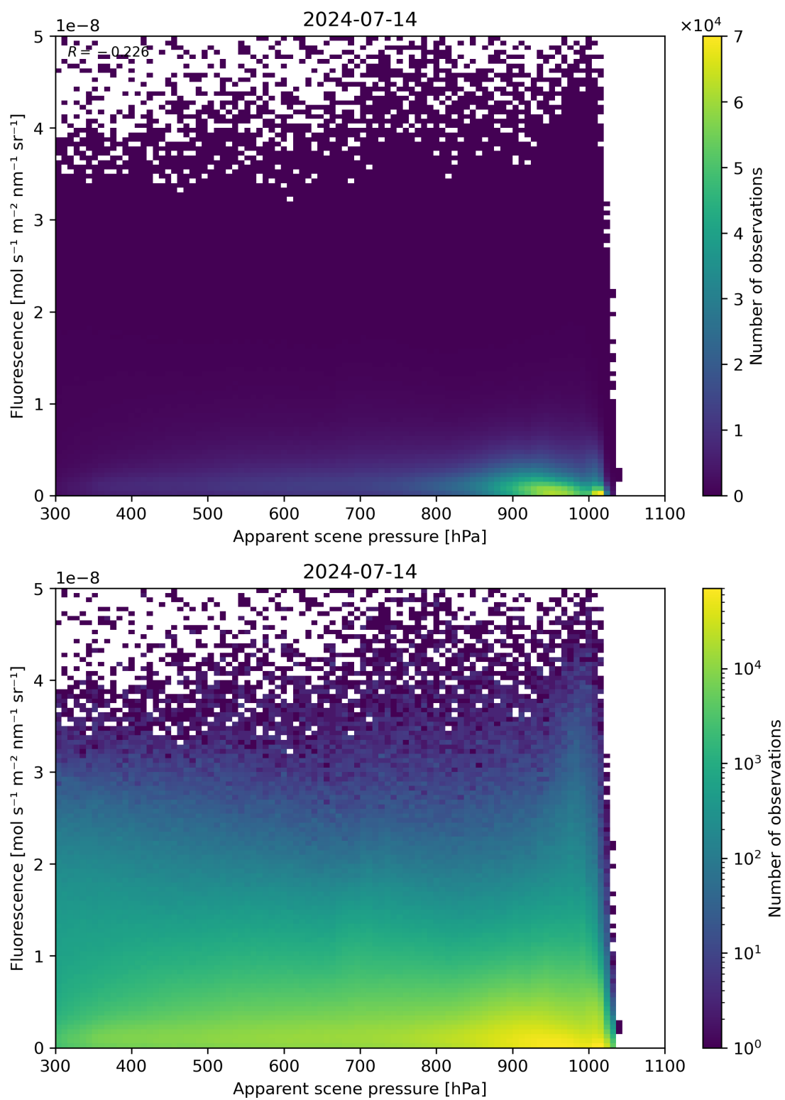
Figure 64: Scatter density plot of “Apparent scene pressure” against “Fluorescence” for 2024-07-13 to 2024-07-15.
