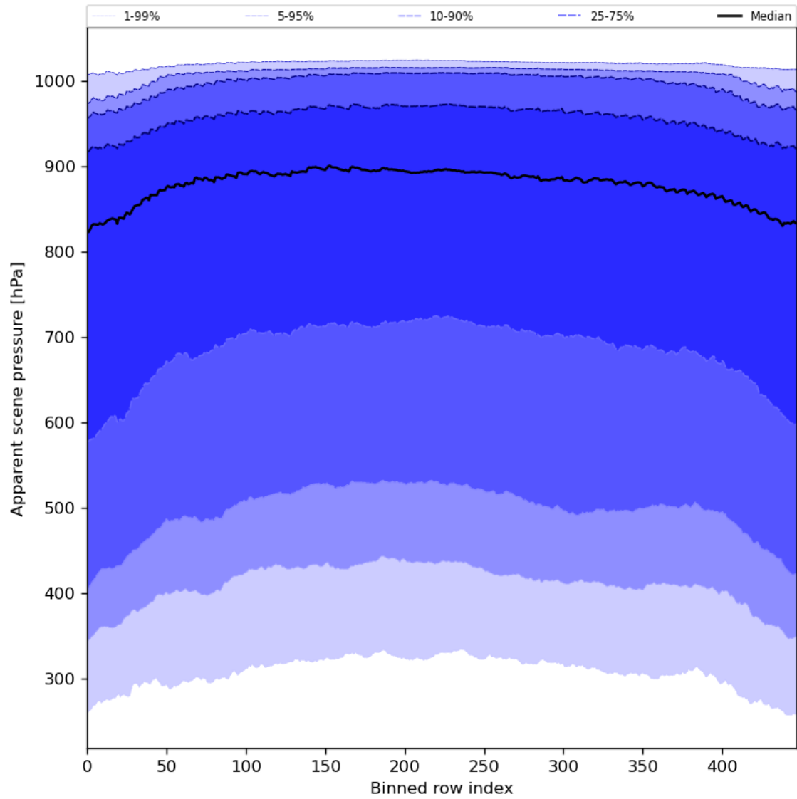
Figure 53: Along track statistics of “Apparent scene pressure” for 2024-07-13 to 2024-07-15
