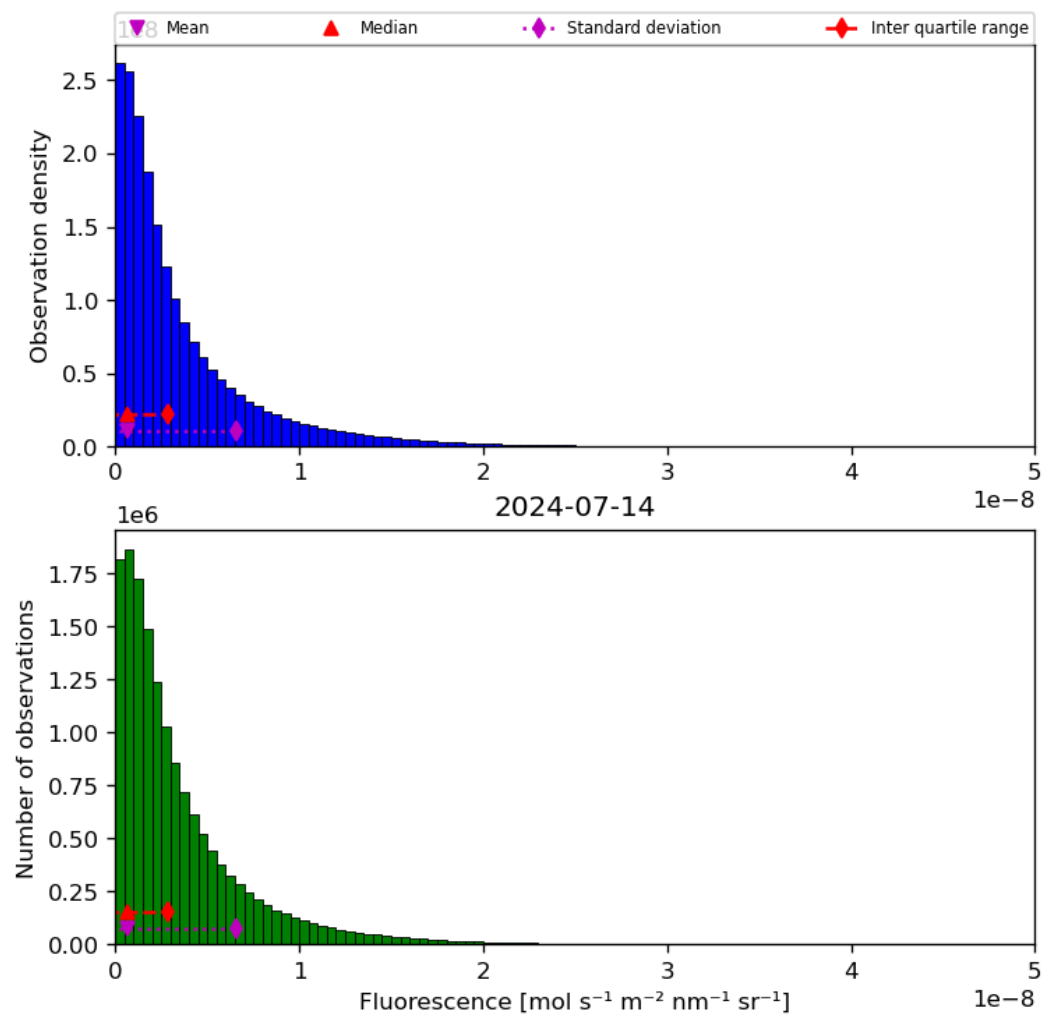
Figure 40: Histogram of “Fluorescence” for 2024-07-13 to 2024-07-15
