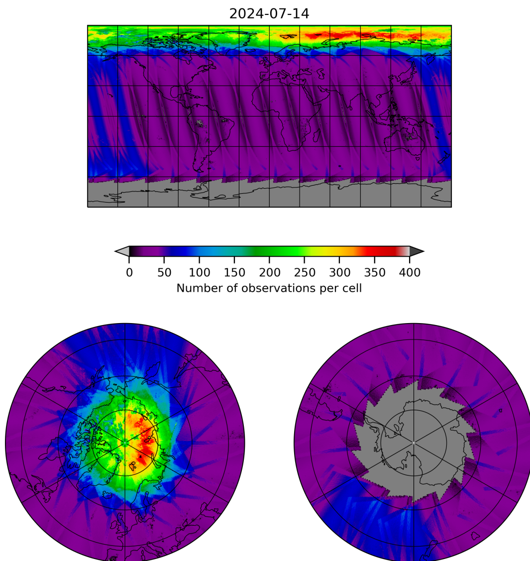
Figure 11: Map of the number of observations for 2024-07-13 to 2024-07-15
