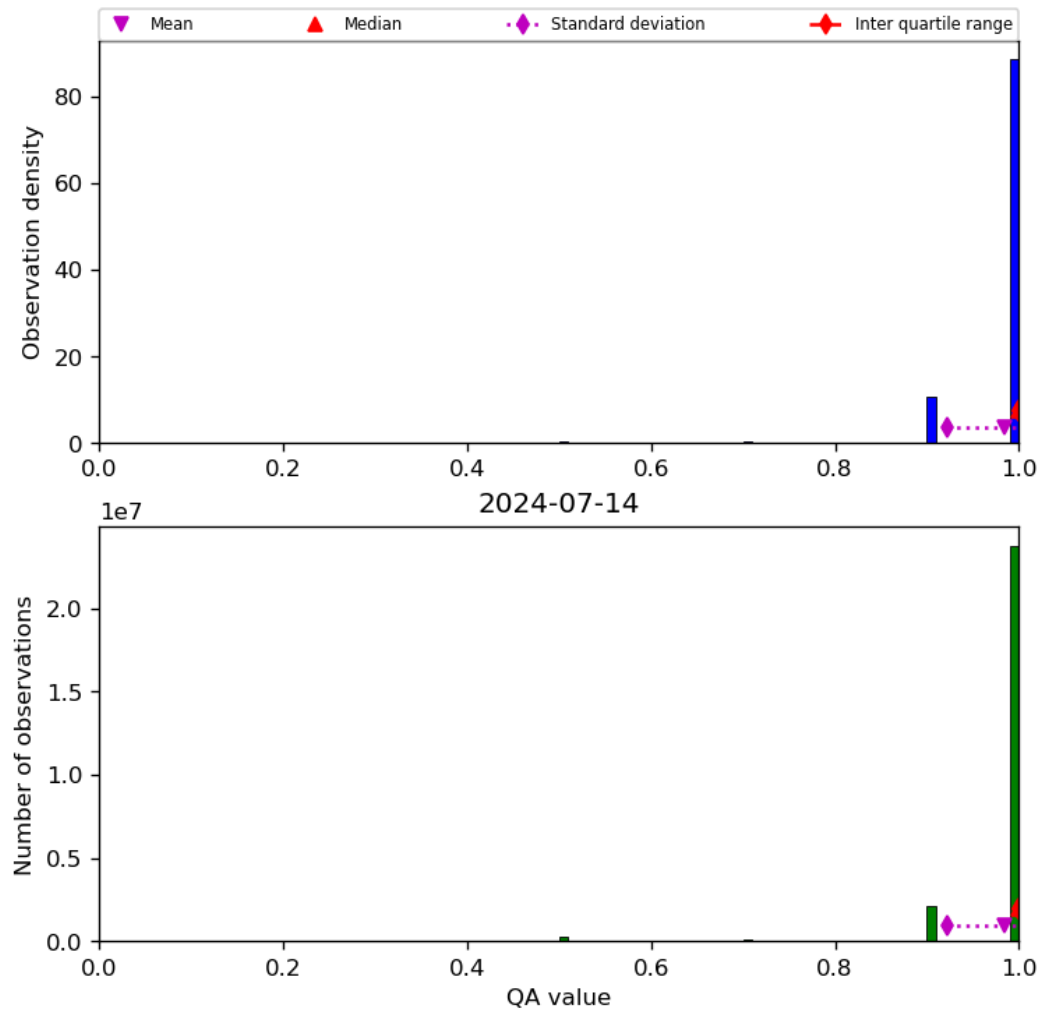
Figure 29: Histogram of “QA value” for 2024-07-13 to 2024-07-15
