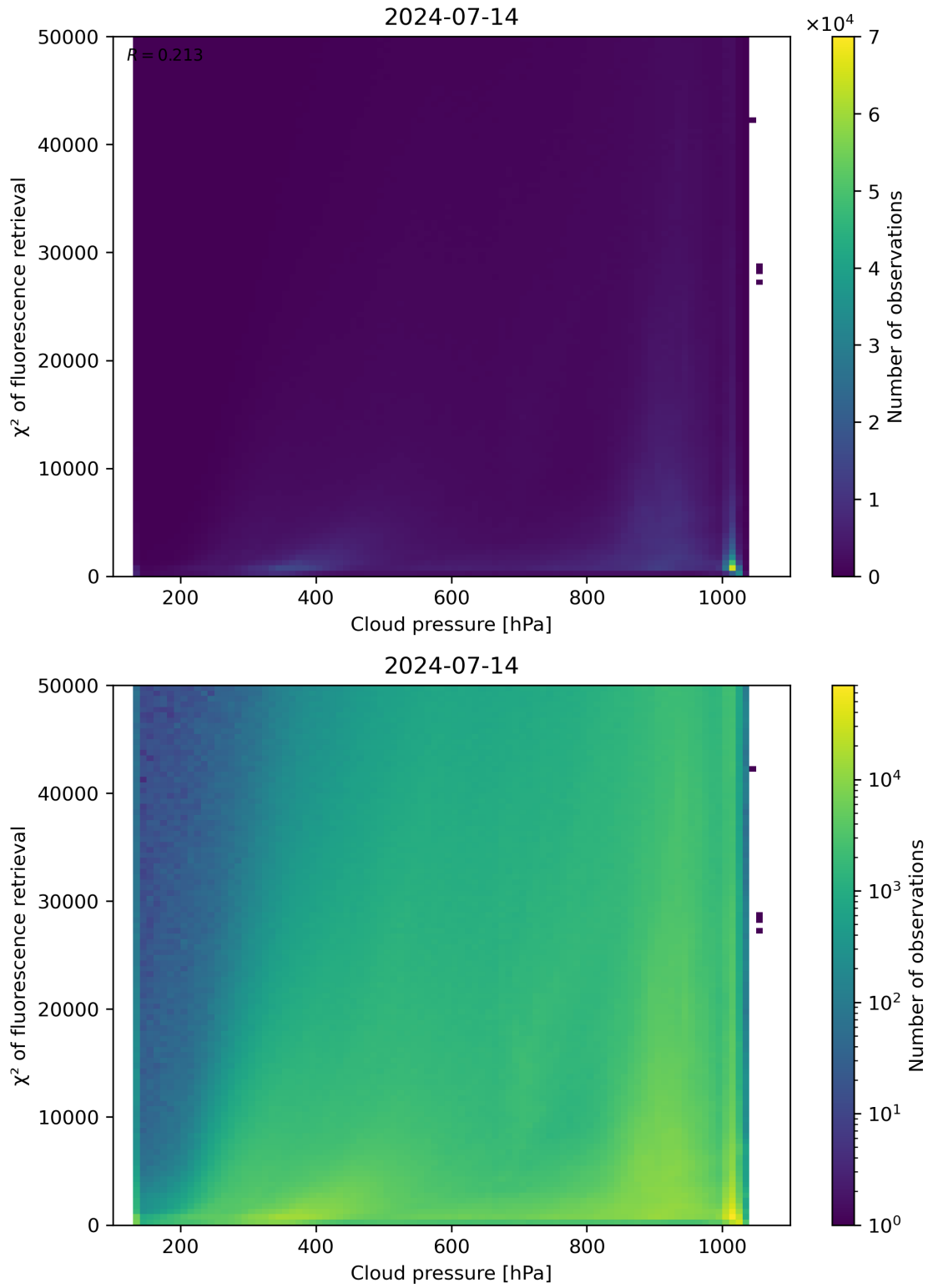
Figure 78: Scatter density plot of “Cloud pressure” against “ \chi^2 of fluorescence retrieval” for 2024-07-13 to 2024-07-15.
