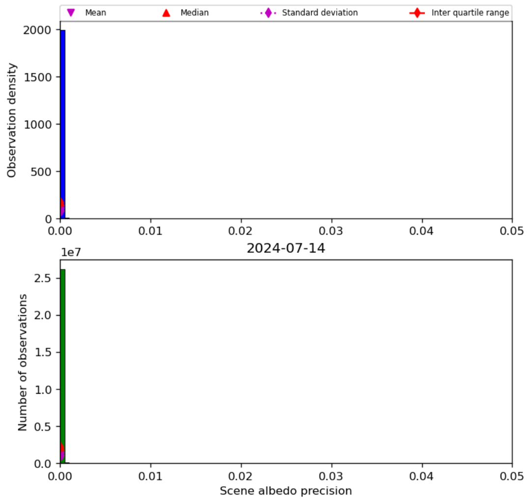
Figure 35: Histogram of “Scene albedo precision” for 2024-07-13 to 2024-07-15
