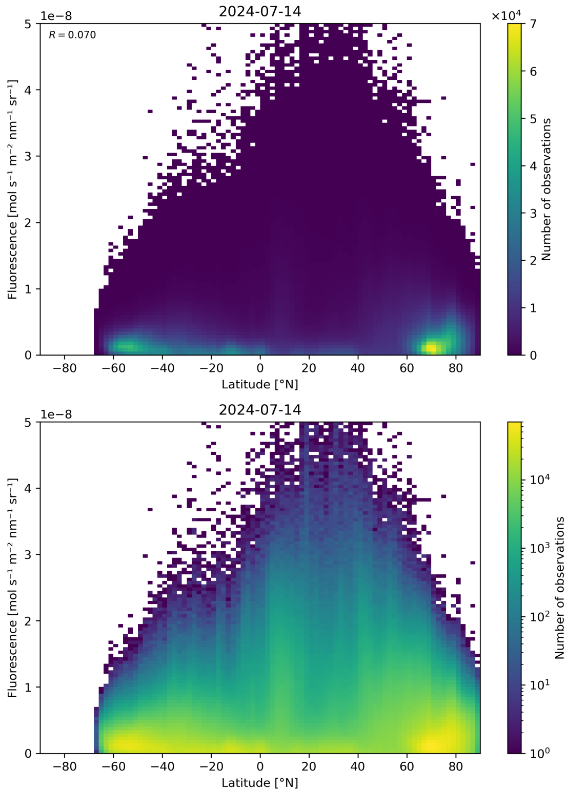
Figure 92: Scatter density plot of “Latitude” against “Fluorescence” for 2024-07-13 to 2024-07-15.
