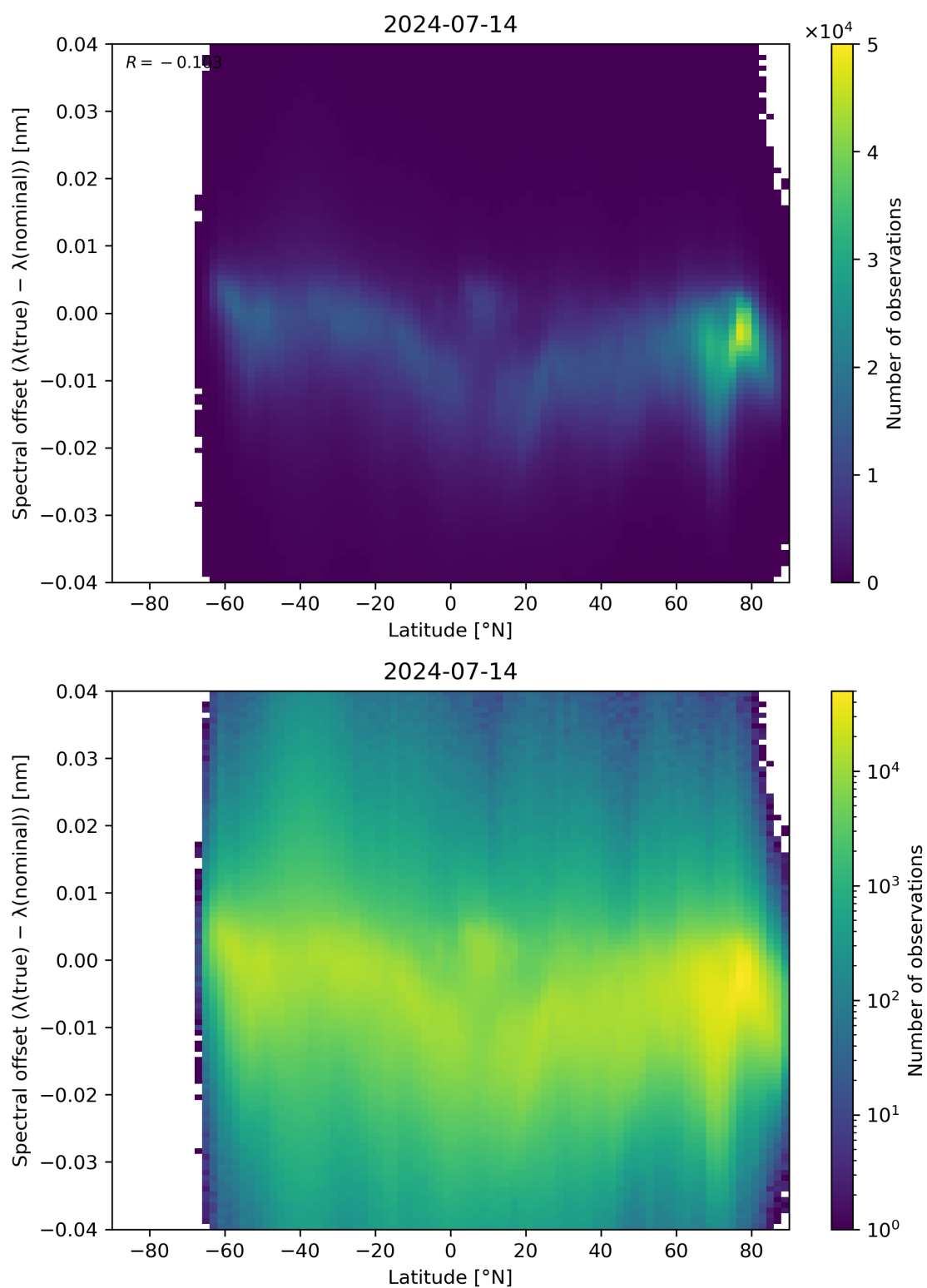
Figure 96: Scatter density plot of “Latitude” against “Spectral offset ( \lambda(\text{true}) - \lambda(\text{nominal}) )” for 2024-07-13 to 2024-07-15.
