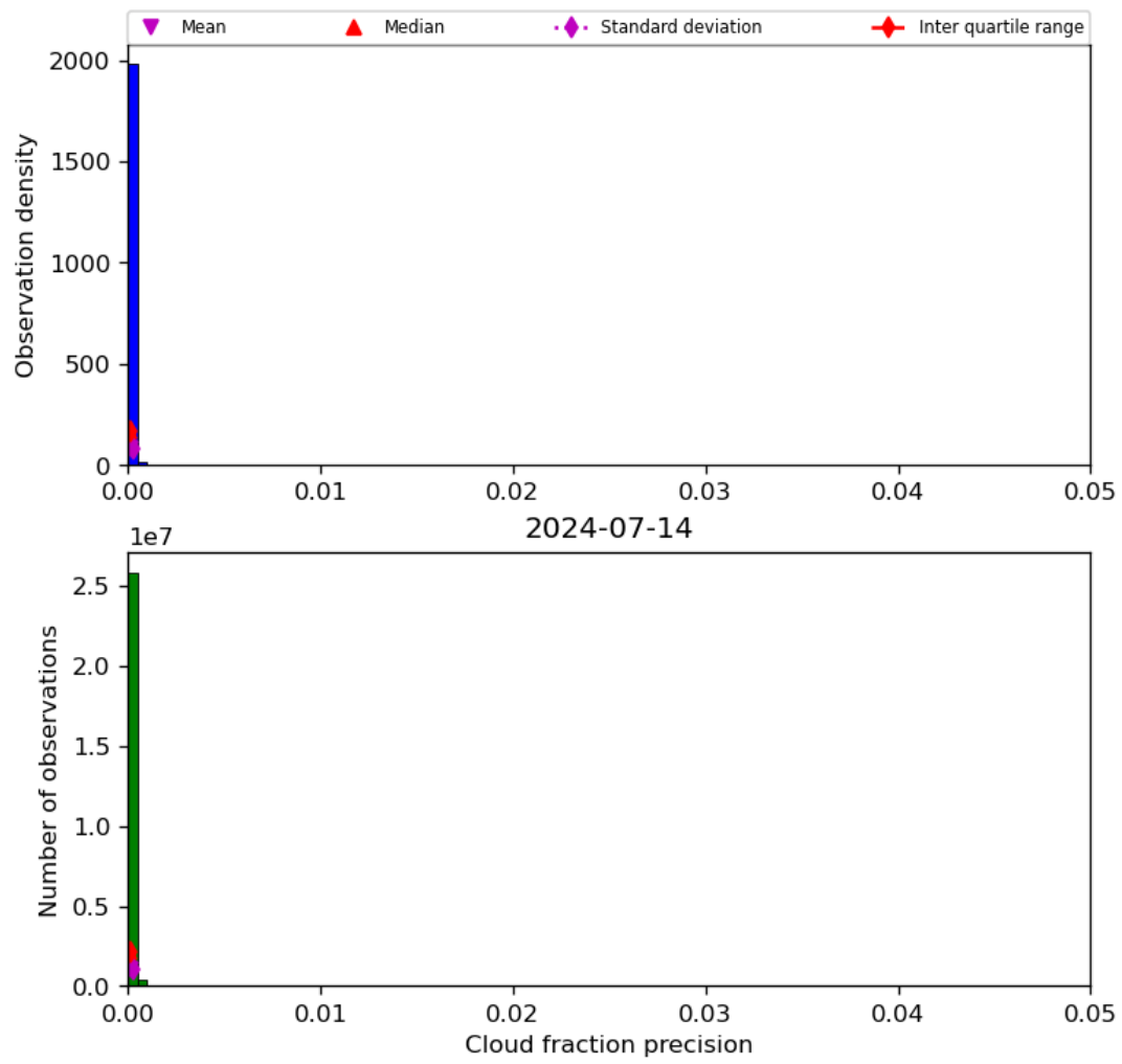
Figure 33: Histogram of “Cloud fraction precision” for 2024-07-13 to 2024-07-15
