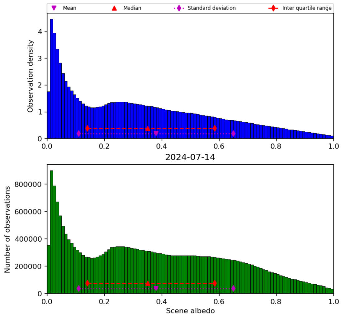
Figure 34: Histogram of “Scene albedo” for 2024-07-13 to 2024-07-15
