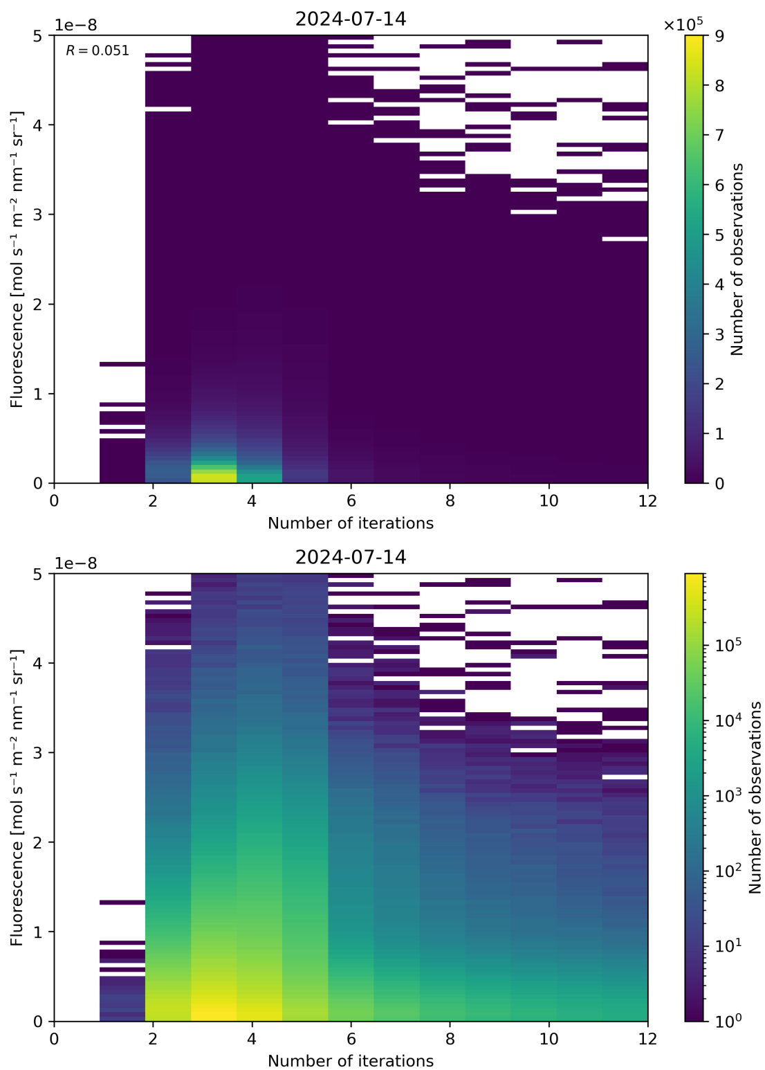
Figure 98: Scatter density plot of “Number of iterations” against “Fluorescence” for 2024-07-13 to 2024-07-15.
