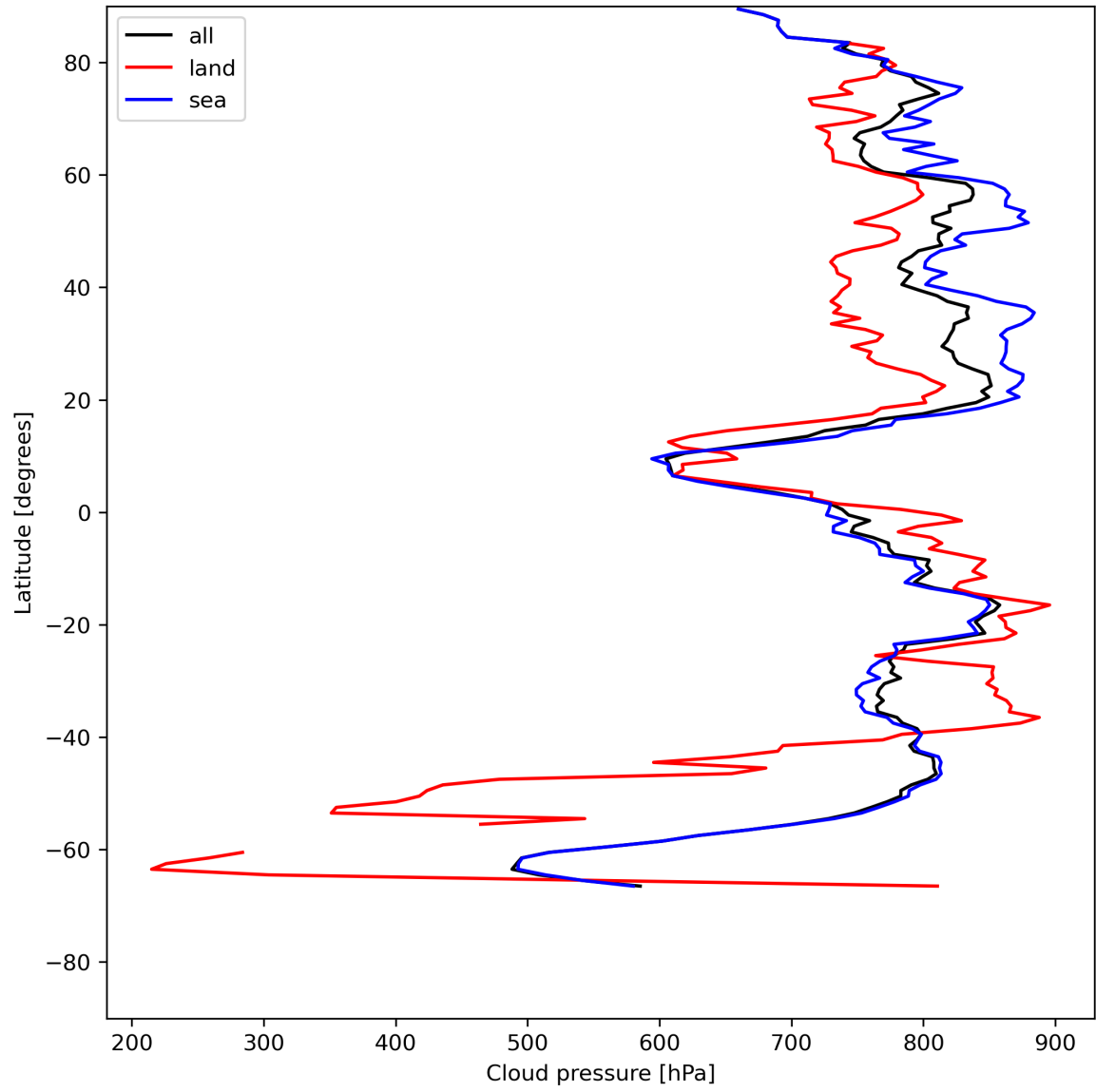
Figure 13: Zonal average of “Cloud pressure” for 2024-07-13 to 2024-07-15.
