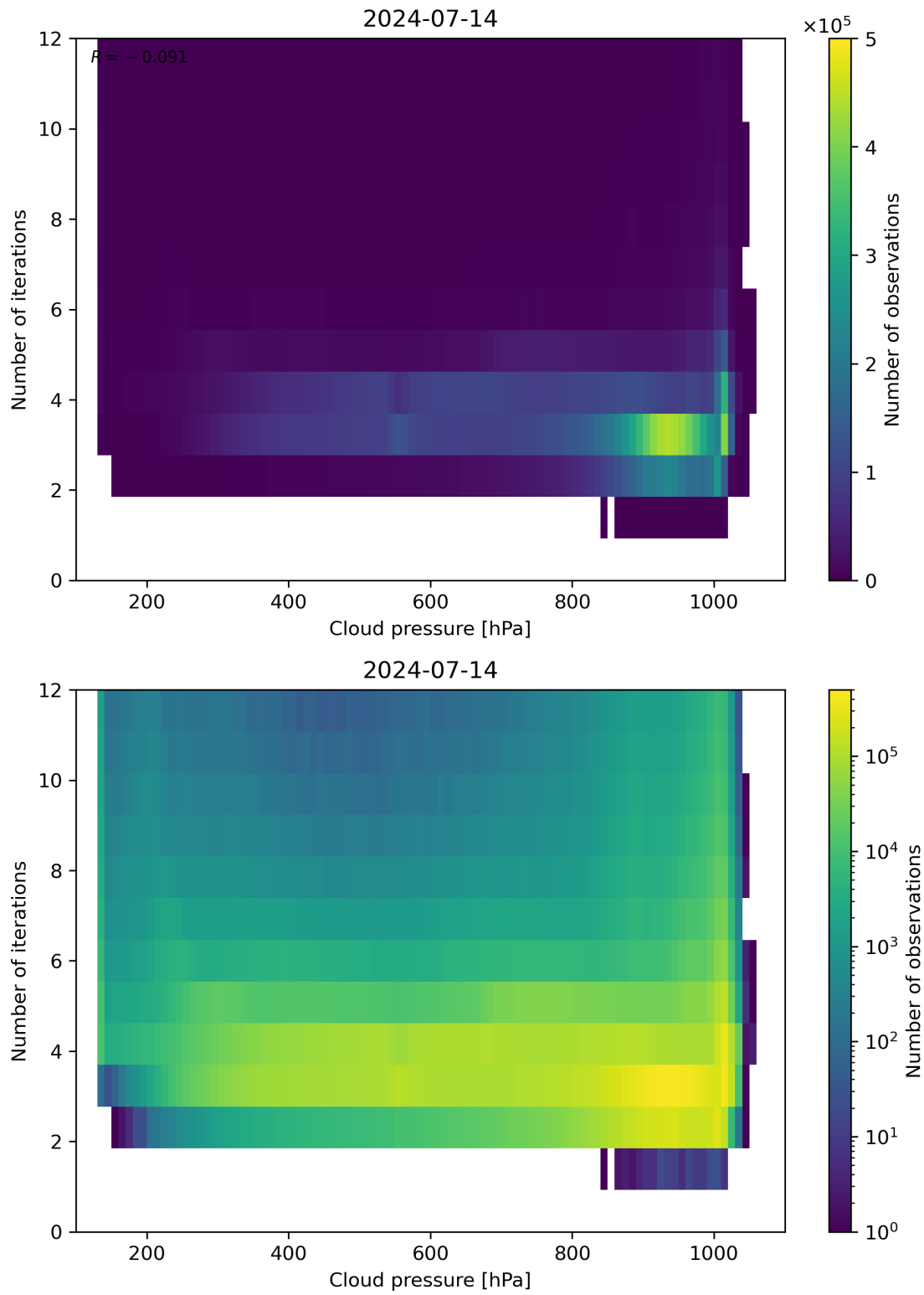
Figure 81: Scatter density plot of “Cloud pressure” against “Number of iterations” for 2024-07-13 to 2024-07-15.
