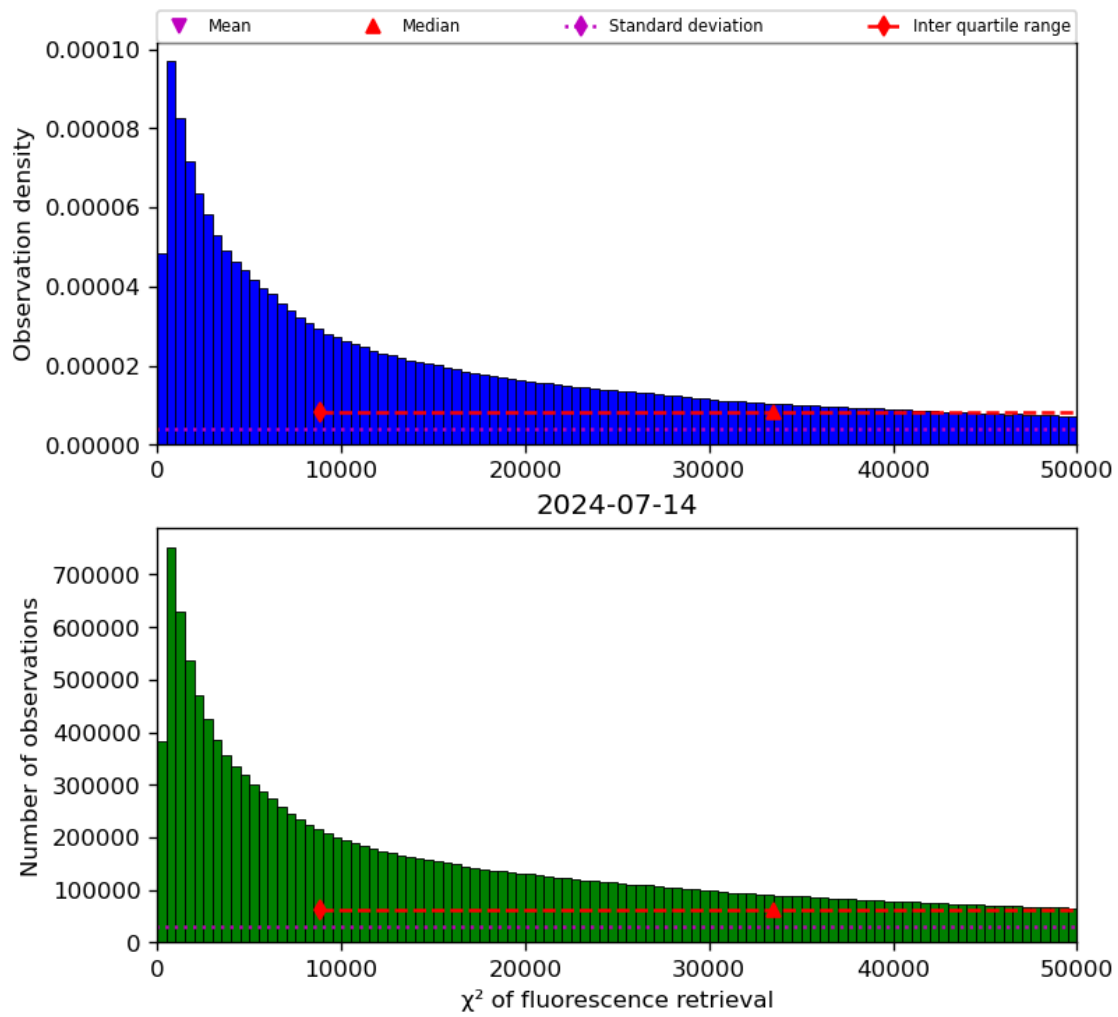
Figure 42: Histogram of “ \chi^2 of fluorescence retrieval” for 2024-07-13 to 2024-07-15
