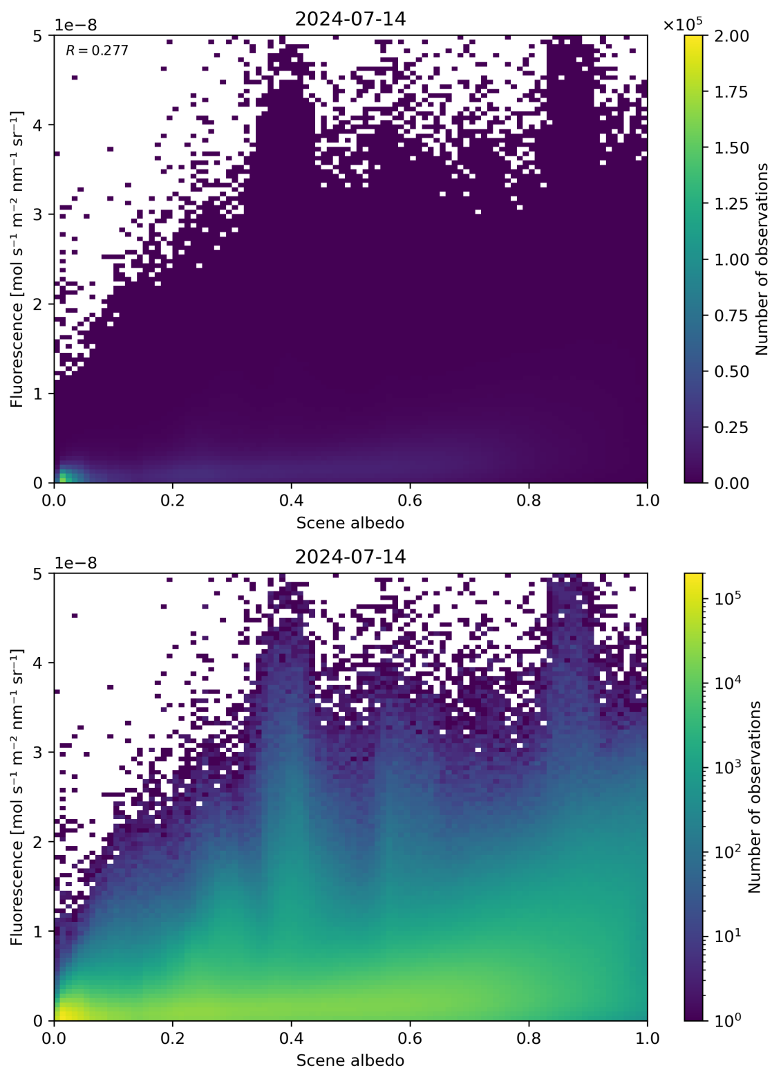
Figure 104: Scatter density plot of “Scene albedo” against “Fluorescence” for 2024-07-13 to 2024-07-15.
