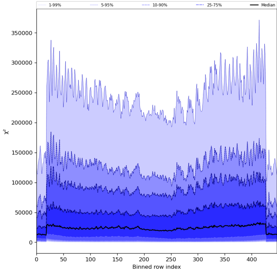
Figure 55: Along track statistics of “ \chi^2 ” for 2024-07-13 to 2024-07-15
