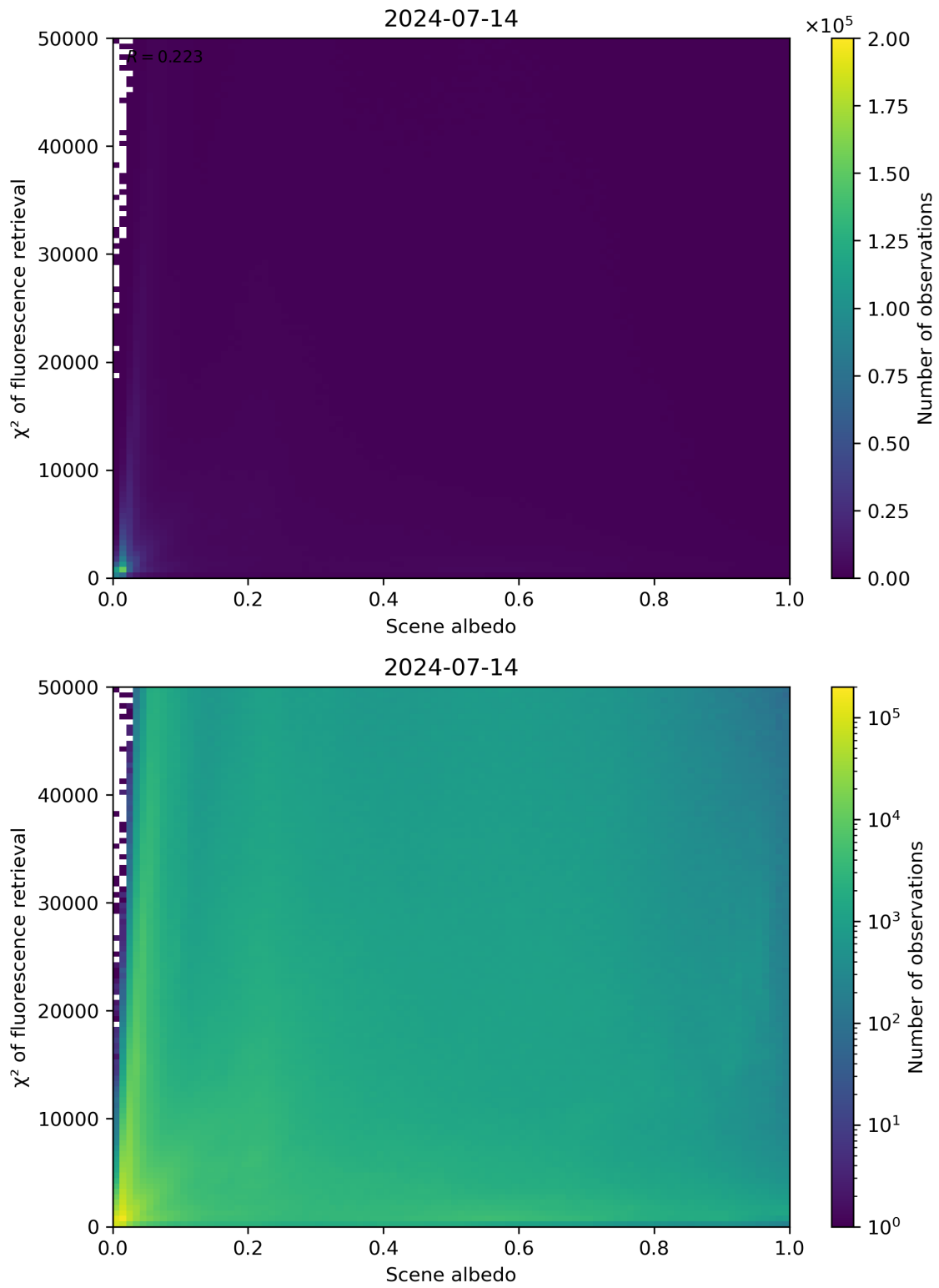
Figure 103: Scatter density plot of “Scene albedo” against “ \chi^2 of fluorescence retrieval” for 2024-07-13 to 2024-07-15.
