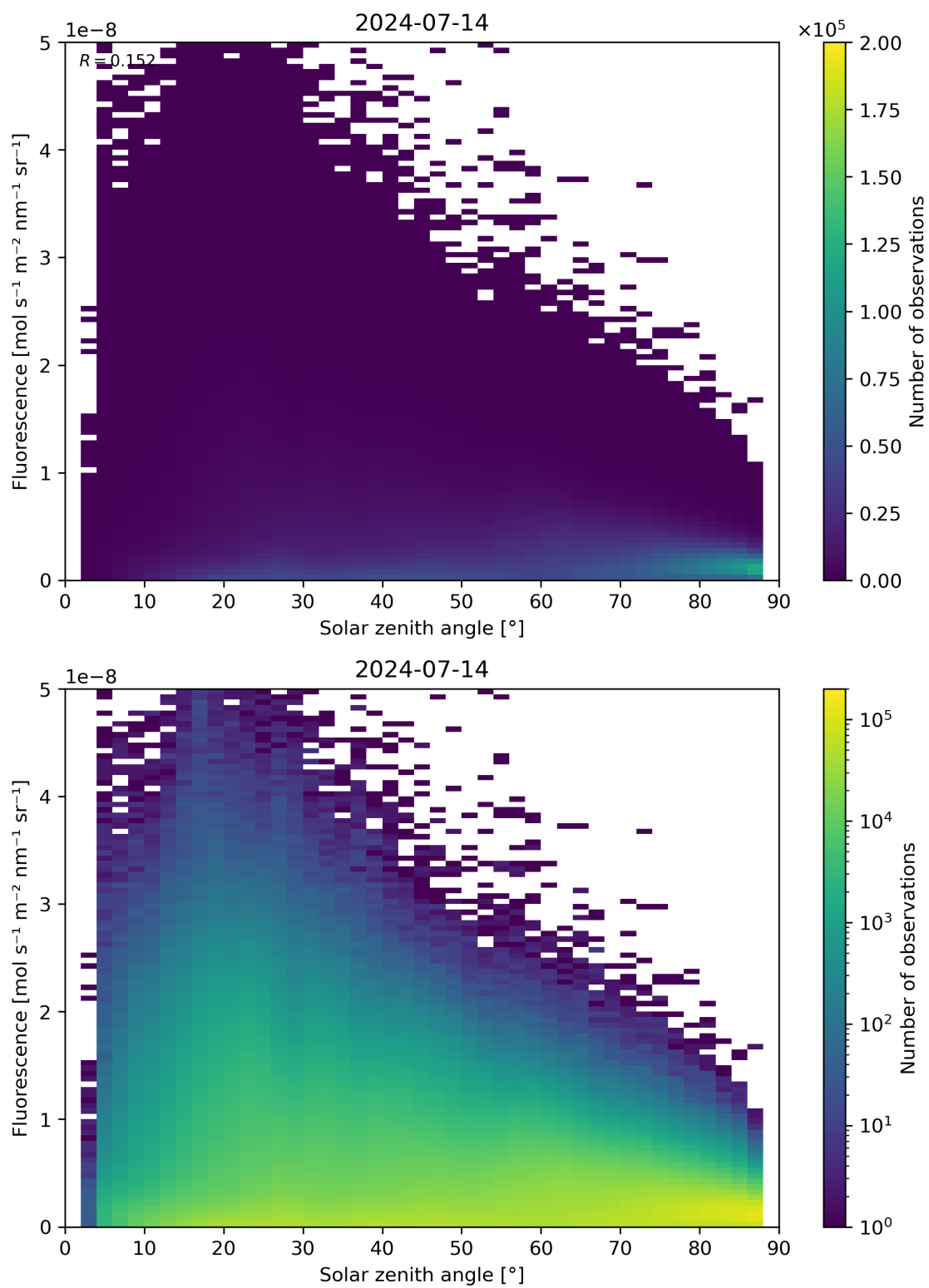
Figure 112: Scatter density plot of “Solar zenith angle” against “Fluorescence” for 2024-07-13 to 2024-07-15.
