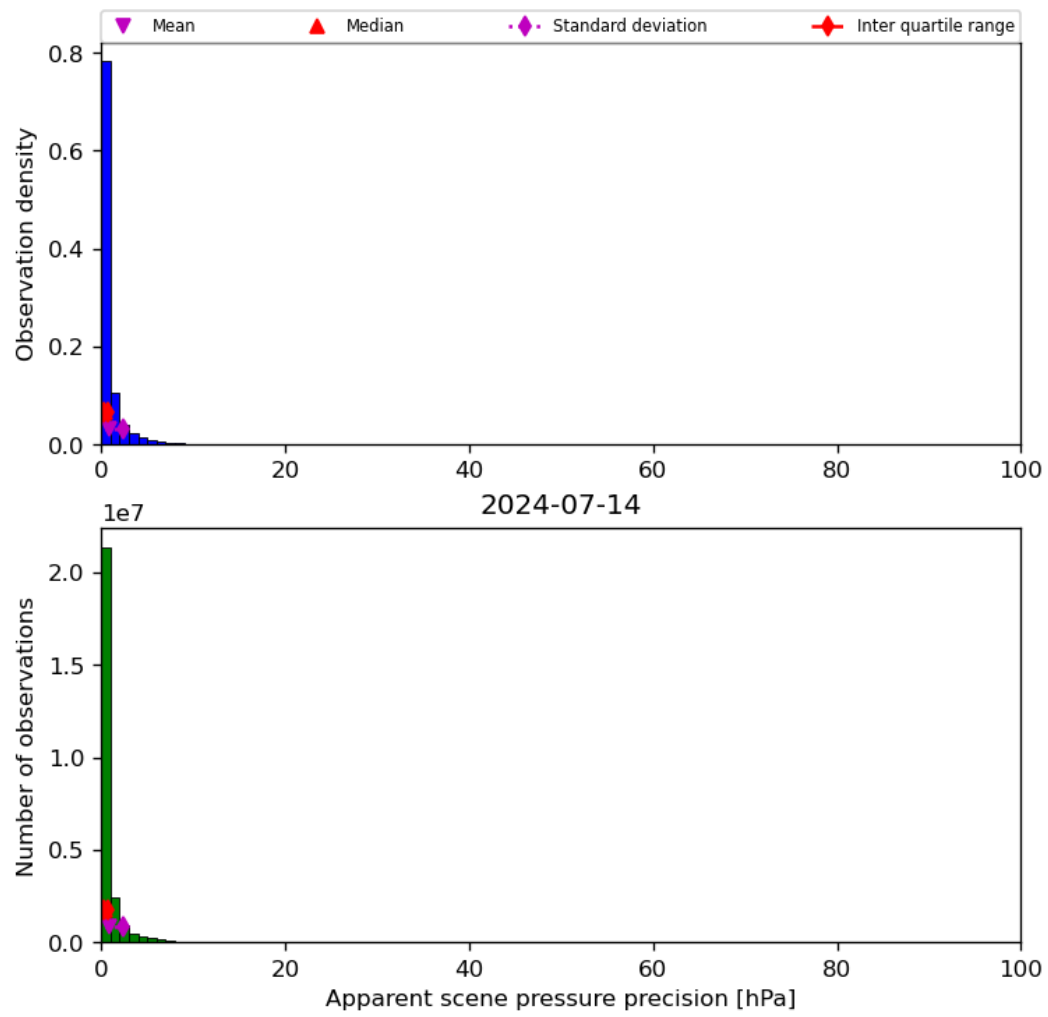
Figure 37: Histogram of “Apparent scene pressure precision” for 2024-07-13 to 2024-07-15
