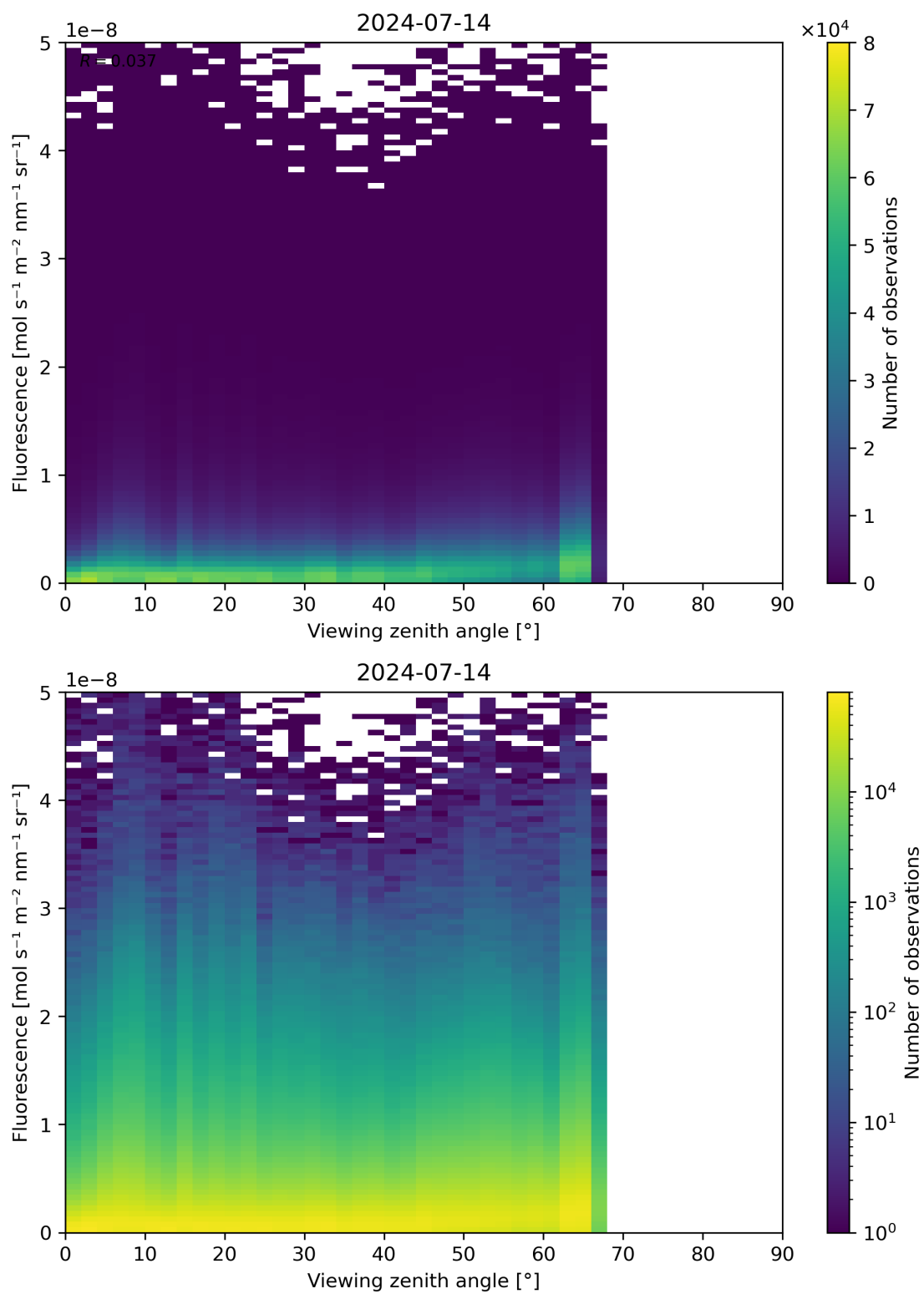
Figure 122: Scatter density plot of “Viewing zenith angle” against “Fluorescence” for 2024-07-13 to 2024-07-15.
