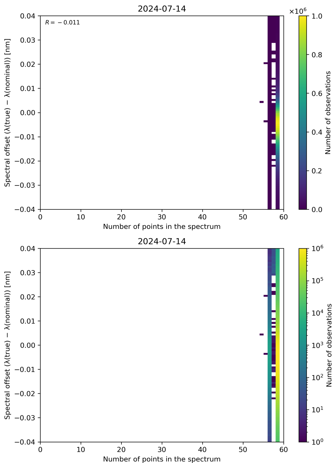
Figure 101: Scatter density plot of “Number of points in the spectrum” against “Spectral offset ( \lambda(\text{true}) - \lambda(\text{nominal}) )” for 2024-07-13 to 2024-07-15.
