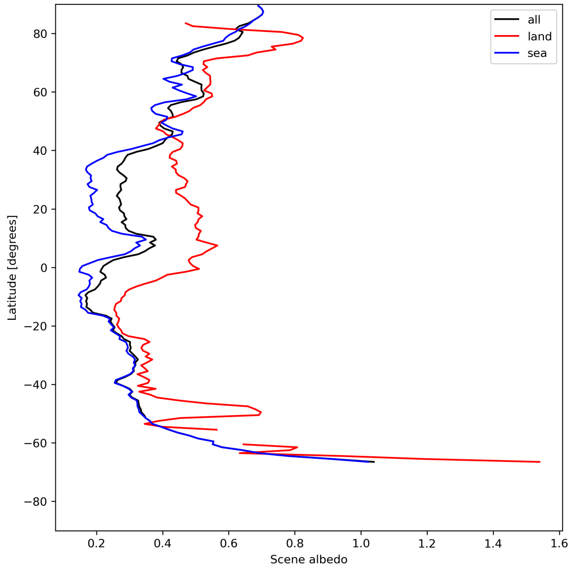
Figure 17: Zonal average of “Scene albedo” for 2024-07-13 to 2024-07-15.
