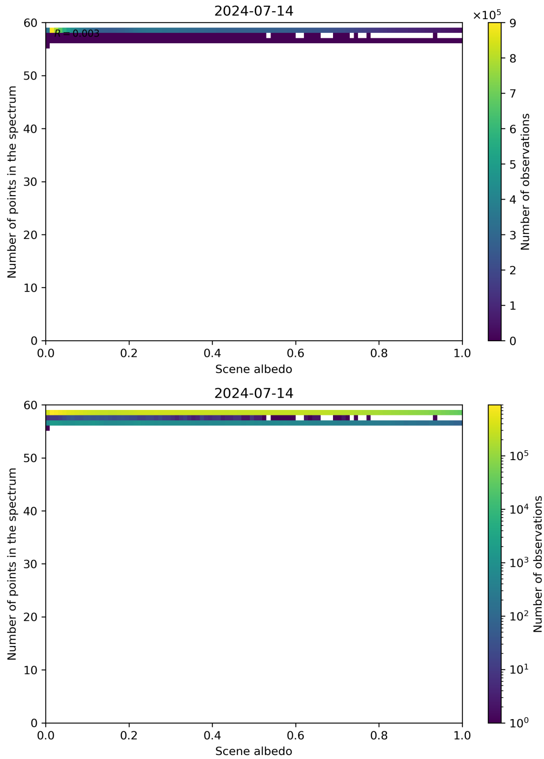
Figure 106: Scatter density plot of “Scene albedo” against “Number of points in the spectrum” for 2024-07-13 to 2024-07-15.
