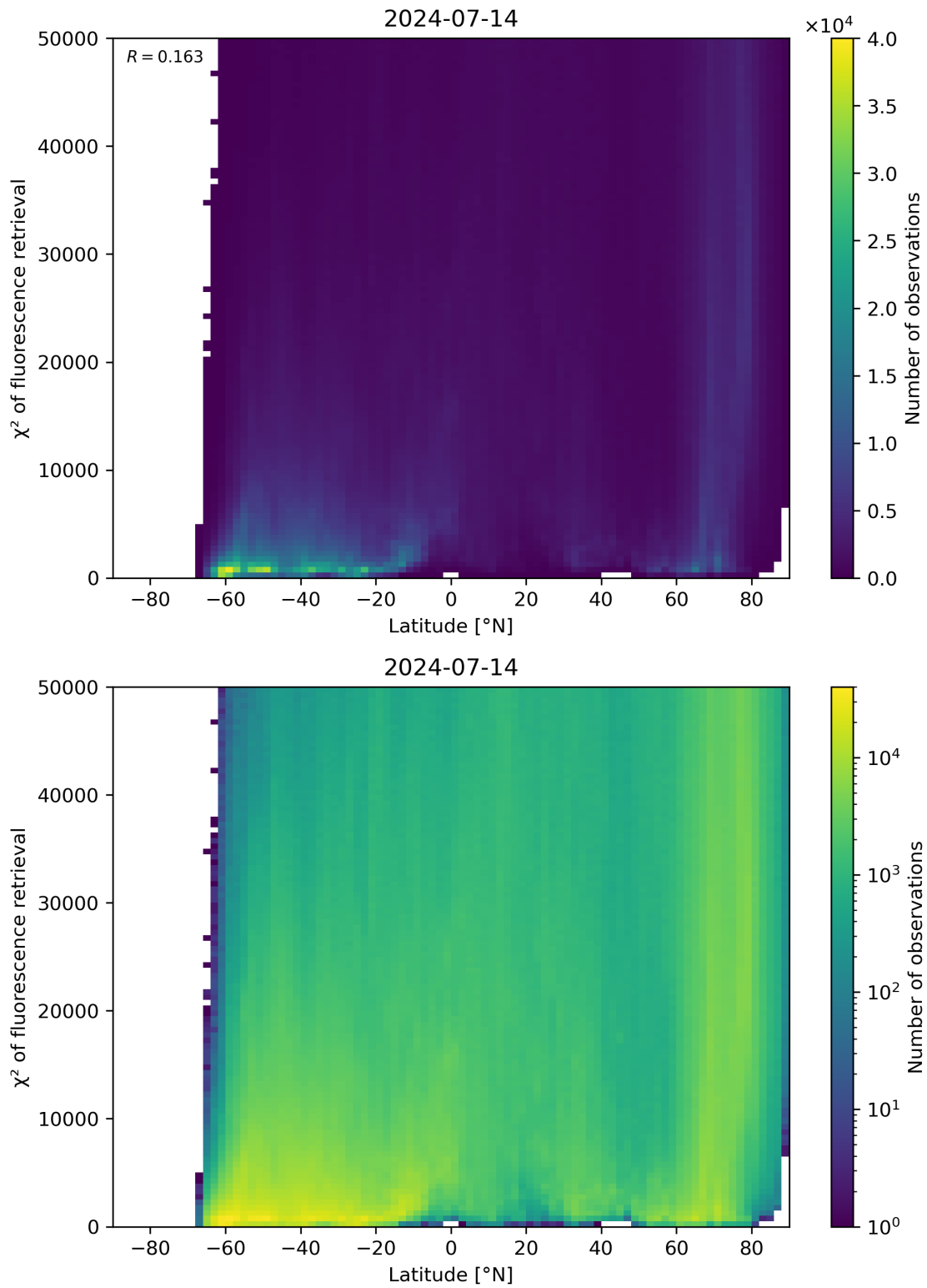
Figure 89: Scatter density plot of “Latitude” against “ \chi^2 of fluorescence retrieval” for 2024-07-13 to 2024-07-15.
