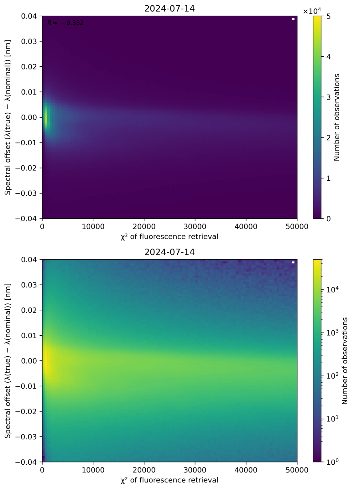
Figure 69: Scatter density plot of “ \chi^2 of fluorescence retrieval” against “Spectral offset ( \lambda(\text{true}) - \lambda(\text{nominal}) )” for 2024-07-13 to 2024-07-15.
