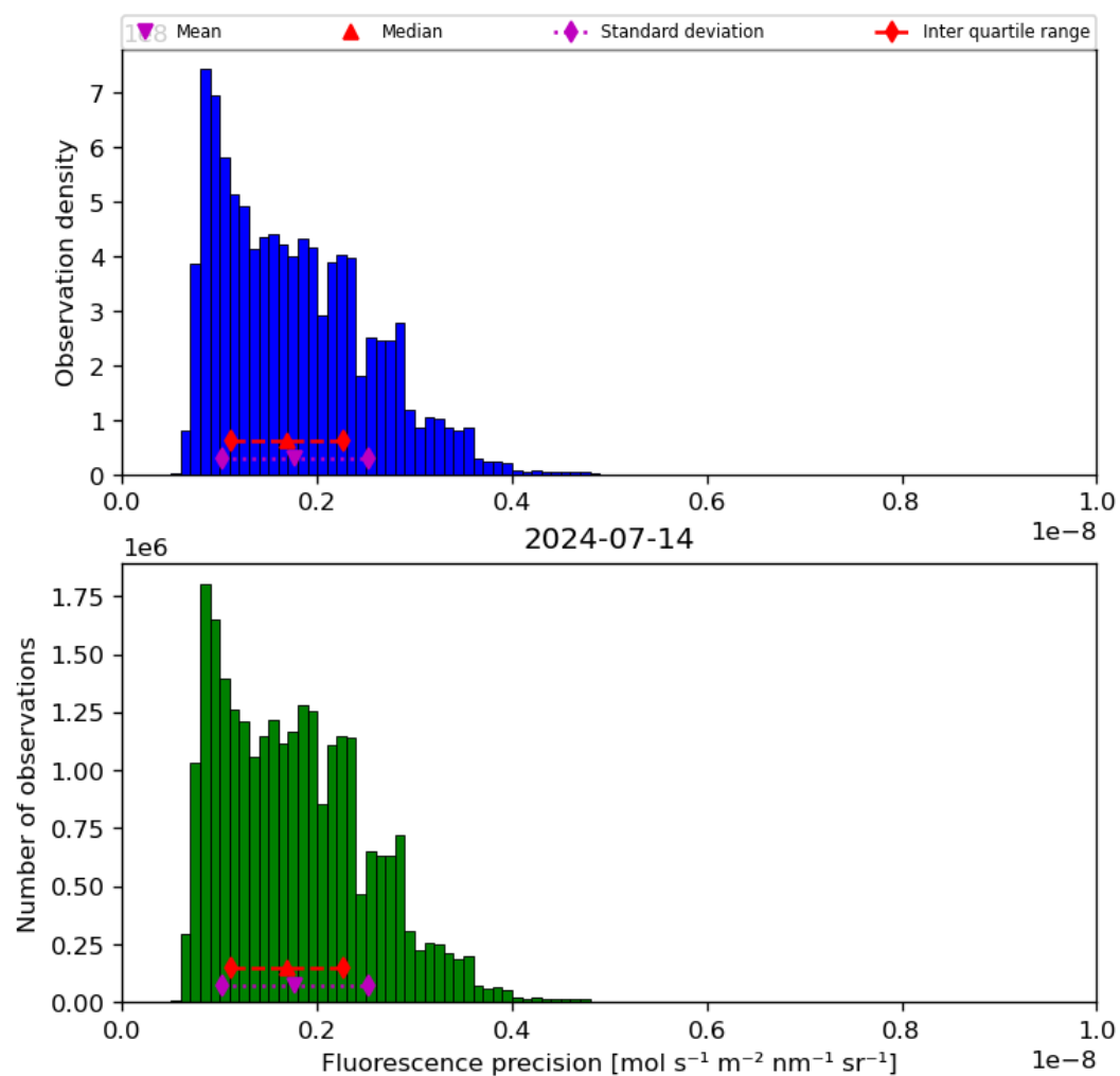
Figure 41: Histogram of “Fluorescence precision” for 2024-07-13 to 2024-07-15
