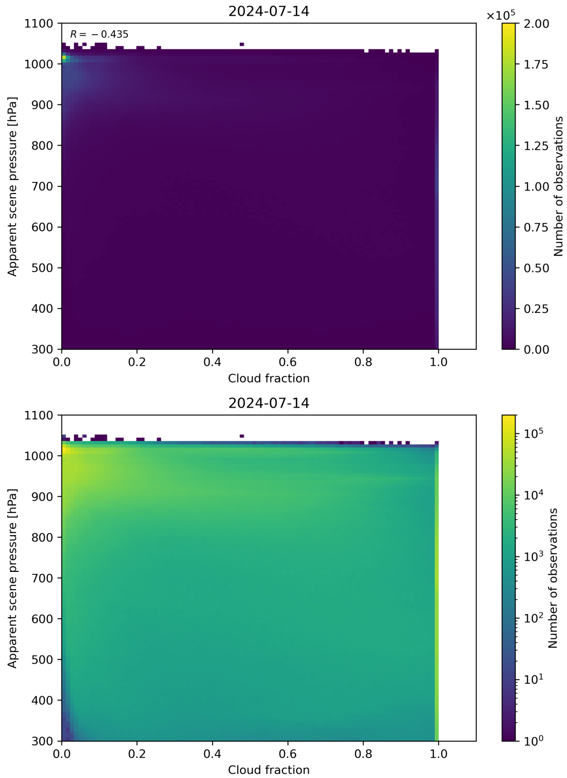
Figure 70: Scatter density plot of “Cloud fraction” against “Apparent scene pressure” for 2024-07-13 to 2024-07-15.
