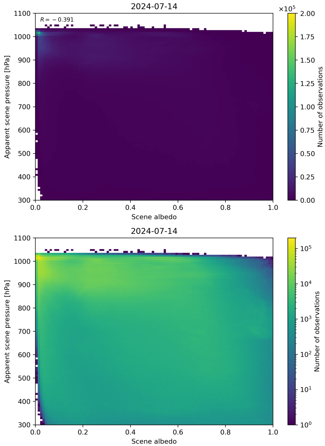
Figure 102: Scatter density plot of “Scene albedo” against “Apparent scene pressure” for 2024-07-13 to 2024-07-15.
