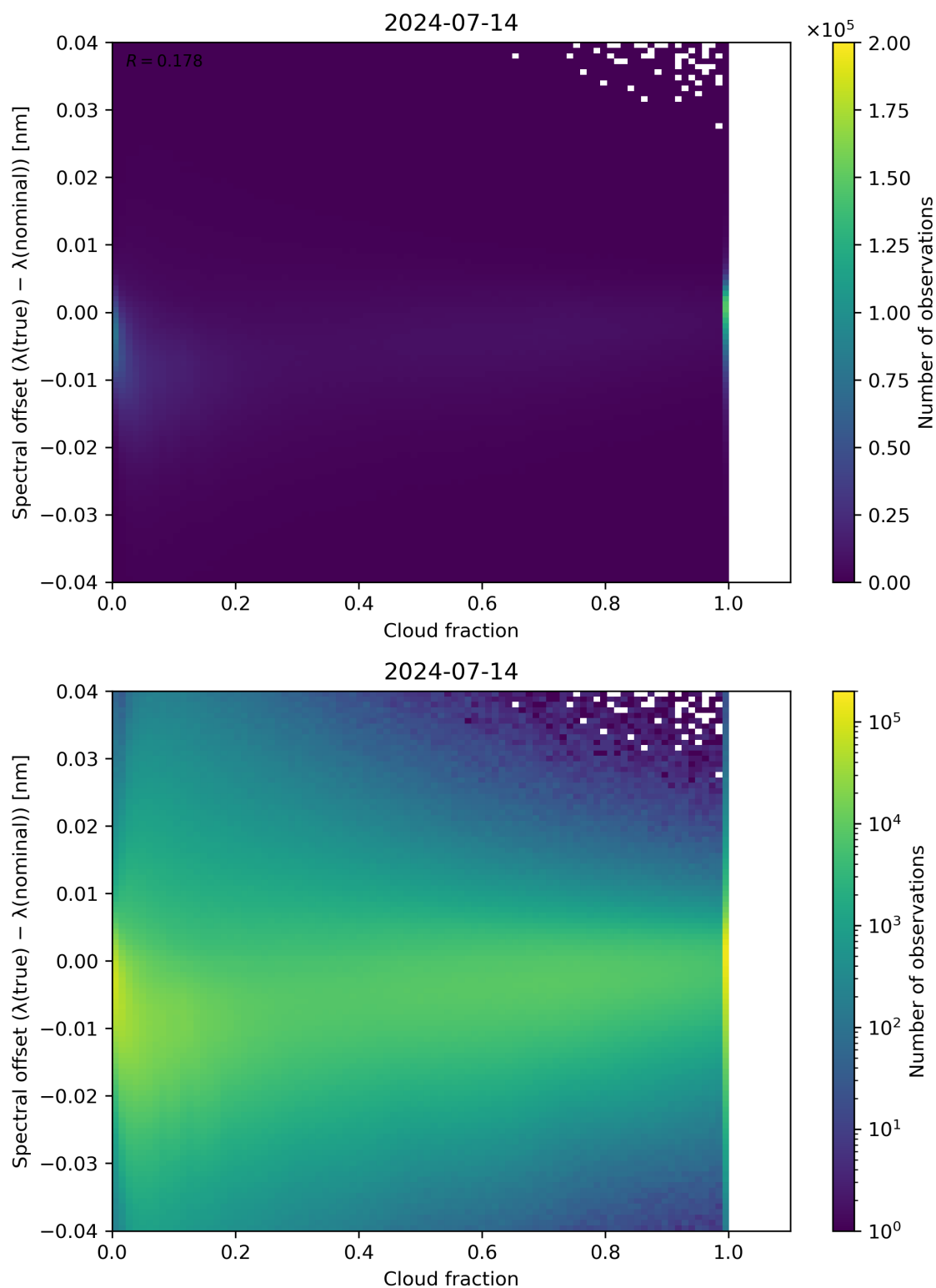
Figure 76: Scatter density plot of “Cloud fraction” against “Spectral offset ( \lambda(\text{true}) - \lambda(\text{nominal}) )” for 2024-07-13 to 2024-07-15.
