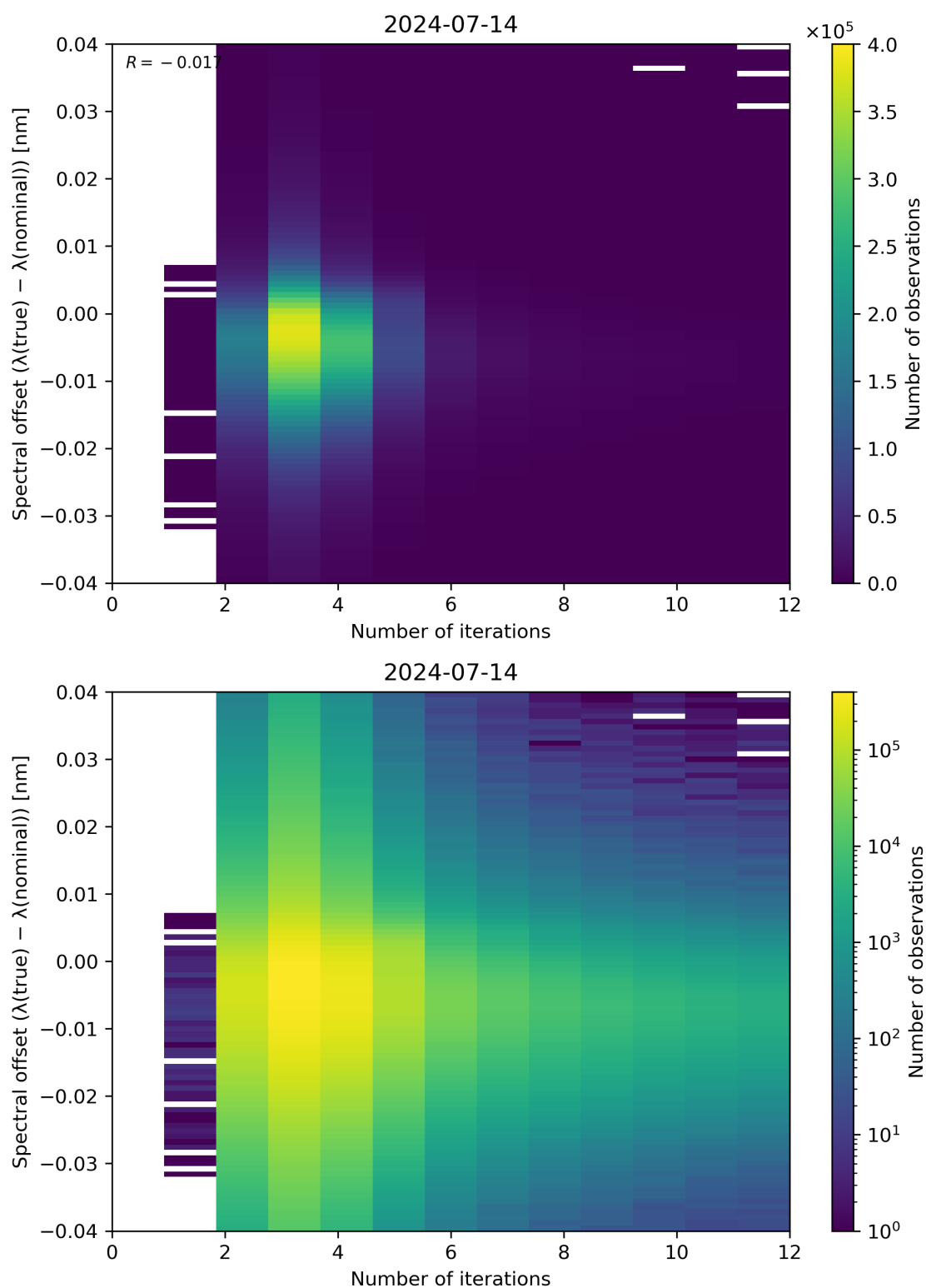
Figure 100: Scatter density plot of “Number of iterations” against “Spectral offset ( \lambda(\text{true}) - \lambda(\text{nominal}) )” for 2024-07-13 to 2024-07-15.
