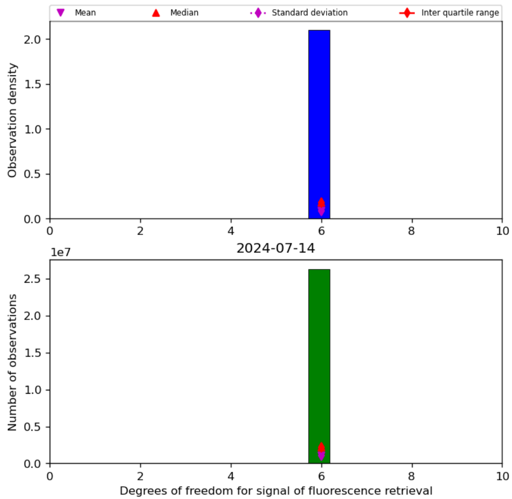
Figure 43: Histogram of “Degrees of freedom for signal of fluorescence retrieval” for 2024-07-13 to 2024-07-15
