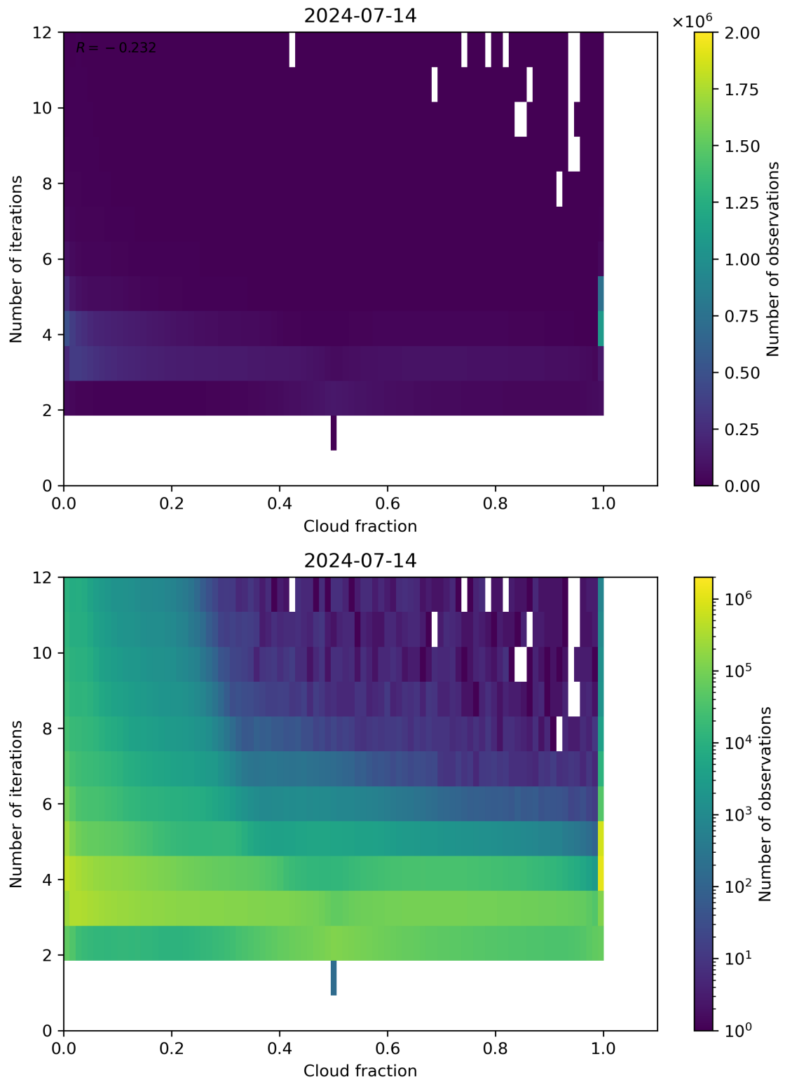
Figure 73: Scatter density plot of “Cloud fraction” against “Number of iterations” for 2024-07-13 to 2024-07-15.
