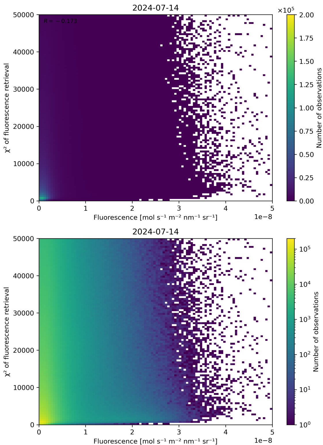
Figure 85: Scatter density plot of “Fluorescence” against “ \chi^2 of fluorescence retrieval” for 2024-07-13 to 2024-07-15.
