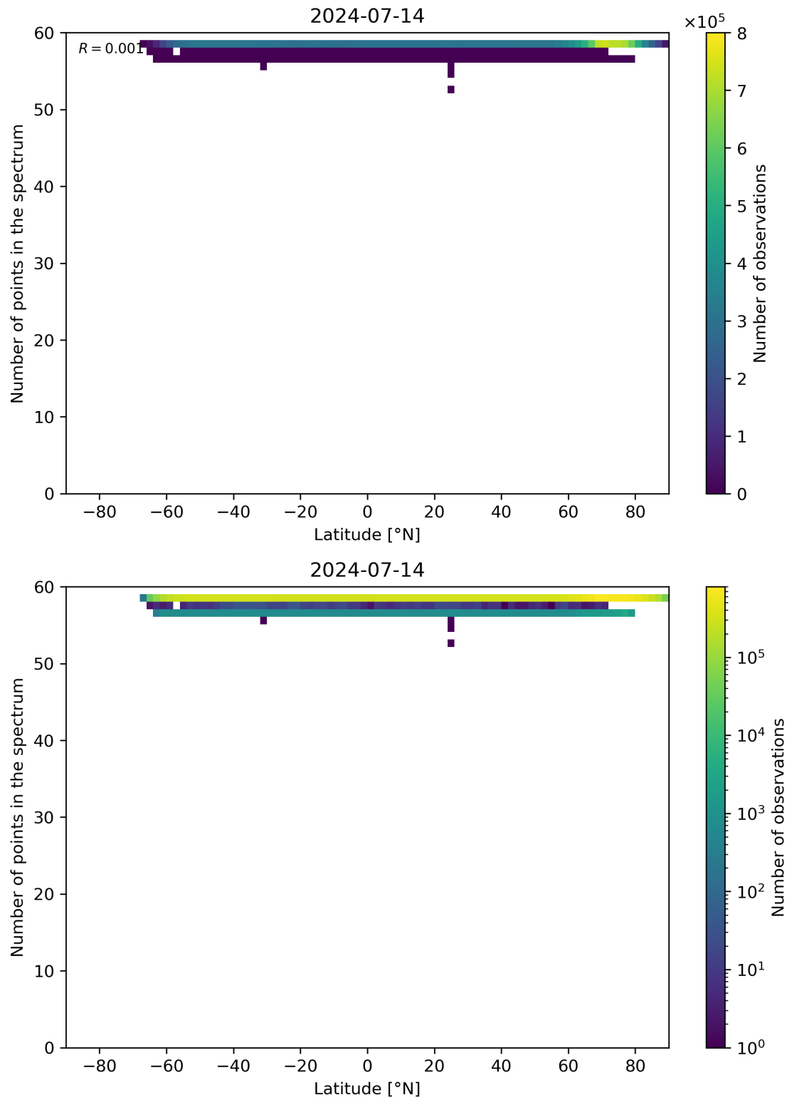
Figure 94: Scatter density plot of “Latitude” against “Number of points in the spectrum” for 2024-07-13 to 2024-07-15.
