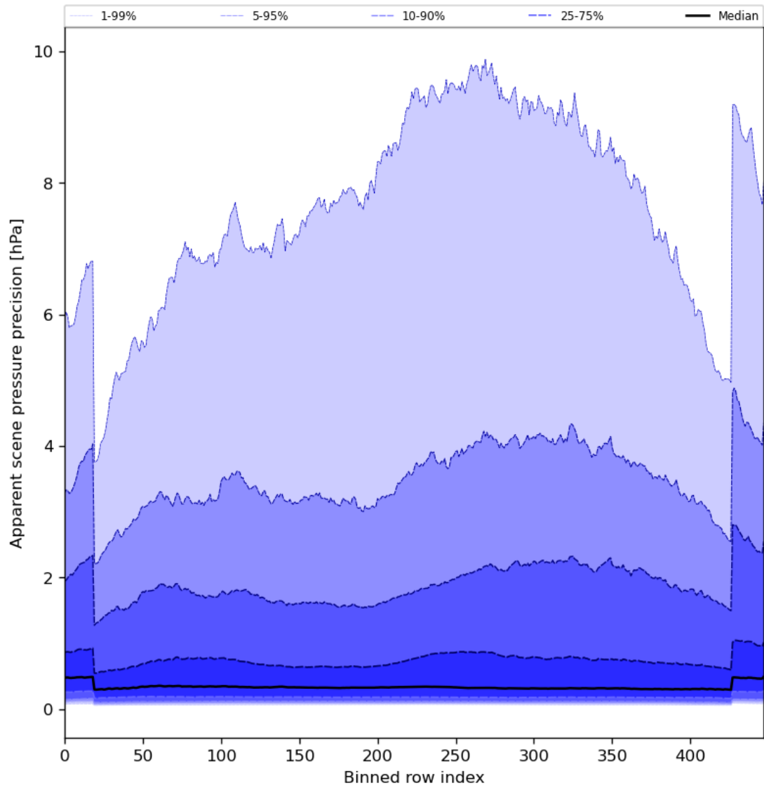
Figure 54: Along track statistics of “Apparent scene pressure precision” for 2024-07-13 to 2024-07-15
