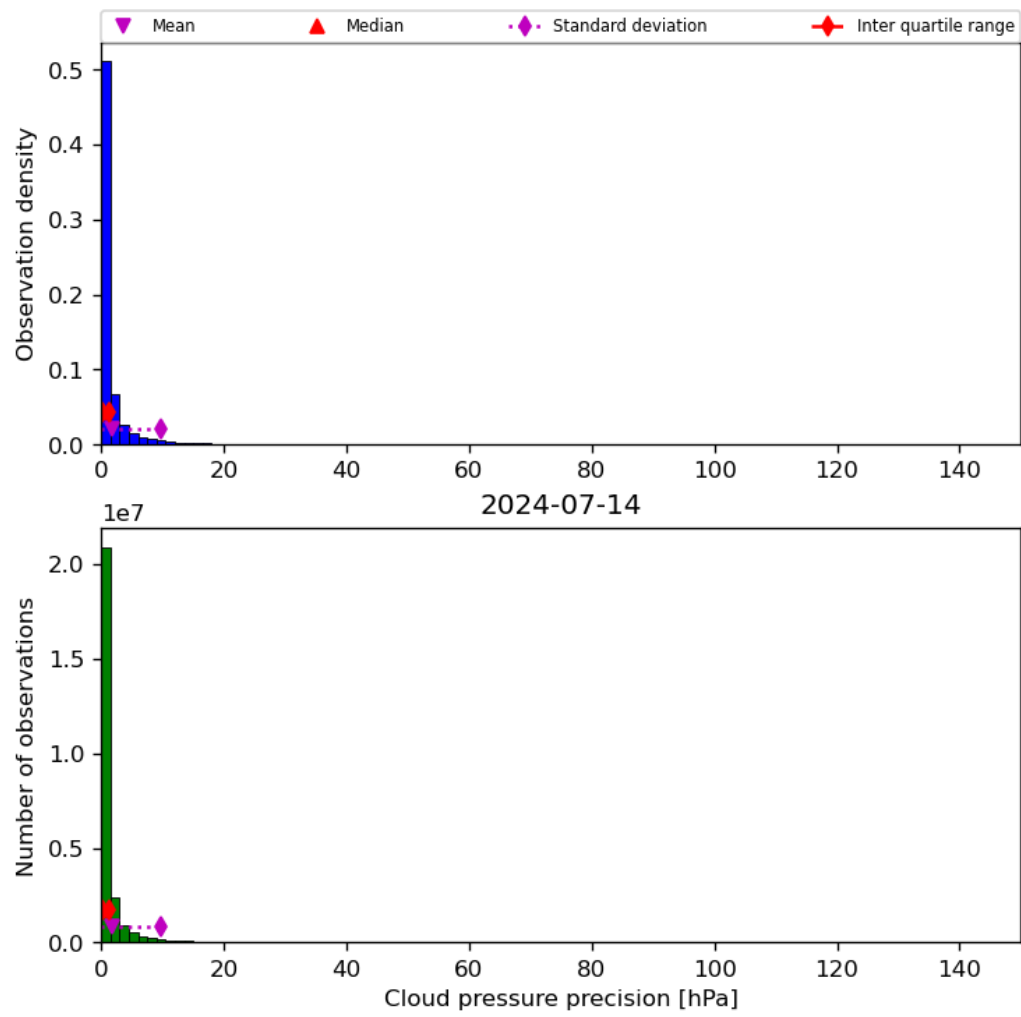
Figure 31: Histogram of “Cloud pressure precision” for 2024-07-13 to 2024-07-15
