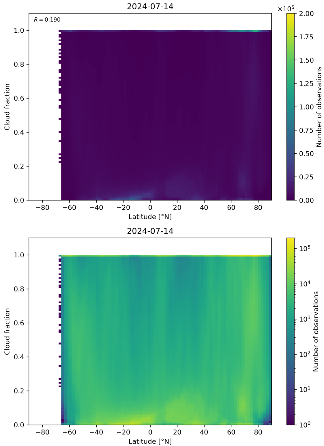
Figure 90: Scatter density plot of “Latitude” against “Cloud fraction” for 2024-07-13 to 2024-07-15.
