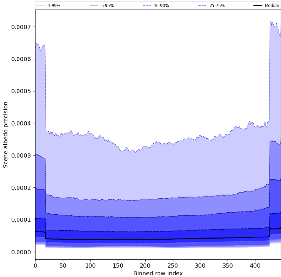
Figure 52: Along track statistics of “Scene albedo precision” for 2024-07-13 to 2024-07-15
