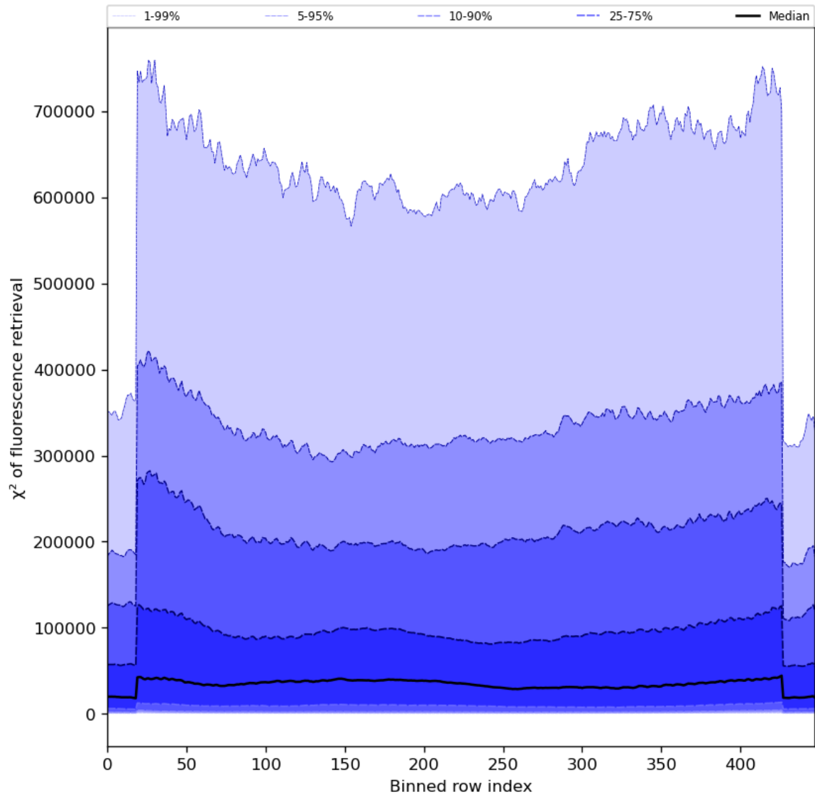
Figure 59: Along track statistics of “ \chi^2 of fluorescence retrieval” for 2024-07-13 to 2024-07-15
