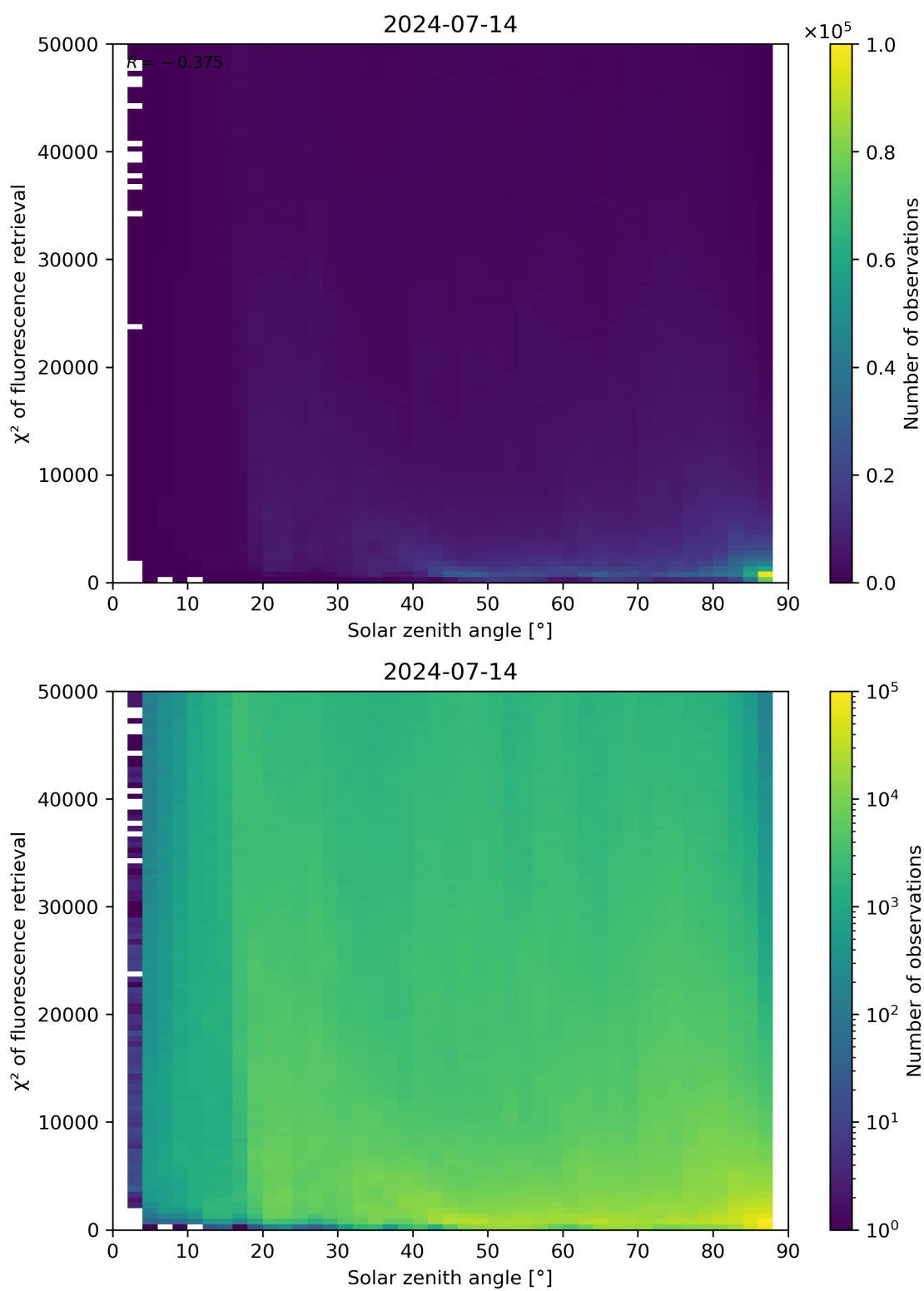
Figure 109: Scatter density plot of “Solar zenith angle” against “ \chi^2 of fluorescence retrieval” for 2024-07-13 to 2024-07-15.
