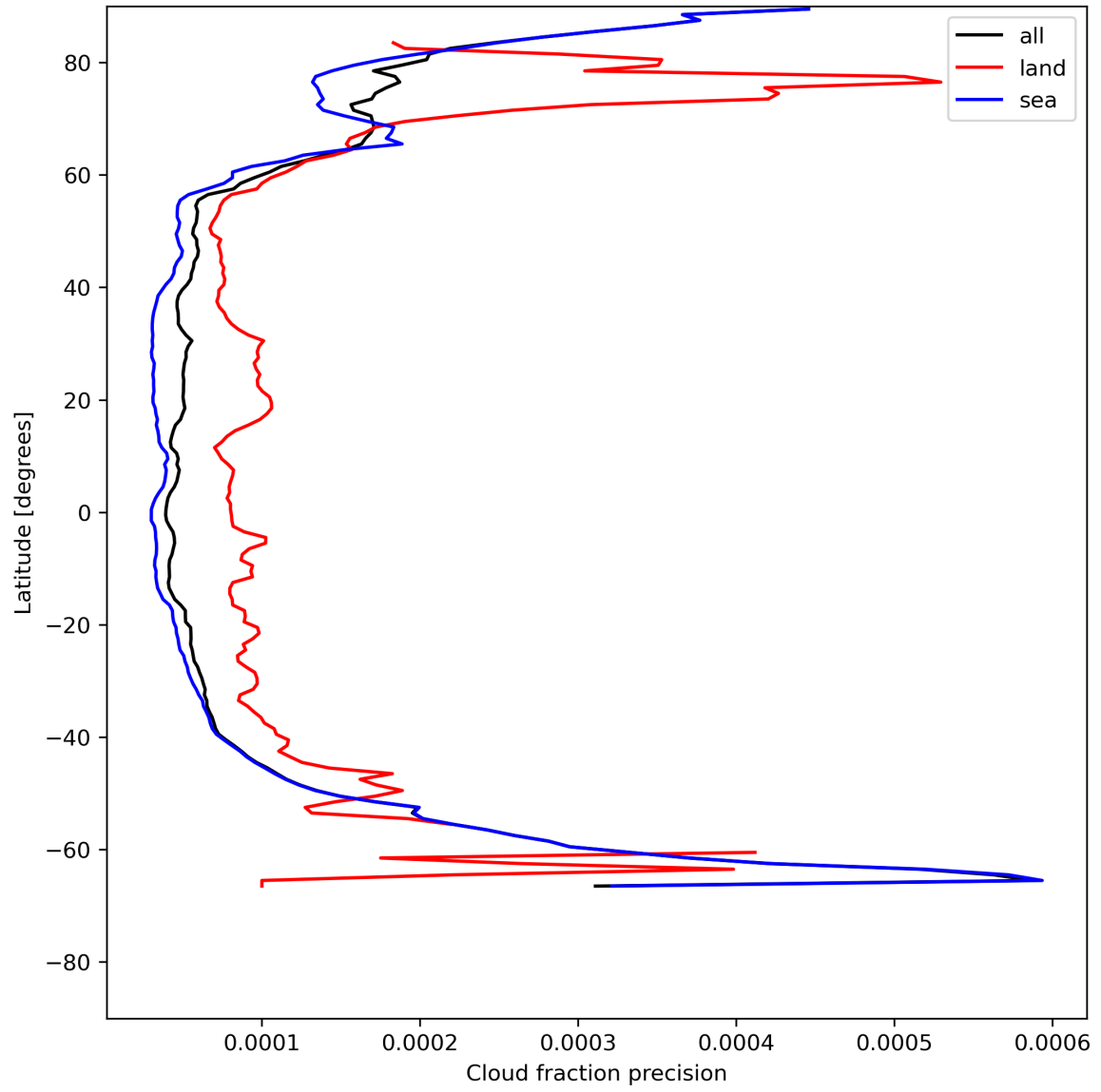
Figure 16: Zonal average of “Cloud fraction precision” for 2024-07-13 to 2024-07-15.
