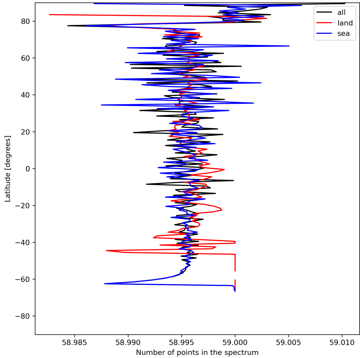
Figure 27: Zonal average of “Number of points in the spectrum” for 2024-07-13 to 2024-07-15.
