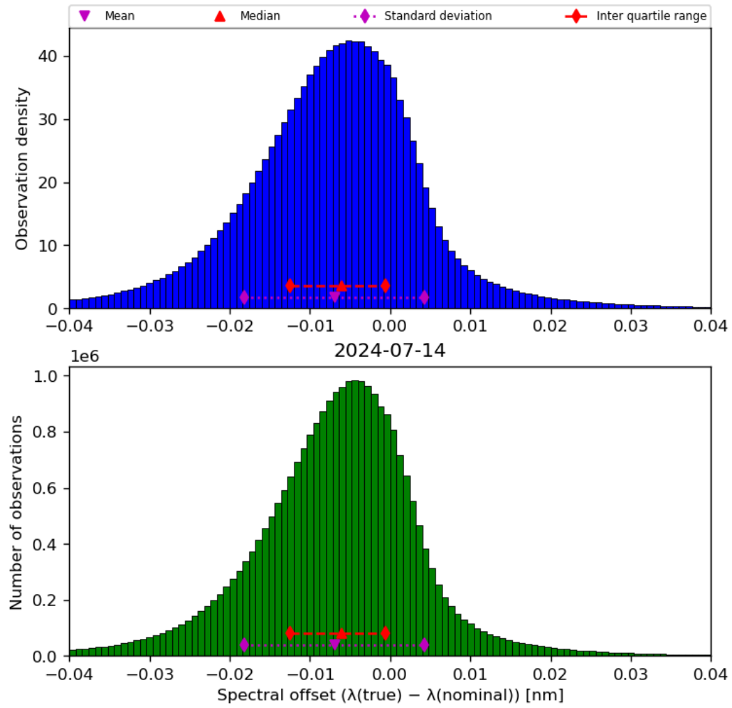
Figure 45: Histogram of “Spectral offset ( \lambda(\text{true}) - \lambda(\text{nominal}) )” for 2024-07-13 to 2024-07-15
