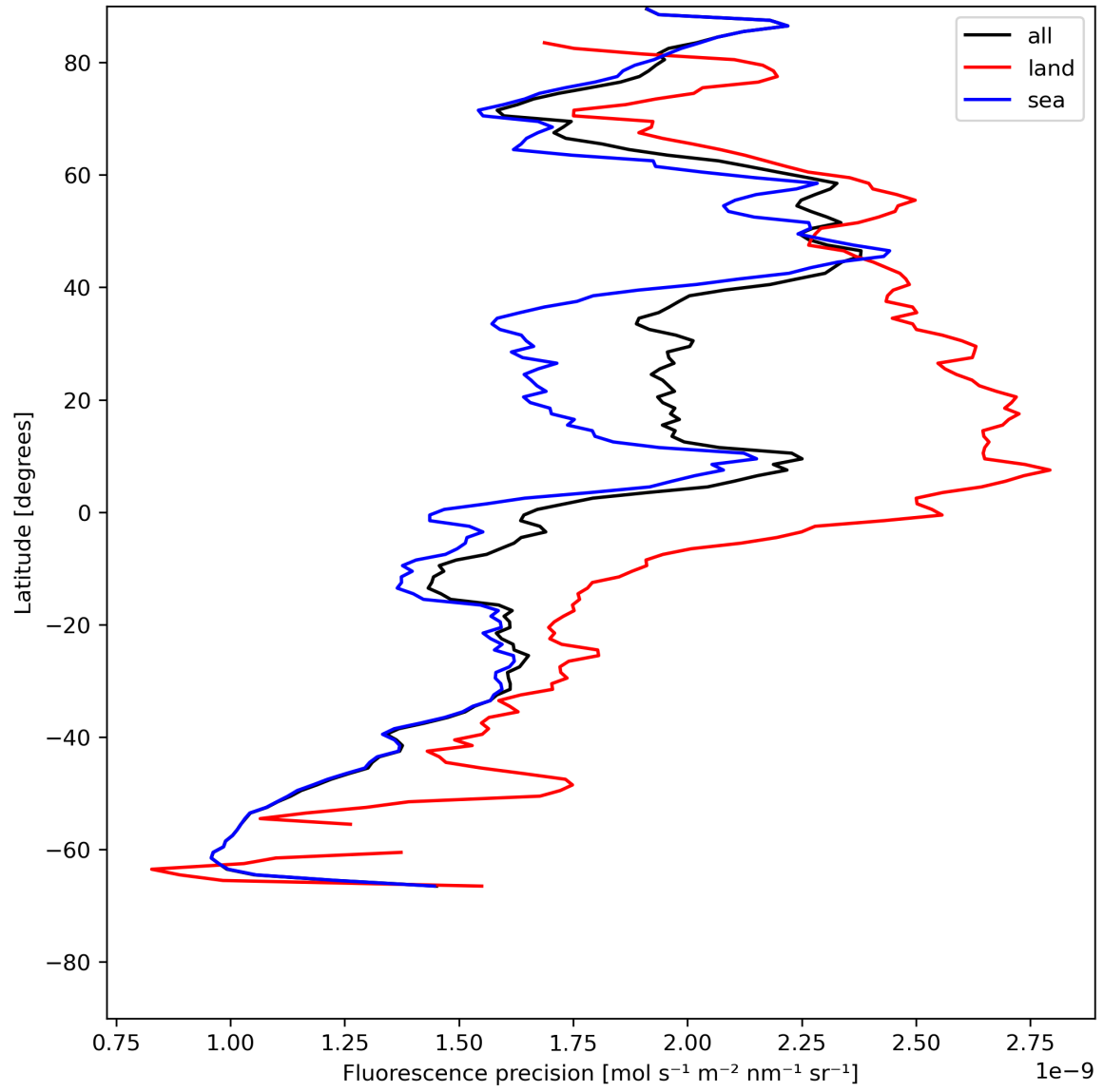
Figure 24: Zonal average of “Fluorescence precision” for 2024-07-13 to 2024-07-15.
