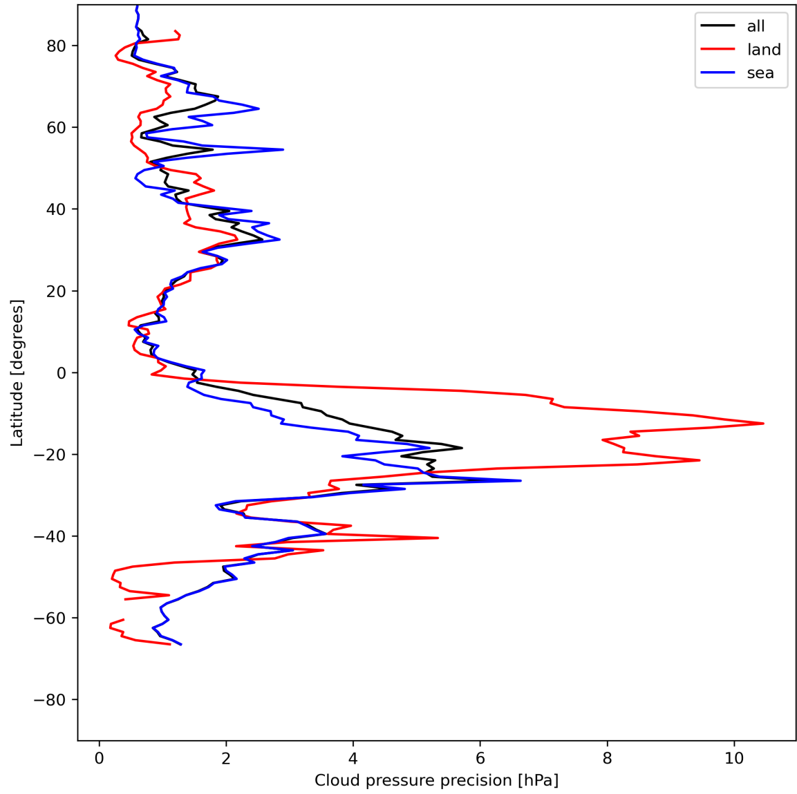
Figure 14: Zonal average of “Cloud pressure precision” for 2024-07-13 to 2024-07-15.
