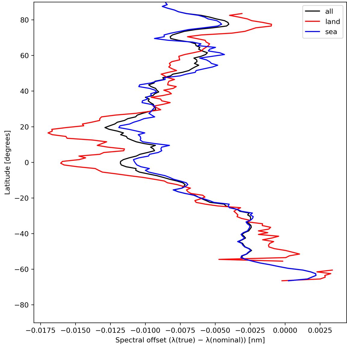
Figure 28: Zonal average of “Spectral offset ( \lambda(\text{true}) - \lambda(\text{nominal}) )” for 2024-07-13 to 2024-07-15.
