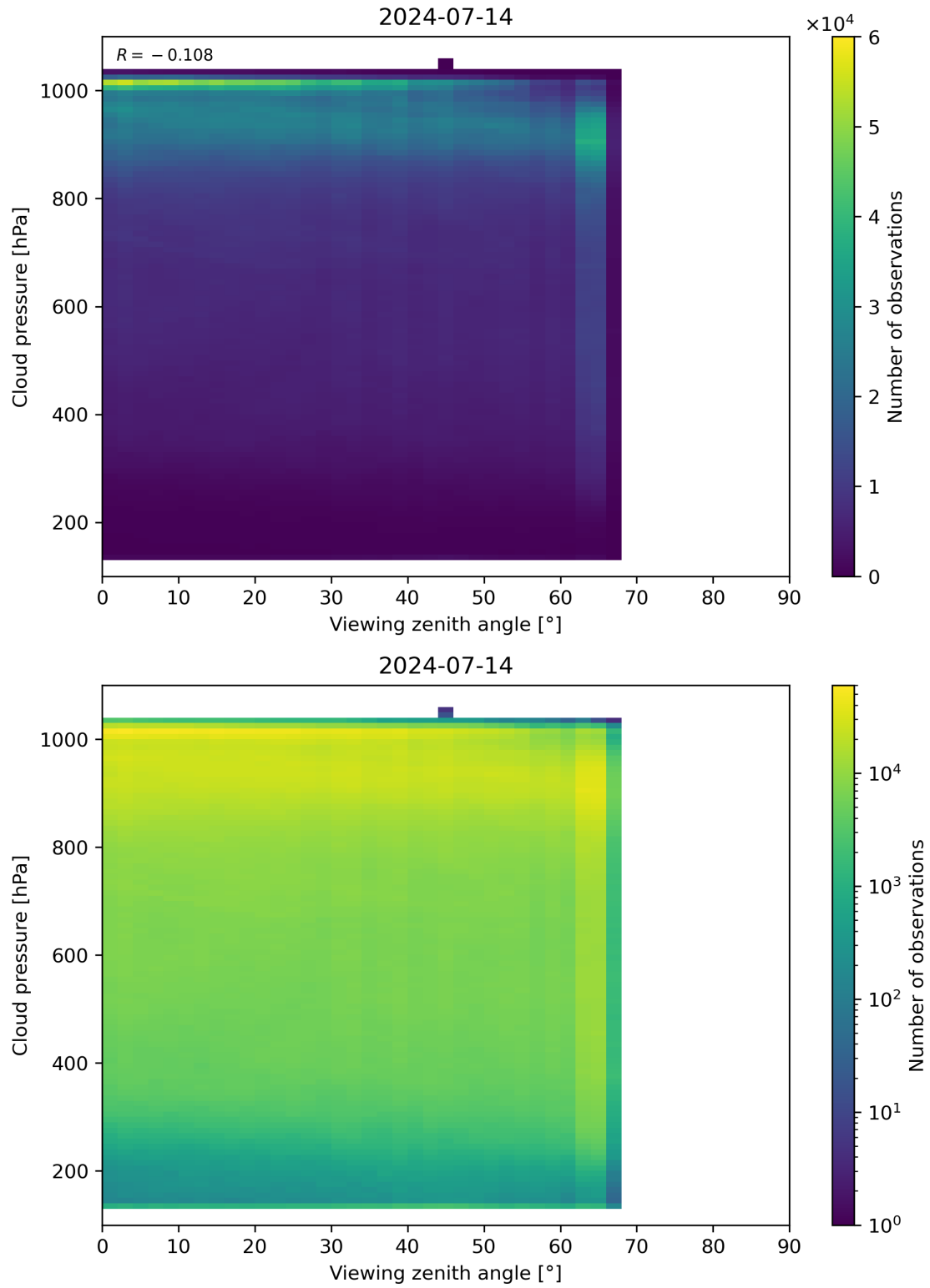
Figure 121: Scatter density plot of “Viewing zenith angle” against “Cloud pressure” for 2024-07-13 to 2024-07-15.
