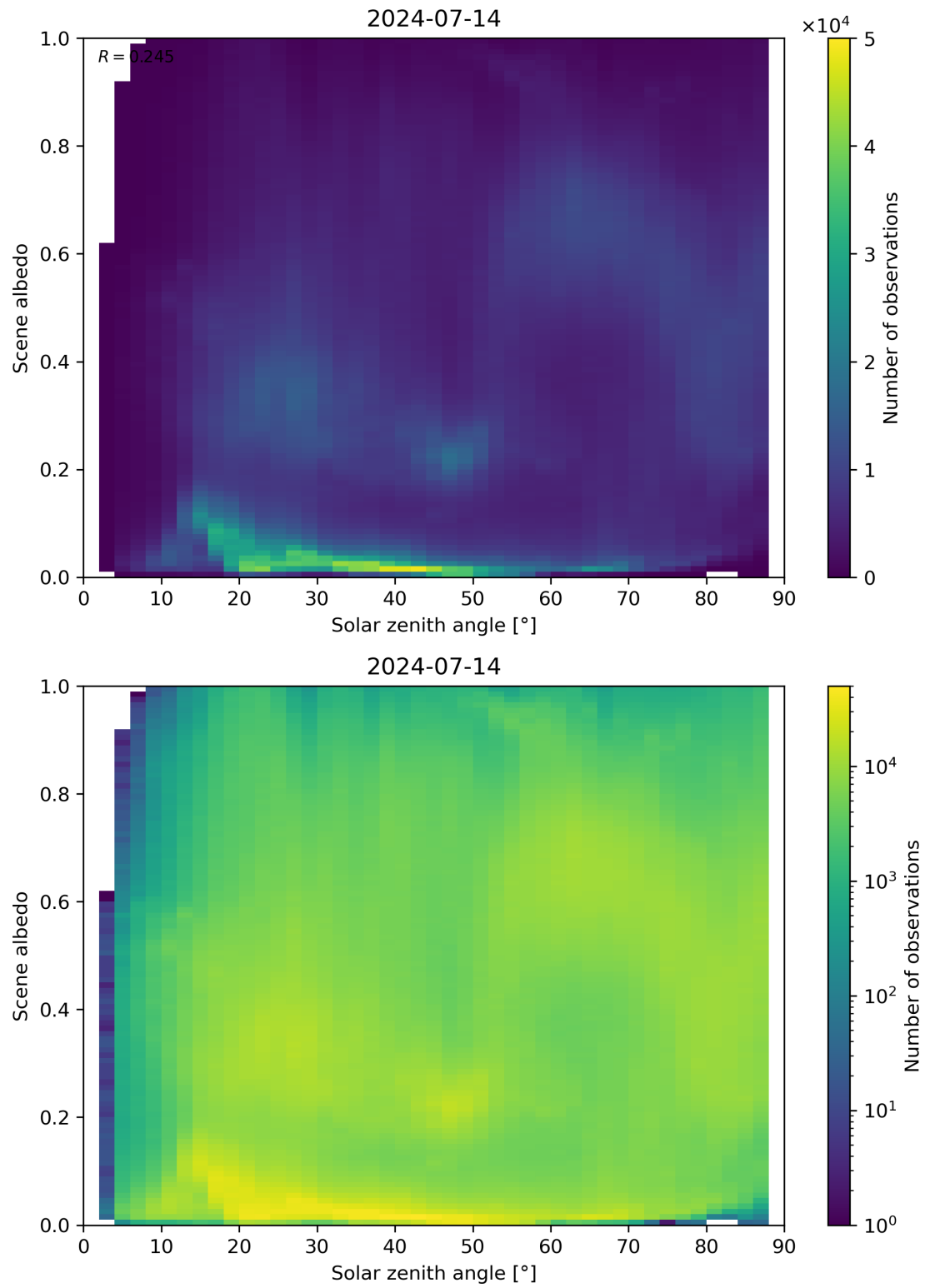
Figure 116: Scatter density plot of “Solar zenith angle” against “Scene albedo” for 2024-07-13 to 2024-07-15.
