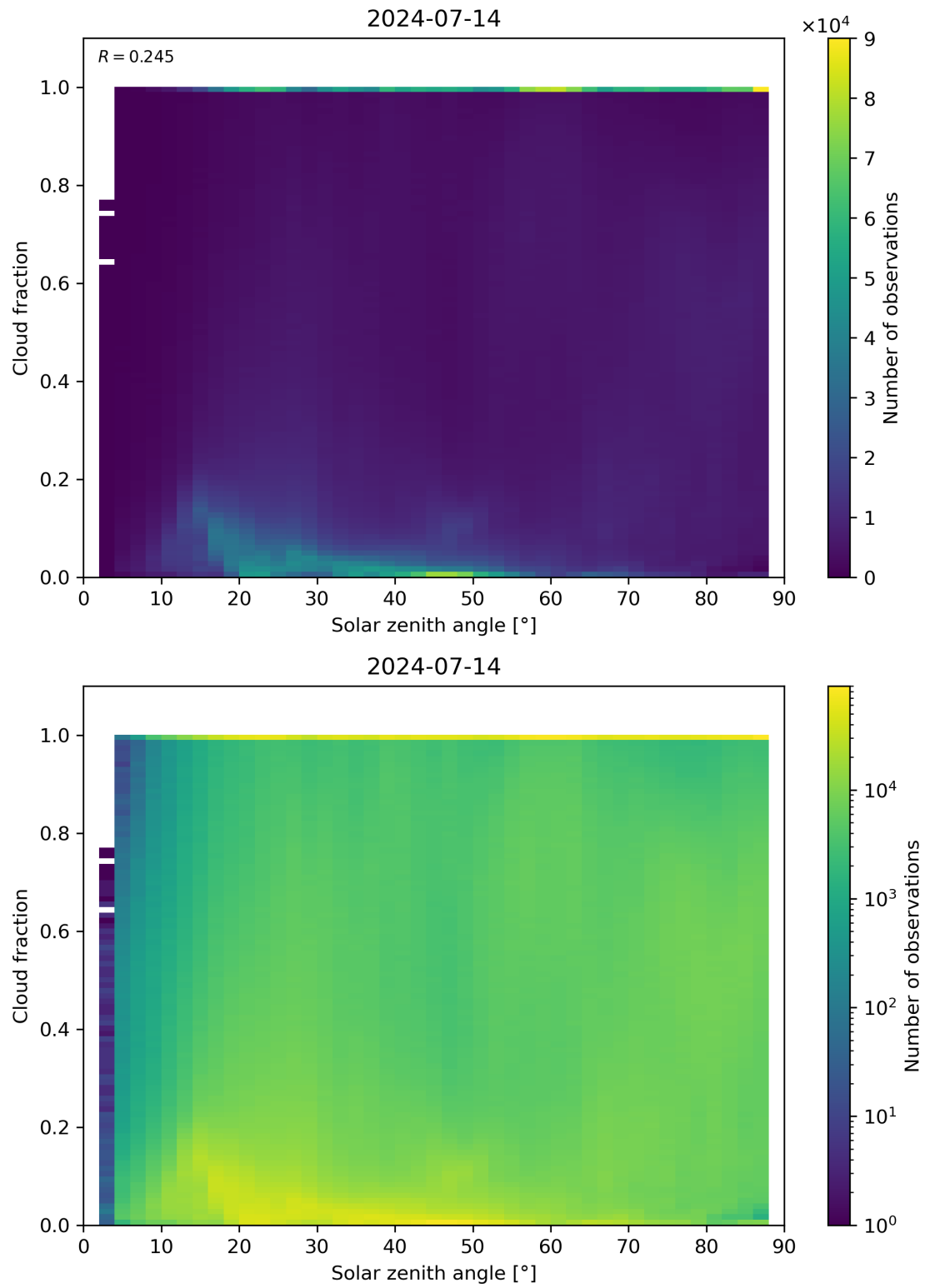
Figure 110: Scatter density plot of “Solar zenith angle” against “Cloud fraction” for 2024-07-13 to 2024-07-15.
