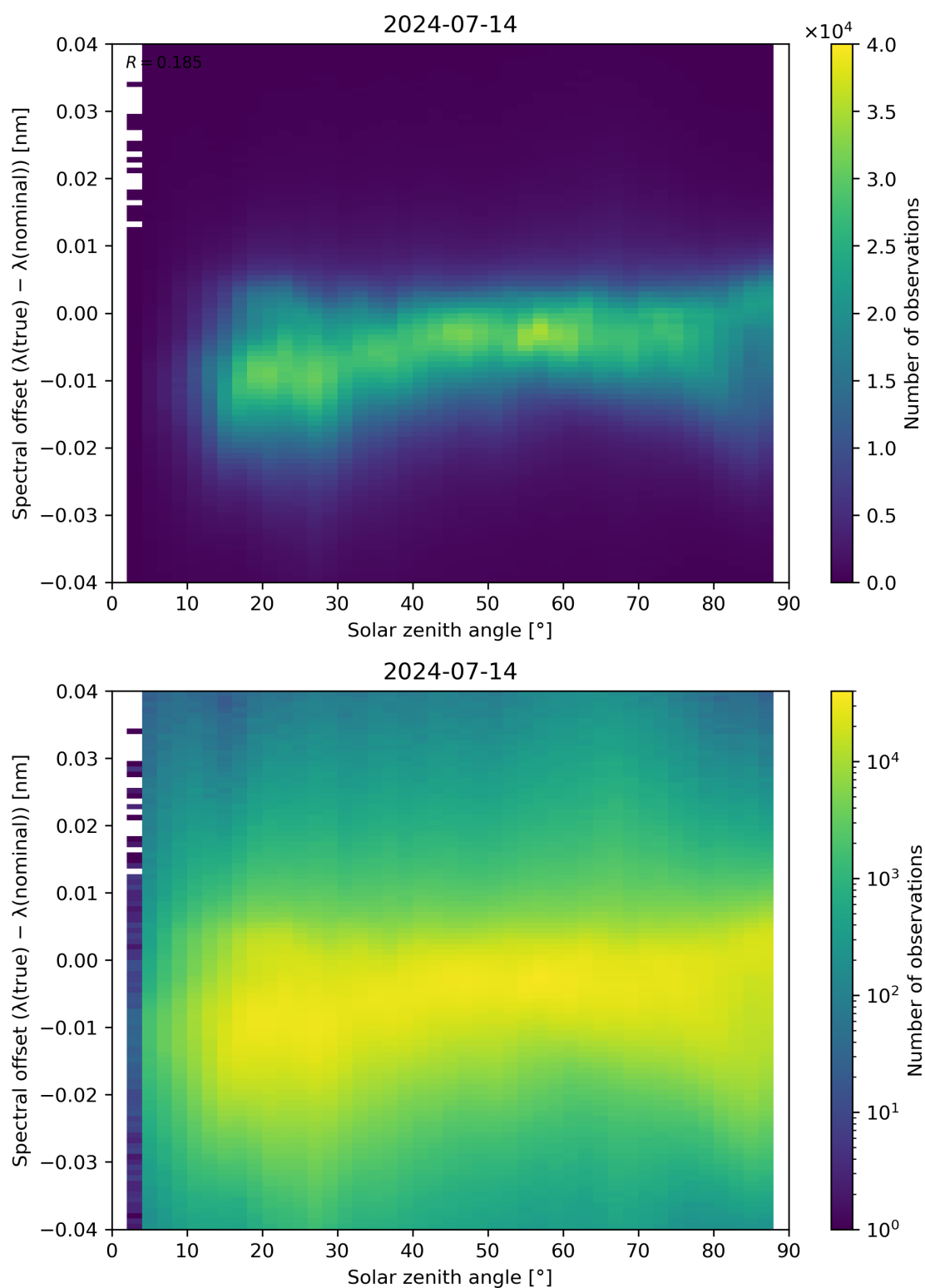
Figure 117: Scatter density plot of “Solar zenith angle” against “Spectral offset ( \lambda(\text{true}) - \lambda(\text{nominal}) )” for 2024-07-13 to 2024-07-15.
