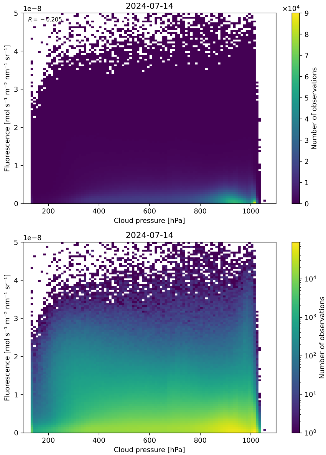
Figure 80: Scatter density plot of “Cloud pressure” against “Fluorescence” for 2024-07-13 to 2024-07-15.
