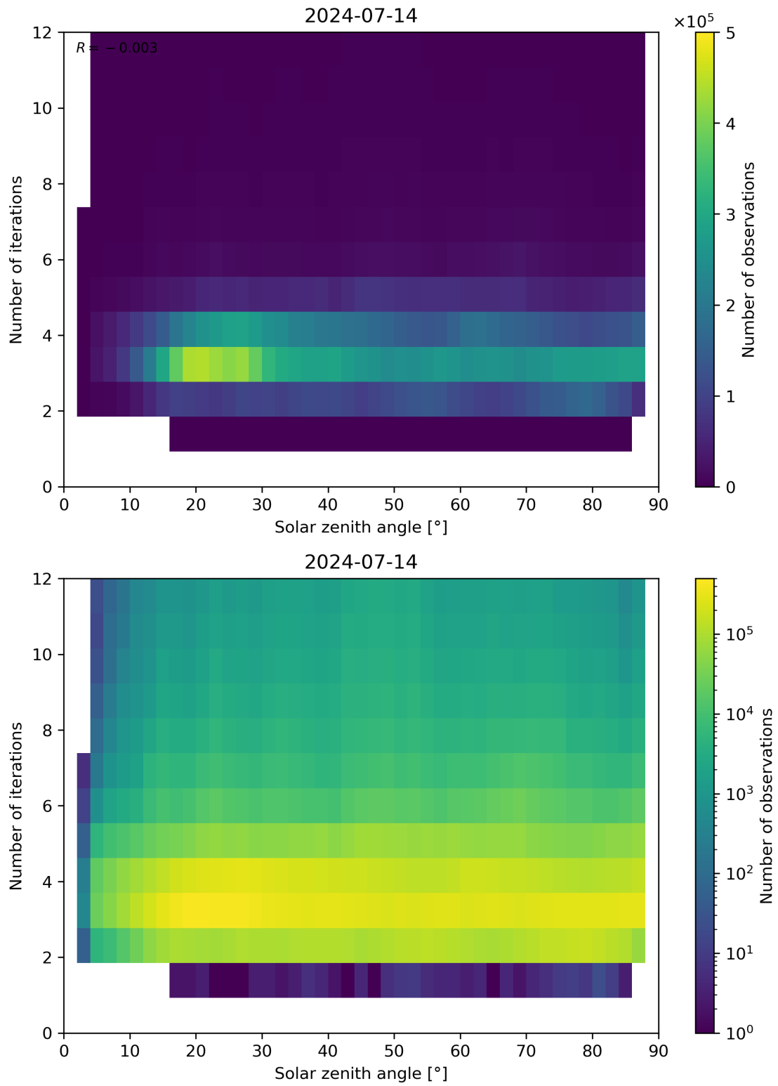
Figure 114: Scatter density plot of “Solar zenith angle” against “Number of iterations” for 2024-07-13 to 2024-07-15.
