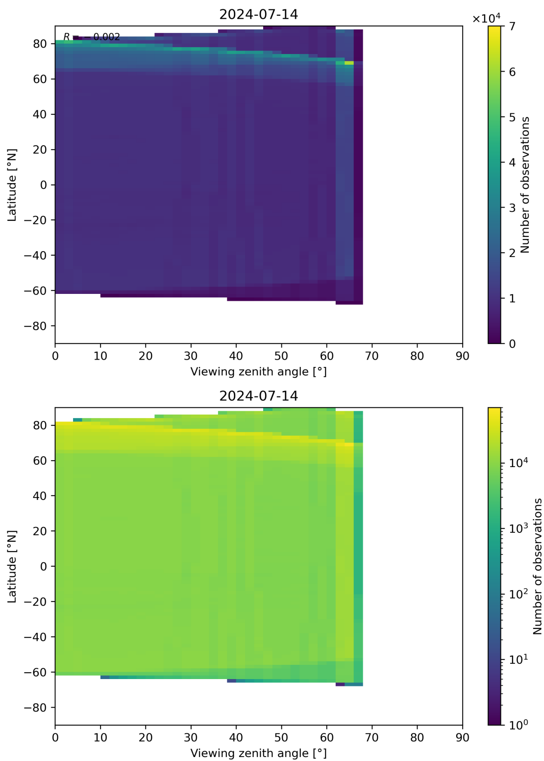
Figure 123: Scatter density plot of “Viewing zenith angle” against “Latitude” for 2024-07-13 to 2024-07-15.
