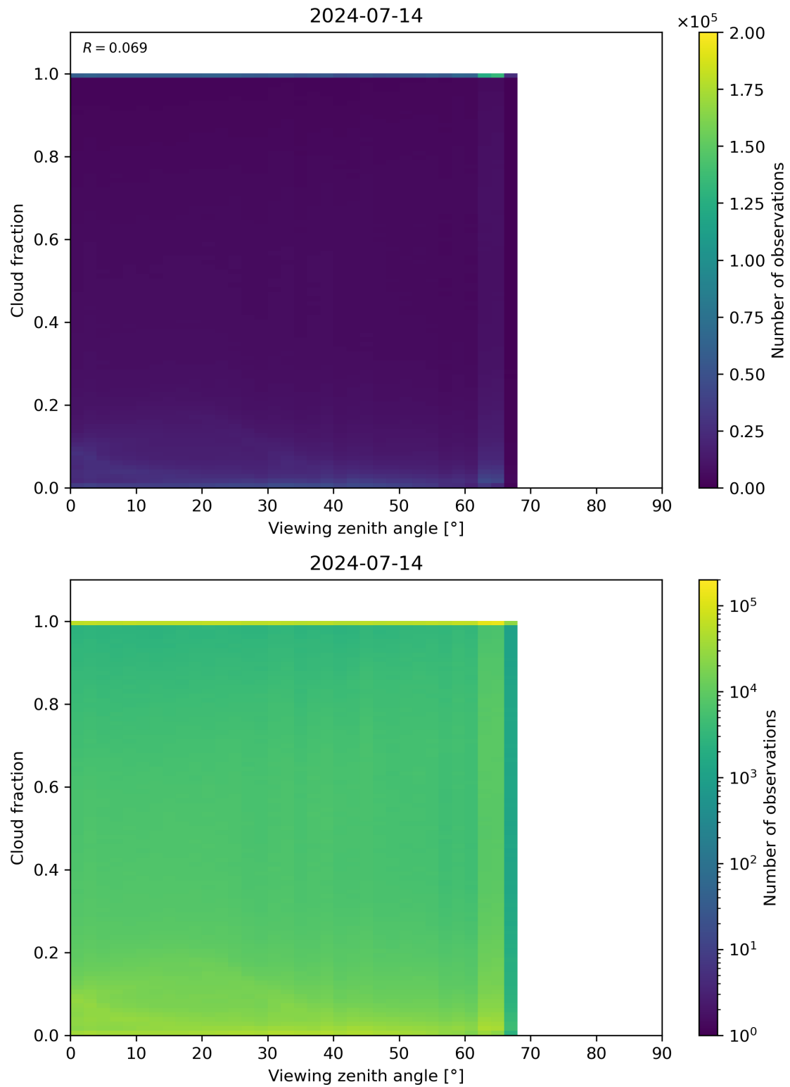
Figure 120: Scatter density plot of “Viewing zenith angle” against “Cloud fraction” for 2024-07-13 to 2024-07-15.
