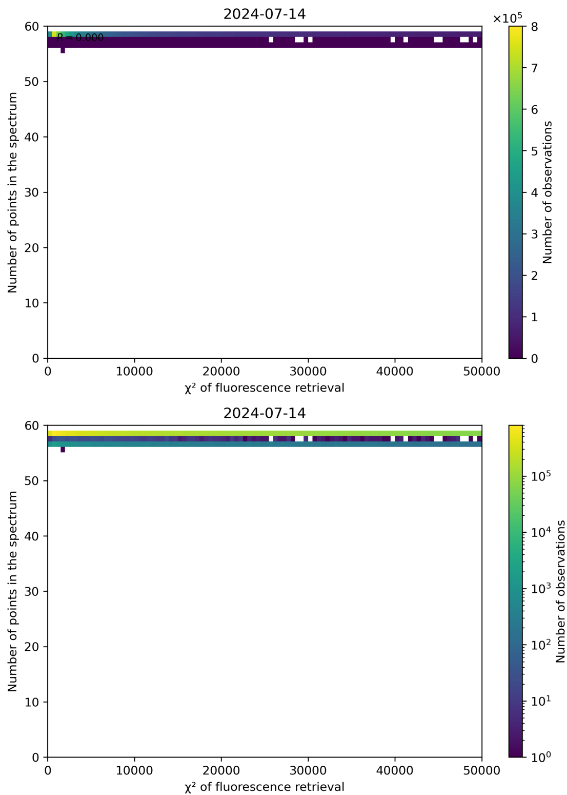
Figure 68: Scatter density plot of " \chi^2 of fluorescence retrieval" against "Number of points in the spectrum" for 2024-07-13 to 2024-07-15.
