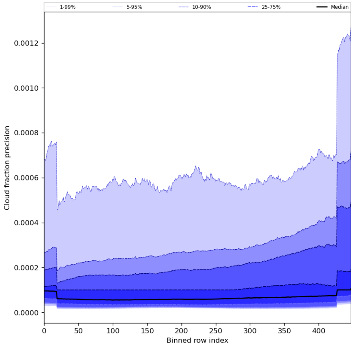
Figure 50: Along track statistics of “Cloud fraction precision” for 2024-07-13 to 2024-07-15
