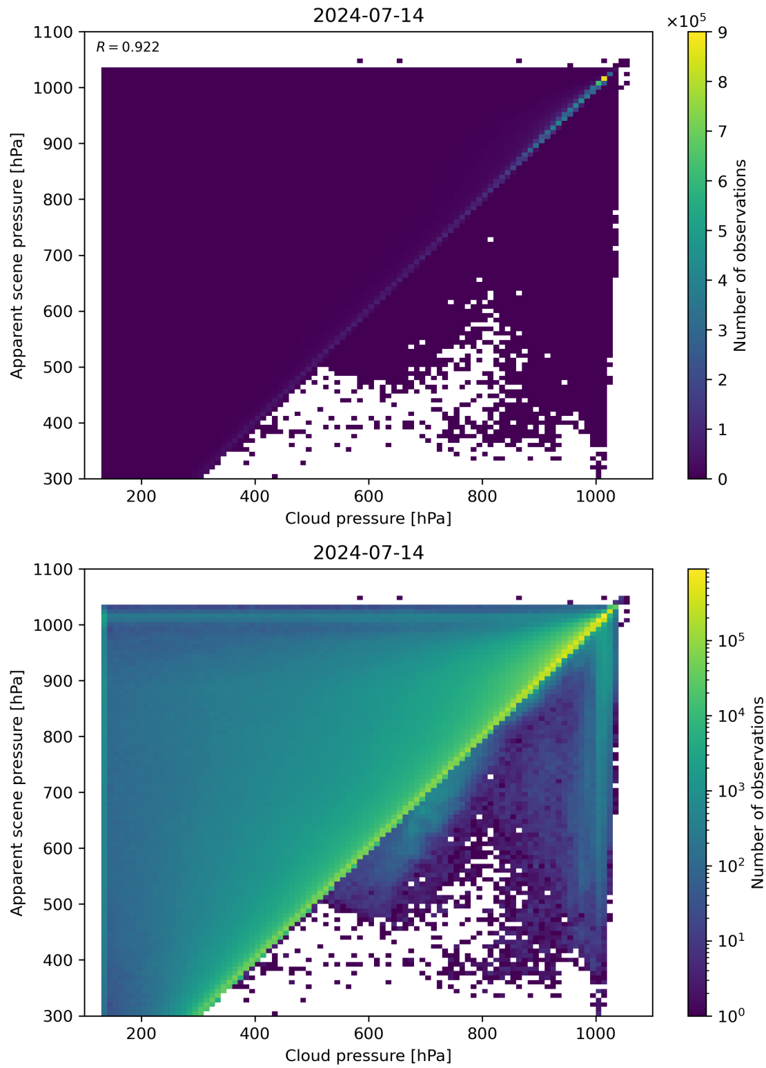
Figure 77: Scatter density plot of “Cloud pressure” against “Apparent scene pressure” for 2024-07-13 to 2024-07-15.
