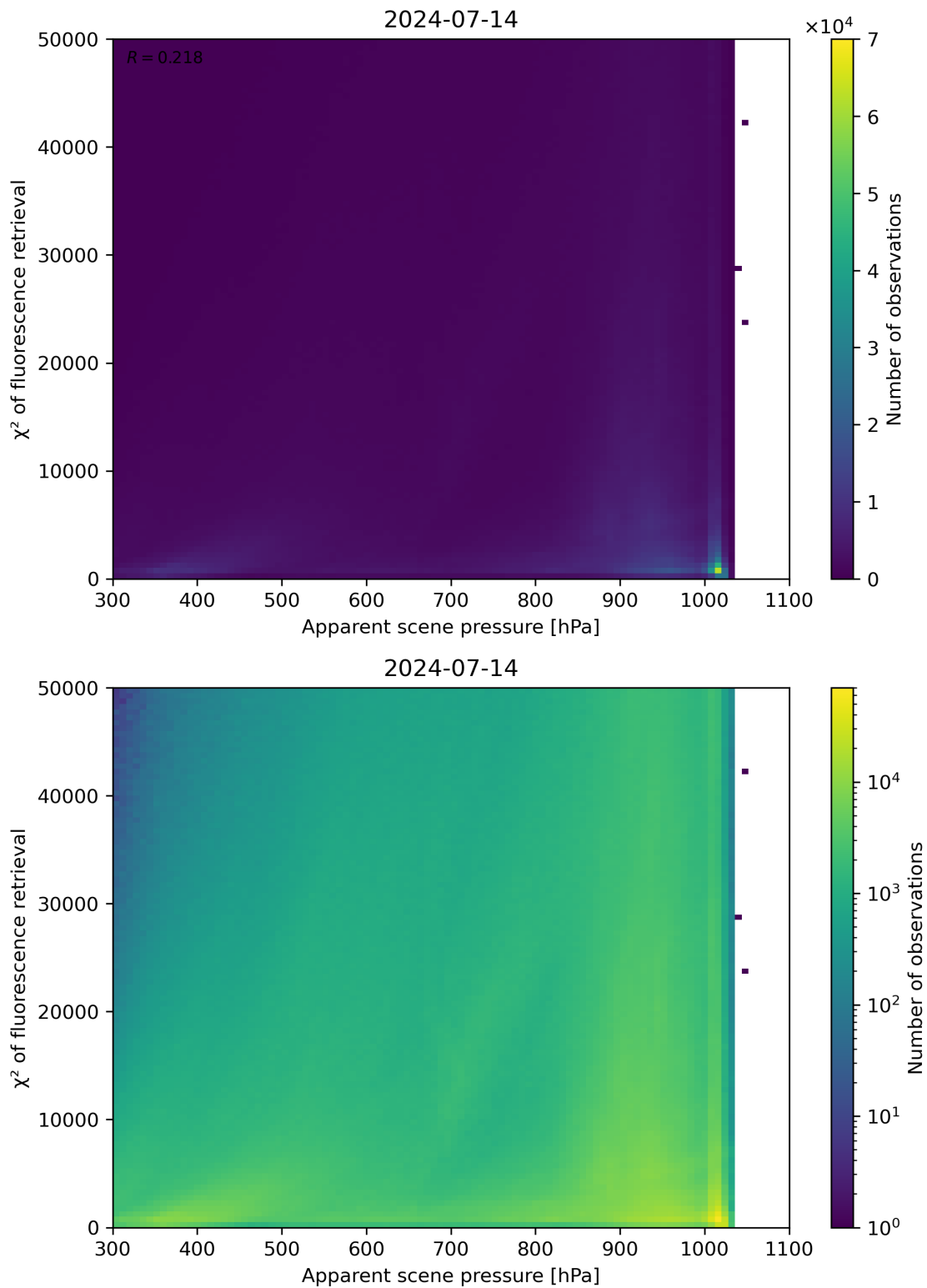
Figure 63: Scatter density plot of “Apparent scene pressure” against “ \chi^2 of fluorescence retrieval” for 2024-07-13 to 2024-07-15.
