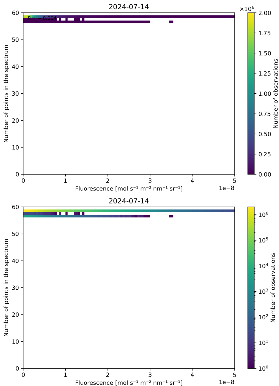
Figure 86: Scatter density plot of “Fluorescence” against “Number of points in the spectrum” for 2024-07-13 to 2024-07-15.
