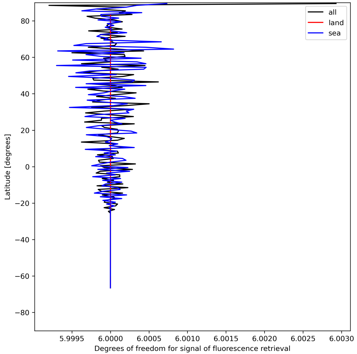
Figure 26: Zonal average of “Degrees of freedom for signal of fluorescence retrieval” for 2024-07-13 to 2024-07-15.
