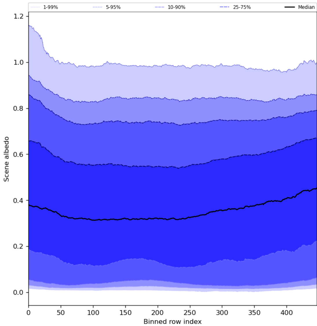
Figure 51: Along track statistics of “Scene albedo” for 2024-07-13 to 2024-07-15
