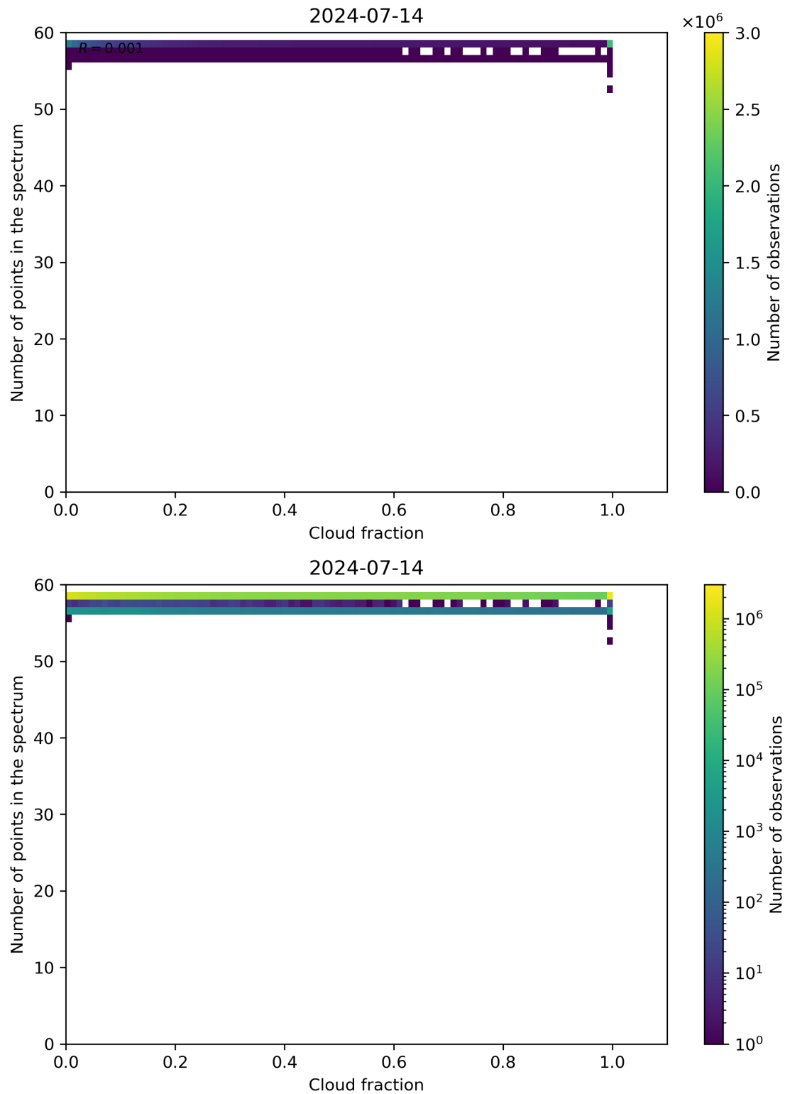
Figure 74: Scatter density plot of “Cloud fraction” against “Number of points in the spectrum” for 2024-07-13 to 2024-07-15.
