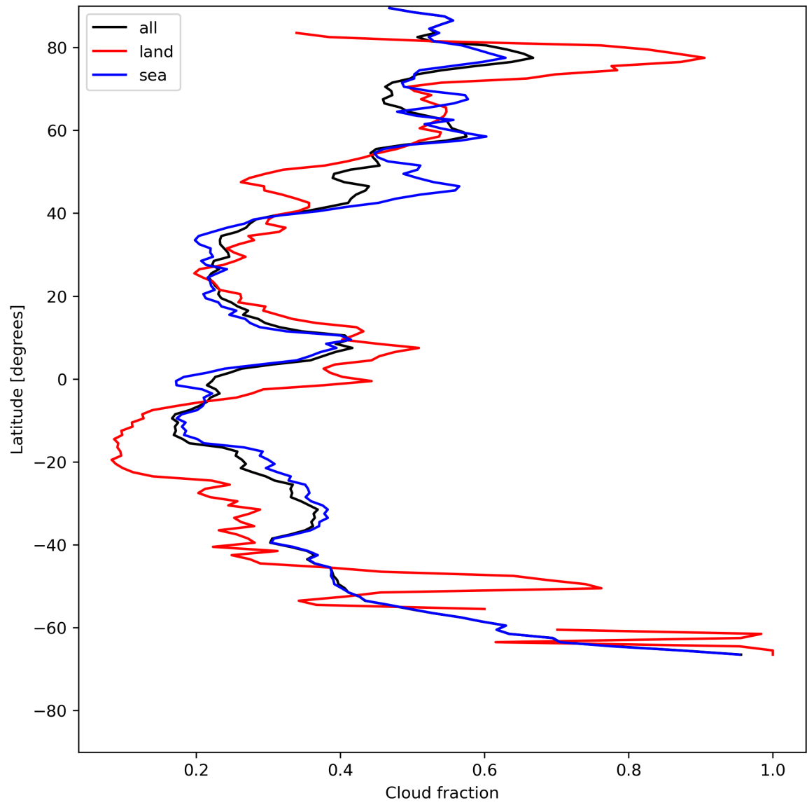
Figure 15: Zonal average of “Cloud fraction” for 2024-07-13 to 2024-07-15.
