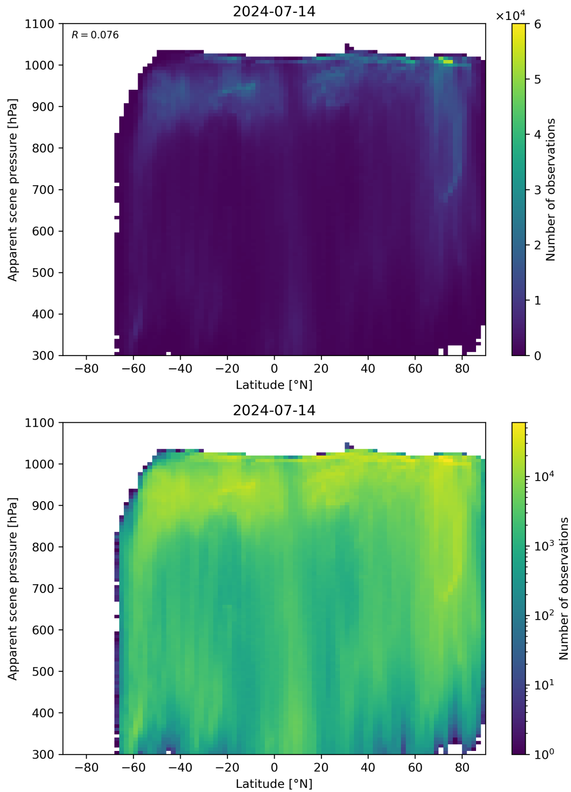
Figure 88: Scatter density plot of “Latitude” against “Apparent scene pressure” for 2024-07-13 to 2024-07-15.
