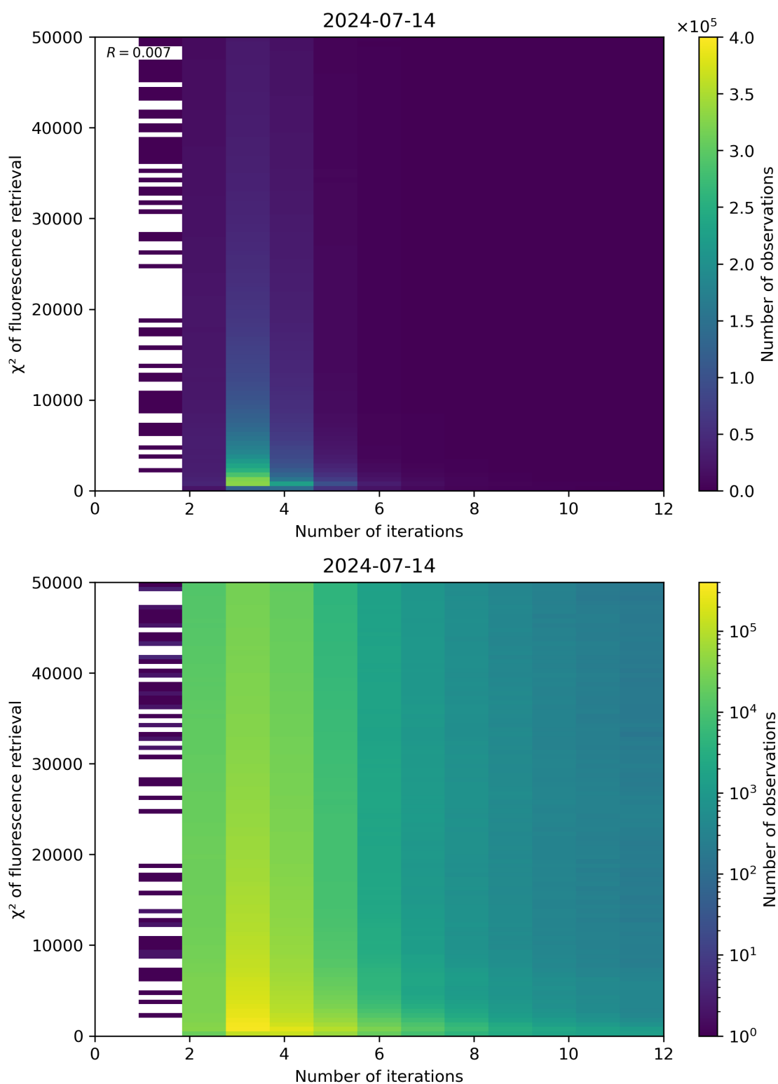
Figure 97: Scatter density plot of “Number of iterations” against “ \chi^2 of fluorescence retrieval” for 2024-07-13 to 2024-07-15.
