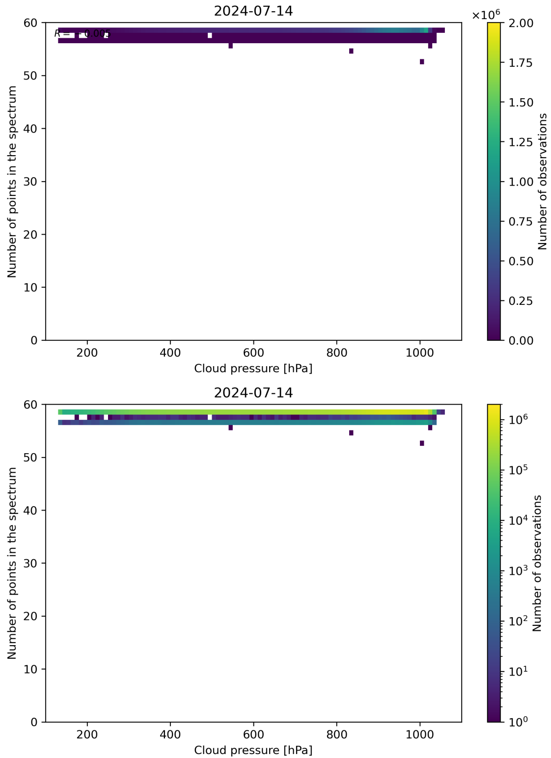
Figure 82: Scatter density plot of “Cloud pressure” against “Number of points in the spectrum” for 2024-07-13 to 2024-07-15.
