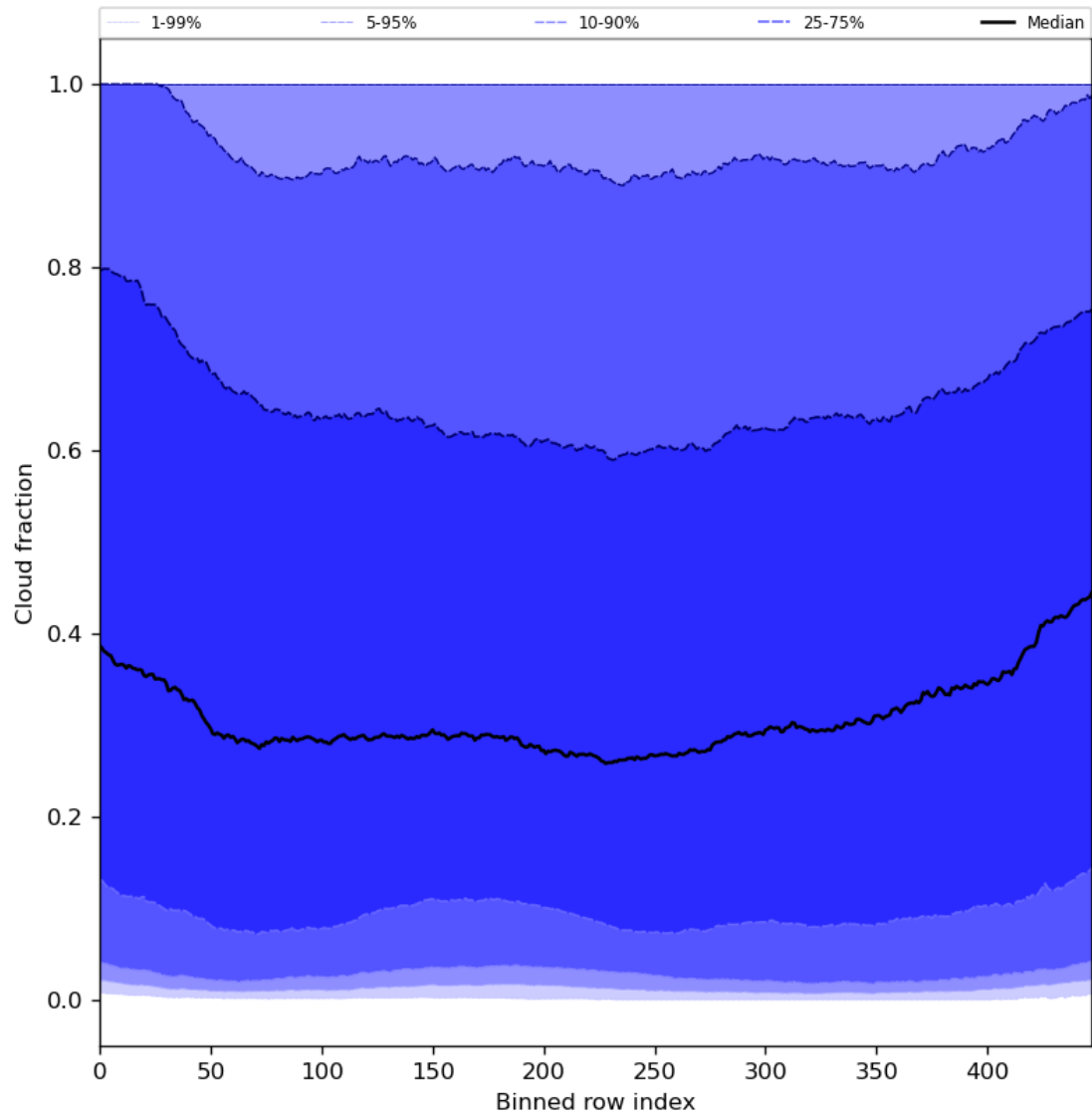
Figure 49: Along track statistics of “Cloud fraction” for 2024-07-13 to 2024-07-15
