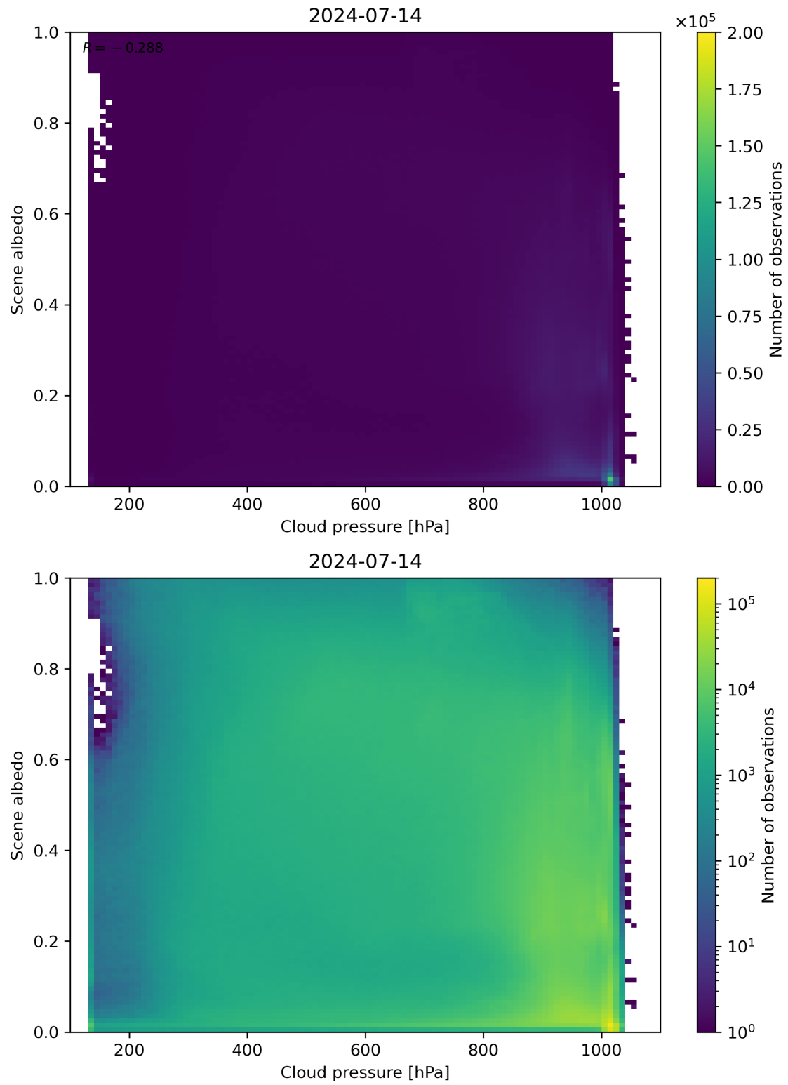
Figure 83: Scatter density plot of “Cloud pressure” against “Scene albedo” for 2024-07-13 to 2024-07-15.
