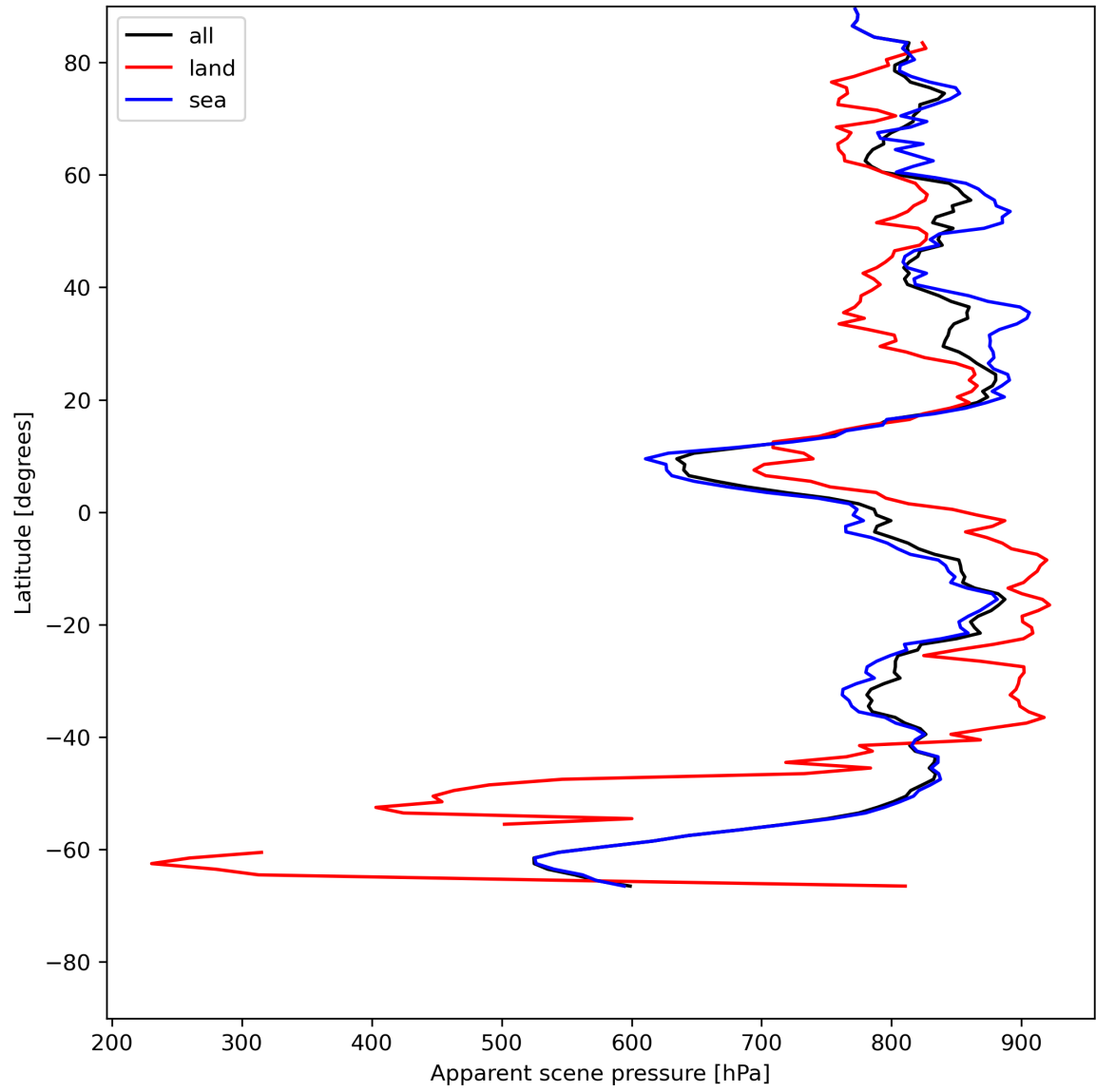
Figure 19: Zonal average of “Apparent scene pressure” for 2024-07-13 to 2024-07-15.
