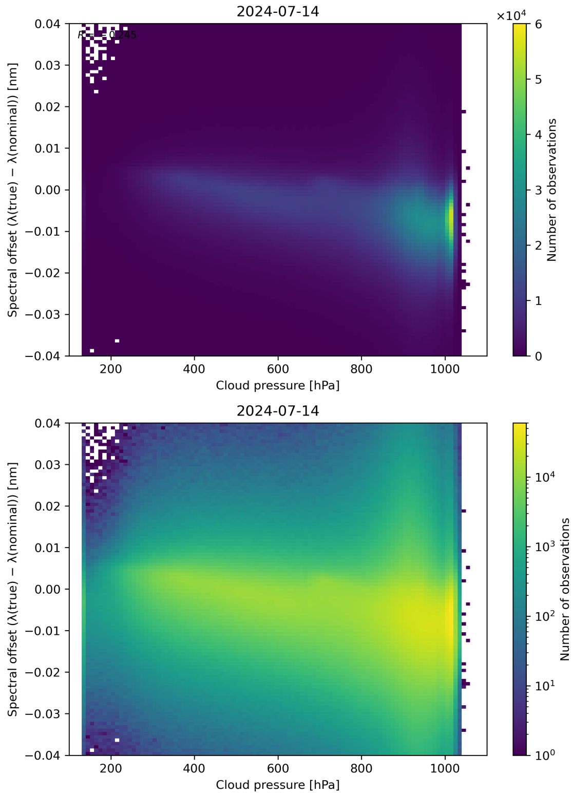
Figure 84: Scatter density plot of “Cloud pressure” against “Spectral offset ( \lambda(\text{true}) - \lambda(\text{nominal}) )” for 2024-07-13 to 2024-07-15.
