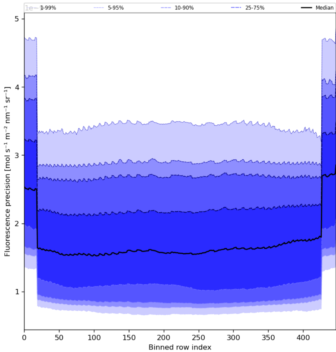
Figure 58: Along track statistics of “Fluorescence precision” for 2024-07-13 to 2024-07-15
