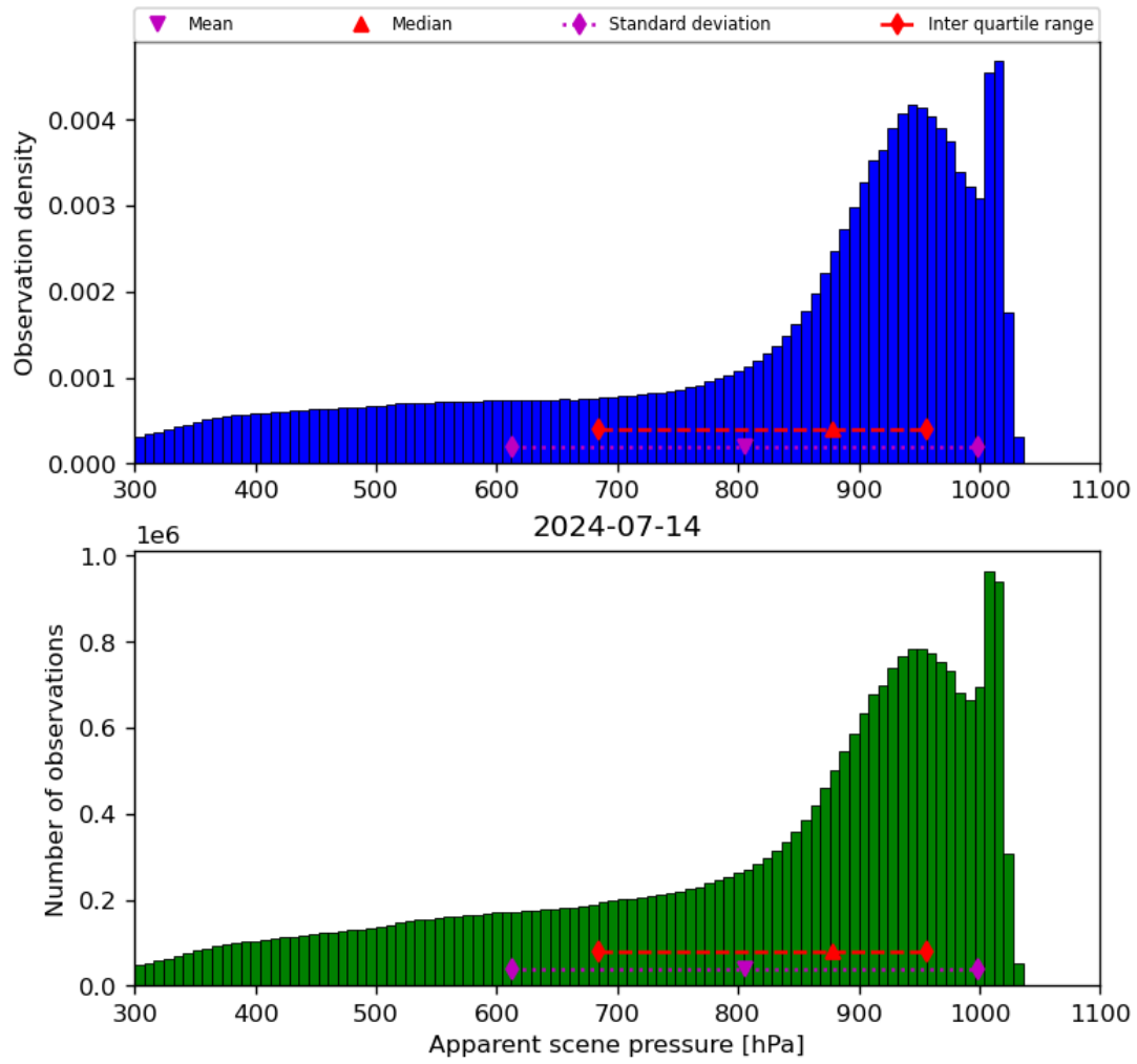
Figure 36: Histogram of “Apparent scene pressure” for 2024-07-13 to 2024-07-15
