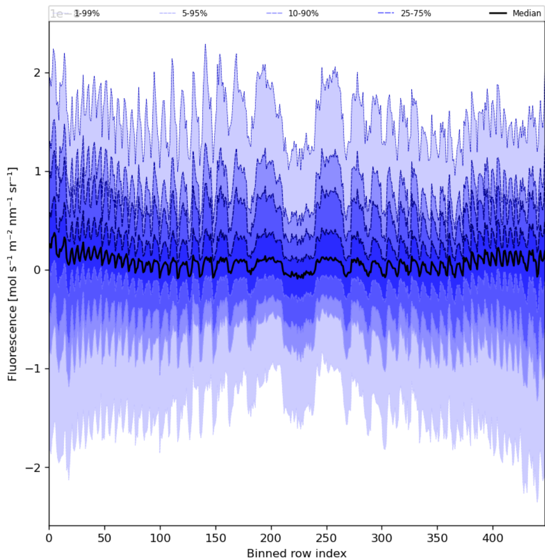
Figure 57: Along track statistics of “Fluorescence” for 2024-07-13 to 2024-07-15
