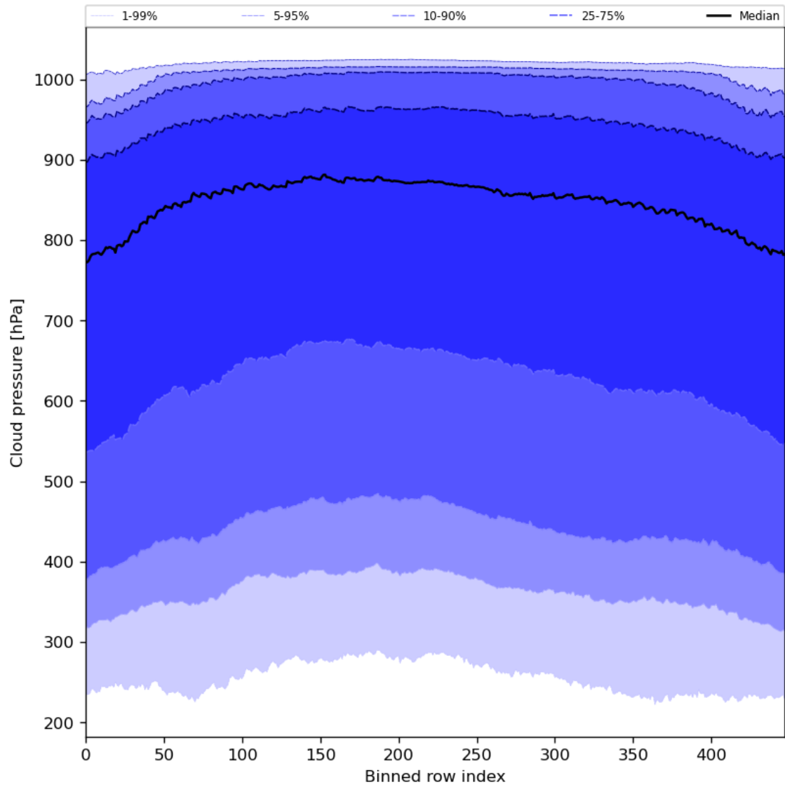
Figure 47: Along track statistics of “Cloud pressure” for 2024-07-13 to 2024-07-15
