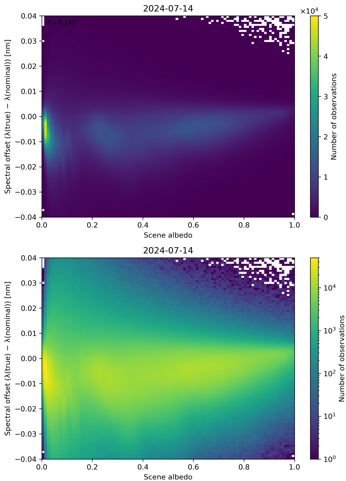
Figure 107: Scatter density plot of “Scene albedo” against “Spectral offset ( \lambda(\text{true}) - \lambda(\text{nominal}) )” for 2024-07-13 to 2024-07-15.
