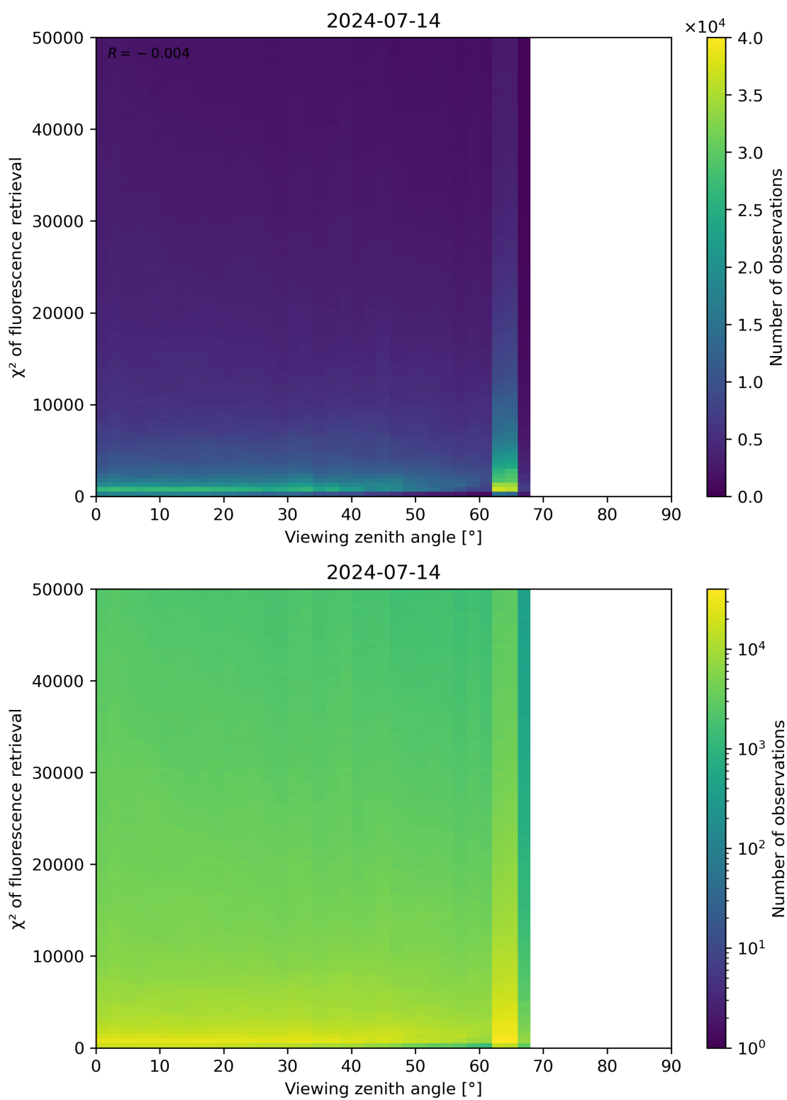
Figure 119: Scatter density plot of “Viewing zenith angle” against “ \chi^2 of fluorescence retrieval” for 2024-07-13 to 2024-07-15.
