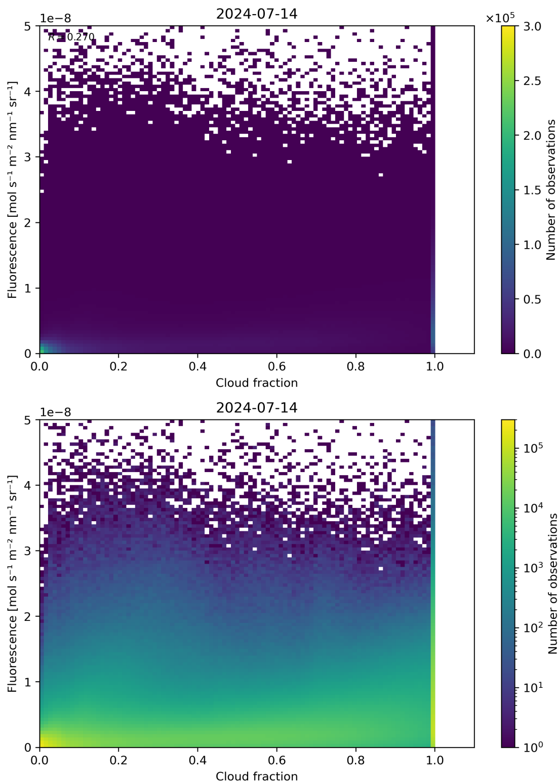
Figure 72: Scatter density plot of “Cloud fraction” against “Fluorescence” for 2024-07-13 to 2024-07-15.
