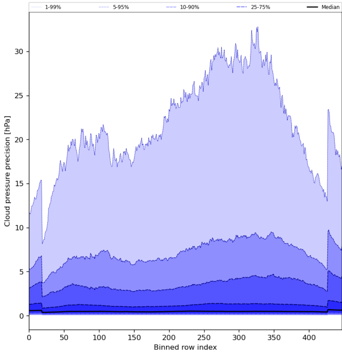
Figure 48: Along track statistics of “Cloud pressure precision” for 2024-07-13 to 2024-07-15
