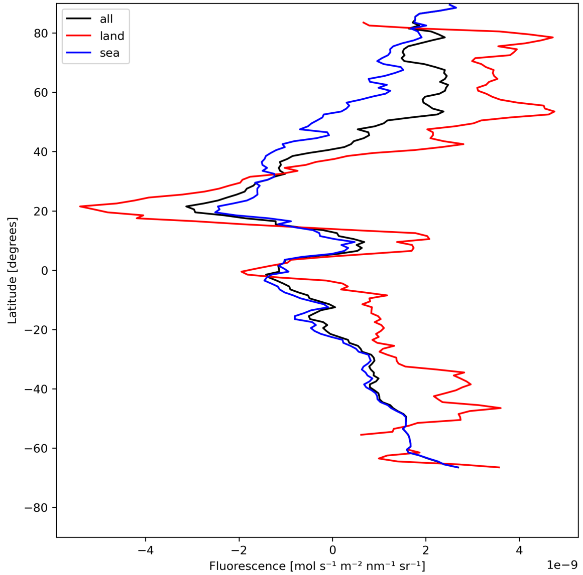
Figure 23: Zonal average of “Fluorescence” for 2024-07-13 to 2024-07-15.
