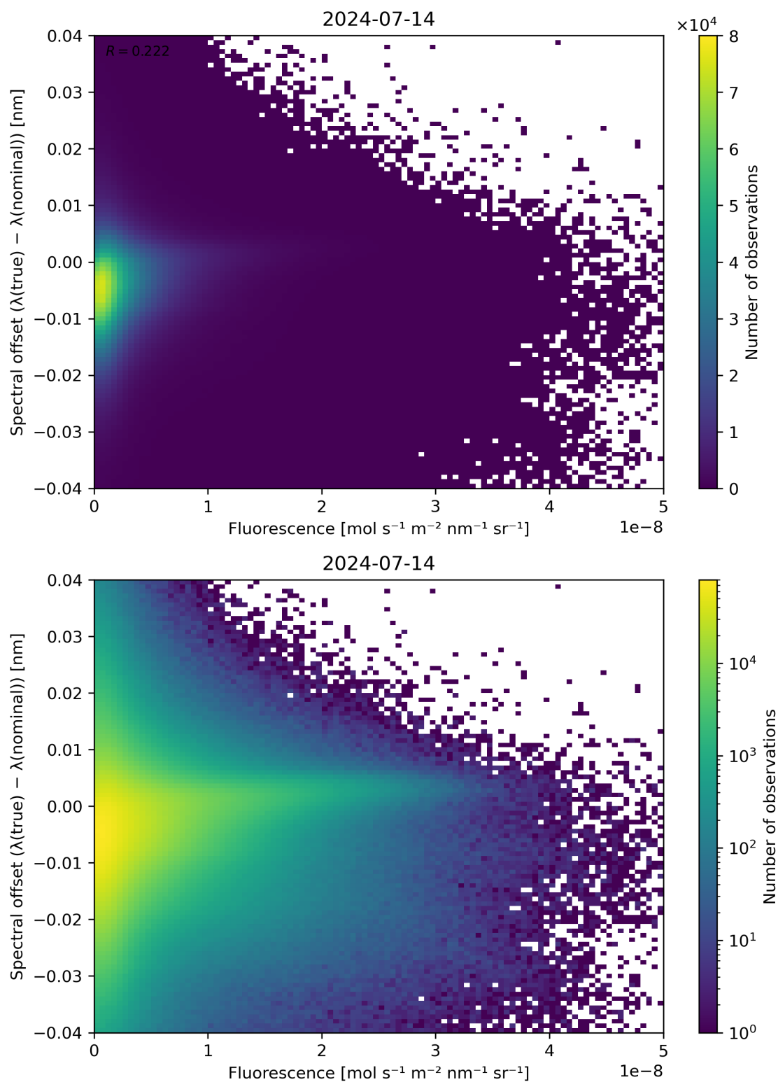
Figure 87: Scatter density plot of “Fluorescence” against “Spectral offset ( \lambda(\text{true}) - \lambda(\text{nominal}) )” for 2024-07-13 to 2024-07-15.
