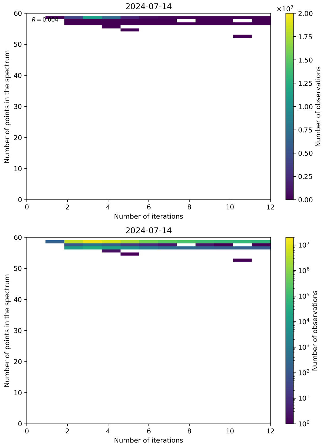
Figure 99: Scatter density plot of “Number of iterations” against “Number of points in the spectrum” for 2024-07-13 to 2024-07-15.
