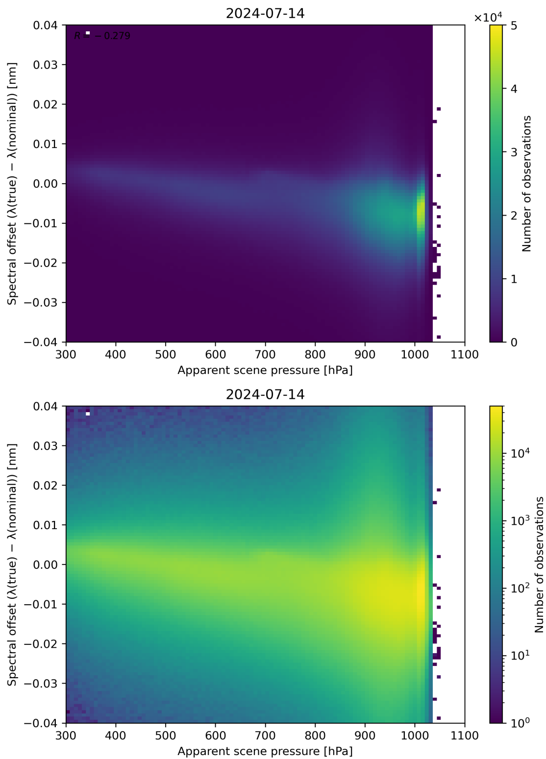
Figure 67: Scatter density plot of “Apparent scene pressure” against “Spectral offset ( \lambda(\text{true}) - \lambda(\text{nominal}) )” for 2024-07-13 to 2024-07-15.
