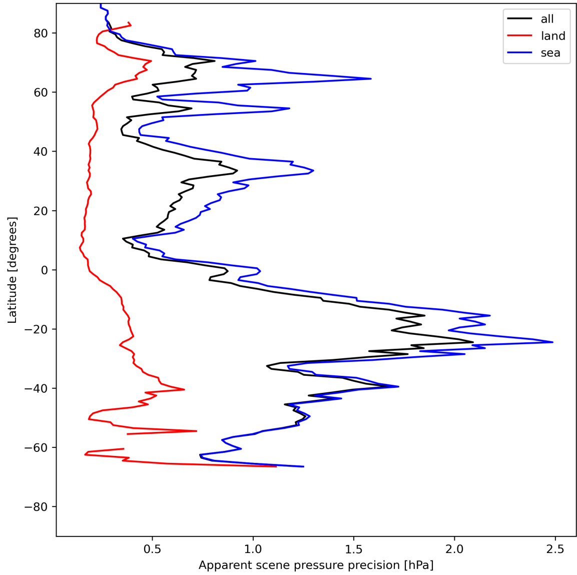
Figure 20: Zonal average of “Apparent scene pressure precision” for 2024-07-13 to 2024-07-15.
