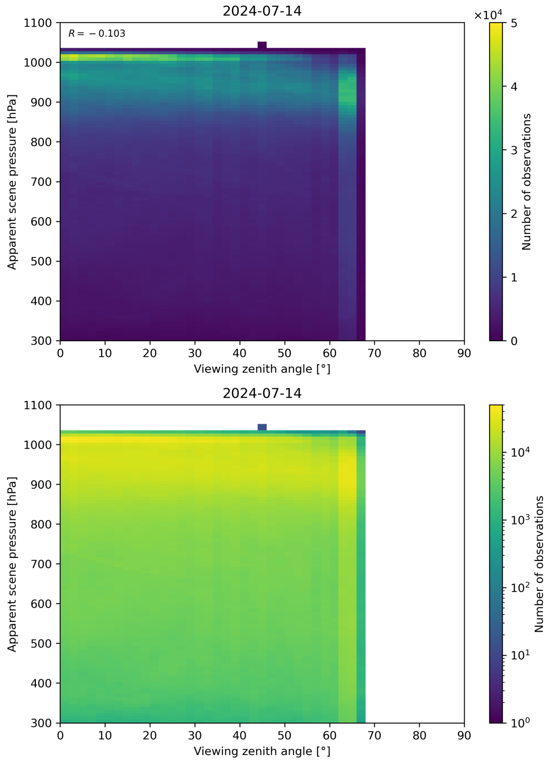
Figure 118: Scatter density plot of “Viewing zenith angle” against “Apparent scene pressure” for 2024-07-13 to 2024-07-15.
