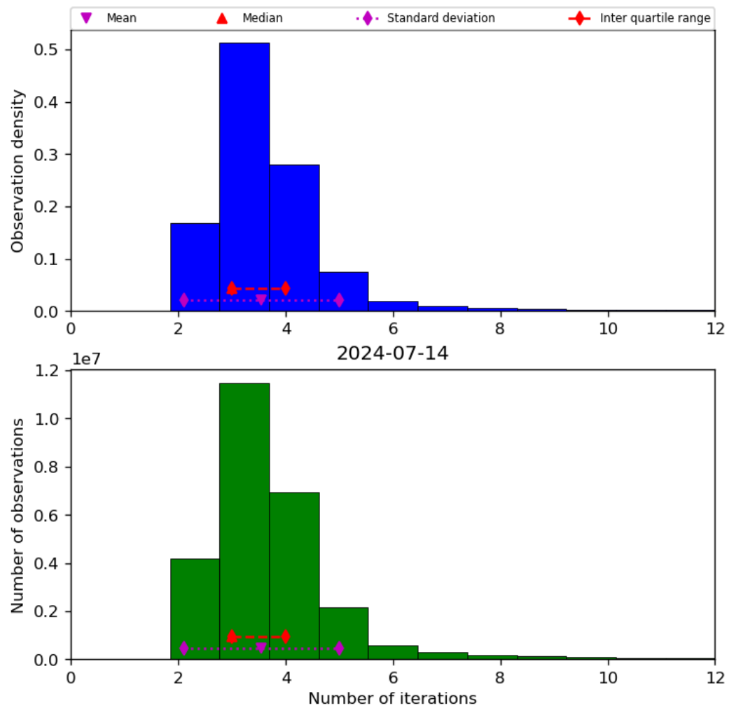
Figure 39: Histogram of “Number of iterations” for 2024-07-13 to 2024-07-15
