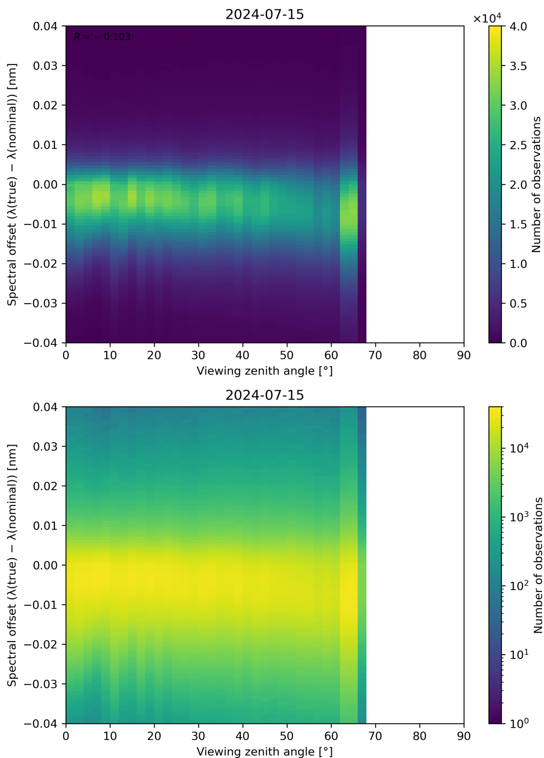
Figure 128: Scatter density plot of “Viewing zenith angle” against “Spectral offset ( \lambda(\text{true}) - \lambda(\text{nominal}) )” for 2024-07-15 to 2024-07-16.
