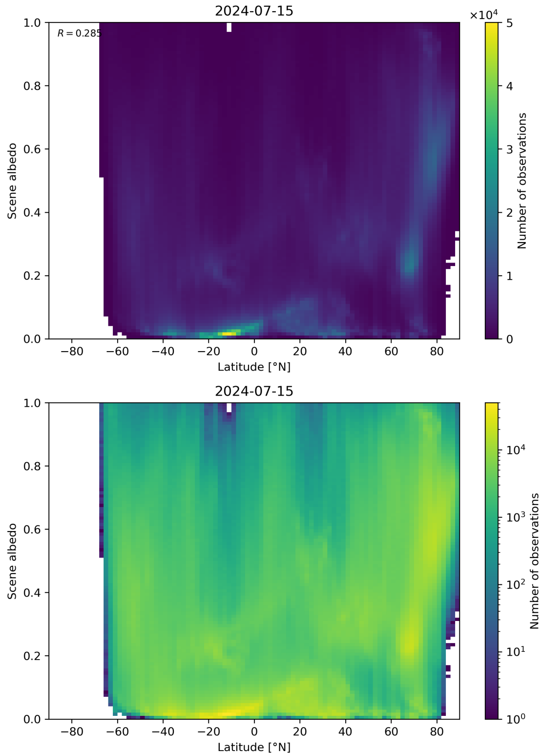
Figure 95: Scatter density plot of “Latitude” against “Scene albedo” for 2024-07-15 to 2024-07-16.
