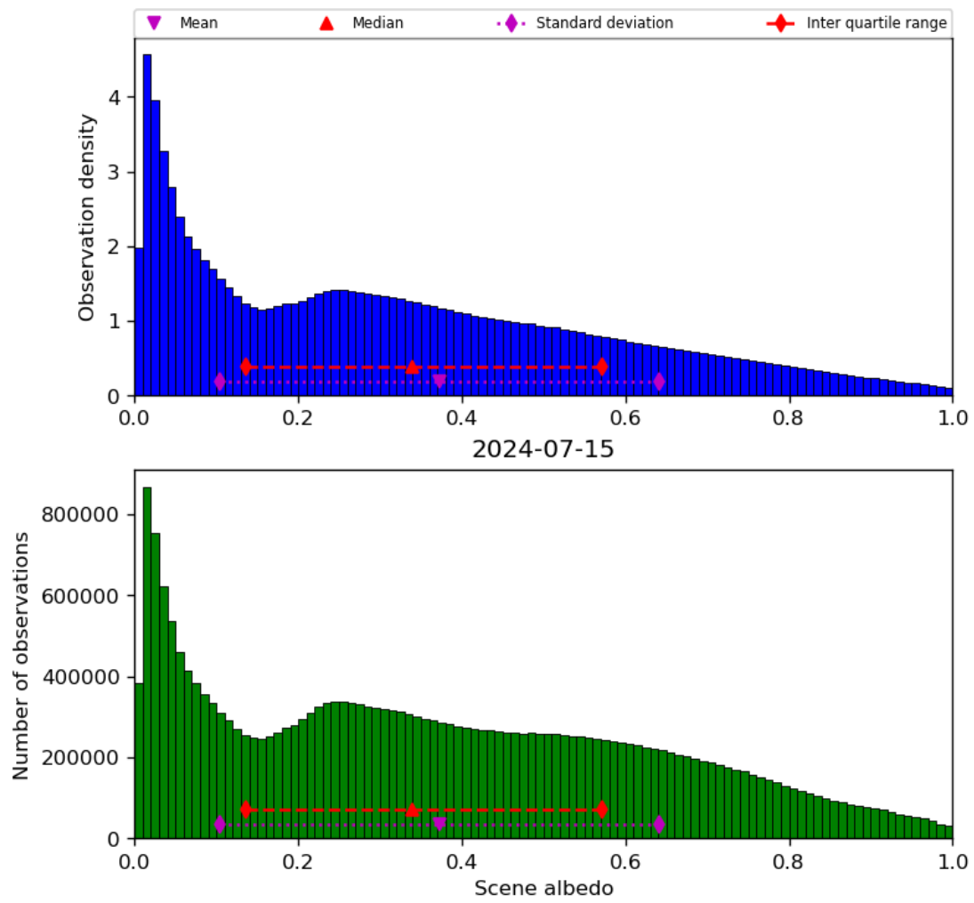
Figure 34: Histogram of “Scene albedo” for 2024-07-15 to 2024-07-16
