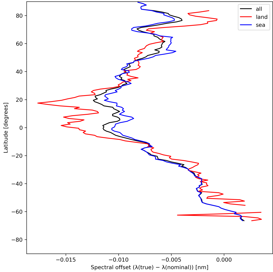
Figure 28: Zonal average of “Spectral offset ( \lambda(\text{true}) - \lambda(\text{nominal}) )” for 2024-07-15 to 2024-07-16.
