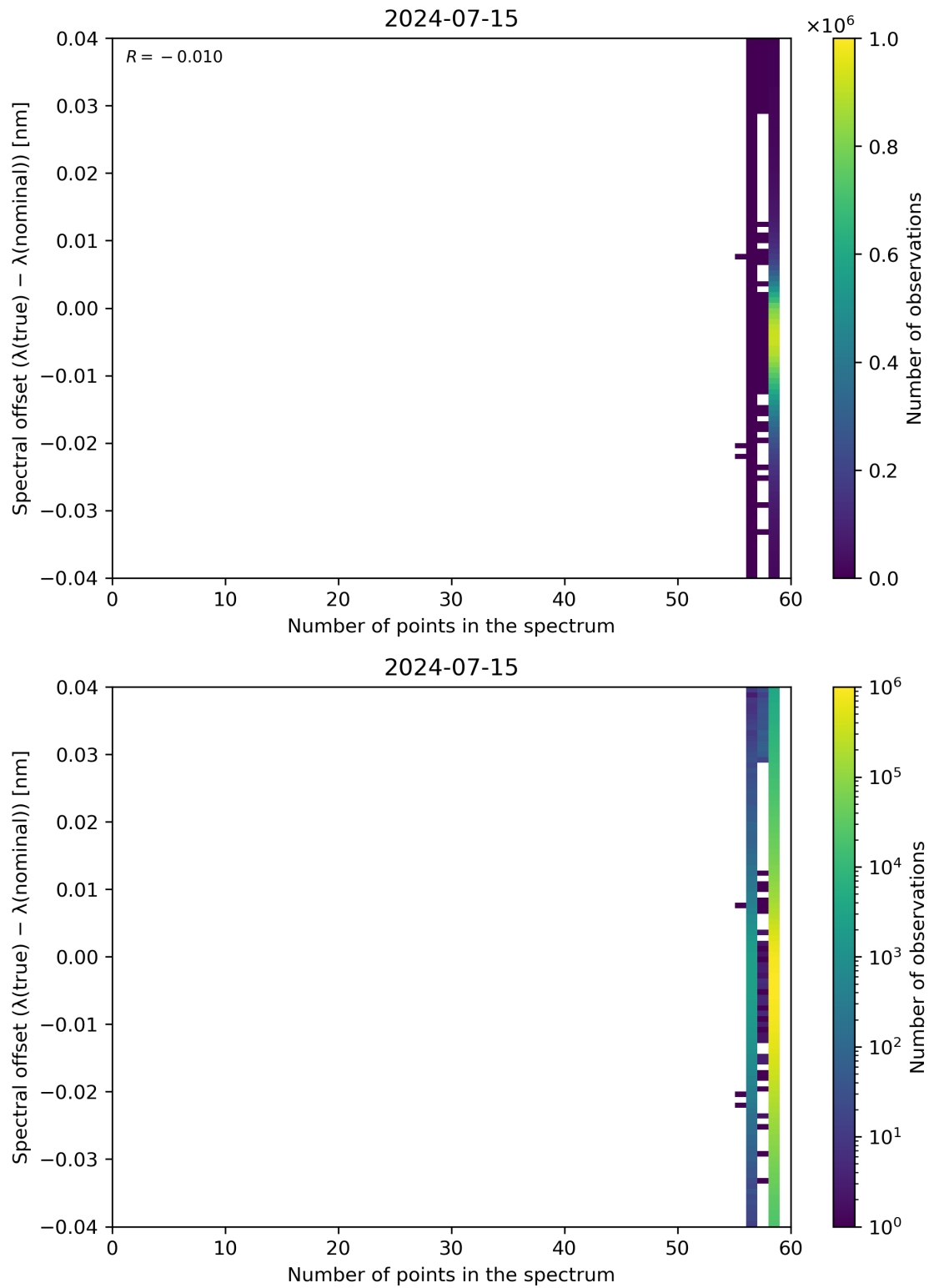
Figure 101: Scatter density plot of “Number of points in the spectrum” against “Spectral offset ( \lambda(\text{true}) - \lambda(\text{nominal}) )” for 2024-07-15 to 2024-07-16.
