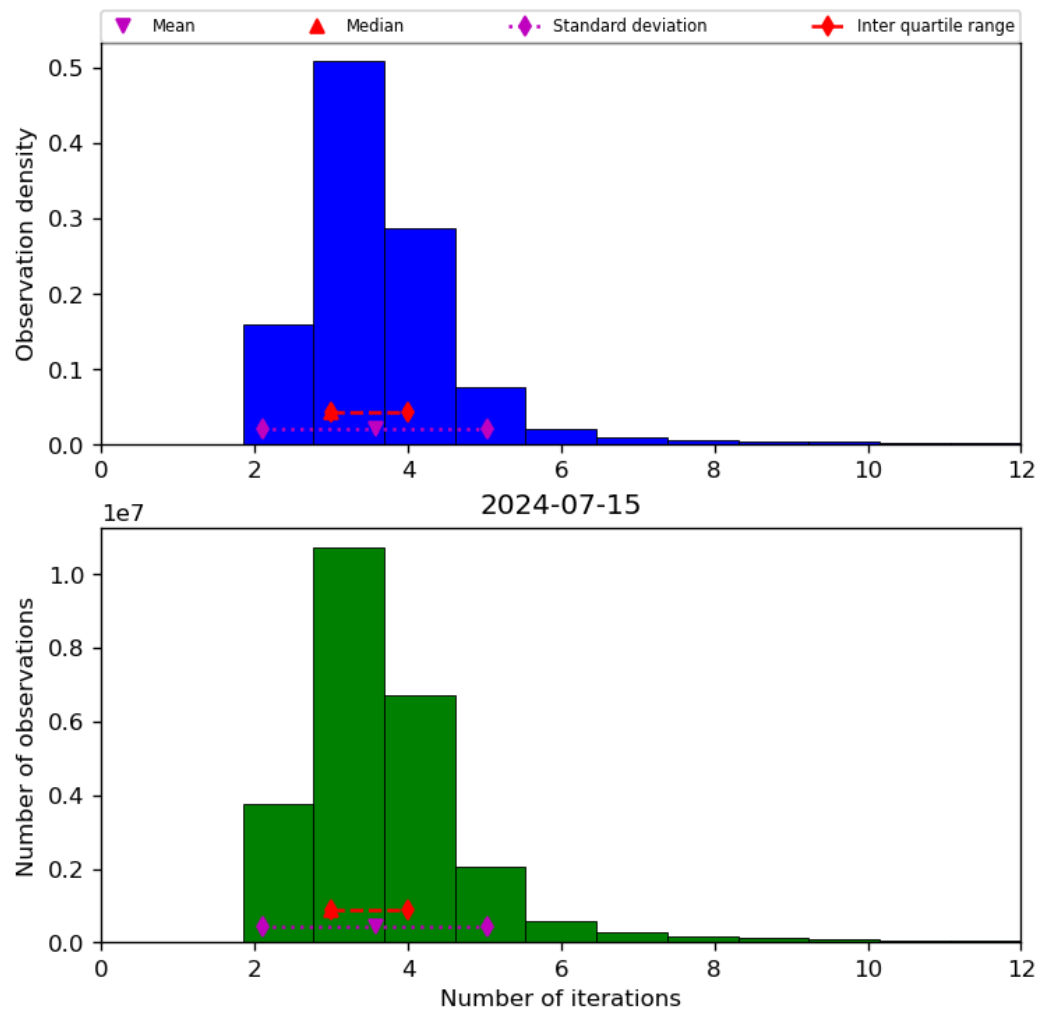
Figure 39: Histogram of “Number of iterations” for 2024-07-15 to 2024-07-16
