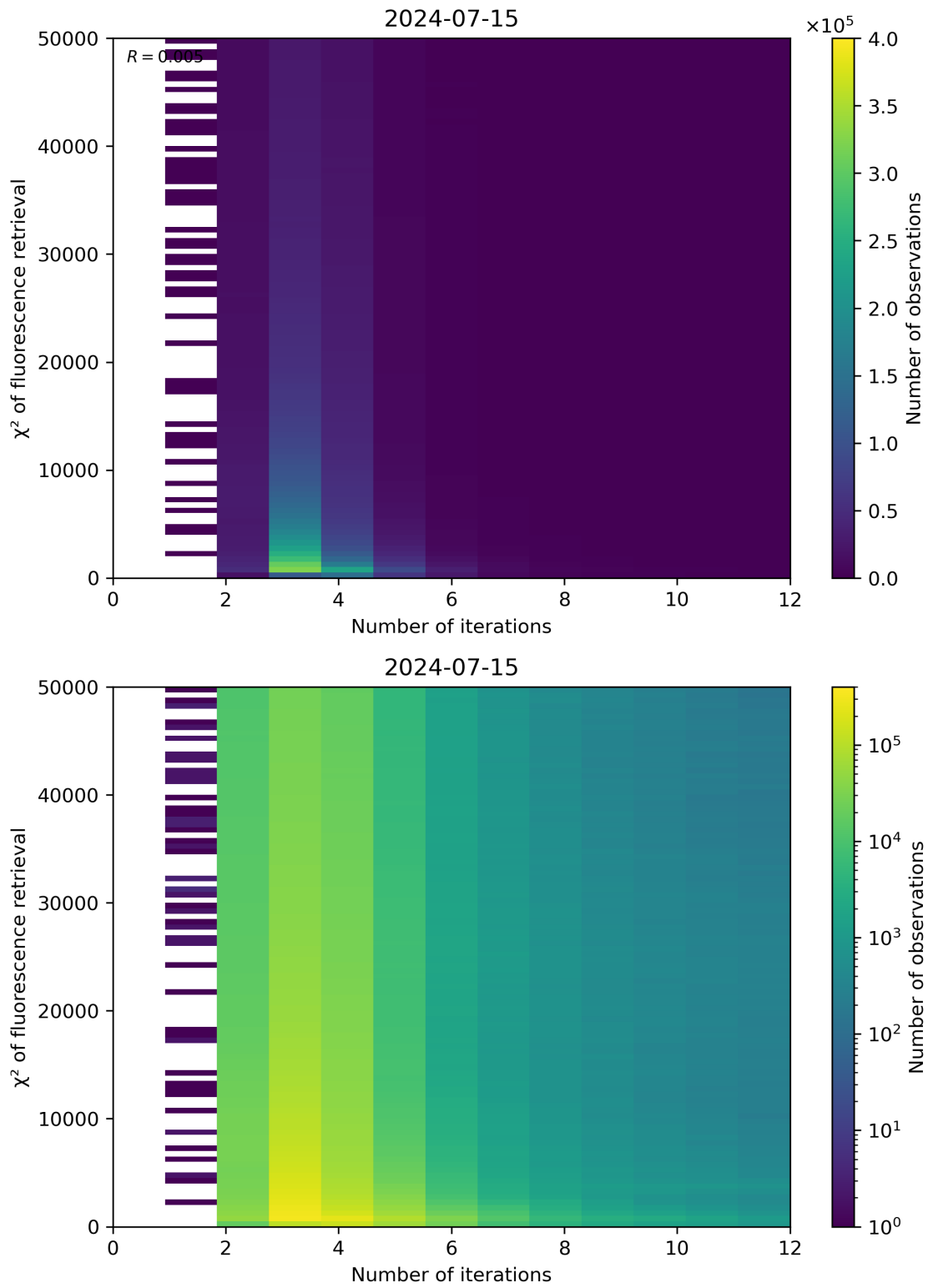
Figure 97: Scatter density plot of “Number of iterations” against “ \chi^2 of fluorescence retrieval” for 2024-07-15 to 2024-07-16.
