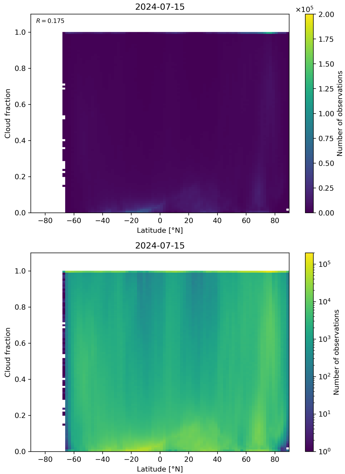
Figure 90: Scatter density plot of “Latitude” against “Cloud fraction” for 2024-07-15 to 2024-07-16.
