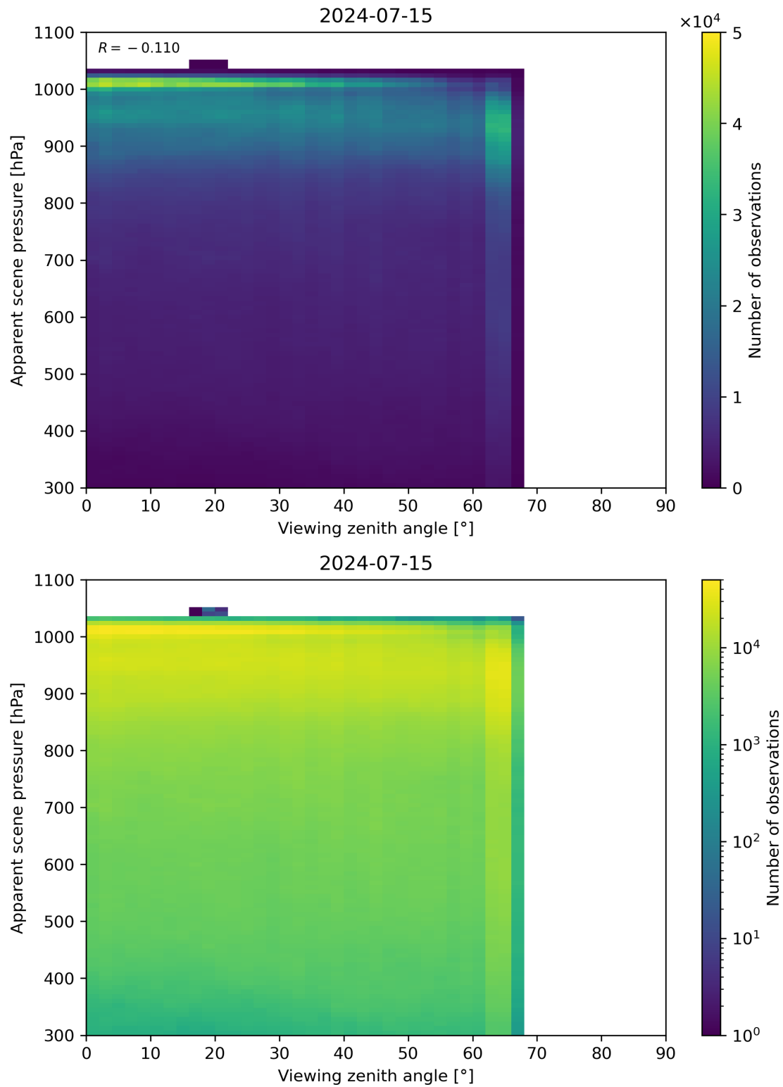
Figure 118: Scatter density plot of “Viewing zenith angle” against “Apparent scene pressure” for 2024-07-15 to 2024-07-16.
