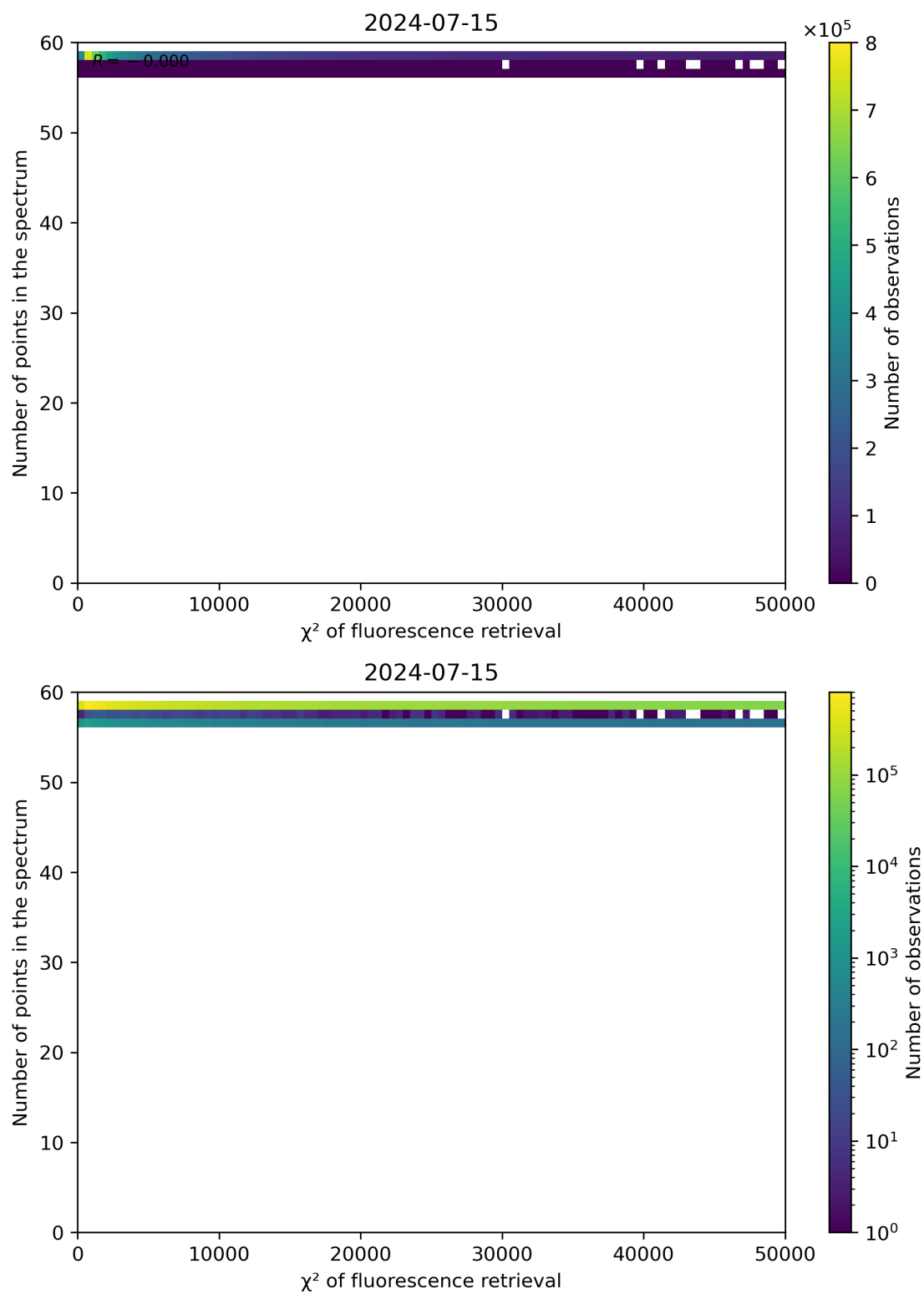
Figure 68: Scatter density plot of “ \chi^2 of fluorescence retrieval” against “Number of points in the spectrum” for 2024-07-15 to 2024-07-16.
