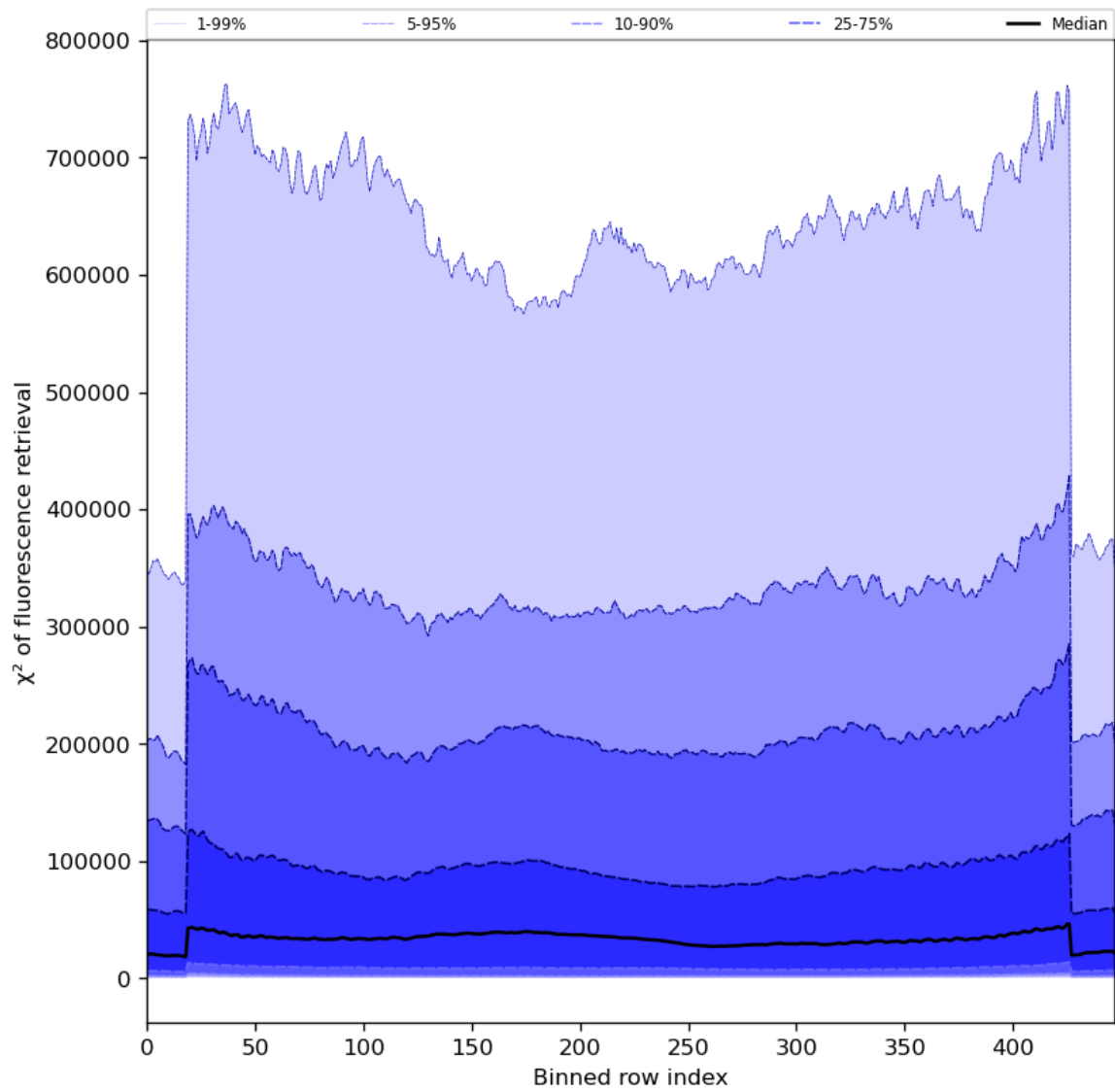
Figure 59: Along track statistics of “ \chi^2 of fluorescence retrieval” for 2024-07-15 to 2024-07-16
