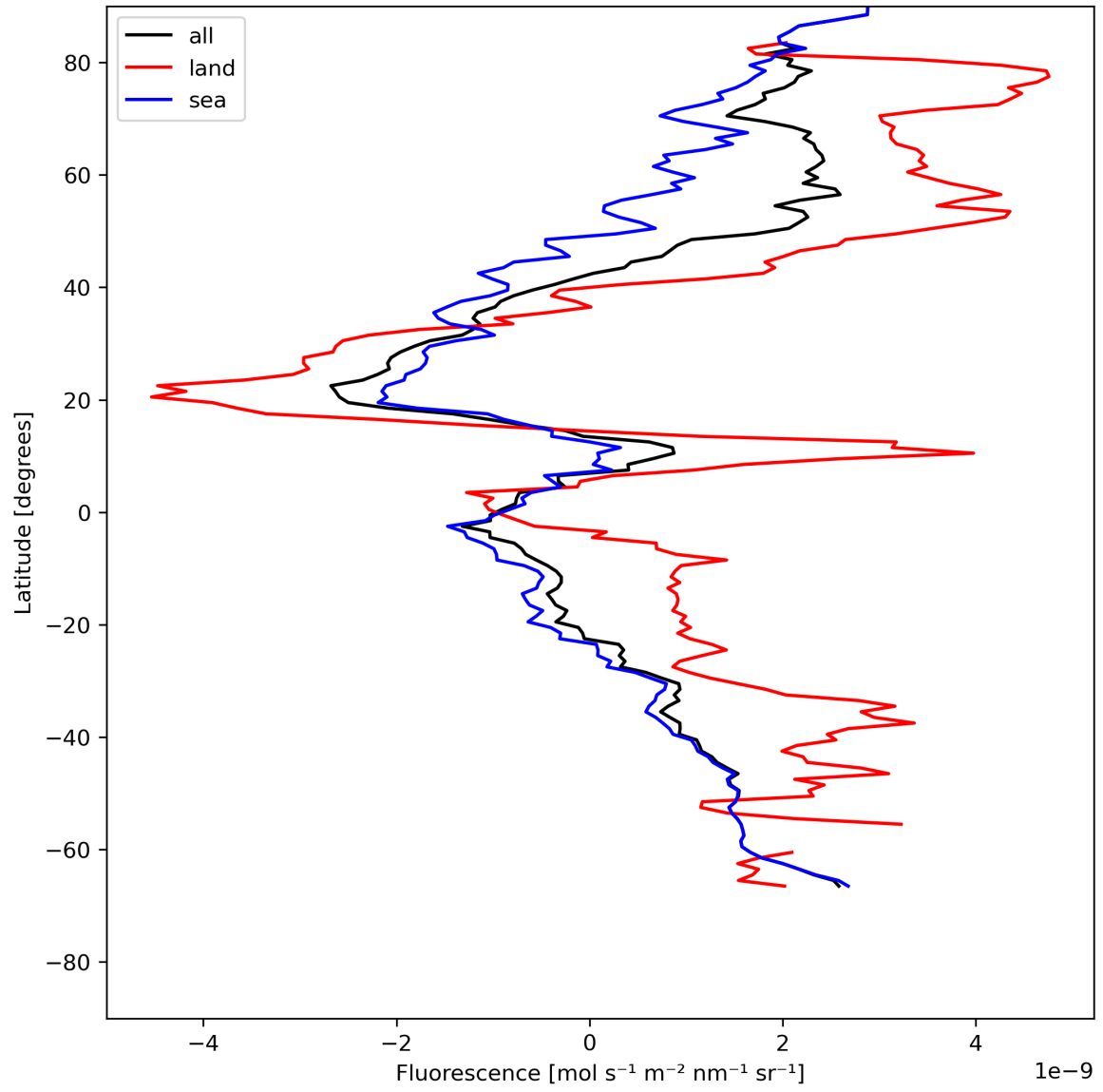
Figure 23: Zonal average of “Fluorescence” for 2024-07-15 to 2024-07-16.
