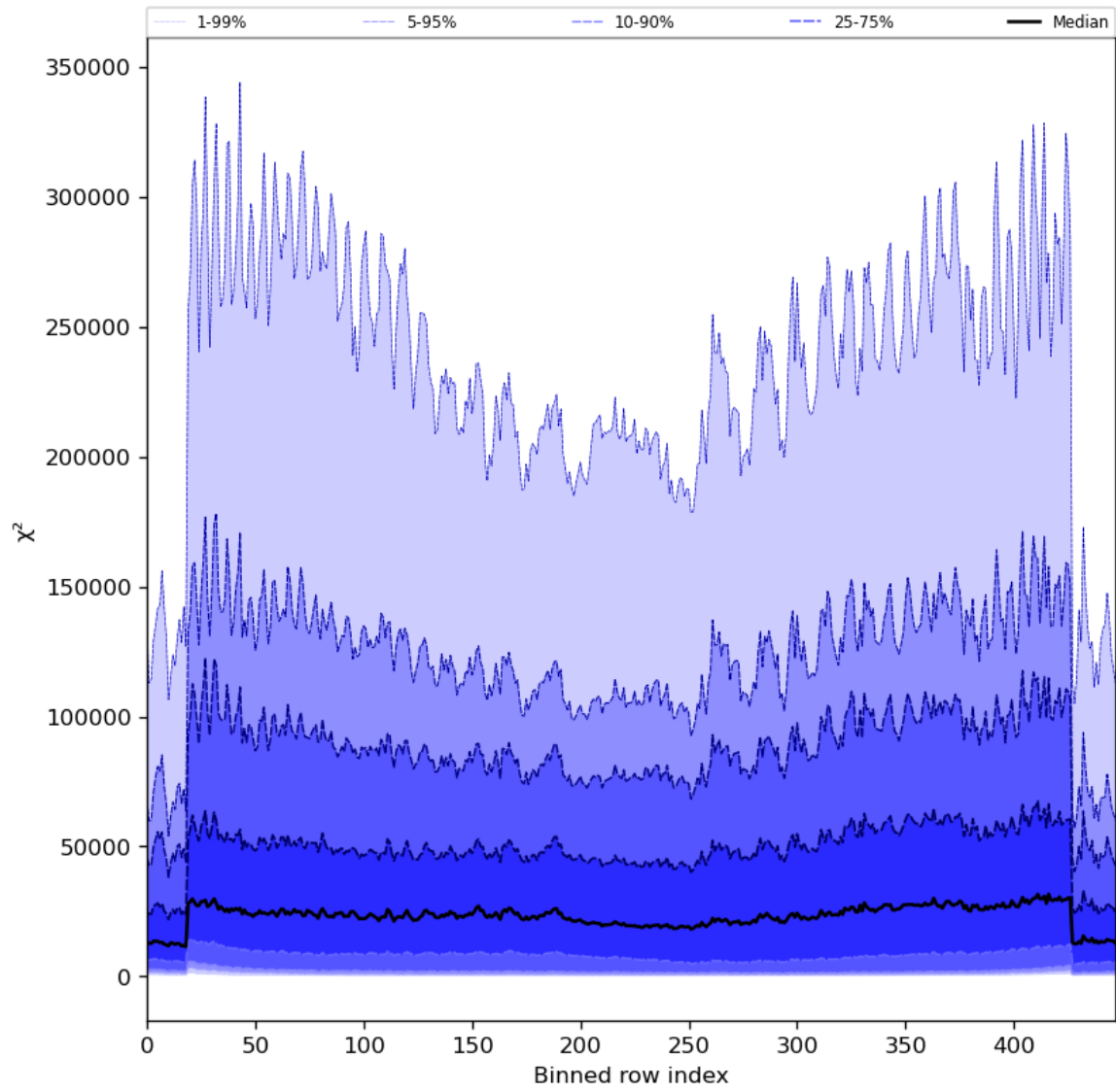
Figure 55: Along track statistics of “ \chi^2 ” for 2024-07-15 to 2024-07-16
