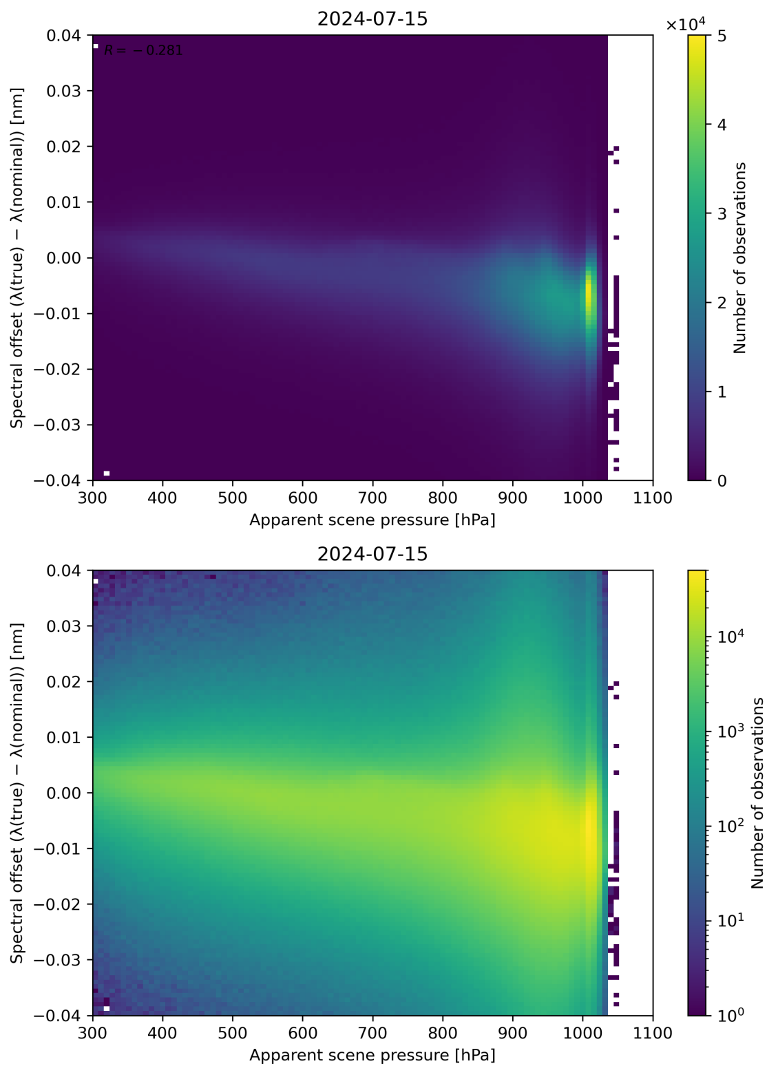
Figure 67: Scatter density plot of “Apparent scene pressure” against “Spectral offset ( \lambda(\text{true}) - \lambda(\text{nominal}) )” for 2024-07-15 to 2024-07-16.
