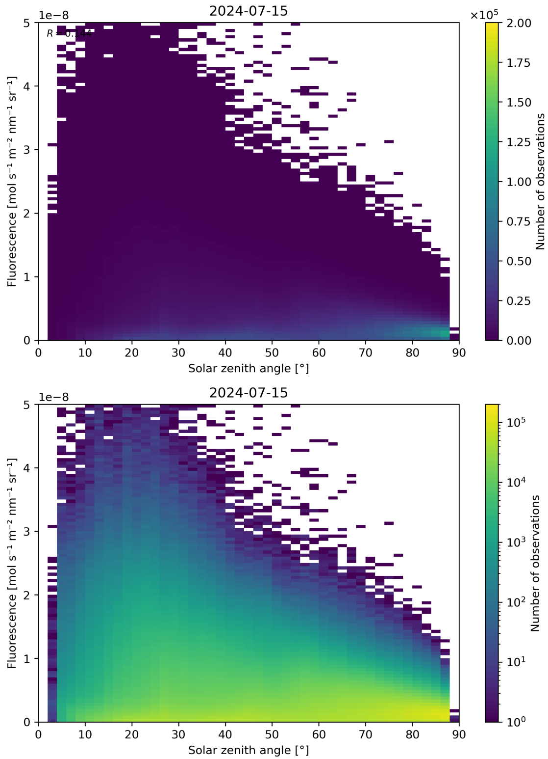
Figure 112: Scatter density plot of “Solar zenith angle” against “Fluorescence” for 2024-07-15 to 2024-07-16.
