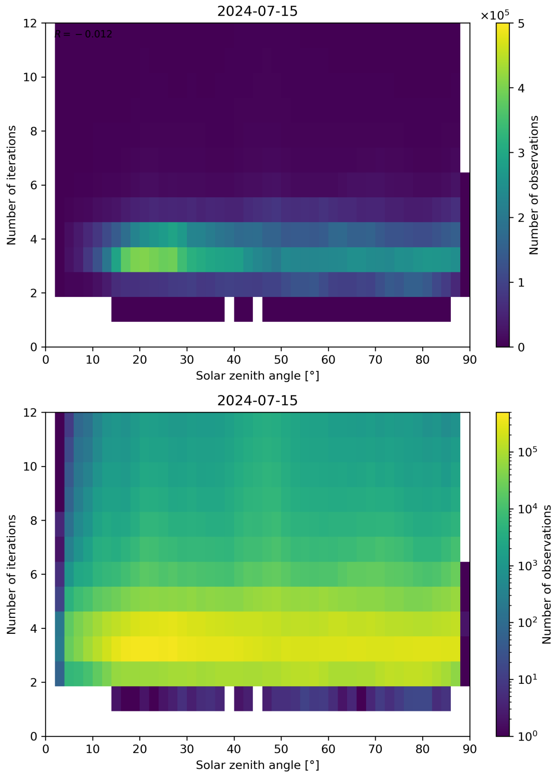
Figure 114: Scatter density plot of “Solar zenith angle” against “Number of iterations” for 2024-07-15 to 2024-07-16.
