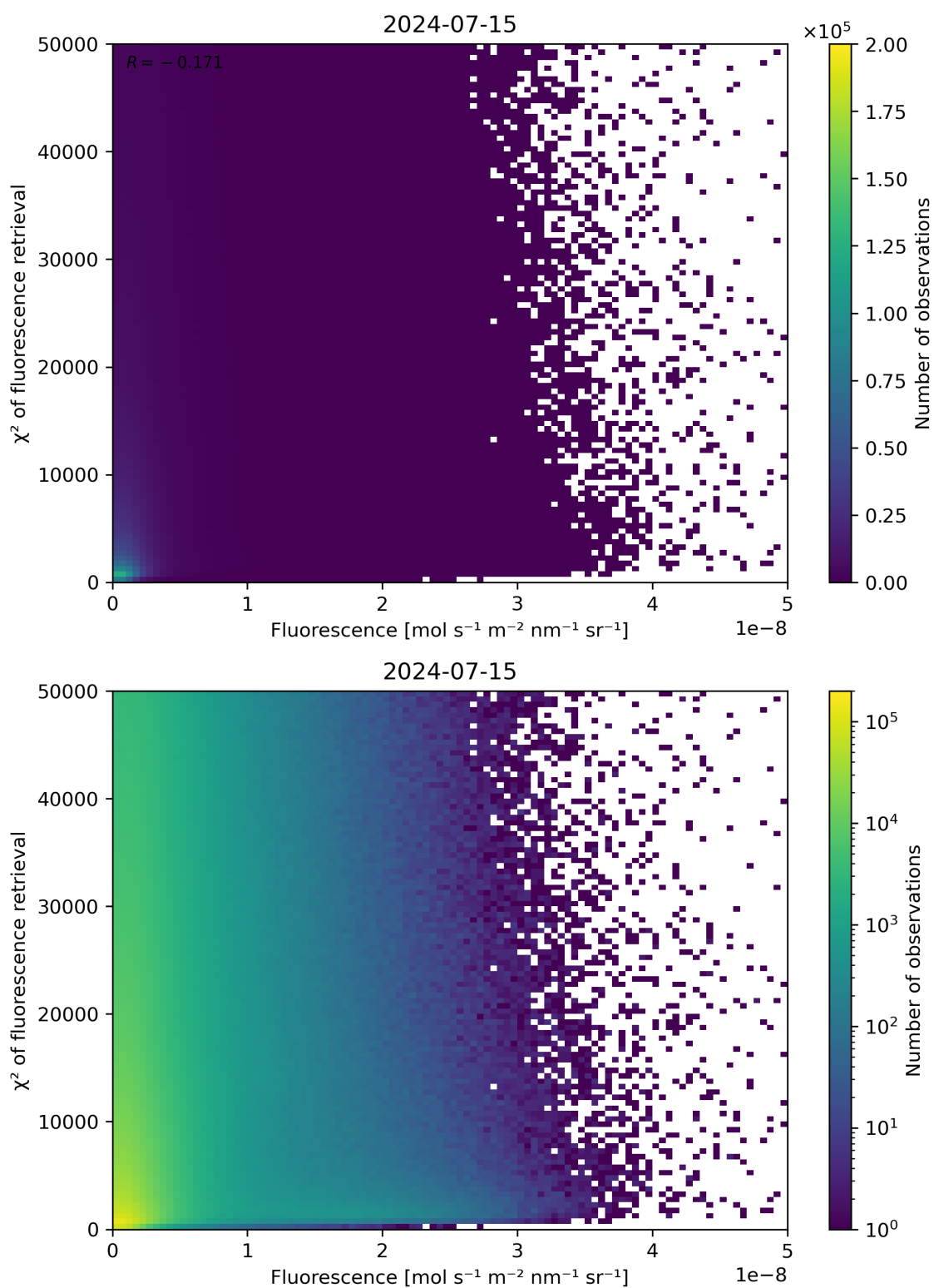
Figure 85: Scatter density plot of “Fluorescence” against “ \chi^2 of fluorescence retrieval” for 2024-07-15 to 2024-07-16.
