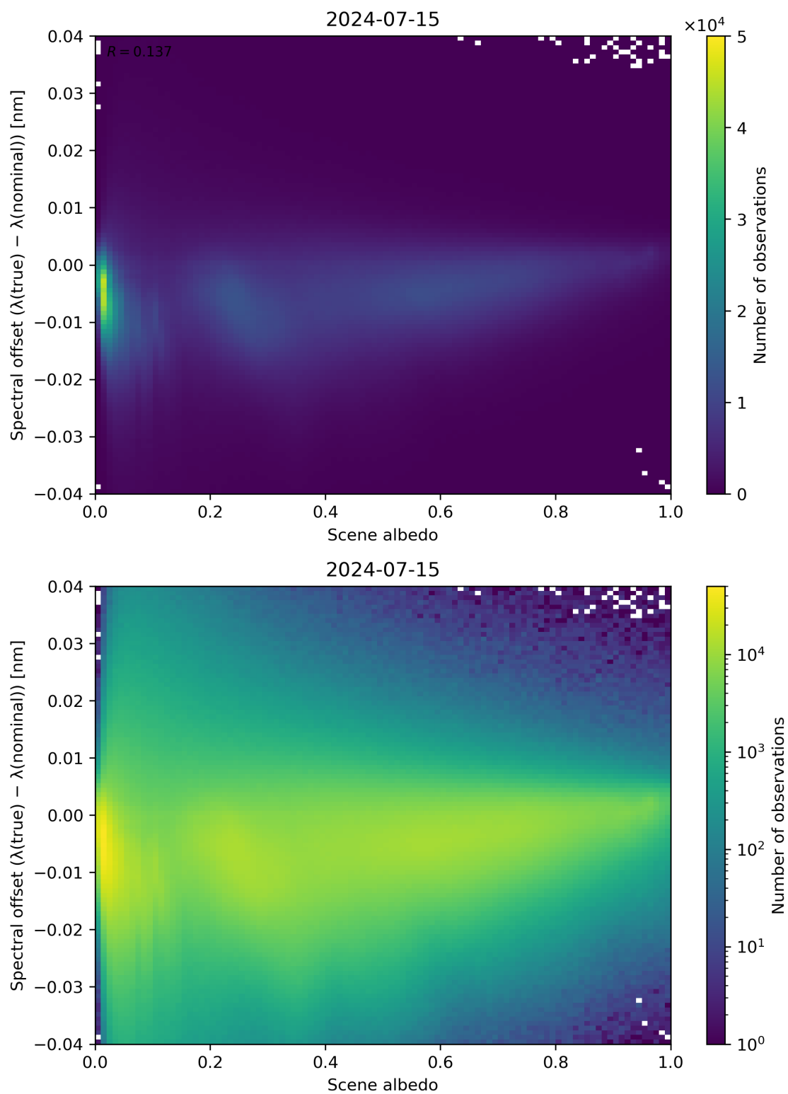
Figure 107: Scatter density plot of “Scene albedo” against “Spectral offset ( \lambda(\text{true}) - \lambda(\text{nominal}) )” for 2024-07-15 to 2024-07-16.
