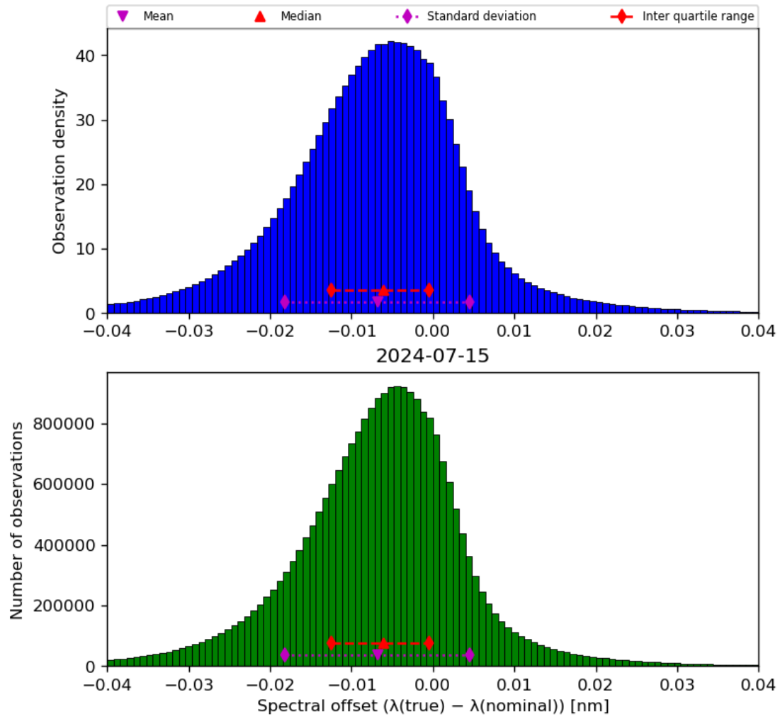
Figure 45: Histogram of “Spectral offset ( \lambda(\text{true}) - \lambda(\text{nominal}) )” for 2024-07-15 to 2024-07-16
