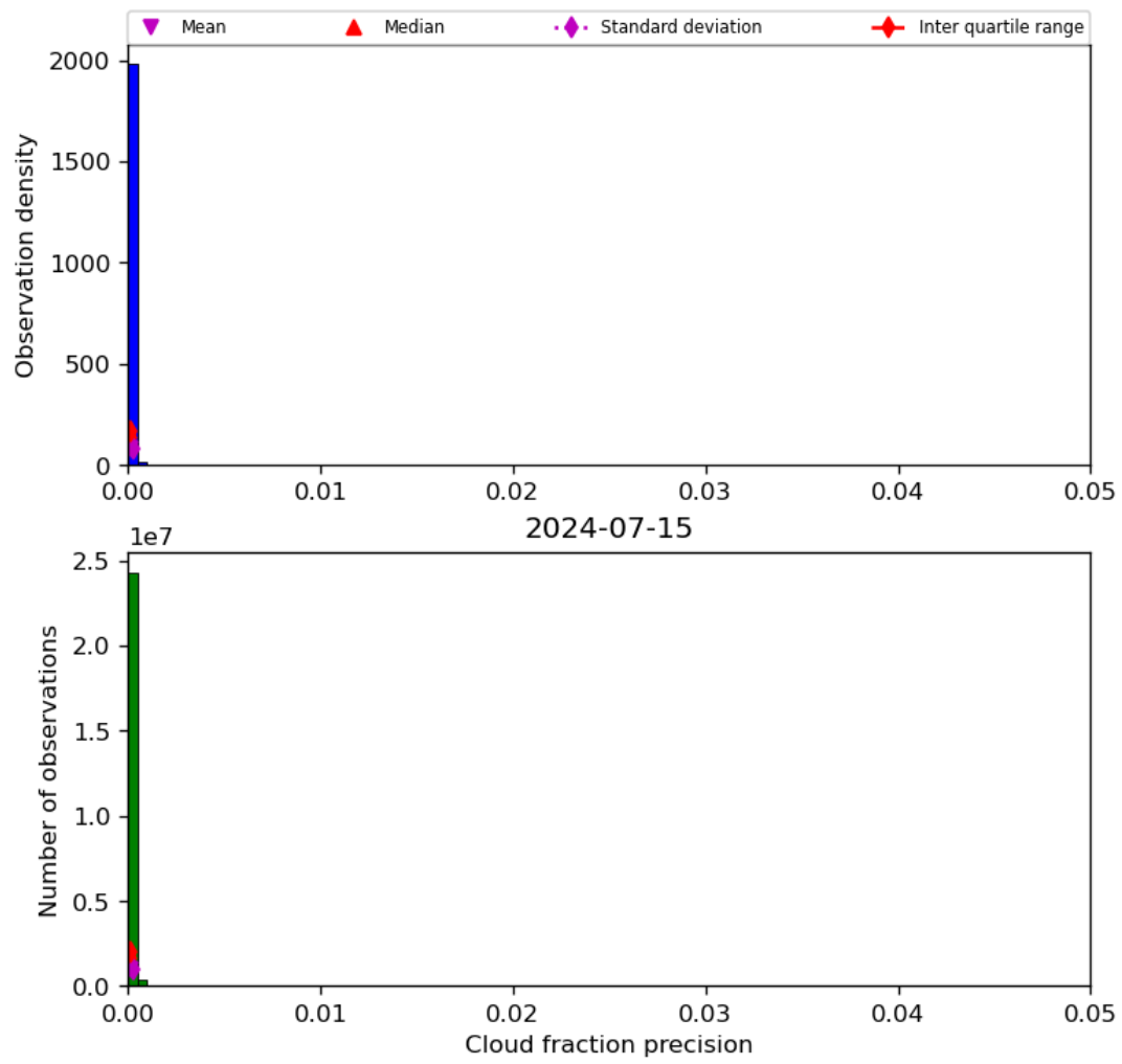
Figure 33: Histogram of “Cloud fraction precision” for 2024-07-15 to 2024-07-16
