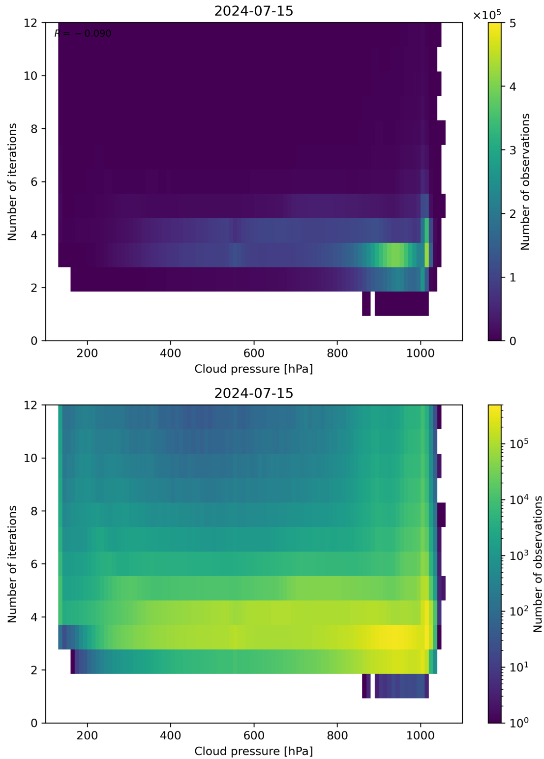
Figure 81: Scatter density plot of “Cloud pressure” against “Number of iterations” for 2024-07-15 to 2024-07-16.
