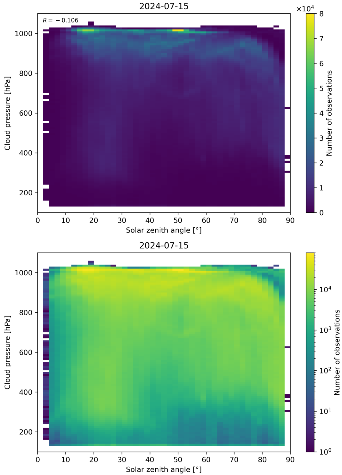
Figure 111: Scatter density plot of “Solar zenith angle” against “Cloud pressure” for 2024-07-15 to 2024-07-16.
