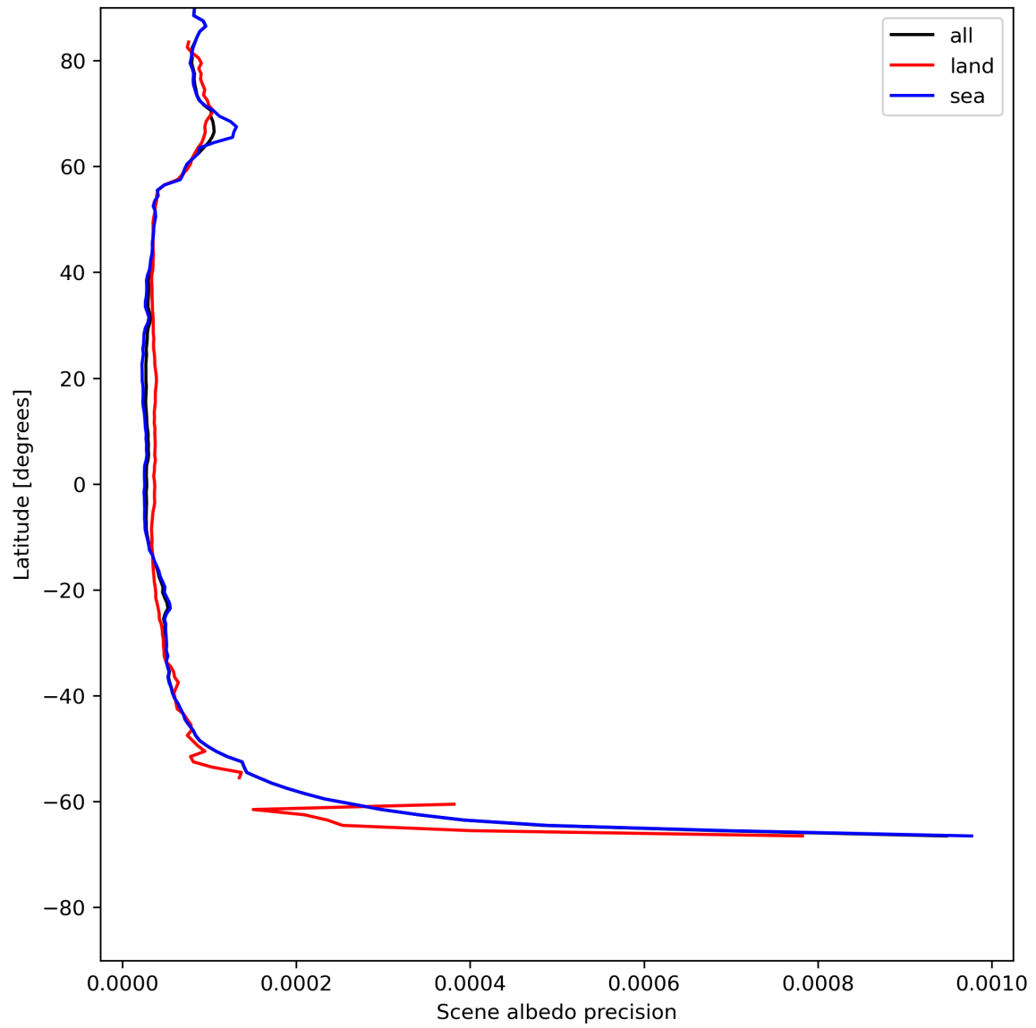
Figure 18: Zonal average of “Scene albedo precision” for 2024-07-15 to 2024-07-16.
