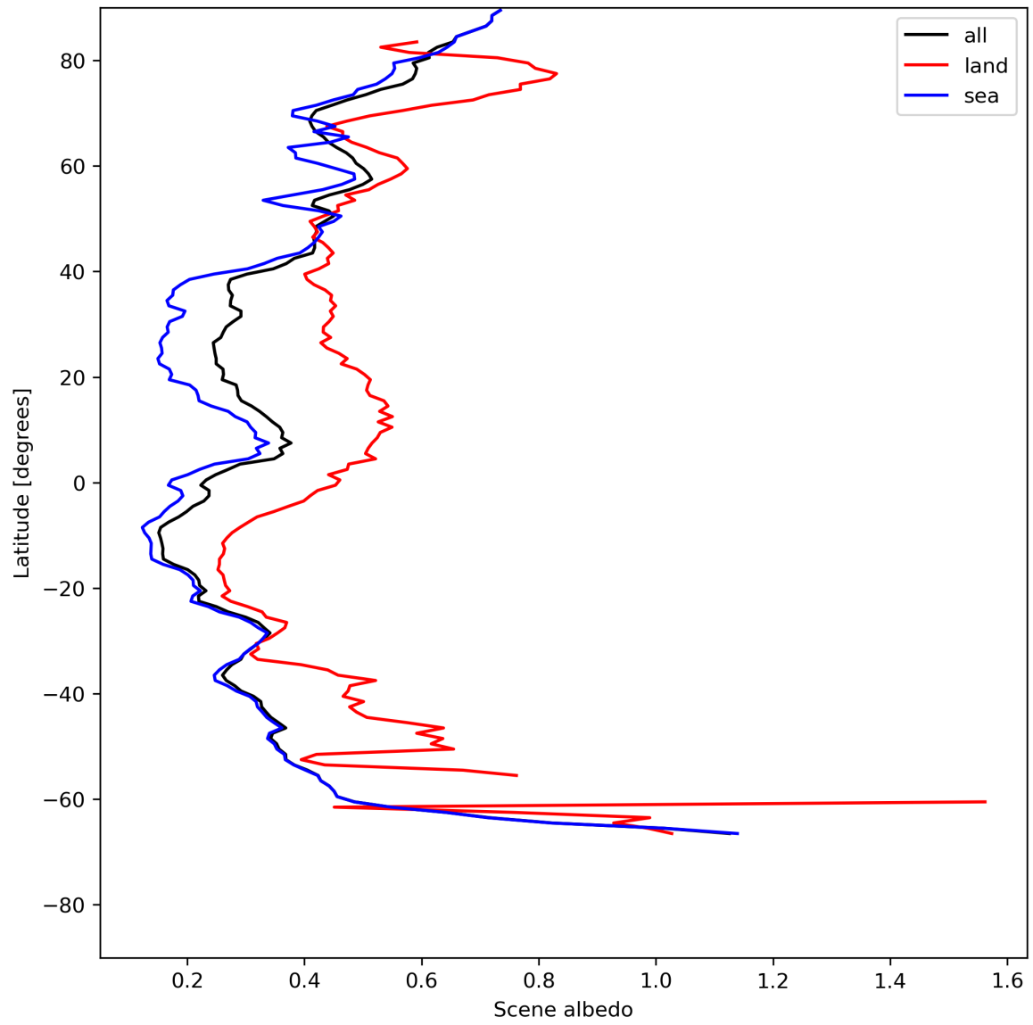
Figure 17: Zonal average of “Scene albedo” for 2024-07-15 to 2024-07-16.
