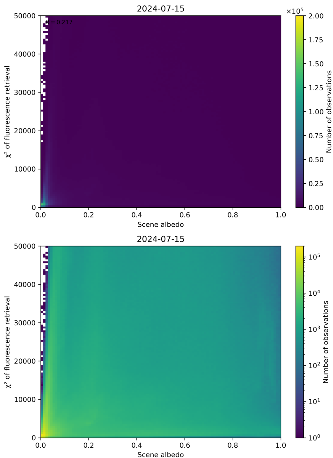
Figure 103: Scatter density plot of “Scene albedo” against “ \chi^2 of fluorescence retrieval” for 2024-07-15 to 2024-07-16.
