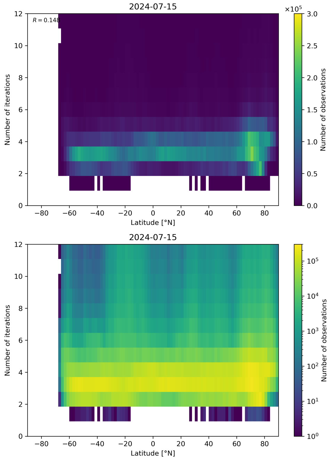
Figure 93: Scatter density plot of “Latitude” against “Number of iterations” for 2024-07-15 to 2024-07-16.
