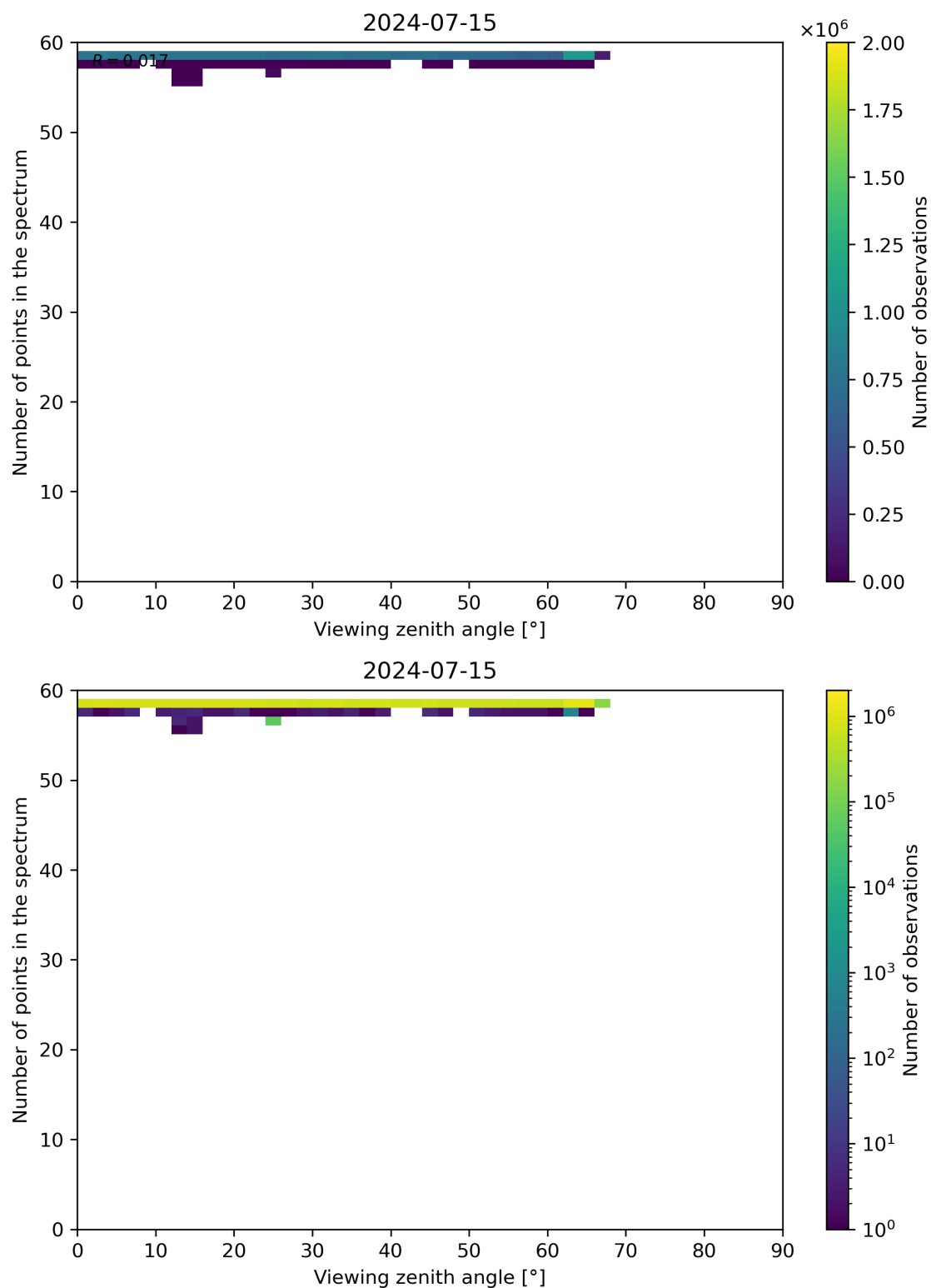
Figure 125: Scatter density plot of “Viewing zenith angle” against “Number of points in the spectrum” for 2024-07-15 to 2024-07-16.
