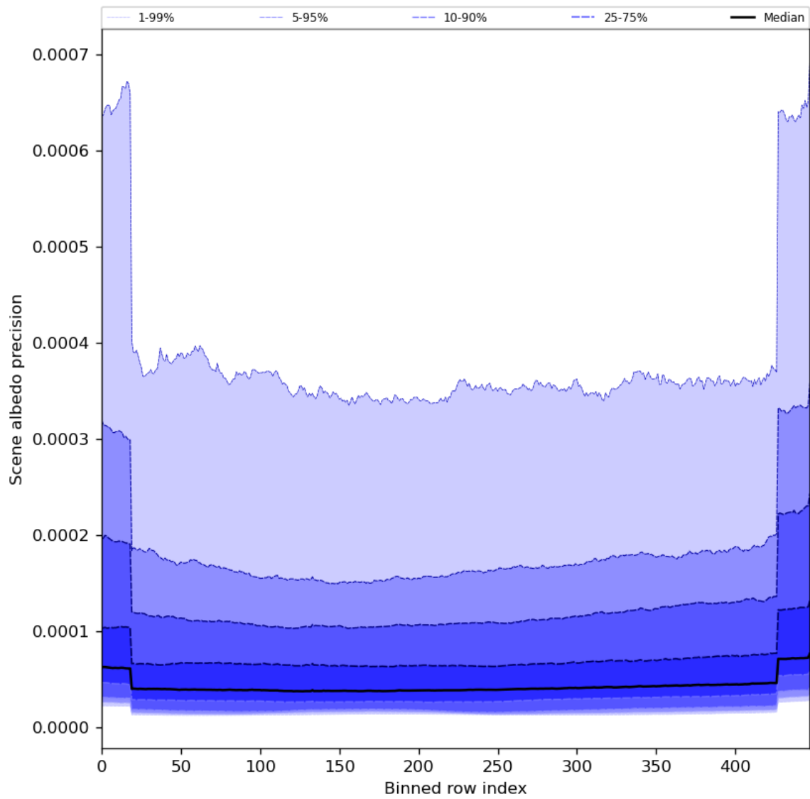
Figure 52: Along track statistics of “Scene albedo precision” for 2024-07-15 to 2024-07-16
