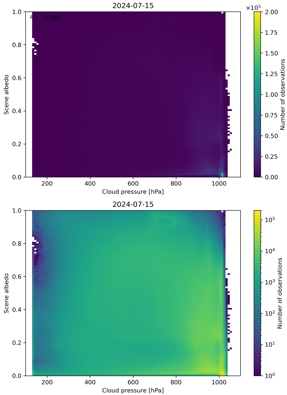
Figure 83: Scatter density plot of “Cloud pressure” against “Scene albedo” for 2024-07-15 to 2024-07-16.
