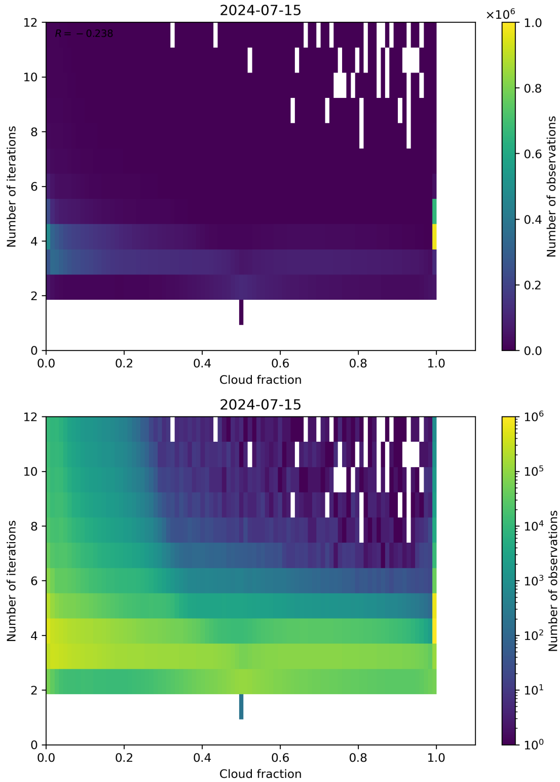
Figure 73: Scatter density plot of “Cloud fraction” against “Number of iterations” for 2024-07-15 to 2024-07-16.
