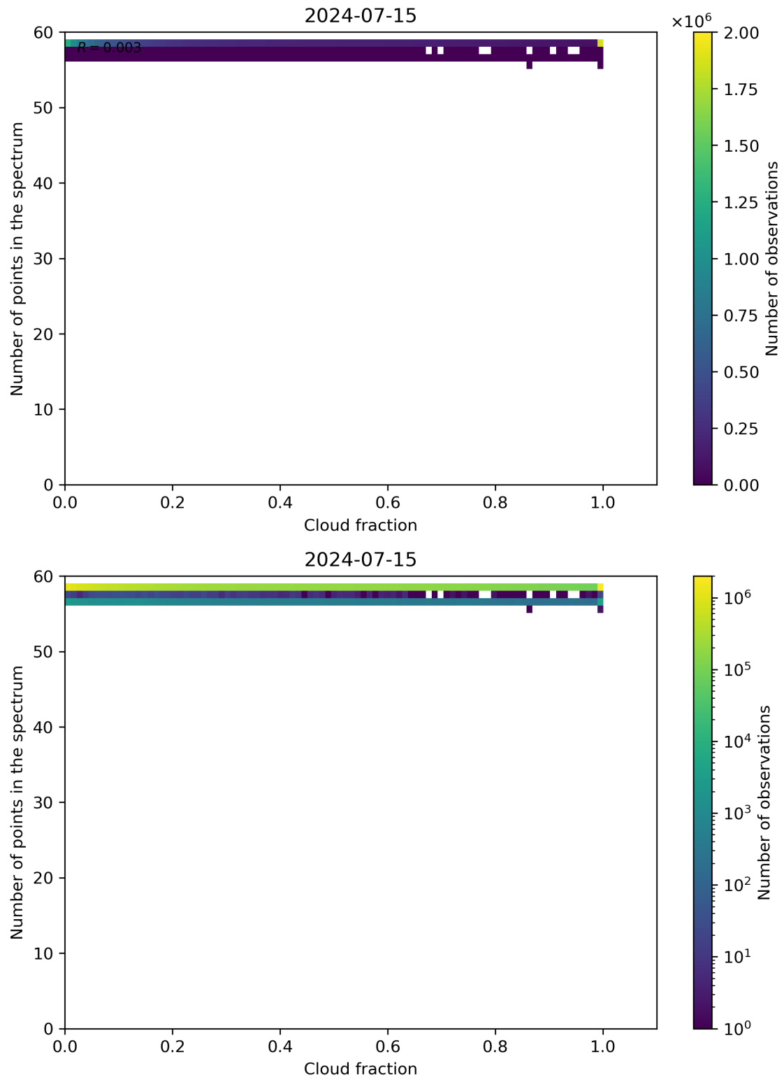
Figure 74: Scatter density plot of “Cloud fraction” against “Number of points in the spectrum” for 2024-07-15 to 2024-07-16.
