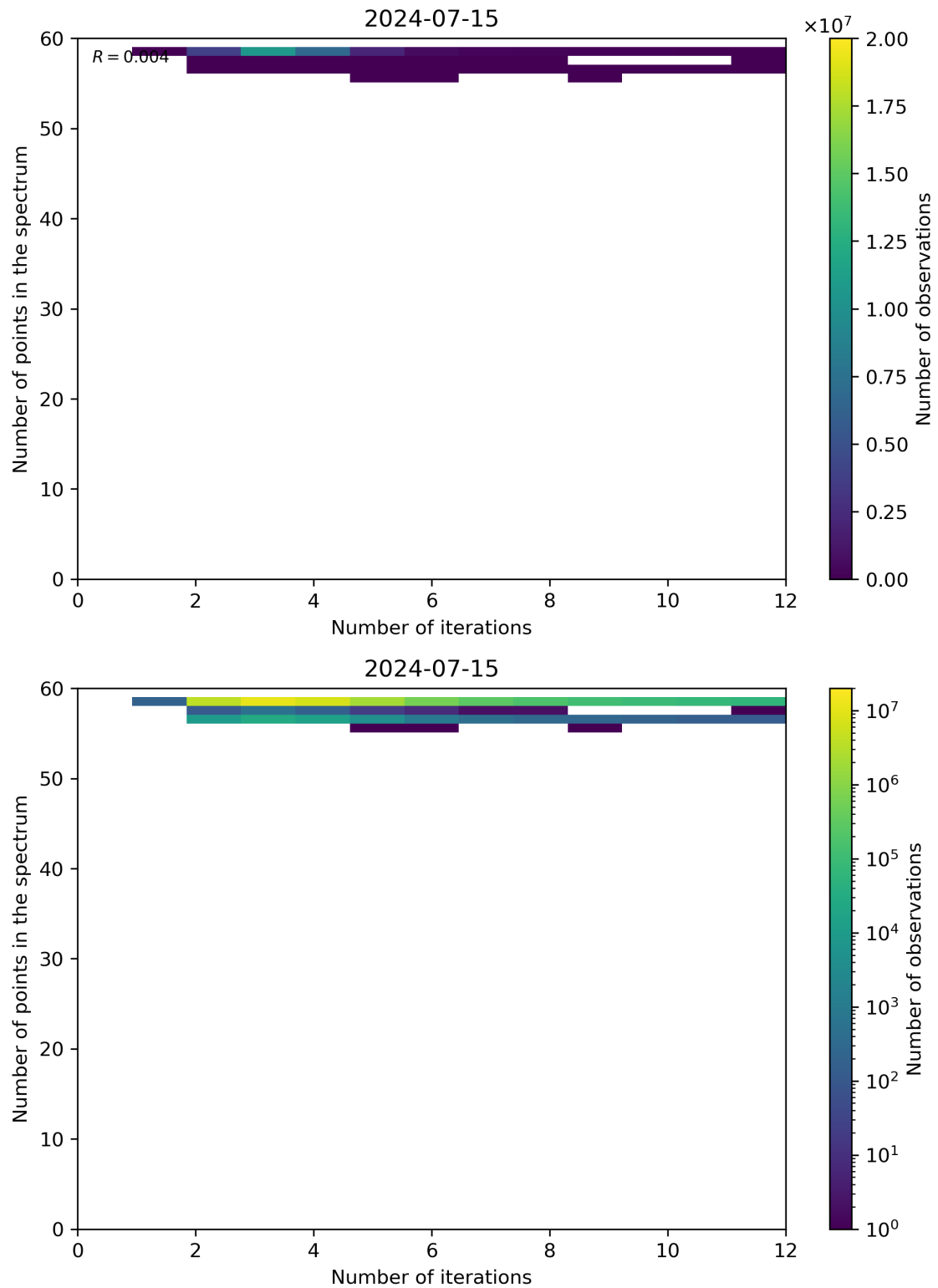
Figure 99: Scatter density plot of “Number of iterations” against “Number of points in the spectrum” for 2024-07-15 to 2024-07-16.
