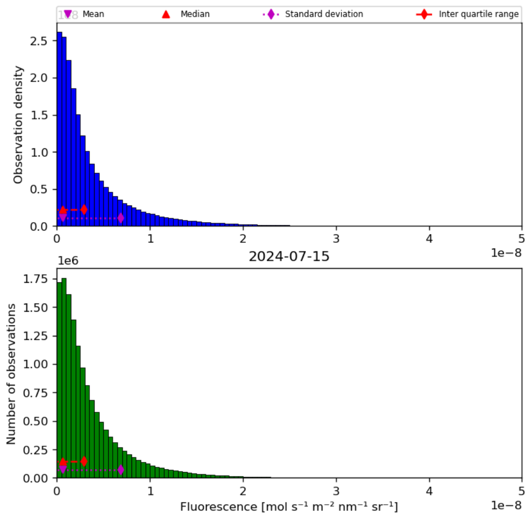
Figure 40: Histogram of “Fluorescence” for 2024-07-15 to 2024-07-16
