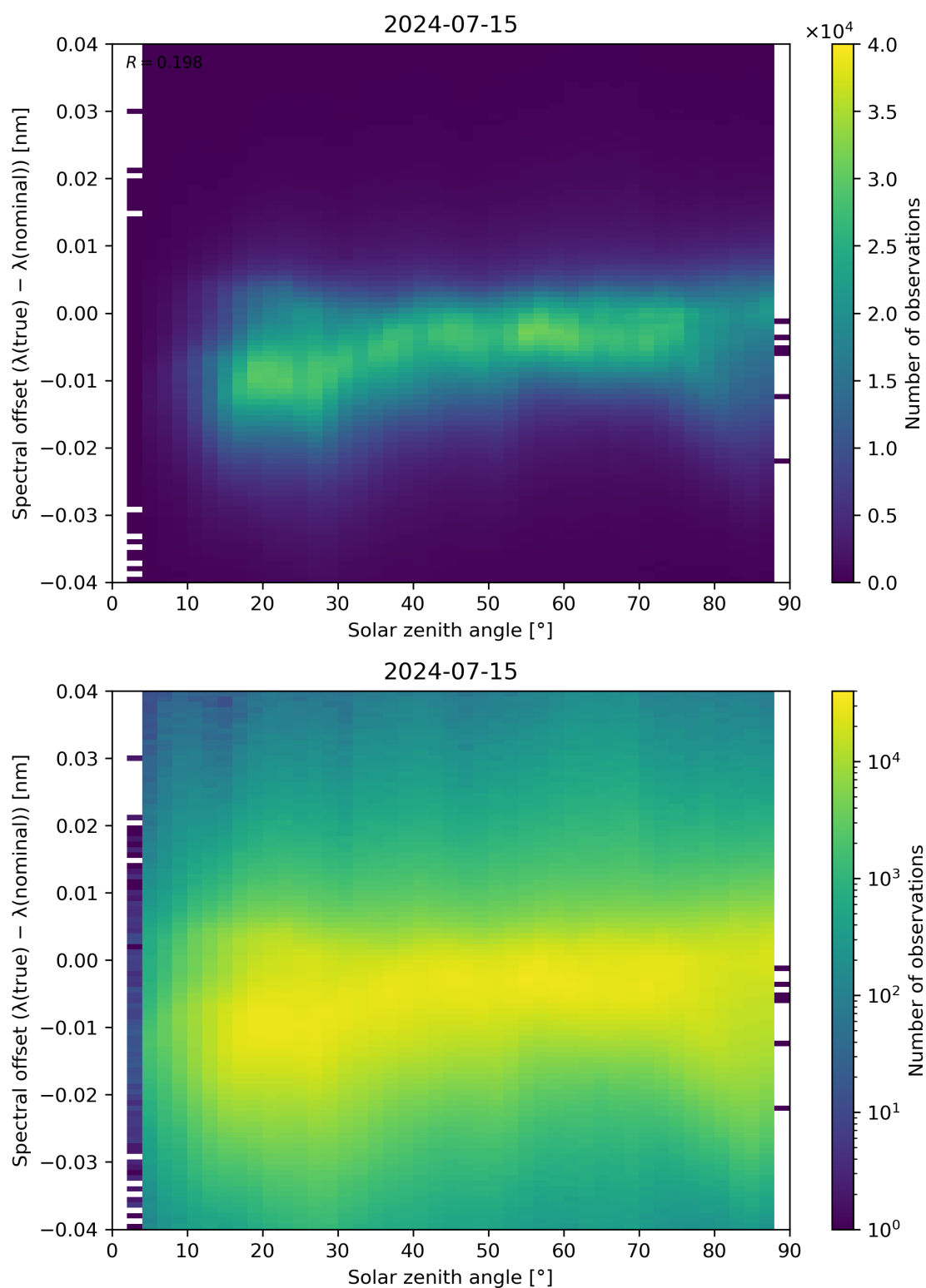
Figure 117: Scatter density plot of “Solar zenith angle” against “Spectral offset ( \lambda(\text{true}) - \lambda(\text{nominal}) )” for 2024-07-15 to 2024-07-16.
