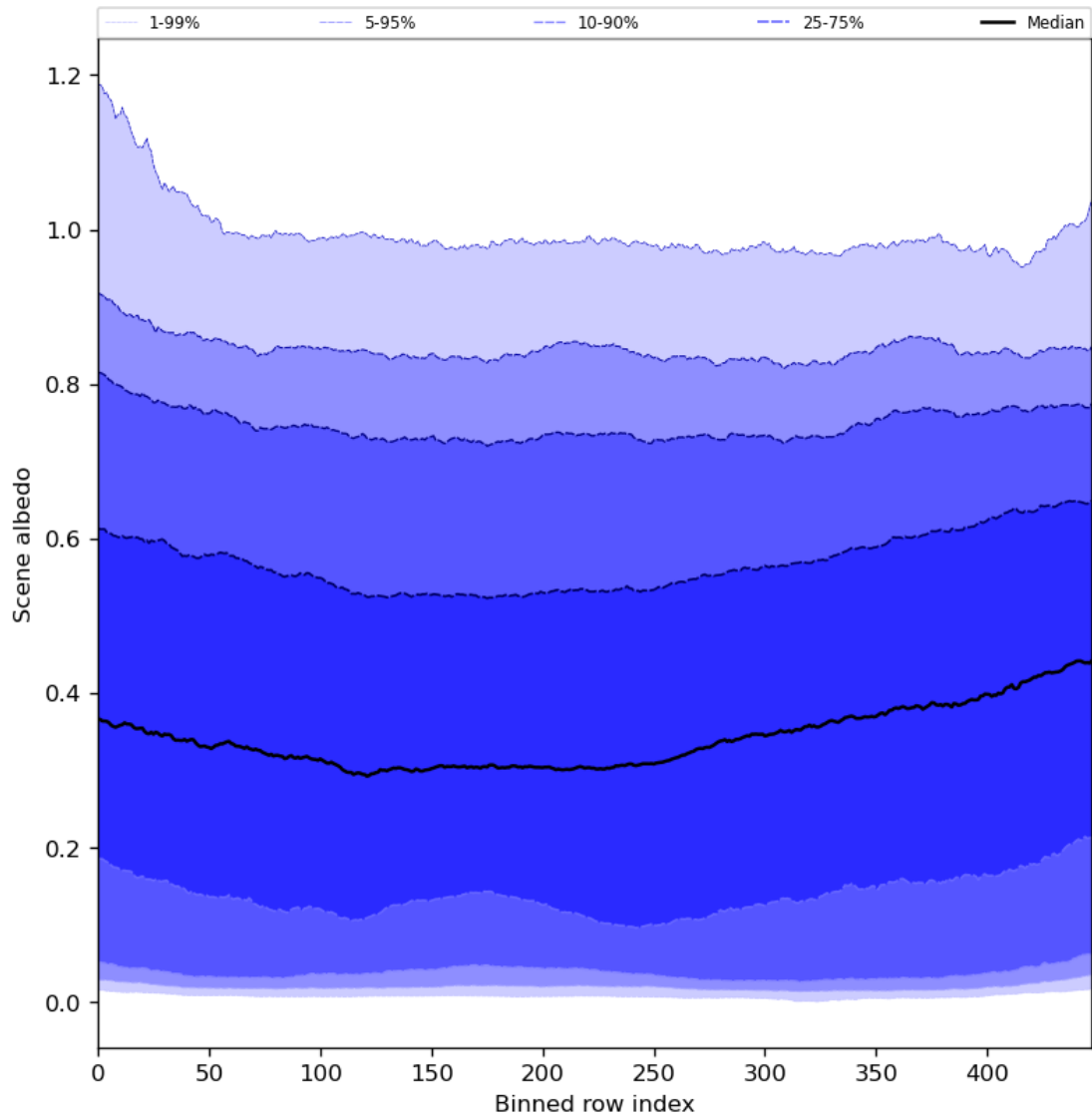
Figure 51: Along track statistics of “Scene albedo” for 2024-07-15 to 2024-07-16
