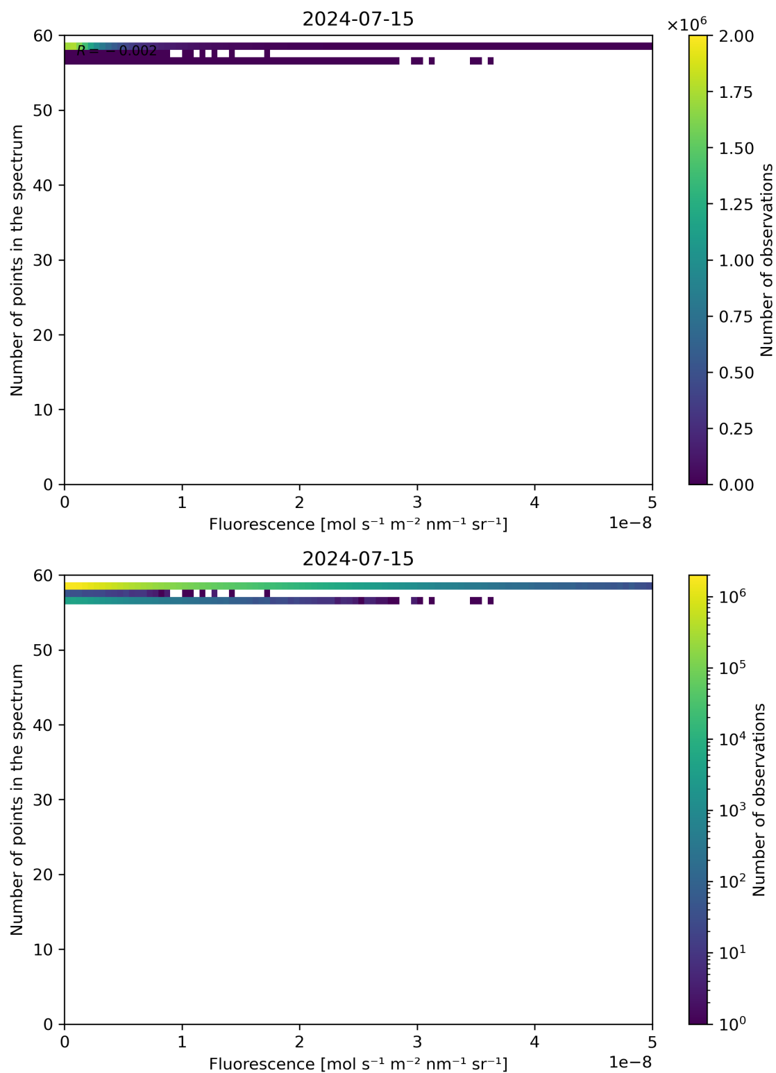
Figure 86: Scatter density plot of “Fluorescence” against “Number of points in the spectrum” for 2024-07-15 to 2024-07-16.
