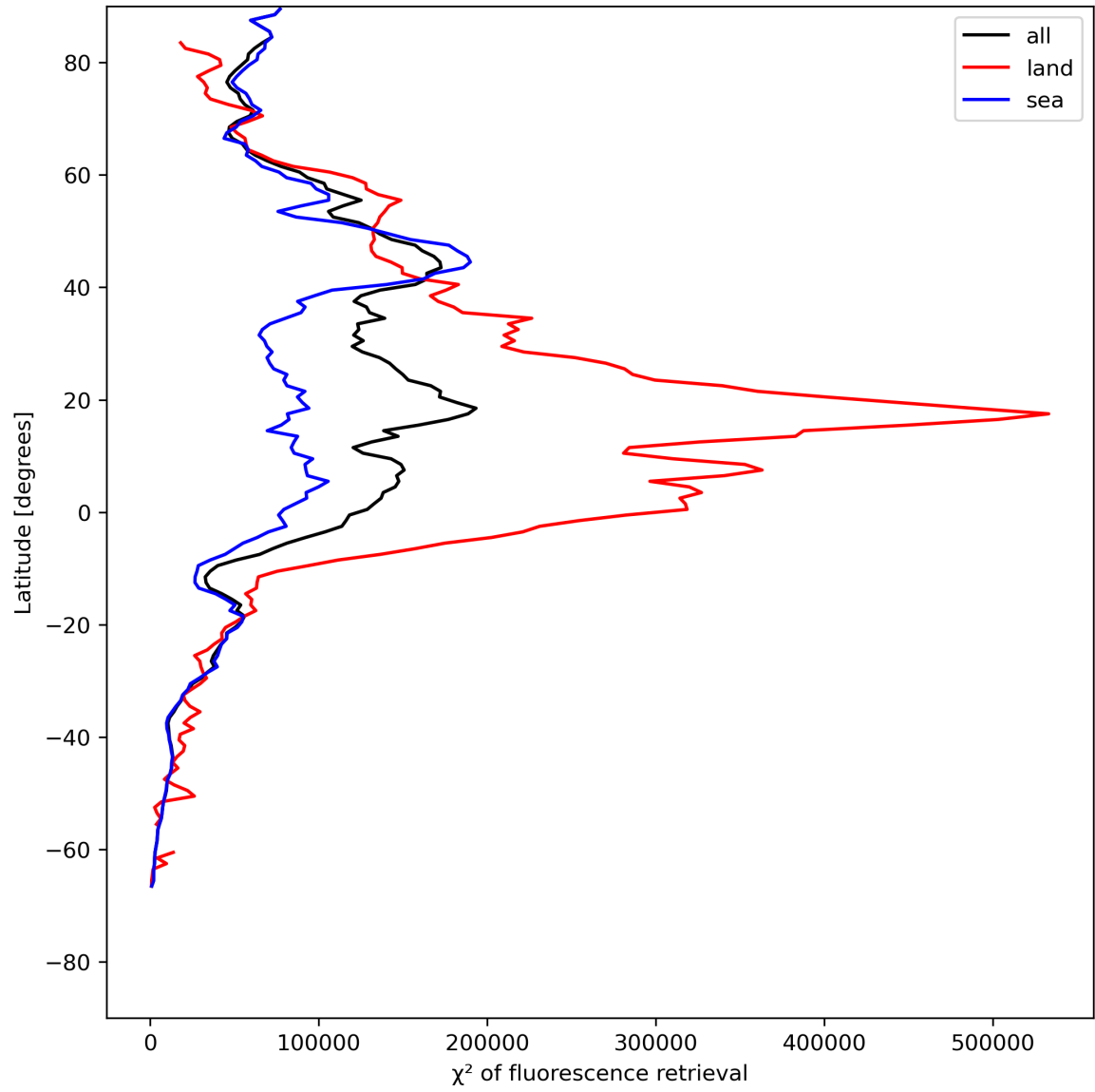
Figure 25: Zonal average of “ \chi^2 of fluorescence retrieval” for 2024-07-15 to 2024-07-16.
