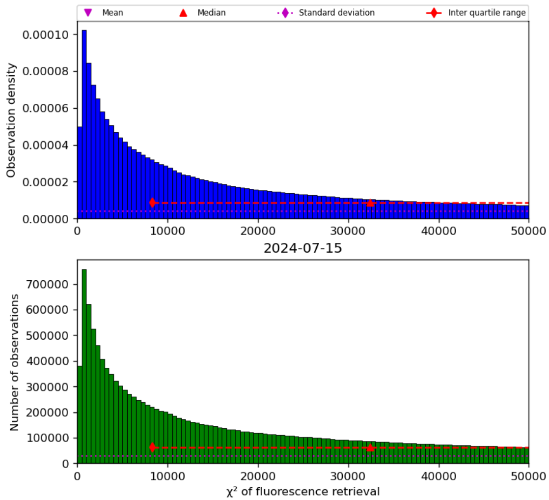
Figure 42: Histogram of “ \chi^2 of fluorescence retrieval” for 2024-07-15 to 2024-07-16
