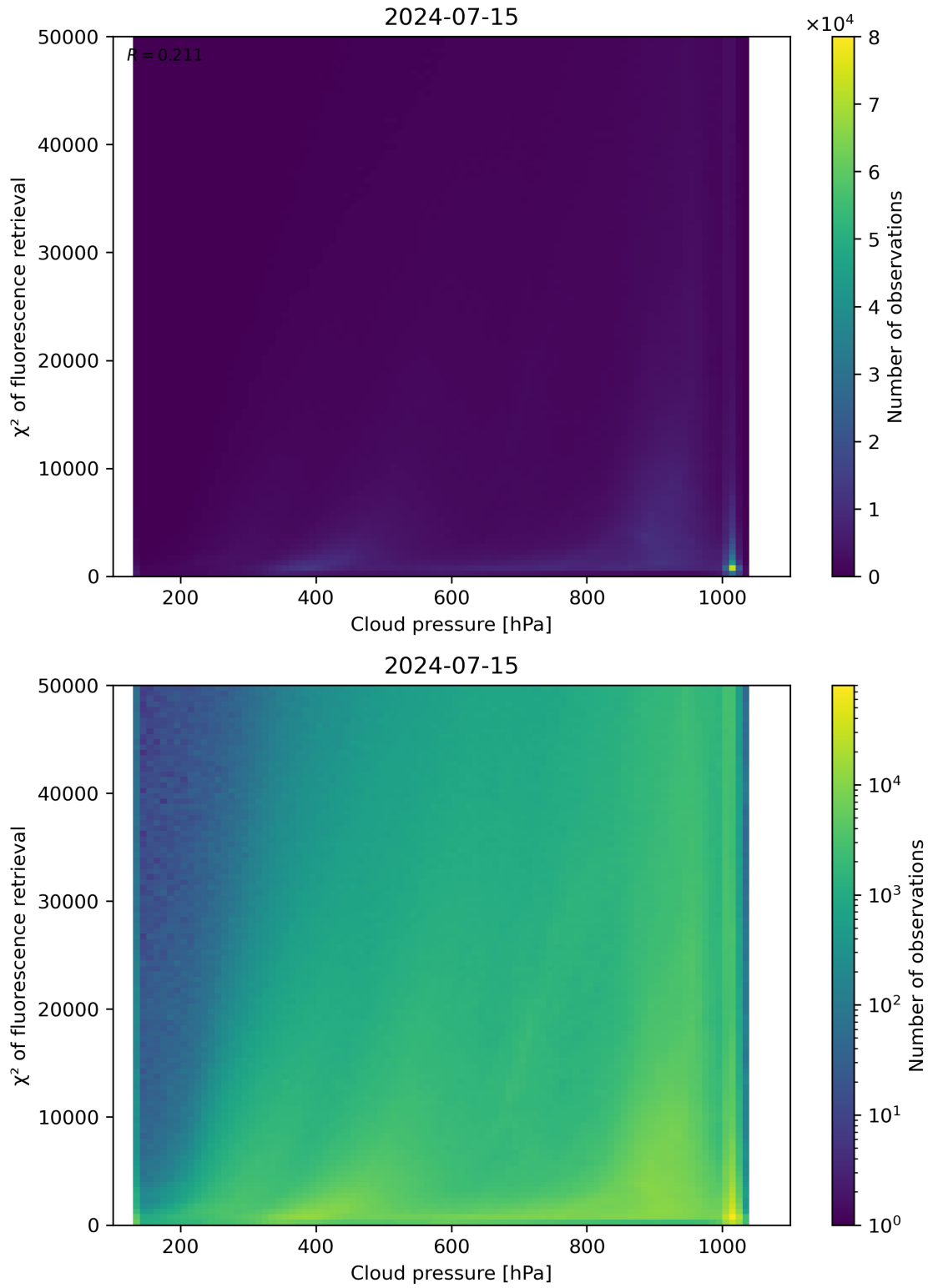
Figure 78: Scatter density plot of “Cloud pressure” against “ \chi^2 of fluorescence retrieval” for 2024-07-15 to 2024-07-16.
