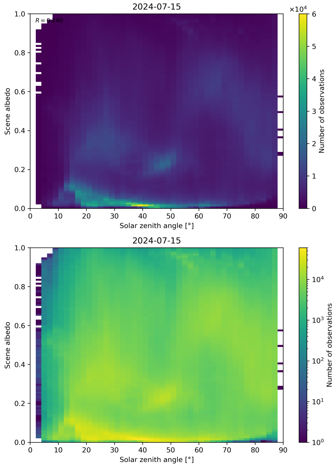
Figure 116: Scatter density plot of “Solar zenith angle” against “Scene albedo” for 2024-07-15 to 2024-07-16.
