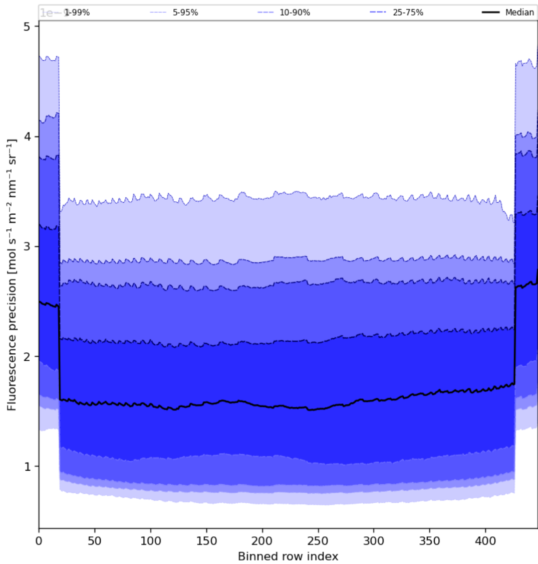
Figure 58: Along track statistics of “Fluorescence precision” for 2024-07-15 to 2024-07-16
