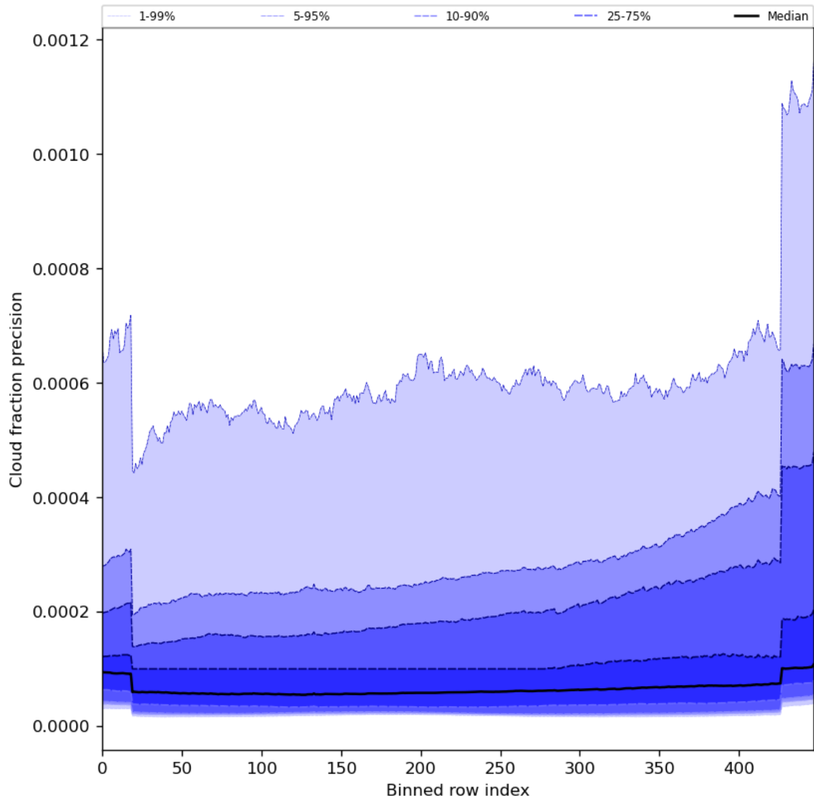
Figure 50: Along track statistics of “Cloud fraction precision” for 2024-07-15 to 2024-07-16
