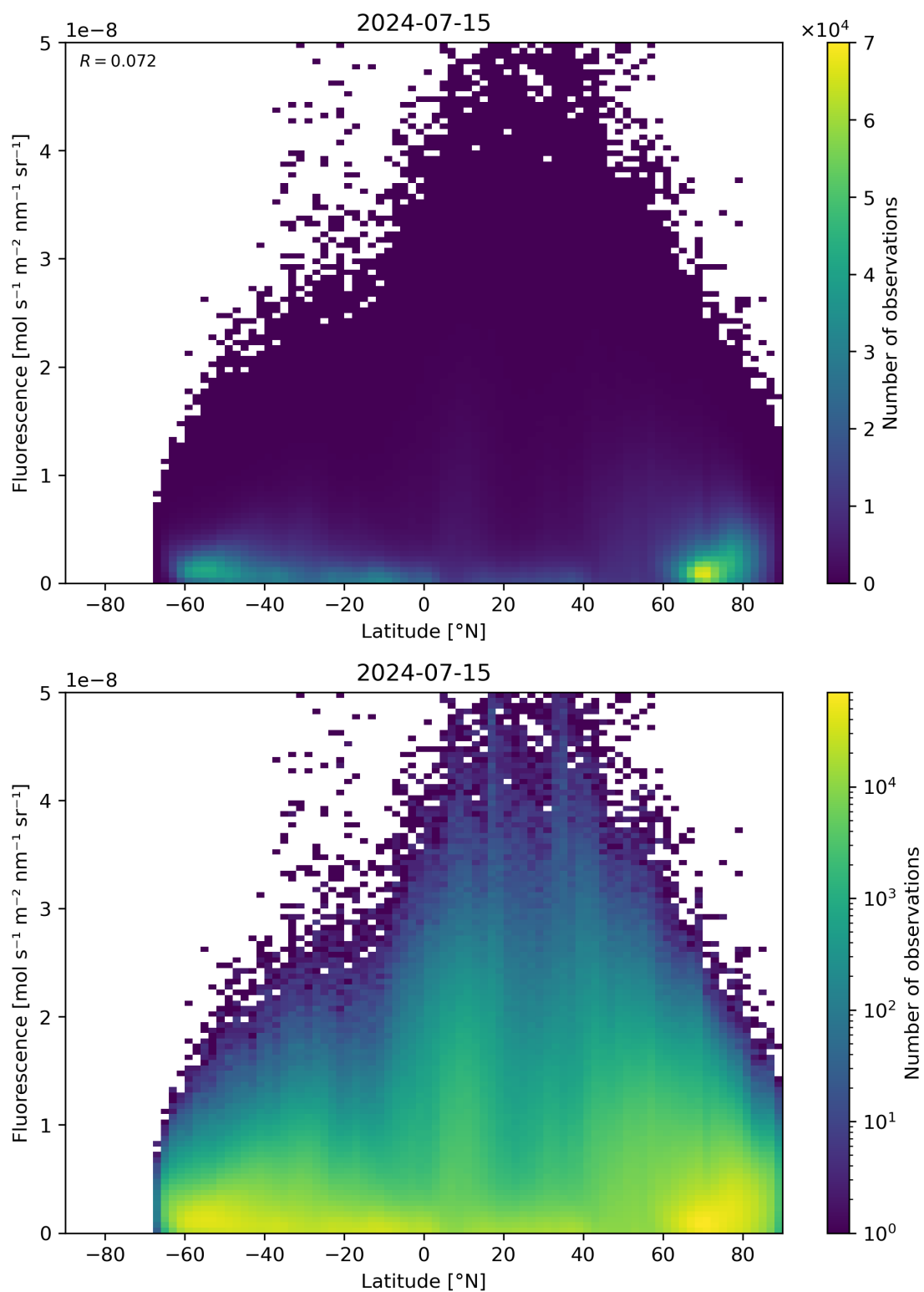
Figure 92: Scatter density plot of “Latitude” against “Fluorescence” for 2024-07-15 to 2024-07-16.
