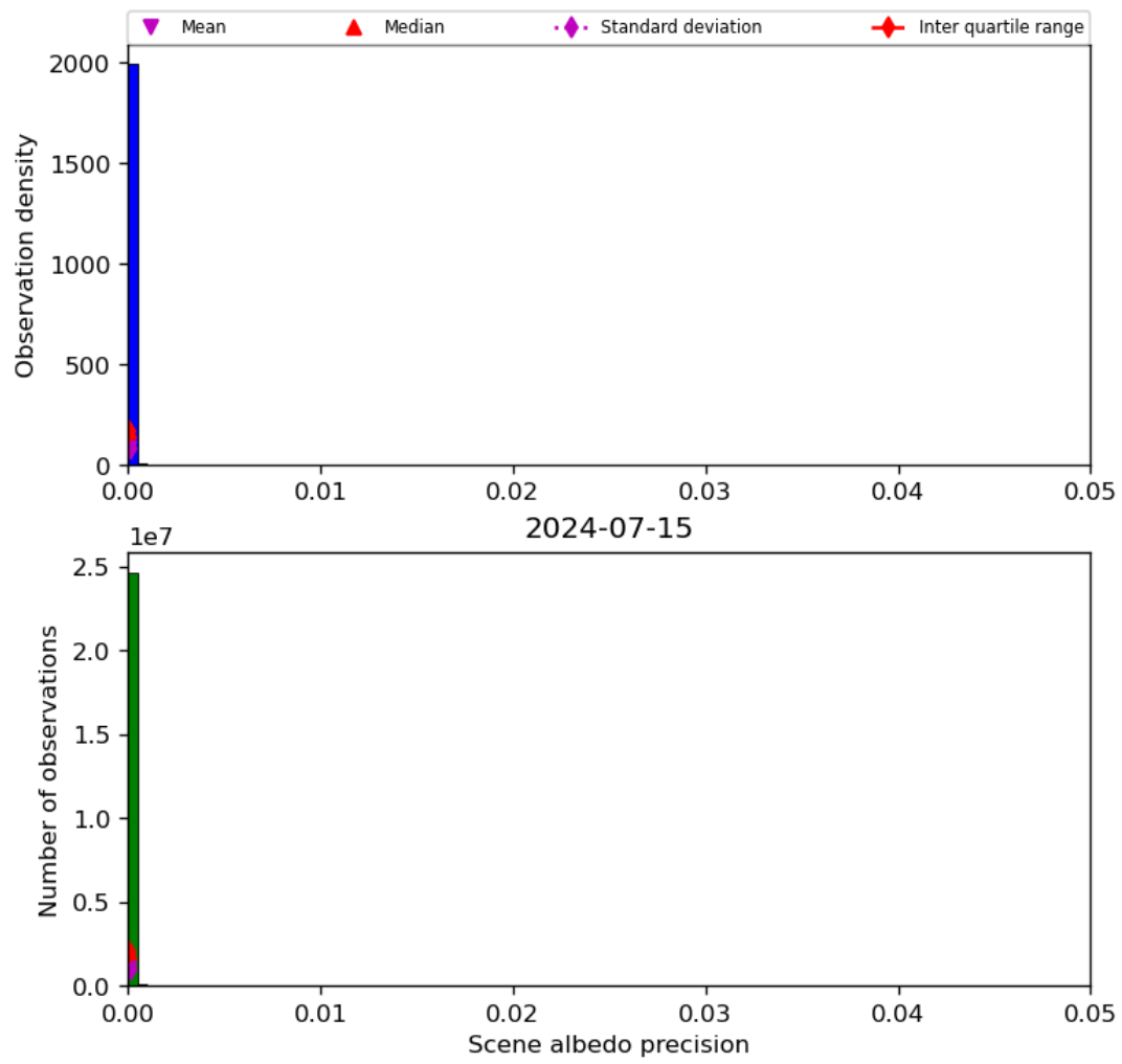
Figure 35: Histogram of “Scene albedo precision” for 2024-07-15 to 2024-07-16
