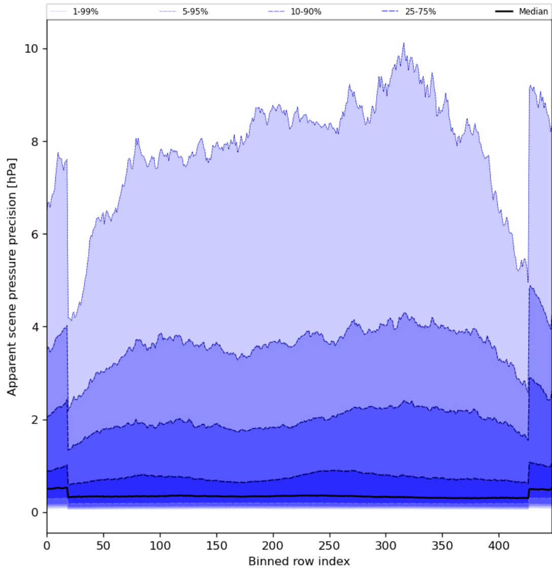
Figure 54: Along track statistics of “Apparent scene pressure precision” for 2024-07-15 to 2024-07-16
