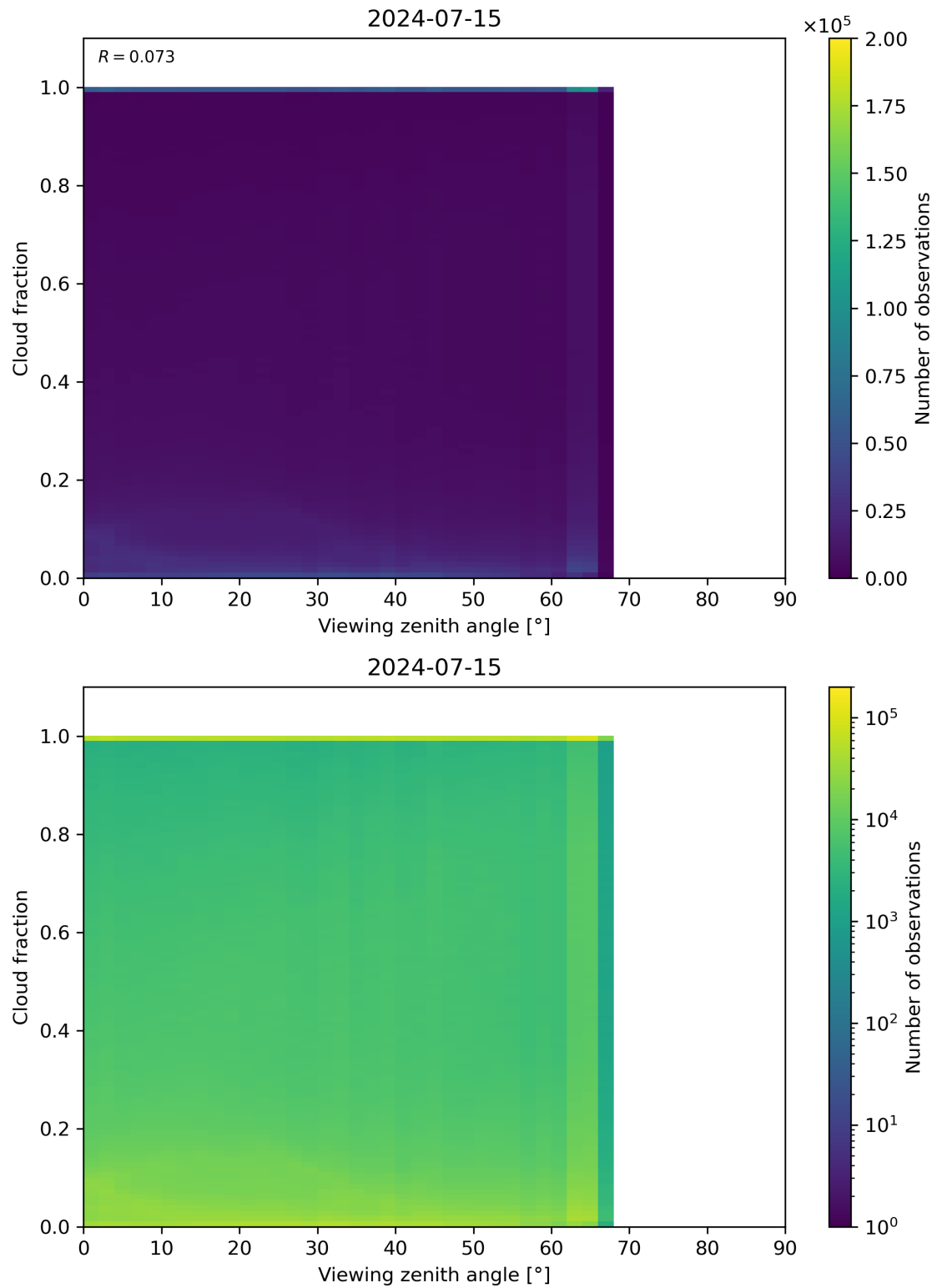
Figure 120: Scatter density plot of “Viewing zenith angle” against “Cloud fraction” for 2024-07-15 to 2024-07-16.
