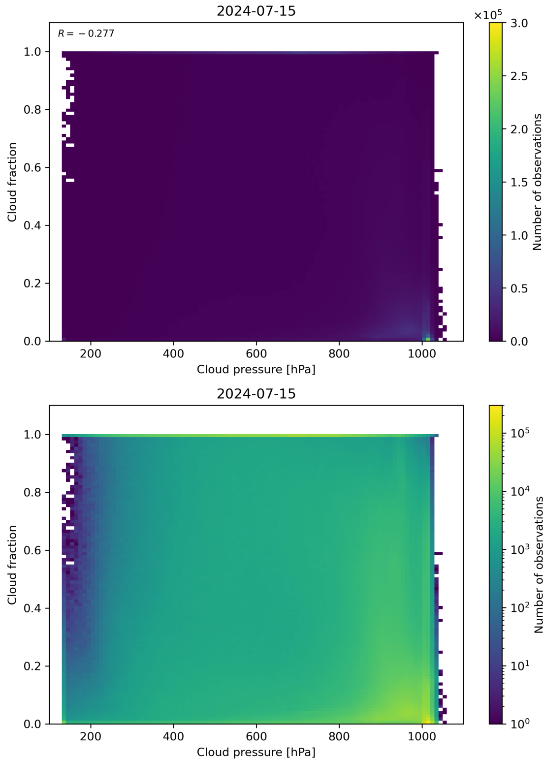
Figure 79: Scatter density plot of “Cloud pressure” against “Cloud fraction” for 2024-07-15 to 2024-07-16.
