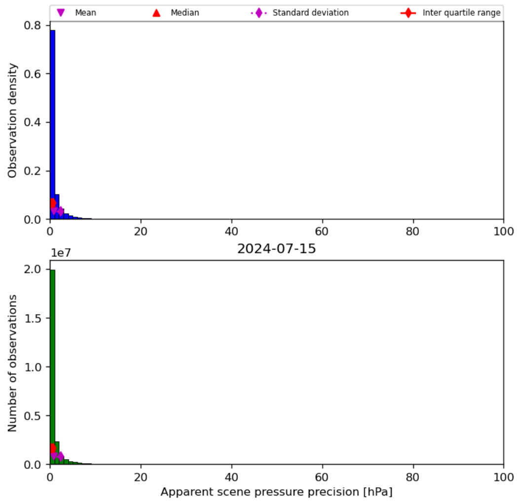
Figure 37: Histogram of “Apparent scene pressure precision” for 2024-07-15 to 2024-07-16
