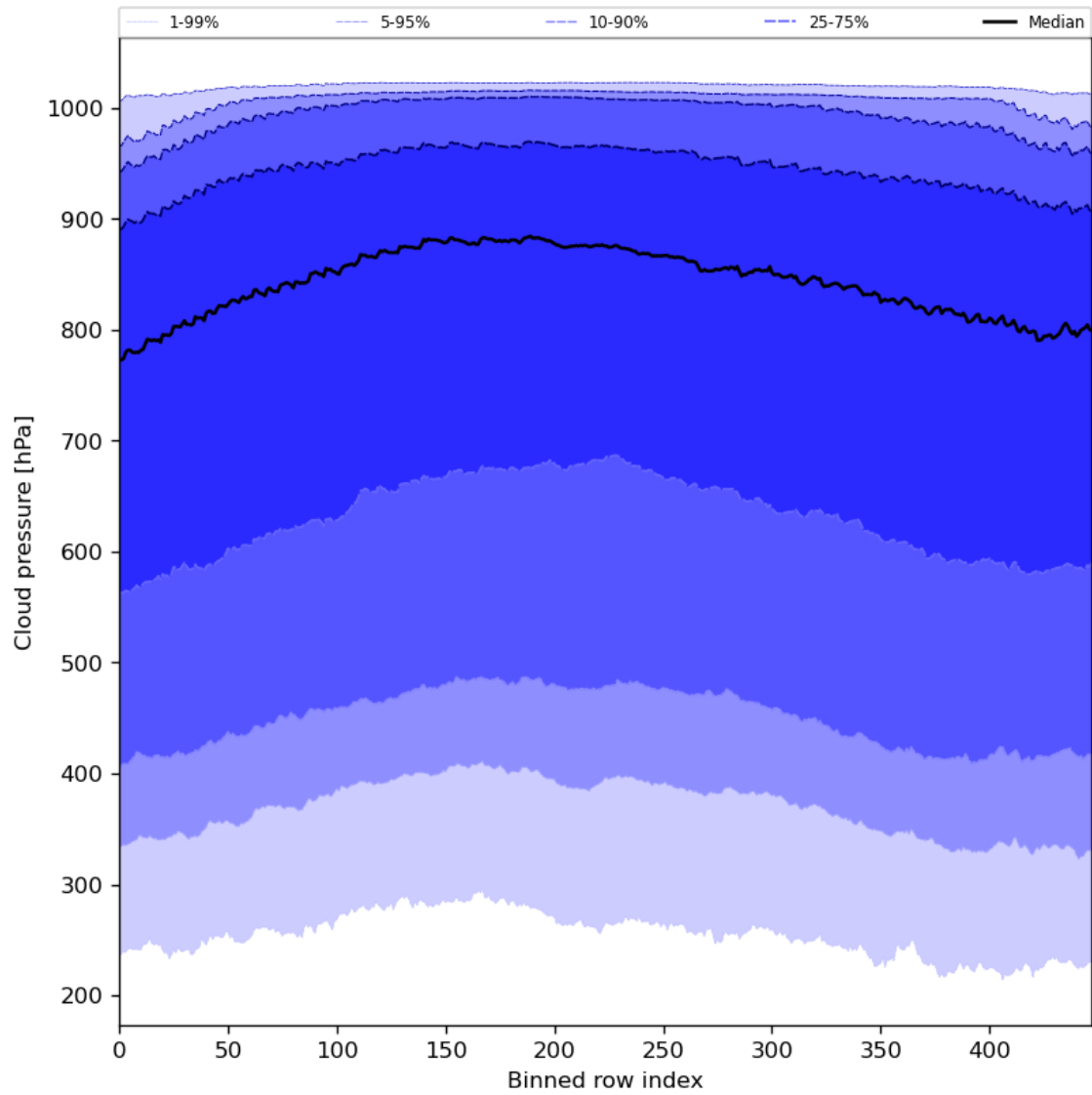
Figure 47: Along track statistics of “Cloud pressure” for 2024-07-15 to 2024-07-16
