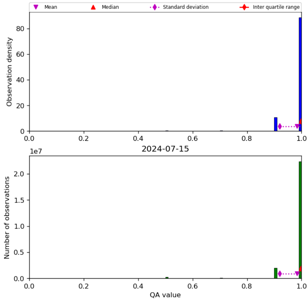
Figure 29: Histogram of “QA value” for 2024-07-15 to 2024-07-16
