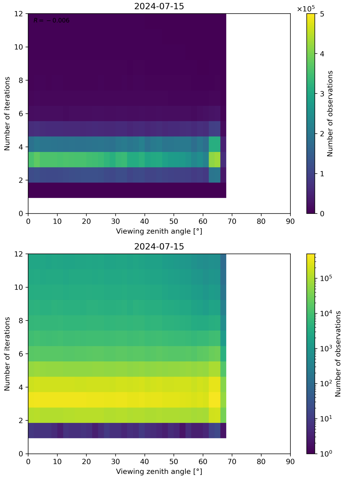
Figure 124: Scatter density plot of “Viewing zenith angle” against “Number of iterations” for 2024-07-15 to 2024-07-16.
