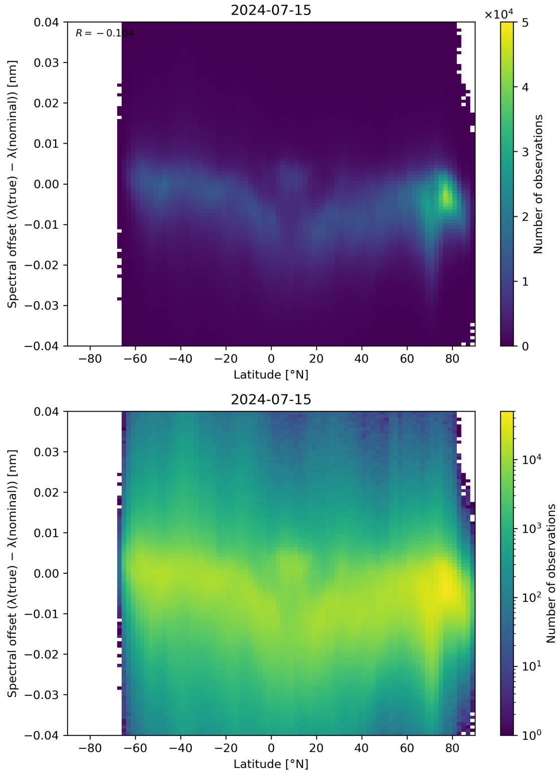
Figure 96: Scatter density plot of “Latitude” against “Spectral offset ( \lambda(\text{true}) - \lambda(\text{nominal}) )” for 2024-07-15 to 2024-07-16.
