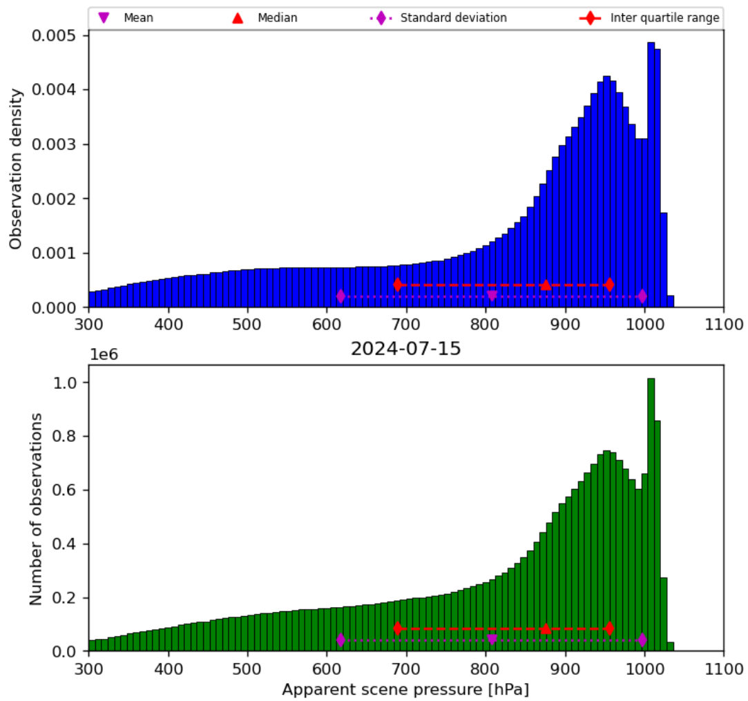
Figure 36: Histogram of “Apparent scene pressure” for 2024-07-15 to 2024-07-16
