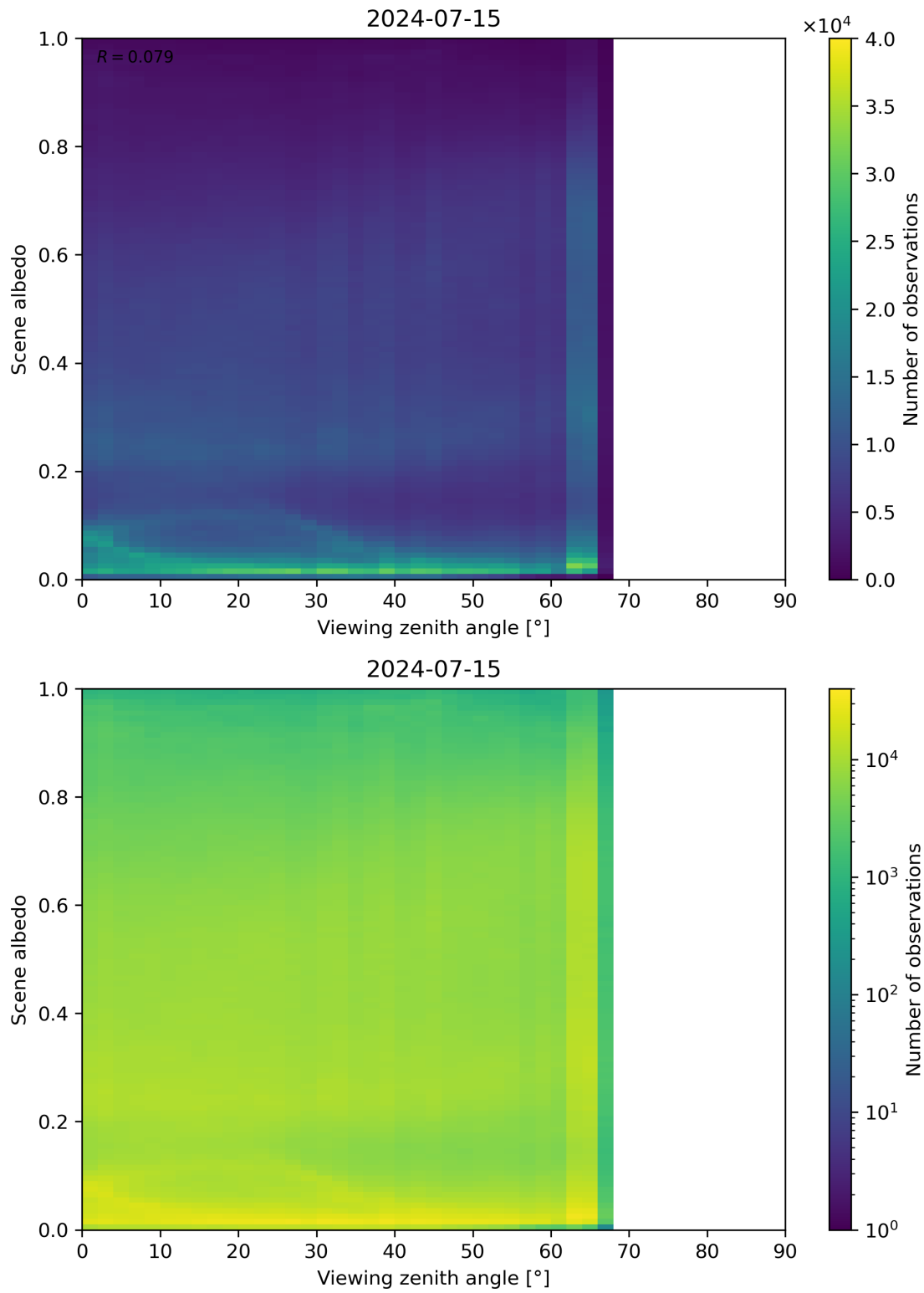
Figure 126: Scatter density plot of “Viewing zenith angle” against “Scene albedo” for 2024-07-15 to 2024-07-16.
