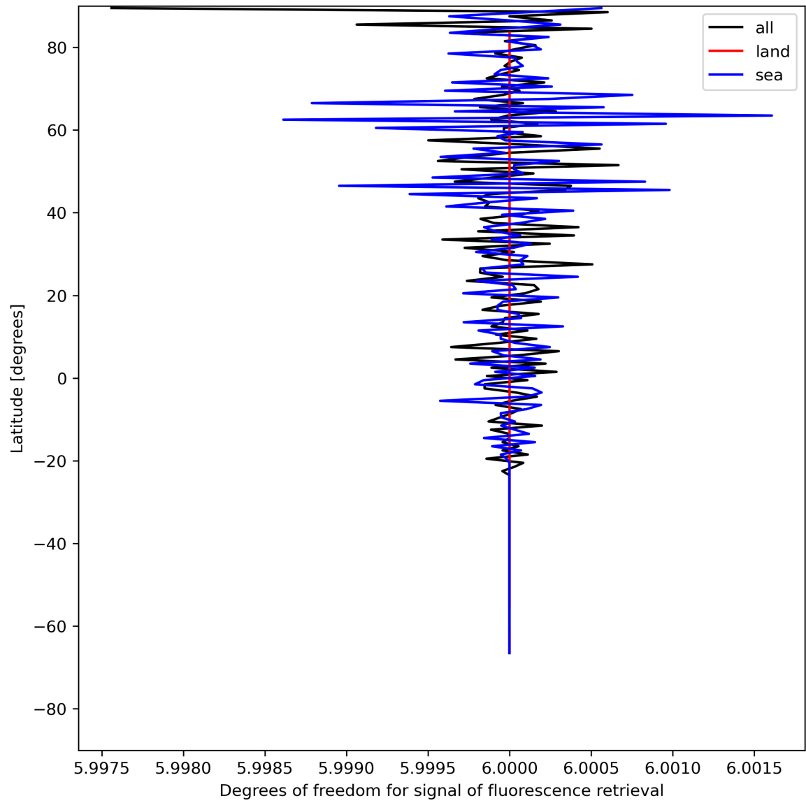
Figure 26: Zonal average of “Degrees of freedom for signal of fluorescence retrieval” for 2024-07-15 to 2024-07-16.
