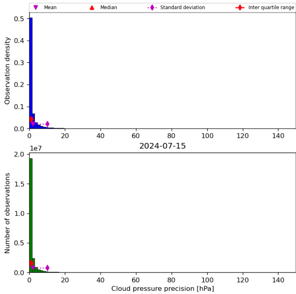
Figure 31: Histogram of “Cloud pressure precision” for 2024-07-15 to 2024-07-16
