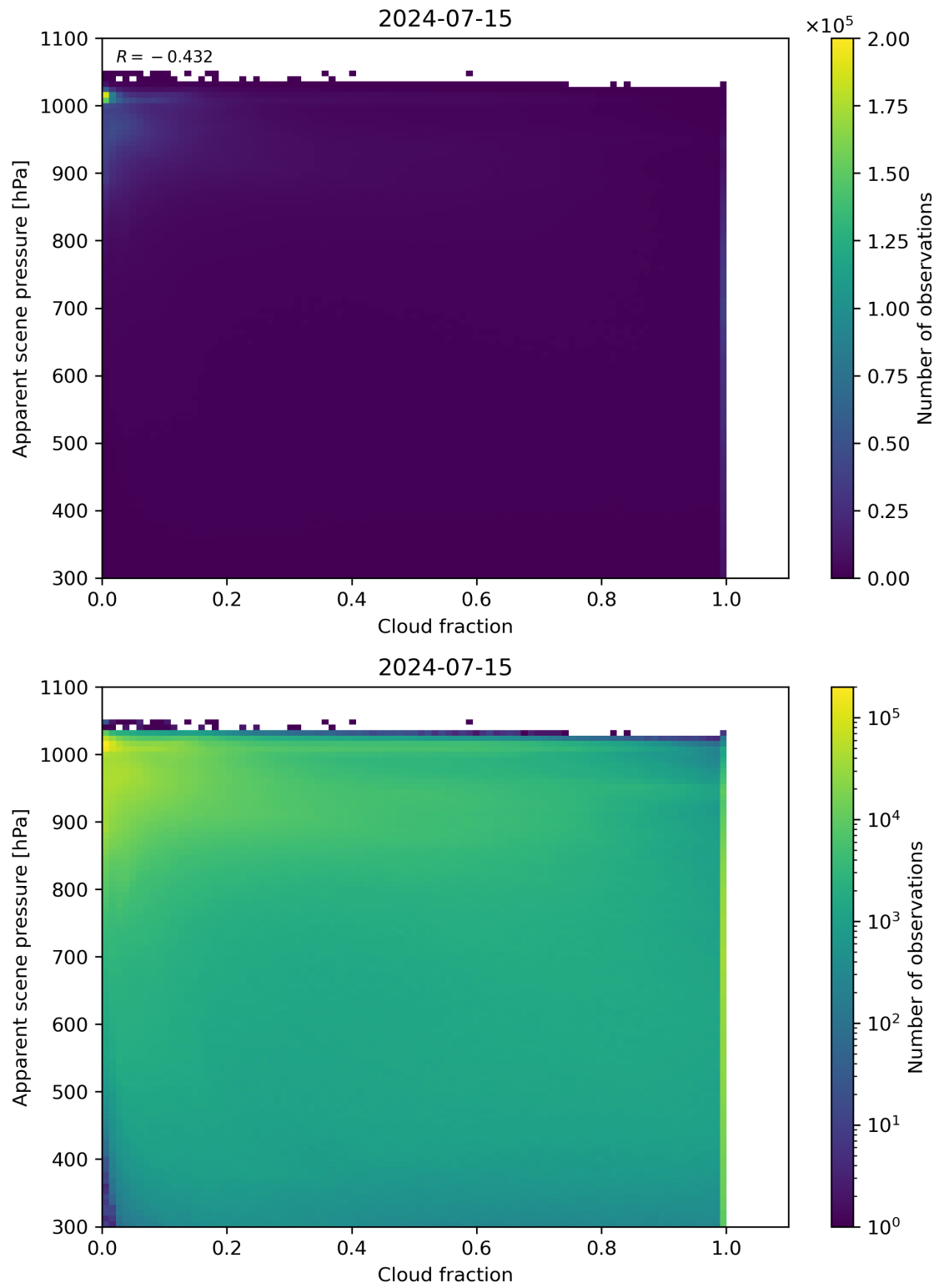
Figure 70: Scatter density plot of “Cloud fraction” against “Apparent scene pressure” for 2024-07-15 to 2024-07-16.
