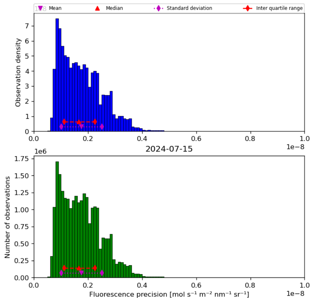
Figure 41: Histogram of “Fluorescence precision” for 2024-07-15 to 2024-07-16
