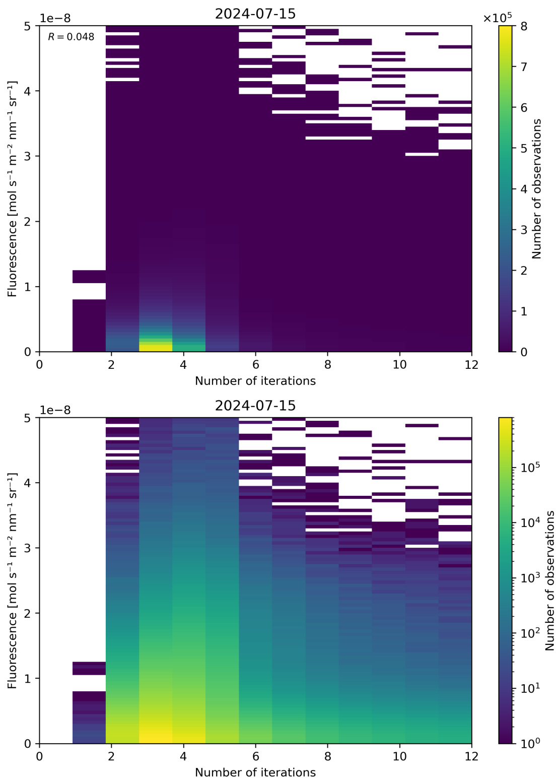
Figure 98: Scatter density plot of “Number of iterations” against “Fluorescence” for 2024-07-15 to 2024-07-16.
