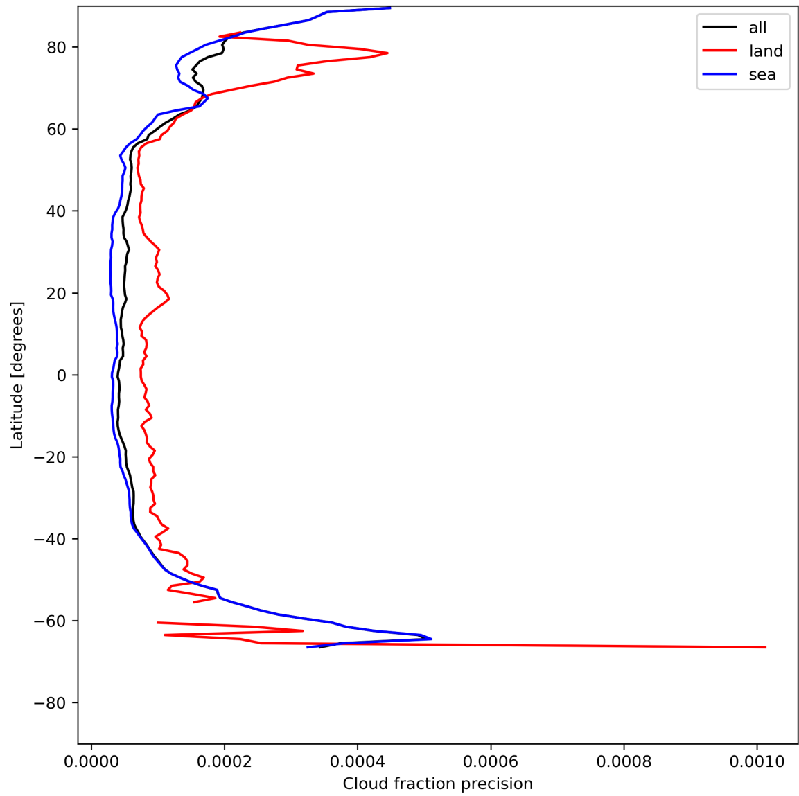
Figure 16: Zonal average of “Cloud fraction precision” for 2024-07-15 to 2024-07-16.
