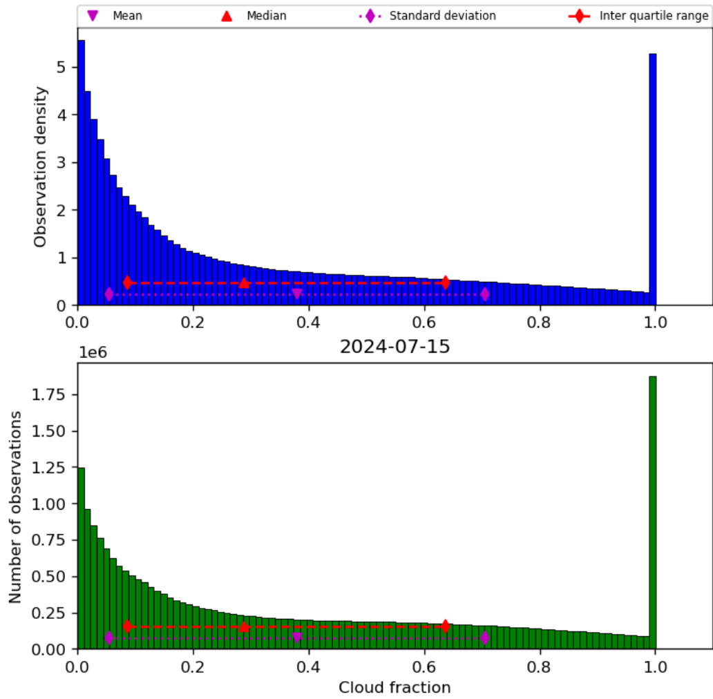
Figure 32: Histogram of “Cloud fraction” for 2024-07-15 to 2024-07-16
