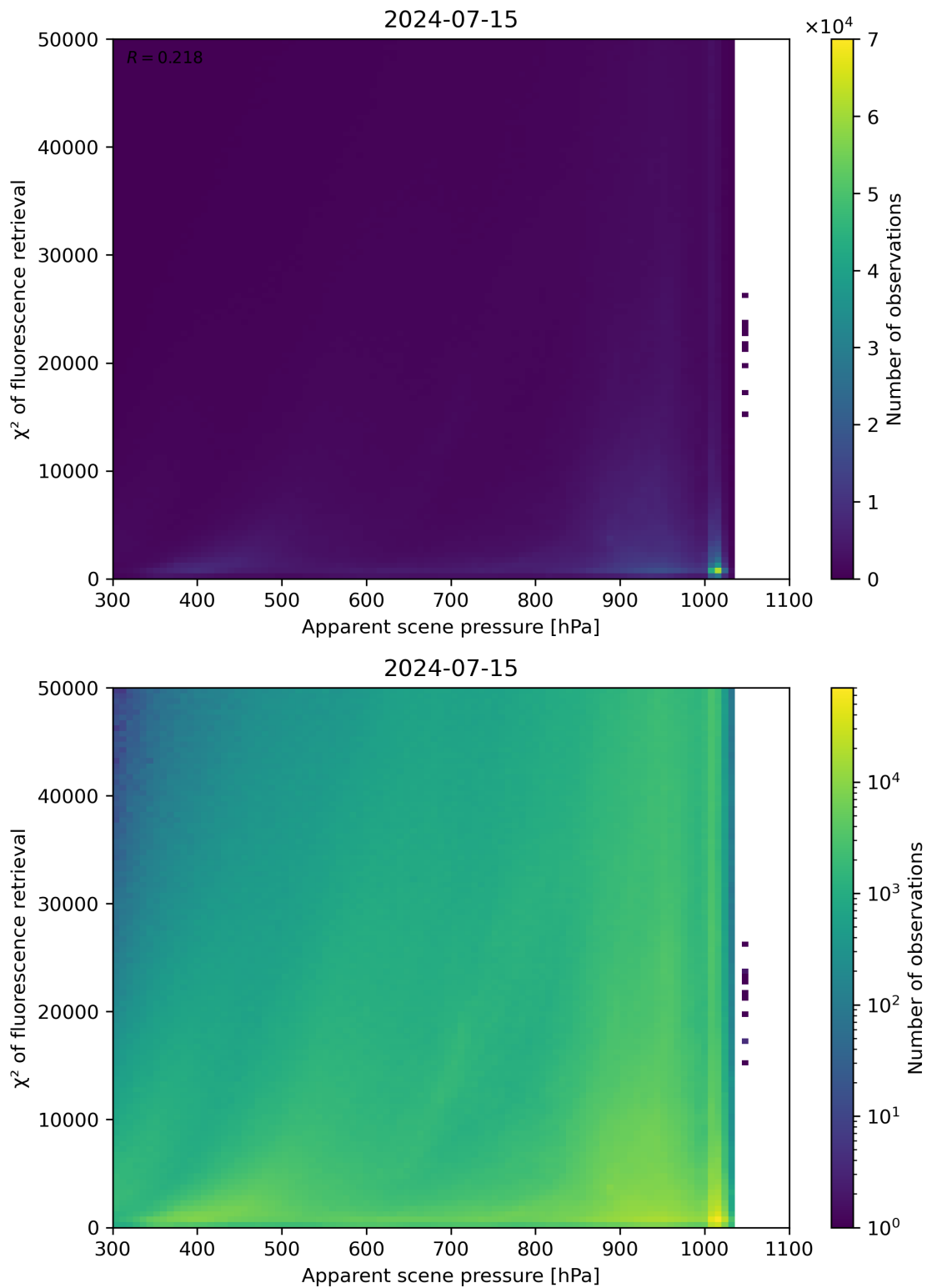
Figure 63: Scatter density plot of “Apparent scene pressure” against “ \chi^2 of fluorescence retrieval” for 2024-07-15 to 2024-07-16.
