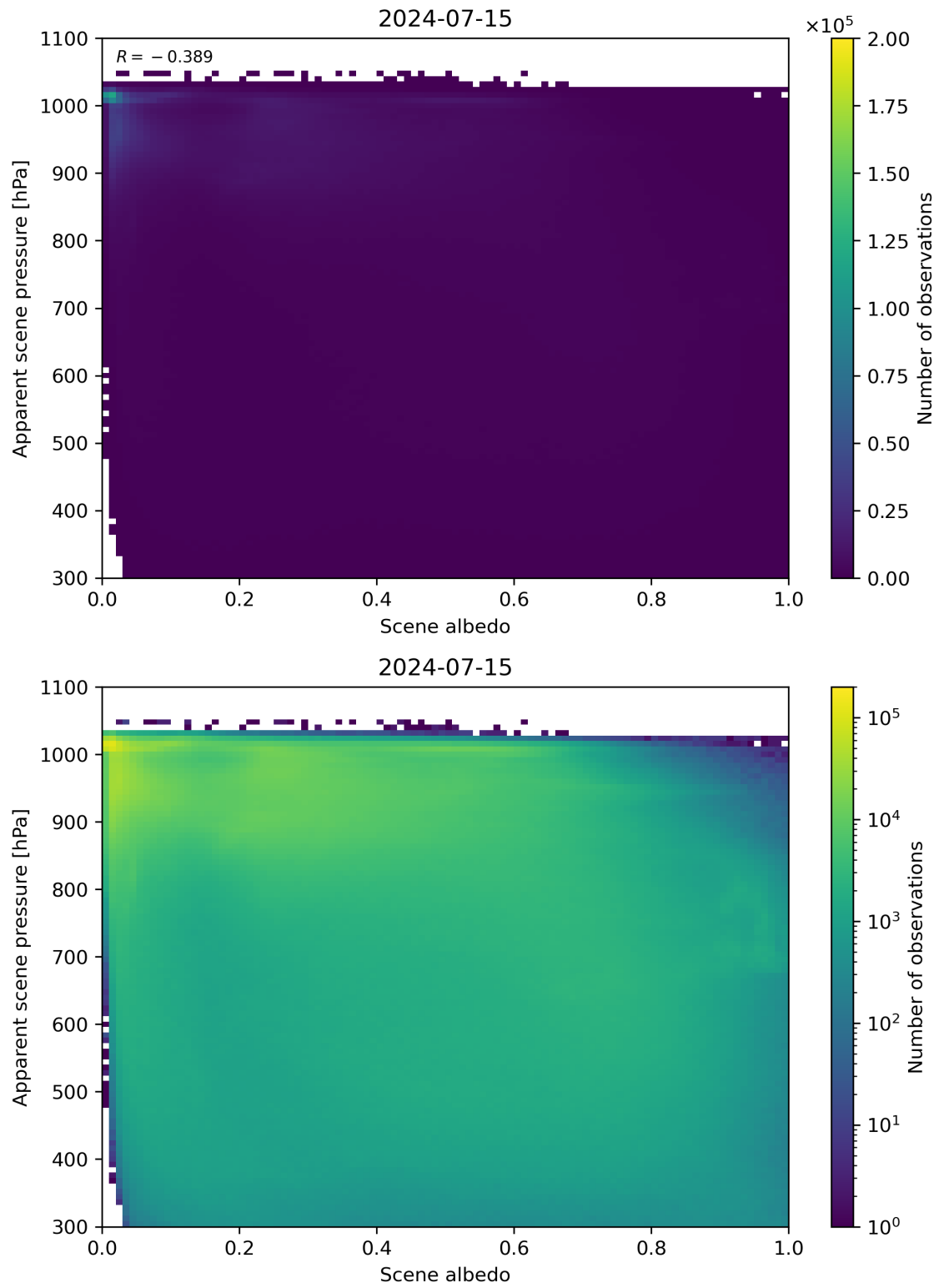
Figure 102: Scatter density plot of “Scene albedo” against “Apparent scene pressure” for 2024-07-15 to 2024-07-16.
