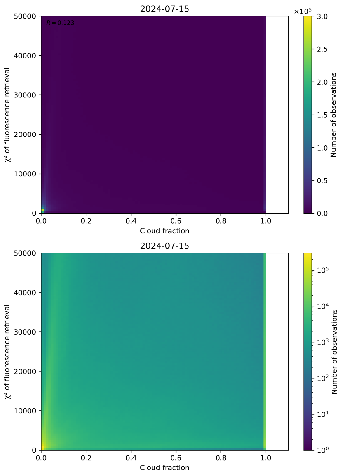
Figure 71: Scatter density plot of “Cloud fraction” against “ \chi^2 of fluorescence retrieval” for 2024-07-15 to 2024-07-16.
