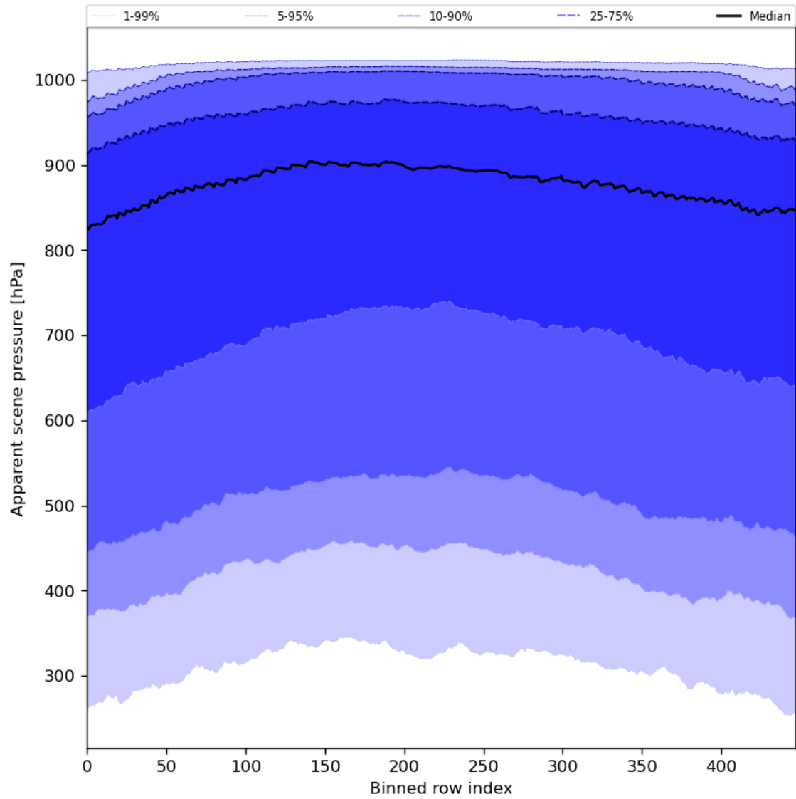
Figure 53: Along track statistics of “Apparent scene pressure” for 2024-07-15 to 2024-07-16
