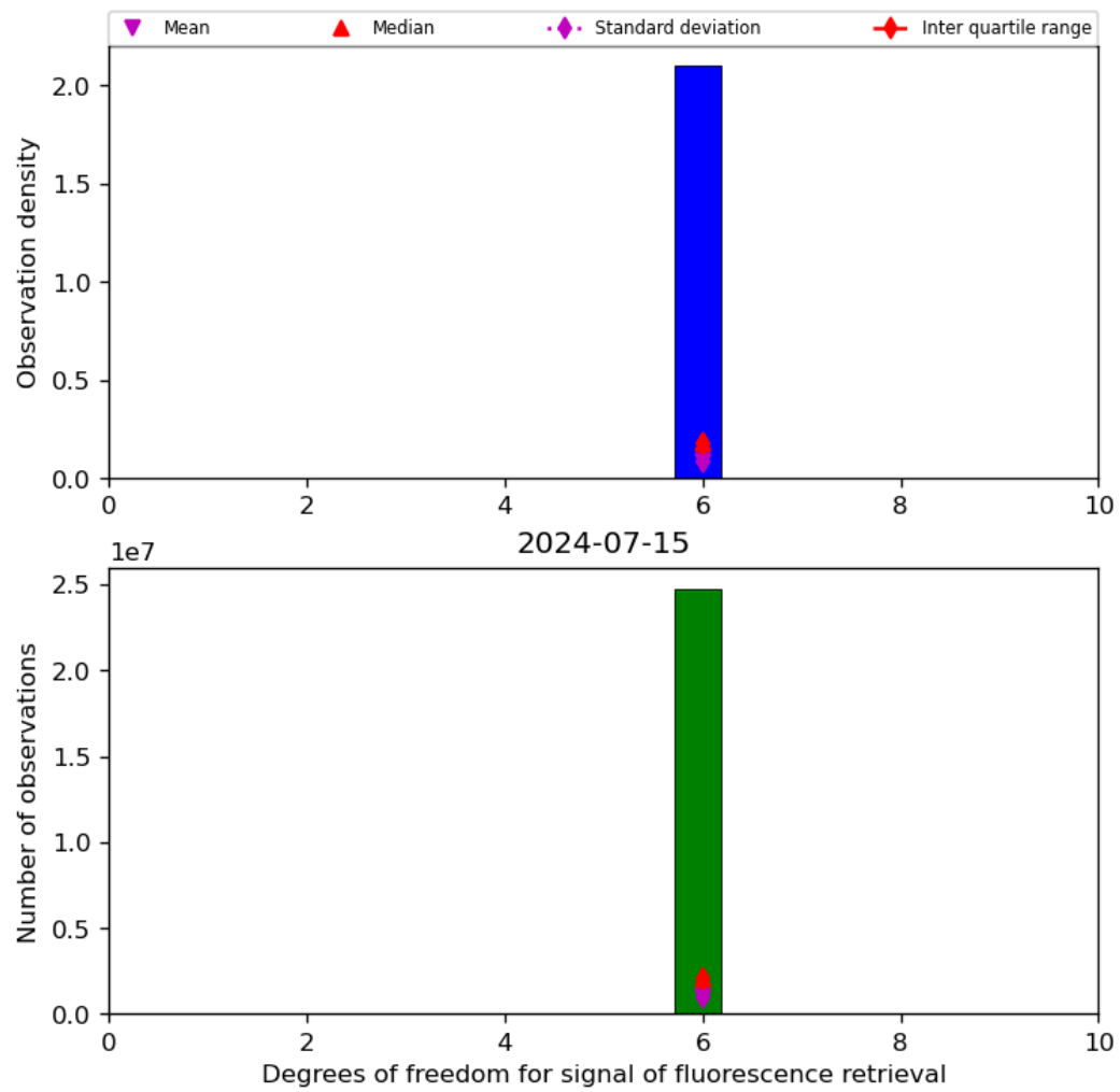
Figure 43: Histogram of “Degrees of freedom for signal of fluorescence retrieval” for 2024-07-15 to 2024-07-16
