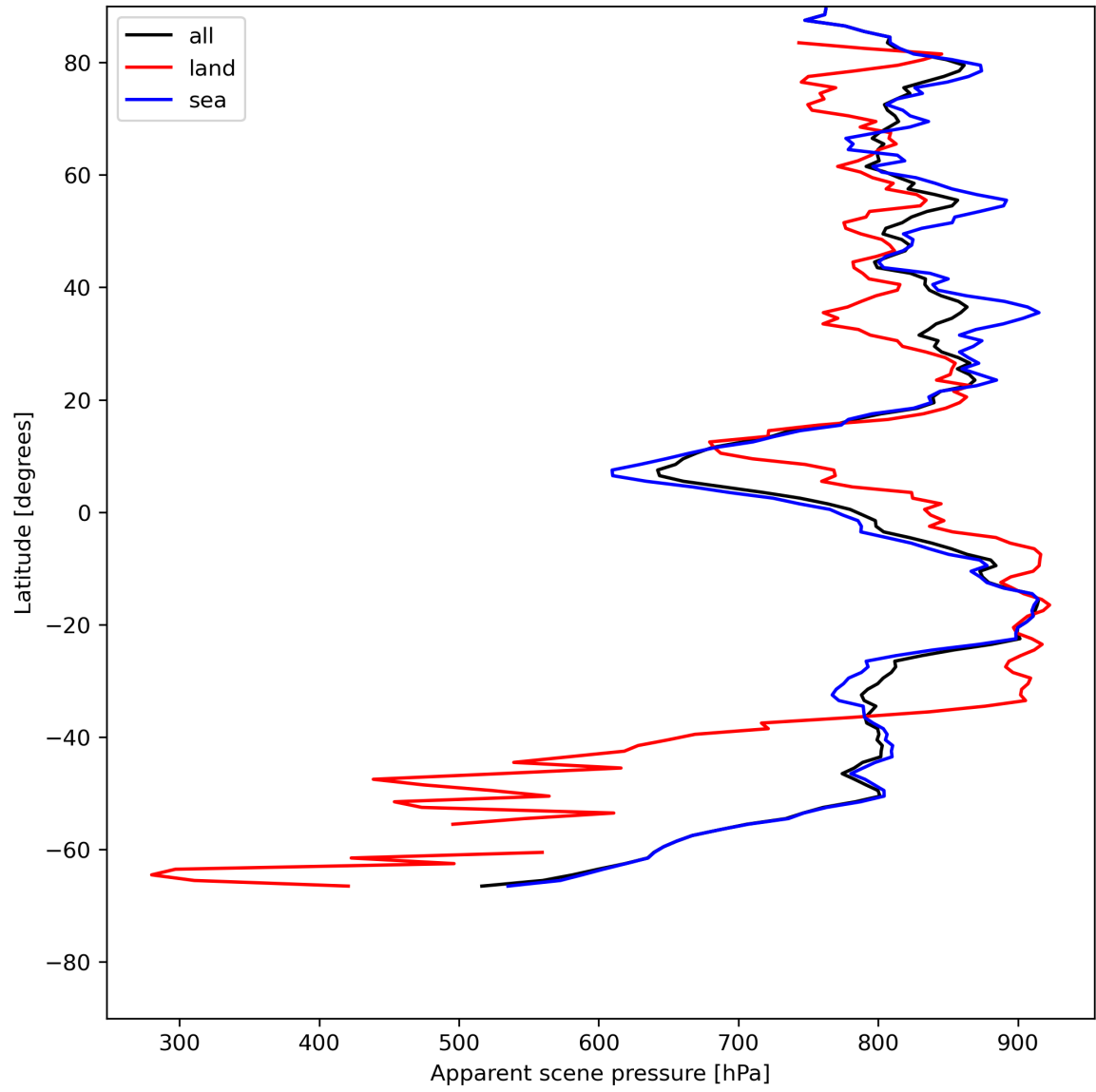
Figure 19: Zonal average of “Apparent scene pressure” for 2024-07-15 to 2024-07-16.
