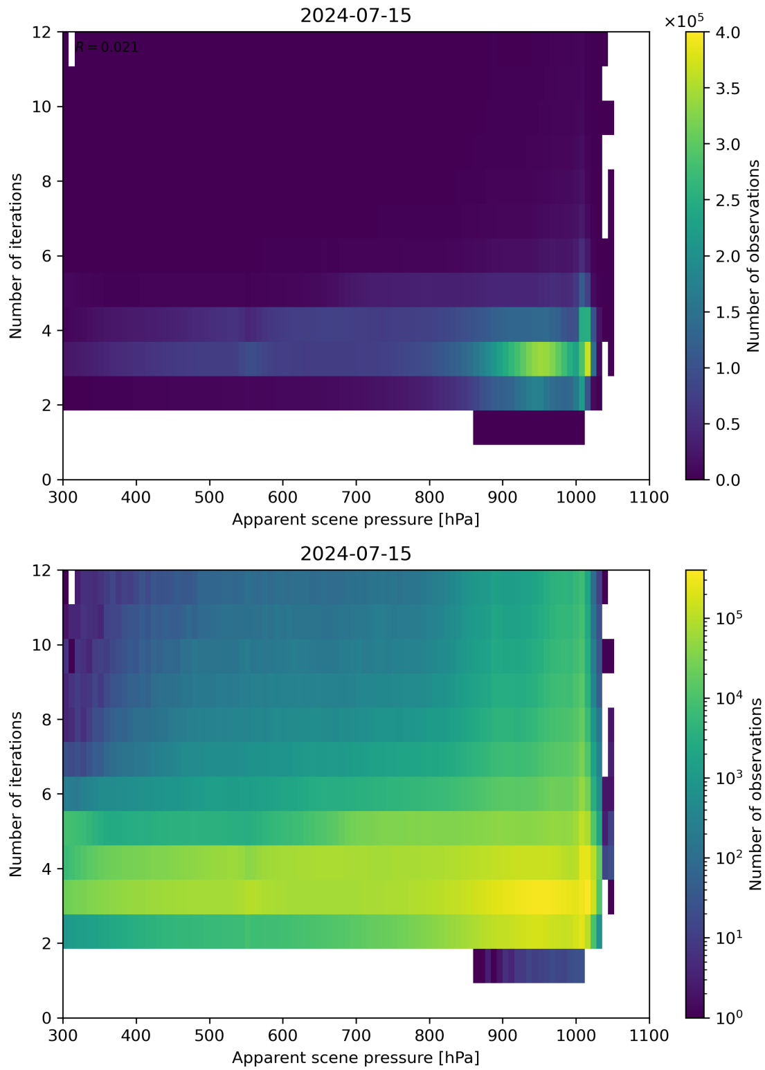
Figure 65: Scatter density plot of “Apparent scene pressure” against “Number of iterations” for 2024-07-15 to 2024-07-16.
