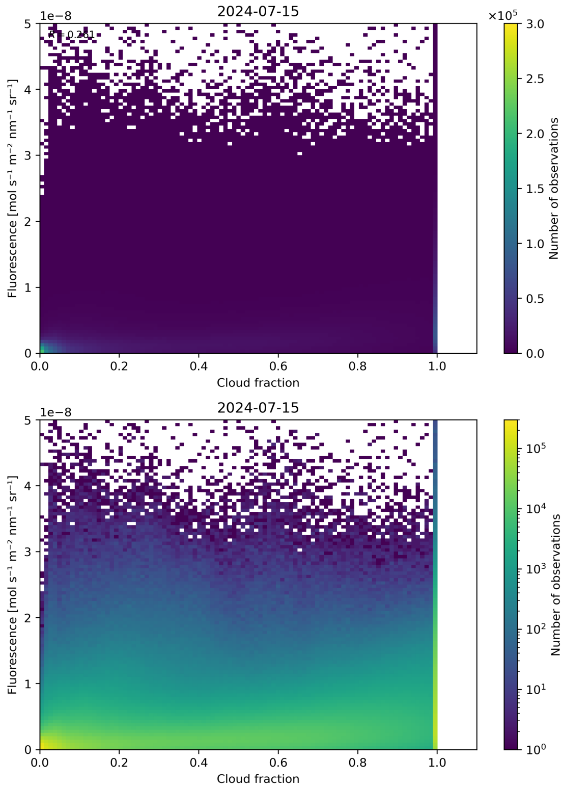
Figure 72: Scatter density plot of “Cloud fraction” against “Fluorescence” for 2024-07-15 to 2024-07-16.
