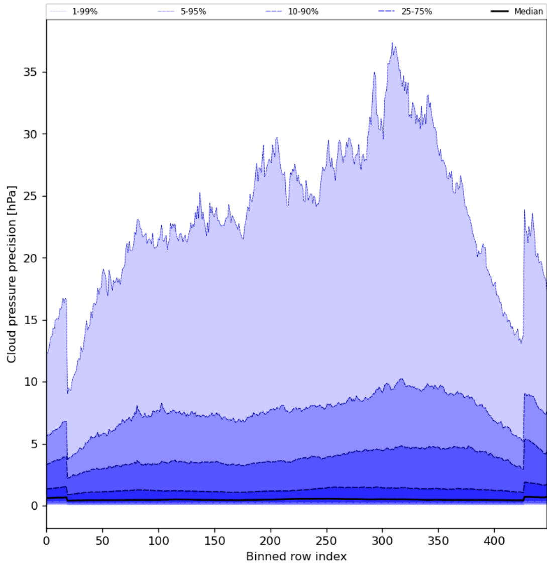
Figure 48: Along track statistics of “Cloud pressure precision” for 2024-07-15 to 2024-07-16
