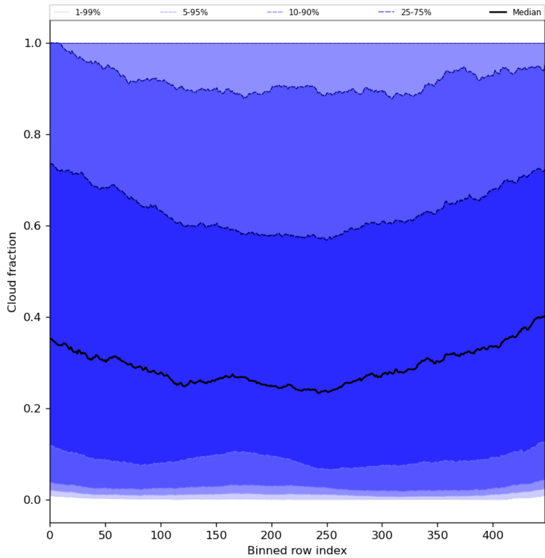
Figure 49: Along track statistics of “Cloud fraction” for 2024-07-15 to 2024-07-16
