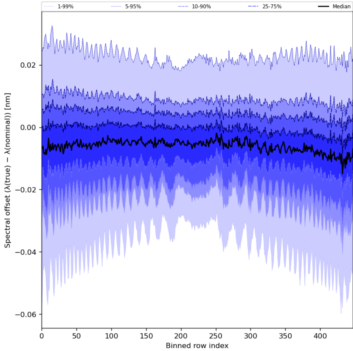
Figure 62: Along track statistics of “Spectral offset ( \lambda(\text{true}) - \lambda(\text{nominal}) )” for 2024-07-15 to 2024-07-16
