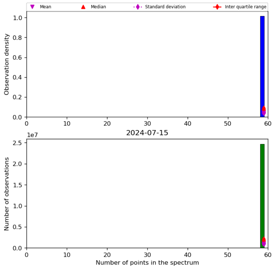
Figure 44: Histogram of “Number of points in the spectrum” for 2024-07-15 to 2024-07-16
