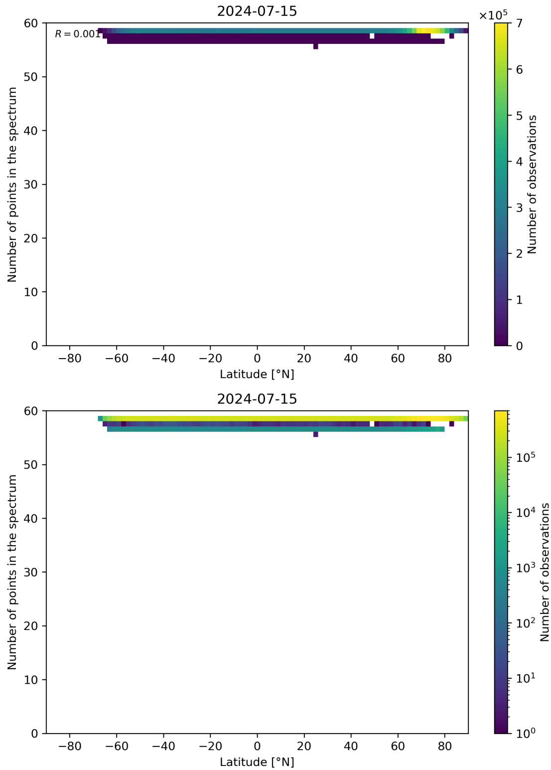
Figure 94: Scatter density plot of “Latitude” against “Number of points in the spectrum” for 2024-07-15 to 2024-07-16.
