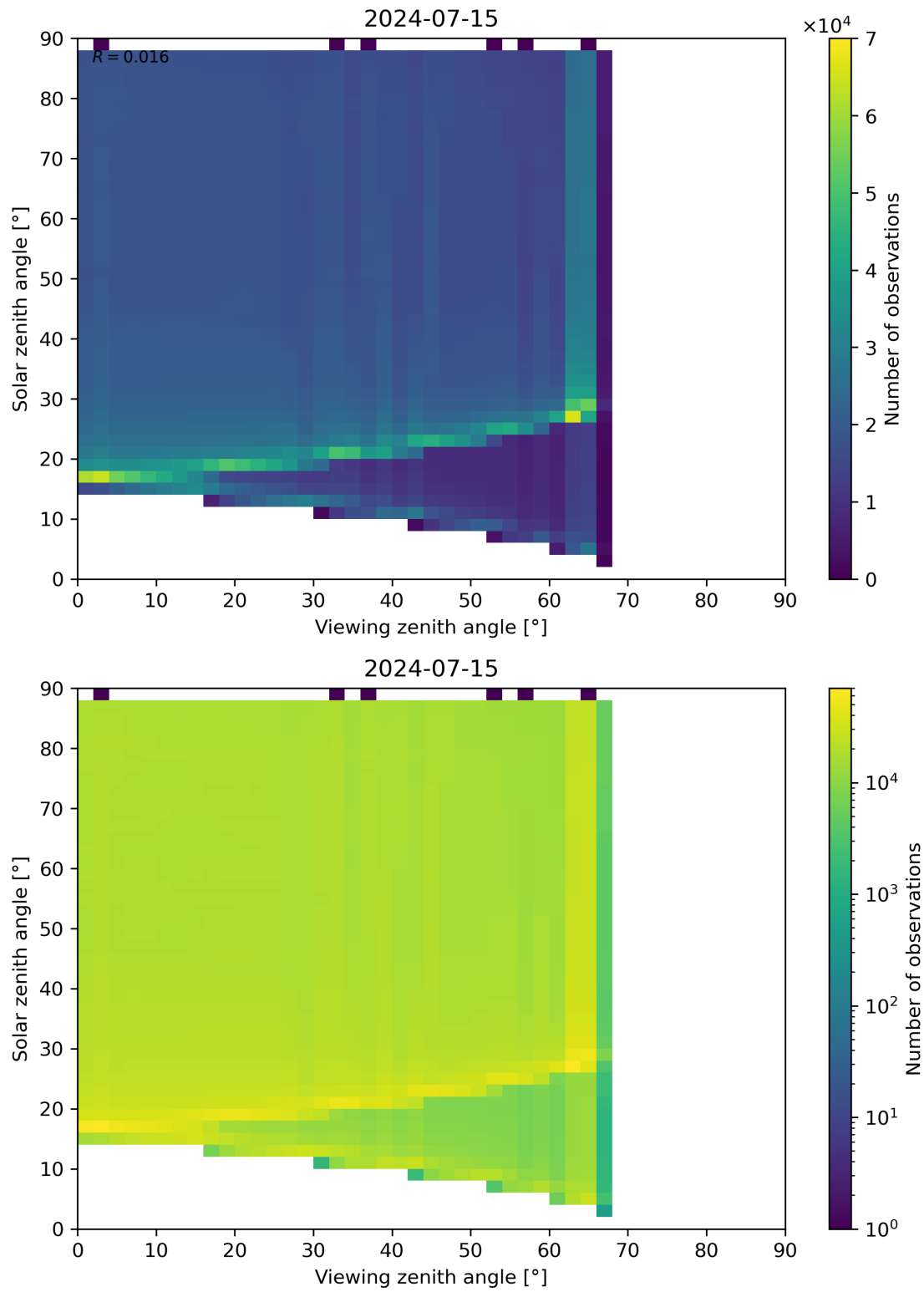
Figure 127: Scatter density plot of “Viewing zenith angle” against “Solar zenith angle” for 2024-07-15 to 2024-07-16.
