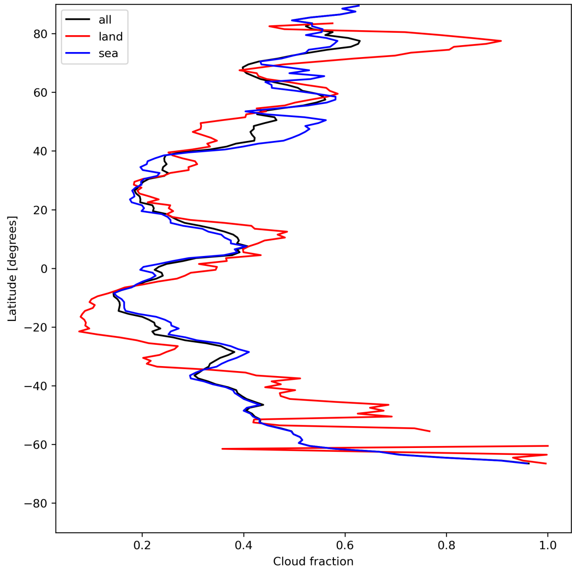
Figure 15: Zonal average of “Cloud fraction” for 2024-07-15 to 2024-07-16.
