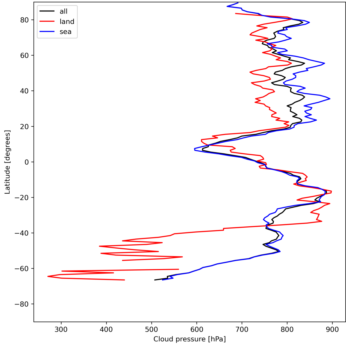
Figure 13: Zonal average of “Cloud pressure” for 2024-07-15 to 2024-07-16.
