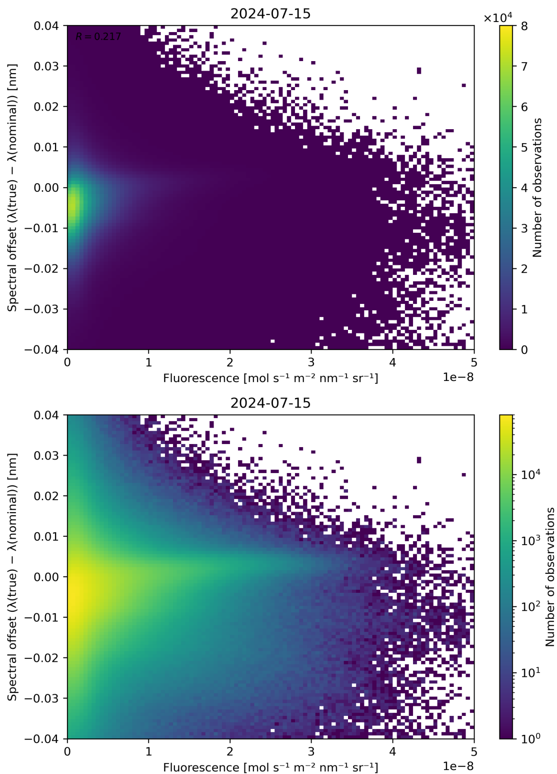
Figure 87: Scatter density plot of “Fluorescence” against “Spectral offset ( \lambda(\text{true}) - \lambda(\text{nominal}) )” for 2024-07-15 to 2024-07-16.
