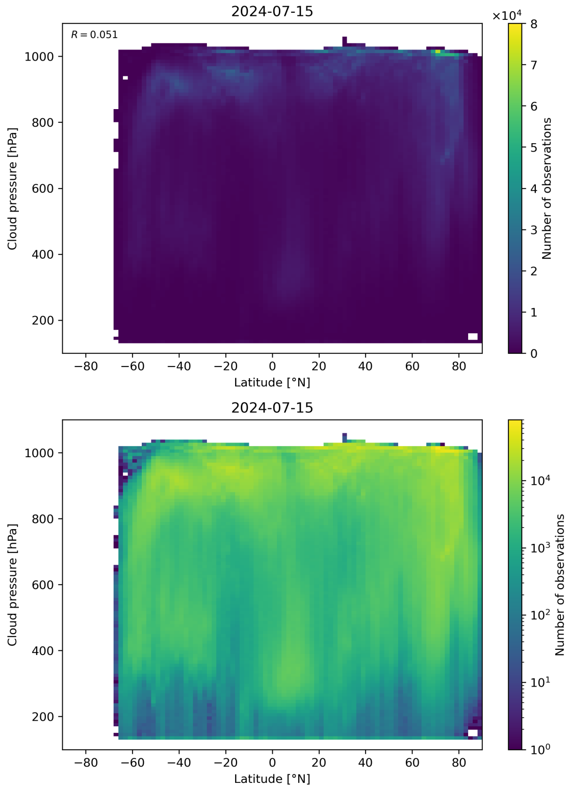
Figure 91: Scatter density plot of “Latitude” against “Cloud pressure” for 2024-07-15 to 2024-07-16.
