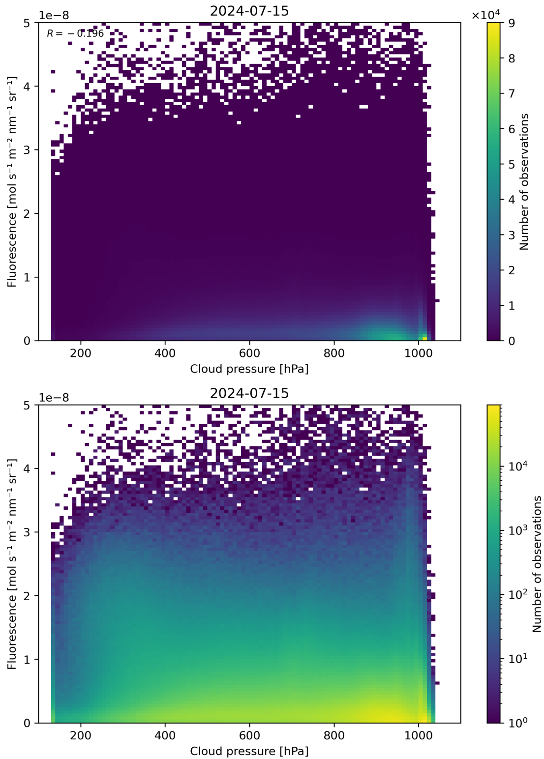
Figure 80: Scatter density plot of “Cloud pressure” against “Fluorescence” for 2024-07-15 to 2024-07-16.
