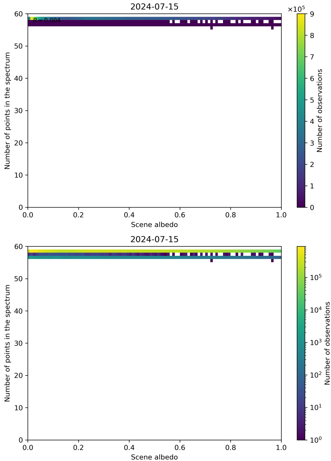
Figure 106: Scatter density plot of “Scene albedo” against “Number of points in the spectrum” for 2024-07-15 to 2024-07-16.
