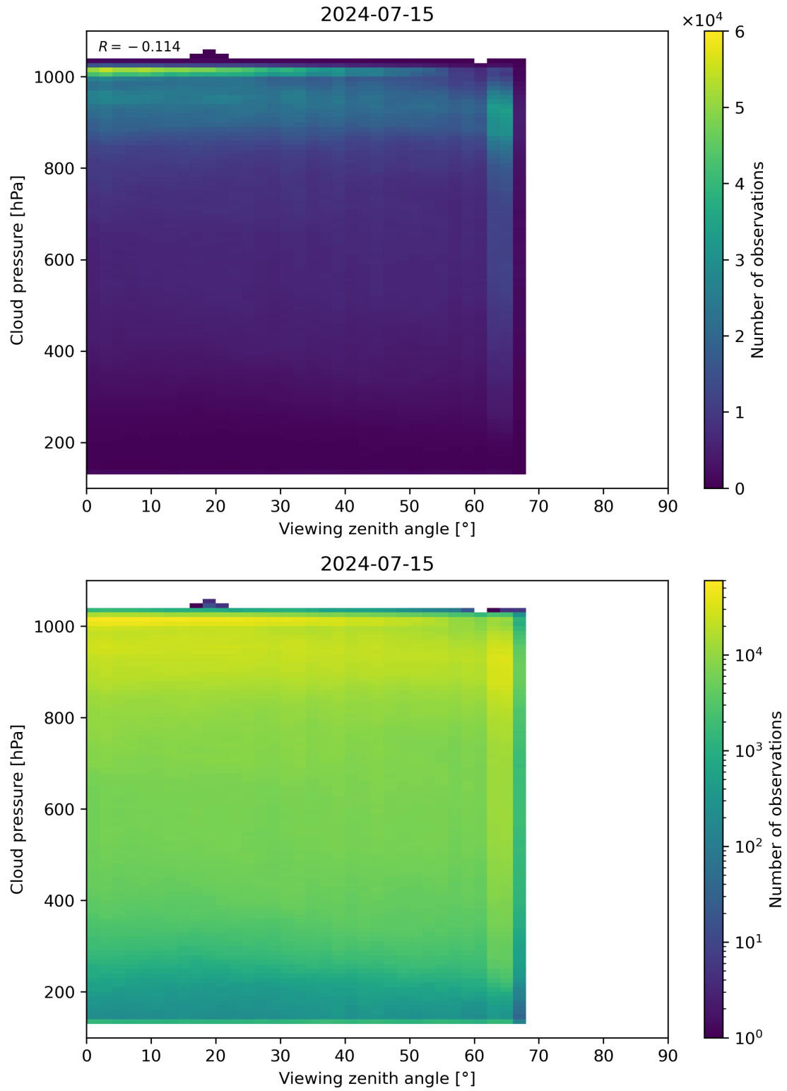
Figure 121: Scatter density plot of “Viewing zenith angle” against “Cloud pressure” for 2024-07-15 to 2024-07-16.
