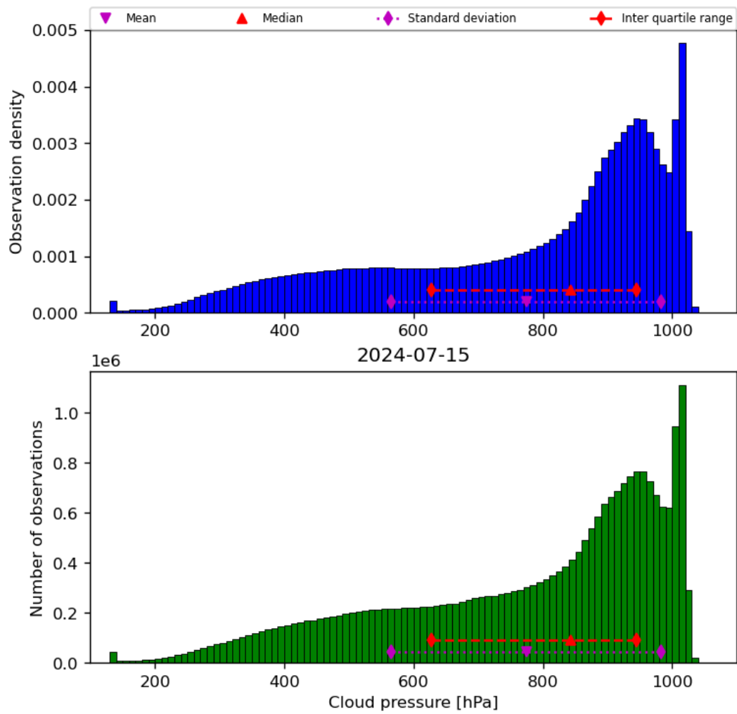
Figure 30: Histogram of “Cloud pressure” for 2024-07-15 to 2024-07-16
