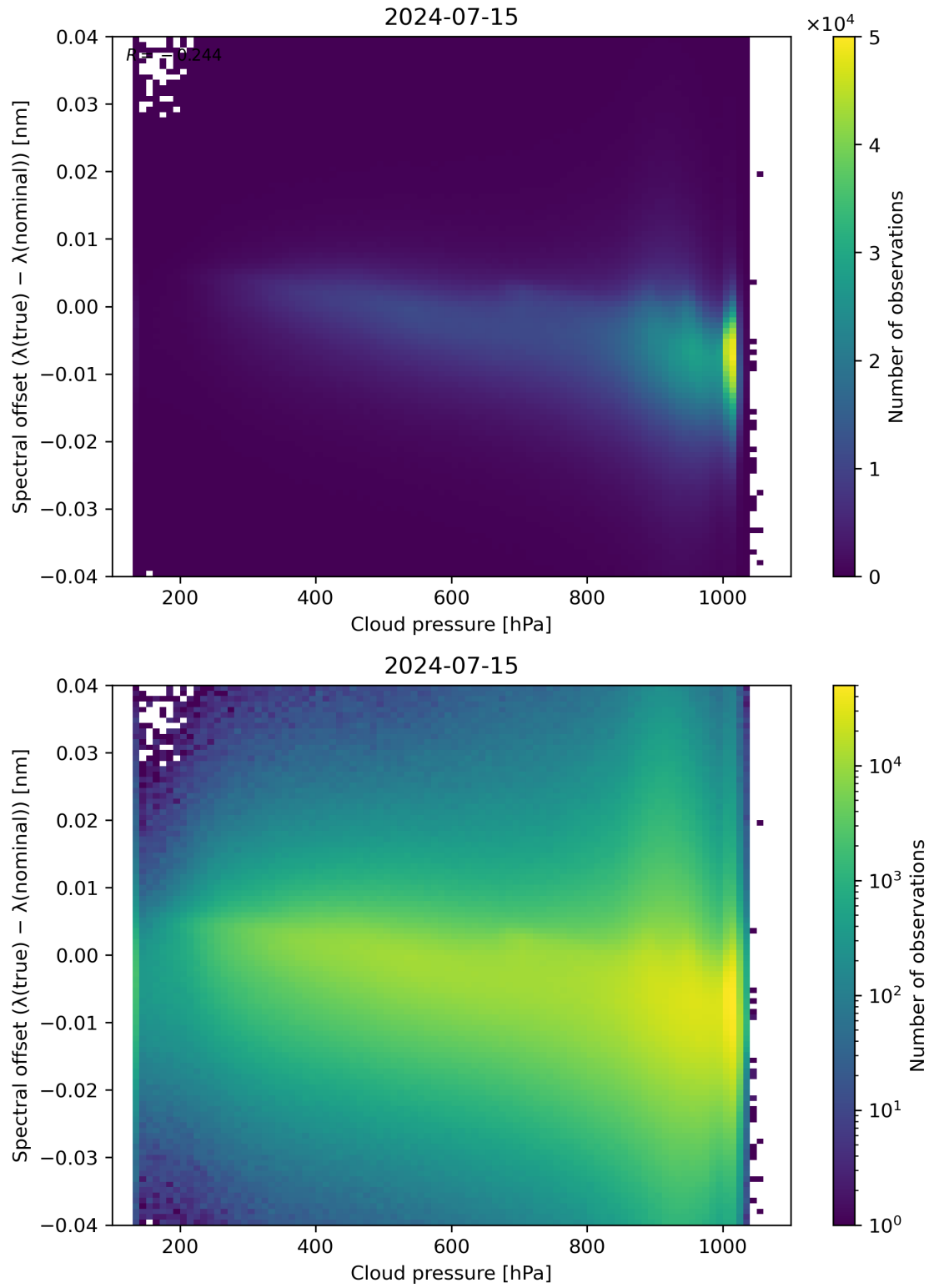
Figure 84: Scatter density plot of “Cloud pressure” against “Spectral offset ( \lambda(\text{true}) - \lambda(\text{nominal}) )” for 2024-07-15 to 2024-07-16.
