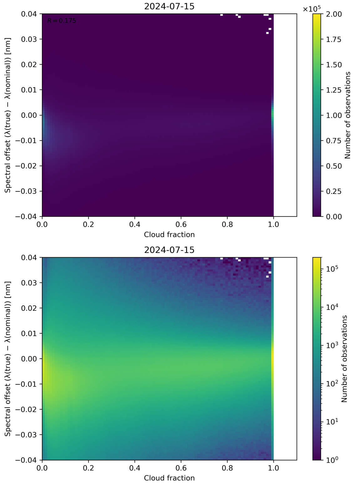
Figure 76: Scatter density plot of “Cloud fraction” against “Spectral offset ( \lambda(\text{true}) - \lambda(\text{nominal}) )” for 2024-07-15 to 2024-07-16.
