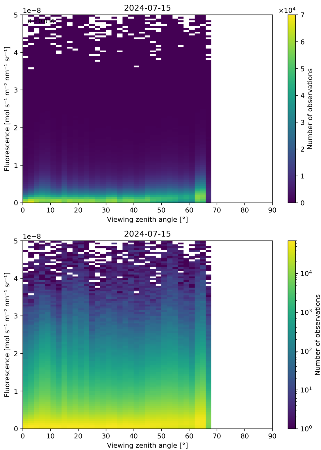
Figure 122: Scatter density plot of “Viewing zenith angle” against “Fluorescence” for 2024-07-15 to 2024-07-16.
