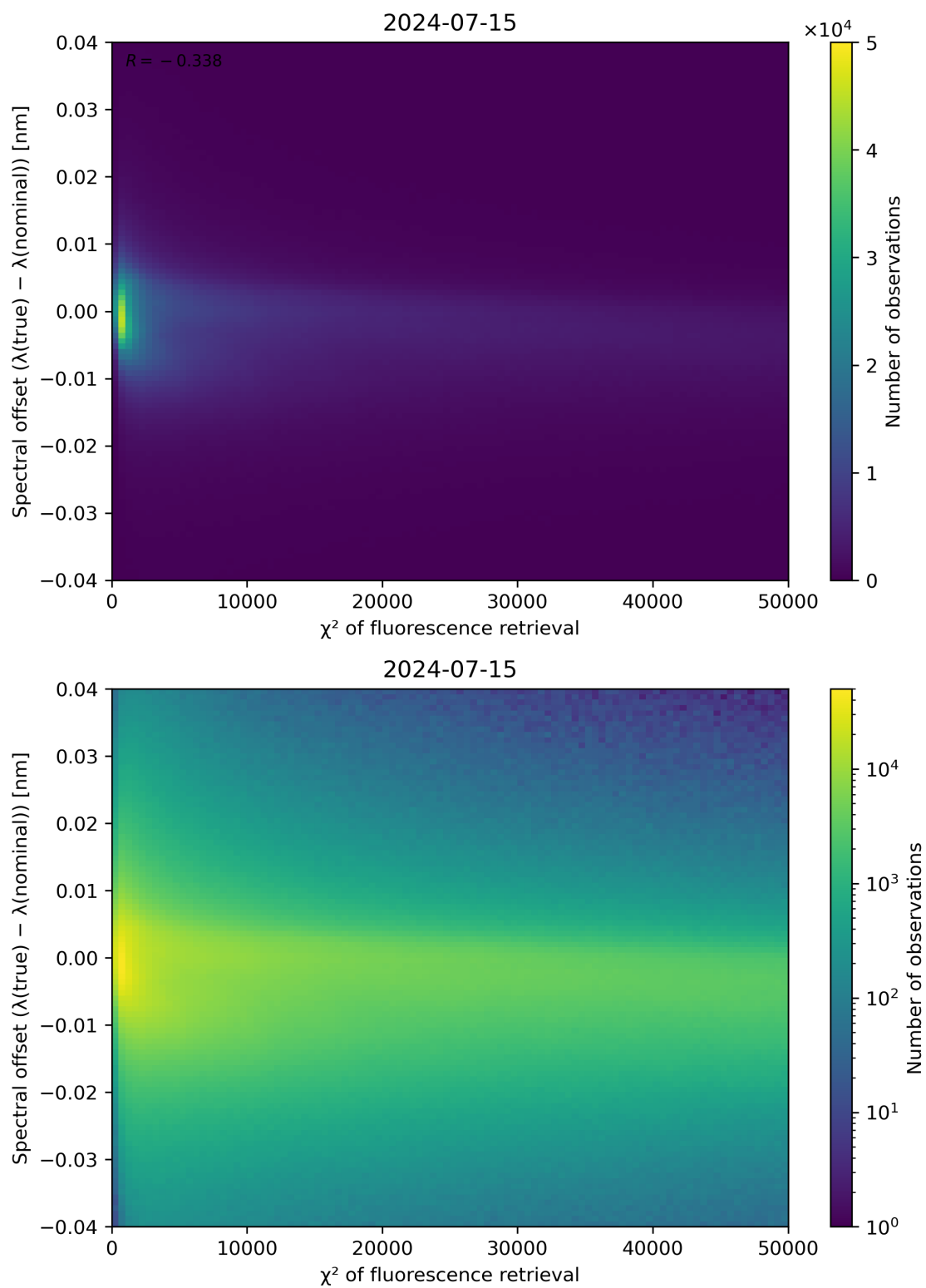
Figure 69: Scatter density plot of “ \chi^2 of fluorescence retrieval” against “Spectral offset ( \lambda(\text{true}) - \lambda(\text{nominal}) )” for 2024-07-15 to 2024-07-16.
