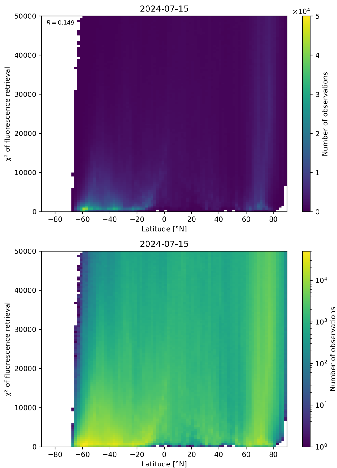
Figure 89: Scatter density plot of “Latitude” against “ \chi^2 of fluorescence retrieval” for 2024-07-15 to 2024-07-16.
