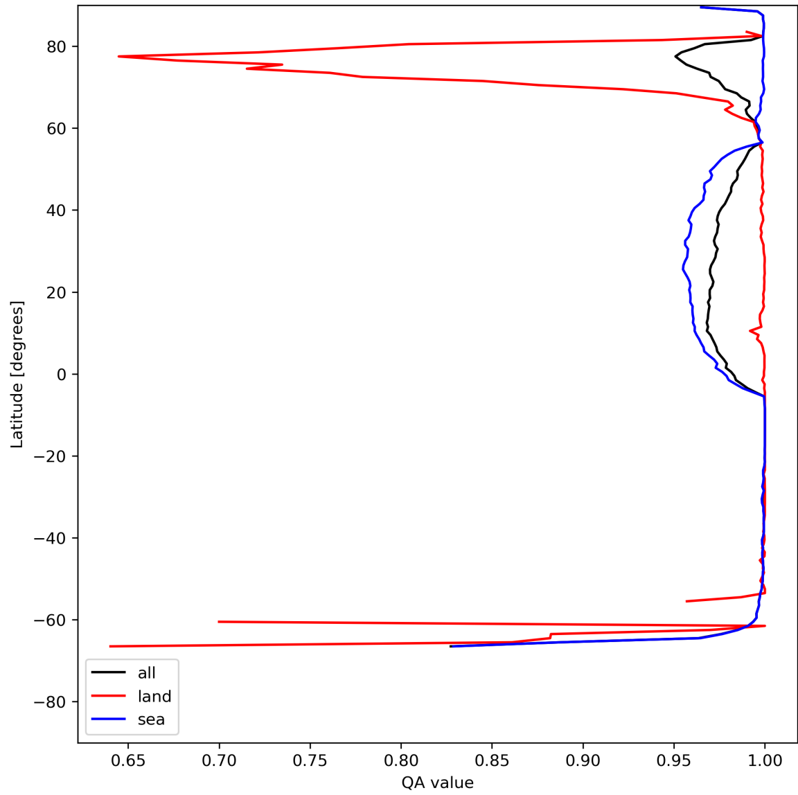
Figure 12: Zonal average of “QA value” for 2024-07-15 to 2024-07-16.
