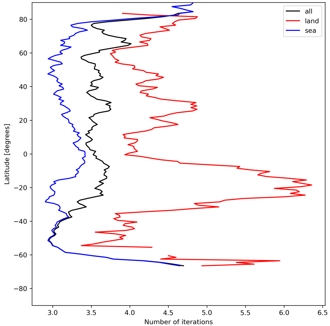
Figure 22: Zonal average of “Number of iterations” for 2024-07-15 to 2024-07-16.
