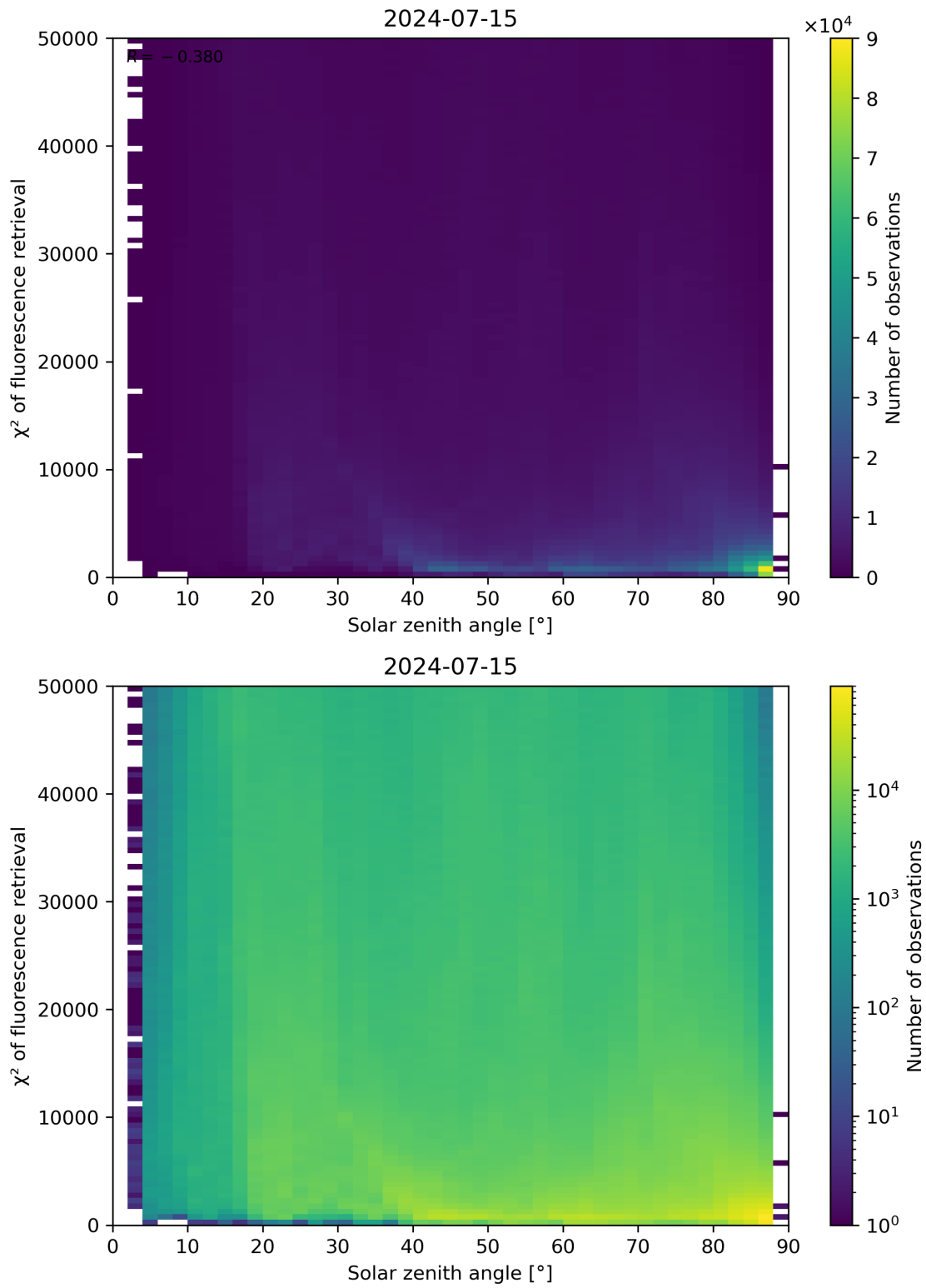
Figure 109: Scatter density plot of “Solar zenith angle” against “ \chi^2 of fluorescence retrieval” for 2024-07-15 to 2024-07-16.
