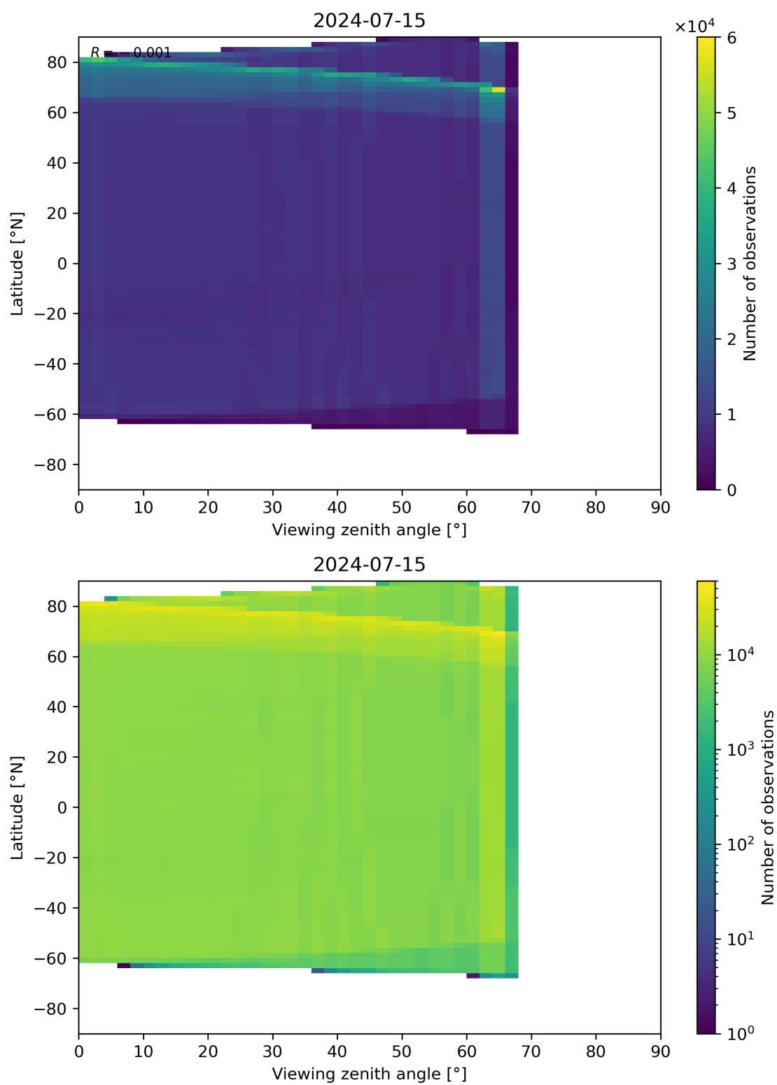
Figure 123: Scatter density plot of “Viewing zenith angle” against “Latitude” for 2024-07-15 to 2024-07-16.
