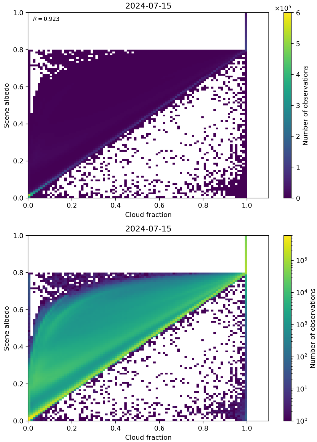
Figure 75: Scatter density plot of “Cloud fraction” against “Scene albedo” for 2024-07-15 to 2024-07-16.
