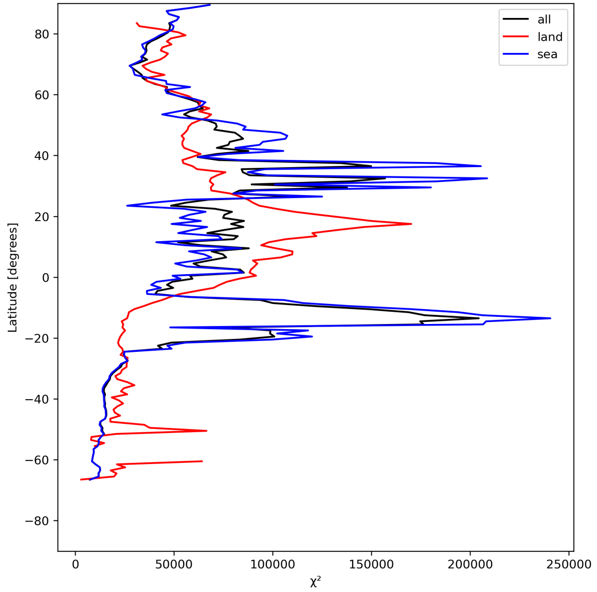
Figure 21: Zonal average of “ \chi^2 ” for 2024-07-15 to 2024-07-16.
