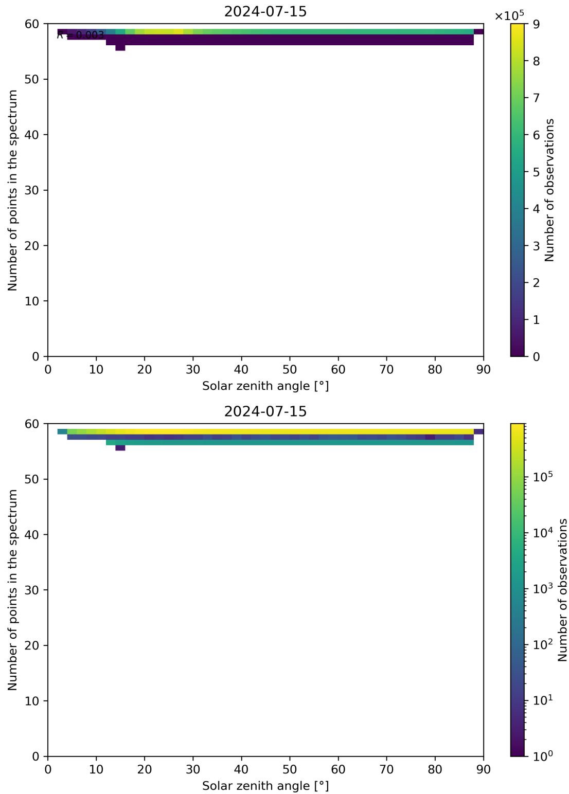
Figure 115: Scatter density plot of “Solar zenith angle” against “Number of points in the spectrum” for 2024-07-15 to 2024-07-16.
