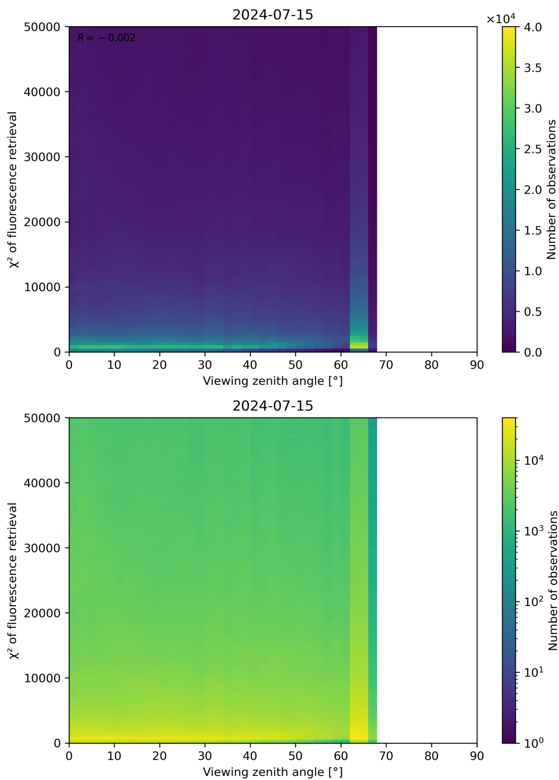
Figure 119: Scatter density plot of “Viewing zenith angle” against “ \chi^2 of fluorescence retrieval” for 2024-07-15 to 2024-07-16.
