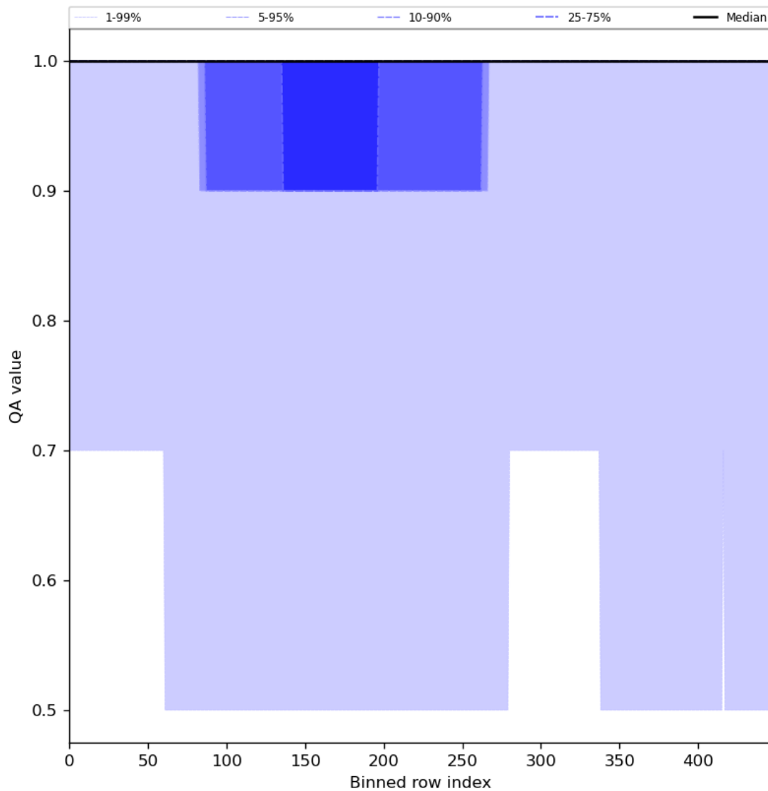
Figure 46: Along track statistics of “QA value” for 2024-07-15 to 2024-07-16
