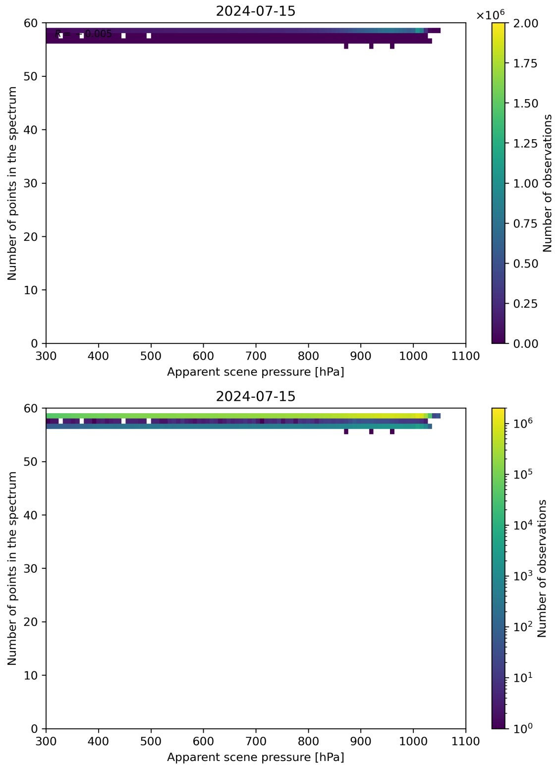
Figure 66: Scatter density plot of “Apparent scene pressure” against “Number of points in the spectrum” for 2024-07-15 to 2024-07-16.
