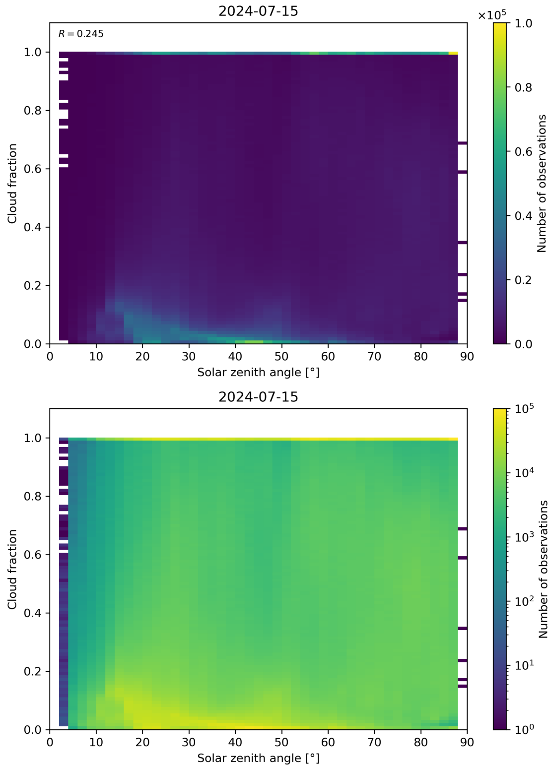
Figure 110: Scatter density plot of “Solar zenith angle” against “Cloud fraction” for 2024-07-15 to 2024-07-16.
