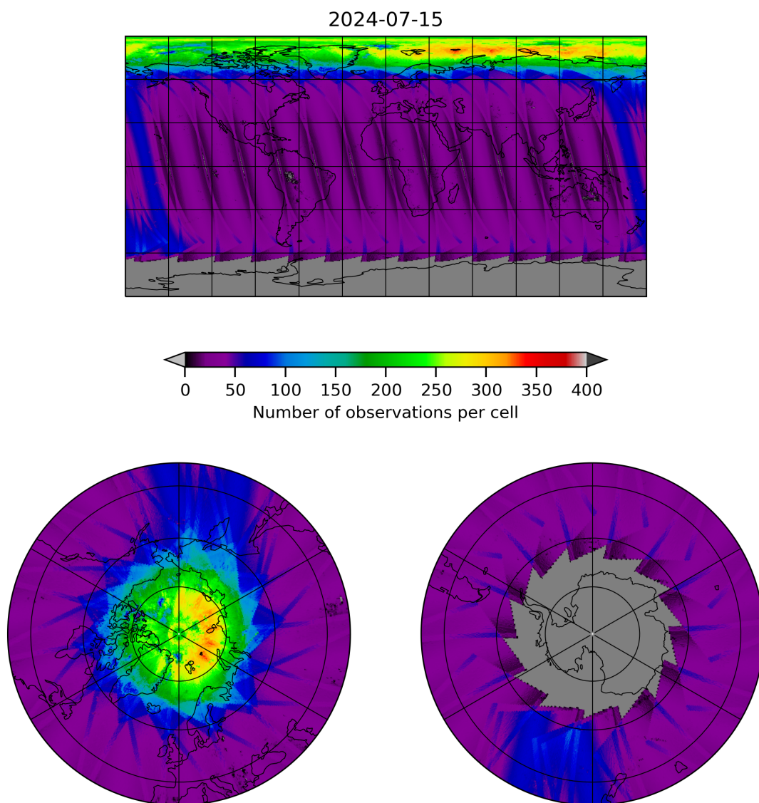
Figure 11: Map of the number of observations for 2024-07-15 to 2024-07-16
