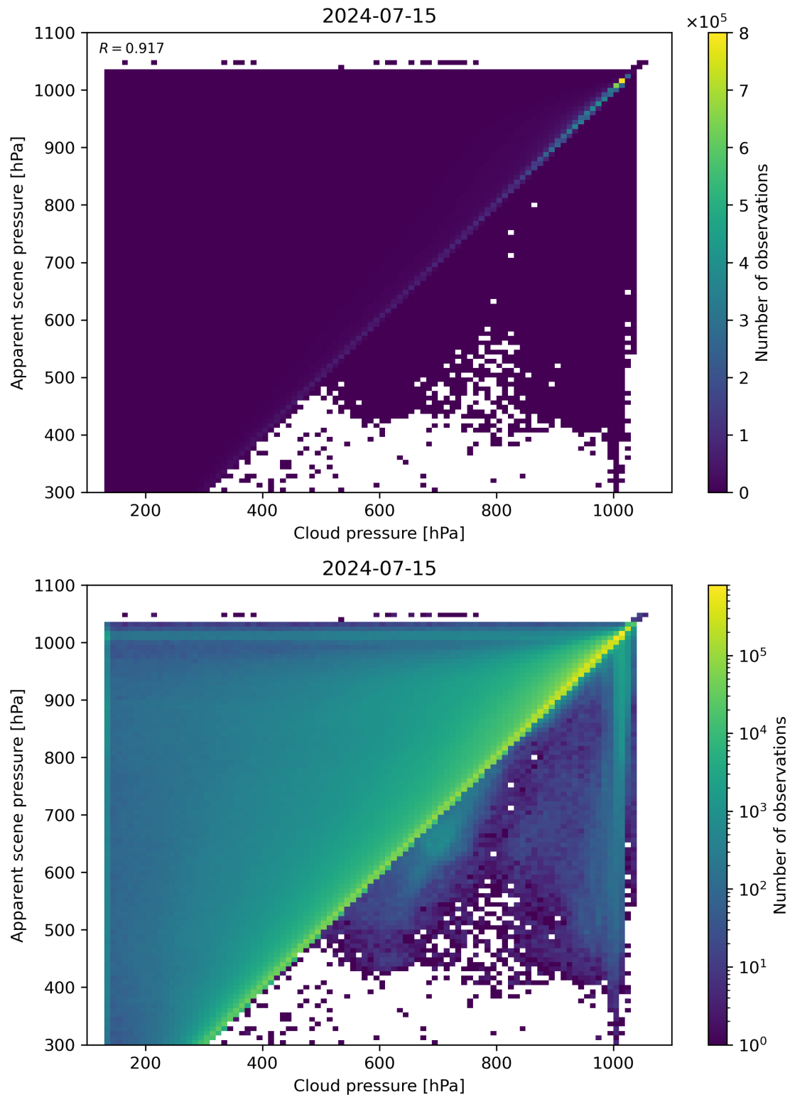
Figure 77: Scatter density plot of “Cloud pressure” against “Apparent scene pressure” for 2024-07-15 to 2024-07-16.
