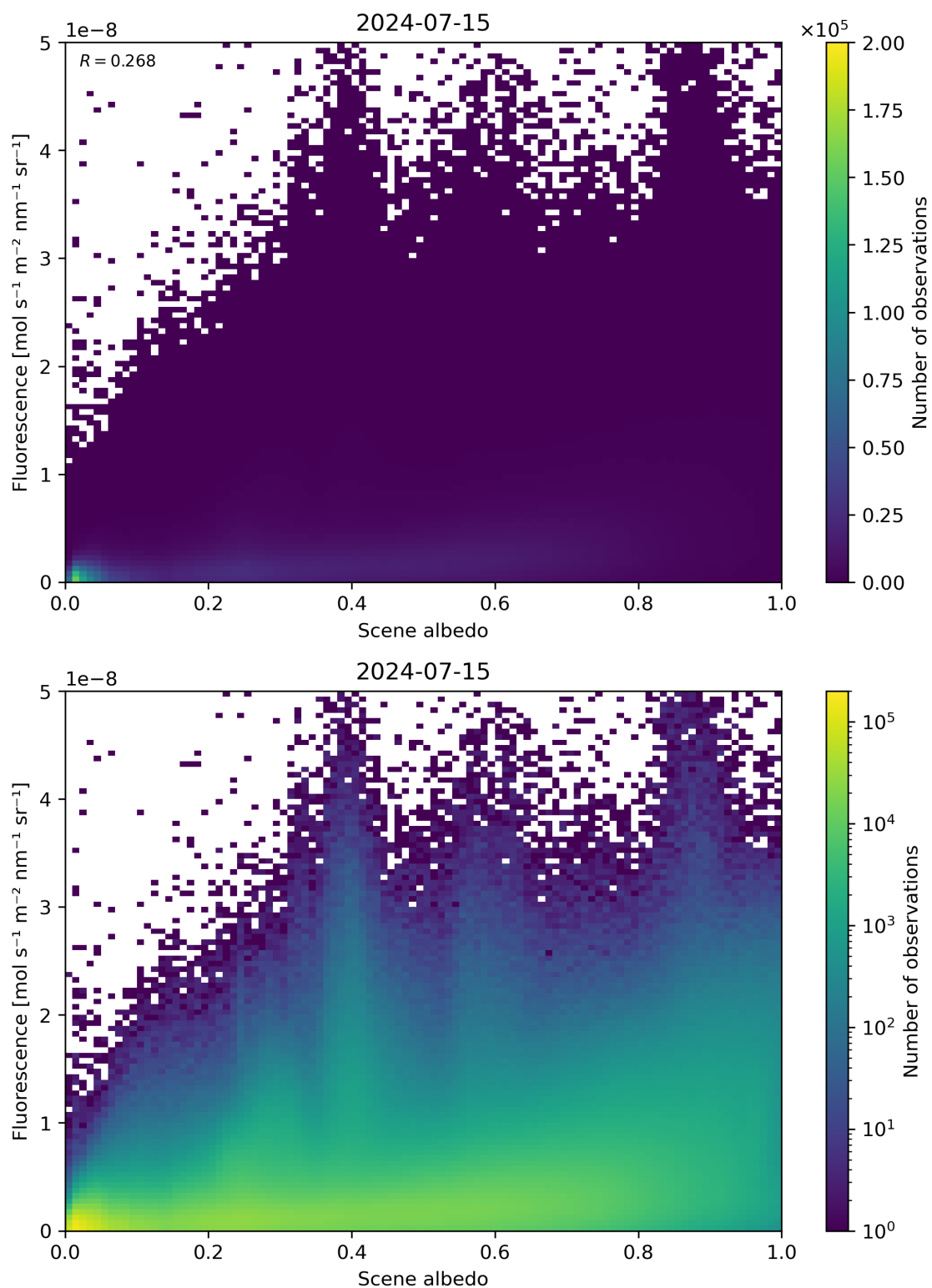
Figure 104: Scatter density plot of “Scene albedo” against “Fluorescence” for 2024-07-15 to 2024-07-16.
