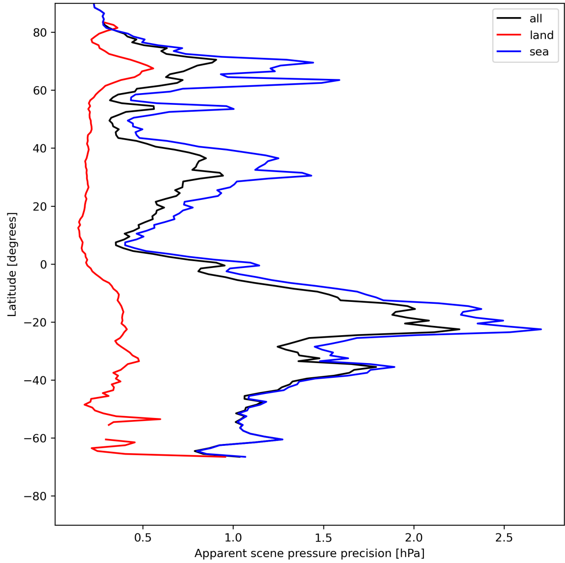
Figure 20: Zonal average of “Apparent scene pressure precision” for 2024-07-15 to 2024-07-16.
