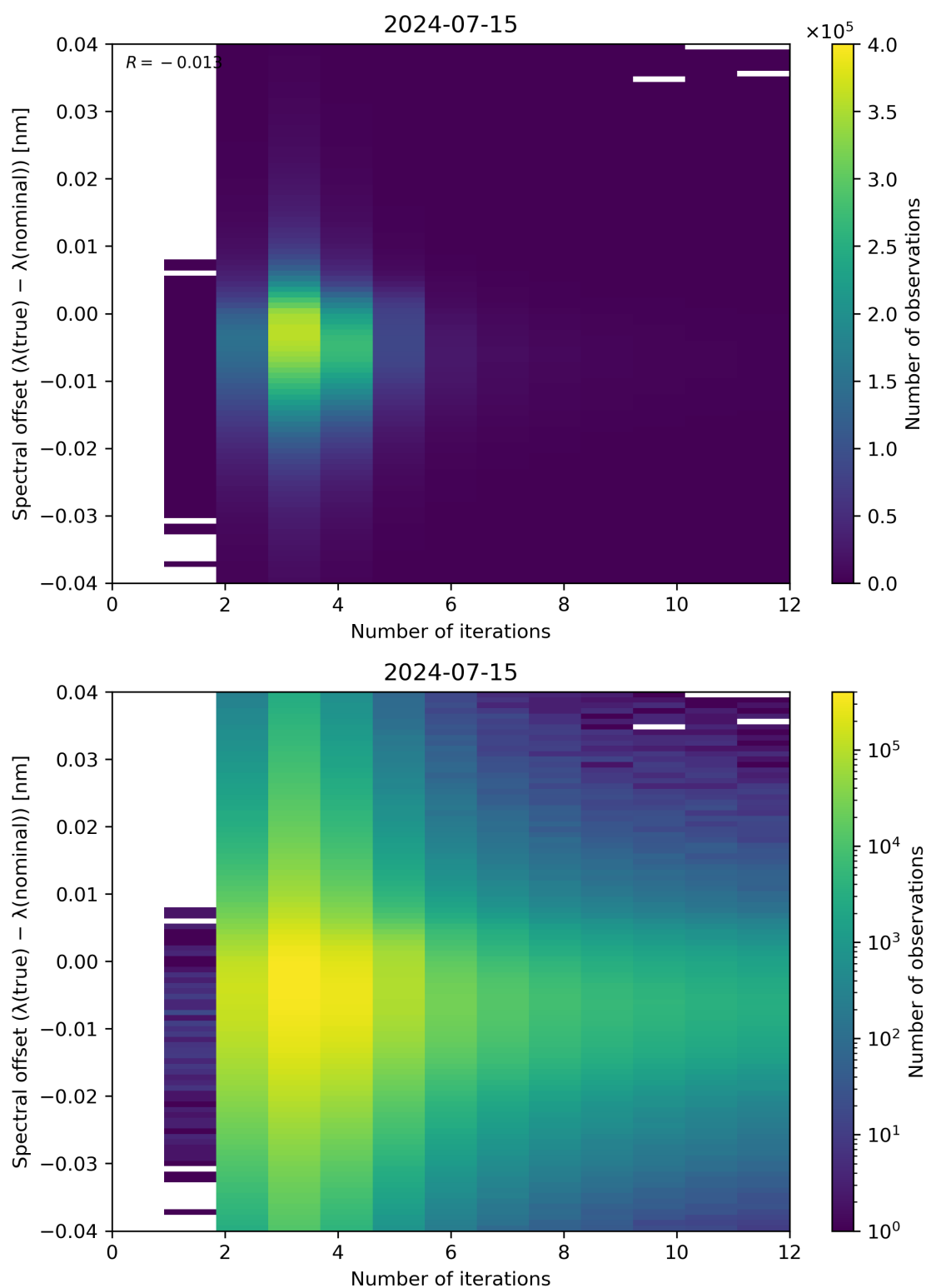
Figure 100: Scatter density plot of “Number of iterations” against “Spectral offset ( \lambda(\text{true}) - \lambda(\text{nominal}) )” for 2024-07-15 to 2024-07-16.
