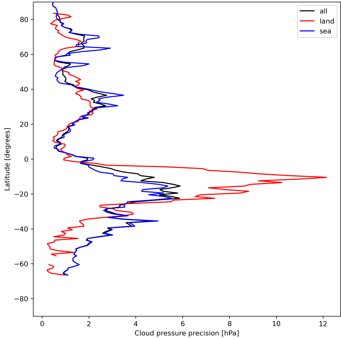
Figure 14: Zonal average of “Cloud pressure precision” for 2024-07-15 to 2024-07-16.
