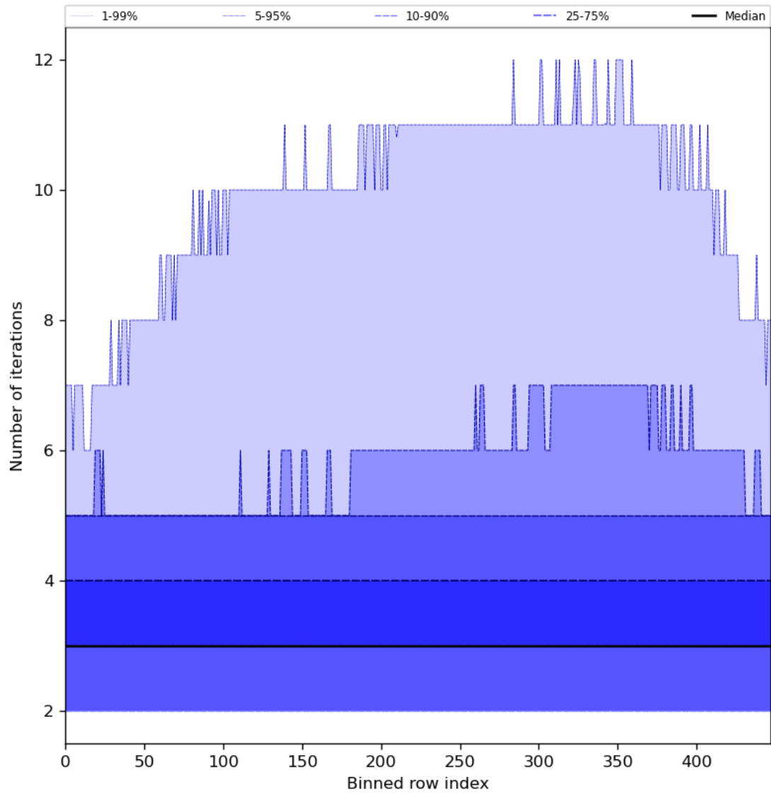
Figure 56: Along track statistics of “Number of iterations” for 2024-07-15 to 2024-07-16
