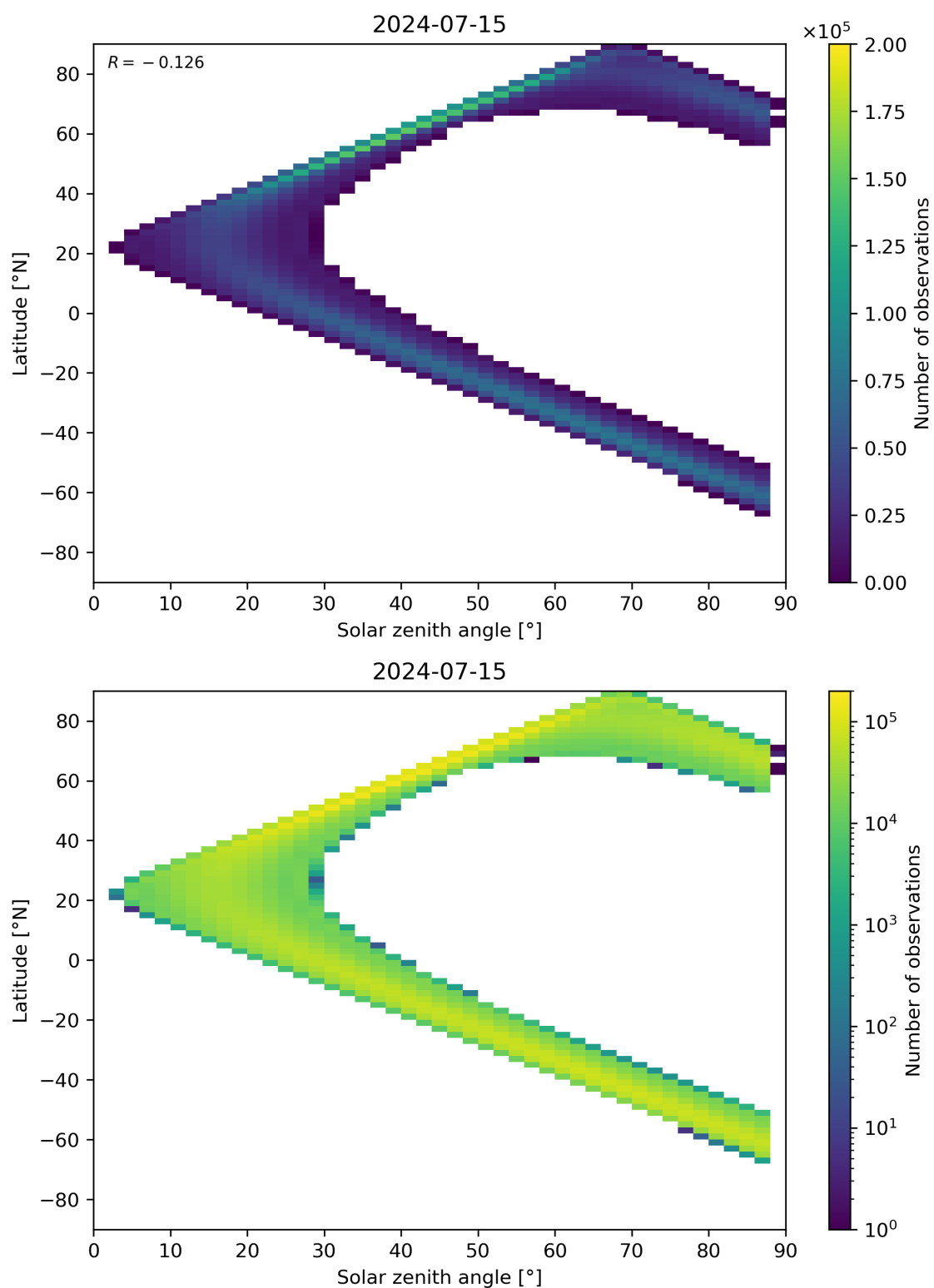
Figure 113: Scatter density plot of “Solar zenith angle” against “Latitude” for 2024-07-15 to 2024-07-16.
