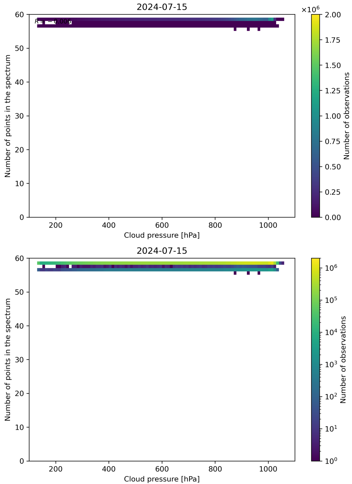
Figure 82: Scatter density plot of “Cloud pressure” against “Number of points in the spectrum” for 2024-07-15 to 2024-07-16.
