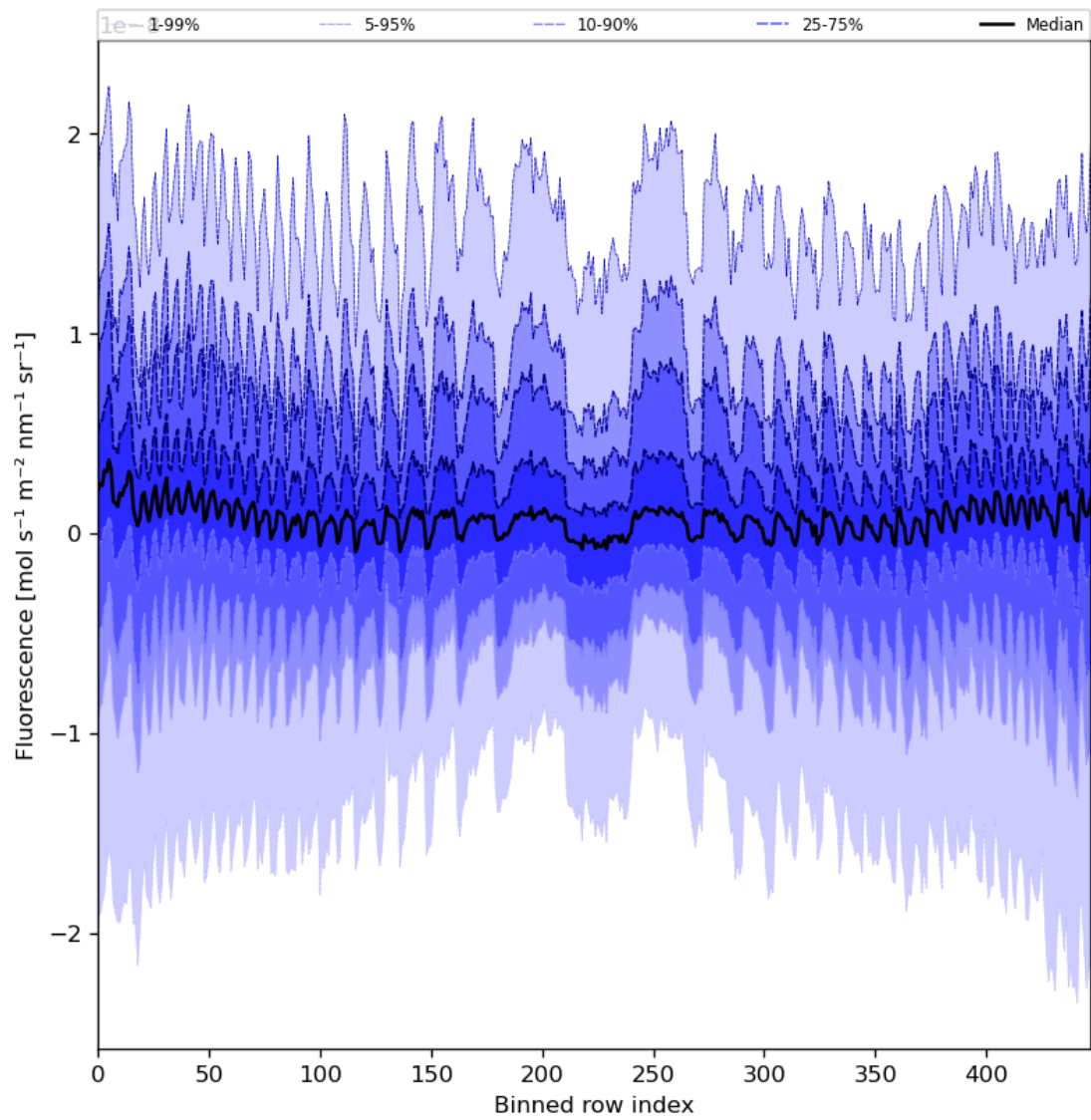
Figure 57: Along track statistics of “Fluorescence” for 2024-07-15 to 2024-07-16
