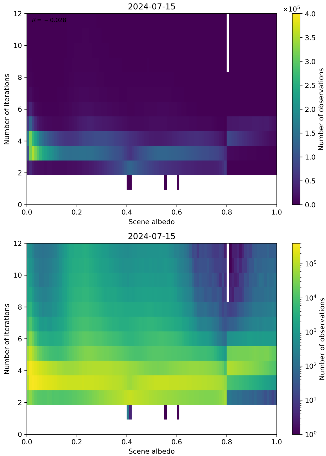
Figure 105: Scatter density plot of “Scene albedo” against “Number of iterations” for 2024-07-15 to 2024-07-16.
