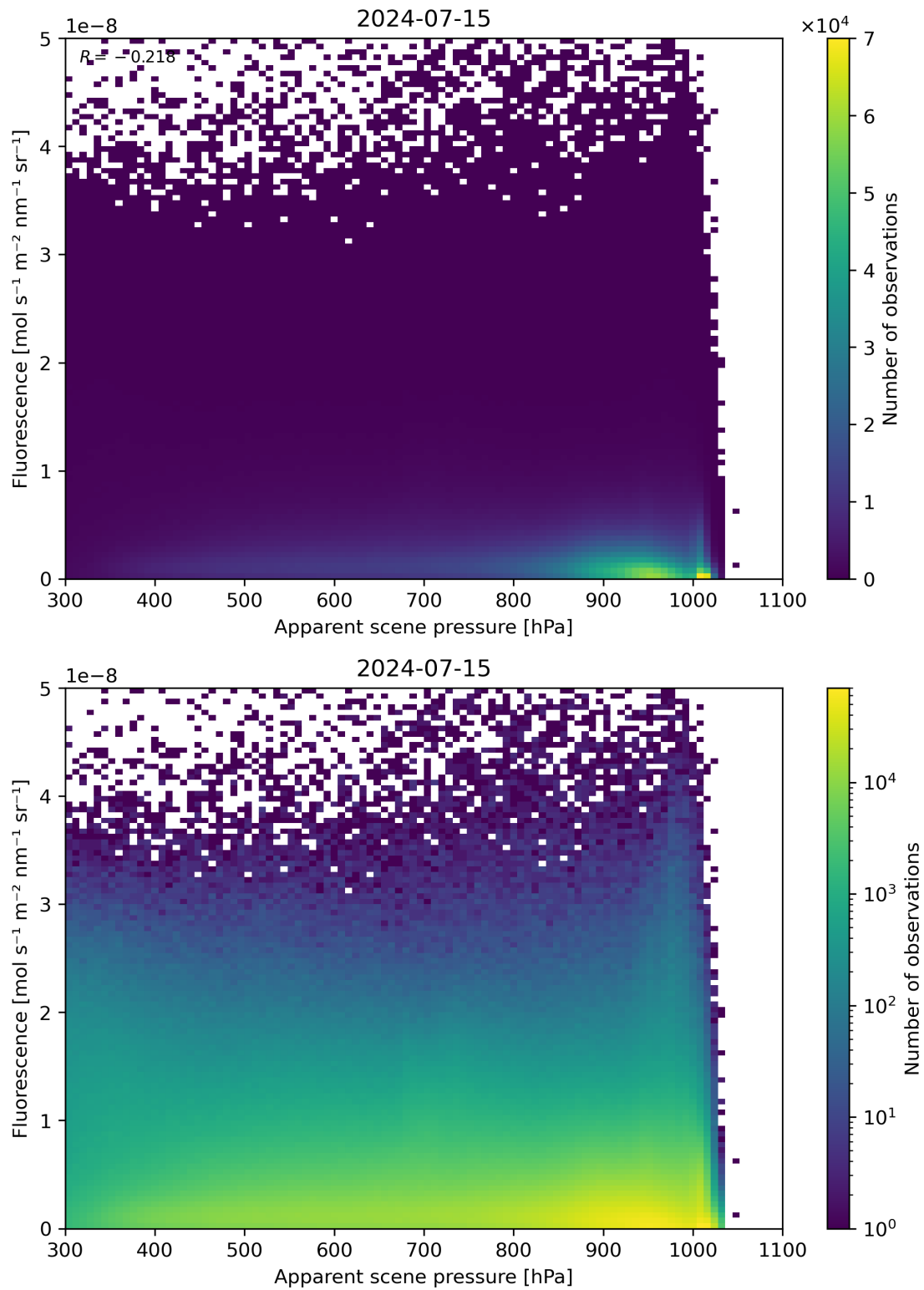
Figure 64: Scatter density plot of “Apparent scene pressure” against “Fluorescence” for 2024-07-15 to 2024-07-16.
