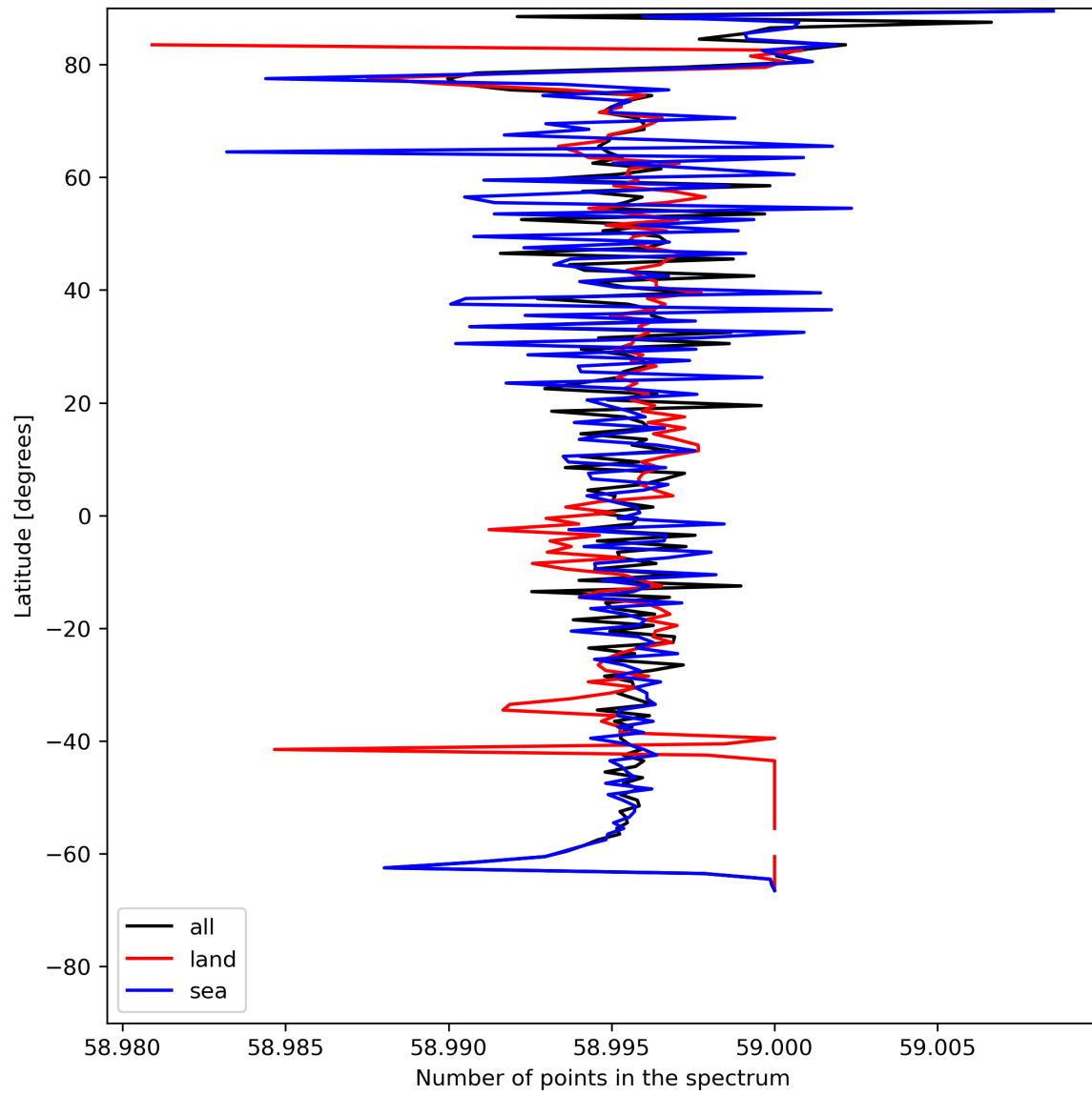
Figure 27: Zonal average of “Number of points in the spectrum” for 2024-07-15 to 2024-07-16.
