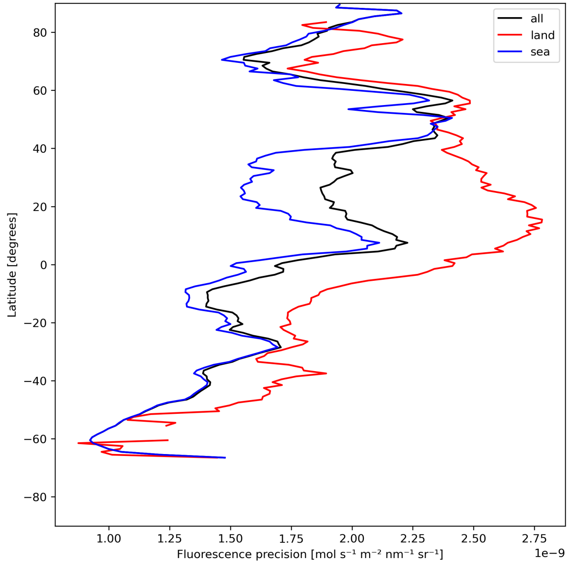
Figure 24: Zonal average of “Fluorescence precision” for 2024-07-15 to 2024-07-16.
