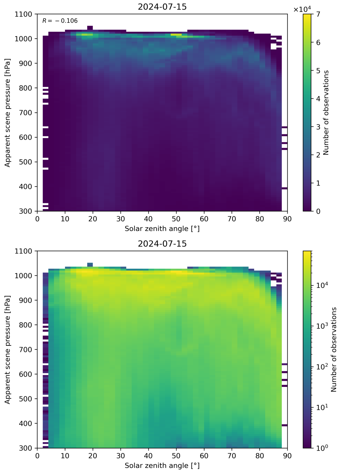
Figure 108: Scatter density plot of “Solar zenith angle” against “Apparent scene pressure” for 2024-07-15 to 2024-07-16.
