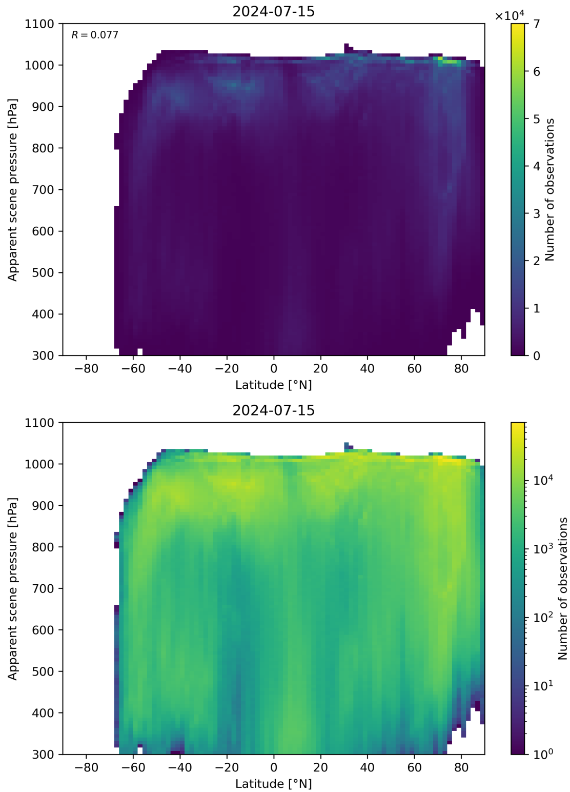
Figure 88: Scatter density plot of “Latitude” against “Apparent scene pressure” for 2024-07-15 to 2024-07-16.
