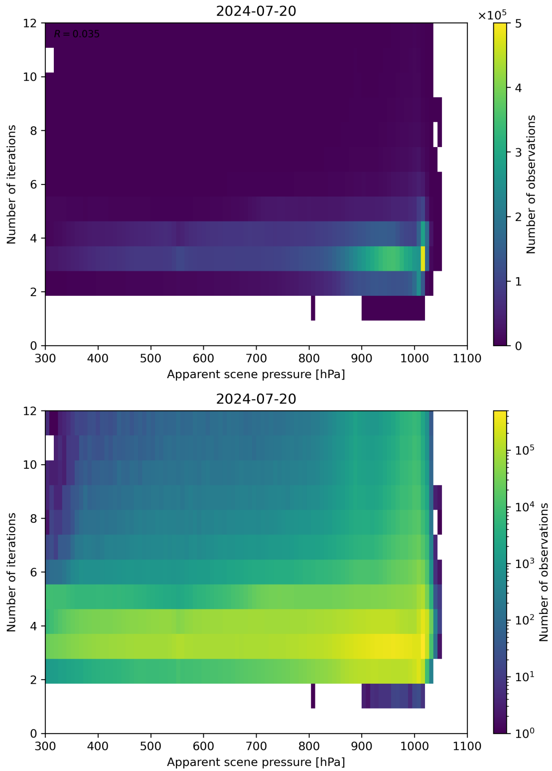
Figure 65: Scatter density plot of “Apparent scene pressure” against “Number of iterations” for 2024-07-19 to 2024-07-21.
