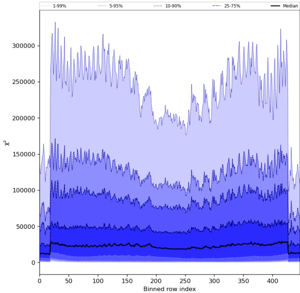
Figure 55: Along track statistics of “ \chi^2 ” for 2024-07-19 to 2024-07-21
