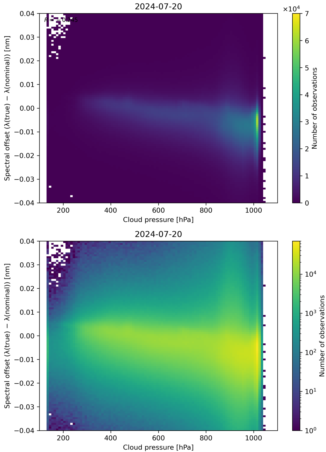
Figure 84: Scatter density plot of “Cloud pressure” against “Spectral offset ( \lambda(\text{true}) - \lambda(\text{nominal}) )” for 2024-07-19 to 2024-07-21.
