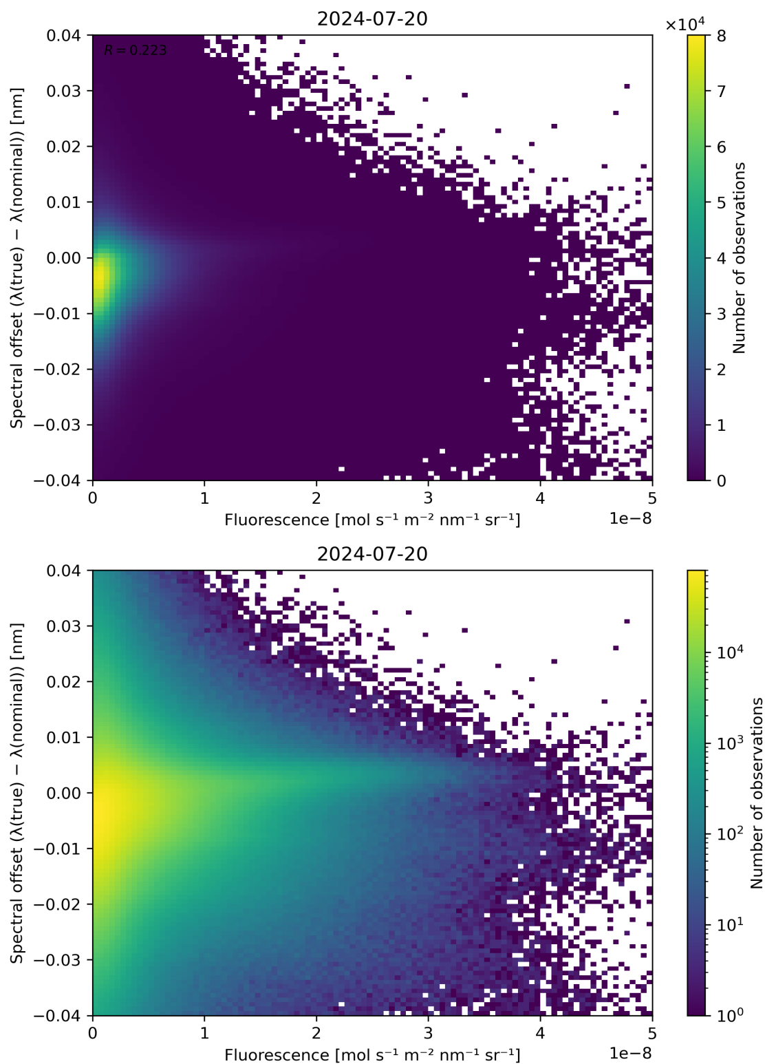
Figure 87: Scatter density plot of “Fluorescence” against “Spectral offset ( \lambda(\text{true}) - \lambda(\text{nominal}) )” for 2024-07-19 to 2024-07-21.
