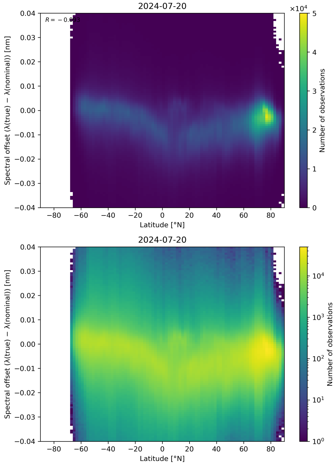
Figure 96: Scatter density plot of “Latitude” against “Spectral offset ( \lambda(\text{true}) - \lambda(\text{nominal}) )” for 2024-07-19 to 2024-07-21.
