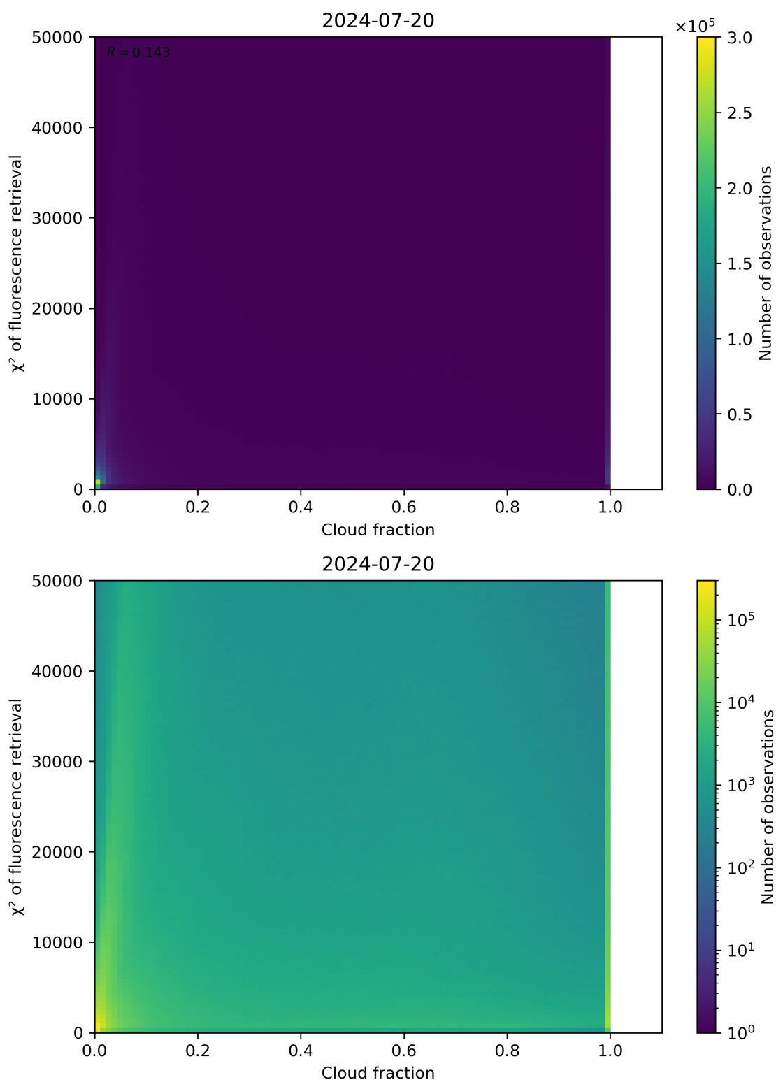
Figure 71: Scatter density plot of “Cloud fraction” against “ \chi^2 of fluorescence retrieval” for 2024-07-19 to 2024-07-21.
