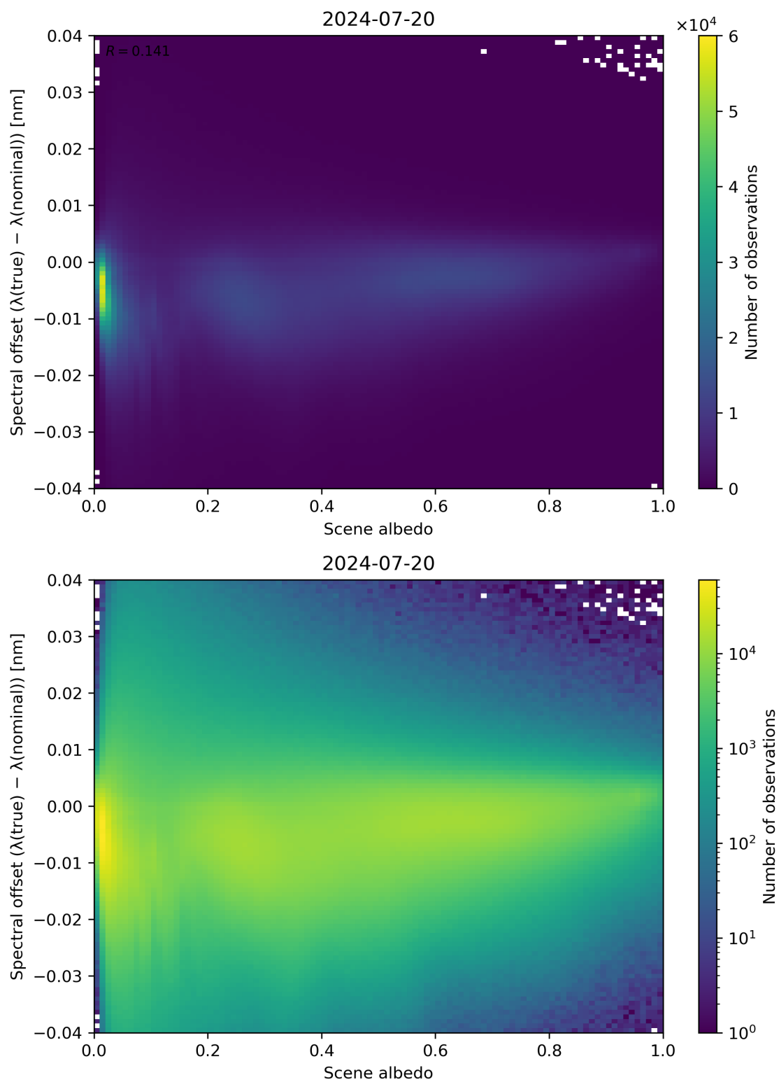
Figure 107: Scatter density plot of “Scene albedo” against “Spectral offset ( \lambda(\text{true}) - \lambda(\text{nominal}) )” for 2024-07-19 to 2024-07-21.
