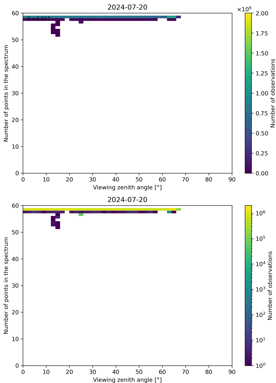
Figure 125: Scatter density plot of “Viewing zenith angle” against “Number of points in the spectrum” for 2024-07-19 to 2024-07-21.
