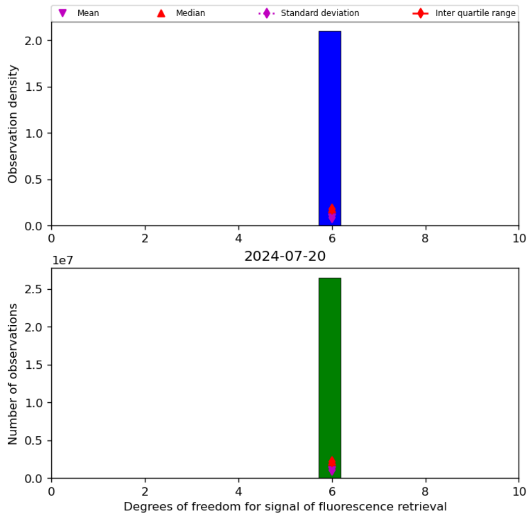
Figure 43: Histogram of “Degrees of freedom for signal of fluorescence retrieval” for 2024-07-19 to 2024-07-21
