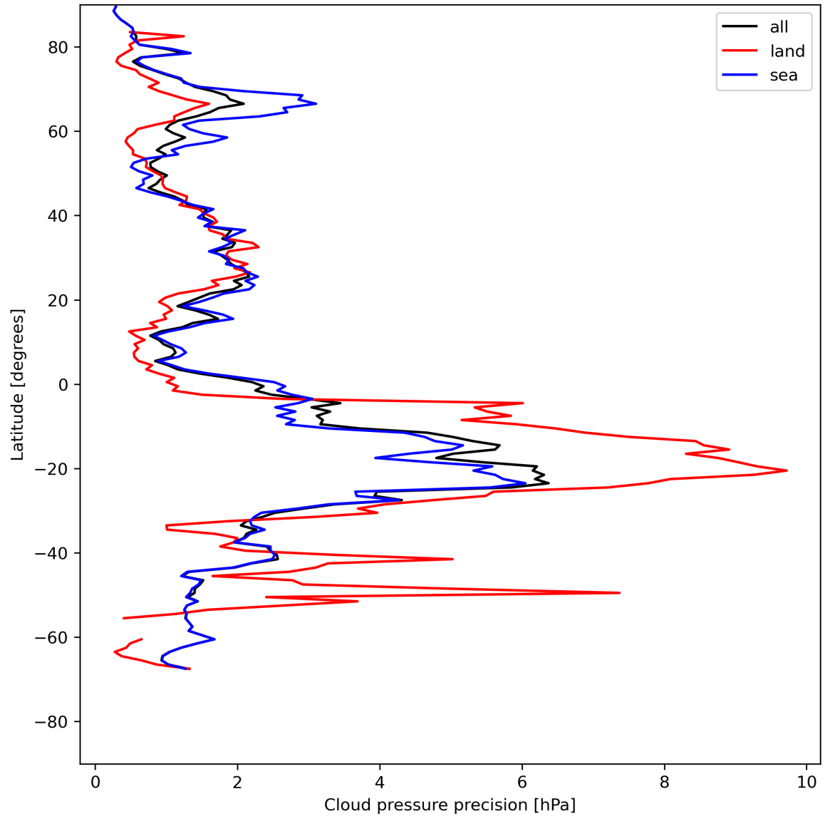
Figure 14: Zonal average of “Cloud pressure precision” for 2024-07-19 to 2024-07-21.
