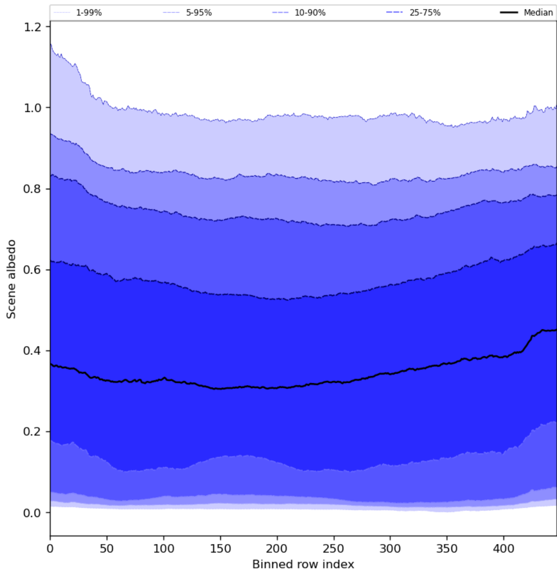
Figure 51: Along track statistics of “Scene albedo” for 2024-07-19 to 2024-07-21
