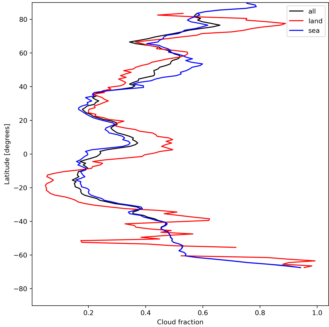
Figure 15: Zonal average of “Cloud fraction” for 2024-07-19 to 2024-07-21.
