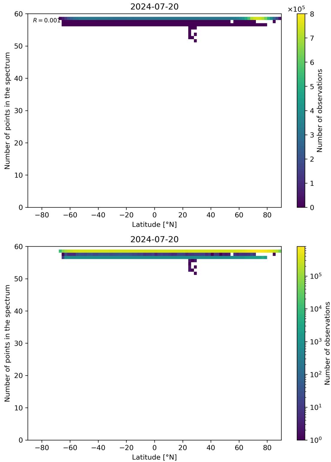
Figure 94: Scatter density plot of “Latitude” against “Number of points in the spectrum” for 2024-07-19 to 2024-07-21.
