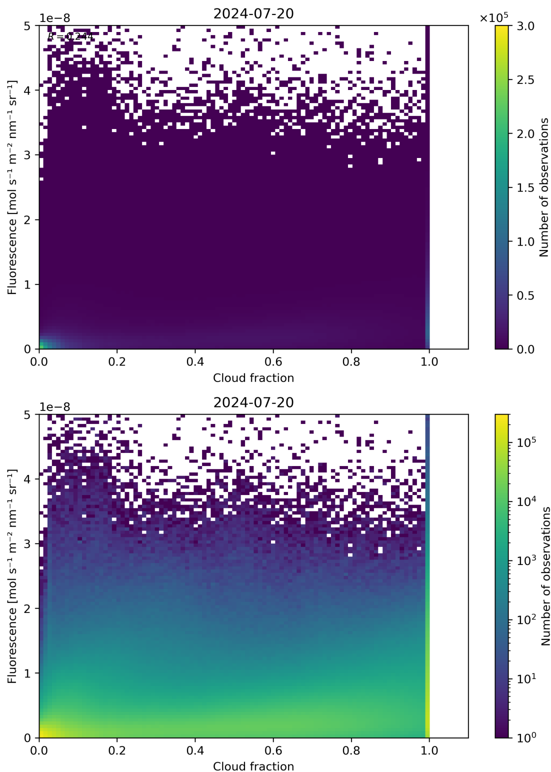
Figure 72: Scatter density plot of “Cloud fraction” against “Fluorescence” for 2024-07-19 to 2024-07-21.
