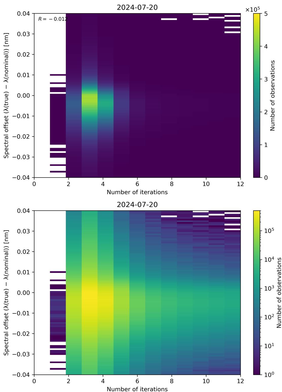
Figure 100: Scatter density plot of “Number of iterations” against “Spectral offset ( \lambda(\text{true}) - \lambda(\text{nominal}) )” for 2024-07-19 to 2024-07-21.
