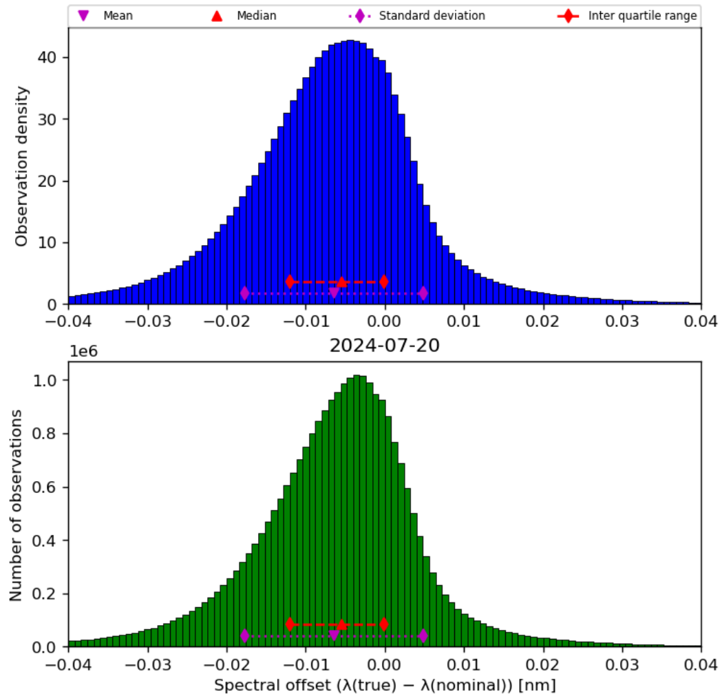
Figure 45: Histogram of “Spectral offset ( \lambda(\text{true}) - \lambda(\text{nominal}) )” for 2024-07-19 to 2024-07-21
