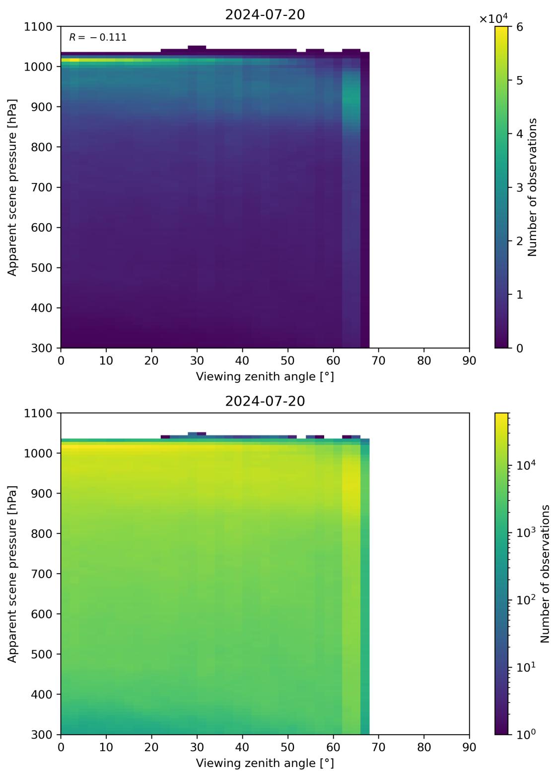
Figure 118: Scatter density plot of “Viewing zenith angle” against “Apparent scene pressure” for 2024-07-19 to 2024-07-21.
