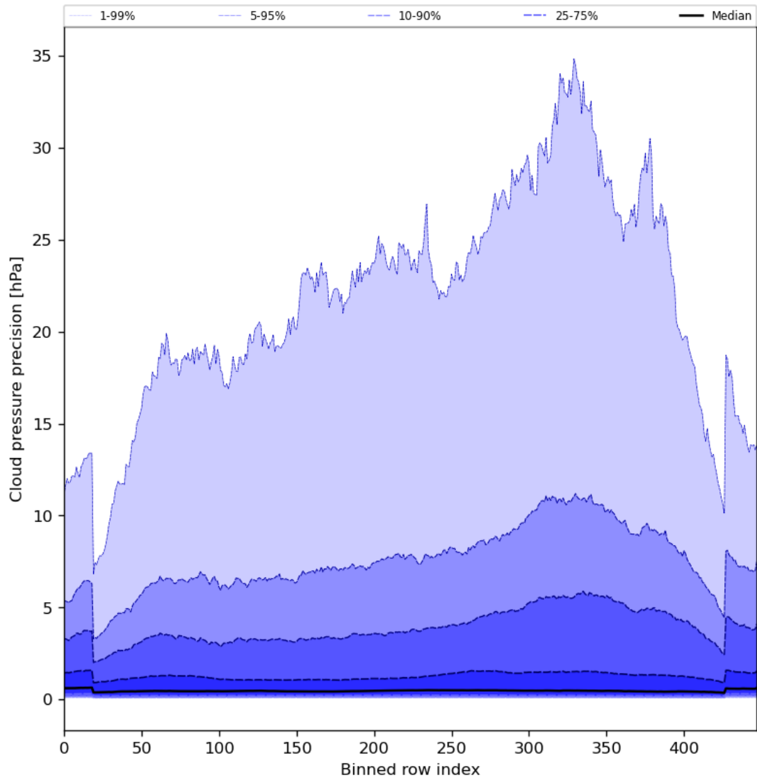
Figure 48: Along track statistics of “Cloud pressure precision” for 2024-07-19 to 2024-07-21
