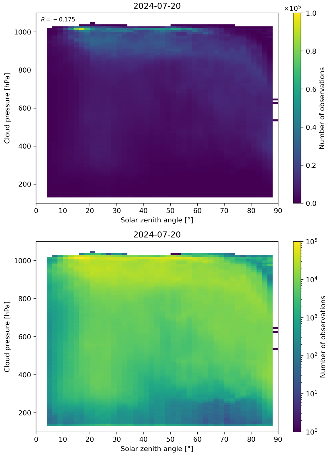
Figure 111: Scatter density plot of “Solar zenith angle” against “Cloud pressure” for 2024-07-19 to 2024-07-21.
