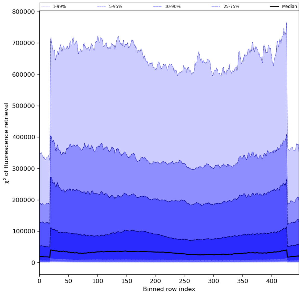
Figure 59: Along track statistics of “ \chi^2 of fluorescence retrieval” for 2024-07-19 to 2024-07-21
