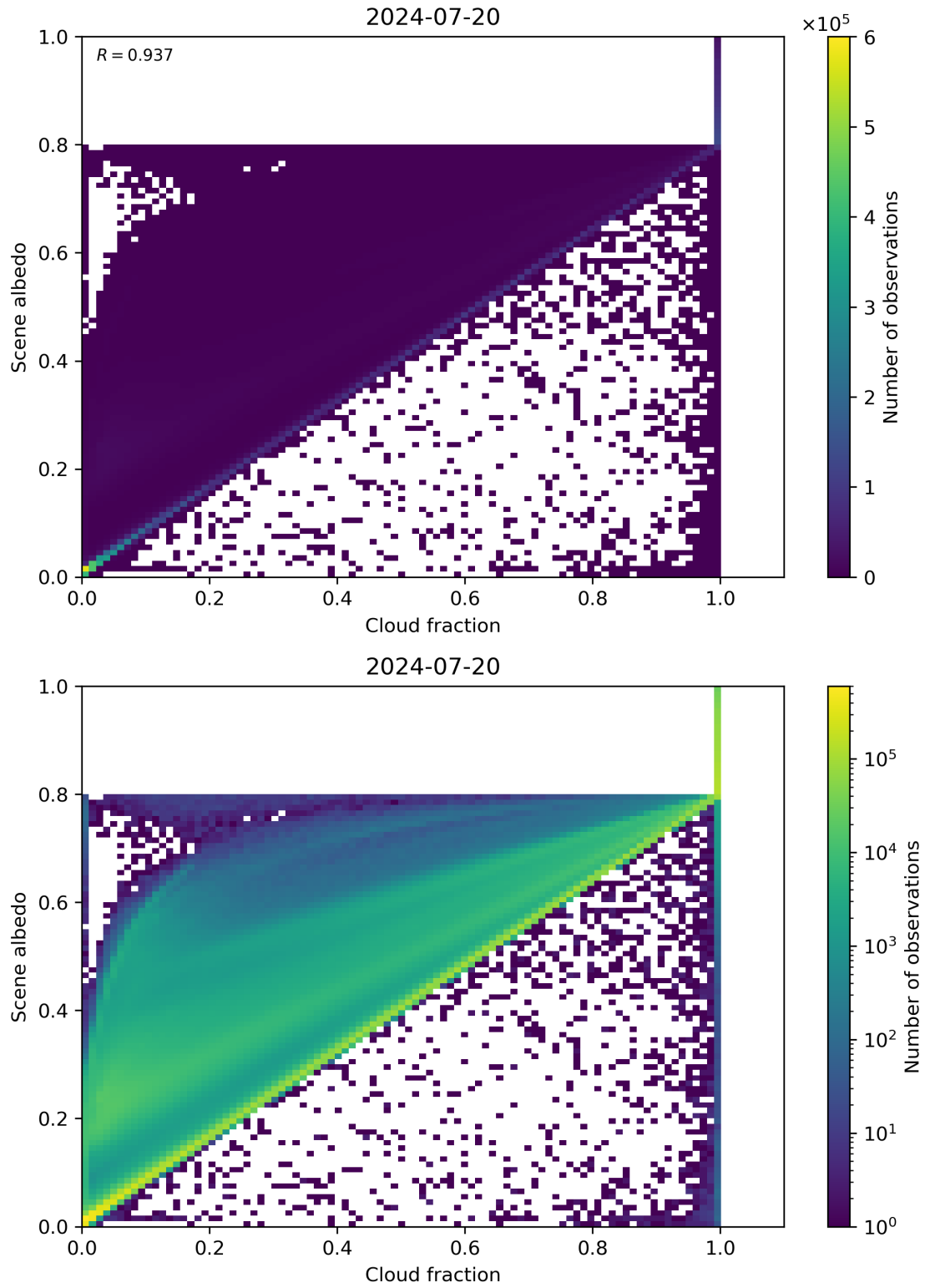
Figure 75: Scatter density plot of “Cloud fraction” against “Scene albedo” for 2024-07-19 to 2024-07-21.
