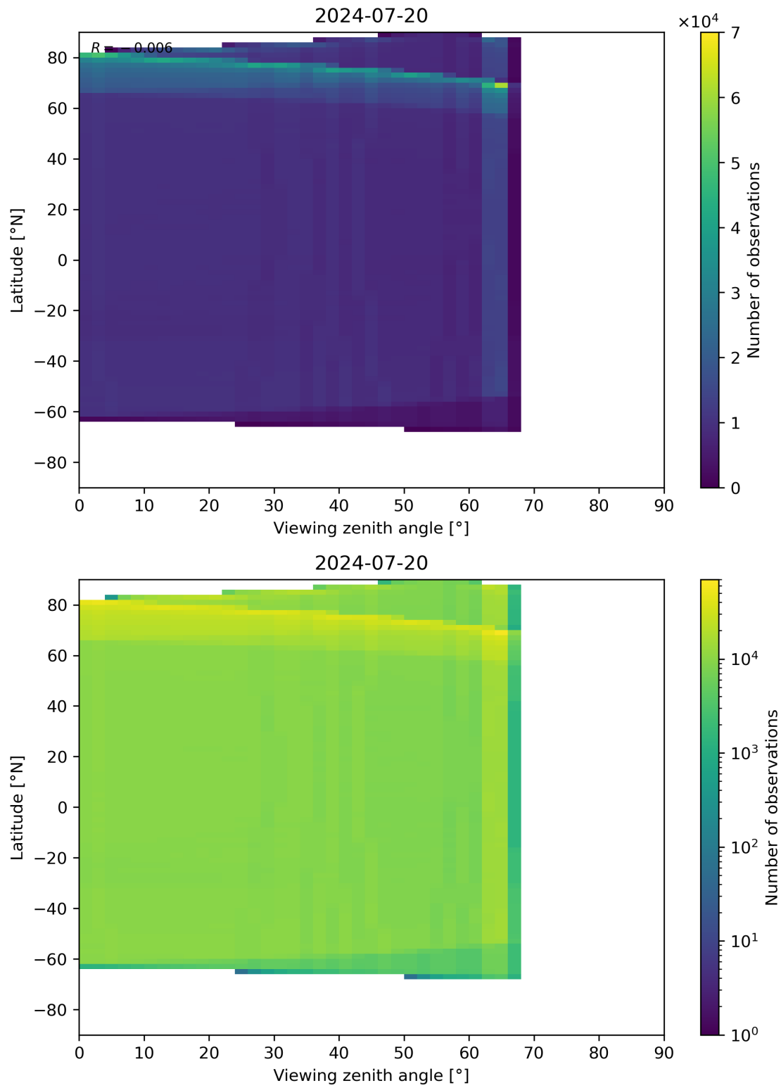
Figure 123: Scatter density plot of “Viewing zenith angle” against “Latitude” for 2024-07-19 to 2024-07-21.
