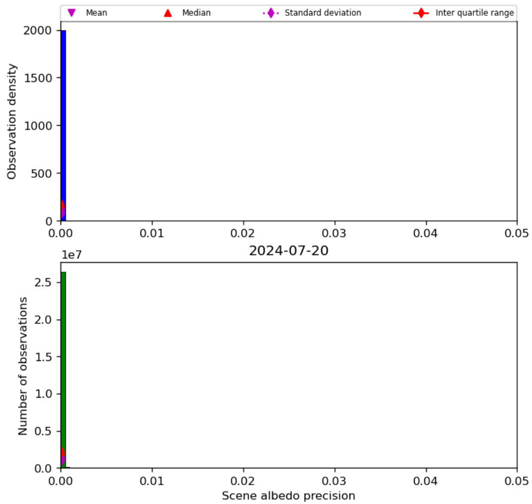
Figure 35: Histogram of “Scene albedo precision” for 2024-07-19 to 2024-07-21
