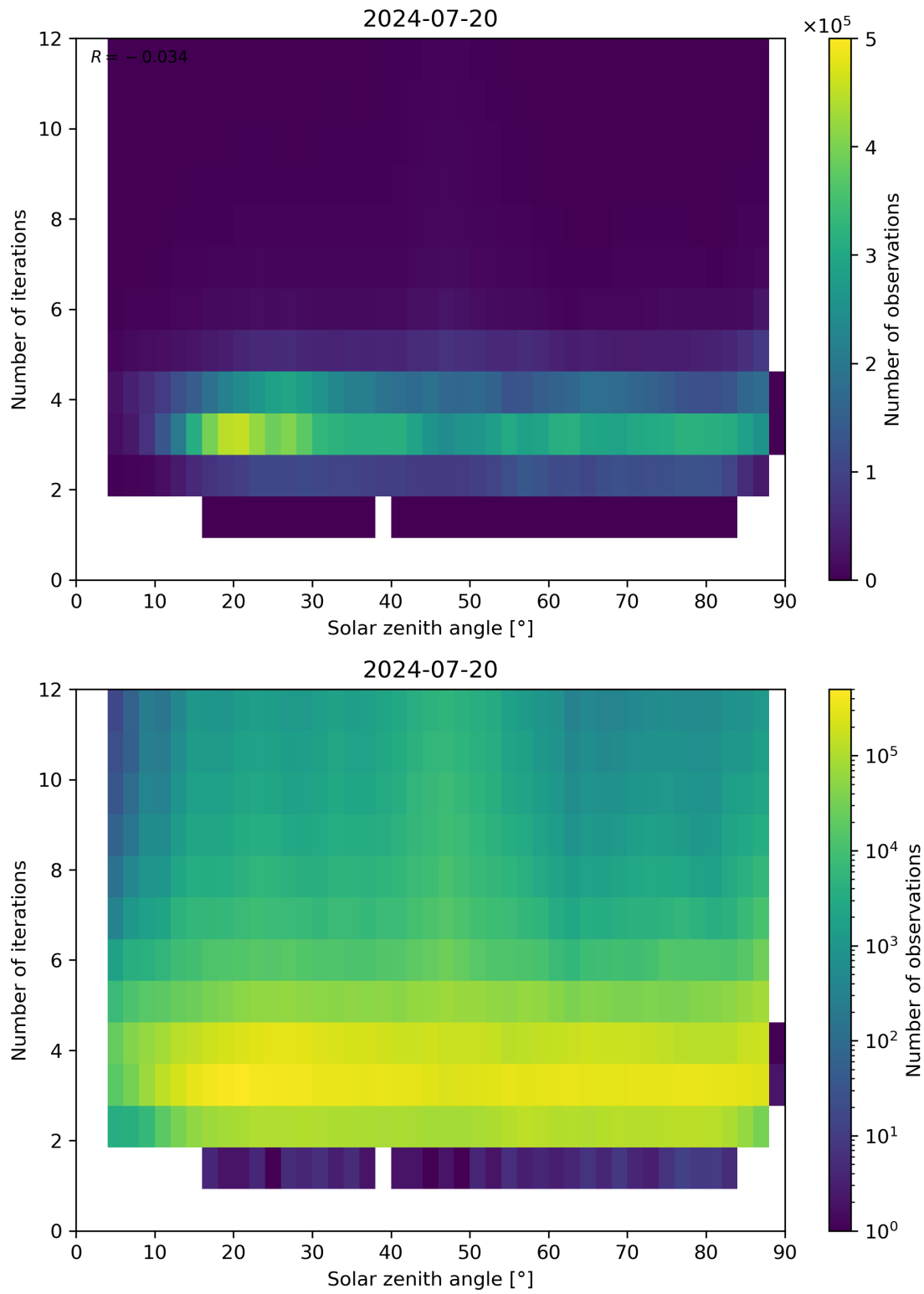
Figure 114: Scatter density plot of “Solar zenith angle” against “Number of iterations” for 2024-07-19 to 2024-07-21.
