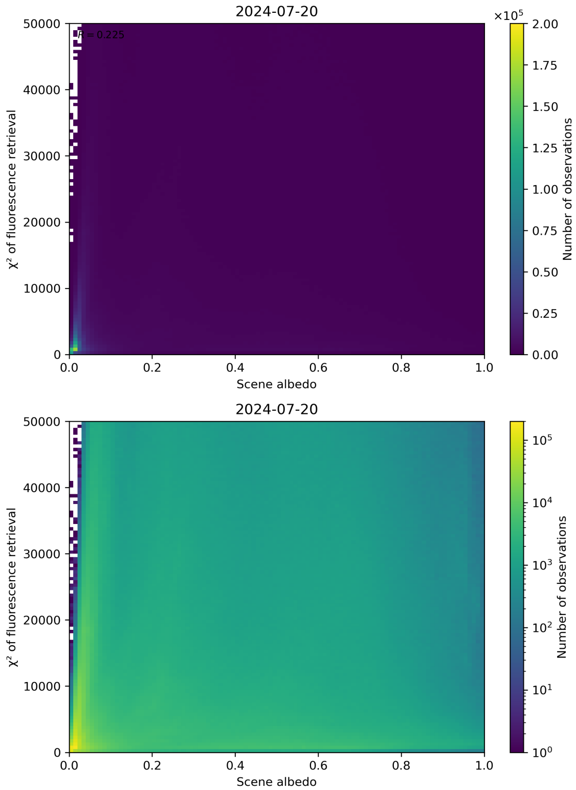
Figure 103: Scatter density plot of “Scene albedo” against “ \chi^2 of fluorescence retrieval” for 2024-07-19 to 2024-07-21.
