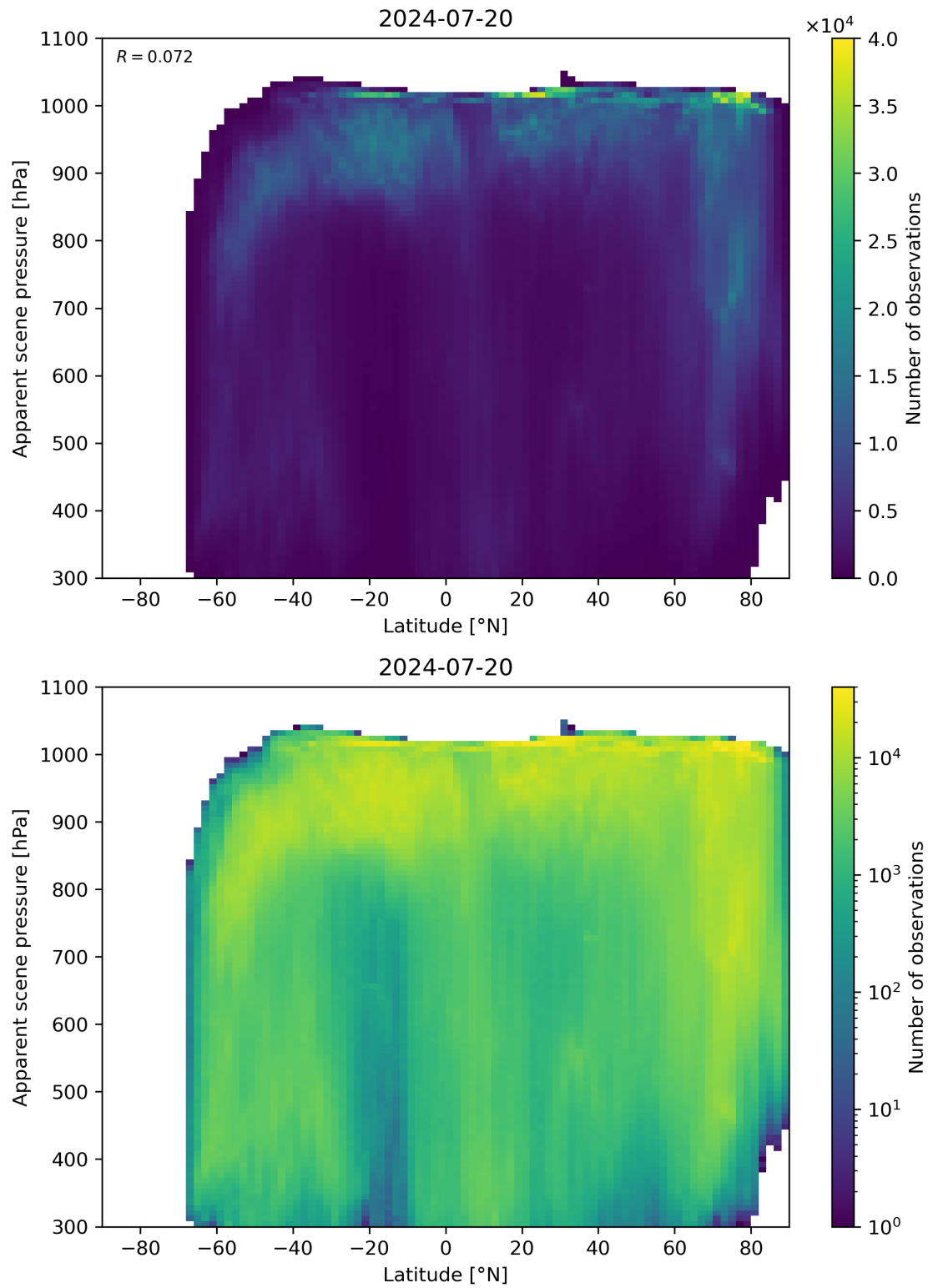
Figure 88: Scatter density plot of “Latitude” against “Apparent scene pressure” for 2024-07-19 to 2024-07-21.
