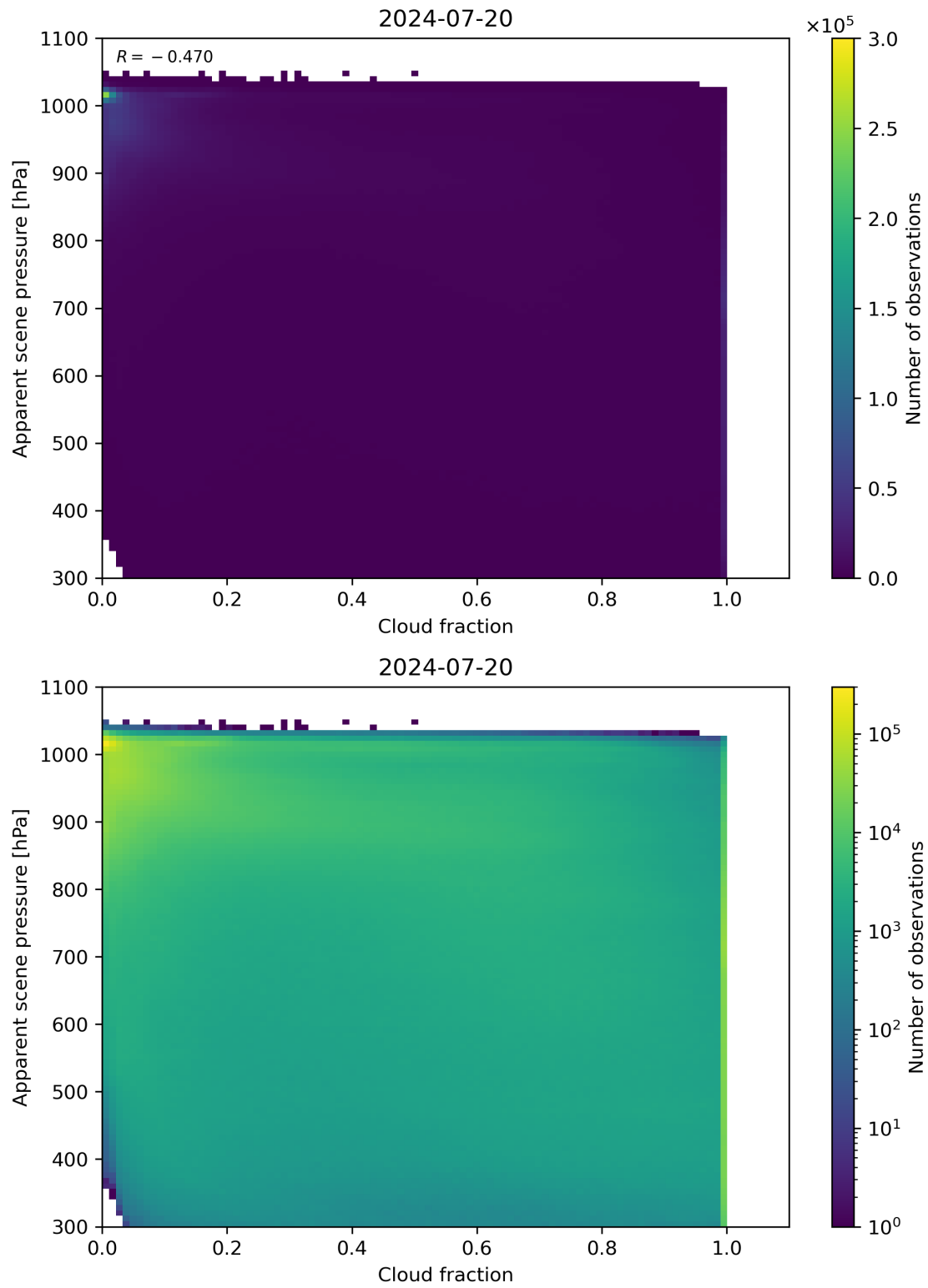
Figure 70: Scatter density plot of “Cloud fraction” against “Apparent scene pressure” for 2024-07-19 to 2024-07-21.
