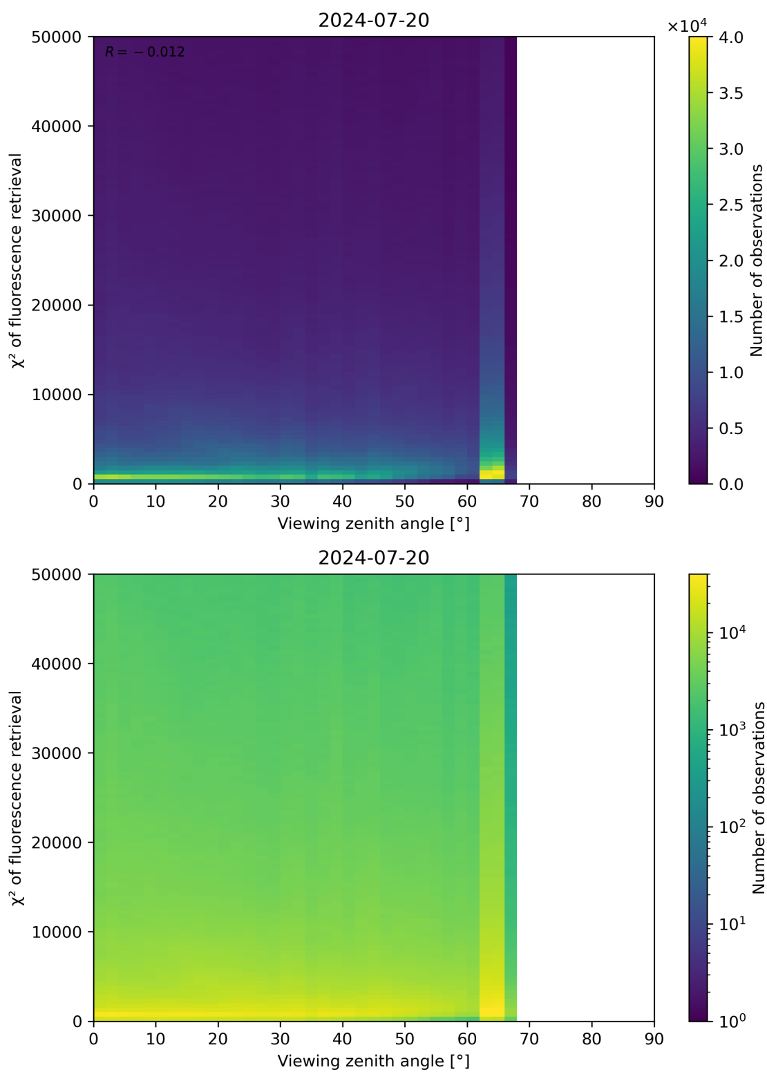
Figure 119: Scatter density plot of “Viewing zenith angle” against “ \chi^2 of fluorescence retrieval” for 2024-07-19 to 2024-07-21.
