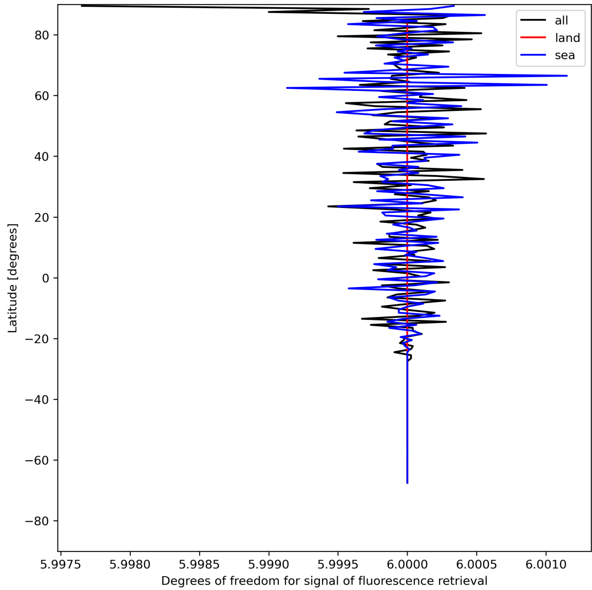
Figure 26: Zonal average of “Degrees of freedom for signal of fluorescence retrieval” for 2024-07-19 to 2024-07-21.
