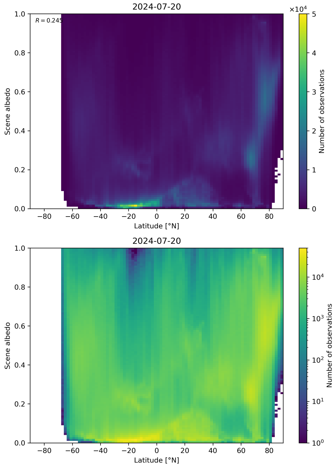
Figure 95: Scatter density plot of “Latitude” against “Scene albedo” for 2024-07-19 to 2024-07-21.
