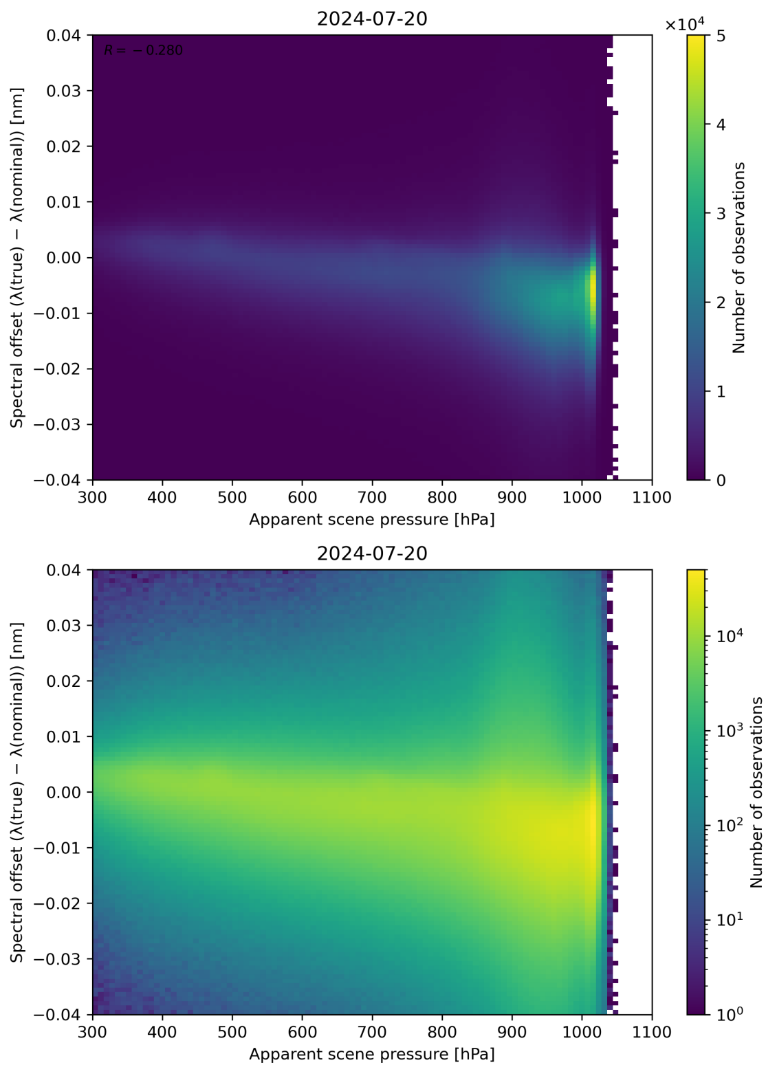
Figure 67: Scatter density plot of “Apparent scene pressure” against “Spectral offset ( \lambda(\text{true}) - \lambda(\text{nominal}) )” for 2024-07-19 to 2024-07-21.
