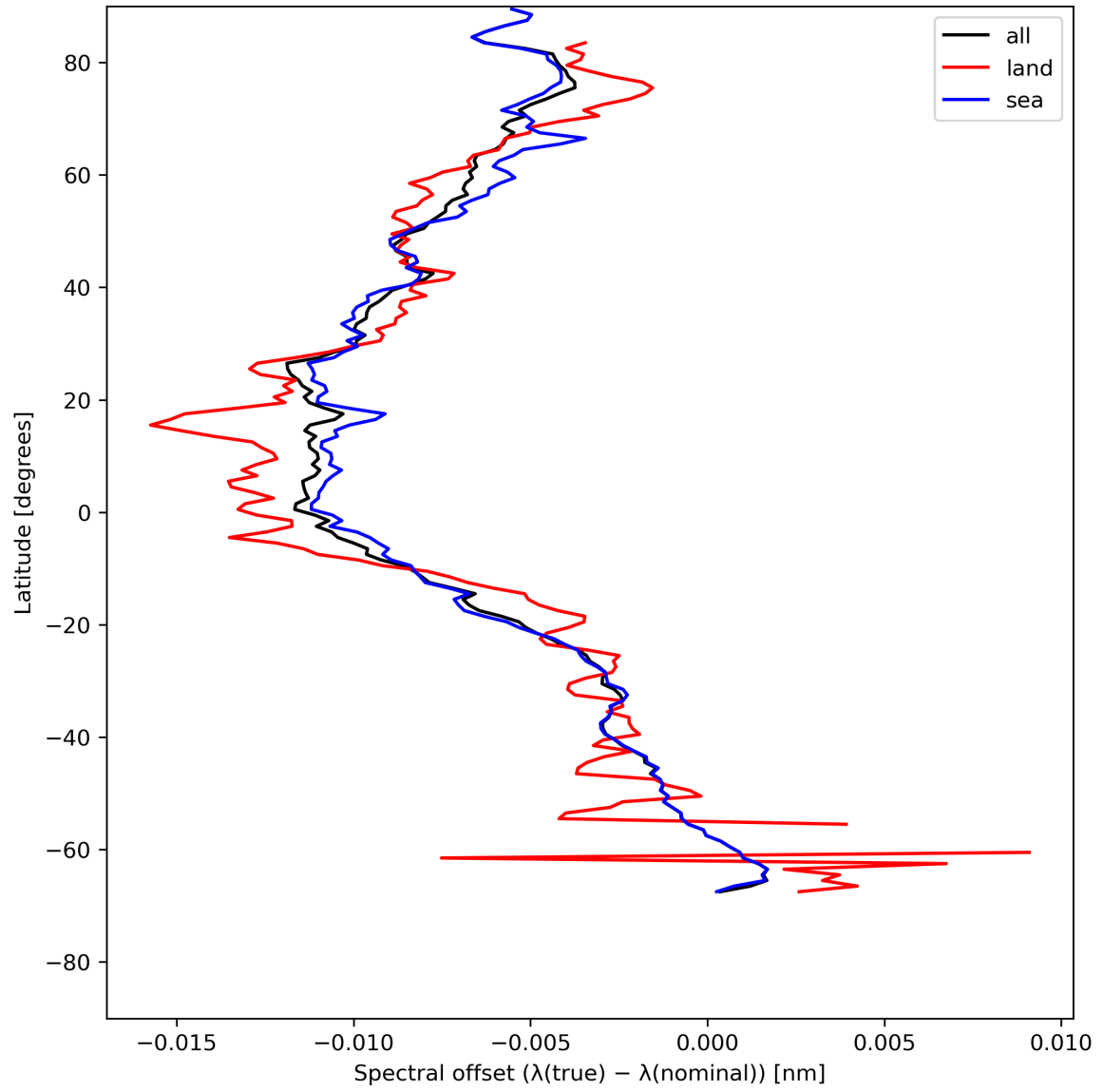
Figure 28: Zonal average of “Spectral offset ( \lambda(\text{true}) - \lambda(\text{nominal}) )” for 2024-07-19 to 2024-07-21.
