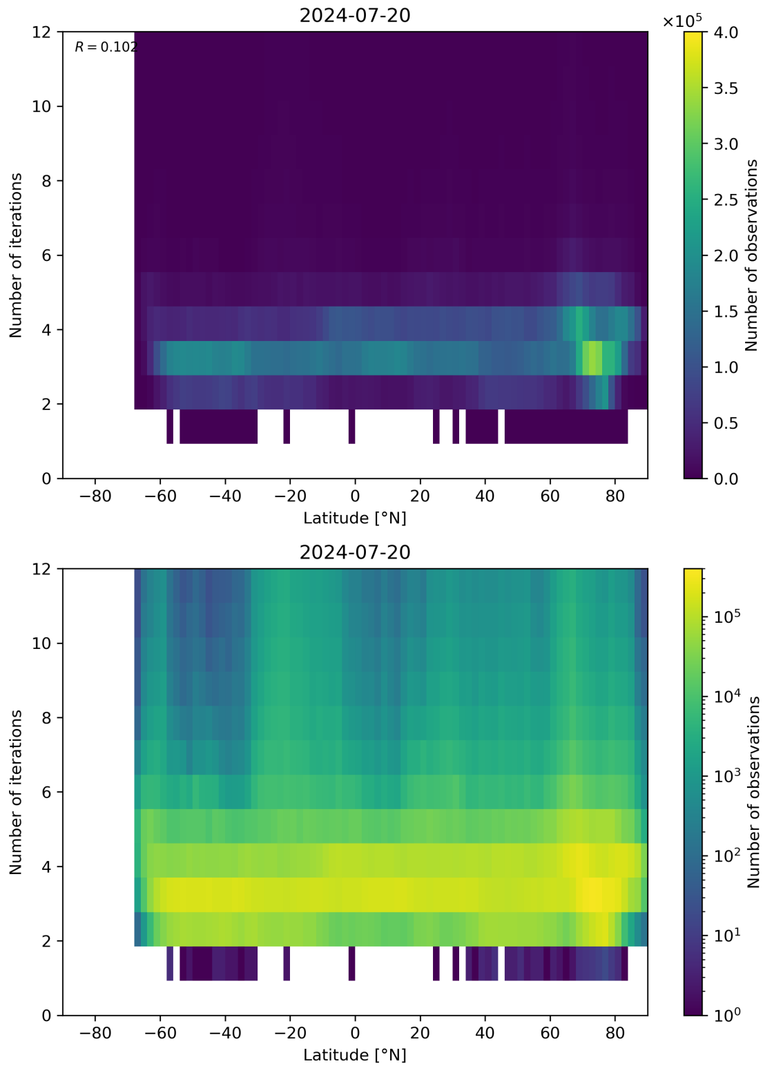
Figure 93: Scatter density plot of “Latitude” against “Number of iterations” for 2024-07-19 to 2024-07-21.
