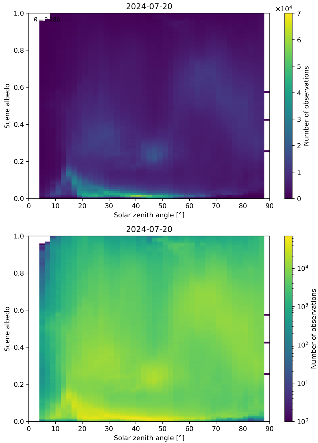
Figure 116: Scatter density plot of “Solar zenith angle” against “Scene albedo” for 2024-07-19 to 2024-07-21.
