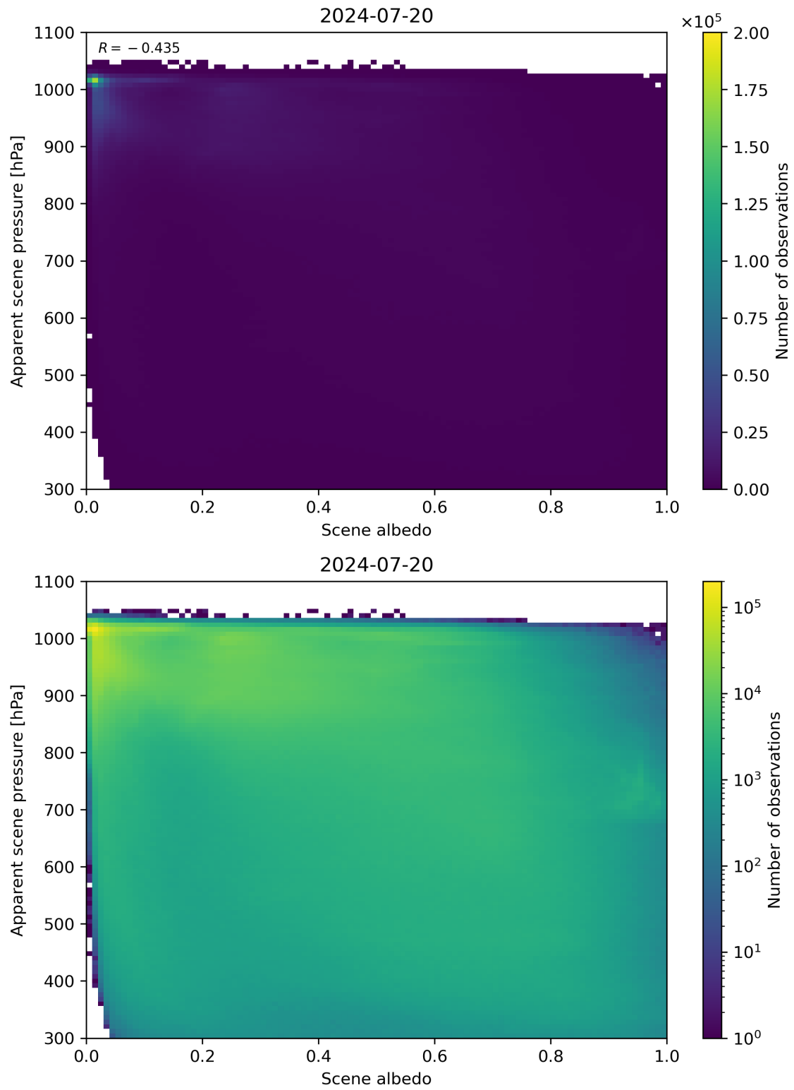
Figure 102: Scatter density plot of “Scene albedo” against “Apparent scene pressure” for 2024-07-19 to 2024-07-21.
