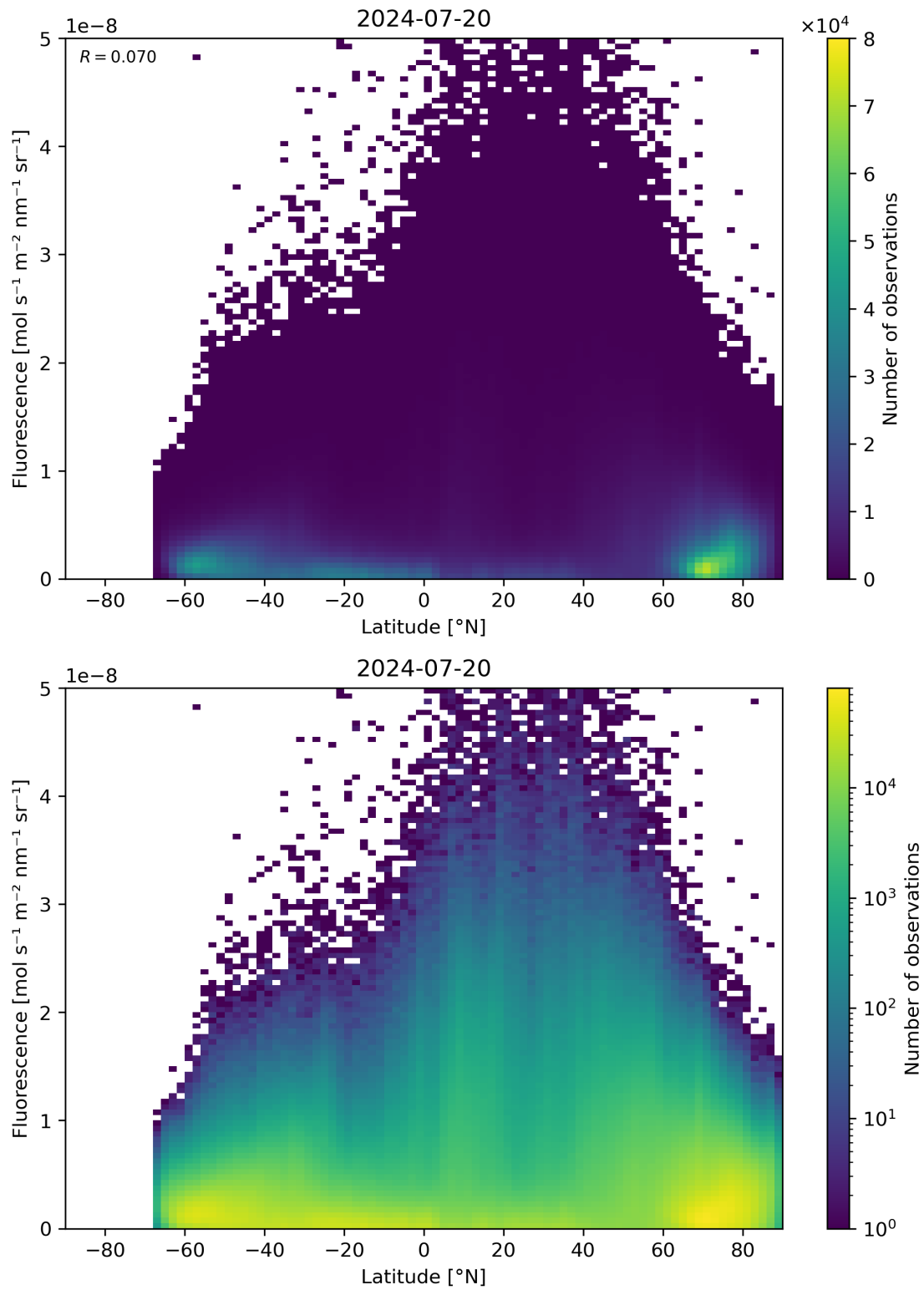
Figure 92: Scatter density plot of “Latitude” against “Fluorescence” for 2024-07-19 to 2024-07-21.
