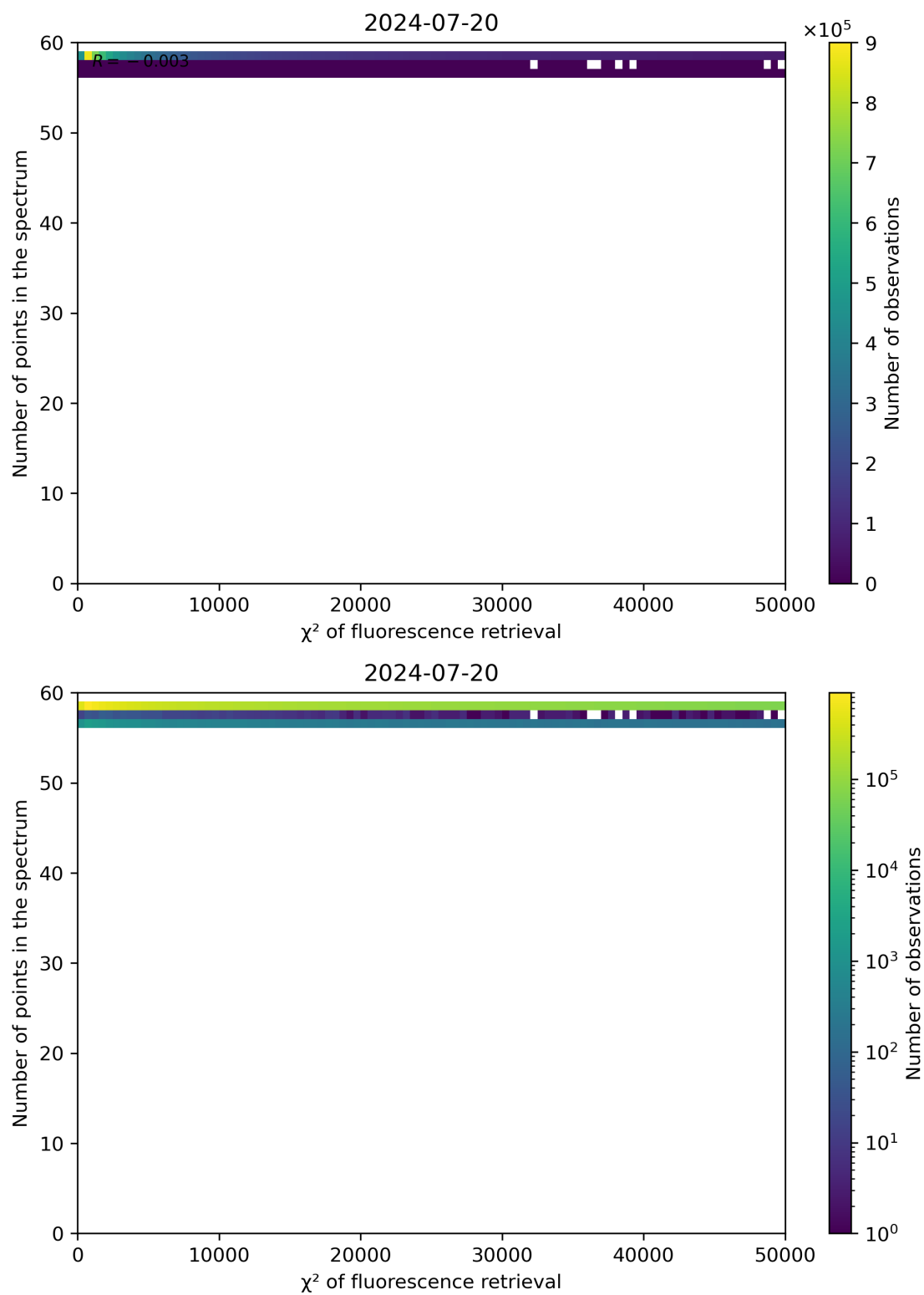
Figure 68: Scatter density plot of " \chi^2 of fluorescence retrieval" against "Number of points in the spectrum" for 2024-07-19 to 2024-07-21.
