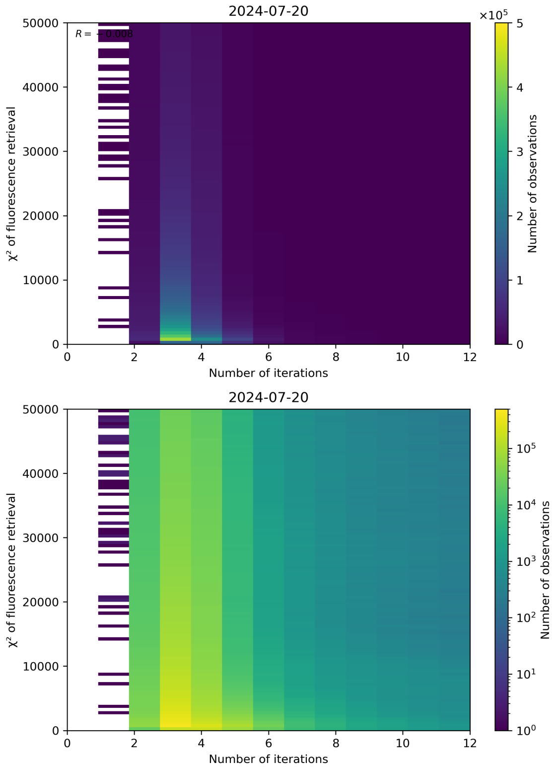
Figure 97: Scatter density plot of “Number of iterations” against “ \chi^2 of fluorescence retrieval” for 2024-07-19 to 2024-07-21.
