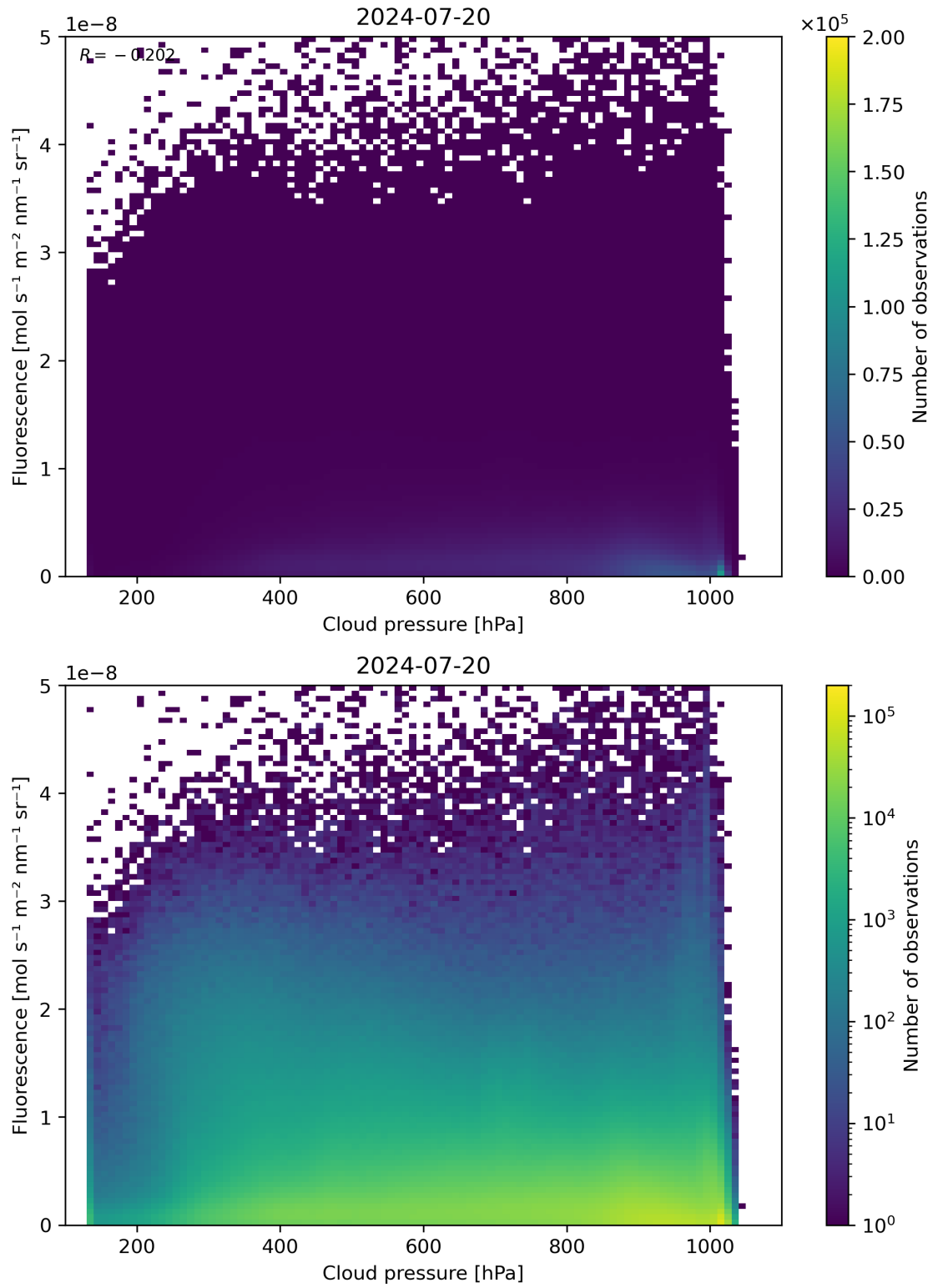
Figure 80: Scatter density plot of “Cloud pressure” against “Fluorescence” for 2024-07-19 to 2024-07-21.
