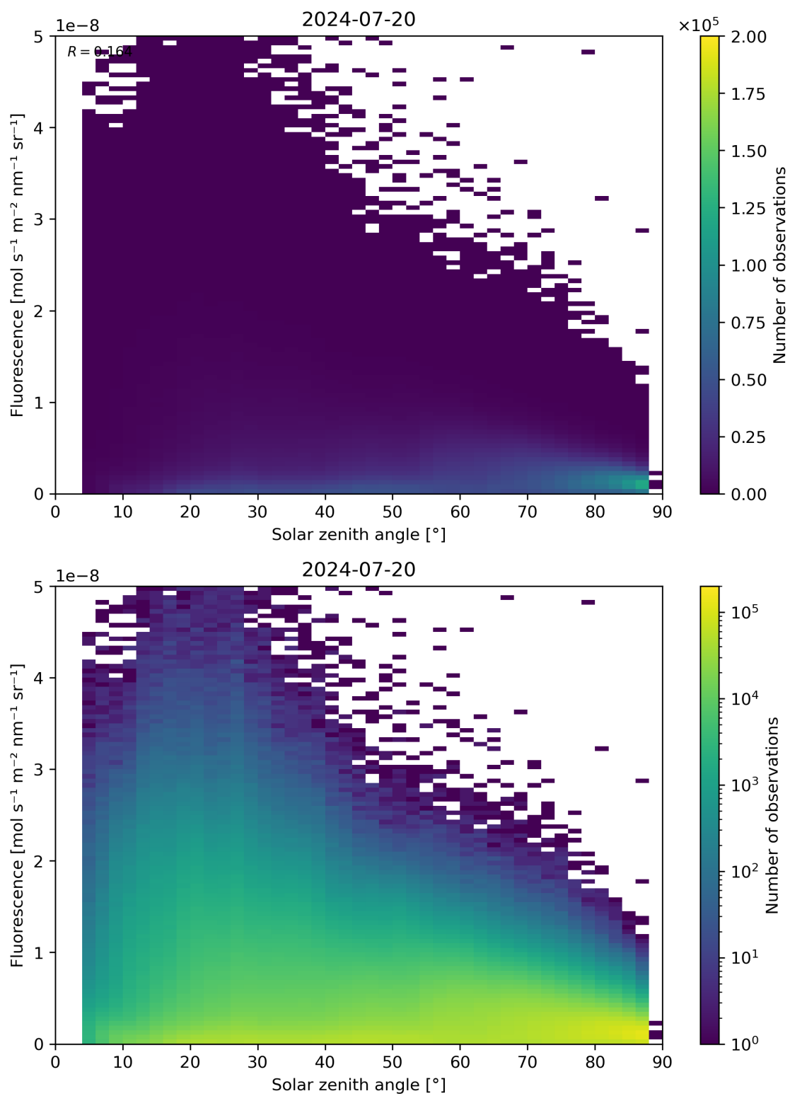
Figure 112: Scatter density plot of “Solar zenith angle” against “Fluorescence” for 2024-07-19 to 2024-07-21.
