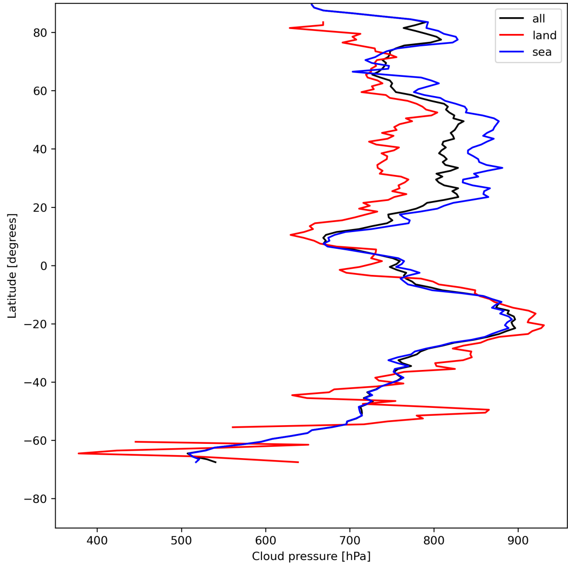
Figure 13: Zonal average of “Cloud pressure” for 2024-07-19 to 2024-07-21.
