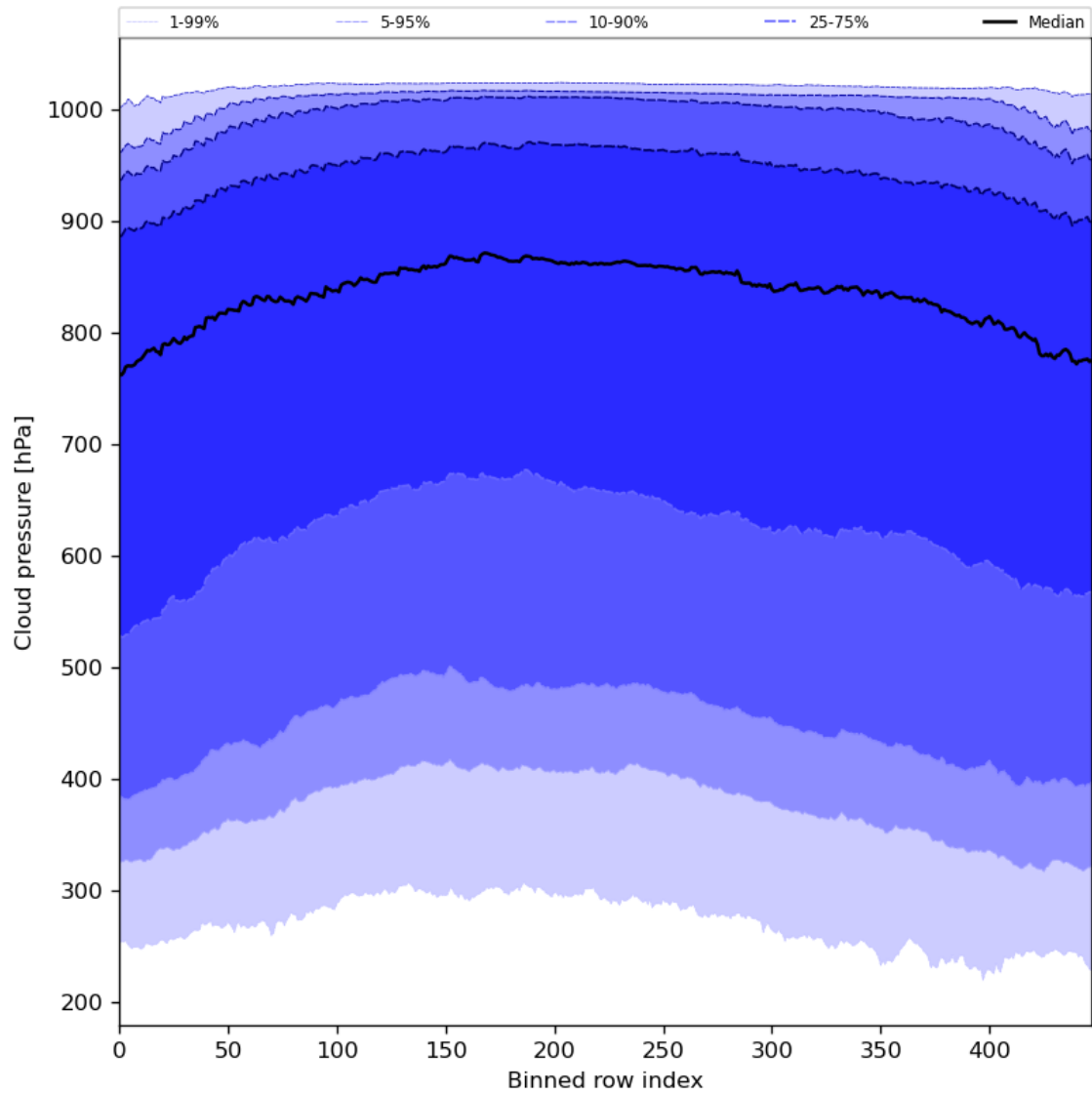
Figure 47: Along track statistics of "Cloud pressure" for 2024-07-19 to 2024-07-21
