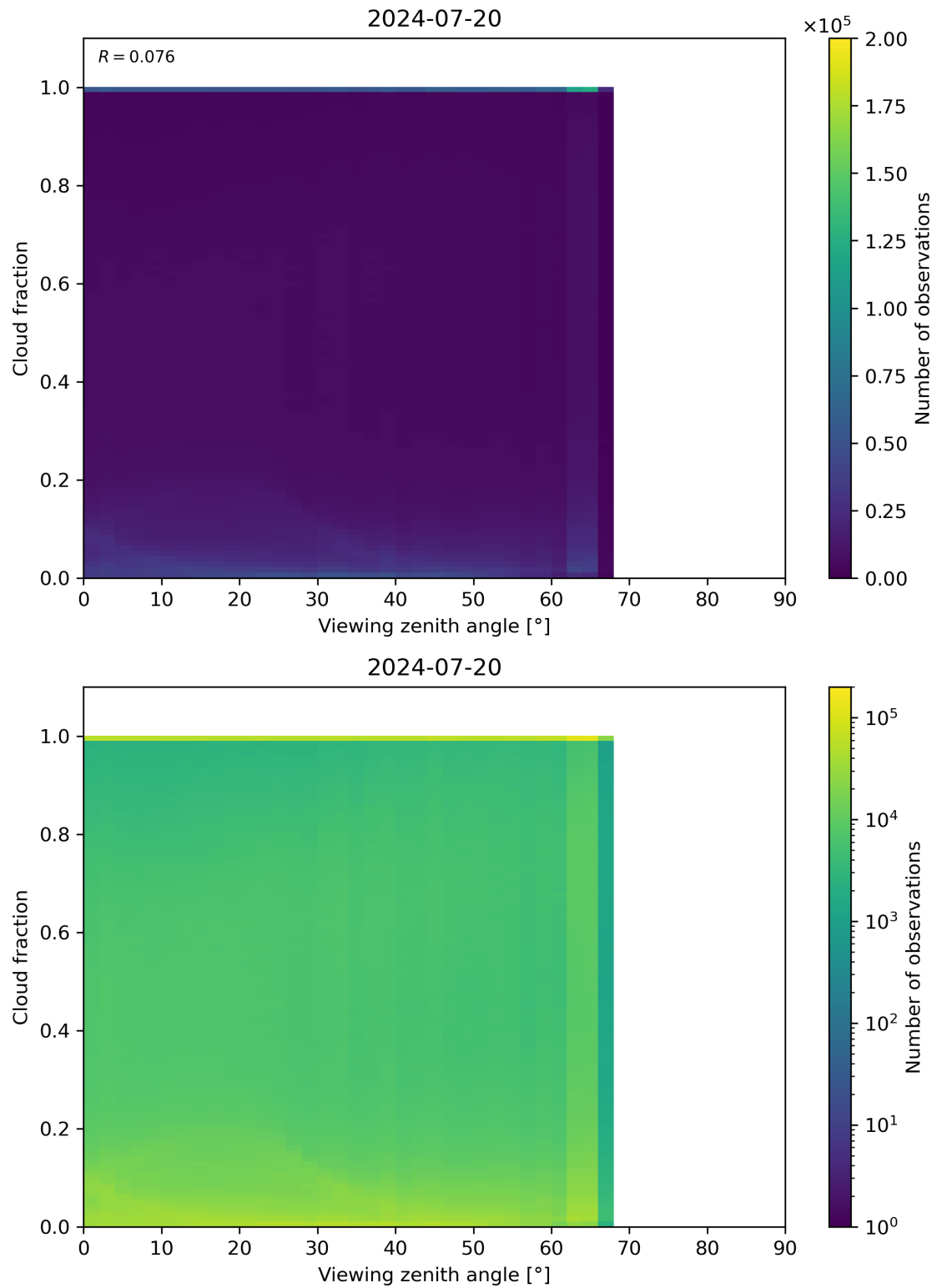
Figure 120: Scatter density plot of “Viewing zenith angle” against “Cloud fraction” for 2024-07-19 to 2024-07-21.
