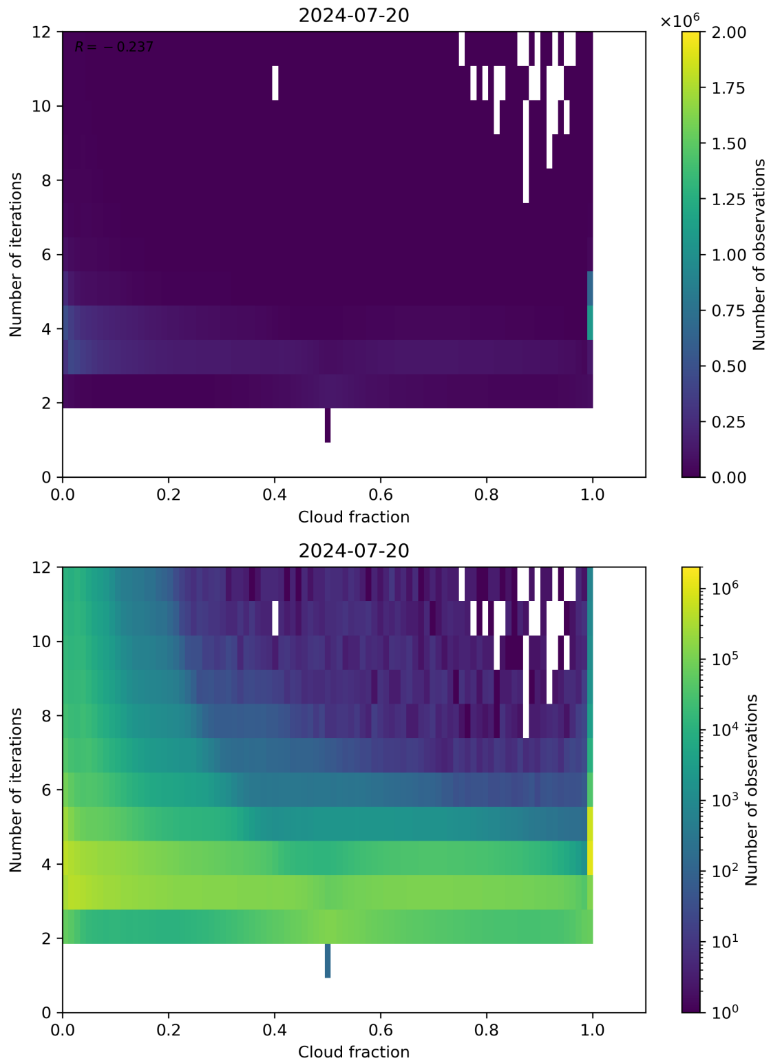
Figure 73: Scatter density plot of “Cloud fraction” against “Number of iterations” for 2024-07-19 to 2024-07-21.
