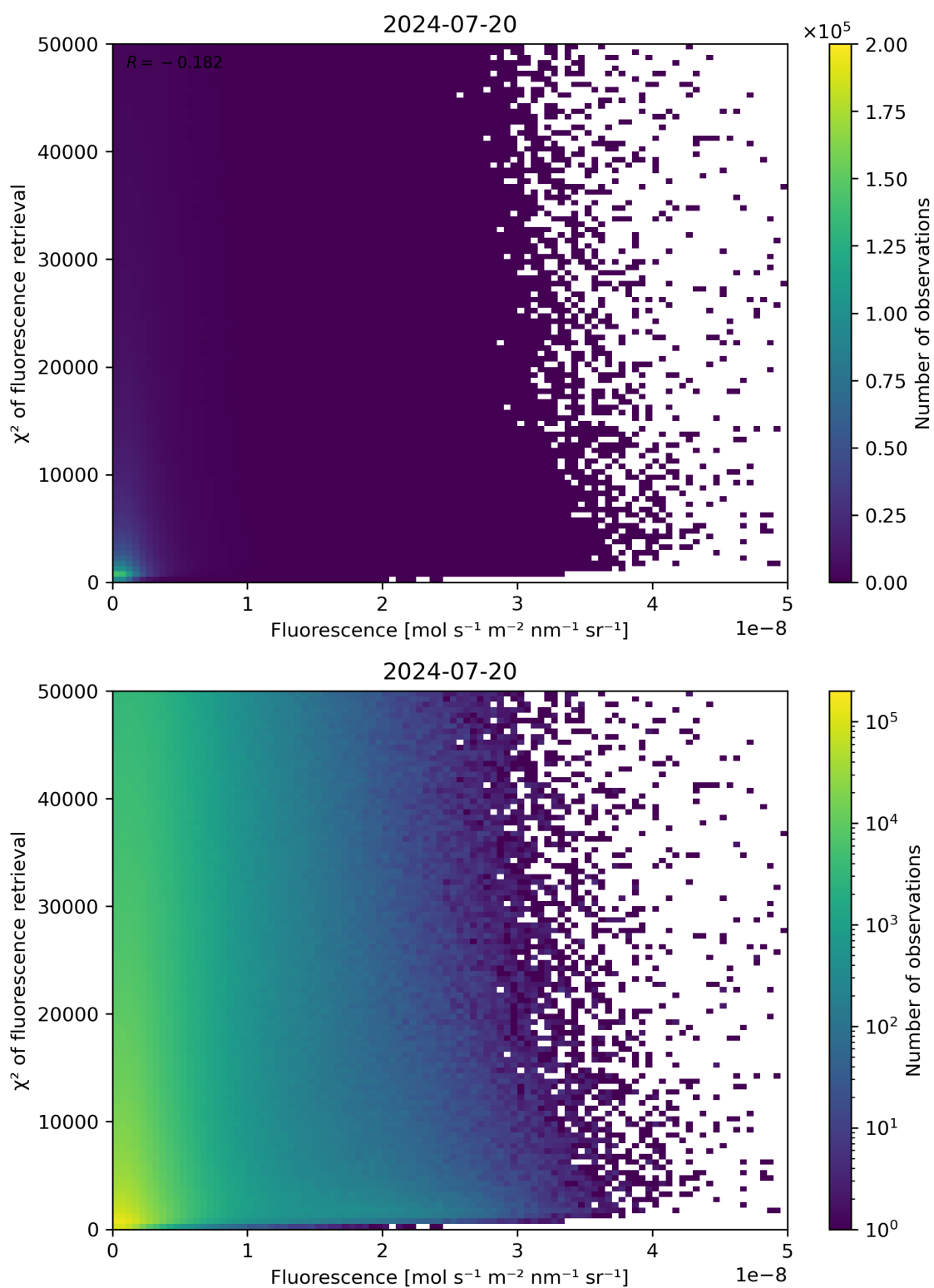
Figure 85: Scatter density plot of “Fluorescence” against “ \chi^2 of fluorescence retrieval” for 2024-07-19 to 2024-07-21.
