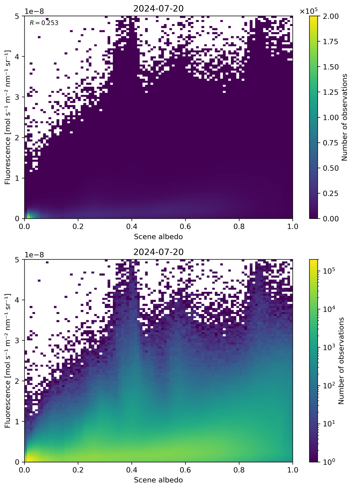
Figure 104: Scatter density plot of “Scene albedo” against “Fluorescence” for 2024-07-19 to 2024-07-21.
