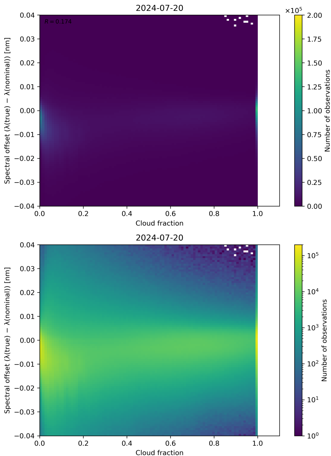
Figure 76: Scatter density plot of “Cloud fraction” against “Spectral offset ( \lambda(\text{true}) - \lambda(\text{nominal}) )” for 2024-07-19 to 2024-07-21.
