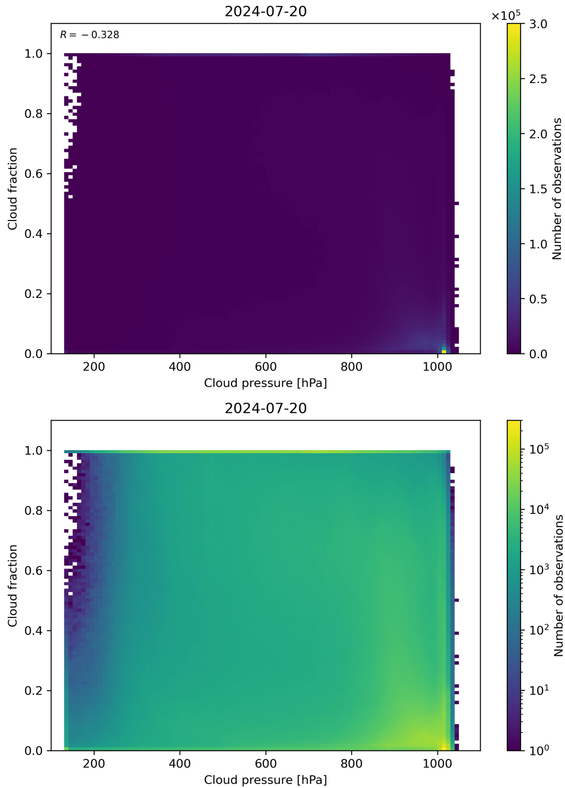
Figure 79: Scatter density plot of “Cloud pressure” against “Cloud fraction” for 2024-07-19 to 2024-07-21.
