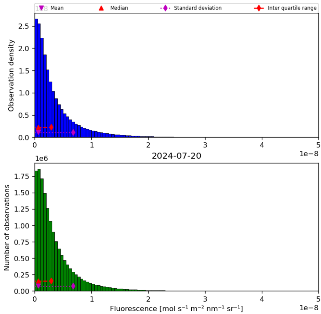
Figure 40: Histogram of “Fluorescence” for 2024-07-19 to 2024-07-21
