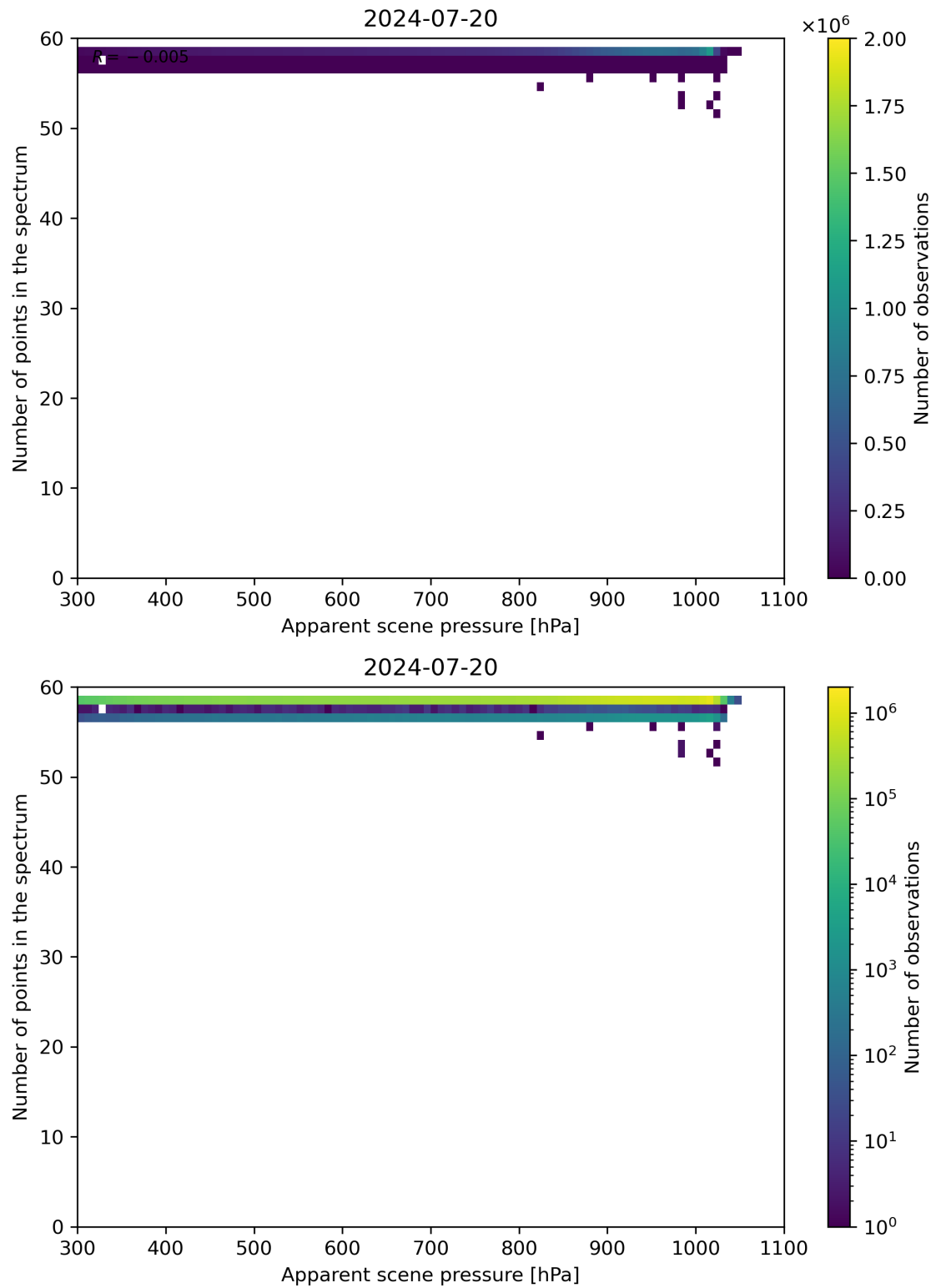
Figure 66: Scatter density plot of “Apparent scene pressure” against “Number of points in the spectrum” for 2024-07-19 to 2024-07-21.
