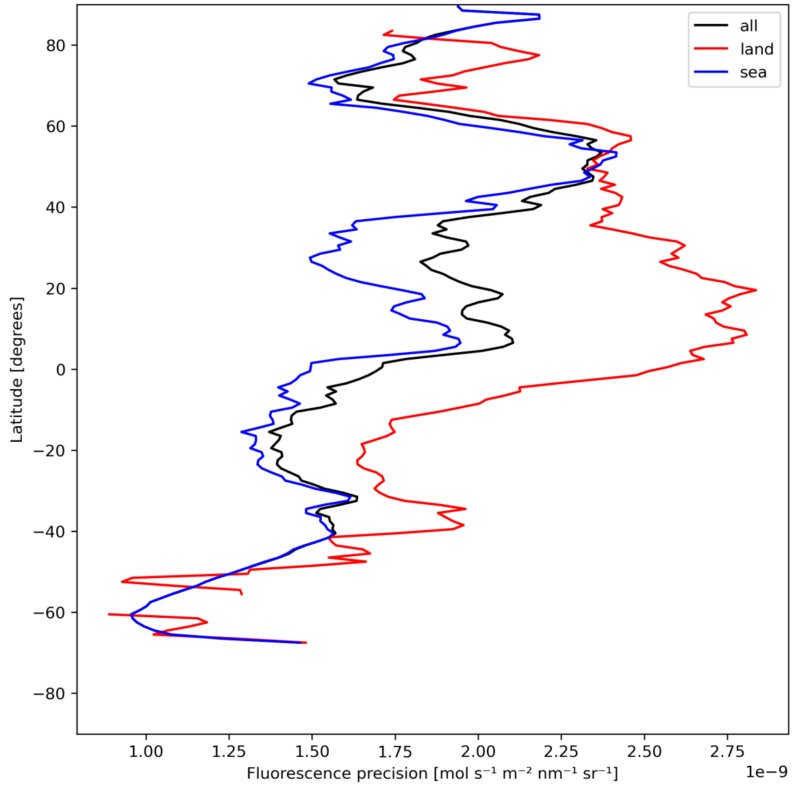
Figure 24: Zonal average of “Fluorescence precision” for 2024-07-19 to 2024-07-21.
