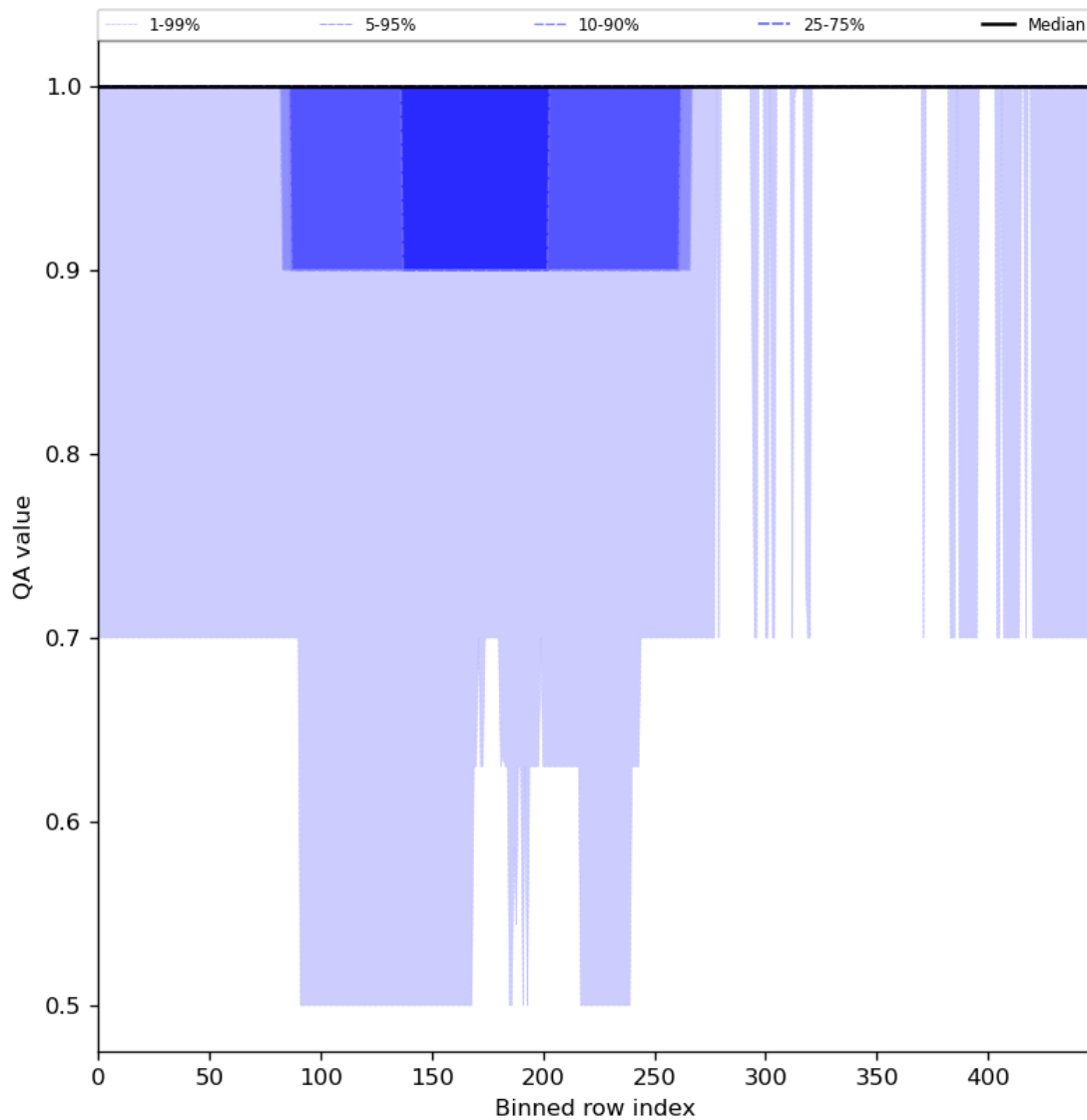
Figure 46: Along track statistics of “QA value” for 2024-07-19 to 2024-07-21
