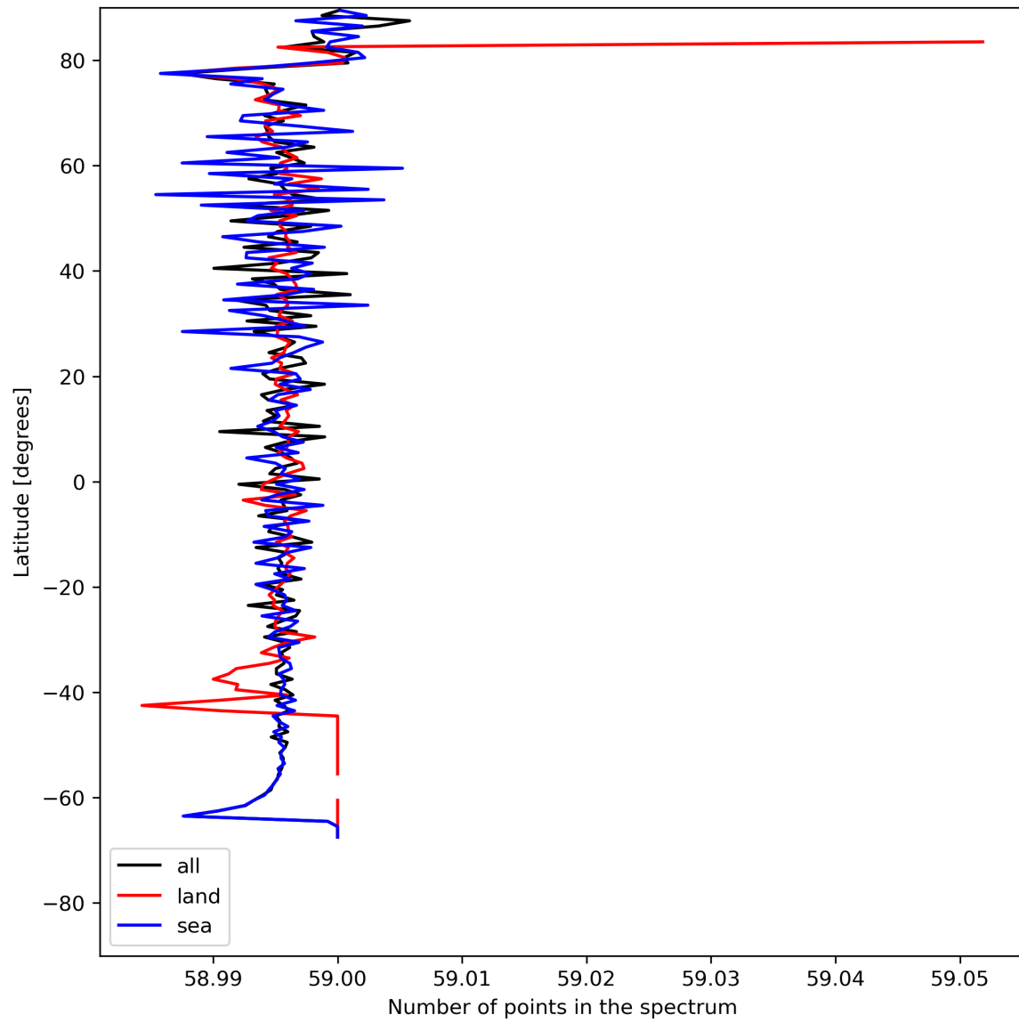
Figure 27: Zonal average of “Number of points in the spectrum” for 2024-07-19 to 2024-07-21.
