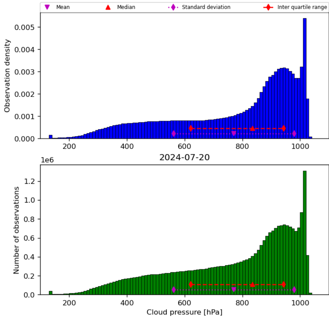
Figure 30: Histogram of “Cloud pressure” for 2024-07-19 to 2024-07-21
