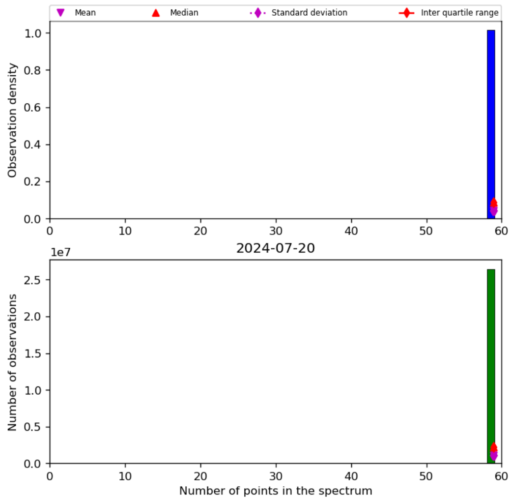
Figure 44: Histogram of “Number of points in the spectrum” for 2024-07-19 to 2024-07-21
