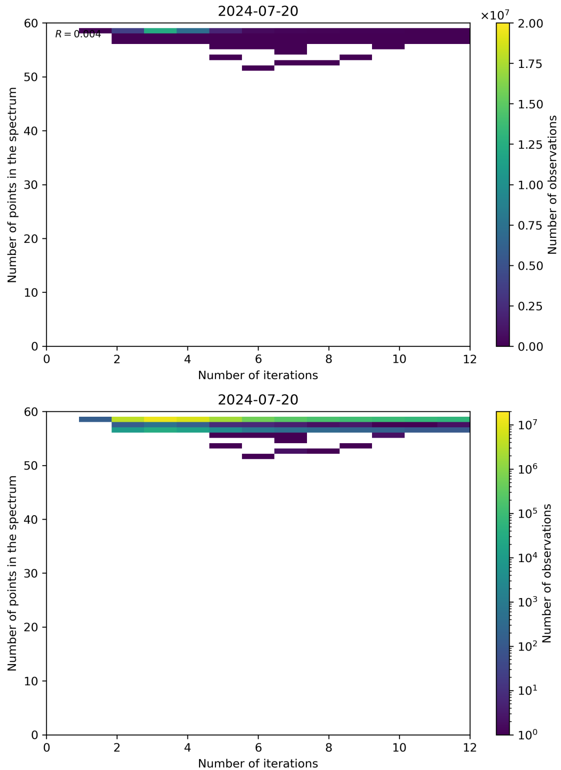
Figure 99: Scatter density plot of “Number of iterations” against “Number of points in the spectrum” for 2024-07-19 to 2024-07-21.
