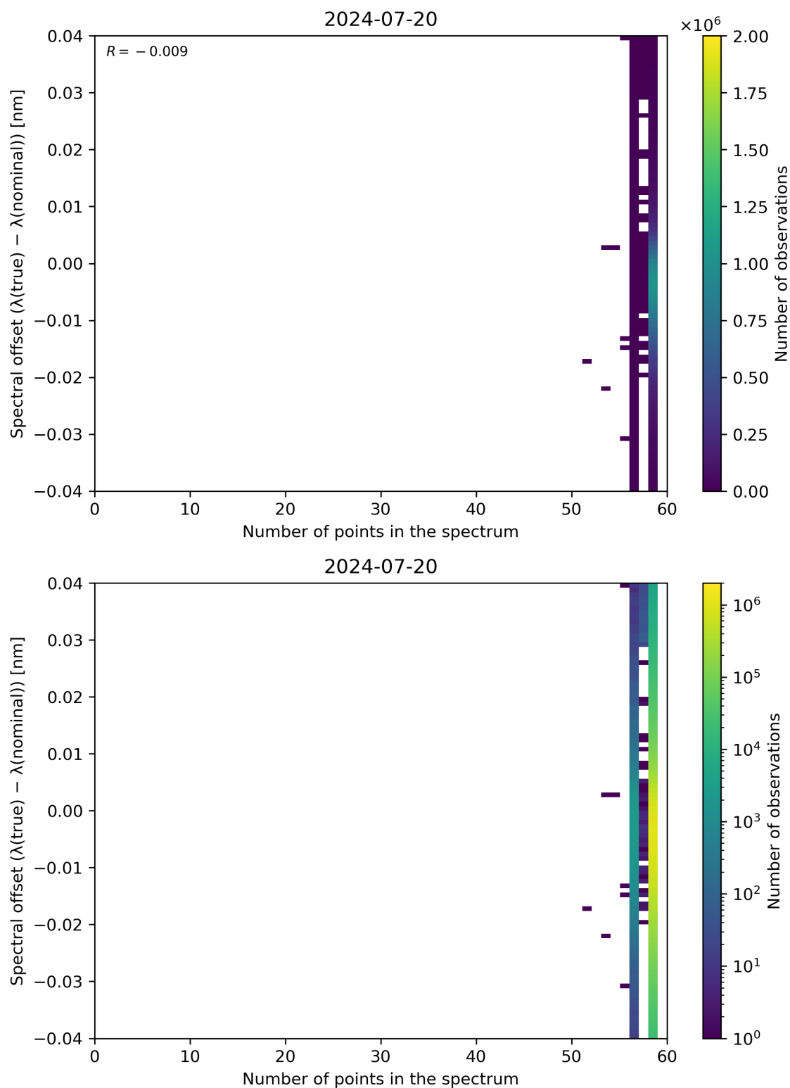
Figure 101: Scatter density plot of “Number of points in the spectrum” against “Spectral offset ( \lambda(\text{true}) - \lambda(\text{nominal}) )” for 2024-07-19 to 2024-07-21.
