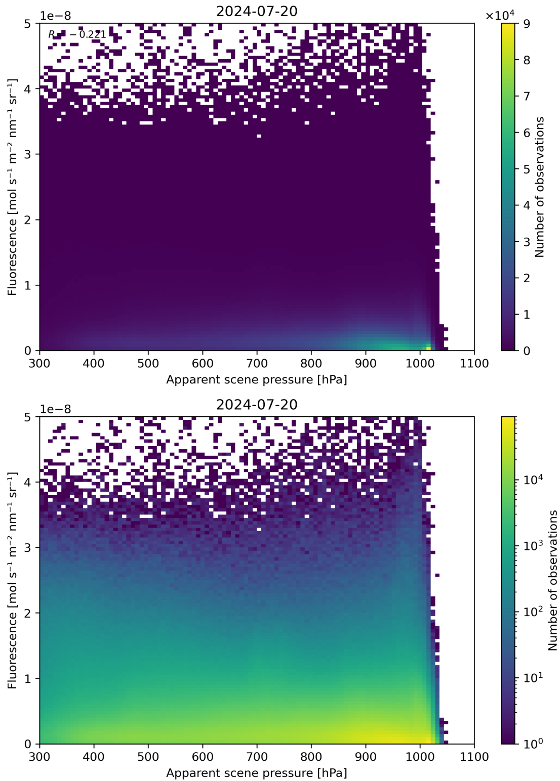
Figure 64: Scatter density plot of “Apparent scene pressure” against “Fluorescence” for 2024-07-19 to 2024-07-21.
