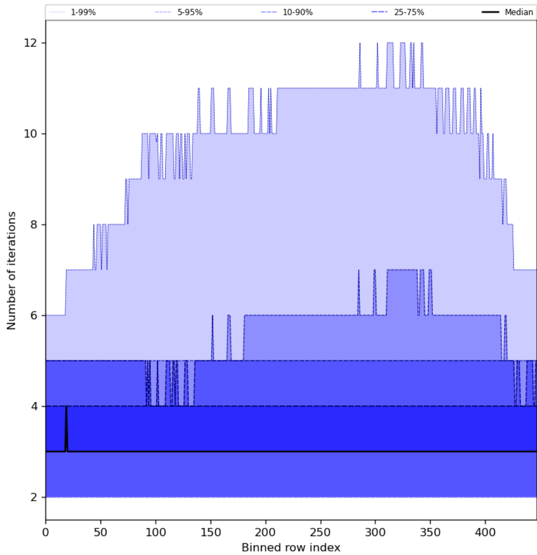
Figure 56: Along track statistics of “Number of iterations” for 2024-07-19 to 2024-07-21
