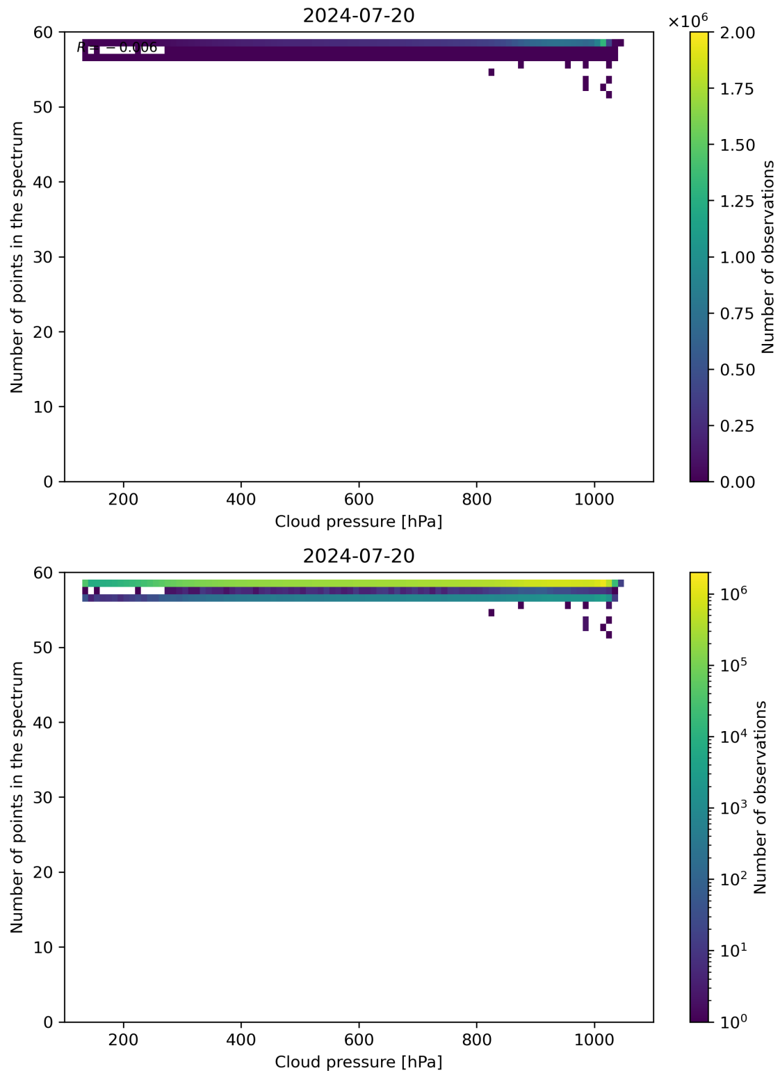
Figure 82: Scatter density plot of “Cloud pressure” against “Number of points in the spectrum” for 2024-07-19 to 2024-07-21.
