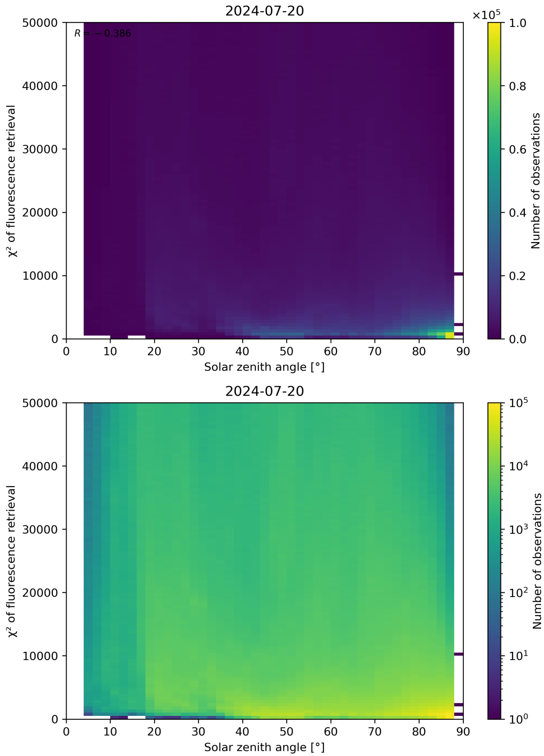
Figure 109: Scatter density plot of “Solar zenith angle” against “ \chi^2 of fluorescence retrieval” for 2024-07-19 to 2024-07-21.
