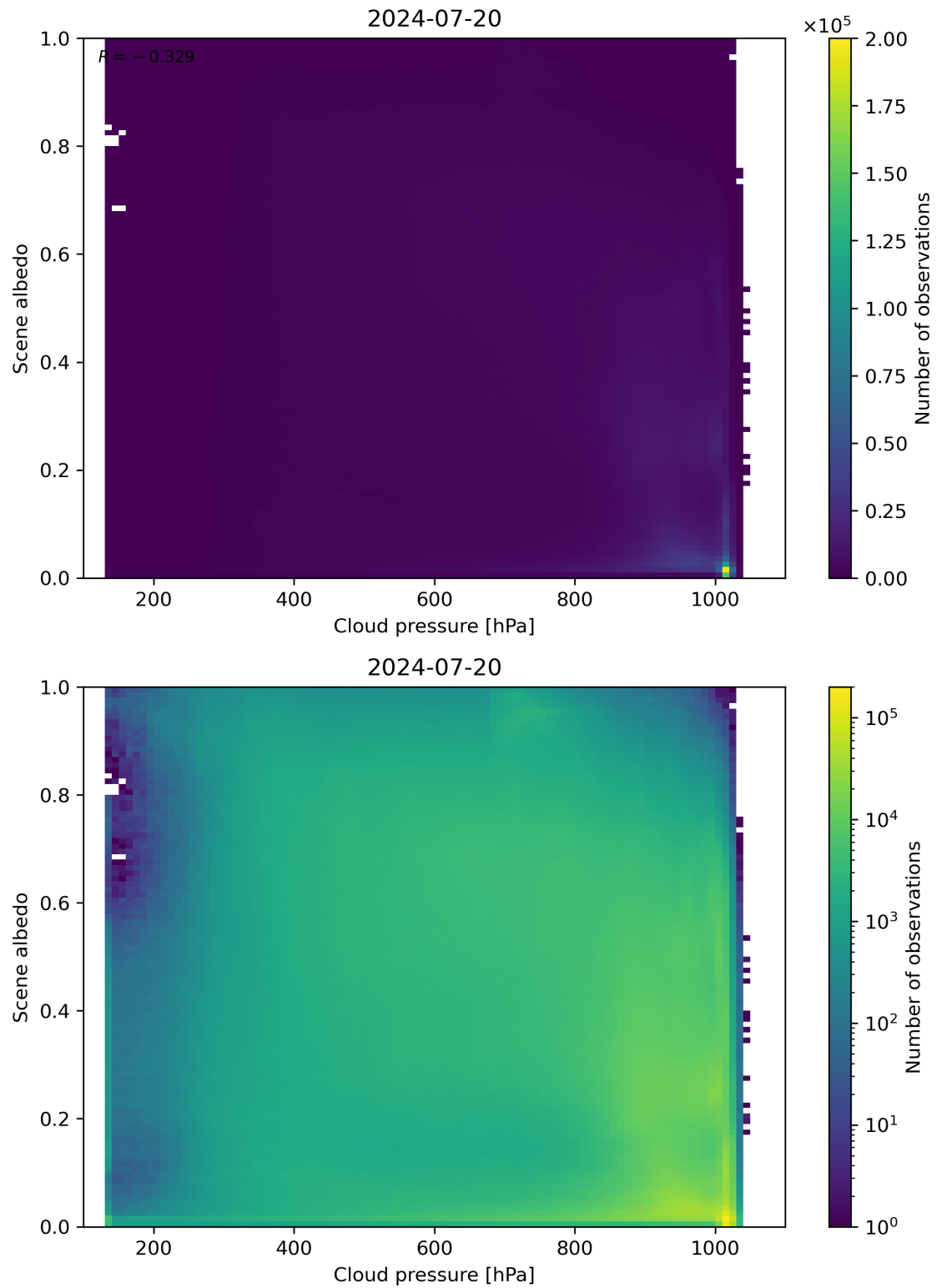
Figure 83: Scatter density plot of “Cloud pressure” against “Scene albedo” for 2024-07-19 to 2024-07-21.
