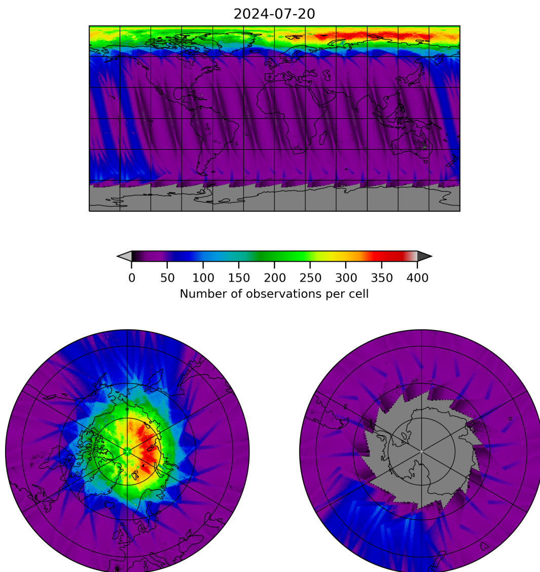
Figure 11: Map of the number of observations for 2024-07-19 to 2024-07-21
