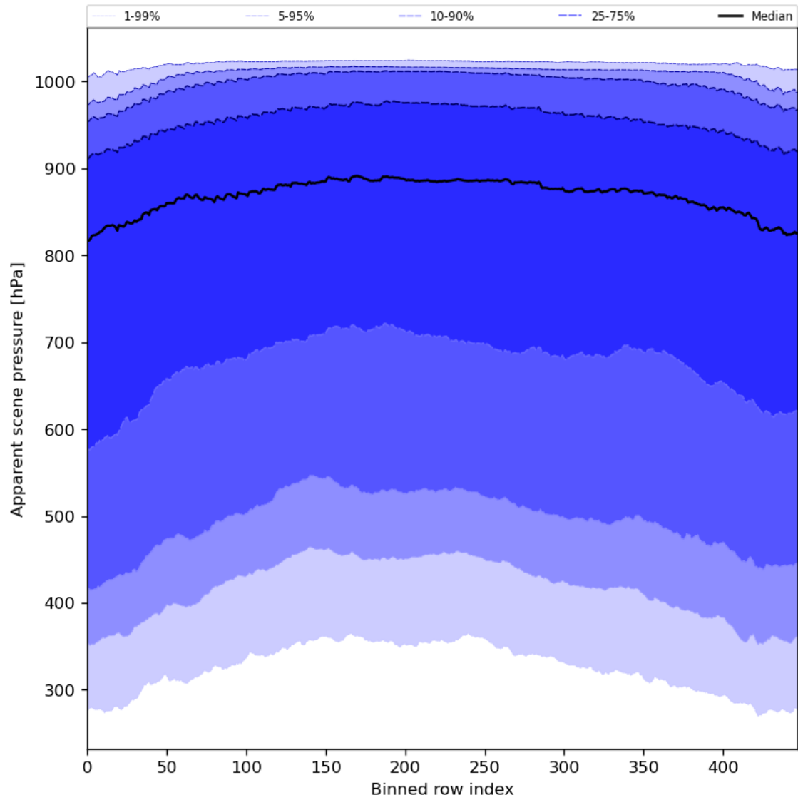
Figure 53: Along track statistics of “Apparent scene pressure” for 2024-07-19 to 2024-07-21
