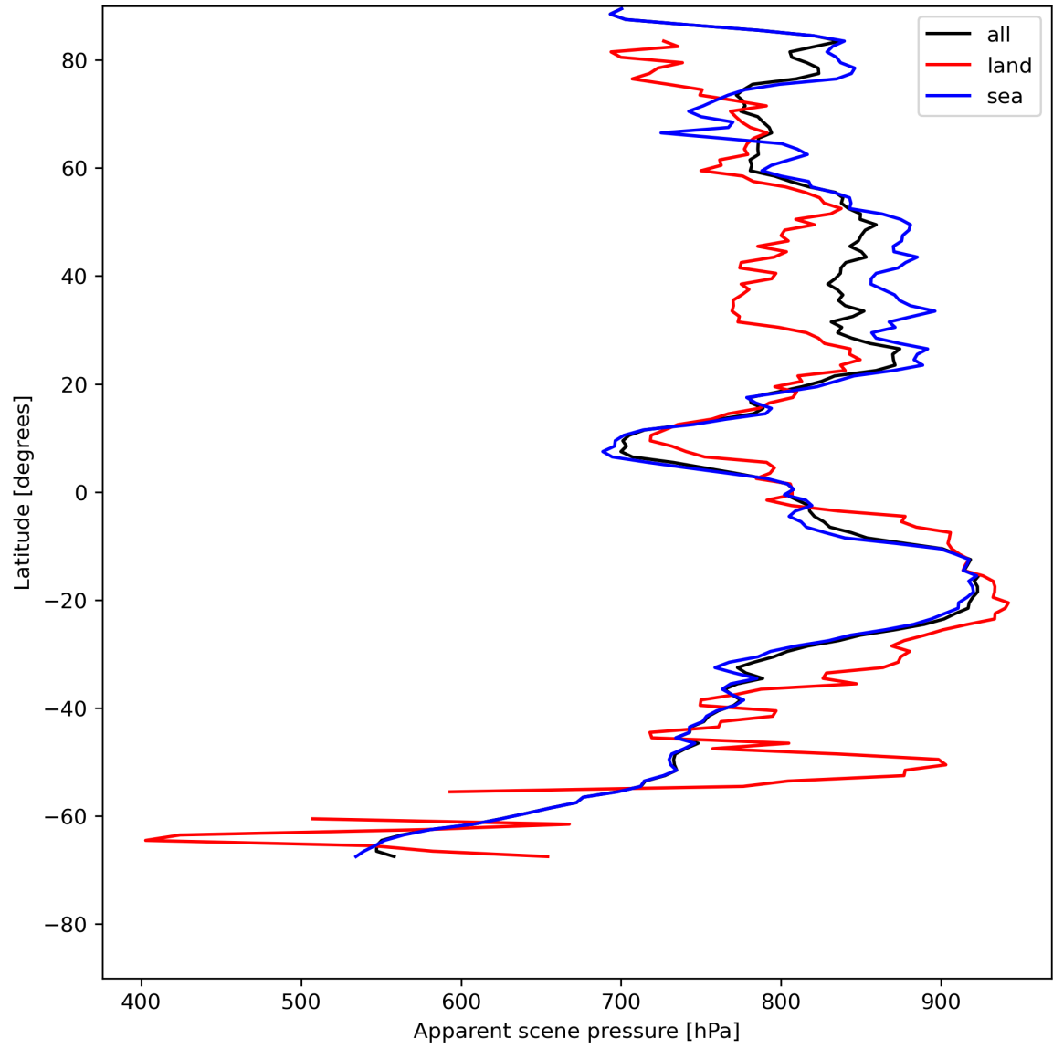
Figure 19: Zonal average of “Apparent scene pressure” for 2024-07-19 to 2024-07-21.
