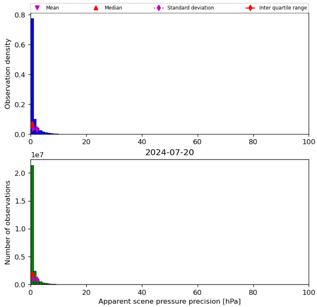
Figure 37: Histogram of “Apparent scene pressure precision” for 2024-07-19 to 2024-07-21
