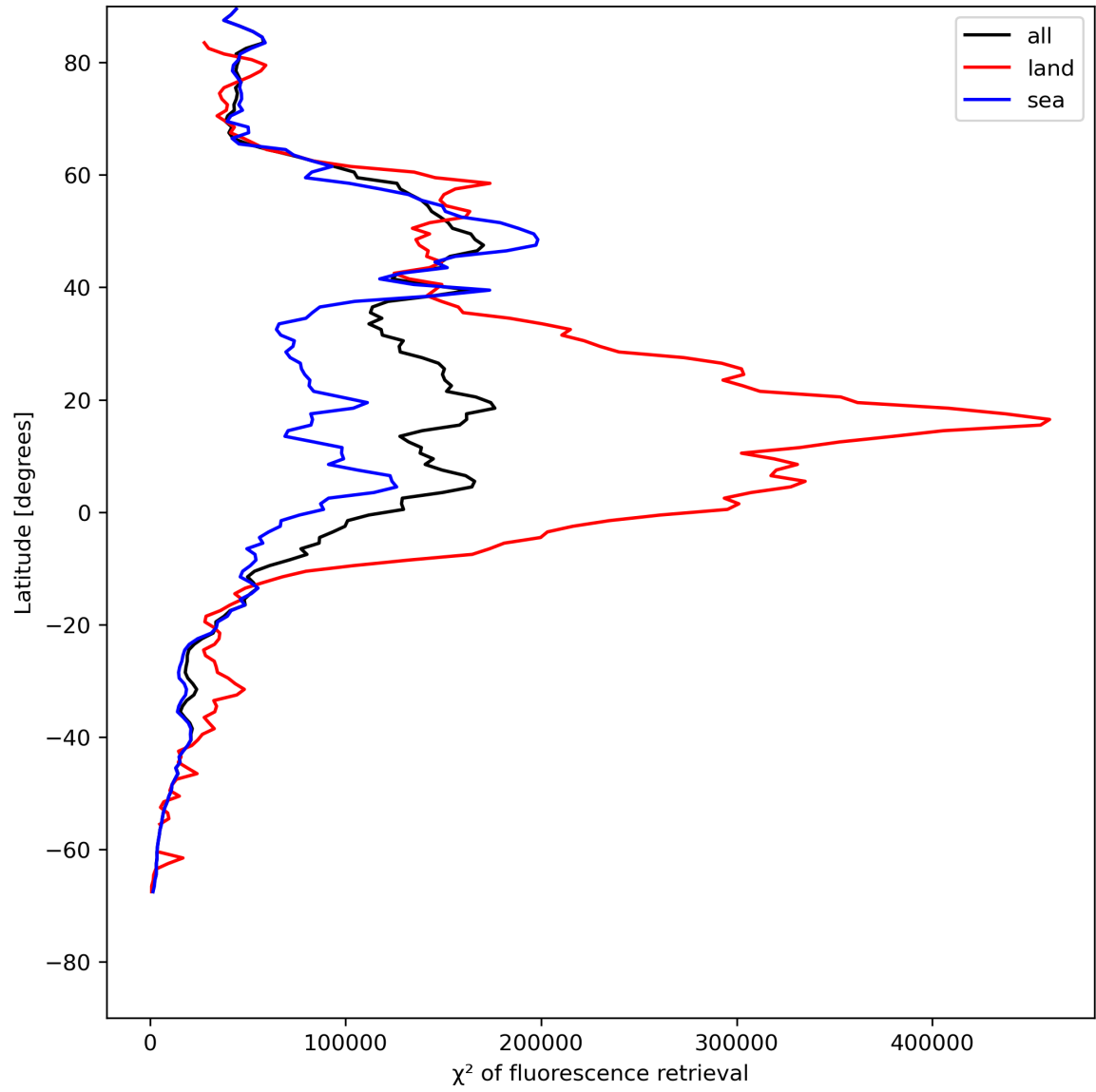
Figure 25: Zonal average of “ \chi^2 of fluorescence retrieval” for 2024-07-19 to 2024-07-21.
