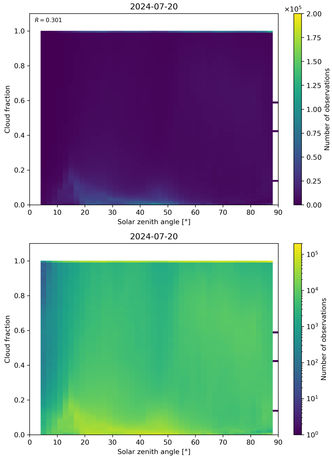
Figure 110: Scatter density plot of “Solar zenith angle” against “Cloud fraction” for 2024-07-19 to 2024-07-21.
