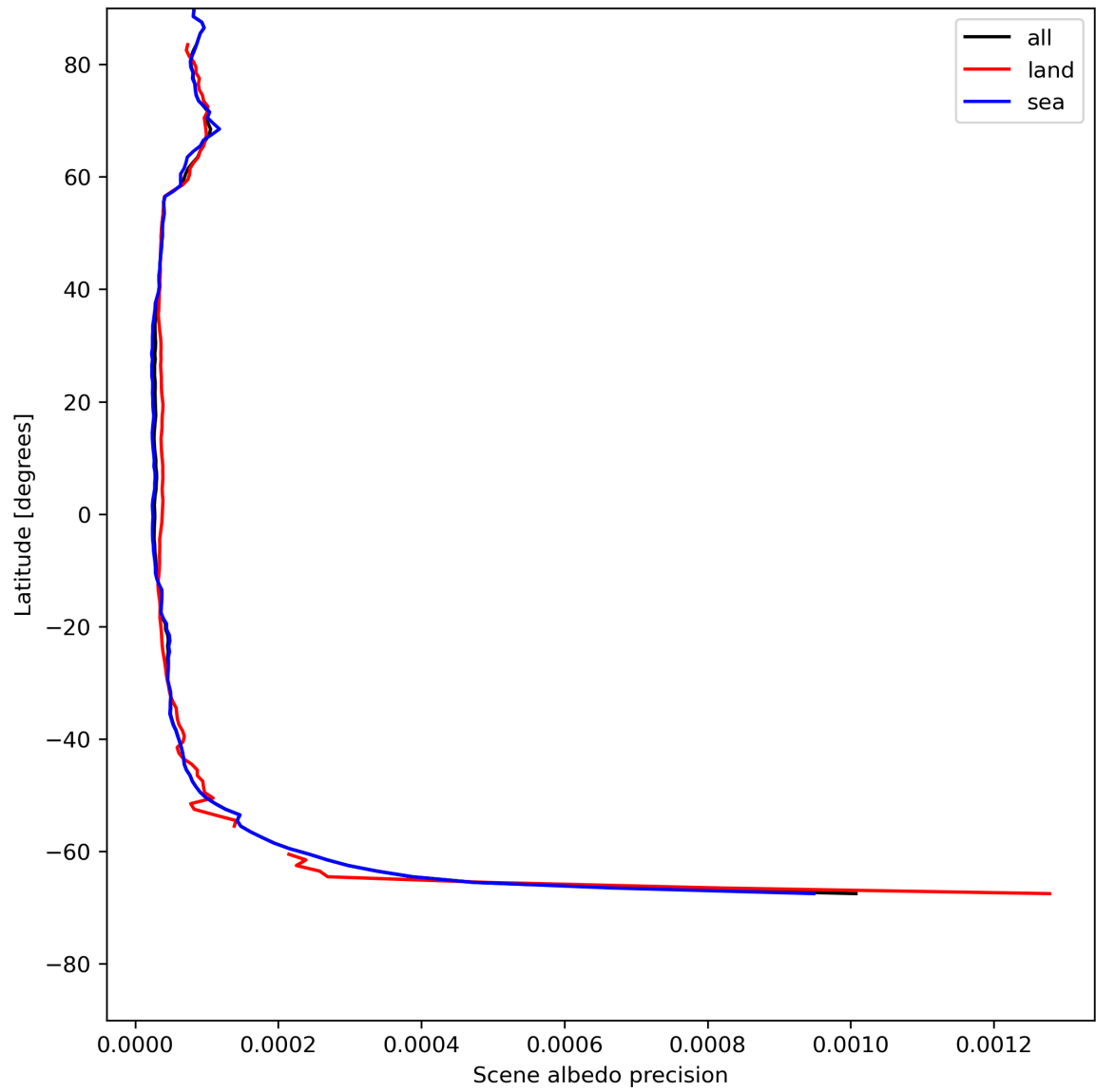
Figure 18: Zonal average of “Scene albedo precision” for 2024-07-19 to 2024-07-21.
