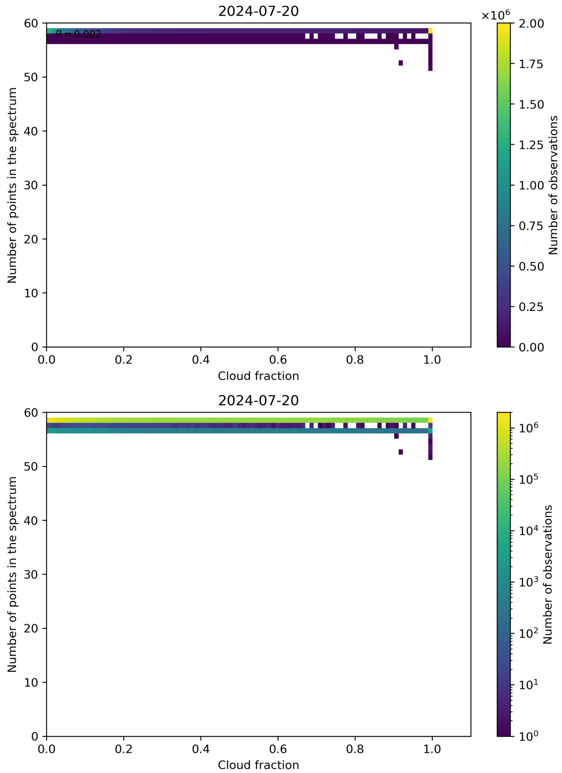
Figure 74: Scatter density plot of “Cloud fraction” against “Number of points in the spectrum” for 2024-07-19 to 2024-07-21.
