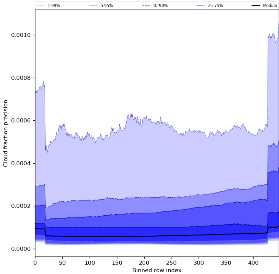
Figure 50: Along track statistics of “Cloud fraction precision” for 2024-07-19 to 2024-07-21
