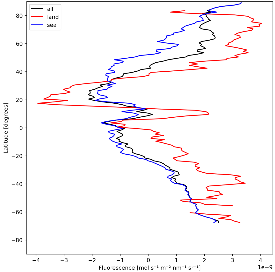
Figure 23: Zonal average of “Fluorescence” for 2024-07-19 to 2024-07-21.
