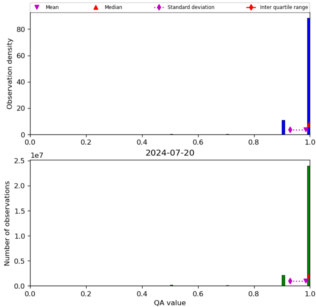
Figure 29: Histogram of “QA value” for 2024-07-19 to 2024-07-21
