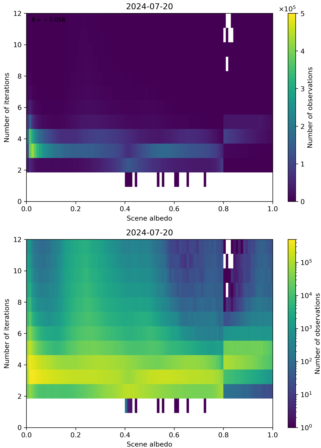
Figure 105: Scatter density plot of “Scene albedo” against “Number of iterations” for 2024-07-19 to 2024-07-21.
