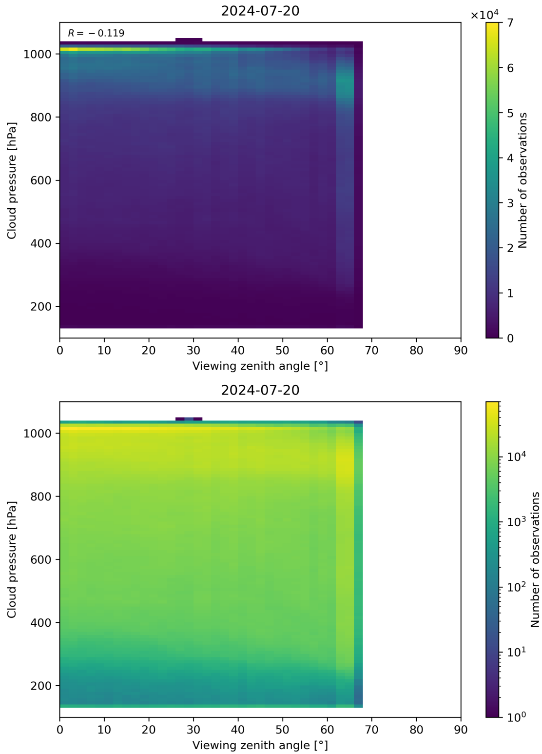
Figure 121: Scatter density plot of “Viewing zenith angle” against “Cloud pressure” for 2024-07-19 to 2024-07-21.
