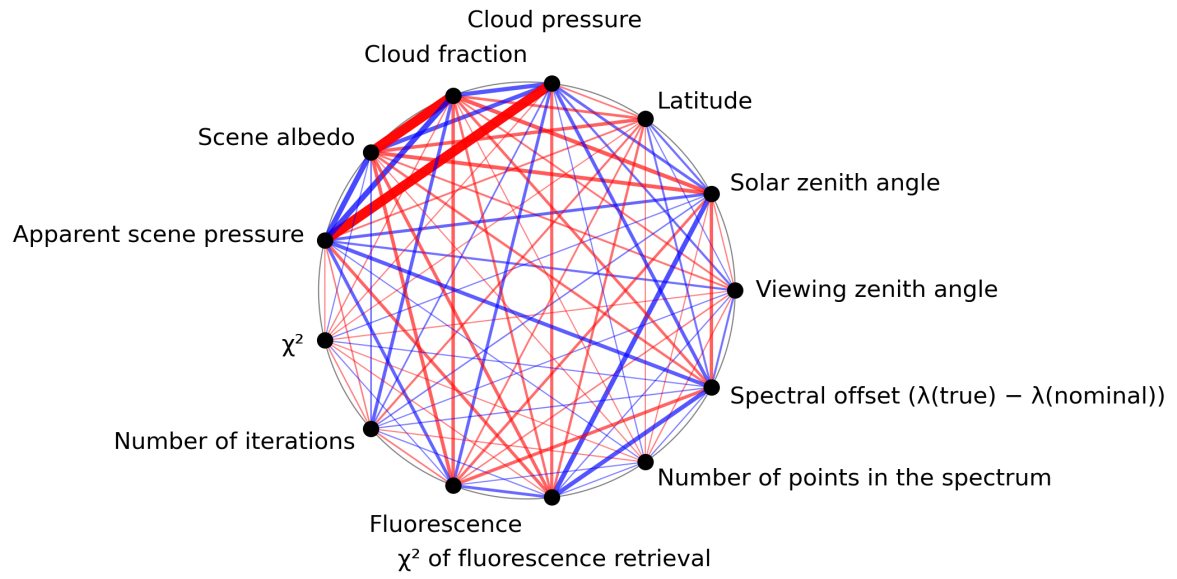
Figure 1: Map of correlation graph for 2024-07-19 to 2024-07-21.
