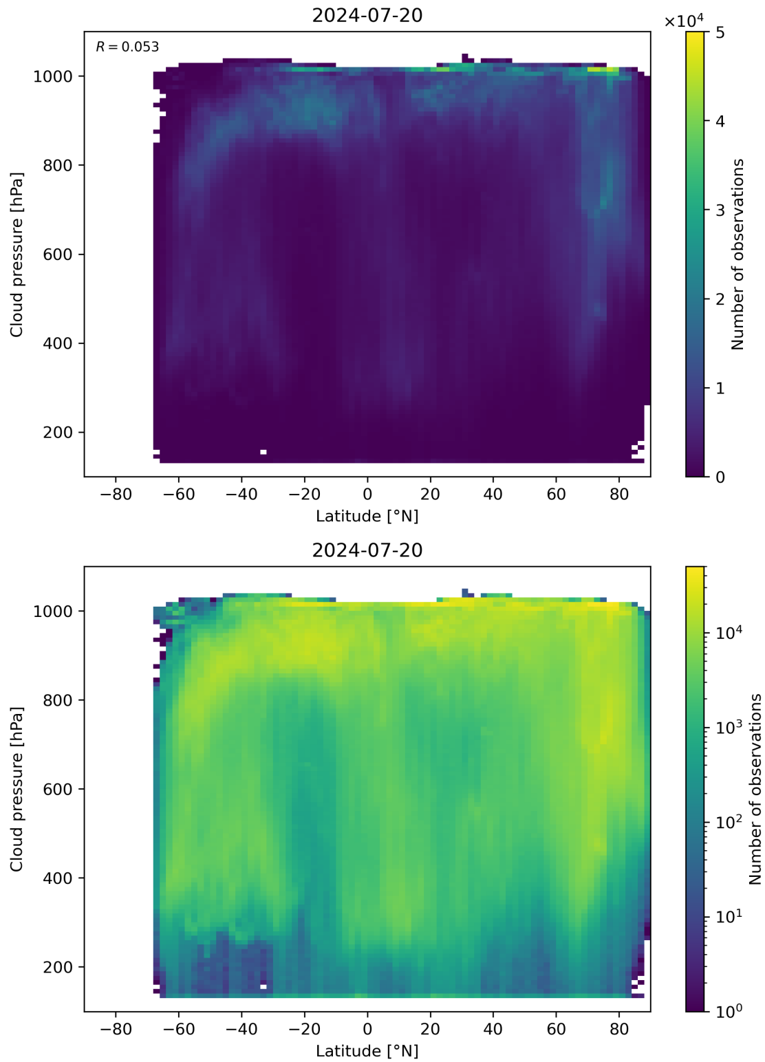
Figure 91: Scatter density plot of “Latitude” against “Cloud pressure” for 2024-07-19 to 2024-07-21.
