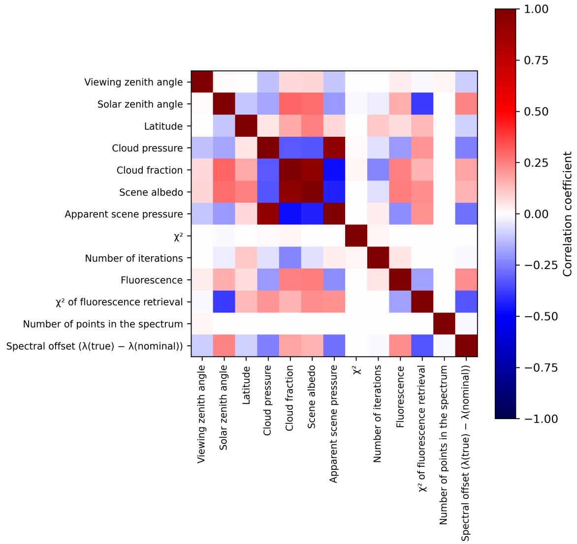
Figure 2: Map of correlation matrix for 2024-07-19 to 2024-07-21.
