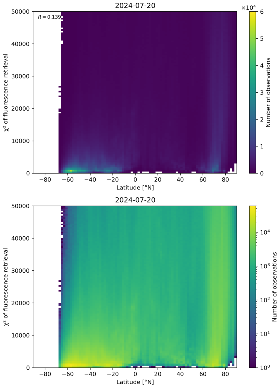
Figure 89: Scatter density plot of “Latitude” against “ \chi^2 of fluorescence retrieval” for 2024-07-19 to 2024-07-21.
