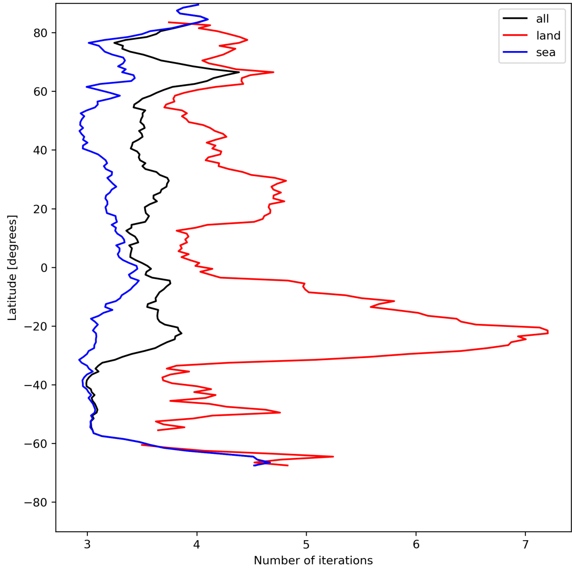
Figure 22: Zonal average of “Number of iterations” for 2024-07-19 to 2024-07-21.
