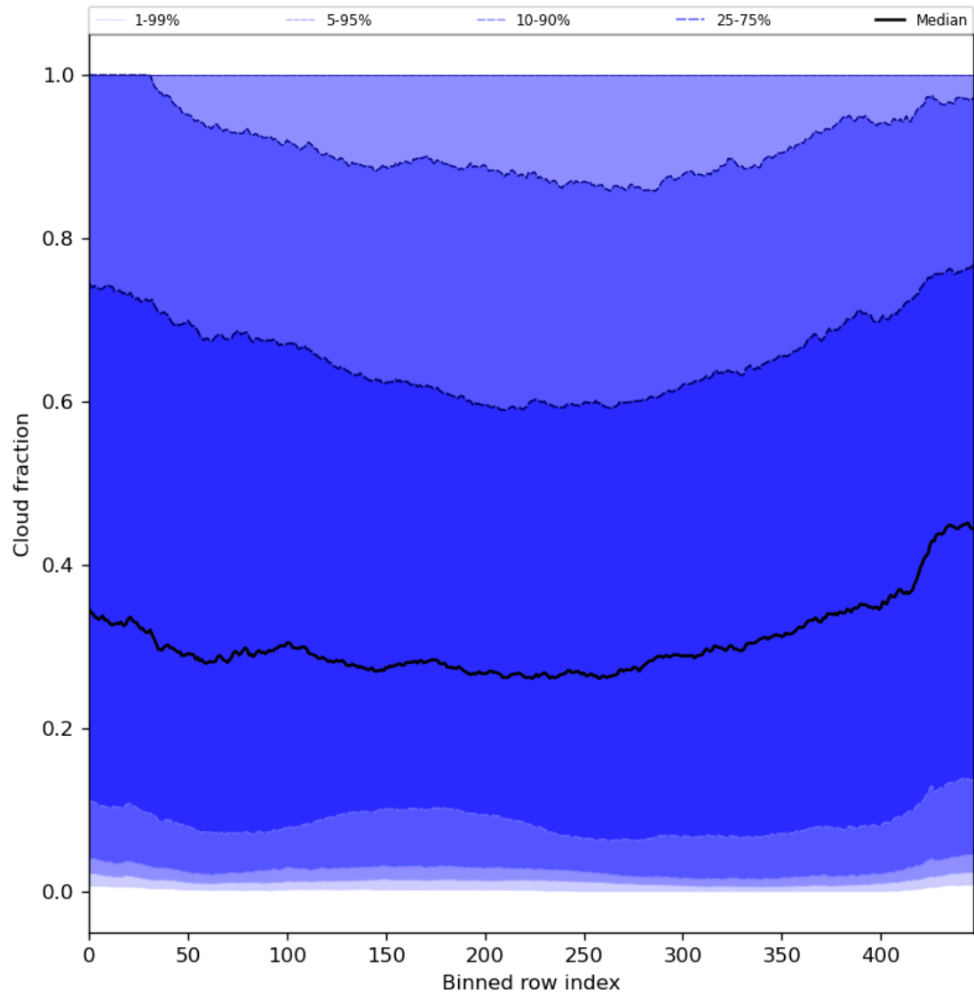
Figure 49: Along track statistics of “Cloud fraction” for 2024-07-19 to 2024-07-21
