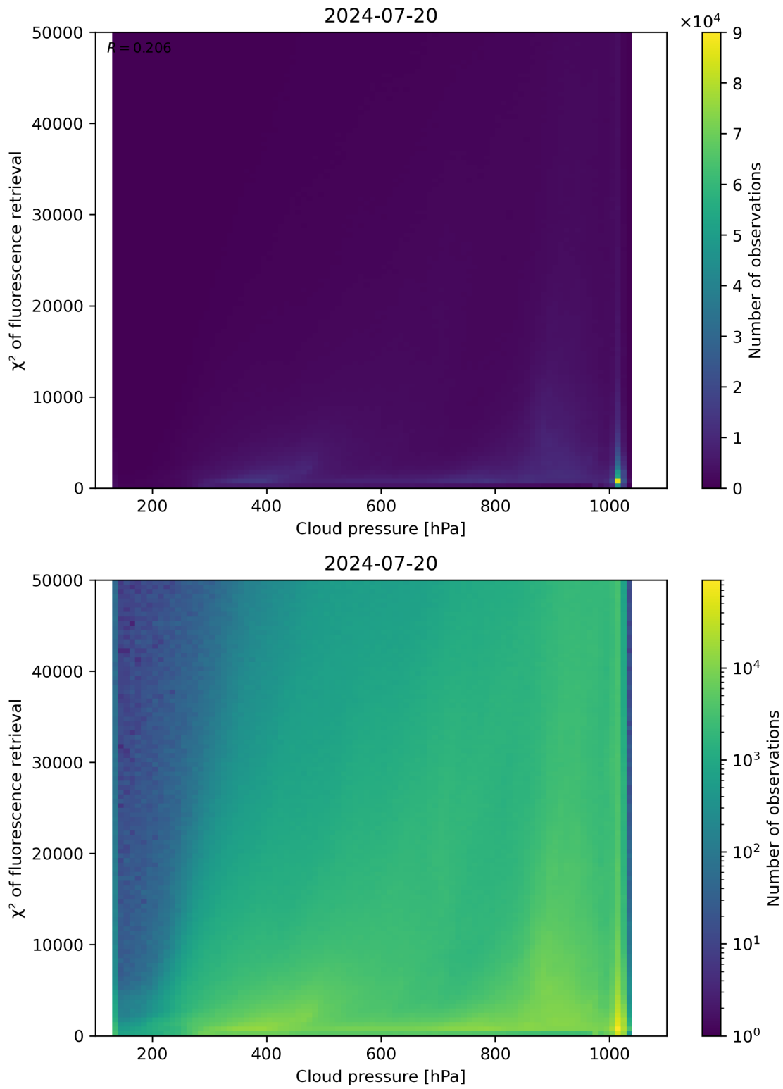
Figure 78: Scatter density plot of “Cloud pressure” against “ \chi^2 of fluorescence retrieval” for 2024-07-19 to 2024-07-21.
