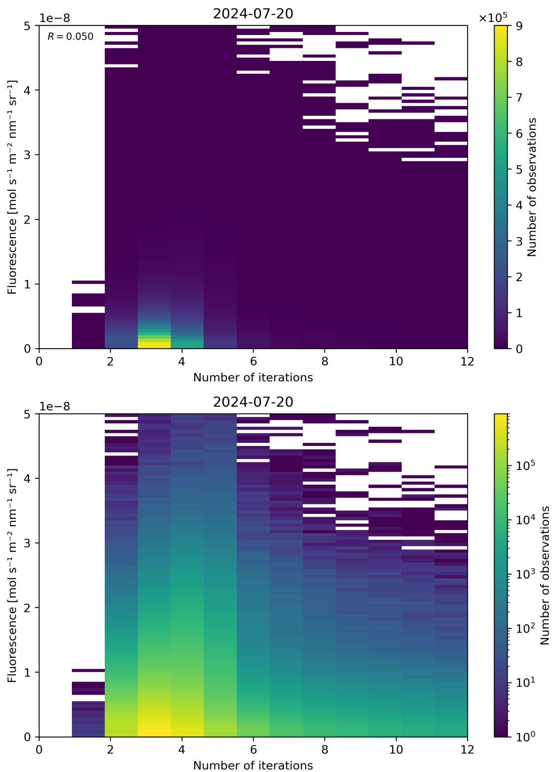
Figure 98: Scatter density plot of “Number of iterations” against “Fluorescence” for 2024-07-19 to 2024-07-21.
