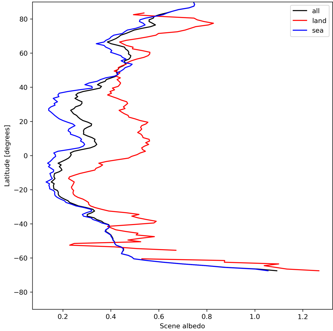
Figure 17: Zonal average of “Scene albedo” for 2024-07-19 to 2024-07-21.
