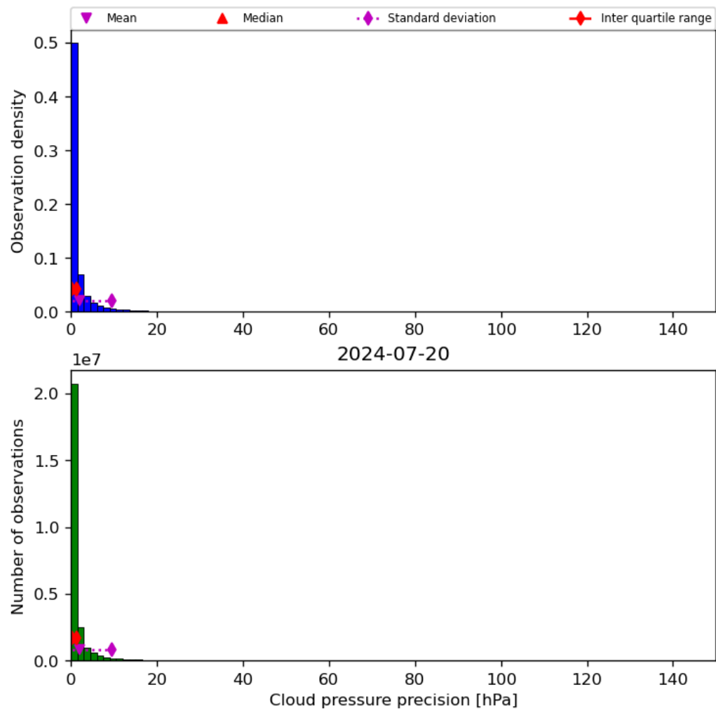
Figure 31: Histogram of “Cloud pressure precision” for 2024-07-19 to 2024-07-21
