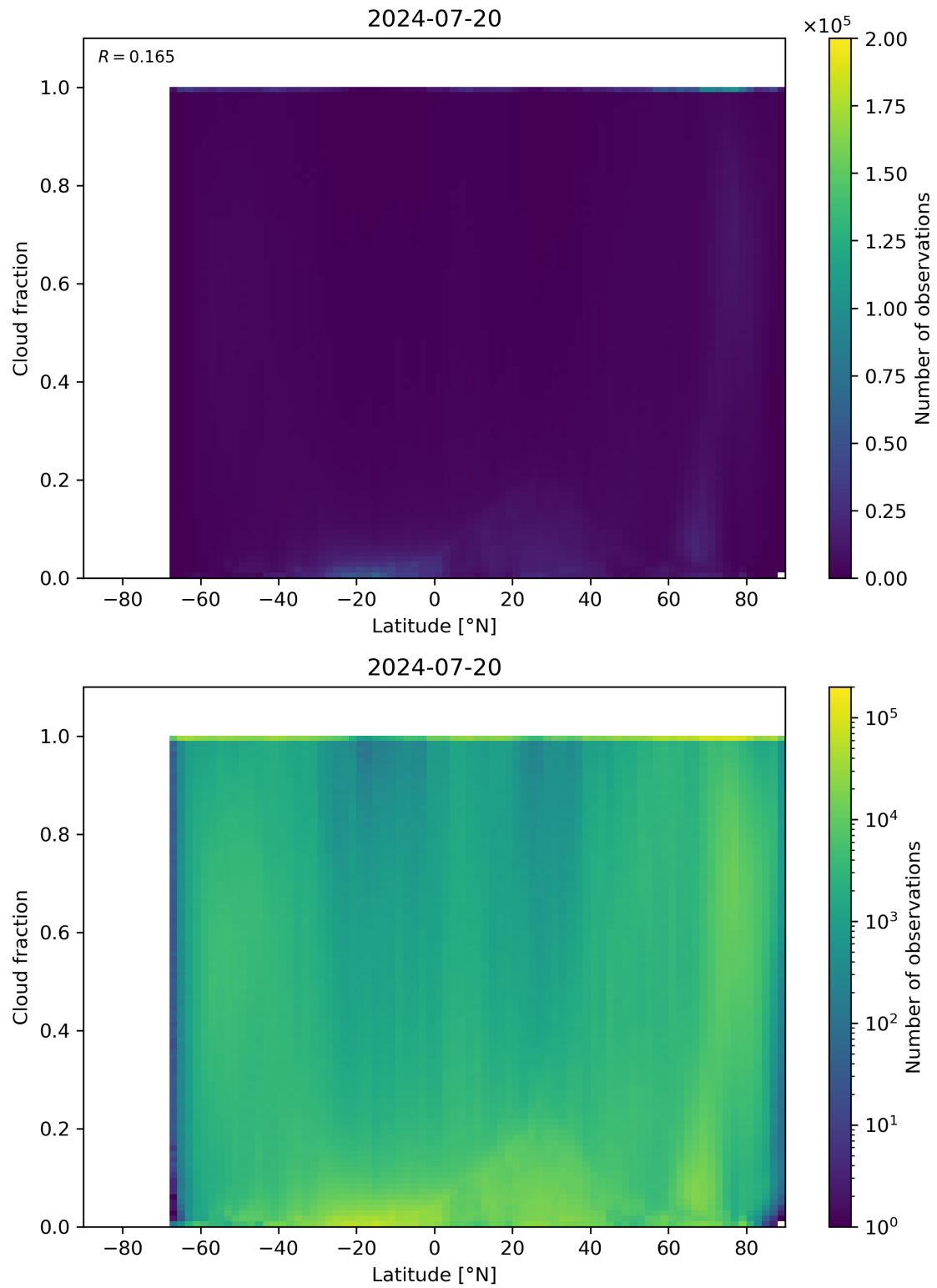
Figure 90: Scatter density plot of “Latitude” against “Cloud fraction” for 2024-07-19 to 2024-07-21.
