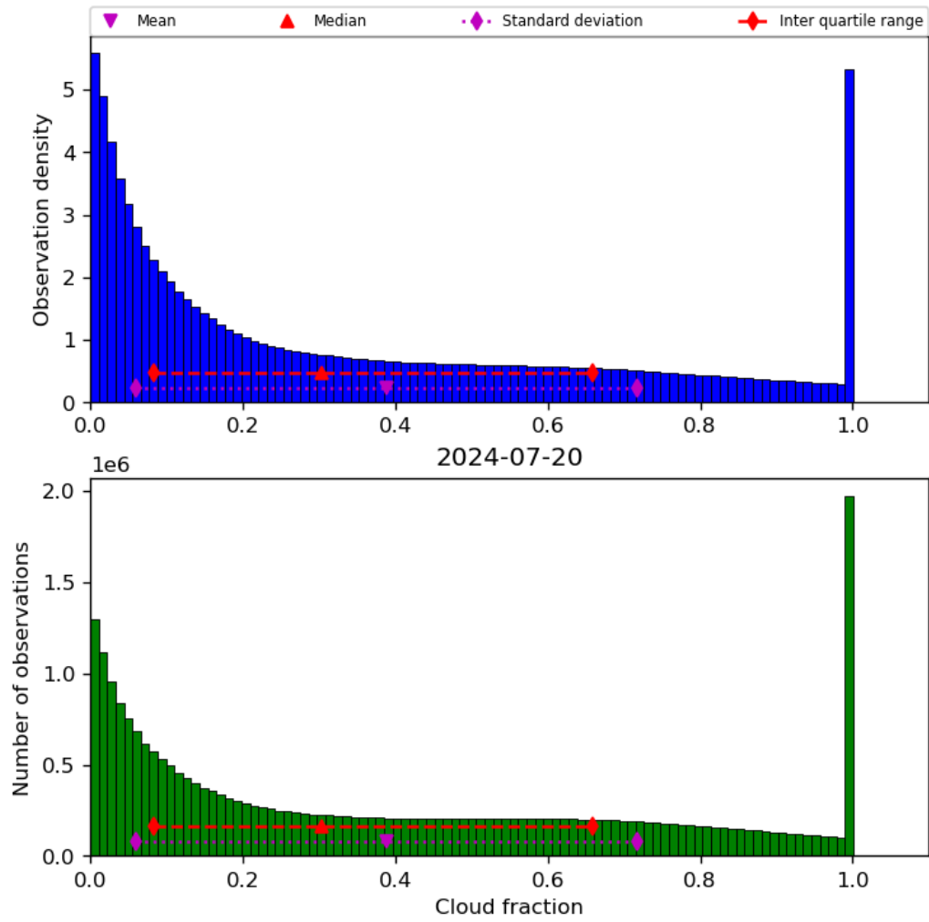
Figure 32: Histogram of “Cloud fraction” for 2024-07-19 to 2024-07-21
