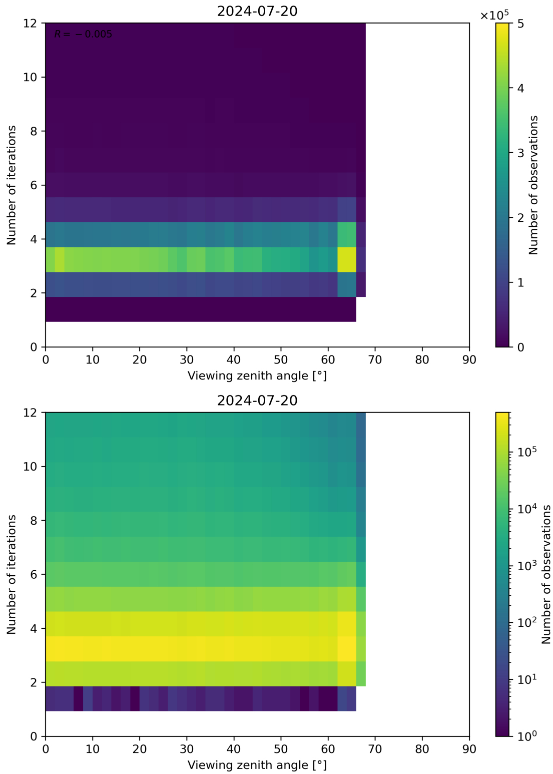
Figure 124: Scatter density plot of “Viewing zenith angle” against “Number of iterations” for 2024-07-19 to 2024-07-21.
