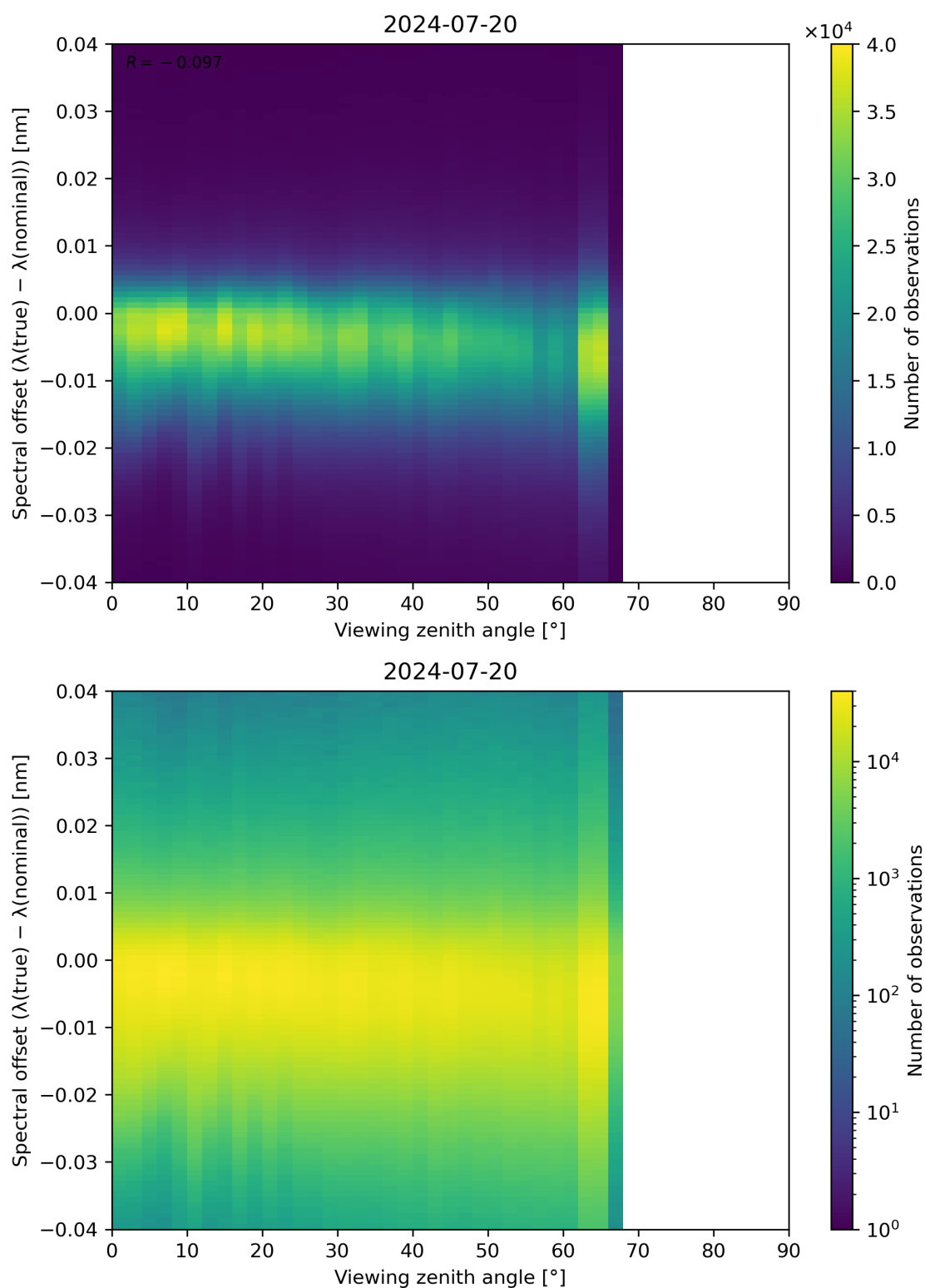
Figure 128: Scatter density plot of “Viewing zenith angle” against “Spectral offset ( \lambda(\text{true}) - \lambda(\text{nominal}) )” for 2024-07-19 to 2024-07-21.
