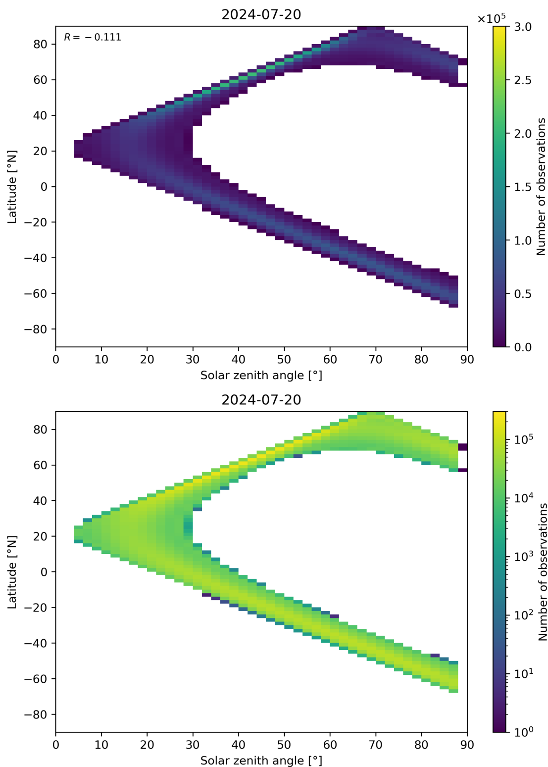
Figure 113: Scatter density plot of “Solar zenith angle” against “Latitude” for 2024-07-19 to 2024-07-21.
