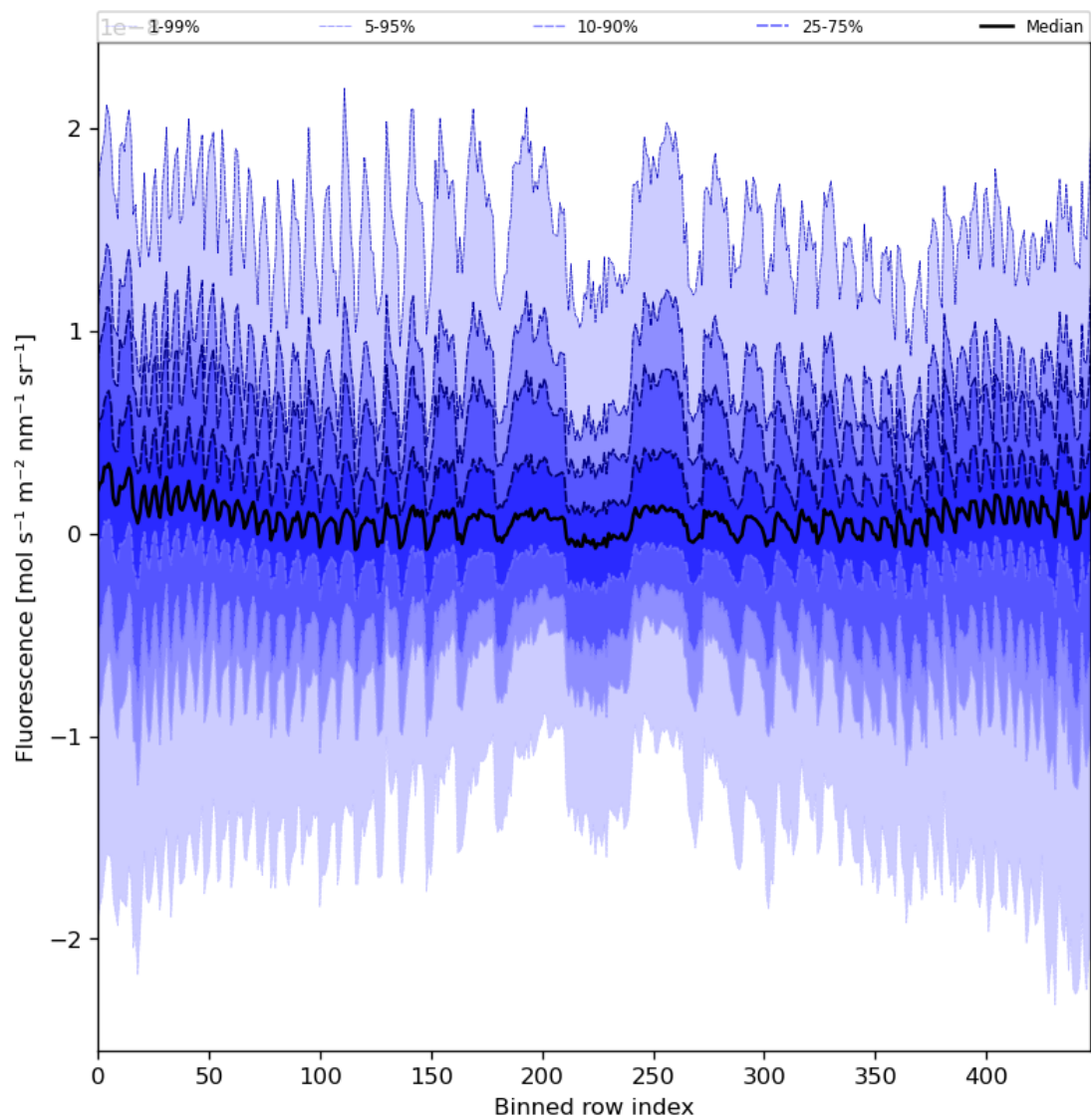
Figure 57: Along track statistics of “Fluorescence” for 2024-07-19 to 2024-07-21
