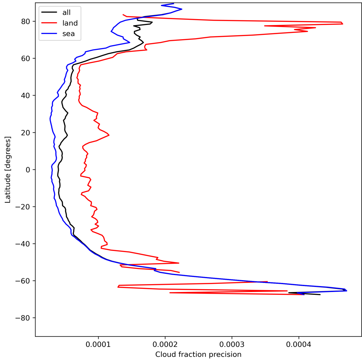
Figure 16: Zonal average of “Cloud fraction precision” for 2024-07-19 to 2024-07-21.
