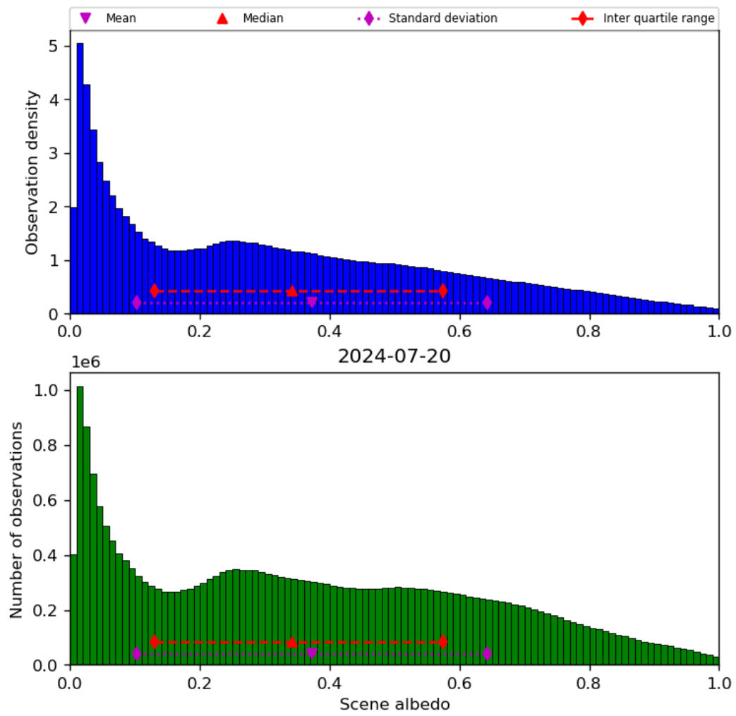
Figure 34: Histogram of “Scene albedo” for 2024-07-19 to 2024-07-21
