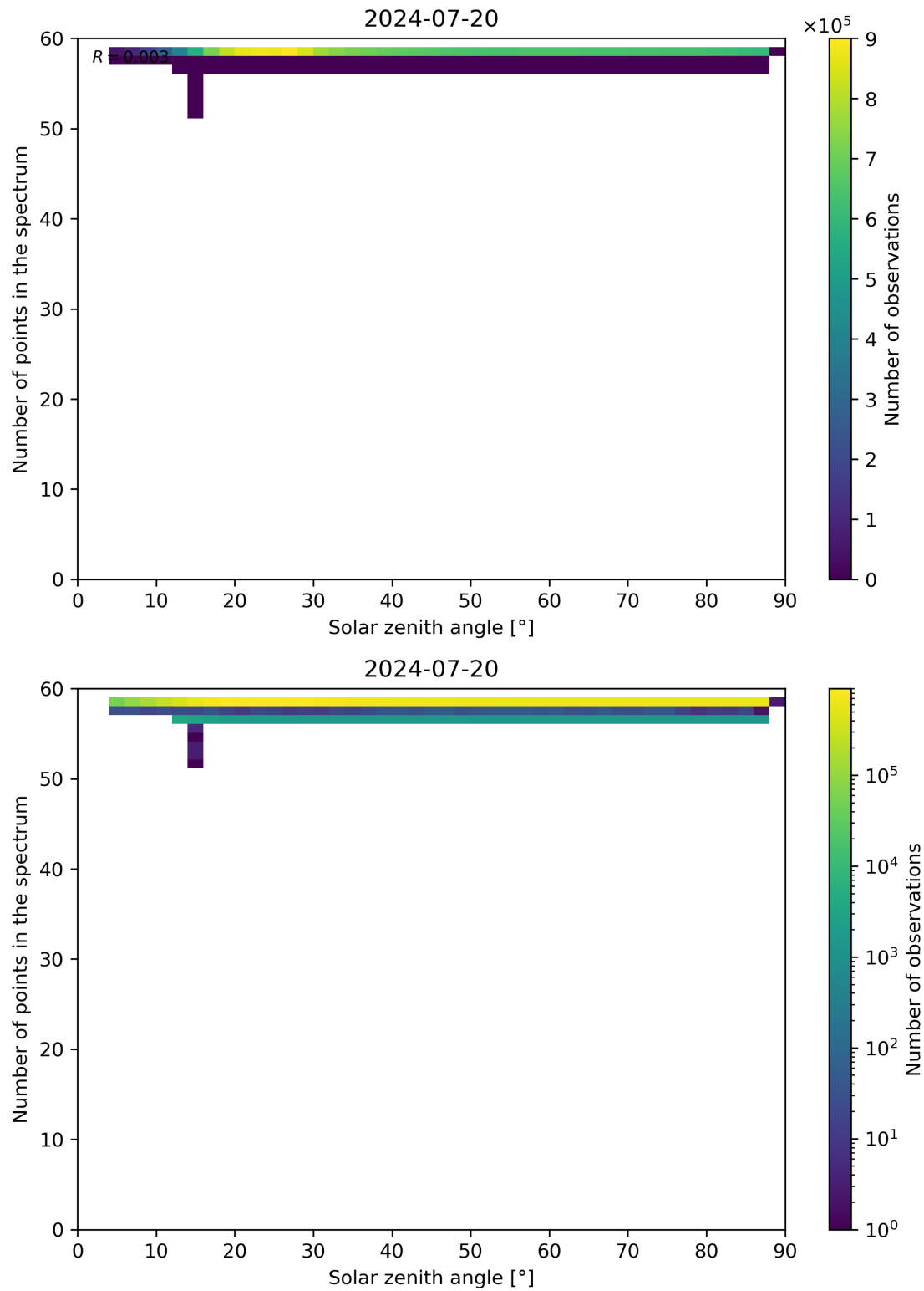
Figure 115: Scatter density plot of “Solar zenith angle” against “Number of points in the spectrum” for 2024-07-19 to 2024-07-21.
