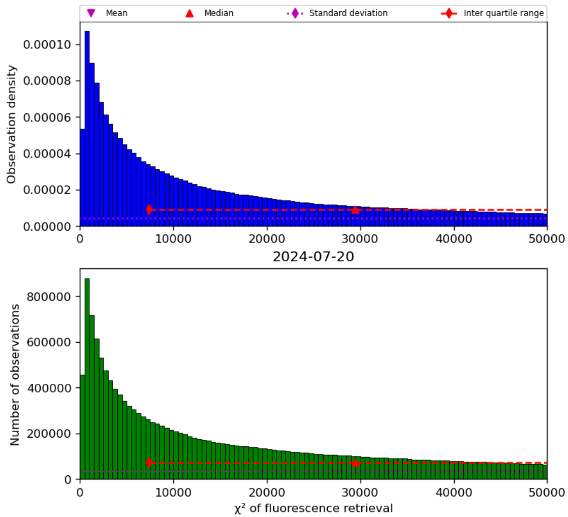
Figure 42: Histogram of “ \chi^2 of fluorescence retrieval” for 2024-07-19 to 2024-07-21
