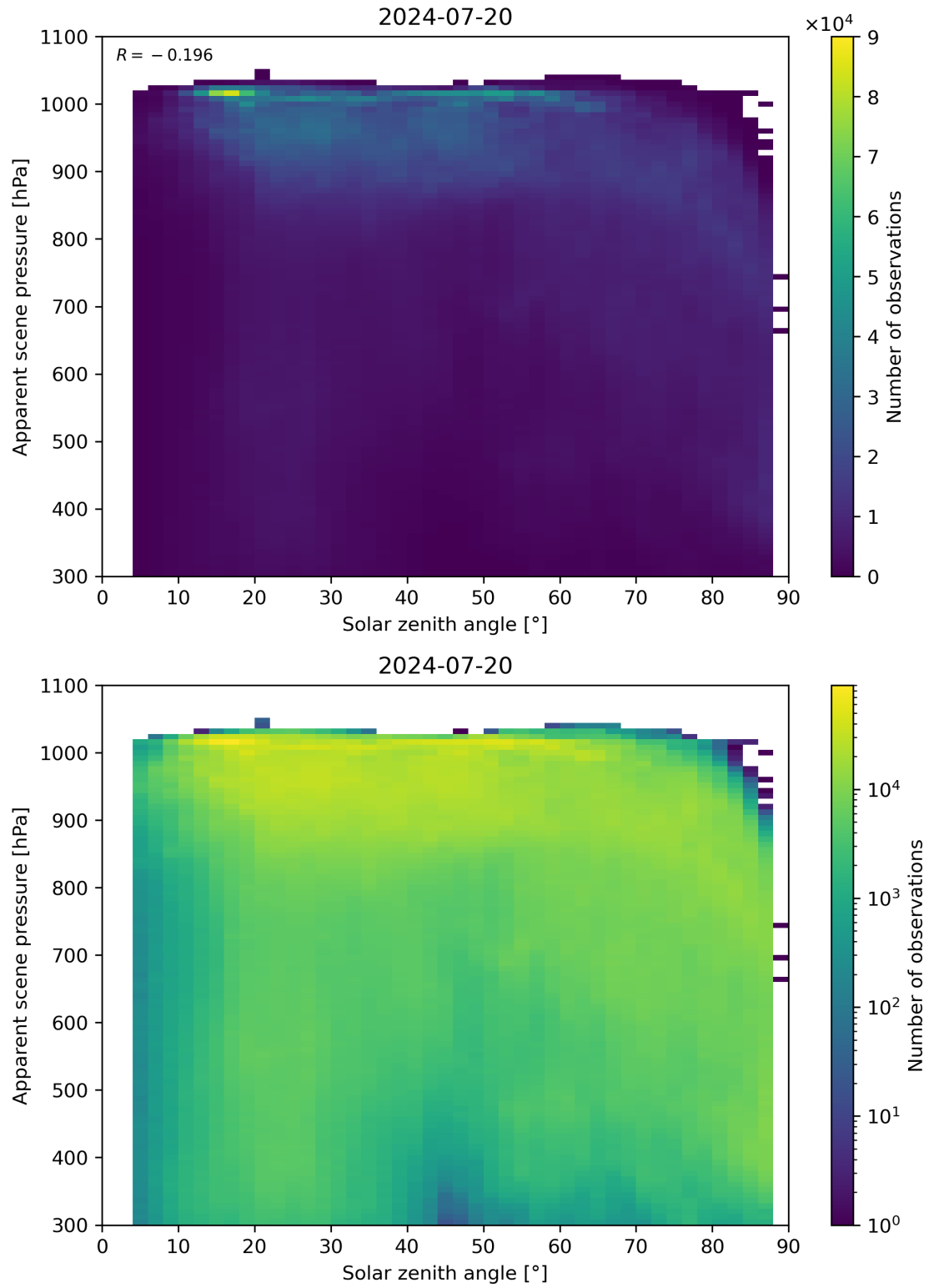
Figure 108: Scatter density plot of “Solar zenith angle” against “Apparent scene pressure” for 2024-07-19 to 2024-07-21.
