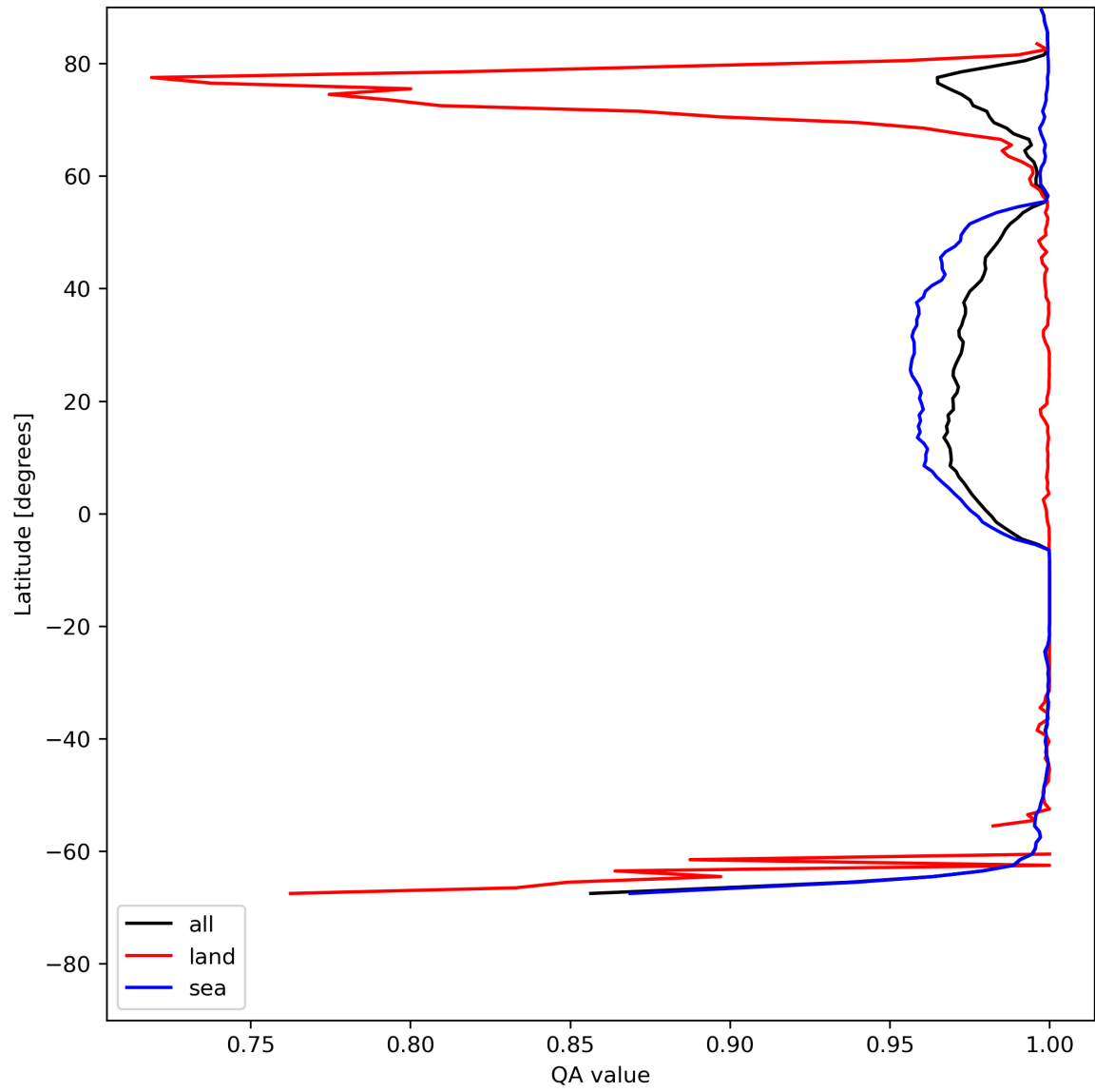
Figure 12: Zonal average of “QA value” for 2024-07-19 to 2024-07-21.
