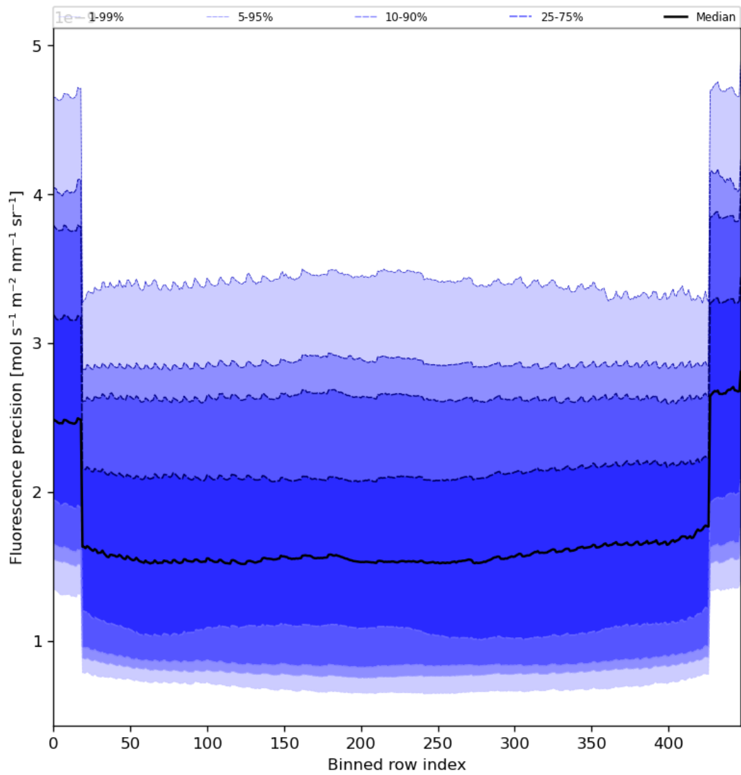
Figure 58: Along track statistics of “Fluorescence precision” for 2024-07-19 to 2024-07-21
