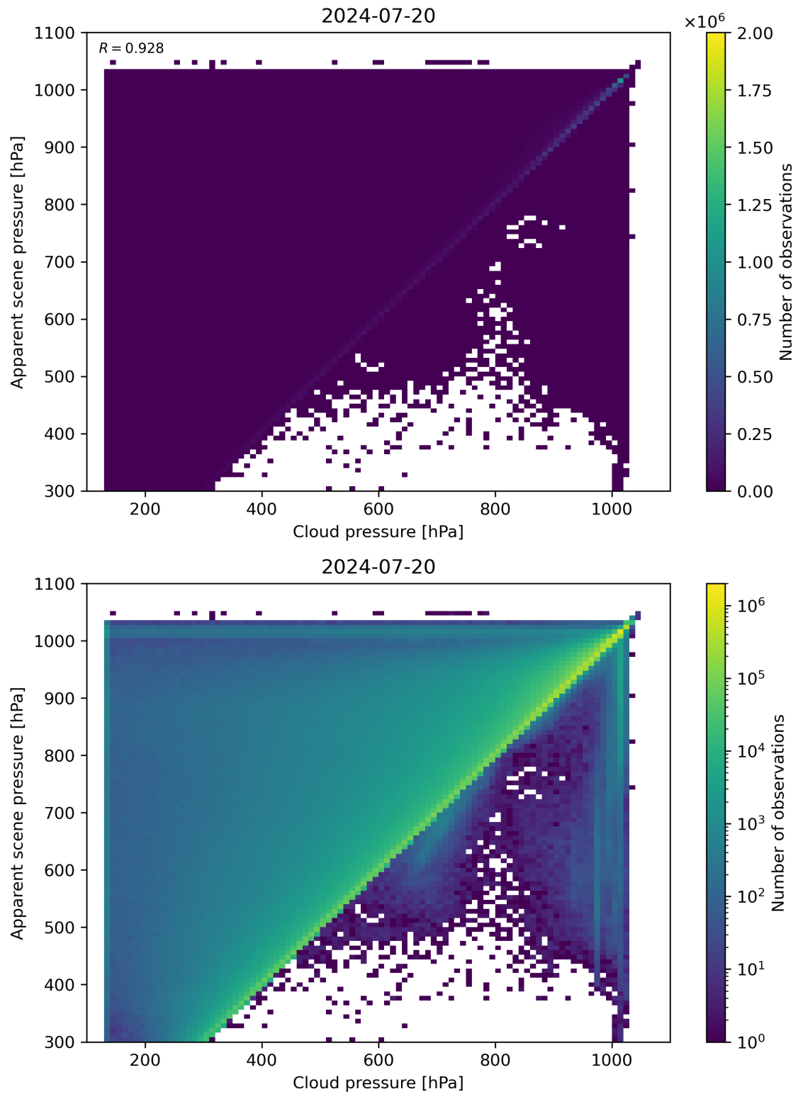
Figure 77: Scatter density plot of “Cloud pressure” against “Apparent scene pressure” for 2024-07-19 to 2024-07-21.
