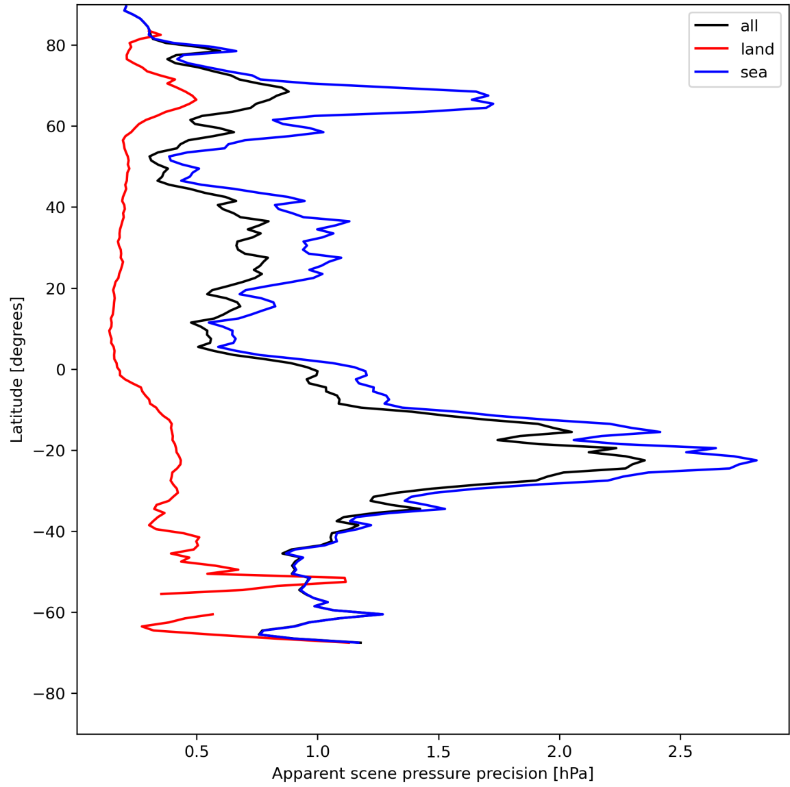
Figure 20: Zonal average of “Apparent scene pressure precision” for 2024-07-19 to 2024-07-21.
