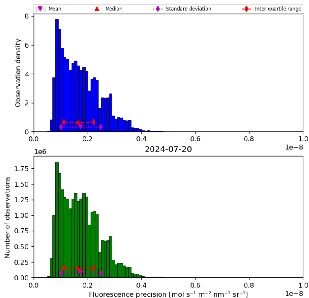
Figure 41: Histogram of “Fluorescence precision” for 2024-07-19 to 2024-07-21
