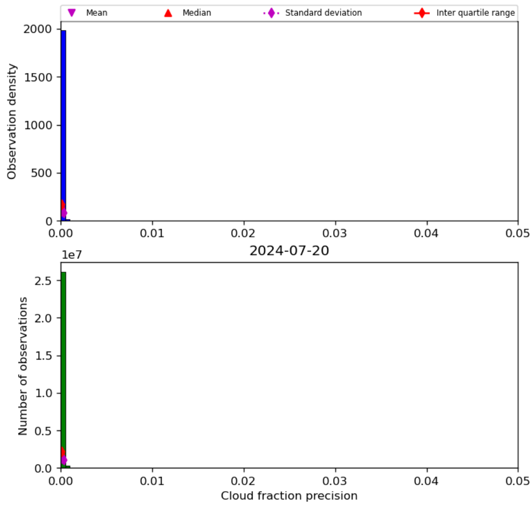
Figure 33: Histogram of “Cloud fraction precision” for 2024-07-19 to 2024-07-21
