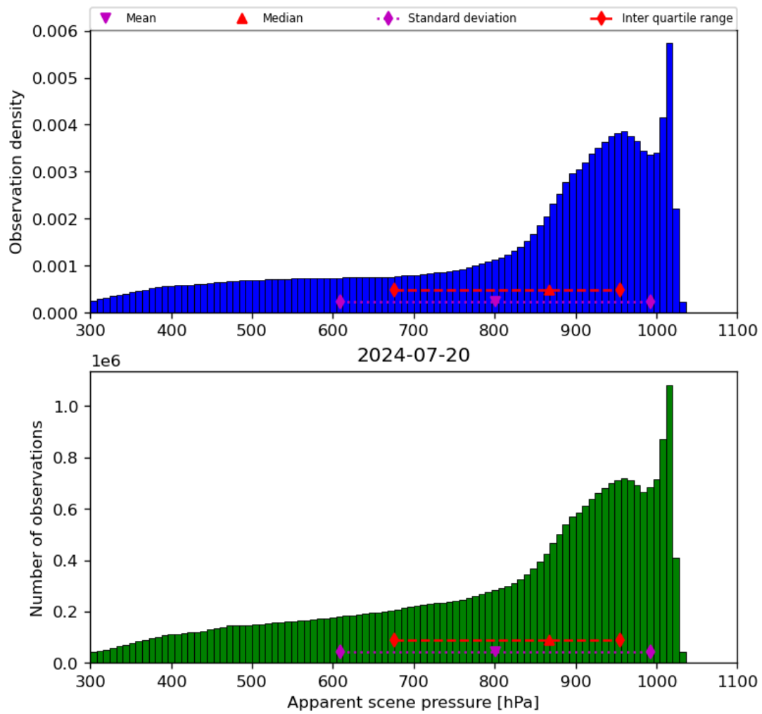
Figure 36: Histogram of “Apparent scene pressure” for 2024-07-19 to 2024-07-21
