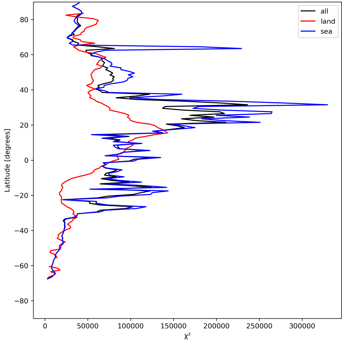
Figure 21: Zonal average of “ \chi^2 ” for 2024-07-19 to 2024-07-21.
