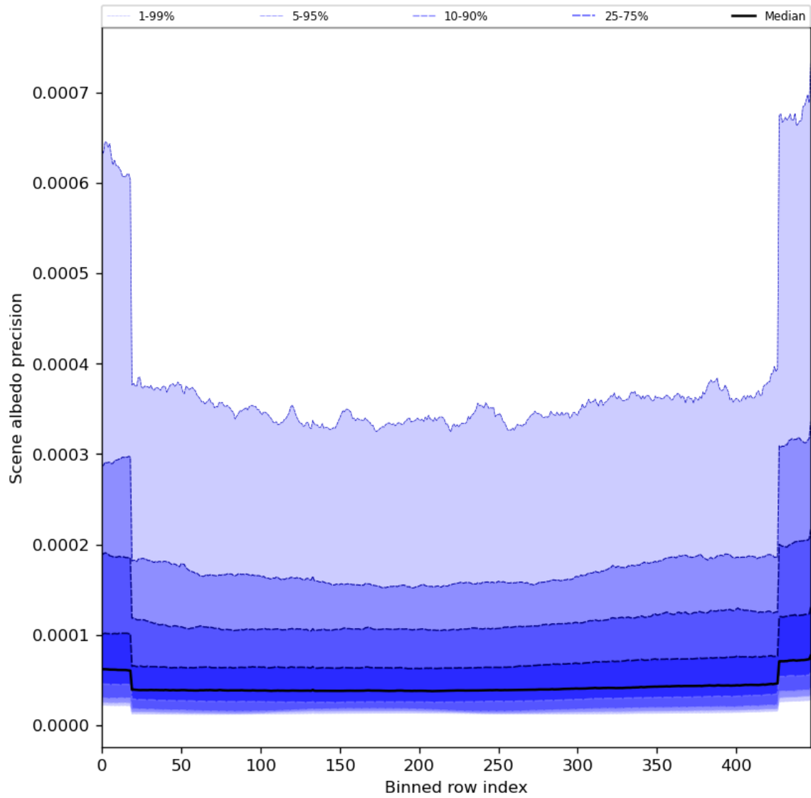
Figure 52: Along track statistics of “Scene albedo precision” for 2024-07-19 to 2024-07-21
