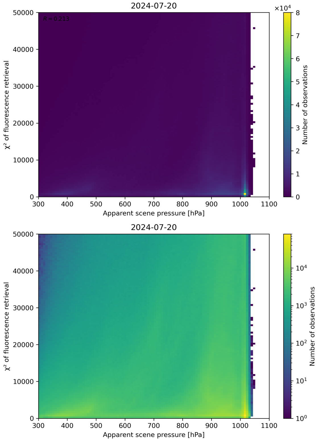
Figure 63: Scatter density plot of “Apparent scene pressure” against “ \chi^2 of fluorescence retrieval” for 2024-07-19 to 2024-07-21.
