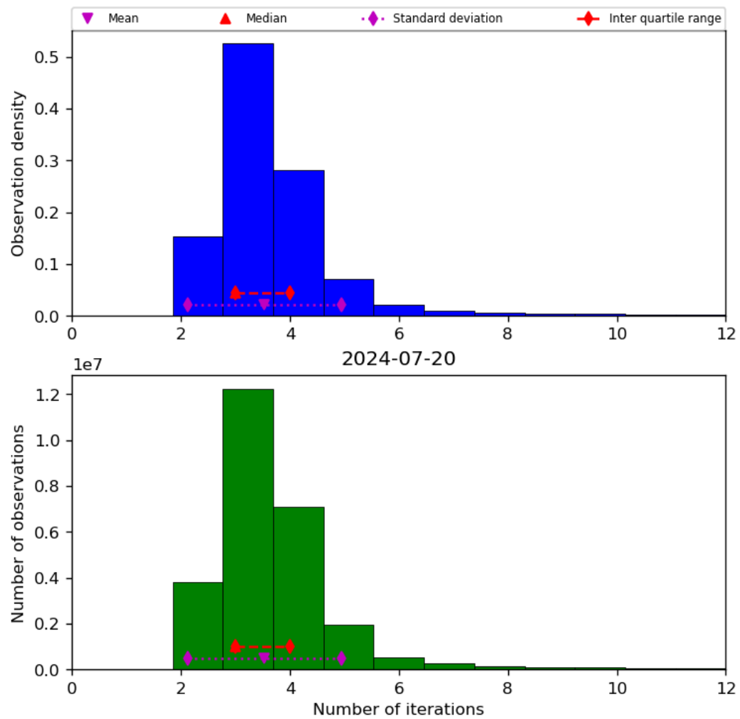
Figure 39: Histogram of “Number of iterations” for 2024-07-19 to 2024-07-21
