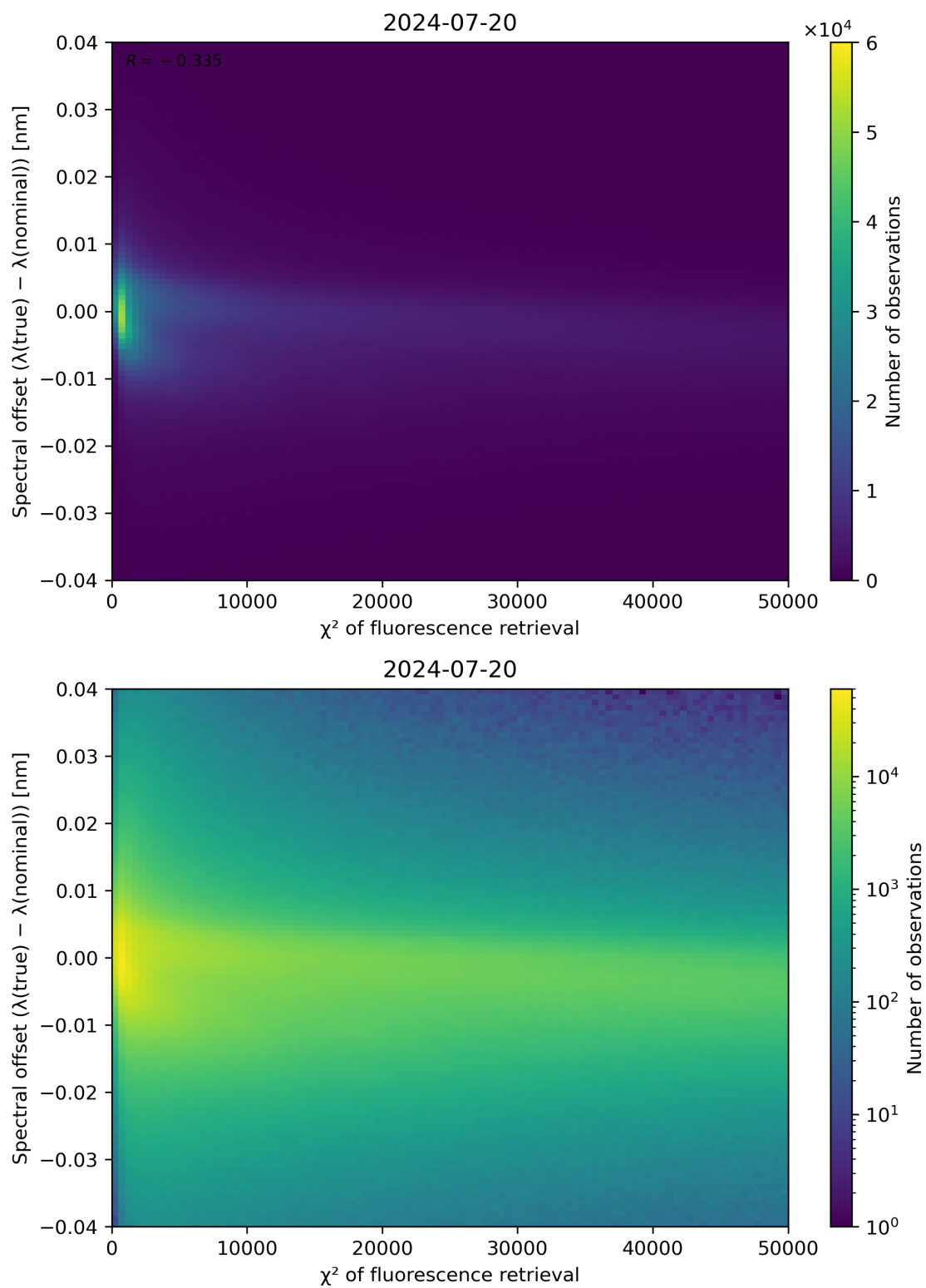
Figure 69: Scatter density plot of " \chi^2 of fluorescence retrieval" against "Spectral offset ( \lambda(\text{true}) - \lambda(\text{nominal})) " for 2024-07-19 to 2024-07-21.
