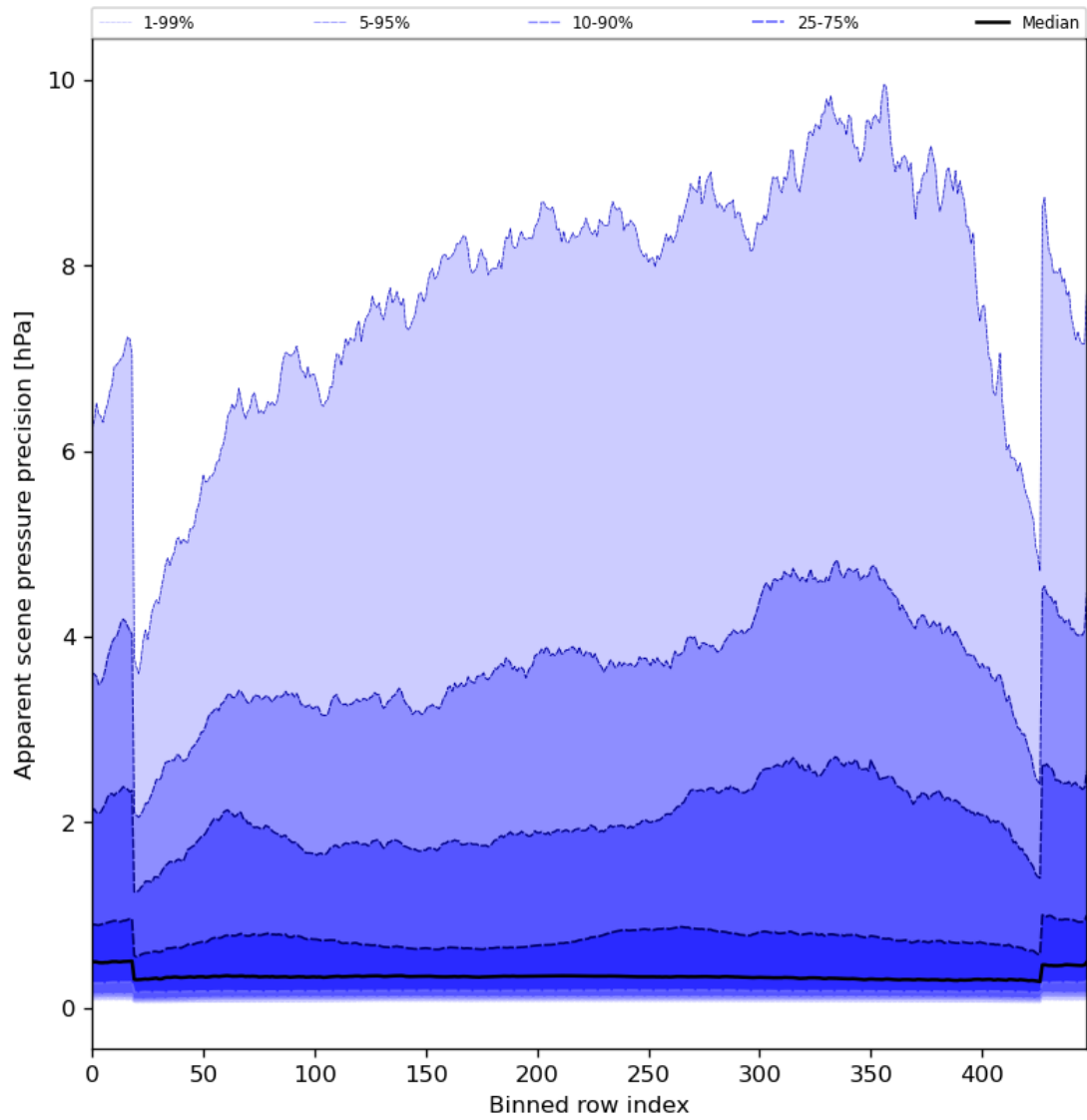
Figure 54: Along track statistics of “Apparent scene pressure precision” for 2024-07-19 to 2024-07-21
