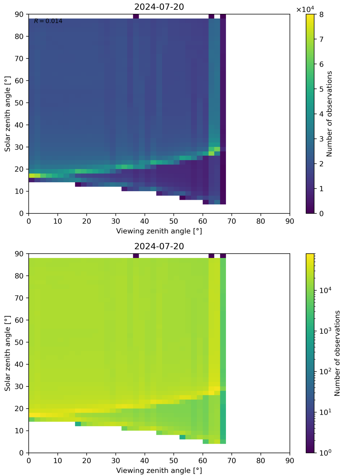
Figure 127: Scatter density plot of “Viewing zenith angle” against “Solar zenith angle” for 2024-07-19 to 2024-07-21.
