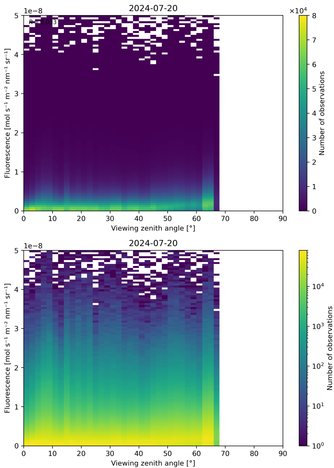
Figure 122: Scatter density plot of “Viewing zenith angle” against “Fluorescence” for 2024-07-19 to 2024-07-21.
