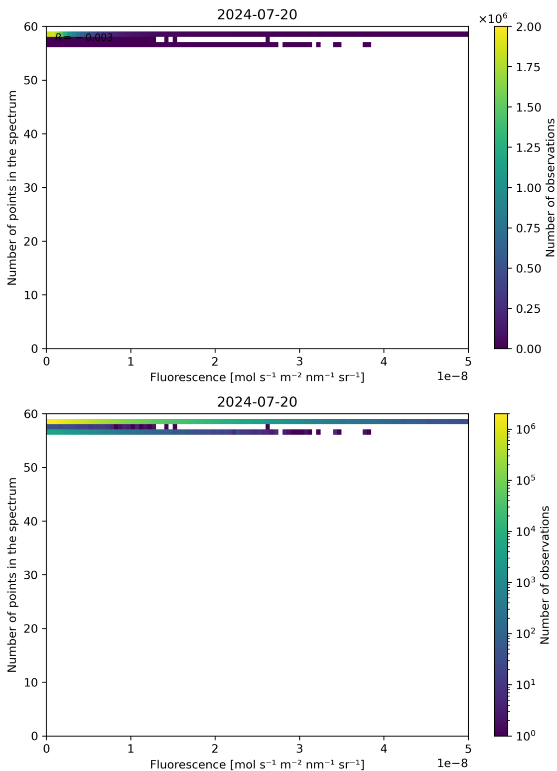
Figure 86: Scatter density plot of “Fluorescence” against “Number of points in the spectrum” for 2024-07-19 to 2024-07-21.
