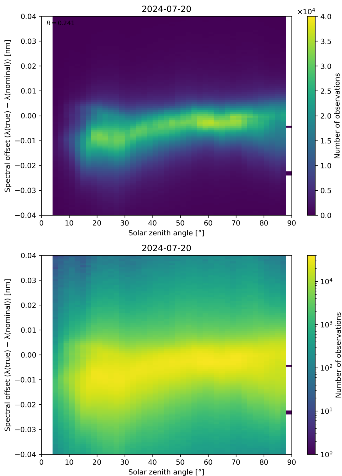
Figure 117: Scatter density plot of “Solar zenith angle” against “Spectral offset ( \lambda(\text{true}) - \lambda(\text{nominal}) )” for 2024-07-19 to 2024-07-21.
