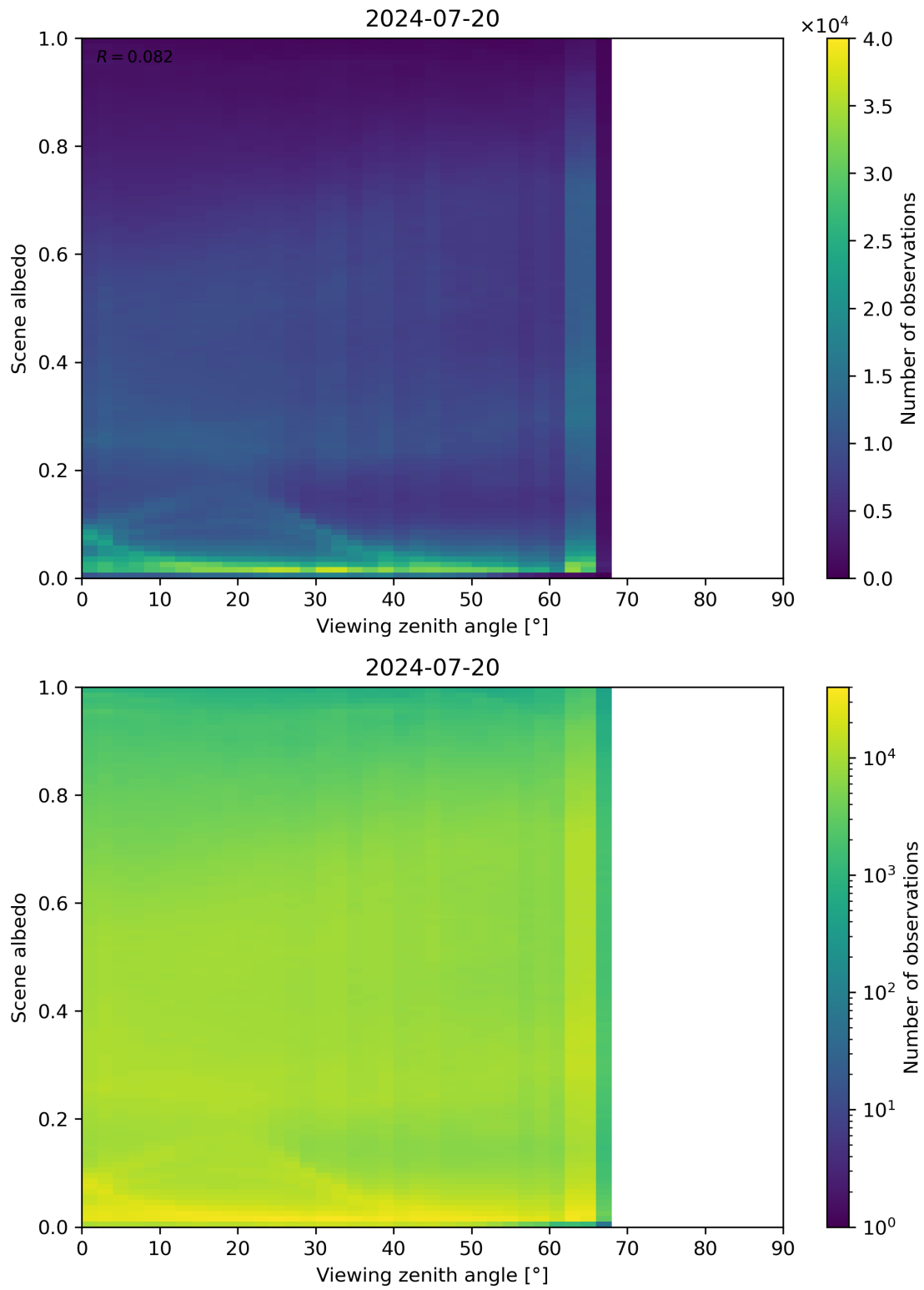
Figure 126: Scatter density plot of “Viewing zenith angle” against “Scene albedo” for 2024-07-19 to 2024-07-21.
