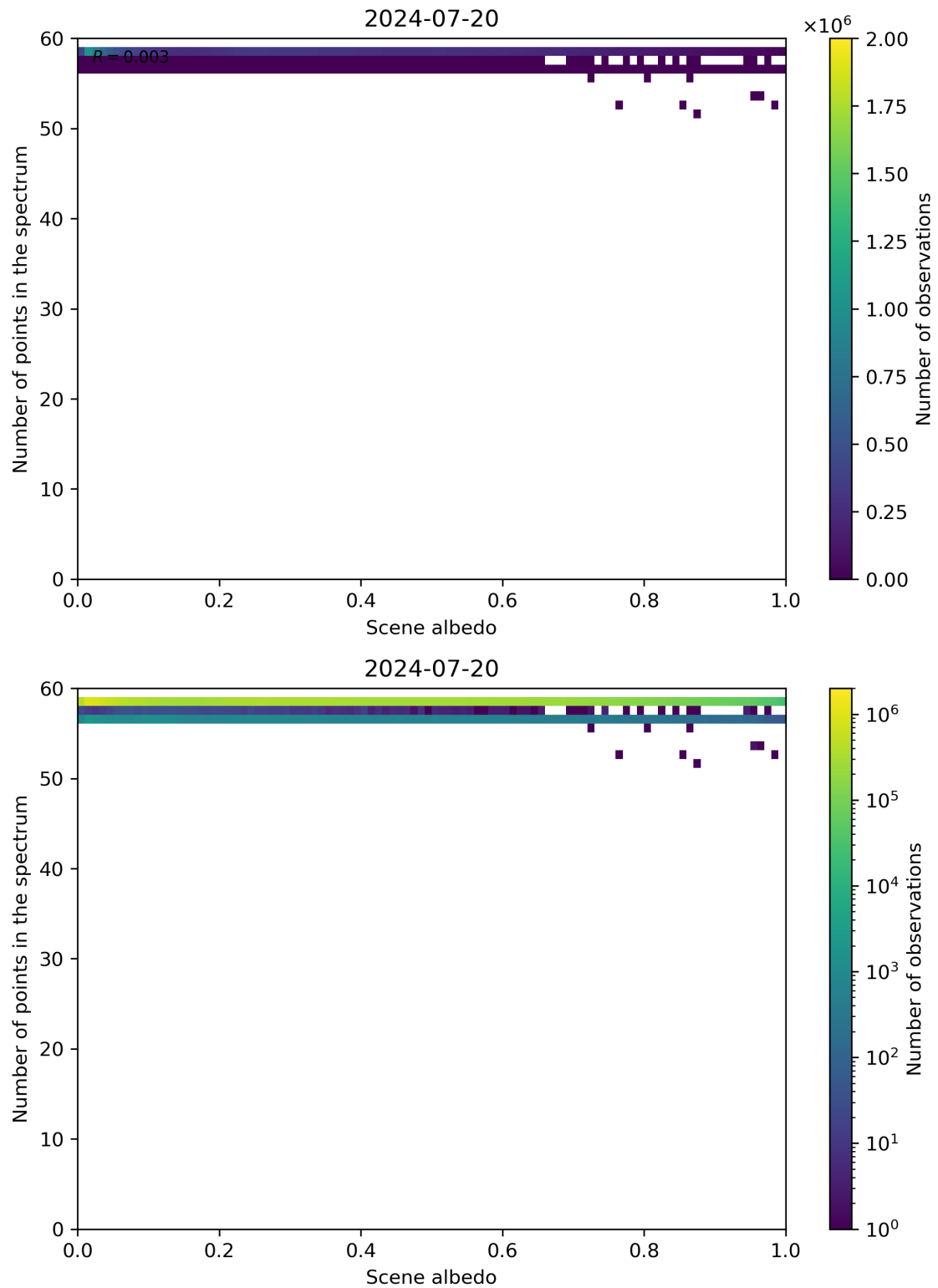
Figure 106: Scatter density plot of “Scene albedo” against “Number of points in the spectrum” for 2024-07-19 to 2024-07-21.
