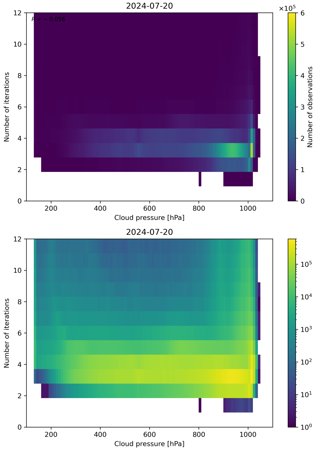
Figure 81: Scatter density plot of “Cloud pressure” against “Number of iterations” for 2024-07-19 to 2024-07-21.
