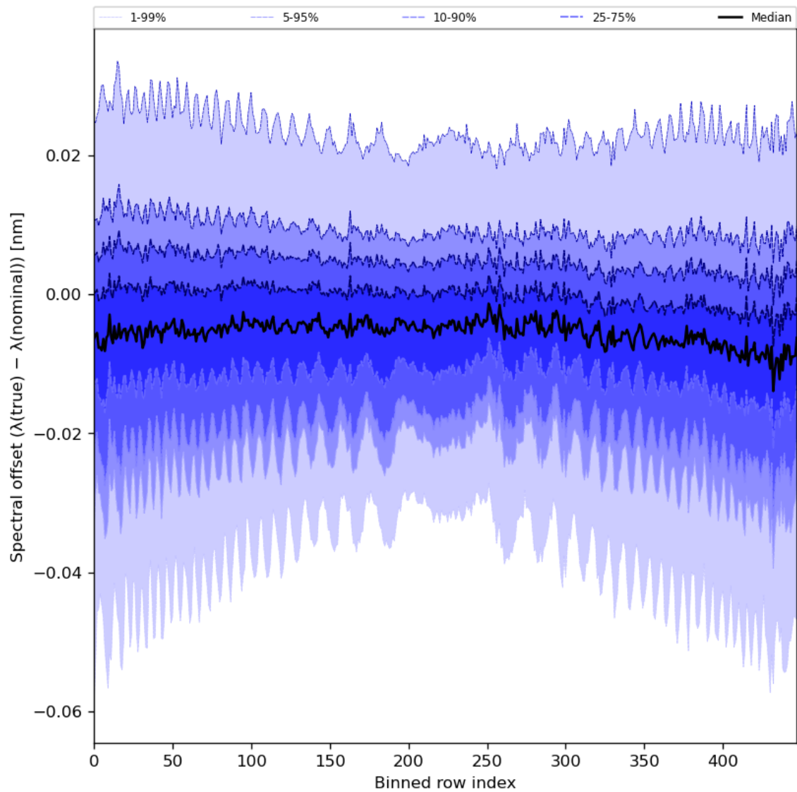
Figure 62: Along track statistics of “Spectral offset ( \lambda(\text{true}) - \lambda(\text{nominal}) )” for 2024-07-19 to 2024-07-21
