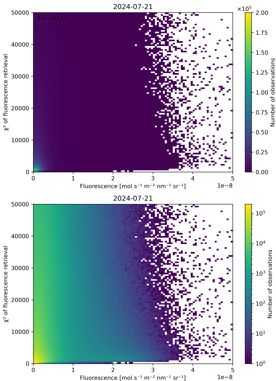
Figure 85: Scatter density plot of “Fluorescence” against “ \chi^2 of fluorescence retrieval” for 2024-07-21 to 2024-07-22.
