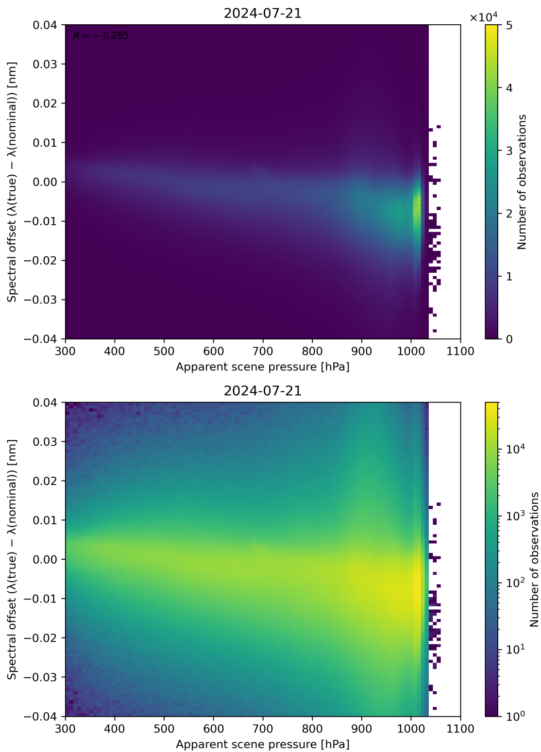
Figure 67: Scatter density plot of “Apparent scene pressure” against “Spectral offset ( \lambda(\text{true}) - \lambda(\text{nominal}) )” for 2024-07-21 to 2024-07-22.
