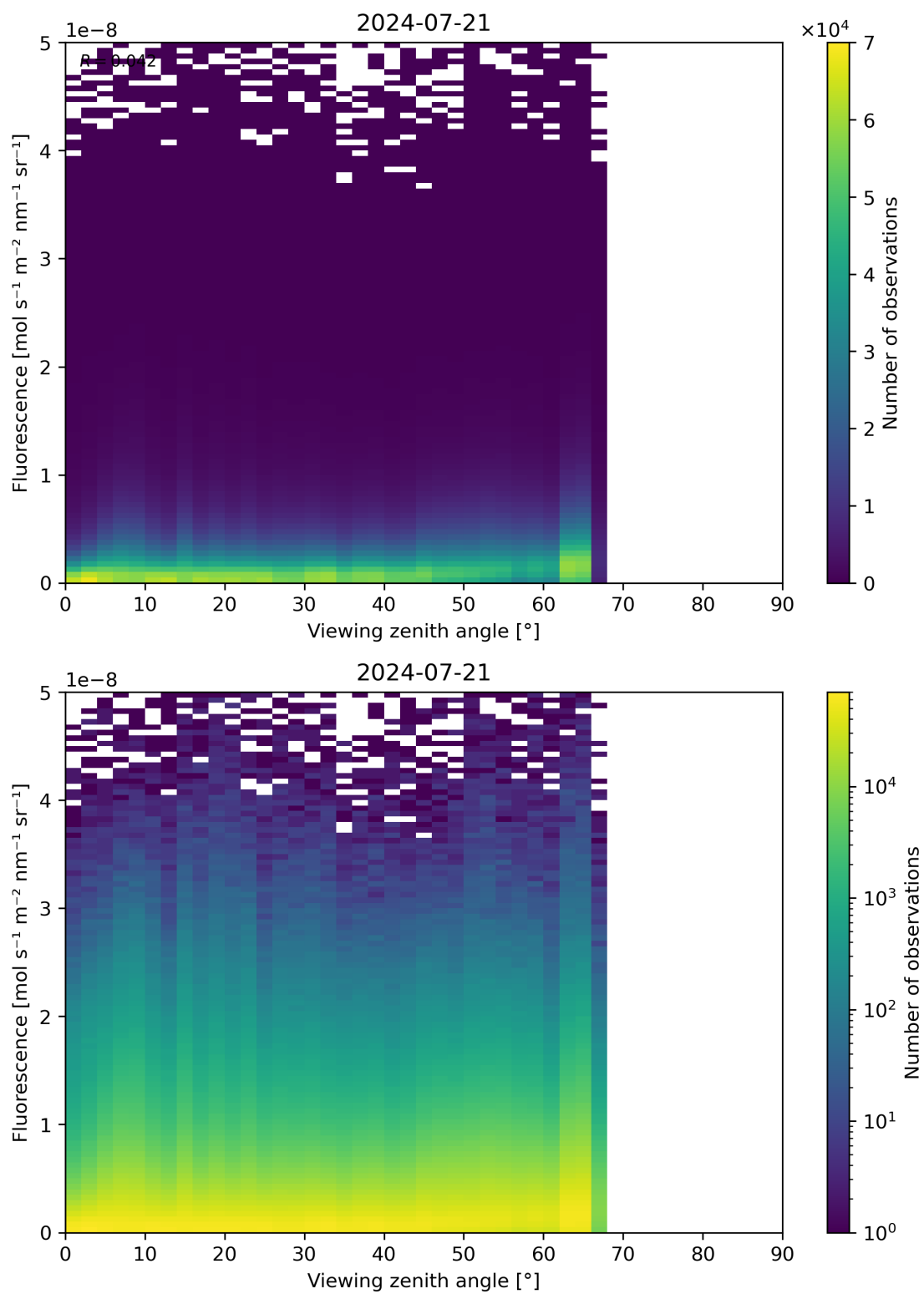
Figure 122: Scatter density plot of “Viewing zenith angle” against “Fluorescence” for 2024-07-21 to 2024-07-22.
