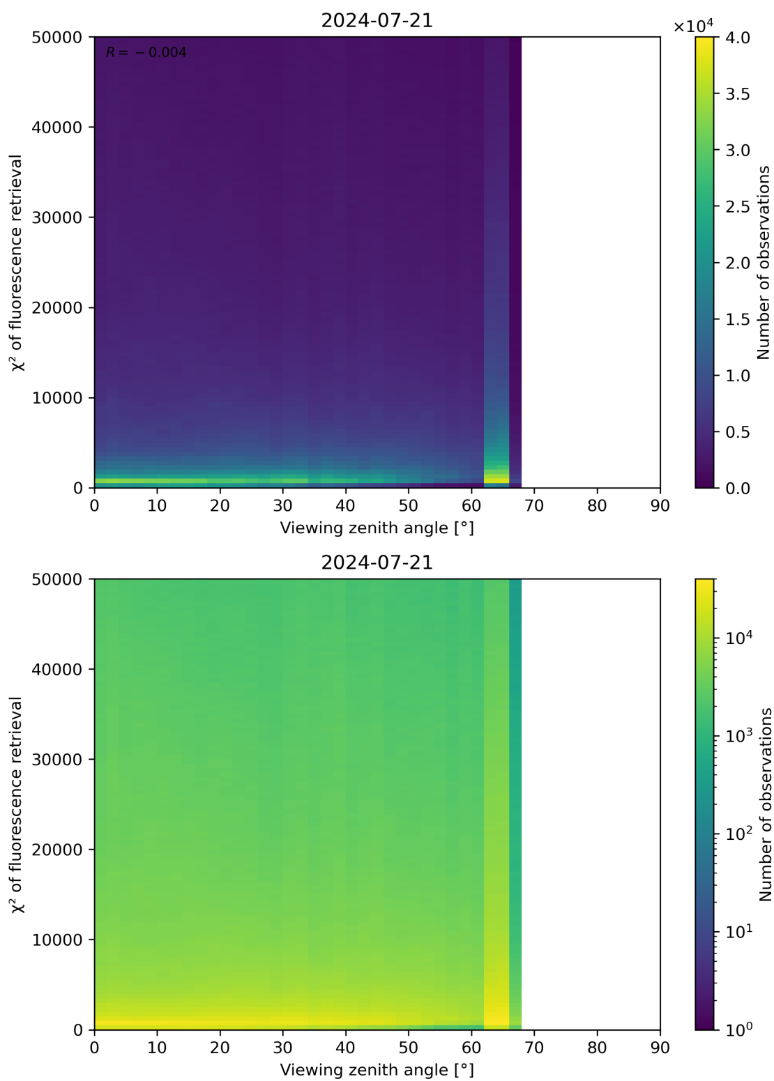
Figure 119: Scatter density plot of “Viewing zenith angle” against “ \chi^2 of fluorescence retrieval” for 2024-07-21 to 2024-07-22.
