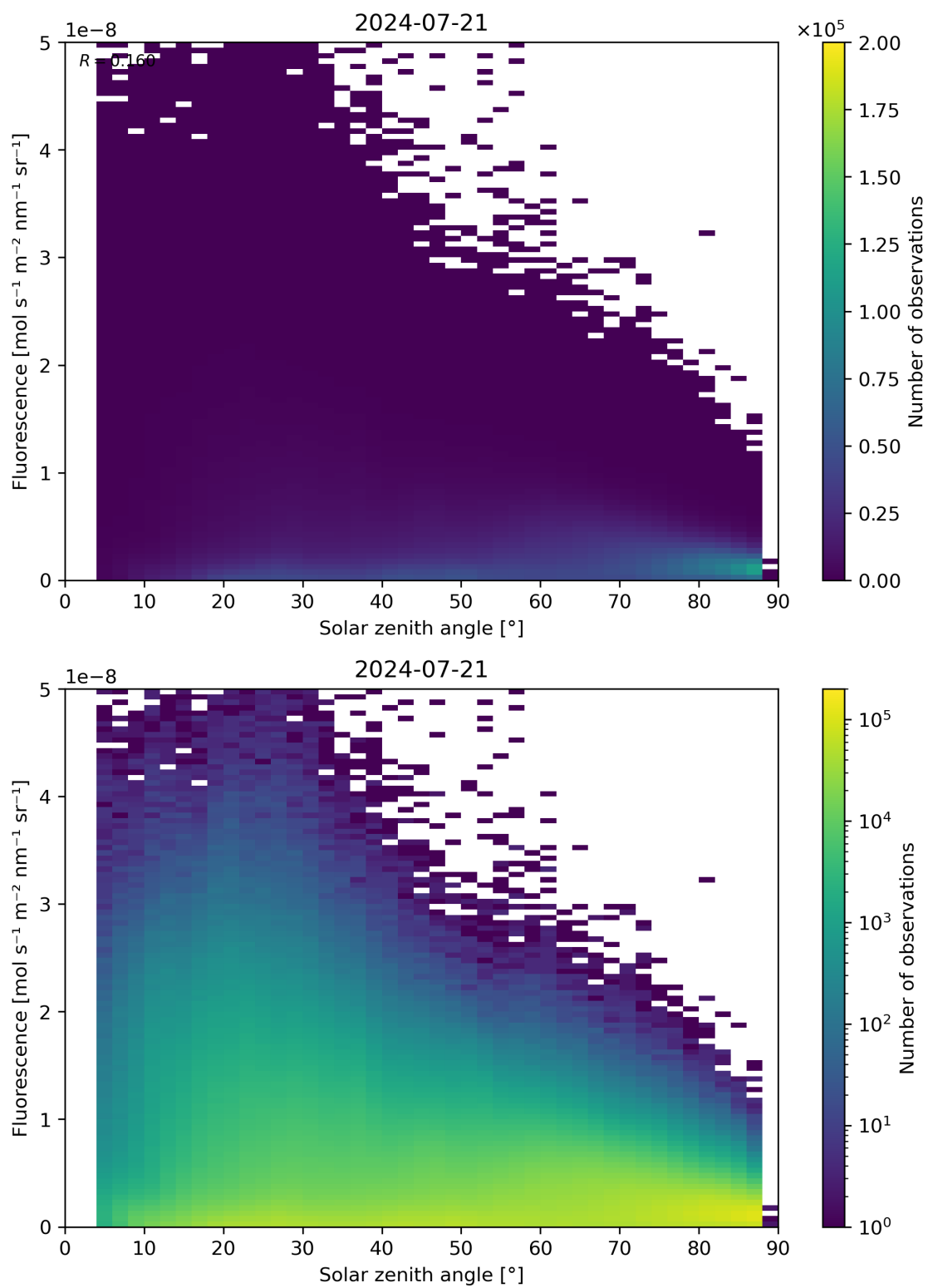
Figure 112: Scatter density plot of “Solar zenith angle” against “Fluorescence” for 2024-07-21 to 2024-07-22.
