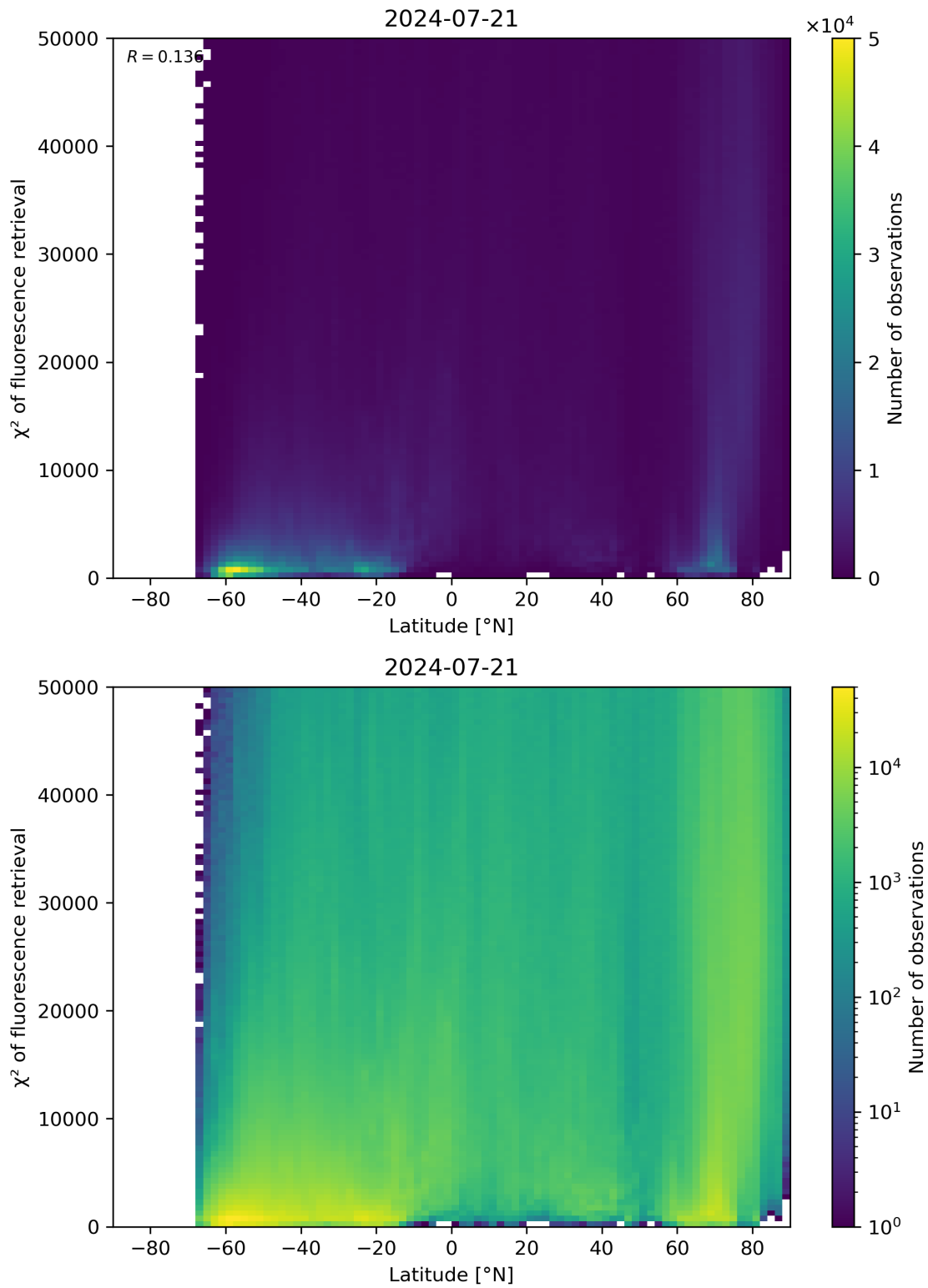
Figure 89: Scatter density plot of “Latitude” against “ \chi^2 of fluorescence retrieval” for 2024-07-21 to 2024-07-22.
