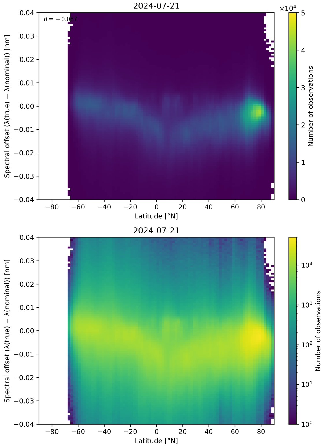
Figure 96: Scatter density plot of “Latitude” against “Spectral offset ( \lambda(\text{true}) - \lambda(\text{nominal}) )” for 2024-07-21 to 2024-07-22.
