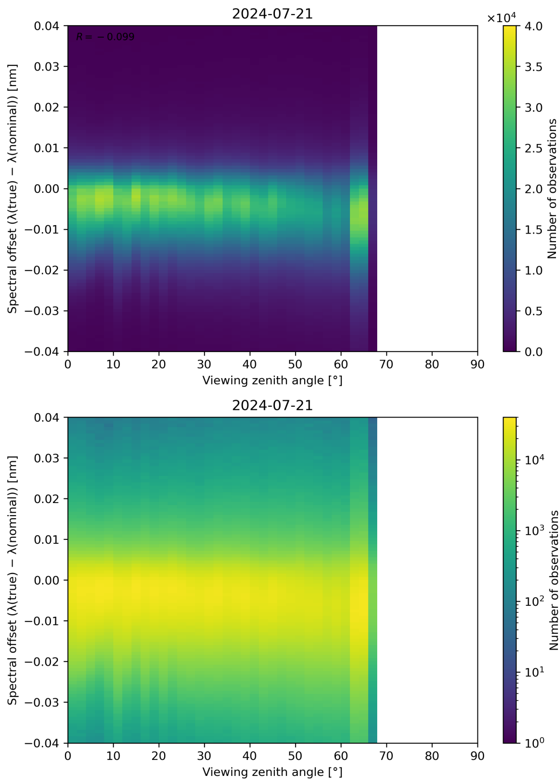
Figure 128: Scatter density plot of “Viewing zenith angle” against “Spectral offset ( \lambda(\text{true}) - \lambda(\text{nominal}) )” for 2024-07-21 to 2024-07-22.
