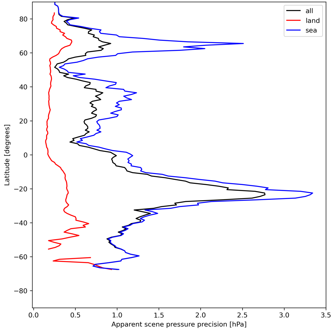
Figure 20: Zonal average of “Apparent scene pressure precision” for 2024-07-21 to 2024-07-22.
