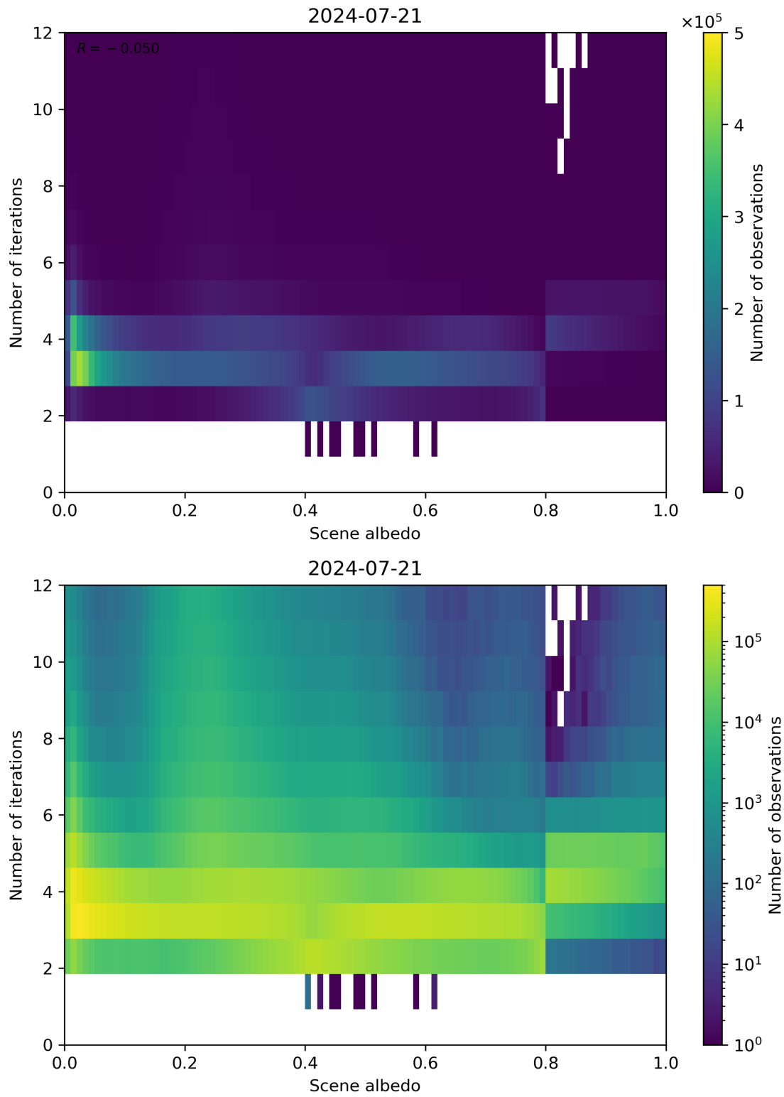
Figure 105: Scatter density plot of “Scene albedo” against “Number of iterations” for 2024-07-21 to 2024-07-22.
