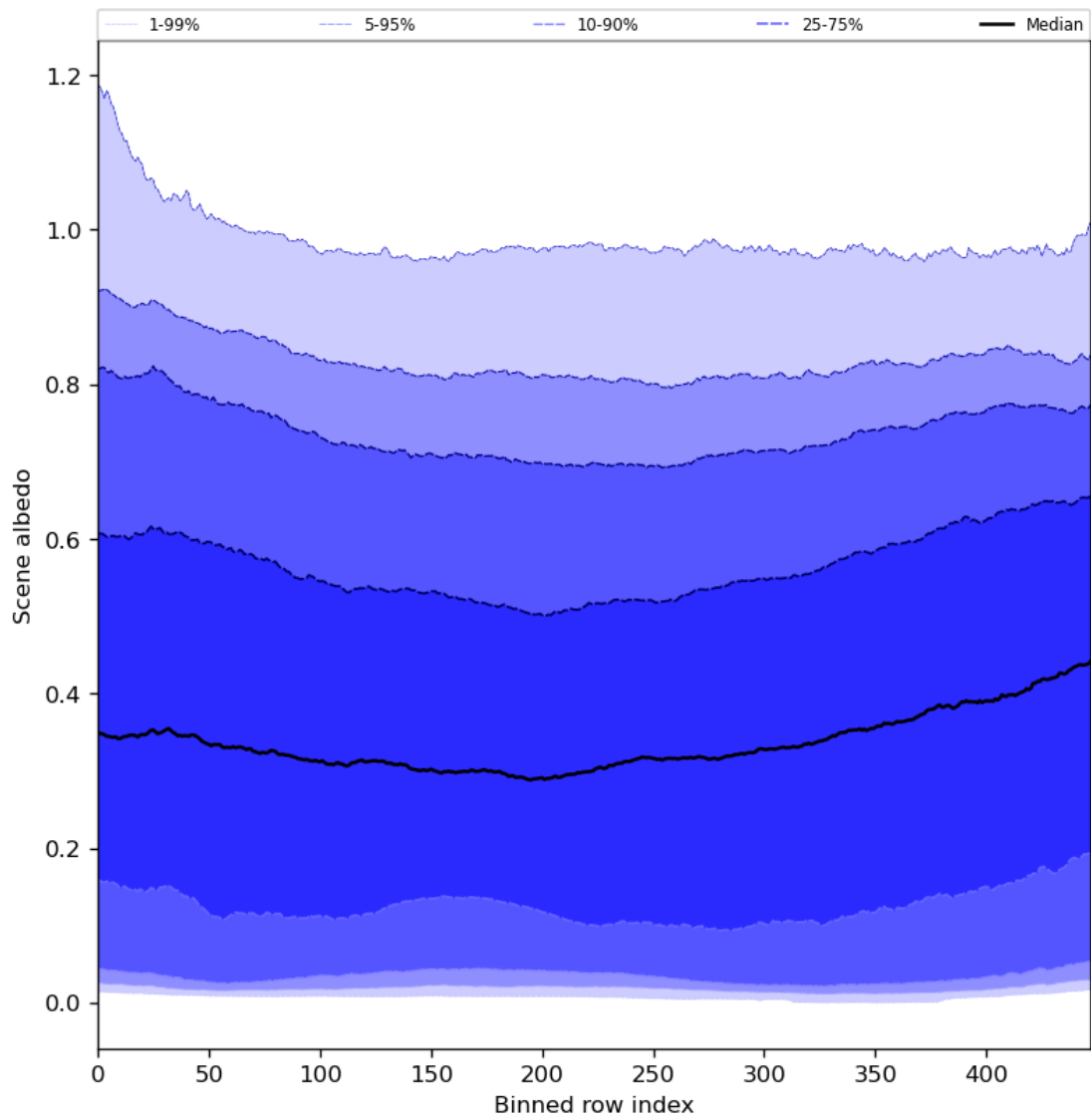
Figure 51: Along track statistics of “Scene albedo” for 2024-07-21 to 2024-07-22
