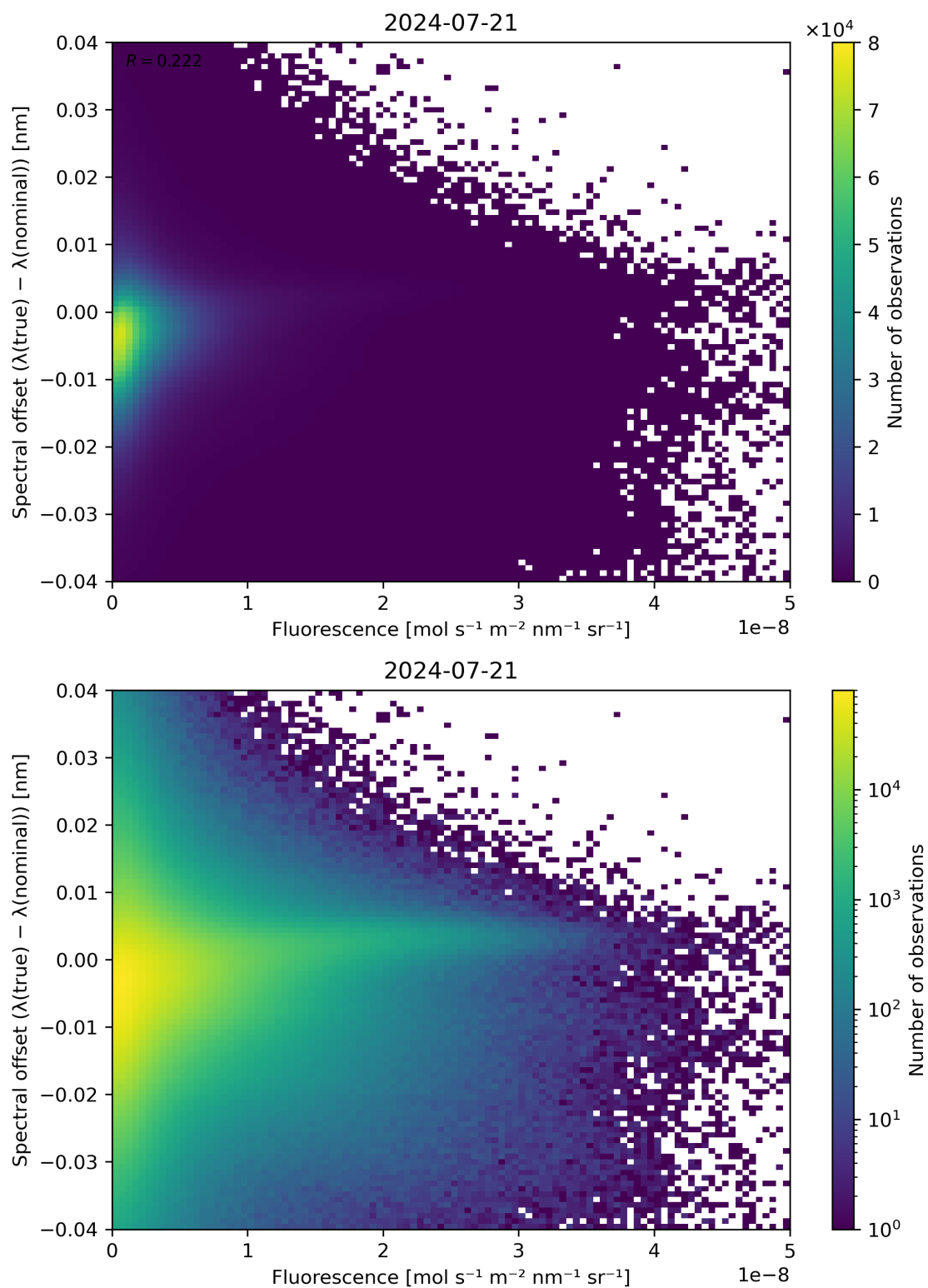
Figure 87: Scatter density plot of “Fluorescence” against “Spectral offset ( \lambda(\text{true}) - \lambda(\text{nominal}) )” for 2024-07-21 to 2024-07-22.
