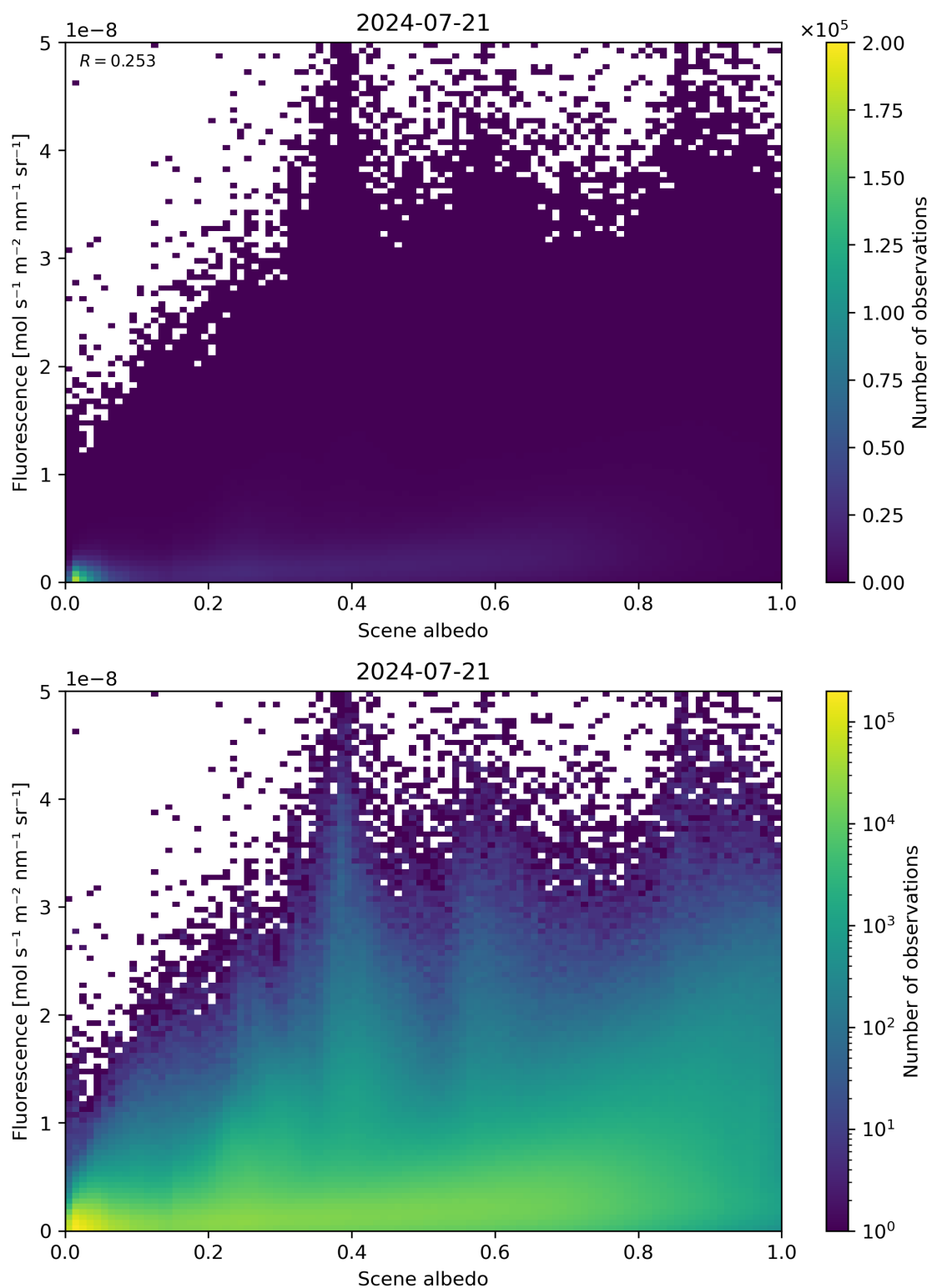
Figure 104: Scatter density plot of “Scene albedo” against “Fluorescence” for 2024-07-21 to 2024-07-22.
