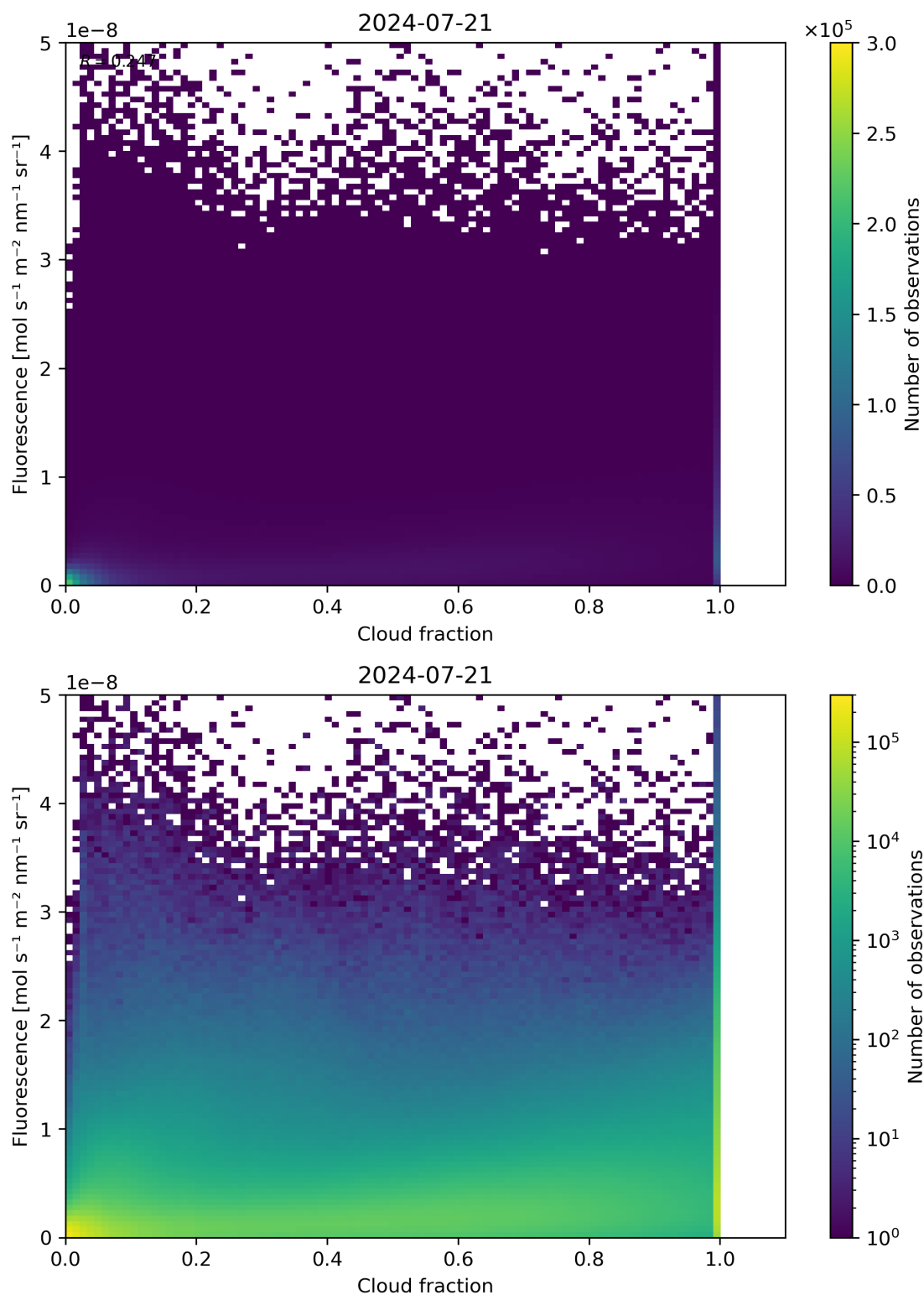
Figure 72: Scatter density plot of “Cloud fraction” against “Fluorescence” for 2024-07-21 to 2024-07-22.
