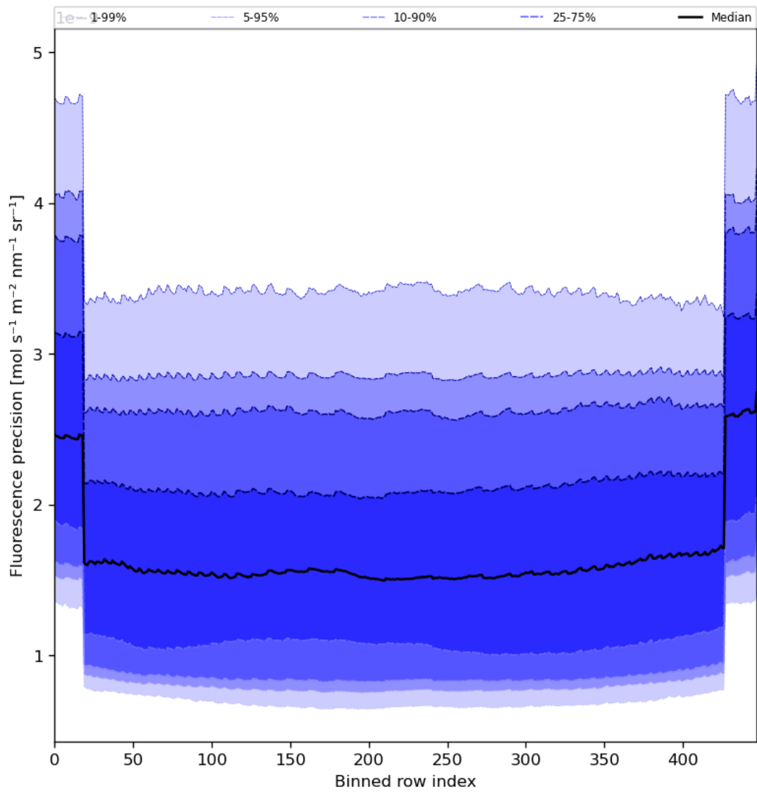
Figure 58: Along track statistics of “Fluorescence precision” for 2024-07-21 to 2024-07-22
