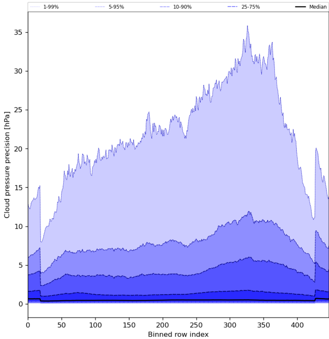
Figure 48: Along track statistics of “Cloud pressure precision” for 2024-07-21 to 2024-07-22
