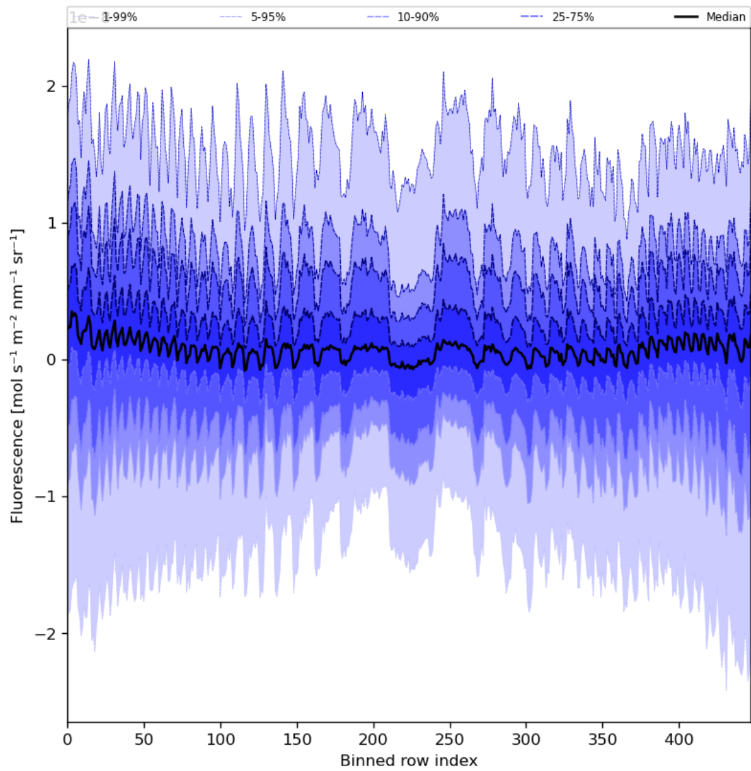
Figure 57: Along track statistics of “Fluorescence” for 2024-07-21 to 2024-07-22
