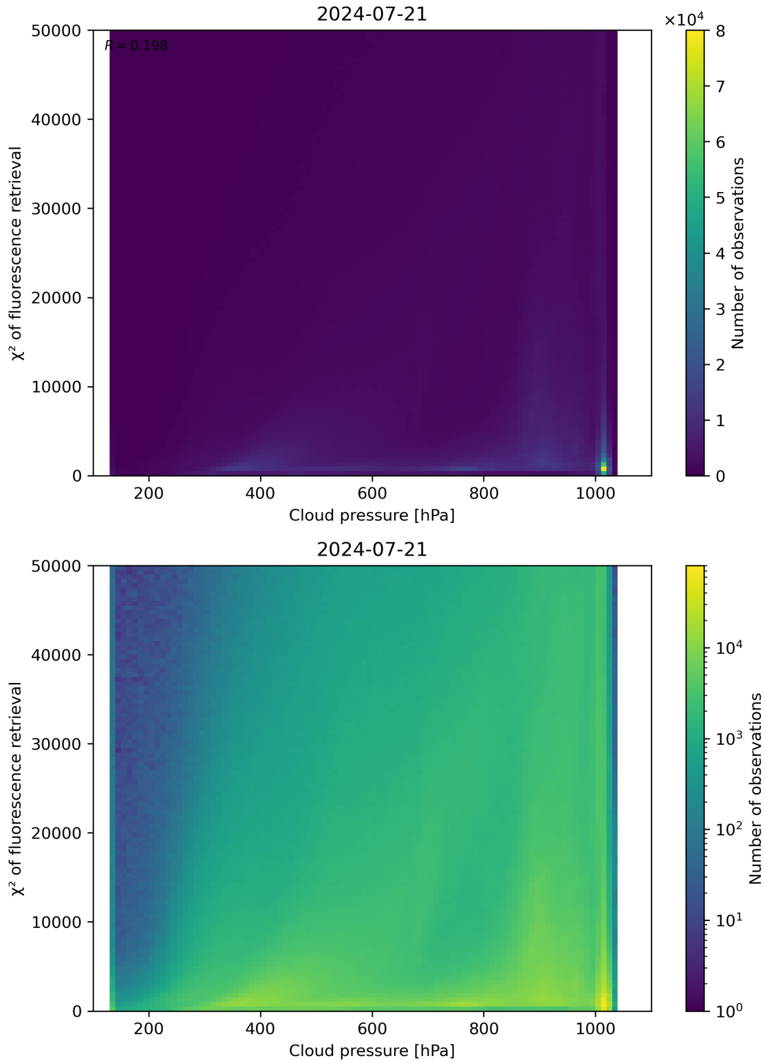
Figure 78: Scatter density plot of “Cloud pressure” against “ \chi^2 of fluorescence retrieval” for 2024-07-21 to 2024-07-22.
