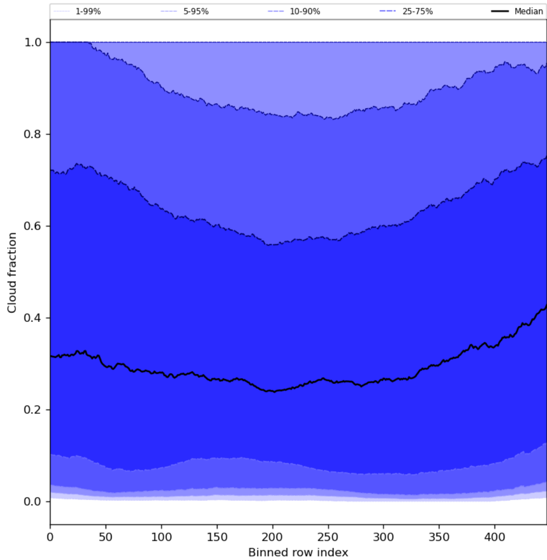
Figure 49: Along track statistics of “Cloud fraction” for 2024-07-21 to 2024-07-22
