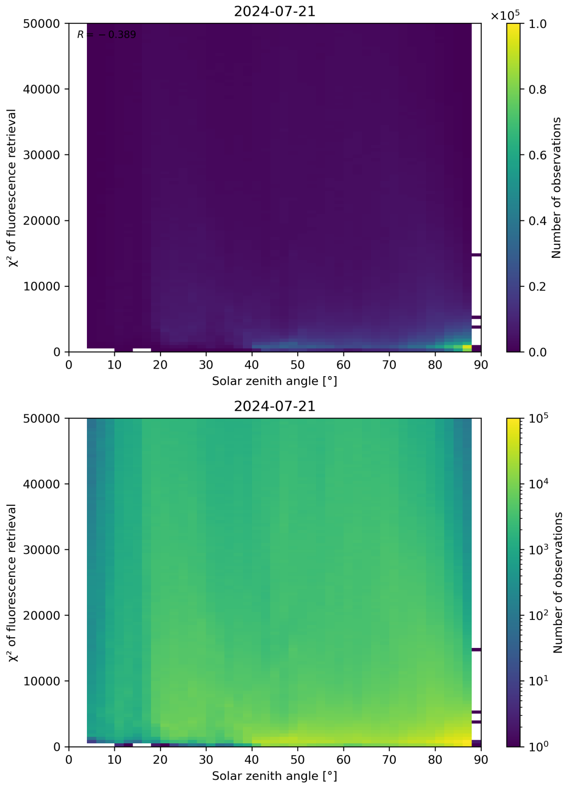
Figure 109: Scatter density plot of “Solar zenith angle” against “ \chi^2 of fluorescence retrieval” for 2024-07-21 to 2024-07-22.
