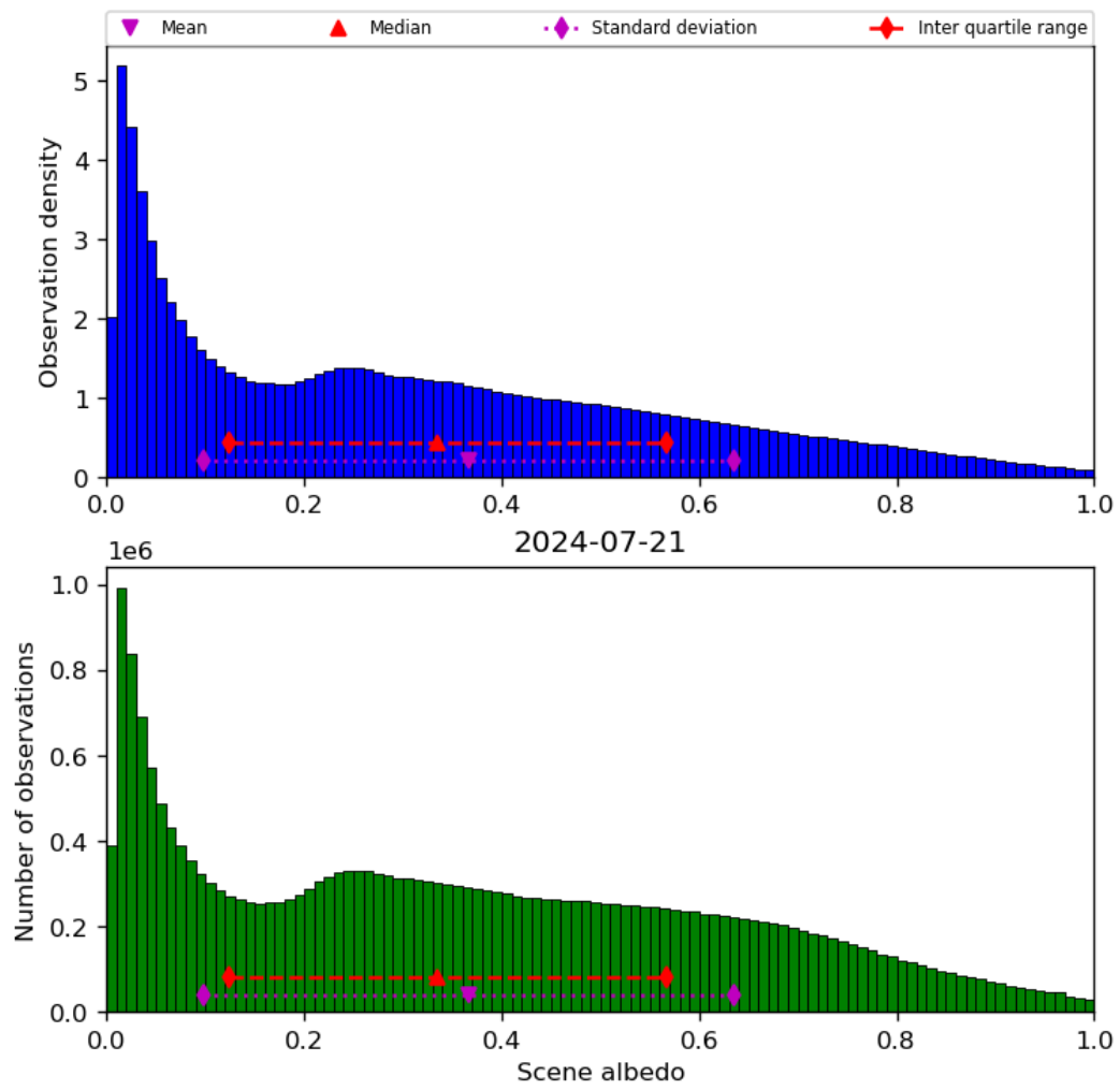
Figure 34: Histogram of “Scene albedo” for 2024-07-21 to 2024-07-22
