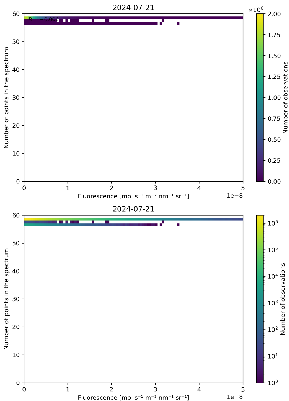
Figure 86: Scatter density plot of “Fluorescence” against “Number of points in the spectrum” for 2024-07-21 to 2024-07-22.
