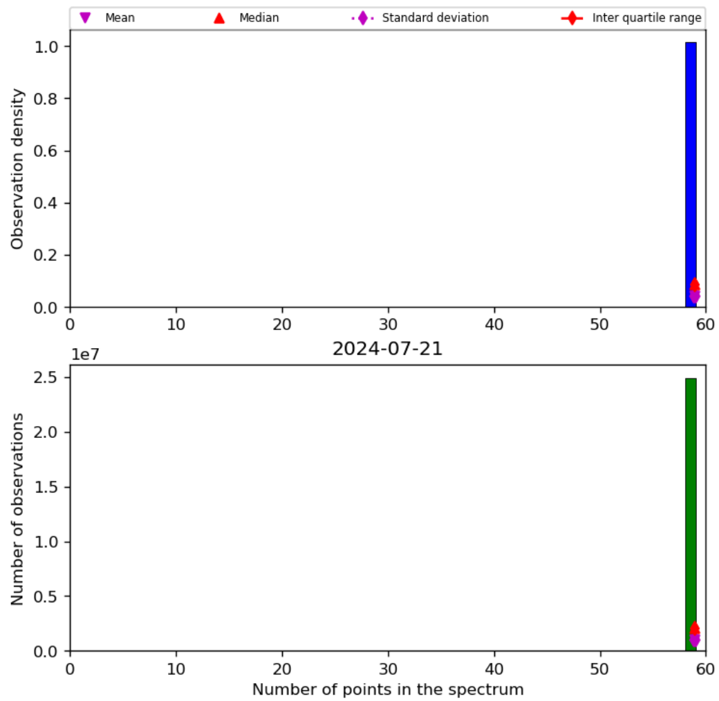
Figure 44: Histogram of “Number of points in the spectrum” for 2024-07-21 to 2024-07-22
