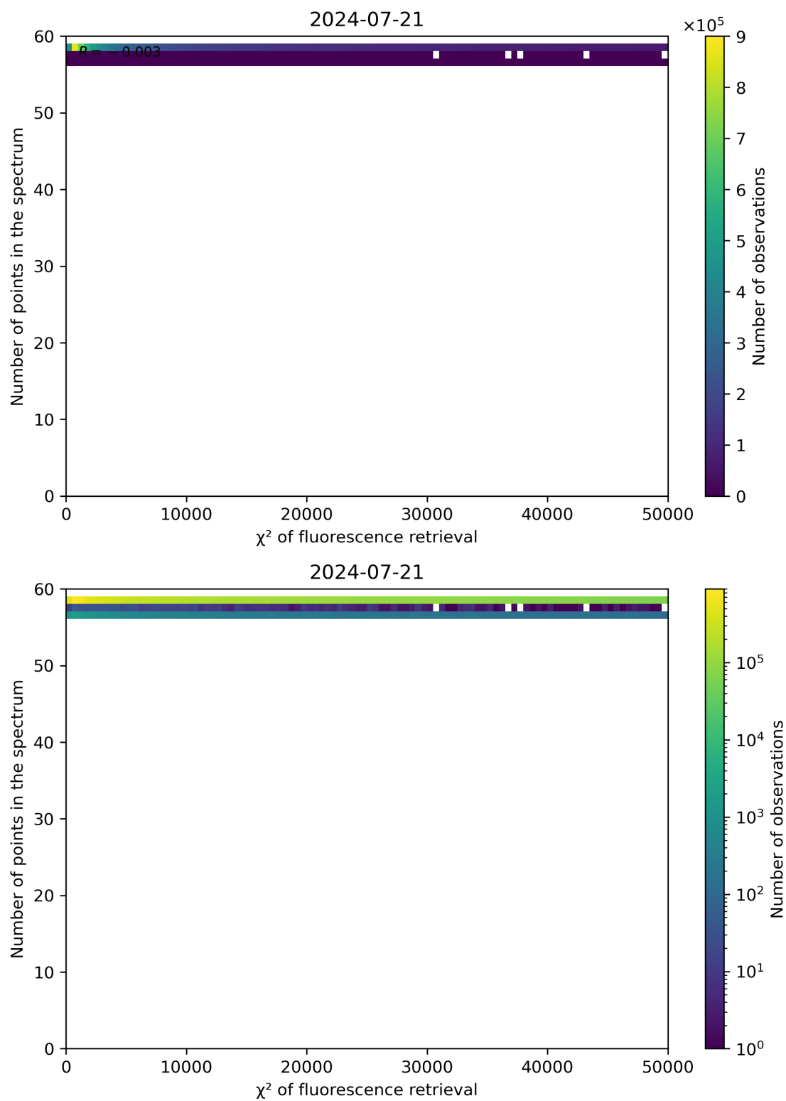
Figure 68: Scatter density plot of “ \chi^2 of fluorescence retrieval” against “Number of points in the spectrum” for 2024-07-21 to 2024-07-22.
