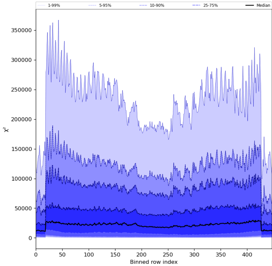
Figure 55: Along track statistics of " \chi^2 " for 2024-07-21 to 2024-07-22
