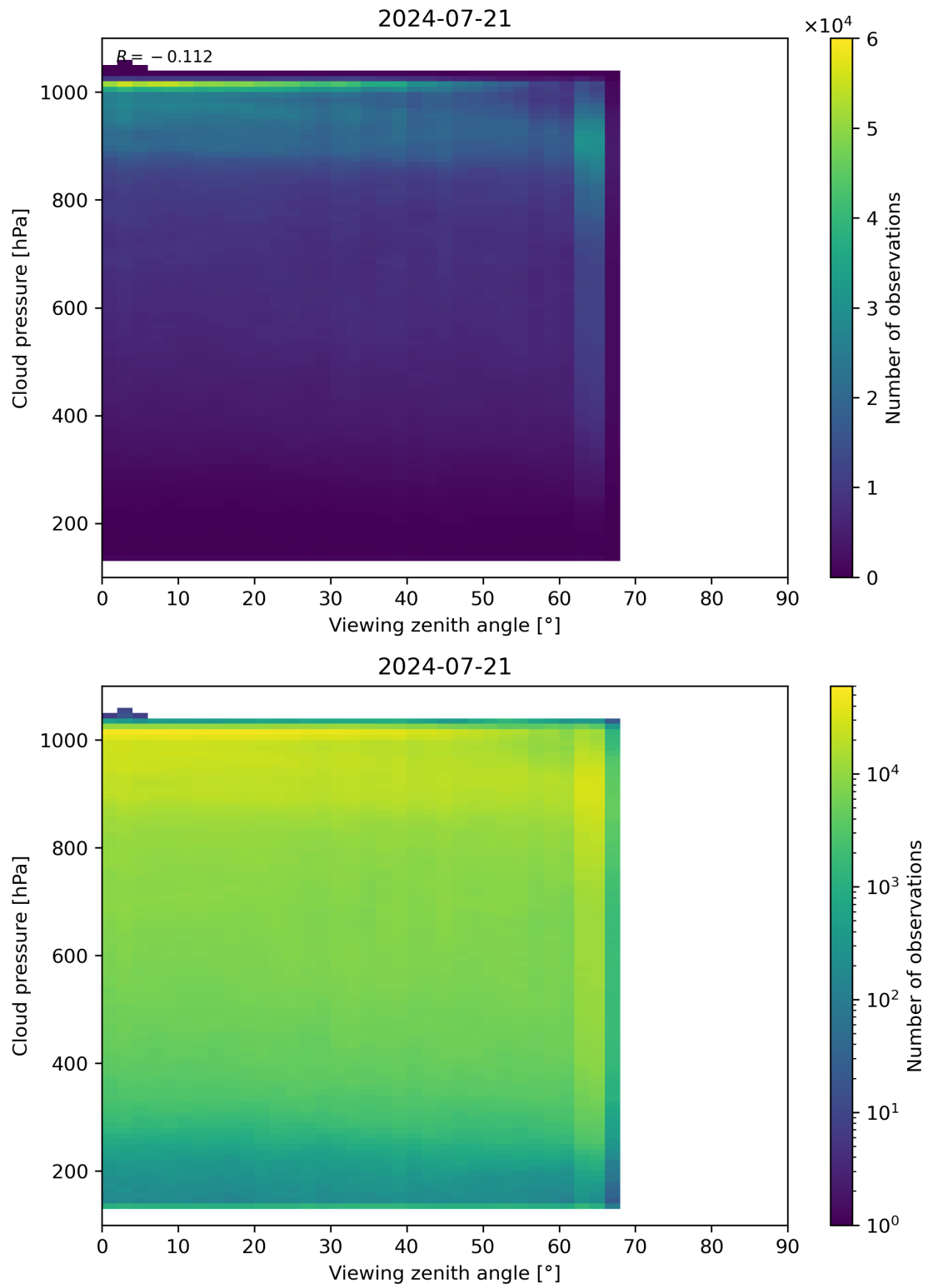
Figure 121: Scatter density plot of “Viewing zenith angle” against “Cloud pressure” for 2024-07-21 to 2024-07-22.
