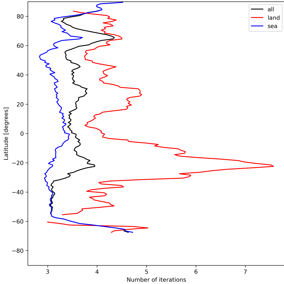
Figure 22: Zonal average of “Number of iterations” for 2024-07-21 to 2024-07-22.
