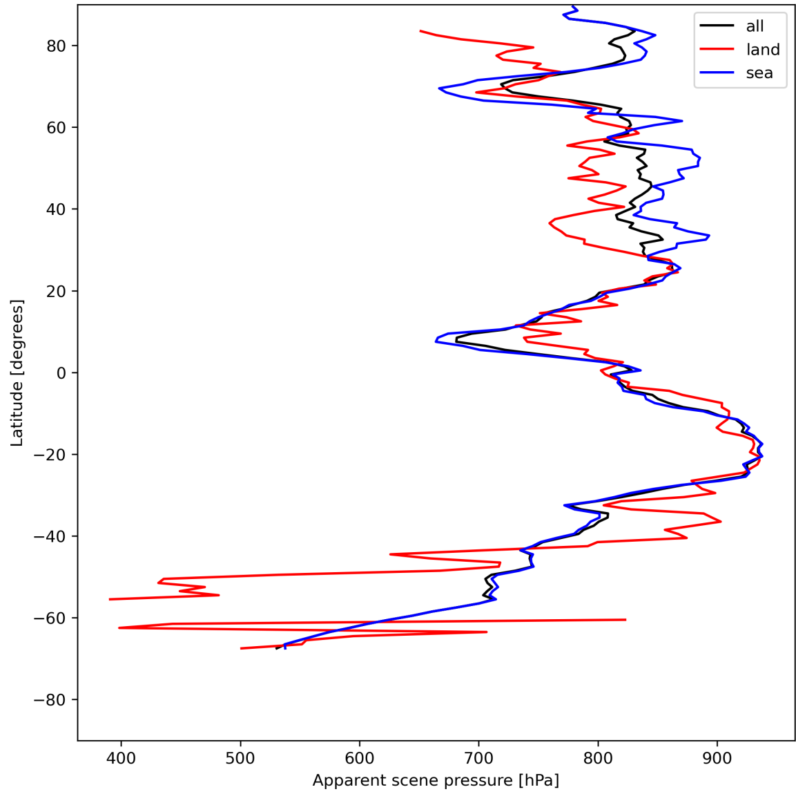
Figure 19: Zonal average of “Apparent scene pressure” for 2024-07-21 to 2024-07-22.
