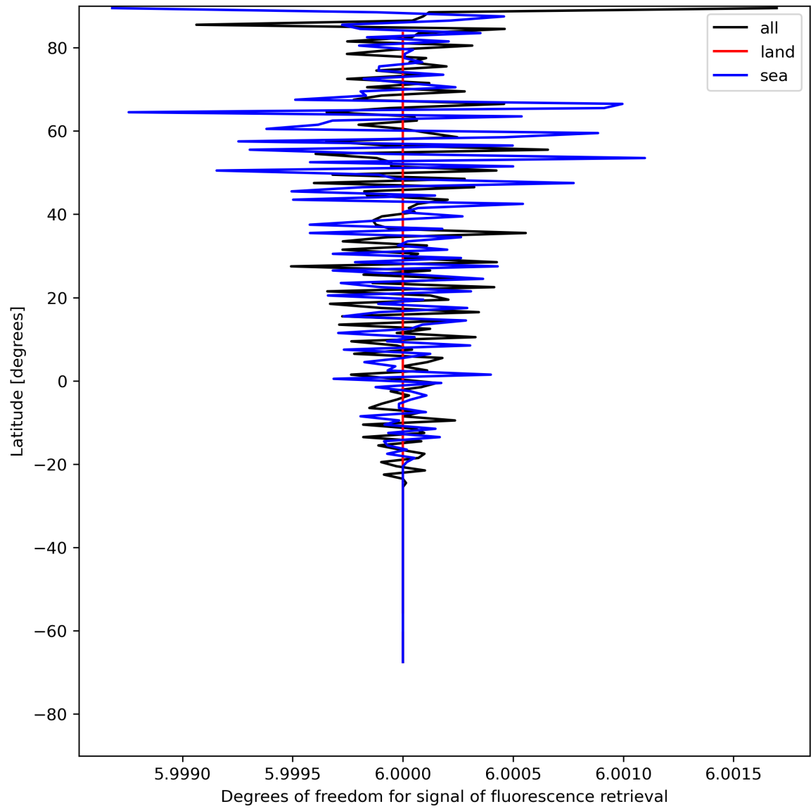
Figure 26: Zonal average of “Degrees of freedom for signal of fluorescence retrieval” for 2024-07-21 to 2024-07-22.
