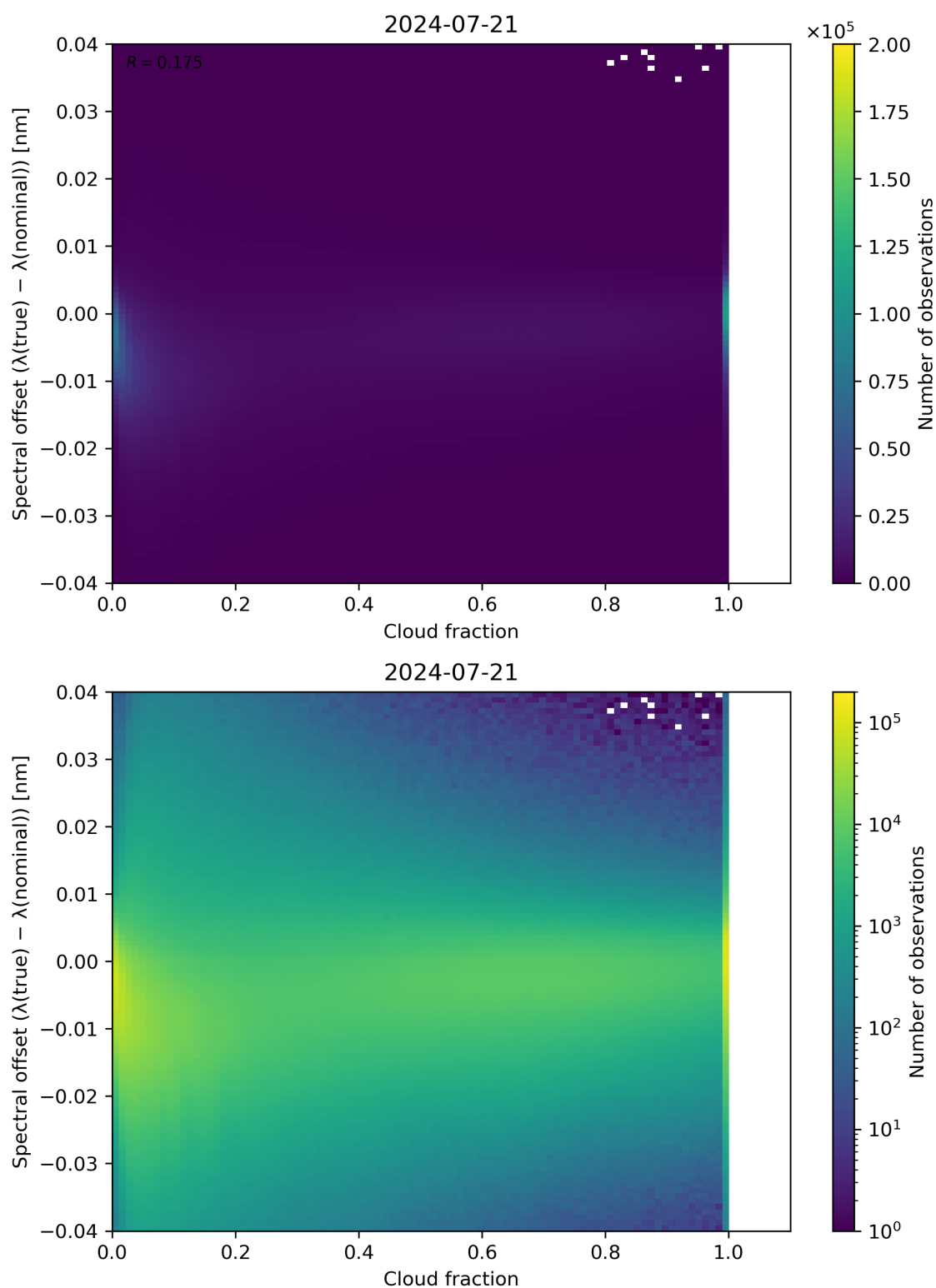
Figure 76: Scatter density plot of “Cloud fraction” against “Spectral offset ( \lambda(\text{true}) - \lambda(\text{nominal}) )” for 2024-07-21 to 2024-07-22.
