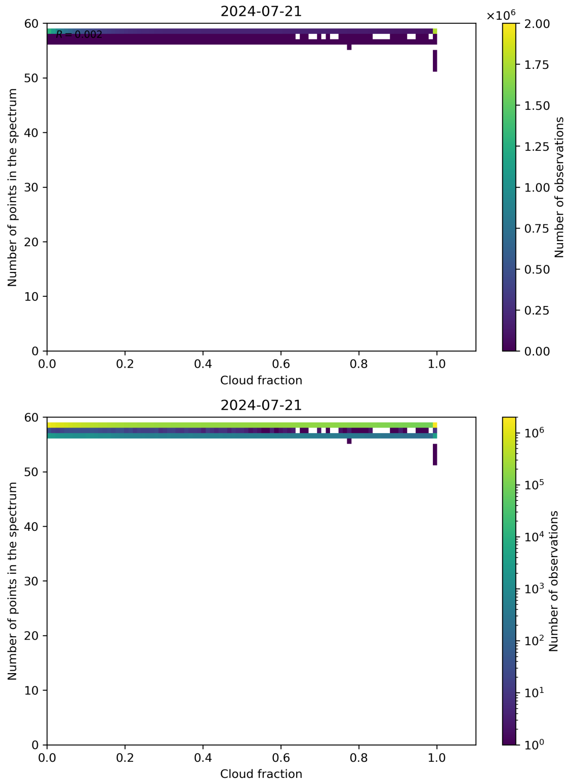
Figure 74: Scatter density plot of “Cloud fraction” against “Number of points in the spectrum” for 2024-07-21 to 2024-07-22.
