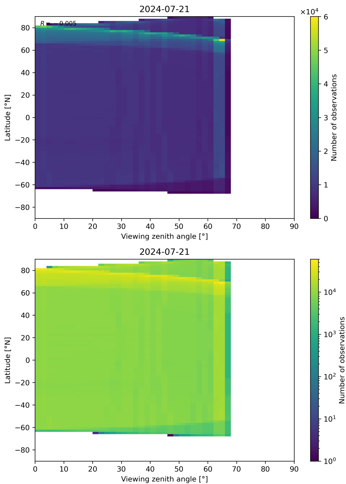
Figure 123: Scatter density plot of “Viewing zenith angle” against “Latitude” for 2024-07-21 to 2024-07-22.
