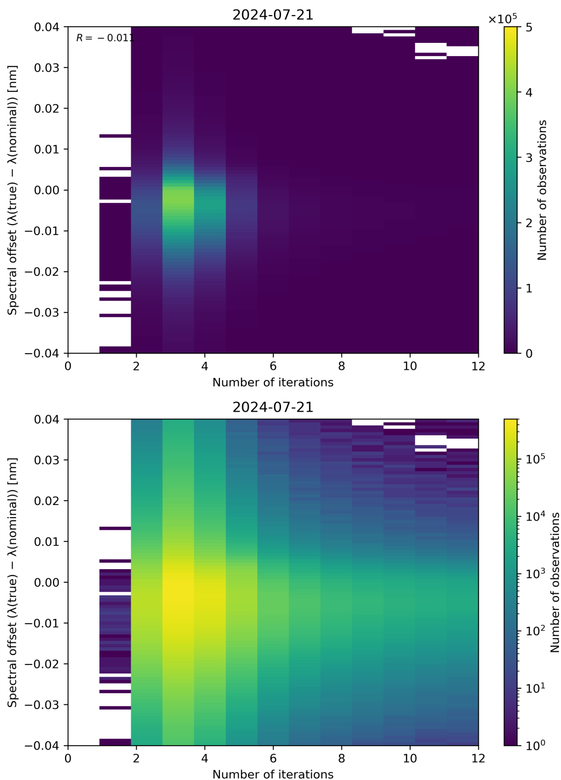
Figure 100: Scatter density plot of “Number of iterations” against “Spectral offset ( \lambda(\text{true}) - \lambda(\text{nominal}) )” for 2024-07-21 to 2024-07-22.
