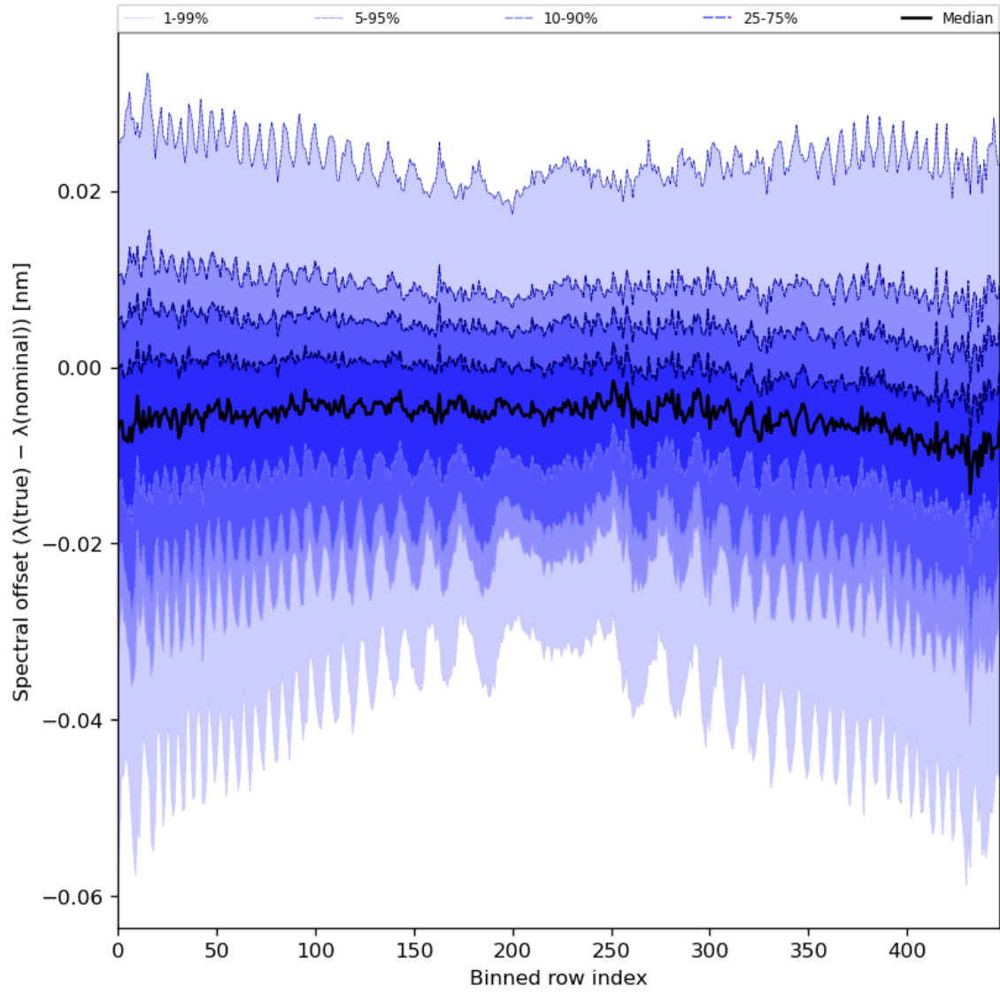
Figure 62: Along track statistics of “Spectral offset ( \lambda(\text{true}) - \lambda(\text{nominal}) )” for 2024-07-21 to 2024-07-22
