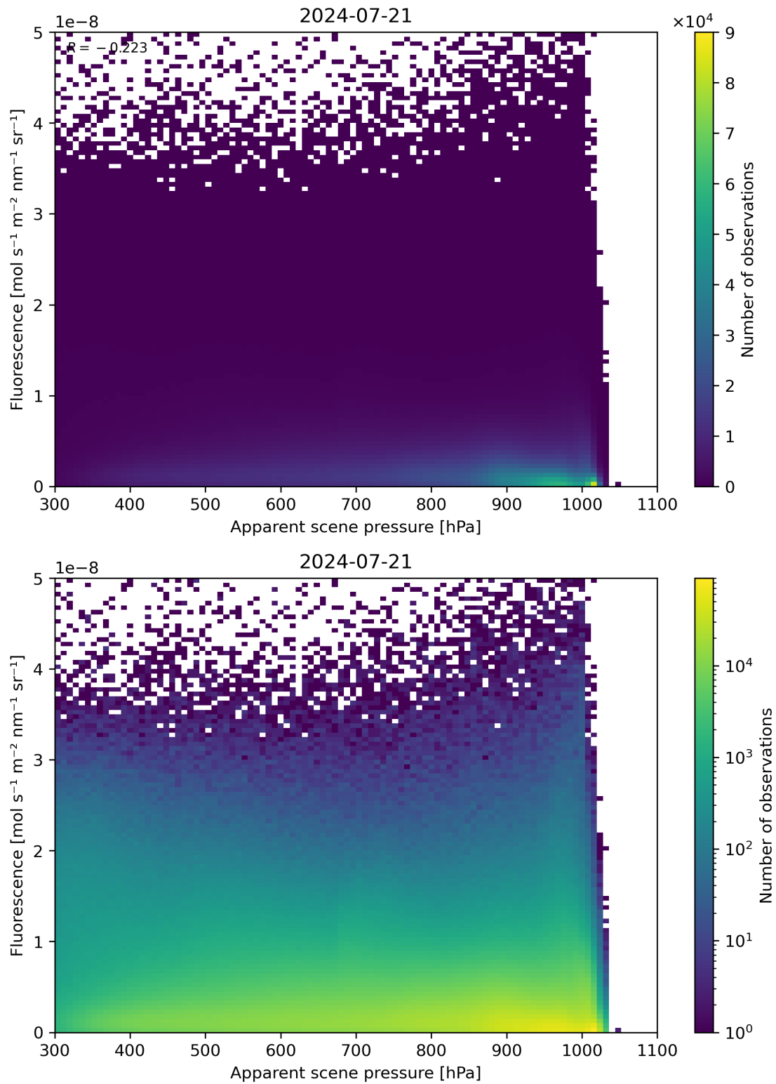
Figure 64: Scatter density plot of “Apparent scene pressure” against “Fluorescence” for 2024-07-21 to 2024-07-22.
