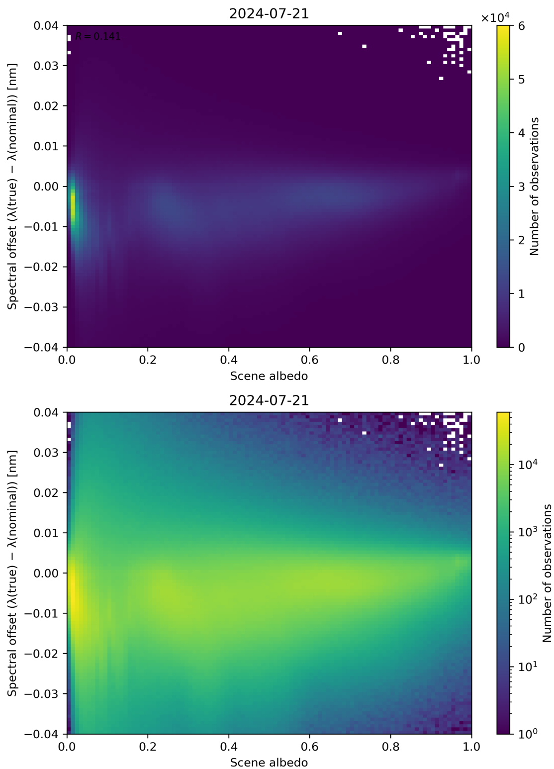
Figure 107: Scatter density plot of “Scene albedo” against “Spectral offset ( \lambda(\text{true}) - \lambda(\text{nominal}) )” for 2024-07-21 to 2024-07-22.
