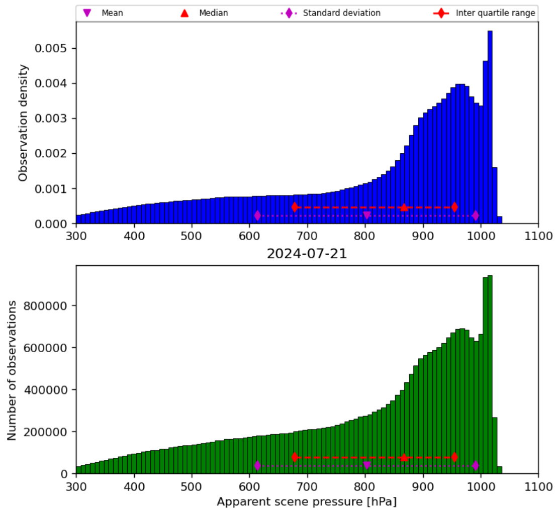
Figure 36: Histogram of “Apparent scene pressure” for 2024-07-21 to 2024-07-22
