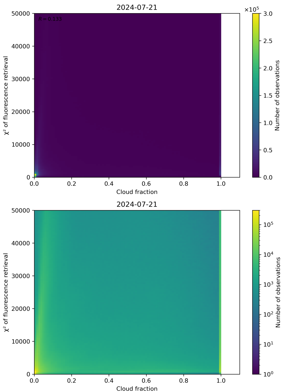
Figure 71: Scatter density plot of “Cloud fraction” against “ \chi^2 of fluorescence retrieval” for 2024-07-21 to 2024-07-22.
