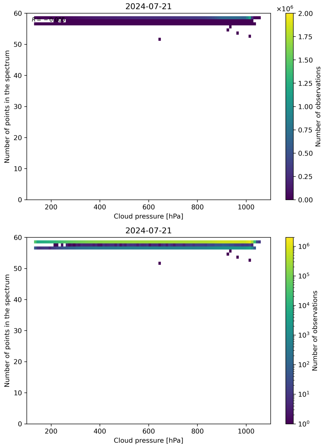
Figure 82: Scatter density plot of “Cloud pressure” against “Number of points in the spectrum” for 2024-07-21 to 2024-07-22.
