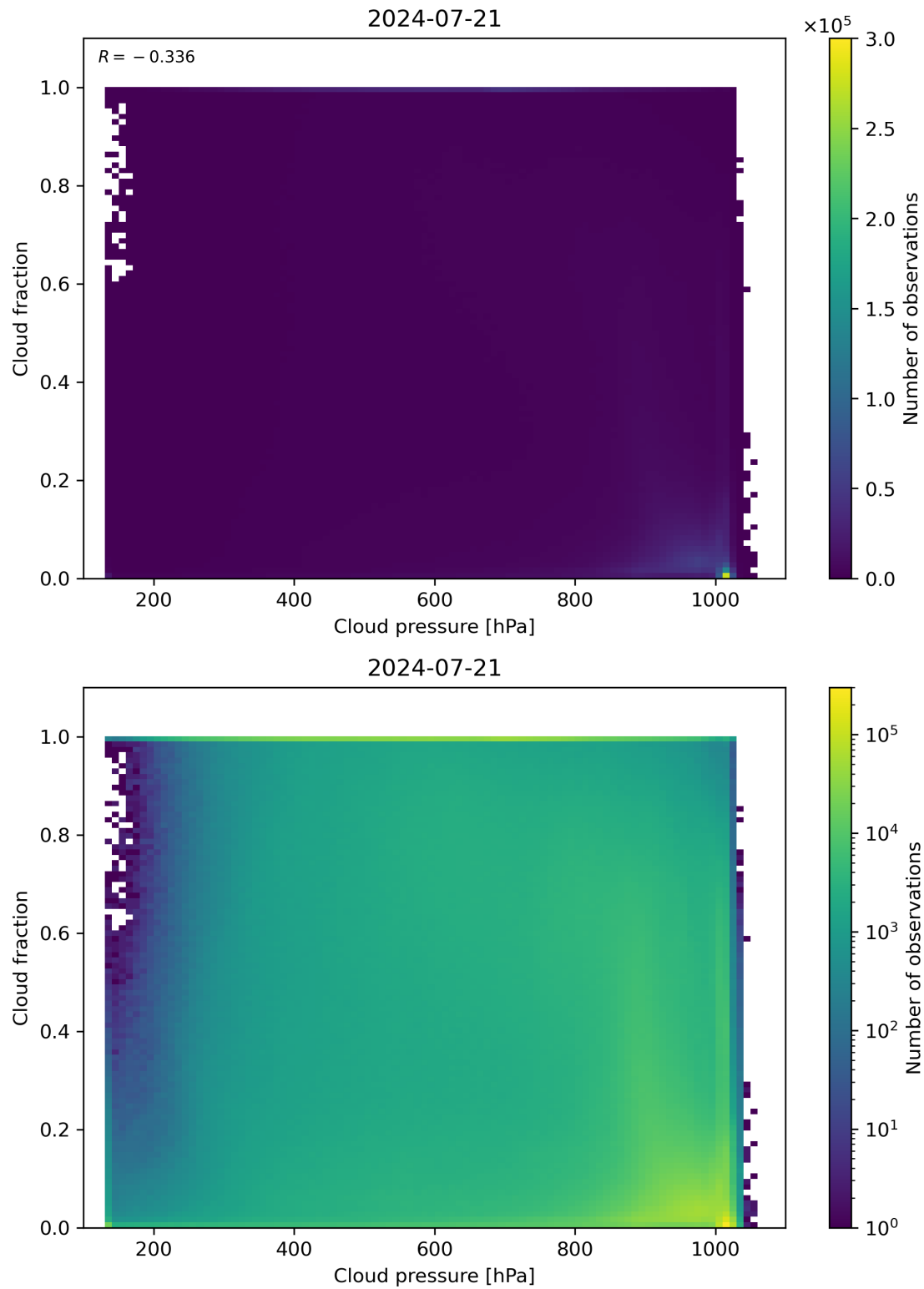
Figure 79: Scatter density plot of “Cloud pressure” against “Cloud fraction” for 2024-07-21 to 2024-07-22.
