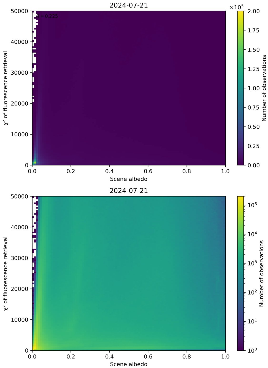
Figure 103: Scatter density plot of “Scene albedo” against “ \chi^2 of fluorescence retrieval” for 2024-07-21 to 2024-07-22.
