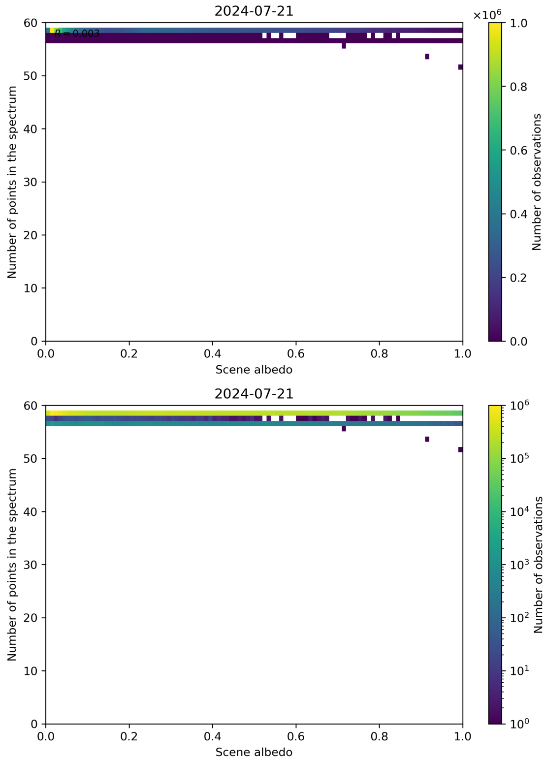
Figure 106: Scatter density plot of “Scene albedo” against “Number of points in the spectrum” for 2024-07-21 to 2024-07-22.
