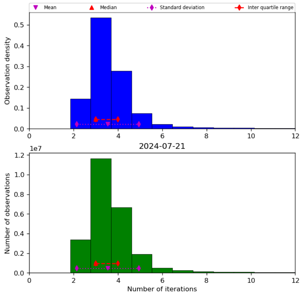
Figure 39: Histogram of “Number of iterations” for 2024-07-21 to 2024-07-22
