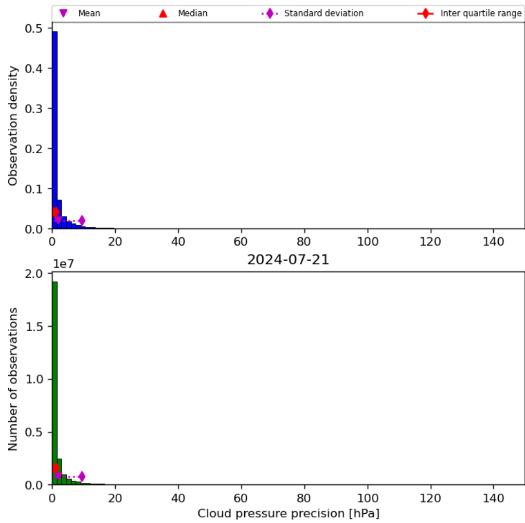
Figure 31: Histogram of “Cloud pressure precision” for 2024-07-21 to 2024-07-22
