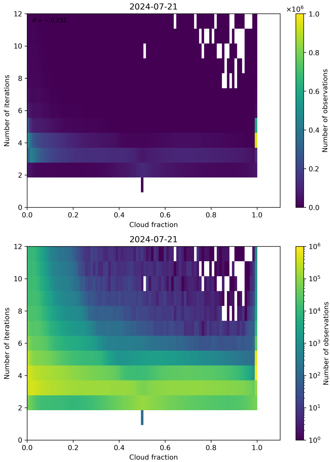
Figure 73: Scatter density plot of “Cloud fraction” against “Number of iterations” for 2024-07-21 to 2024-07-22.
