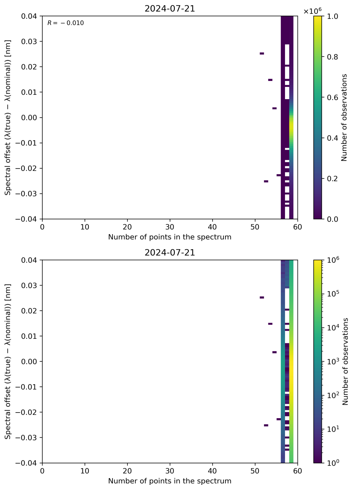
Figure 101: Scatter density plot of “Number of points in the spectrum” against “Spectral offset ( \lambda(\text{true}) - \lambda(\text{nominal}) )” for 2024-07-21 to 2024-07-22.
