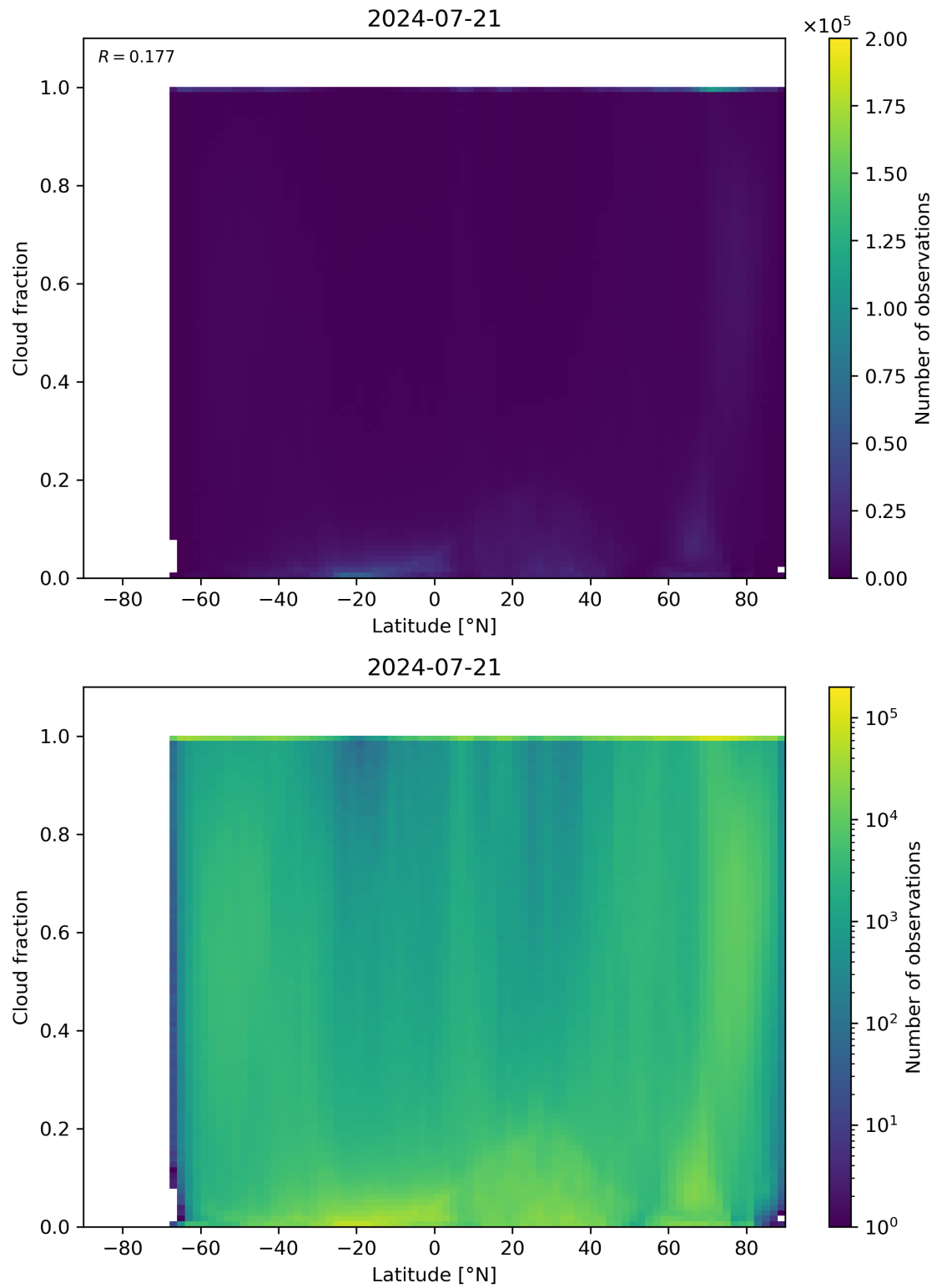
Figure 90: Scatter density plot of “Latitude” against “Cloud fraction” for 2024-07-21 to 2024-07-22.
