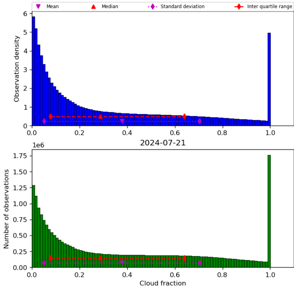
Figure 32: Histogram of “Cloud fraction” for 2024-07-21 to 2024-07-22
