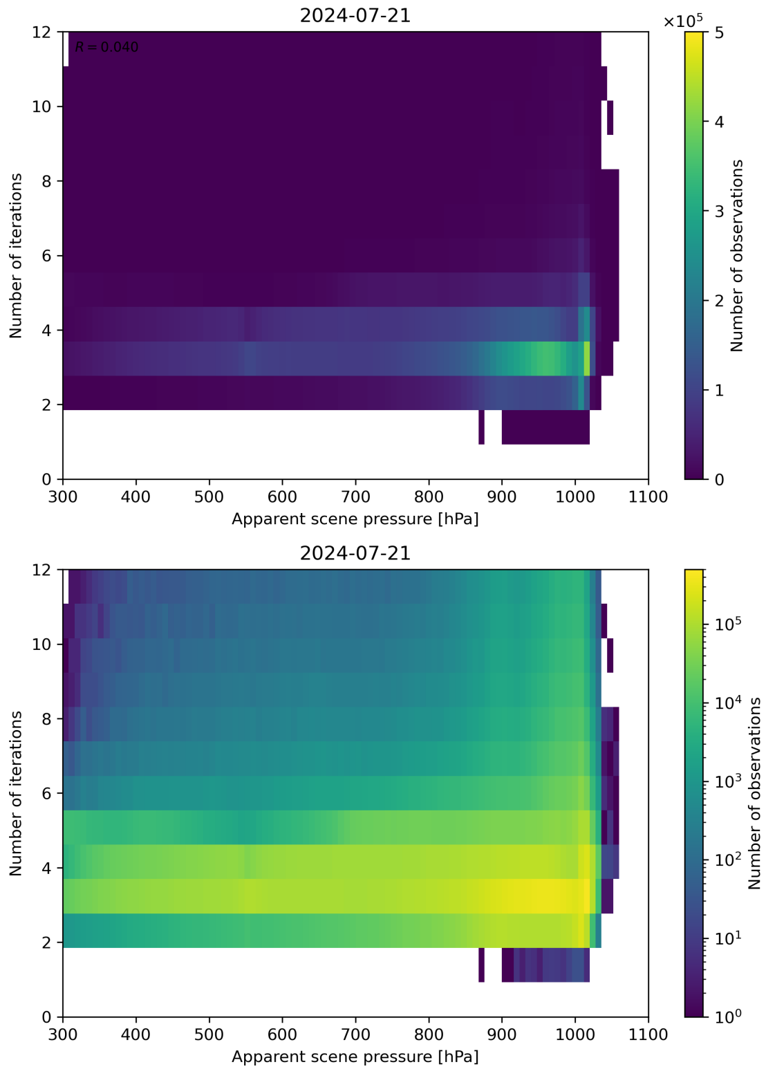
Figure 65: Scatter density plot of “Apparent scene pressure” against “Number of iterations” for 2024-07-21 to 2024-07-22.
