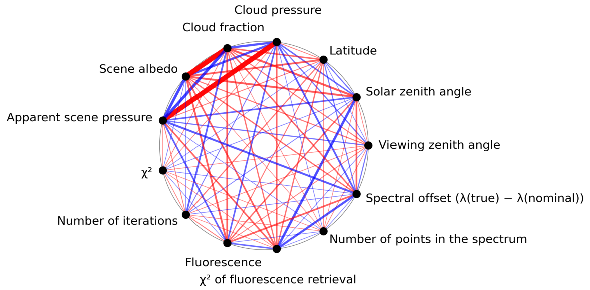
Figure 1: Map of correlation graph for 2024-07-21 to 2024-07-22.
