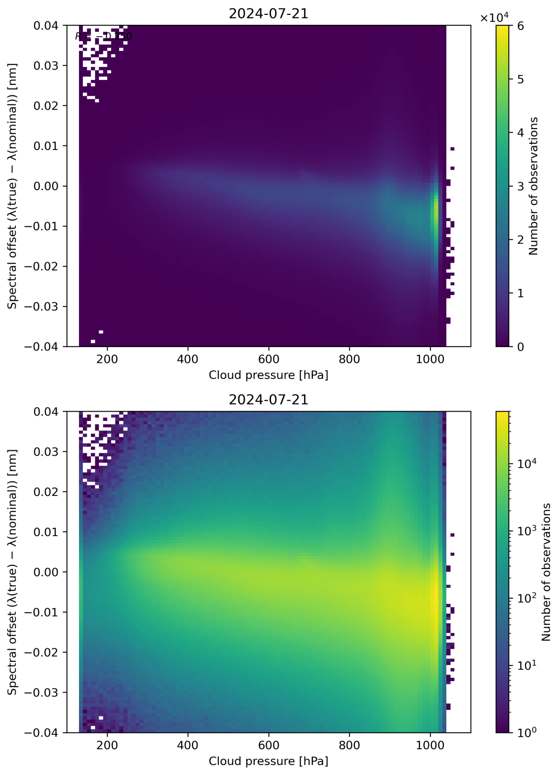
Figure 84: Scatter density plot of “Cloud pressure” against “Spectral offset ( \lambda(\text{true}) - \lambda(\text{nominal}) )” for 2024-07-21 to 2024-07-22.
