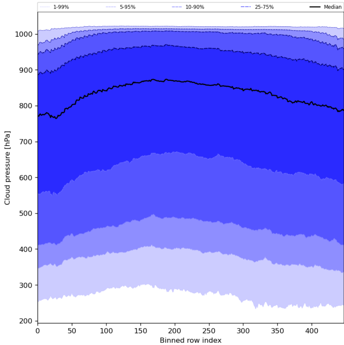
Figure 47: Along track statistics of “Cloud pressure” for 2024-07-21 to 2024-07-22
