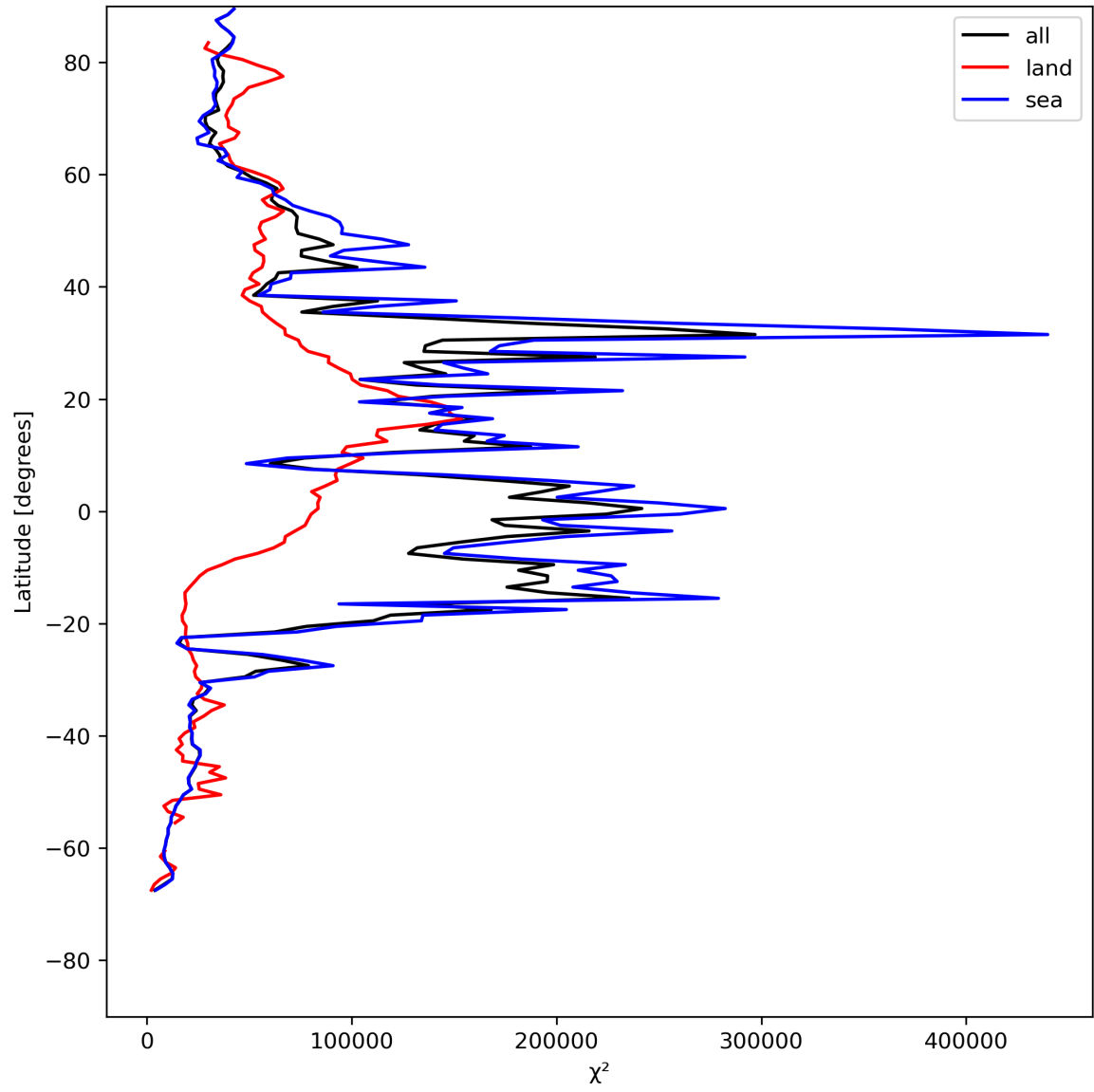
Figure 21: Zonal average of “ \chi^2 ” for 2024-07-21 to 2024-07-22.
