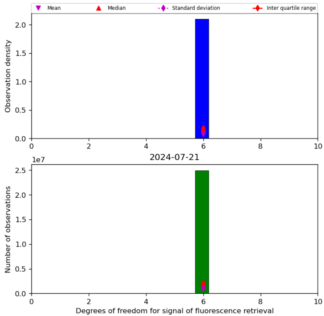
Figure 43: Histogram of “Degrees of freedom for signal of fluorescence retrieval” for 2024-07-21 to 2024-07-22
