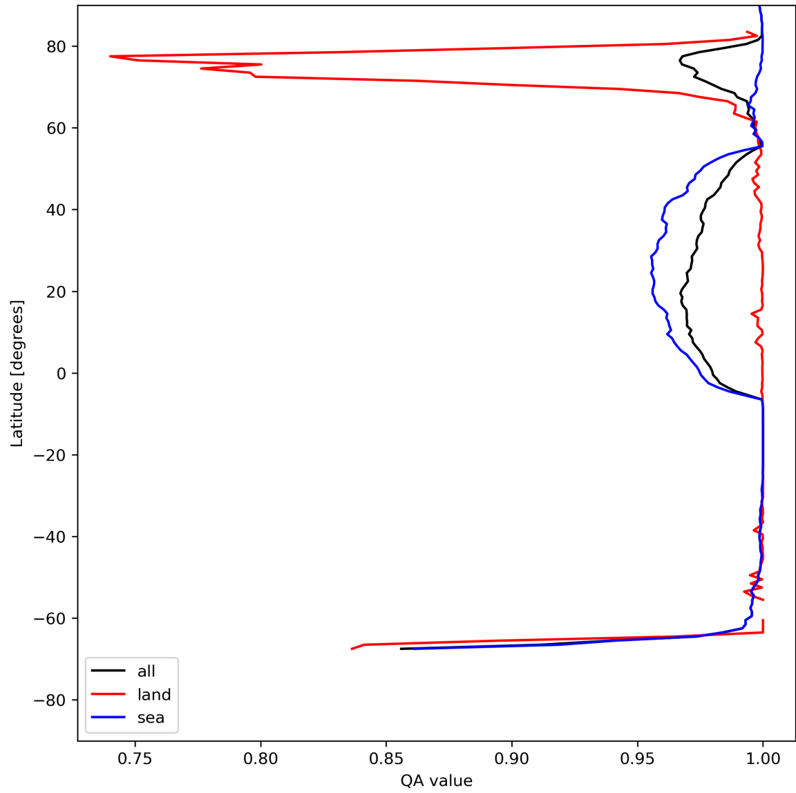
Figure 12: Zonal average of “QA value” for 2024-07-21 to 2024-07-22.
