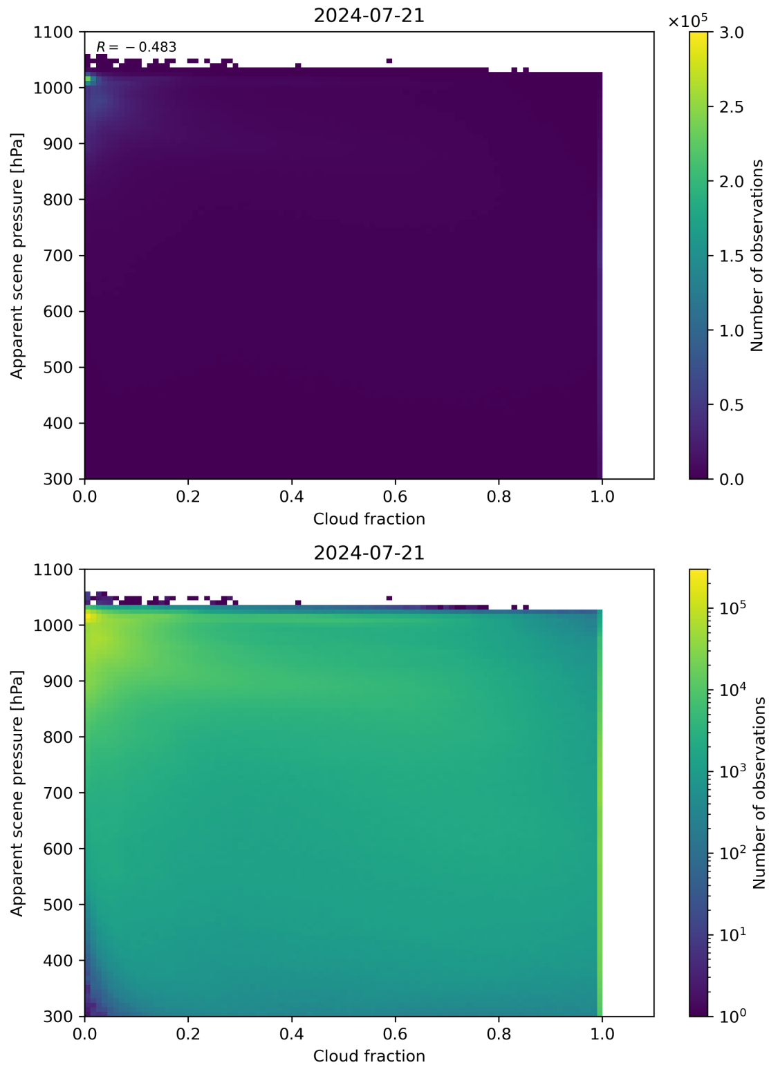
Figure 70: Scatter density plot of “Cloud fraction” against “Apparent scene pressure” for 2024-07-21 to 2024-07-22.
