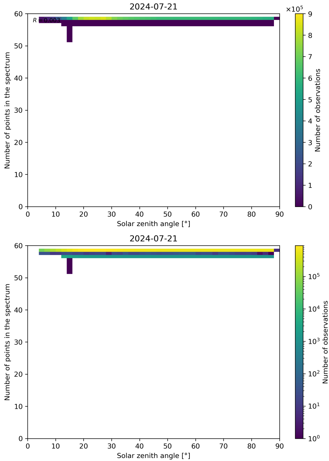
Figure 115: Scatter density plot of “Solar zenith angle” against “Number of points in the spectrum” for 2024-07-21 to 2024-07-22.
