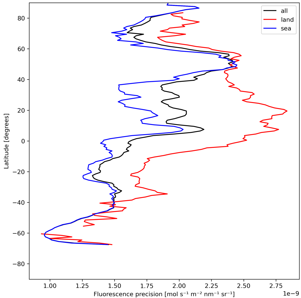
Figure 24: Zonal average of “Fluorescence precision” for 2024-07-21 to 2024-07-22.
