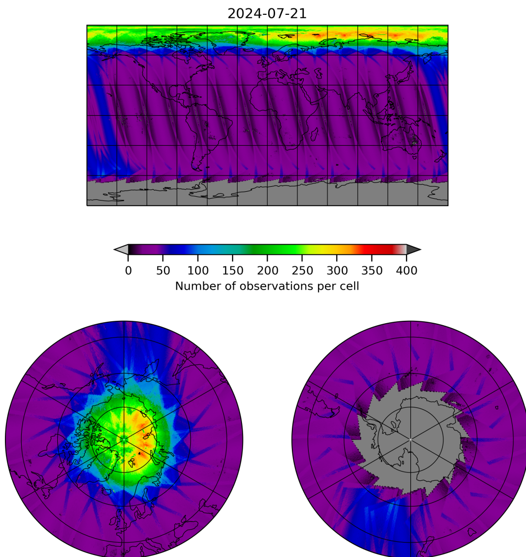
Figure 11: Map of the number of observations for 2024-07-21 to 2024-07-22
