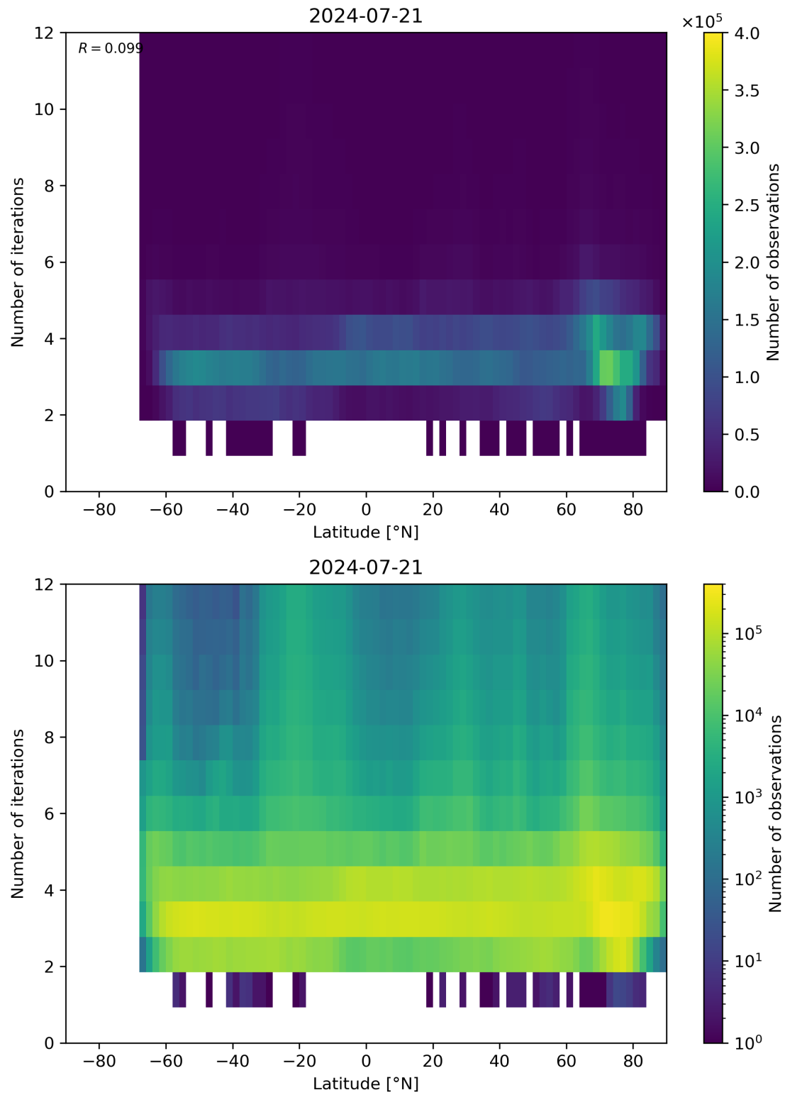
Figure 93: Scatter density plot of “Latitude” against “Number of iterations” for 2024-07-21 to 2024-07-22.
