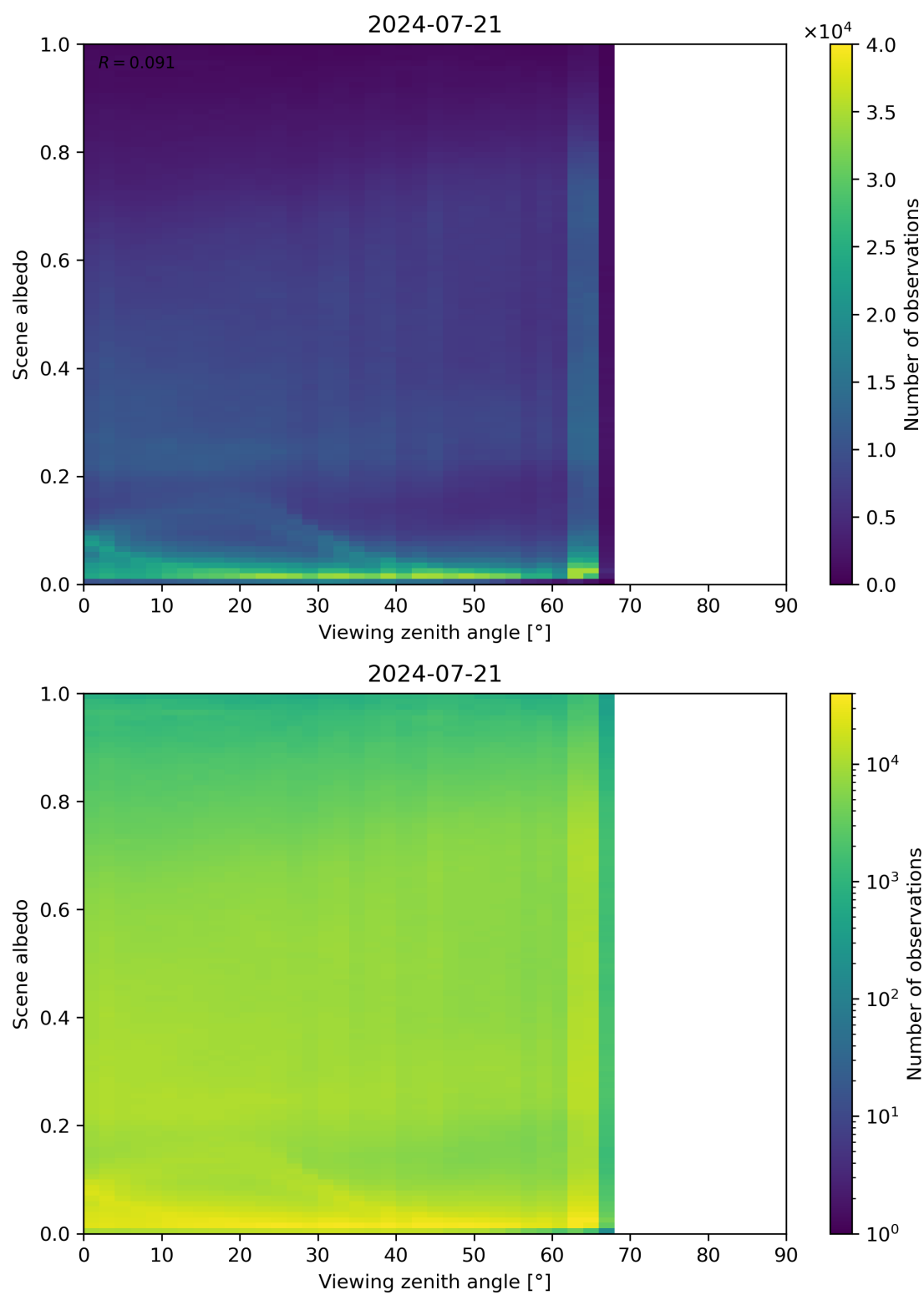
Figure 126: Scatter density plot of “Viewing zenith angle” against “Scene albedo” for 2024-07-21 to 2024-07-22.
