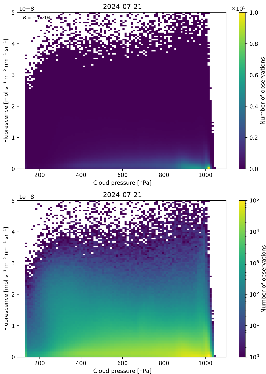
Figure 80: Scatter density plot of “Cloud pressure” against “Fluorescence” for 2024-07-21 to 2024-07-22.
