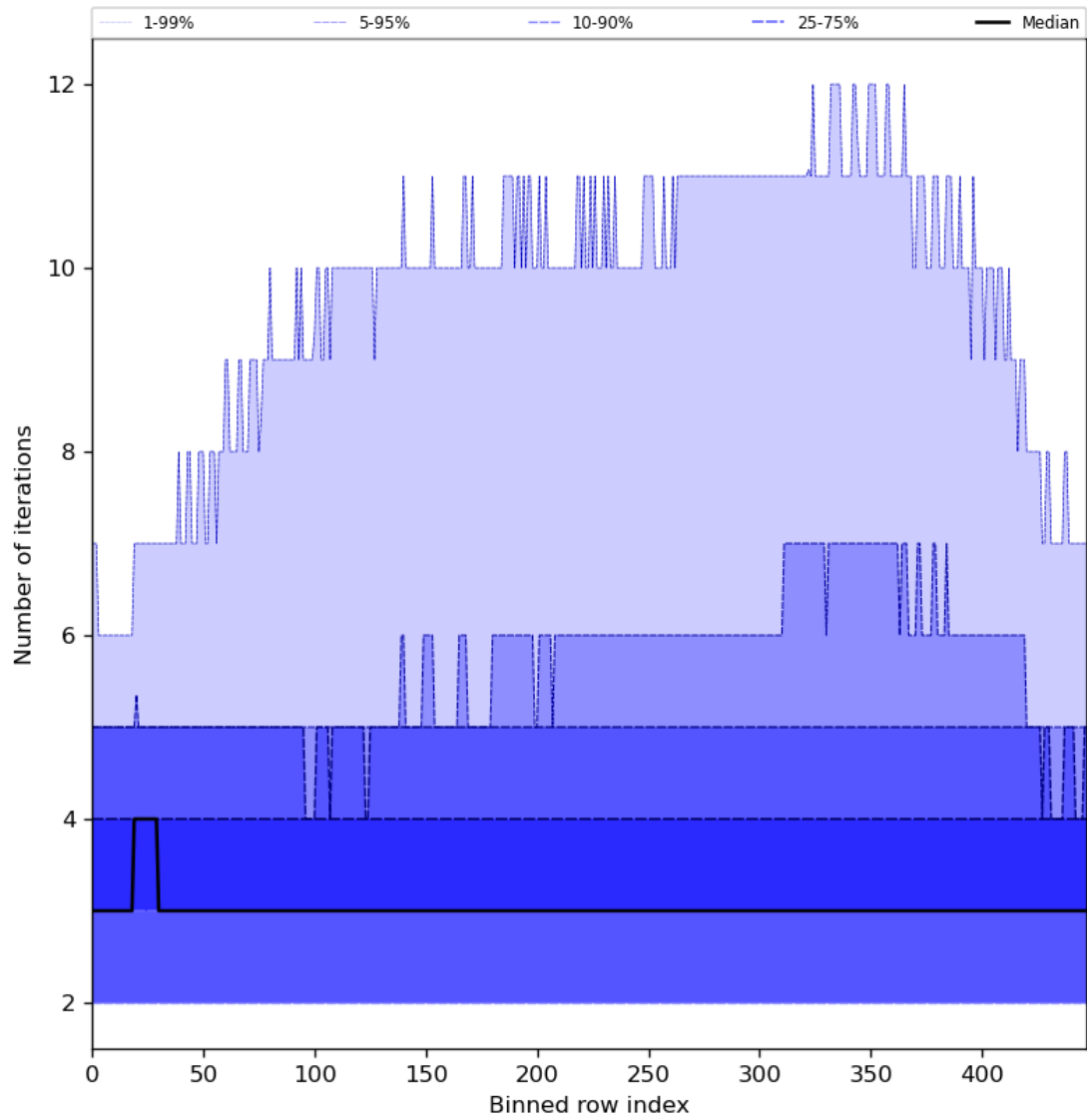
Figure 56: Along track statistics of “Number of iterations” for 2024-07-21 to 2024-07-22
