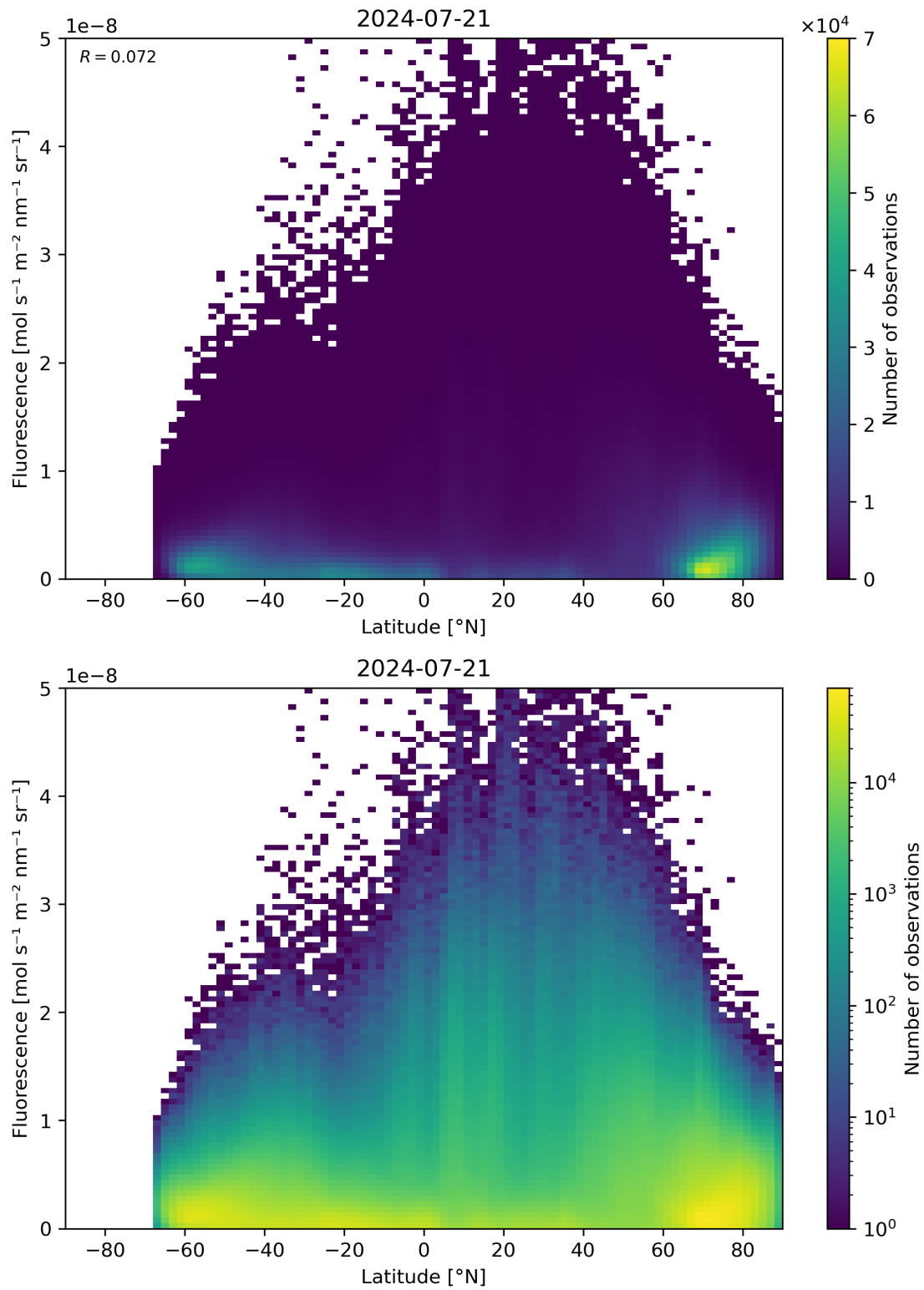
Figure 92: Scatter density plot of “Latitude” against “Fluorescence” for 2024-07-21 to 2024-07-22.
