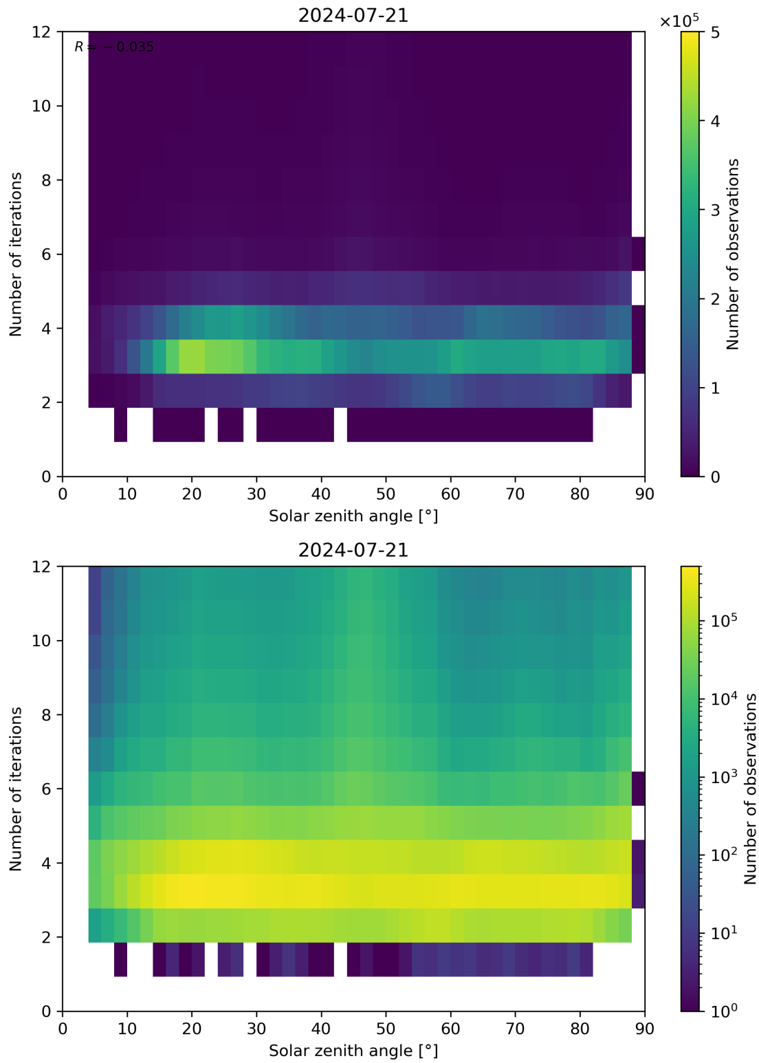
Figure 114: Scatter density plot of “Solar zenith angle” against “Number of iterations” for 2024-07-21 to 2024-07-22.
