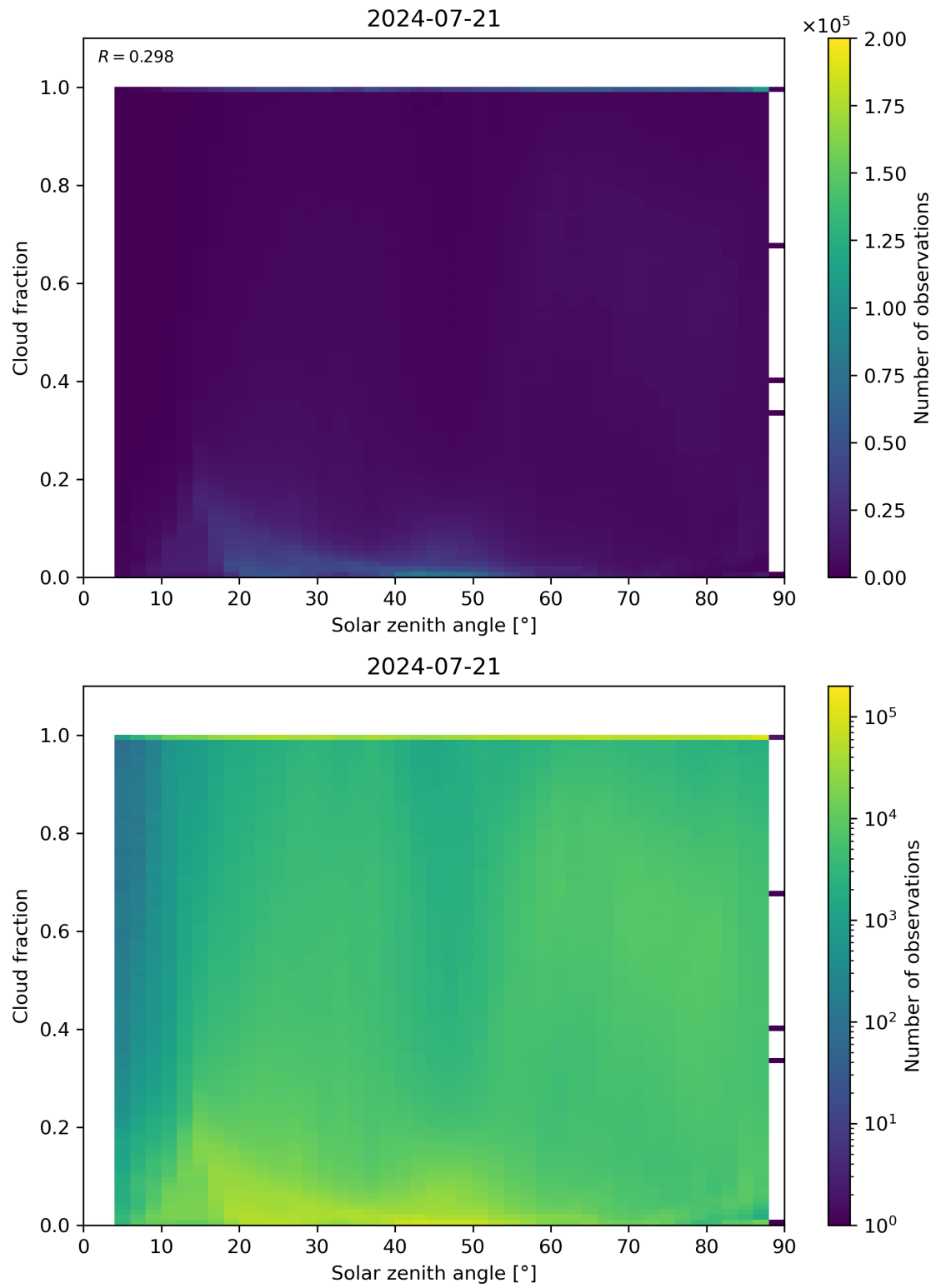
Figure 110: Scatter density plot of “Solar zenith angle” against “Cloud fraction” for 2024-07-21 to 2024-07-22.
