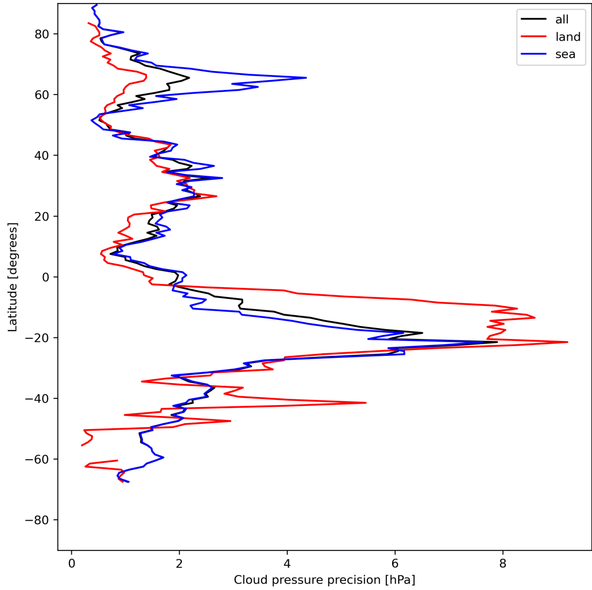
Figure 14: Zonal average of “Cloud pressure precision” for 2024-07-21 to 2024-07-22.
