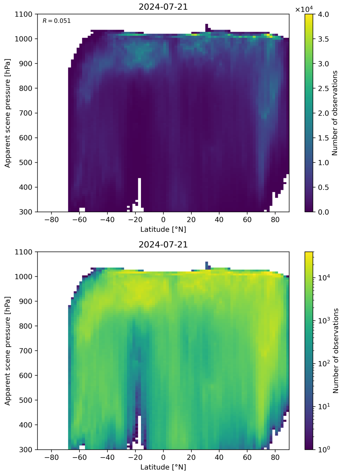
Figure 88: Scatter density plot of “Latitude” against “Apparent scene pressure” for 2024-07-21 to 2024-07-22.
