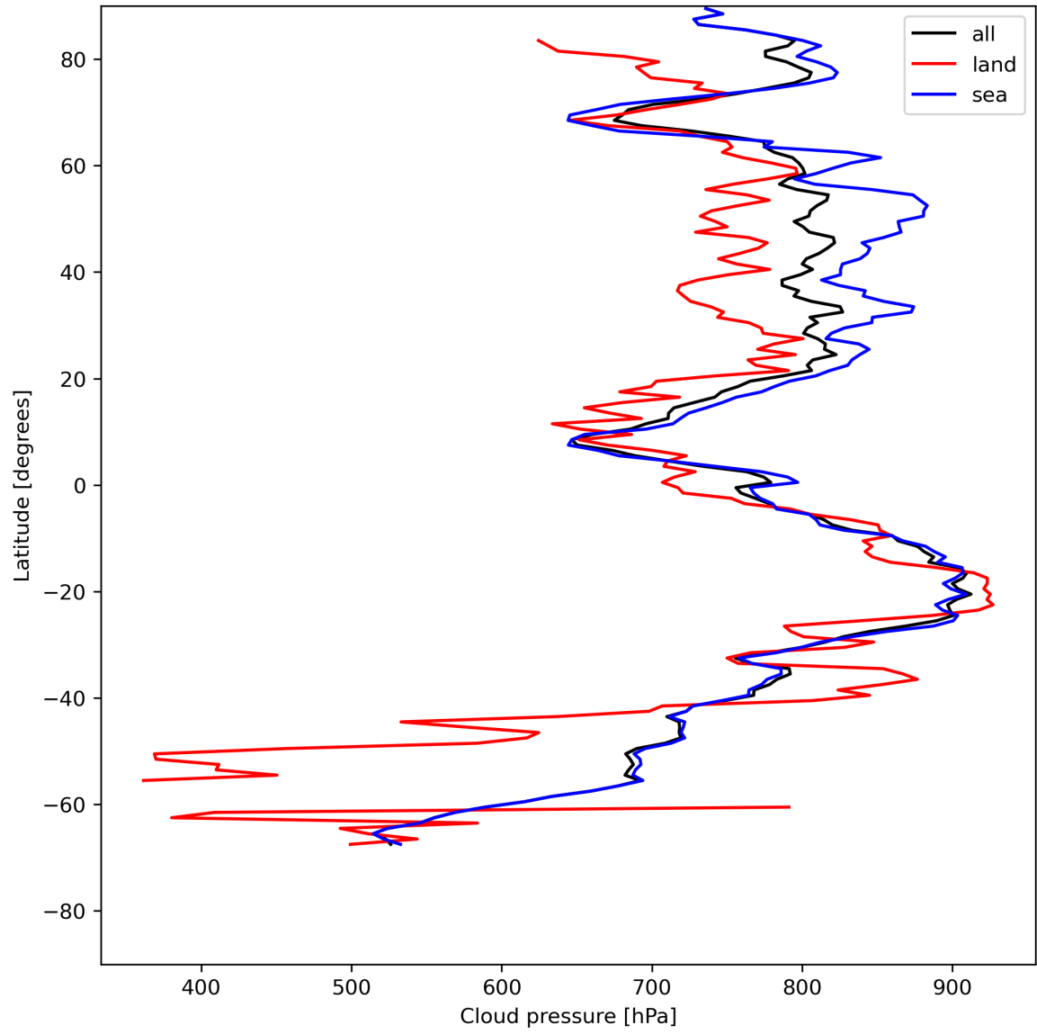
Figure 13: Zonal average of “Cloud pressure” for 2024-07-21 to 2024-07-22.
