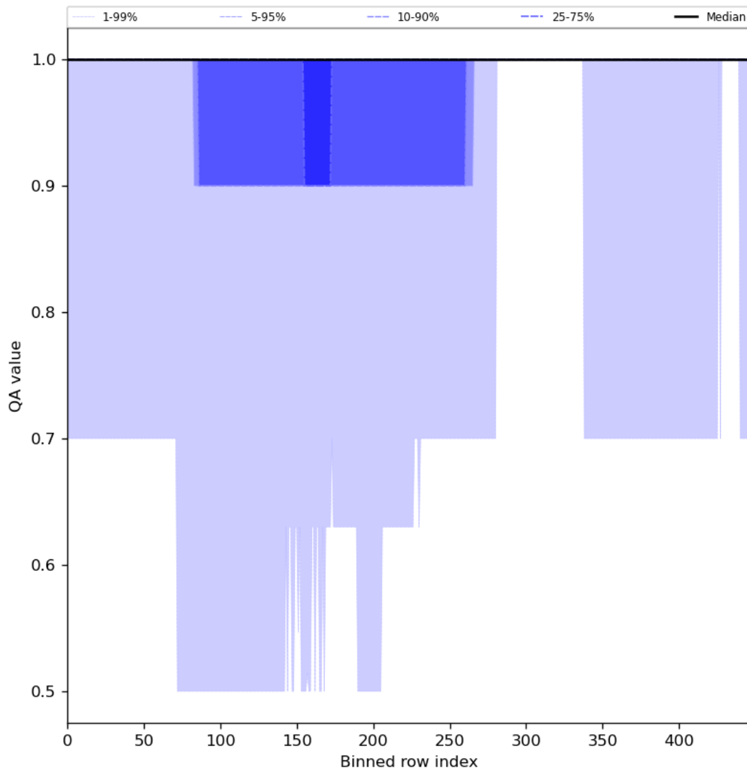
Figure 46: Along track statistics of “QA value” for 2024-07-21 to 2024-07-22
