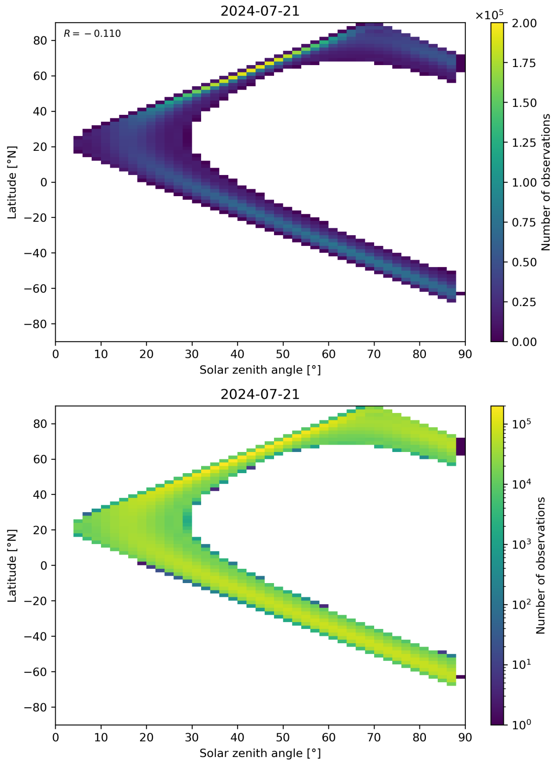
Figure 113: Scatter density plot of “Solar zenith angle” against “Latitude” for 2024-07-21 to 2024-07-22.
