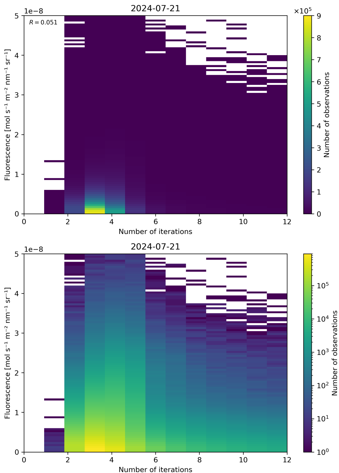
Figure 98: Scatter density plot of “Number of iterations” against “Fluorescence” for 2024-07-21 to 2024-07-22.
