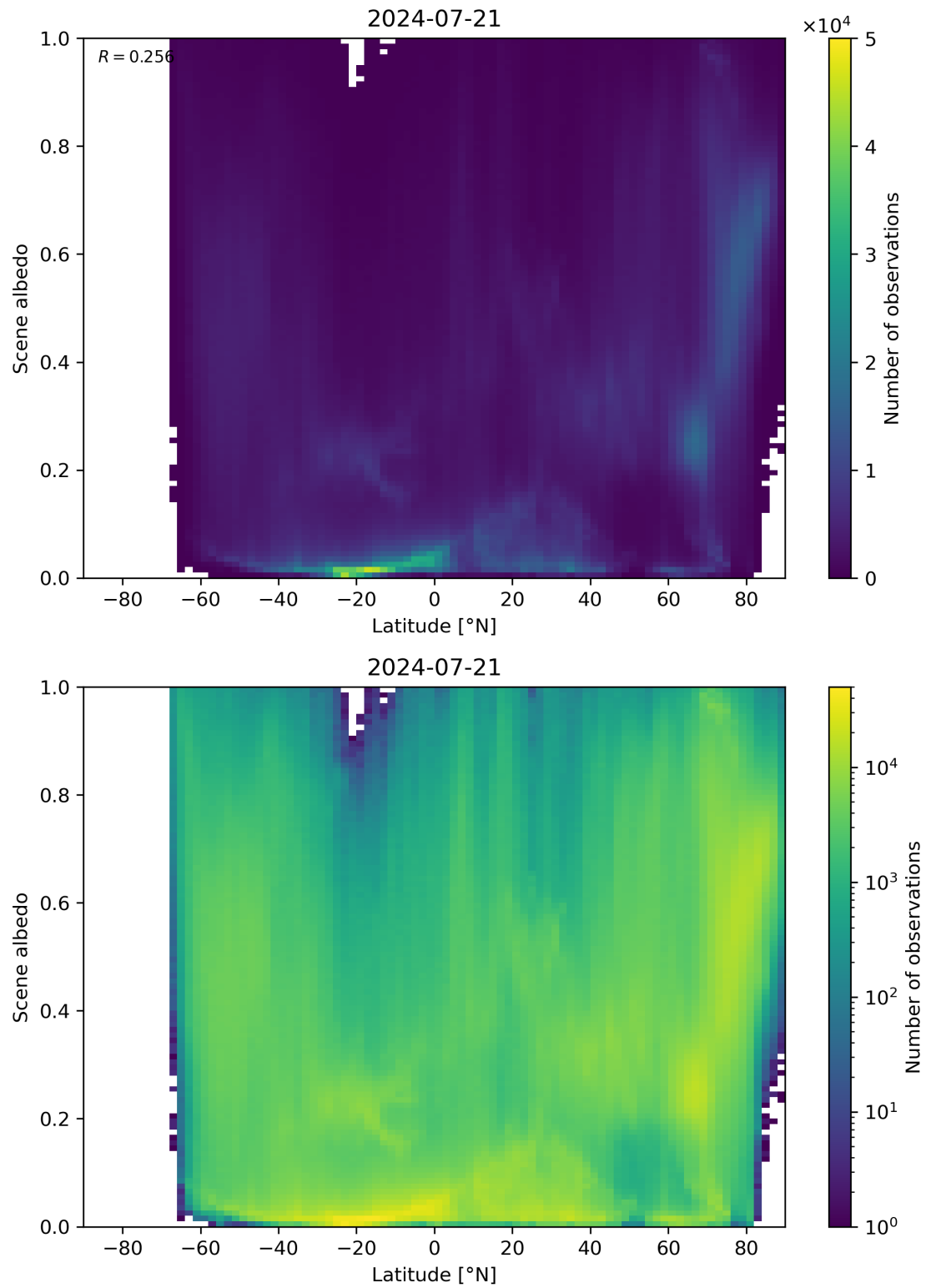
Figure 95: Scatter density plot of “Latitude” against “Scene albedo” for 2024-07-21 to 2024-07-22.
