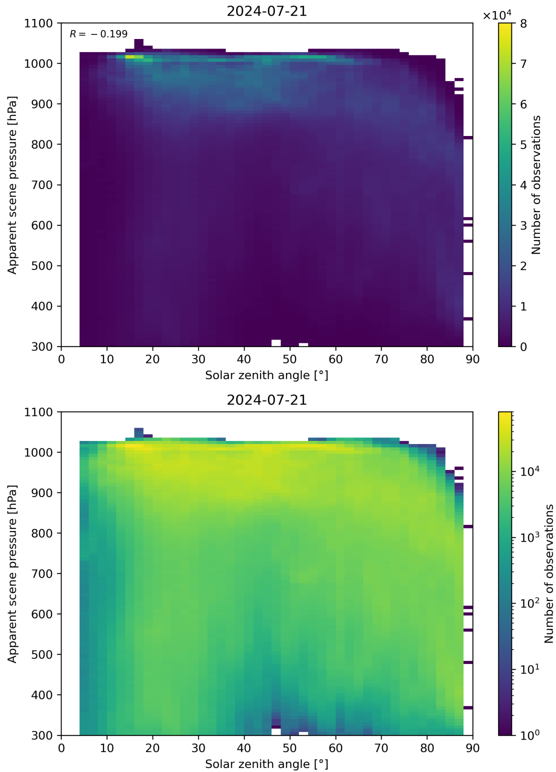
Figure 108: Scatter density plot of “Solar zenith angle” against “Apparent scene pressure” for 2024-07-21 to 2024-07-22.
