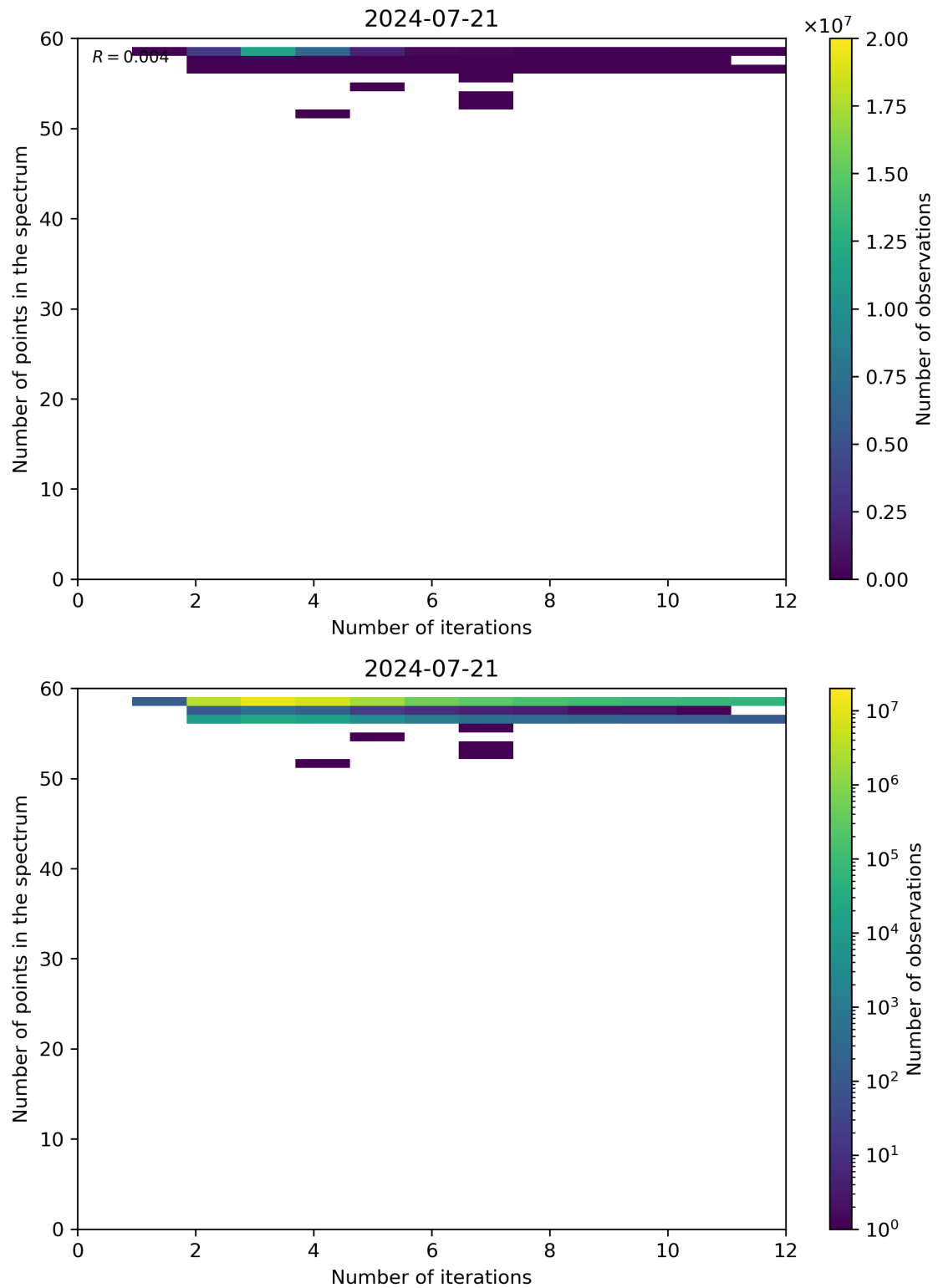
Figure 99: Scatter density plot of “Number of iterations” against “Number of points in the spectrum” for 2024-07-21 to 2024-07-22.
