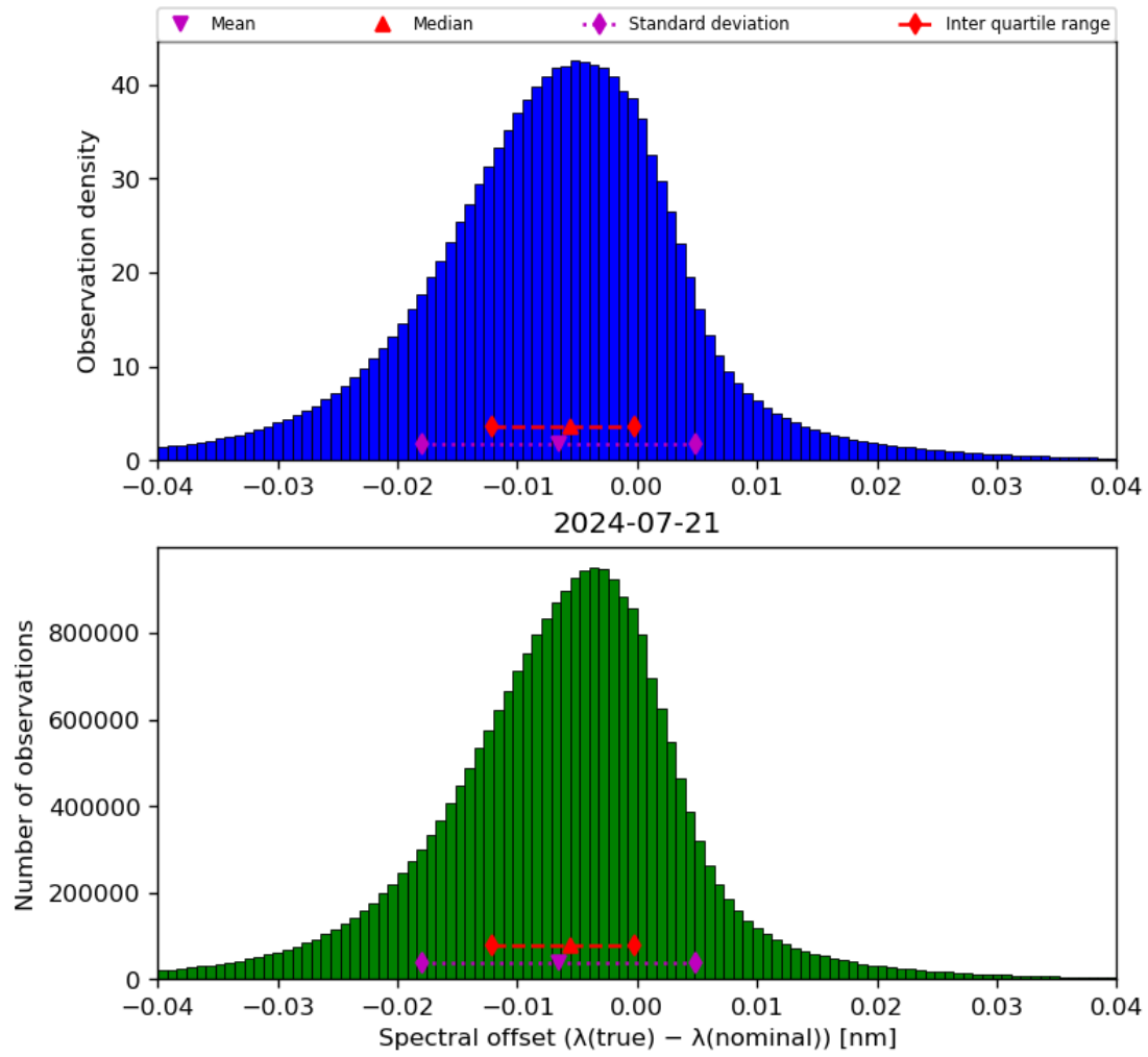
Figure 45: Histogram of “Spectral offset ( \lambda(\text{true}) - \lambda(\text{nominal}) )” for 2024-07-21 to 2024-07-22
