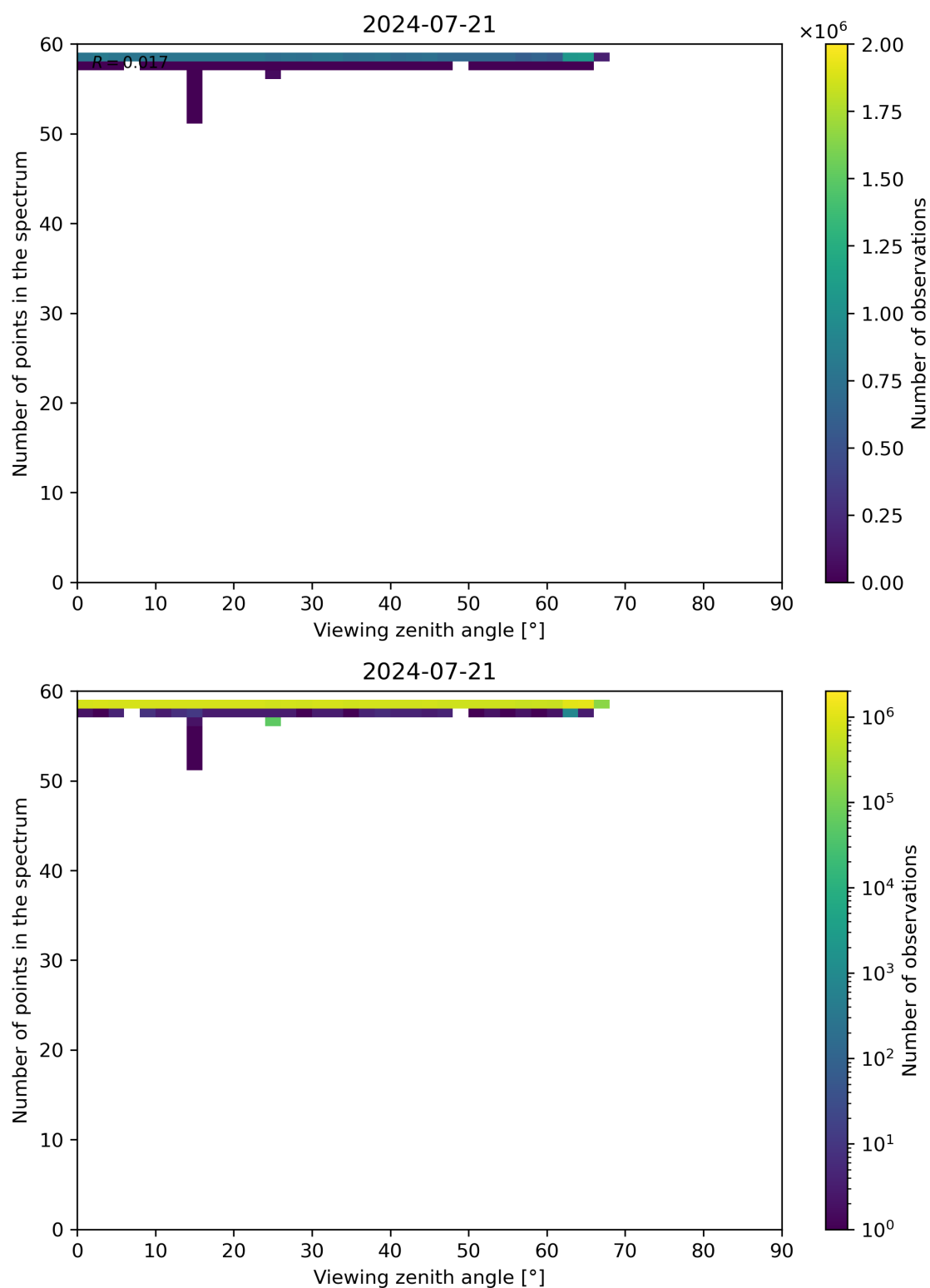
Figure 125: Scatter density plot of “Viewing zenith angle” against “Number of points in the spectrum” for 2024-07-21 to 2024-07-22.
