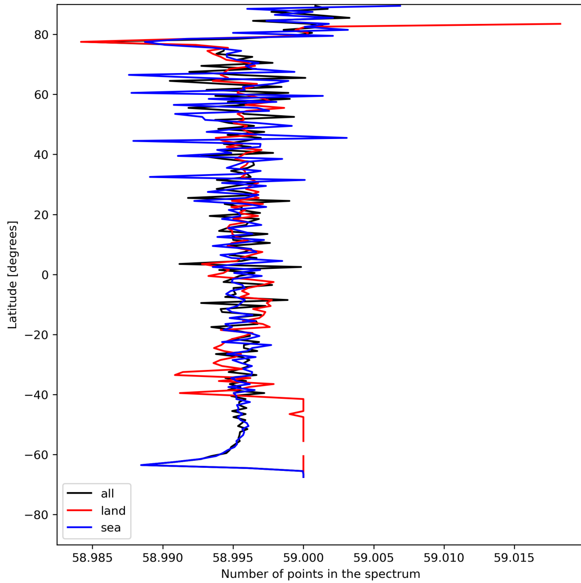
Figure 27: Zonal average of “Number of points in the spectrum” for 2024-07-21 to 2024-07-22.
