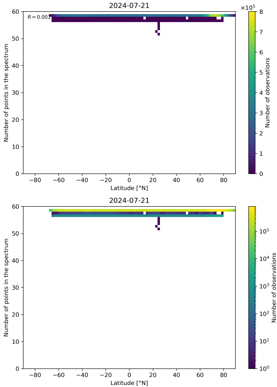
Figure 94: Scatter density plot of “Latitude” against “Number of points in the spectrum” for 2024-07-21 to 2024-07-22.
