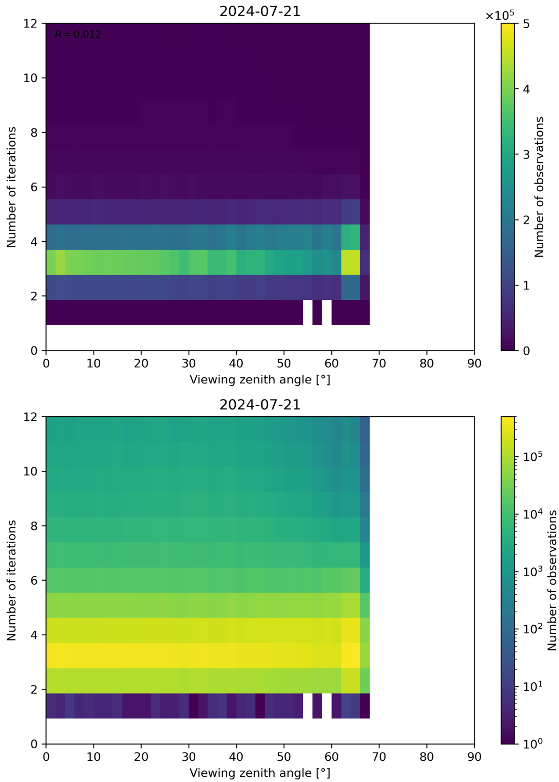
Figure 124: Scatter density plot of “Viewing zenith angle” against “Number of iterations” for 2024-07-21 to 2024-07-22.
