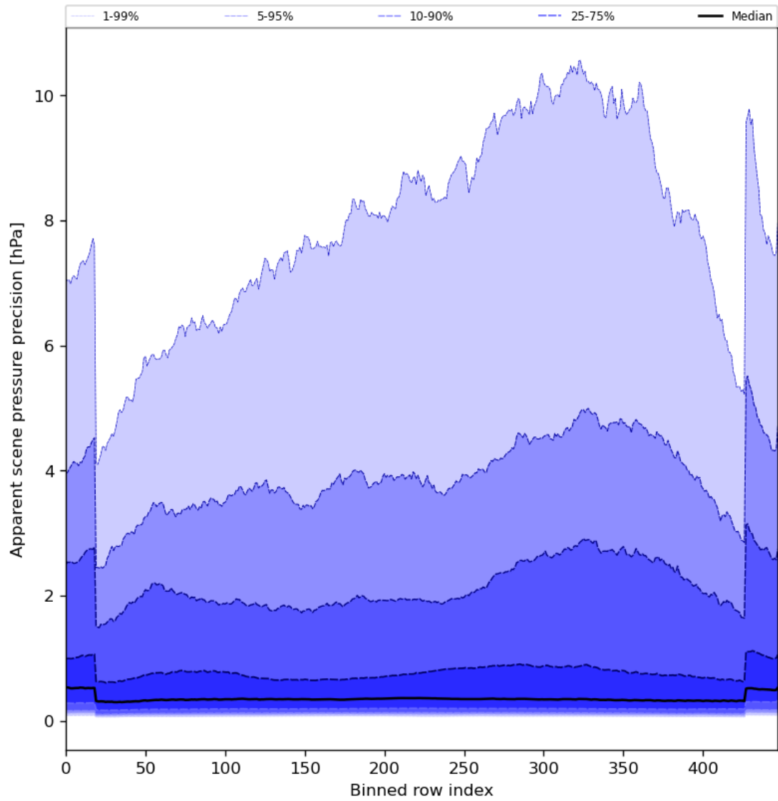
Figure 54: Along track statistics of “Apparent scene pressure precision” for 2024-07-21 to 2024-07-22
