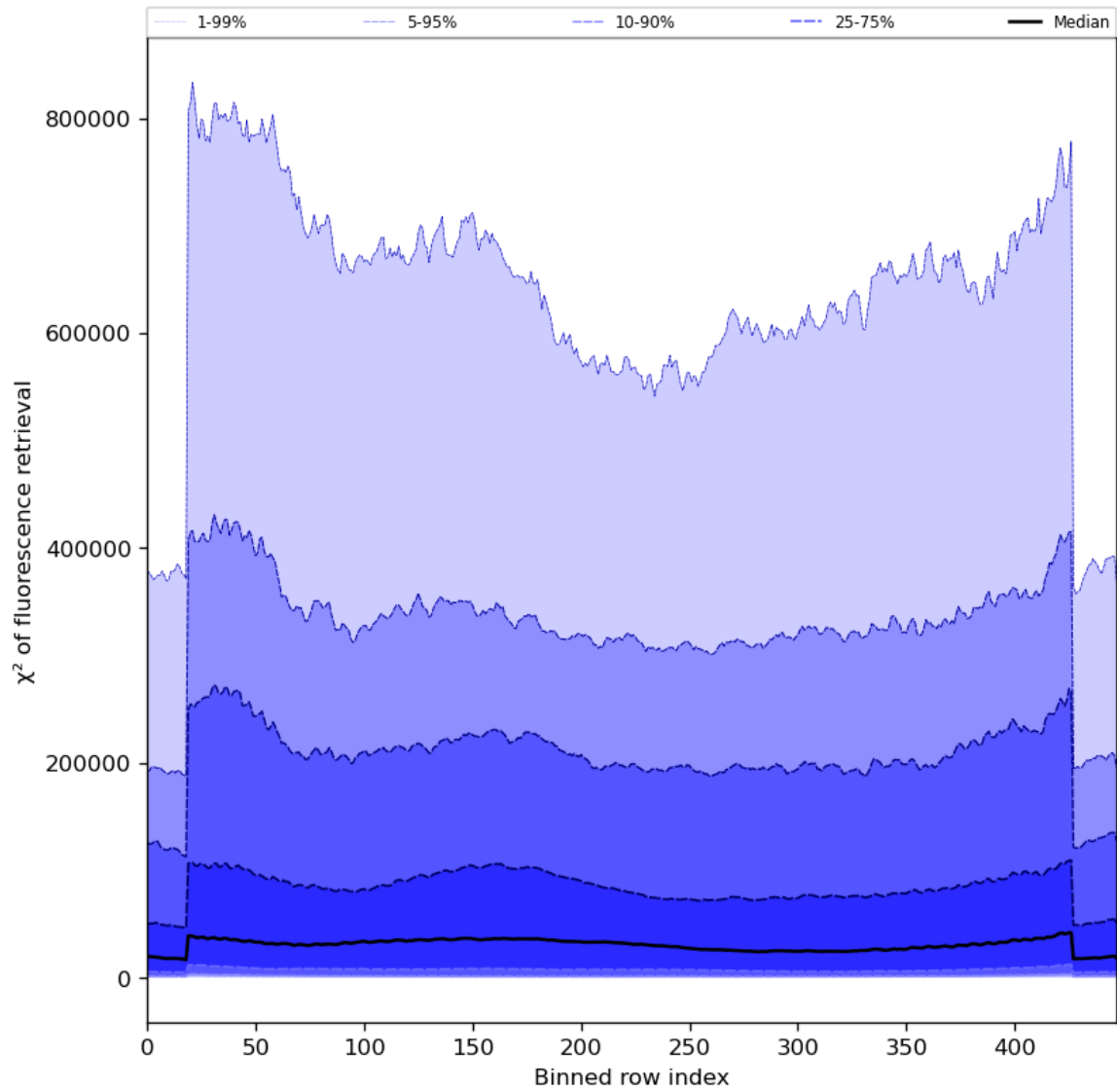
Figure 59: Along track statistics of “ \chi^2 of fluorescence retrieval” for 2024-07-21 to 2024-07-22
