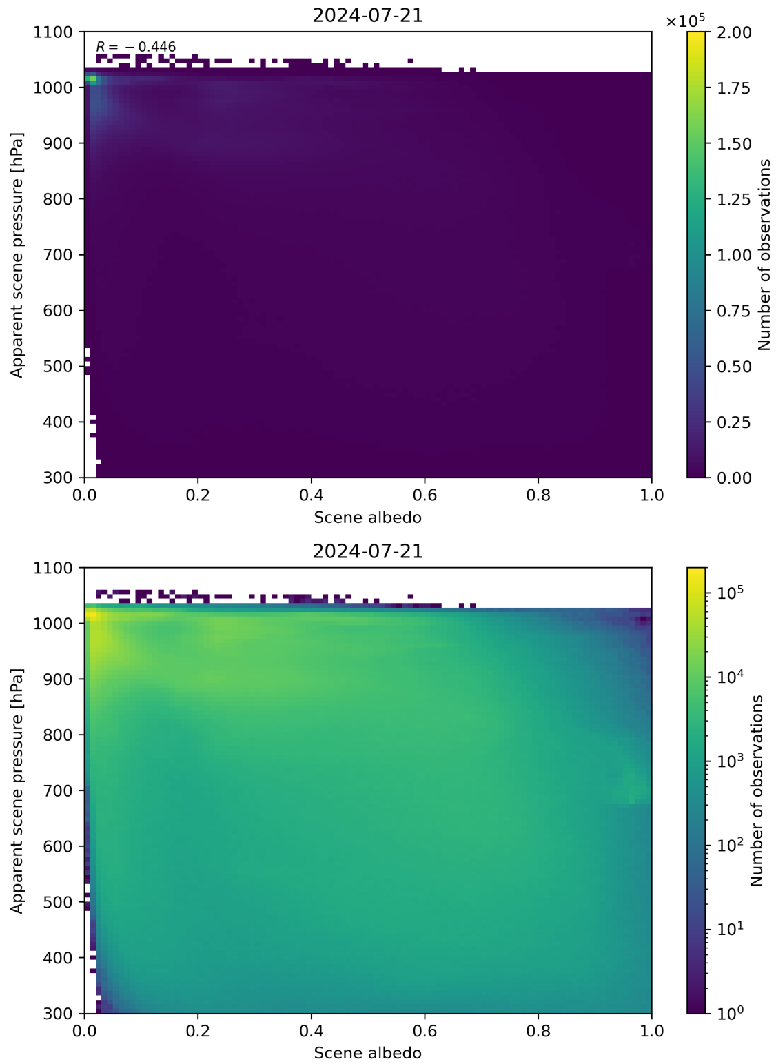
Figure 102: Scatter density plot of “Scene albedo” against “Apparent scene pressure” for 2024-07-21 to 2024-07-22.
