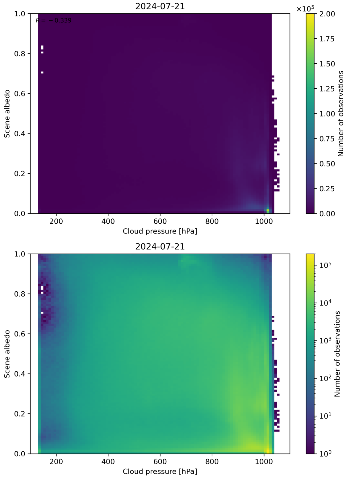
Figure 83: Scatter density plot of “Cloud pressure” against “Scene albedo” for 2024-07-21 to 2024-07-22.
