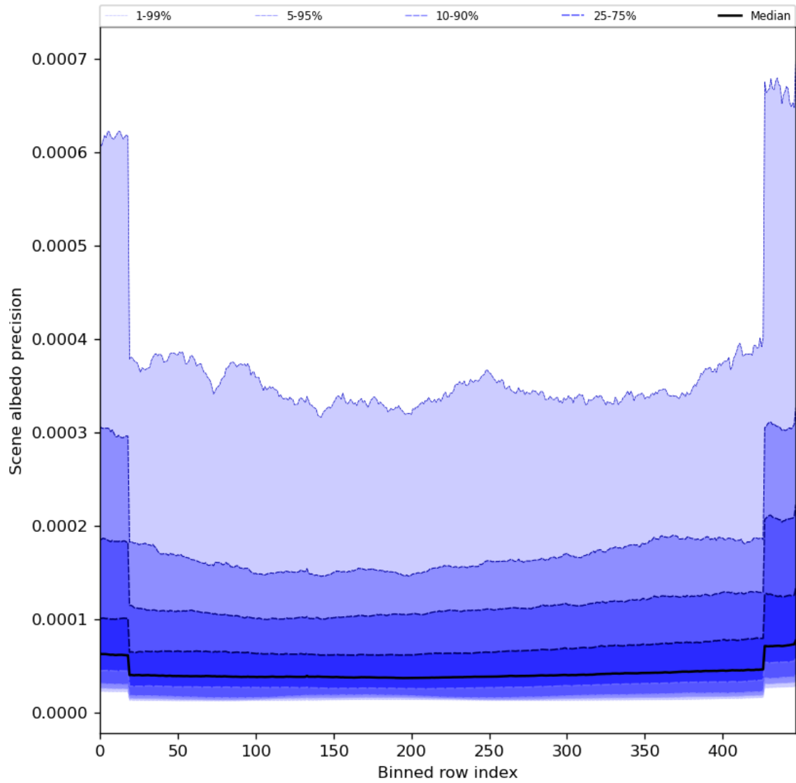
Figure 52: Along track statistics of “Scene albedo precision” for 2024-07-21 to 2024-07-22
