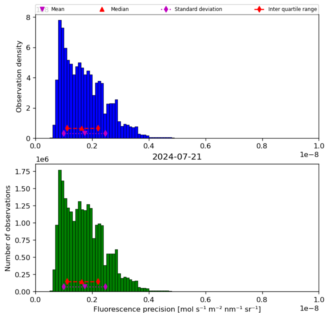
Figure 41: Histogram of “Fluorescence precision” for 2024-07-21 to 2024-07-22
