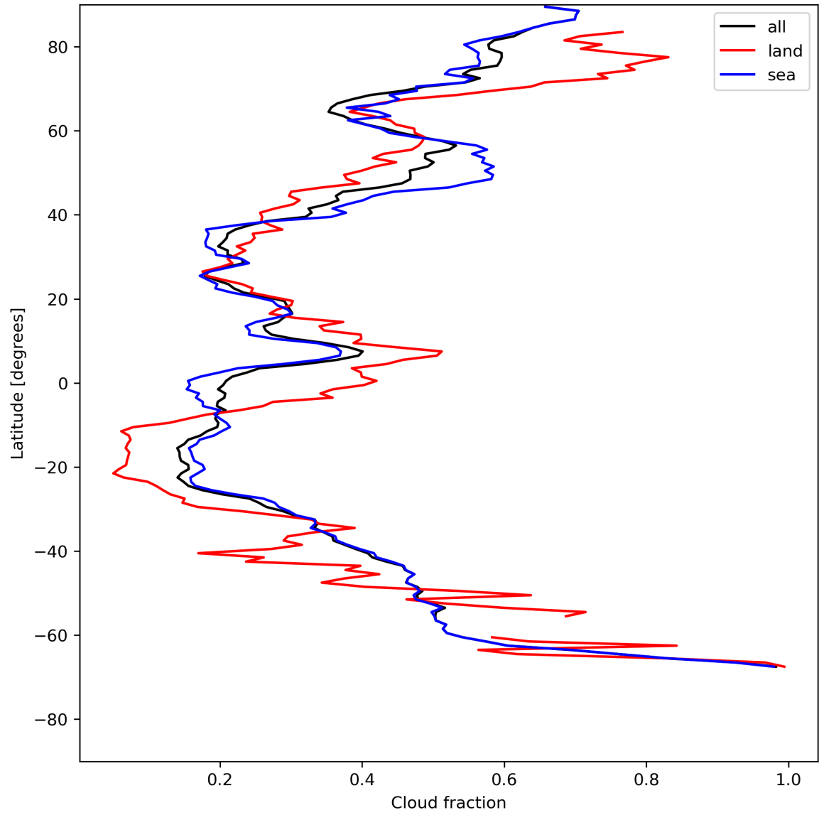
Figure 15: Zonal average of “Cloud fraction” for 2024-07-21 to 2024-07-22.
