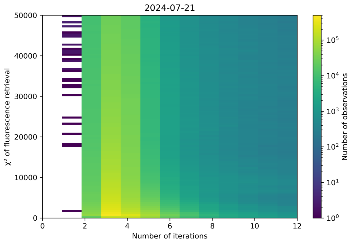
Figure 97: Scatter density plot of “Number of iterations” against “ \chi^2 of fluorescence retrieval” for 2024-07-21 to 2024-07-22.
