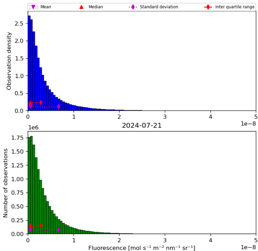
Figure 40: Histogram of “Fluorescence” for 2024-07-21 to 2024-07-22
