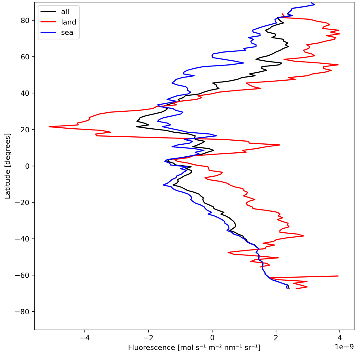
Figure 23: Zonal average of “Fluorescence” for 2024-07-21 to 2024-07-22.
