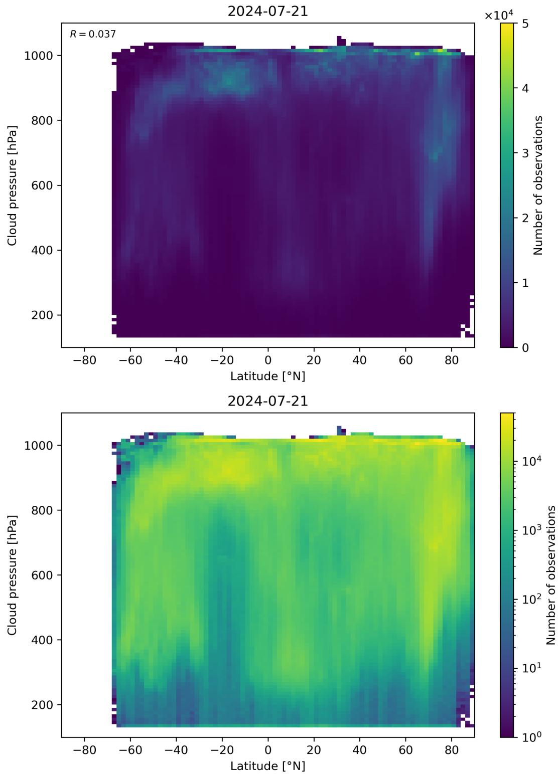
Figure 91: Scatter density plot of “Latitude” against “Cloud pressure” for 2024-07-21 to 2024-07-22.
