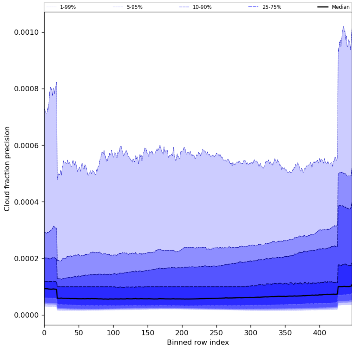
Figure 50: Along track statistics of “Cloud fraction precision” for 2024-07-21 to 2024-07-22
