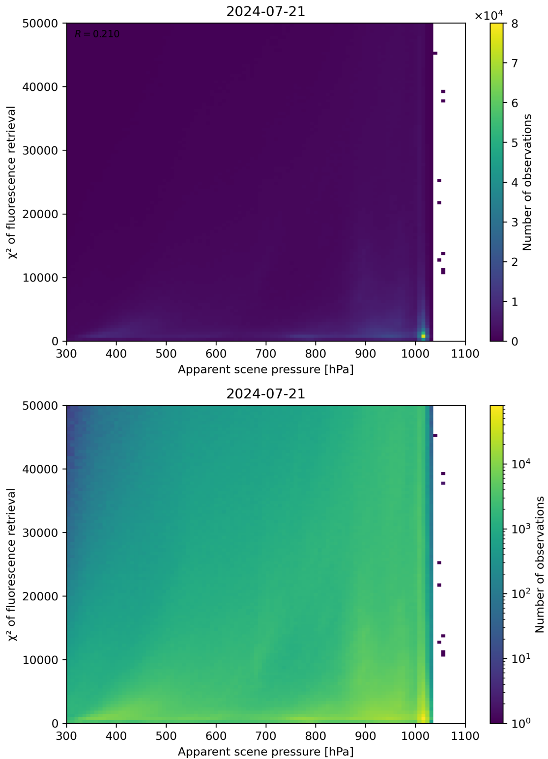
Figure 63: Scatter density plot of “Apparent scene pressure” against “ \chi^2 of fluorescence retrieval” for 2024-07-21 to 2024-07-22.
