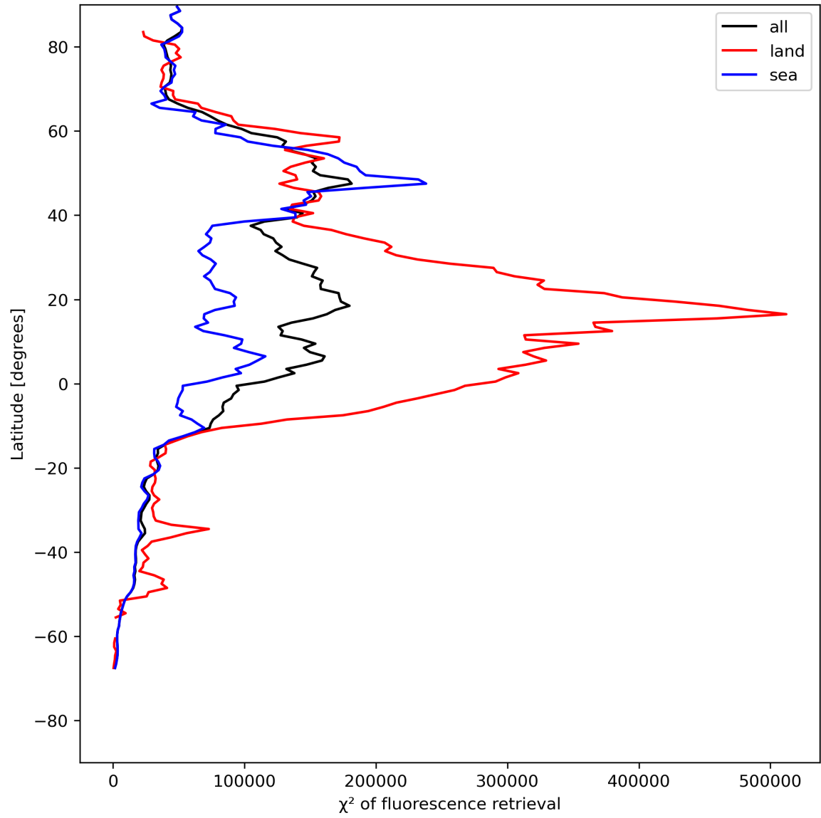
Figure 25: Zonal average of “ \chi^2 of fluorescence retrieval” for 2024-07-21 to 2024-07-22.
