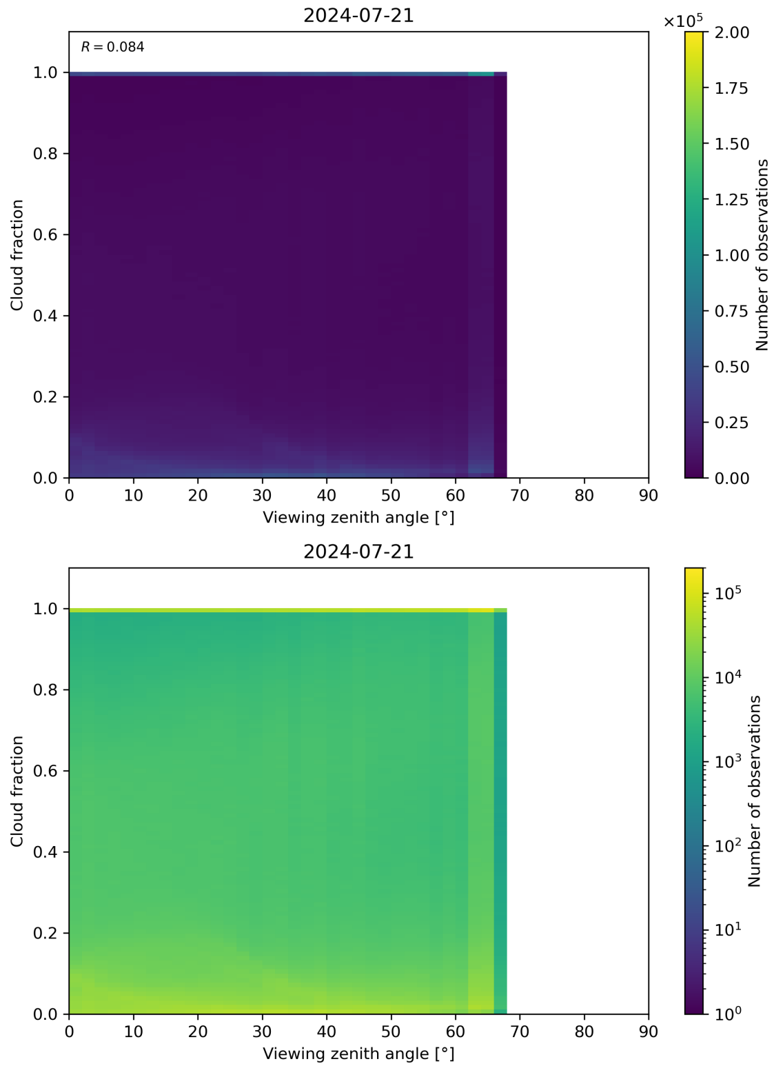
Figure 120: Scatter density plot of “Viewing zenith angle” against “Cloud fraction” for 2024-07-21 to 2024-07-22.
