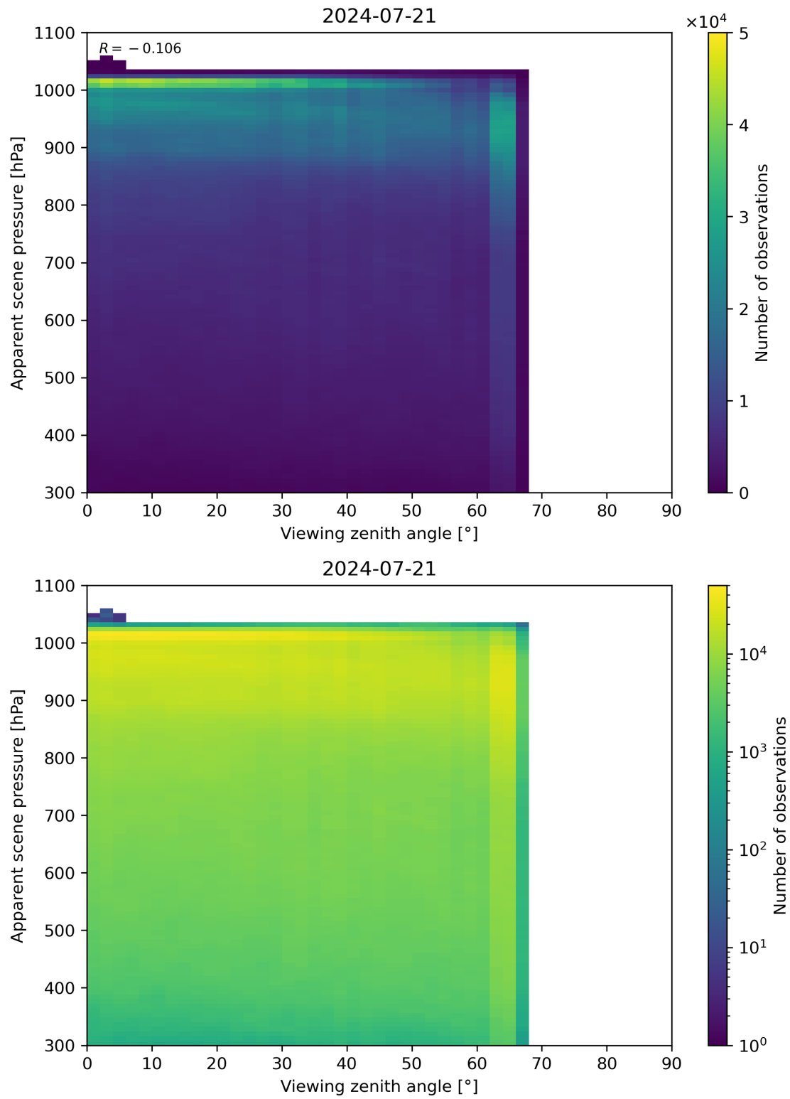
Figure 118: Scatter density plot of “Viewing zenith angle” against “Apparent scene pressure” for 2024-07-21 to 2024-07-22.
