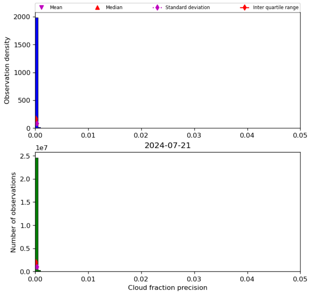
Figure 33: Histogram of “Cloud fraction precision” for 2024-07-21 to 2024-07-22
