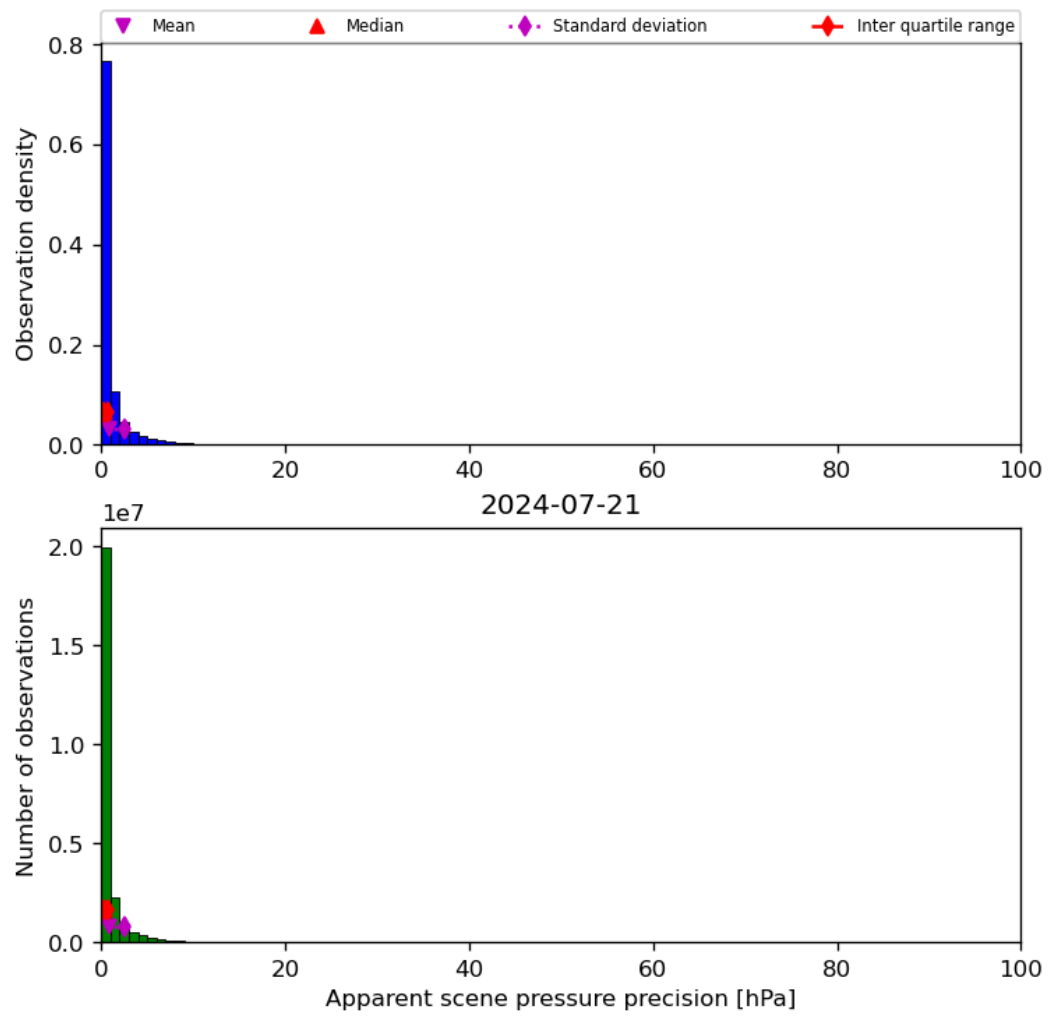
Figure 37: Histogram of “Apparent scene pressure precision” for 2024-07-21 to 2024-07-22
