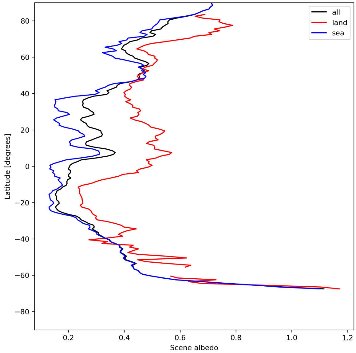
Figure 17: Zonal average of “Scene albedo” for 2024-07-21 to 2024-07-22.
