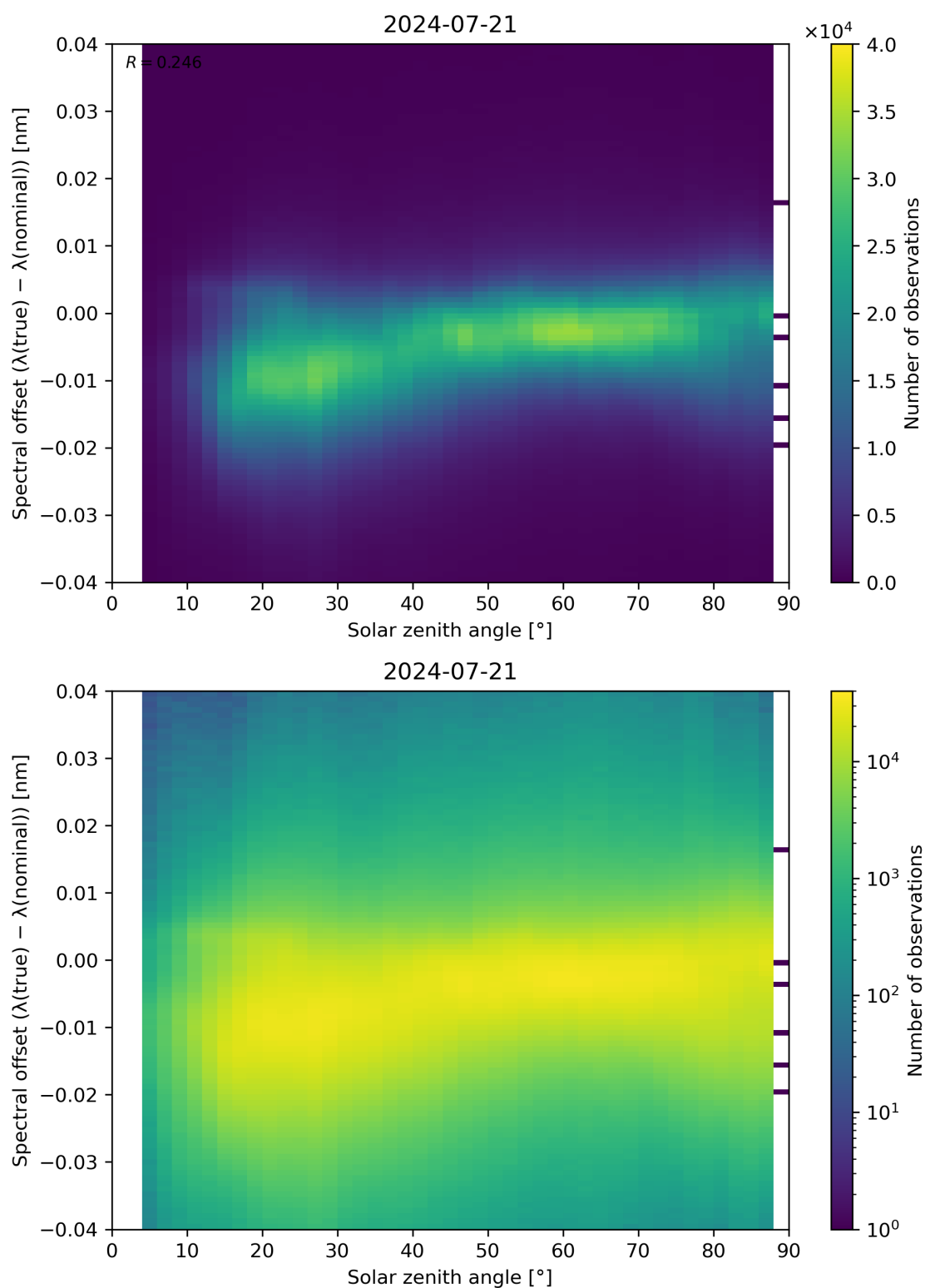
Figure 117: Scatter density plot of “Solar zenith angle” against “Spectral offset ( \lambda(\text{true}) - \lambda(\text{nominal}) )” for 2024-07-21 to 2024-07-22.
