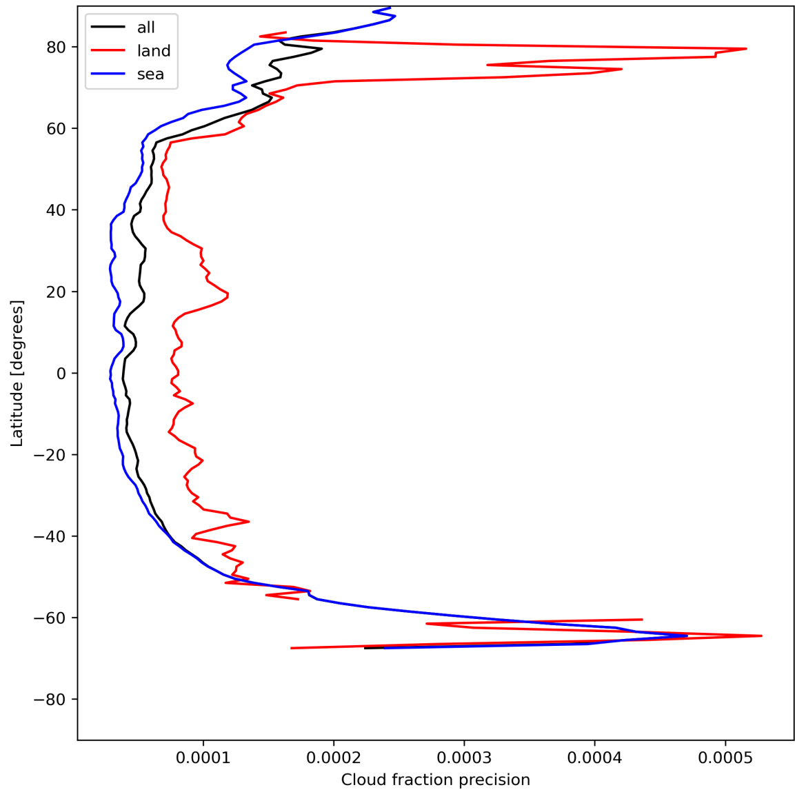
Figure 16: Zonal average of “Cloud fraction precision” for 2024-07-21 to 2024-07-22.
