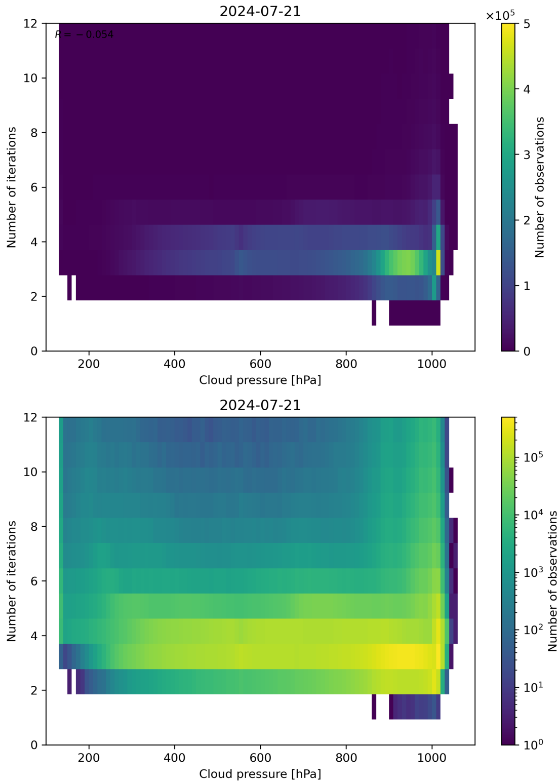
Figure 81: Scatter density plot of “Cloud pressure” against “Number of iterations” for 2024-07-21 to 2024-07-22.
