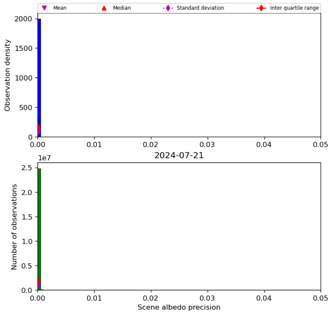
Figure 35: Histogram of “Scene albedo precision” for 2024-07-21 to 2024-07-22
