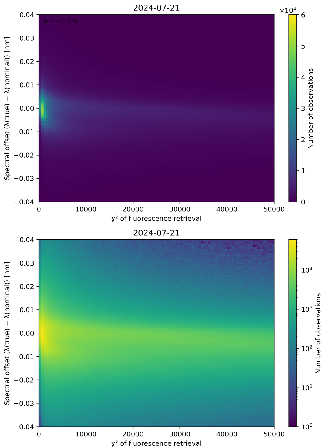
Figure 69: Scatter density plot of " \chi^2 of fluorescence retrieval" against "Spectral offset ( \lambda(\text{true}) - \lambda(\text{nominal}) )" for 2024-07-21 to 2024-07-22.
