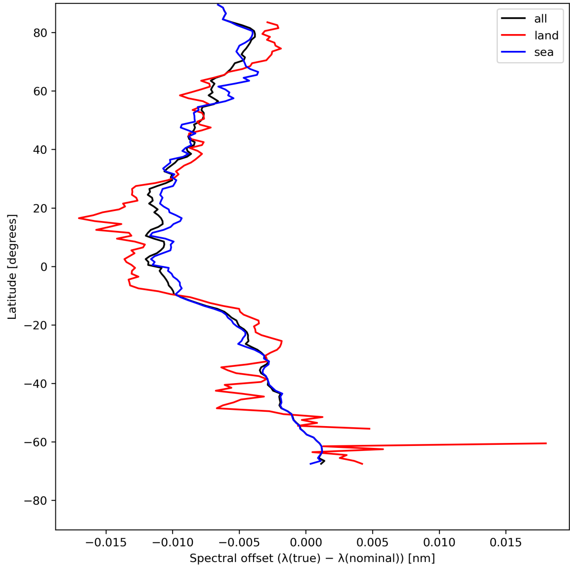
Figure 28: Zonal average of “Spectral offset ( \lambda(\text{true}) - \lambda(\text{nominal}) )” for 2024-07-21 to 2024-07-22.
