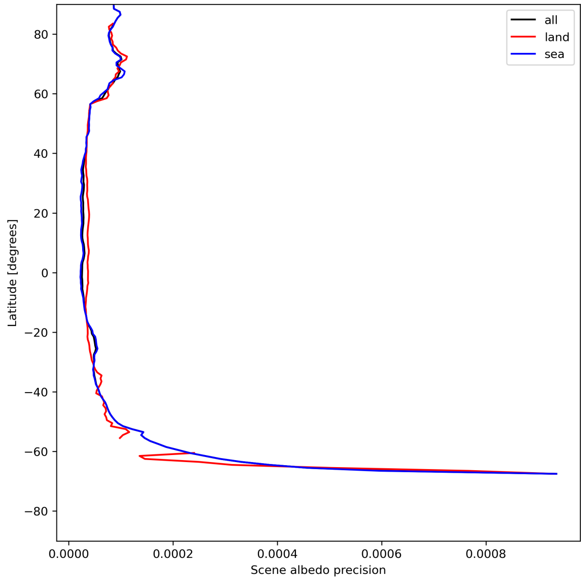
Figure 18: Zonal average of “Scene albedo precision” for 2024-07-21 to 2024-07-22.
