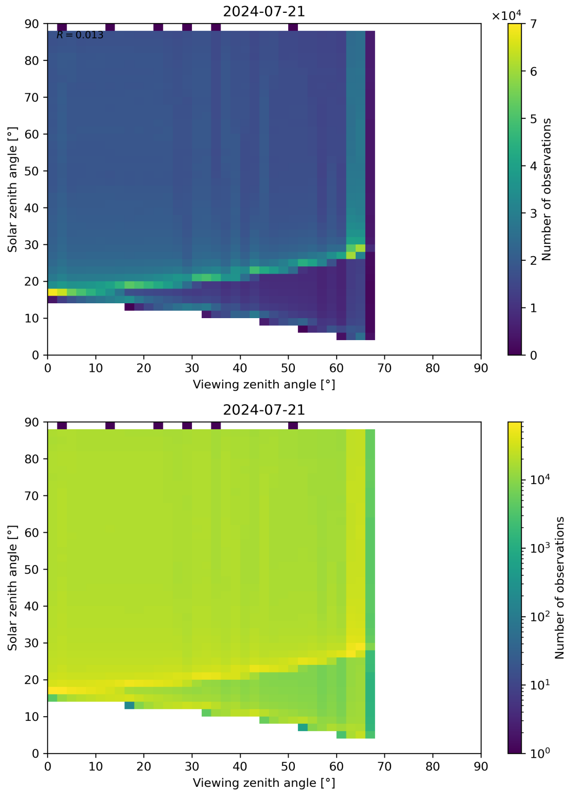
Figure 127: Scatter density plot of “Viewing zenith angle” against “Solar zenith angle” for 2024-07-21 to 2024-07-22.
