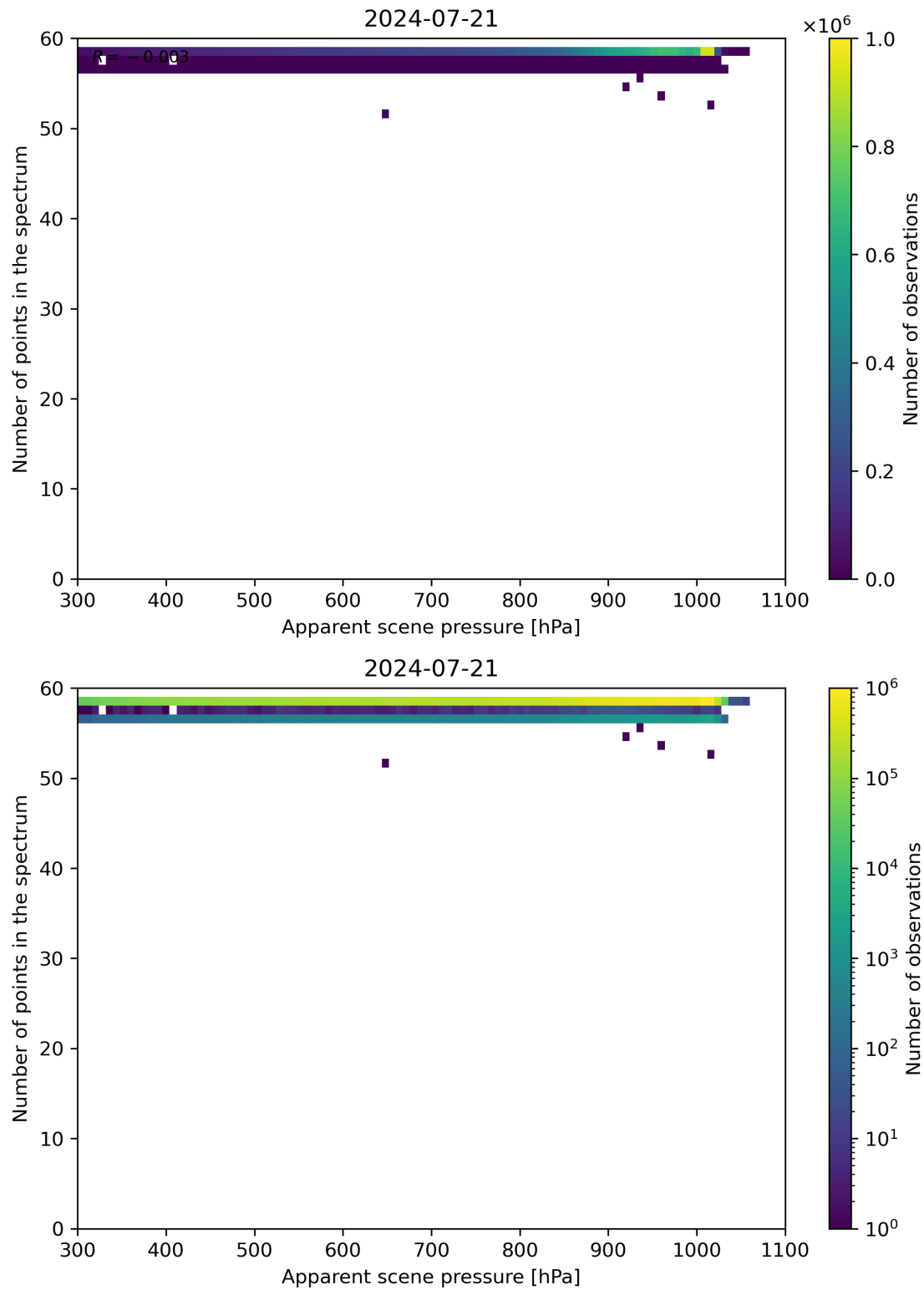
Figure 66: Scatter density plot of “Apparent scene pressure” against “Number of points in the spectrum” for 2024-07-21 to 2024-07-22.
