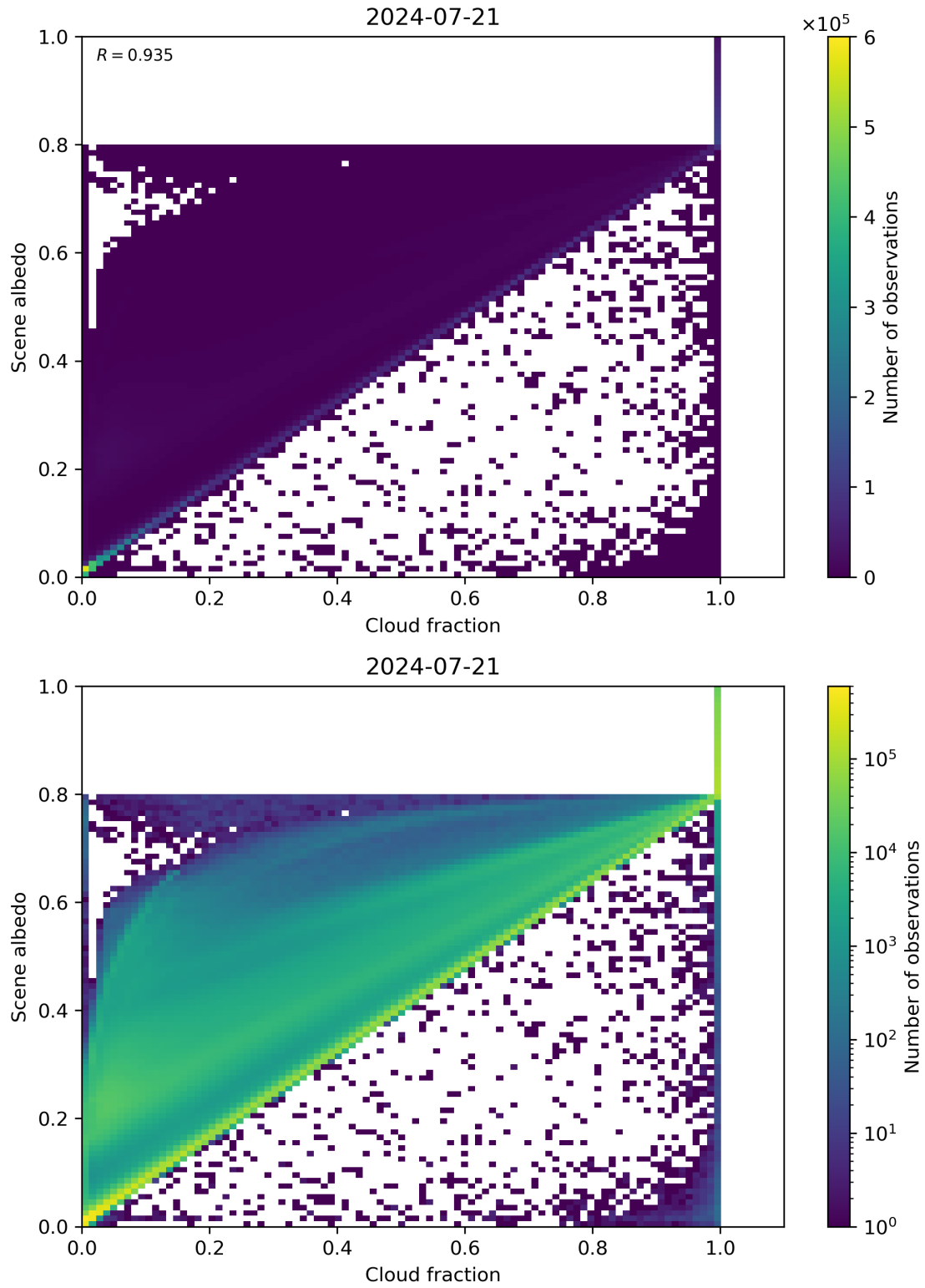
Figure 75: Scatter density plot of “Cloud fraction” against “Scene albedo” for 2024-07-21 to 2024-07-22.
