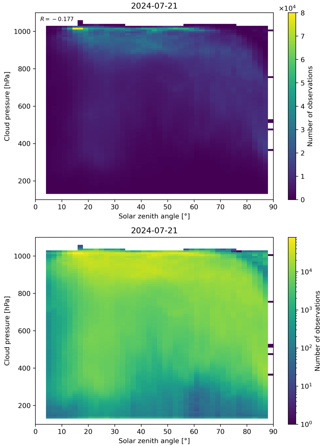
Figure 111: Scatter density plot of “Solar zenith angle” against “Cloud pressure” for 2024-07-21 to 2024-07-22.
