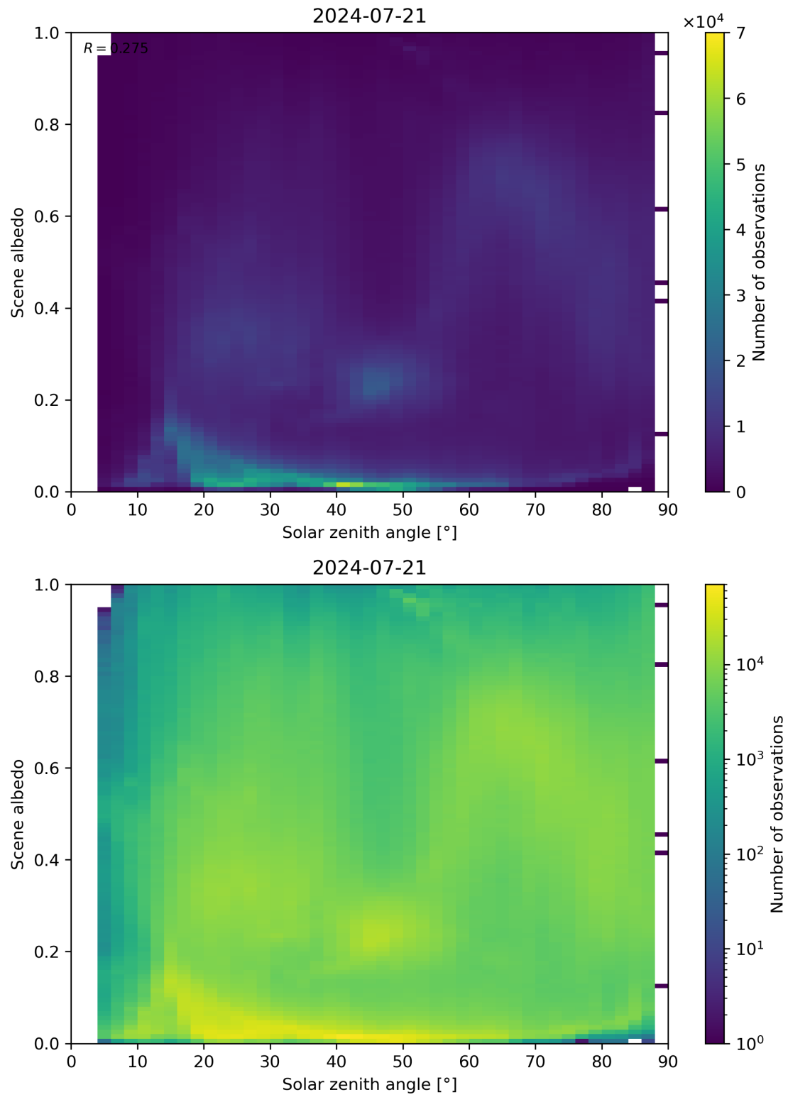
Figure 116: Scatter density plot of “Solar zenith angle” against “Scene albedo” for 2024-07-21 to 2024-07-22.
