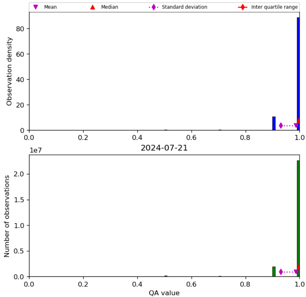
Figure 29: Histogram of “QA value” for 2024-07-21 to 2024-07-22
