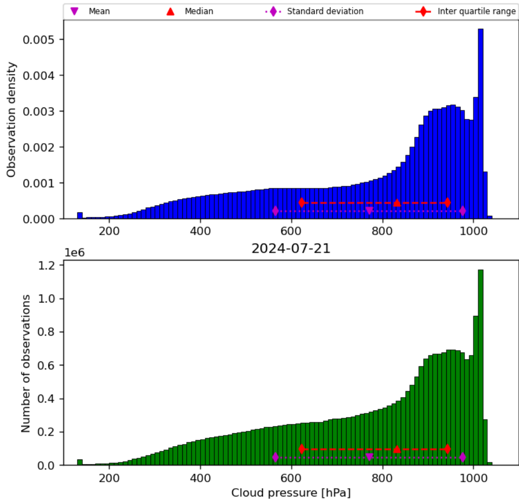
Figure 30: Histogram of “Cloud pressure” for 2024-07-21 to 2024-07-22
