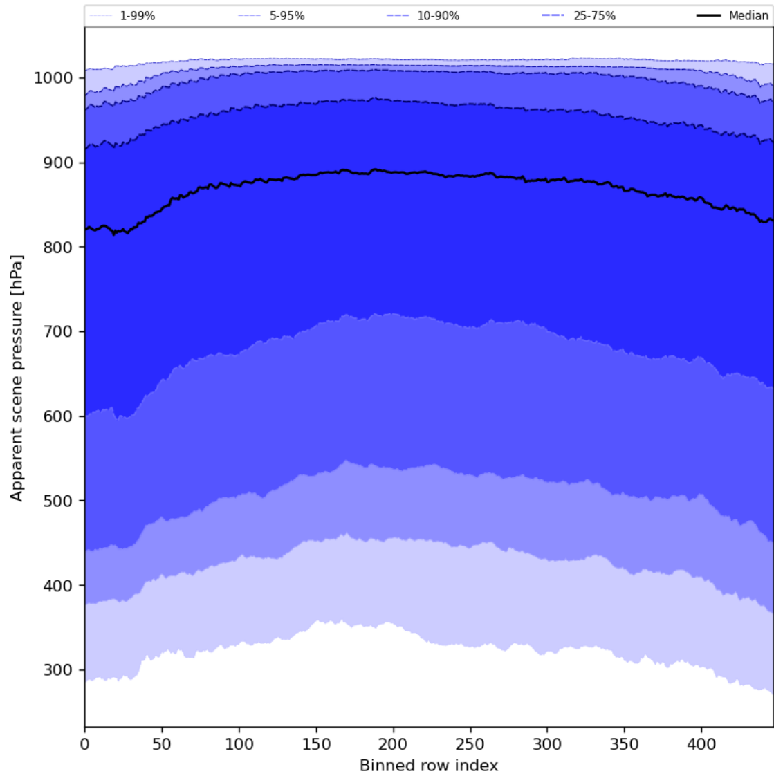
Figure 53: Along track statistics of “Apparent scene pressure” for 2024-07-21 to 2024-07-22
