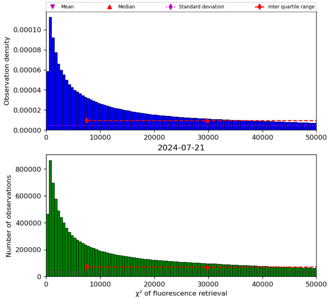
Figure 42: Histogram of “ \chi^2 of fluorescence retrieval” for 2024-07-21 to 2024-07-22
