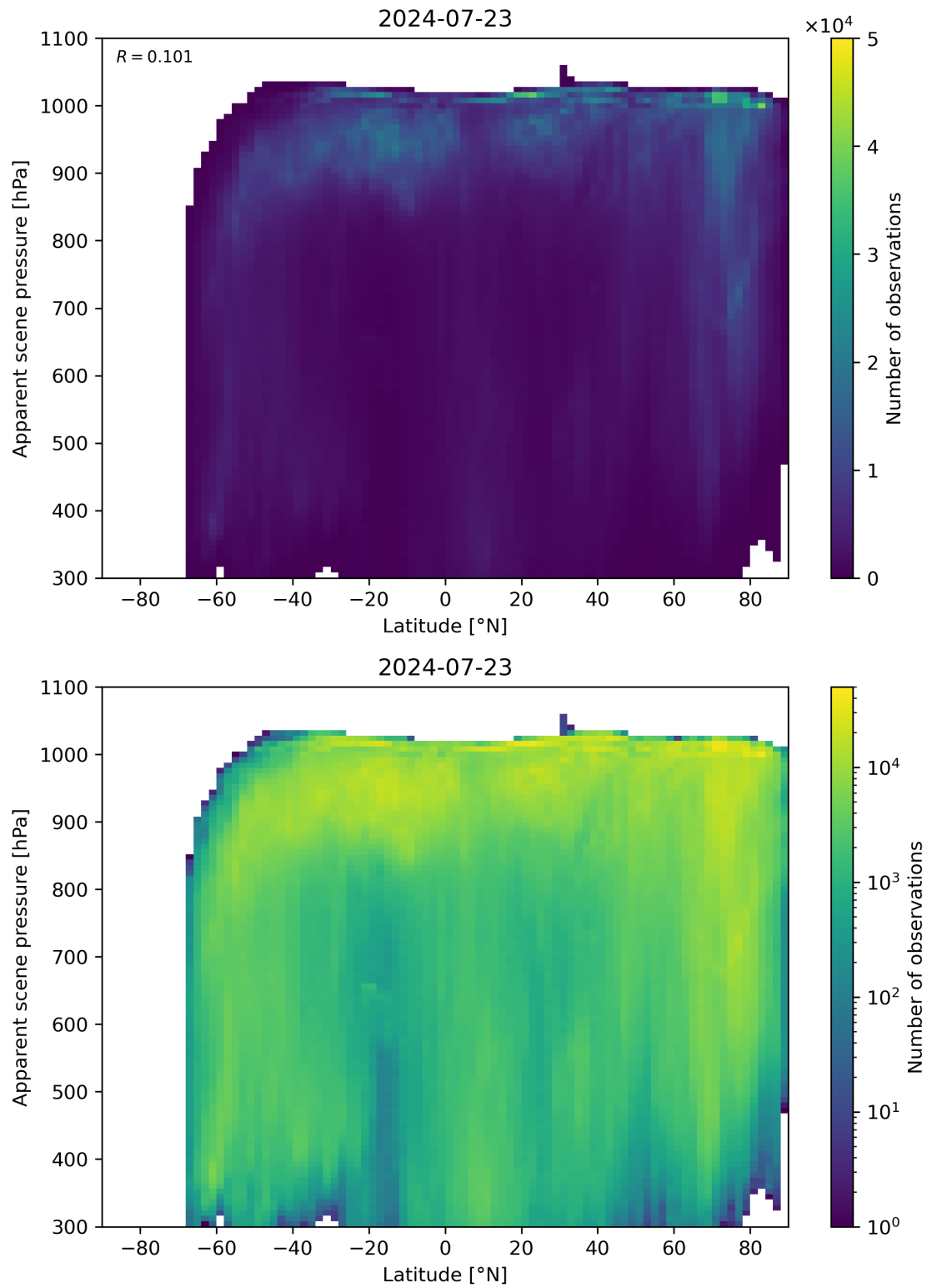
Figure 88: Scatter density plot of “Latitude” against “Apparent scene pressure” for 2024-07-22 to 2024-07-24.
