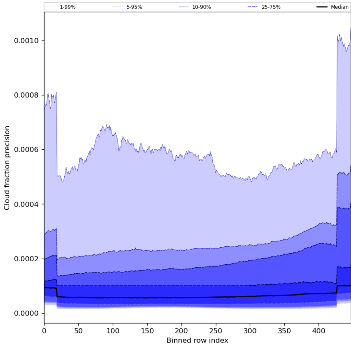
Figure 50: Along track statistics of “Cloud fraction precision” for 2024-07-22 to 2024-07-24
