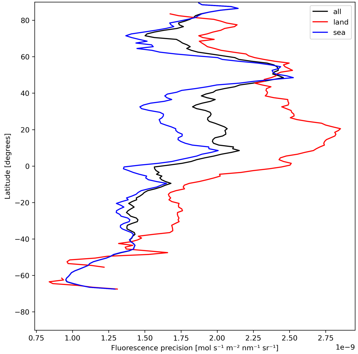
Figure 24: Zonal average of “Fluorescence precision” for 2024-07-22 to 2024-07-24.
