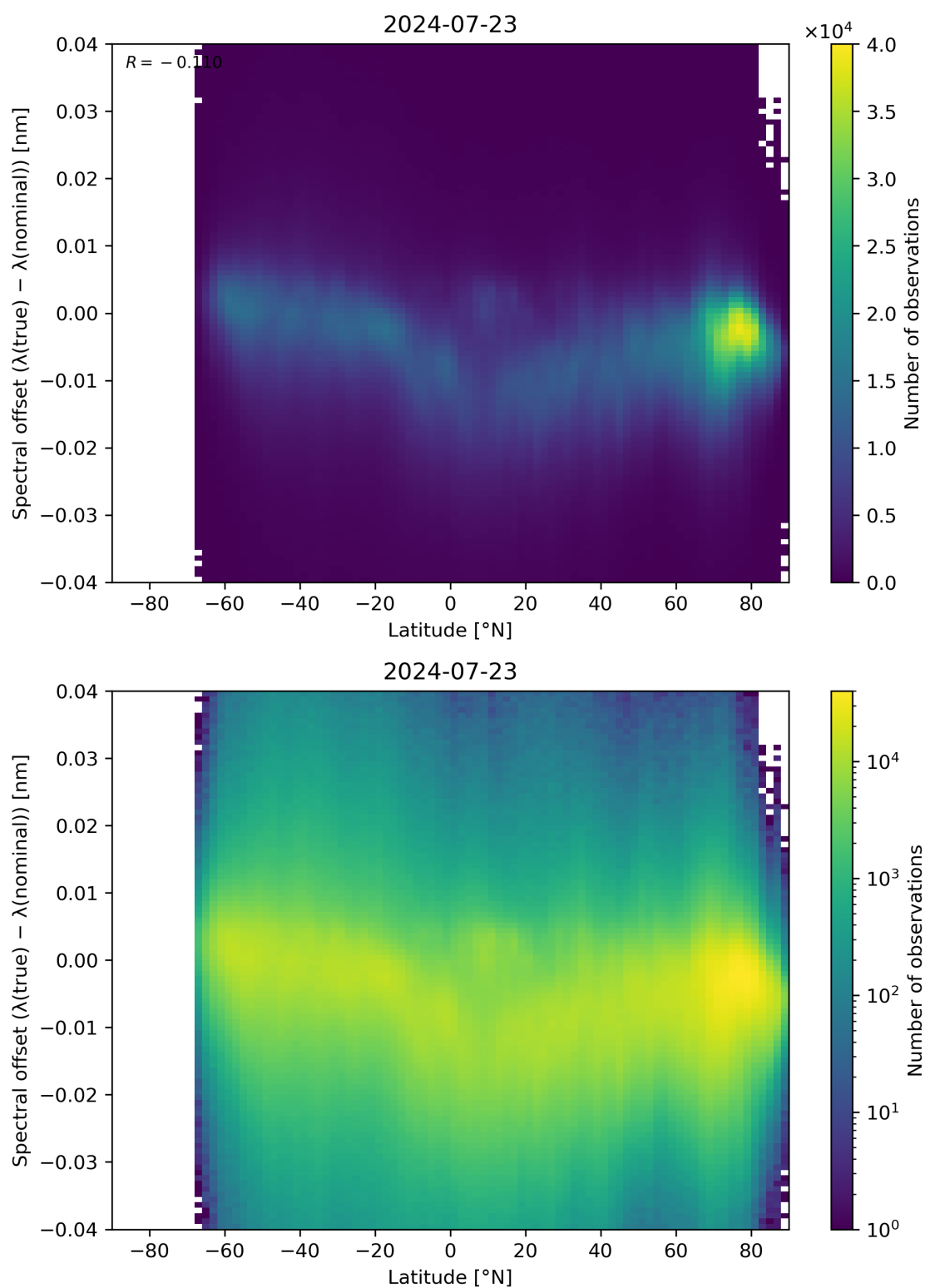
Figure 96: Scatter density plot of “Latitude” against “Spectral offset ( \lambda(\text{true}) - \lambda(\text{nominal}) )” for 2024-07-22 to 2024-07-24.
