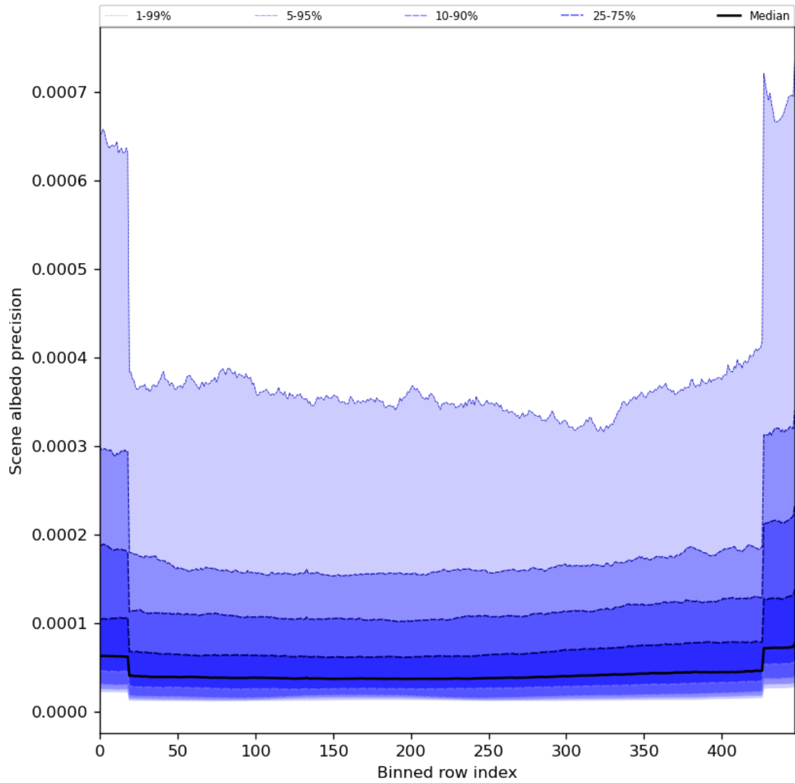
Figure 52: Along track statistics of “Scene albedo precision” for 2024-07-22 to 2024-07-24
