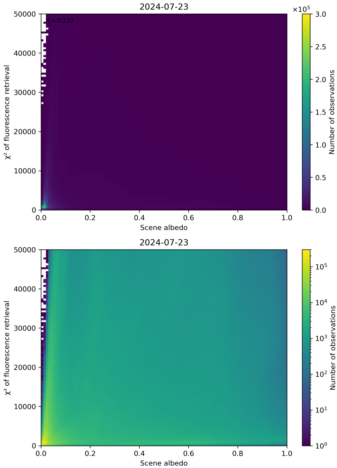
Figure 103: Scatter density plot of “Scene albedo” against “ \chi^2 of fluorescence retrieval” for 2024-07-22 to 2024-07-24.
