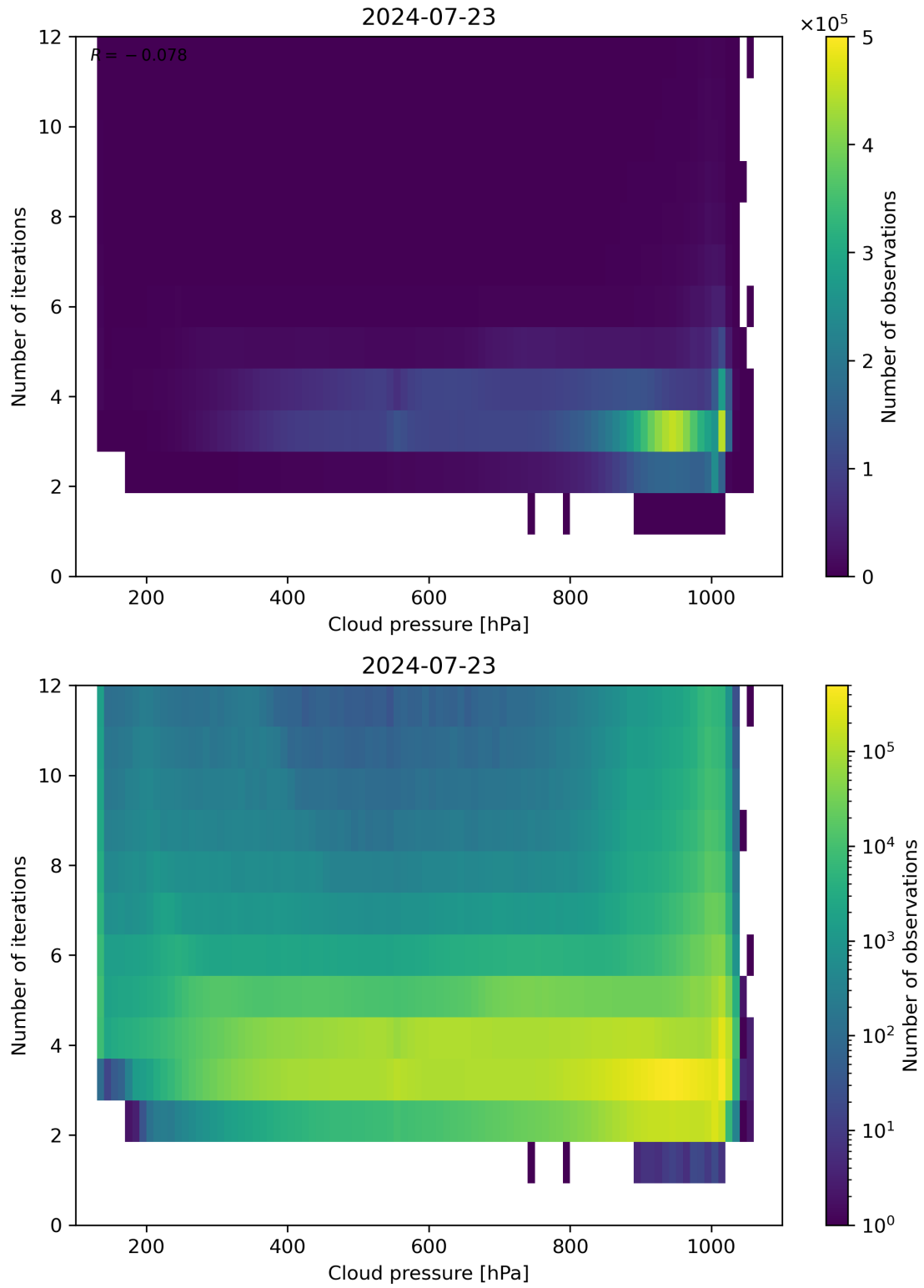
Figure 81: Scatter density plot of “Cloud pressure” against “Number of iterations” for 2024-07-22 to 2024-07-24.
