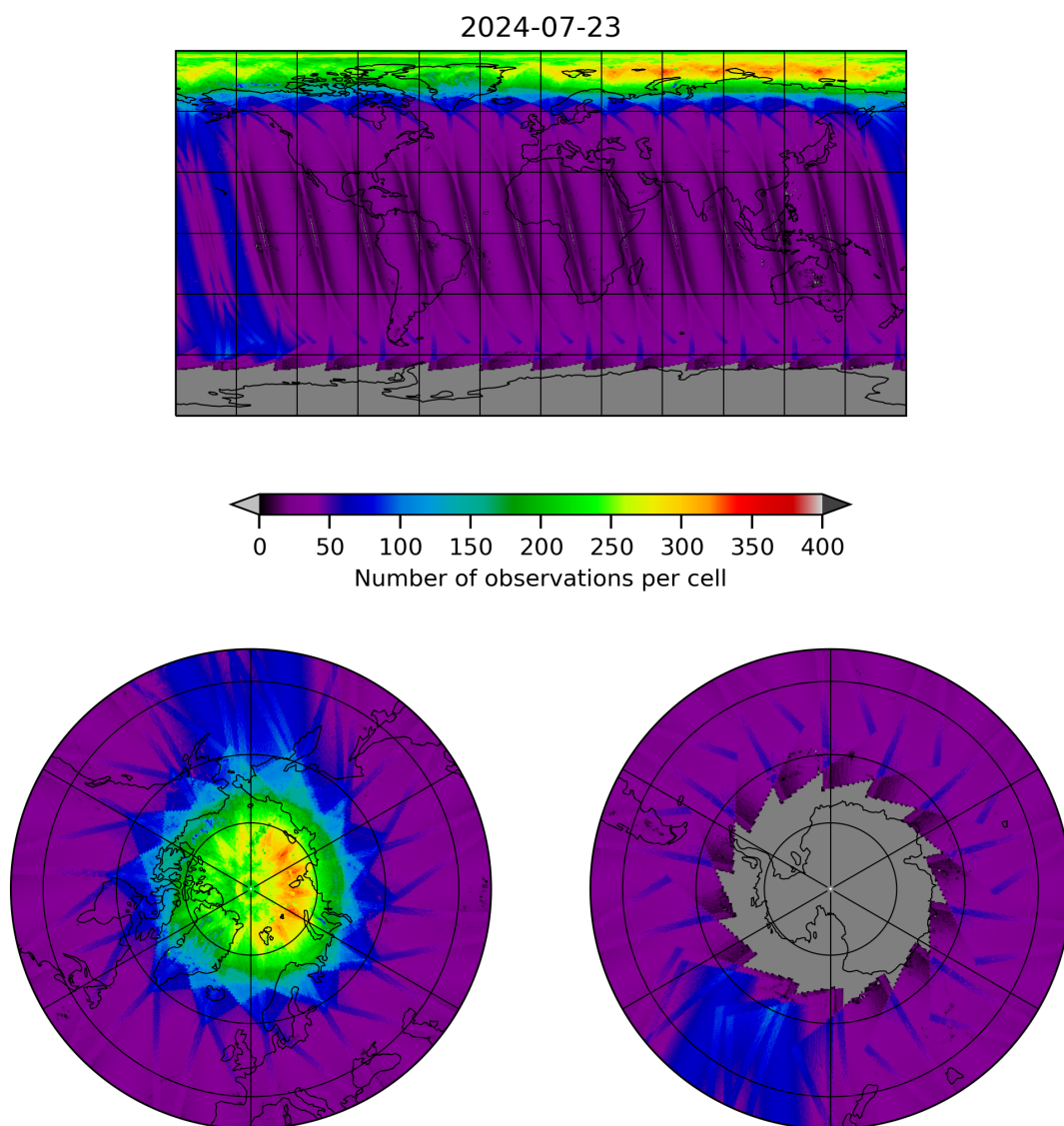
Figure 11: Map of the number of observations for 2024-07-22 to 2024-07-24
