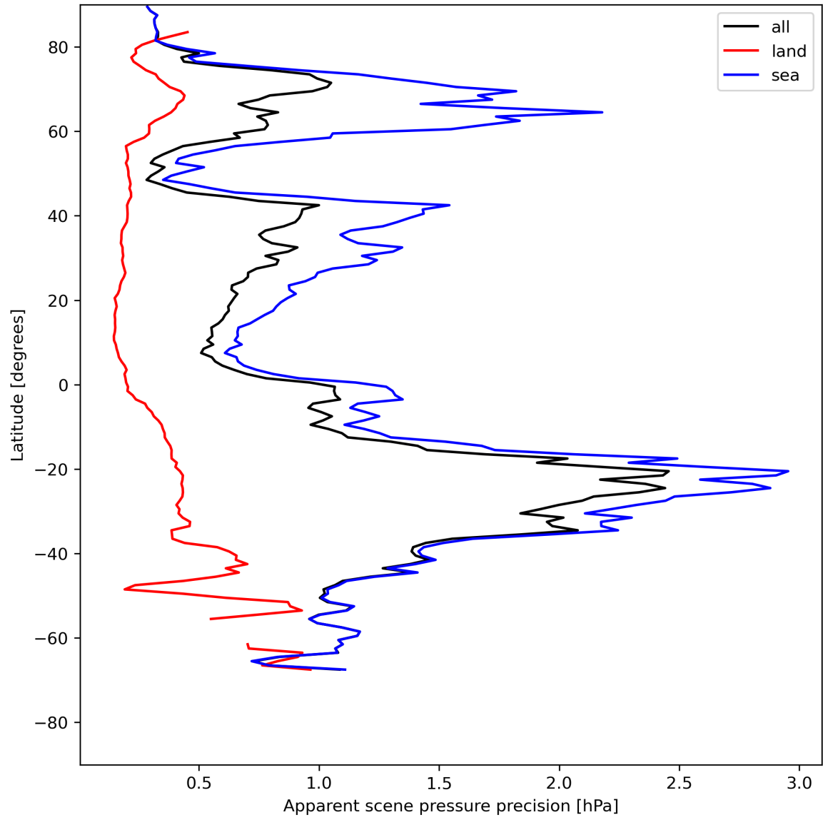
Figure 20: Zonal average of “Apparent scene pressure precision” for 2024-07-22 to 2024-07-24.
