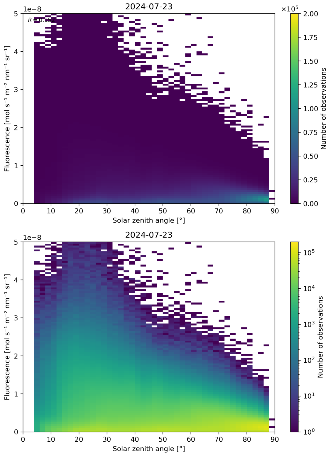
Figure 112: Scatter density plot of “Solar zenith angle” against “Fluorescence” for 2024-07-22 to 2024-07-24.
