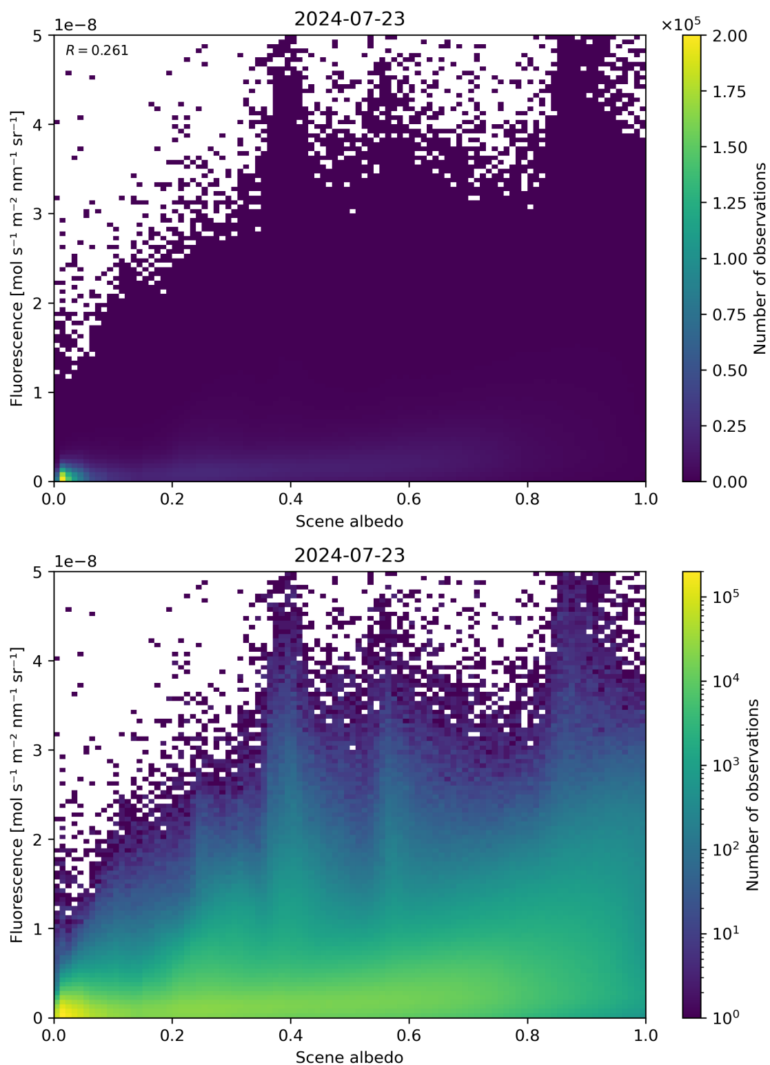
Figure 104: Scatter density plot of “Scene albedo” against “Fluorescence” for 2024-07-22 to 2024-07-24.
