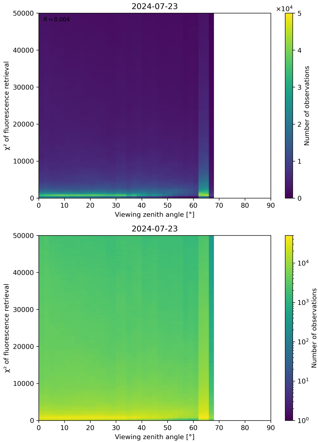
Figure 119: Scatter density plot of “Viewing zenith angle” against “ \chi^2 of fluorescence retrieval” for 2024-07-22 to 2024-07-24.
