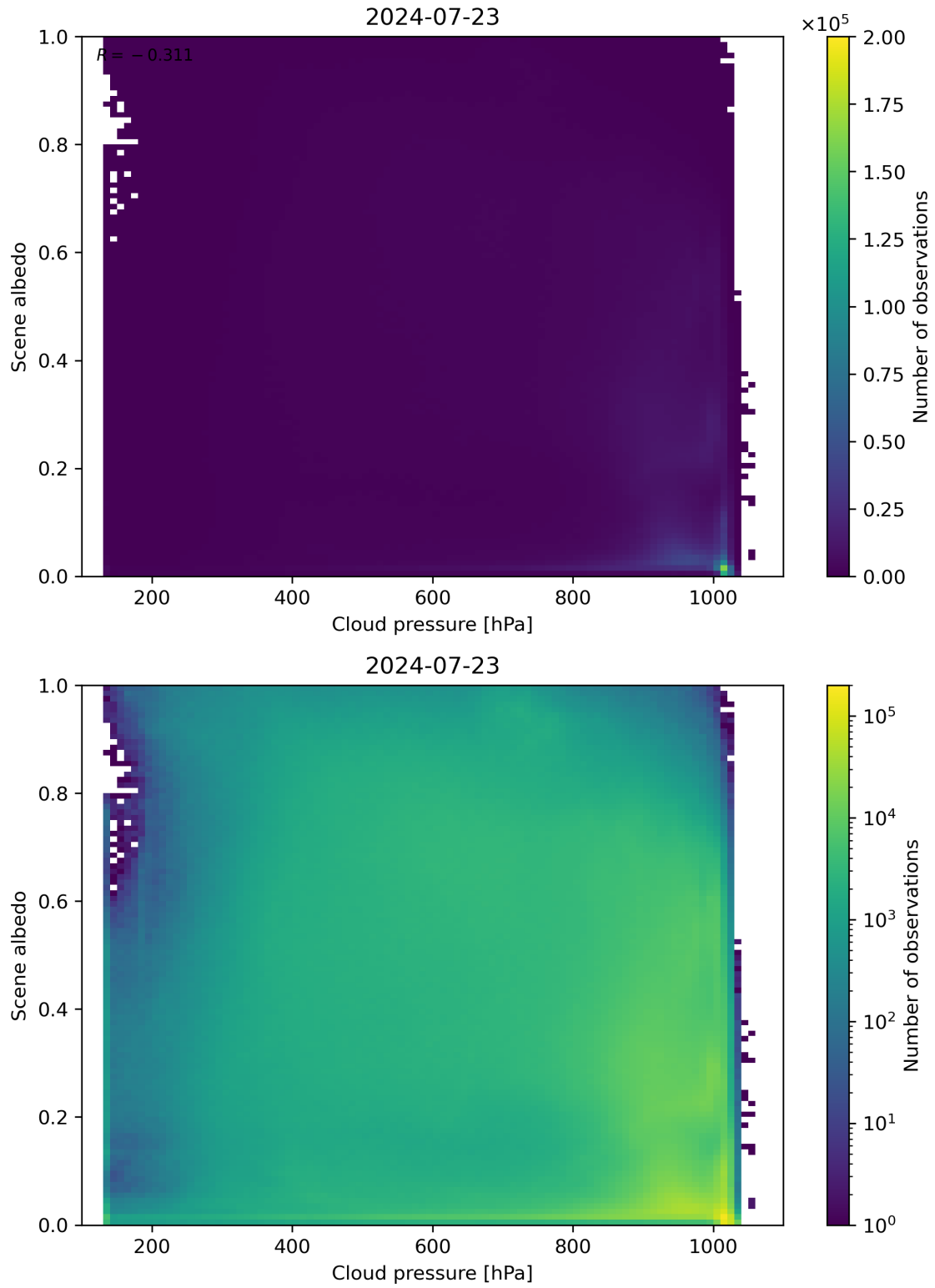
Figure 83: Scatter density plot of “Cloud pressure” against “Scene albedo” for 2024-07-22 to 2024-07-24.
