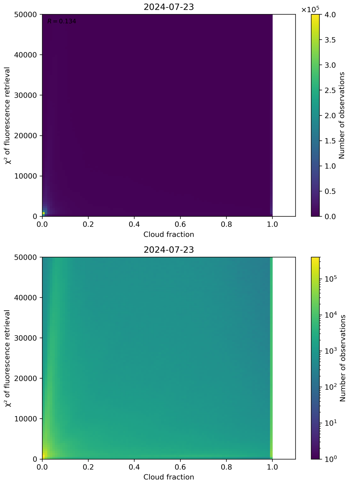
Figure 71: Scatter density plot of “Cloud fraction” against “ \chi^2 of fluorescence retrieval” for 2024-07-22 to 2024-07-24.
