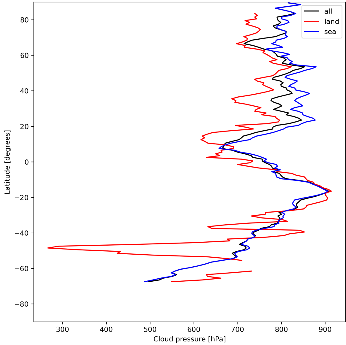
Figure 13: Zonal average of “Cloud pressure” for 2024-07-22 to 2024-07-24.
