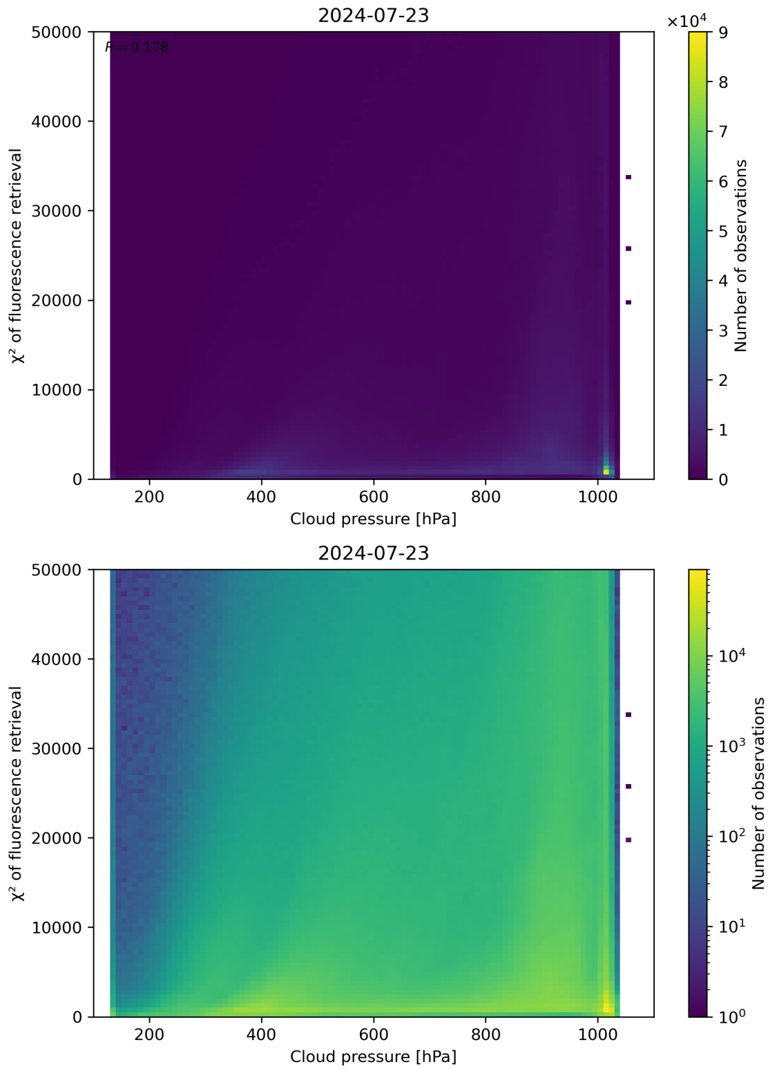
Figure 78: Scatter density plot of “Cloud pressure” against “ \chi^2 of fluorescence retrieval” for 2024-07-22 to 2024-07-24.
