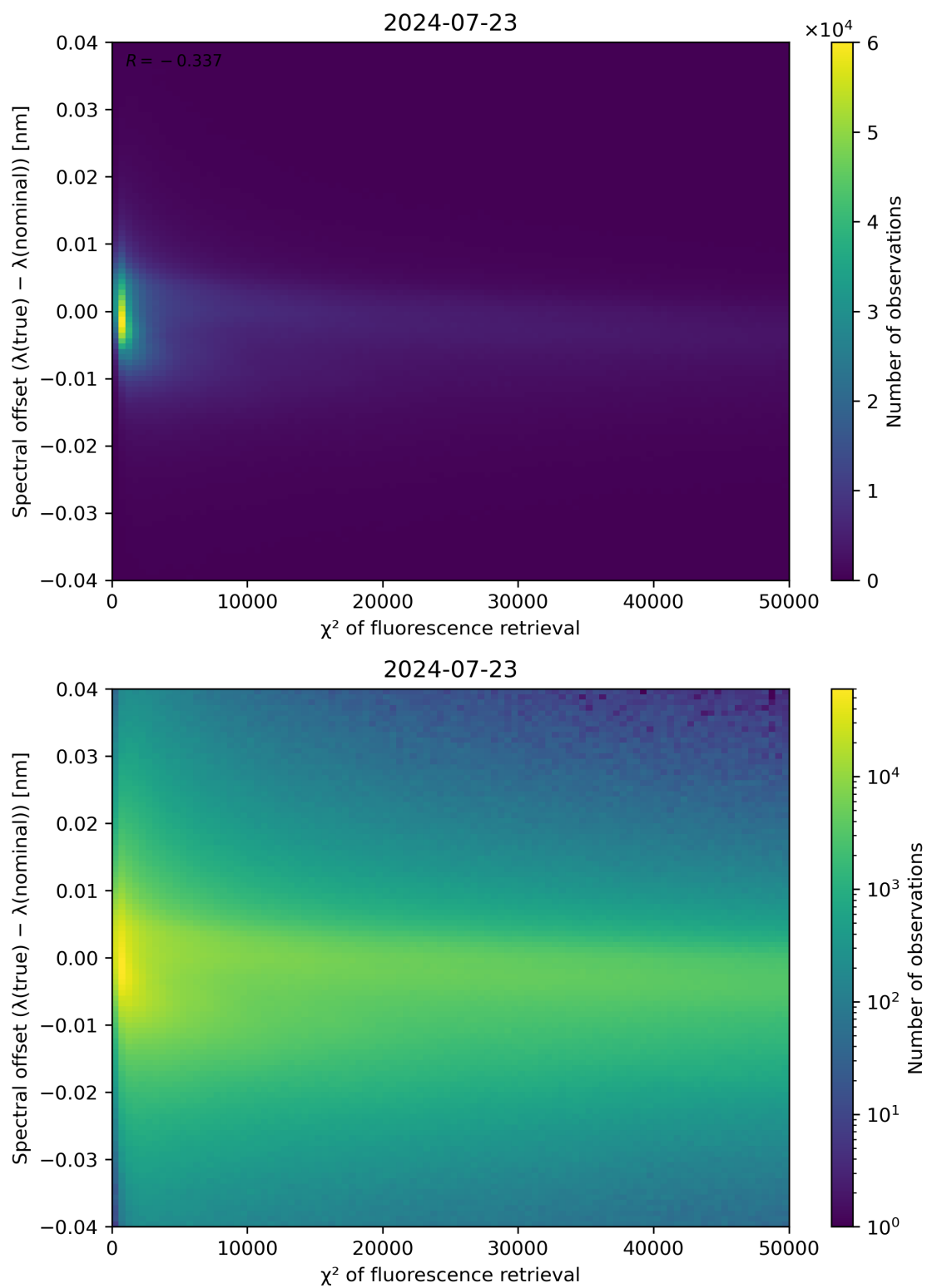
Figure 69: Scatter density plot of “ \chi^2 of fluorescence retrieval” against “Spectral offset ( \lambda(\text{true}) - \lambda(\text{nominal}) )” for 2024-07-22 to 2024-07-24.
