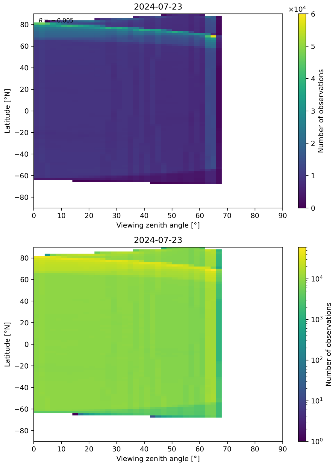
Figure 123: Scatter density plot of “Viewing zenith angle” against “Latitude” for 2024-07-22 to 2024-07-24.
