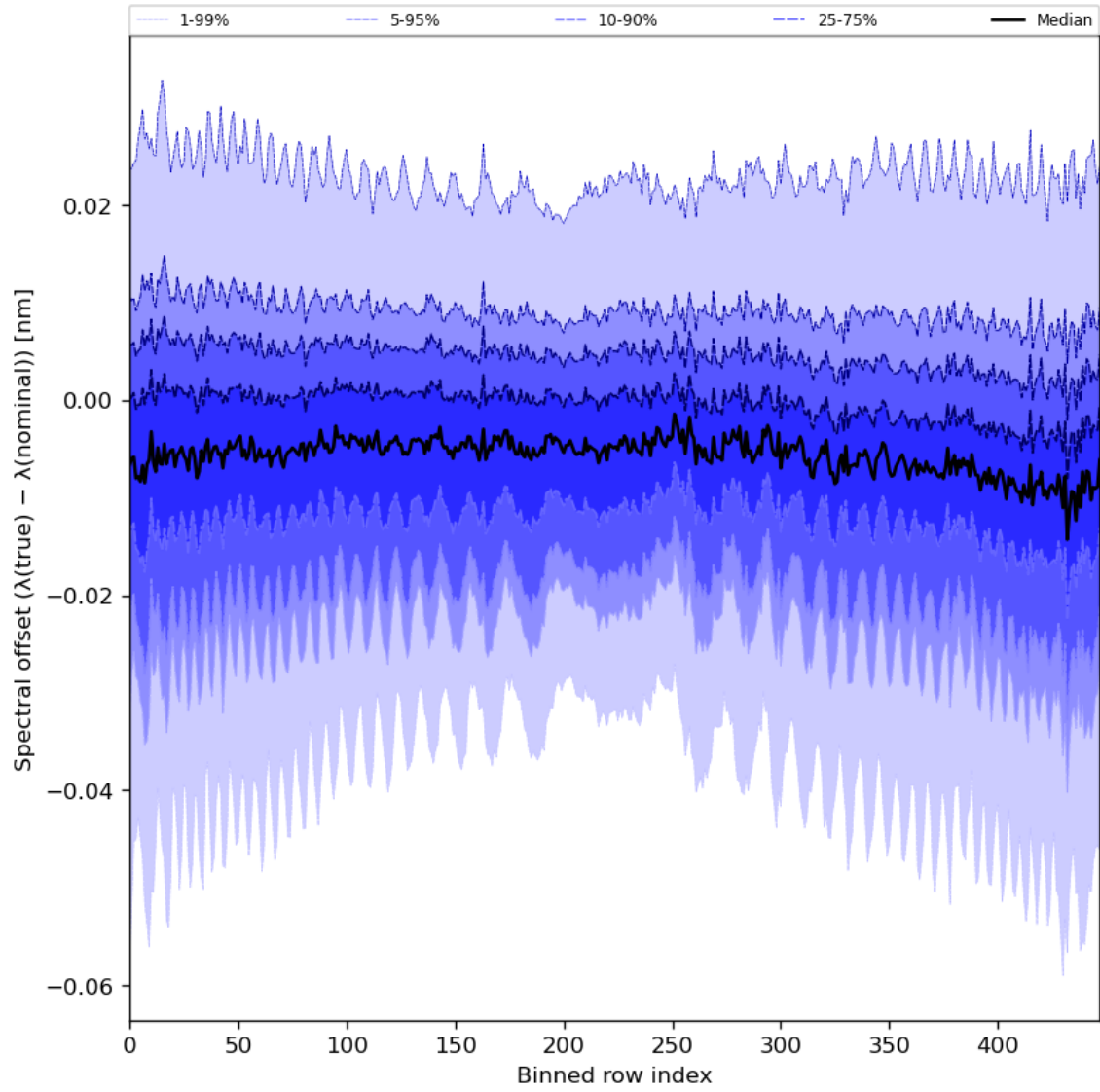
Figure 62: Along track statistics of “Spectral offset ( \lambda(\text{true}) - \lambda(\text{nominal}) )” for 2024-07-22 to 2024-07-24
