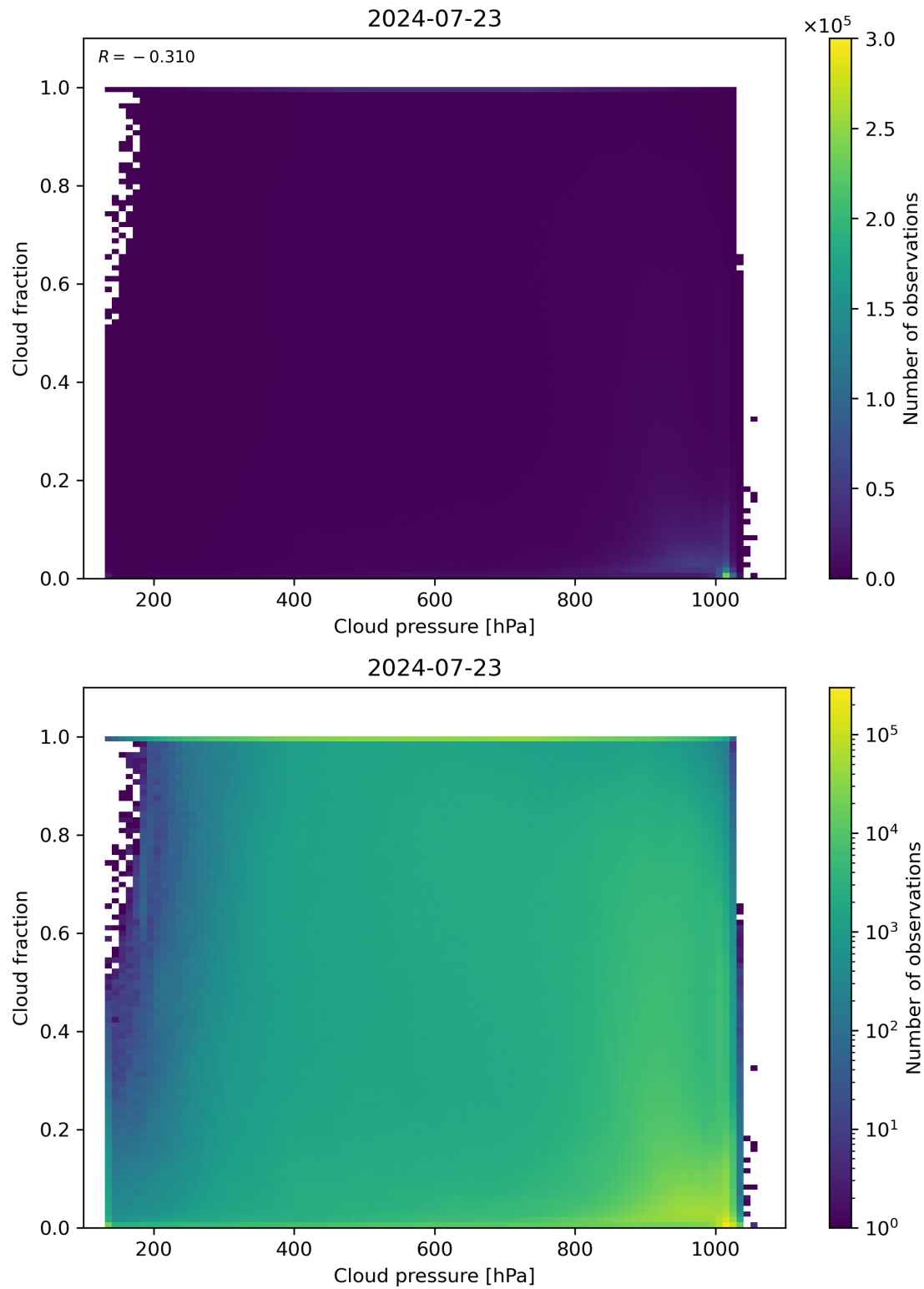
Figure 79: Scatter density plot of “Cloud pressure” against “Cloud fraction” for 2024-07-22 to 2024-07-24.
