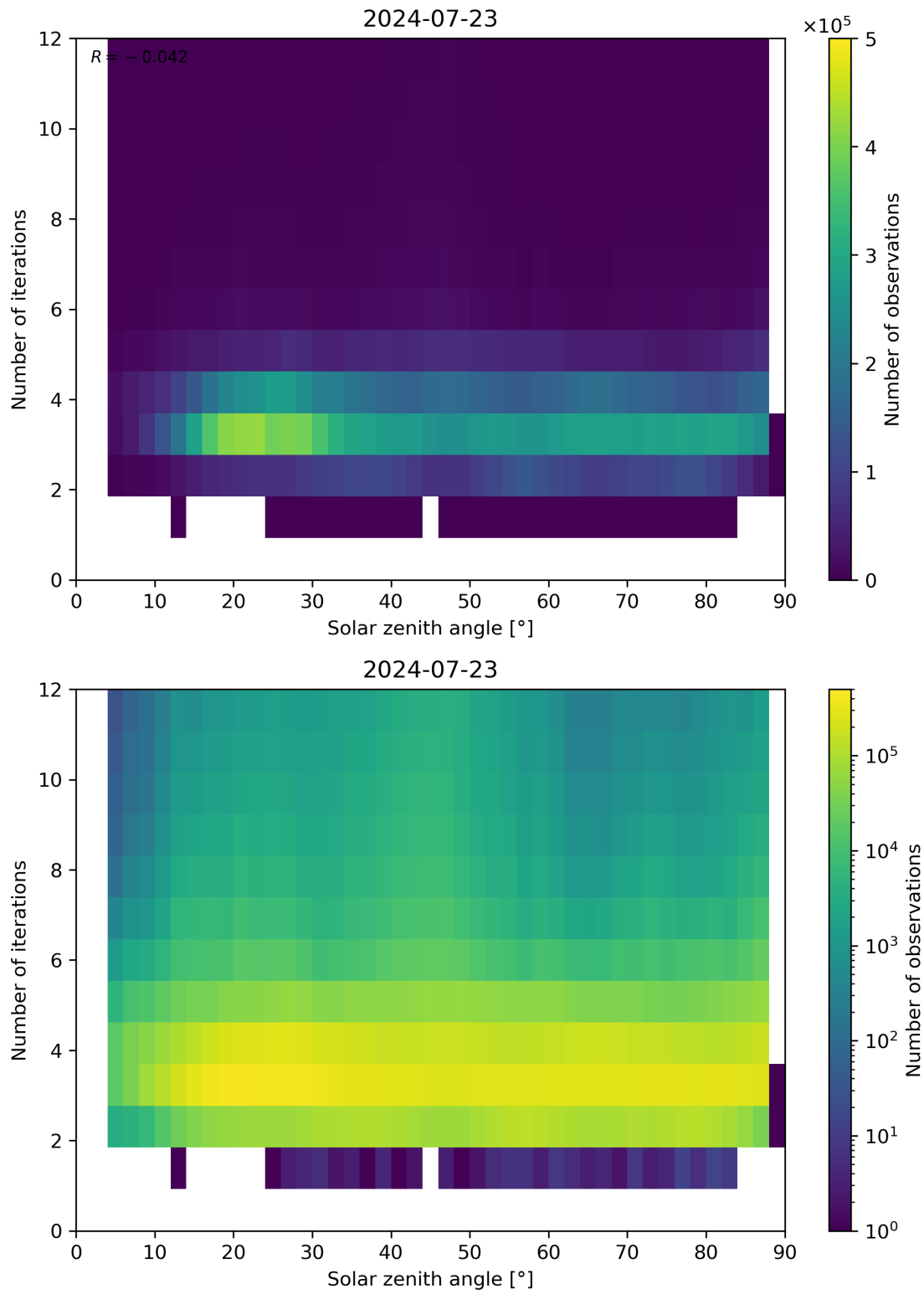
Figure 114: Scatter density plot of “Solar zenith angle” against “Number of iterations” for 2024-07-22 to 2024-07-24.
