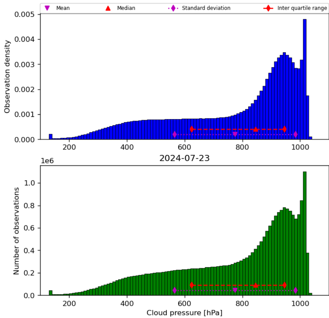
Figure 30: Histogram of “Cloud pressure” for 2024-07-22 to 2024-07-24
