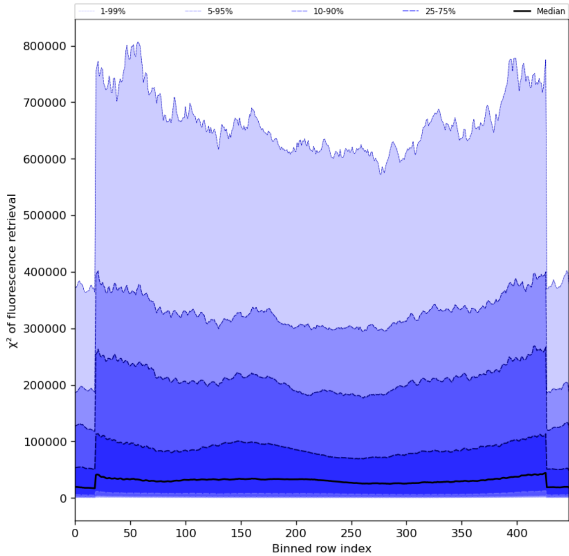
Figure 59: Along track statistics of “ \chi^2 of fluorescence retrieval” for 2024-07-22 to 2024-07-24
