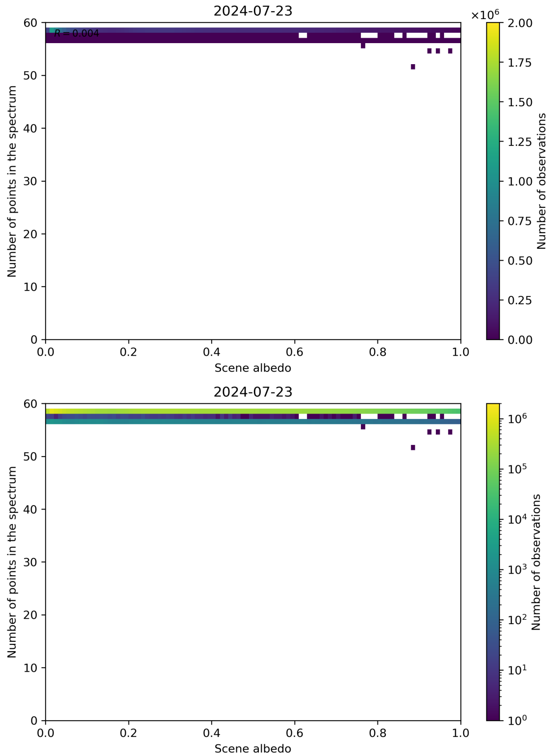
Figure 106: Scatter density plot of “Scene albedo” against “Number of points in the spectrum” for 2024-07-22 to 2024-07-24.
