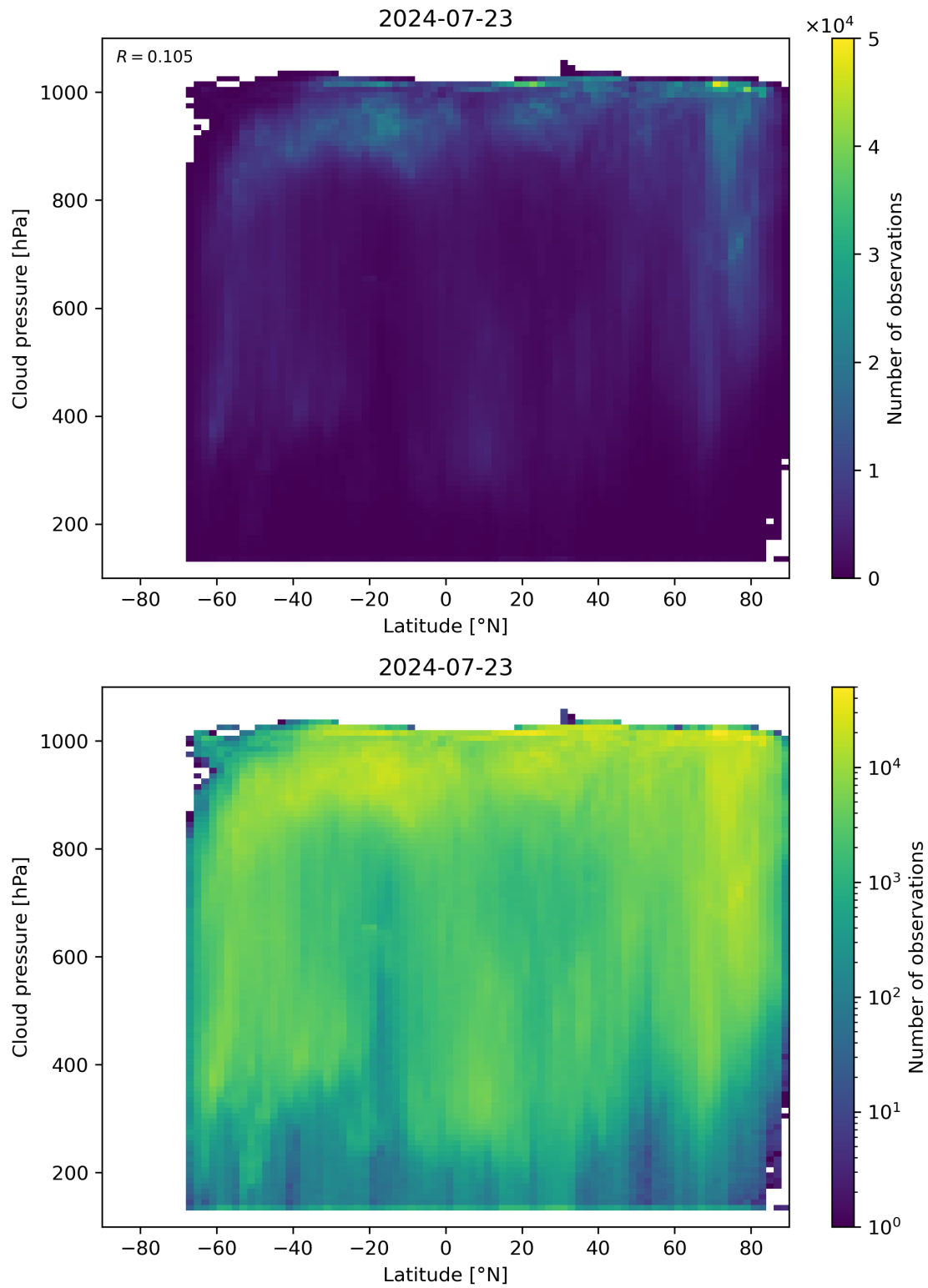
Figure 91: Scatter density plot of “Latitude” against “Cloud pressure” for 2024-07-22 to 2024-07-24.
