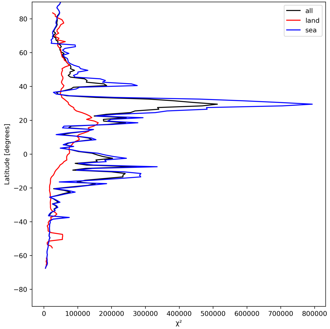
Figure 21: Zonal average of “ \chi^2 ” for 2024-07-22 to 2024-07-24.
