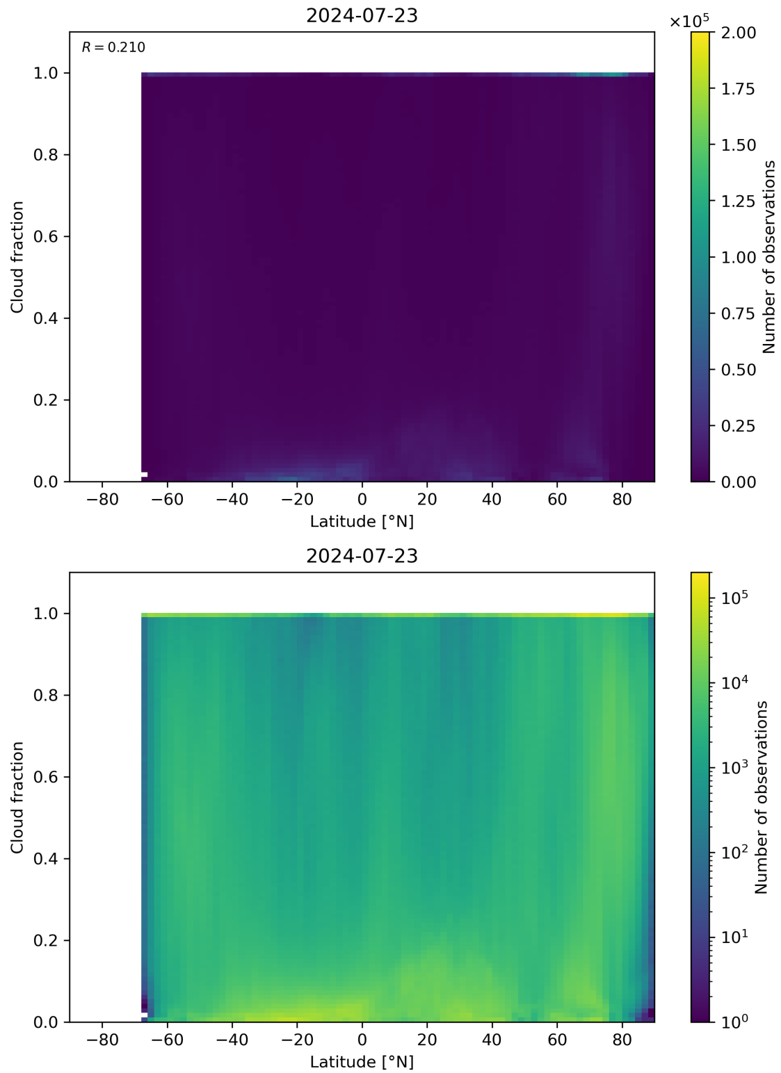
Figure 90: Scatter density plot of “Latitude” against “Cloud fraction” for 2024-07-22 to 2024-07-24.
