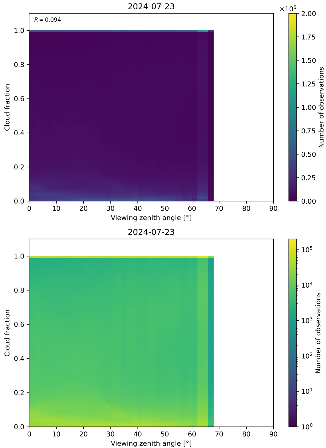
Figure 120: Scatter density plot of “Viewing zenith angle” against “Cloud fraction” for 2024-07-22 to 2024-07-24.
