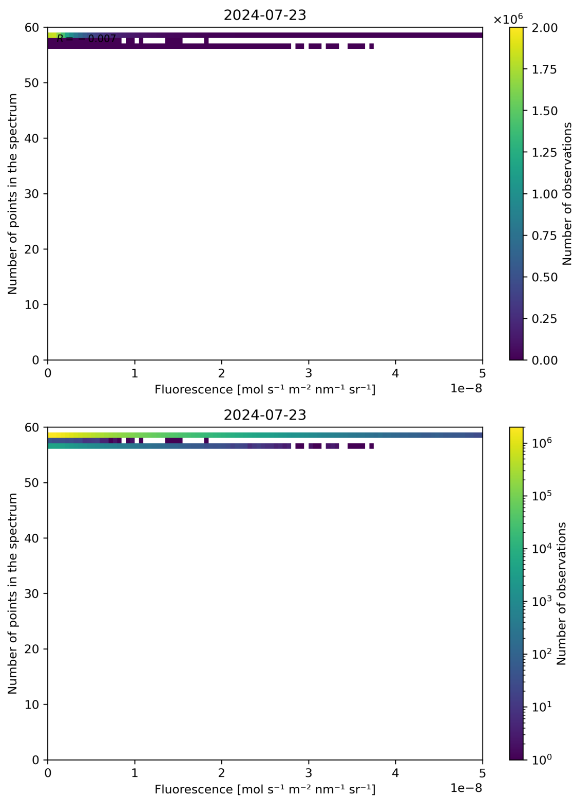
Figure 86: Scatter density plot of “Fluorescence” against “Number of points in the spectrum” for 2024-07-22 to 2024-07-24.
