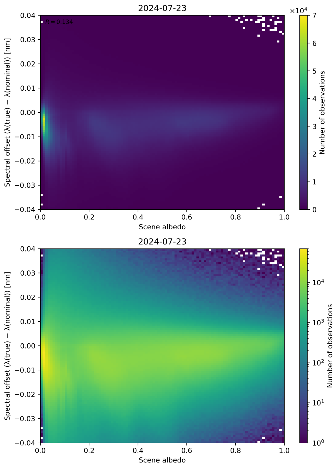
Figure 107: Scatter density plot of “Scene albedo” against “Spectral offset ( \lambda(\text{true}) - \lambda(\text{nominal}) )” for 2024-07-22 to 2024-07-24.
