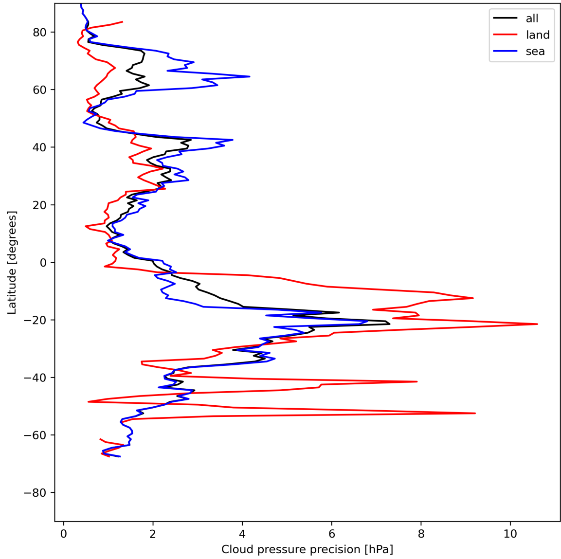
Figure 14: Zonal average of “Cloud pressure precision” for 2024-07-22 to 2024-07-24.
