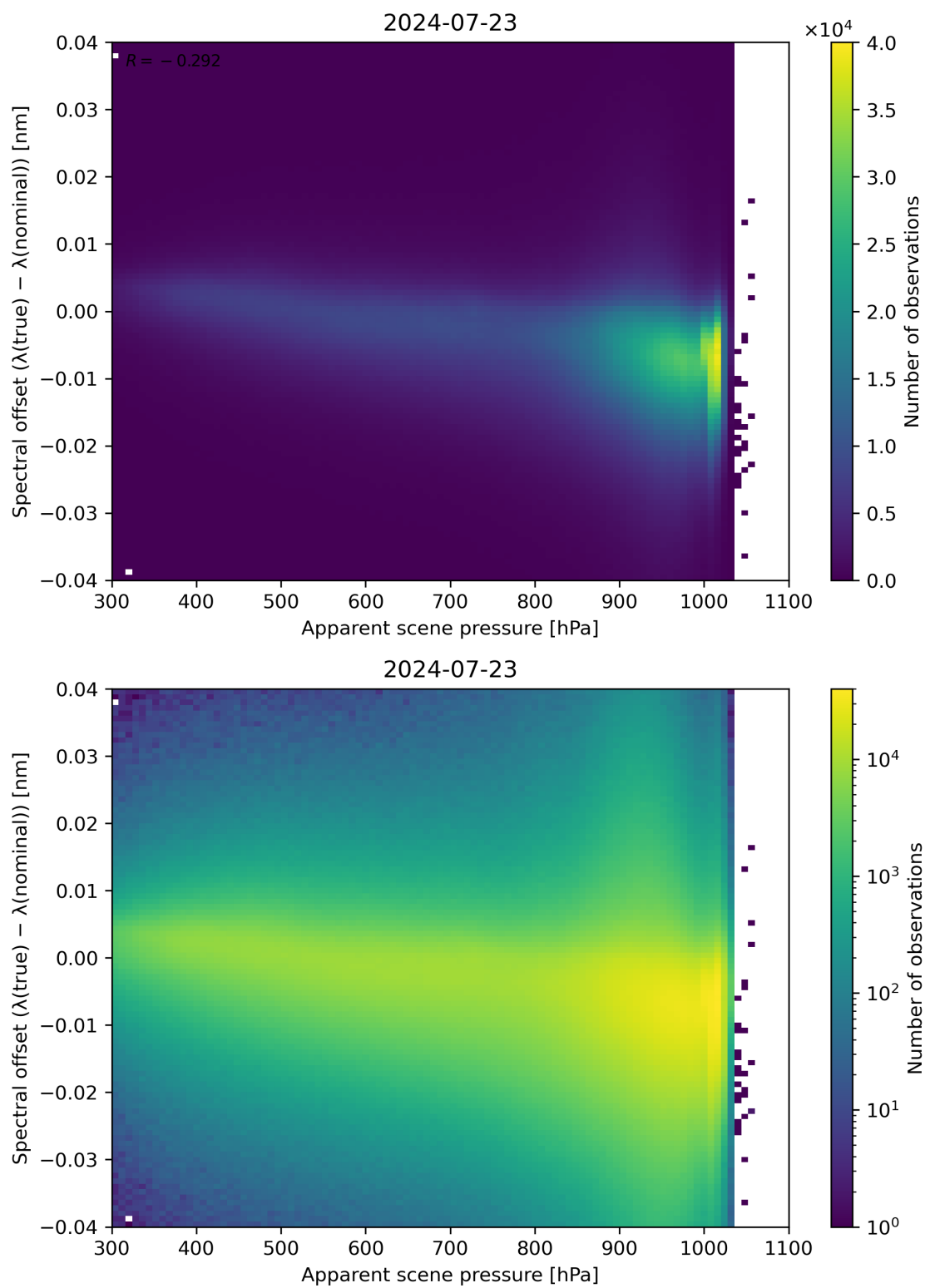
Figure 67: Scatter density plot of “Apparent scene pressure” against “Spectral offset ( \lambda(\text{true}) - \lambda(\text{nominal}) )” for 2024-07-22 to 2024-07-24.
