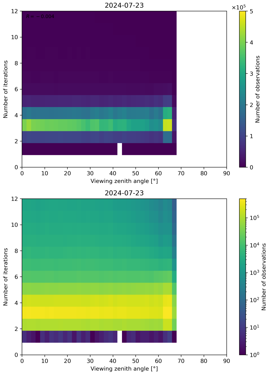
Figure 124: Scatter density plot of “Viewing zenith angle” against “Number of iterations” for 2024-07-22 to 2024-07-24.
