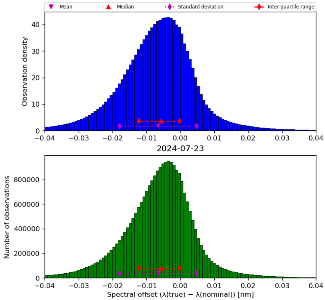
Figure 45: Histogram of “Spectral offset ( \lambda(\text{true}) - \lambda(\text{nominal}) )” for 2024-07-22 to 2024-07-24
