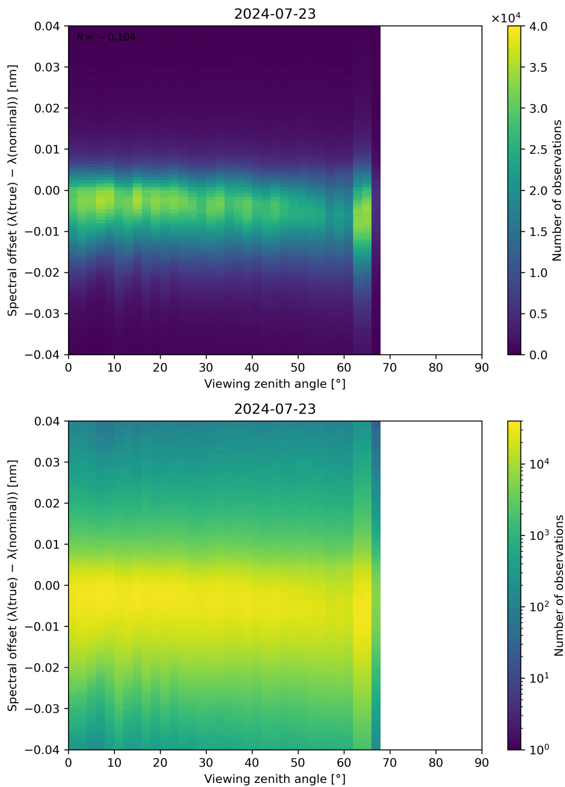
Figure 128: Scatter density plot of “Viewing zenith angle” against “Spectral offset ( \lambda(\text{true}) - \lambda(\text{nominal}) )” for 2024-07-22 to 2024-07-24.
