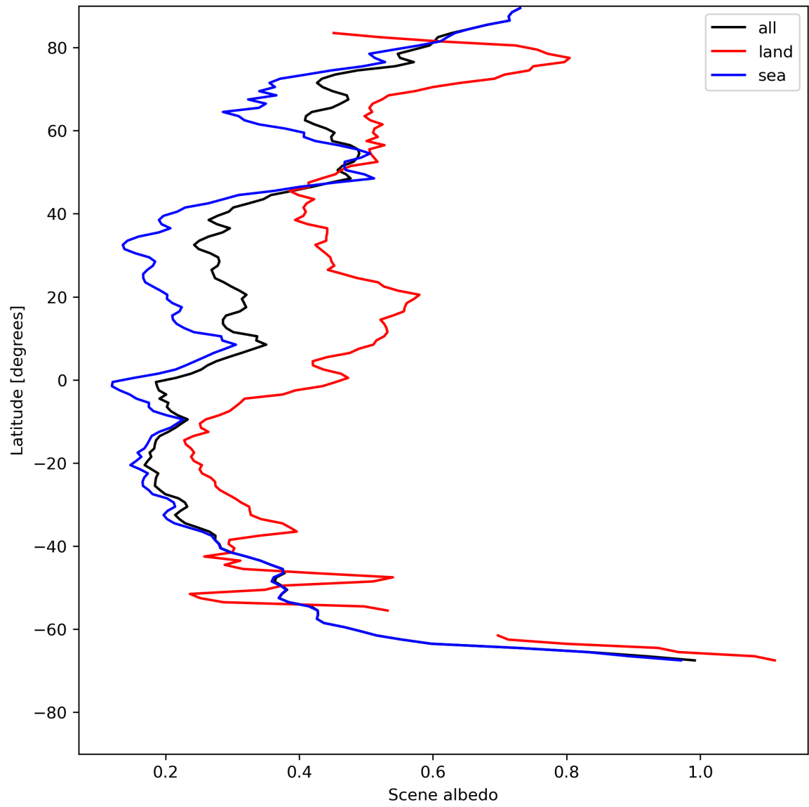
Figure 17: Zonal average of “Scene albedo” for 2024-07-22 to 2024-07-24.
