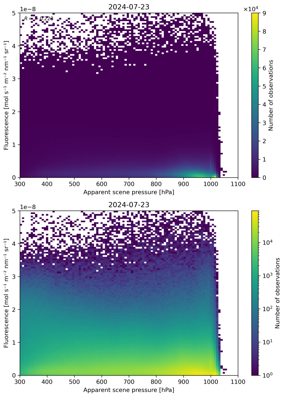
Figure 64: Scatter density plot of “Apparent scene pressure” against “Fluorescence” for 2024-07-22 to 2024-07-24.
