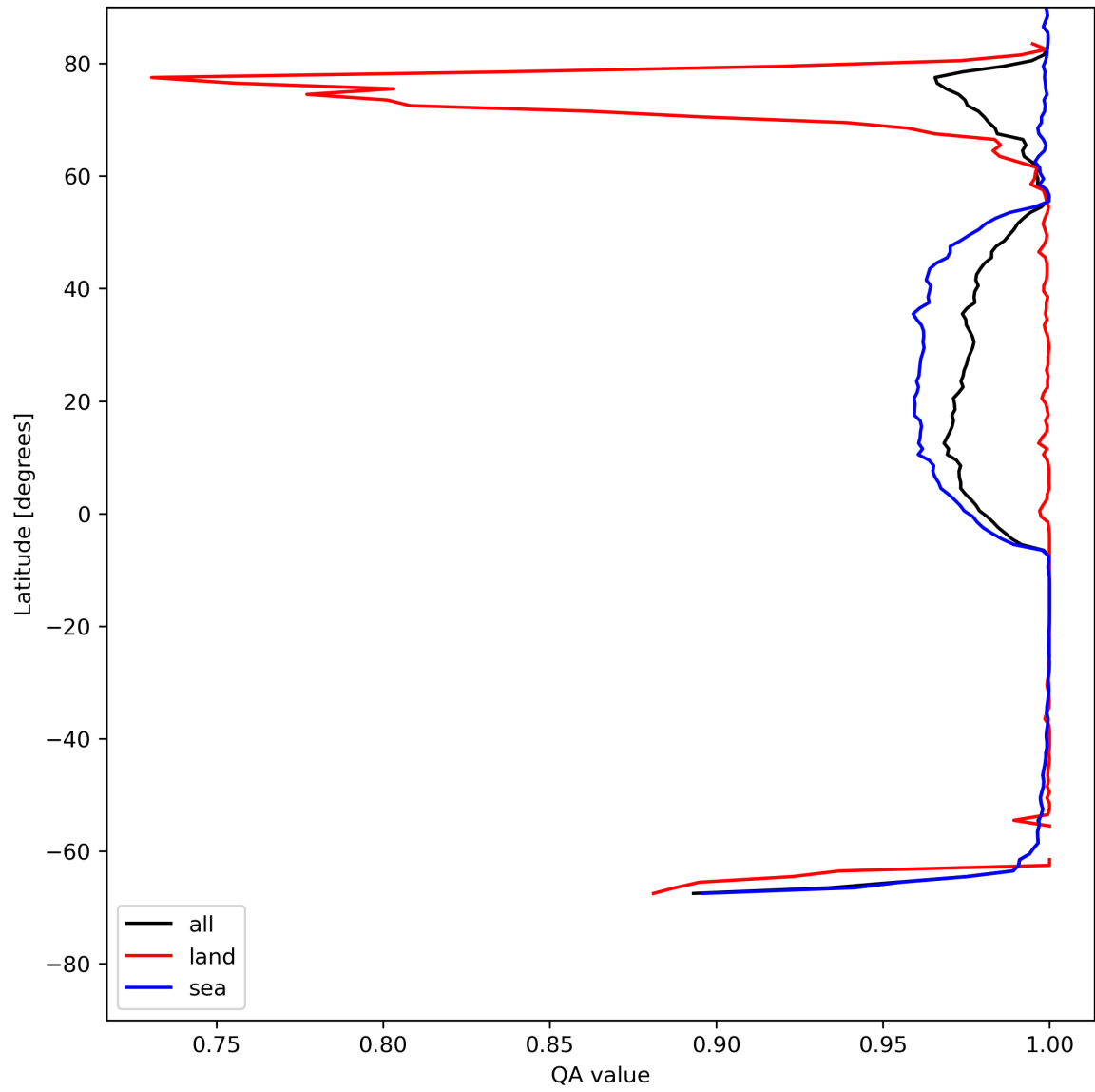
Figure 12: Zonal average of “QA value” for 2024-07-22 to 2024-07-24.
