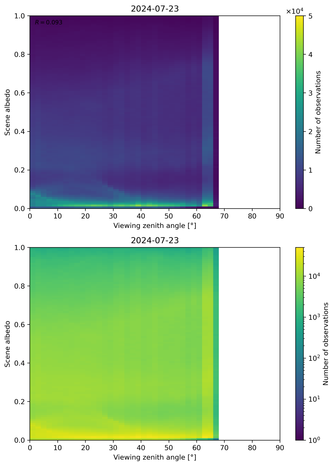
Figure 126: Scatter density plot of “Viewing zenith angle” against “Scene albedo” for 2024-07-22 to 2024-07-24.
