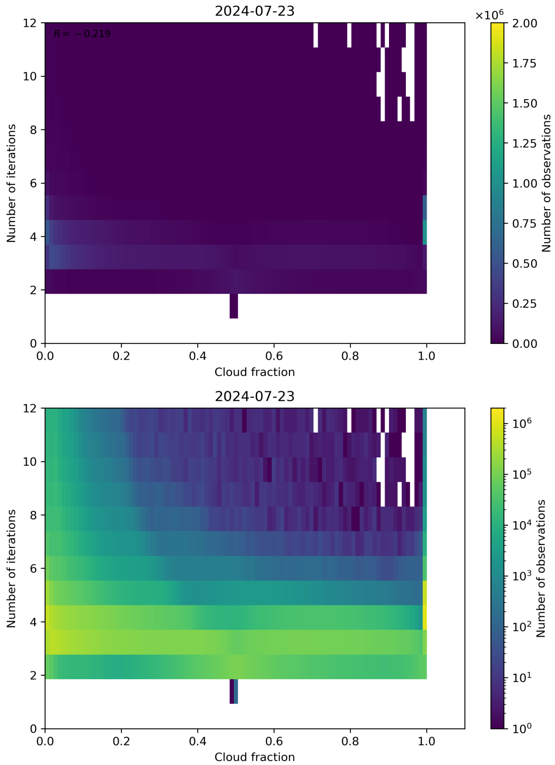
Figure 73: Scatter density plot of “Cloud fraction” against “Number of iterations” for 2024-07-22 to 2024-07-24.
