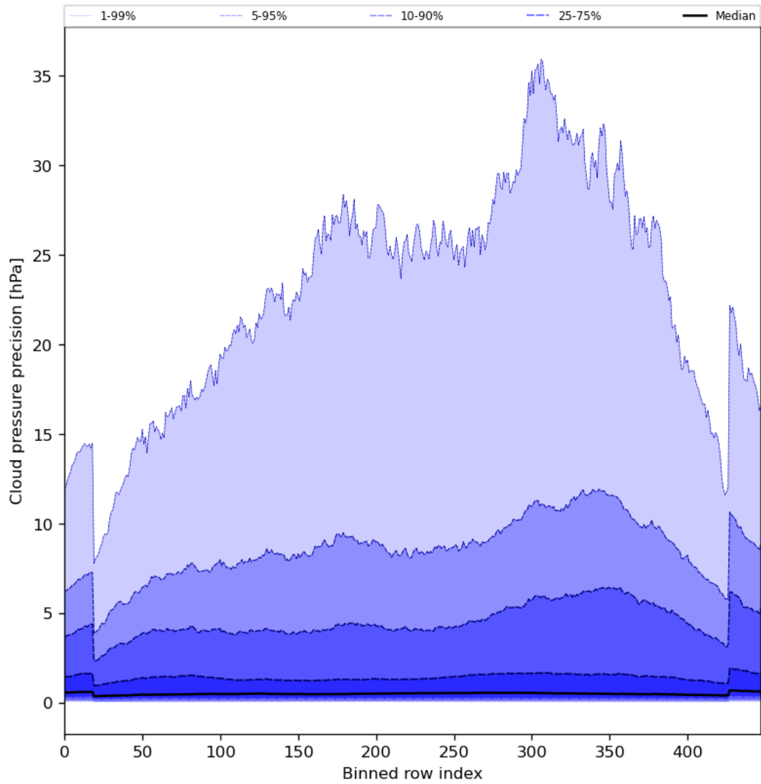
Figure 48: Along track statistics of “Cloud pressure precision” for 2024-07-22 to 2024-07-24
