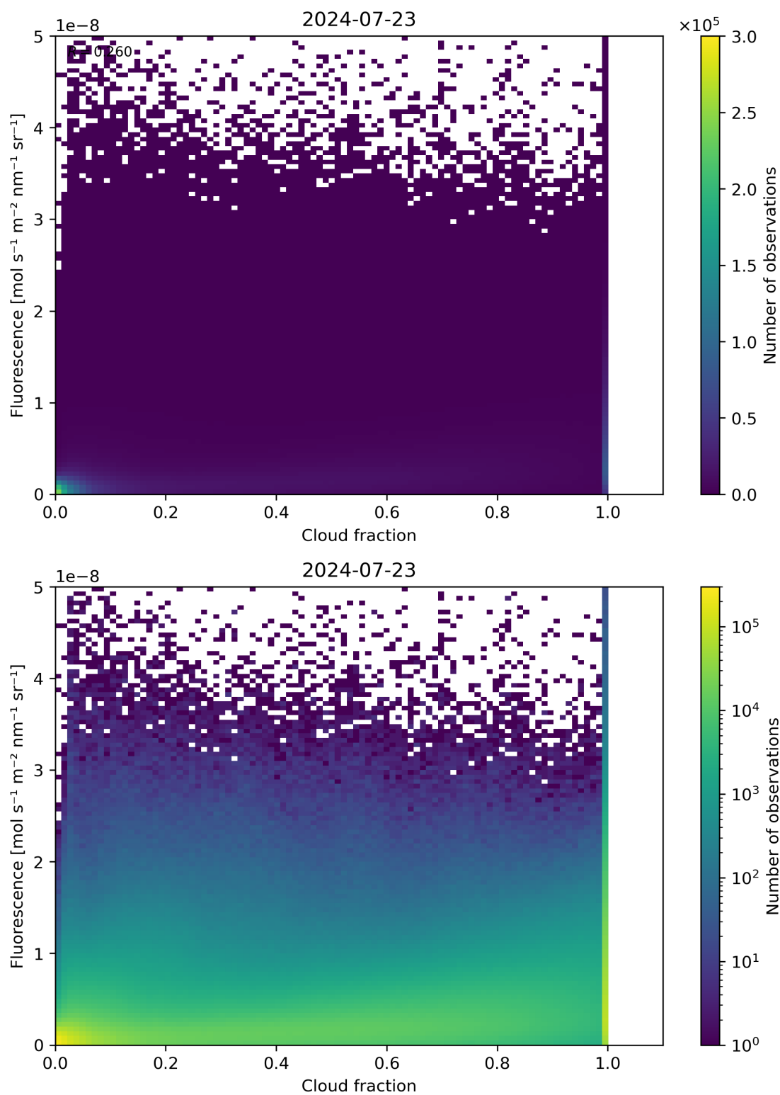
Figure 72: Scatter density plot of “Cloud fraction” against “Fluorescence” for 2024-07-22 to 2024-07-24.
