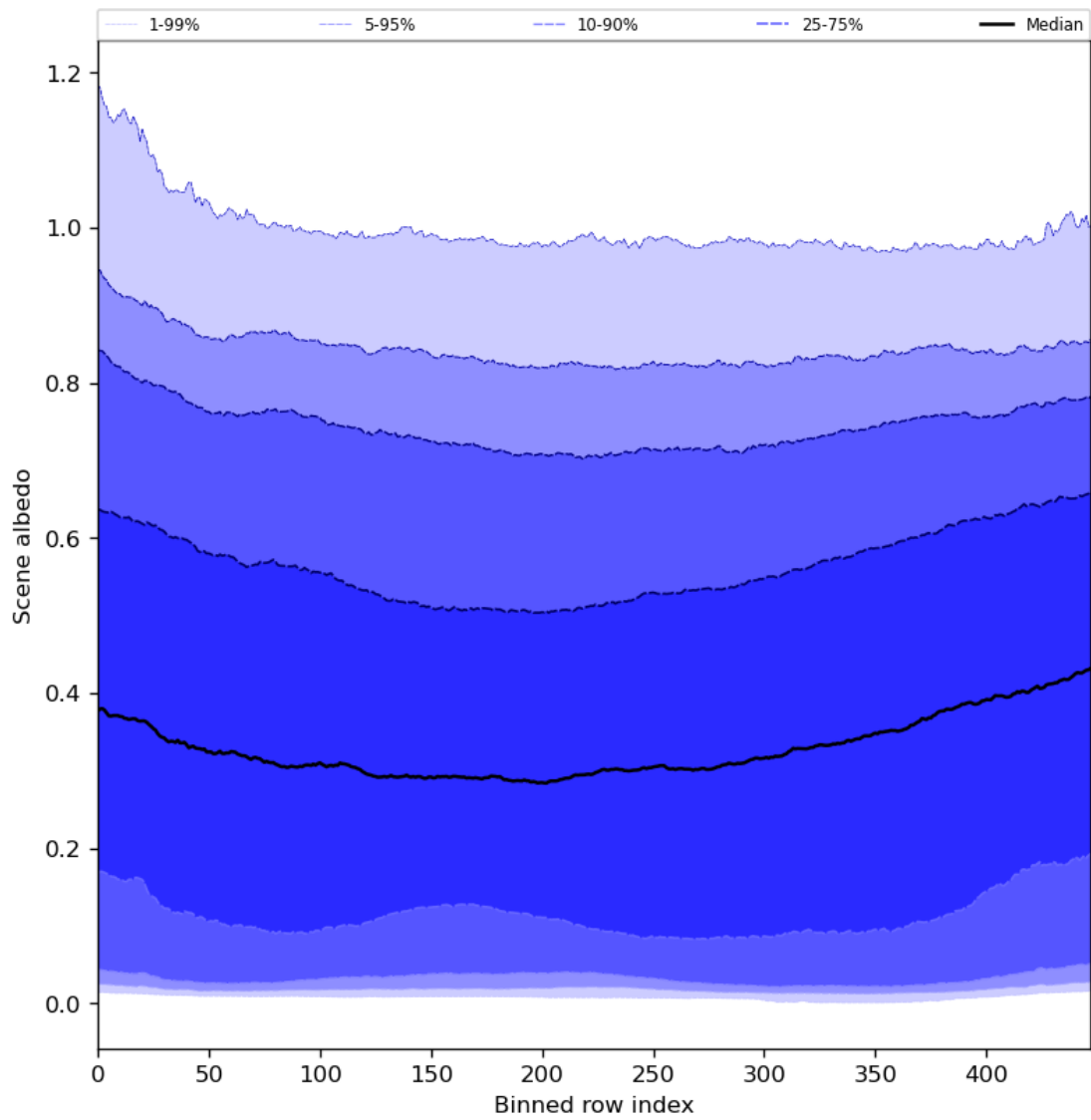
Figure 51: Along track statistics of “Scene albedo” for 2024-07-22 to 2024-07-24
