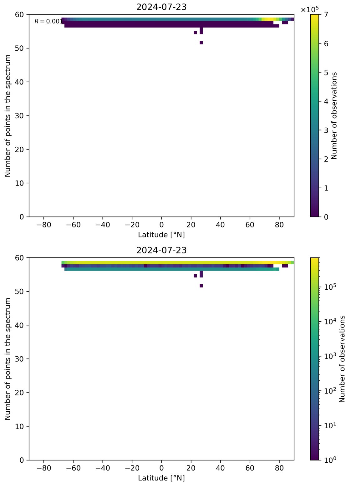
Figure 94: Scatter density plot of “Latitude” against “Number of points in the spectrum” for 2024-07-22 to 2024-07-24.
