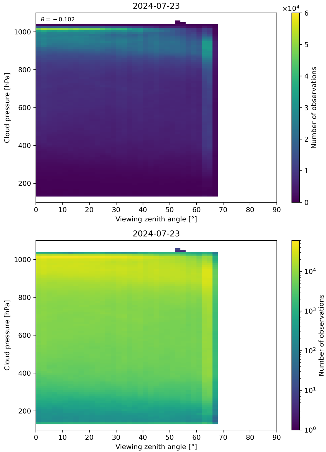
Figure 121: Scatter density plot of “Viewing zenith angle” against “Cloud pressure” for 2024-07-22 to 2024-07-24.
