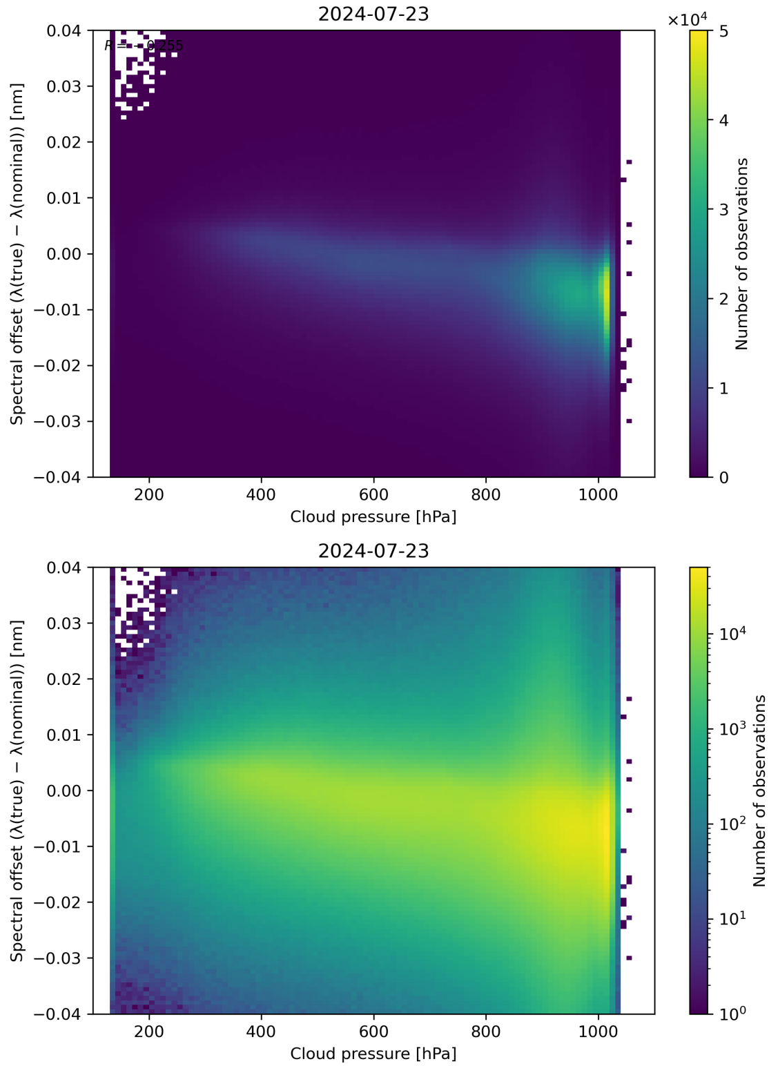
Figure 84: Scatter density plot of “Cloud pressure” against “Spectral offset ( \lambda(\text{true}) - \lambda(\text{nominal}) )” for 2024-07-22 to 2024-07-24.
