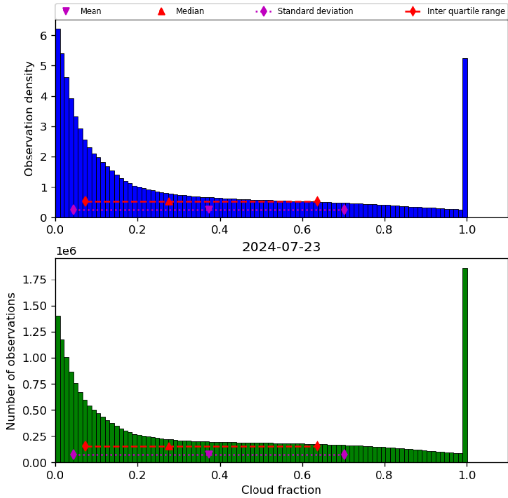
Figure 32: Histogram of “Cloud fraction” for 2024-07-22 to 2024-07-24
