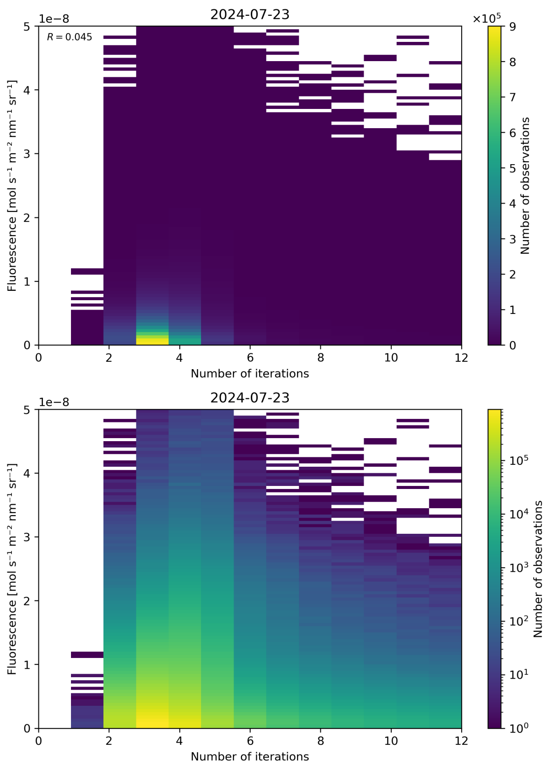
Figure 98: Scatter density plot of “Number of iterations” against “Fluorescence” for 2024-07-22 to 2024-07-24.
