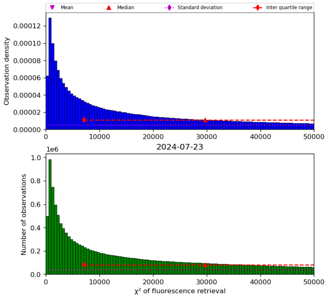
Figure 42: Histogram of “ \chi^2 of fluorescence retrieval” for 2024-07-22 to 2024-07-24
