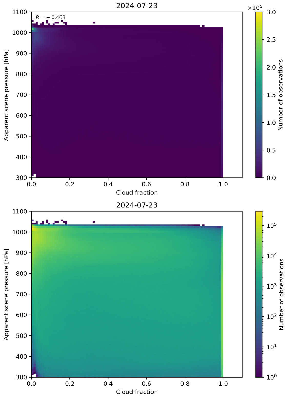
Figure 70: Scatter density plot of “Cloud fraction” against “Apparent scene pressure” for 2024-07-22 to 2024-07-24.
