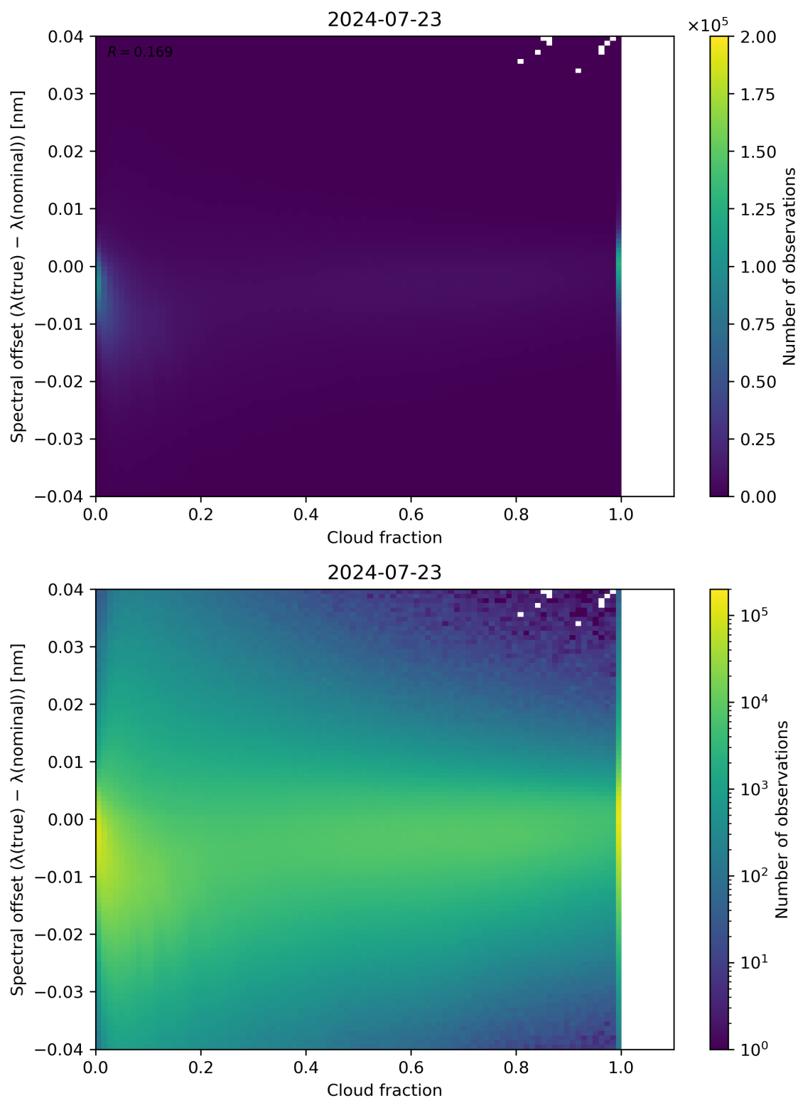
Figure 76: Scatter density plot of “Cloud fraction” against “Spectral offset ( \lambda(\text{true}) - \lambda(\text{nominal}) )” for 2024-07-22 to 2024-07-24.
