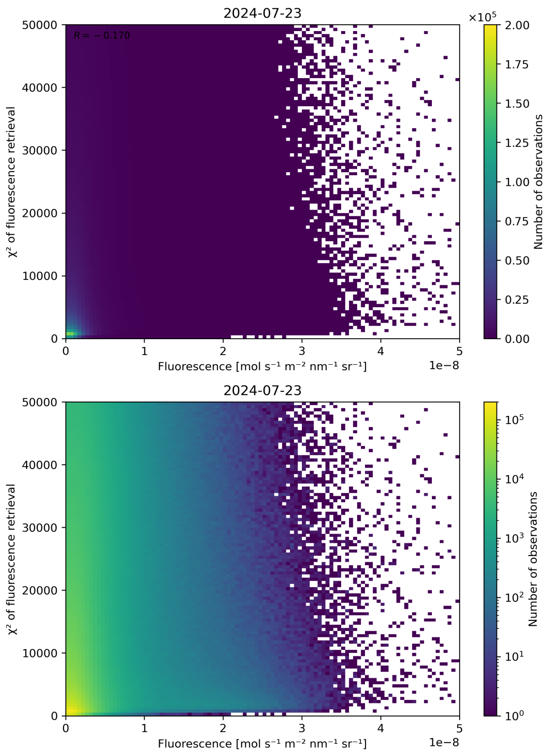
Figure 85: Scatter density plot of “Fluorescence” against “ \chi^2 of fluorescence retrieval” for 2024-07-22 to 2024-07-24.
