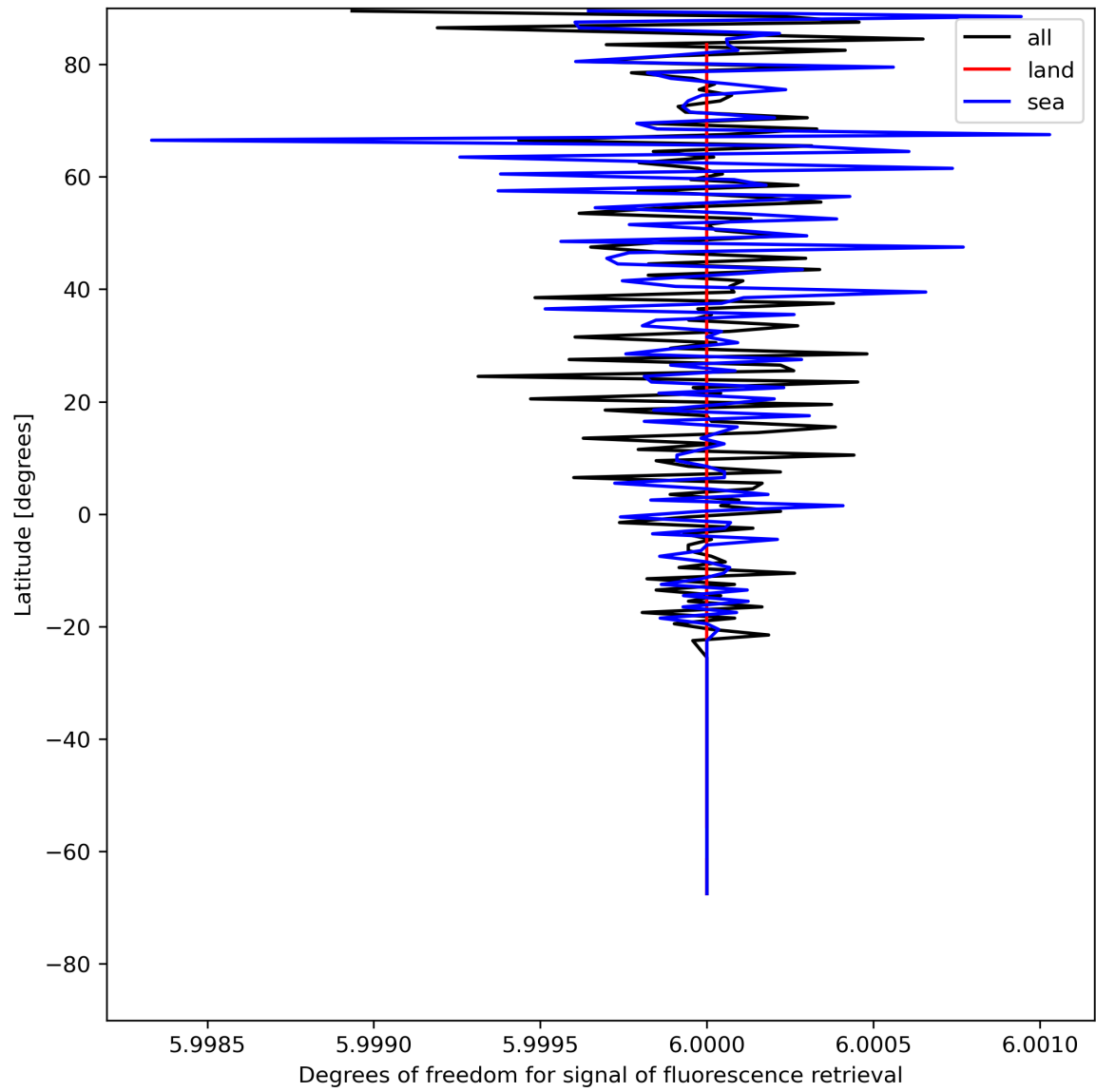
Figure 26: Zonal average of “Degrees of freedom for signal of fluorescence retrieval” for 2024-07-22 to 2024-07-24.
