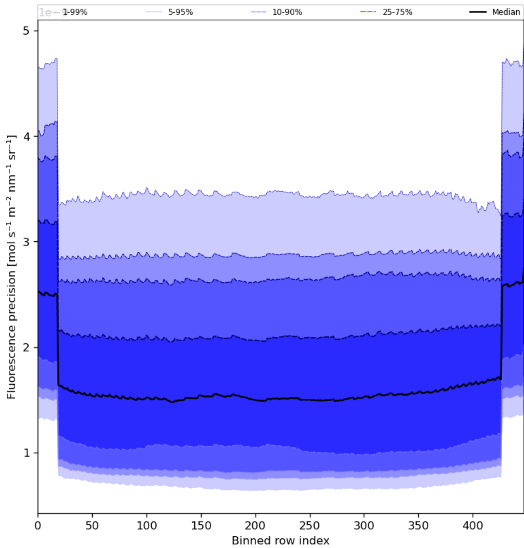
Figure 58: Along track statistics of “Fluorescence precision” for 2024-07-22 to 2024-07-24
