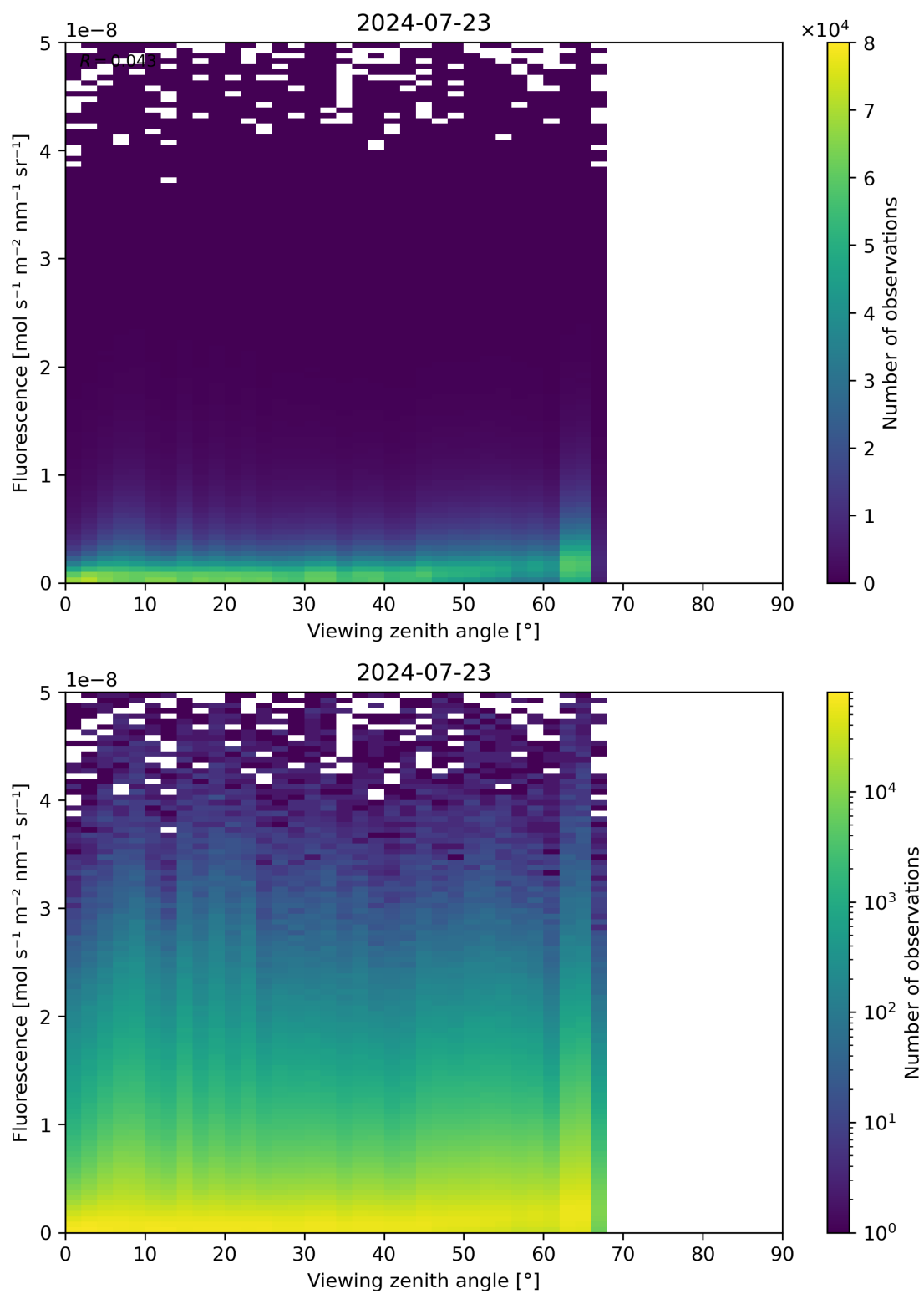
Figure 122: Scatter density plot of “Viewing zenith angle” against “Fluorescence” for 2024-07-22 to 2024-07-24.
