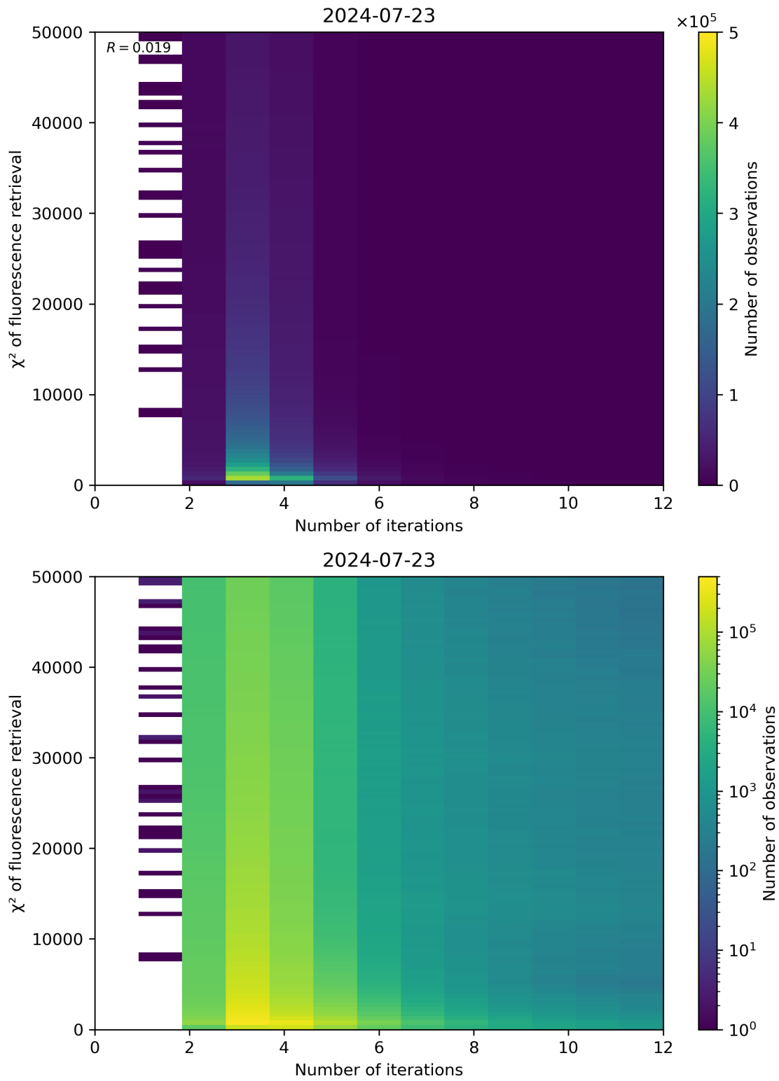
Figure 97: Scatter density plot of “Number of iterations” against “ \chi^2 of fluorescence retrieval” for 2024-07-22 to 2024-07-24.
