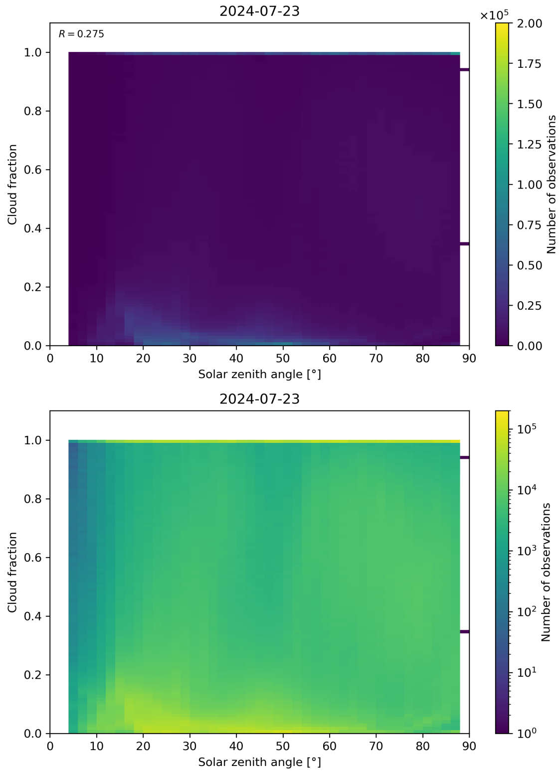
Figure 110: Scatter density plot of “Solar zenith angle” against “Cloud fraction” for 2024-07-22 to 2024-07-24.
