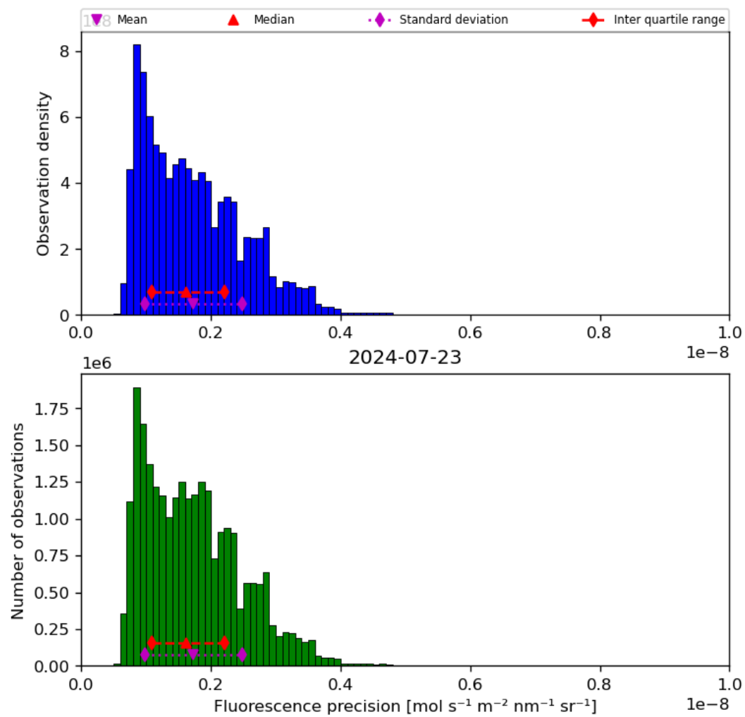
Figure 41: Histogram of “Fluorescence precision” for 2024-07-22 to 2024-07-24
