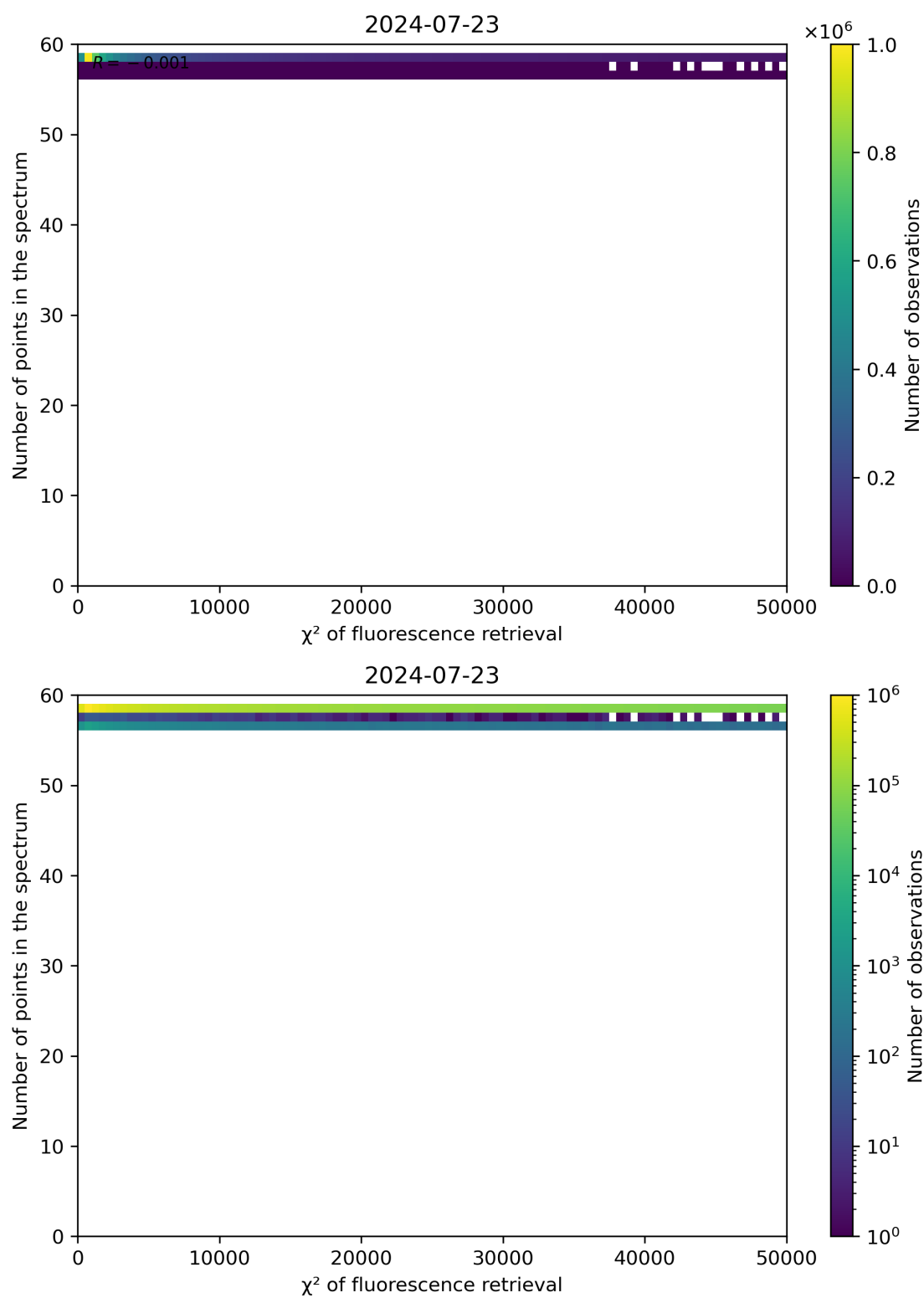
Figure 68: Scatter density plot of “ \chi^2 of fluorescence retrieval” against “Number of points in the spectrum” for 2024-07-22 to 2024-07-24.
