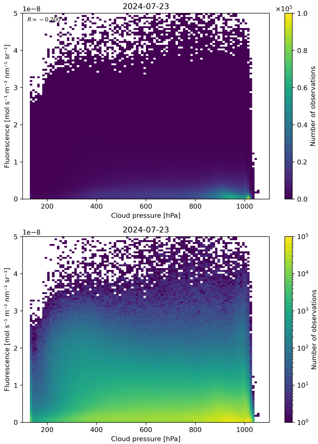
Figure 80: Scatter density plot of “Cloud pressure” against “Fluorescence” for 2024-07-22 to 2024-07-24.
