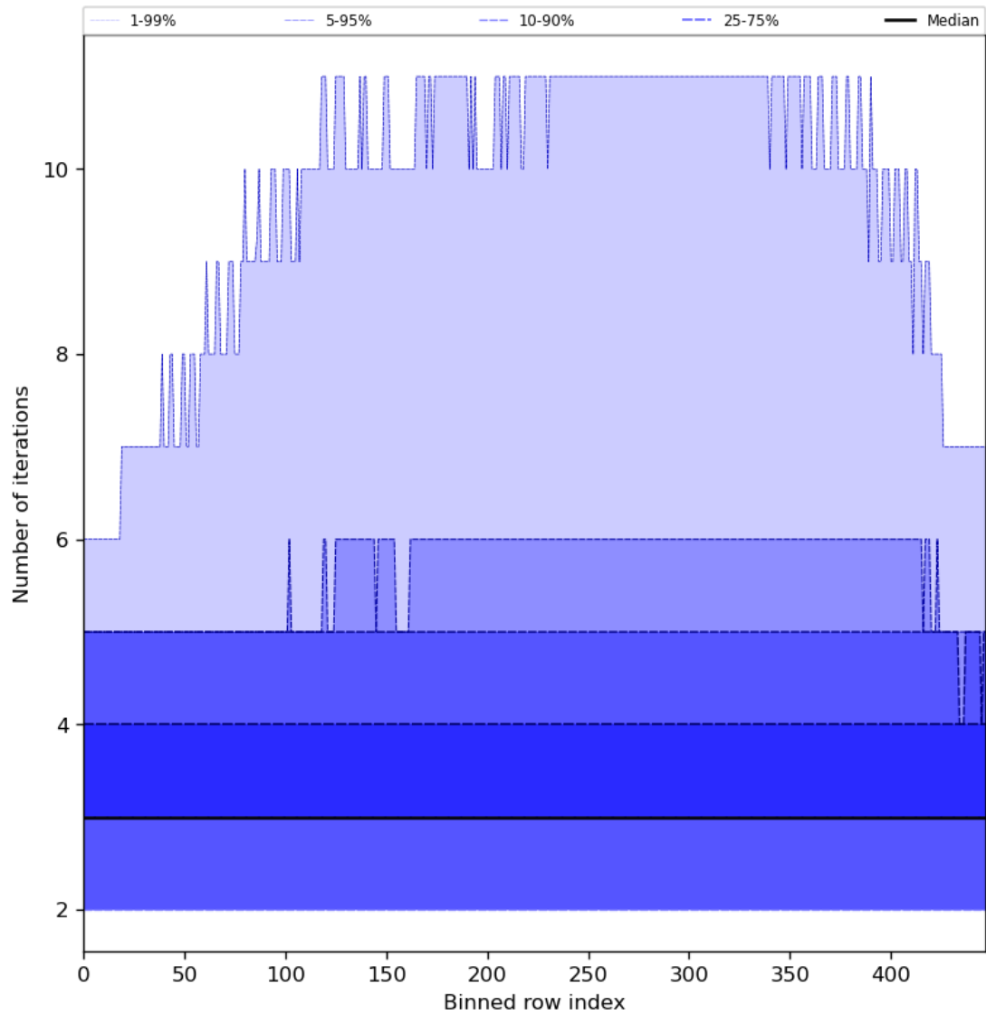
Figure 56: Along track statistics of “Number of iterations” for 2024-07-22 to 2024-07-24
