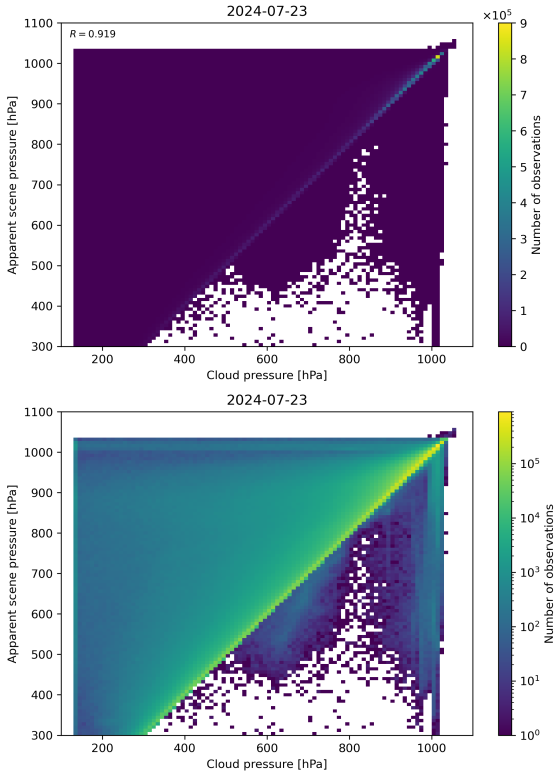
Figure 77: Scatter density plot of “Cloud pressure” against “Apparent scene pressure” for 2024-07-22 to 2024-07-24.
