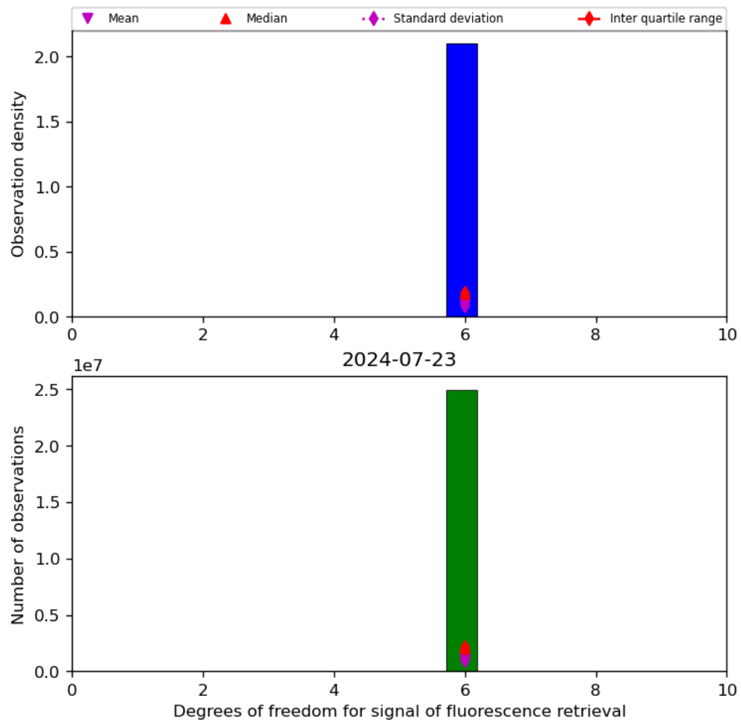
Figure 43: Histogram of “Degrees of freedom for signal of fluorescence retrieval” for 2024-07-22 to 2024-07-24
