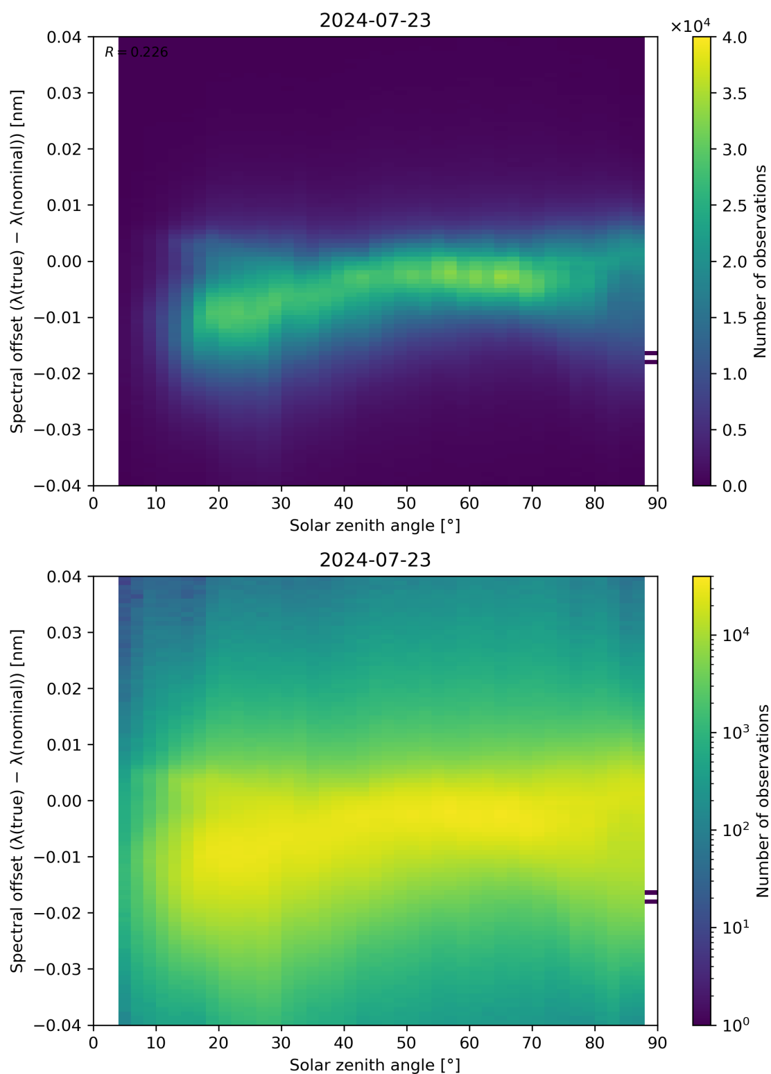
Figure 117: Scatter density plot of “Solar zenith angle” against “Spectral offset ( \lambda(\text{true}) - \lambda(\text{nominal}) )” for 2024-07-22 to 2024-07-24.
