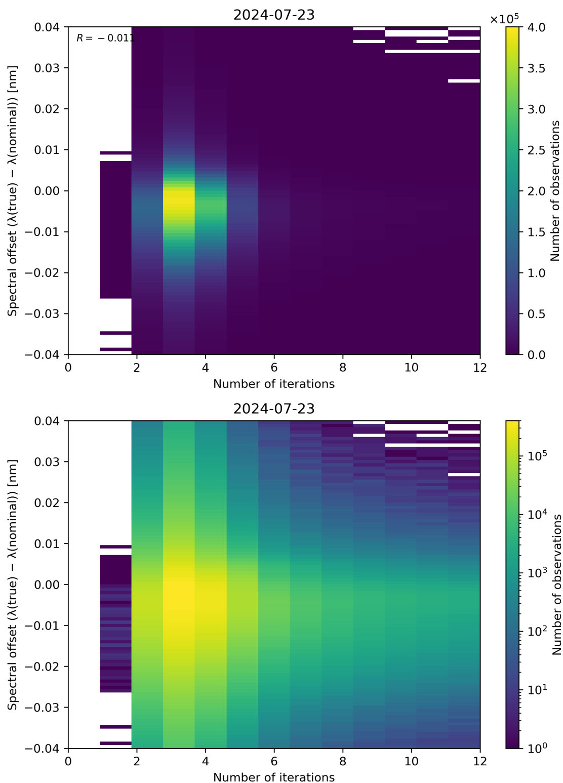
Figure 100: Scatter density plot of “Number of iterations” against “Spectral offset ( \lambda(\text{true}) - \lambda(\text{nominal}) )” for 2024-07-22 to 2024-07-24.
