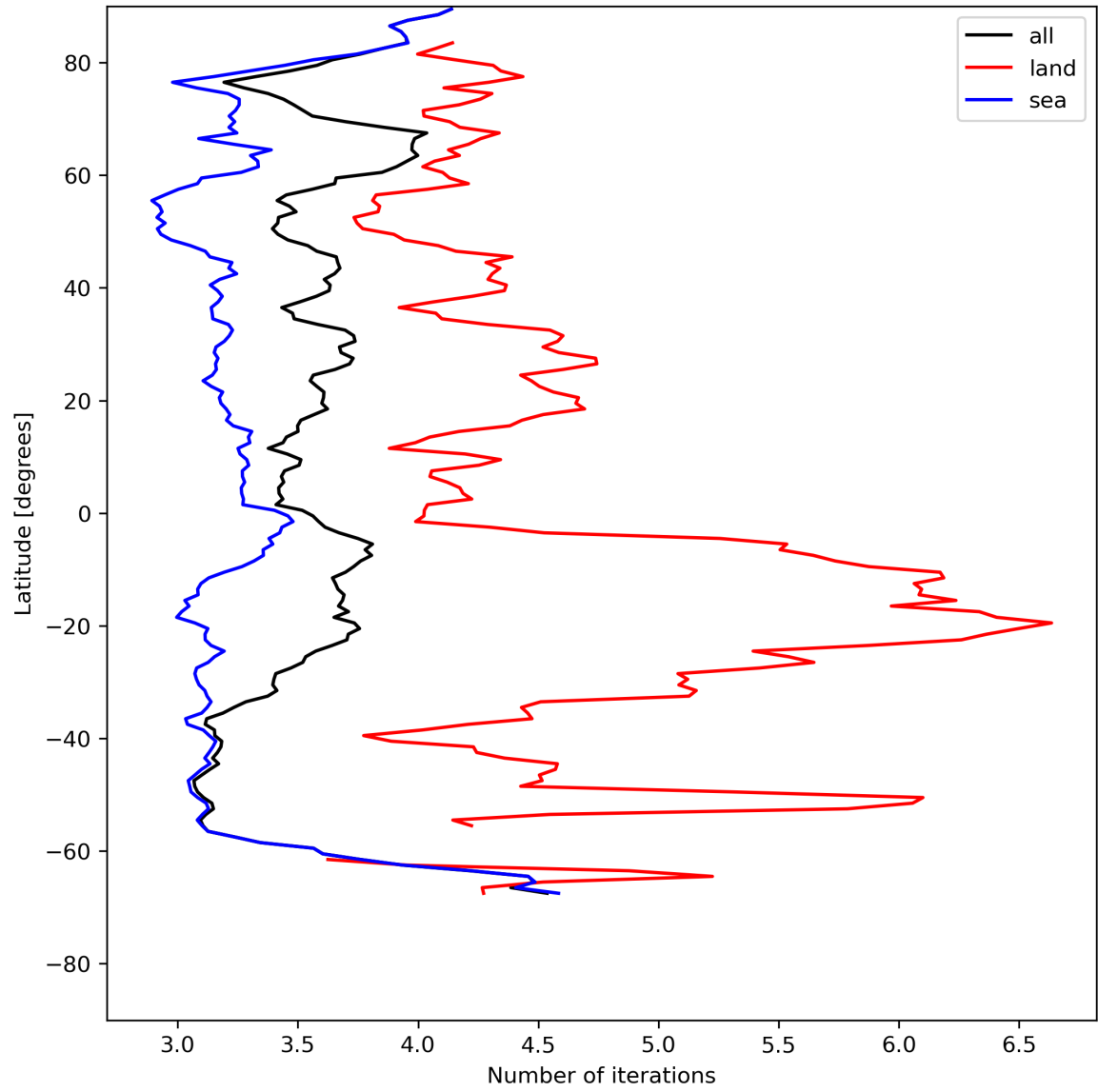
Figure 22: Zonal average of “Number of iterations” for 2024-07-22 to 2024-07-24.
