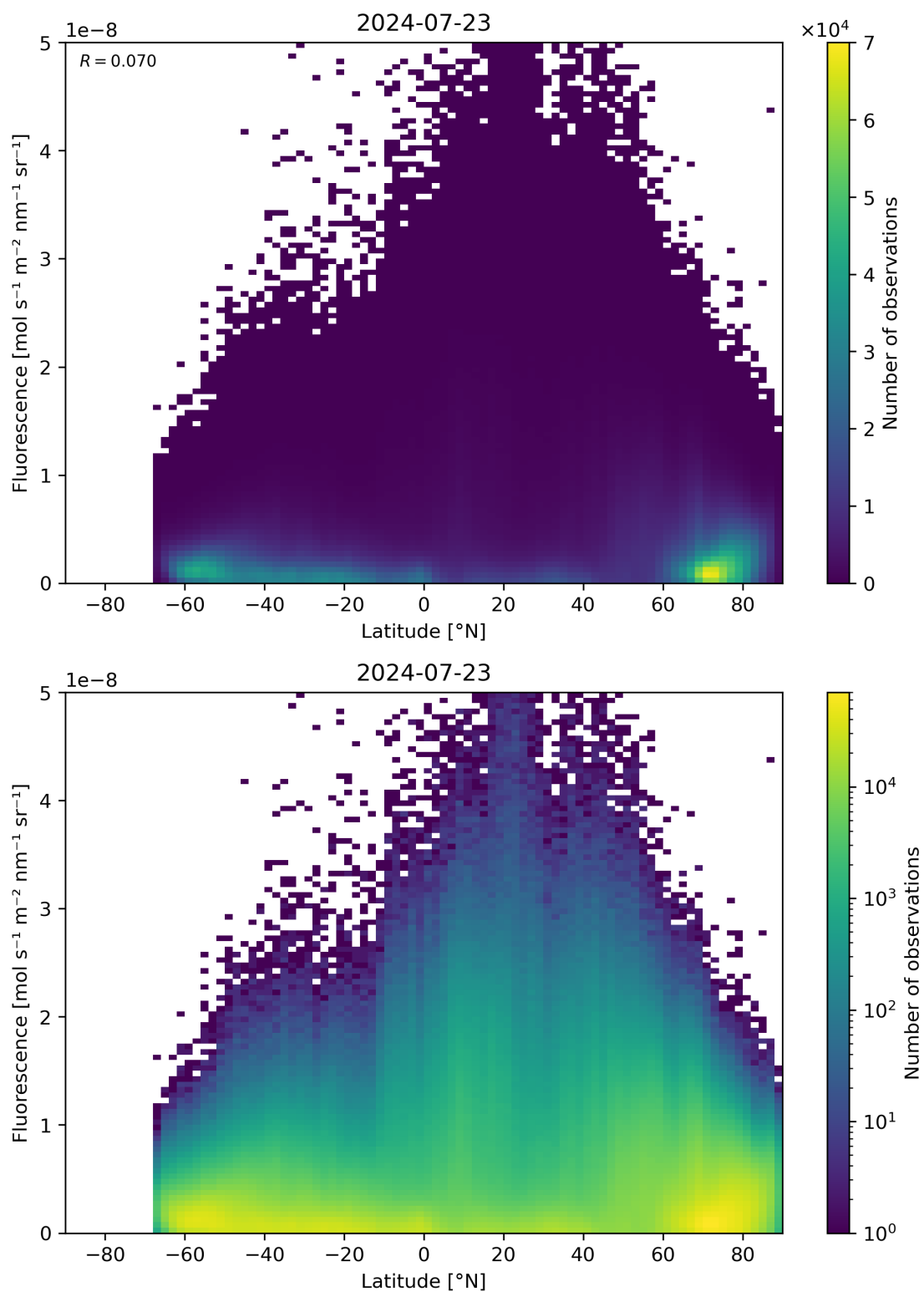
Figure 92: Scatter density plot of “Latitude” against “Fluorescence” for 2024-07-22 to 2024-07-24.
