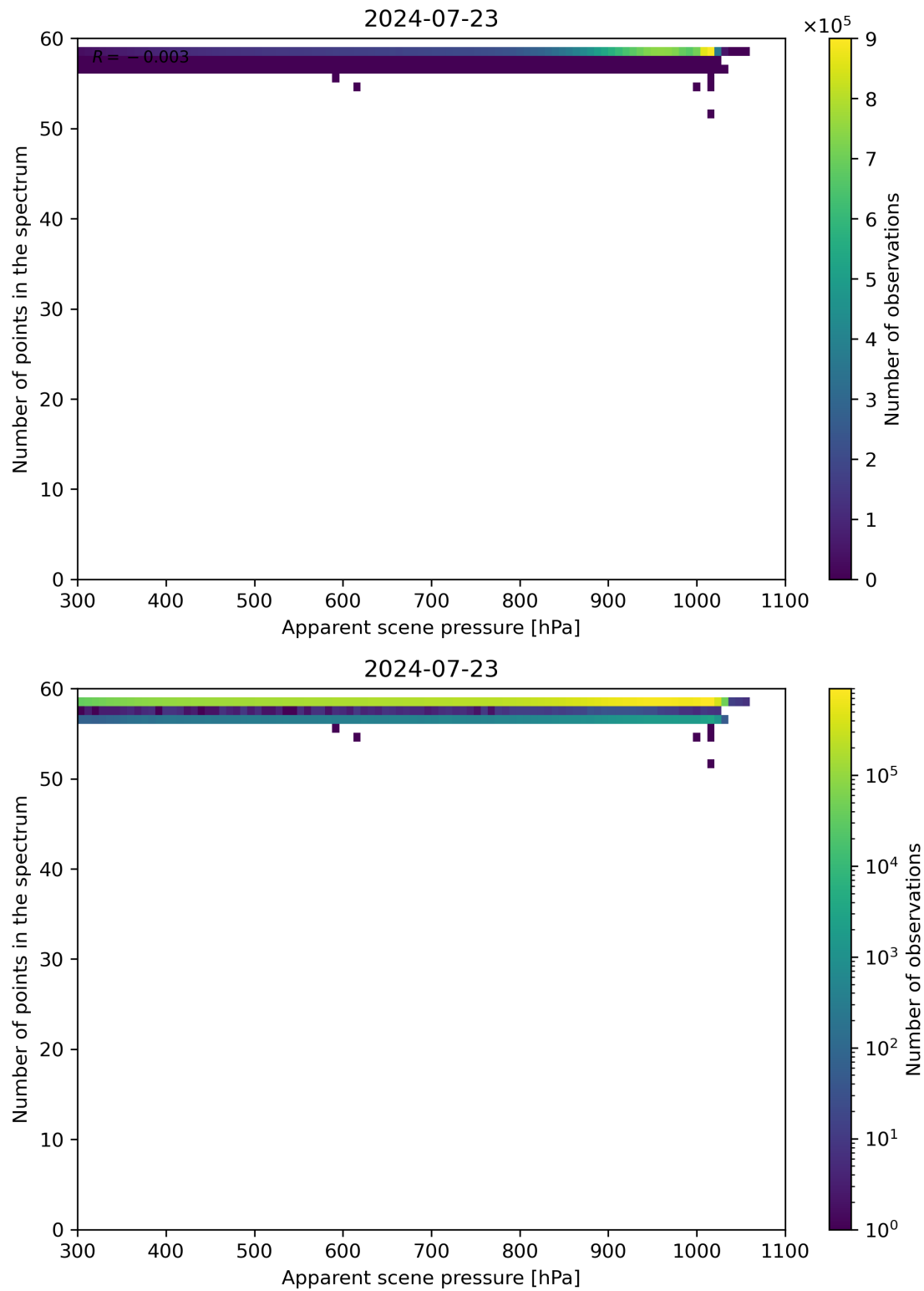
Figure 66: Scatter density plot of “Apparent scene pressure” against “Number of points in the spectrum” for 2024-07-22 to 2024-07-24.
