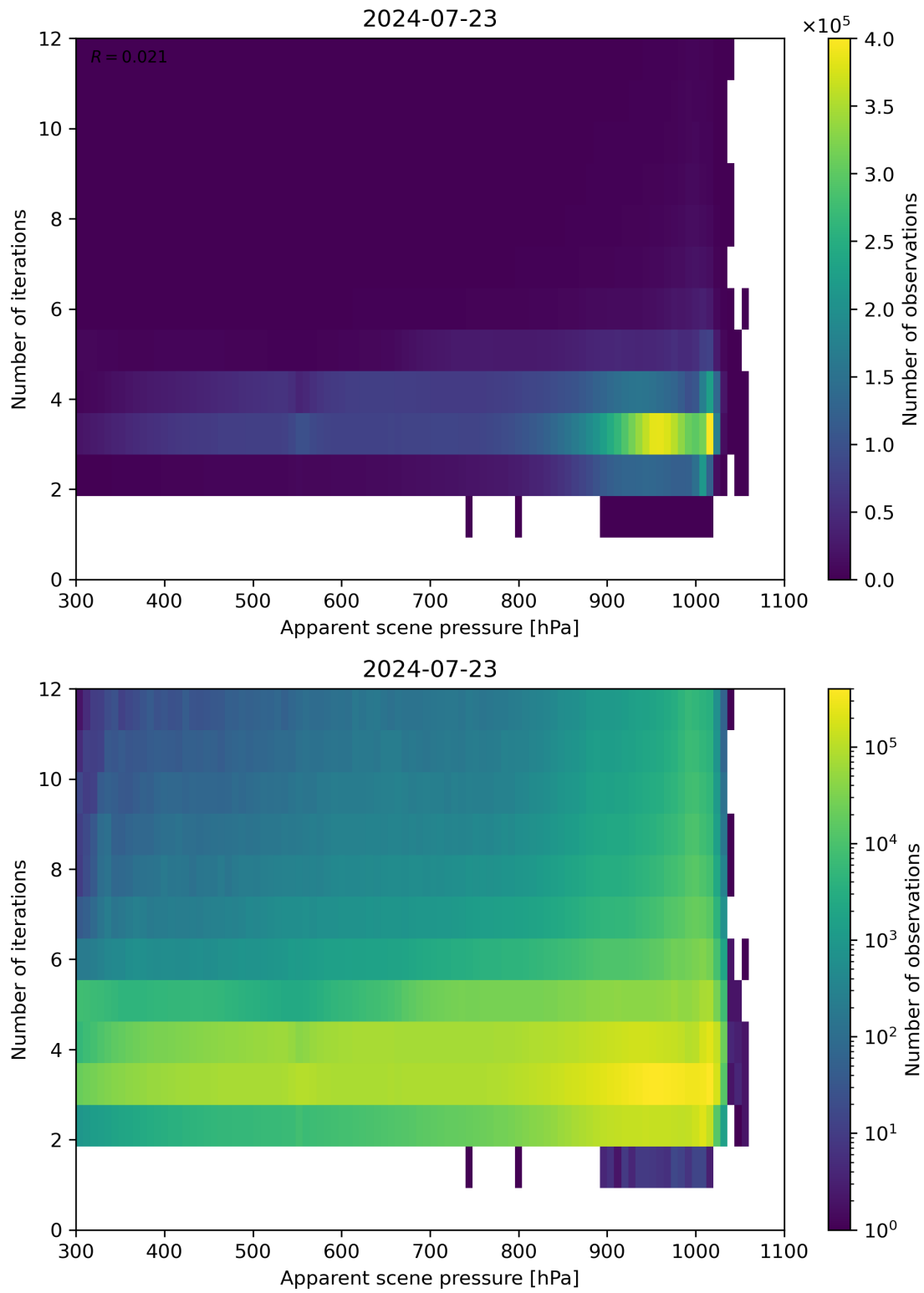
Figure 65: Scatter density plot of “Apparent scene pressure” against “Number of iterations” for 2024-07-22 to 2024-07-24.
