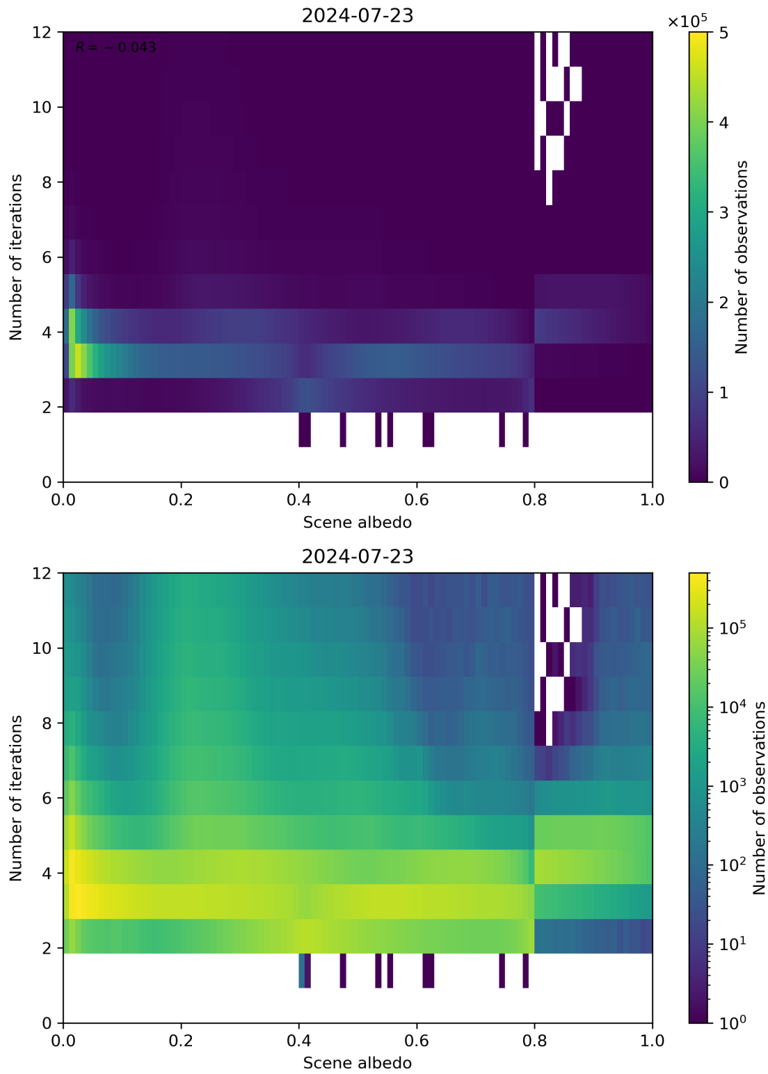
Figure 105: Scatter density plot of “Scene albedo” against “Number of iterations” for 2024-07-22 to 2024-07-24.
