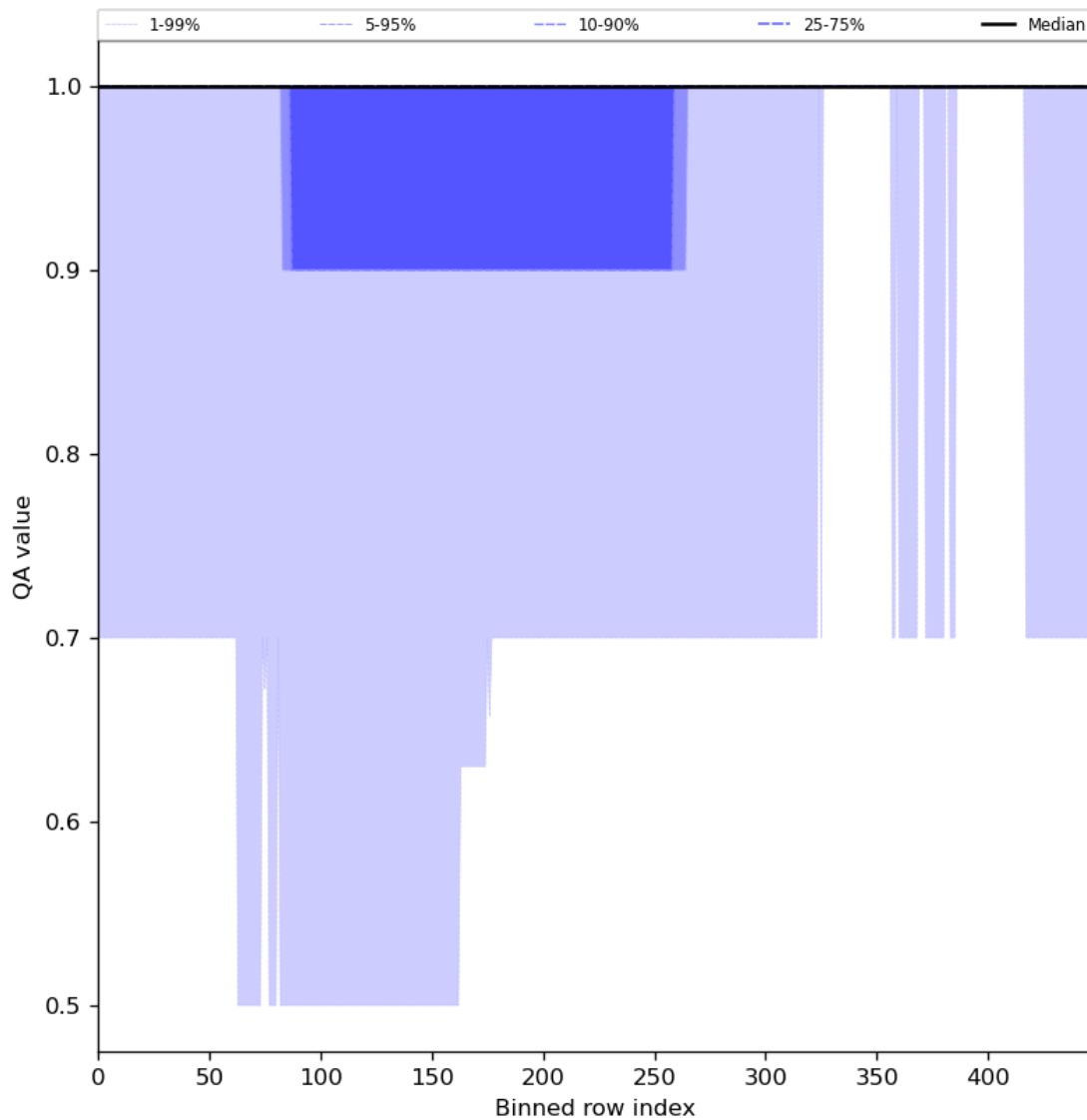
Figure 46: Along track statistics of “QA value” for 2024-07-22 to 2024-07-24
