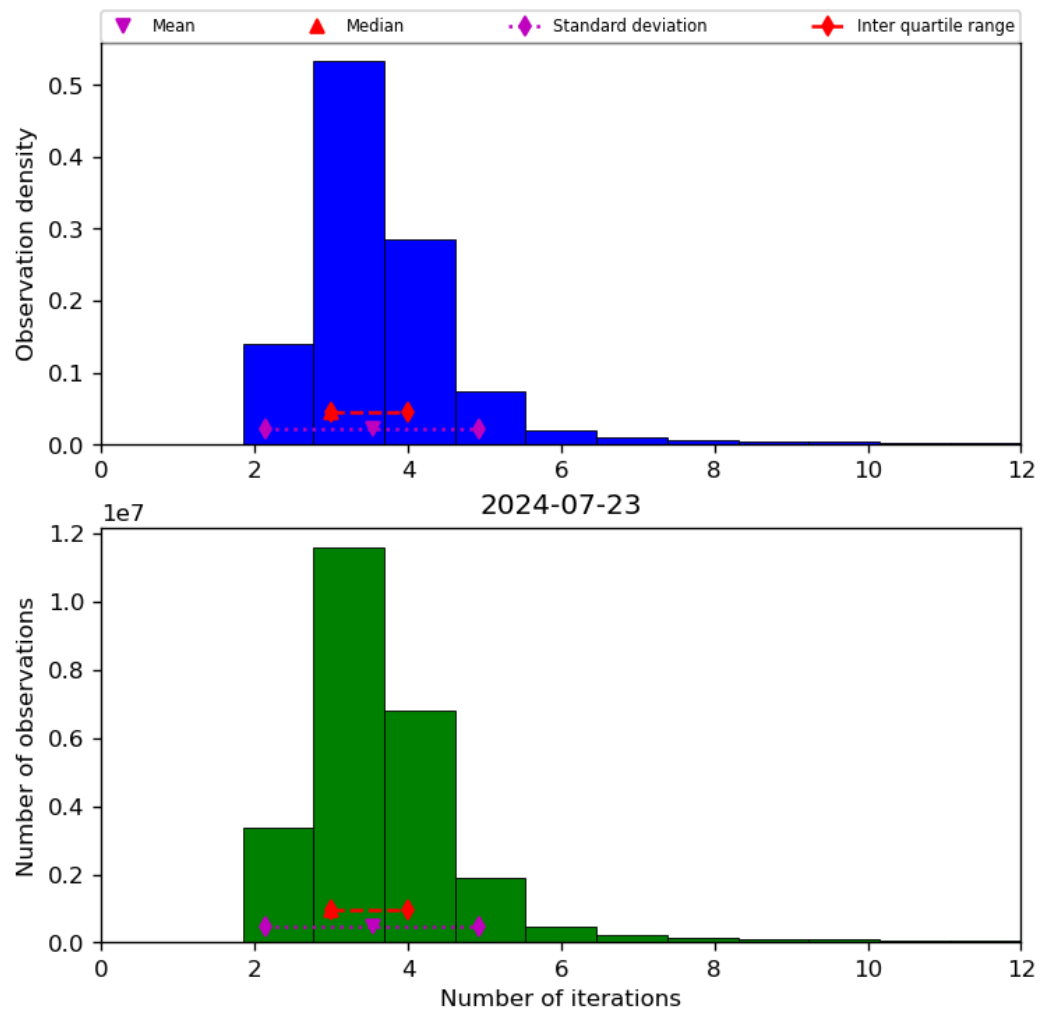
Figure 39: Histogram of “Number of iterations” for 2024-07-22 to 2024-07-24
