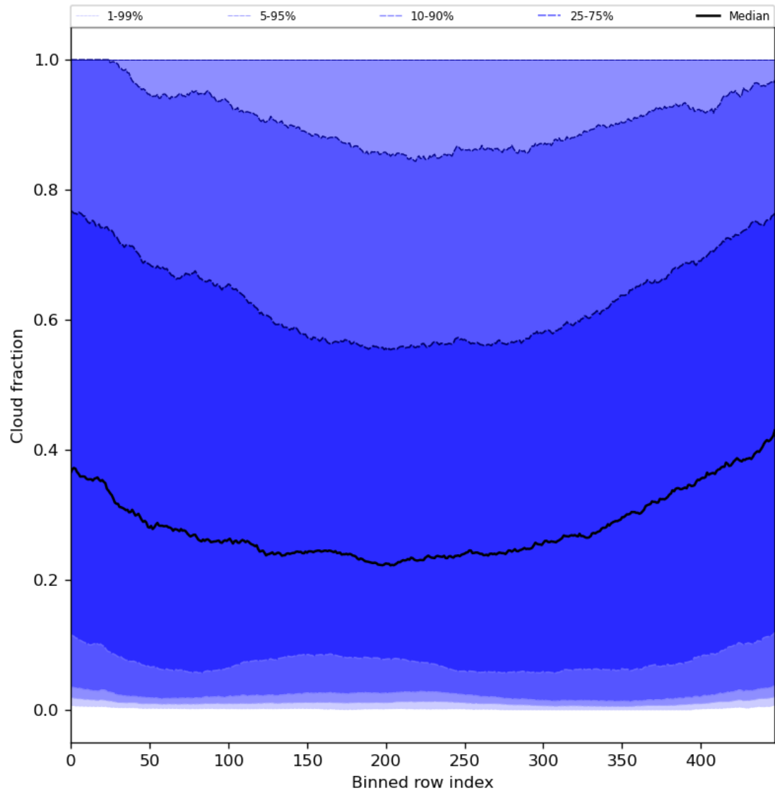
Figure 49: Along track statistics of “Cloud fraction” for 2024-07-22 to 2024-07-24
