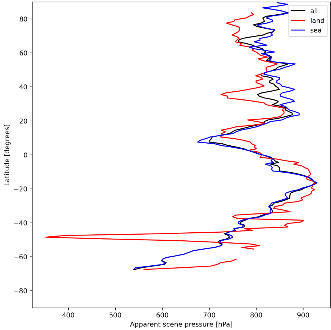
Figure 19: Zonal average of “Apparent scene pressure” for 2024-07-22 to 2024-07-24.
