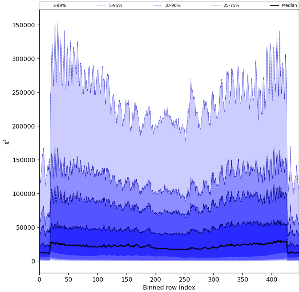
Figure 55: Along track statistics of “ \chi^2 ” for 2024-07-22 to 2024-07-24
