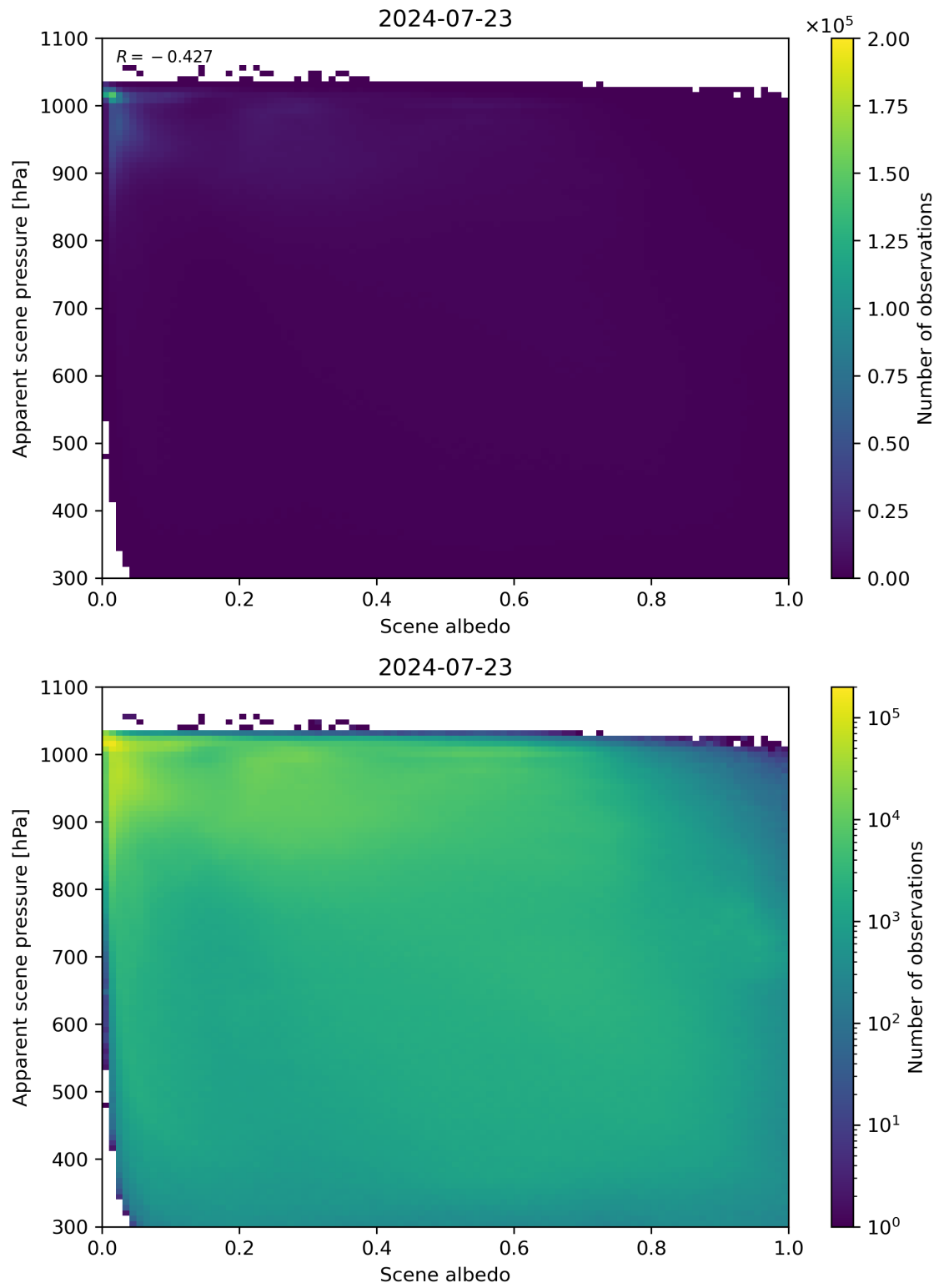
Figure 102: Scatter density plot of “Scene albedo” against “Apparent scene pressure” for 2024-07-22 to 2024-07-24.
