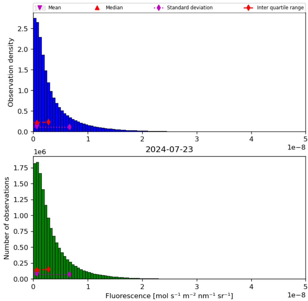
Figure 40: Histogram of “Fluorescence” for 2024-07-22 to 2024-07-24
