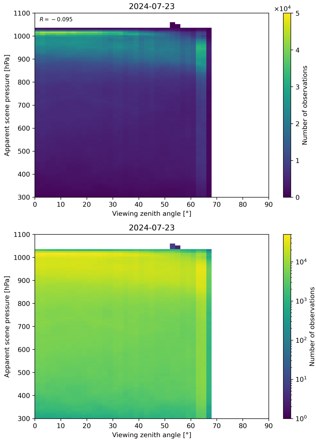
Figure 118: Scatter density plot of “Viewing zenith angle” against “Apparent scene pressure” for 2024-07-22 to 2024-07-24.
