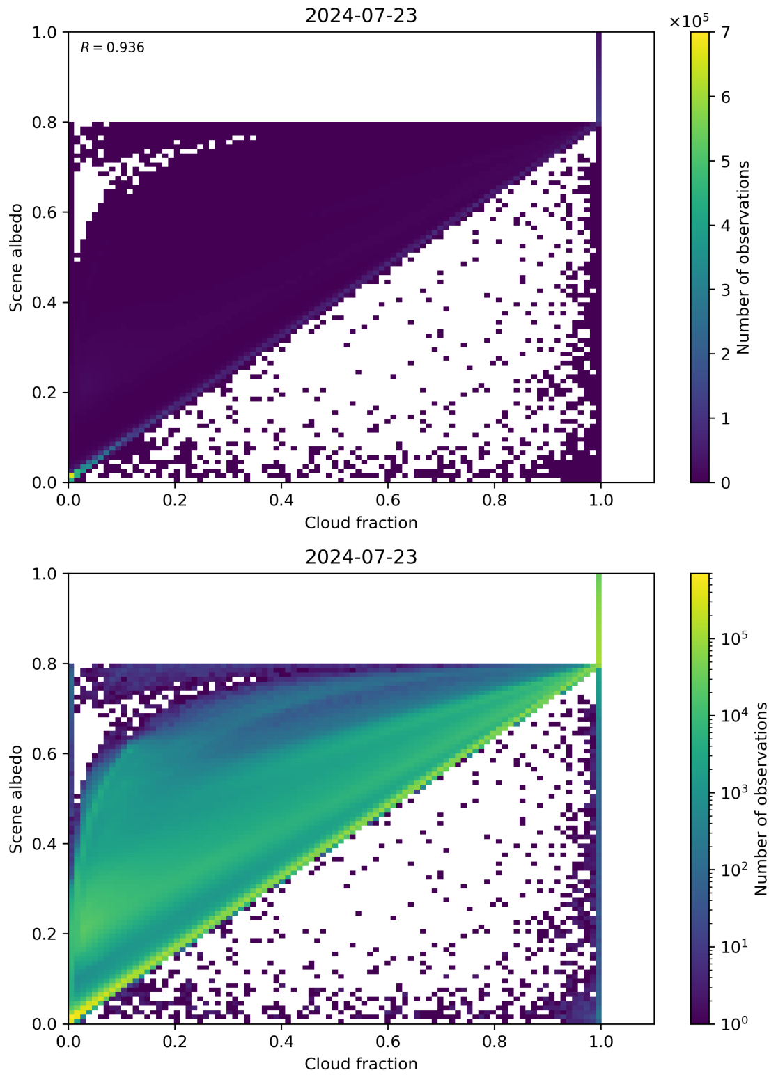
Figure 75: Scatter density plot of “Cloud fraction” against “Scene albedo” for 2024-07-22 to 2024-07-24.
