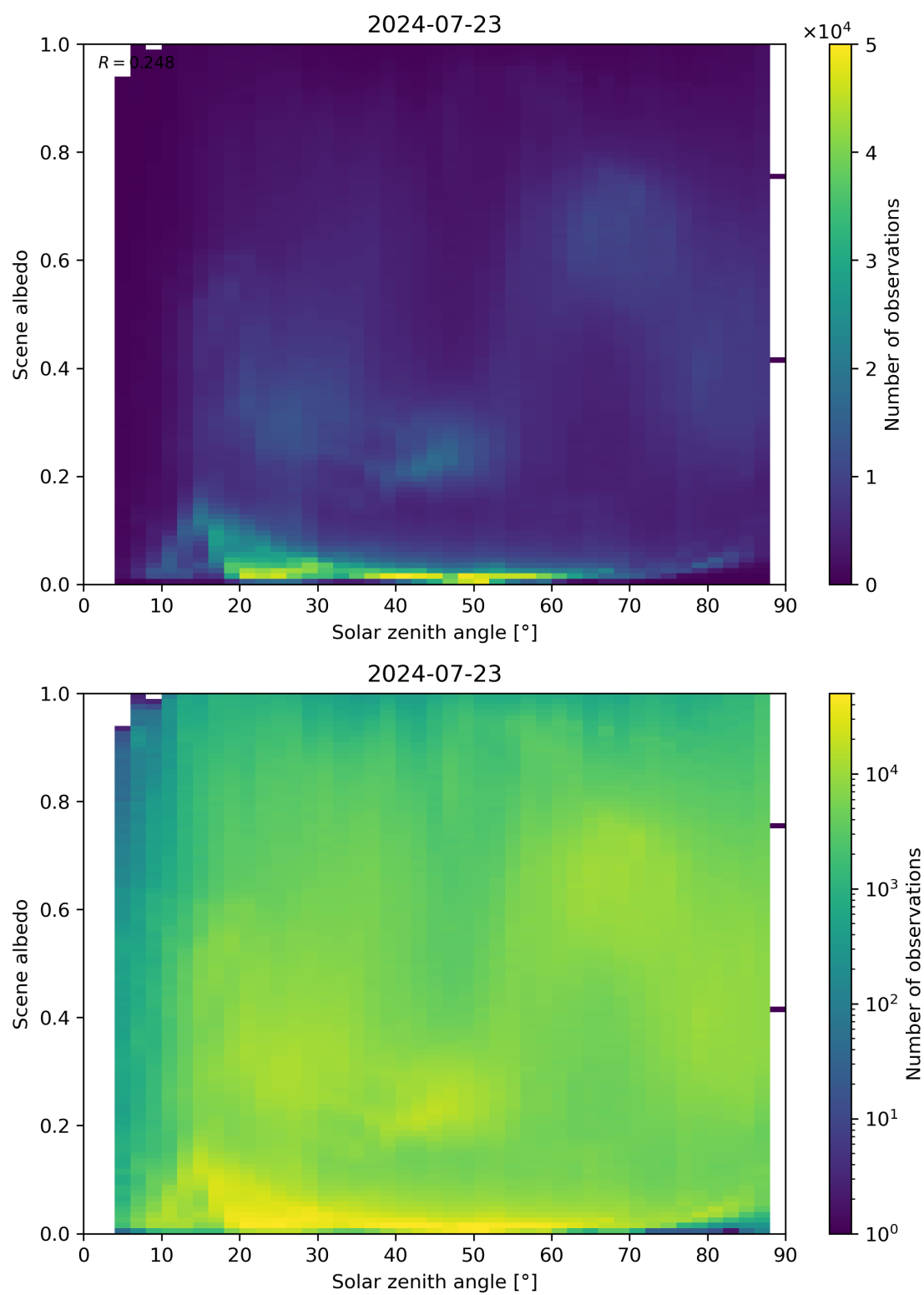
Figure 116: Scatter density plot of “Solar zenith angle” against “Scene albedo” for 2024-07-22 to 2024-07-24.
