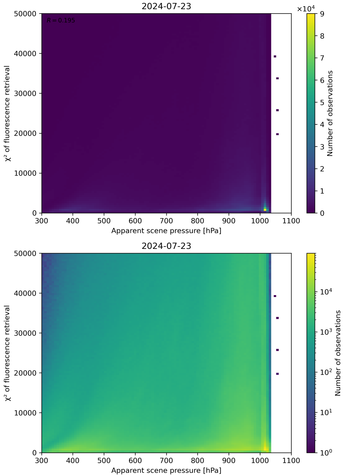
Figure 63: Scatter density plot of “Apparent scene pressure” against “ \chi^2 of fluorescence retrieval” for 2024-07-22 to 2024-07-24.
