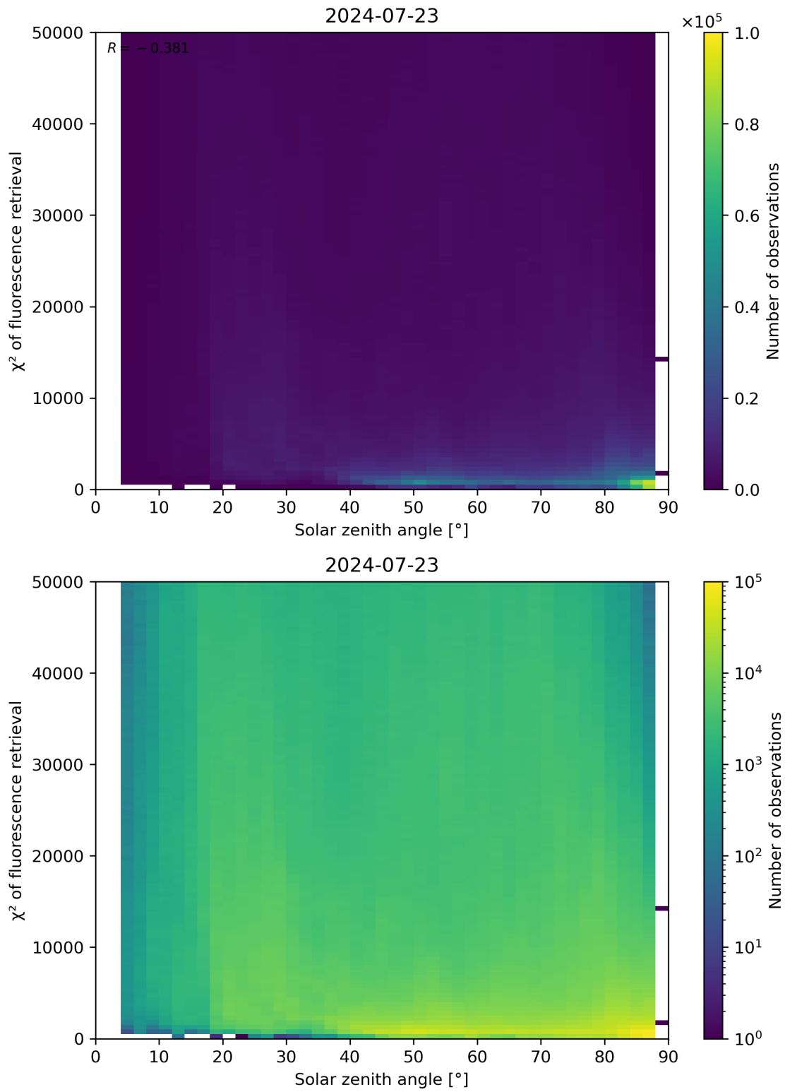
Figure 109: Scatter density plot of “Solar zenith angle” against “ \chi^2 of fluorescence retrieval” for 2024-07-22 to 2024-07-24.
