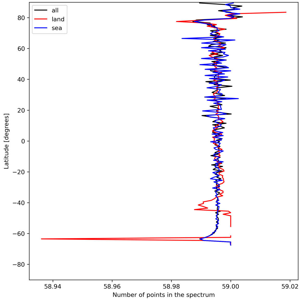
Figure 27: Zonal average of “Number of points in the spectrum” for 2024-07-22 to 2024-07-24.
