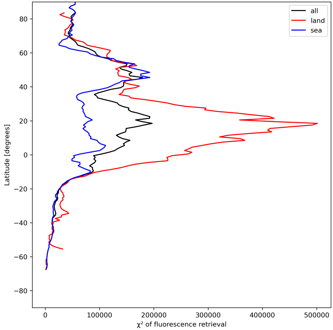
Figure 25: Zonal average of “ \chi^2 of fluorescence retrieval” for 2024-07-22 to 2024-07-24.
