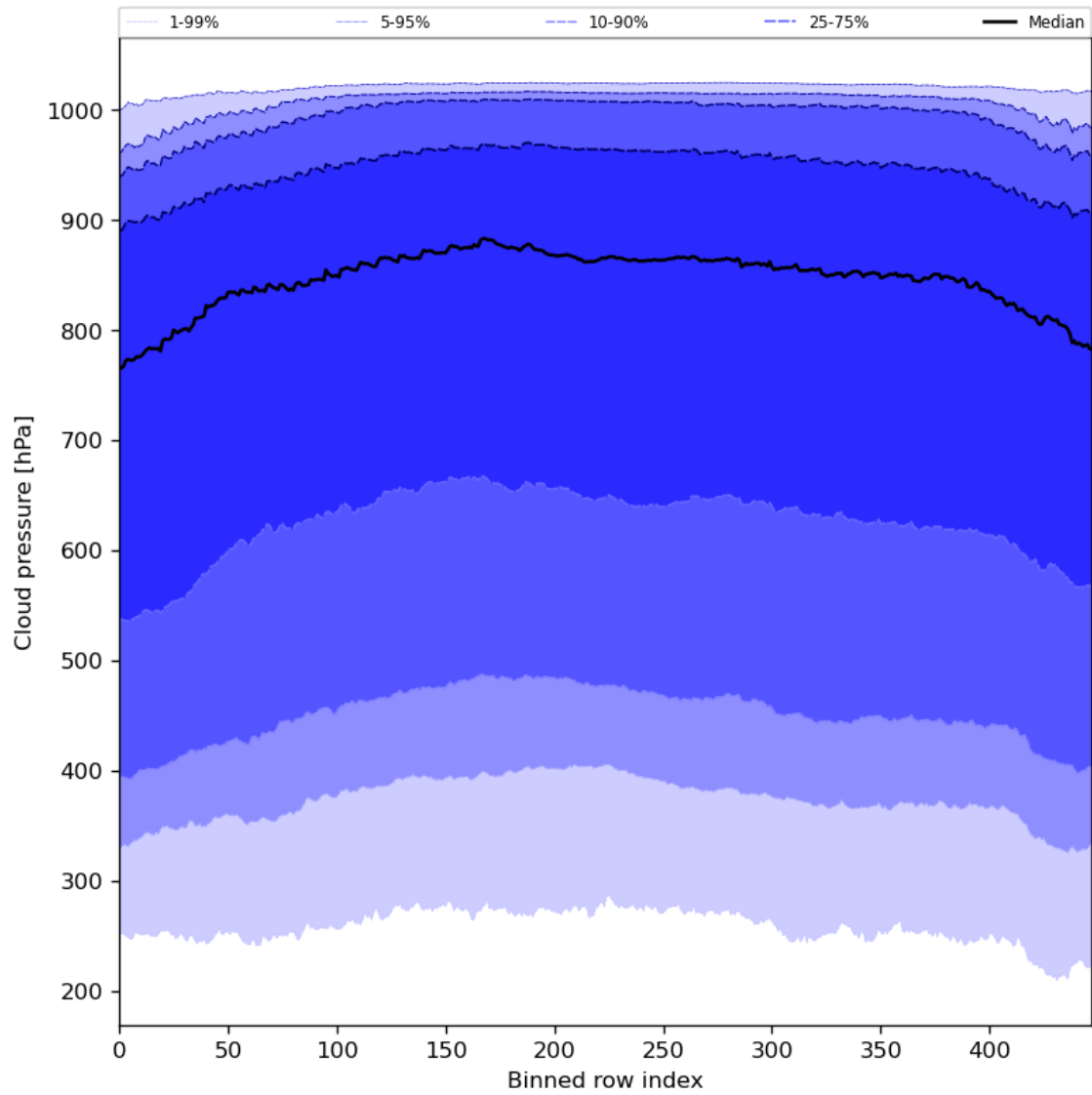
Figure 47: Along track statistics of “Cloud pressure” for 2024-07-22 to 2024-07-24
