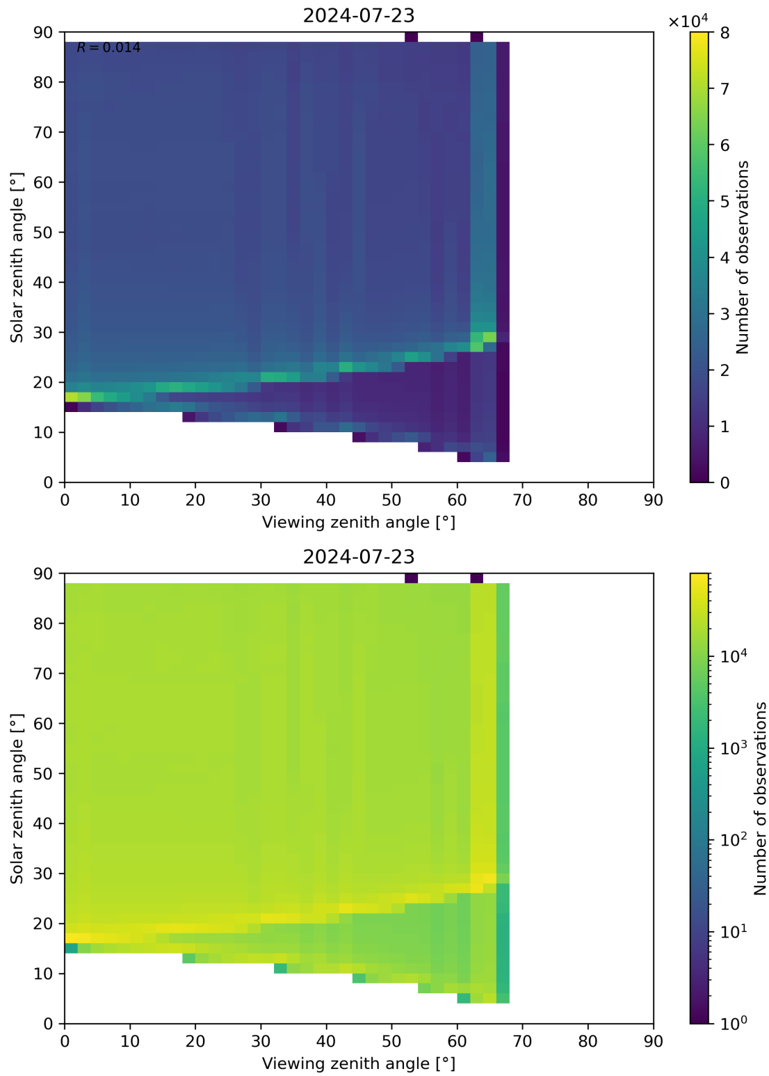
Figure 127: Scatter density plot of “Viewing zenith angle” against “Solar zenith angle” for 2024-07-22 to 2024-07-24.
