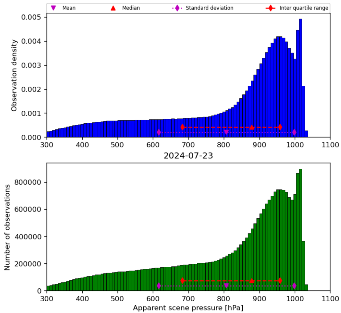
Figure 36: Histogram of “Apparent scene pressure” for 2024-07-22 to 2024-07-24
