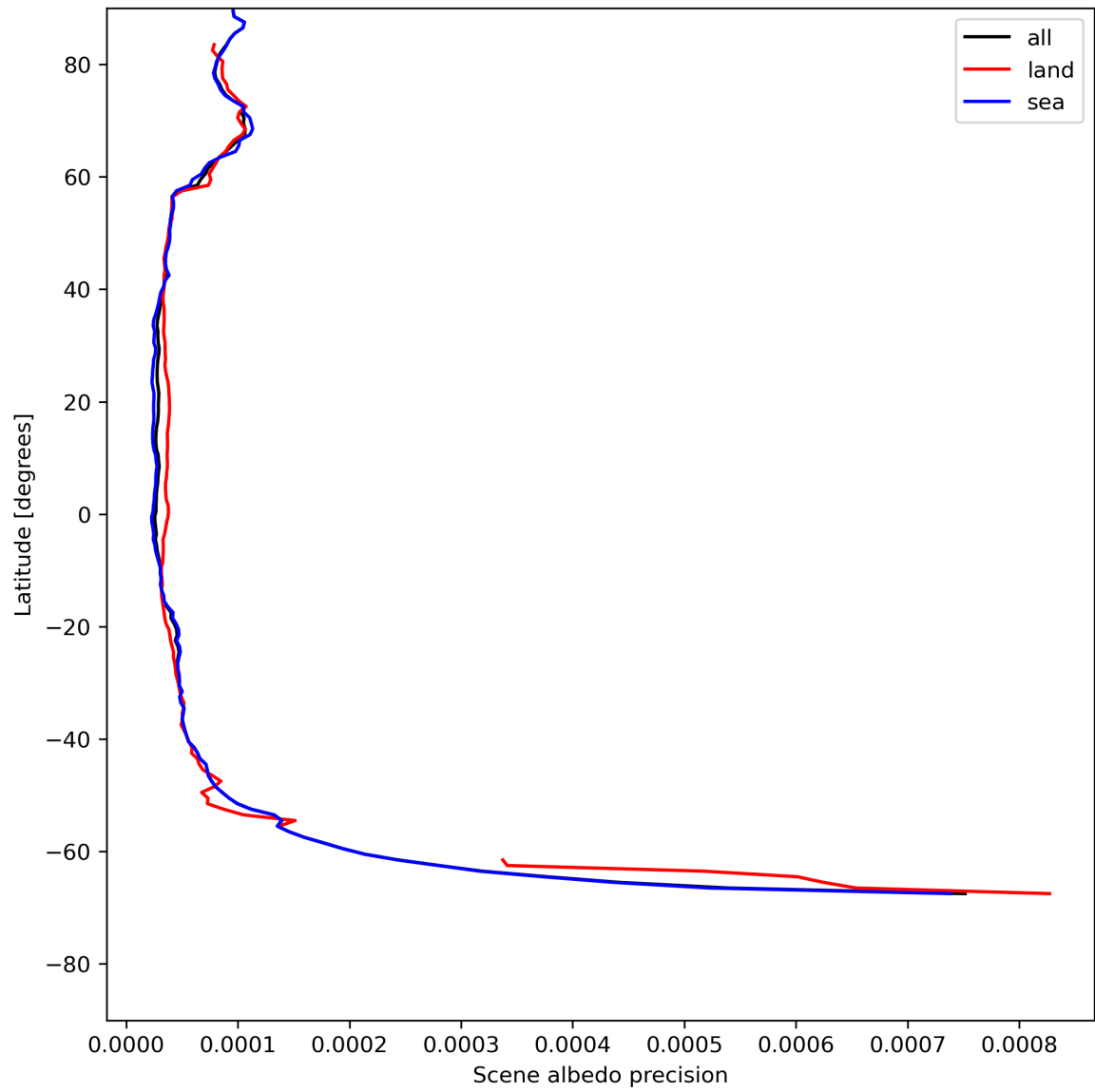
Figure 18: Zonal average of “Scene albedo precision” for 2024-07-22 to 2024-07-24.
