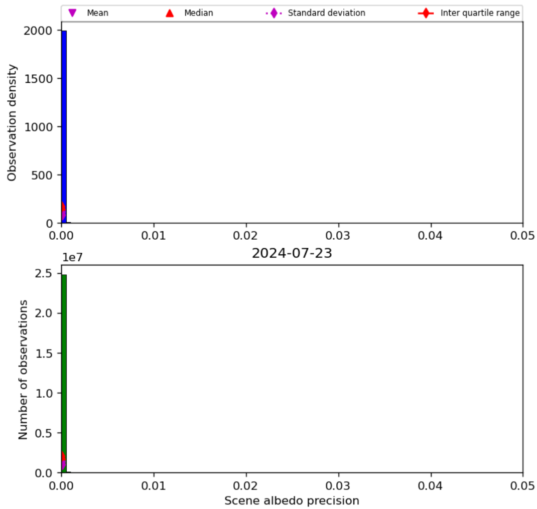
Figure 35: Histogram of “Scene albedo precision” for 2024-07-22 to 2024-07-24
