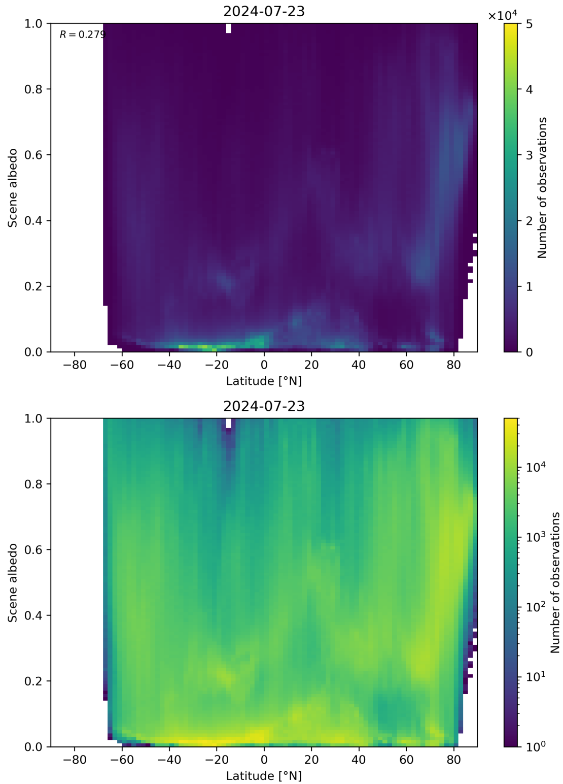
Figure 95: Scatter density plot of “Latitude” against “Scene albedo” for 2024-07-22 to 2024-07-24.
