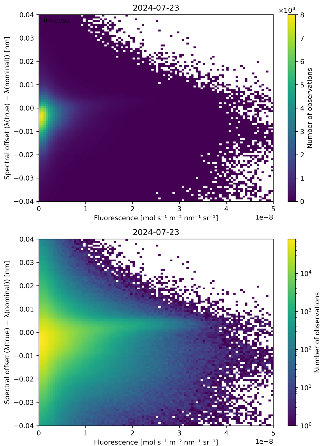
Figure 87: Scatter density plot of “Fluorescence” against “Spectral offset ( \lambda(\text{true}) - \lambda(\text{nominal}) )” for 2024-07-22 to 2024-07-24.
