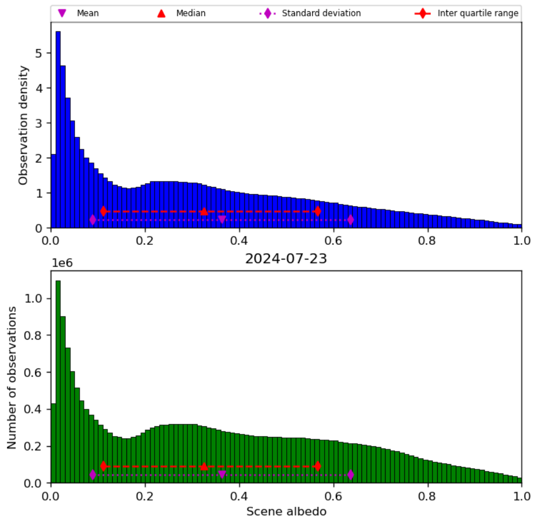
Figure 34: Histogram of “Scene albedo” for 2024-07-22 to 2024-07-24
