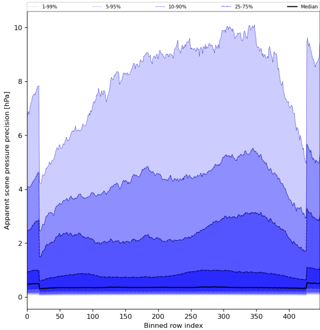
Figure 54: Along track statistics of “Apparent scene pressure precision” for 2024-07-22 to 2024-07-24
