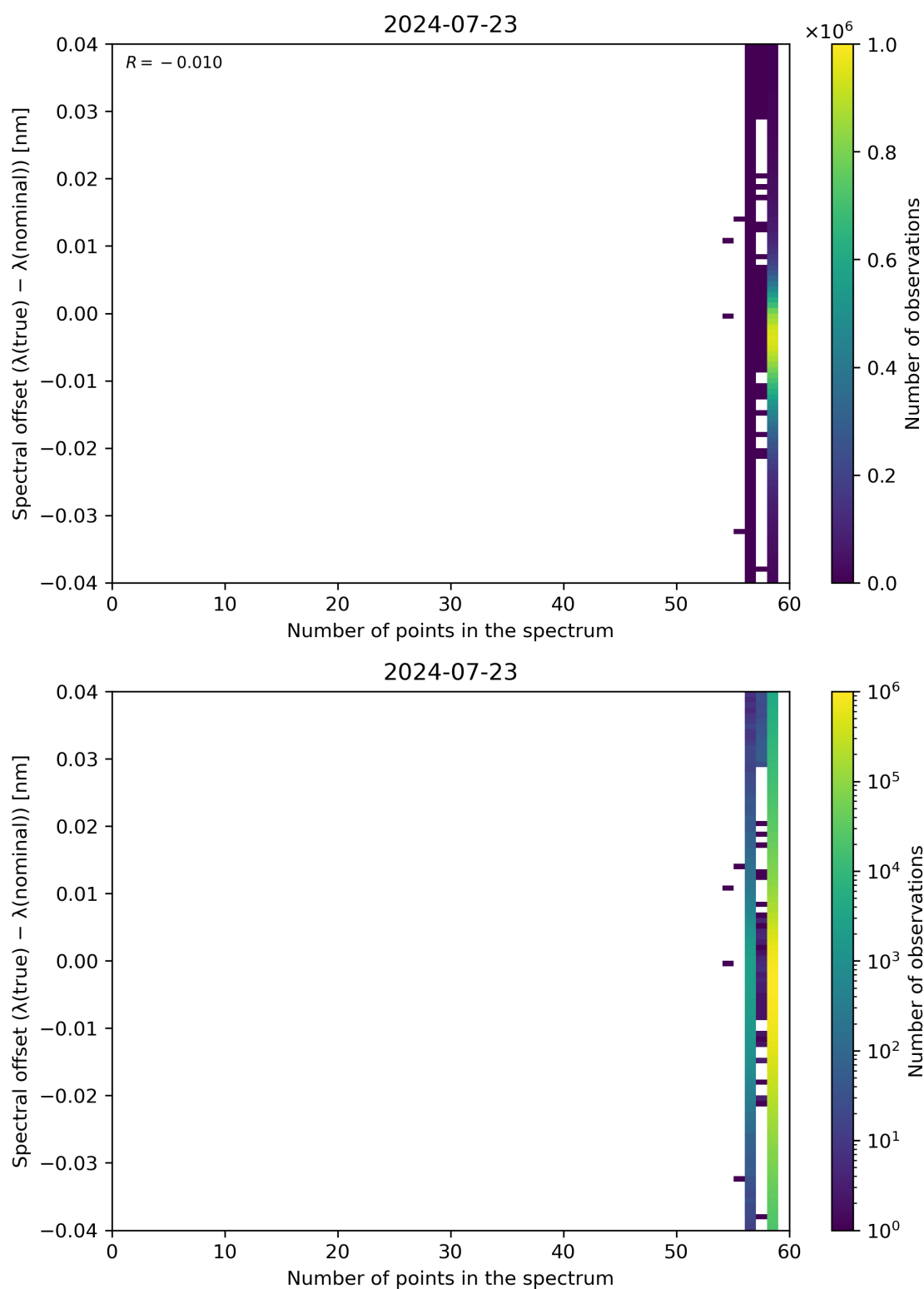
Figure 101: Scatter density plot of “Number of points in the spectrum” against “Spectral offset ( \lambda(\text{true}) - \lambda(\text{nominal}) )” for 2024-07-22 to 2024-07-24.
