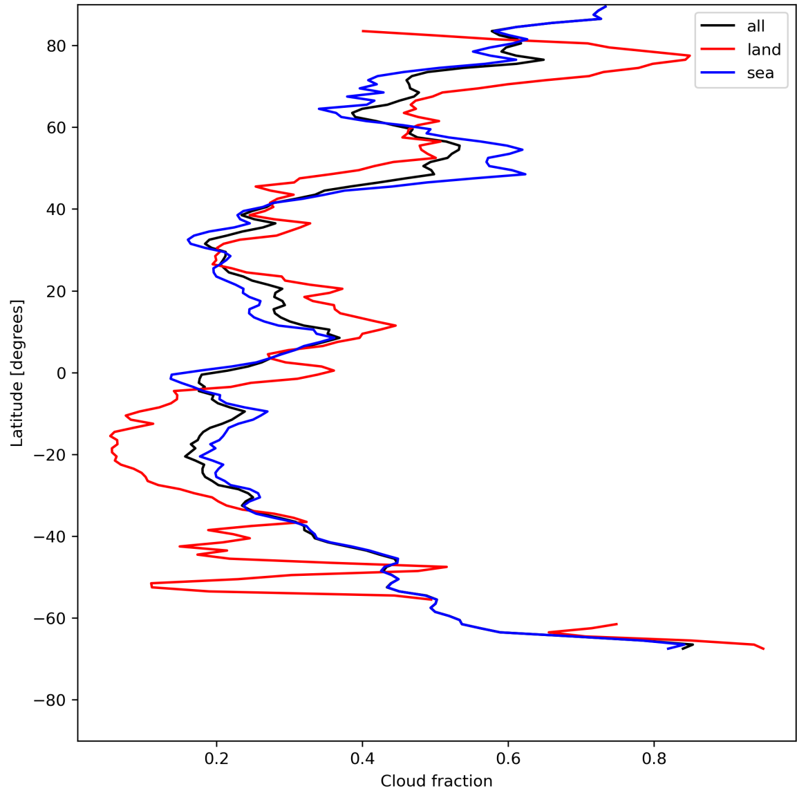
Figure 15: Zonal average of “Cloud fraction” for 2024-07-22 to 2024-07-24.
