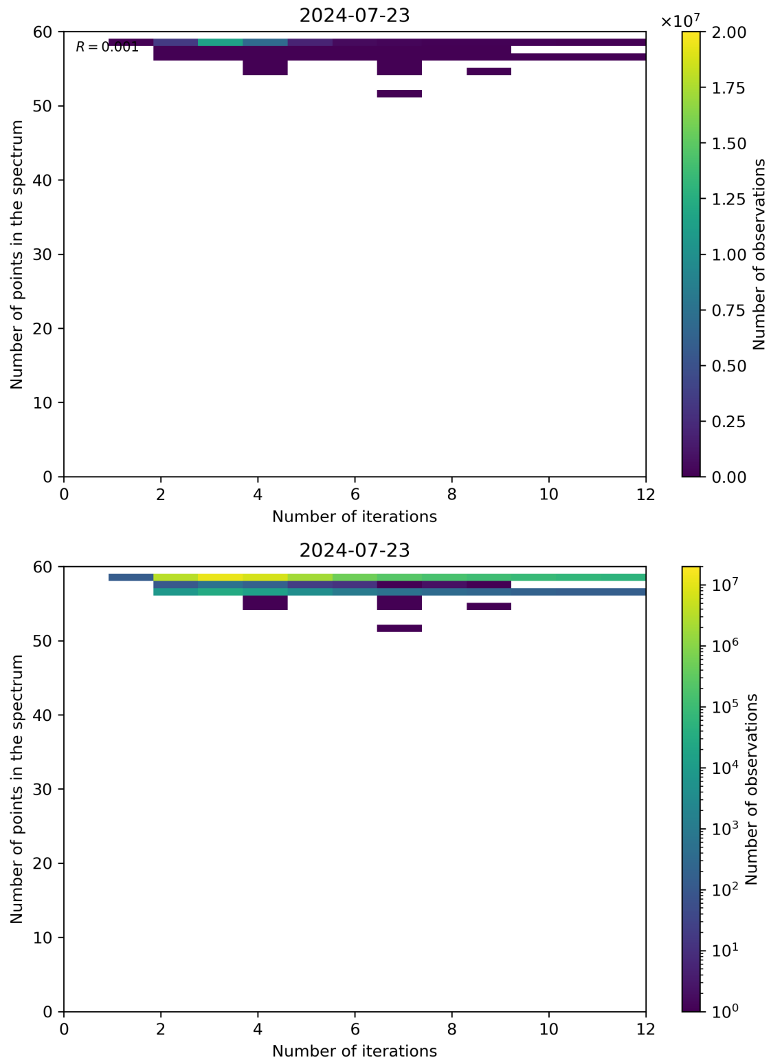
Figure 99: Scatter density plot of “Number of iterations” against “Number of points in the spectrum” for 2024-07-22 to 2024-07-24.
