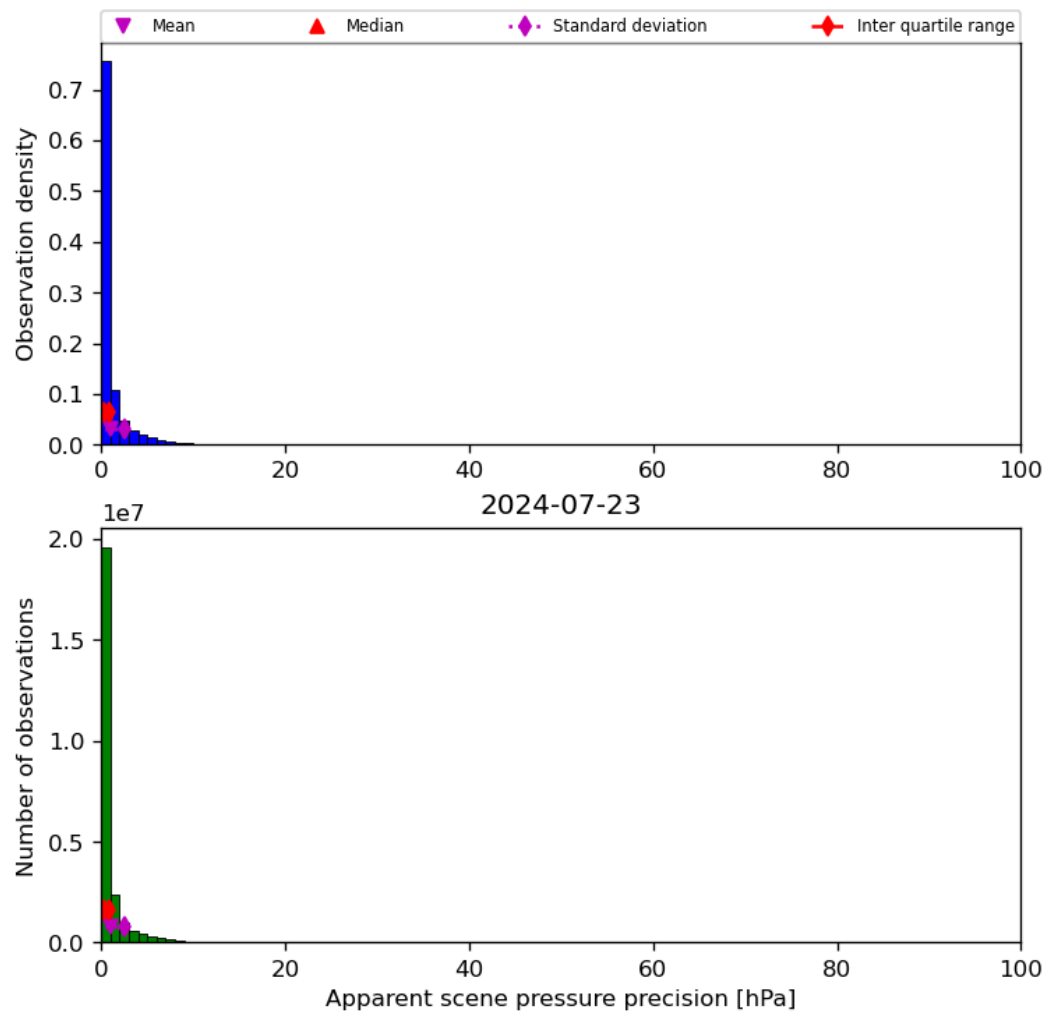
Figure 37: Histogram of “Apparent scene pressure precision” for 2024-07-22 to 2024-07-24
