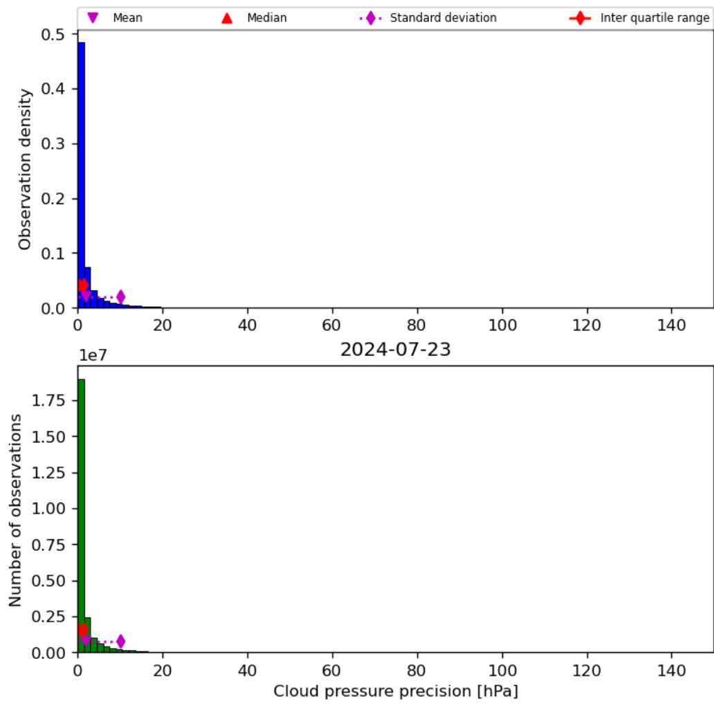
Figure 31: Histogram of “Cloud pressure precision” for 2024-07-22 to 2024-07-24
