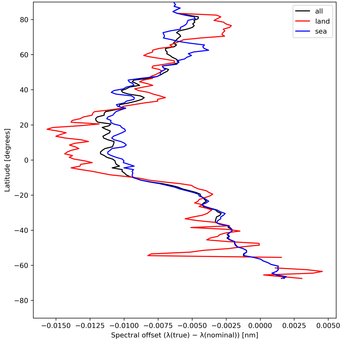
Figure 28: Zonal average of “Spectral offset ( \lambda(\text{true}) - \lambda(\text{nominal}) )” for 2024-07-22 to 2024-07-24.
