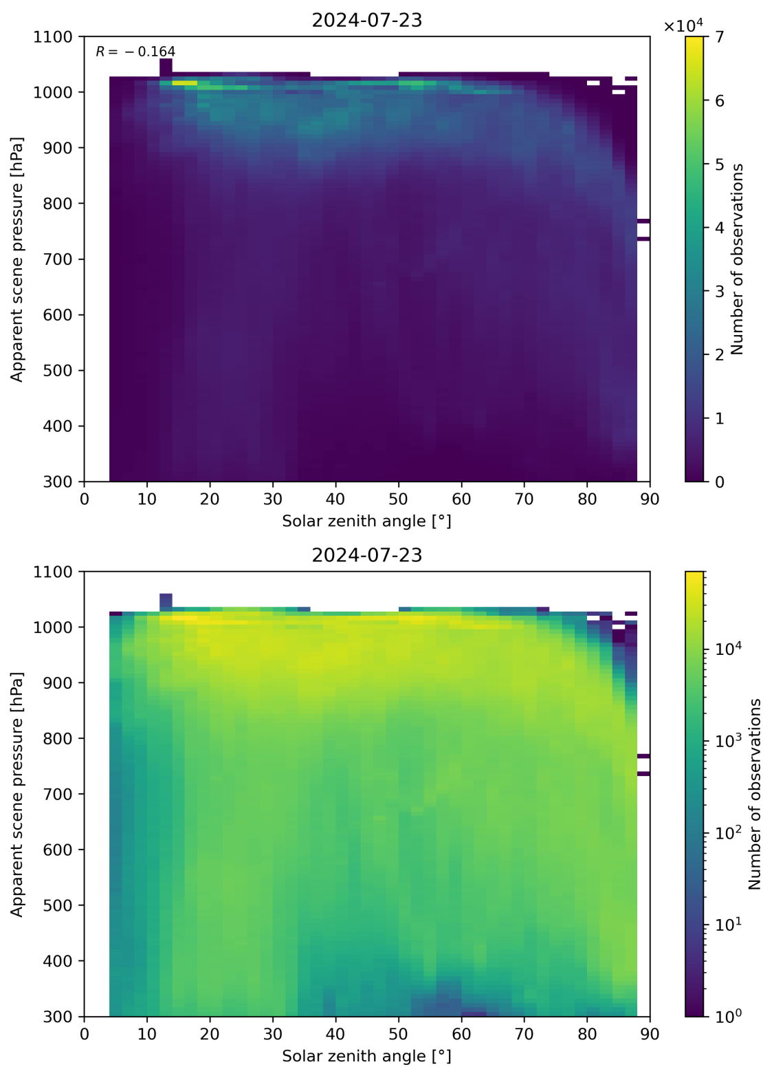
Figure 108: Scatter density plot of “Solar zenith angle” against “Apparent scene pressure” for 2024-07-22 to 2024-07-24.
