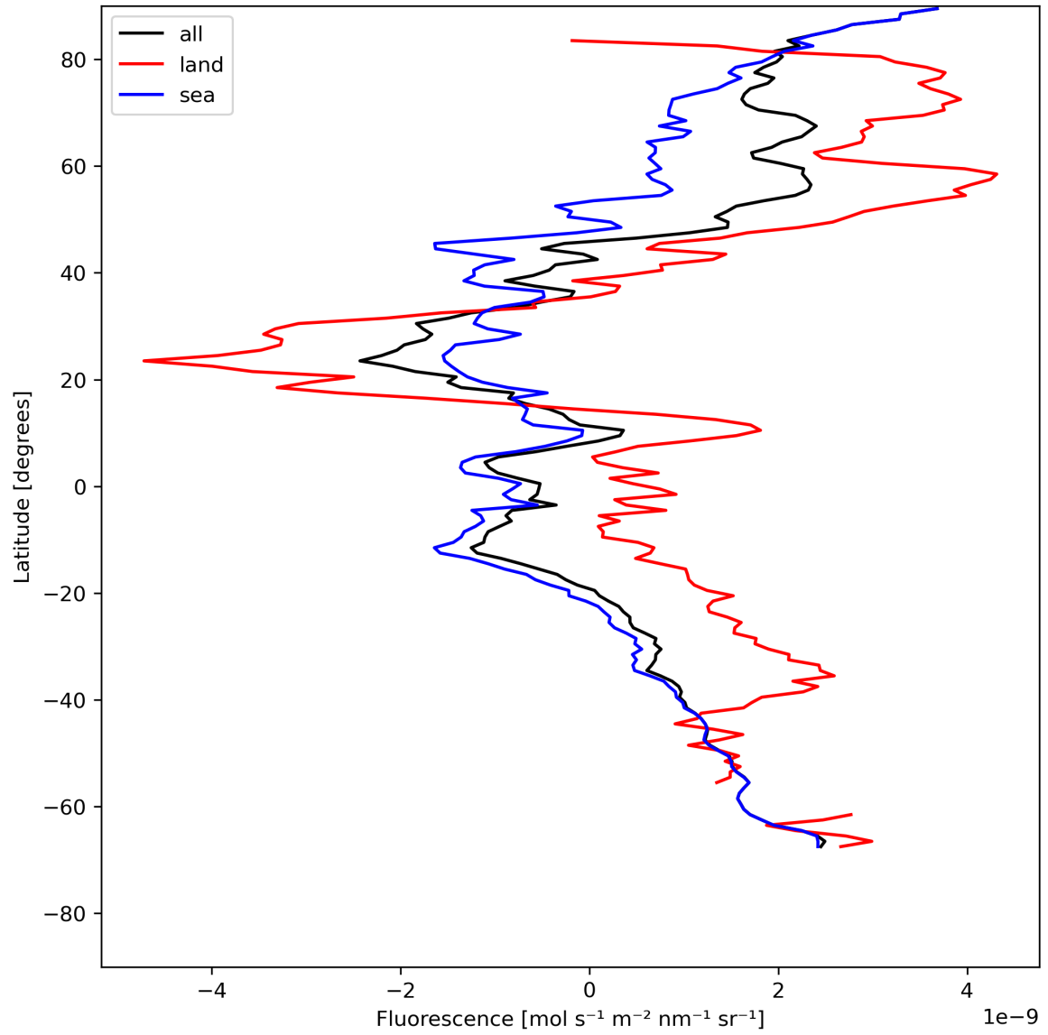
Figure 23: Zonal average of “Fluorescence” for 2024-07-22 to 2024-07-24.
