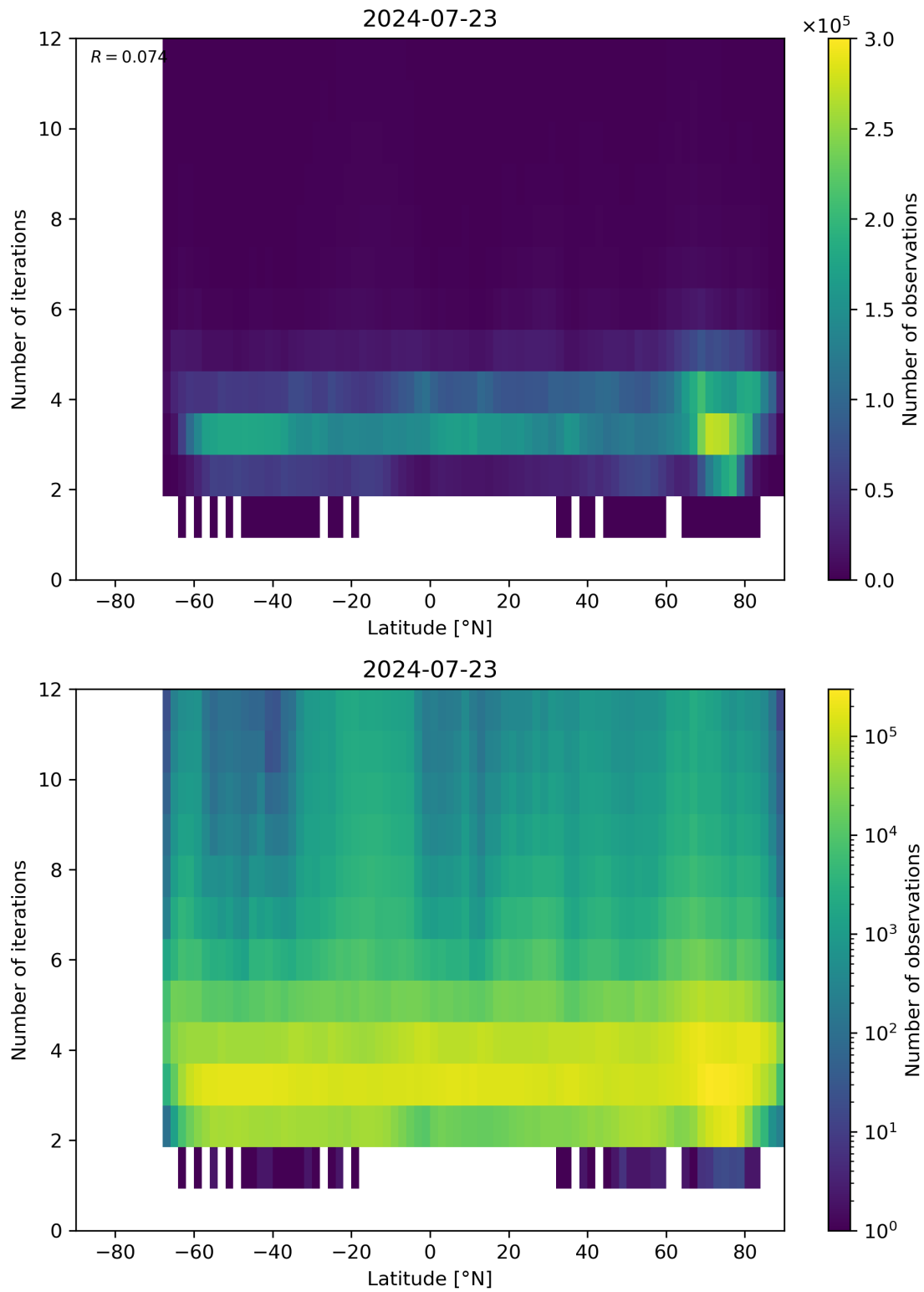
Figure 93: Scatter density plot of “Latitude” against “Number of iterations” for 2024-07-22 to 2024-07-24.
