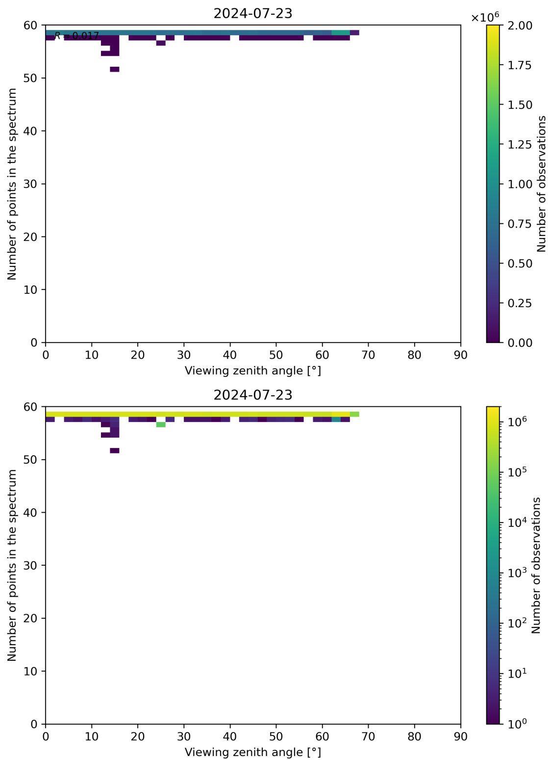
Figure 125: Scatter density plot of “Viewing zenith angle” against “Number of points in the spectrum” for 2024-07-22 to 2024-07-24.
