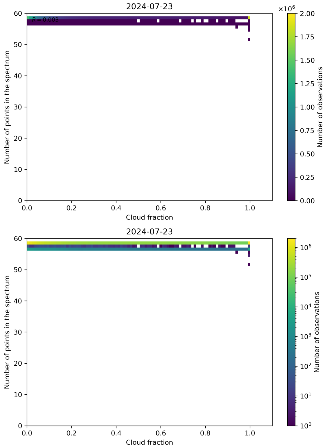
Figure 74: Scatter density plot of “Cloud fraction” against “Number of points in the spectrum” for 2024-07-22 to 2024-07-24.
