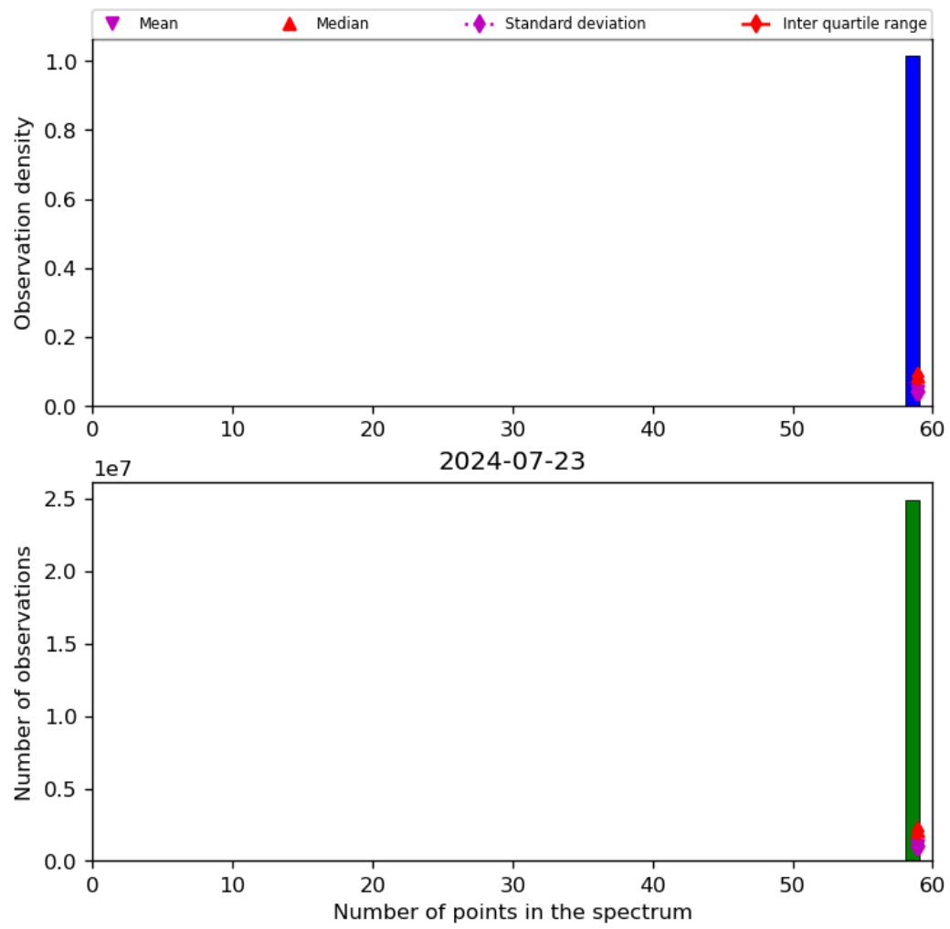
Figure 44: Histogram of “Number of points in the spectrum” for 2024-07-22 to 2024-07-24
