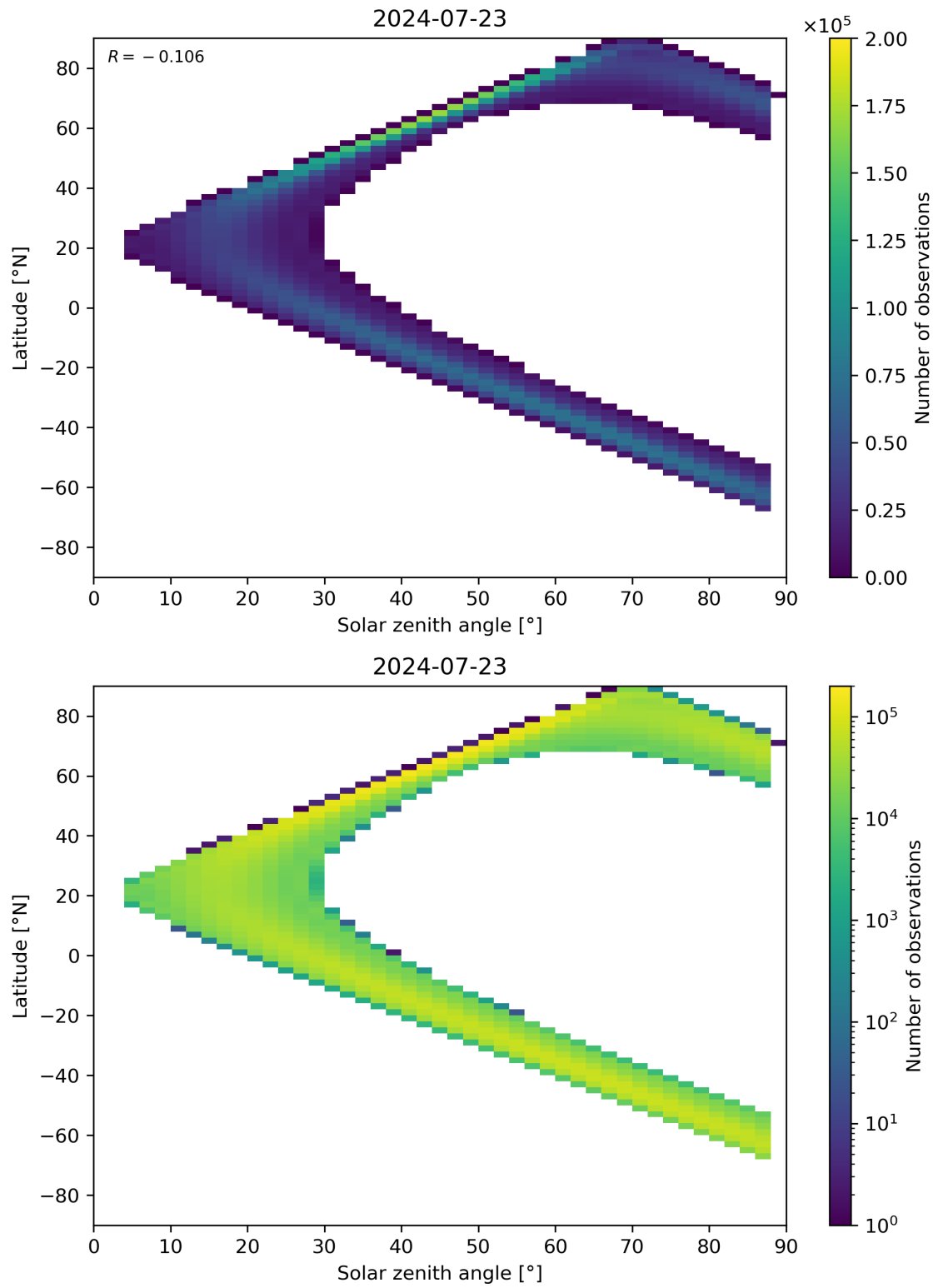
Figure 113: Scatter density plot of “Solar zenith angle” against “Latitude” for 2024-07-22 to 2024-07-24.
