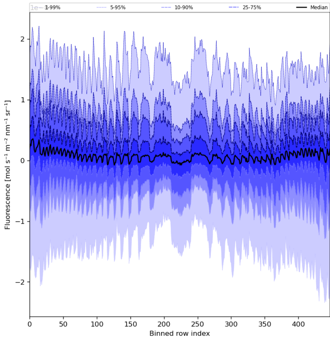
Figure 57: Along track statistics of “Fluorescence” for 2024-07-22 to 2024-07-24
