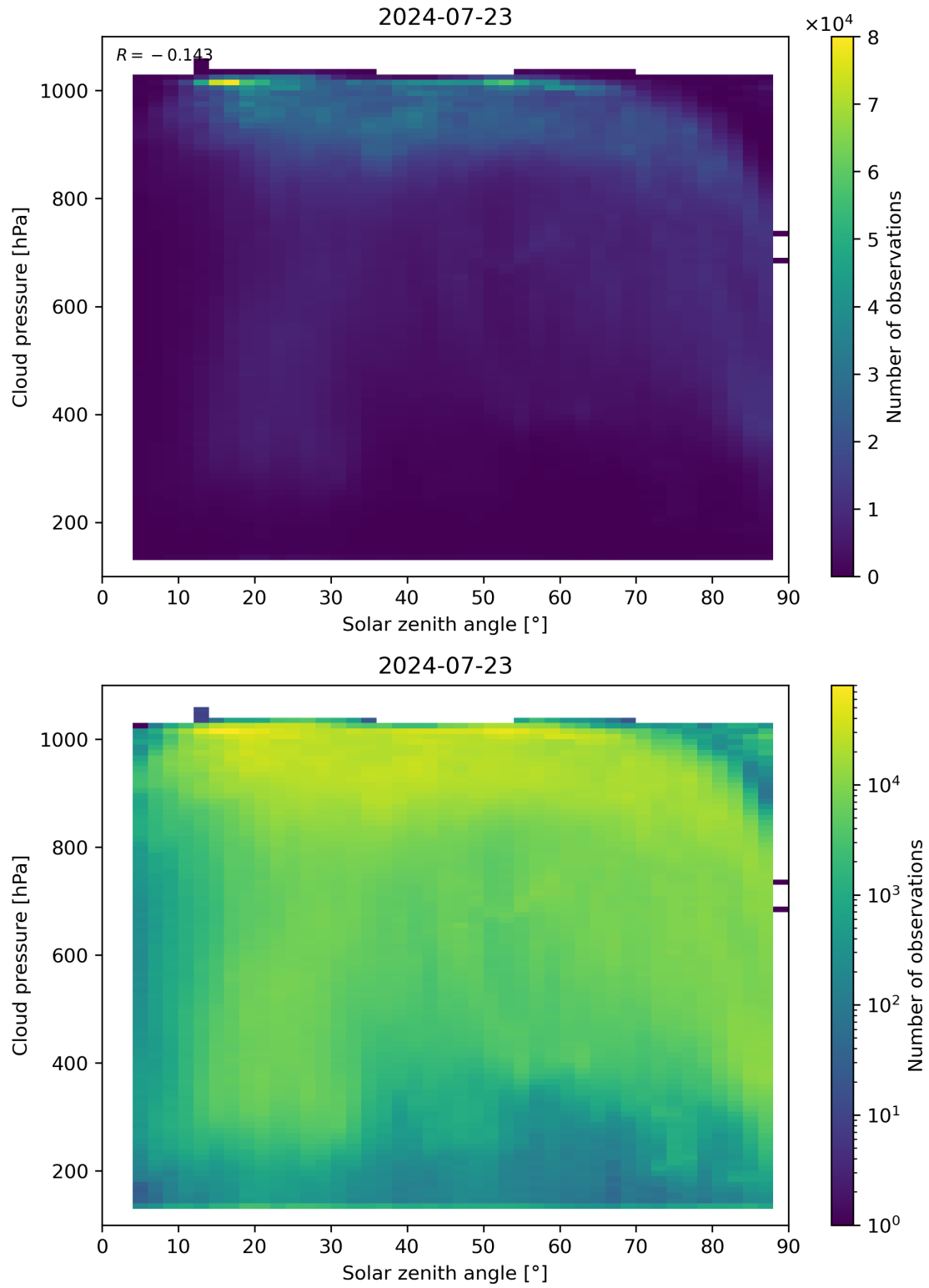
Figure 111: Scatter density plot of “Solar zenith angle” against “Cloud pressure” for 2024-07-22 to 2024-07-24.
