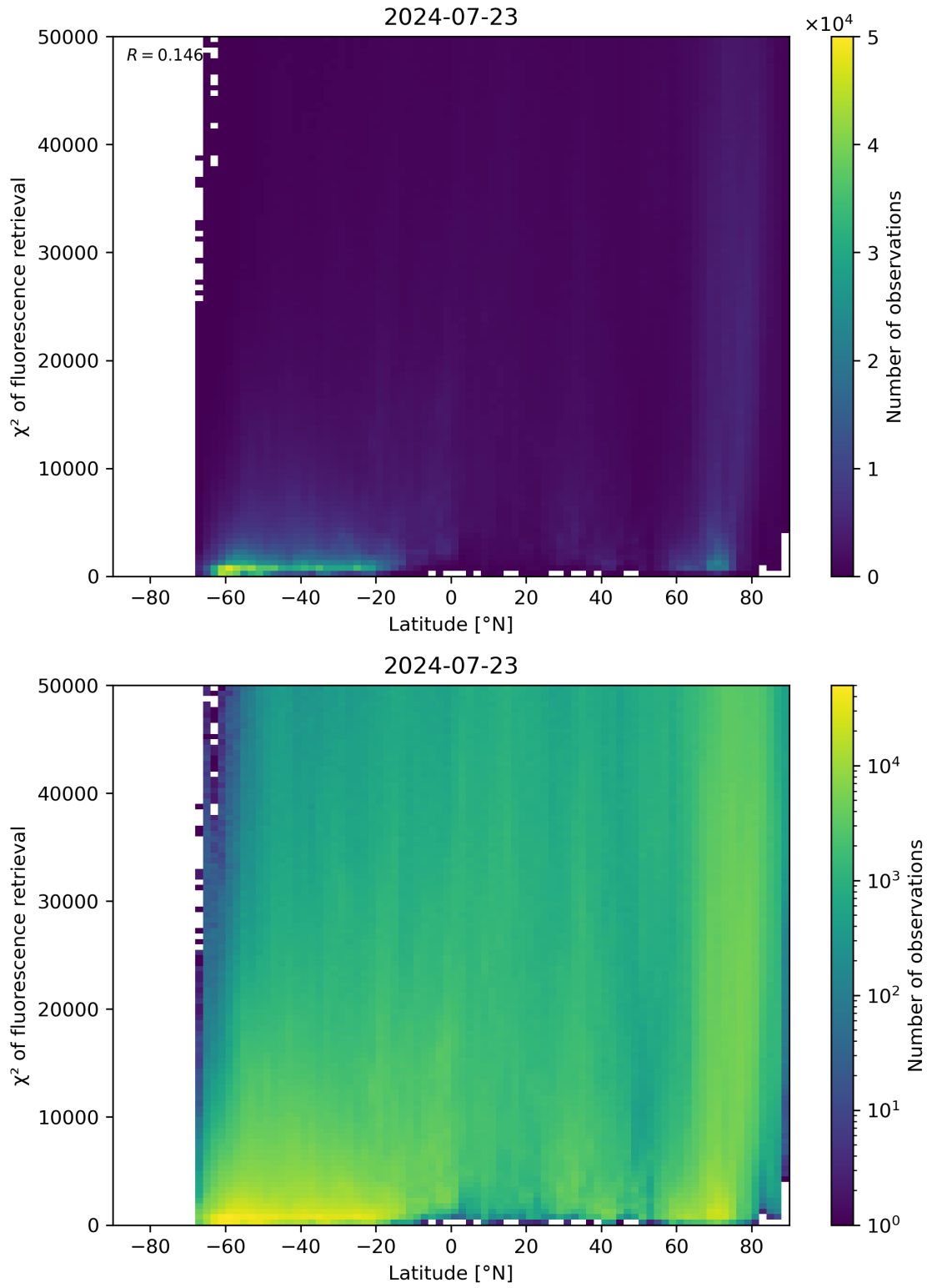
Figure 89: Scatter density plot of “Latitude” against “ \chi^2 of fluorescence retrieval” for 2024-07-22 to 2024-07-24.
