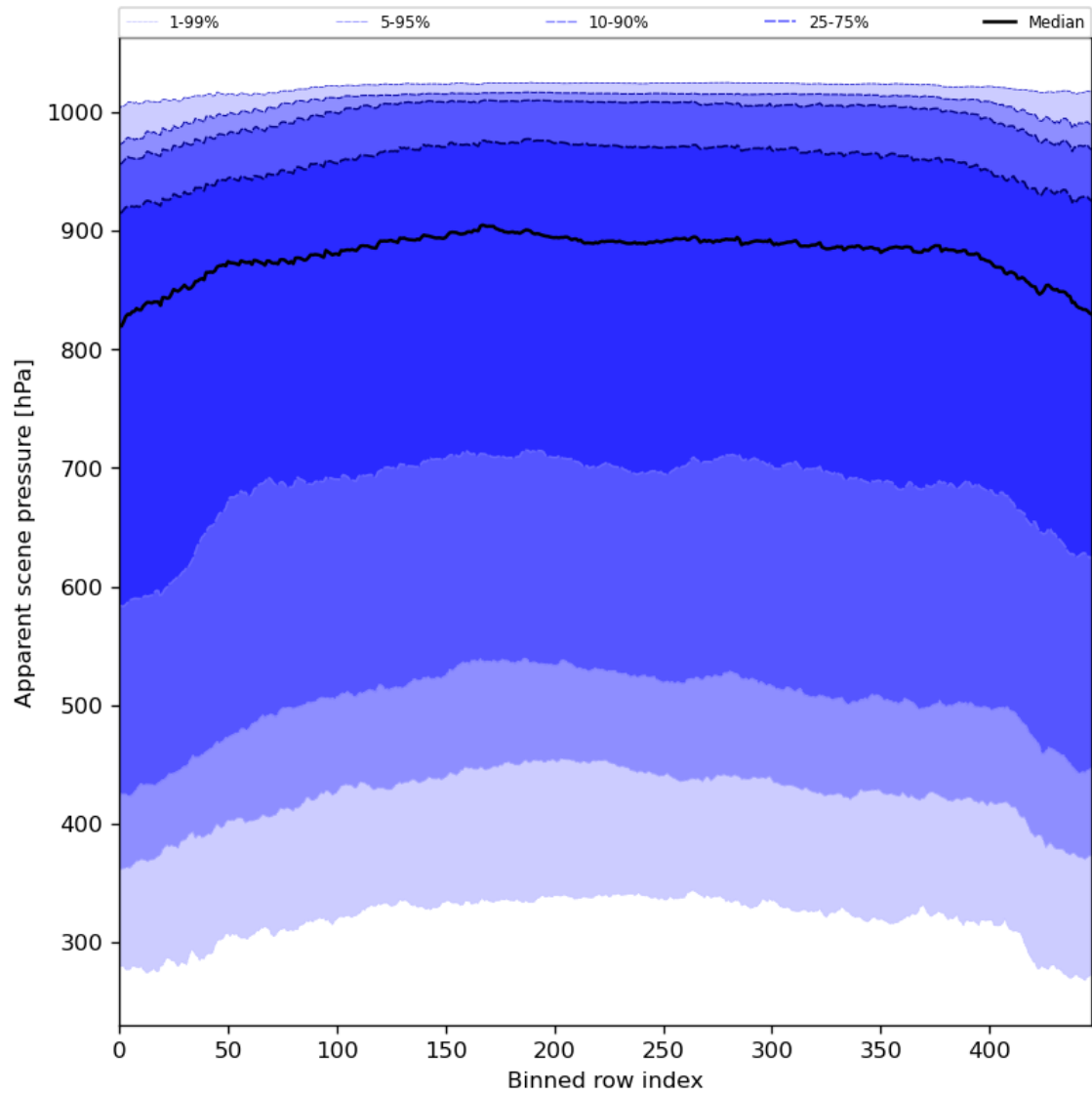
Figure 53: Along track statistics of “Apparent scene pressure” for 2024-07-22 to 2024-07-24
