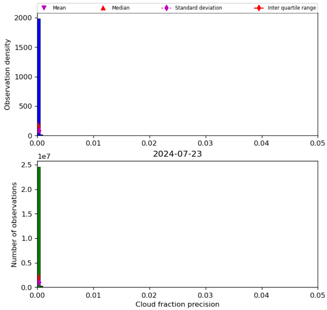
Figure 33: Histogram of “Cloud fraction precision” for 2024-07-22 to 2024-07-24
