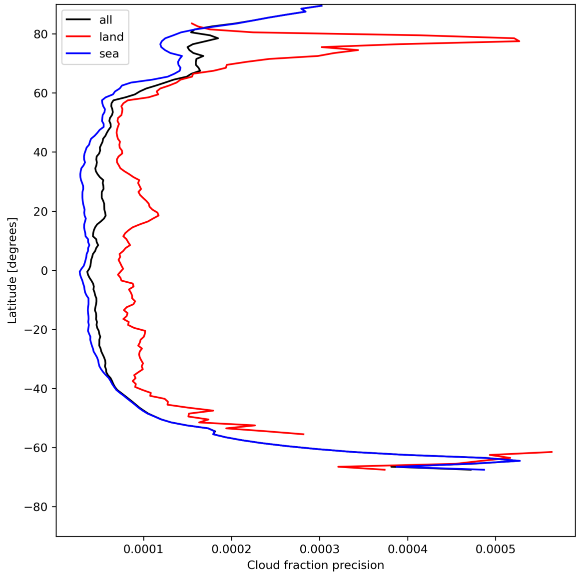
Figure 16: Zonal average of “Cloud fraction precision” for 2024-07-22 to 2024-07-24.
