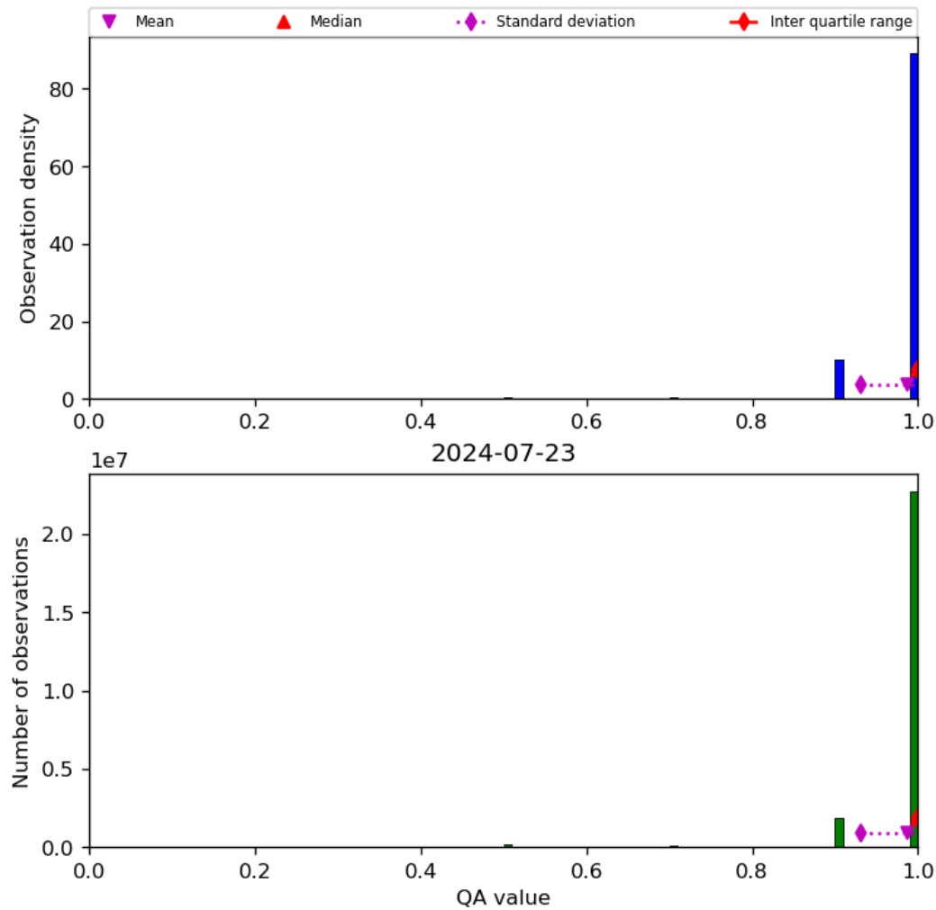
Figure 29: Histogram of “QA value” for 2024-07-22 to 2024-07-24
