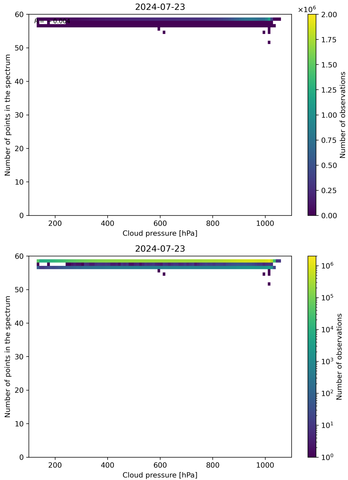
Figure 82: Scatter density plot of “Cloud pressure” against “Number of points in the spectrum” for 2024-07-22 to 2024-07-24.
