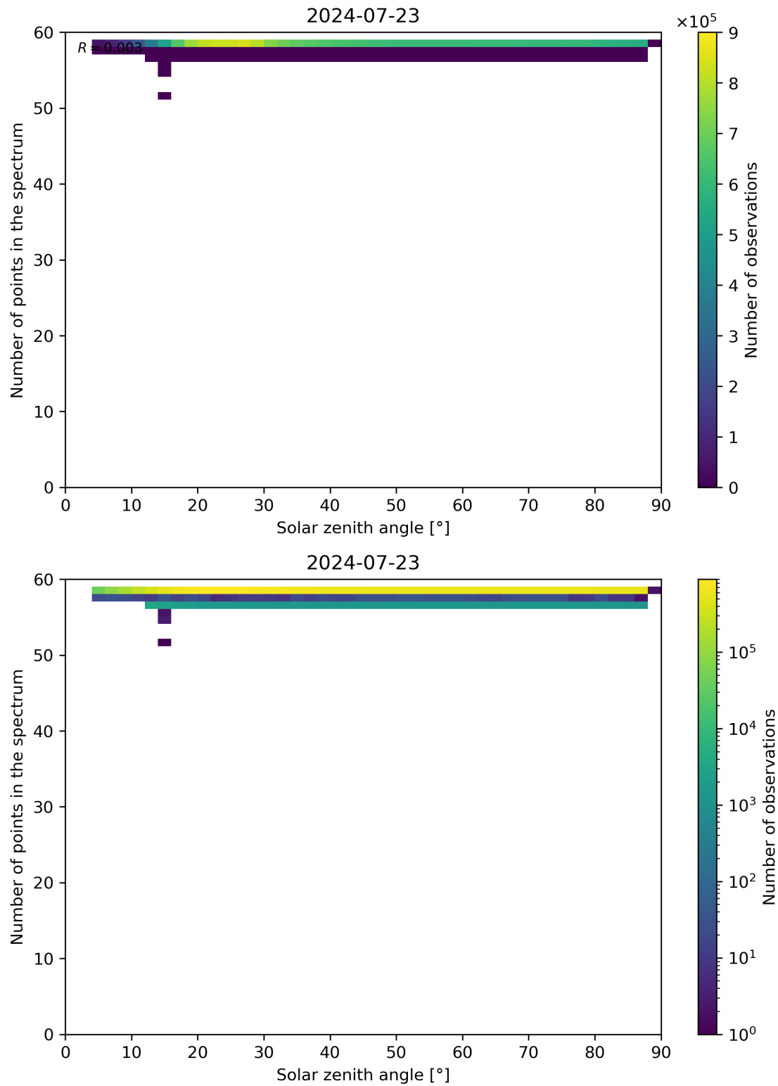
Figure 115: Scatter density plot of “Solar zenith angle” against “Number of points in the spectrum” for 2024-07-22 to 2024-07-24.
