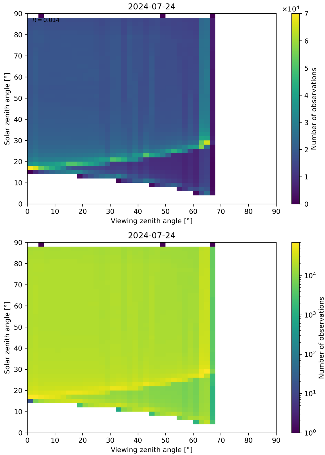
Figure 127: Scatter density plot of “Viewing zenith angle” against “Solar zenith angle” for 2024-07-23 to 2024-07-25.
