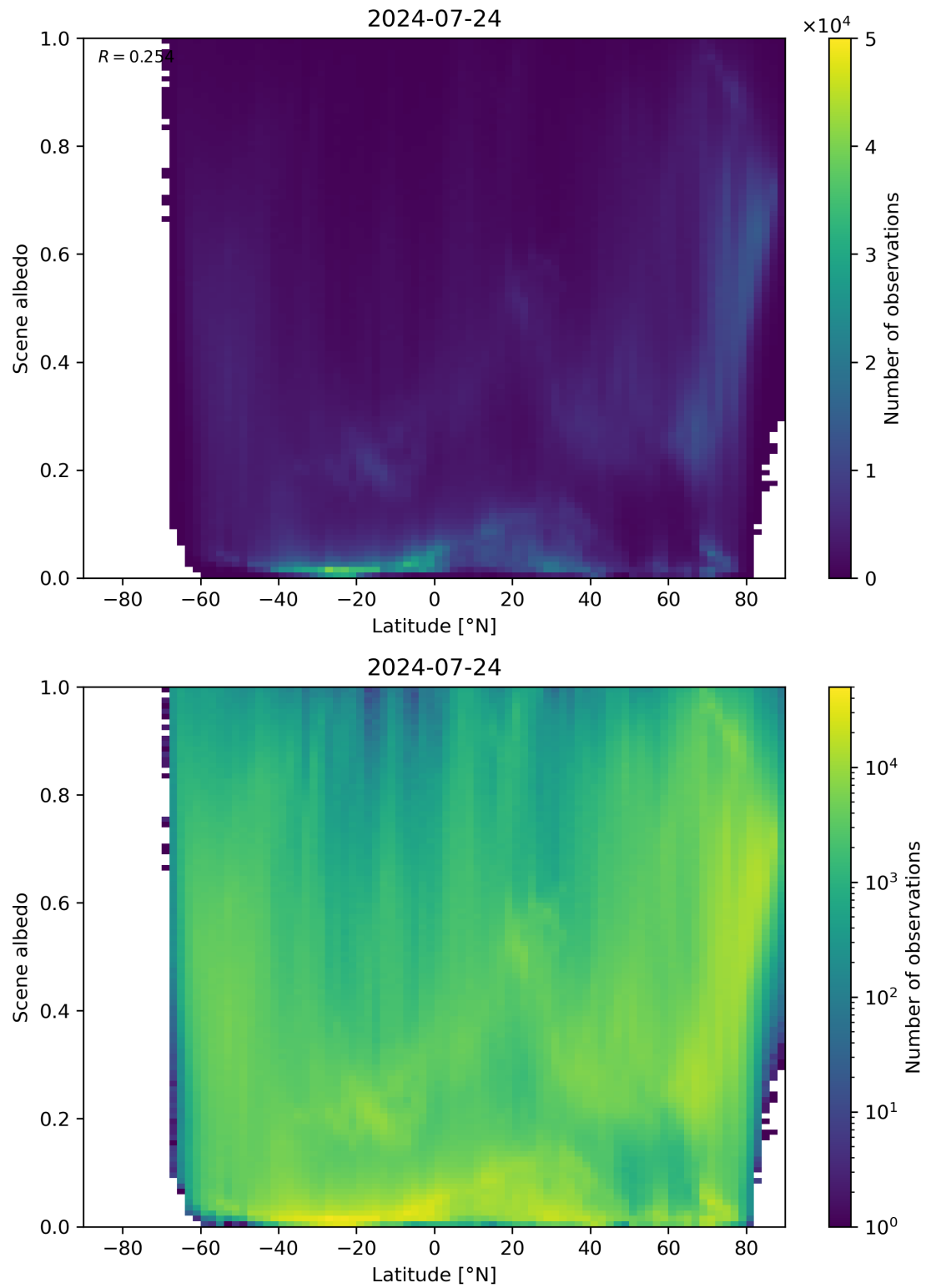
Figure 95: Scatter density plot of “Latitude” against “Scene albedo” for 2024-07-23 to 2024-07-25.
