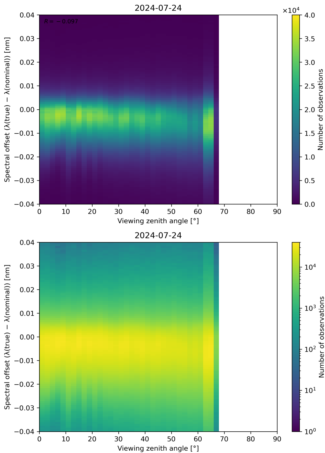
Figure 128: Scatter density plot of “Viewing zenith angle” against “Spectral offset ( \lambda(\text{true}) - \lambda(\text{nominal}) )” for 2024-07-23 to 2024-07-25.
