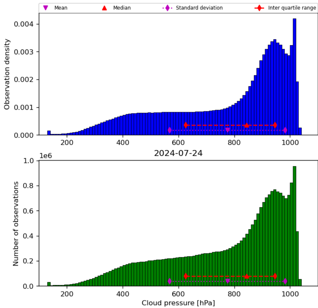
Figure 30: Histogram of “Cloud pressure” for 2024-07-23 to 2024-07-25
