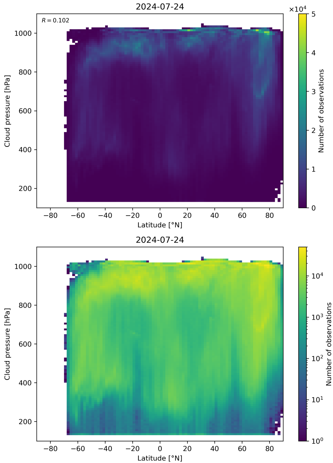
Figure 91: Scatter density plot of “Latitude” against “Cloud pressure” for 2024-07-23 to 2024-07-25.
