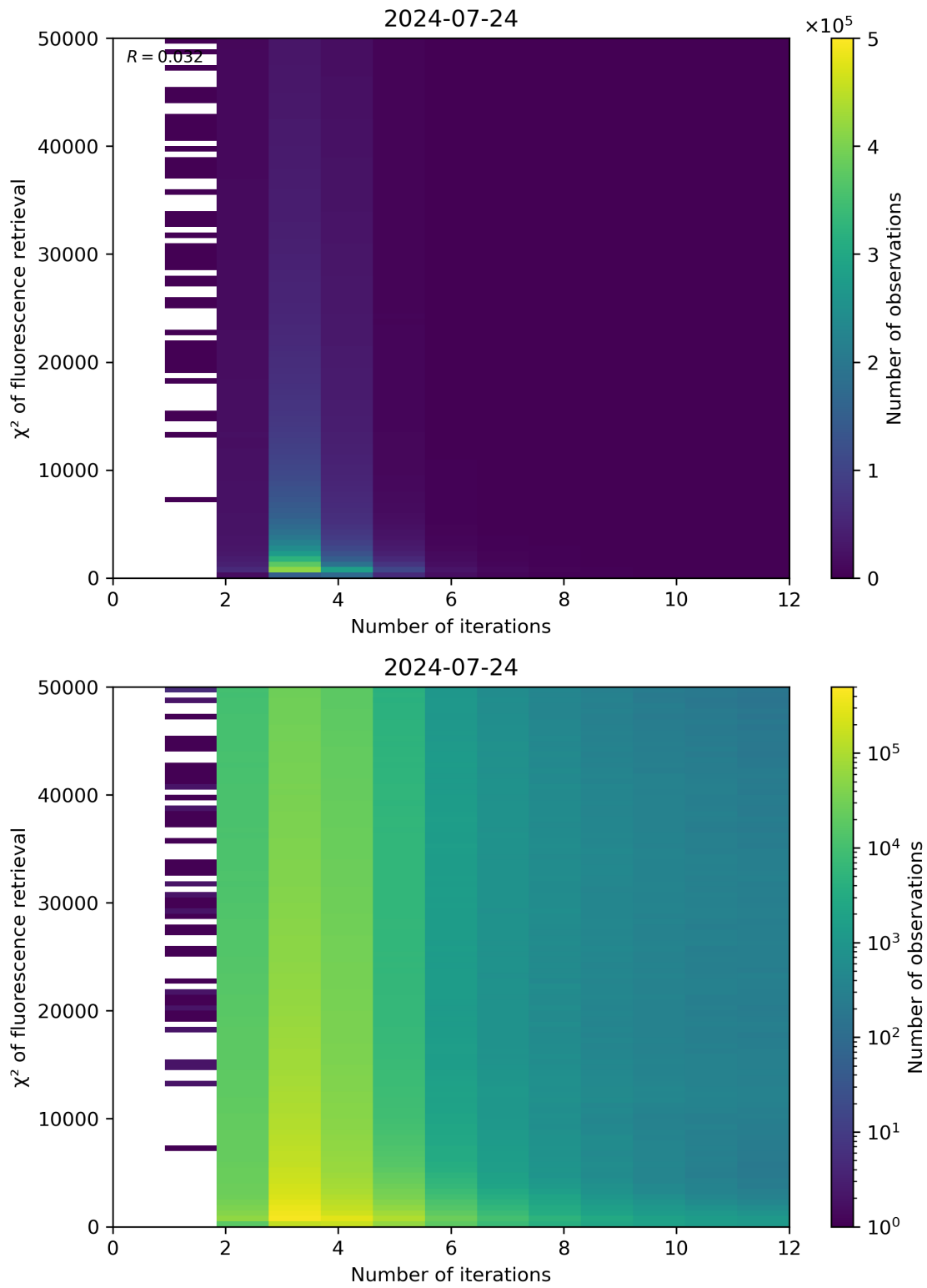
Figure 97: Scatter density plot of “Number of iterations” against “ \chi^2 of fluorescence retrieval” for 2024-07-23 to 2024-07-25.
