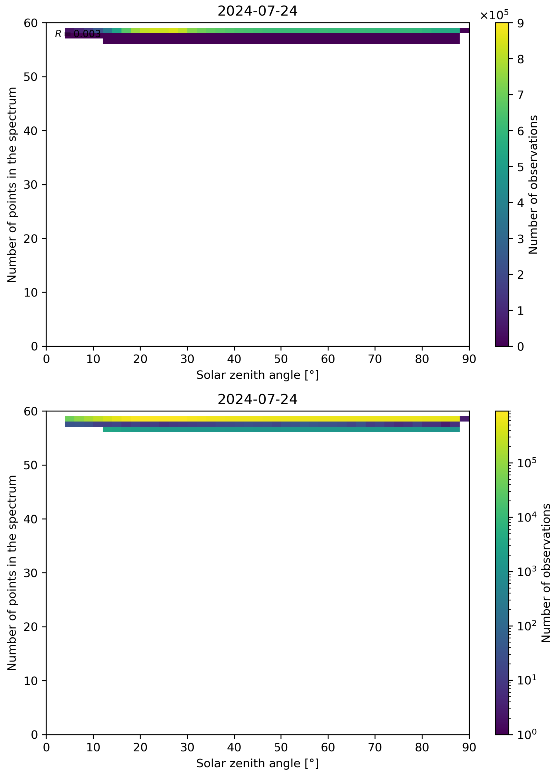
Figure 115: Scatter density plot of “Solar zenith angle” against “Number of points in the spectrum” for 2024-07-23 to 2024-07-25.
