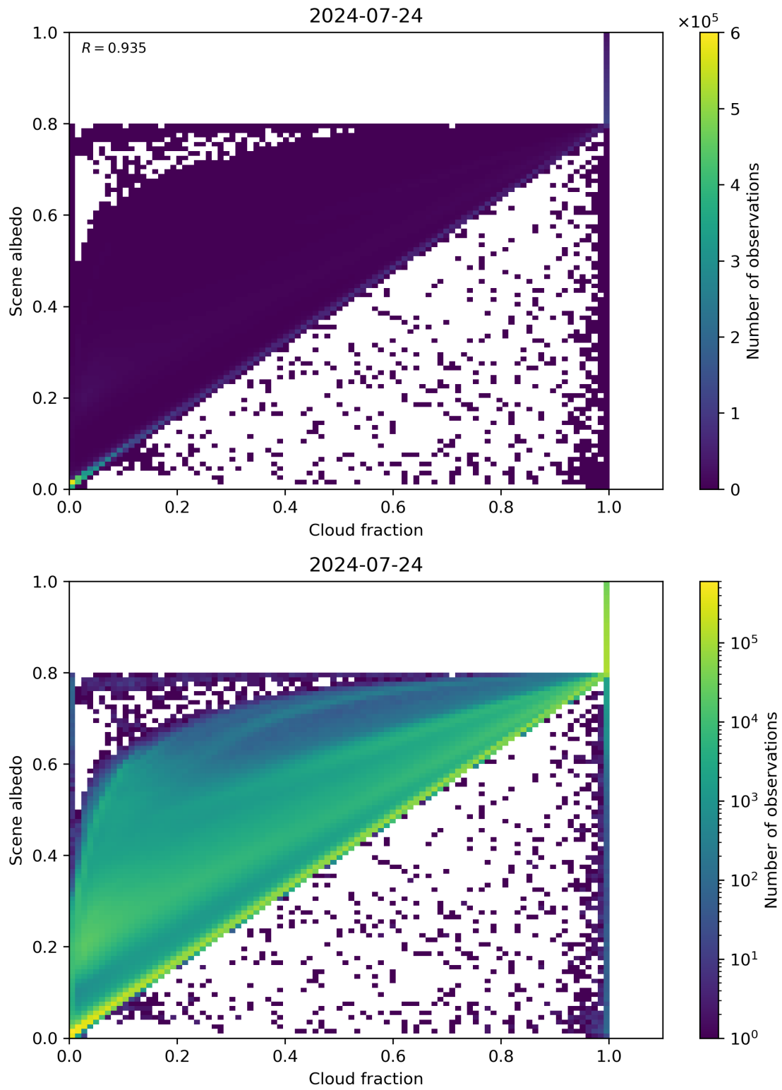
Figure 75: Scatter density plot of “Cloud fraction” against “Scene albedo” for 2024-07-23 to 2024-07-25.
