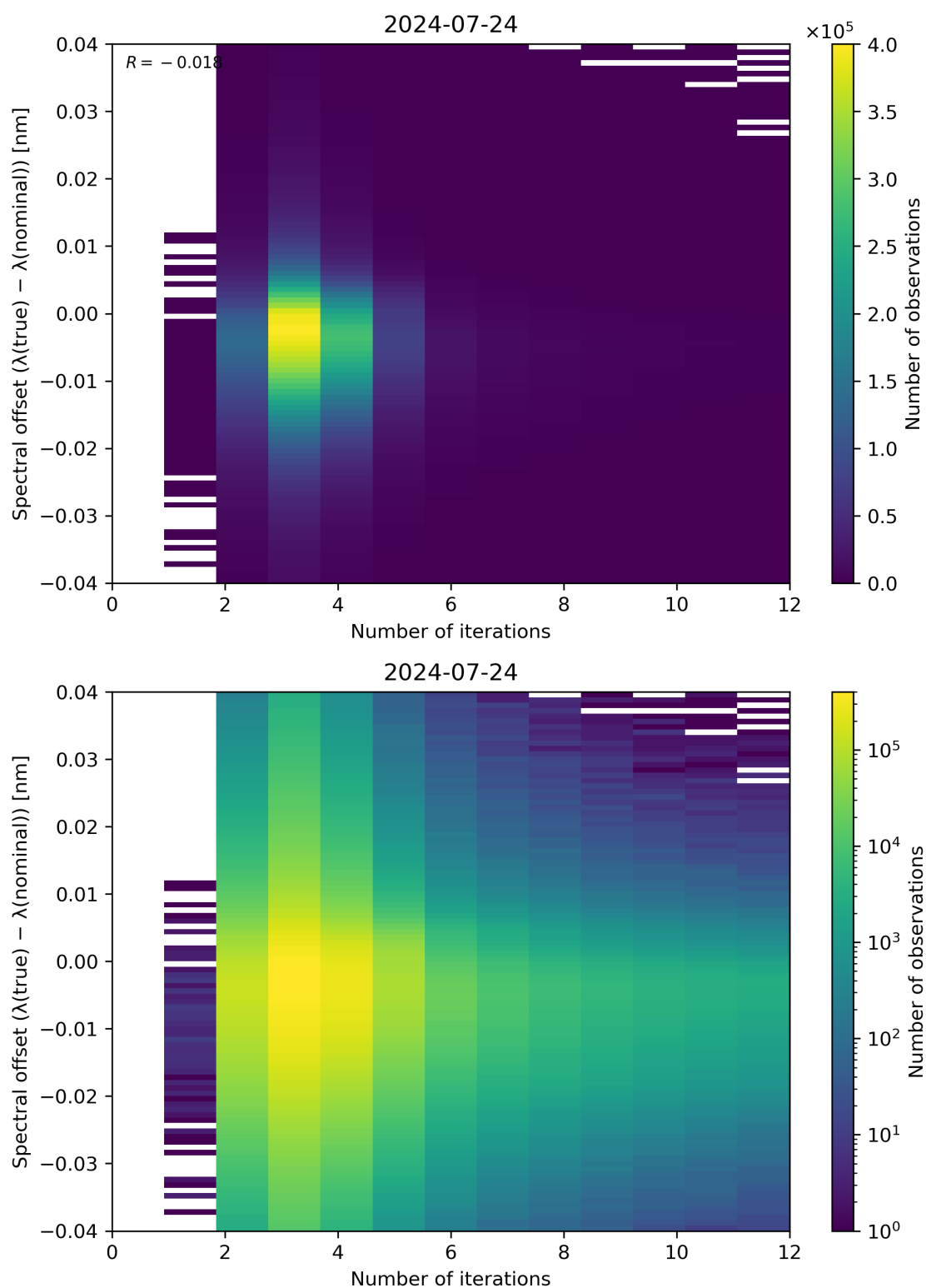
Figure 100: Scatter density plot of “Number of iterations” against “Spectral offset ( \lambda(\text{true}) - \lambda(\text{nominal}) )” for 2024-07-23 to 2024-07-25.
