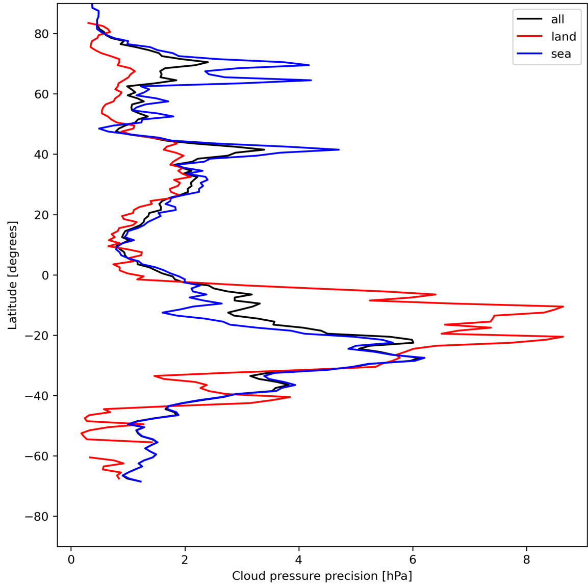
Figure 14: Zonal average of “Cloud pressure precision” for 2024-07-23 to 2024-07-25.
