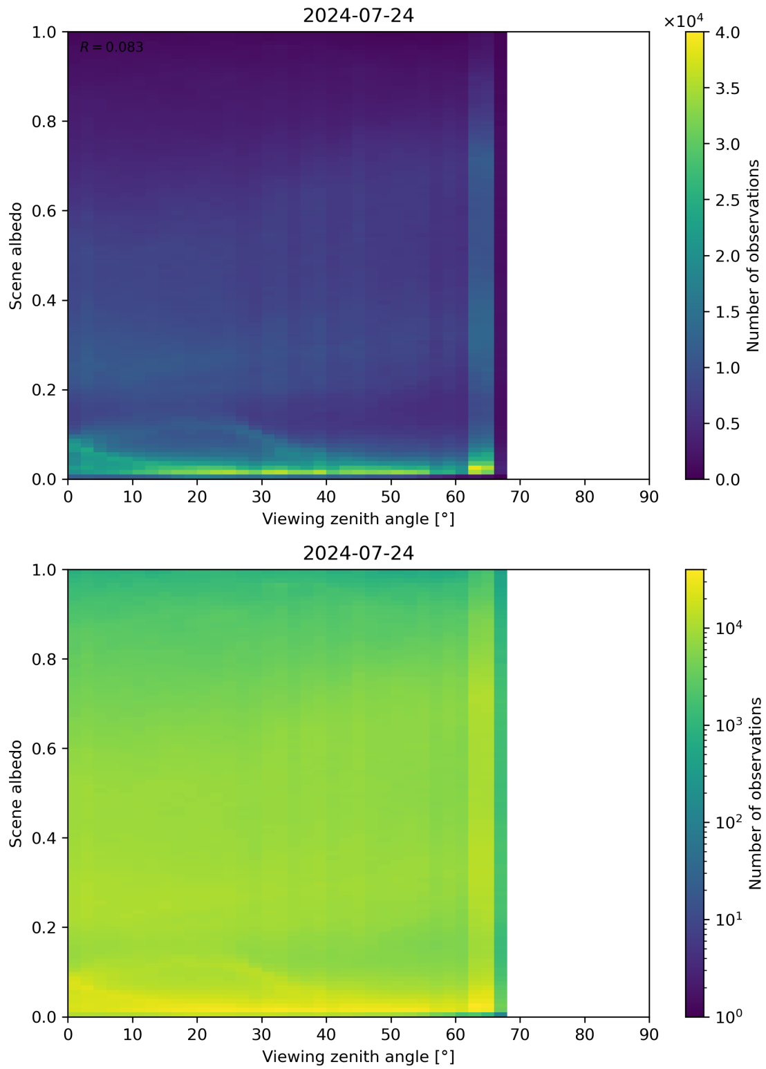
Figure 126: Scatter density plot of “Viewing zenith angle” against “Scene albedo” for 2024-07-23 to 2024-07-25.
