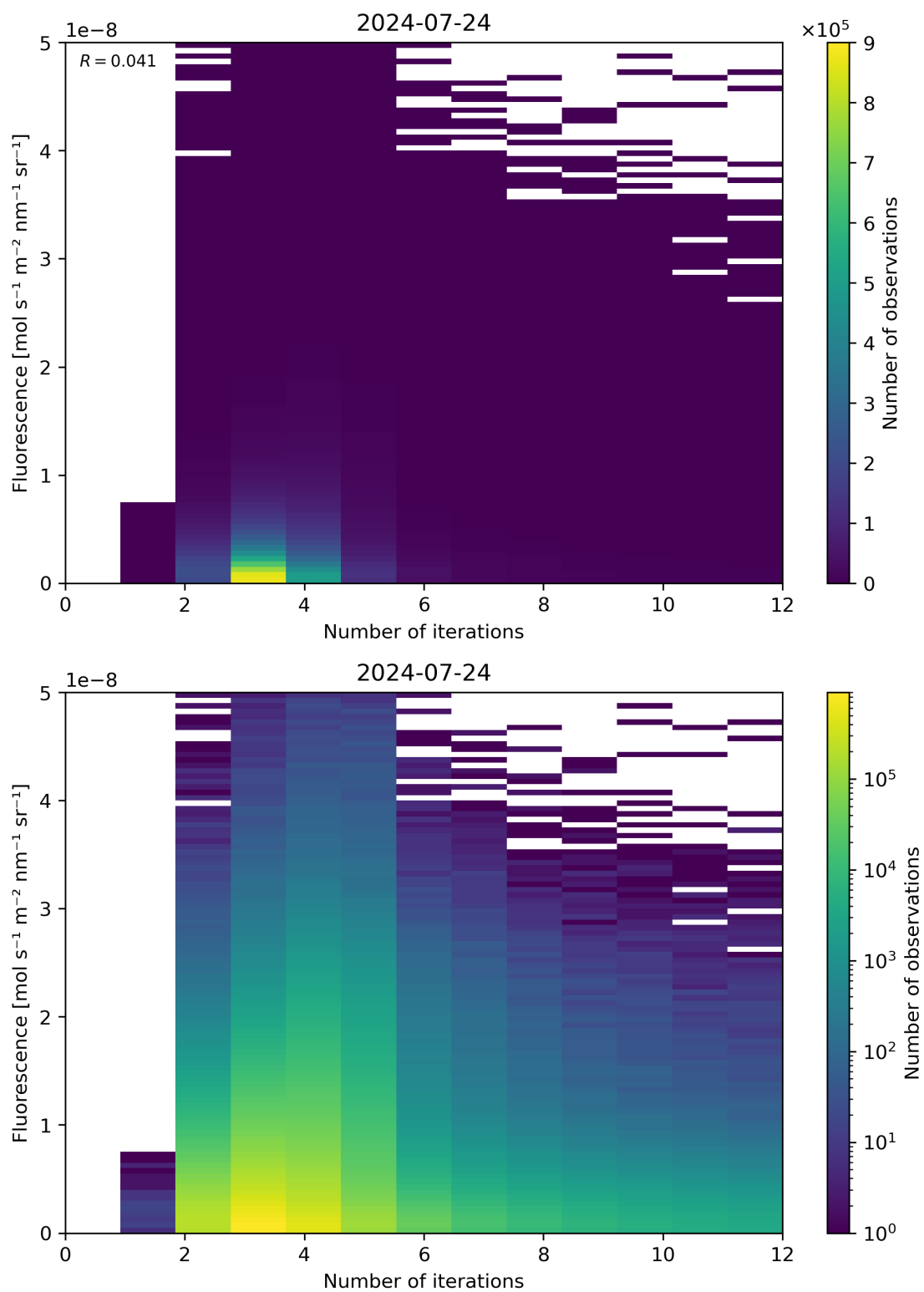
Figure 98: Scatter density plot of “Number of iterations” against “Fluorescence” for 2024-07-23 to 2024-07-25.
