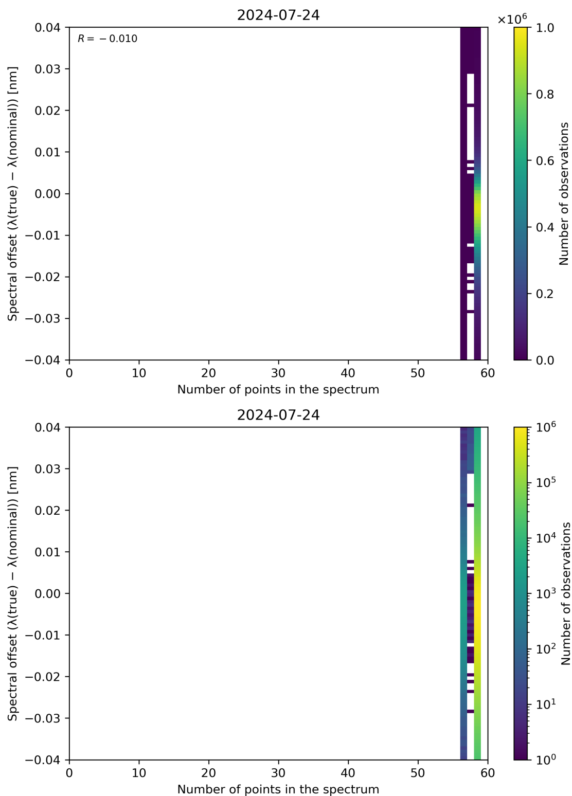
Figure 101: Scatter density plot of “Number of points in the spectrum” against “Spectral offset ( \lambda(\text{true}) - \lambda(\text{nominal}) )” for 2024-07-23 to 2024-07-25.
