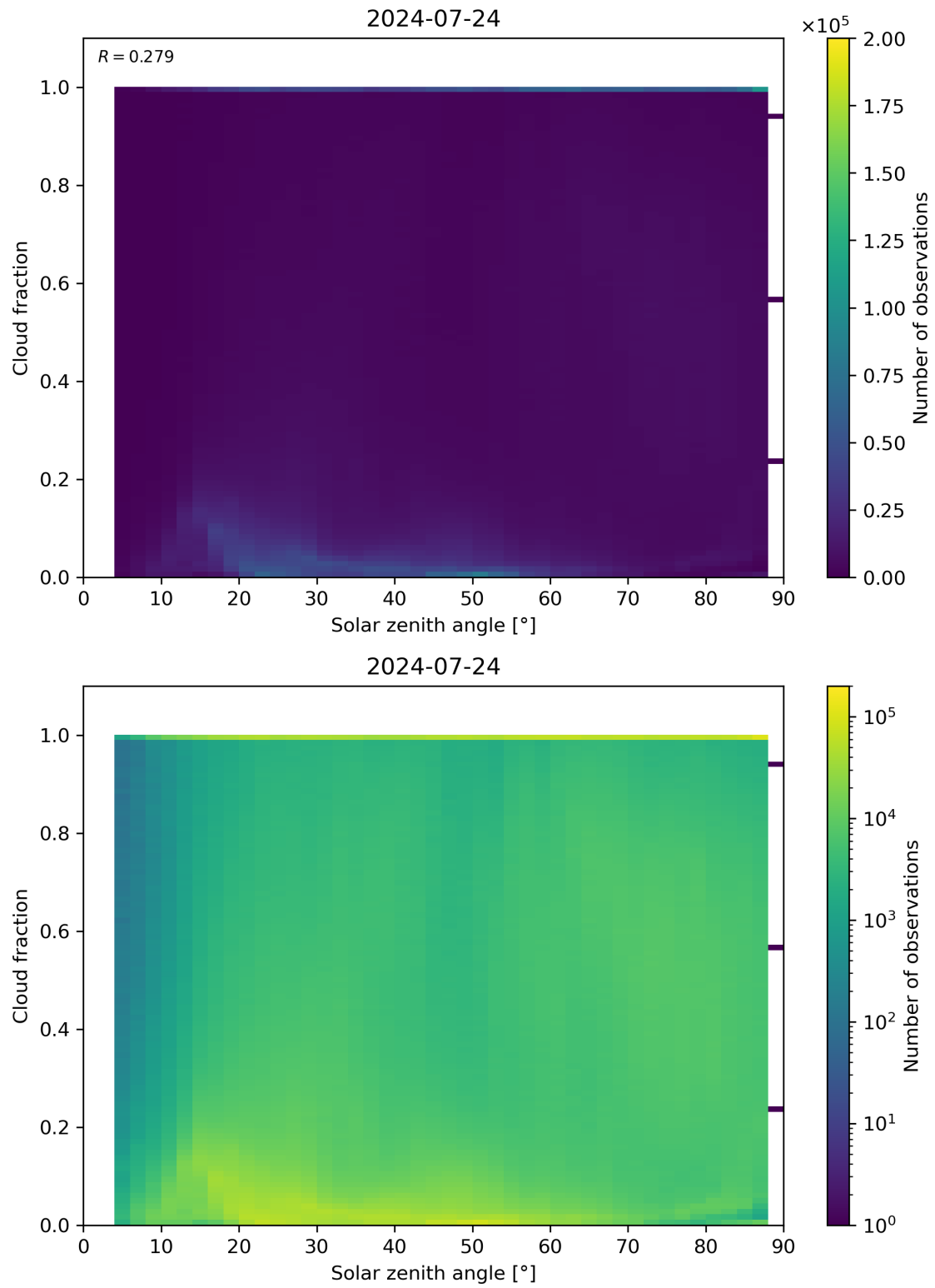
Figure 110: Scatter density plot of “Solar zenith angle” against “Cloud fraction” for 2024-07-23 to 2024-07-25.
