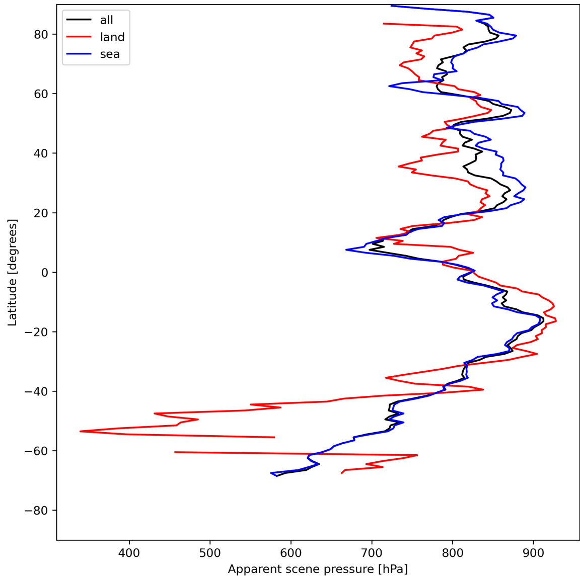
Figure 19: Zonal average of “Apparent scene pressure” for 2024-07-23 to 2024-07-25.
