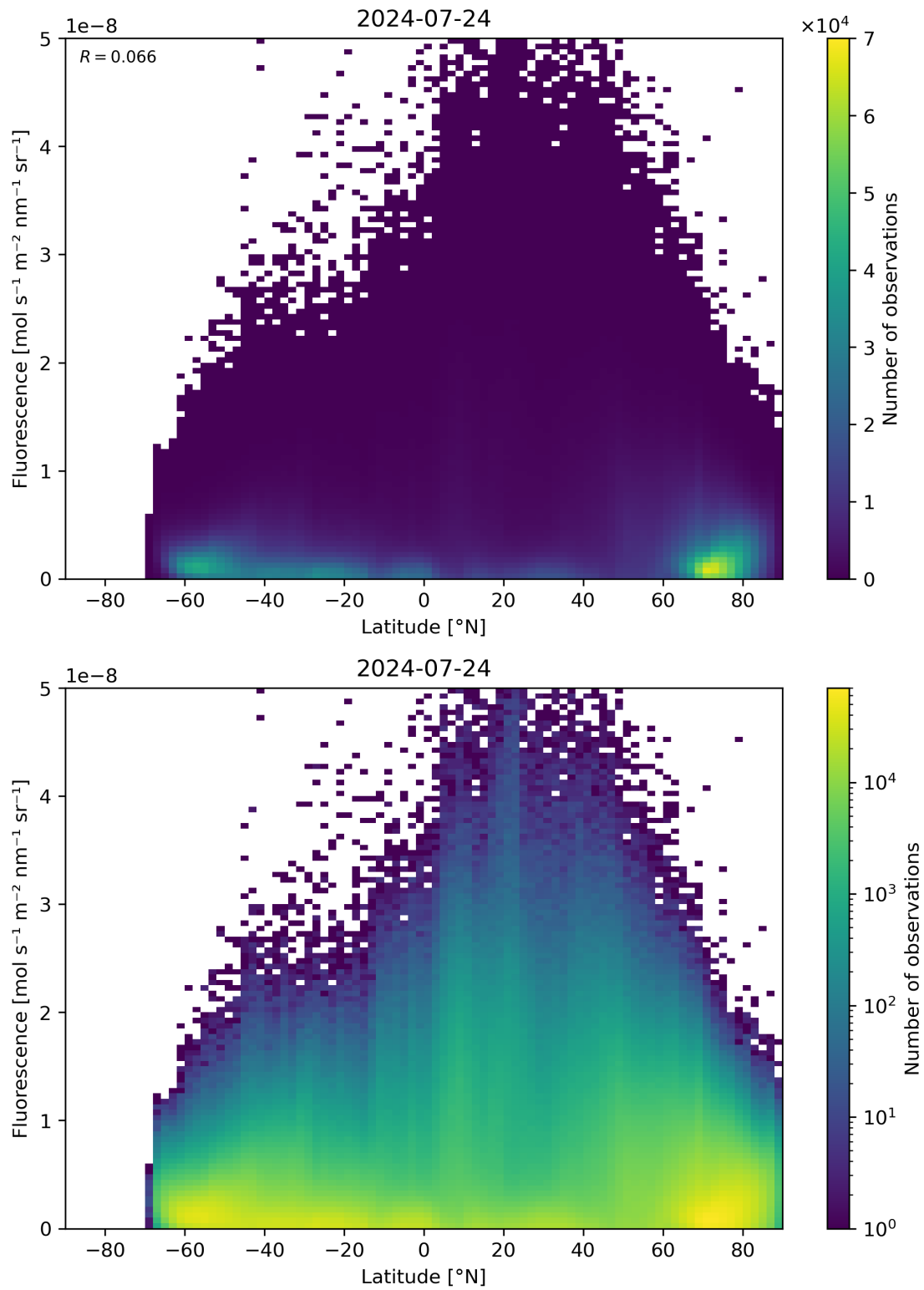
Figure 92: Scatter density plot of “Latitude” against “Fluorescence” for 2024-07-23 to 2024-07-25.
