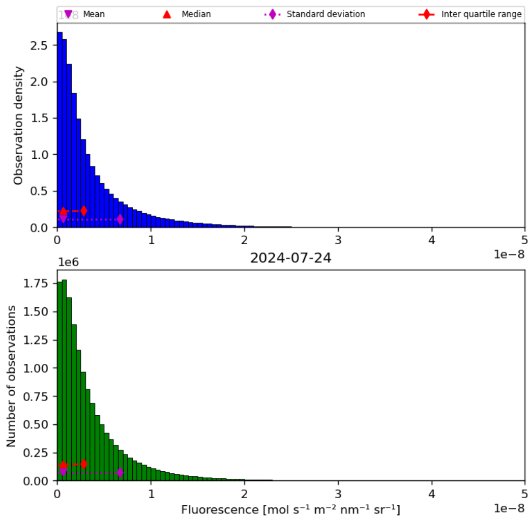
Figure 40: Histogram of “Fluorescence” for 2024-07-23 to 2024-07-25
