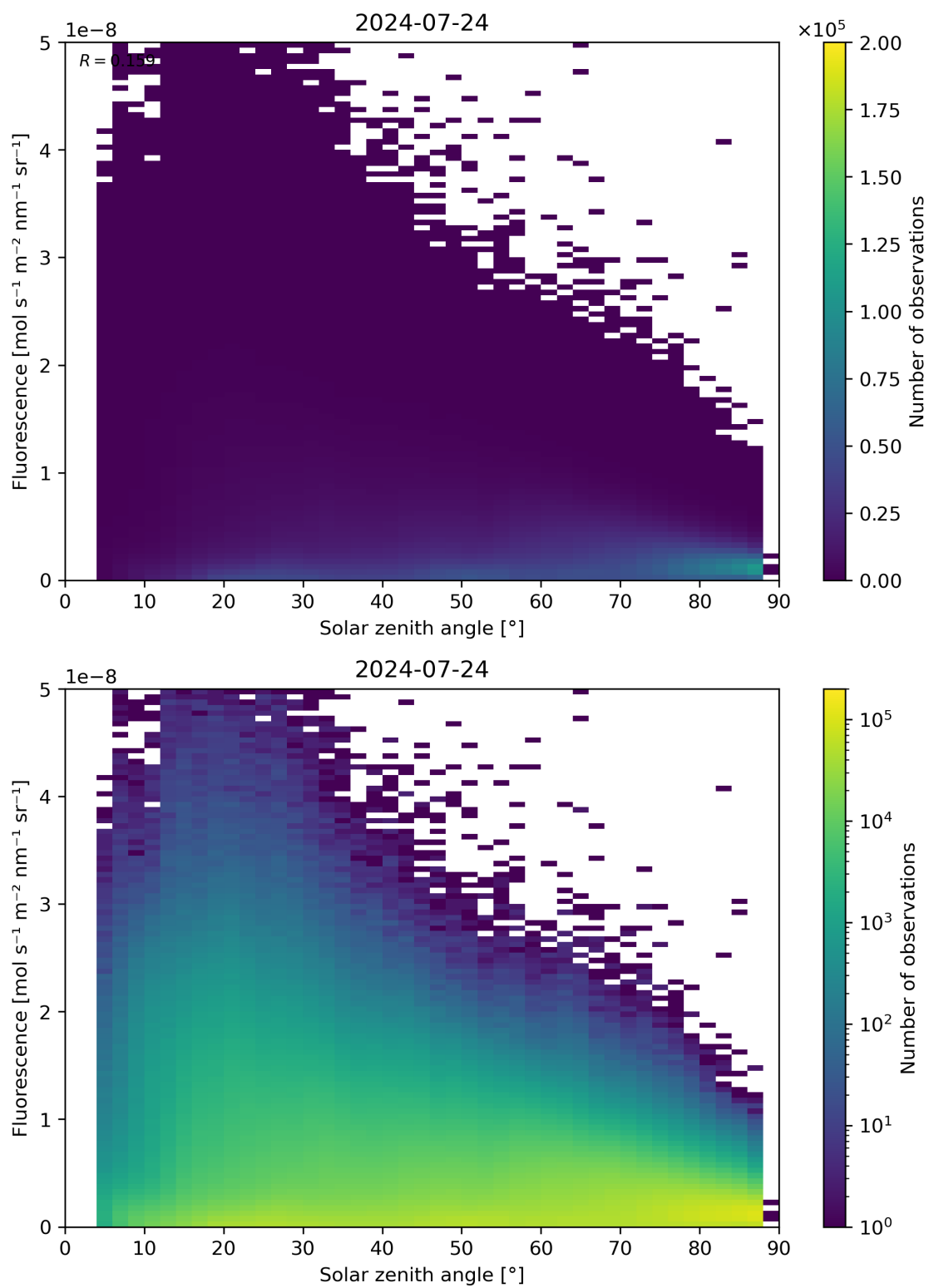
Figure 112: Scatter density plot of “Solar zenith angle” against “Fluorescence” for 2024-07-23 to 2024-07-25.
