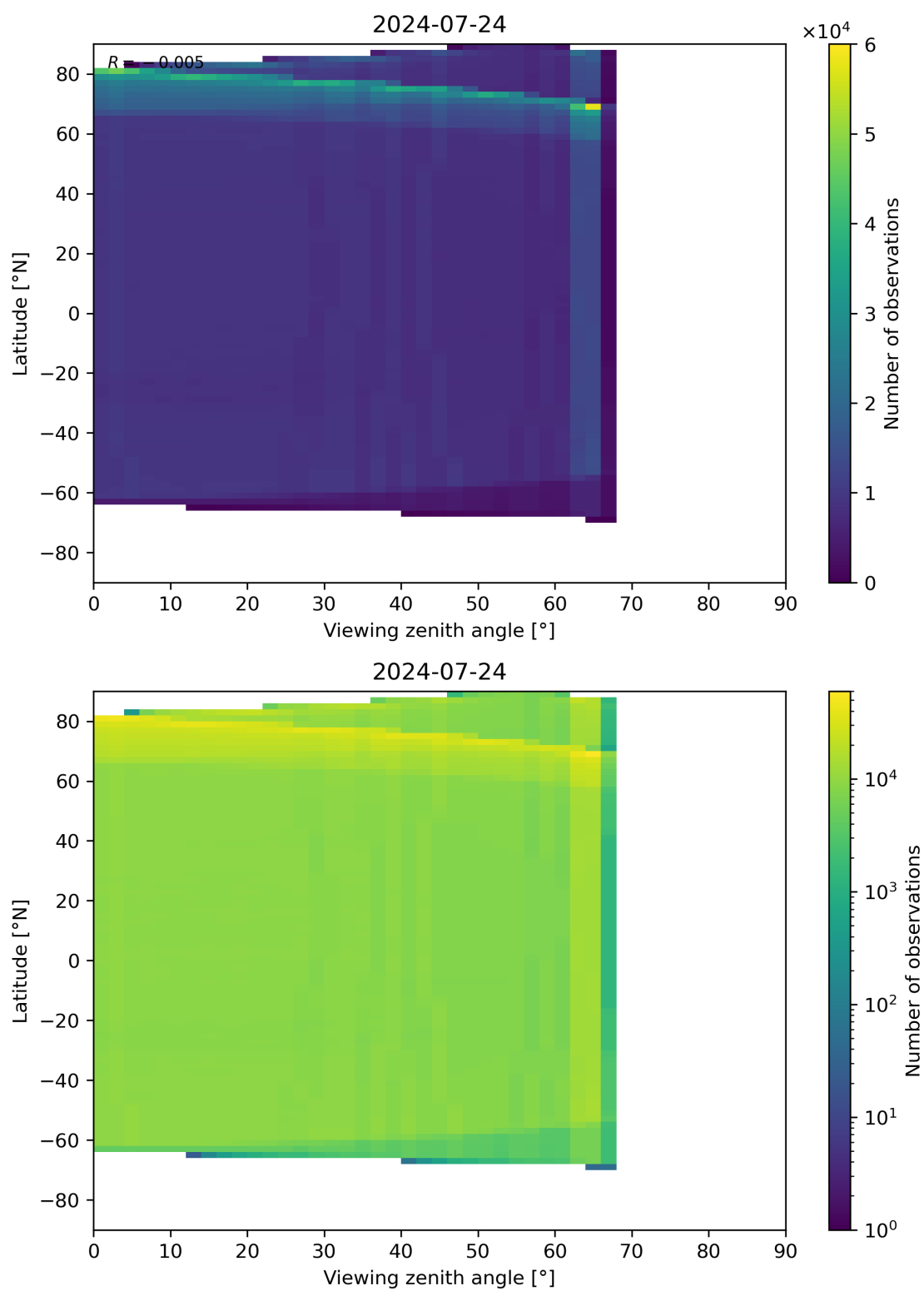
Figure 123: Scatter density plot of “Viewing zenith angle” against “Latitude” for 2024-07-23 to 2024-07-25.
