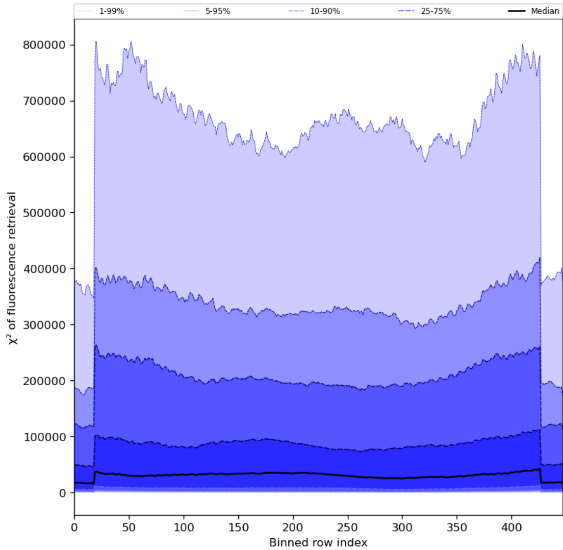
Figure 59: Along track statistics of “ \chi^2 of fluorescence retrieval” for 2024-07-23 to 2024-07-25
