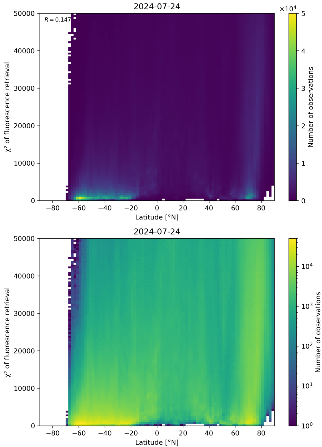
Figure 89: Scatter density plot of “Latitude” against “ \chi^2 of fluorescence retrieval” for 2024-07-23 to 2024-07-25.
