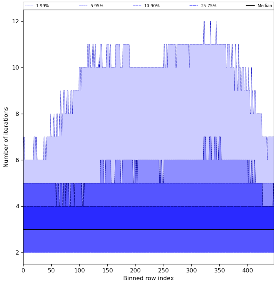
Figure 56: Along track statistics of “Number of iterations” for 2024-07-23 to 2024-07-25
