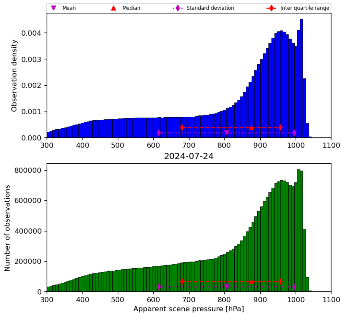
Figure 36: Histogram of “Apparent scene pressure” for 2024-07-23 to 2024-07-25
