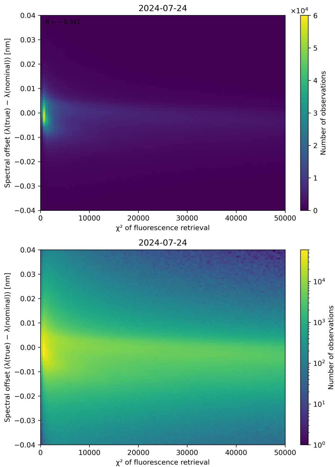
Figure 69: Scatter density plot of " \chi^2 of fluorescence retrieval" against "Spectral offset ( \lambda(\text{true}) - \lambda(\text{nominal}) )" for 2024-07-23 to 2024-07-25.
