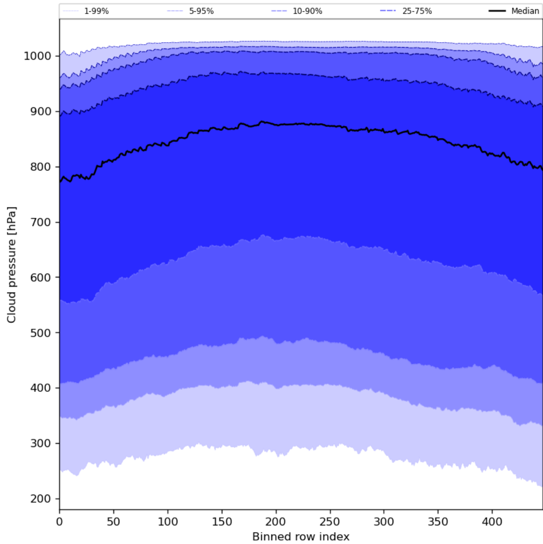
Figure 47: Along track statistics of “Cloud pressure” for 2024-07-23 to 2024-07-25
