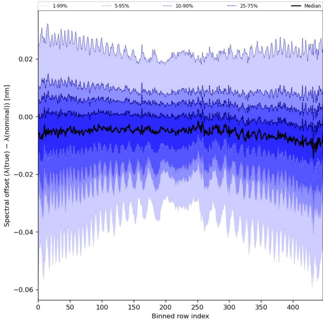
Figure 62: Along track statistics of “Spectral offset ( \lambda(\text{true}) - \lambda(\text{nominal}) )” for 2024-07-23 to 2024-07-25
