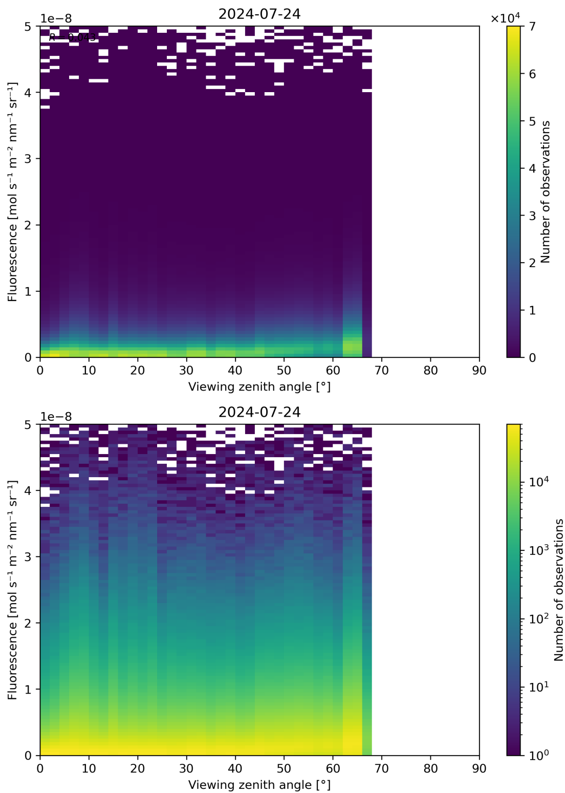
Figure 122: Scatter density plot of “Viewing zenith angle” against “Fluorescence” for 2024-07-23 to 2024-07-25.
