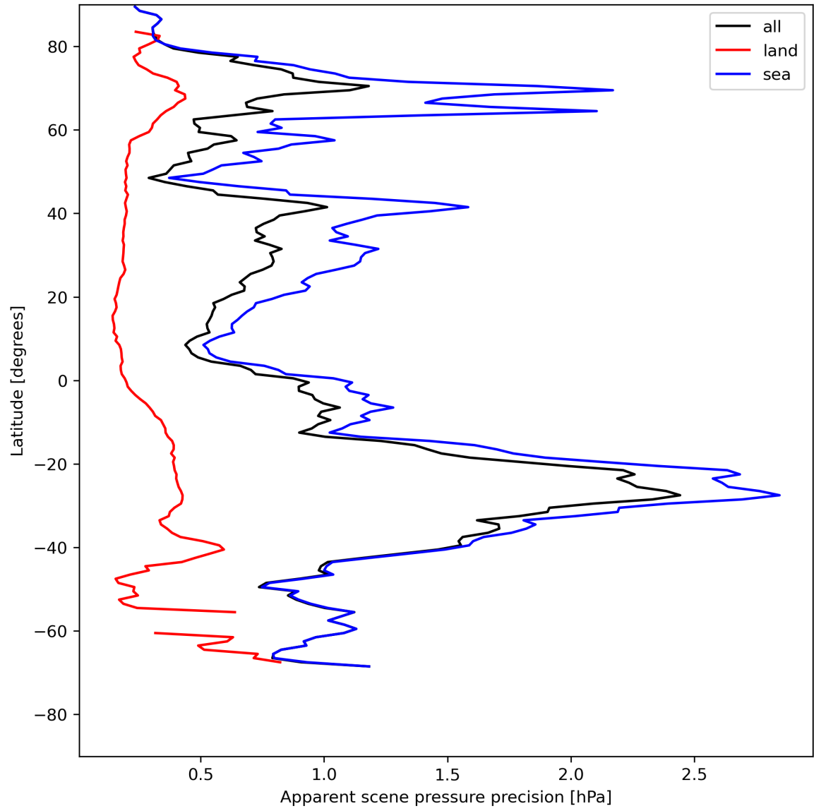
Figure 20: Zonal average of “Apparent scene pressure precision” for 2024-07-23 to 2024-07-25.
