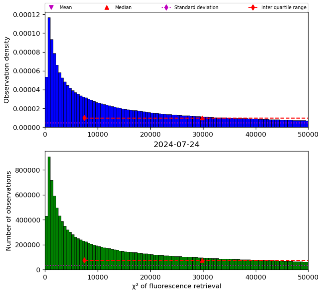
Figure 42: Histogram of “ \chi^2 of fluorescence retrieval” for 2024-07-23 to 2024-07-25
