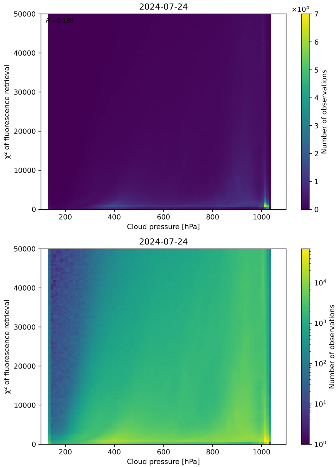
Figure 78: Scatter density plot of “Cloud pressure” against “ \chi^2 of fluorescence retrieval” for 2024-07-23 to 2024-07-25.
