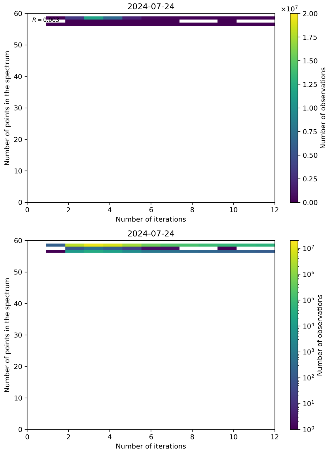
Figure 99: Scatter density plot of “Number of iterations” against “Number of points in the spectrum” for 2024-07-23 to 2024-07-25.
