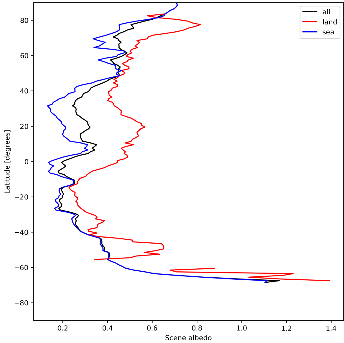
Figure 17: Zonal average of “Scene albedo” for 2024-07-23 to 2024-07-25.
