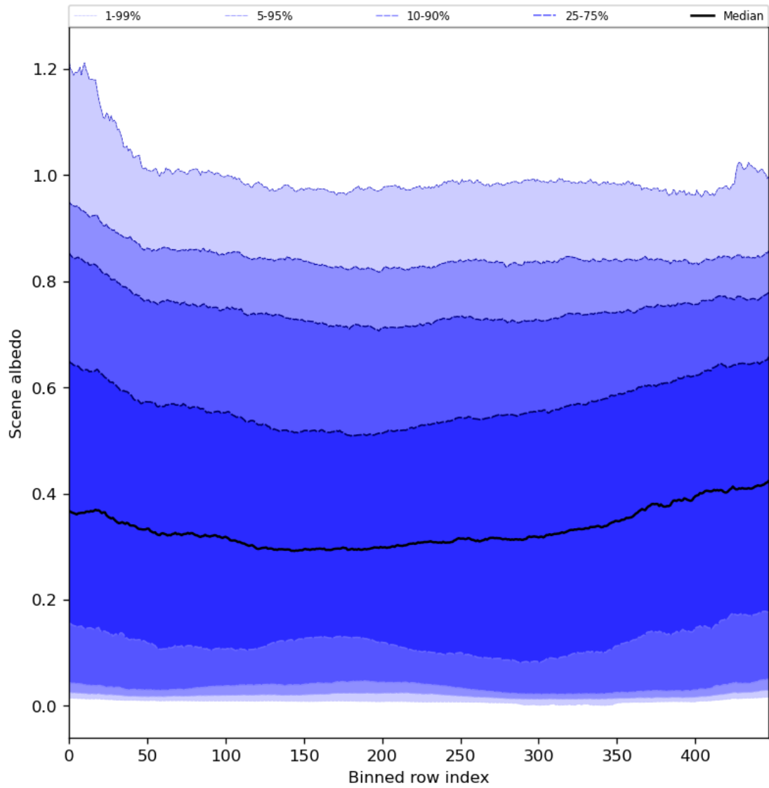
Figure 51: Along track statistics of “Scene albedo” for 2024-07-23 to 2024-07-25
