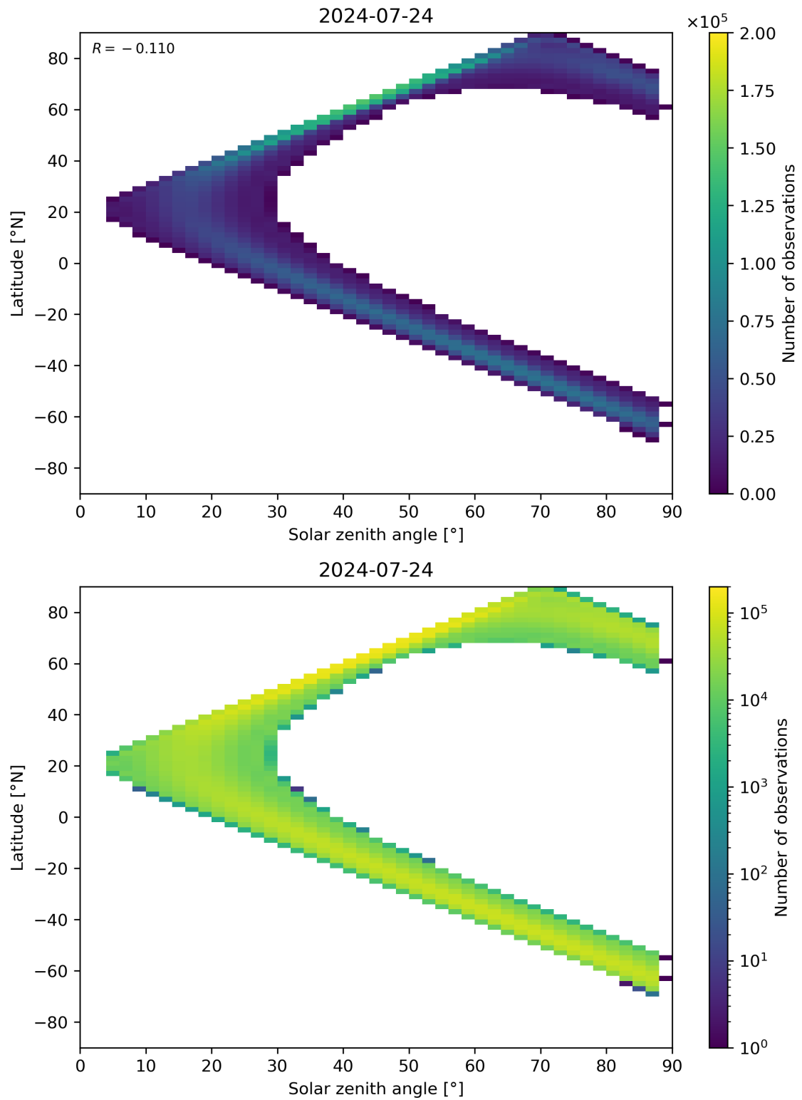
Figure 113: Scatter density plot of “Solar zenith angle” against “Latitude” for 2024-07-23 to 2024-07-25.
