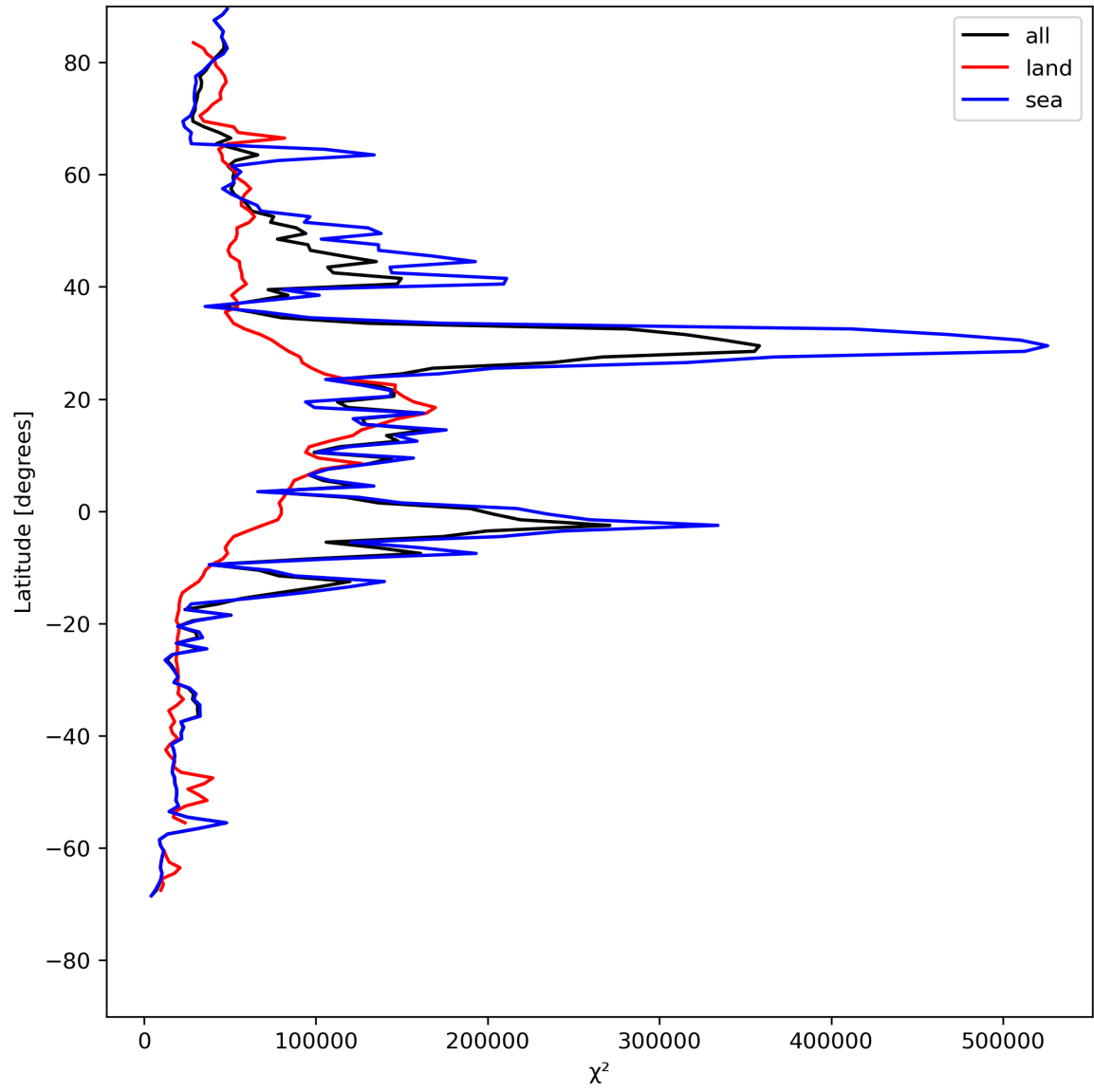
Figure 21: Zonal average of “ \chi^2 ” for 2024-07-23 to 2024-07-25.
