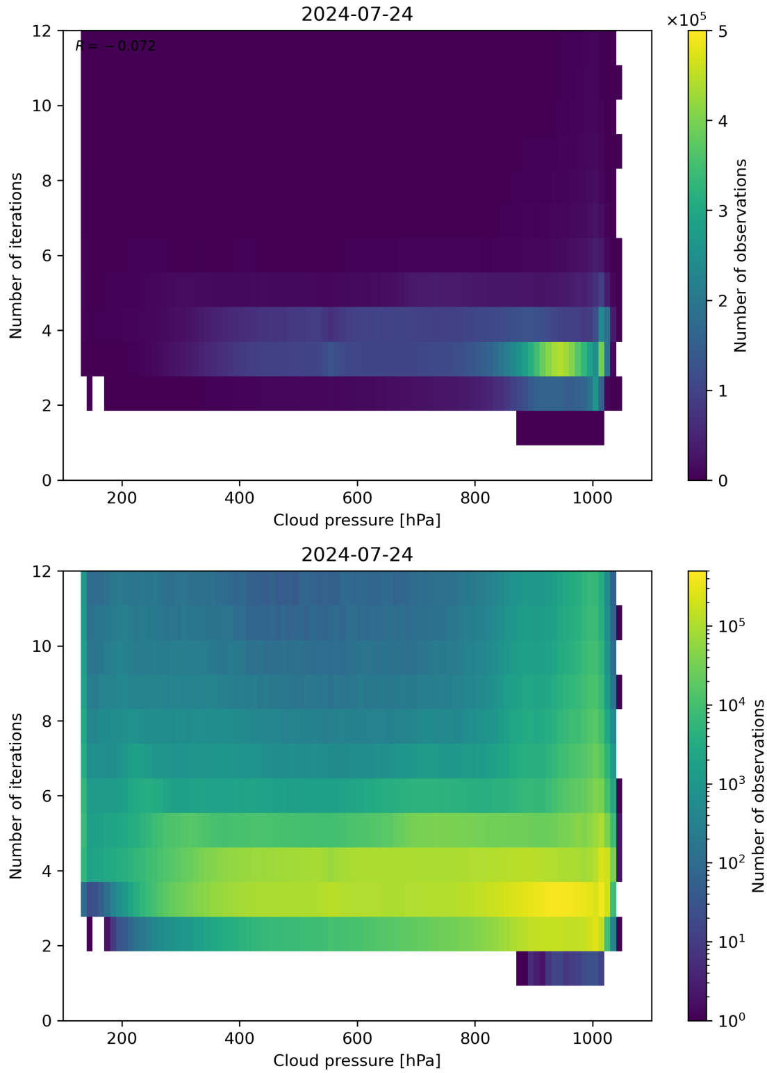
Figure 81: Scatter density plot of “Cloud pressure” against “Number of iterations” for 2024-07-23 to 2024-07-25.
