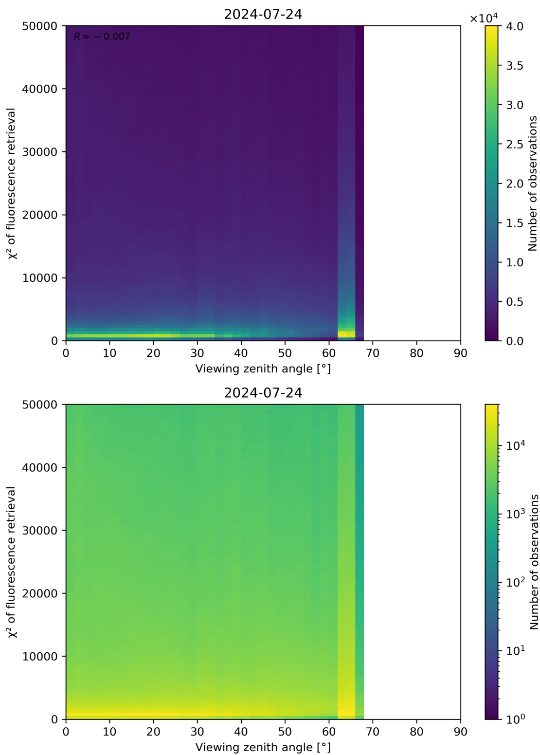
Figure 119: Scatter density plot of “Viewing zenith angle” against “ \chi^2 of fluorescence retrieval” for 2024-07-23 to 2024-07-25.
