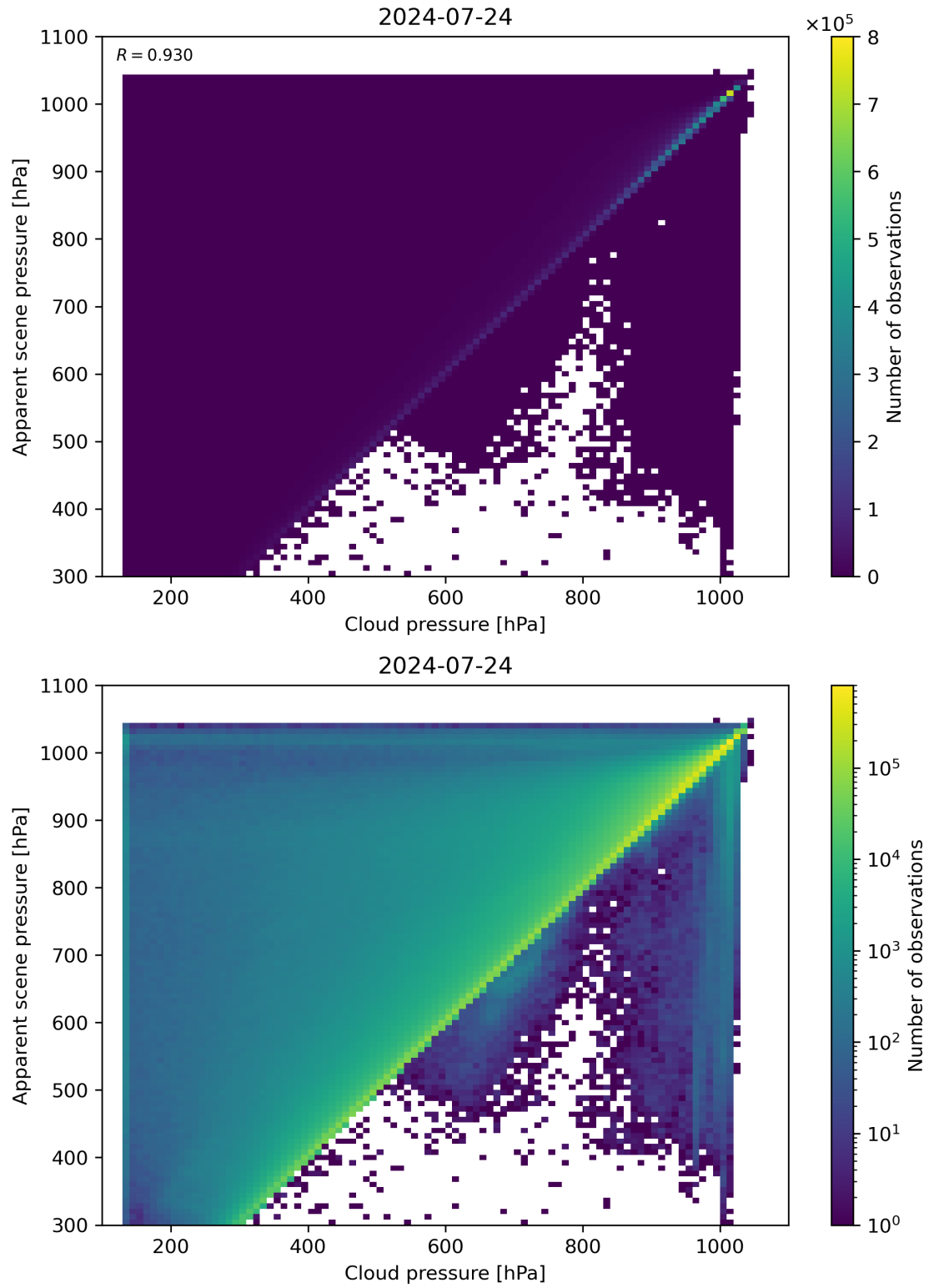
Figure 77: Scatter density plot of “Cloud pressure” against “Apparent scene pressure” for 2024-07-23 to 2024-07-25.
