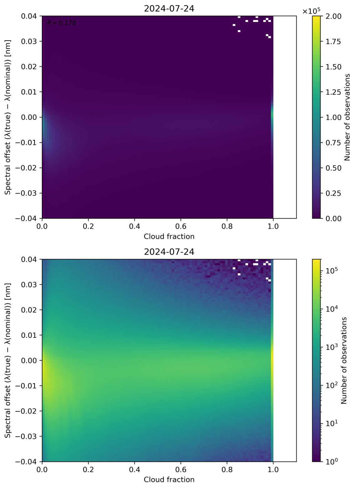
Figure 76: Scatter density plot of “Cloud fraction” against “Spectral offset ( \lambda(\text{true}) - \lambda(\text{nominal}) )” for 2024-07-23 to 2024-07-25.
