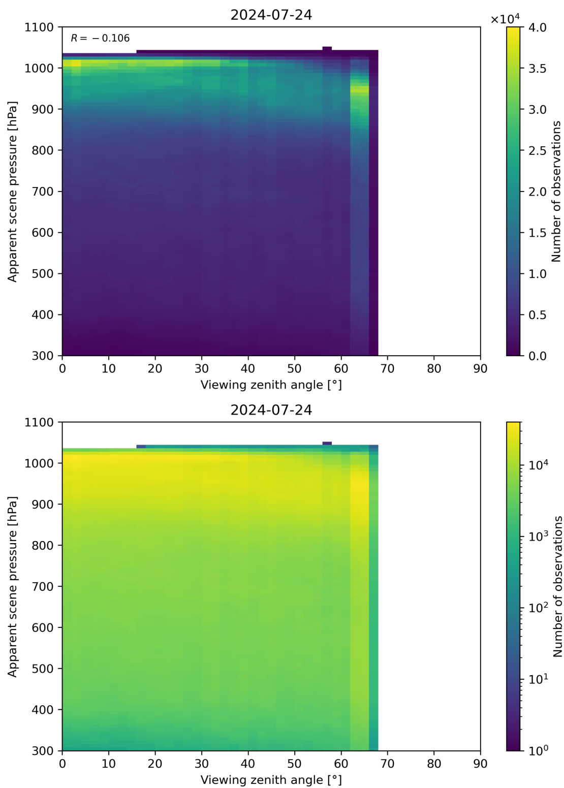
Figure 118: Scatter density plot of “Viewing zenith angle” against “Apparent scene pressure” for 2024-07-23 to 2024-07-25.
