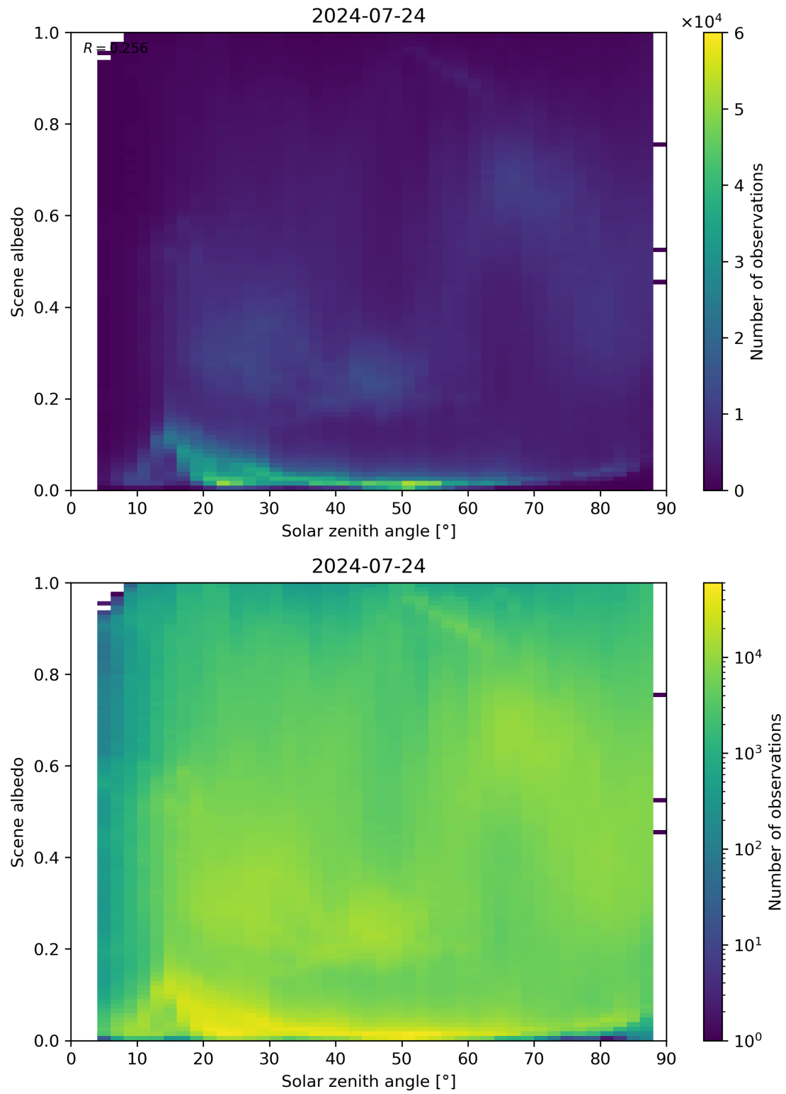
Figure 116: Scatter density plot of “Solar zenith angle” against “Scene albedo” for 2024-07-23 to 2024-07-25.
