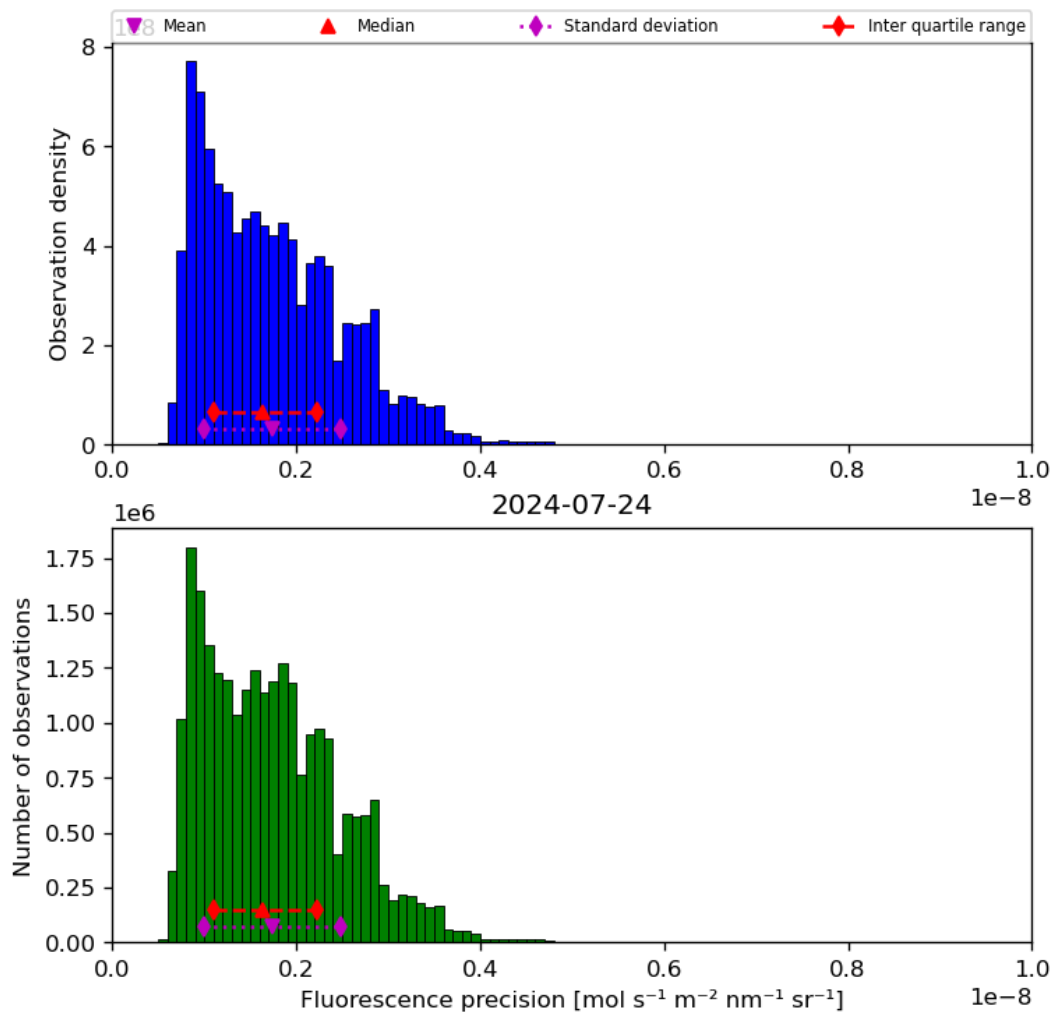
Figure 41: Histogram of “Fluorescence precision” for 2024-07-23 to 2024-07-25
