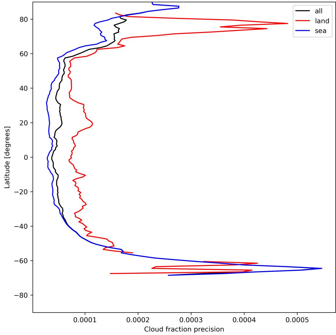
Figure 16: Zonal average of “Cloud fraction precision” for 2024-07-23 to 2024-07-25.
