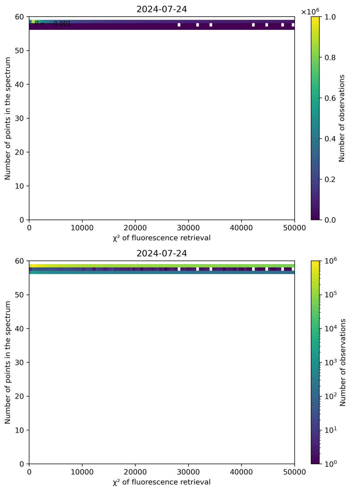
Figure 68: Scatter density plot of “ \chi^2 of fluorescence retrieval” against “Number of points in the spectrum” for 2024-07-23 to 2024-07-25.
