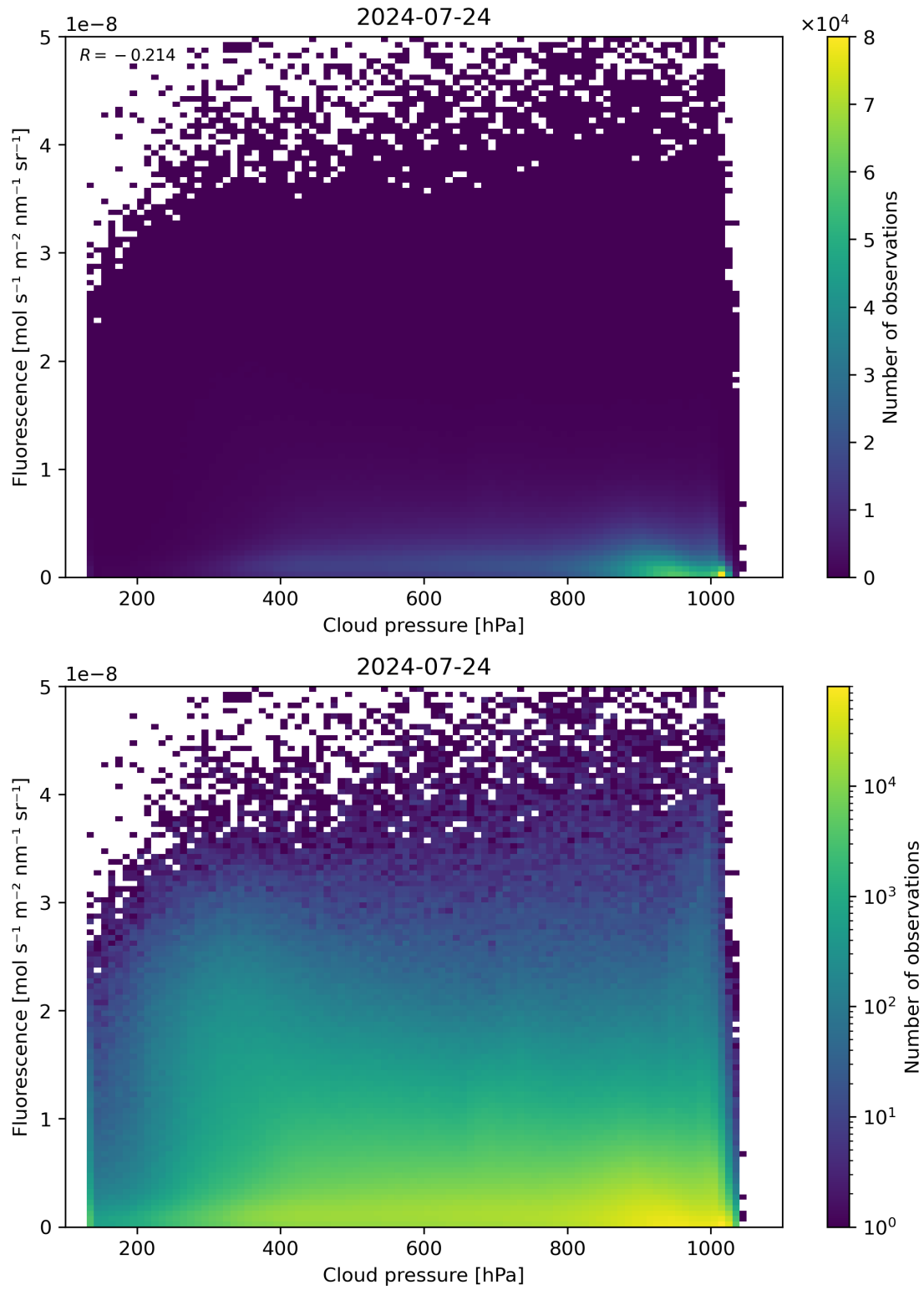
Figure 80: Scatter density plot of “Cloud pressure” against “Fluorescence” for 2024-07-23 to 2024-07-25.
