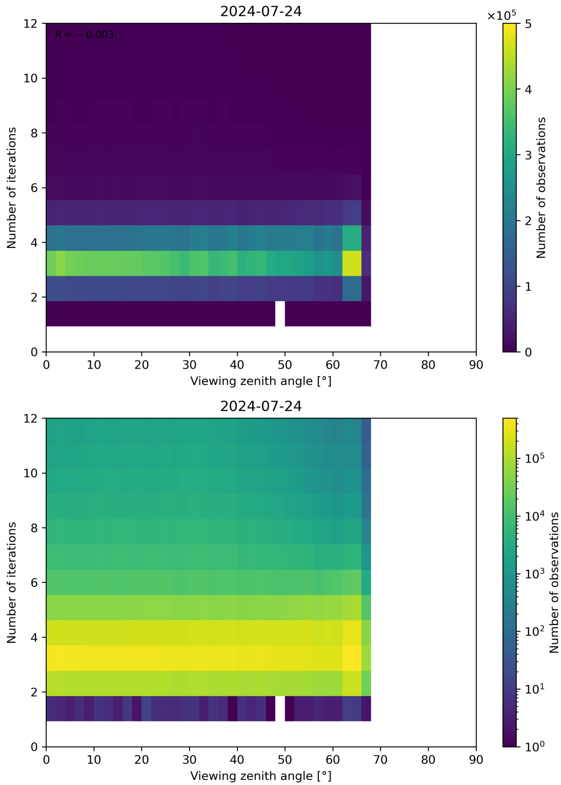
Figure 124: Scatter density plot of “Viewing zenith angle” against “Number of iterations” for 2024-07-23 to 2024-07-25.
