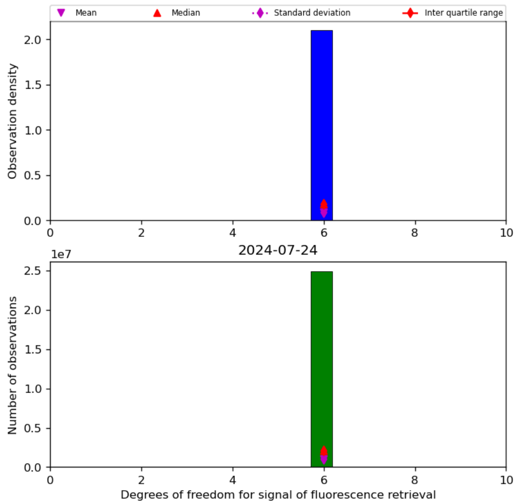
Figure 43: Histogram of “Degrees of freedom for signal of fluorescence retrieval” for 2024-07-23 to 2024-07-25
