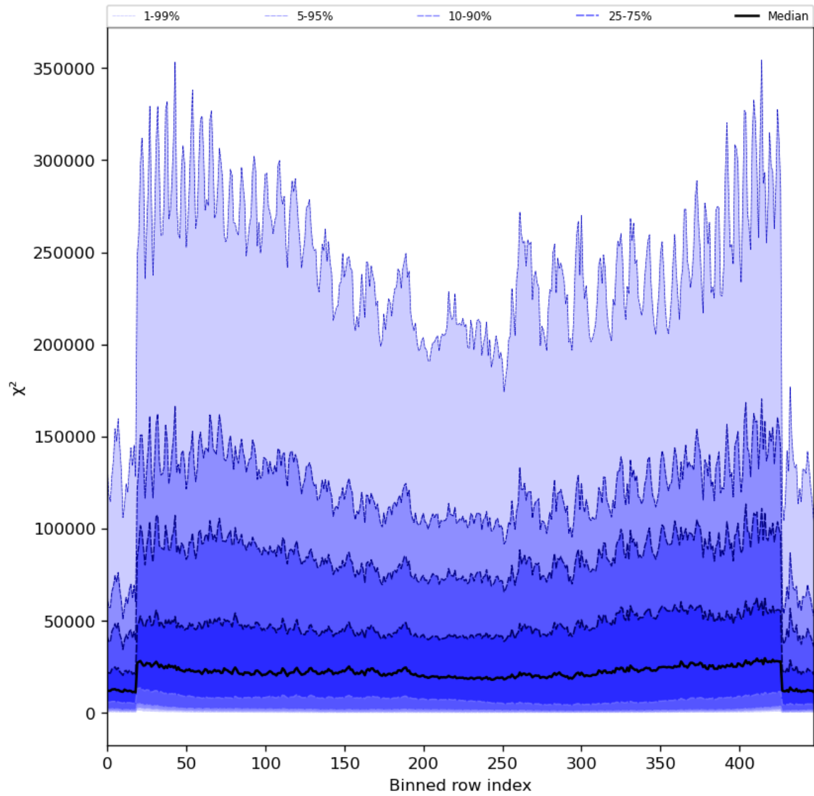
Figure 55: Along track statistics of “ \chi^2 ” for 2024-07-23 to 2024-07-25
