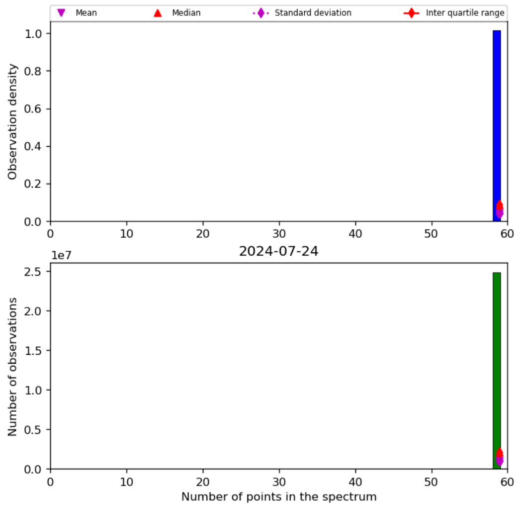
Figure 44: Histogram of “Number of points in the spectrum” for 2024-07-23 to 2024-07-25
