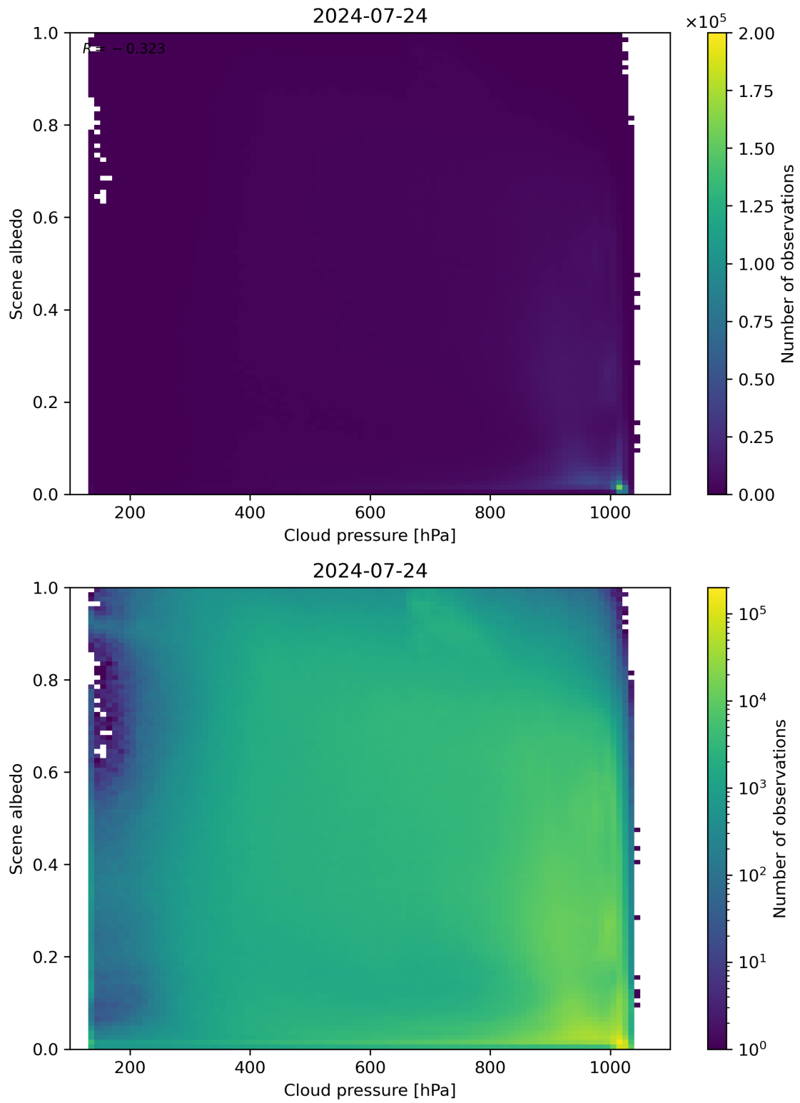
Figure 83: Scatter density plot of “Cloud pressure” against “Scene albedo” for 2024-07-23 to 2024-07-25.
