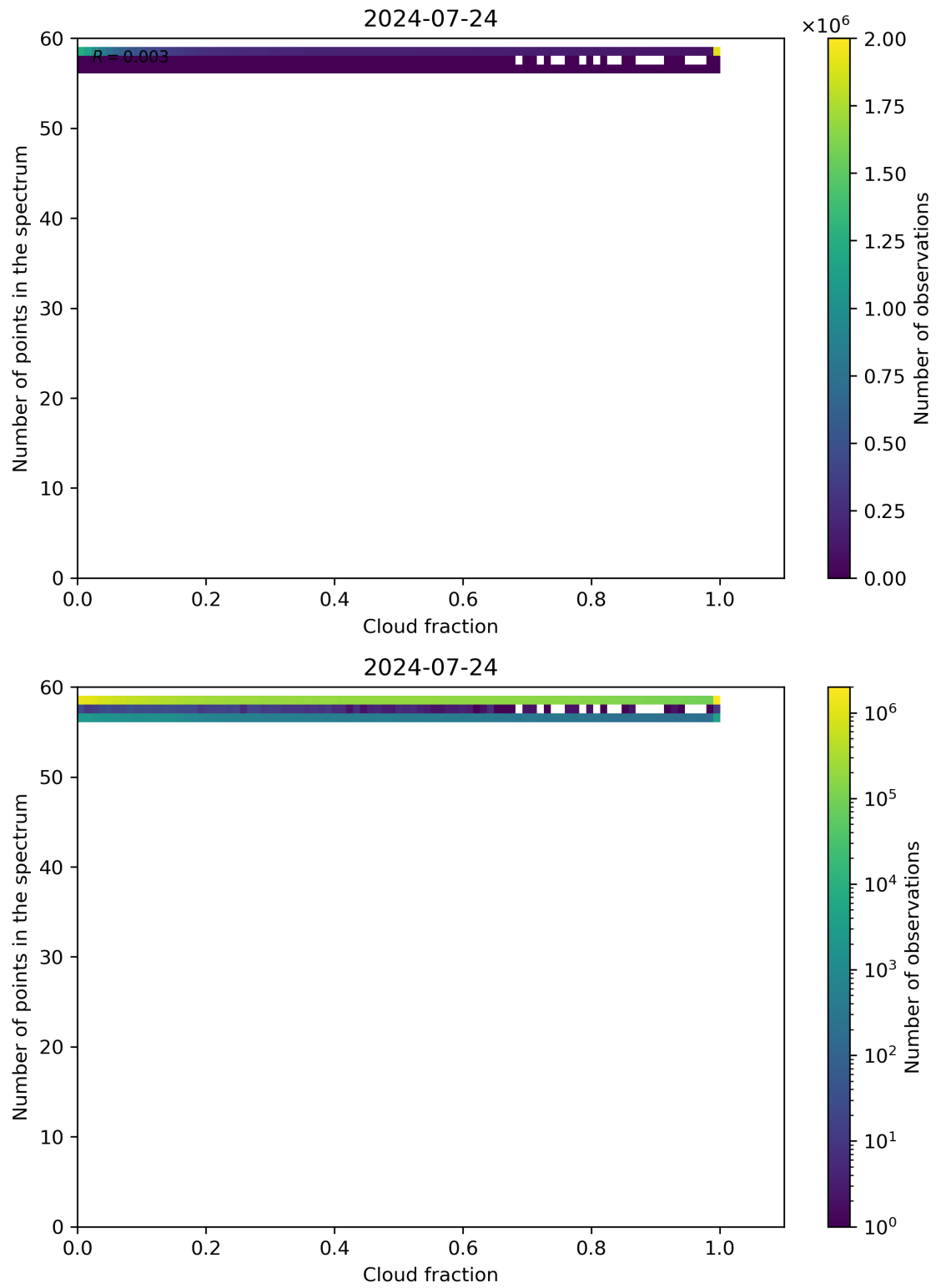
Figure 74: Scatter density plot of “Cloud fraction” against “Number of points in the spectrum” for 2024-07-23 to 2024-07-25.
