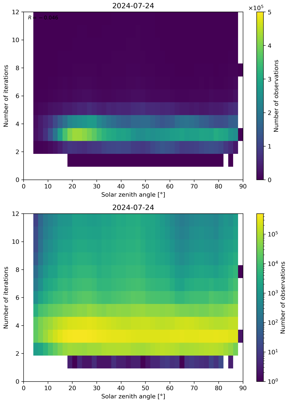
Figure 114: Scatter density plot of “Solar zenith angle” against “Number of iterations” for 2024-07-23 to 2024-07-25.
