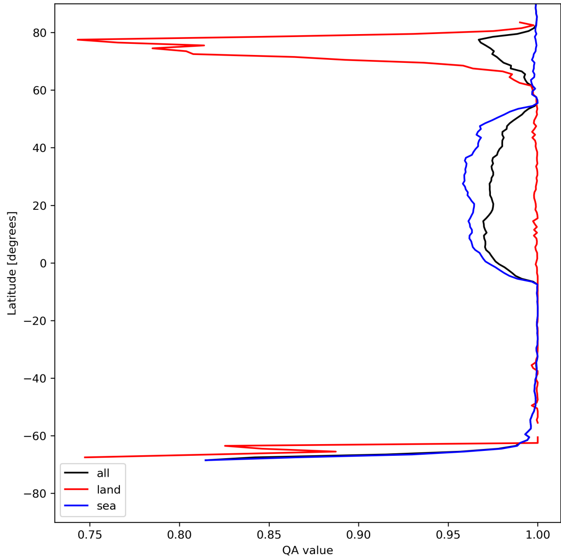
Figure 12: Zonal average of “QA value” for 2024-07-23 to 2024-07-25.
