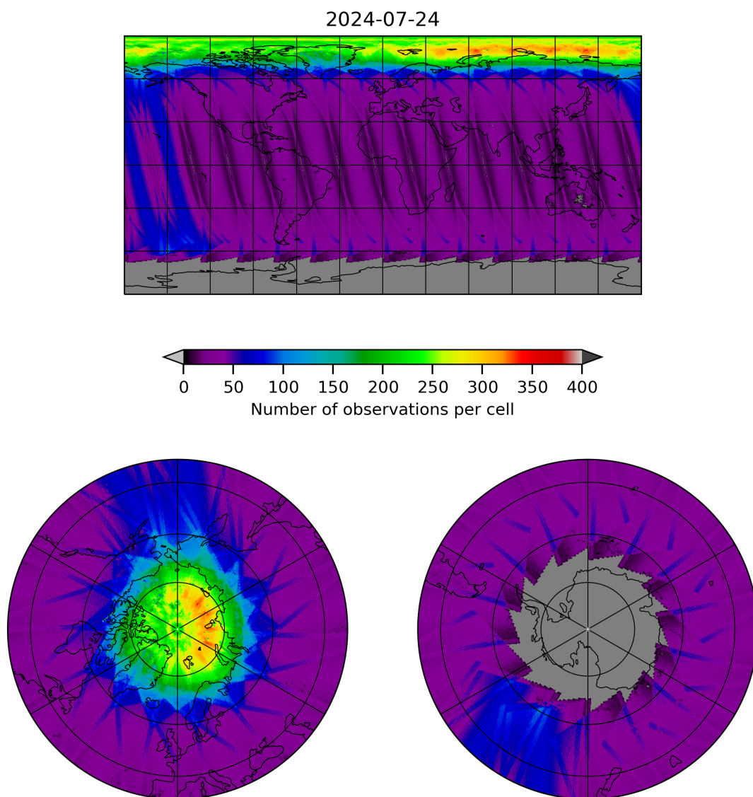
Figure 11: Map of the number of observations for 2024-07-23 to 2024-07-25
