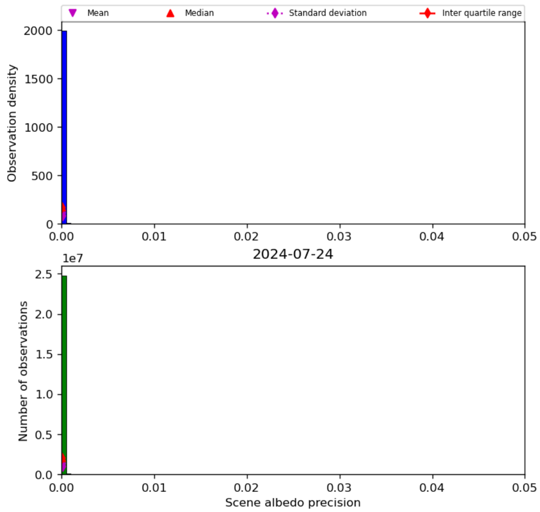
Figure 35: Histogram of “Scene albedo precision” for 2024-07-23 to 2024-07-25
