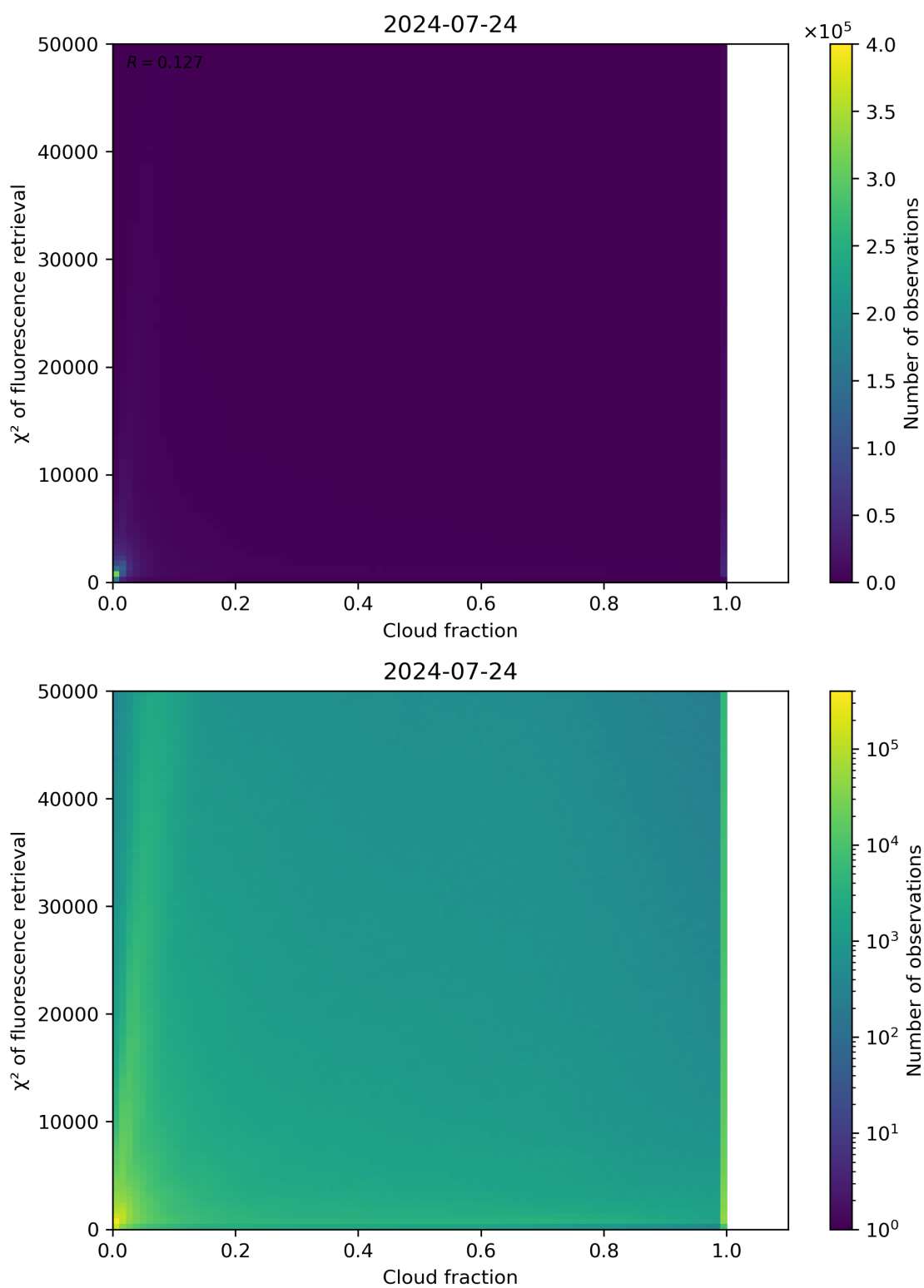
Figure 71: Scatter density plot of “Cloud fraction” against “ \chi^2 of fluorescence retrieval” for 2024-07-23 to 2024-07-25.
