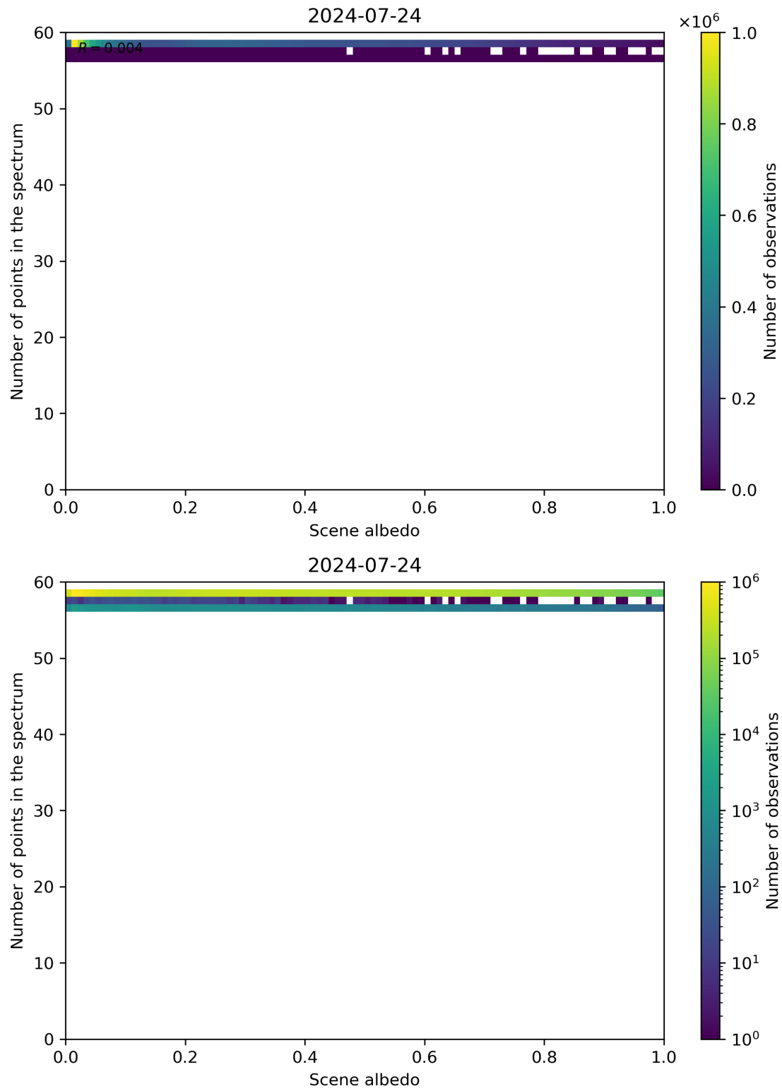
Figure 106: Scatter density plot of “Scene albedo” against “Number of points in the spectrum” for 2024-07-23 to 2024-07-25.
