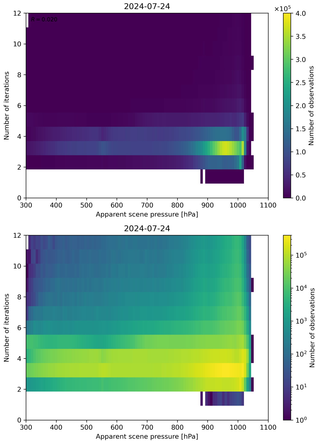
Figure 65: Scatter density plot of “Apparent scene pressure” against “Number of iterations” for 2024-07-23 to 2024-07-25.
