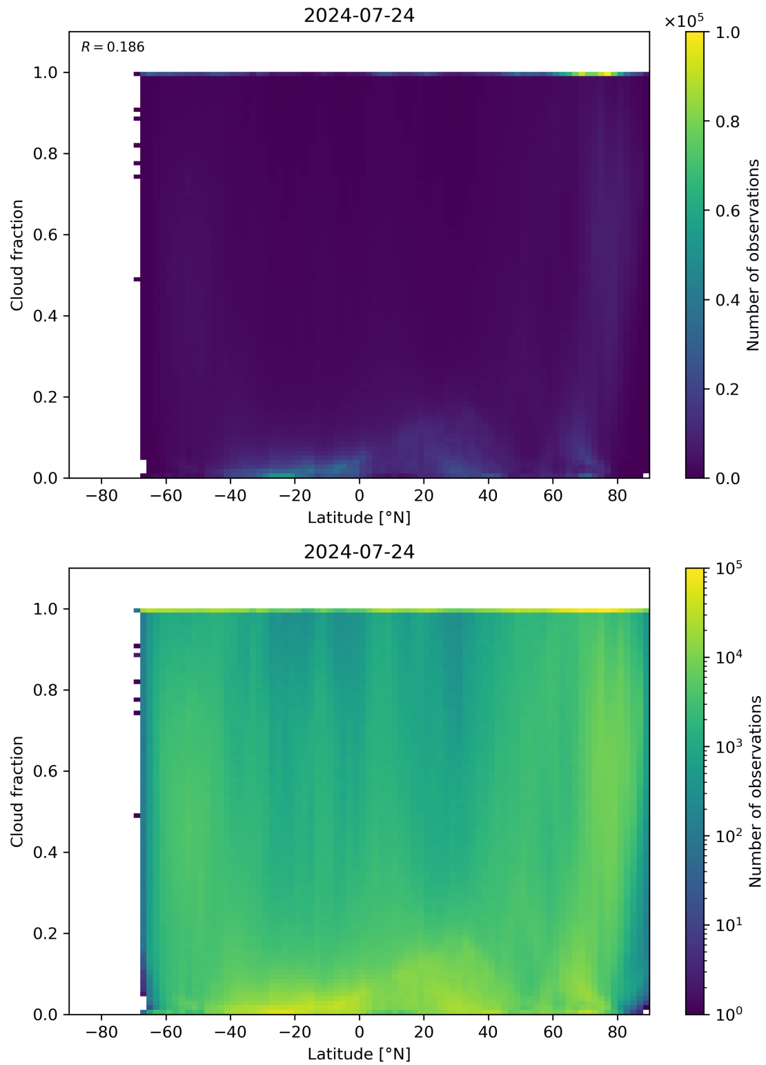
Figure 90: Scatter density plot of “Latitude” against “Cloud fraction” for 2024-07-23 to 2024-07-25.
