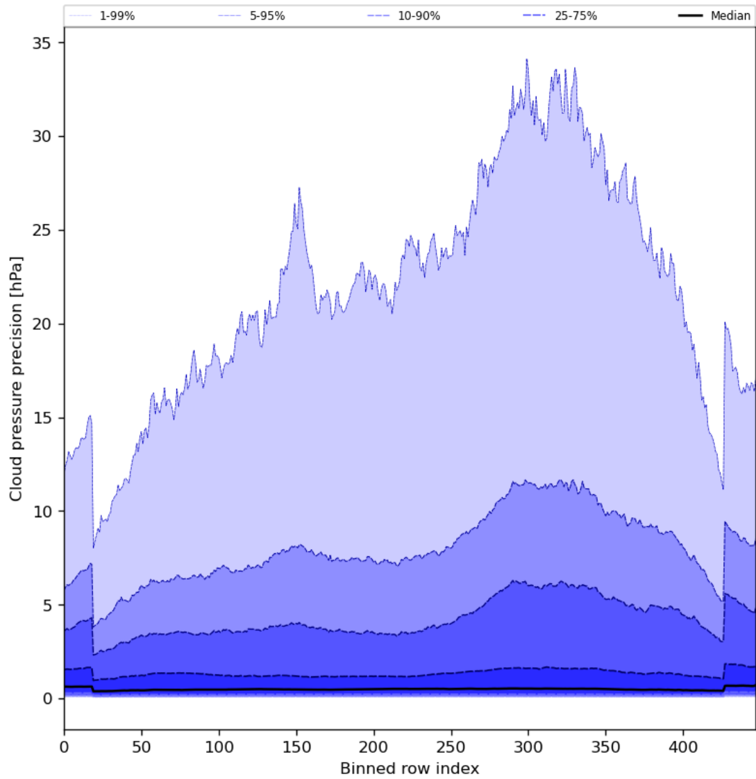
Figure 48: Along track statistics of “Cloud pressure precision” for 2024-07-23 to 2024-07-25
