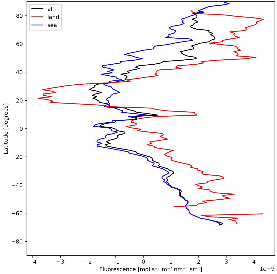
Figure 23: Zonal average of “Fluorescence” for 2024-07-23 to 2024-07-25.
