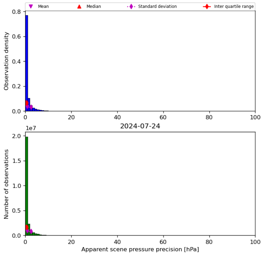
Figure 37: Histogram of “Apparent scene pressure precision” for 2024-07-23 to 2024-07-25
