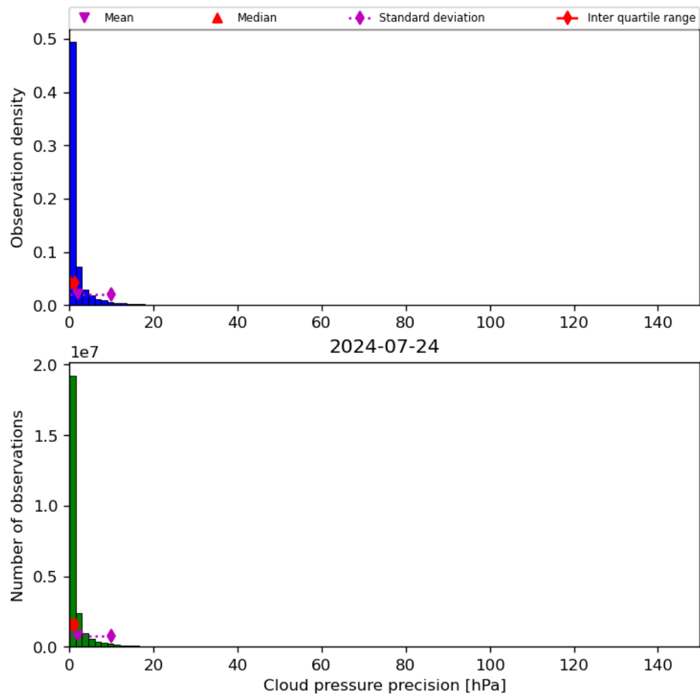
Figure 31: Histogram of “Cloud pressure precision” for 2024-07-23 to 2024-07-25
