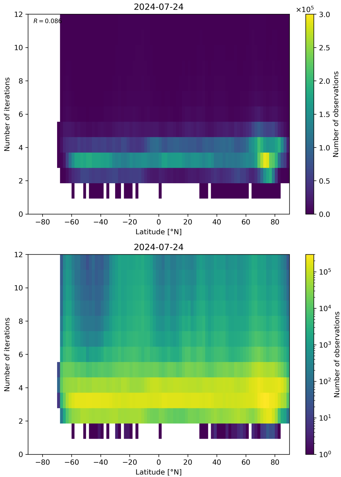
Figure 93: Scatter density plot of “Latitude” against “Number of iterations” for 2024-07-23 to 2024-07-25.
