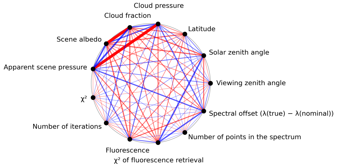
Figure 1: Map of correlation graph for 2024-07-23 to 2024-07-25.
