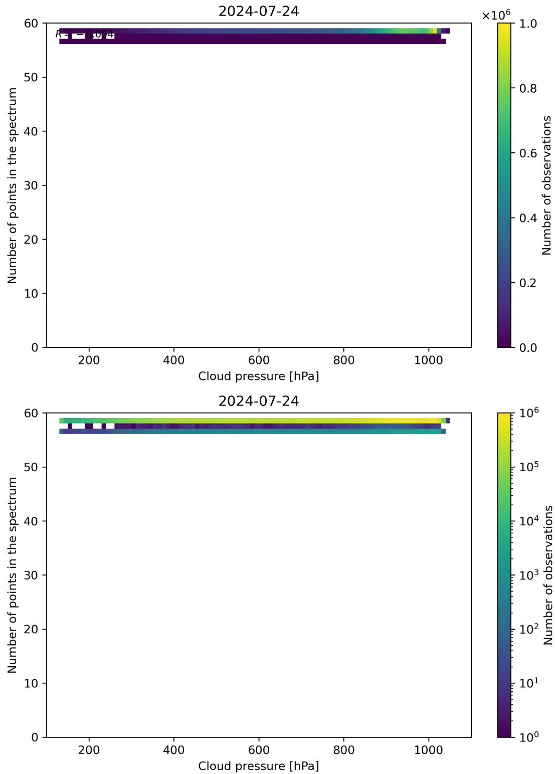
Figure 82: Scatter density plot of “Cloud pressure” against “Number of points in the spectrum” for 2024-07-23 to 2024-07-25.
