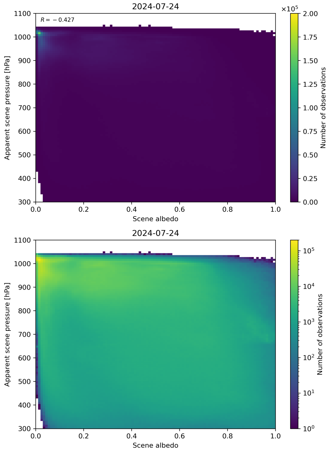
Figure 102: Scatter density plot of “Scene albedo” against “Apparent scene pressure” for 2024-07-23 to 2024-07-25.
