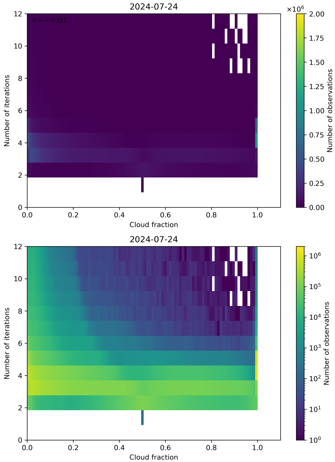
Figure 73: Scatter density plot of “Cloud fraction” against “Number of iterations” for 2024-07-23 to 2024-07-25.
