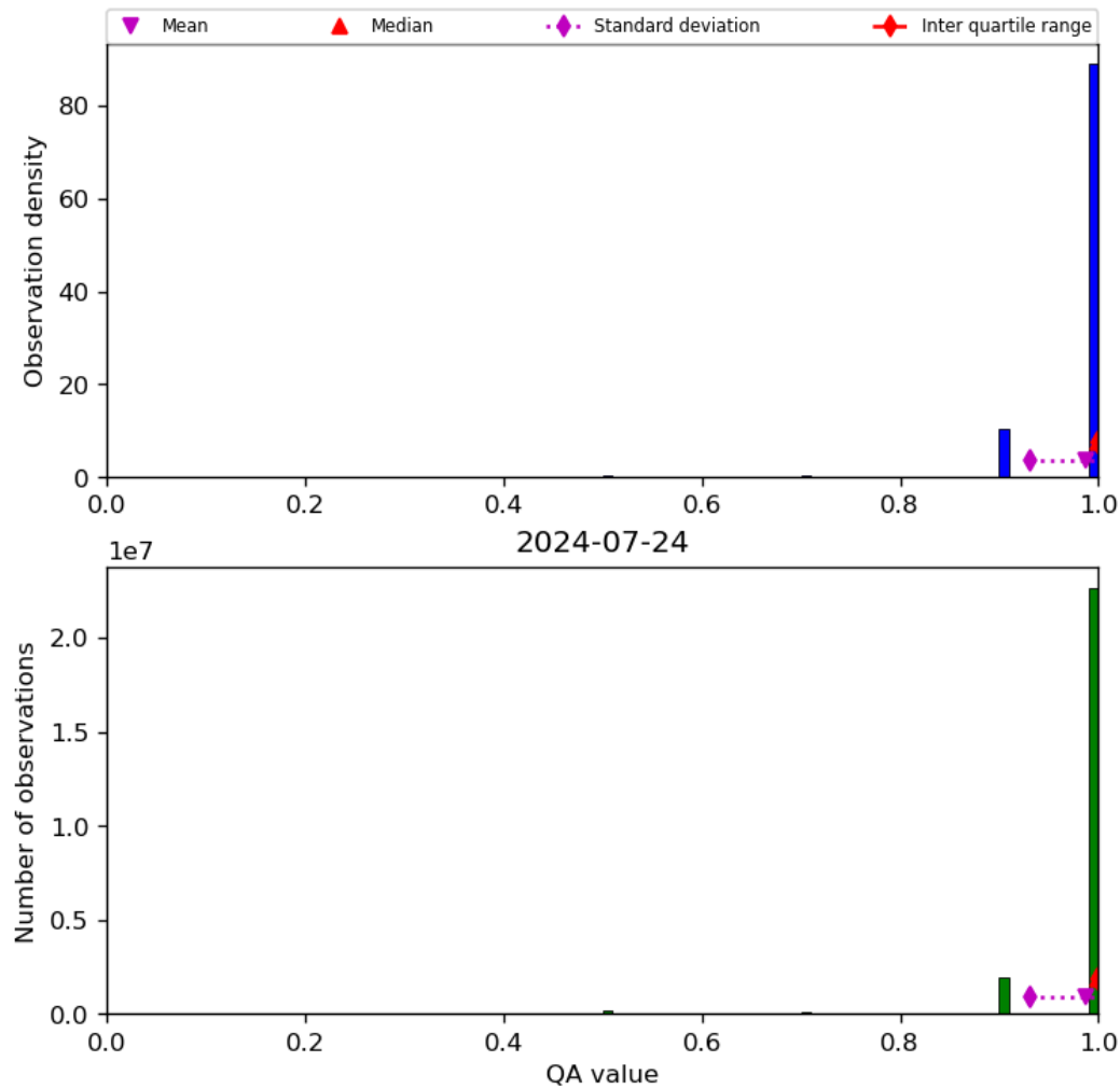
Figure 29: Histogram of “QA value” for 2024-07-23 to 2024-07-25
