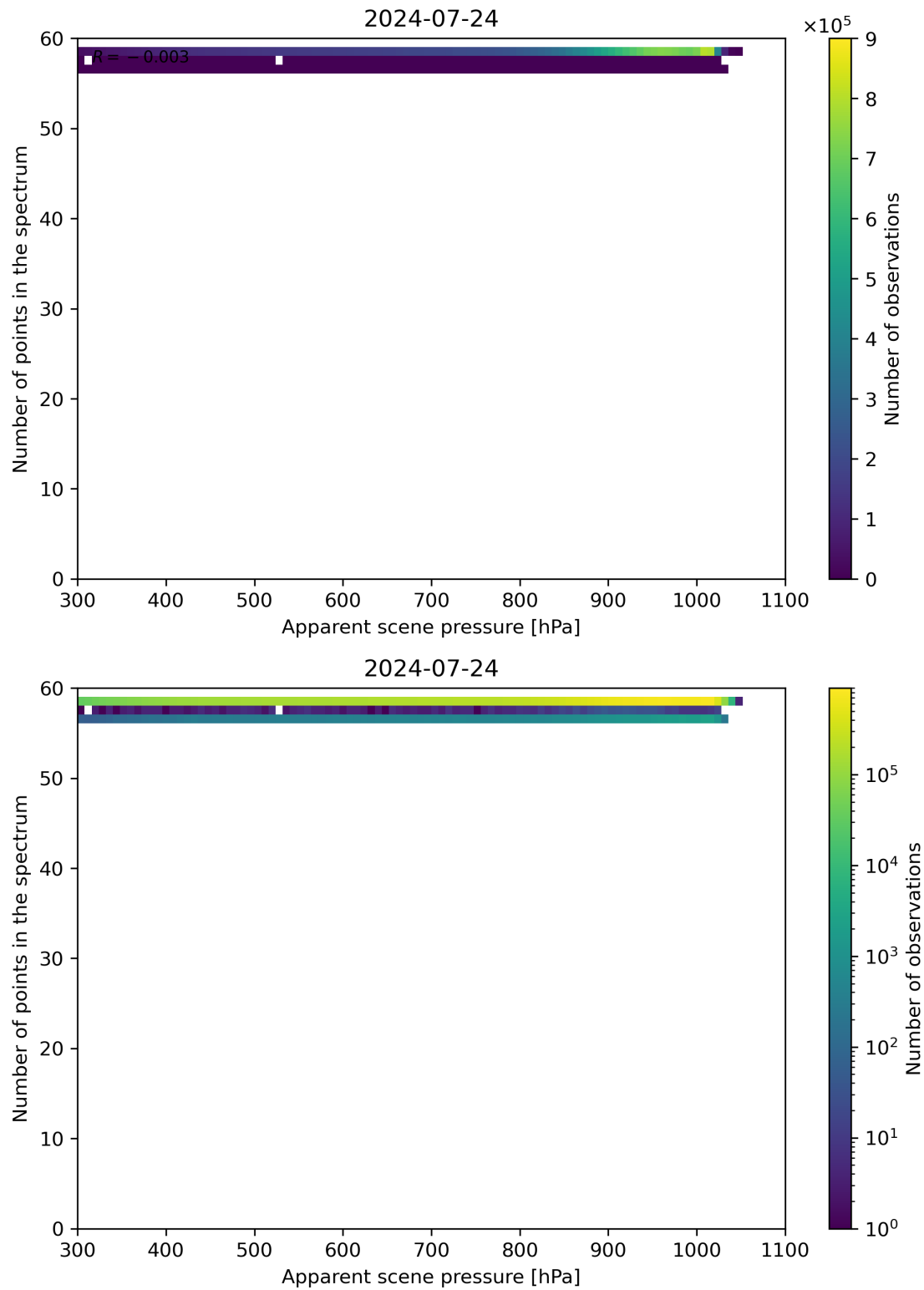
Figure 66: Scatter density plot of “Apparent scene pressure” against “Number of points in the spectrum” for 2024-07-23 to 2024-07-25.
