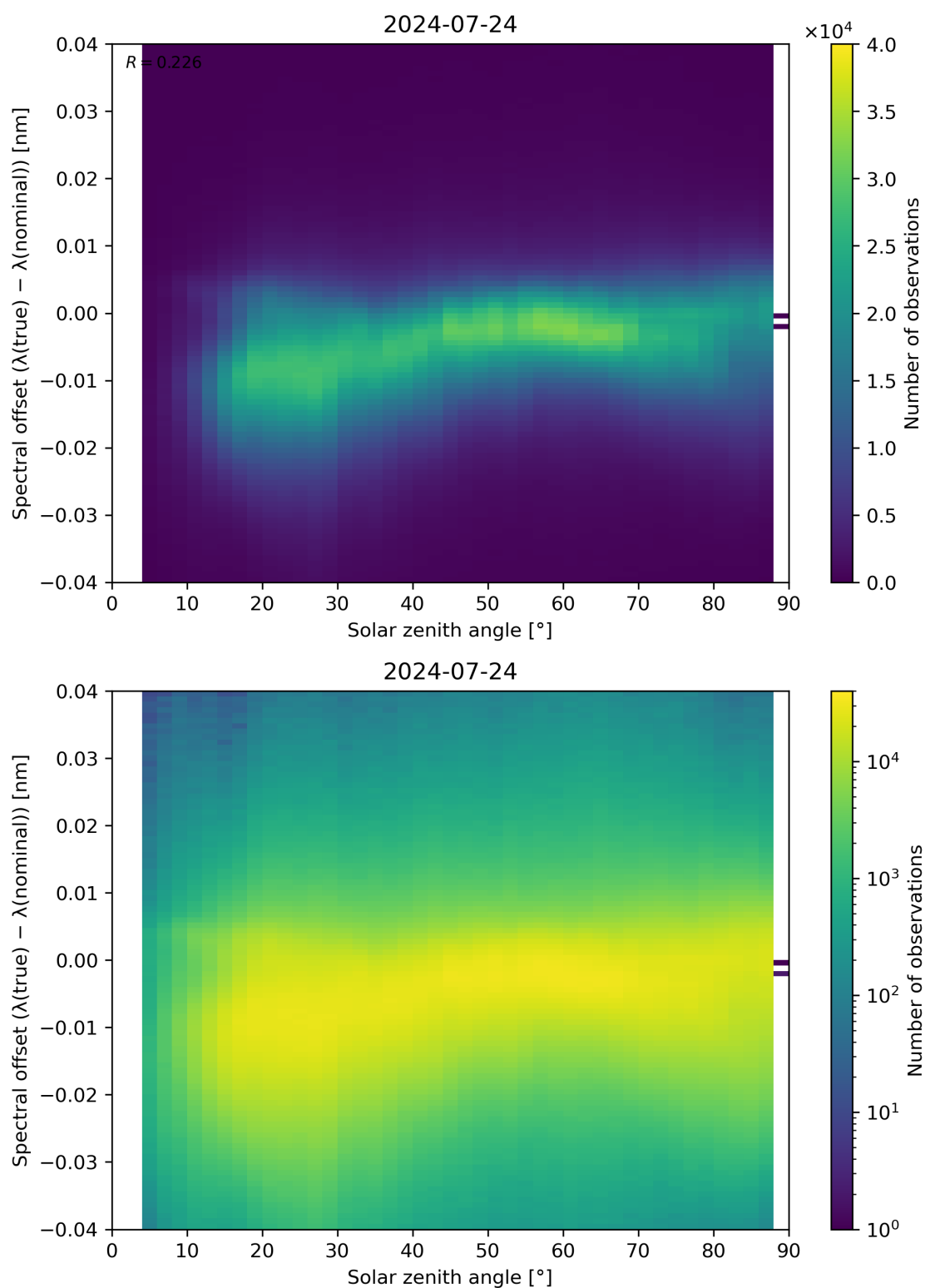
Figure 117: Scatter density plot of “Solar zenith angle” against “Spectral offset ( \lambda(\text{true}) - \lambda(\text{nominal}) )” for 2024-07-23 to 2024-07-25.
