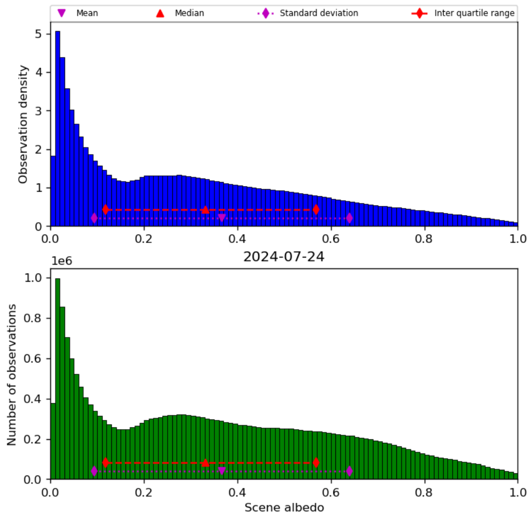
Figure 34: Histogram of “Scene albedo” for 2024-07-23 to 2024-07-25
