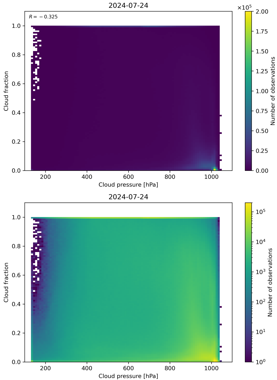
Figure 79: Scatter density plot of “Cloud pressure” against “Cloud fraction” for 2024-07-23 to 2024-07-25.
