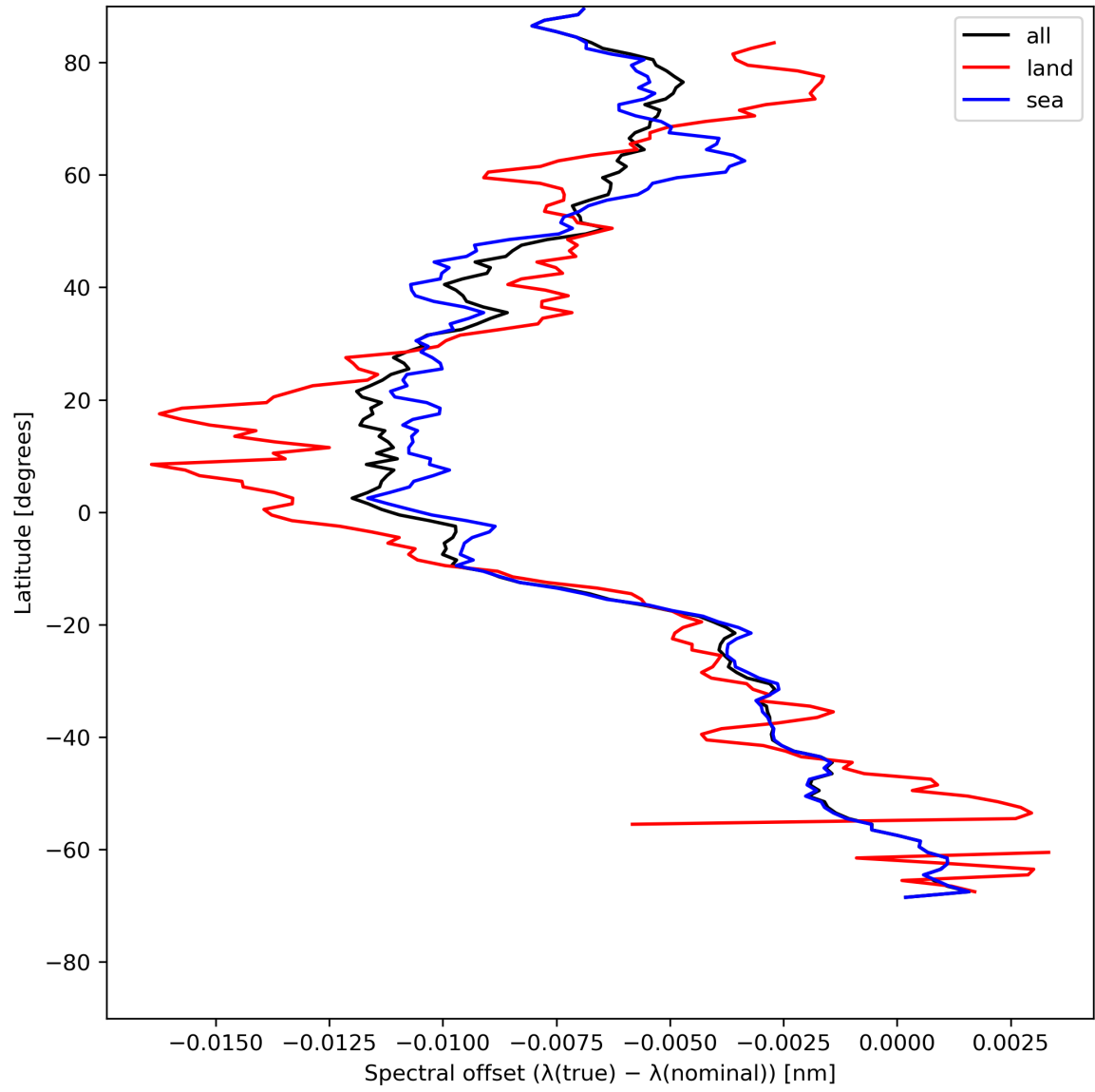
Figure 28: Zonal average of “Spectral offset ( \lambda(\text{true}) - \lambda(\text{nominal}) )” for 2024-07-23 to 2024-07-25.
