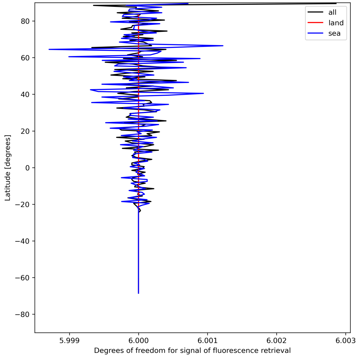
Figure 26: Zonal average of “Degrees of freedom for signal of fluorescence retrieval” for 2024-07-23 to 2024-07-25.
