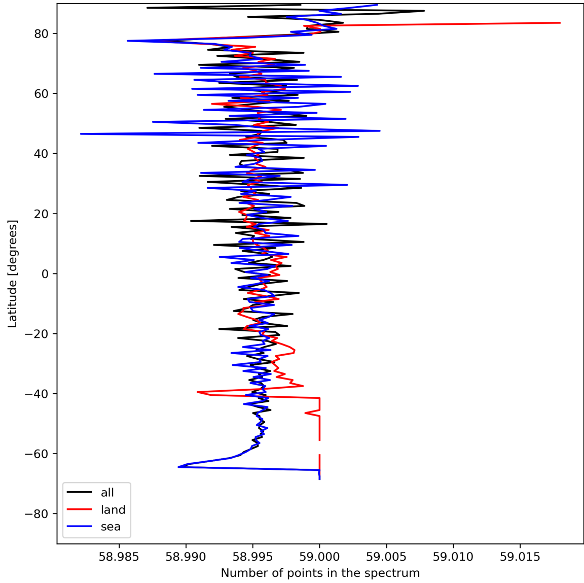
Figure 27: Zonal average of “Number of points in the spectrum” for 2024-07-23 to 2024-07-25.
