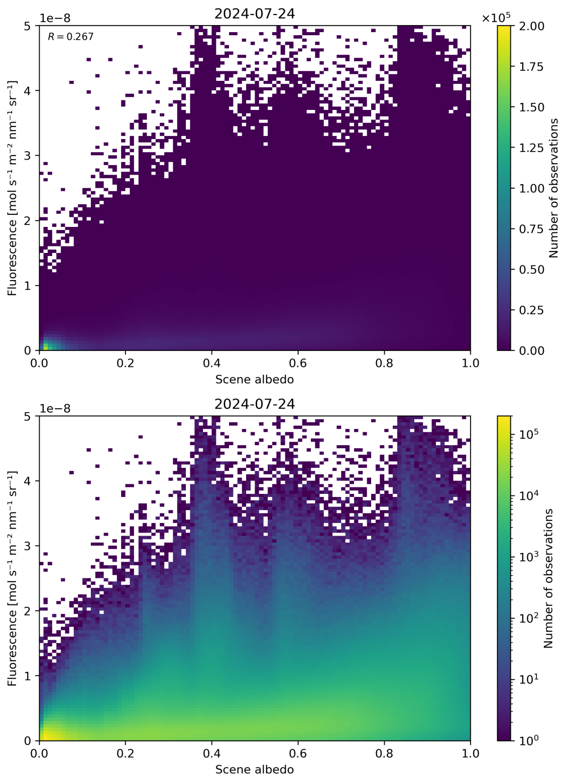
Figure 104: Scatter density plot of “Scene albedo” against “Fluorescence” for 2024-07-23 to 2024-07-25.
