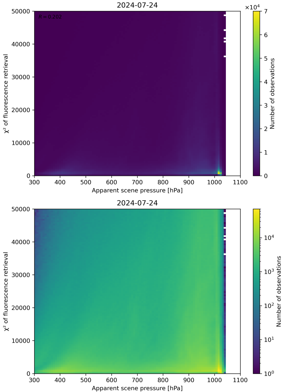
Figure 63: Scatter density plot of “Apparent scene pressure” against “ \chi^2 of fluorescence retrieval” for 2024-07-23 to 2024-07-25.
