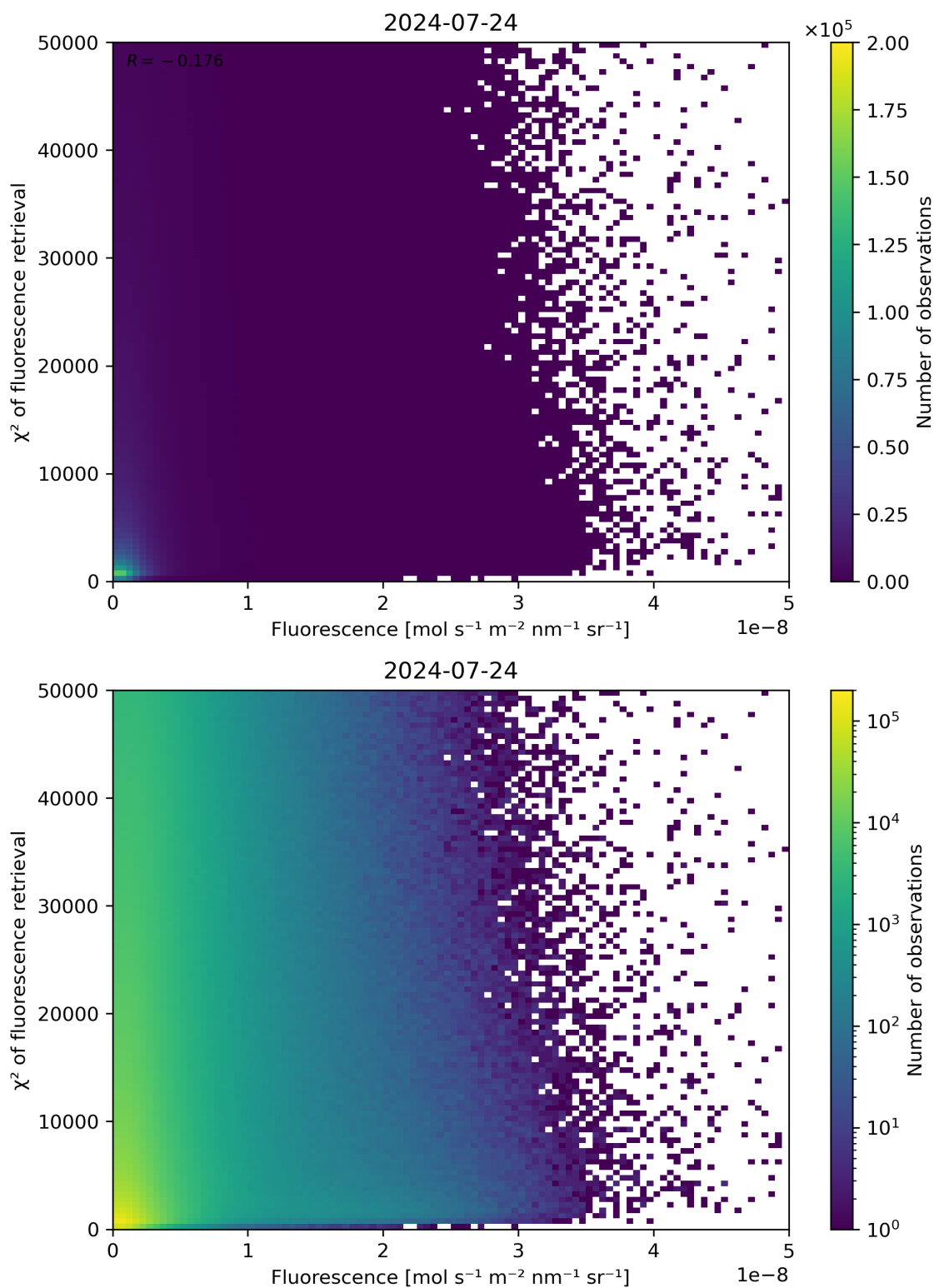
Figure 85: Scatter density plot of “Fluorescence” against “ \chi^2 of fluorescence retrieval” for 2024-07-23 to 2024-07-25.
