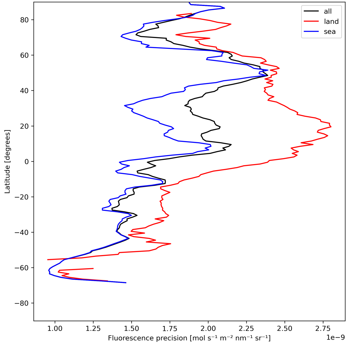
Figure 24: Zonal average of “Fluorescence precision” for 2024-07-23 to 2024-07-25.
