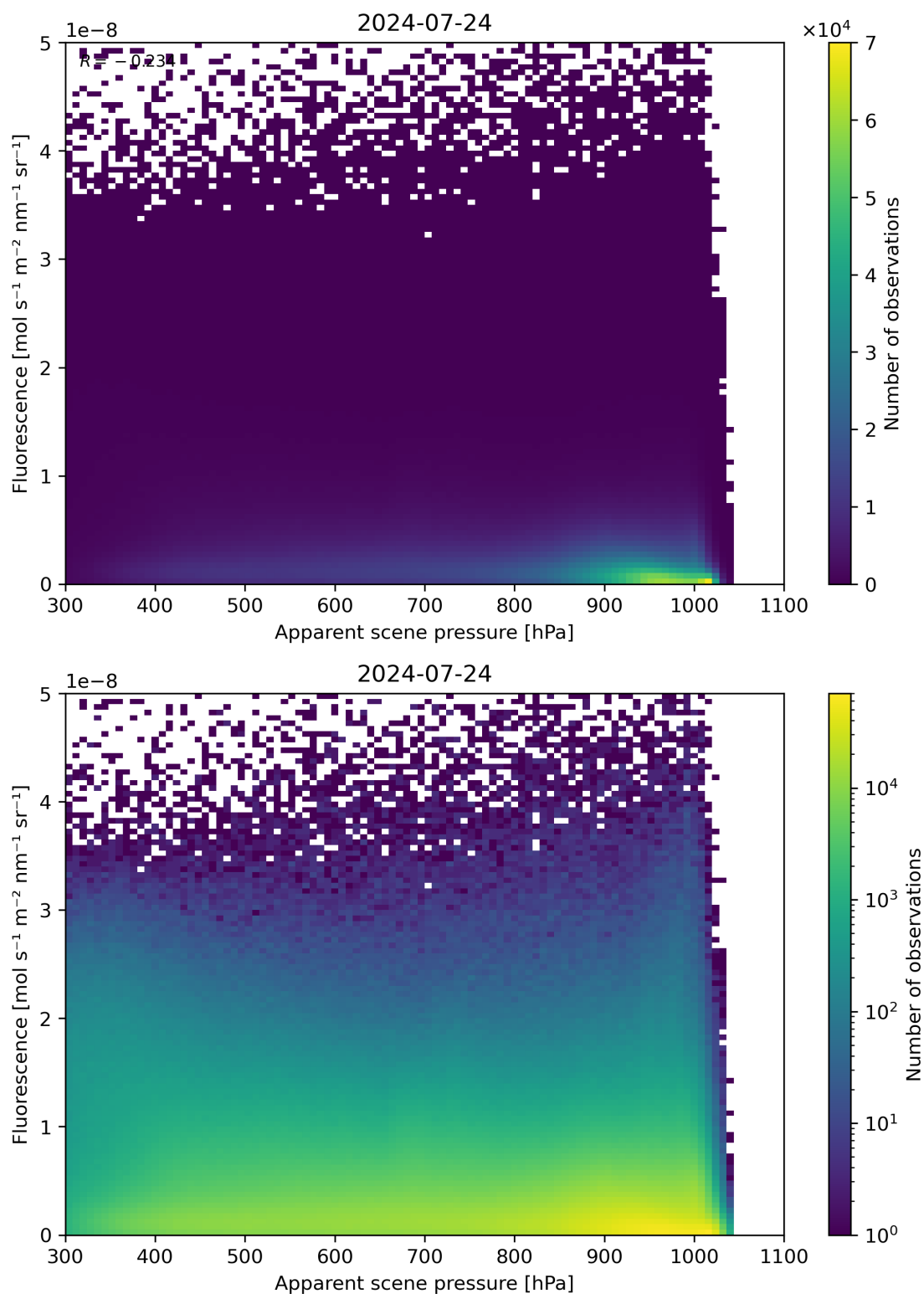
Figure 64: Scatter density plot of “Apparent scene pressure” against “Fluorescence” for 2024-07-23 to 2024-07-25.
