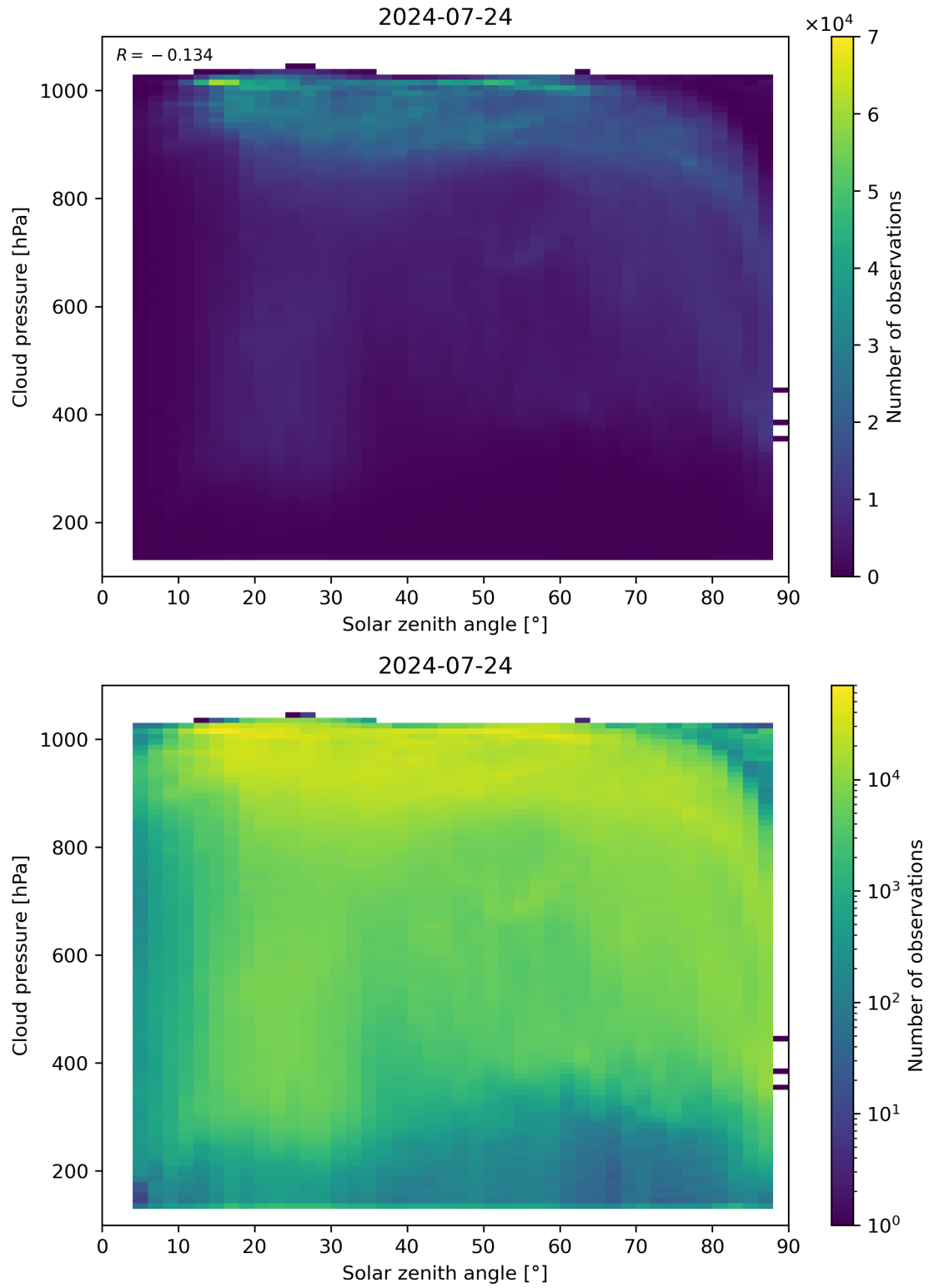
Figure 111: Scatter density plot of “Solar zenith angle” against “Cloud pressure” for 2024-07-23 to 2024-07-25.
