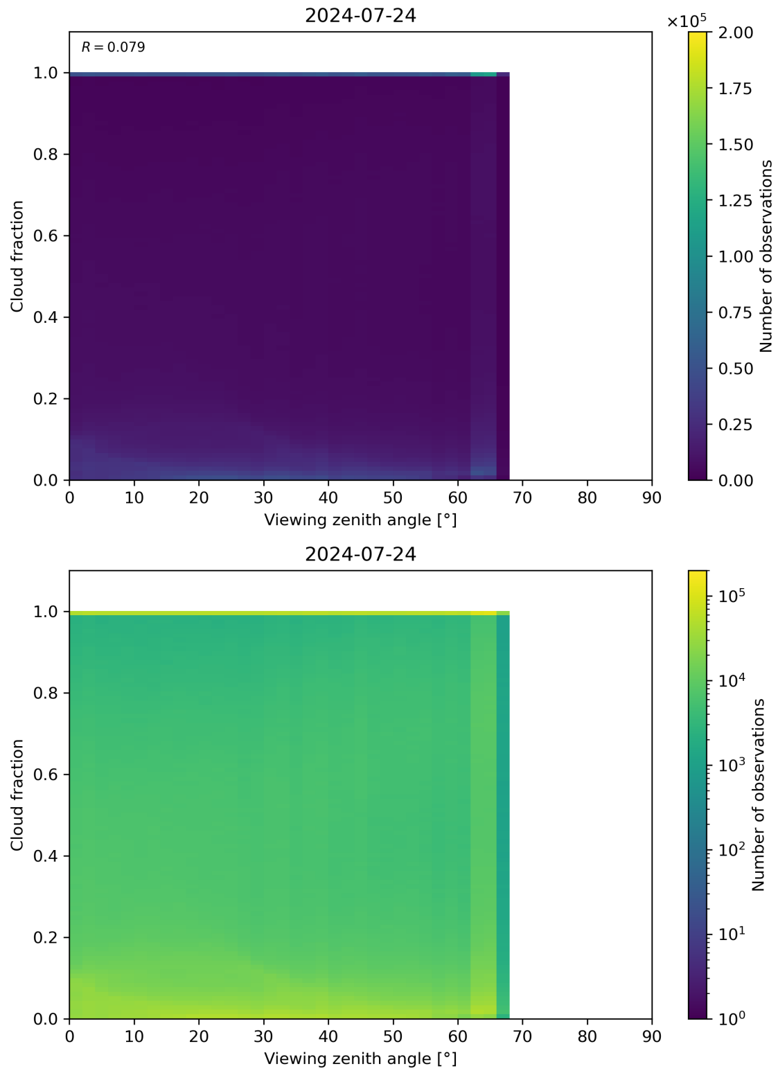
Figure 120: Scatter density plot of “Viewing zenith angle” against “Cloud fraction” for 2024-07-23 to 2024-07-25.
