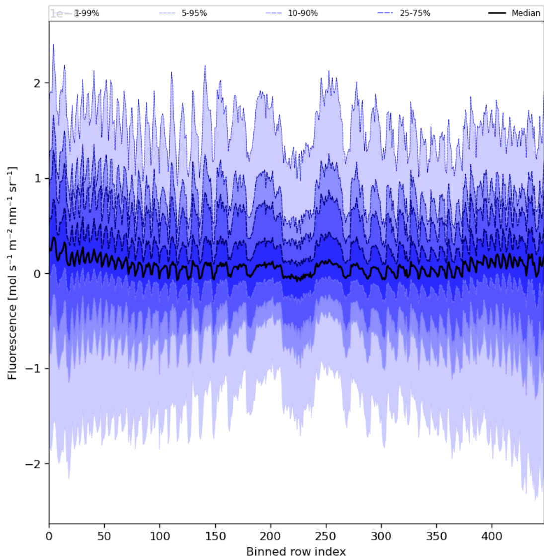
Figure 57: Along track statistics of “Fluorescence” for 2024-07-23 to 2024-07-25
