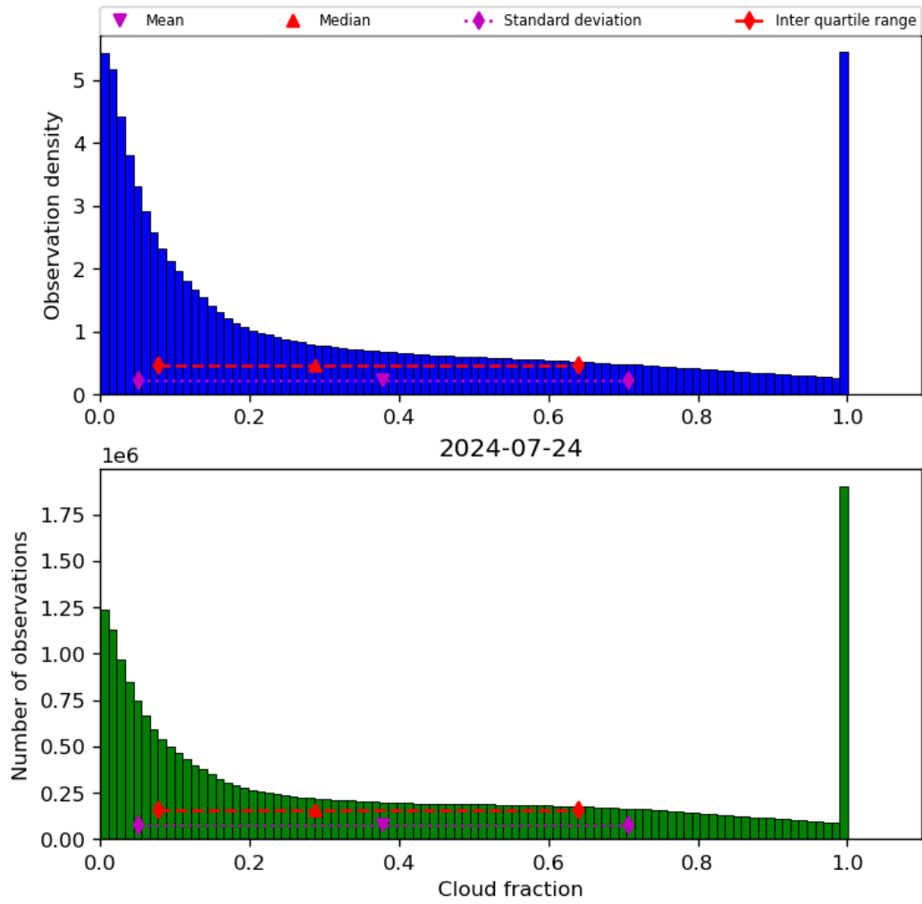
Figure 32: Histogram of “Cloud fraction” for 2024-07-23 to 2024-07-25
