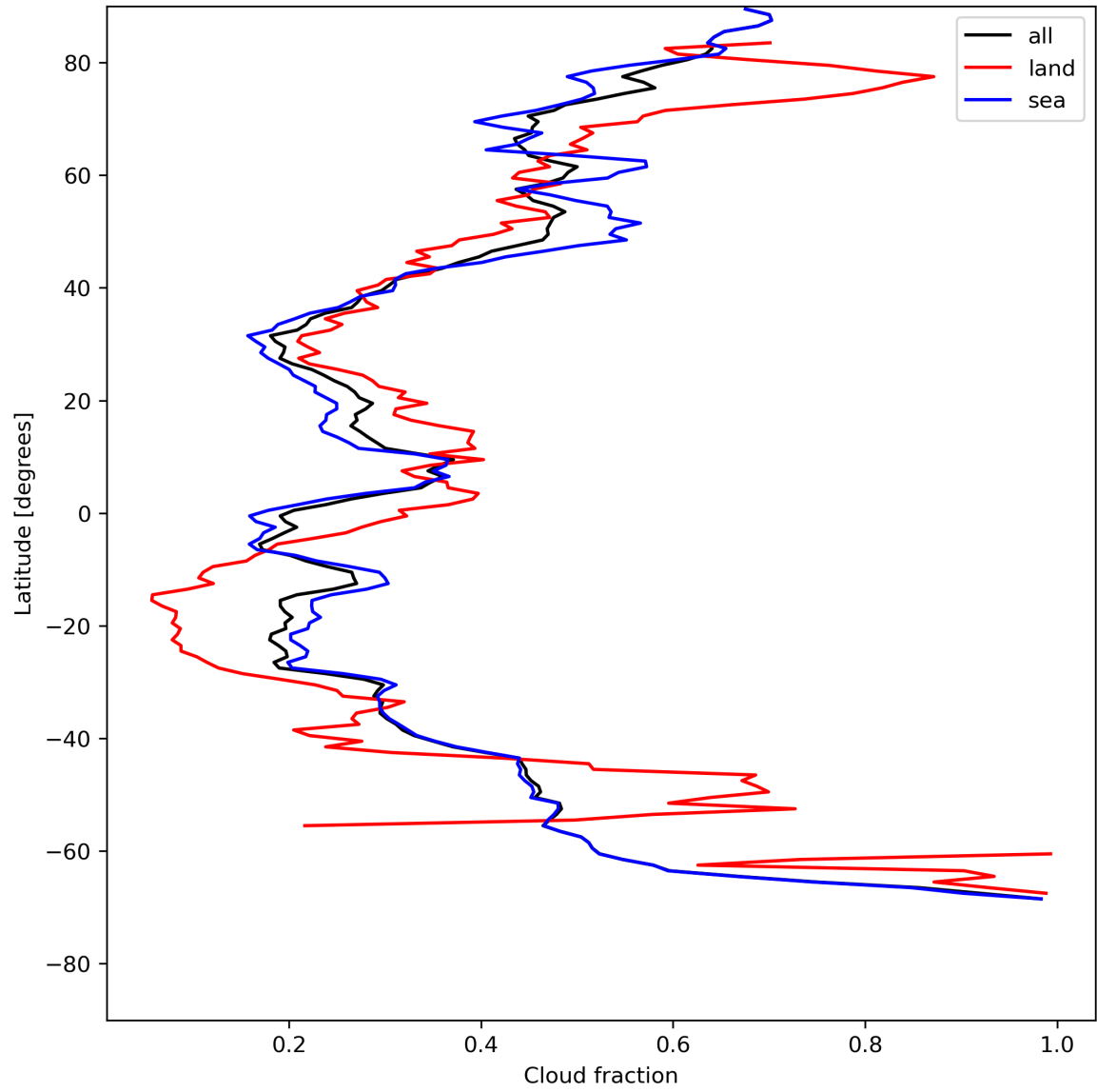
Figure 15: Zonal average of “Cloud fraction” for 2024-07-23 to 2024-07-25.
