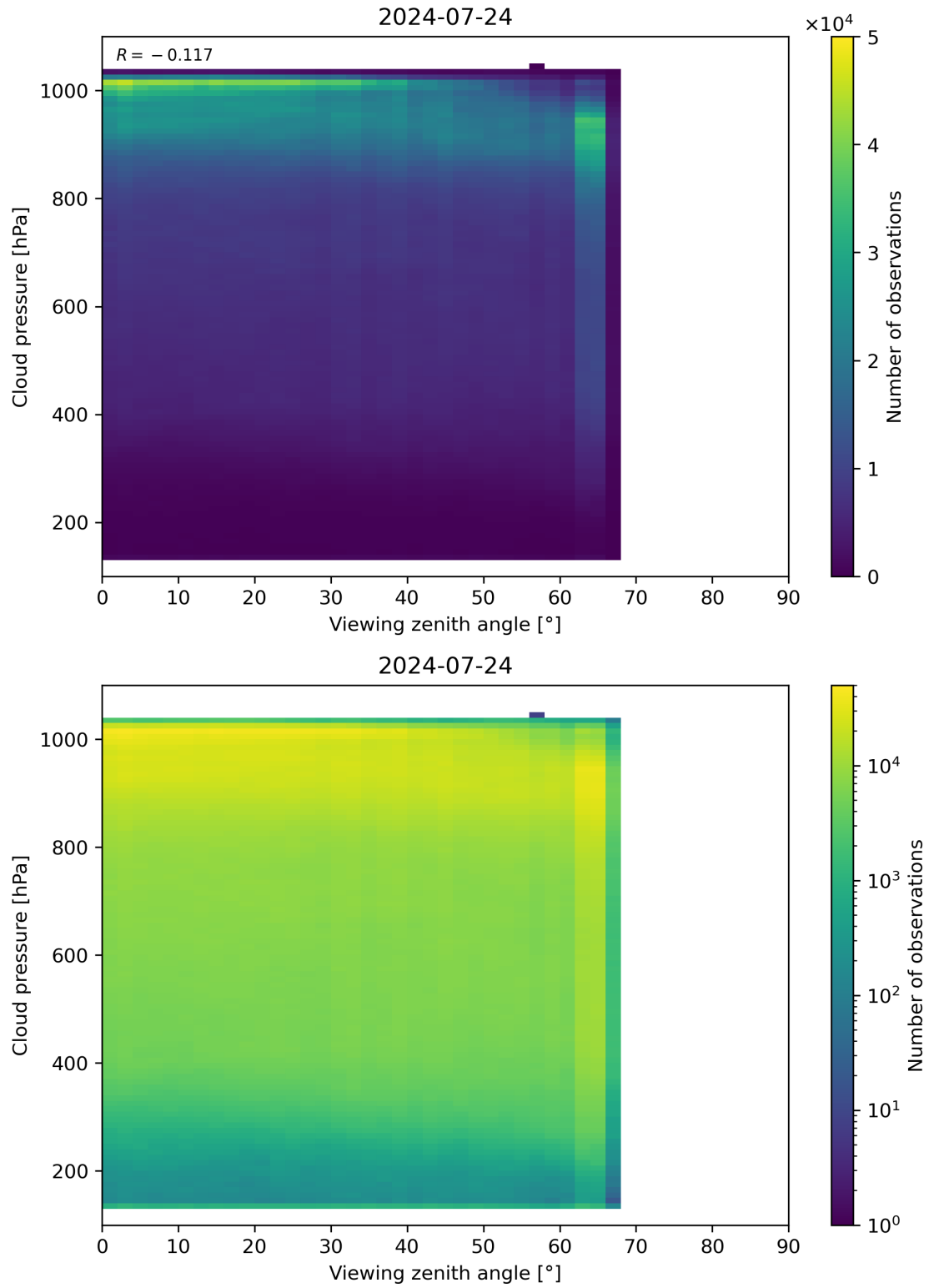
Figure 121: Scatter density plot of “Viewing zenith angle” against “Cloud pressure” for 2024-07-23 to 2024-07-25.
