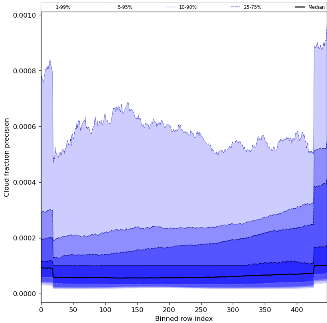
Figure 50: Along track statistics of “Cloud fraction precision” for 2024-07-23 to 2024-07-25
