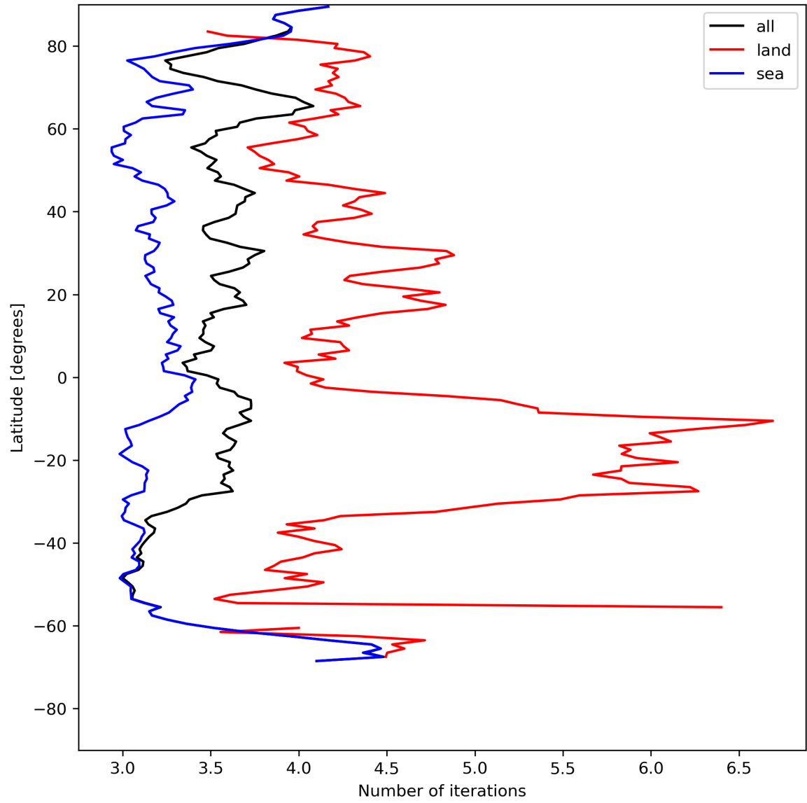
Figure 22: Zonal average of “Number of iterations” for 2024-07-23 to 2024-07-25.
