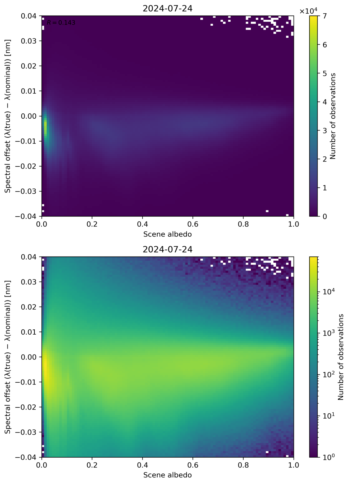
Figure 107: Scatter density plot of “Scene albedo” against “Spectral offset ( \lambda(\text{true}) - \lambda(\text{nominal}) )” for 2024-07-23 to 2024-07-25.
