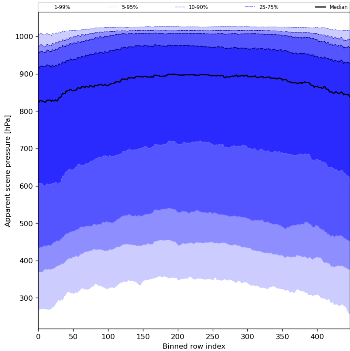
Figure 53: Along track statistics of “Apparent scene pressure” for 2024-07-23 to 2024-07-25
