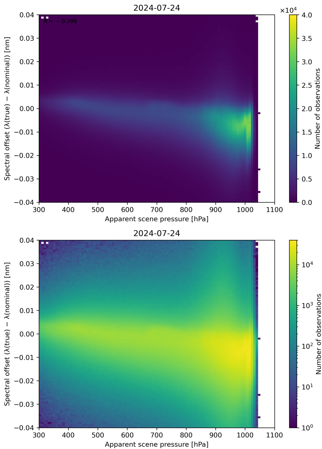
Figure 67: Scatter density plot of “Apparent scene pressure” against “Spectral offset ( \lambda(\text{true}) - \lambda(\text{nominal}) )” for 2024-07-23 to 2024-07-25.
