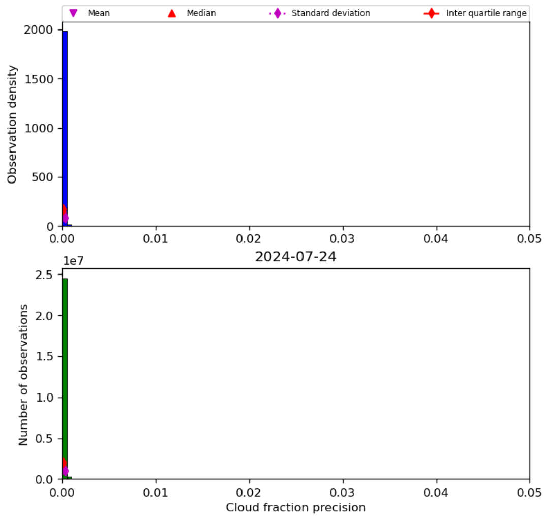
Figure 33: Histogram of “Cloud fraction precision” for 2024-07-23 to 2024-07-25
