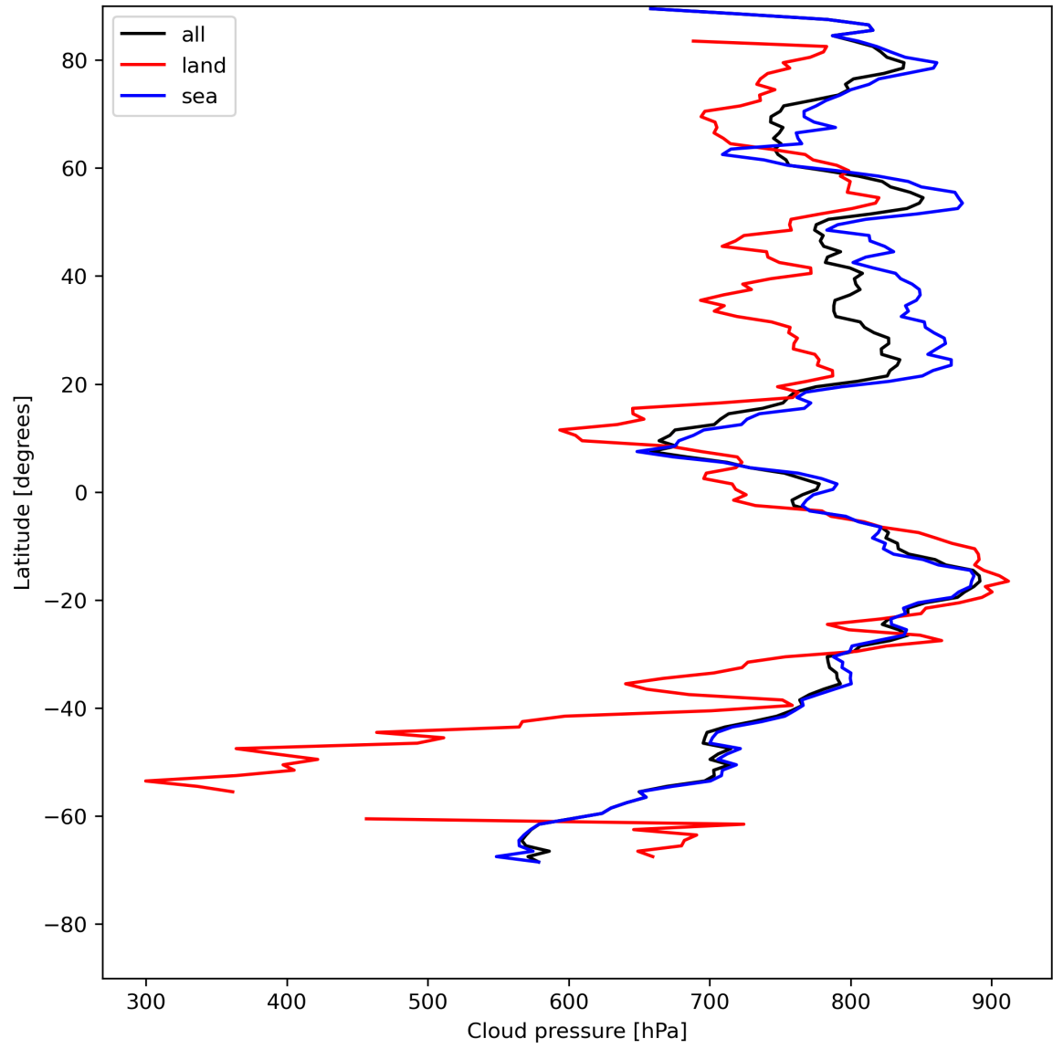
Figure 13: Zonal average of “Cloud pressure” for 2024-07-23 to 2024-07-25.
