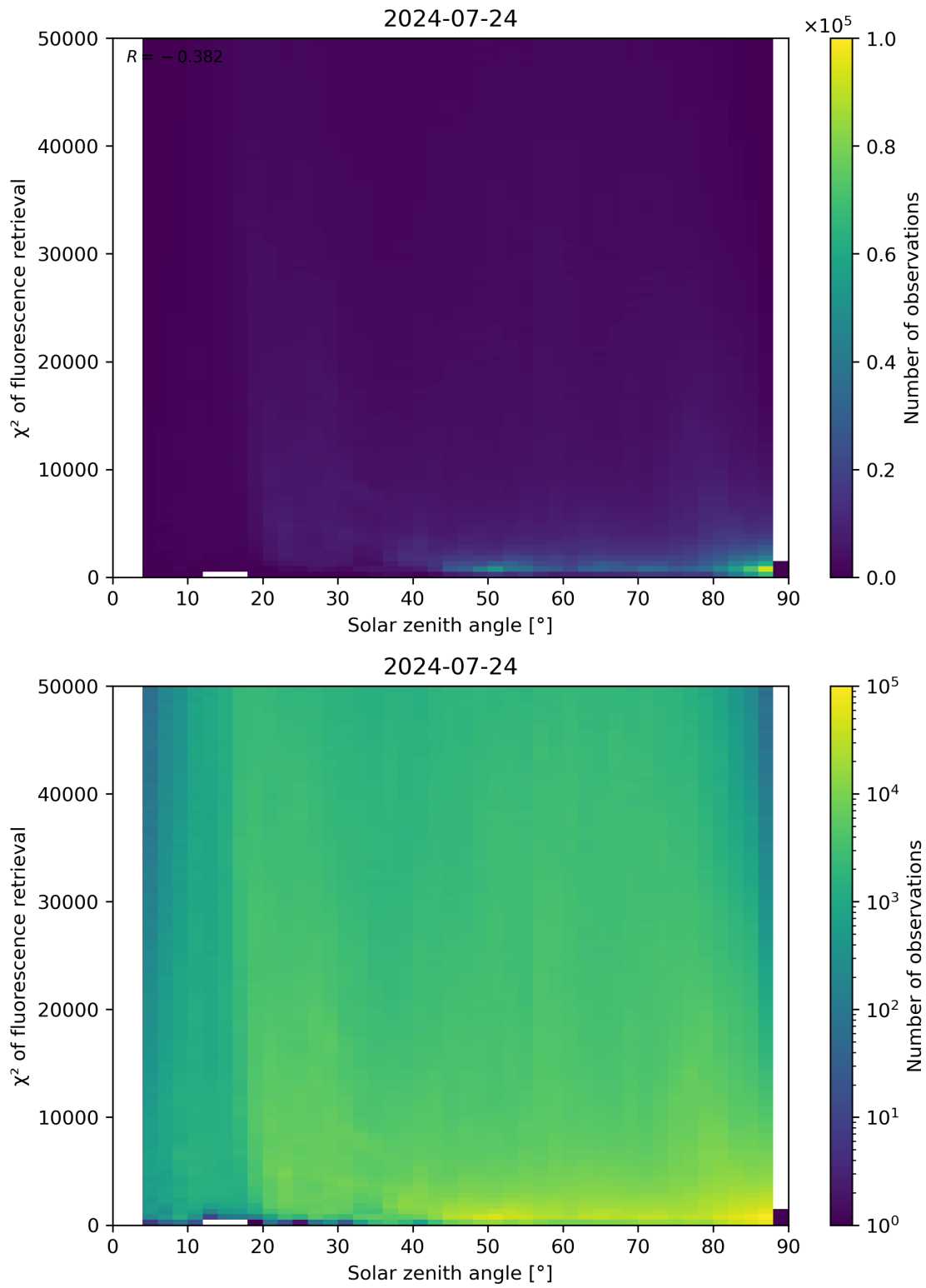
Figure 109: Scatter density plot of “Solar zenith angle” against “ \chi^2 of fluorescence retrieval” for 2024-07-23 to 2024-07-25.
