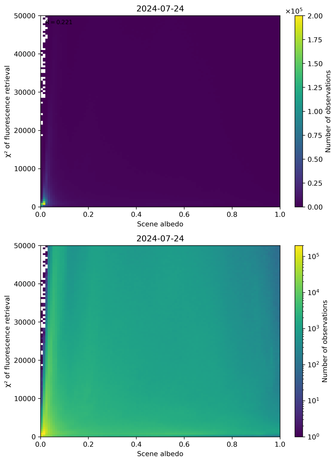
Figure 103: Scatter density plot of “Scene albedo” against “ \chi^2 of fluorescence retrieval” for 2024-07-23 to 2024-07-25.
