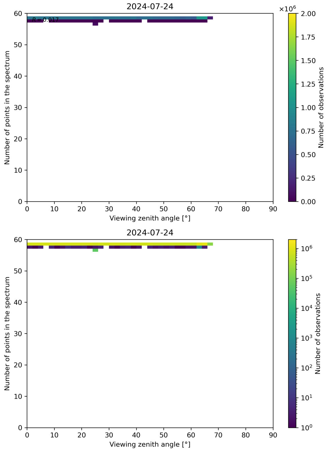
Figure 125: Scatter density plot of “Viewing zenith angle” against “Number of points in the spectrum” for 2024-07-23 to 2024-07-25.
