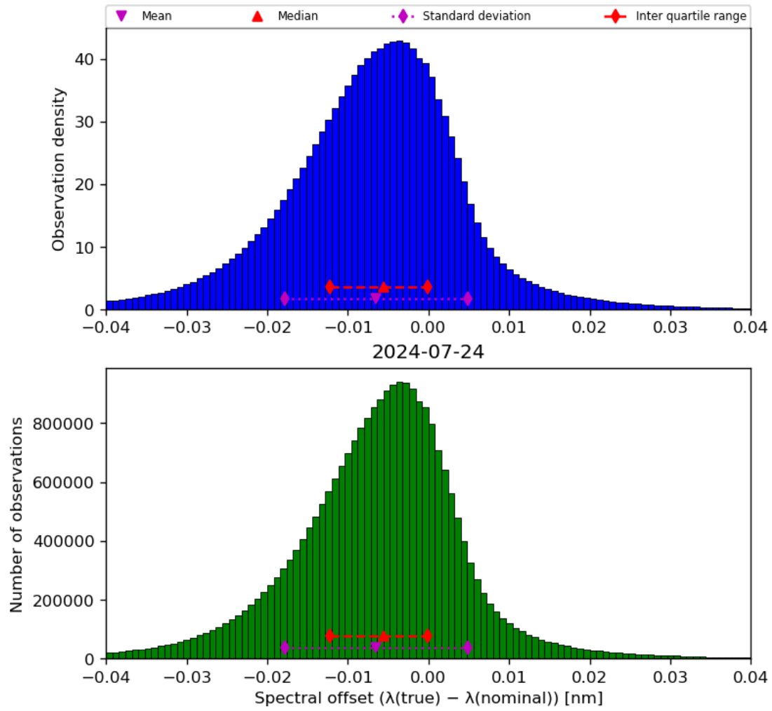
Figure 45: Histogram of “Spectral offset ( \lambda(\text{true}) - \lambda(\text{nominal}) )” for 2024-07-23 to 2024-07-25
