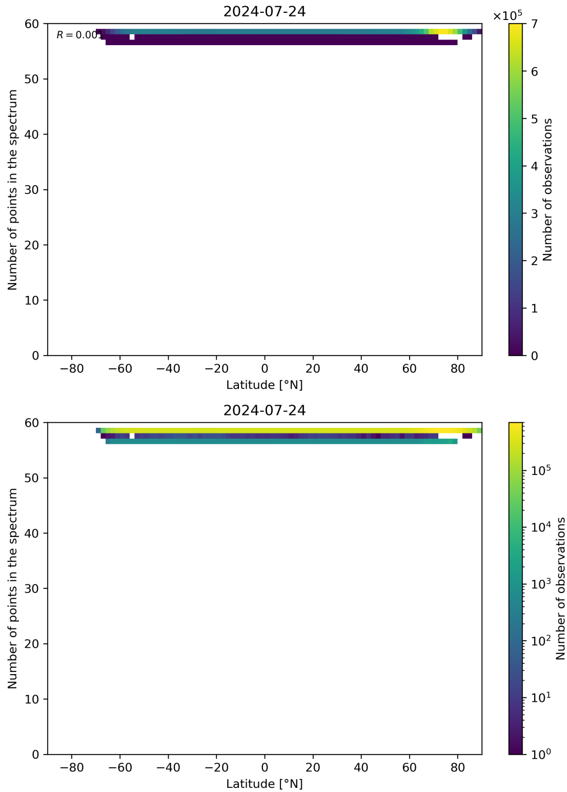
Figure 94: Scatter density plot of “Latitude” against “Number of points in the spectrum” for 2024-07-23 to 2024-07-25.
