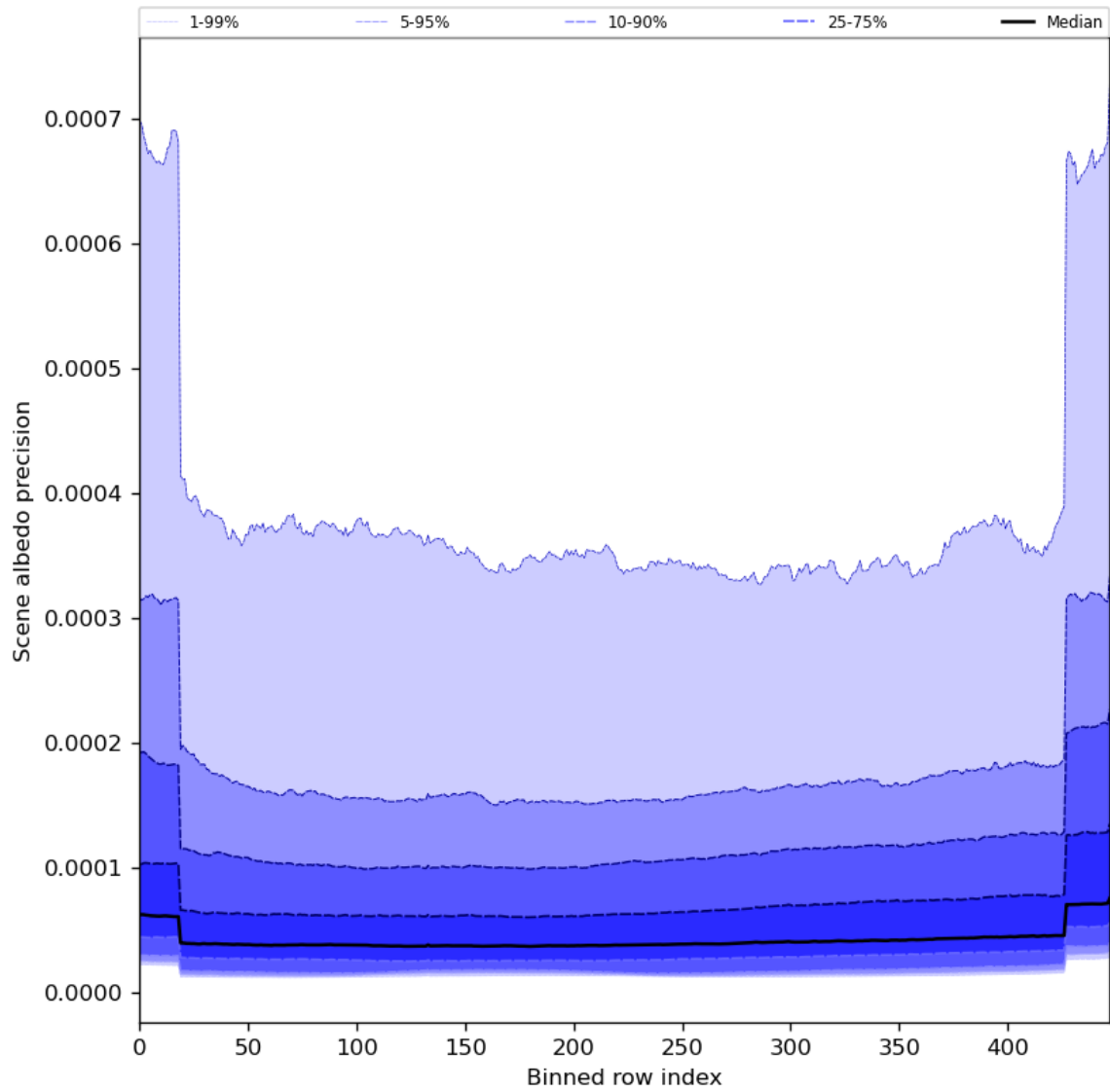
Figure 52: Along track statistics of “Scene albedo precision” for 2024-07-23 to 2024-07-25
