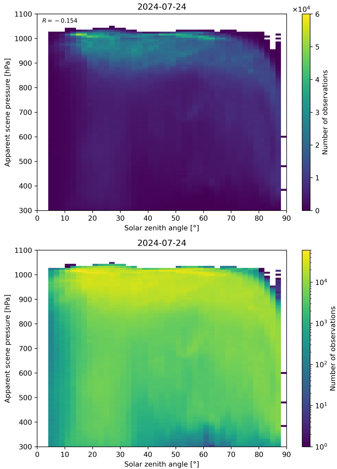
Figure 108: Scatter density plot of “Solar zenith angle” against “Apparent scene pressure” for 2024-07-23 to 2024-07-25.
