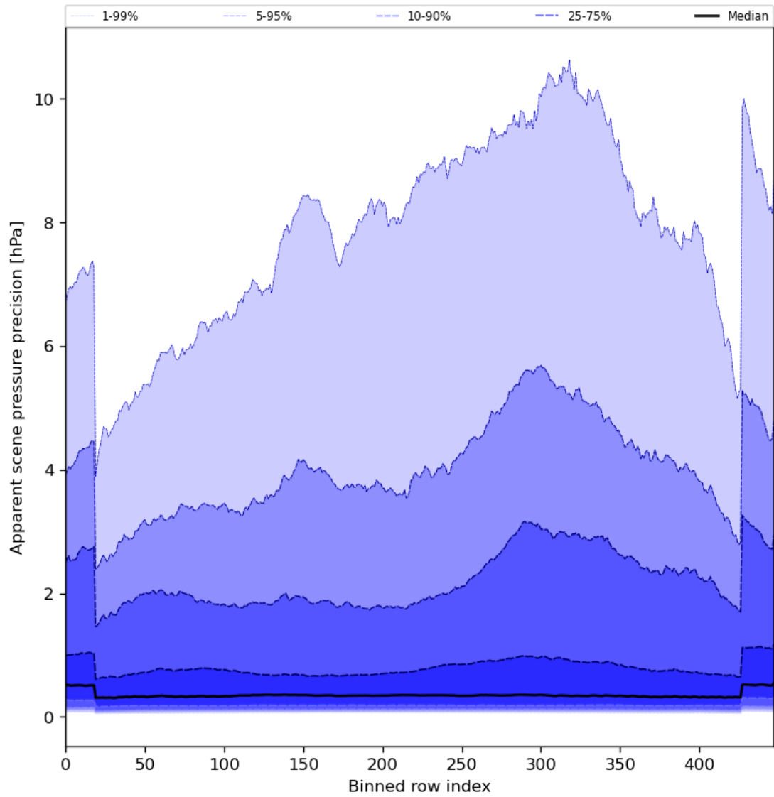
Figure 54: Along track statistics of “Apparent scene pressure precision” for 2024-07-23 to 2024-07-25
