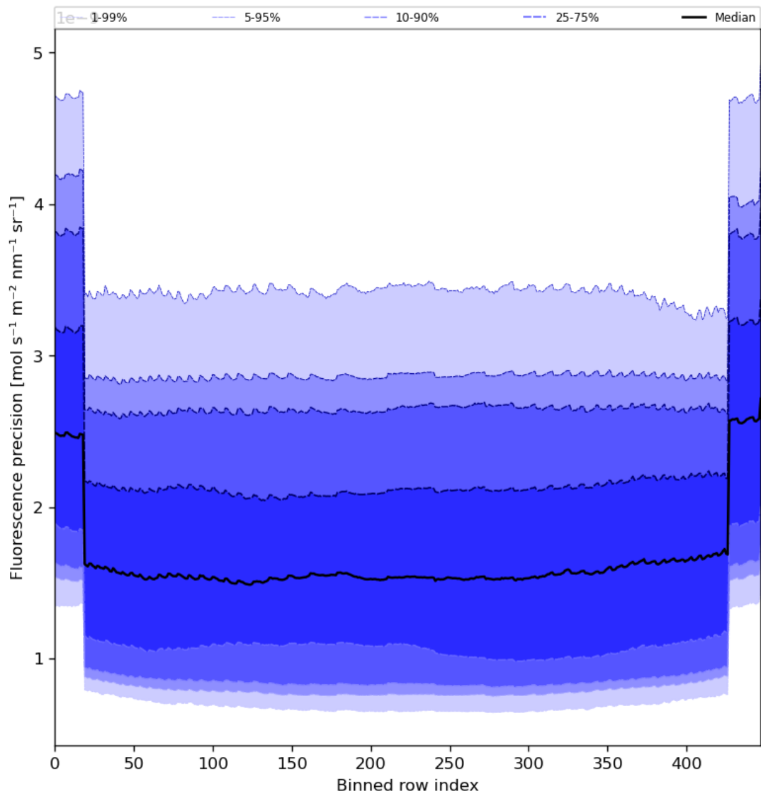
Figure 58: Along track statistics of “Fluorescence precision” for 2024-07-23 to 2024-07-25
