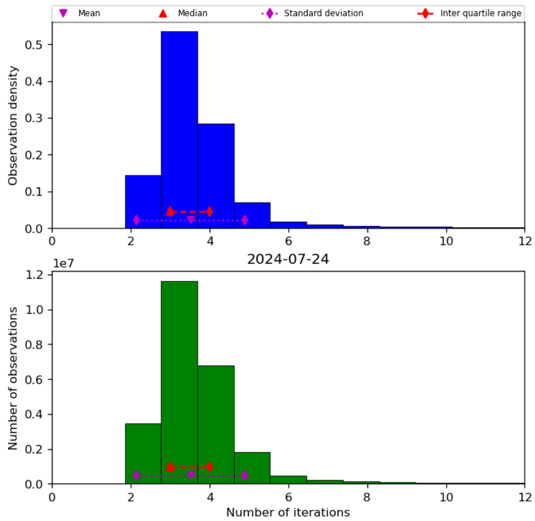
Figure 39: Histogram of “Number of iterations” for 2024-07-23 to 2024-07-25
