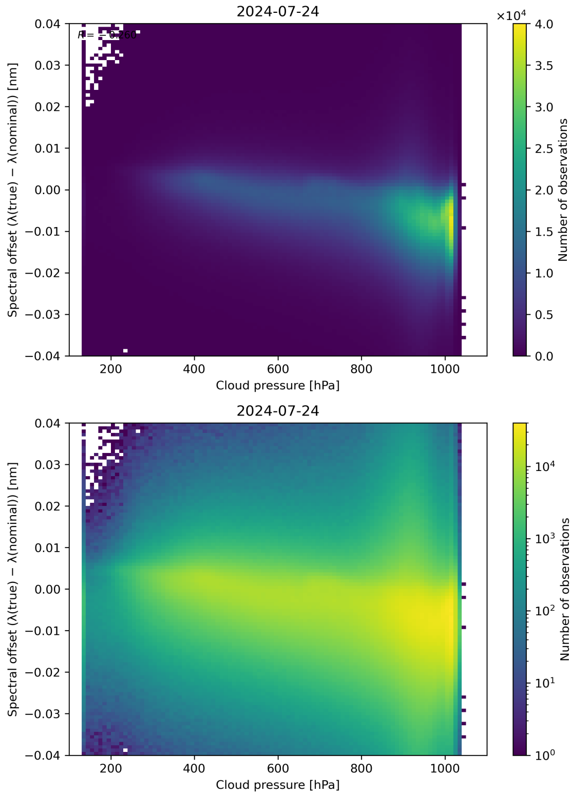
Figure 84: Scatter density plot of “Cloud pressure” against “Spectral offset ( \lambda(\text{true}) - \lambda(\text{nominal}) )” for 2024-07-23 to 2024-07-25.
