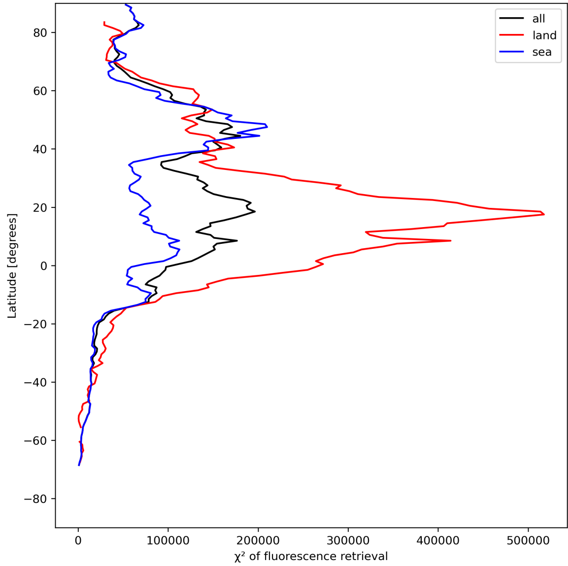
Figure 25: Zonal average of “ \chi^2 of fluorescence retrieval” for 2024-07-23 to 2024-07-25.
