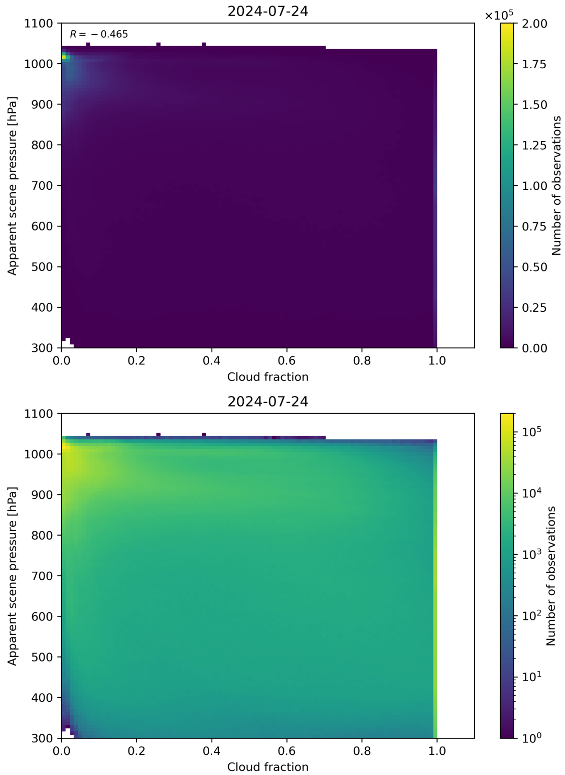
Figure 70: Scatter density plot of “Cloud fraction” against “Apparent scene pressure” for 2024-07-23 to 2024-07-25.
