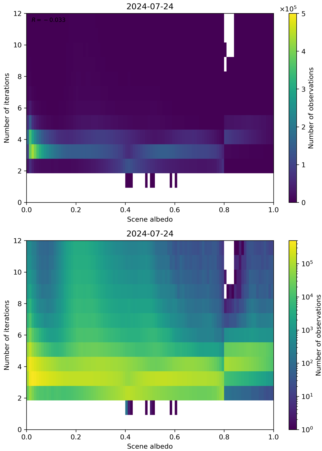
Figure 105: Scatter density plot of “Scene albedo” against “Number of iterations” for 2024-07-23 to 2024-07-25.
