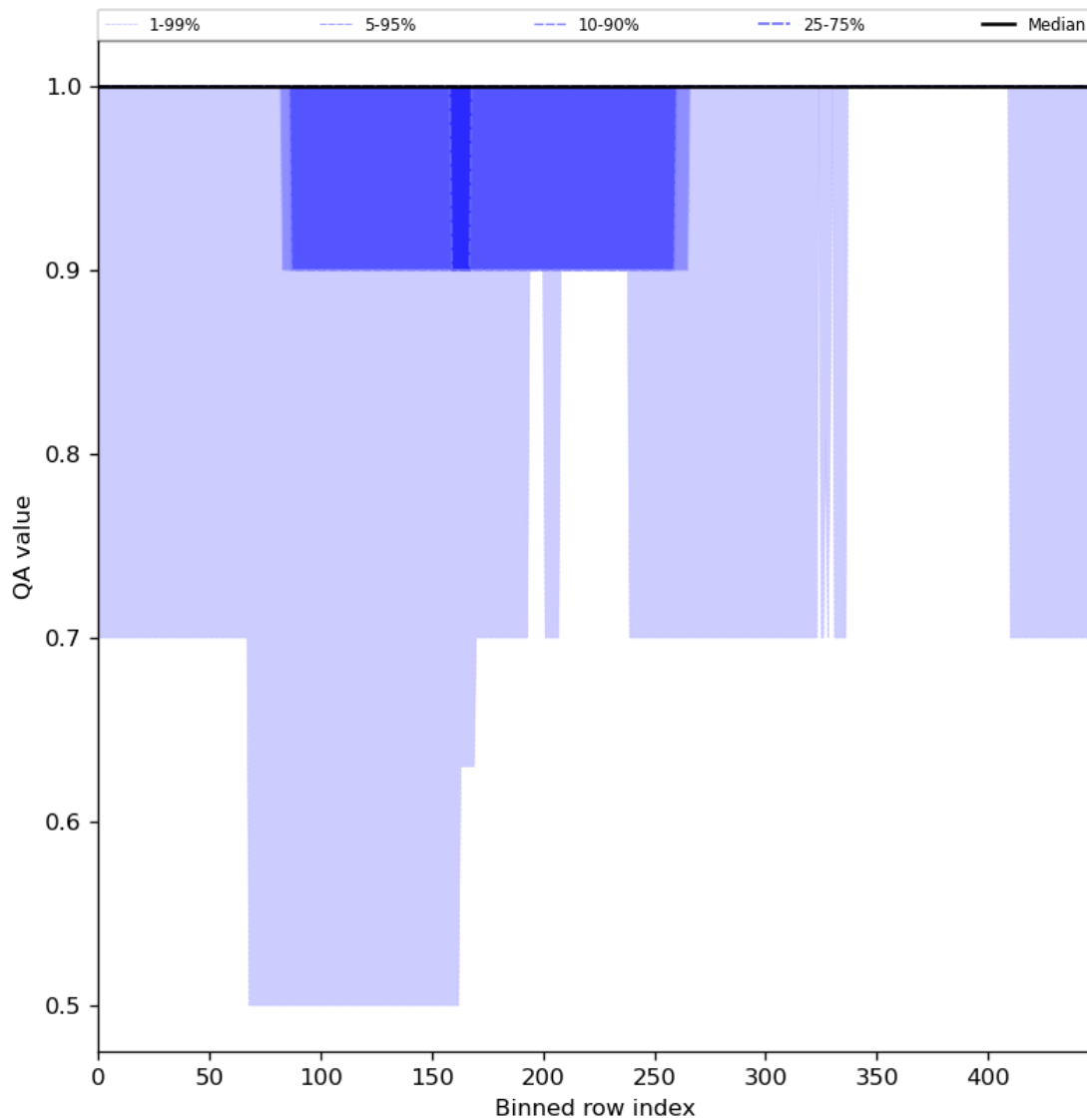
Figure 46: Along track statistics of “QA value” for 2024-07-23 to 2024-07-25
