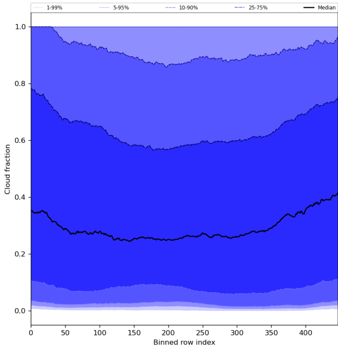
Figure 49: Along track statistics of “Cloud fraction” for 2024-07-23 to 2024-07-25
