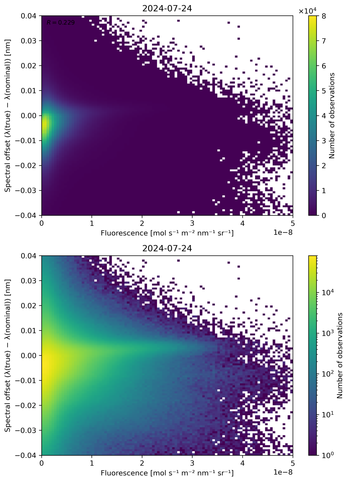
Figure 87: Scatter density plot of “Fluorescence” against “Spectral offset ( \lambda(\text{true}) - \lambda(\text{nominal}) )” for 2024-07-23 to 2024-07-25.
