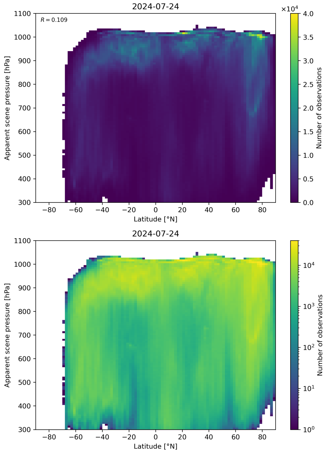
Figure 88: Scatter density plot of “Latitude” against “Apparent scene pressure” for 2024-07-23 to 2024-07-25.
