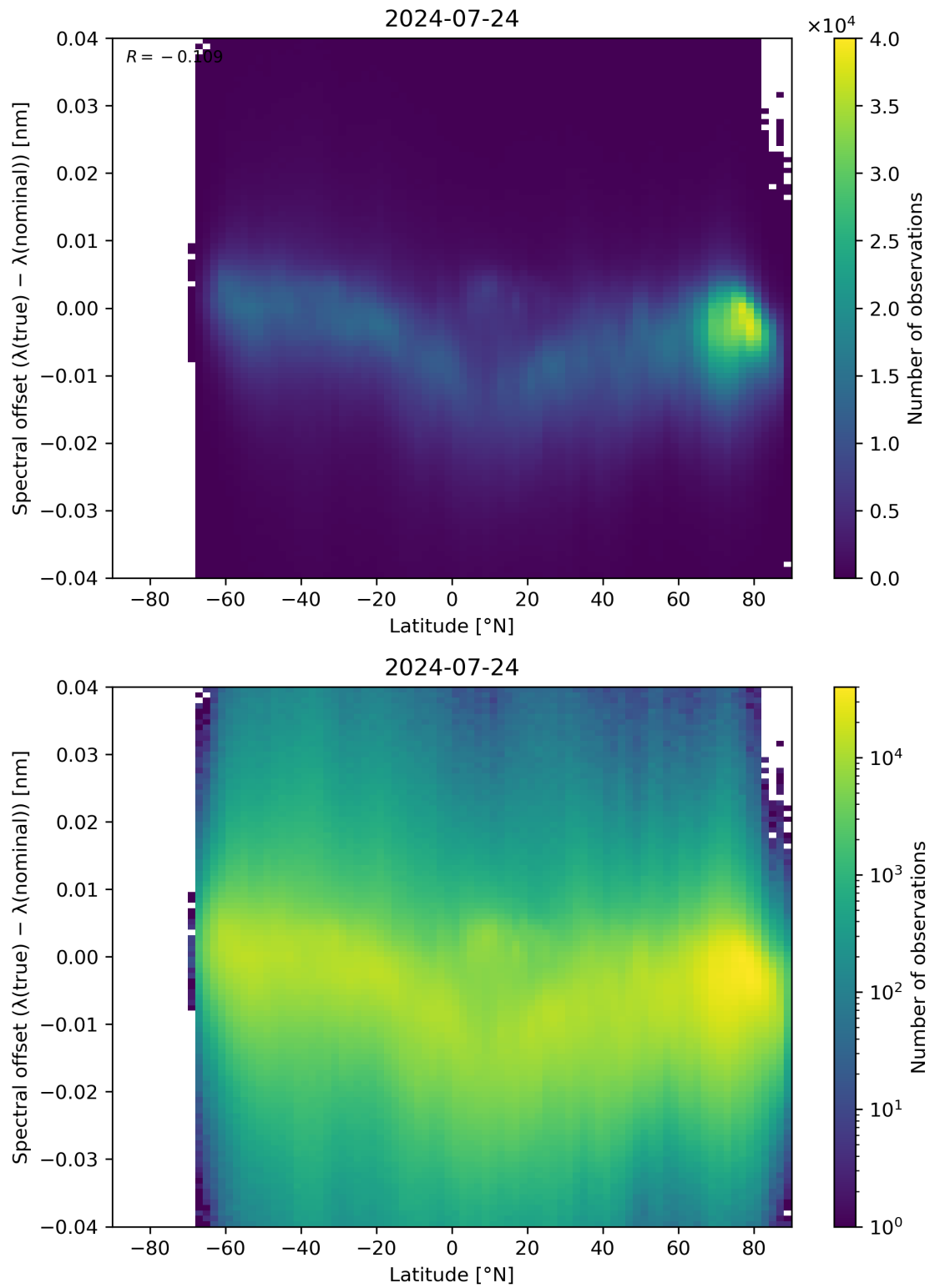
Figure 96: Scatter density plot of “Latitude” against “Spectral offset ( \lambda(\text{true}) - \lambda(\text{nominal}) )” for 2024-07-23 to 2024-07-25.
