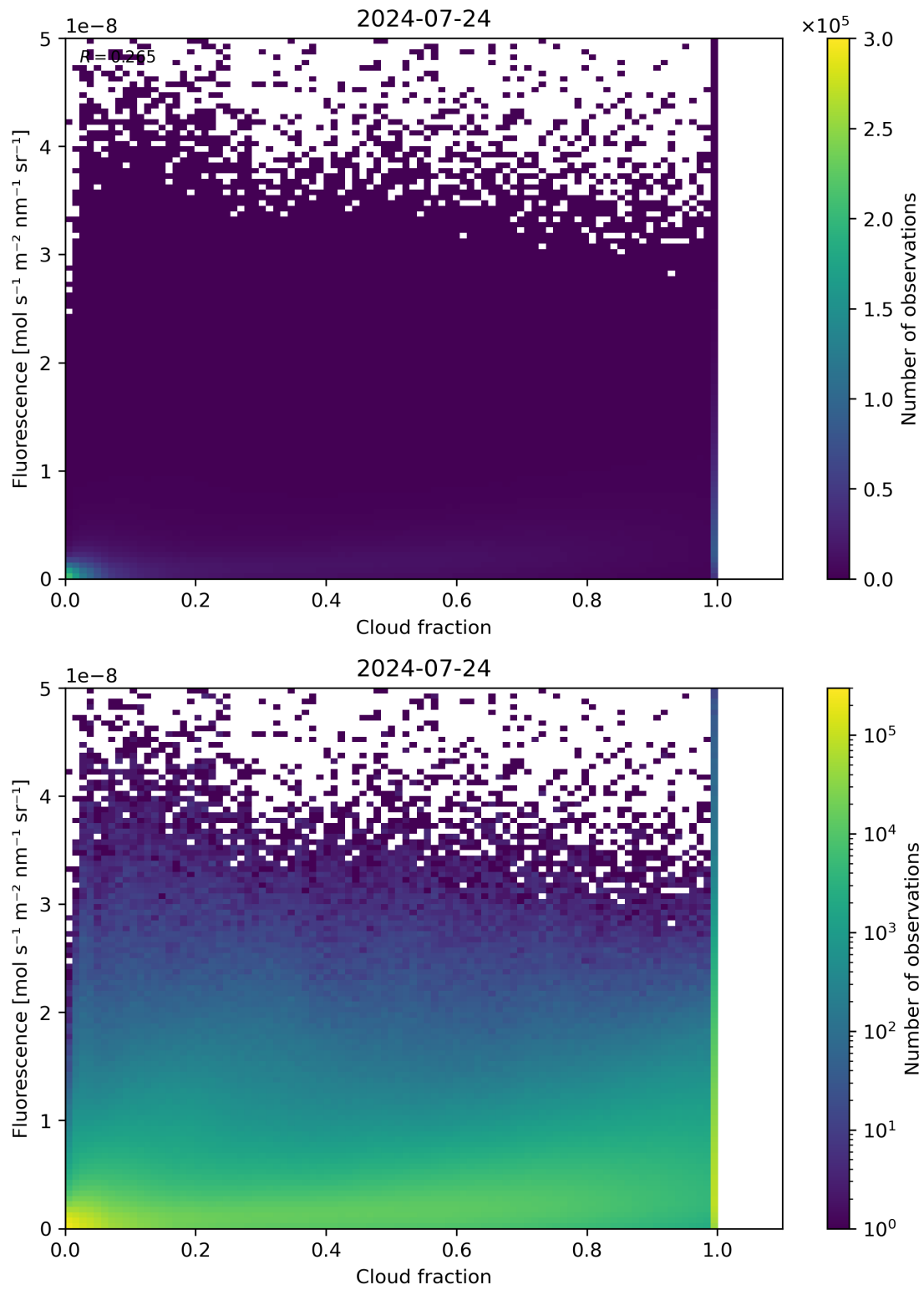
Figure 72: Scatter density plot of “Cloud fraction” against “Fluorescence” for 2024-07-23 to 2024-07-25.
