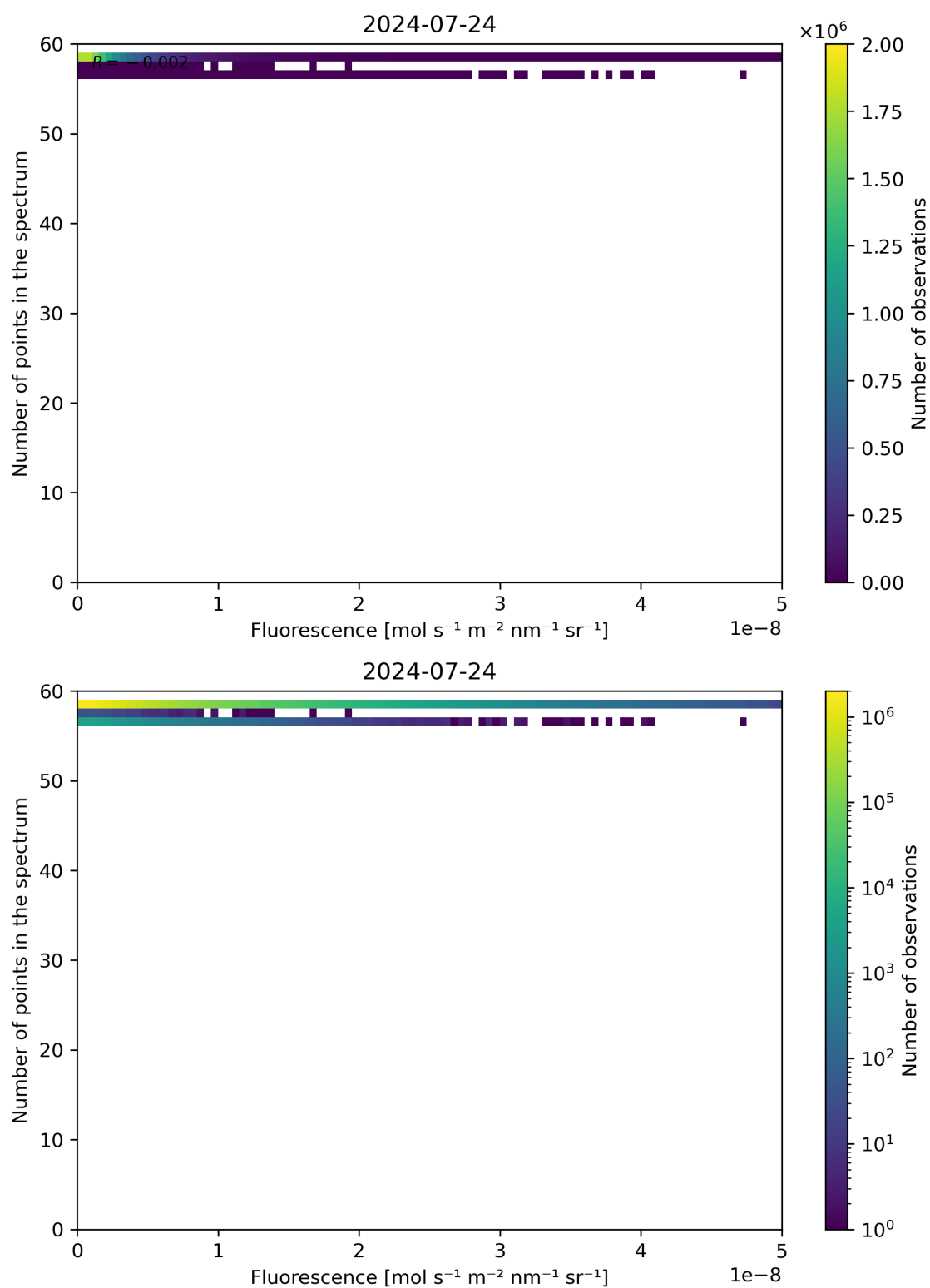
Figure 86: Scatter density plot of “Fluorescence” against “Number of points in the spectrum” for 2024-07-23 to 2024-07-25.
