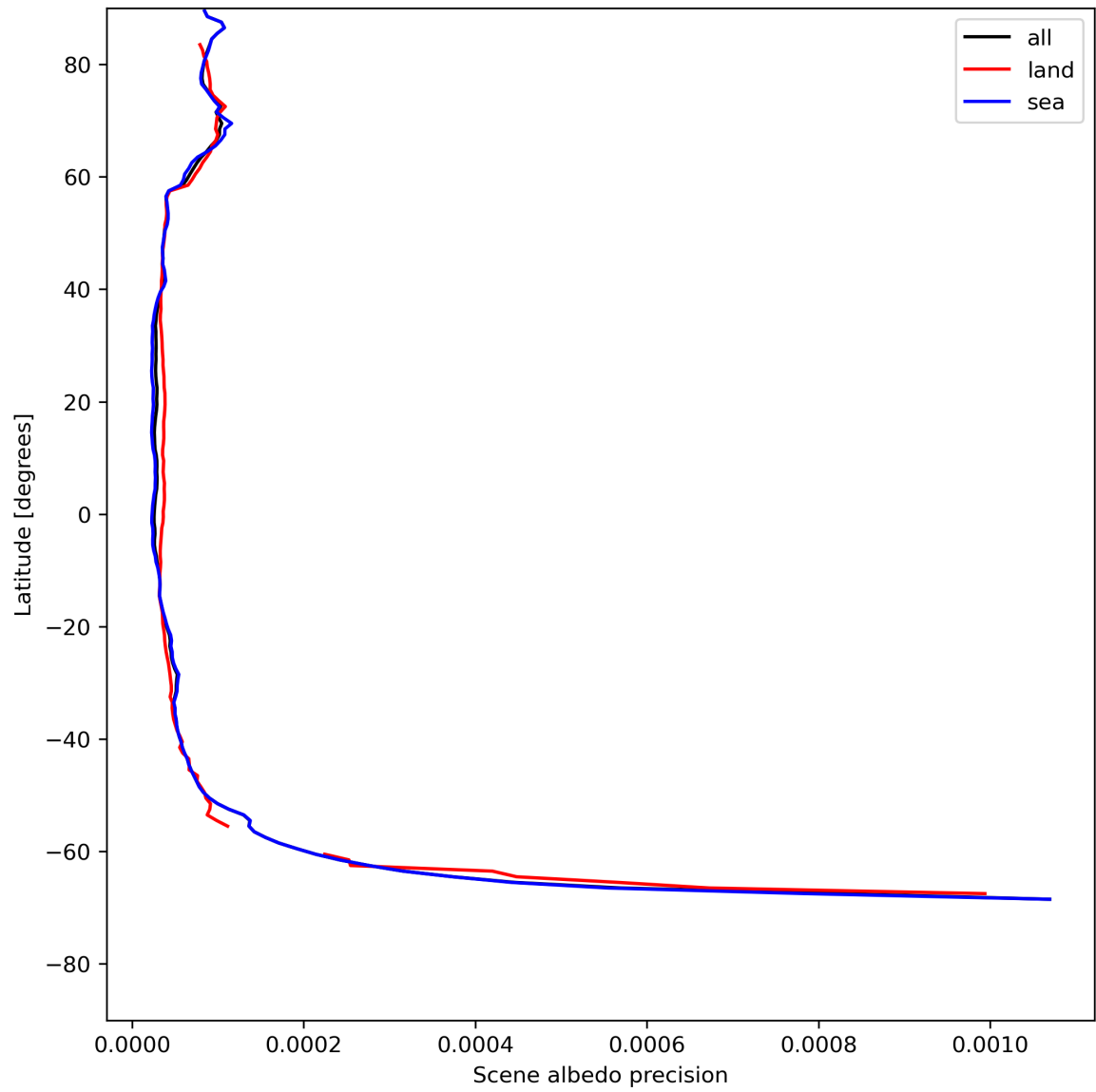
Figure 18: Zonal average of “Scene albedo precision” for 2024-07-23 to 2024-07-25.
