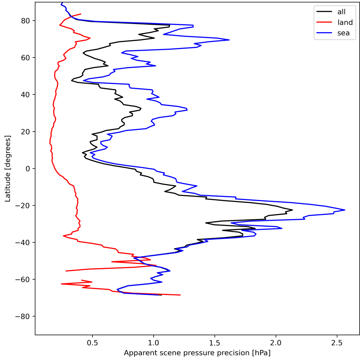
Figure 20: Zonal average of “Apparent scene pressure precision” for 2024-07-24 to 2024-07-26.
