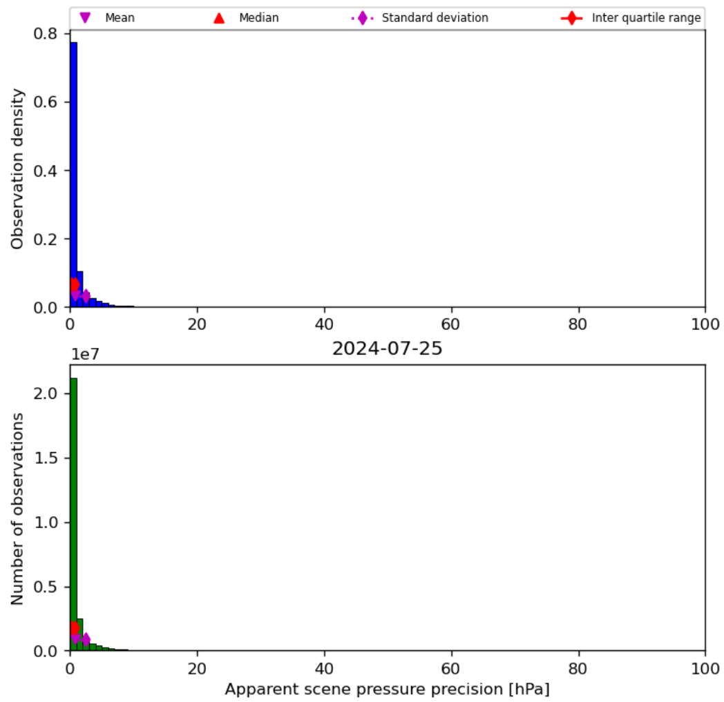
Figure 37: Histogram of “Apparent scene pressure precision” for 2024-07-24 to 2024-07-26
