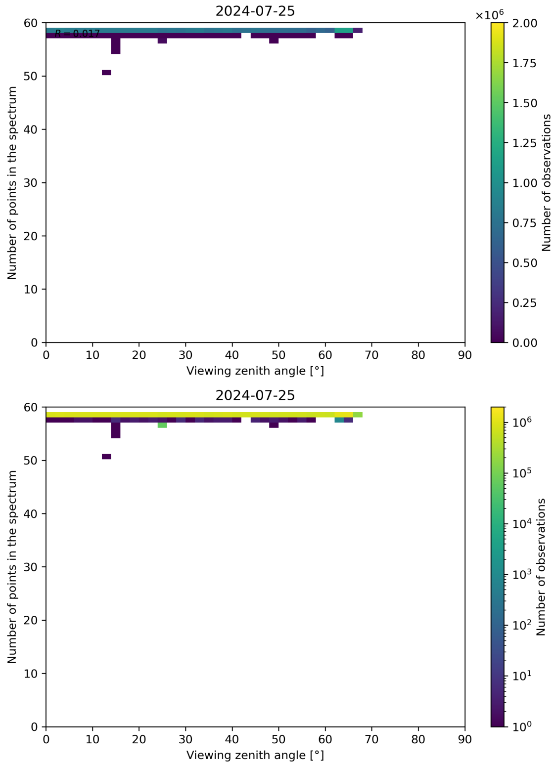
Figure 125: Scatter density plot of “Viewing zenith angle” against “Number of points in the spectrum” for 2024-07-24 to 2024-07-26.
