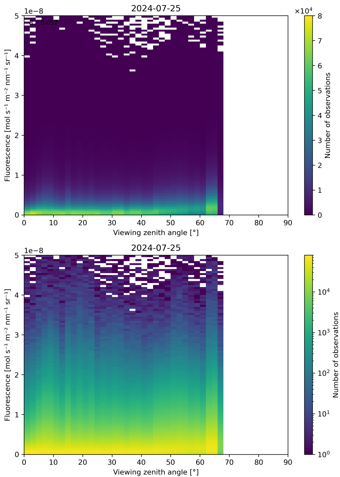
Figure 122: Scatter density plot of “Viewing zenith angle” against “Fluorescence” for 2024-07-24 to 2024-07-26.
