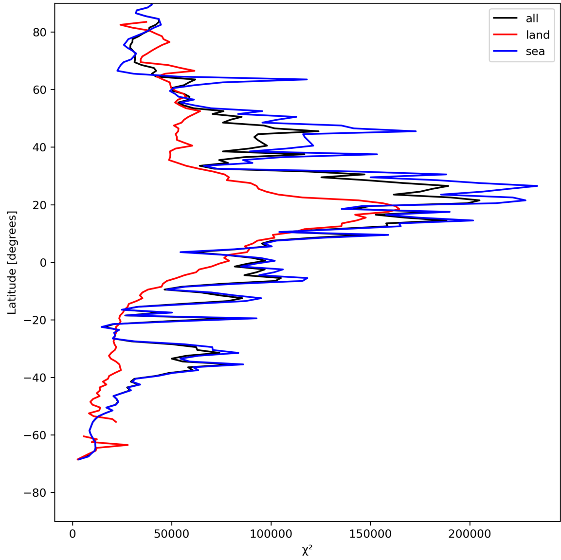
Figure 21: Zonal average of “ \chi^2 ” for 2024-07-24 to 2024-07-26.
