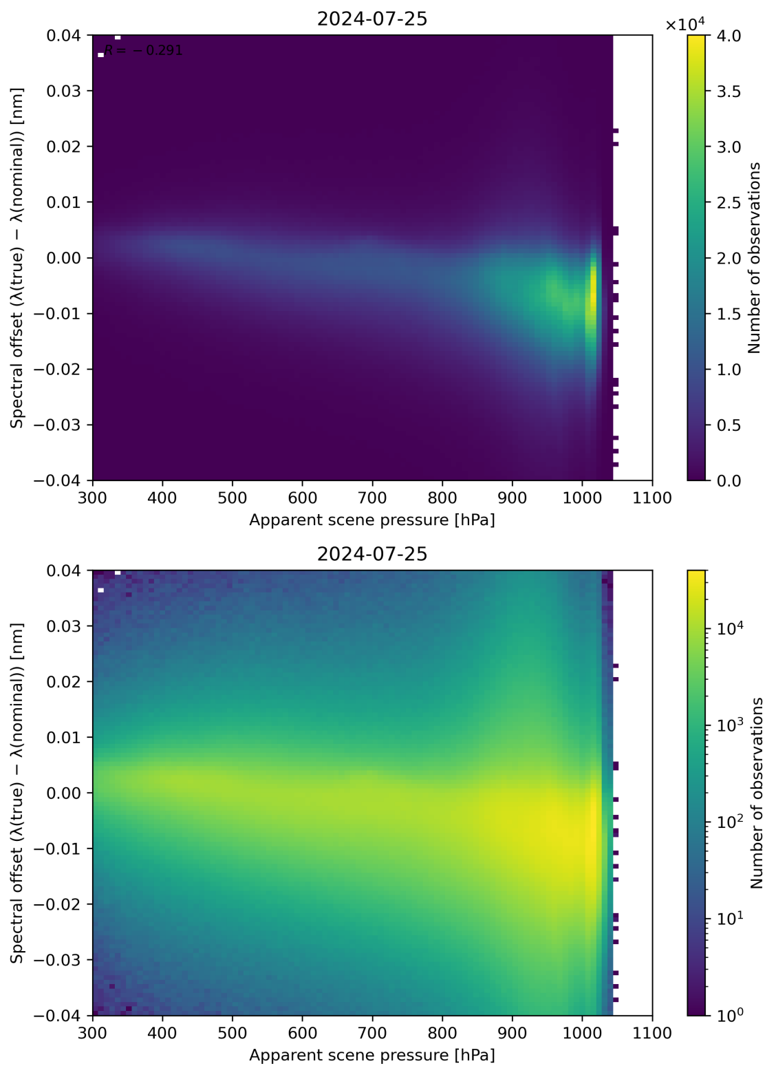
Figure 67: Scatter density plot of “Apparent scene pressure” against “Spectral offset ( \lambda(\text{true}) - \lambda(\text{nominal}) )” for 2024-07-24 to 2024-07-26.
