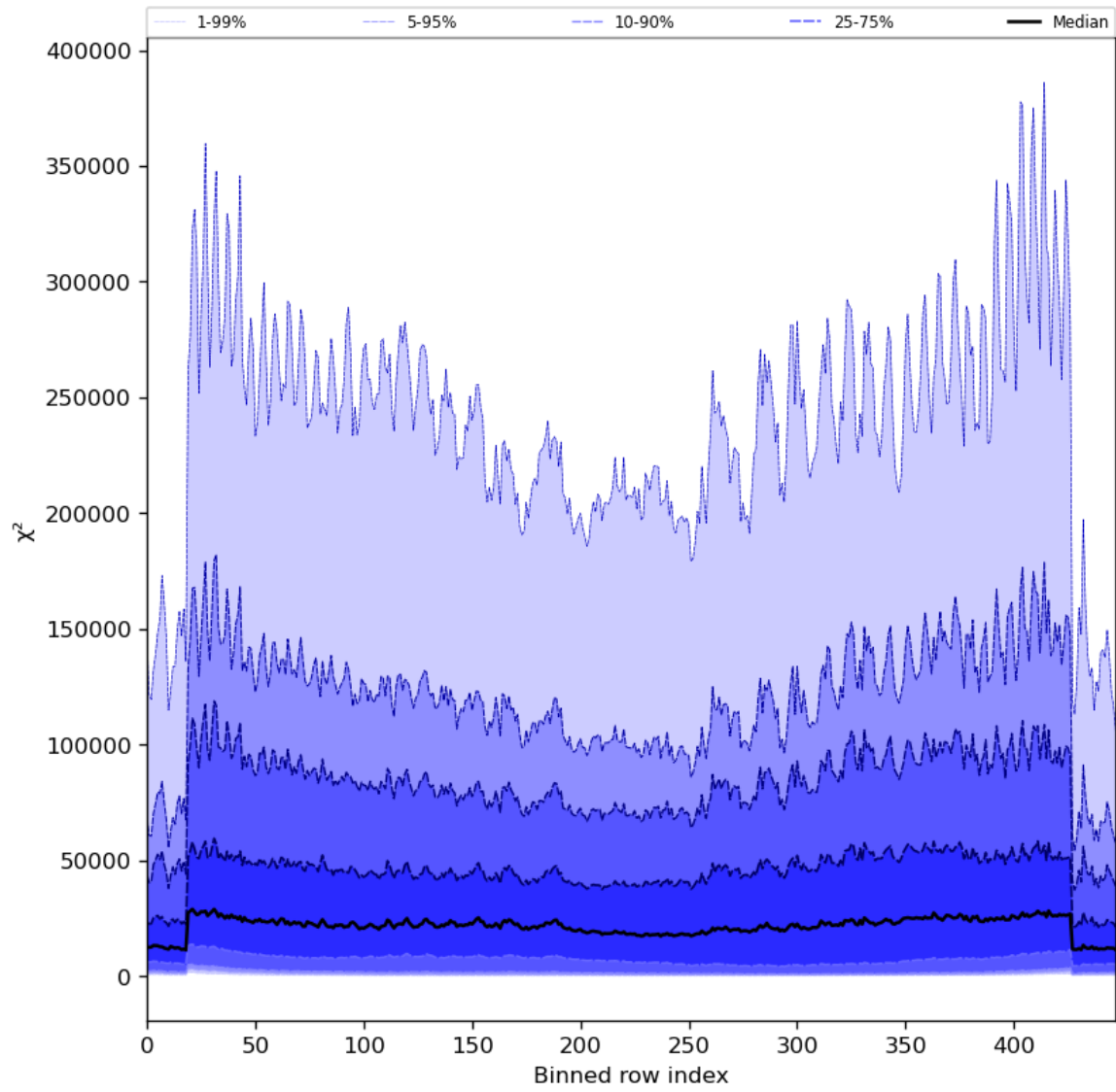
Figure 55: Along track statistics of “ \chi^2 ” for 2024-07-24 to 2024-07-26
