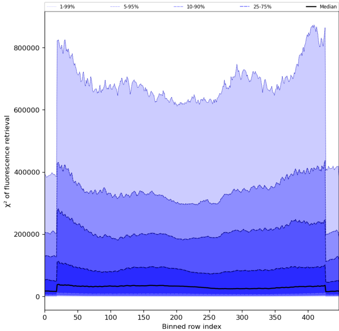
Figure 59: Along track statistics of “ \chi^2 of fluorescence retrieval” for 2024-07-24 to 2024-07-26
