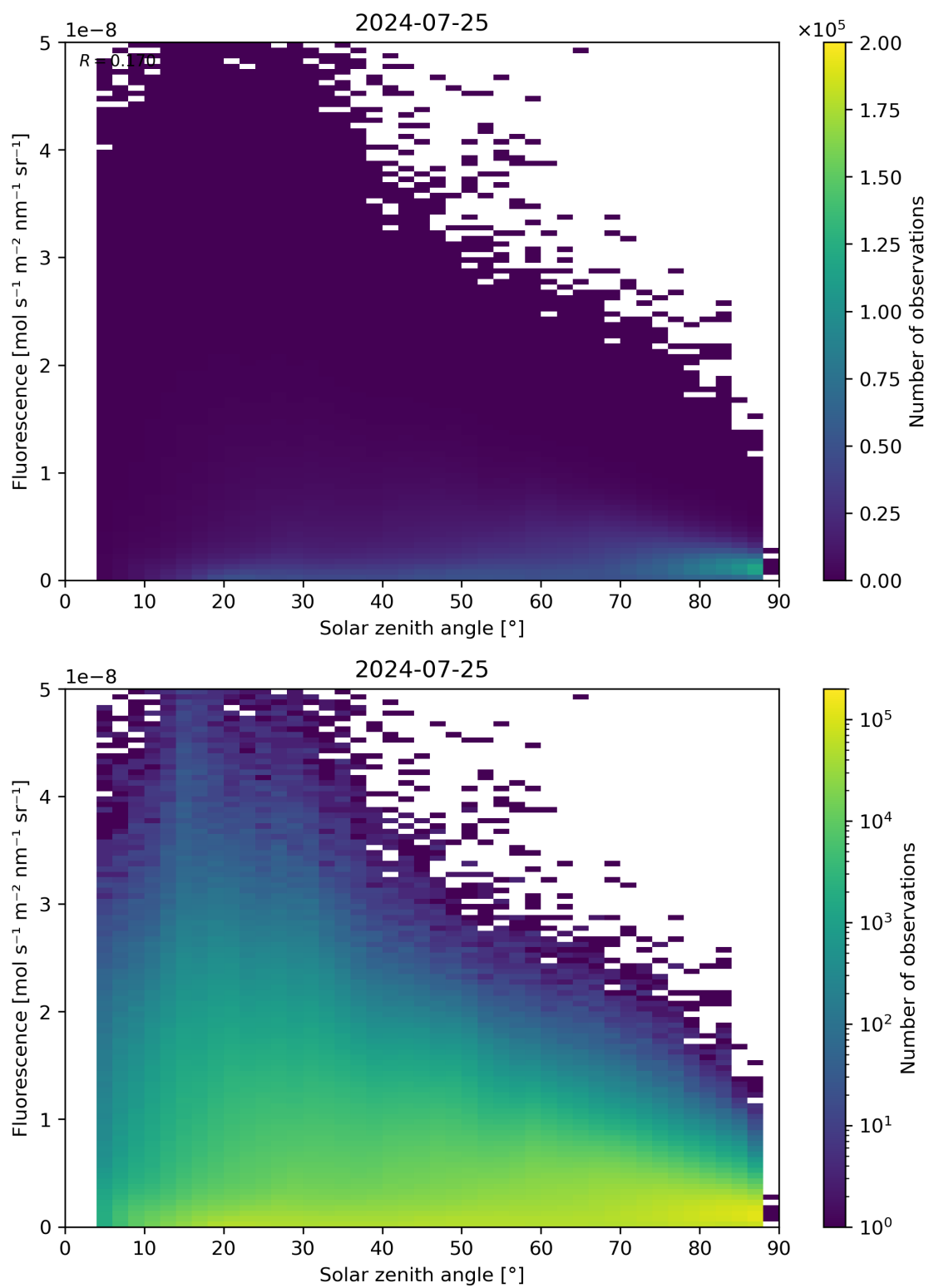
Figure 112: Scatter density plot of “Solar zenith angle” against “Fluorescence” for 2024-07-24 to 2024-07-26.
