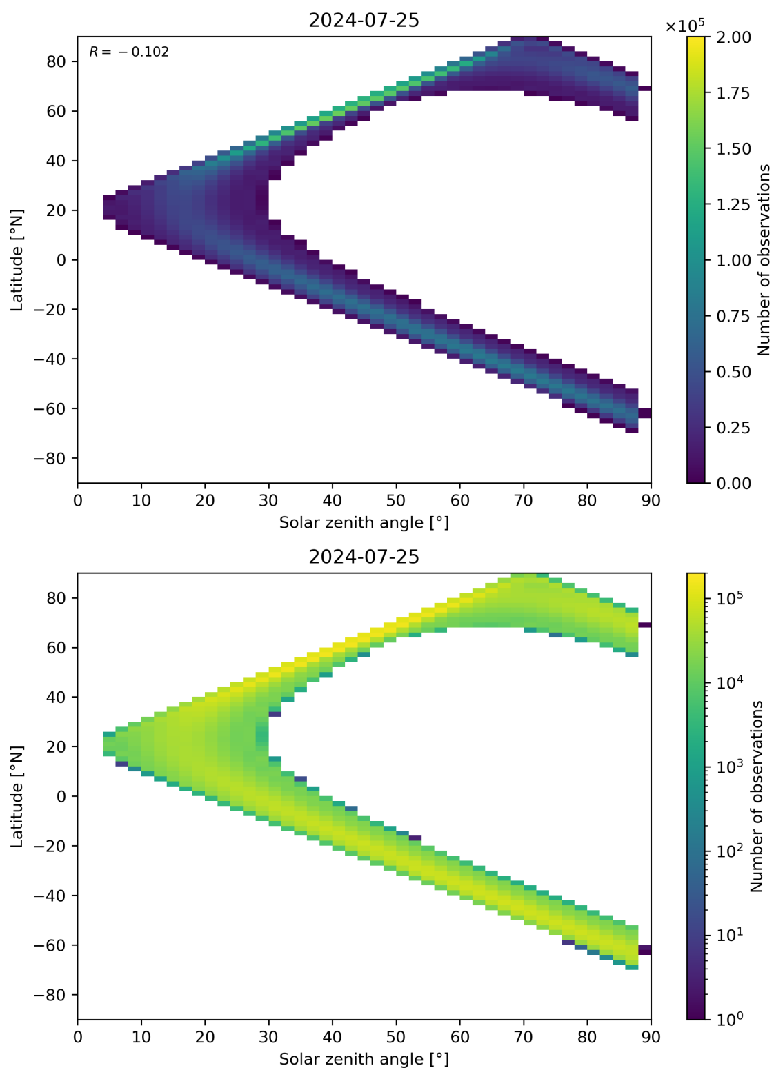
Figure 113: Scatter density plot of “Solar zenith angle” against “Latitude” for 2024-07-24 to 2024-07-26.
