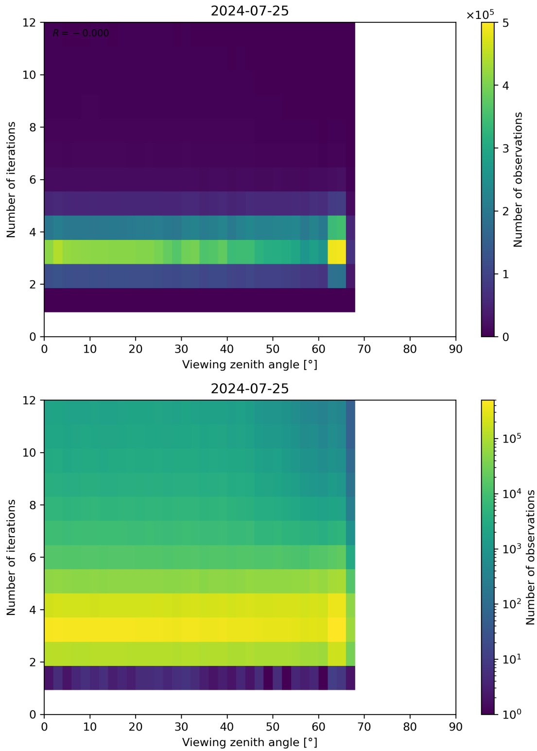
Figure 124: Scatter density plot of “Viewing zenith angle” against “Number of iterations” for 2024-07-24 to 2024-07-26.
