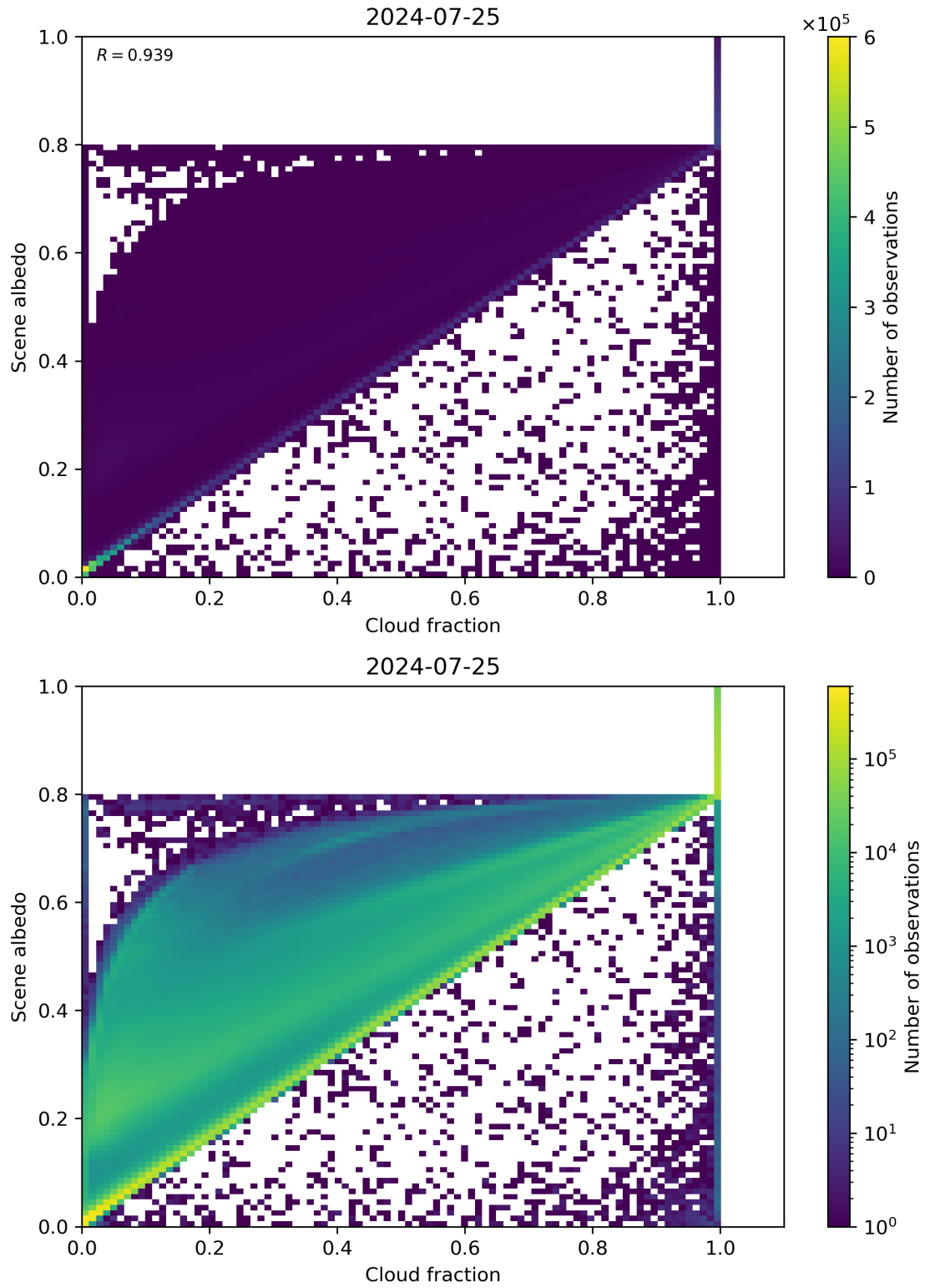
Figure 75: Scatter density plot of “Cloud fraction” against “Scene albedo” for 2024-07-24 to 2024-07-26.
