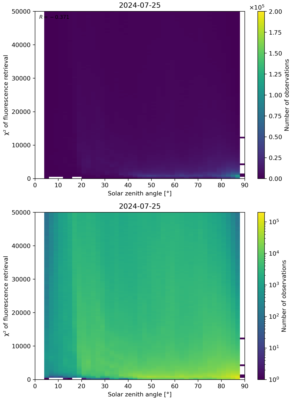
Figure 109: Scatter density plot of “Solar zenith angle” against “ \chi^2 of fluorescence retrieval” for 2024-07-24 to 2024-07-26.
