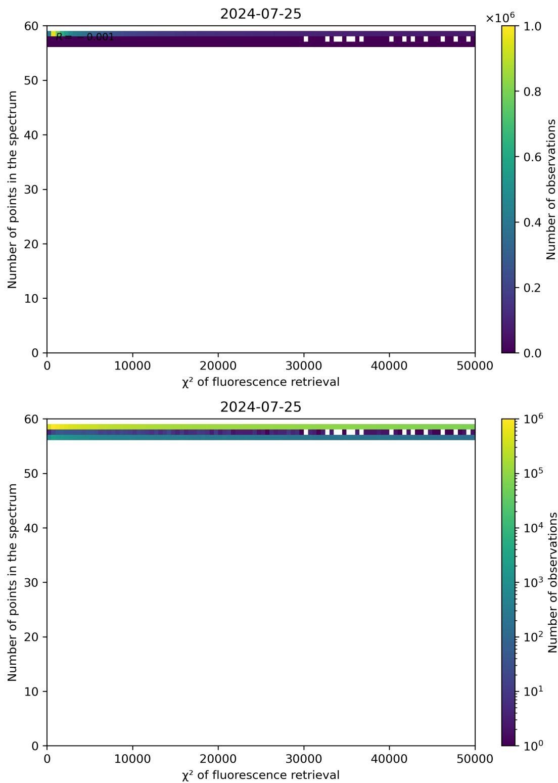
Figure 68: Scatter density plot of “ \chi^2 of fluorescence retrieval” against “Number of points in the spectrum” for 2024-07-24 to 2024-07-26.
