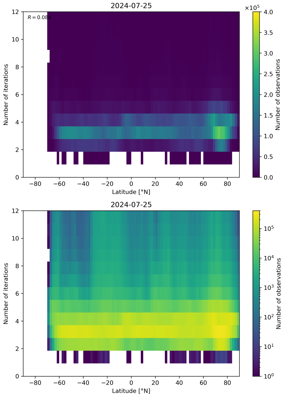
Figure 93: Scatter density plot of “Latitude” against “Number of iterations” for 2024-07-24 to 2024-07-26.
