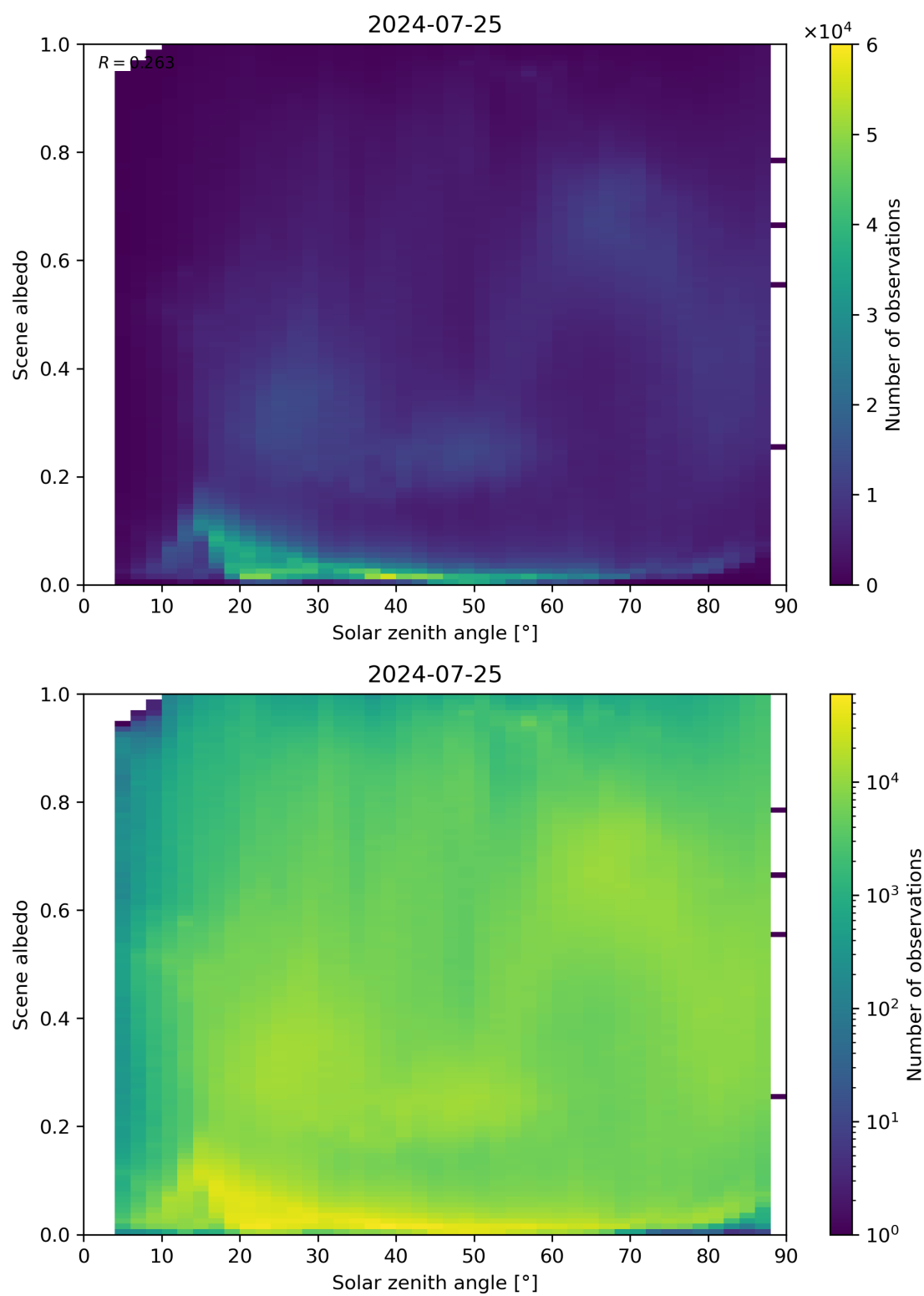
Figure 116: Scatter density plot of “Solar zenith angle” against “Scene albedo” for 2024-07-24 to 2024-07-26.
