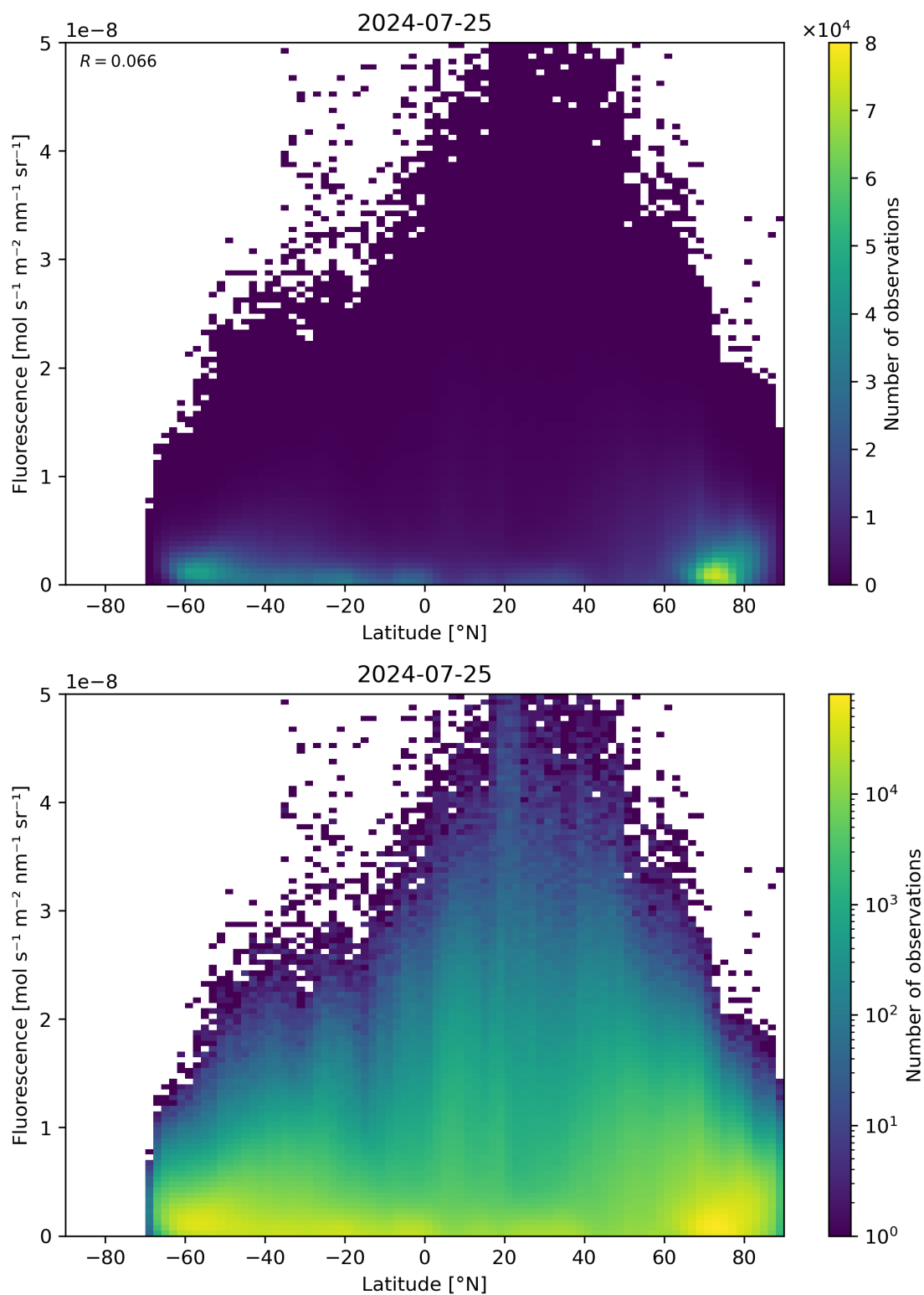
Figure 92: Scatter density plot of “Latitude” against “Fluorescence” for 2024-07-24 to 2024-07-26.
