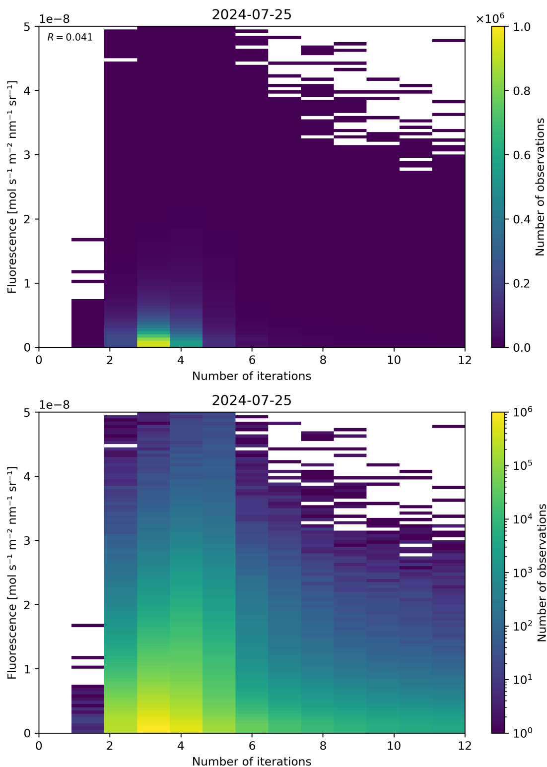
Figure 98: Scatter density plot of “Number of iterations” against “Fluorescence” for 2024-07-24 to 2024-07-26.
