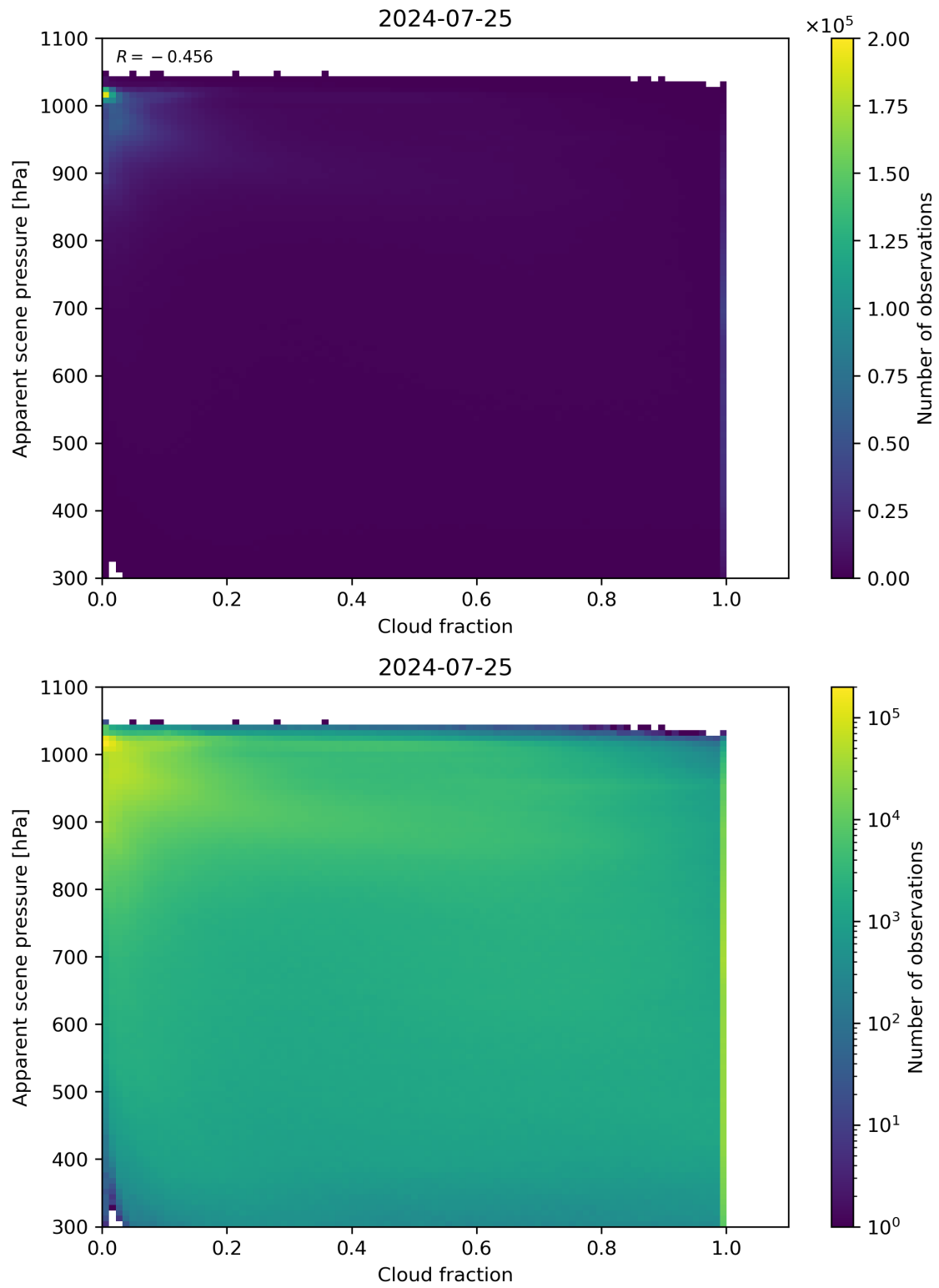
Figure 70: Scatter density plot of “Cloud fraction” against “Apparent scene pressure” for 2024-07-24 to 2024-07-26.
