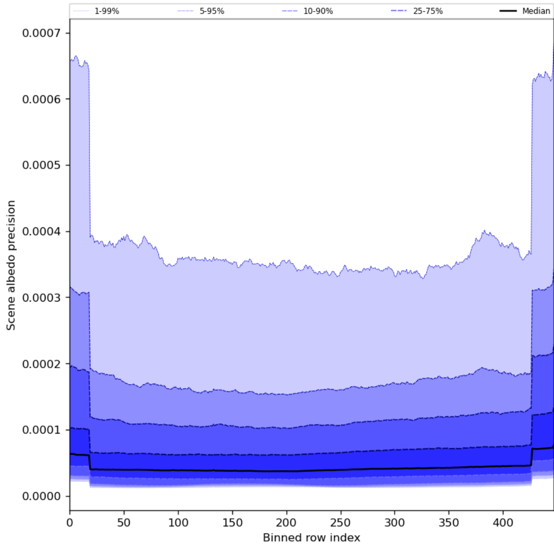
Figure 52: Along track statistics of “Scene albedo precision” for 2024-07-24 to 2024-07-26
