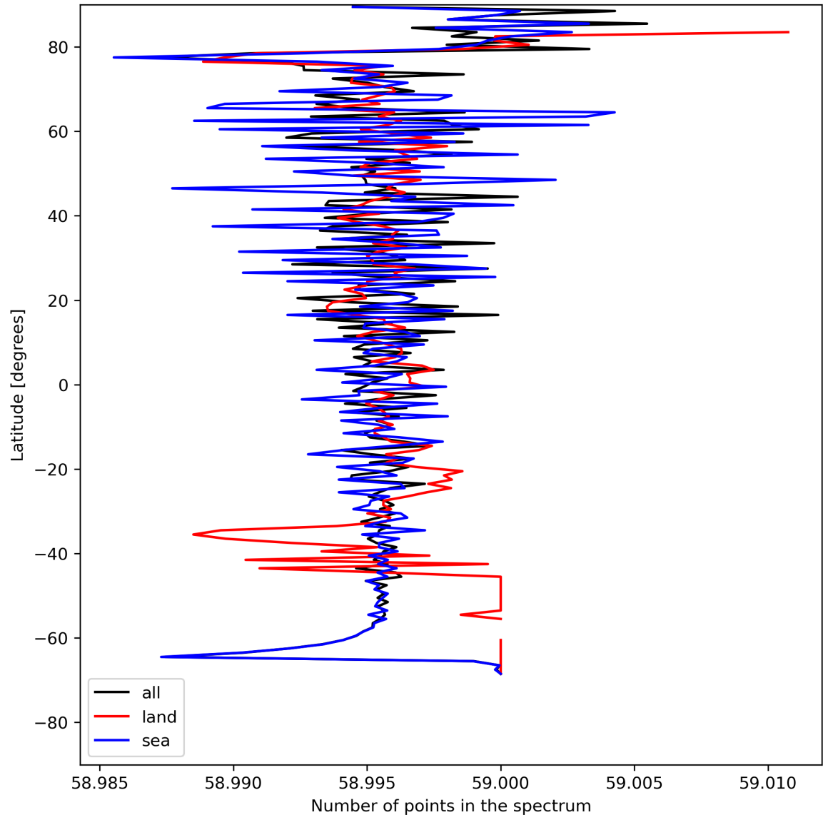
Figure 27: Zonal average of “Number of points in the spectrum” for 2024-07-24 to 2024-07-26.
