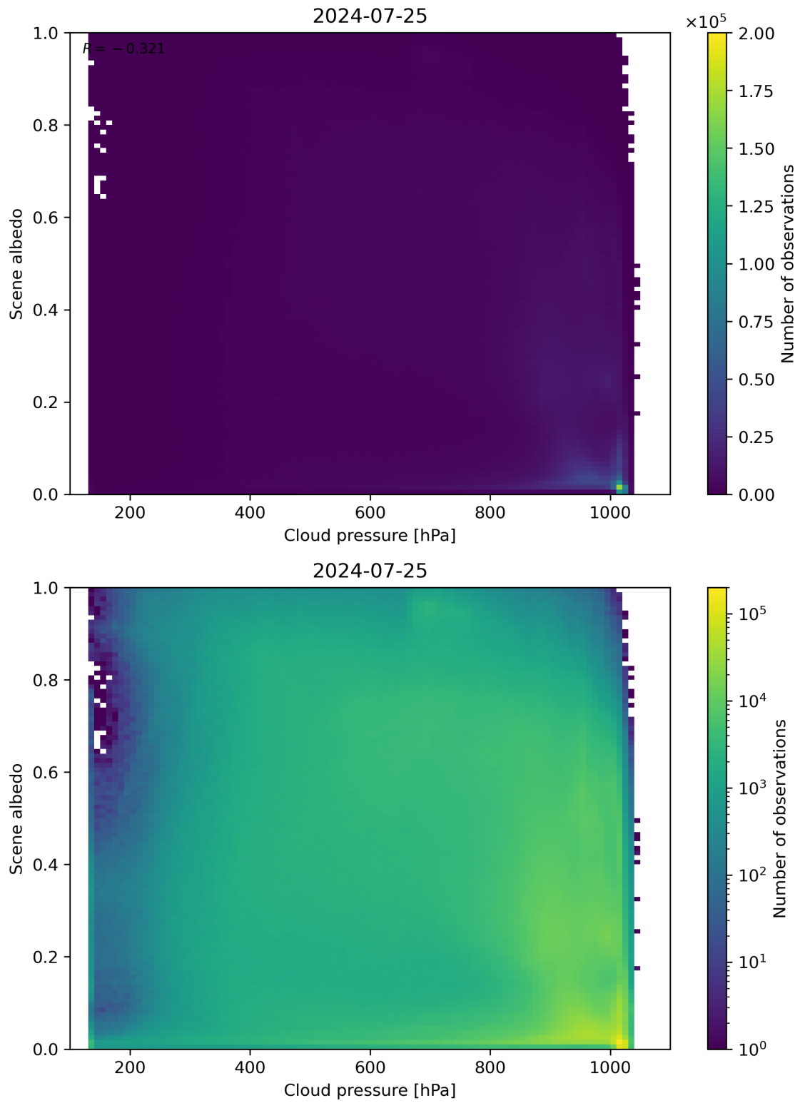
Figure 83: Scatter density plot of “Cloud pressure” against “Scene albedo” for 2024-07-24 to 2024-07-26.
