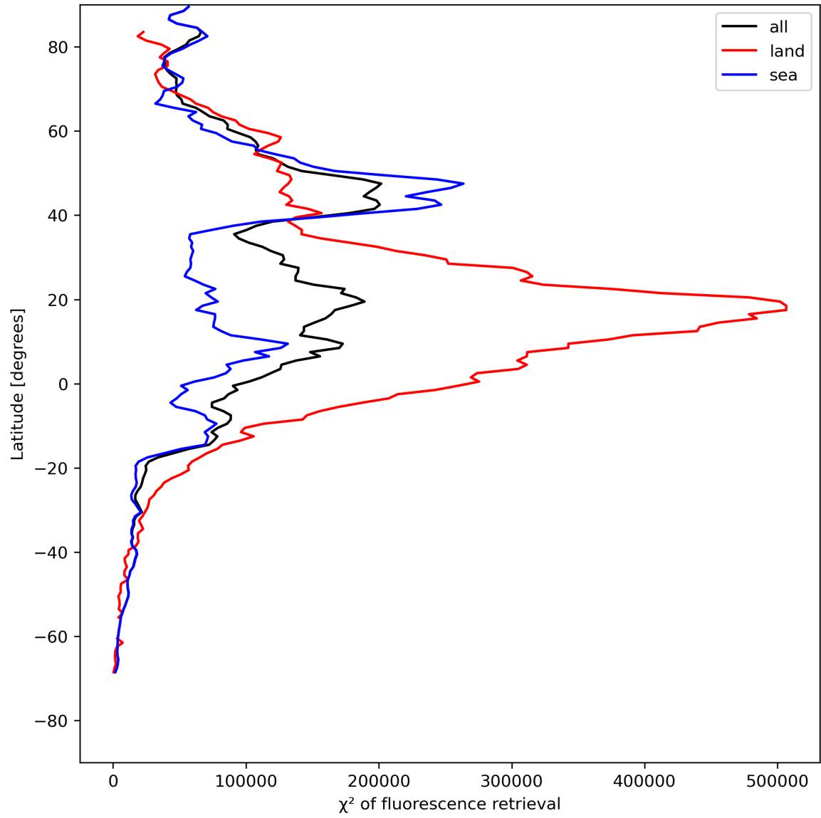
Figure 25: Zonal average of “ \chi^2 of fluorescence retrieval” for 2024-07-24 to 2024-07-26.
