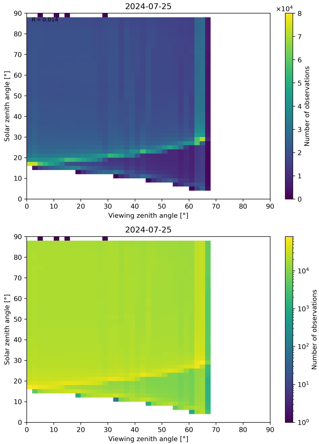
Figure 127: Scatter density plot of “Viewing zenith angle” against “Solar zenith angle” for 2024-07-24 to 2024-07-26.
