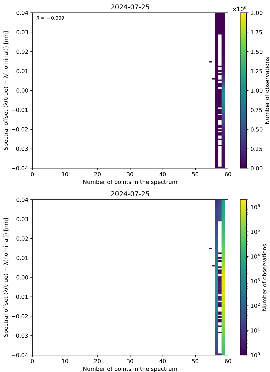
Figure 101: Scatter density plot of “Number of points in the spectrum” against “Spectral offset ( \lambda(\text{true}) - \lambda(\text{nominal}) )” for 2024-07-24 to 2024-07-26.
