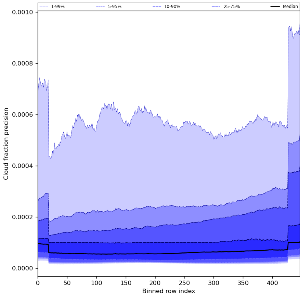
Figure 50: Along track statistics of “Cloud fraction precision” for 2024-07-24 to 2024-07-26
