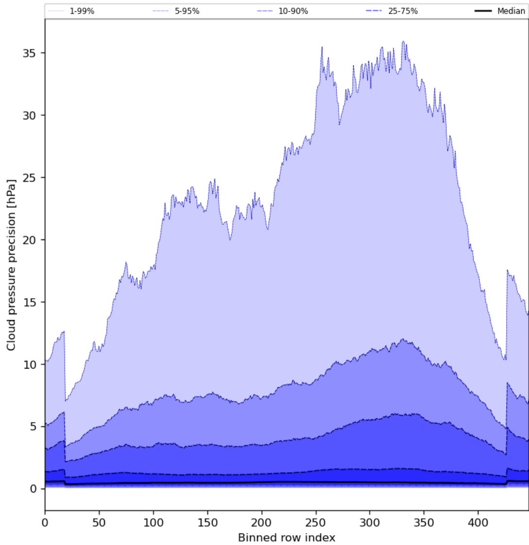
Figure 48: Along track statistics of “Cloud pressure precision” for 2024-07-24 to 2024-07-26
