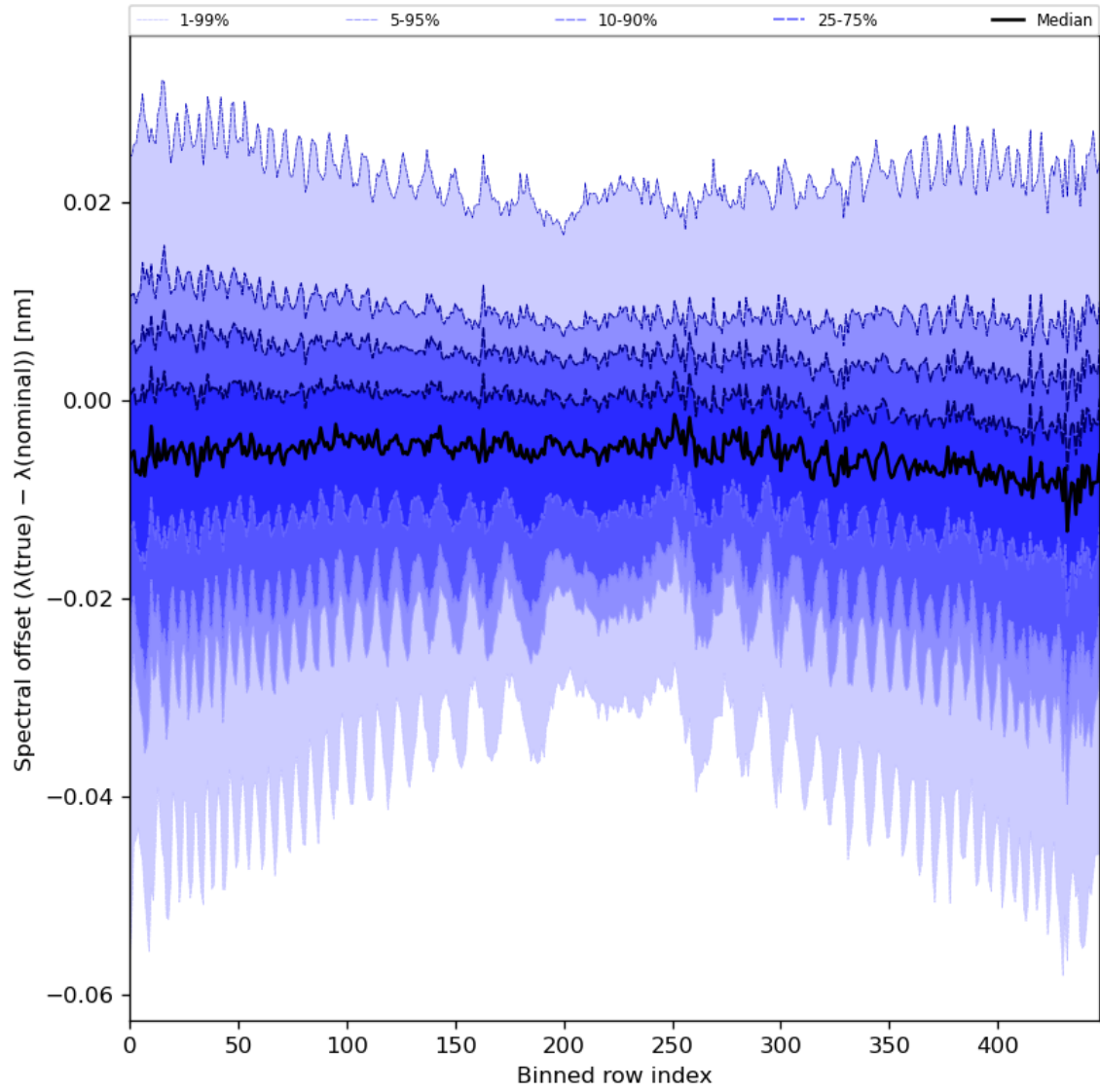
Figure 62: Along track statistics of “Spectral offset ( \lambda(\text{true}) - \lambda(\text{nominal}) )” for 2024-07-24 to 2024-07-26
