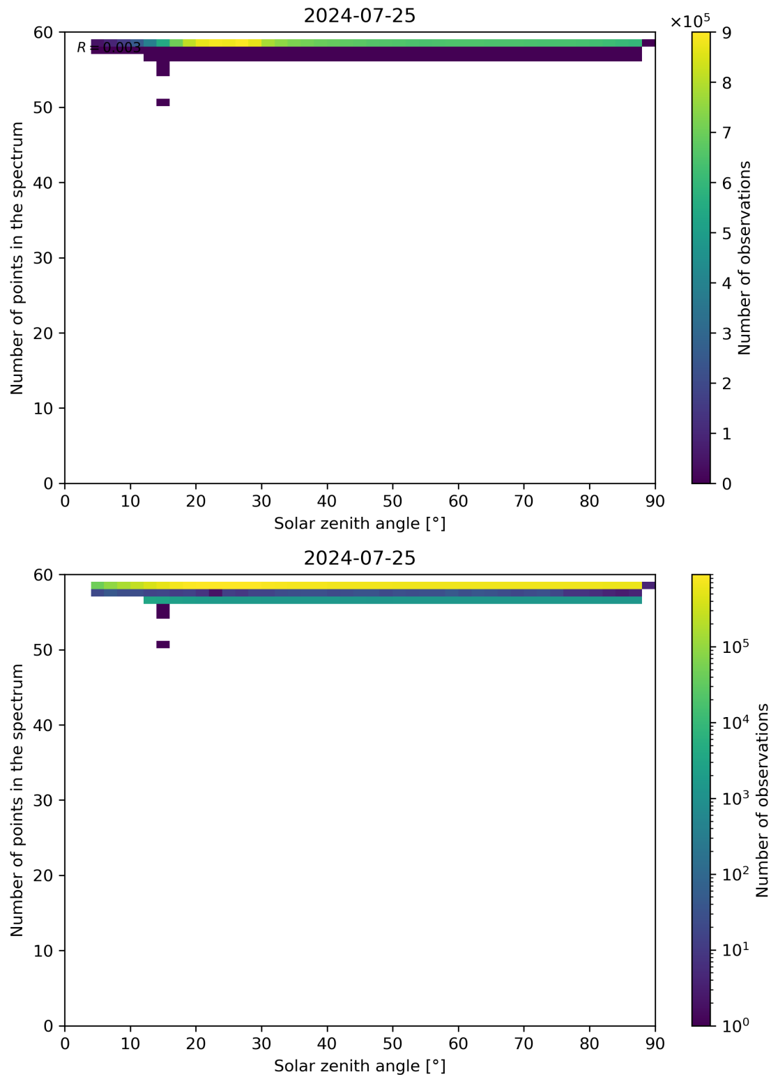
Figure 115: Scatter density plot of “Solar zenith angle” against “Number of points in the spectrum” for 2024-07-24 to 2024-07-26.
