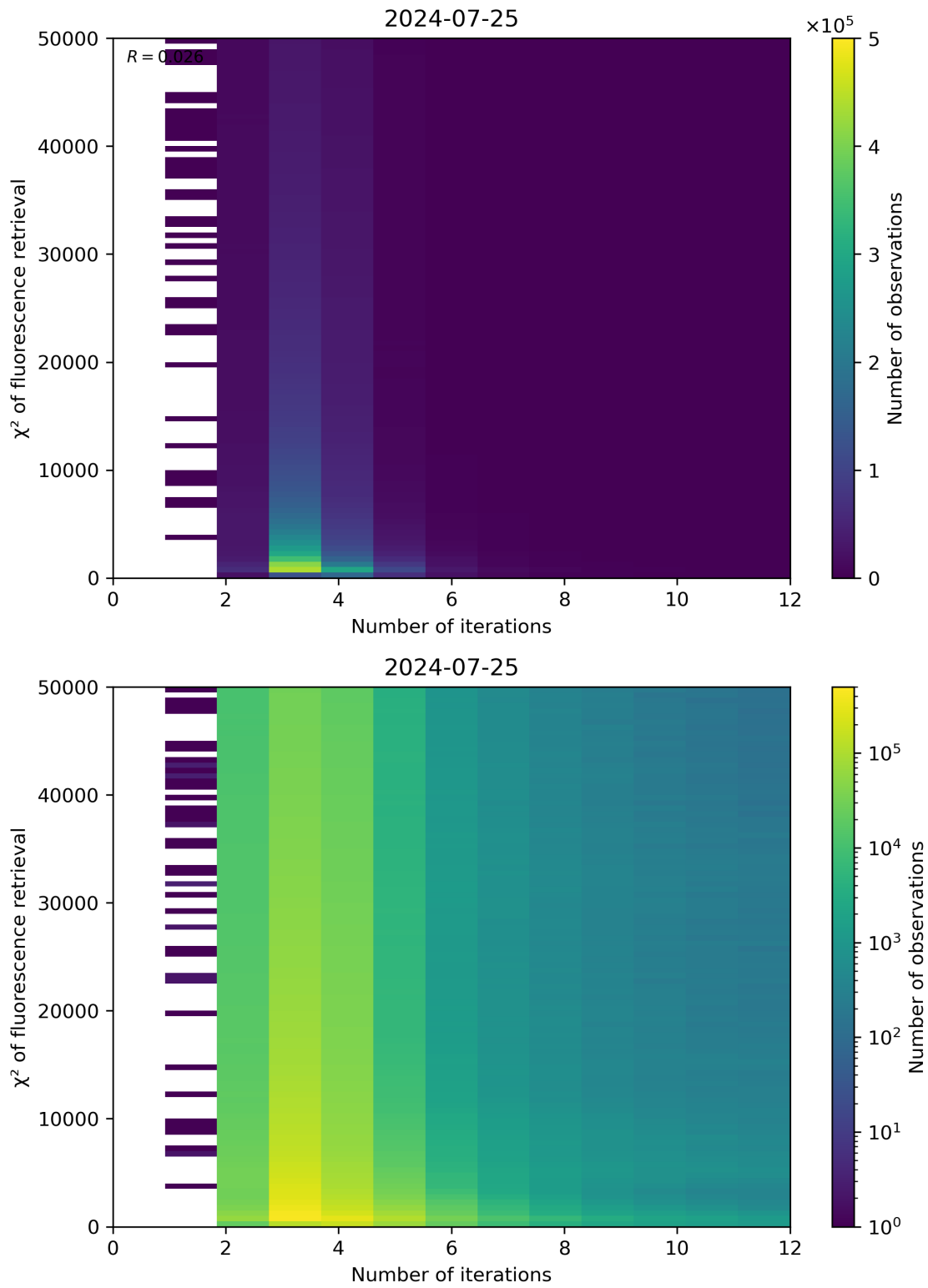
Figure 97: Scatter density plot of “Number of iterations” against “ \chi^2 of fluorescence retrieval” for 2024-07-24 to 2024-07-26.
