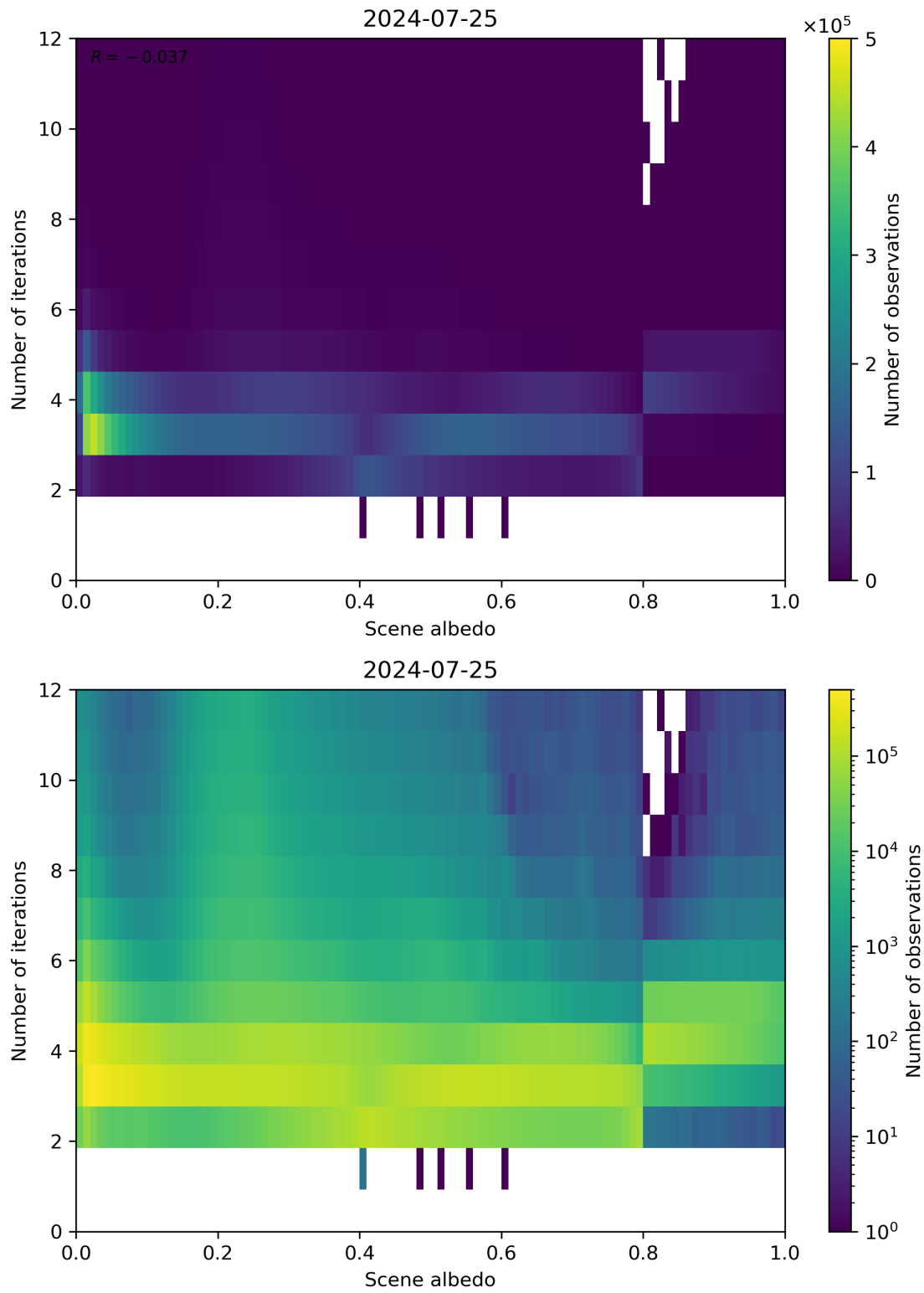
Figure 105: Scatter density plot of “Scene albedo” against “Number of iterations” for 2024-07-24 to 2024-07-26.
