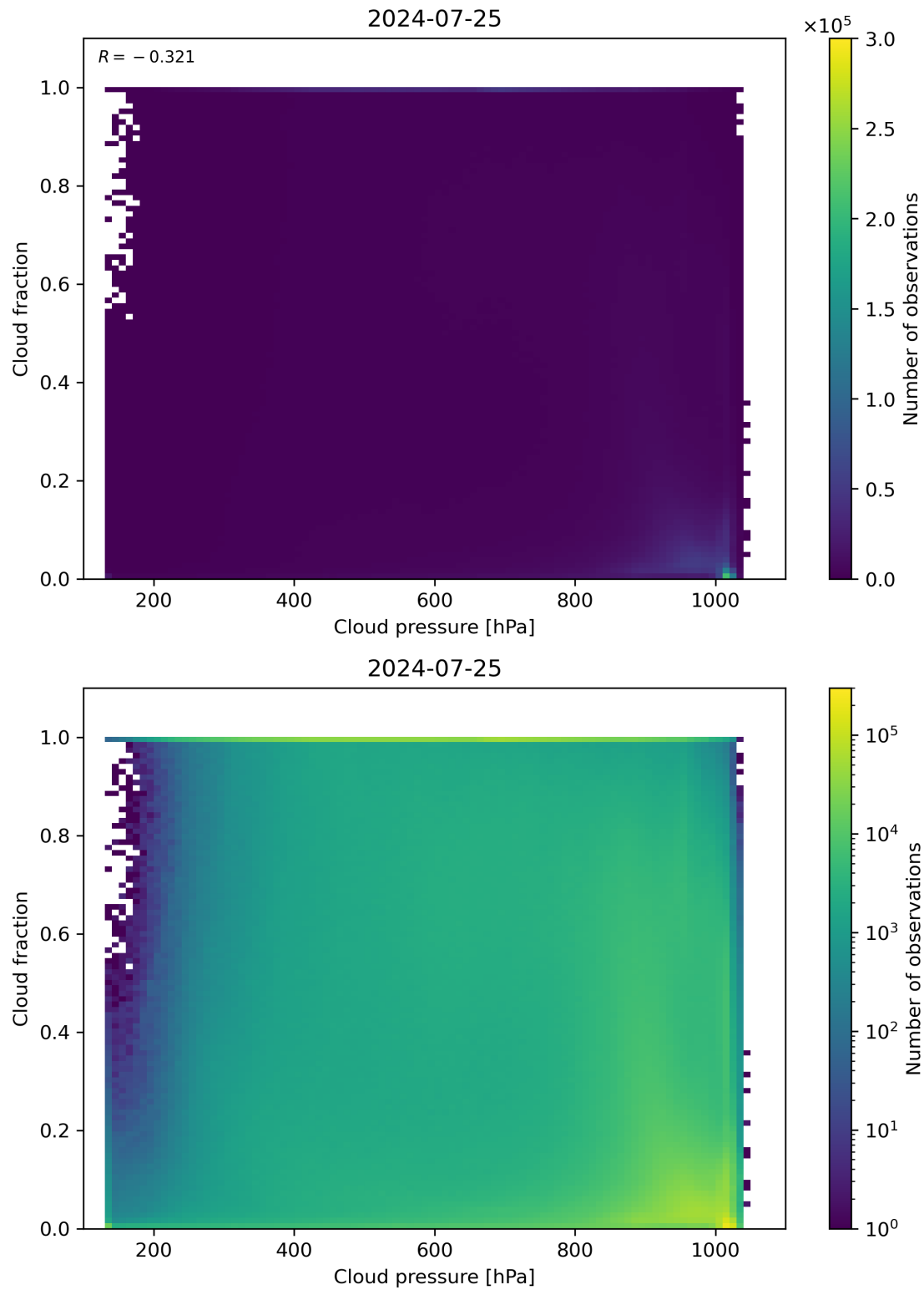
Figure 79: Scatter density plot of “Cloud pressure” against “Cloud fraction” for 2024-07-24 to 2024-07-26.
