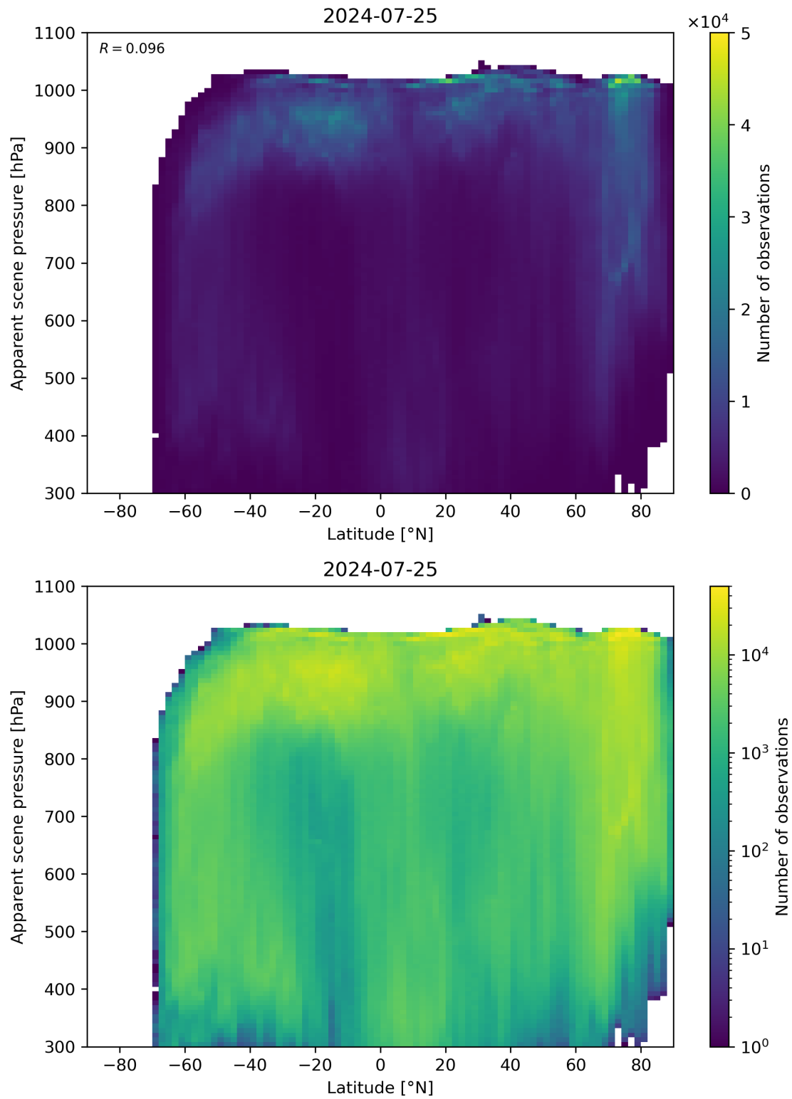
Figure 88: Scatter density plot of “Latitude” against “Apparent scene pressure” for 2024-07-24 to 2024-07-26.
