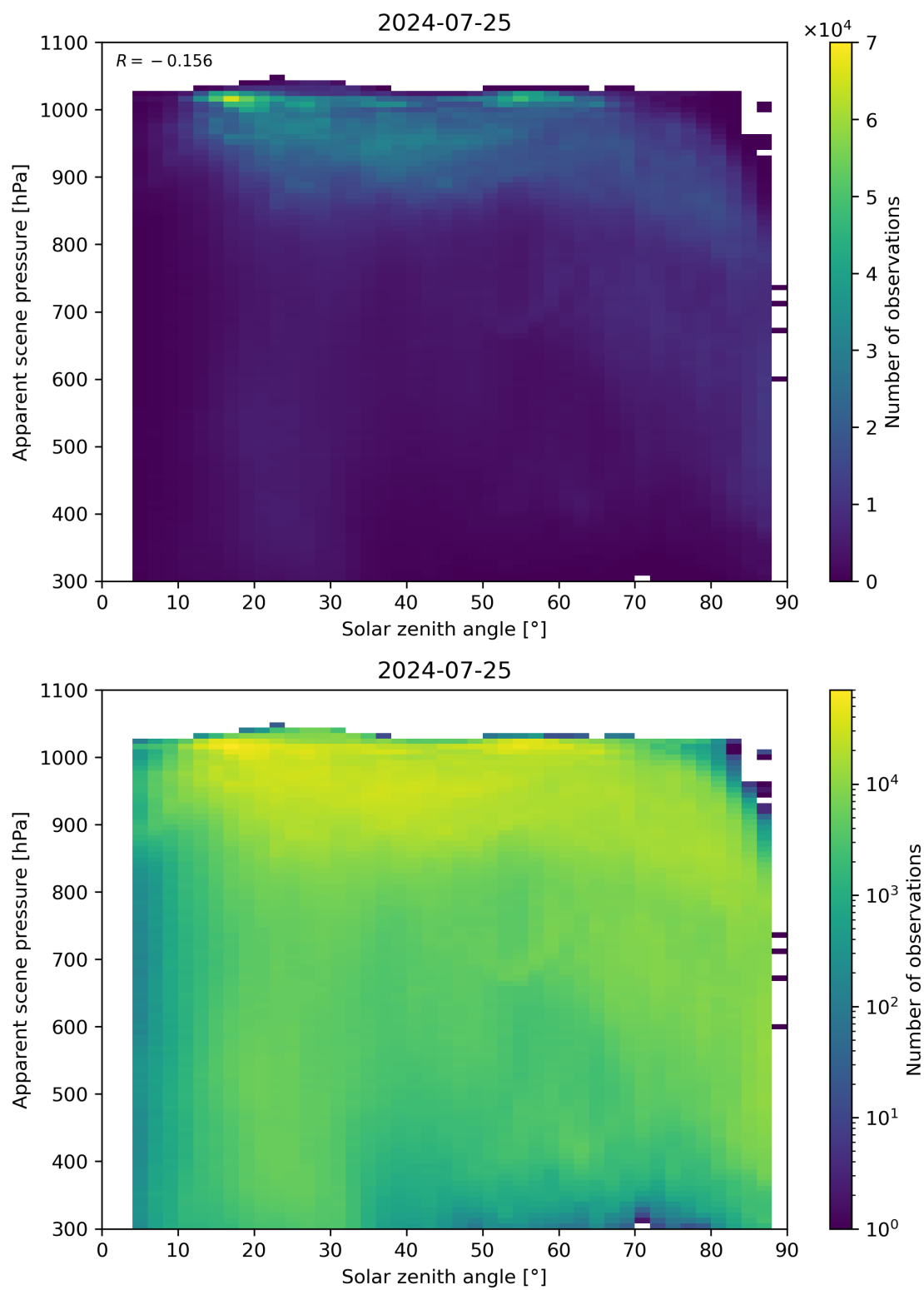
Figure 108: Scatter density plot of “Solar zenith angle” against “Apparent scene pressure” for 2024-07-24 to 2024-07-26.
