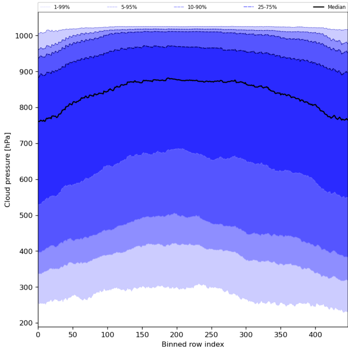
Figure 47: Along track statistics of “Cloud pressure” for 2024-07-24 to 2024-07-26
