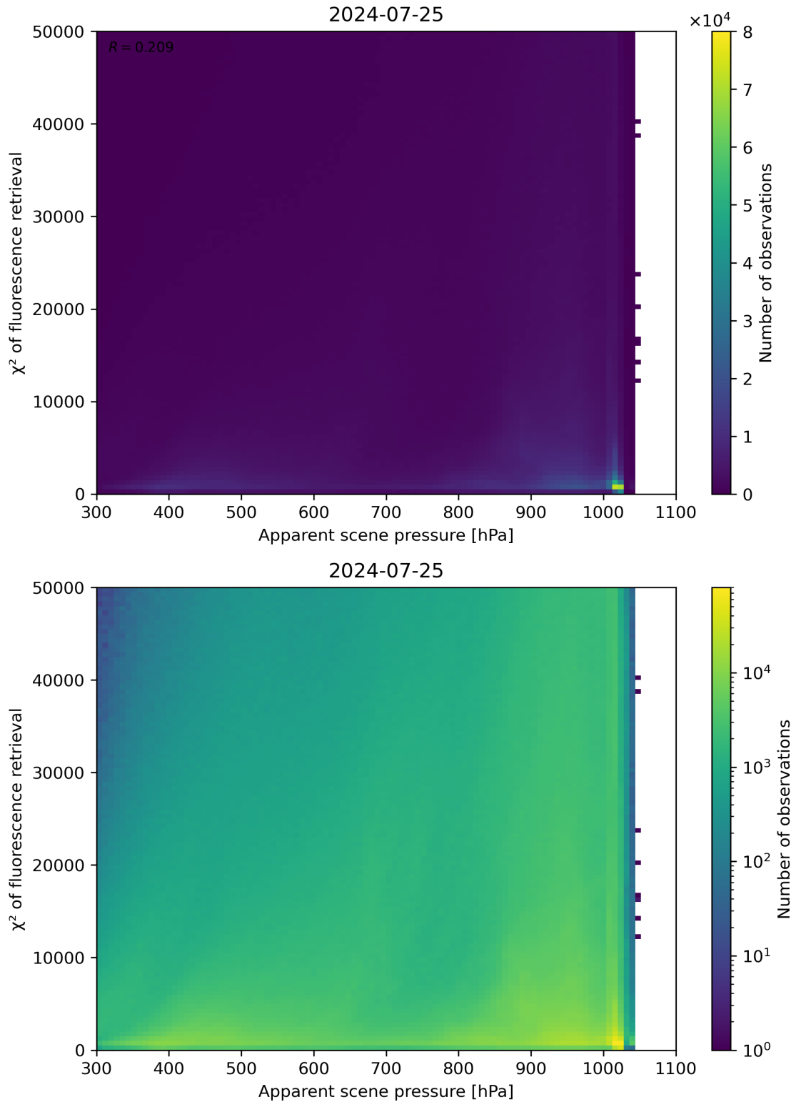
Figure 63: Scatter density plot of “Apparent scene pressure” against “ \chi^2 of fluorescence retrieval” for 2024-07-24 to 2024-07-26.
