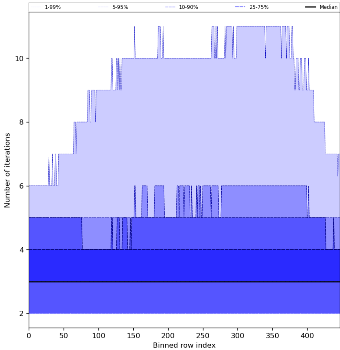
Figure 56: Along track statistics of “Number of iterations” for 2024-07-24 to 2024-07-26
