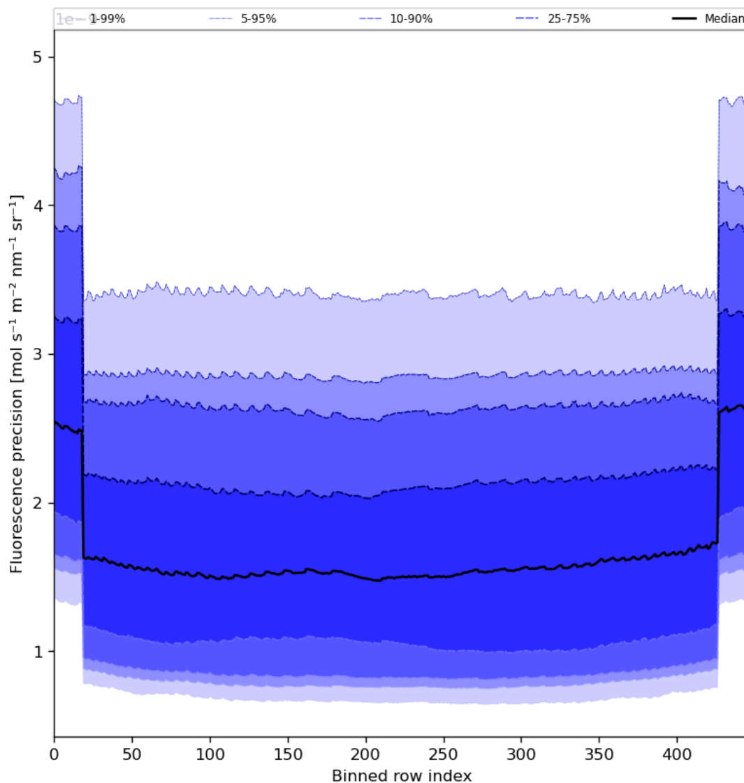
Figure 58: Along track statistics of “Fluorescence precision” for 2024-07-24 to 2024-07-26
