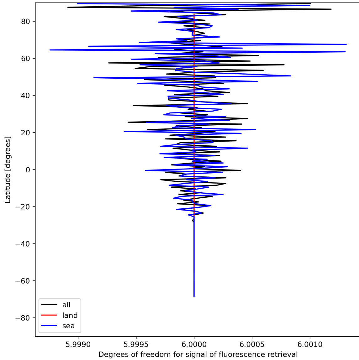
Figure 26: Zonal average of “Degrees of freedom for signal of fluorescence retrieval” for 2024-07-24 to 2024-07-26.
