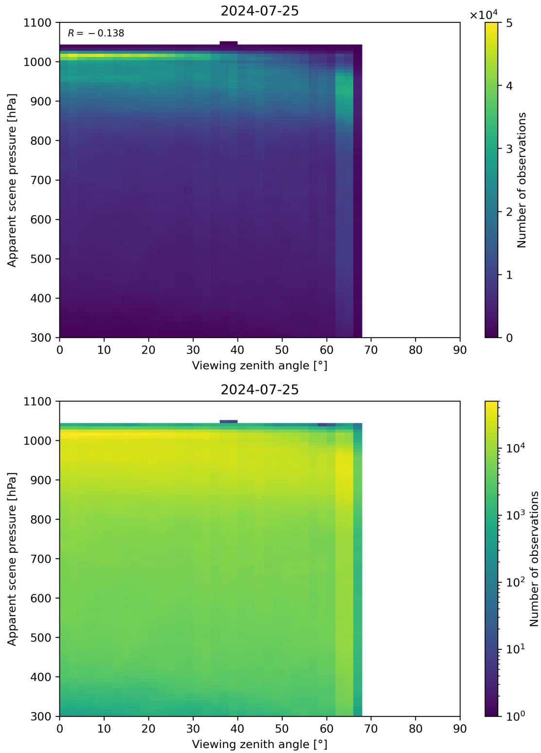
Figure 118: Scatter density plot of “Viewing zenith angle” against “Apparent scene pressure” for 2024-07-24 to 2024-07-26.
