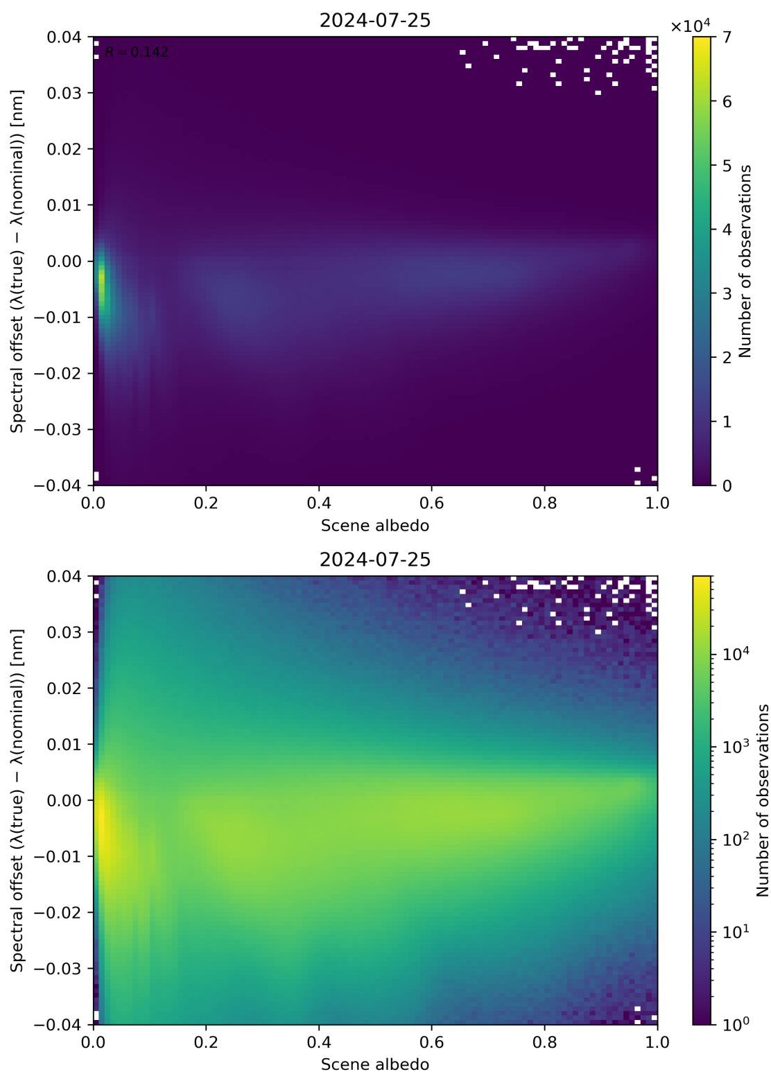
Figure 107: Scatter density plot of “Scene albedo” against “Spectral offset ( \lambda(\text{true}) - \lambda(\text{nominal}) )” for 2024-07-24 to 2024-07-26.
