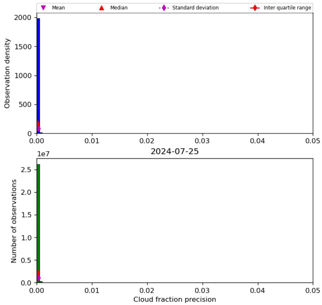
Figure 33: Histogram of “Cloud fraction precision” for 2024-07-24 to 2024-07-26
