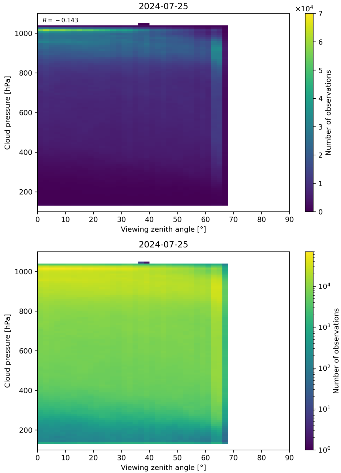
Figure 121: Scatter density plot of “Viewing zenith angle” against “Cloud pressure” for 2024-07-24 to 2024-07-26.
