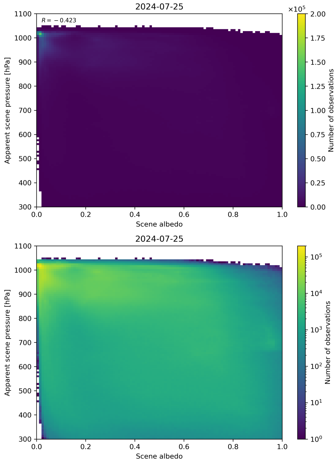
Figure 102: Scatter density plot of “Scene albedo” against “Apparent scene pressure” for 2024-07-24 to 2024-07-26.
