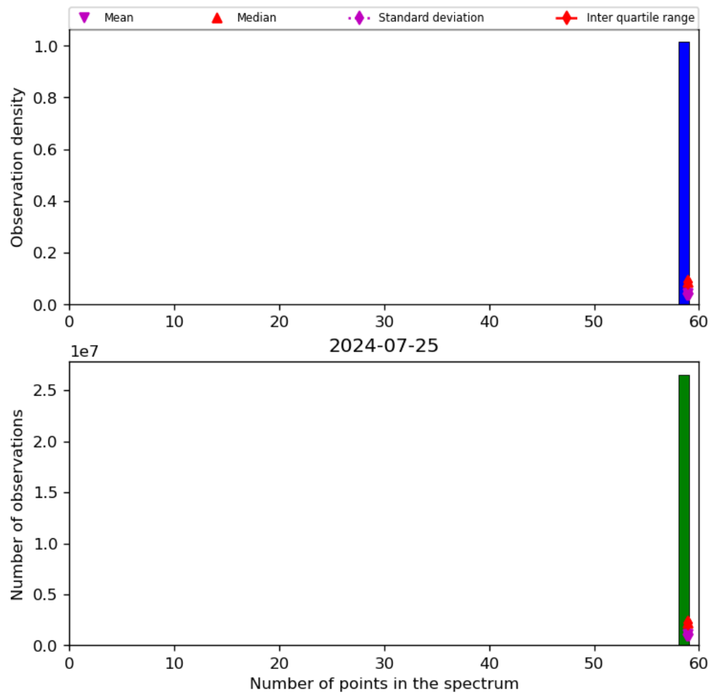
Figure 44: Histogram of “Number of points in the spectrum” for 2024-07-24 to 2024-07-26
