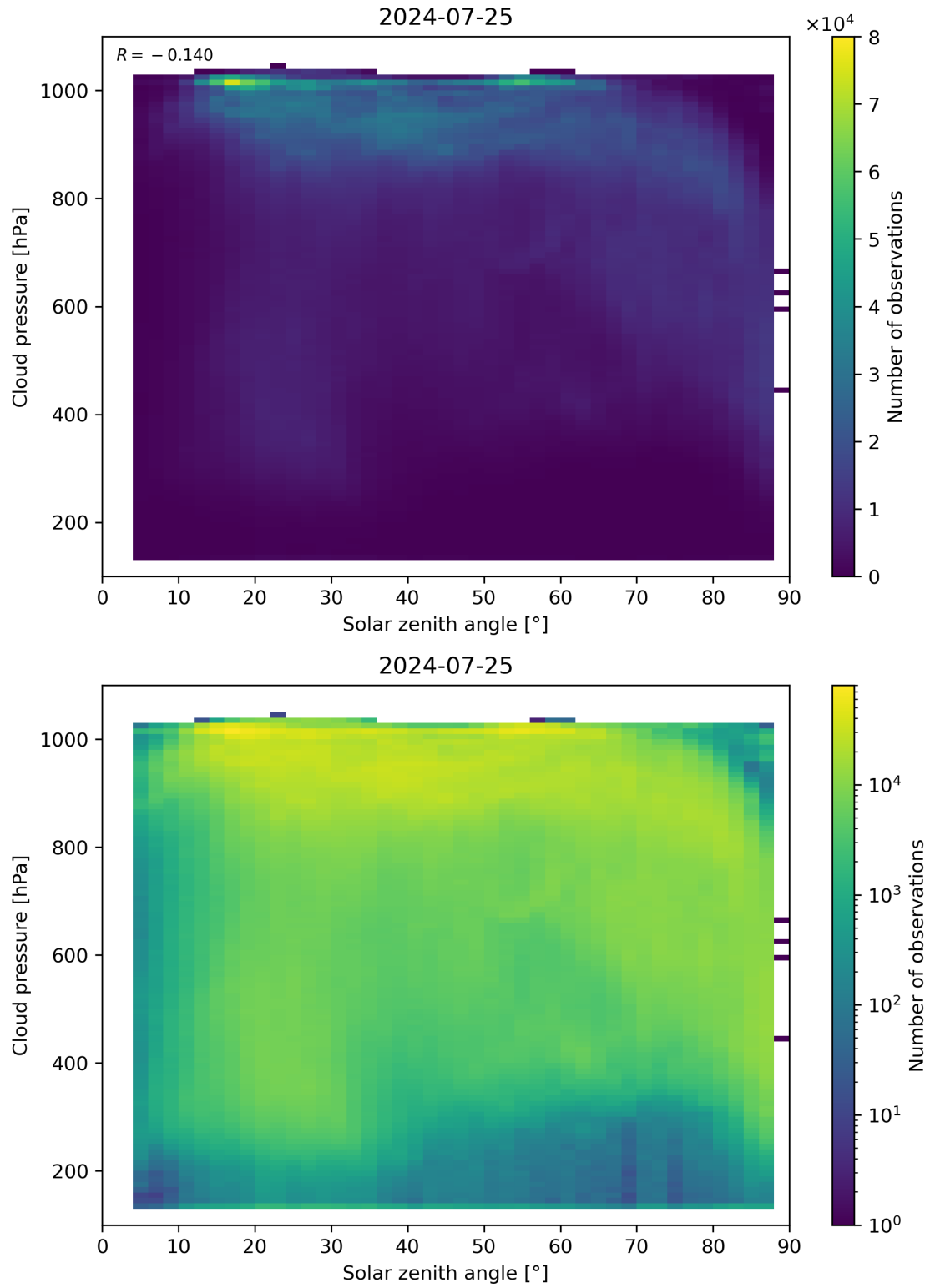
Figure 111: Scatter density plot of “Solar zenith angle” against “Cloud pressure” for 2024-07-24 to 2024-07-26.
