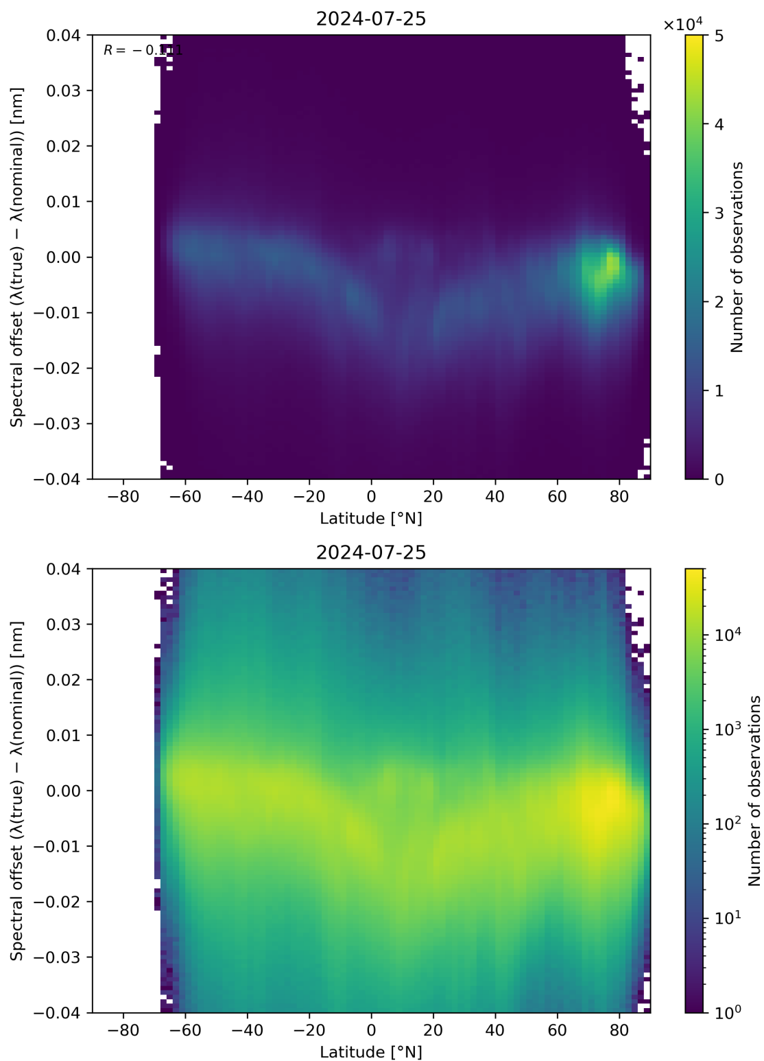
Figure 96: Scatter density plot of “Latitude” against “Spectral offset ( \lambda(\text{true}) - \lambda(\text{nominal}) )” for 2024-07-24 to 2024-07-26.
