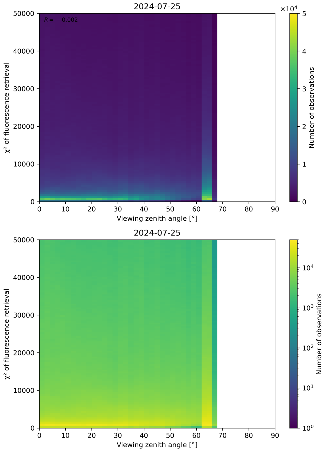
Figure 119: Scatter density plot of “Viewing zenith angle” against “ \chi^2 of fluorescence retrieval” for 2024-07-24 to 2024-07-26.
