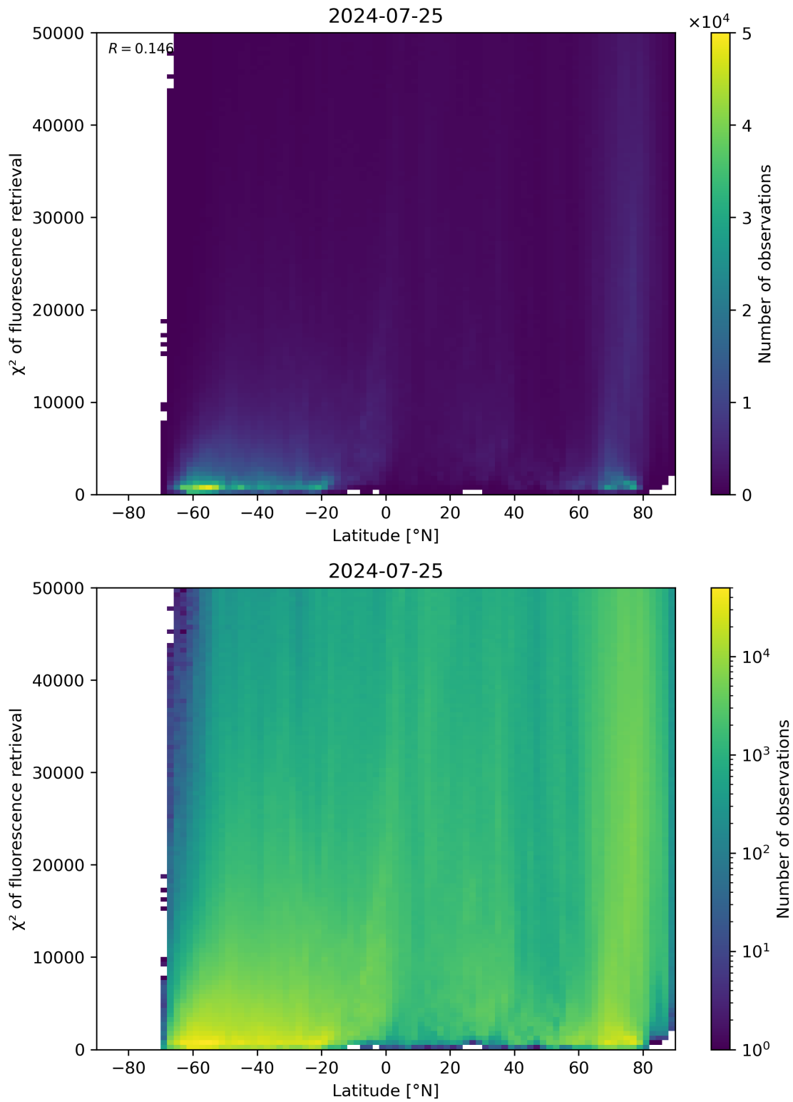
Figure 89: Scatter density plot of “Latitude” against “ \chi^2 of fluorescence retrieval” for 2024-07-24 to 2024-07-26.
