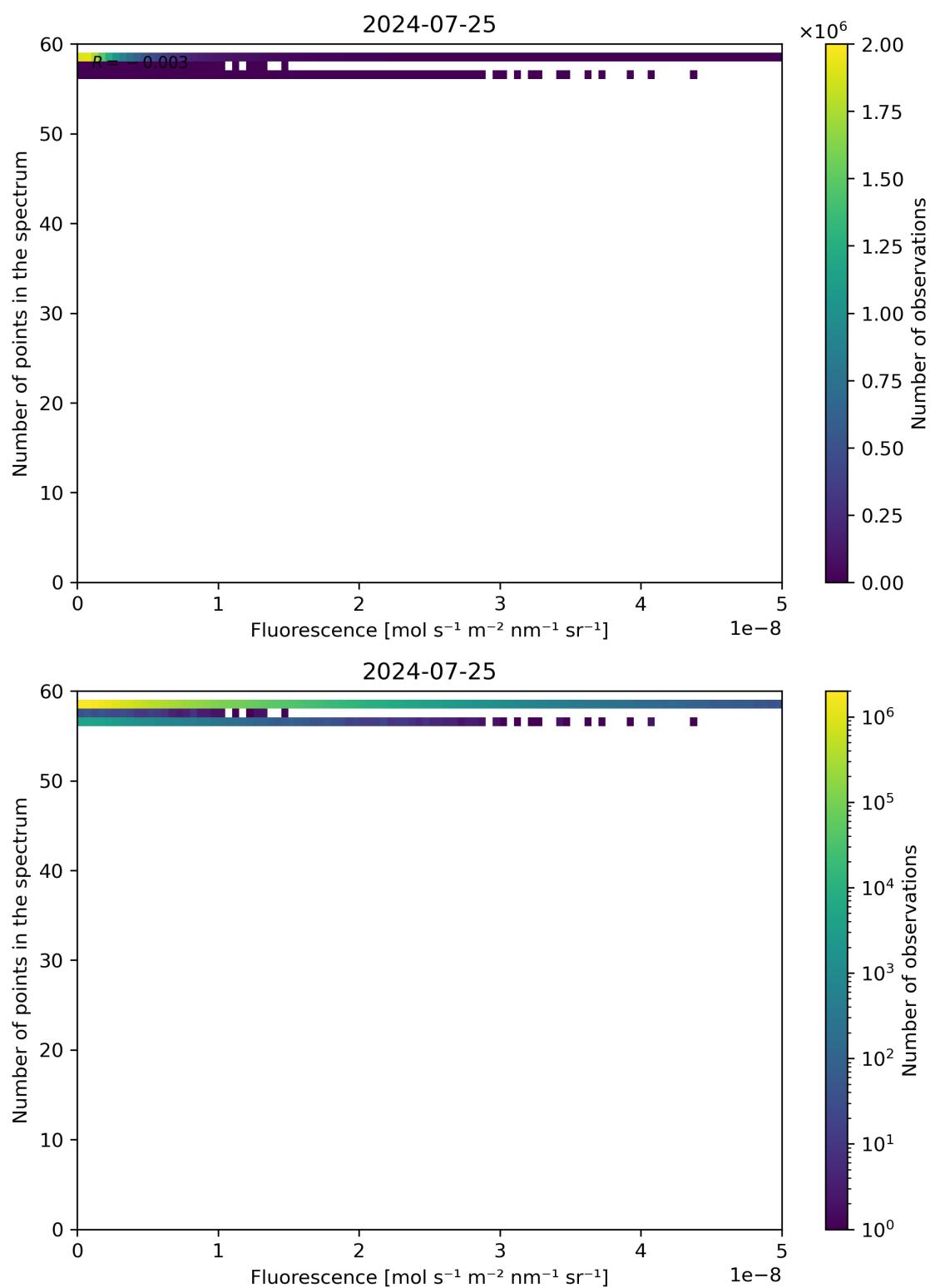
Figure 86: Scatter density plot of “Fluorescence” against “Number of points in the spectrum” for 2024-07-24 to 2024-07-26.
