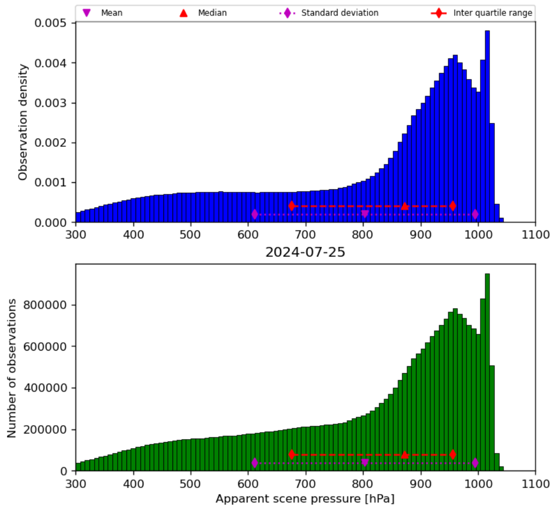
Figure 36: Histogram of “Apparent scene pressure” for 2024-07-24 to 2024-07-26
