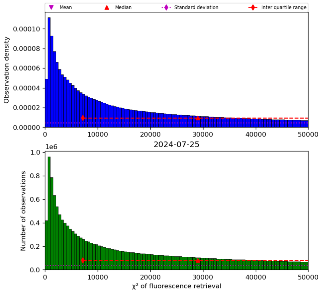
Figure 42: Histogram of “ \chi^2 of fluorescence retrieval” for 2024-07-24 to 2024-07-26
