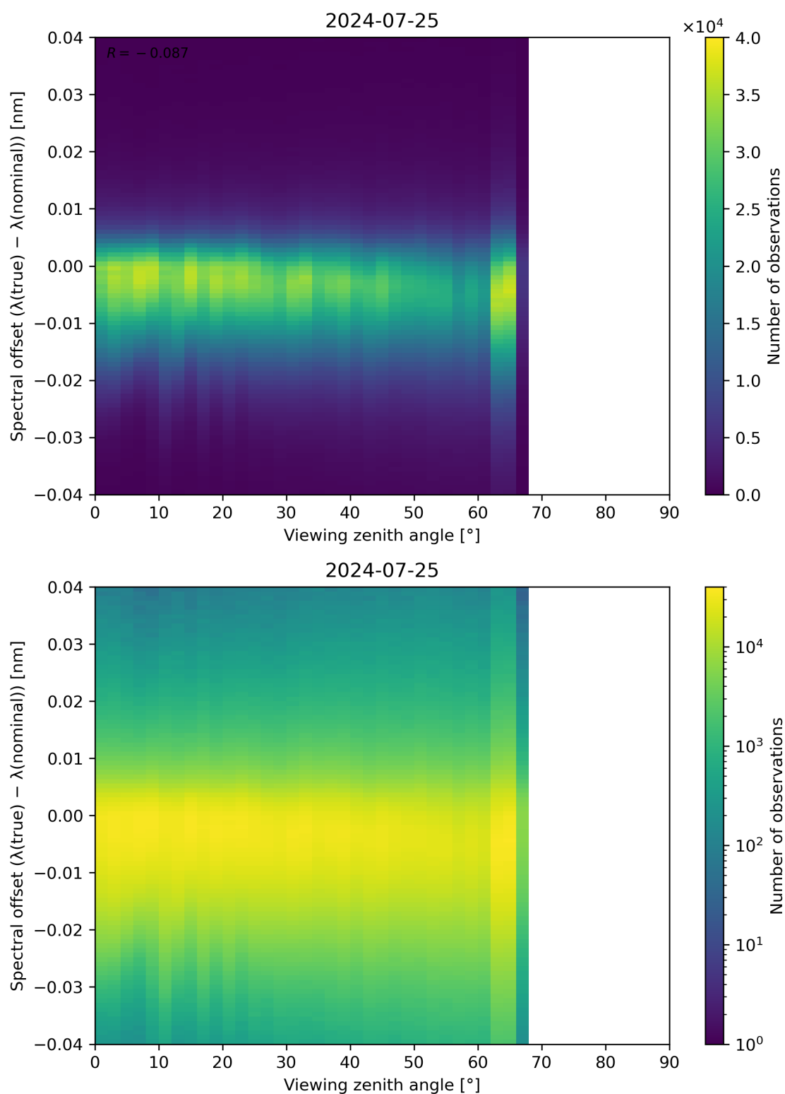
Figure 128: Scatter density plot of “Viewing zenith angle” against “Spectral offset ( \lambda(\text{true}) - \lambda(\text{nominal}) )” for 2024-07-24 to 2024-07-26.
