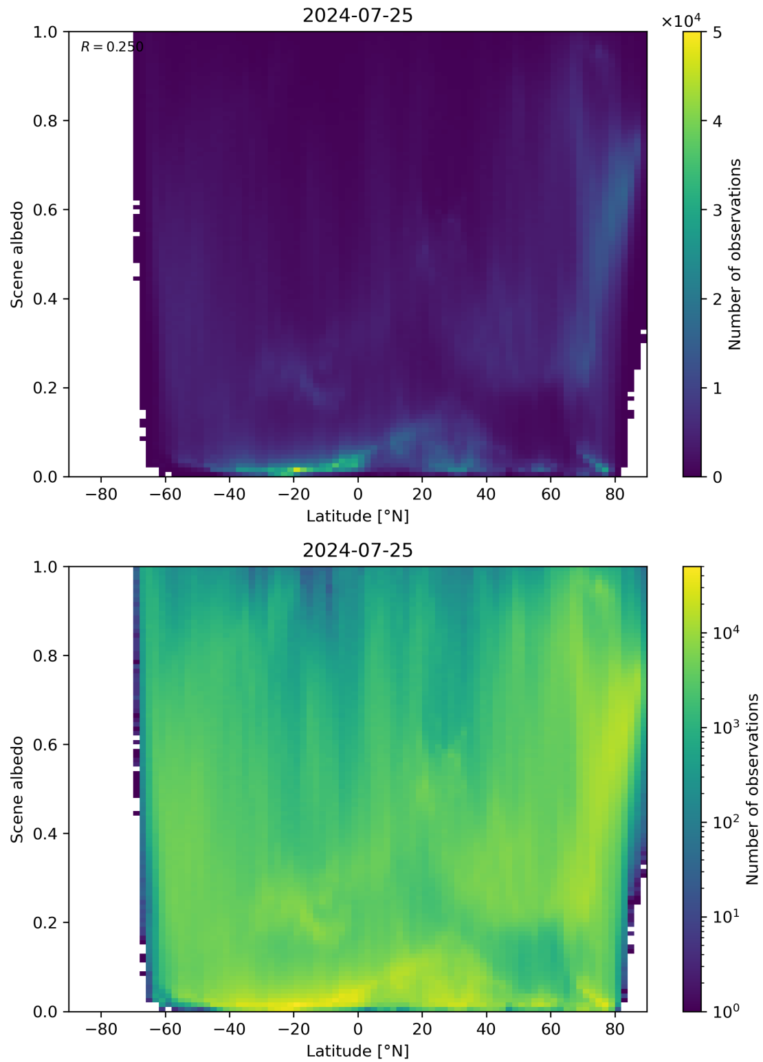
Figure 95: Scatter density plot of “Latitude” against “Scene albedo” for 2024-07-24 to 2024-07-26.
