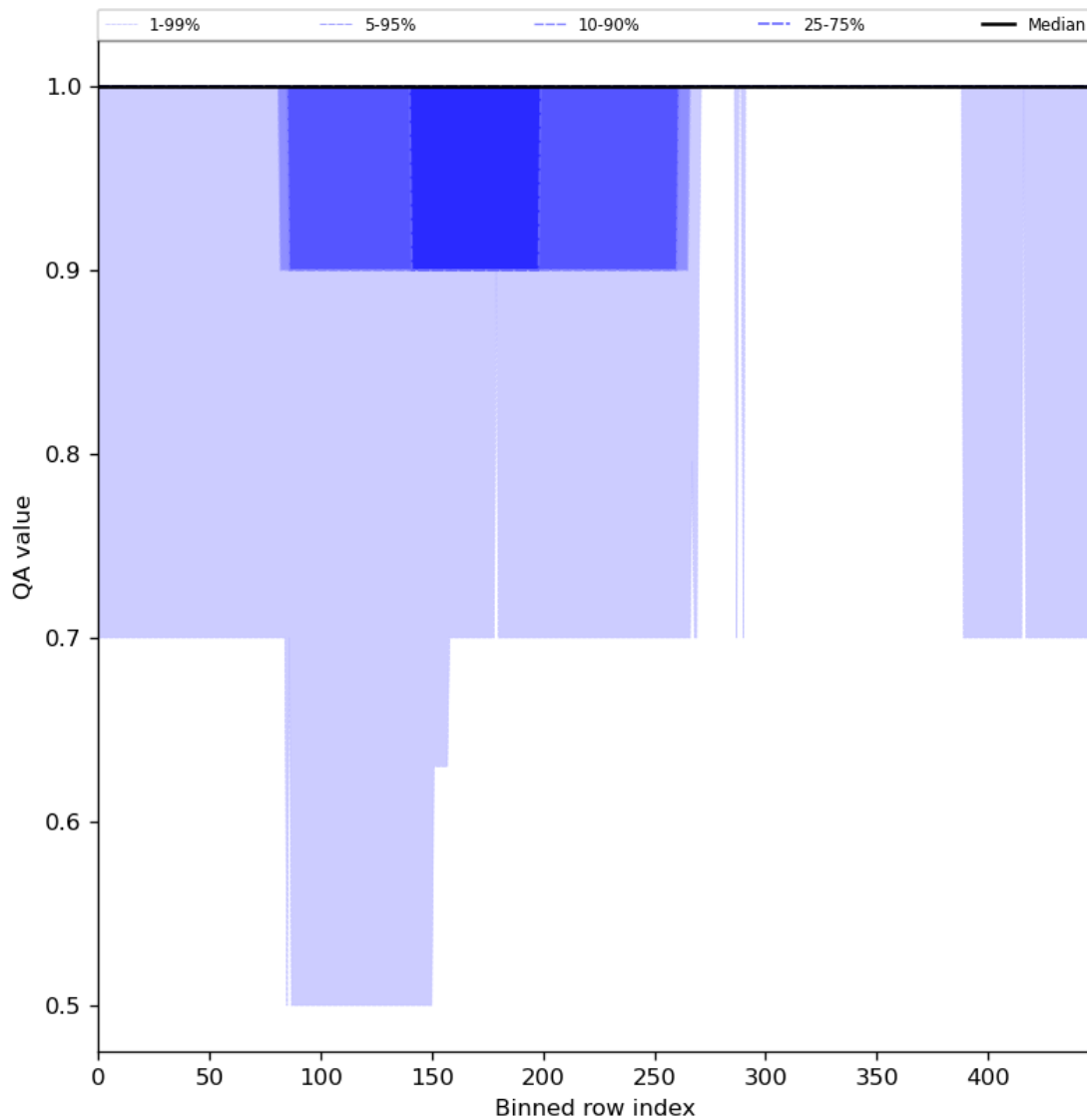
Figure 46: Along track statistics of “QA value” for 2024-07-24 to 2024-07-26
