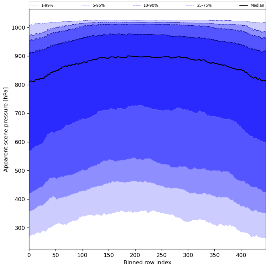
Figure 53: Along track statistics of “Apparent scene pressure” for 2024-07-24 to 2024-07-26
