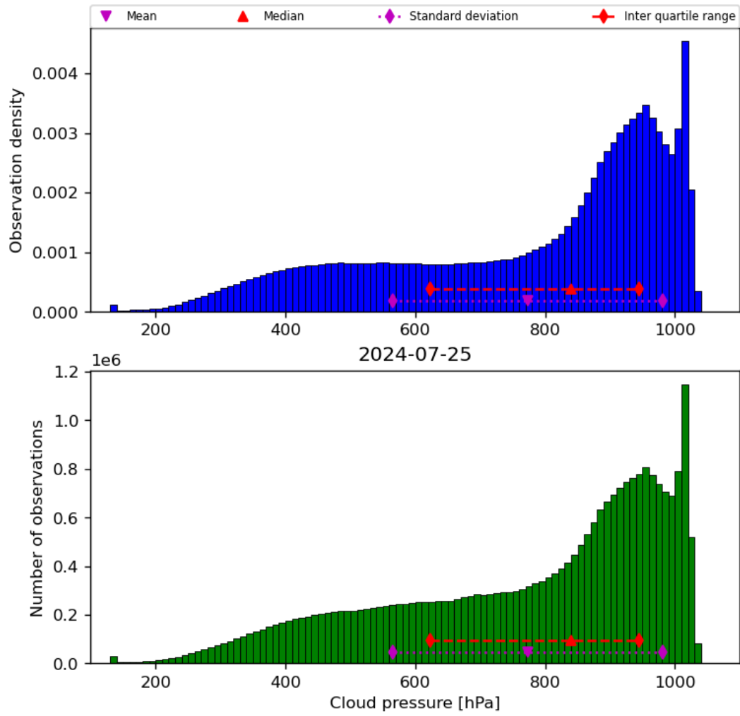
Figure 30: Histogram of “Cloud pressure” for 2024-07-24 to 2024-07-26
