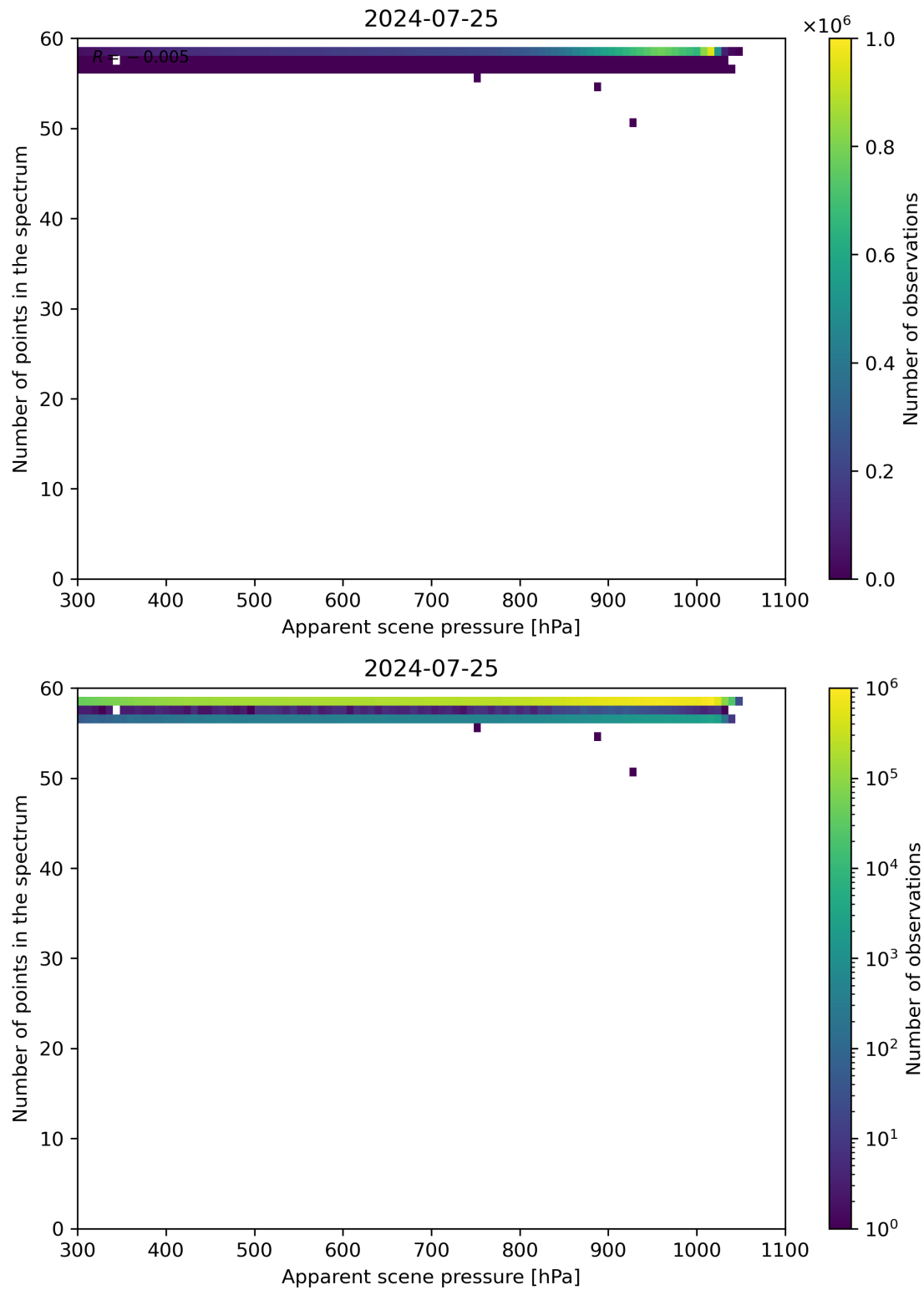
Figure 66: Scatter density plot of “Apparent scene pressure” against “Number of points in the spectrum” for 2024-07-24 to 2024-07-26.
