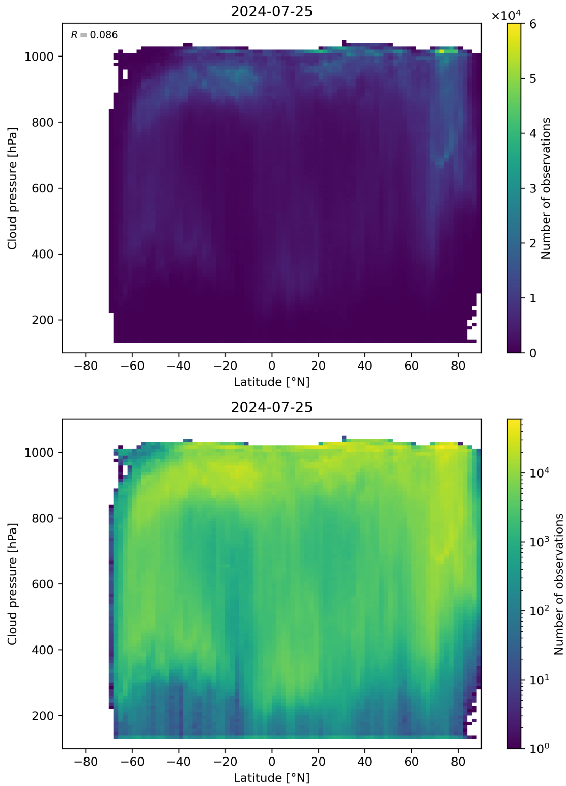
Figure 91: Scatter density plot of “Latitude” against “Cloud pressure” for 2024-07-24 to 2024-07-26.
