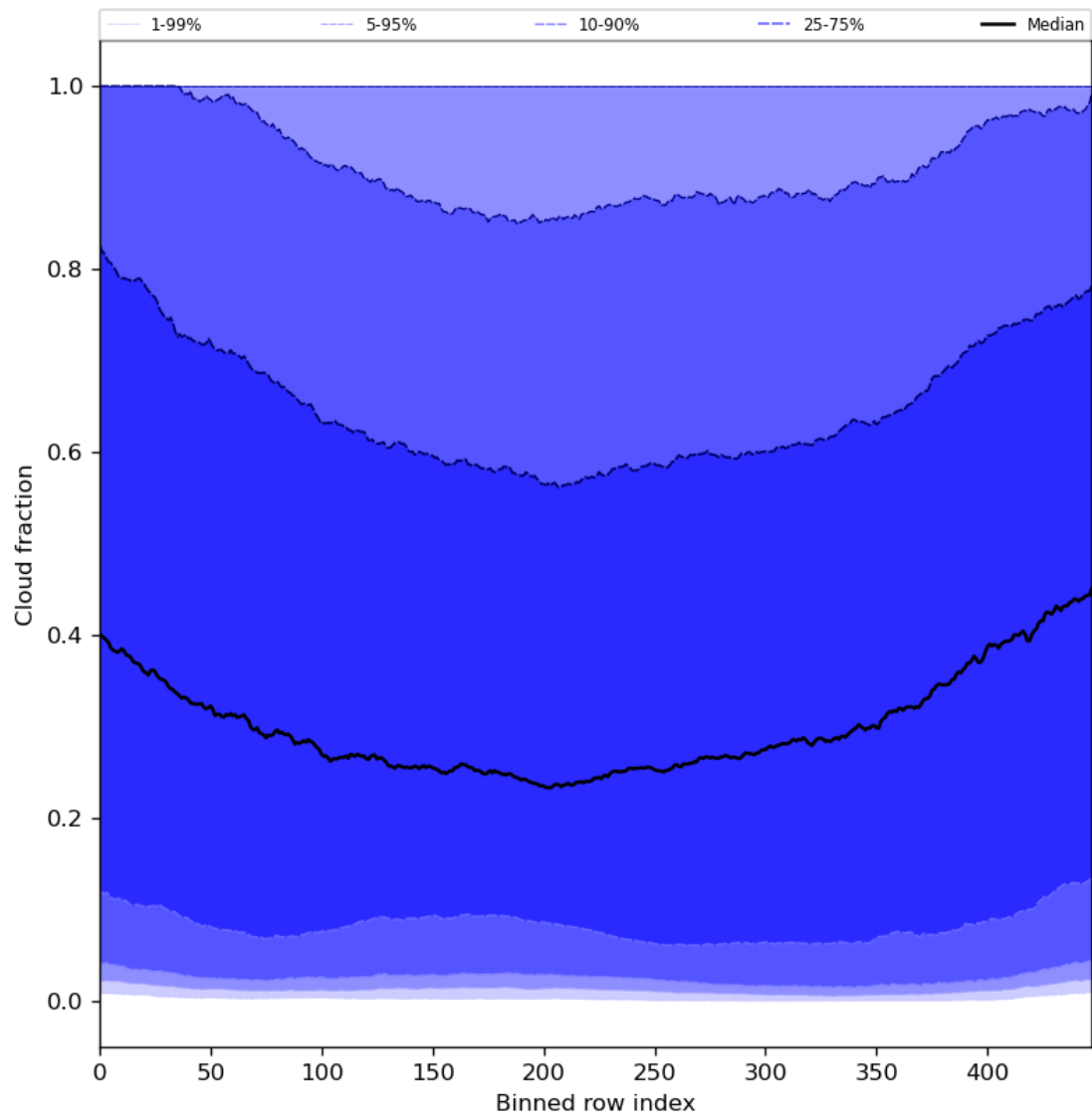
Figure 49: Along track statistics of “Cloud fraction” for 2024-07-24 to 2024-07-26
