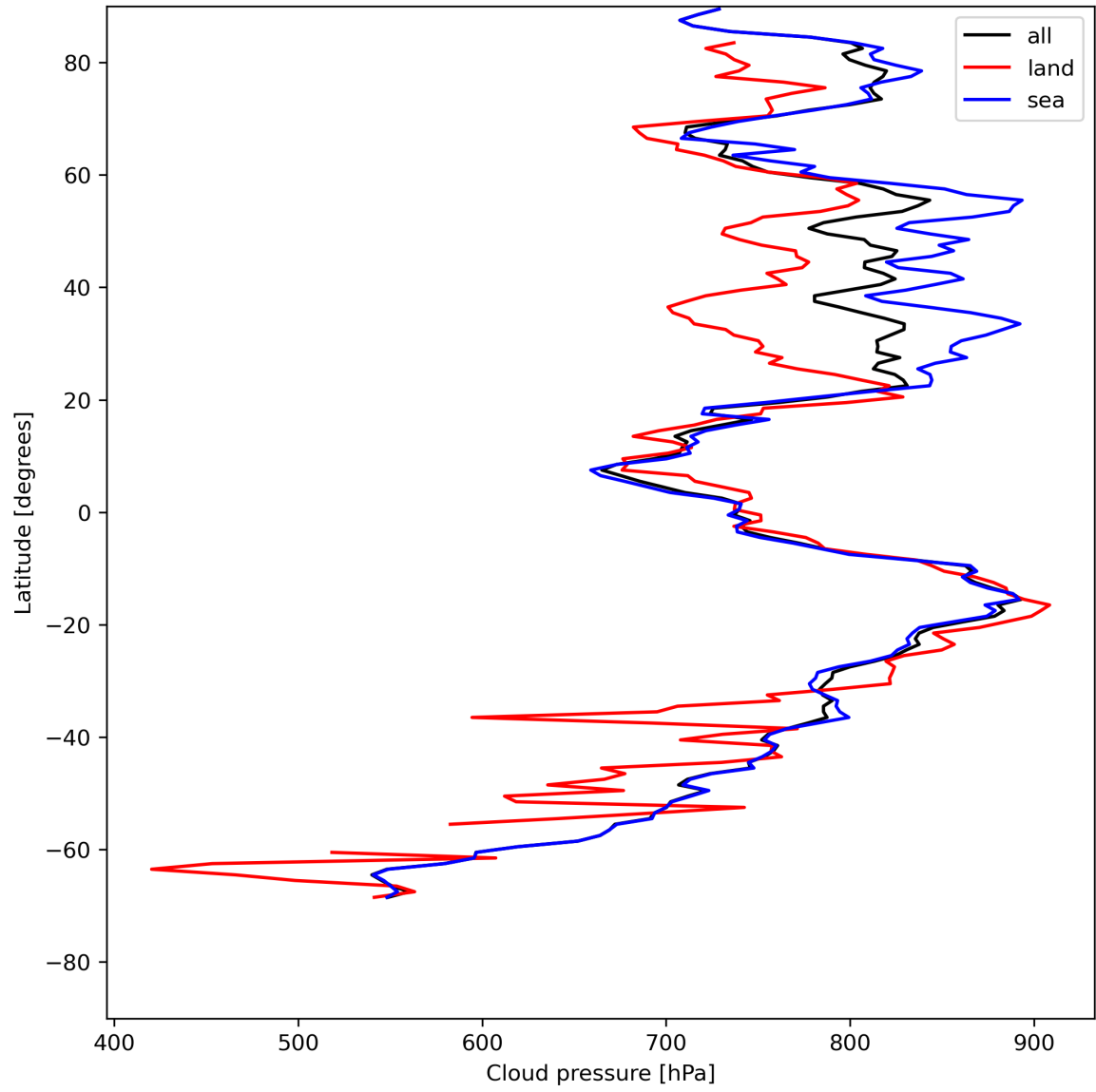
Figure 13: Zonal average of “Cloud pressure” for 2024-07-24 to 2024-07-26.
