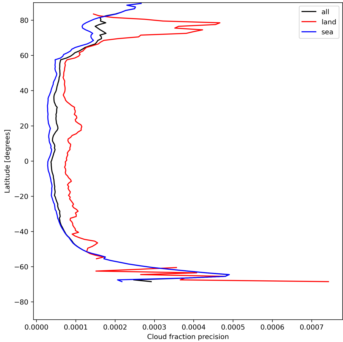
Figure 16: Zonal average of “Cloud fraction precision” for 2024-07-24 to 2024-07-26.
