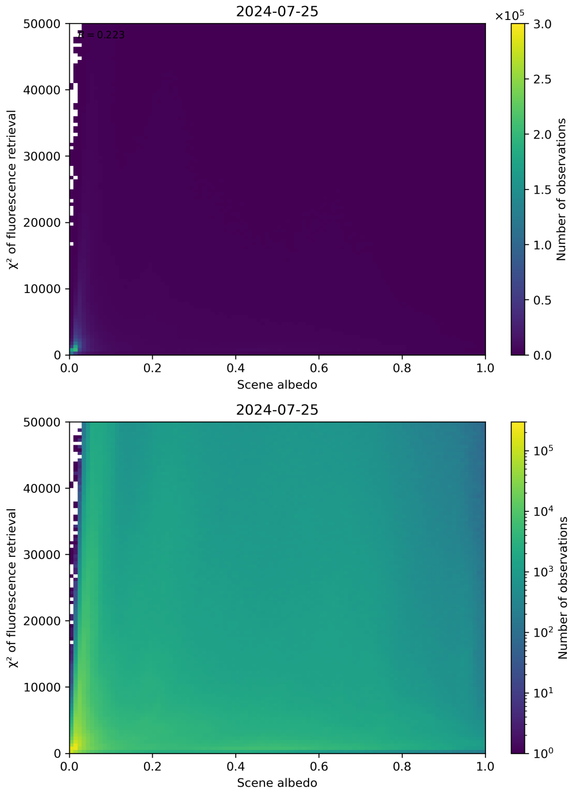
Figure 103: Scatter density plot of “Scene albedo” against “ \chi^2 of fluorescence retrieval” for 2024-07-24 to 2024-07-26.
