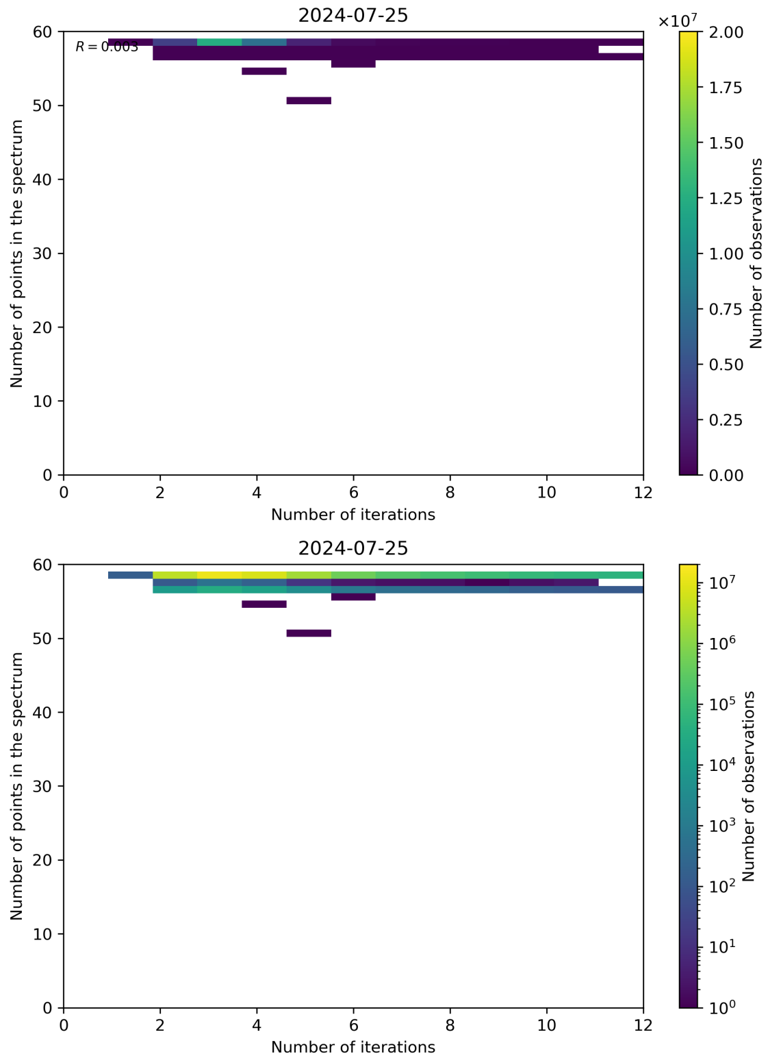
Figure 99: Scatter density plot of “Number of iterations” against “Number of points in the spectrum” for 2024-07-24 to 2024-07-26.
