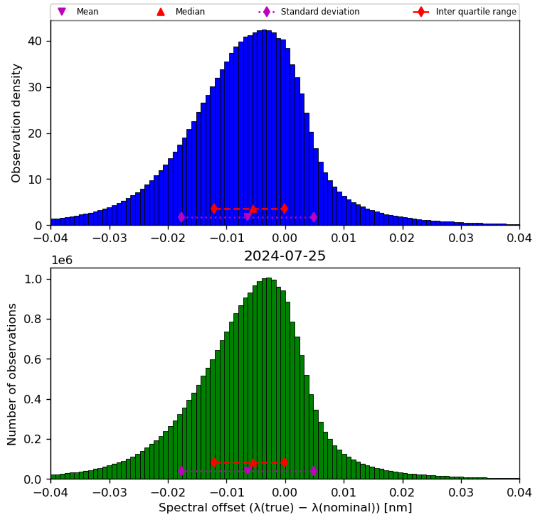
Figure 45: Histogram of “Spectral offset ( \lambda(\text{true}) - \lambda(\text{nominal}) )” for 2024-07-24 to 2024-07-26
