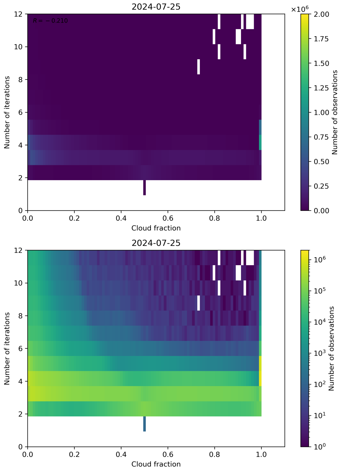
Figure 73: Scatter density plot of “Cloud fraction” against “Number of iterations” for 2024-07-24 to 2024-07-26.
