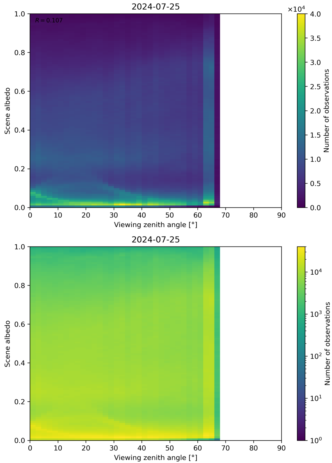
Figure 126: Scatter density plot of “Viewing zenith angle” against “Scene albedo” for 2024-07-24 to 2024-07-26.
