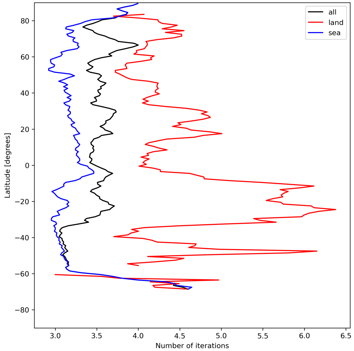
Figure 22: Zonal average of “Number of iterations” for 2024-07-24 to 2024-07-26.
