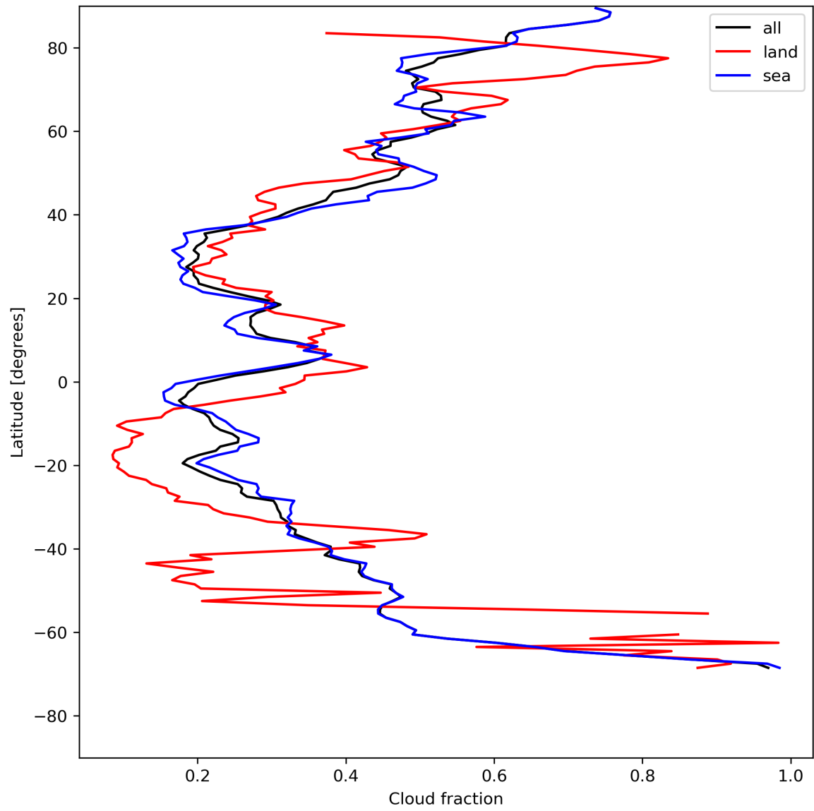
Figure 15: Zonal average of “Cloud fraction” for 2024-07-24 to 2024-07-26.
