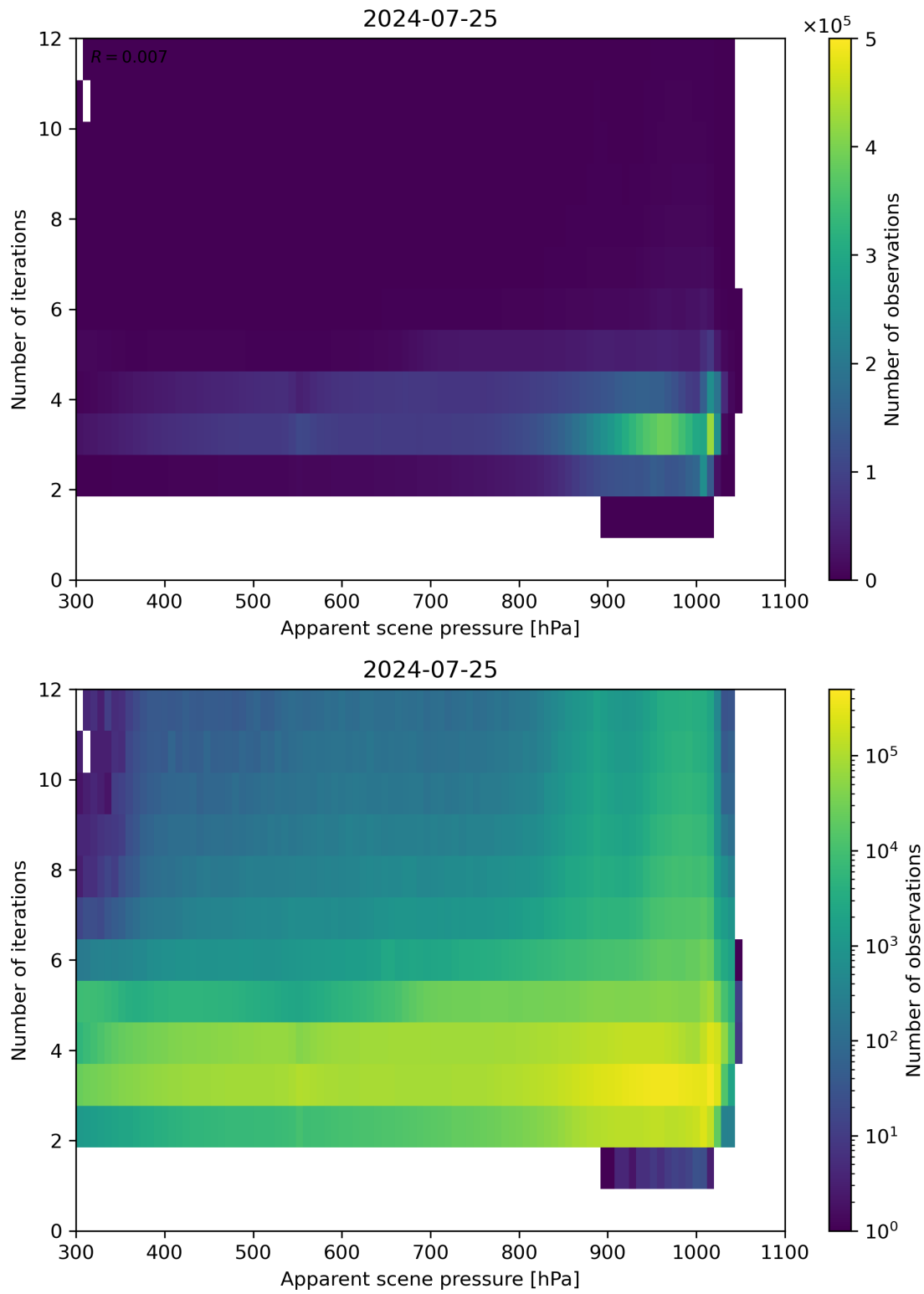
Figure 65: Scatter density plot of “Apparent scene pressure” against “Number of iterations” for 2024-07-24 to 2024-07-26.
