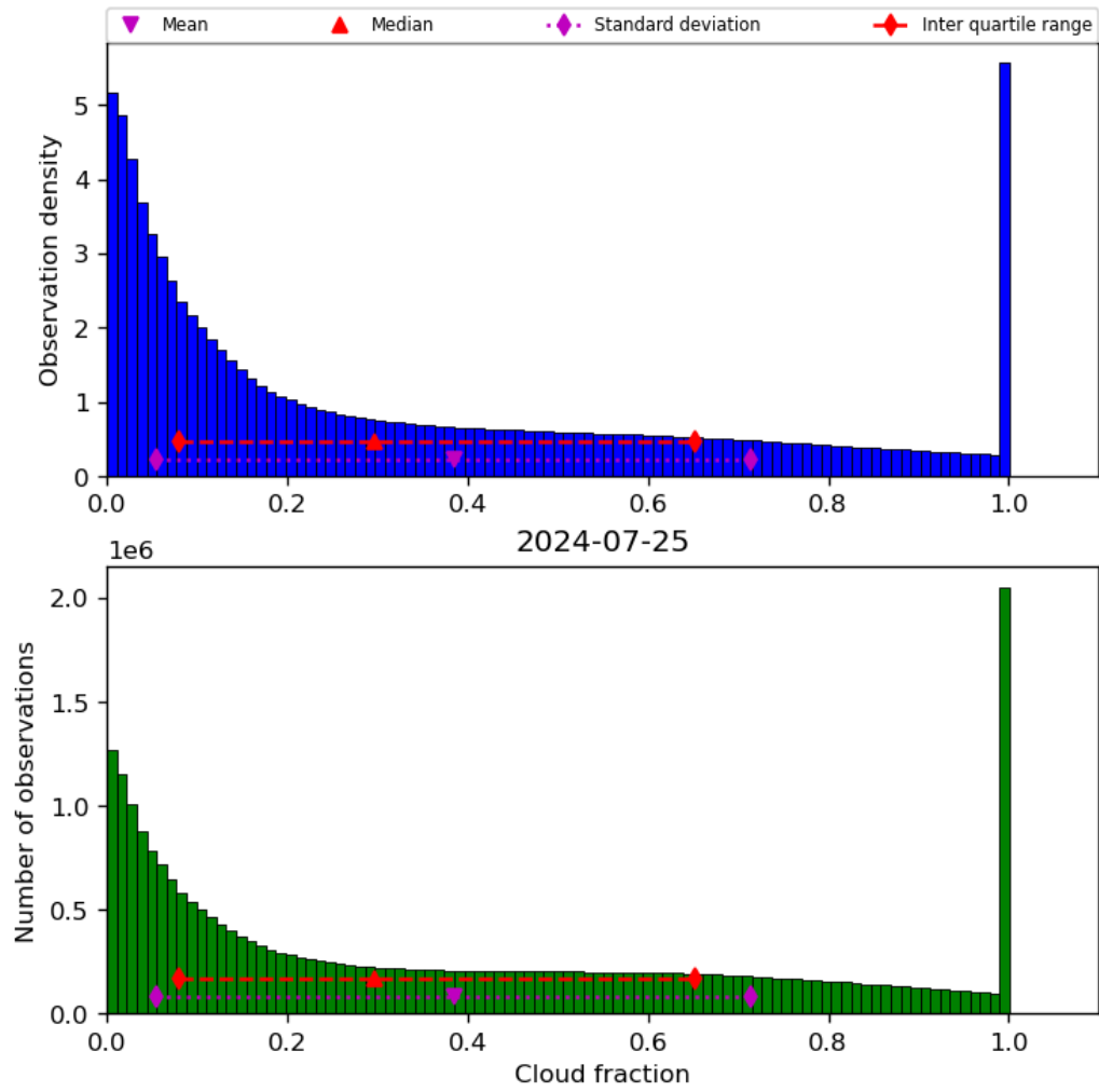
Figure 32: Histogram of “Cloud fraction” for 2024-07-24 to 2024-07-26
