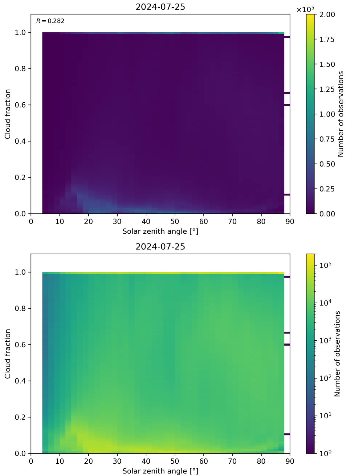
Figure 110: Scatter density plot of “Solar zenith angle” against “Cloud fraction” for 2024-07-24 to 2024-07-26.
