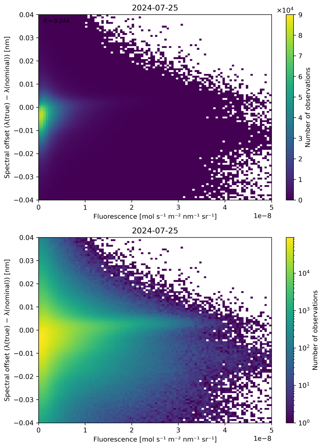
Figure 87: Scatter density plot of “Fluorescence” against “Spectral offset ( \lambda(\text{true}) - \lambda(\text{nominal}) )” for 2024-07-24 to 2024-07-26.
