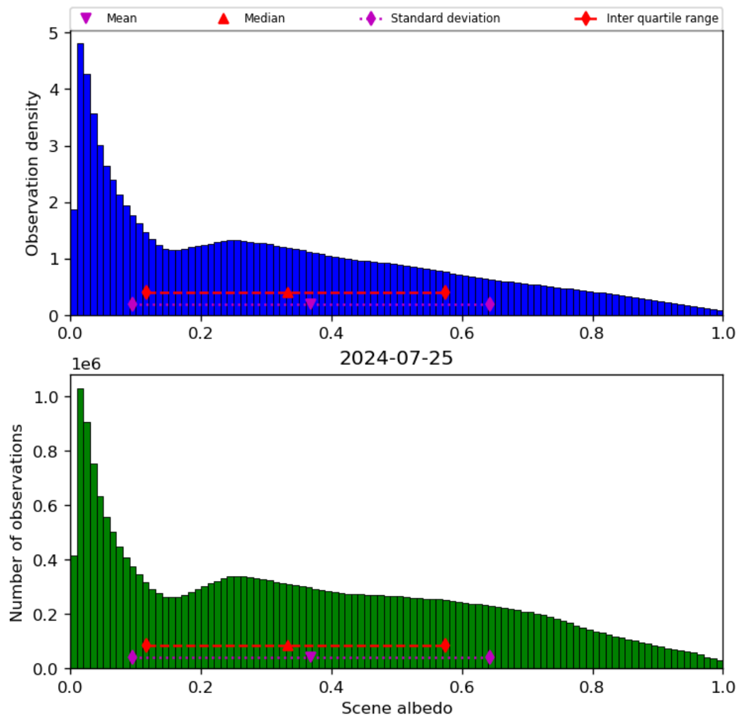
Figure 34: Histogram of “Scene albedo” for 2024-07-24 to 2024-07-26
