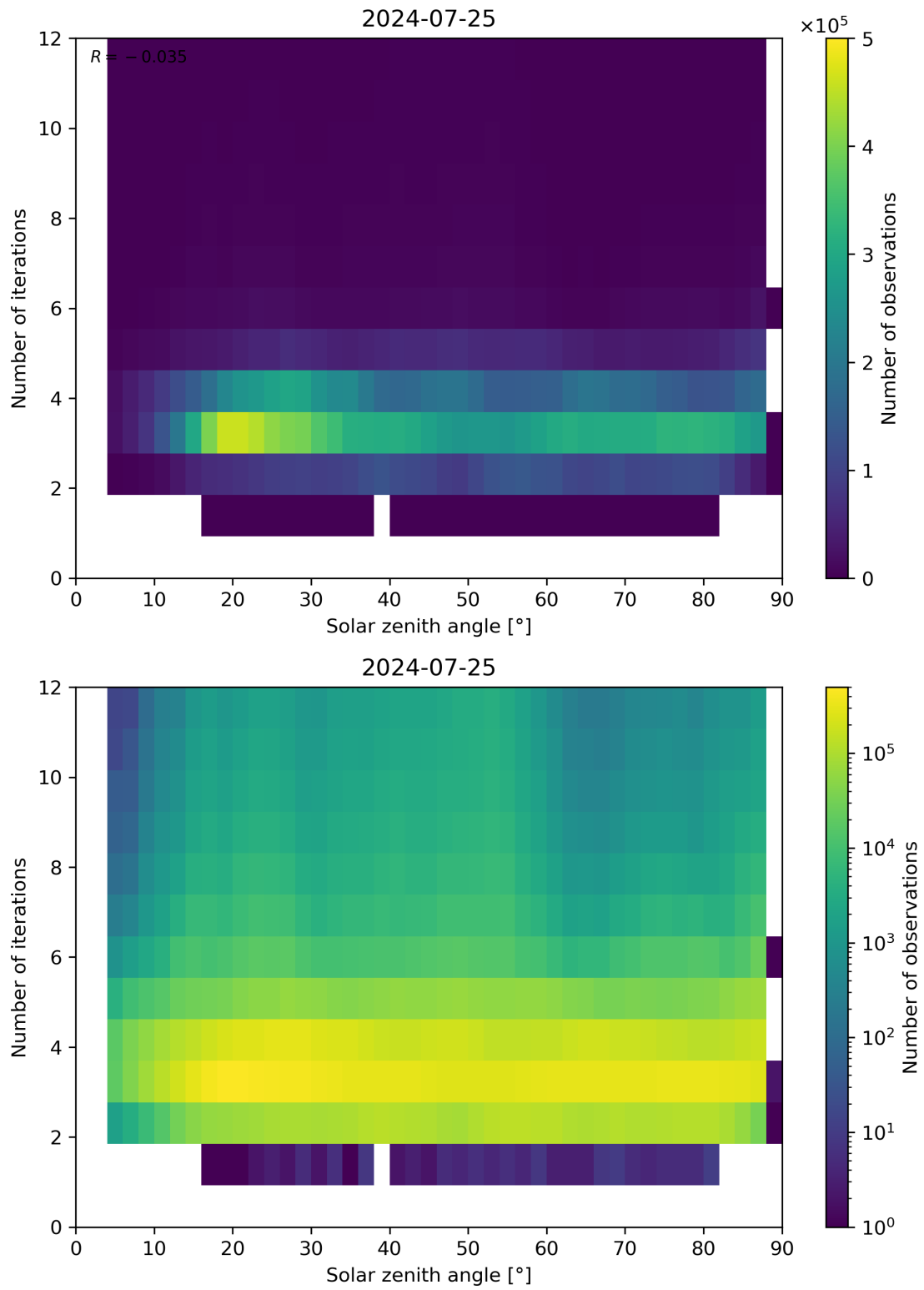
Figure 114: Scatter density plot of “Solar zenith angle” against “Number of iterations” for 2024-07-24 to 2024-07-26.
