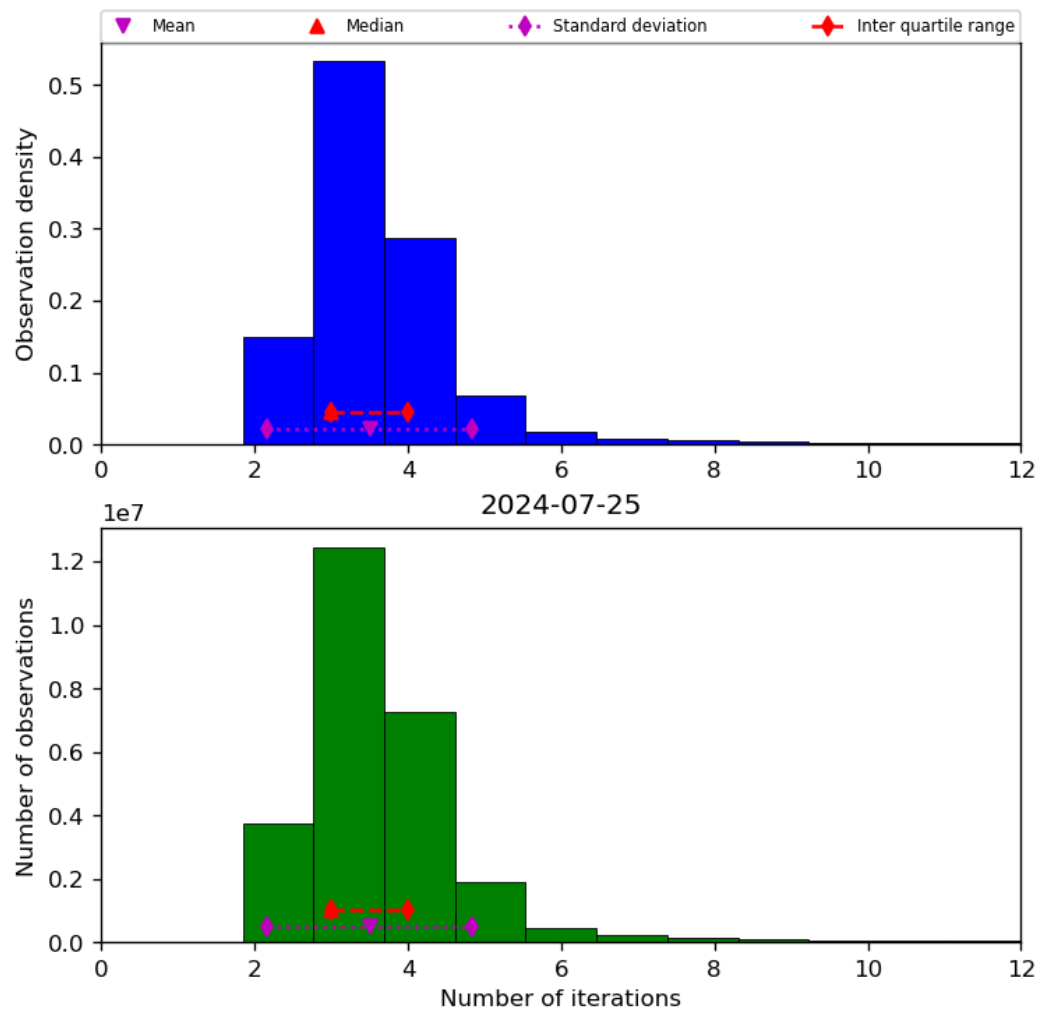
Figure 39: Histogram of “Number of iterations” for 2024-07-24 to 2024-07-26
