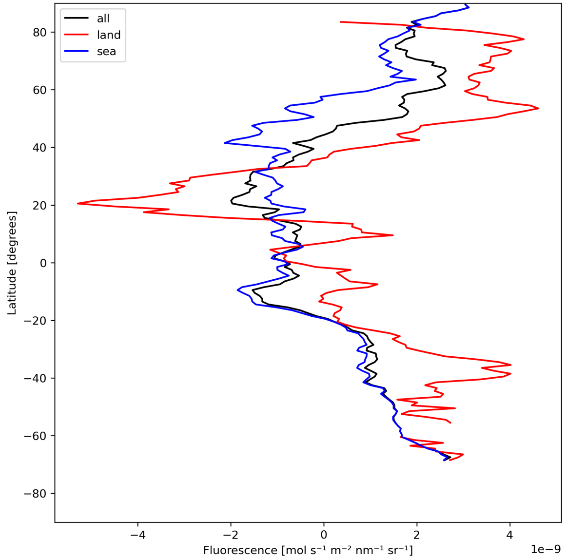
Figure 23: Zonal average of “Fluorescence” for 2024-07-24 to 2024-07-26.
