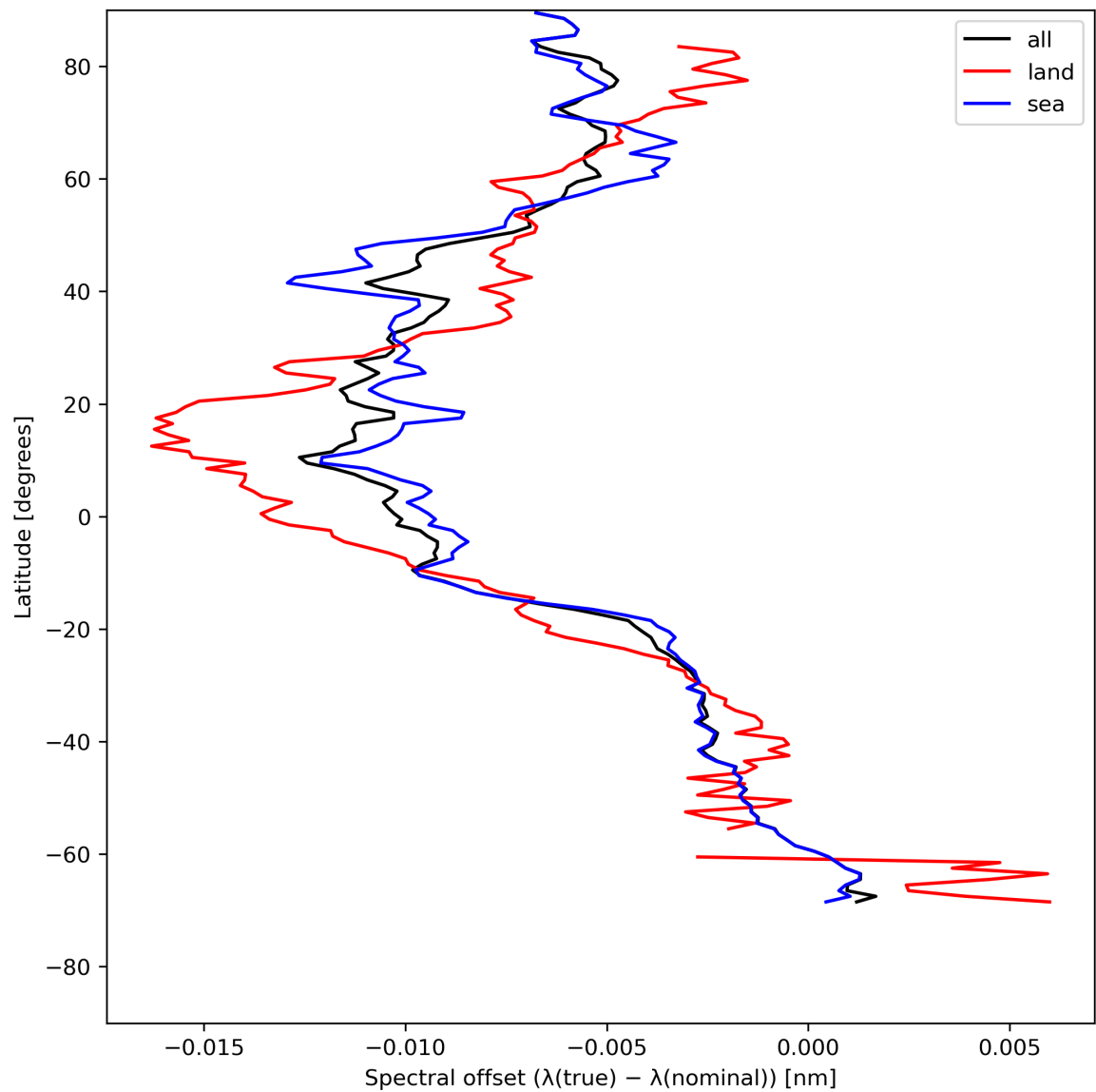
Figure 28: Zonal average of “Spectral offset ( \lambda(\text{true}) - \lambda(\text{nominal}) )” for 2024-07-24 to 2024-07-26.
