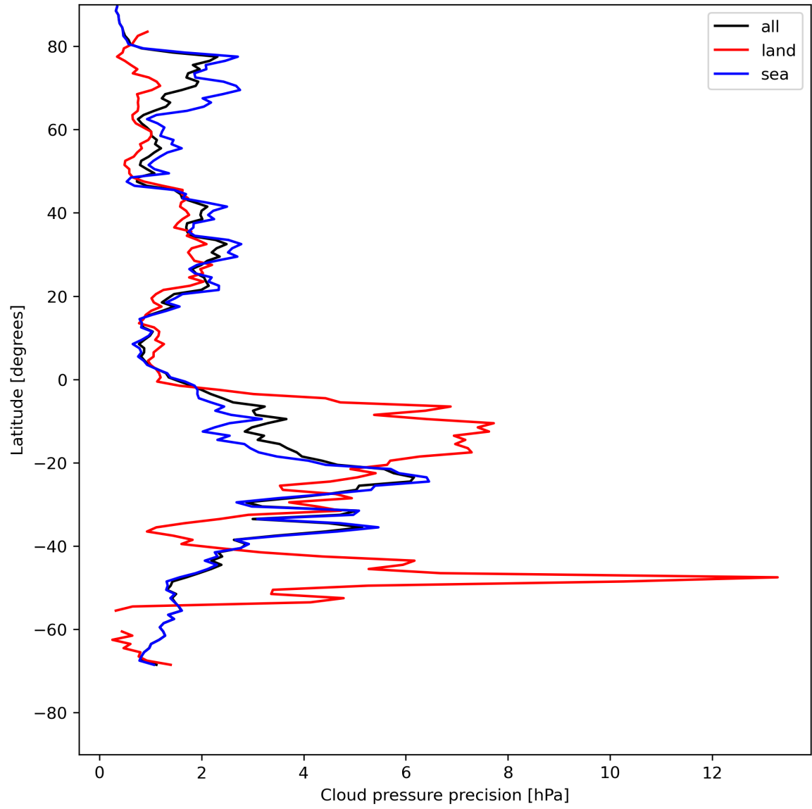
Figure 14: Zonal average of “Cloud pressure precision” for 2024-07-24 to 2024-07-26.
