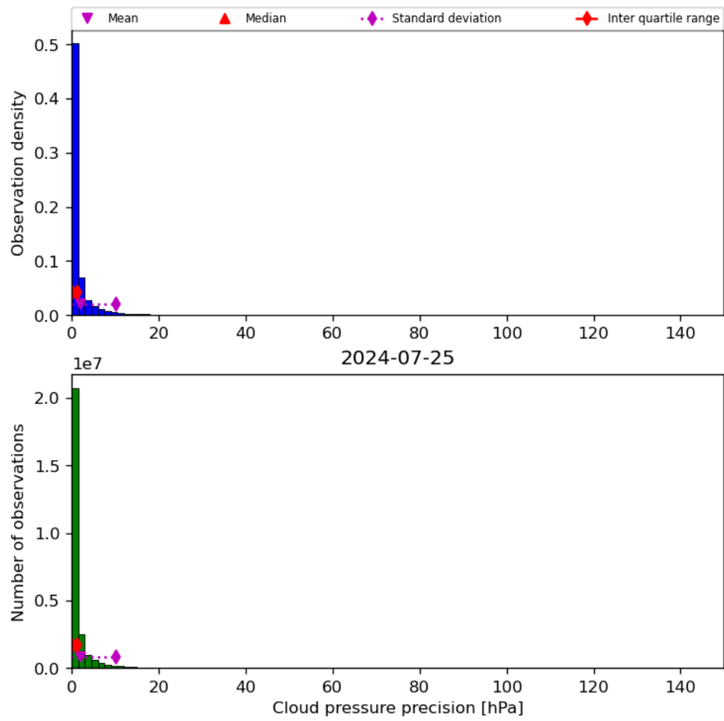
Figure 31: Histogram of “Cloud pressure precision” for 2024-07-24 to 2024-07-26
