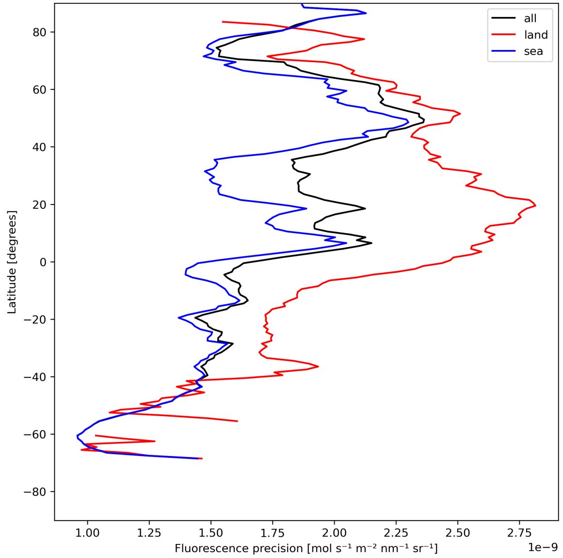
Figure 24: Zonal average of “Fluorescence precision” for 2024-07-24 to 2024-07-26.
