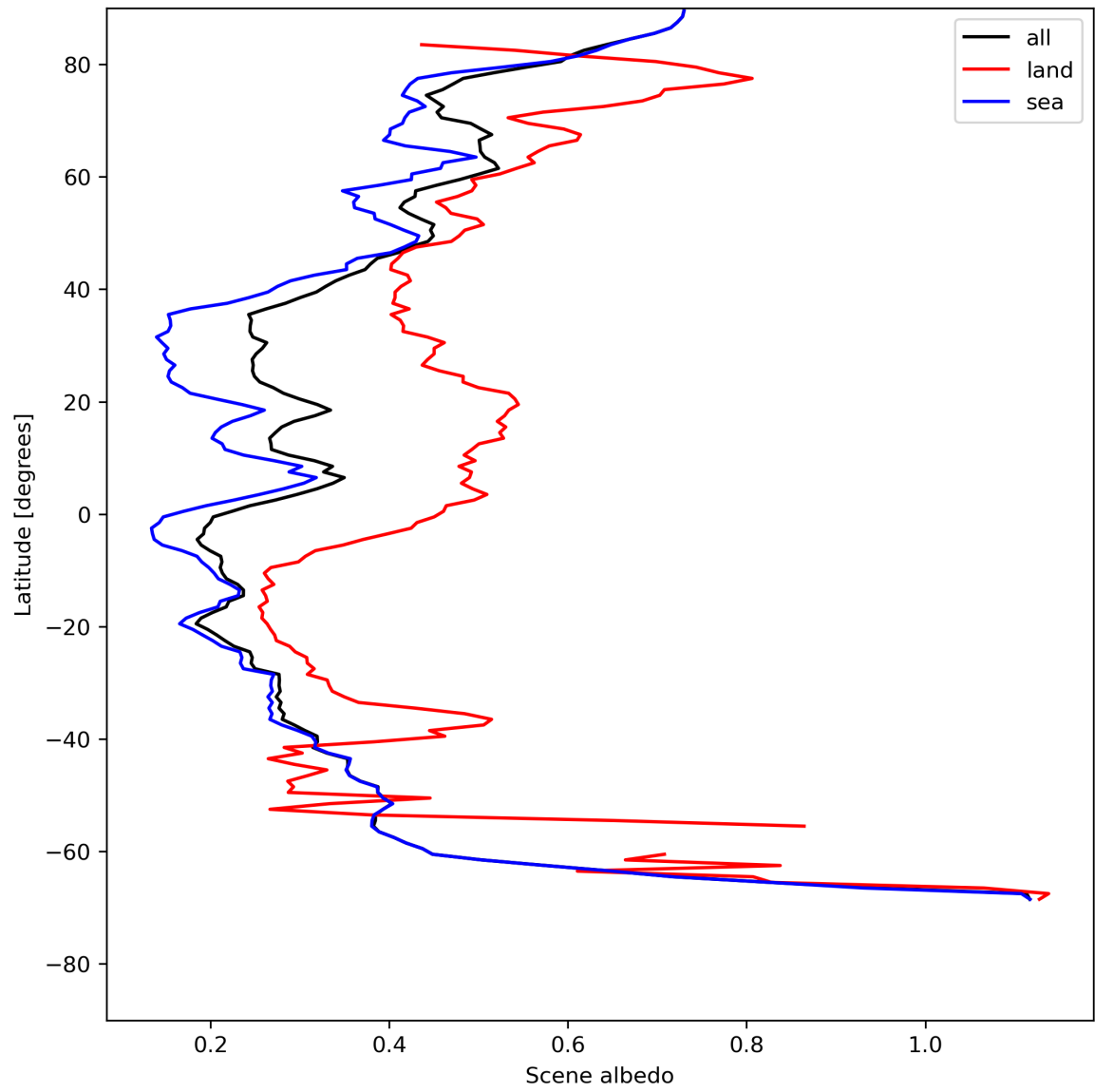
Figure 17: Zonal average of “Scene albedo” for 2024-07-24 to 2024-07-26.
