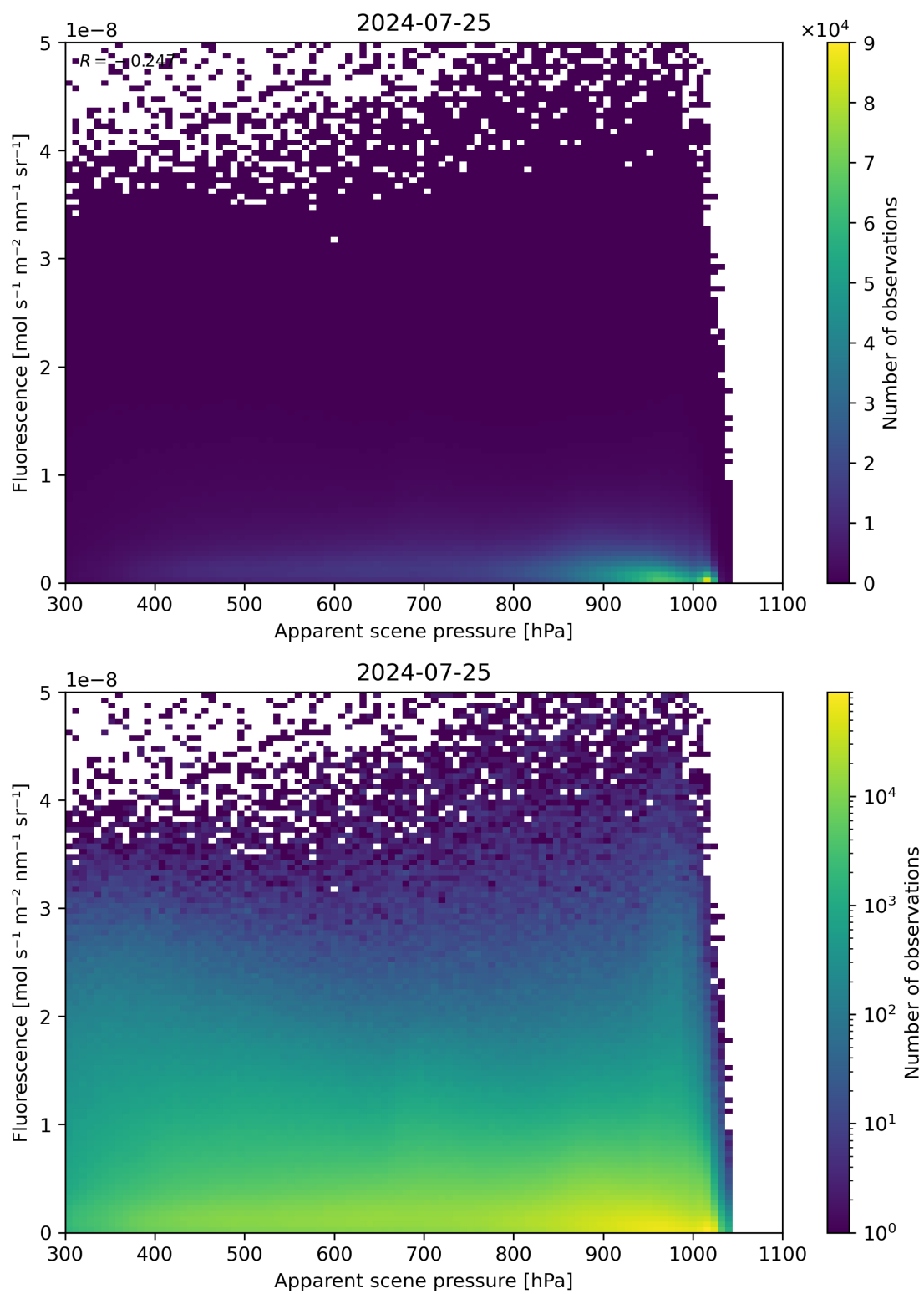
Figure 64: Scatter density plot of “Apparent scene pressure” against “Fluorescence” for 2024-07-24 to 2024-07-26.
