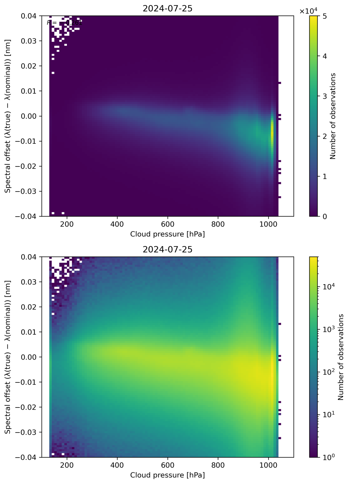
Figure 84: Scatter density plot of “Cloud pressure” against “Spectral offset ( \lambda(\text{true}) - \lambda(\text{nominal}) )” for 2024-07-24 to 2024-07-26.
