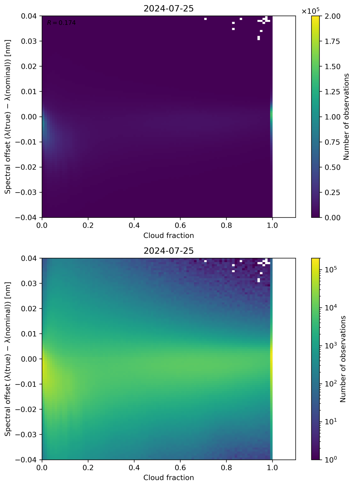
Figure 76: Scatter density plot of “Cloud fraction” against “Spectral offset ( \lambda(\text{true}) - \lambda(\text{nominal}) )” for 2024-07-24 to 2024-07-26.
