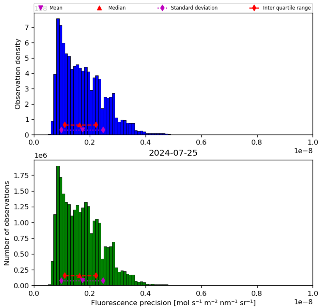
Figure 41: Histogram of “Fluorescence precision” for 2024-07-24 to 2024-07-26
