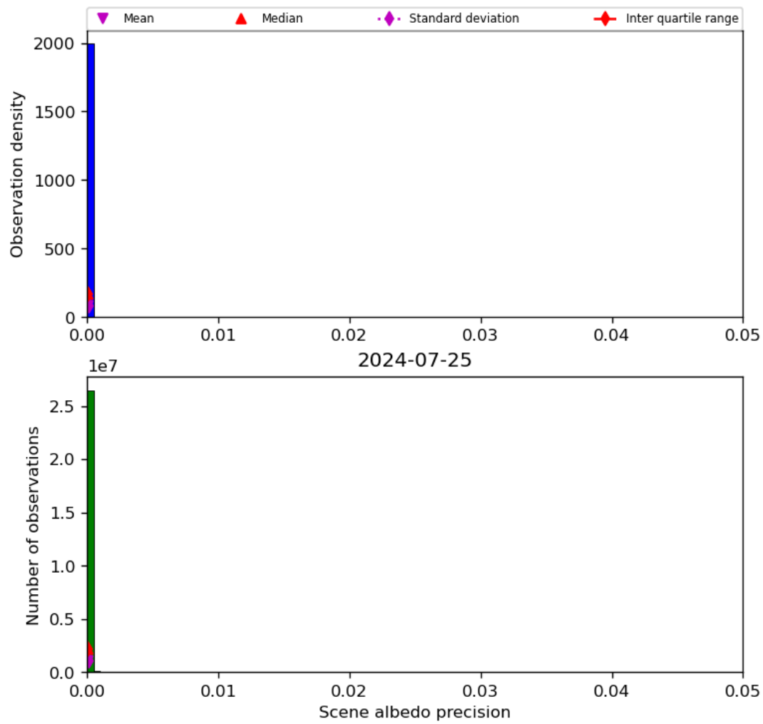
Figure 35: Histogram of “Scene albedo precision” for 2024-07-24 to 2024-07-26
