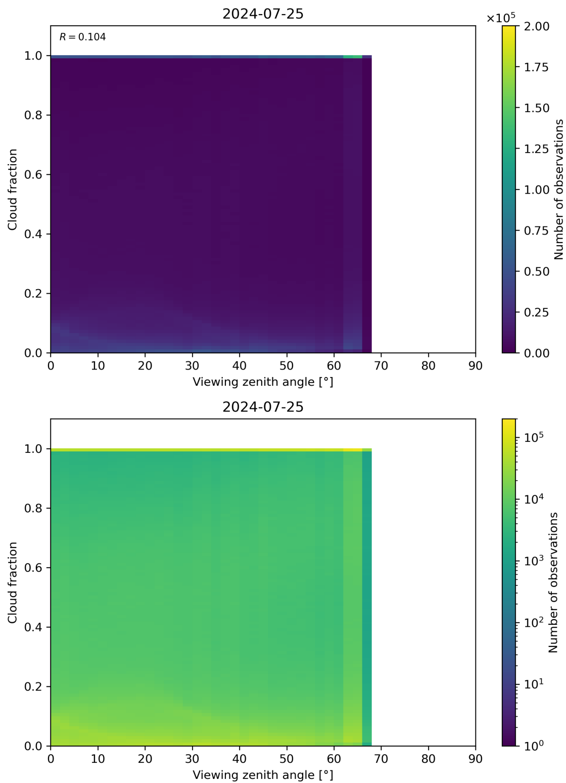
Figure 120: Scatter density plot of “Viewing zenith angle” against “Cloud fraction” for 2024-07-24 to 2024-07-26.
