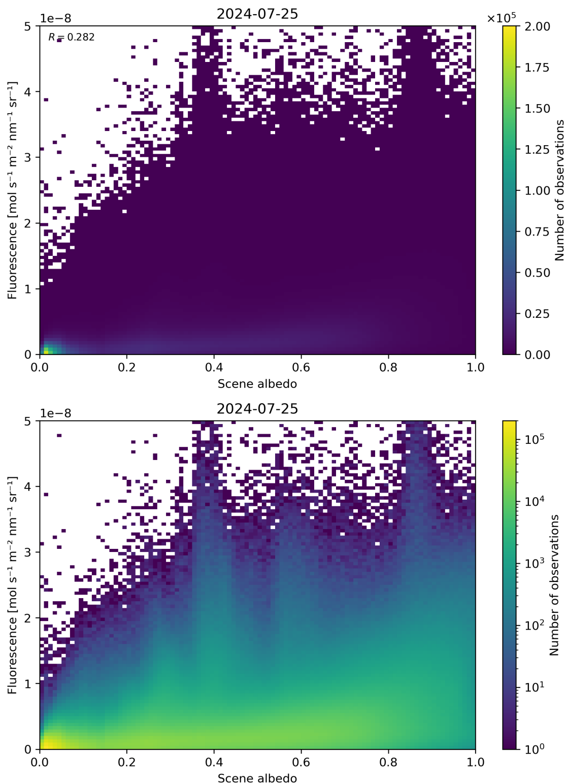
Figure 104: Scatter density plot of “Scene albedo” against “Fluorescence” for 2024-07-24 to 2024-07-26.
