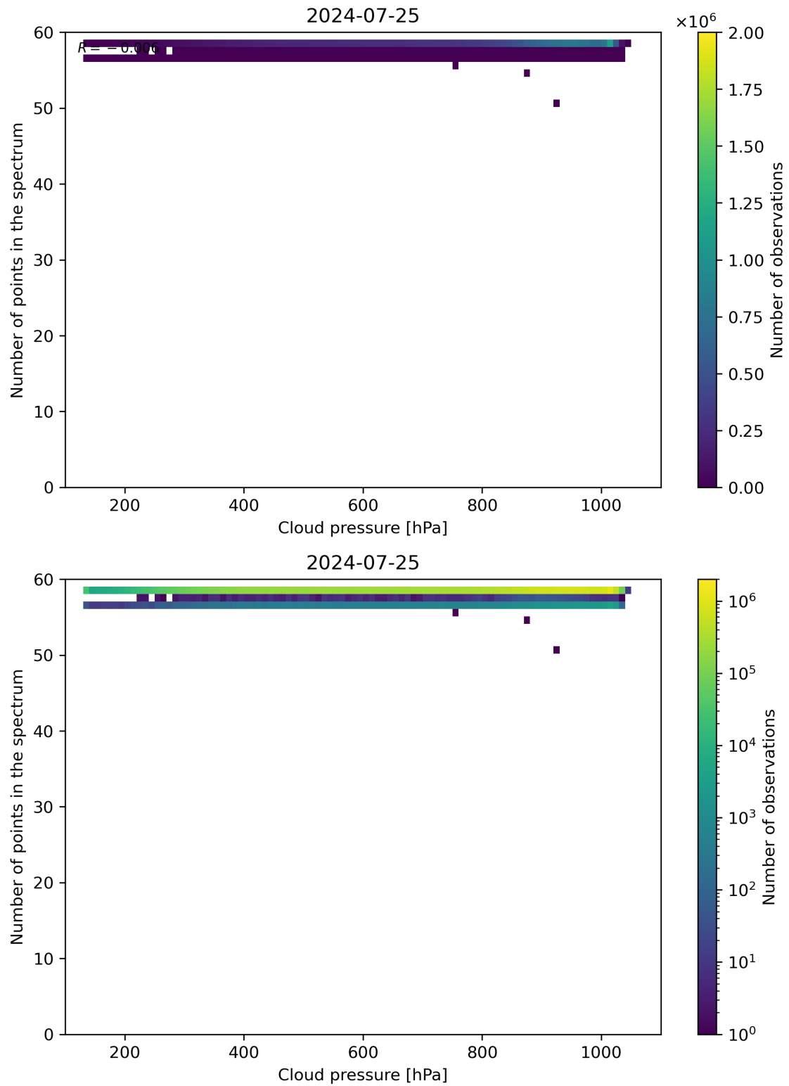
Figure 82: Scatter density plot of “Cloud pressure” against “Number of points in the spectrum” for 2024-07-24 to 2024-07-26.
