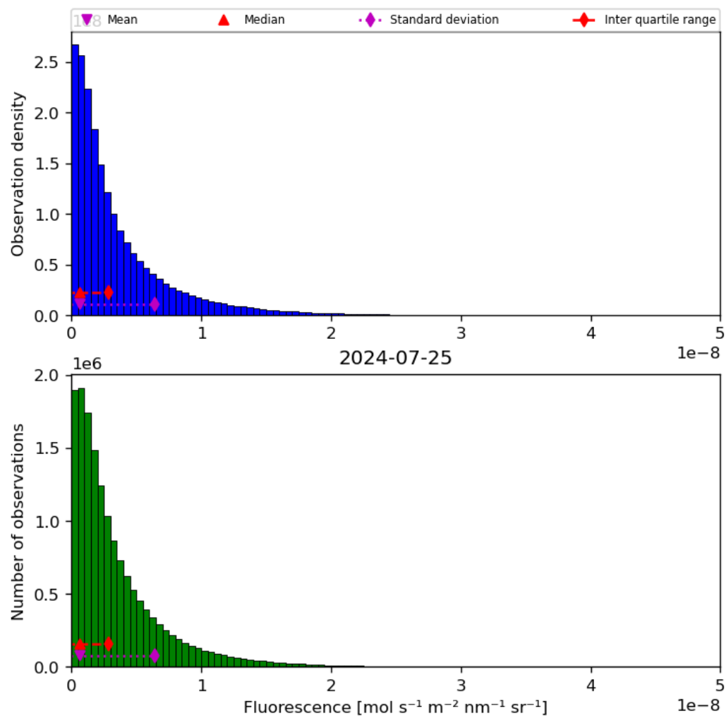
Figure 40: Histogram of “Fluorescence” for 2024-07-24 to 2024-07-26
