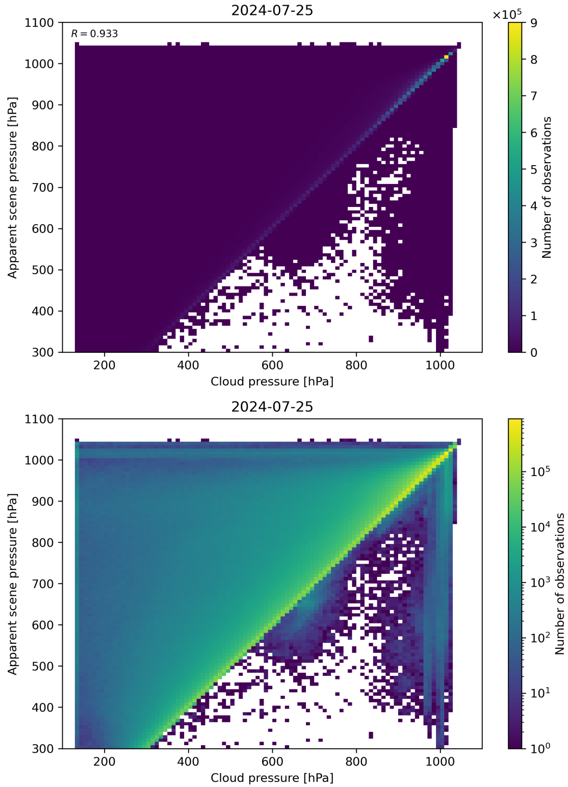
Figure 77: Scatter density plot of “Cloud pressure” against “Apparent scene pressure” for 2024-07-24 to 2024-07-26.
