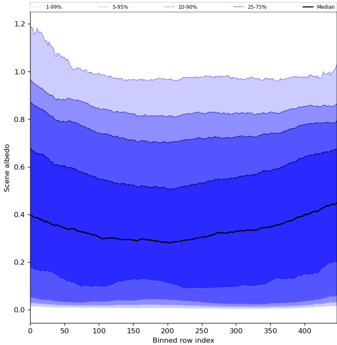
Figure 51: Along track statistics of “Scene albedo” for 2024-07-24 to 2024-07-26
