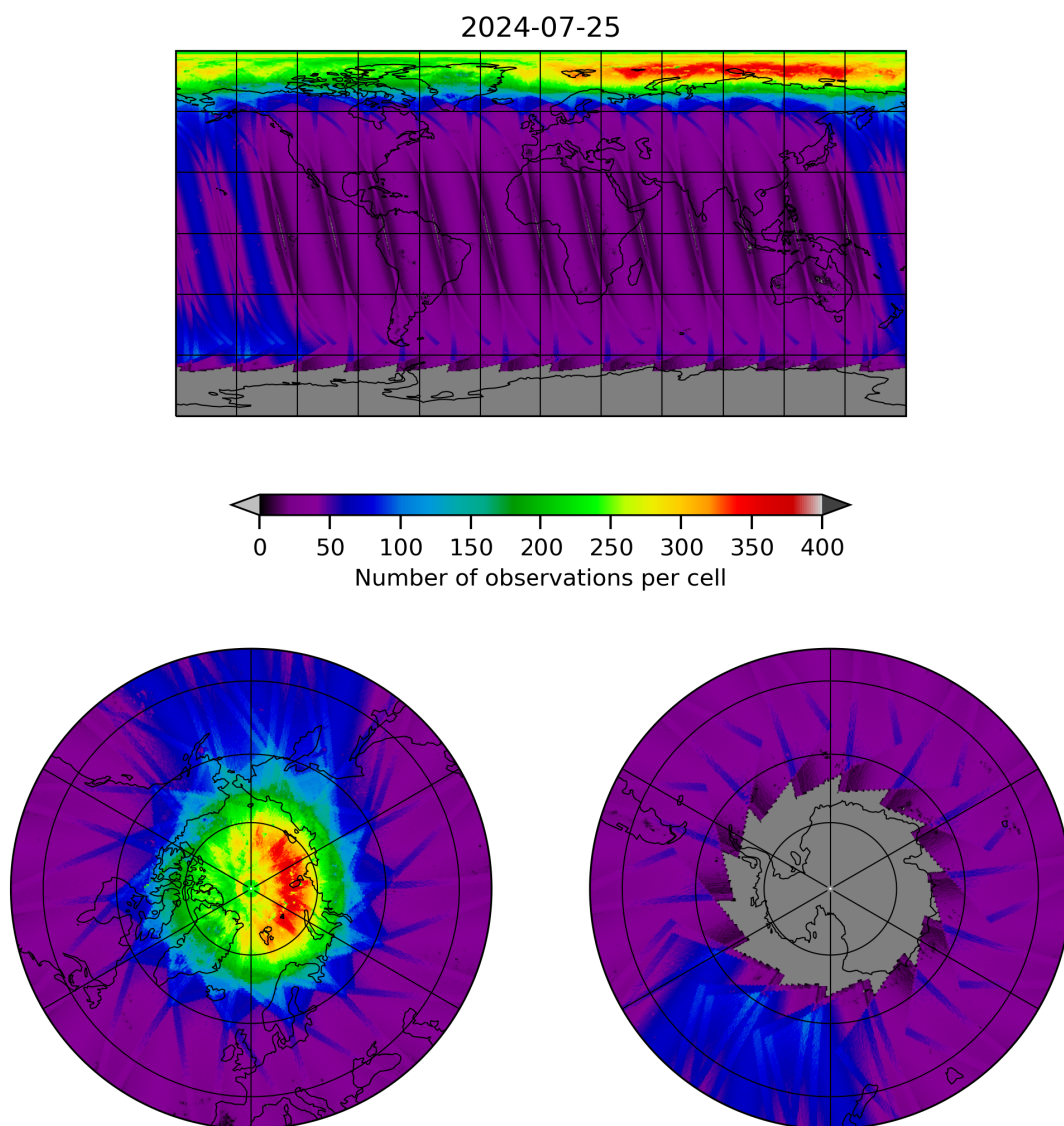
Figure 11: Map of the number of observations for 2024-07-24 to 2024-07-26
