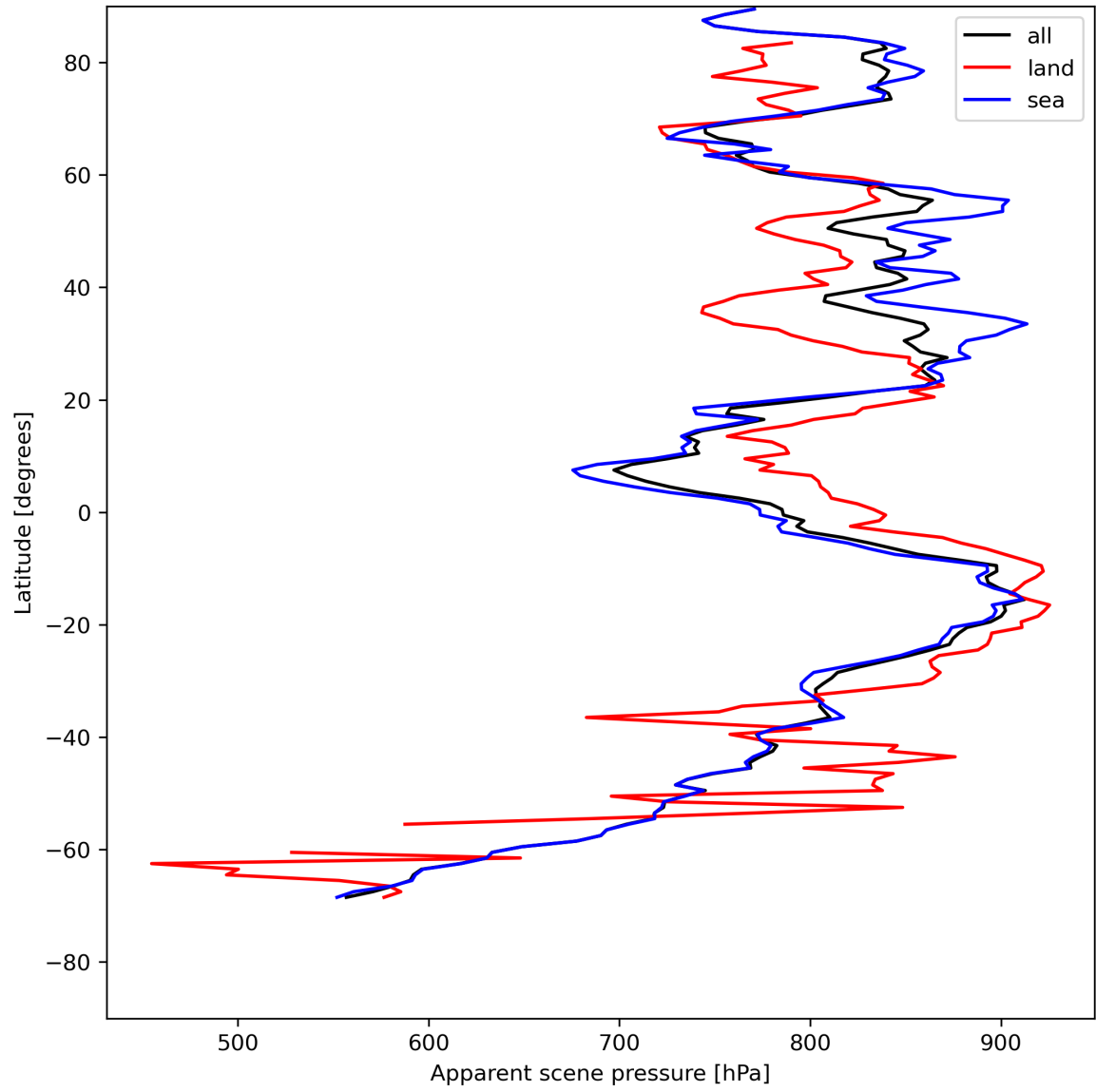
Figure 19: Zonal average of “Apparent scene pressure” for 2024-07-24 to 2024-07-26.
