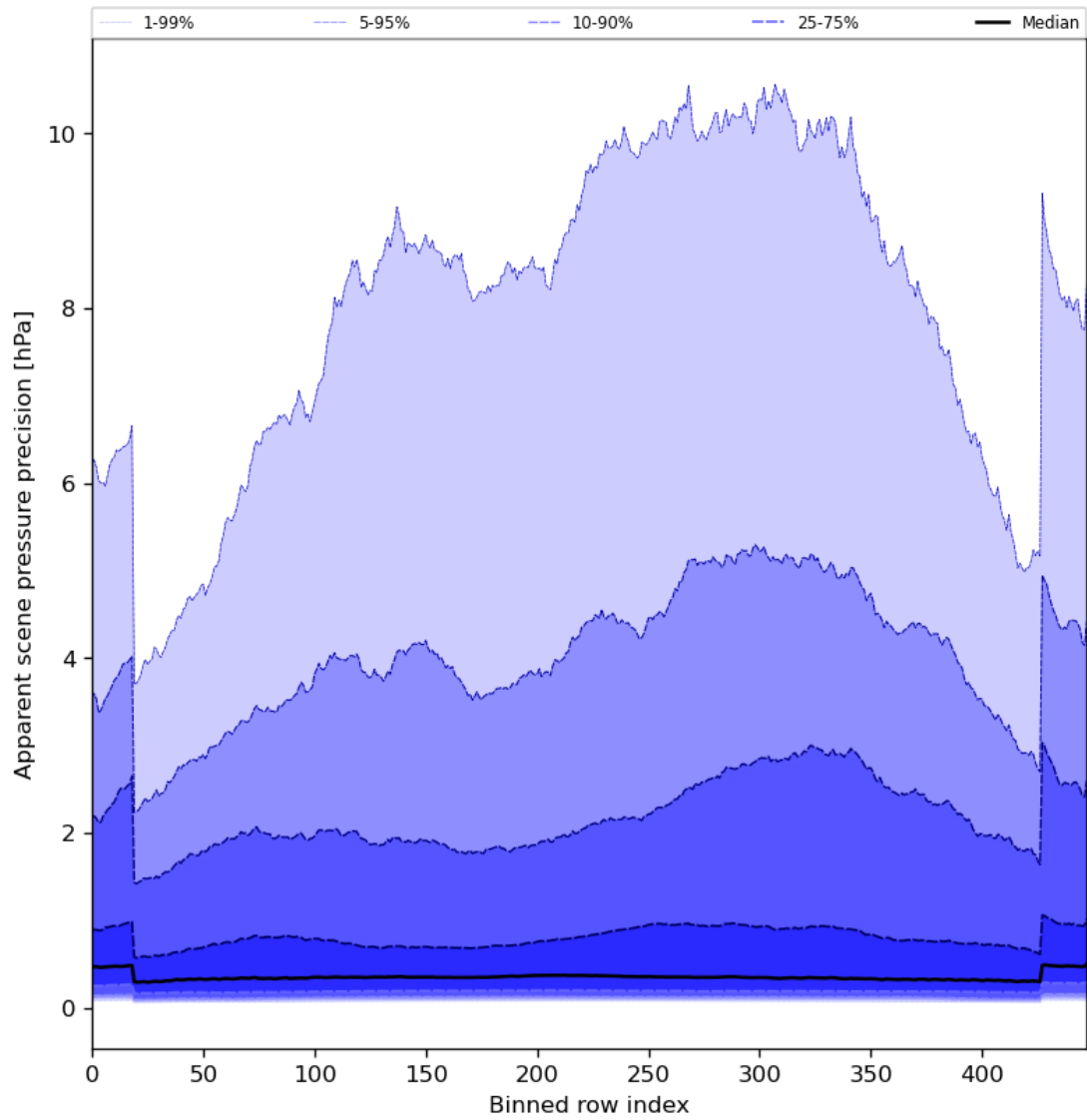
Figure 54: Along track statistics of “Apparent scene pressure precision” for 2024-07-24 to 2024-07-26
