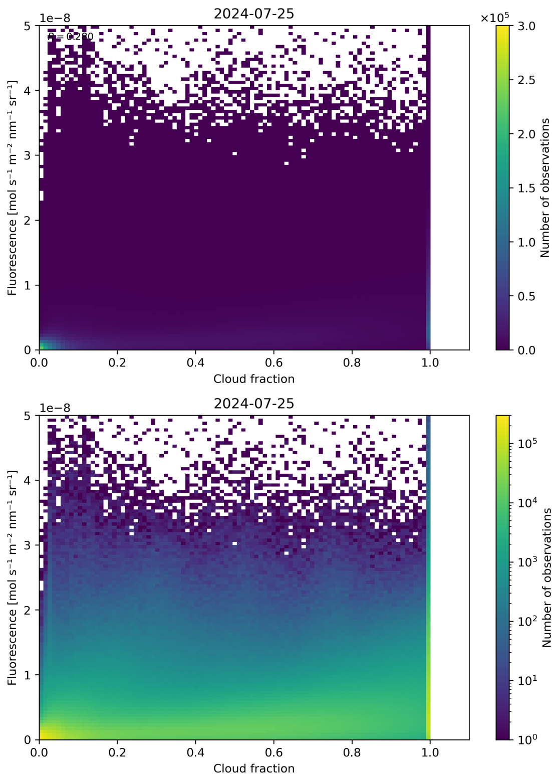
Figure 72: Scatter density plot of “Cloud fraction” against “Fluorescence” for 2024-07-24 to 2024-07-26.
