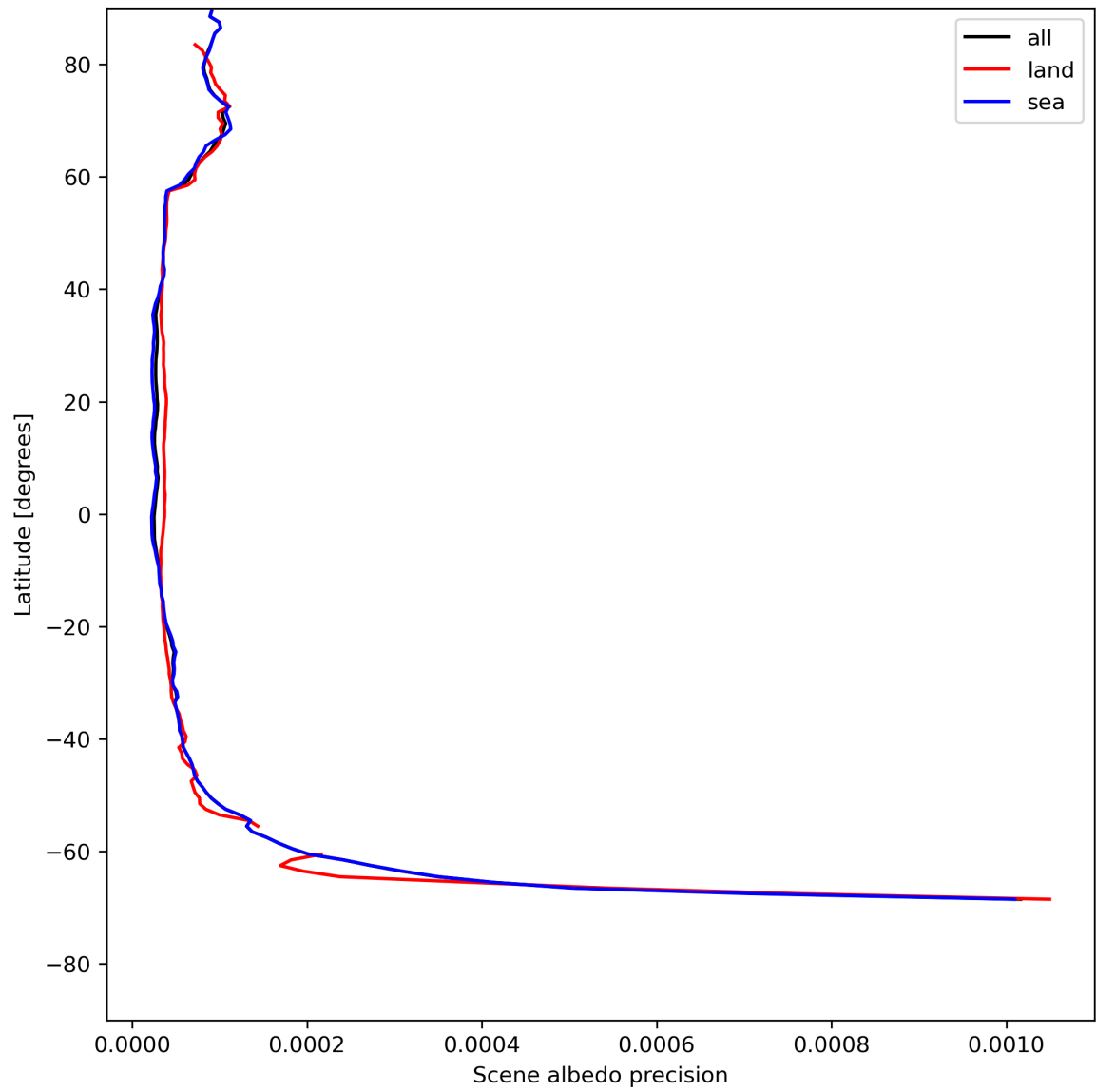
Figure 18: Zonal average of “Scene albedo precision” for 2024-07-24 to 2024-07-26.
