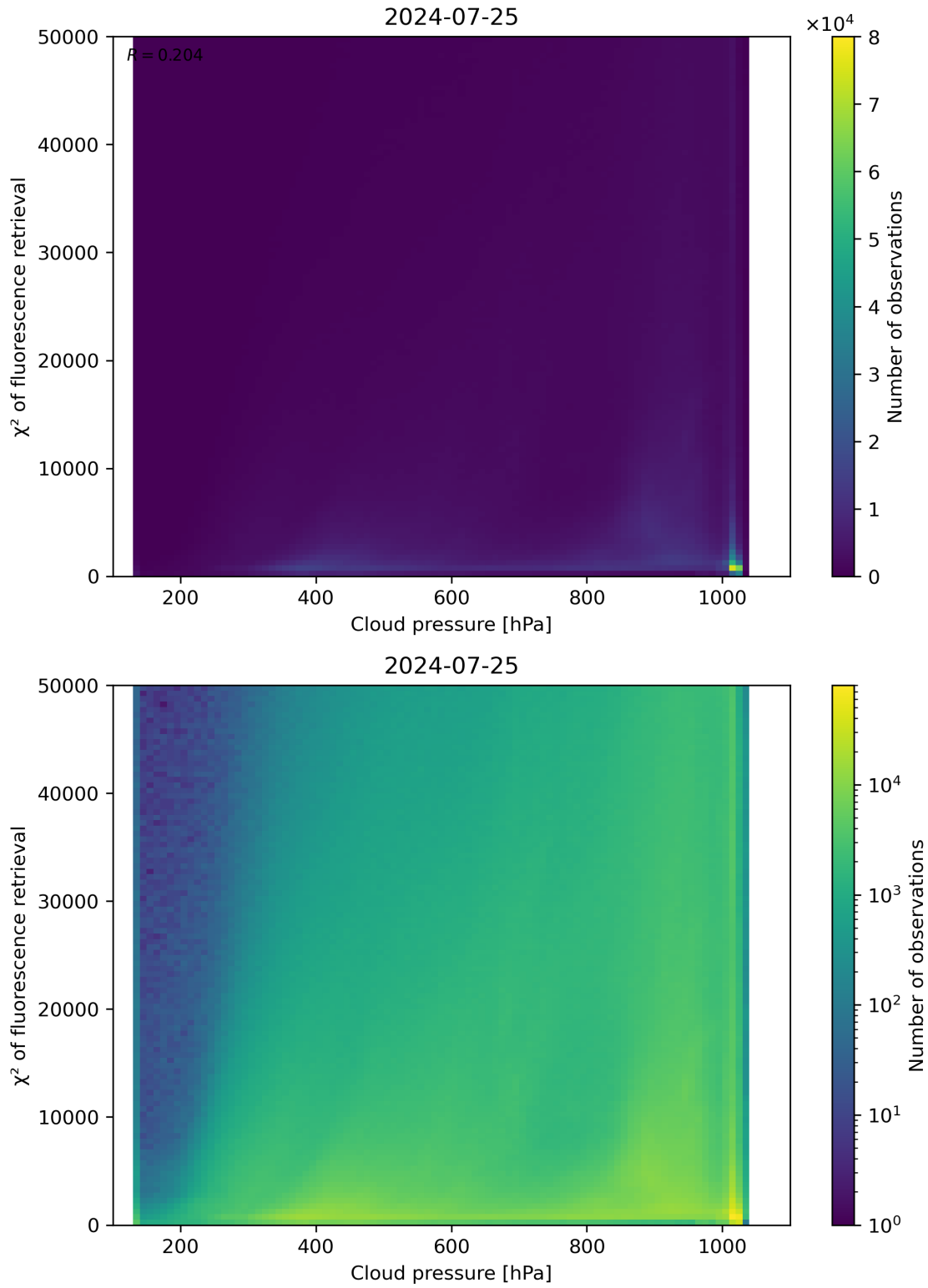
Figure 78: Scatter density plot of “Cloud pressure” against “ \chi^2 of fluorescence retrieval” for 2024-07-24 to 2024-07-26.
