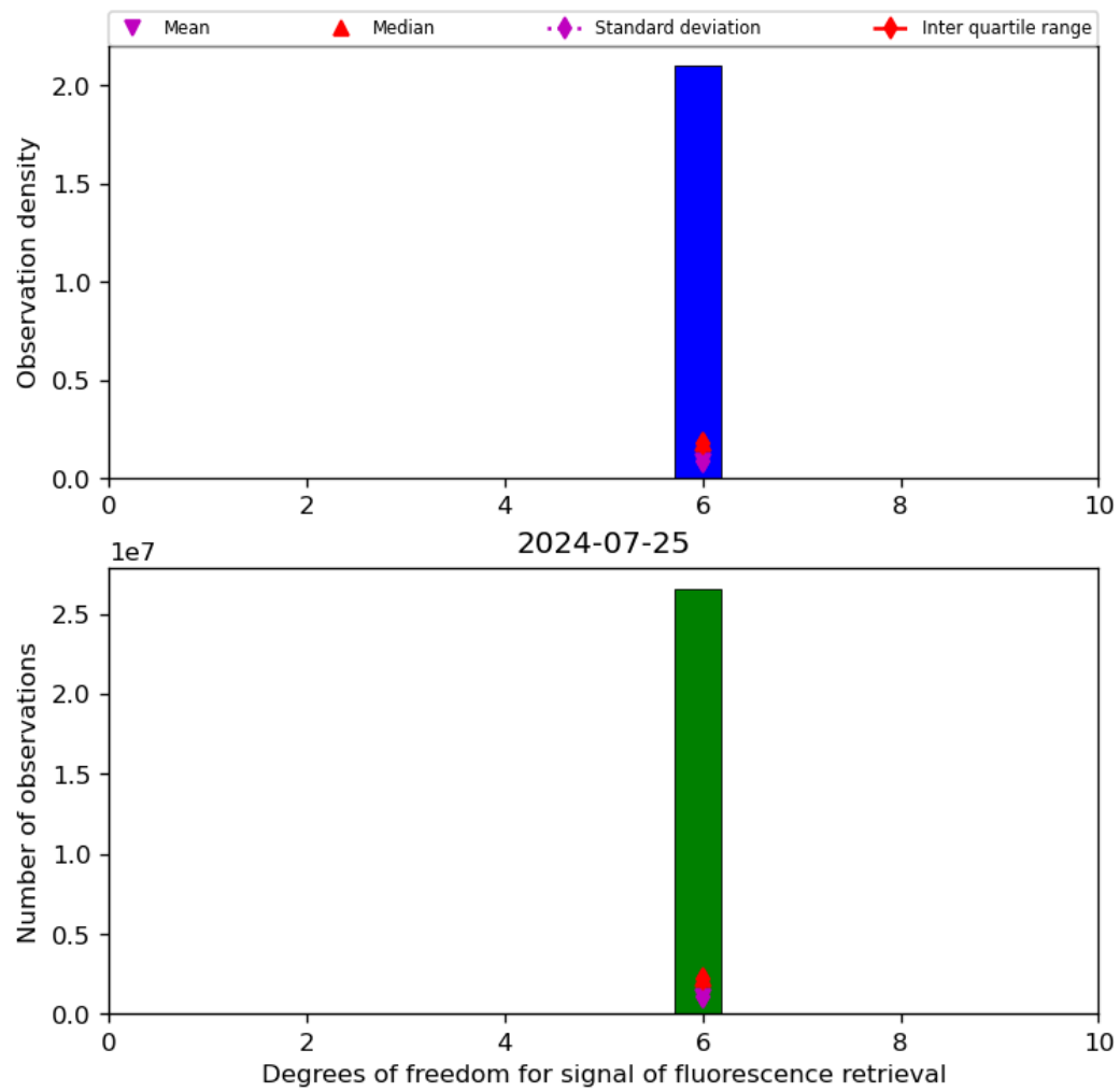
Figure 43: Histogram of “Degrees of freedom for signal of fluorescence retrieval” for 2024-07-24 to 2024-07-26
