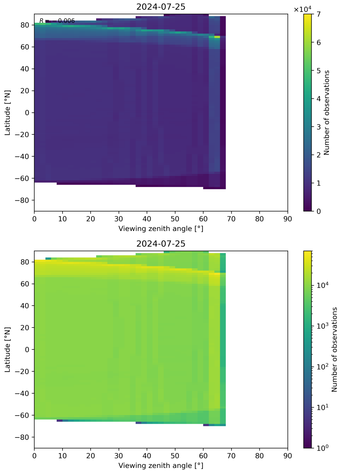
Figure 123: Scatter density plot of “Viewing zenith angle” against “Latitude” for 2024-07-24 to 2024-07-26.
