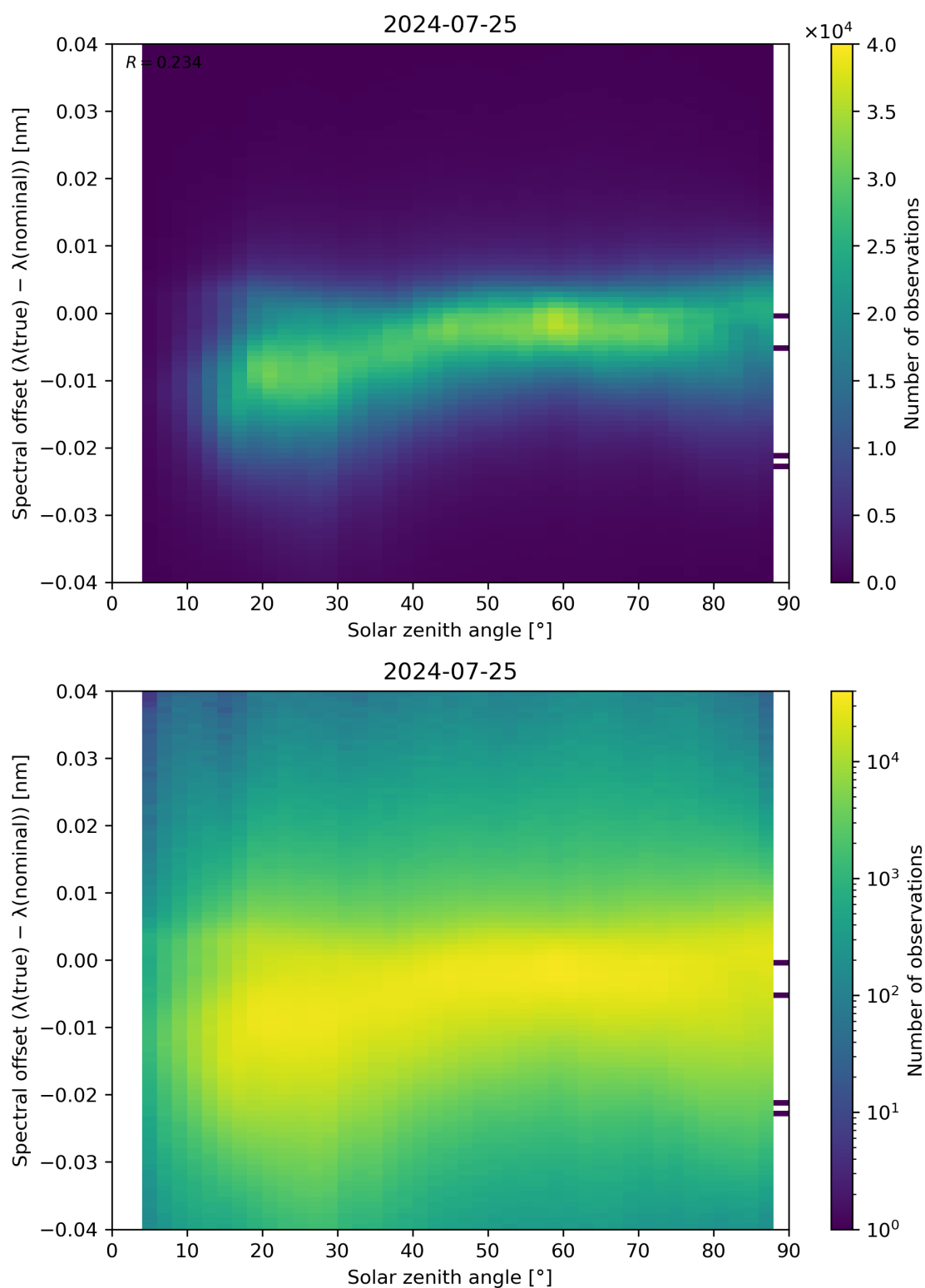
Figure 117: Scatter density plot of “Solar zenith angle” against “Spectral offset ( \lambda(\text{true}) - \lambda(\text{nominal}) )” for 2024-07-24 to 2024-07-26.
