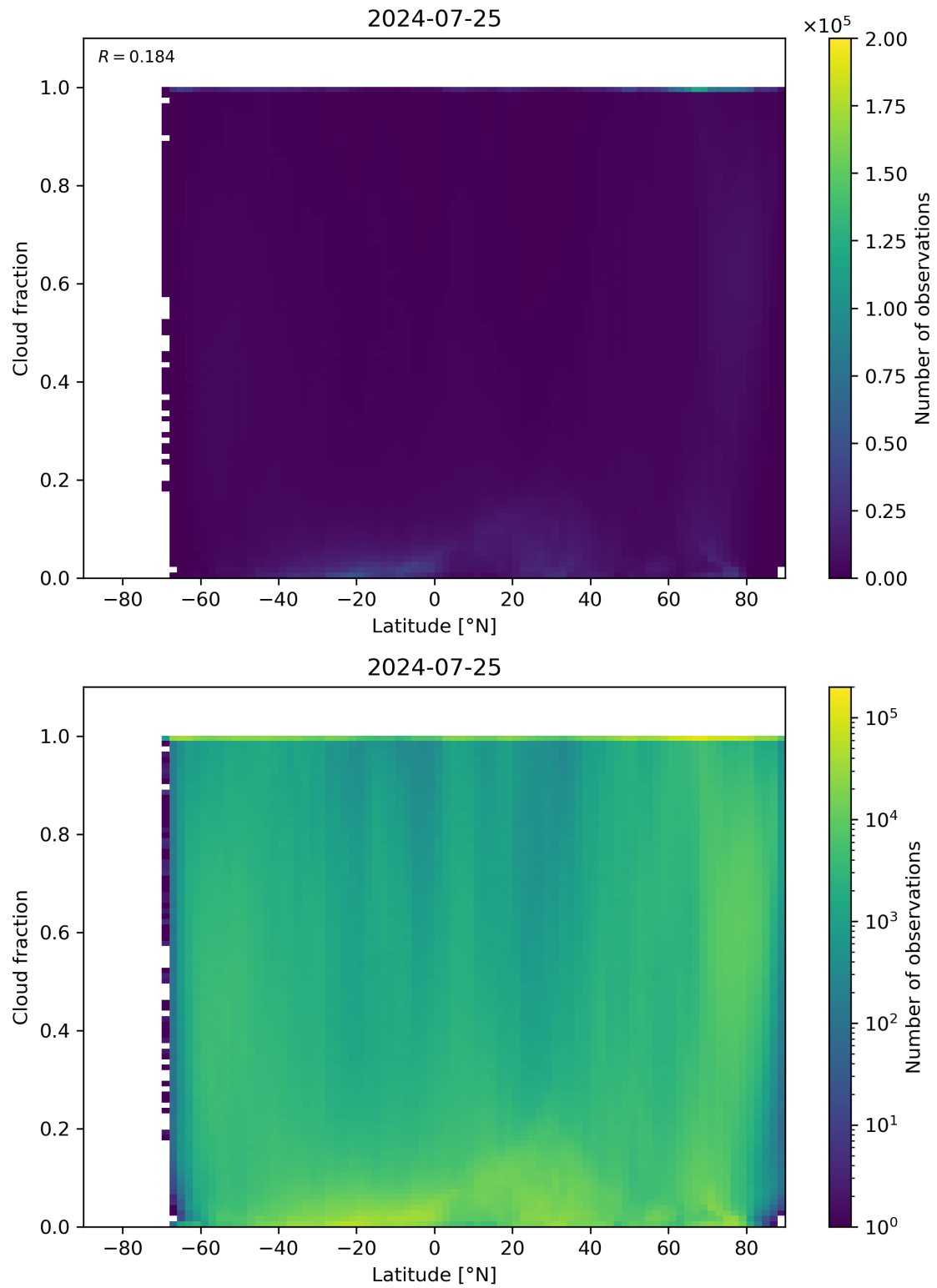
Figure 90: Scatter density plot of “Latitude” against “Cloud fraction” for 2024-07-24 to 2024-07-26.
