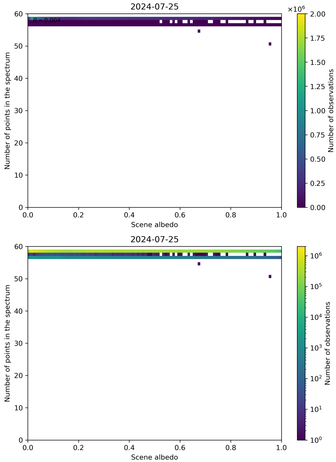
Figure 106: Scatter density plot of “Scene albedo” against “Number of points in the spectrum” for 2024-07-24 to 2024-07-26.
