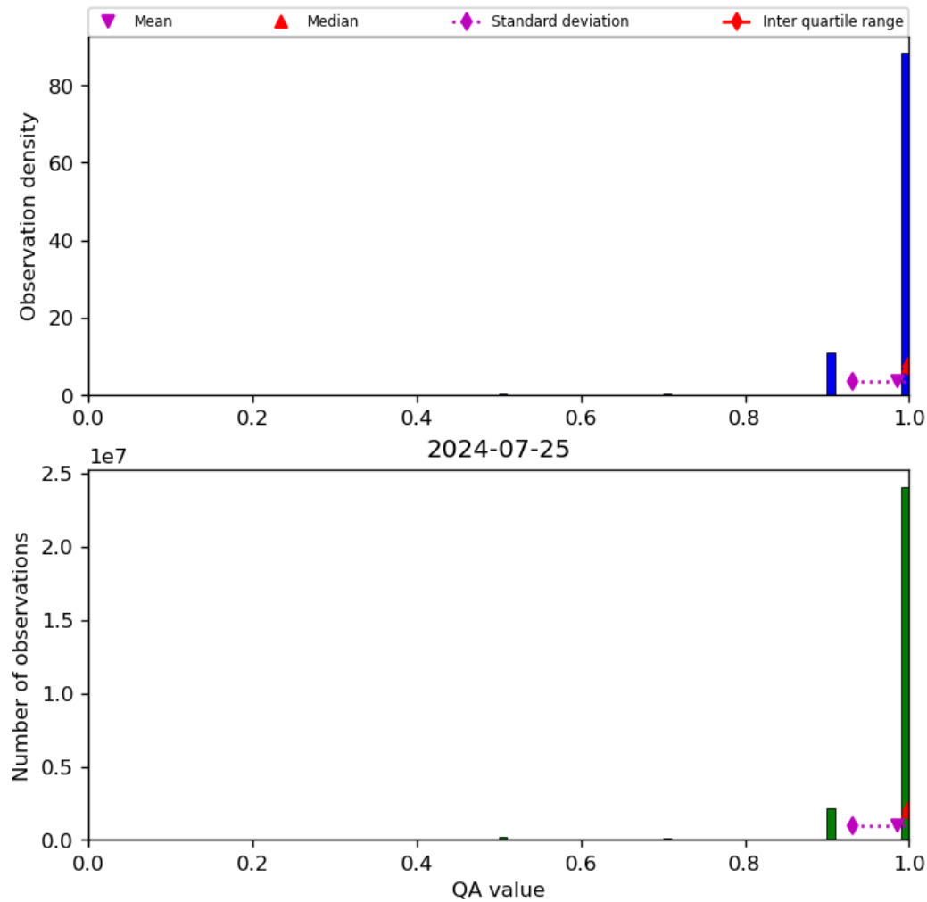
Figure 29: Histogram of “QA value” for 2024-07-24 to 2024-07-26
