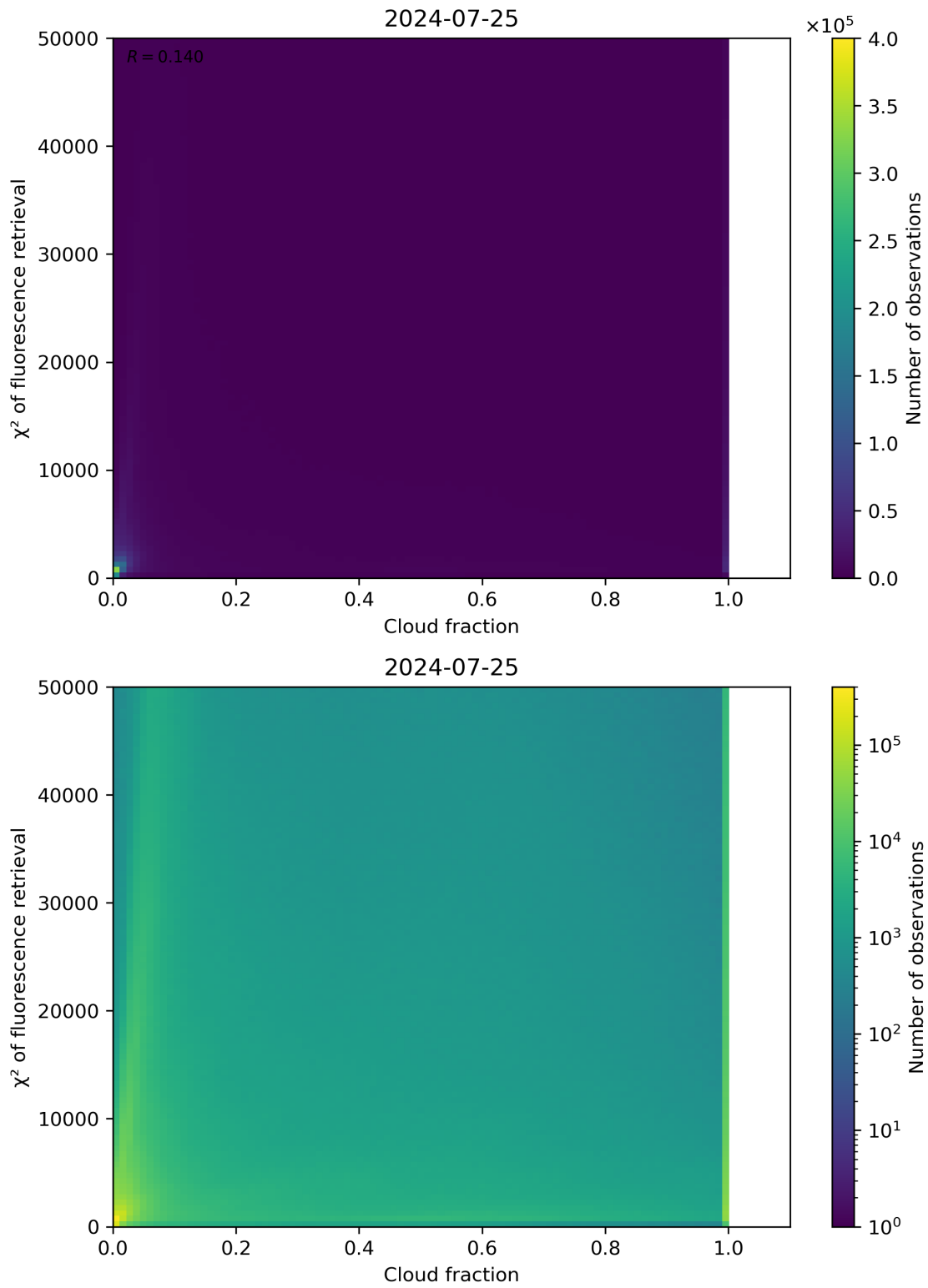
Figure 71: Scatter density plot of “Cloud fraction” against “ \chi^2 of fluorescence retrieval” for 2024-07-24 to 2024-07-26.
