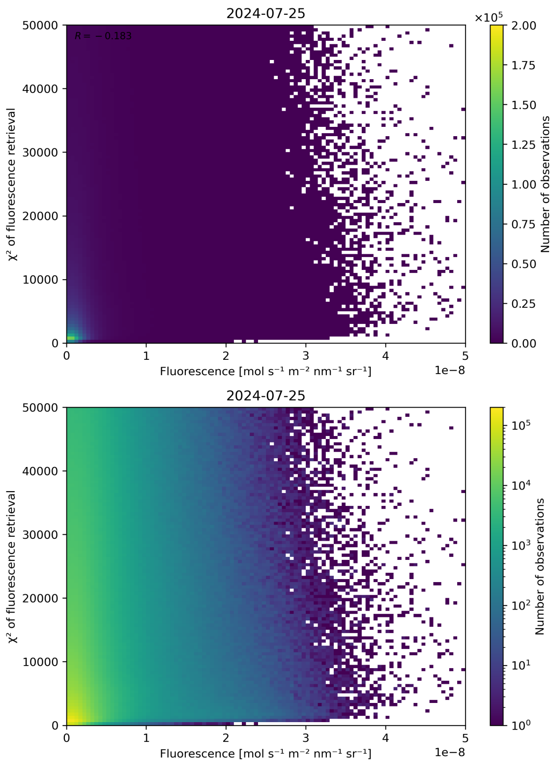
Figure 85: Scatter density plot of “Fluorescence” against “ \chi^2 of fluorescence retrieval” for 2024-07-24 to 2024-07-26.
