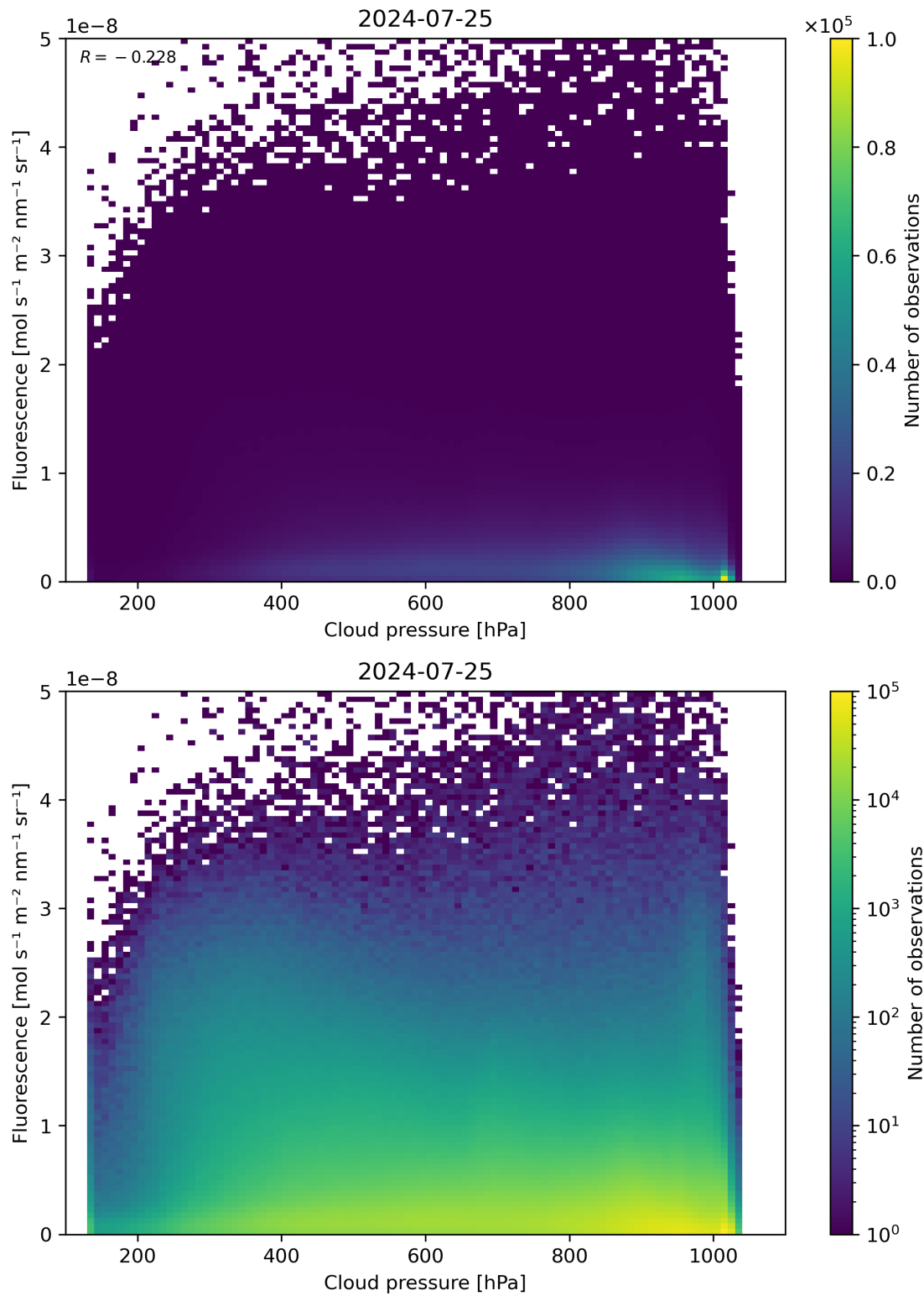
Figure 80: Scatter density plot of “Cloud pressure” against “Fluorescence” for 2024-07-24 to 2024-07-26.
