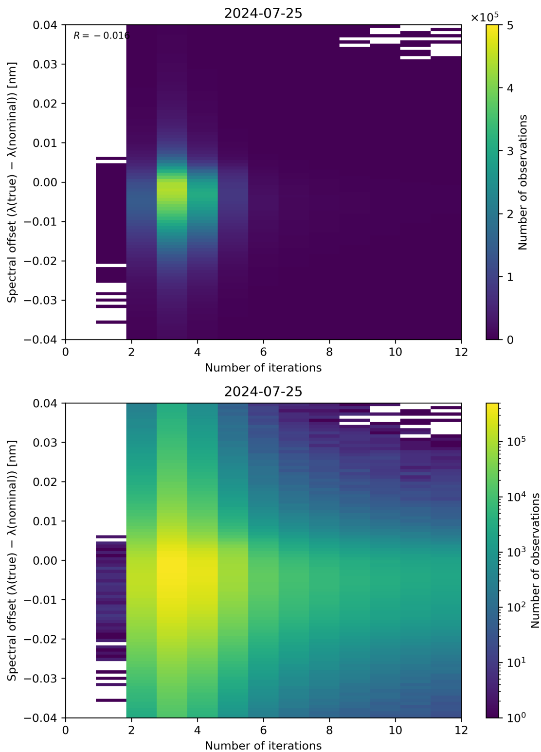
Figure 100: Scatter density plot of “Number of iterations” against “Spectral offset ( \lambda(\text{true}) - \lambda(\text{nominal}) )” for 2024-07-24 to 2024-07-26.
