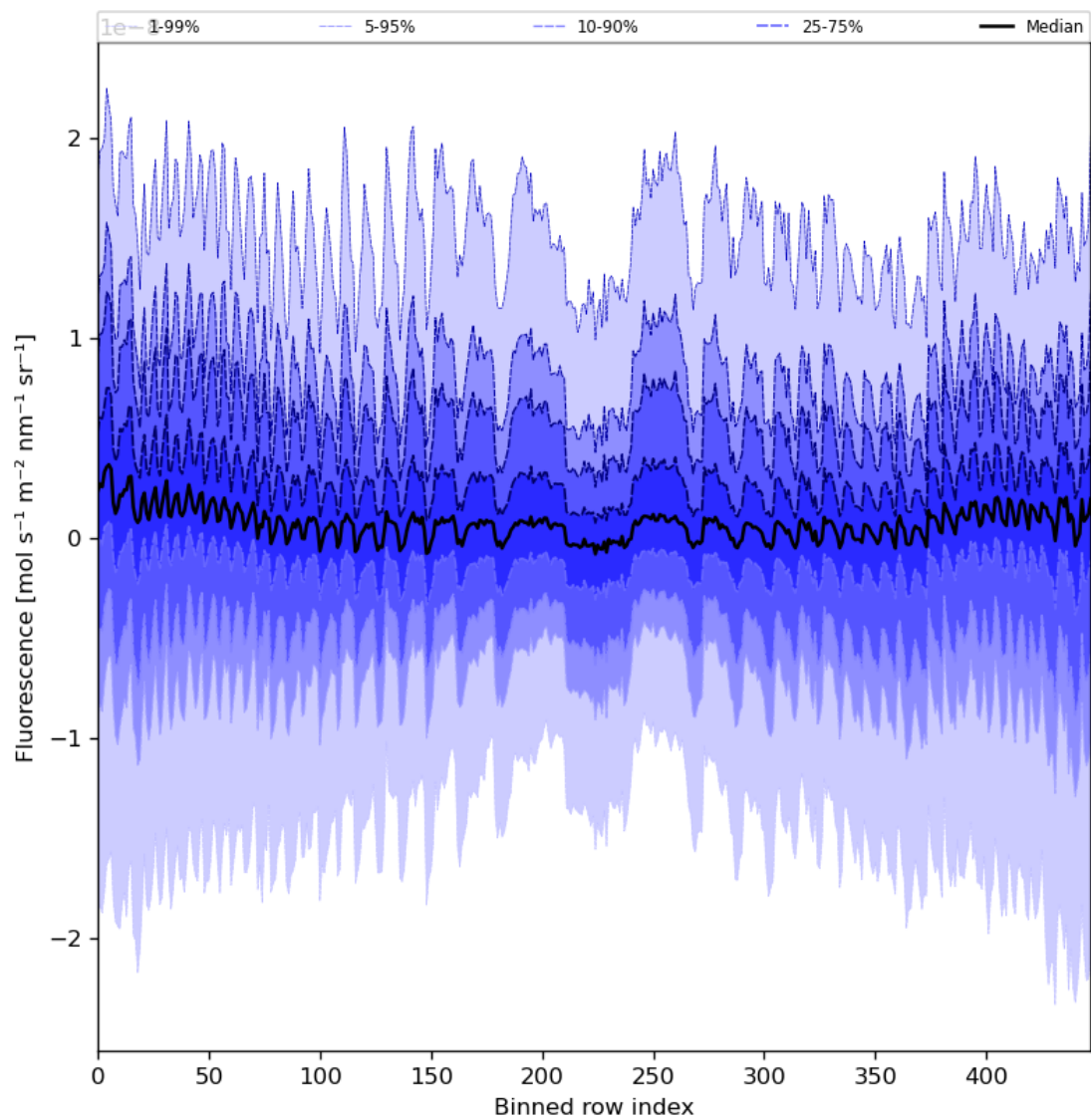
Figure 57: Along track statistics of “Fluorescence” for 2024-07-24 to 2024-07-26
