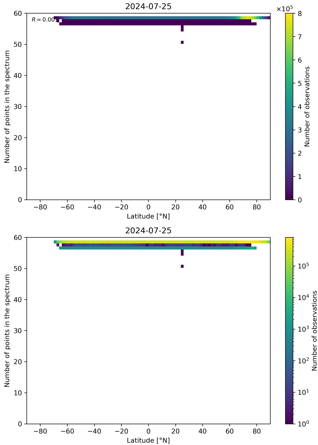
Figure 94: Scatter density plot of “Latitude” against “Number of points in the spectrum” for 2024-07-24 to 2024-07-26.
