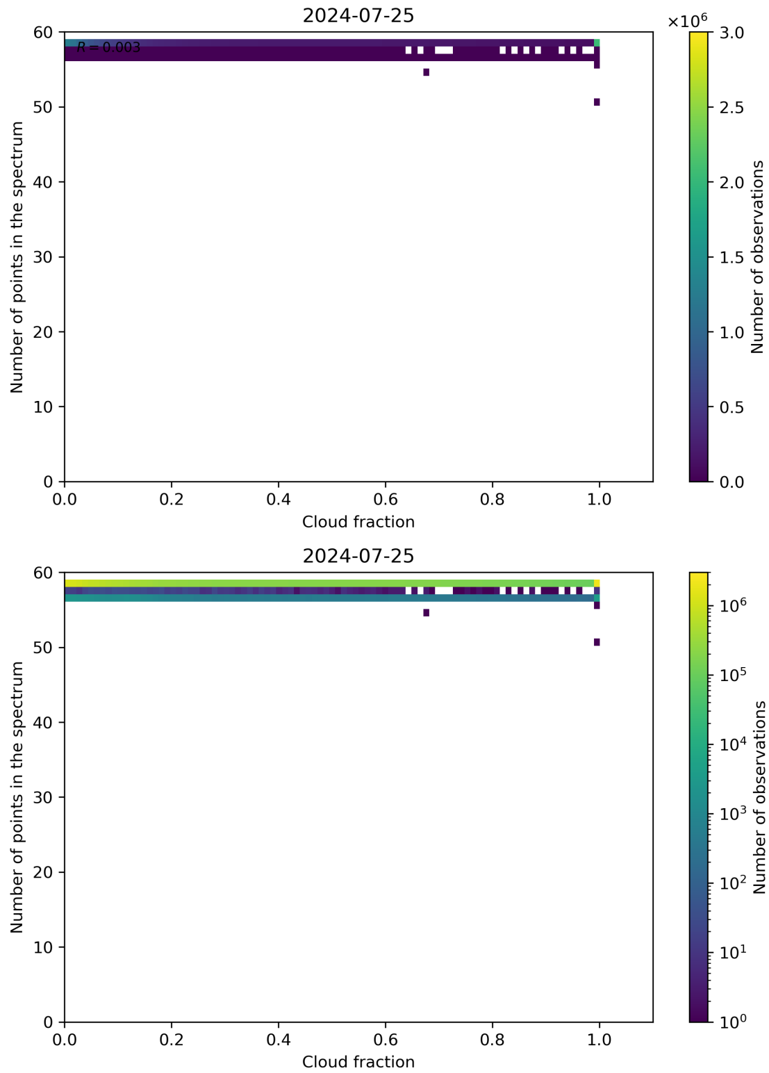
Figure 74: Scatter density plot of “Cloud fraction” against “Number of points in the spectrum” for 2024-07-24 to 2024-07-26.
