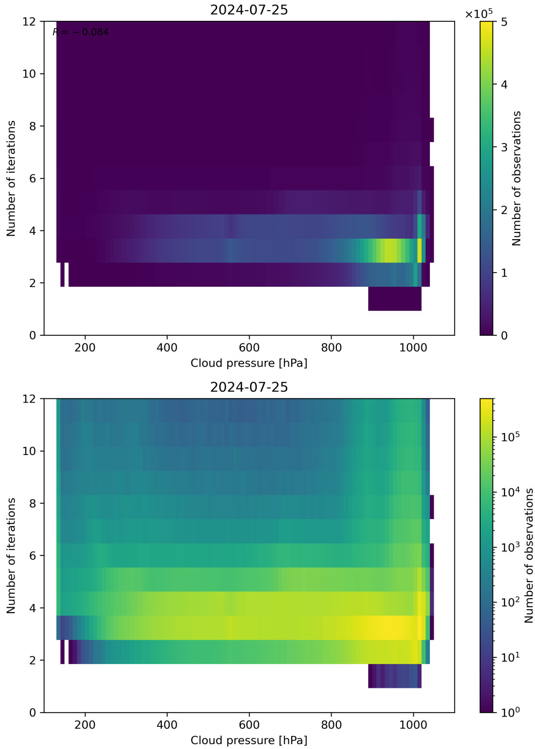
Figure 81: Scatter density plot of “Cloud pressure” against “Number of iterations” for 2024-07-24 to 2024-07-26.
