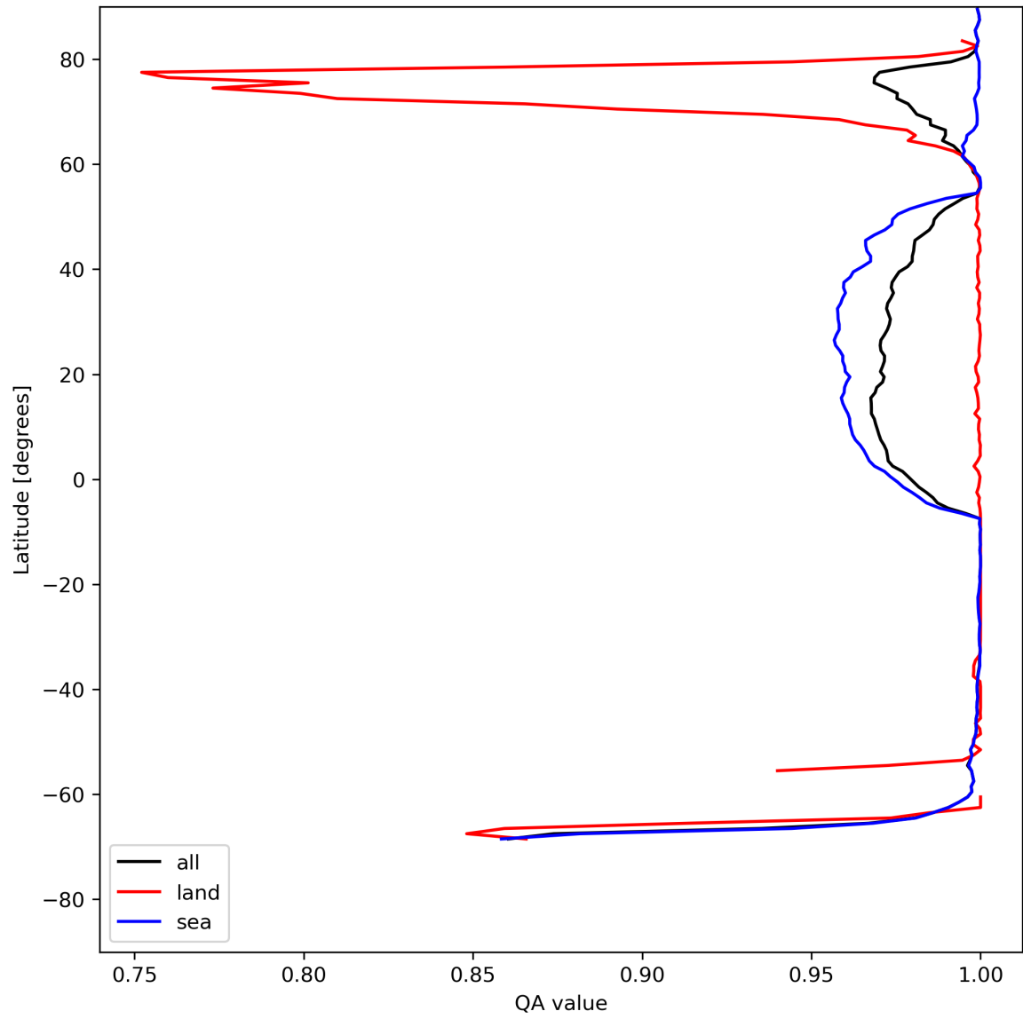
Figure 12: Zonal average of “QA value” for 2024-07-24 to 2024-07-26.
