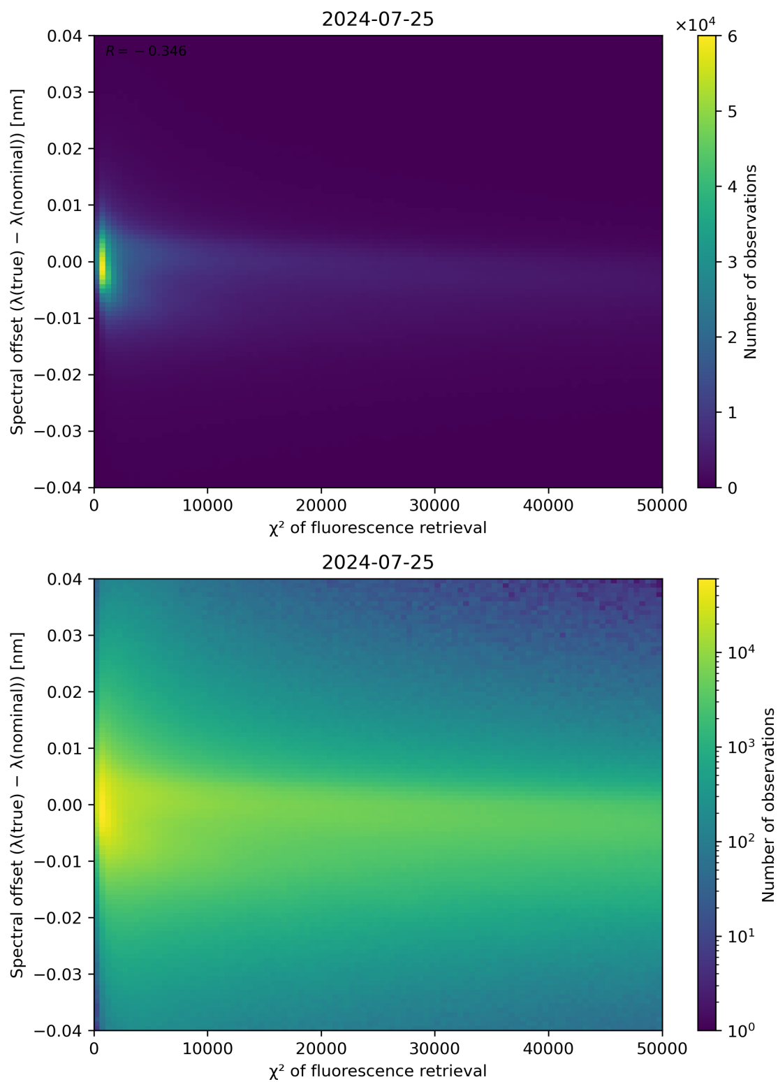
Figure 69: Scatter density plot of " \chi^2 of fluorescence retrieval" against "Spectral offset ( \lambda(\text{true}) - \lambda(\text{nominal}) )" for 2024-07-24 to 2024-07-26.
