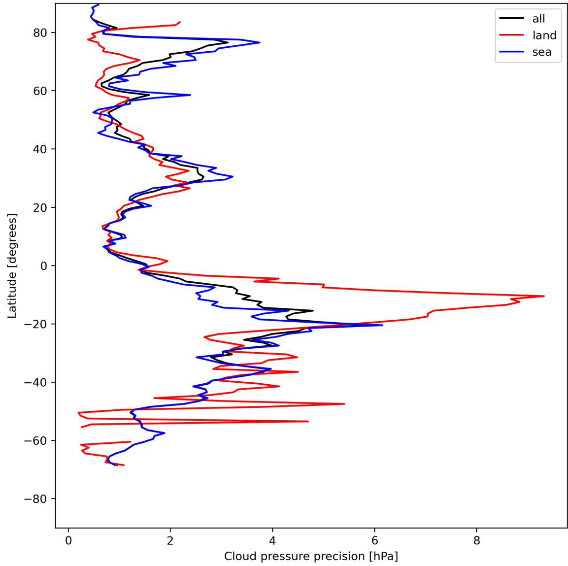
Figure 14: Zonal average of “Cloud pressure precision” for 2024-07-26 to 2024-07-27.
