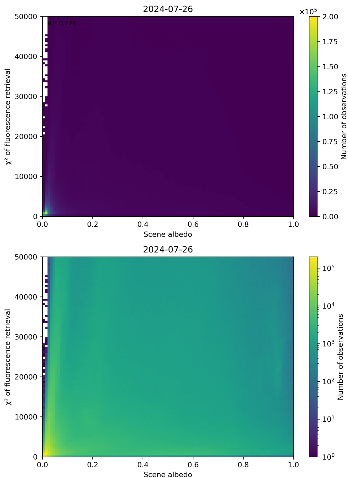
Figure 103: Scatter density plot of “Scene albedo” against “ \chi^2 of fluorescence retrieval” for 2024-07-26 to 2024-07-27.
