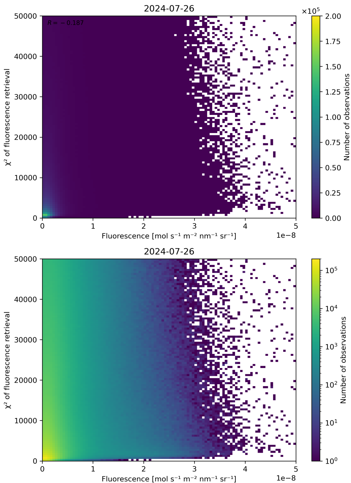
Figure 85: Scatter density plot of “Fluorescence” against “ \chi^2 of fluorescence retrieval” for 2024-07-26 to 2024-07-27.
