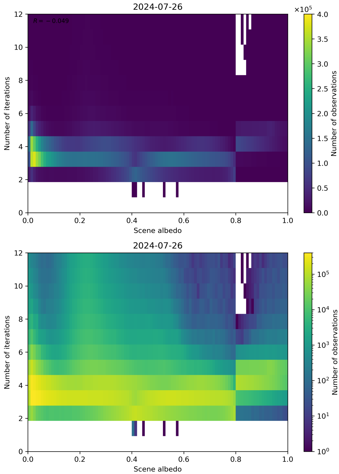
Figure 105: Scatter density plot of “Scene albedo” against “Number of iterations” for 2024-07-26 to 2024-07-27.
