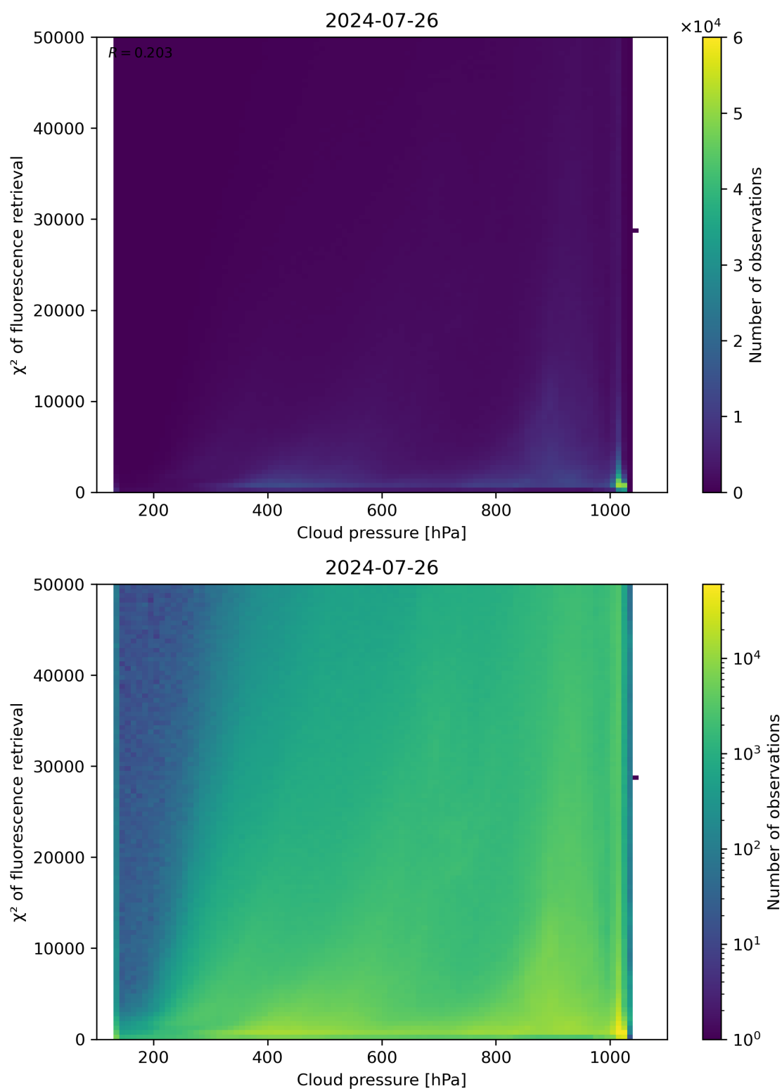
Figure 78: Scatter density plot of “Cloud pressure” against “ \chi^2 of fluorescence retrieval” for 2024-07-26 to 2024-07-27.
