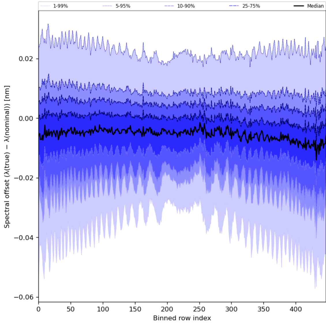
Figure 62: Along track statistics of “Spectral offset ( \lambda(\text{true}) - \lambda(\text{nominal}) )” for 2024-07-26 to 2024-07-27
