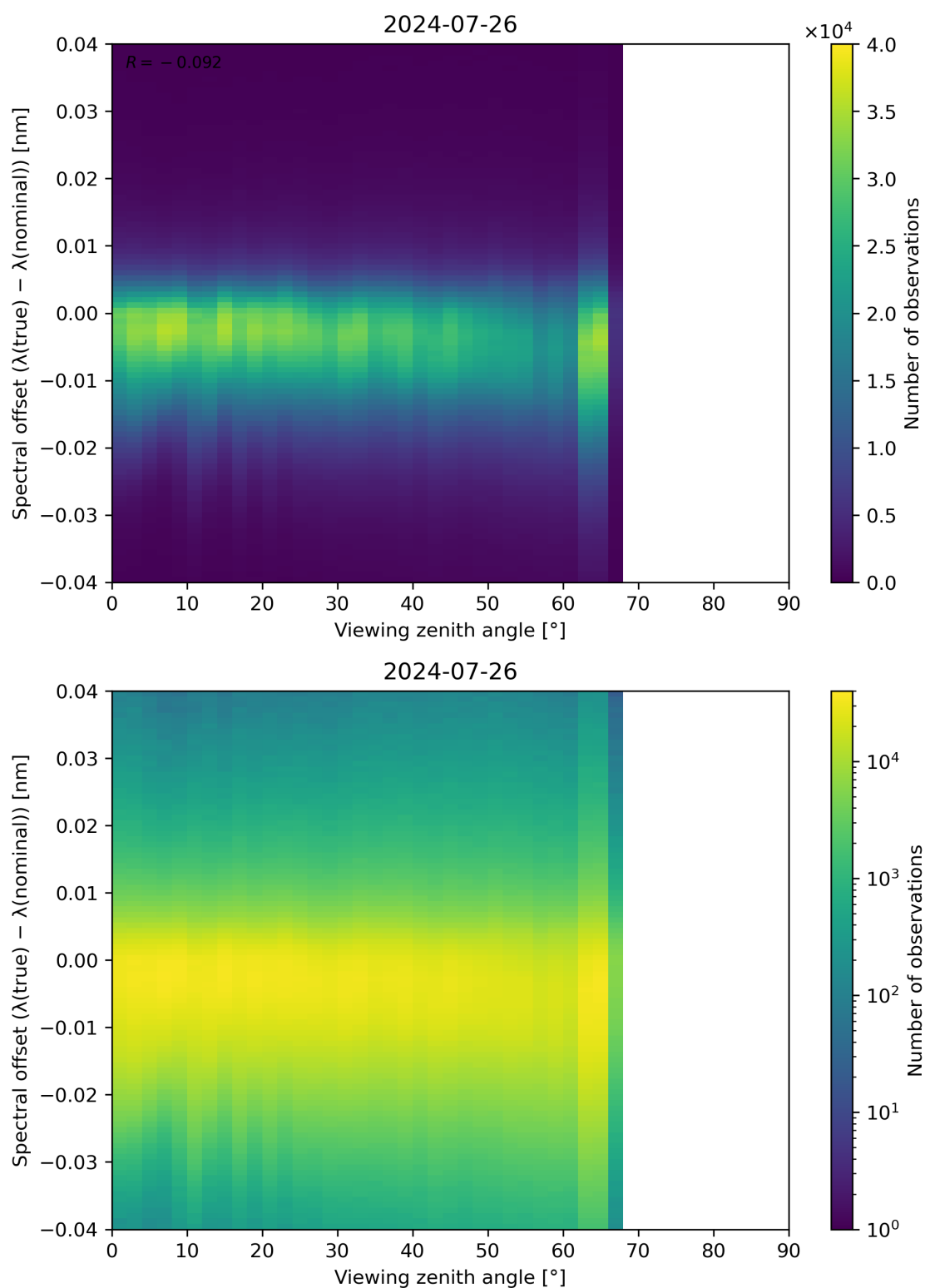
Figure 128: Scatter density plot of “Viewing zenith angle” against “Spectral offset ( \lambda(\text{true}) - \lambda(\text{nominal}) )” for 2024-07-26 to 2024-07-27.
