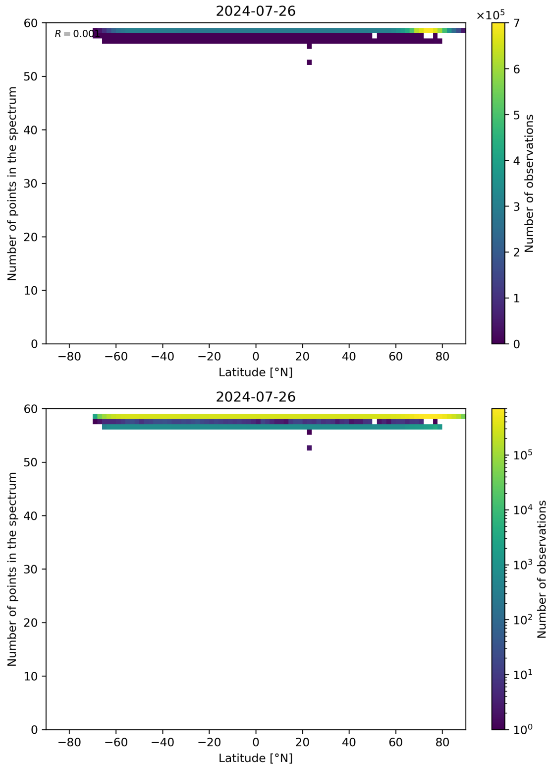
Figure 94: Scatter density plot of “Latitude” against “Number of points in the spectrum” for 2024-07-26 to 2024-07-27.
