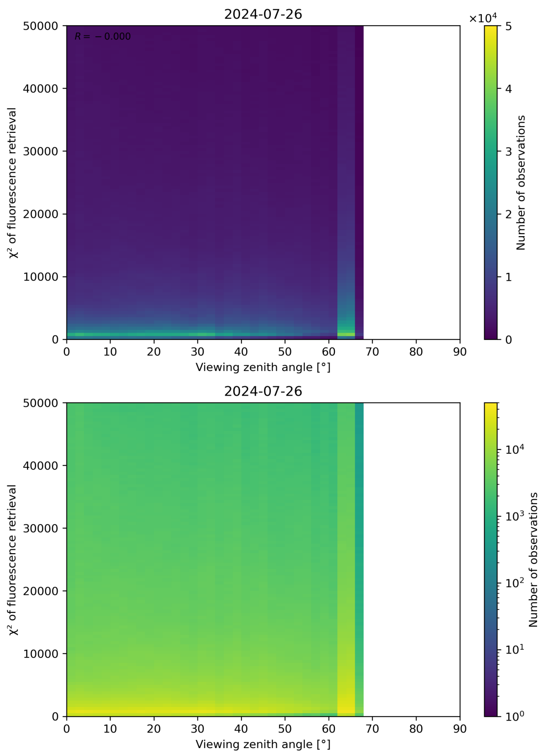
Figure 119: Scatter density plot of “Viewing zenith angle” against “ \chi^2 of fluorescence retrieval” for 2024-07-26 to 2024-07-27.
