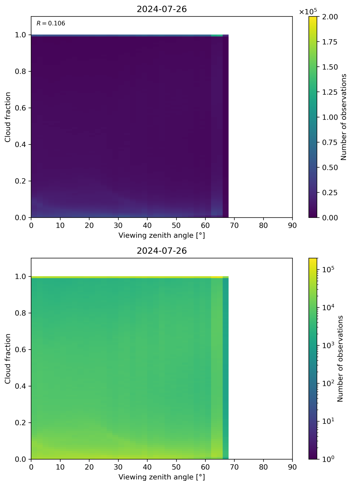
Figure 120: Scatter density plot of “Viewing zenith angle” against “Cloud fraction” for 2024-07-26 to 2024-07-27.
