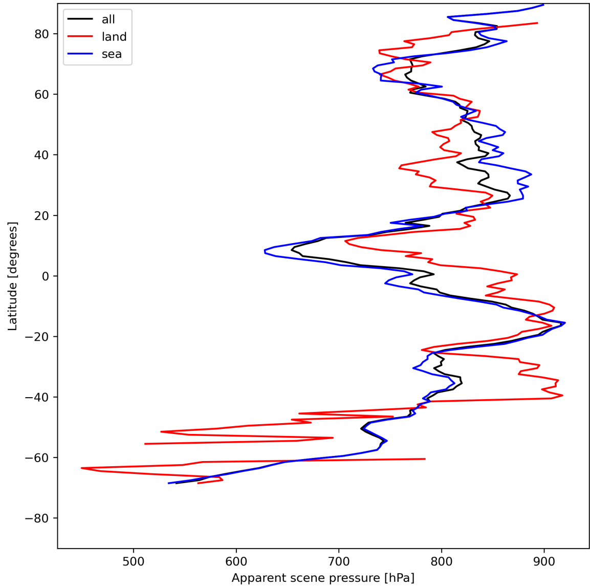
Figure 19: Zonal average of “Apparent scene pressure” for 2024-07-26 to 2024-07-27.
