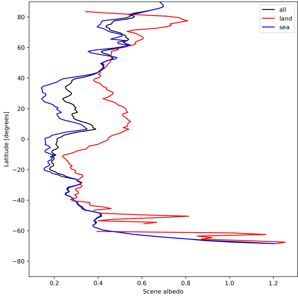
Figure 17: Zonal average of “Scene albedo” for 2024-07-26 to 2024-07-27.
