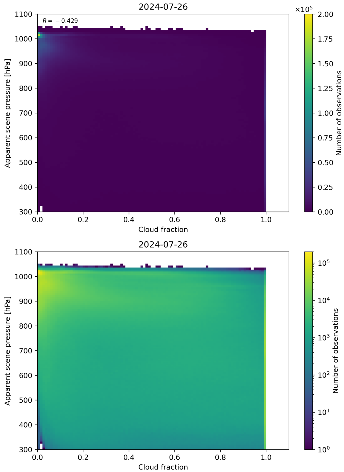
Figure 70: Scatter density plot of “Cloud fraction” against “Apparent scene pressure” for 2024-07-26 to 2024-07-27.
