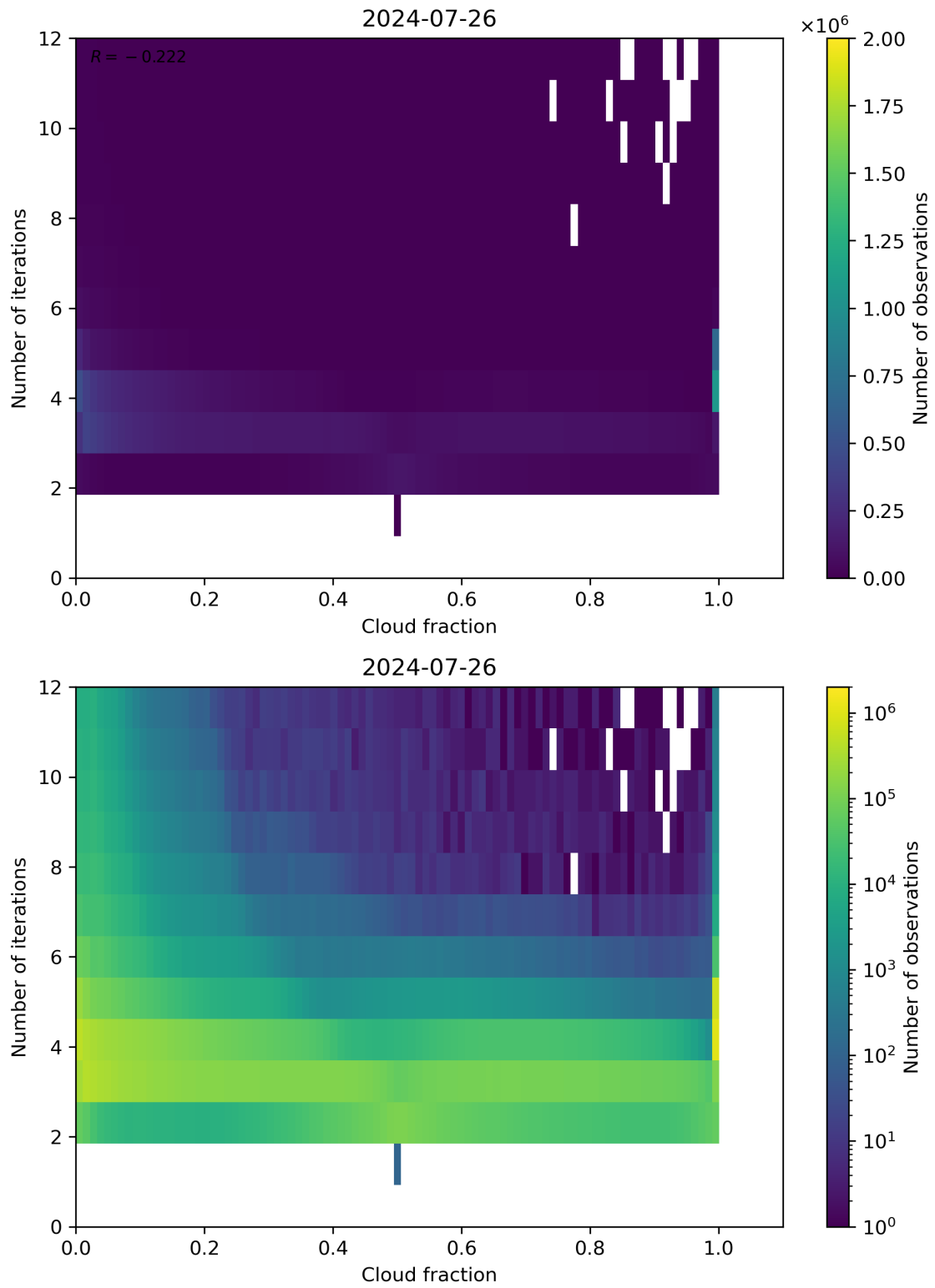
Figure 73: Scatter density plot of “Cloud fraction” against “Number of iterations” for 2024-07-26 to 2024-07-27.
