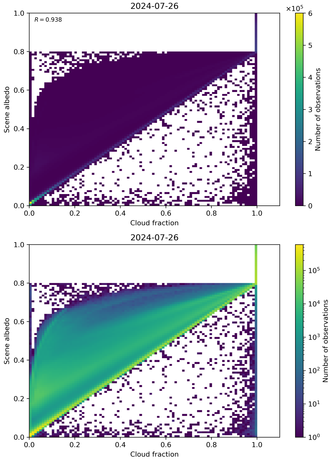
Figure 75: Scatter density plot of “Cloud fraction” against “Scene albedo” for 2024-07-26 to 2024-07-27.
