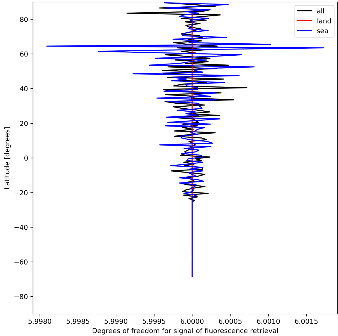
Figure 26: Zonal average of “Degrees of freedom for signal of fluorescence retrieval” for 2024-07-26 to 2024-07-27.
