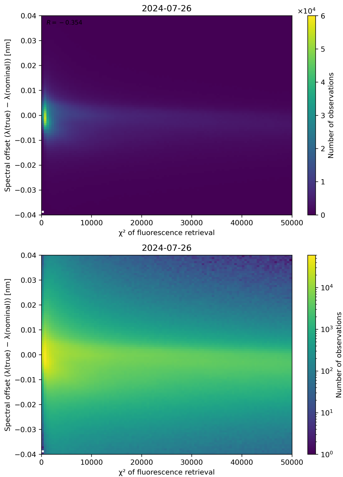
Figure 69: Scatter density plot of " \chi^2 of fluorescence retrieval" against "Spectral offset ( \lambda(\text{true}) - \lambda(\text{nominal}) )" for 2024-07-26 to 2024-07-27.
