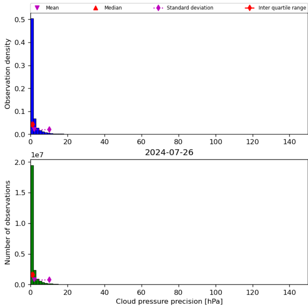
Figure 31: Histogram of “Cloud pressure precision” for 2024-07-26 to 2024-07-27
