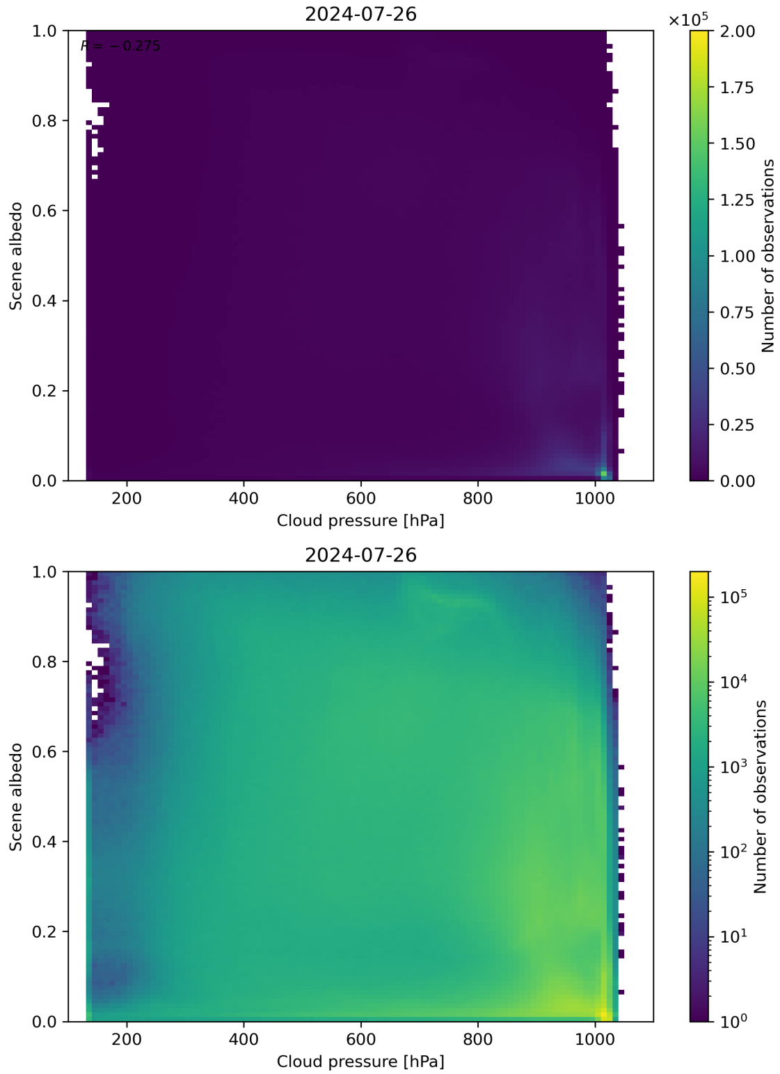
Figure 83: Scatter density plot of “Cloud pressure” against “Scene albedo” for 2024-07-26 to 2024-07-27.
