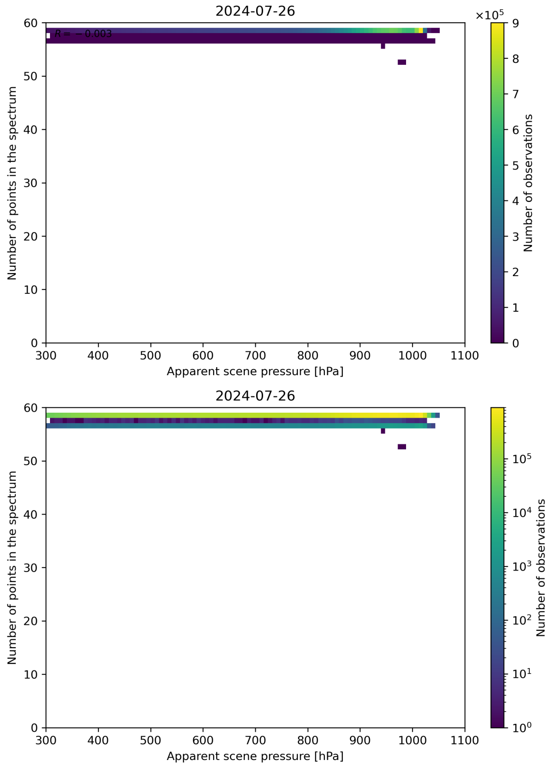
Figure 66: Scatter density plot of “Apparent scene pressure” against “Number of points in the spectrum” for 2024-07-26 to 2024-07-27.
