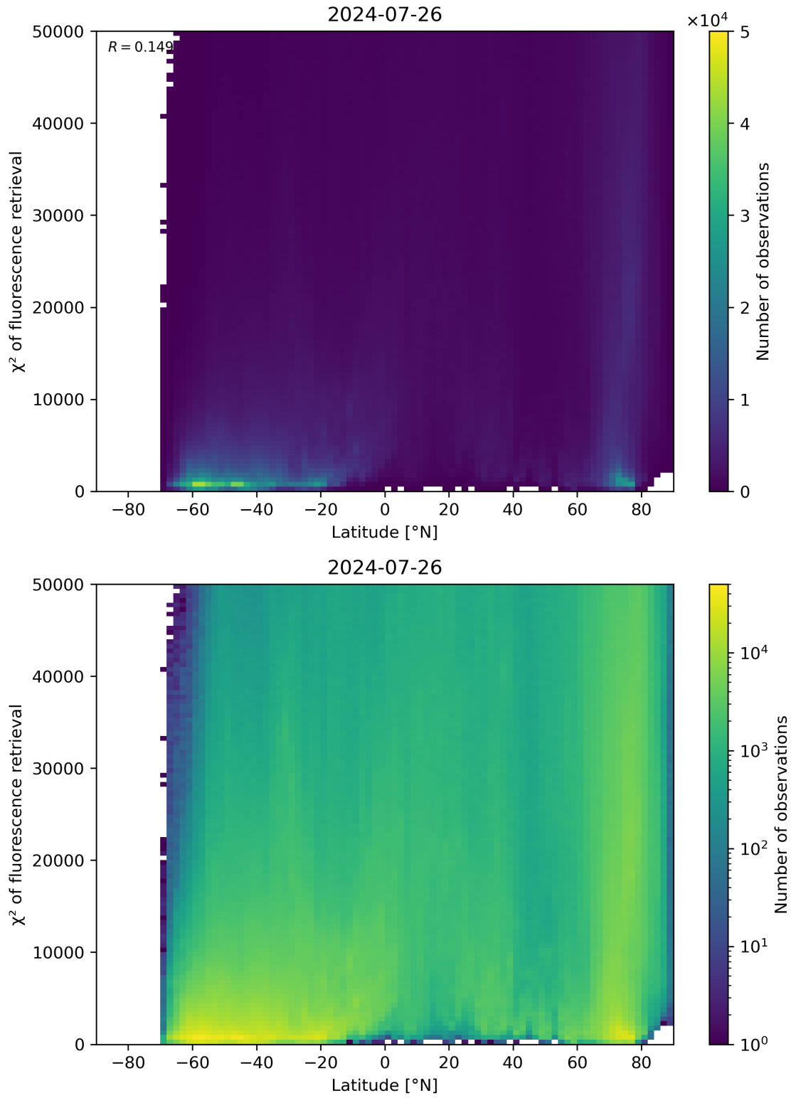
Figure 89: Scatter density plot of “Latitude” against “ \chi^2 of fluorescence retrieval” for 2024-07-26 to 2024-07-27.
