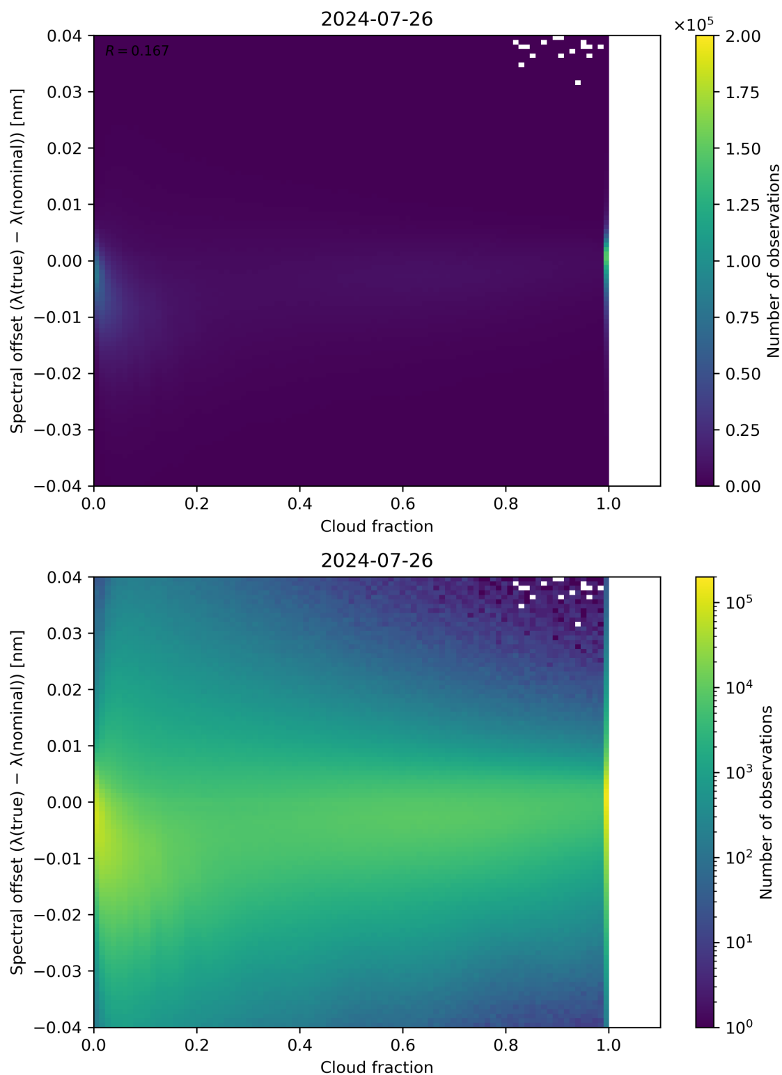
Figure 76: Scatter density plot of “Cloud fraction” against “Spectral offset ( \lambda(\text{true}) - \lambda(\text{nominal}) )” for 2024-07-26 to 2024-07-27.
