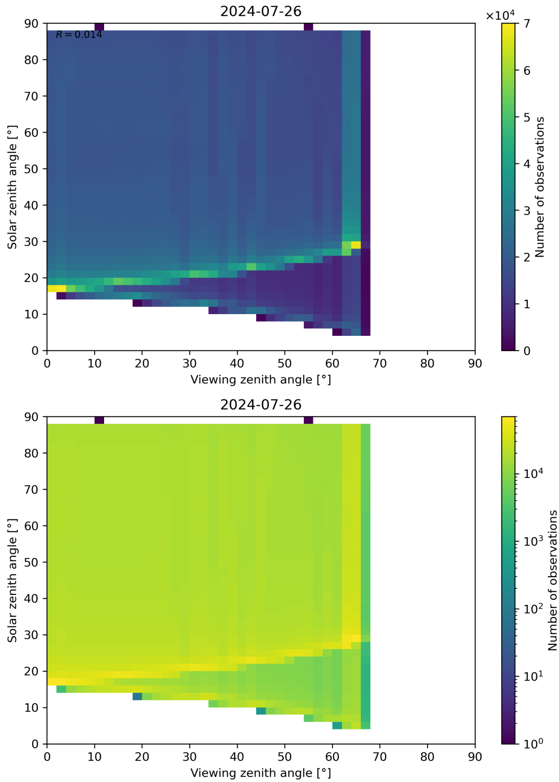
Figure 127: Scatter density plot of “Viewing zenith angle” against “Solar zenith angle” for 2024-07-26 to 2024-07-27.
