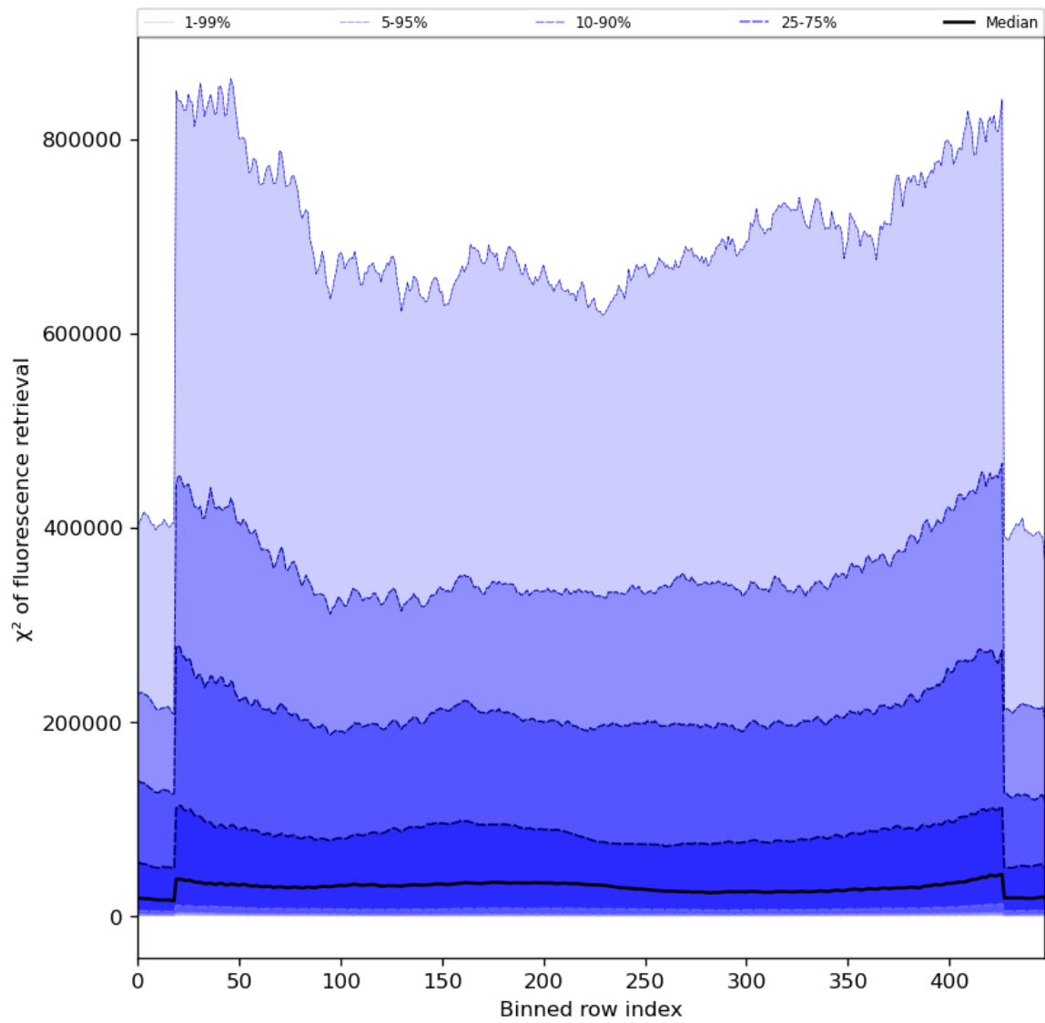
Figure 59: Along track statistics of “ \chi^2 of fluorescence retrieval” for 2024-07-26 to 2024-07-27
