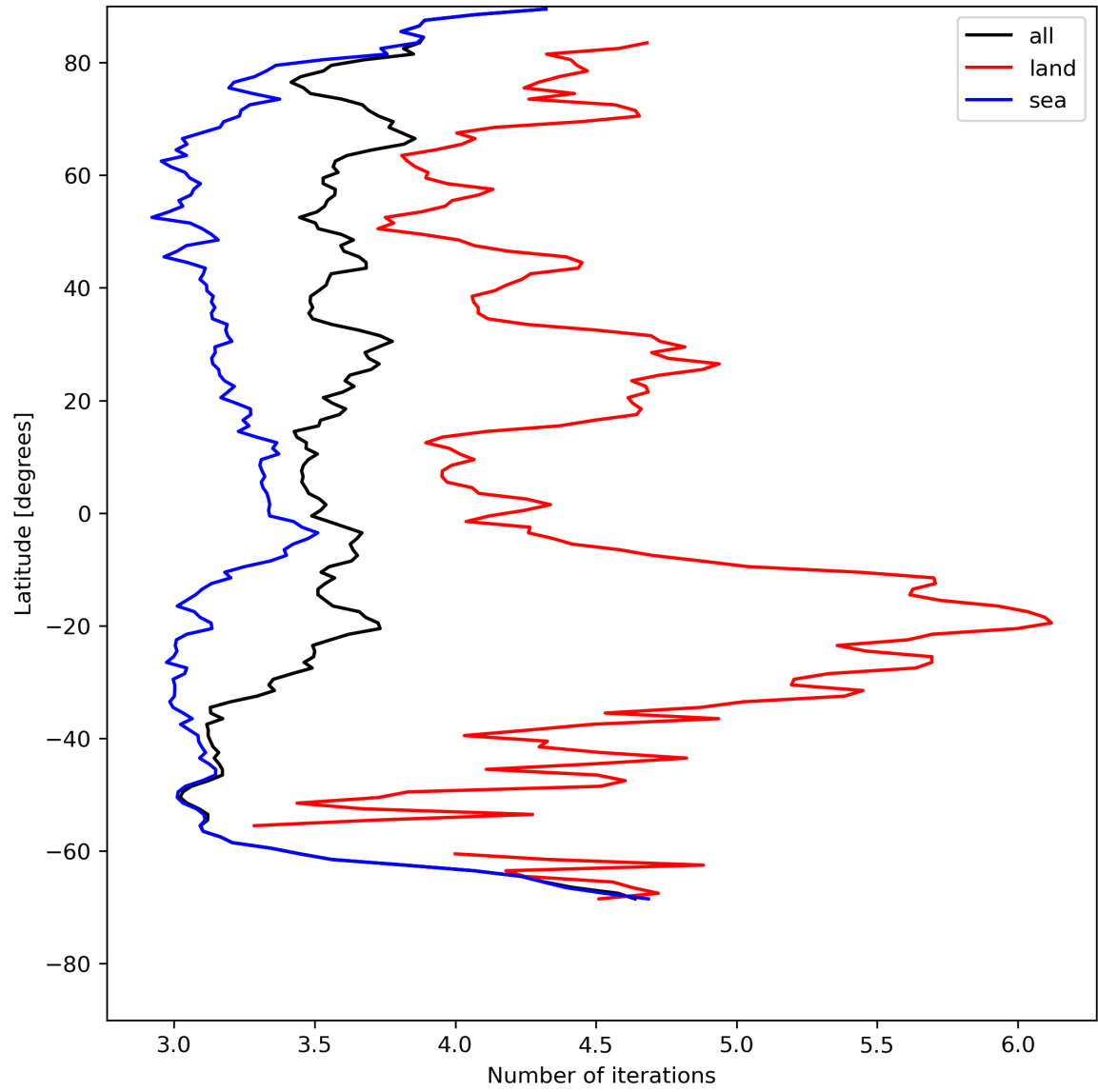
Figure 22: Zonal average of “Number of iterations” for 2024-07-26 to 2024-07-27.
