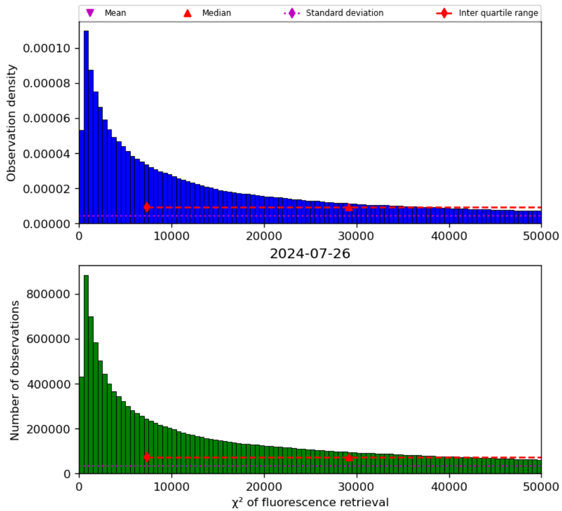
Figure 42: Histogram of “ \chi^2 of fluorescence retrieval” for 2024-07-26 to 2024-07-27
