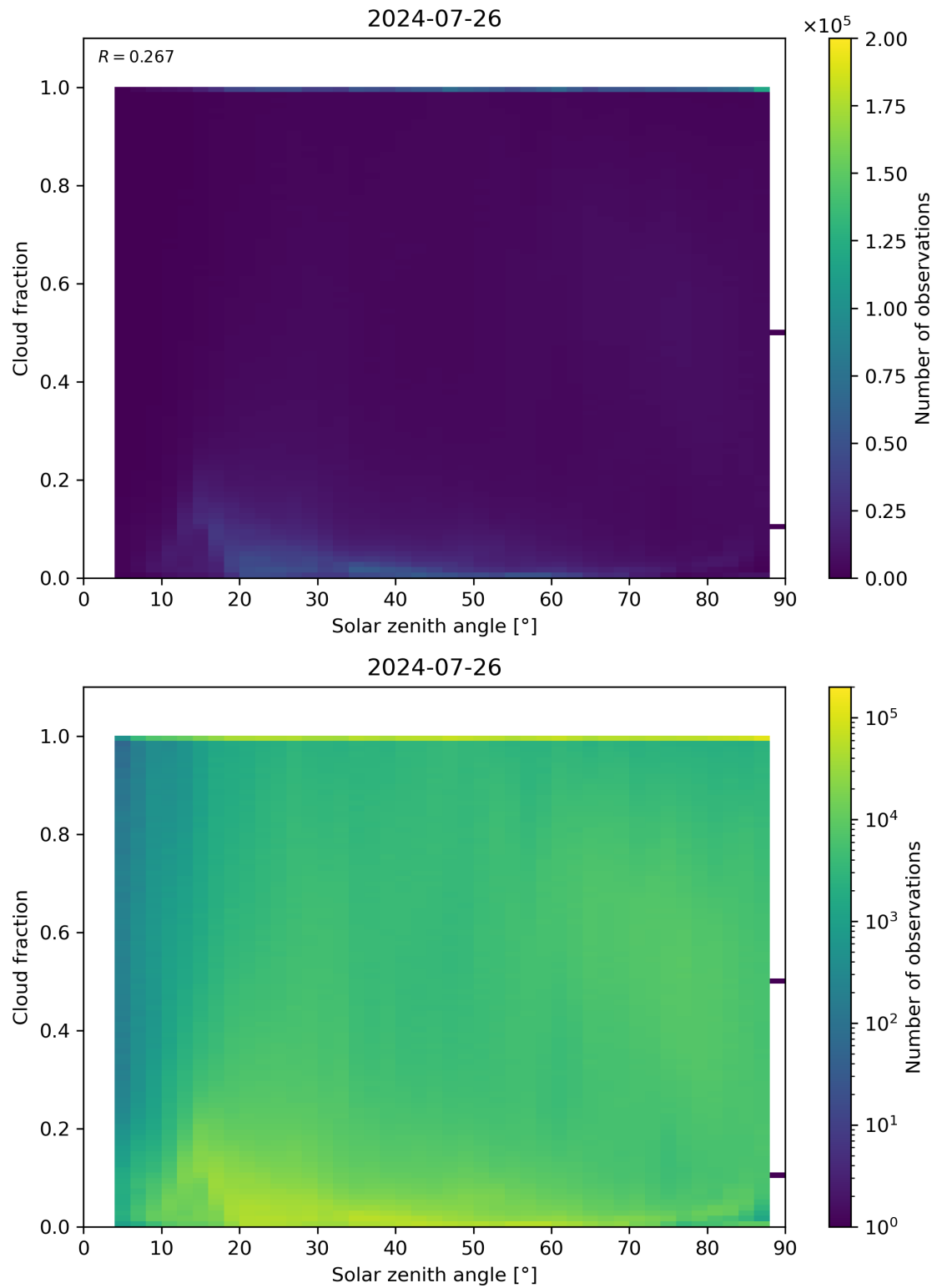
Figure 110: Scatter density plot of “Solar zenith angle” against “Cloud fraction” for 2024-07-26 to 2024-07-27.
