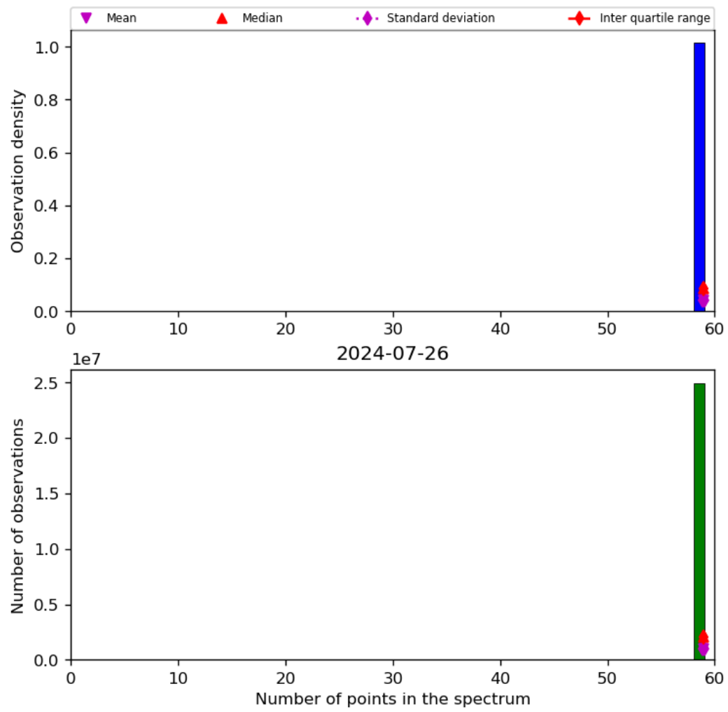
Figure 44: Histogram of “Number of points in the spectrum” for 2024-07-26 to 2024-07-27
