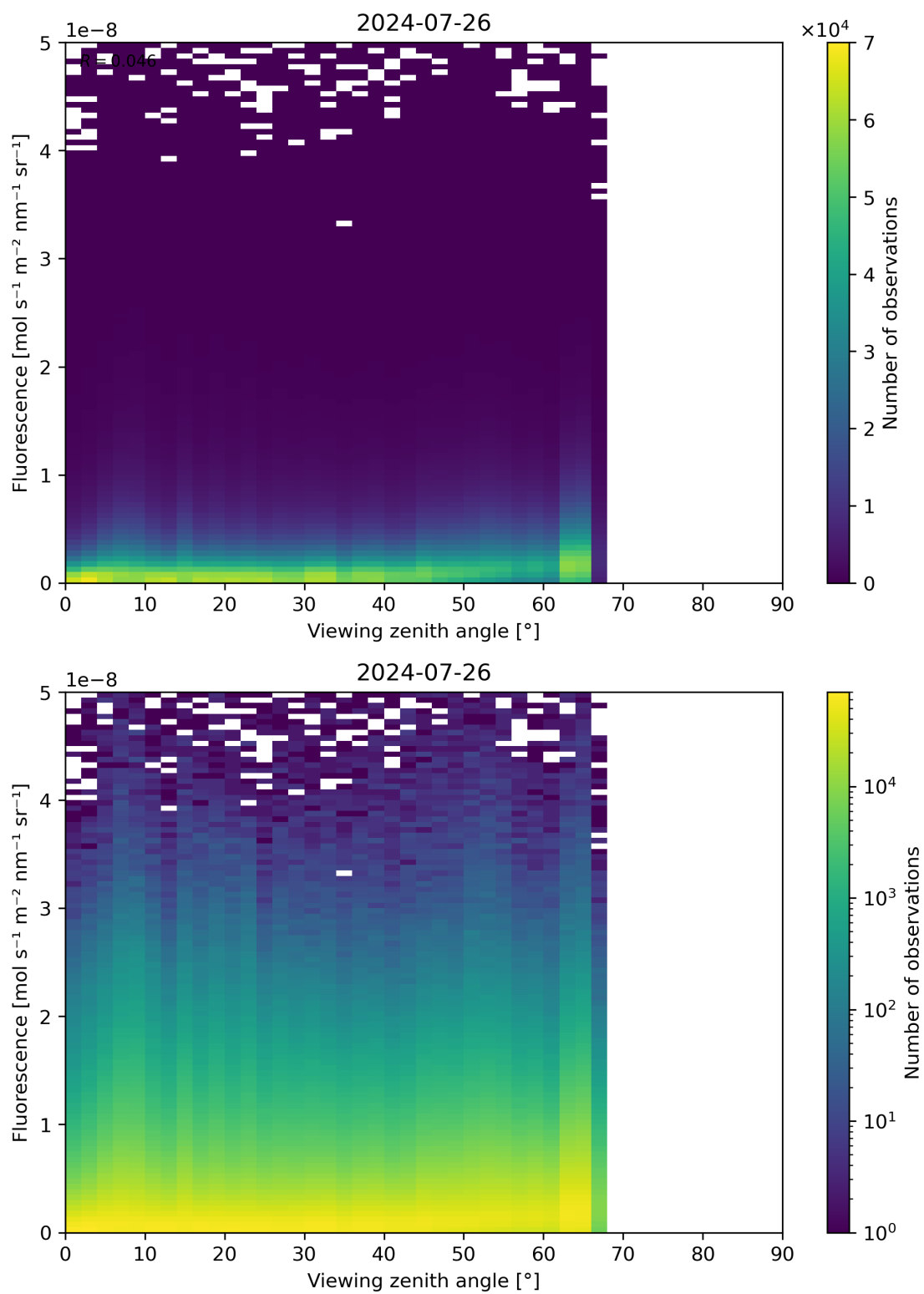
Figure 122: Scatter density plot of “Viewing zenith angle” against “Fluorescence” for 2024-07-26 to 2024-07-27.
