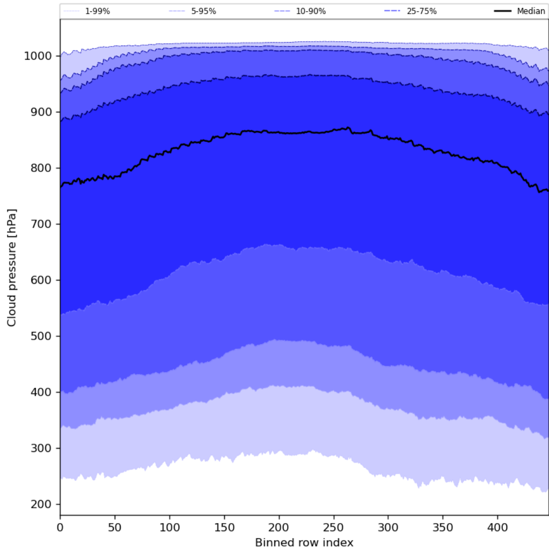
Figure 47: Along track statistics of “Cloud pressure” for 2024-07-26 to 2024-07-27
