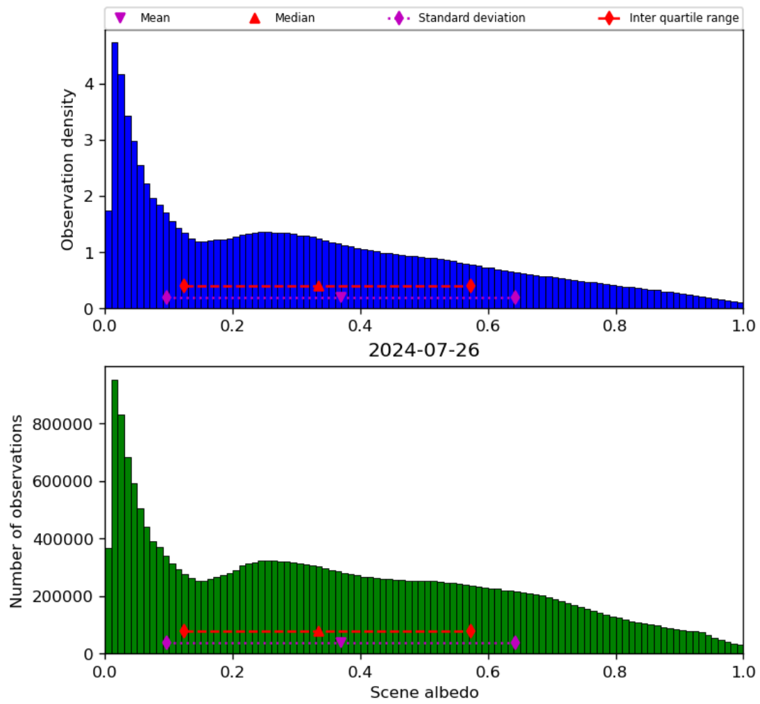
Figure 34: Histogram of “Scene albedo” for 2024-07-26 to 2024-07-27
