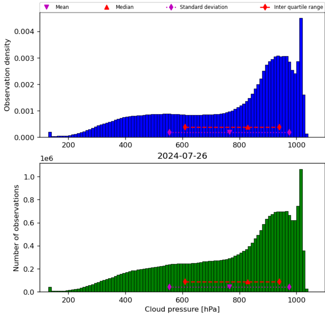
Figure 30: Histogram of “Cloud pressure” for 2024-07-26 to 2024-07-27
