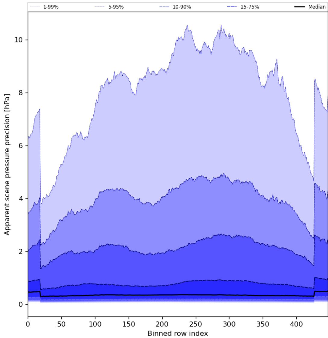
Figure 54: Along track statistics of “Apparent scene pressure precision” for 2024-07-26 to 2024-07-27
