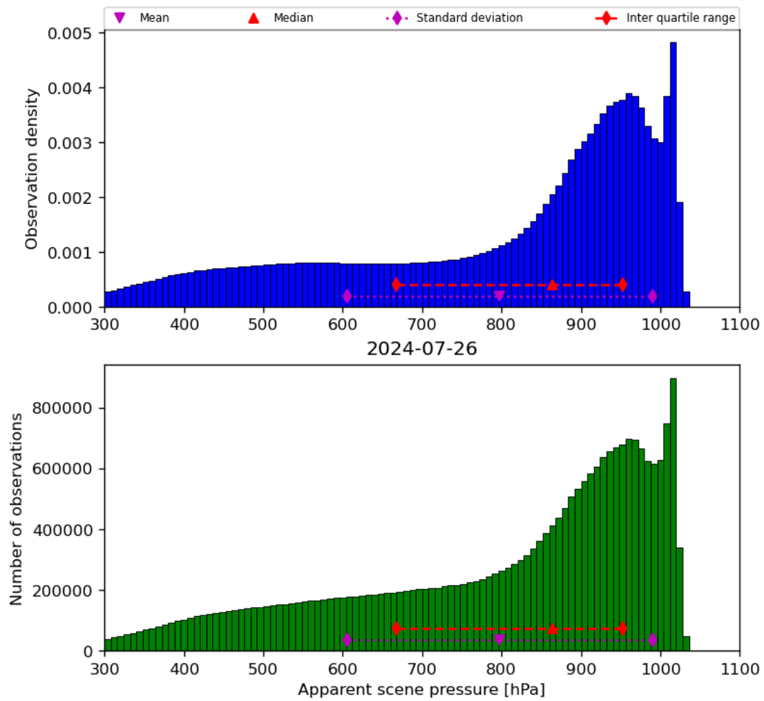
Figure 36: Histogram of “Apparent scene pressure” for 2024-07-26 to 2024-07-27
