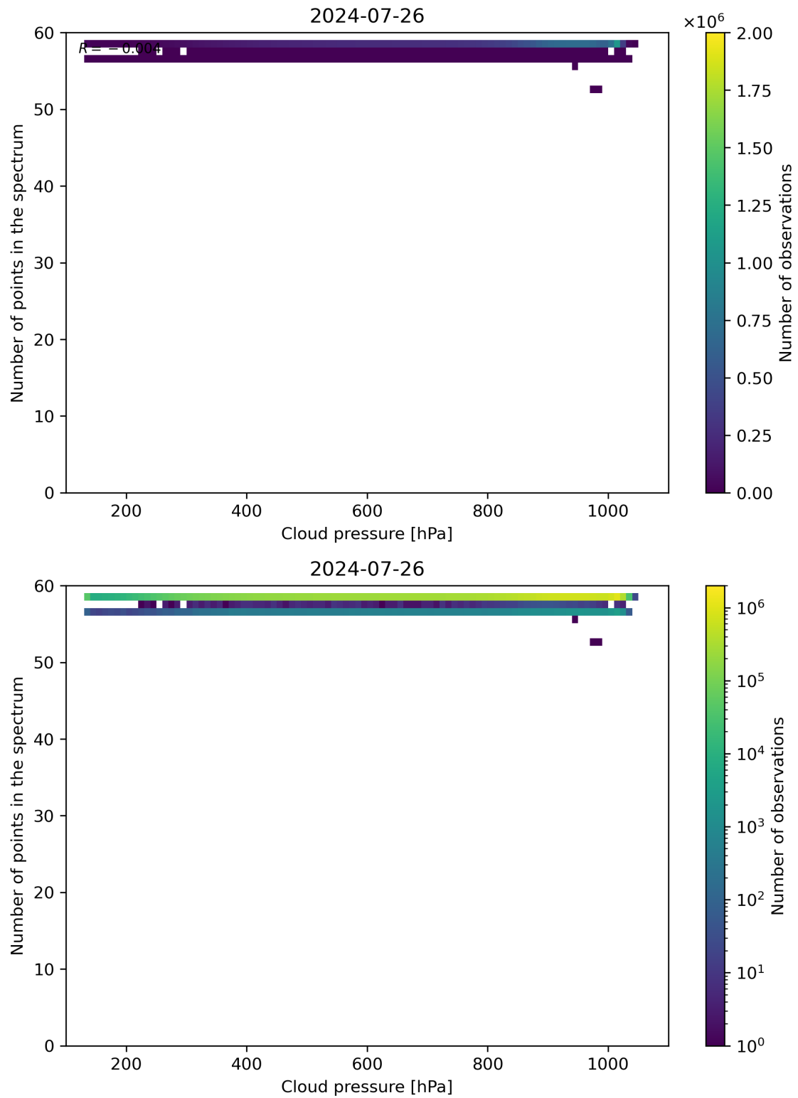
Figure 82: Scatter density plot of “Cloud pressure” against “Number of points in the spectrum” for 2024-07-26 to 2024-07-27.
