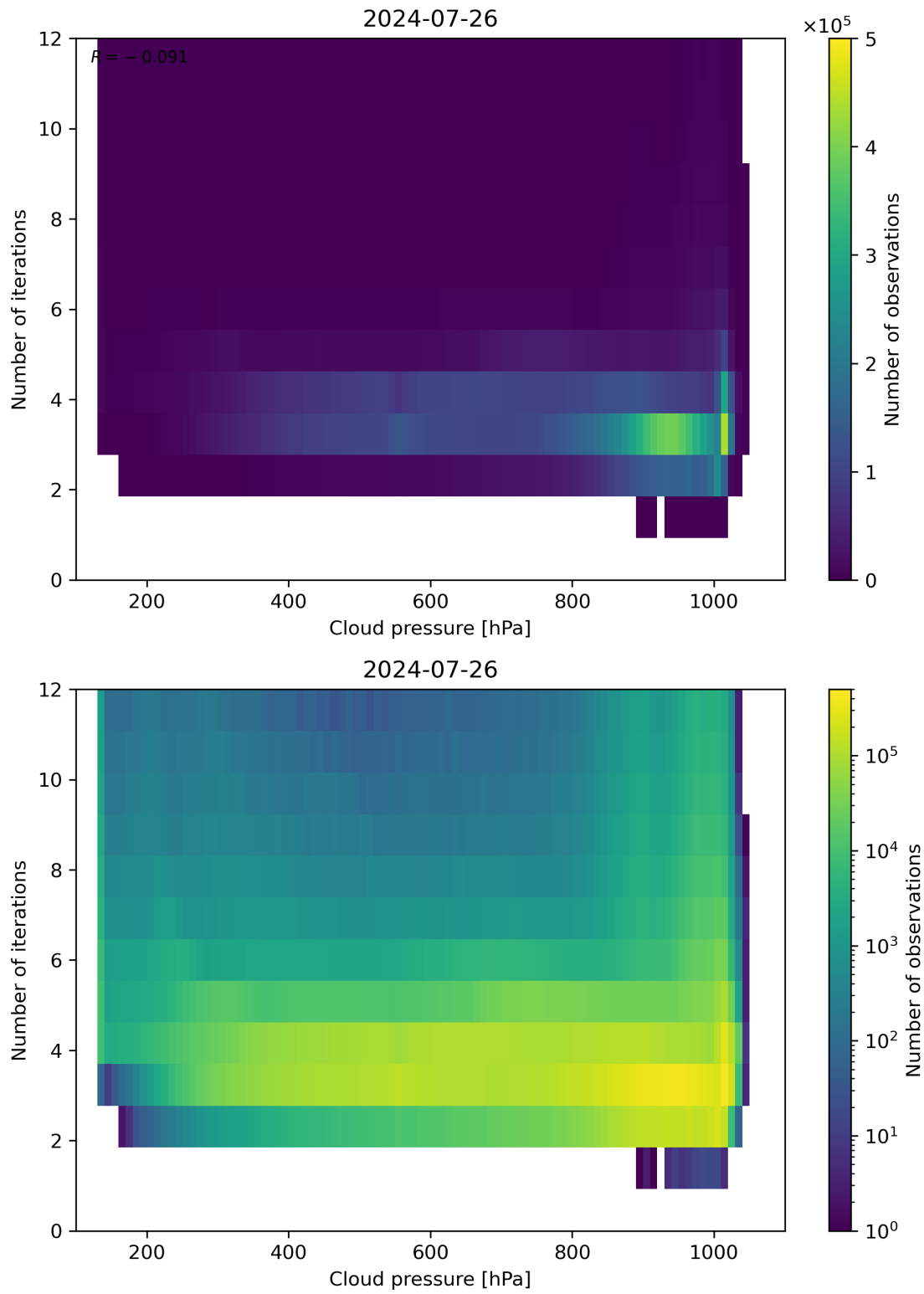
Figure 81: Scatter density plot of “Cloud pressure” against “Number of iterations” for 2024-07-26 to 2024-07-27.
