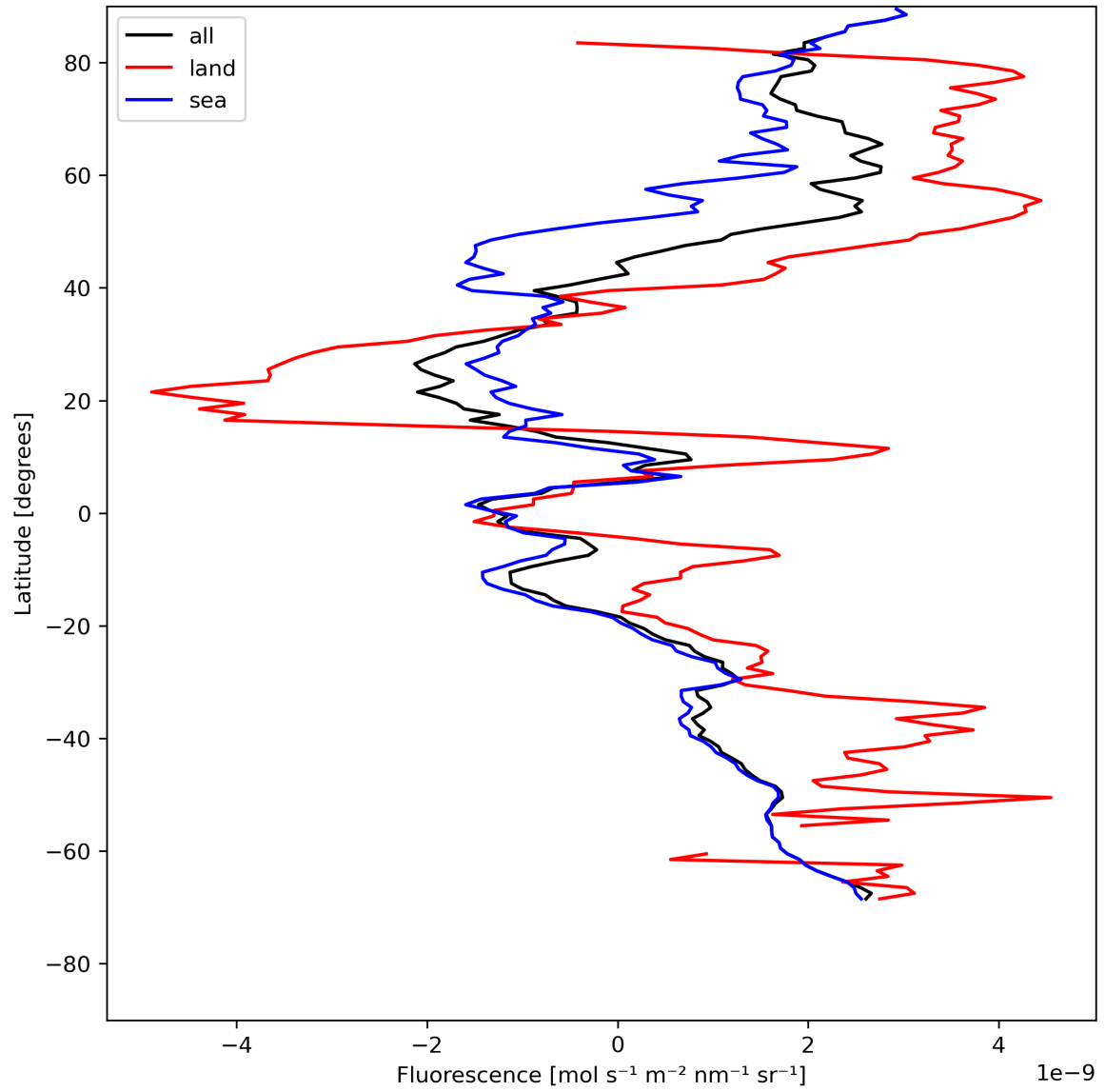
Figure 23: Zonal average of “Fluorescence” for 2024-07-26 to 2024-07-27.
