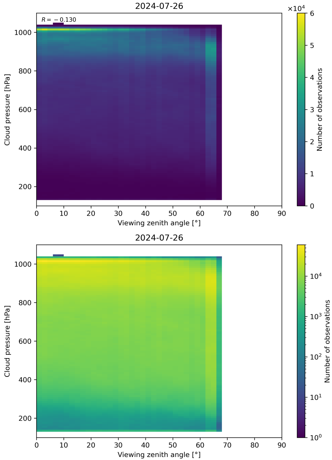
Figure 121: Scatter density plot of “Viewing zenith angle” against “Cloud pressure” for 2024-07-26 to 2024-07-27.
