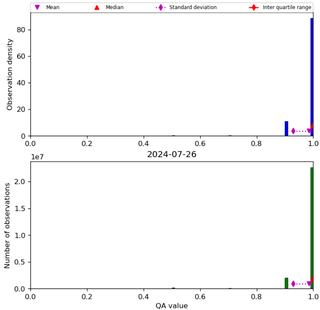
Figure 29: Histogram of “QA value” for 2024-07-26 to 2024-07-27
