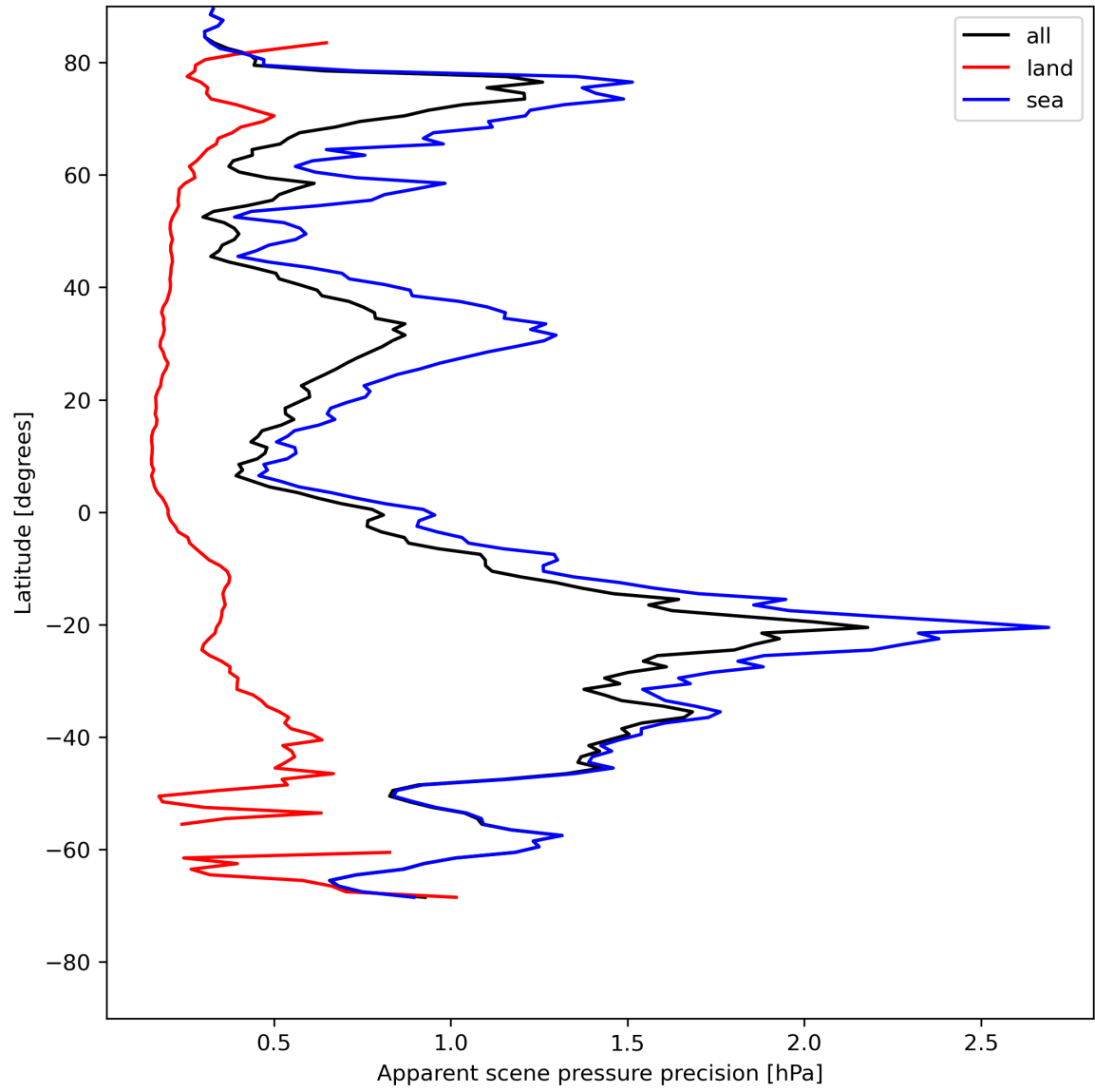
Figure 20: Zonal average of “Apparent scene pressure precision” for 2024-07-26 to 2024-07-27.
