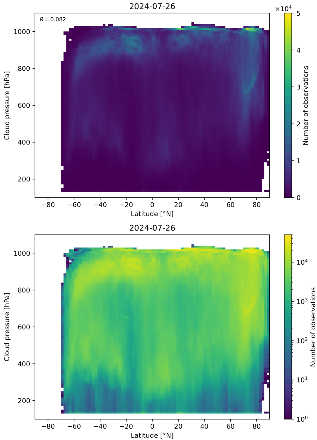
Figure 91: Scatter density plot of “Latitude” against “Cloud pressure” for 2024-07-26 to 2024-07-27.
