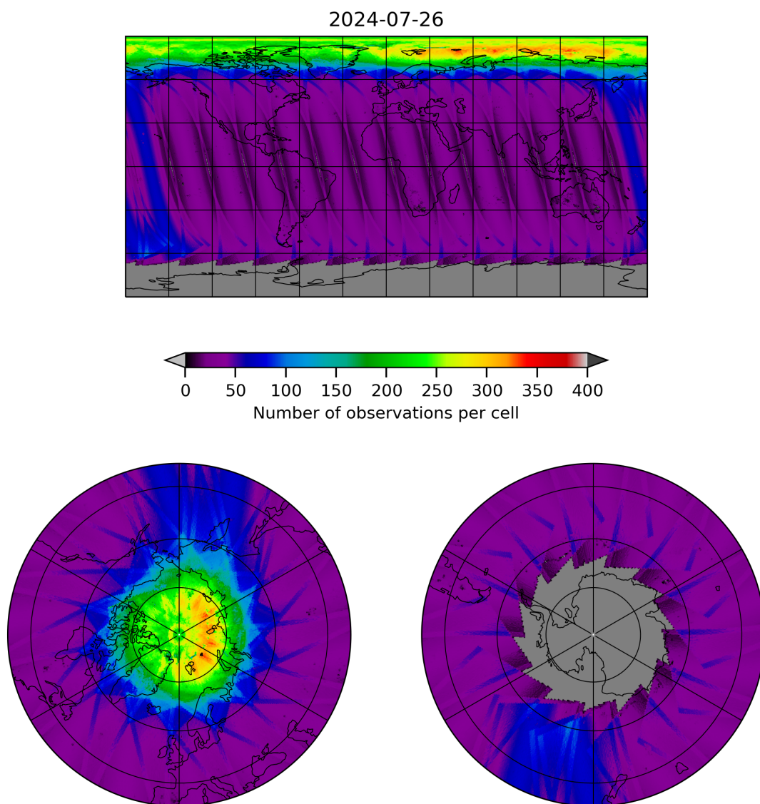
Figure 11: Map of the number of observations for 2024-07-26 to 2024-07-27
