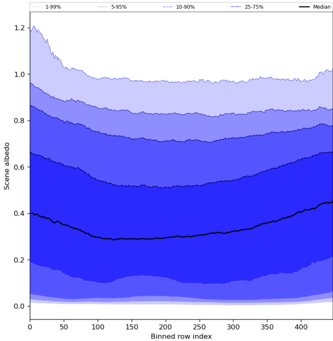
Figure 51: Along track statistics of “Scene albedo” for 2024-07-26 to 2024-07-27
