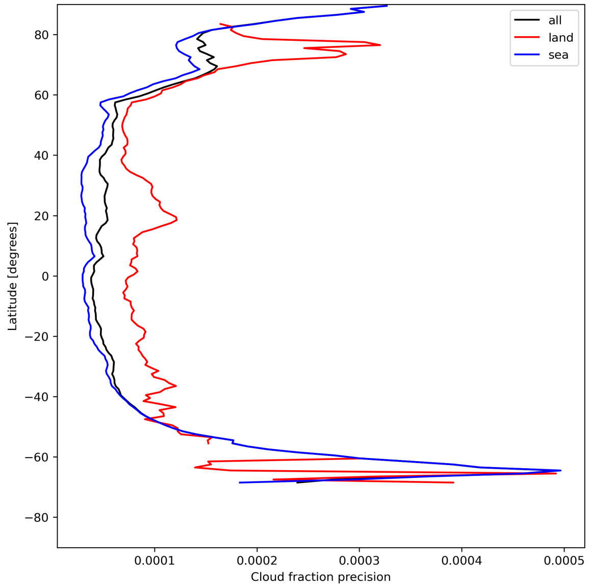
Figure 16: Zonal average of “Cloud fraction precision” for 2024-07-26 to 2024-07-27.
