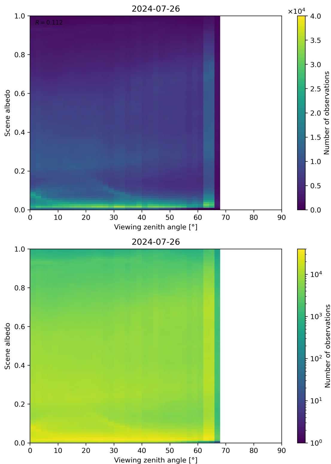
Figure 126: Scatter density plot of “Viewing zenith angle” against “Scene albedo” for 2024-07-26 to 2024-07-27.
