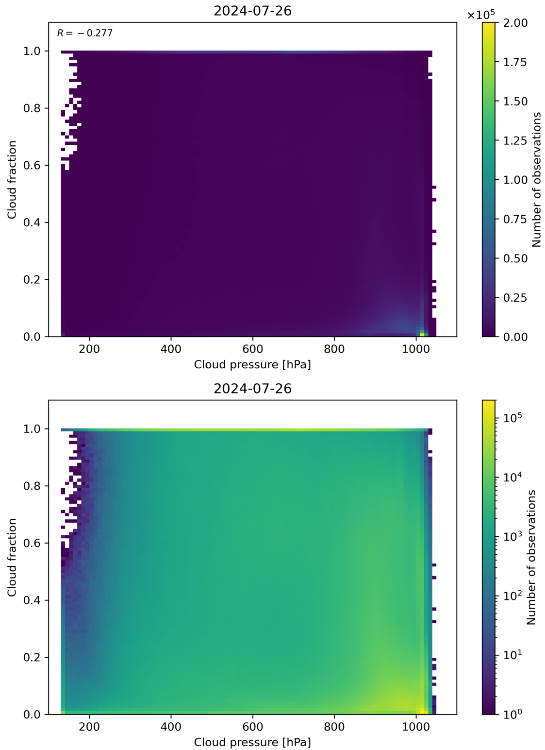
Figure 79: Scatter density plot of “Cloud pressure” against “Cloud fraction” for 2024-07-26 to 2024-07-27.
