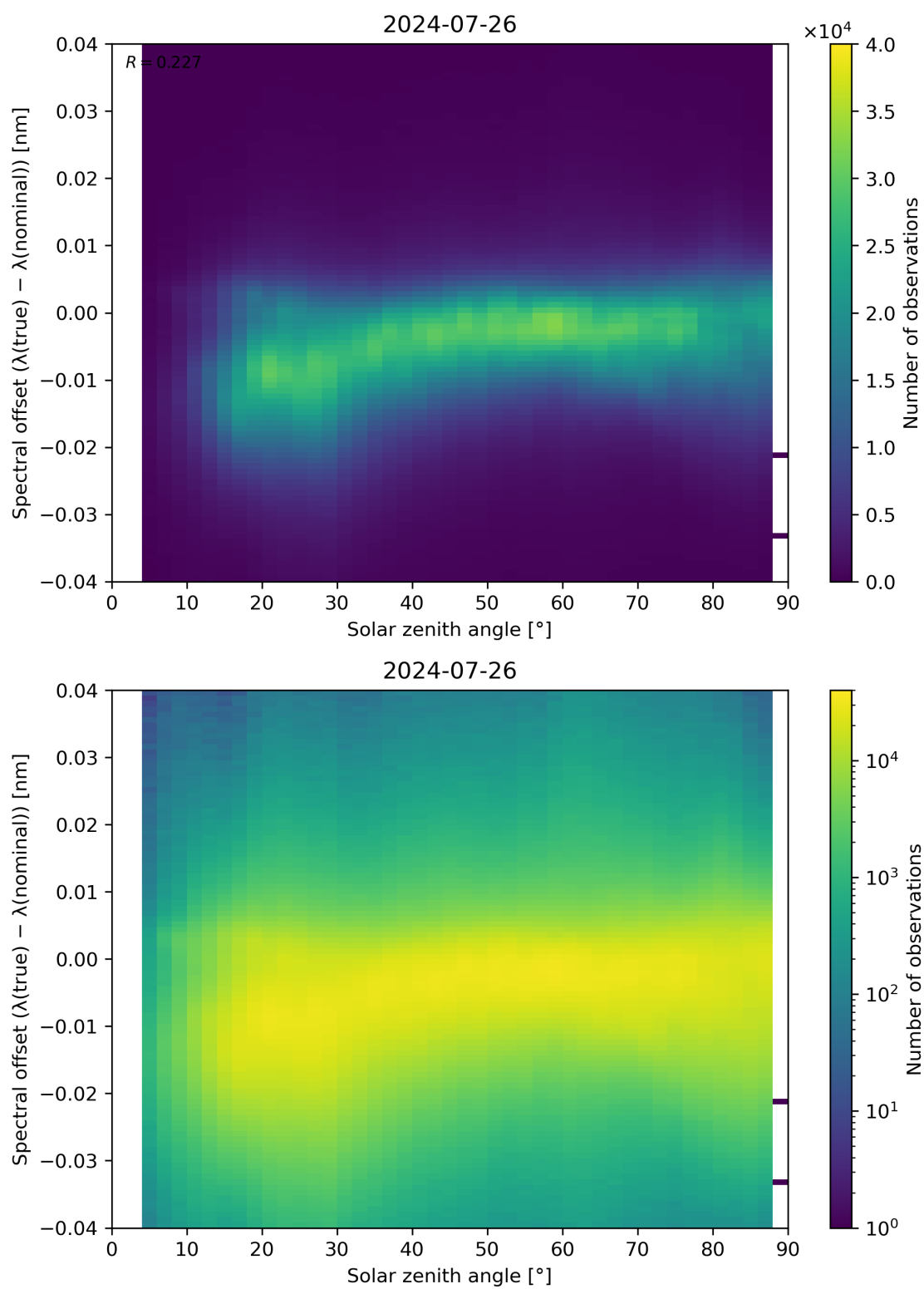
Figure 117: Scatter density plot of “Solar zenith angle” against “Spectral offset ( \lambda(\text{true}) - \lambda(\text{nominal}) )” for 2024-07-26 to 2024-07-27.
