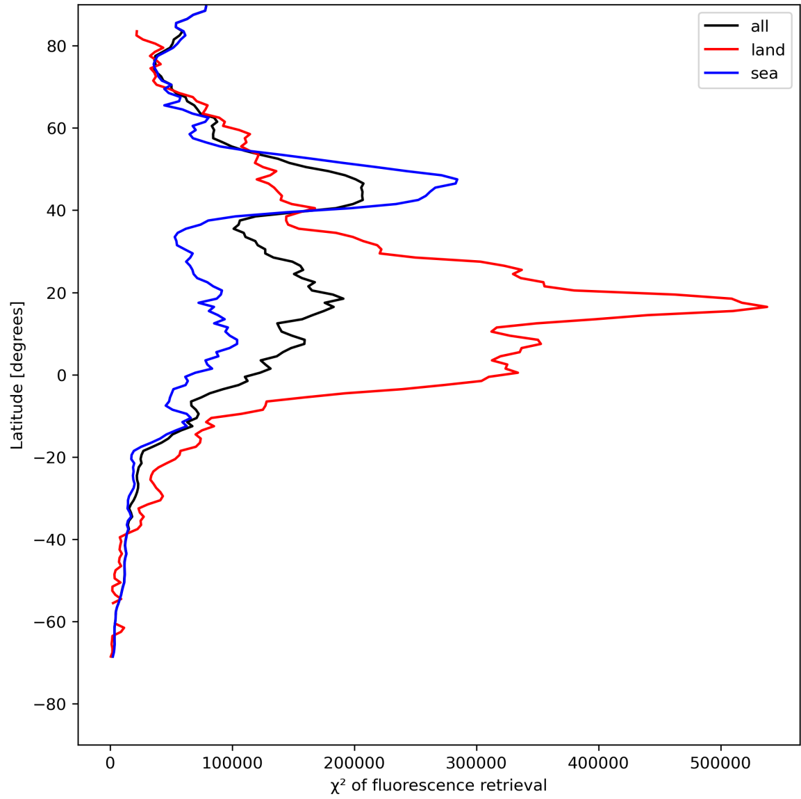
Figure 25: Zonal average of “ \chi^2 of fluorescence retrieval” for 2024-07-26 to 2024-07-27.
