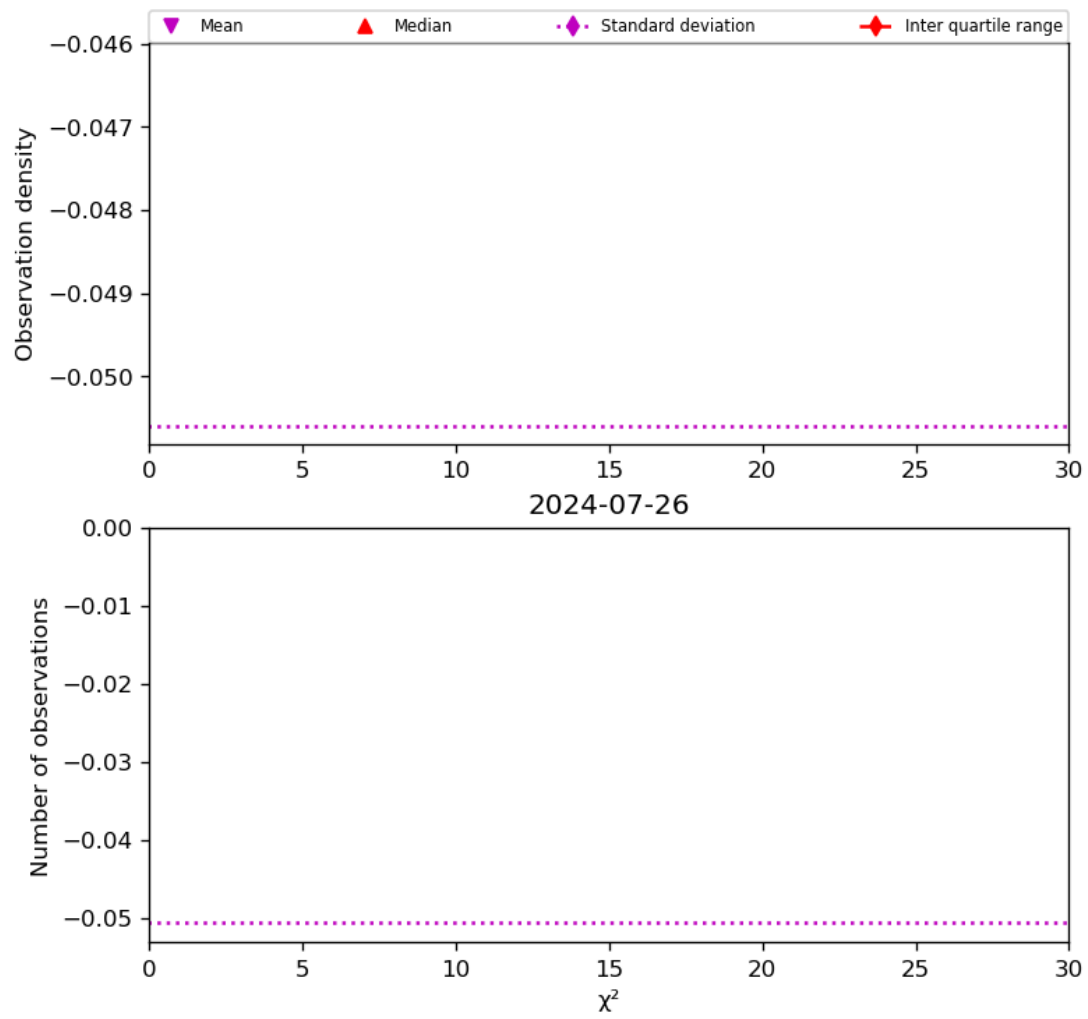
Figure 38: Histogram of “ \chi^2 ” for 2024-07-26 to 2024-07-27
