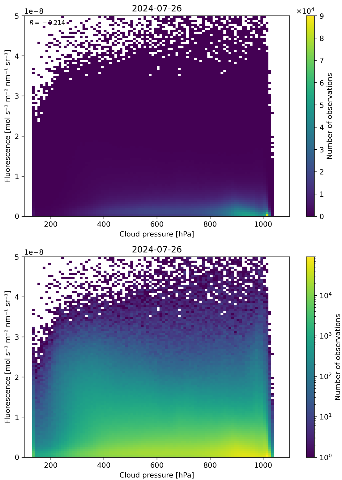
Figure 80: Scatter density plot of “Cloud pressure” against “Fluorescence” for 2024-07-26 to 2024-07-27.
