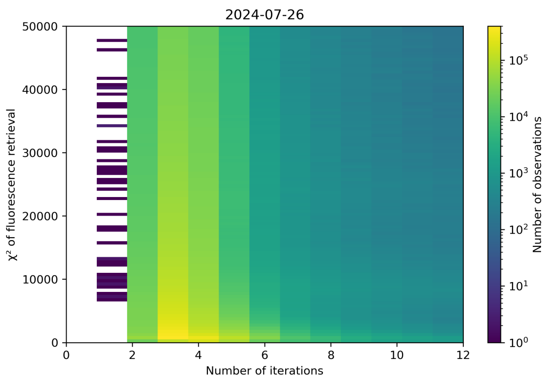
Figure 97: Scatter density plot of “Number of iterations” against “ \chi^2 of fluorescence retrieval” for 2024-07-26 to 2024-07-27.
