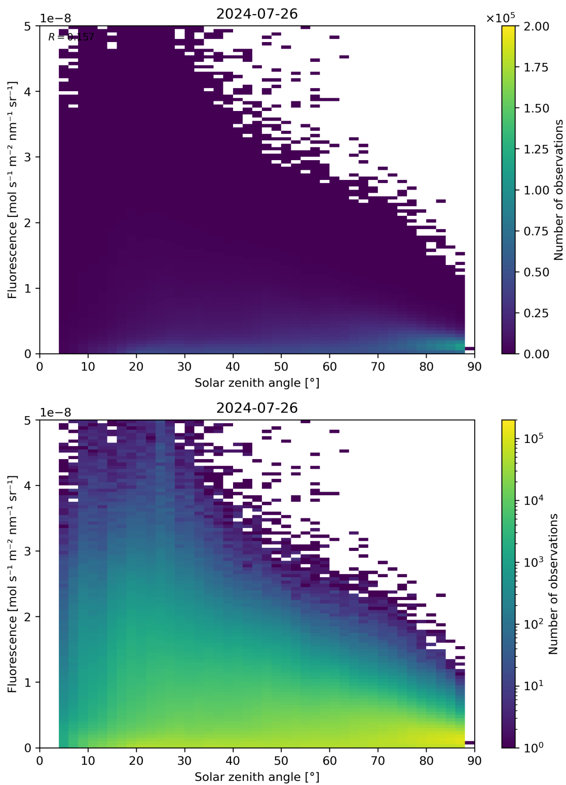
Figure 112: Scatter density plot of “Solar zenith angle” against “Fluorescence” for 2024-07-26 to 2024-07-27.
