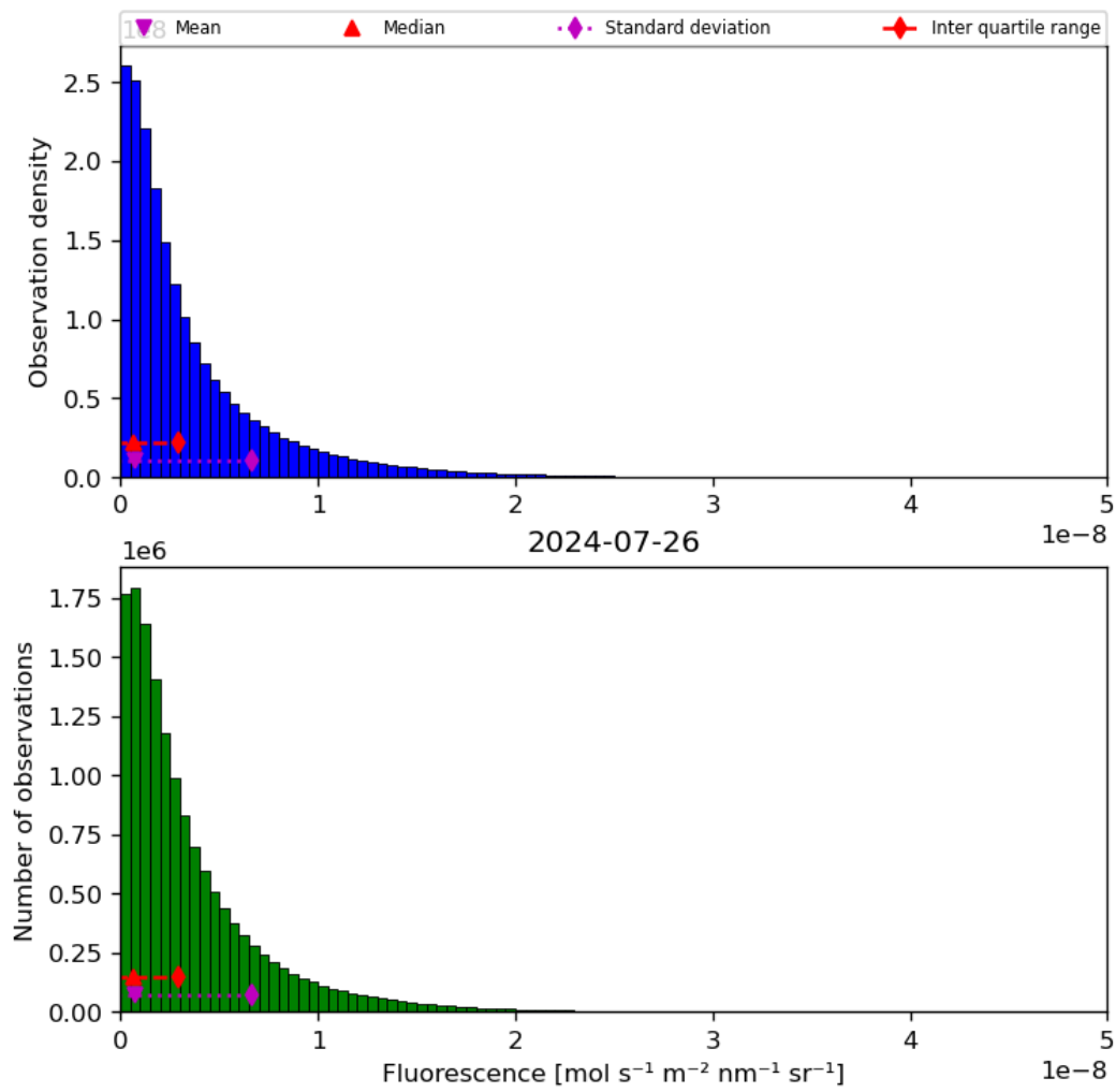
Figure 40: Histogram of “Fluorescence” for 2024-07-26 to 2024-07-27
