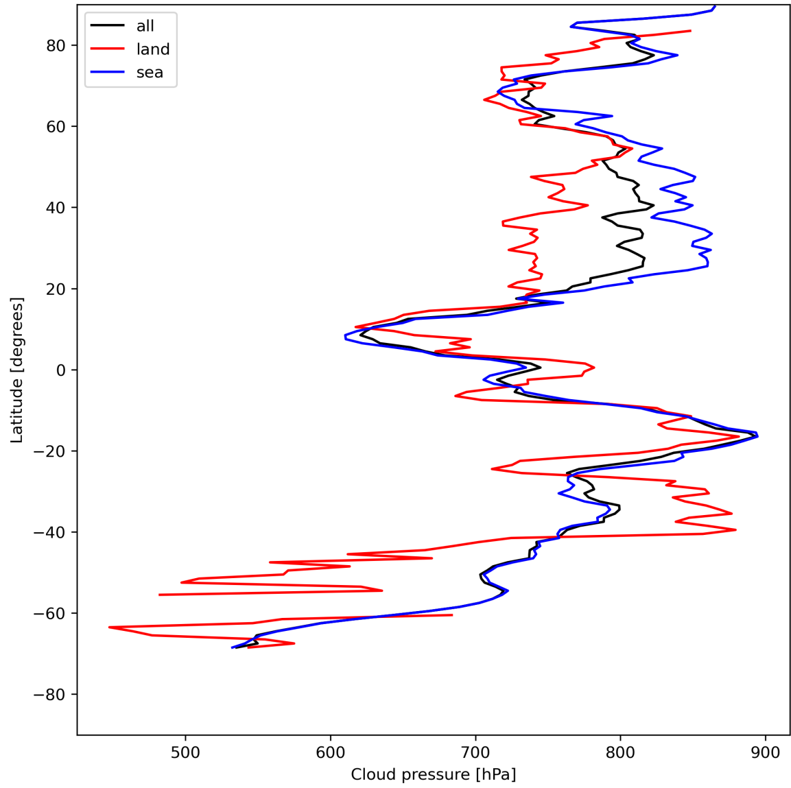
Figure 13: Zonal average of “Cloud pressure” for 2024-07-26 to 2024-07-27.
