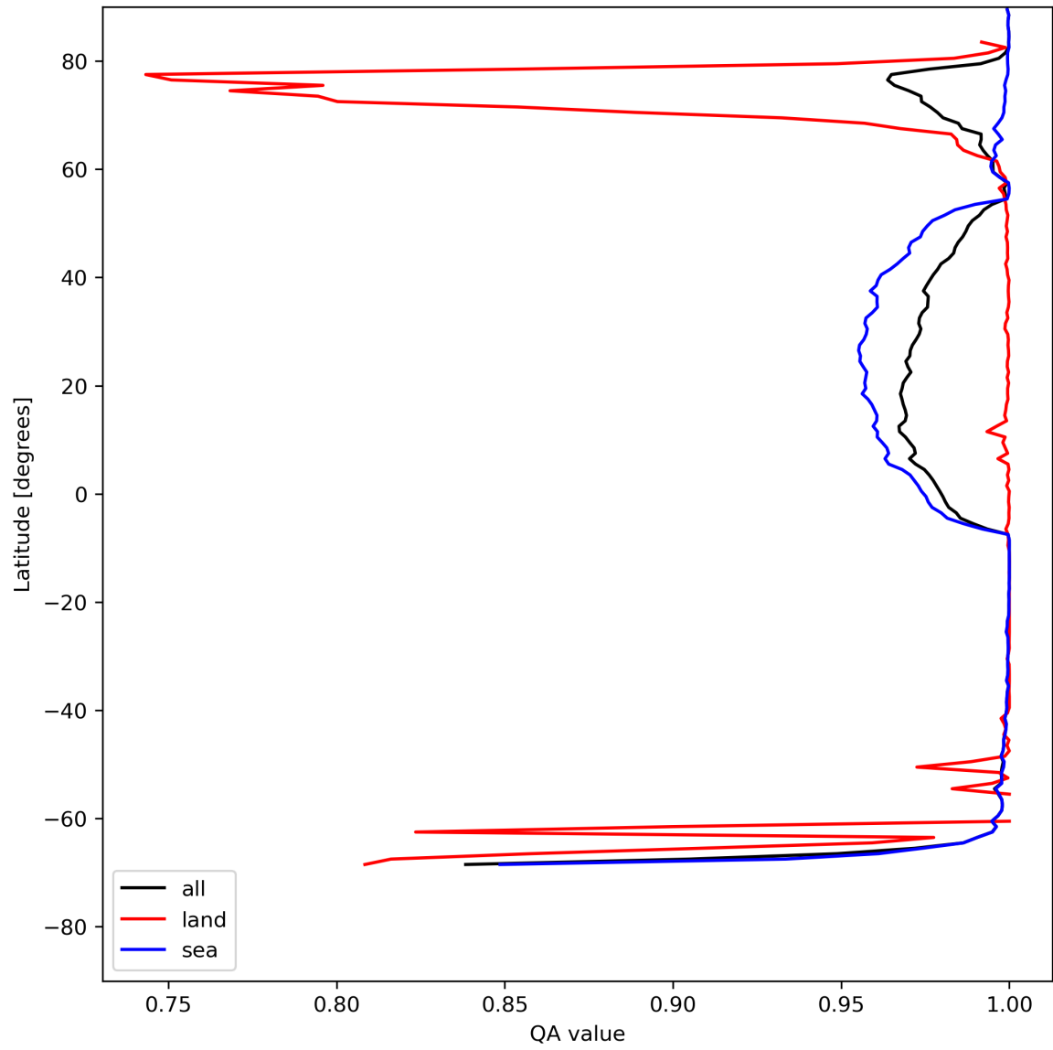
Figure 12: Zonal average of “QA value” for 2024-07-26 to 2024-07-27.
