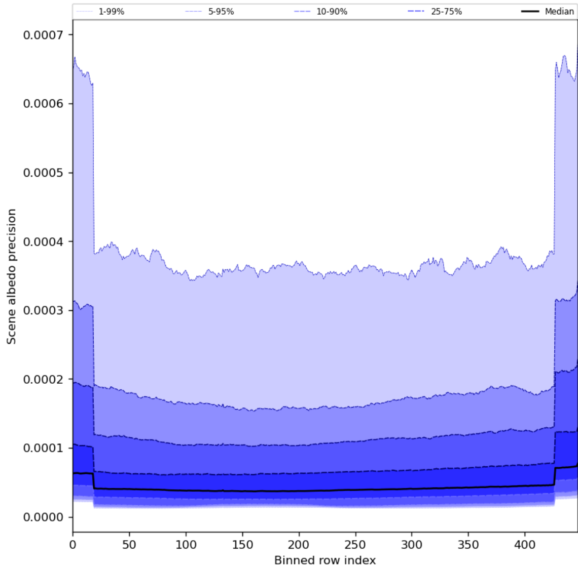
Figure 52: Along track statistics of “Scene albedo precision” for 2024-07-26 to 2024-07-27
