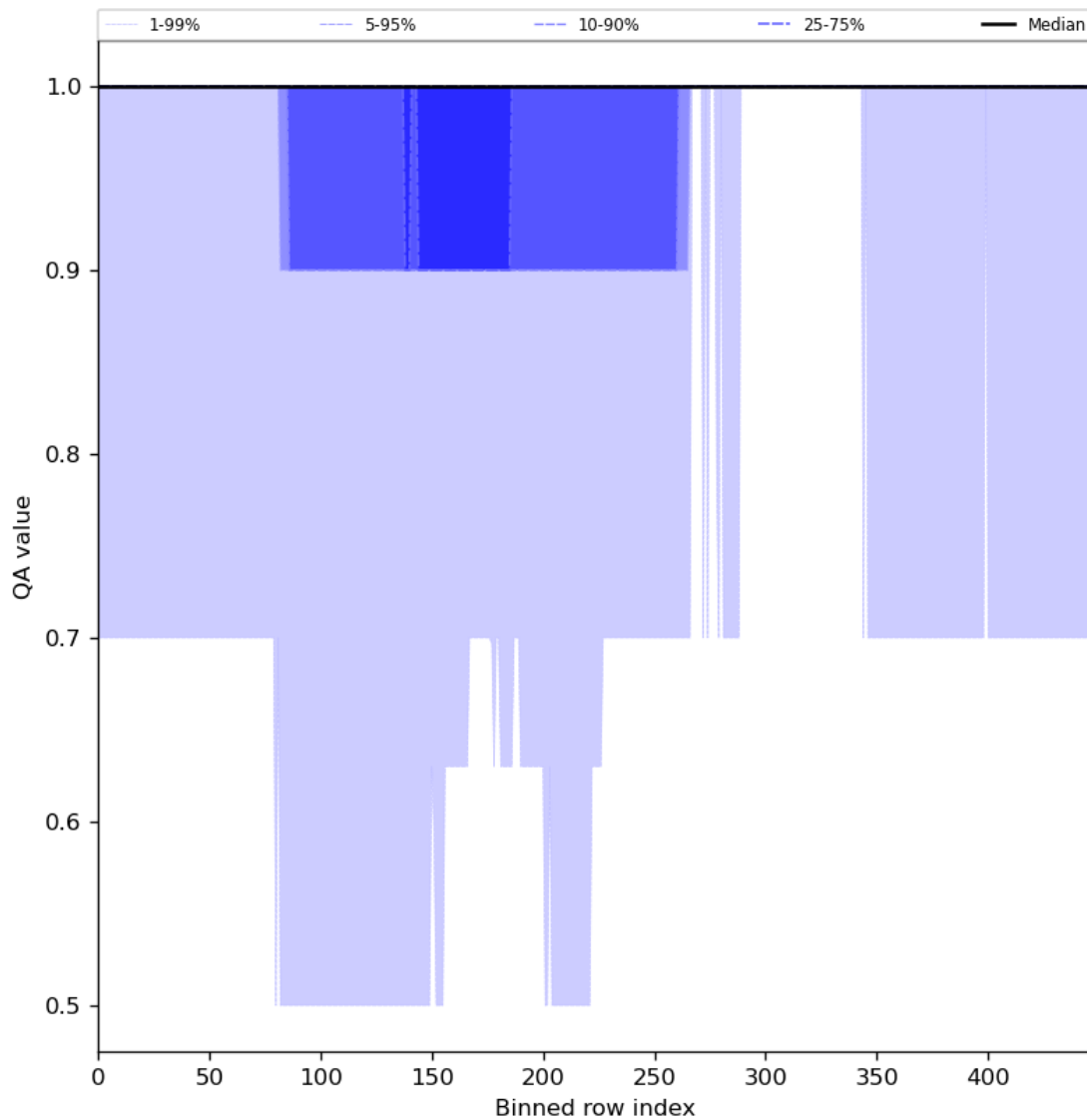
Figure 46: Along track statistics of “QA value” for 2024-07-26 to 2024-07-27
