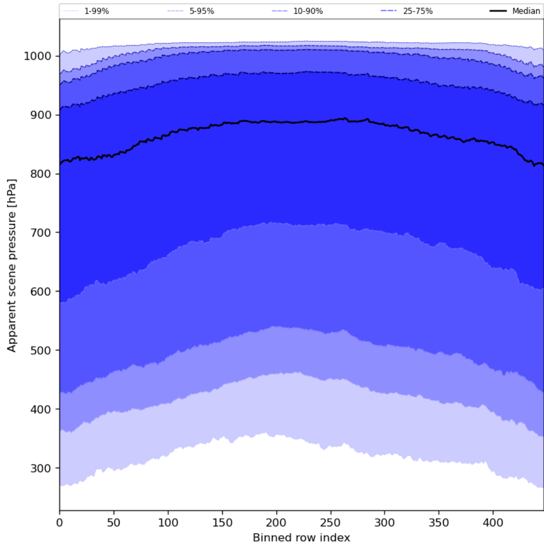
Figure 53: Along track statistics of “Apparent scene pressure” for 2024-07-26 to 2024-07-27
