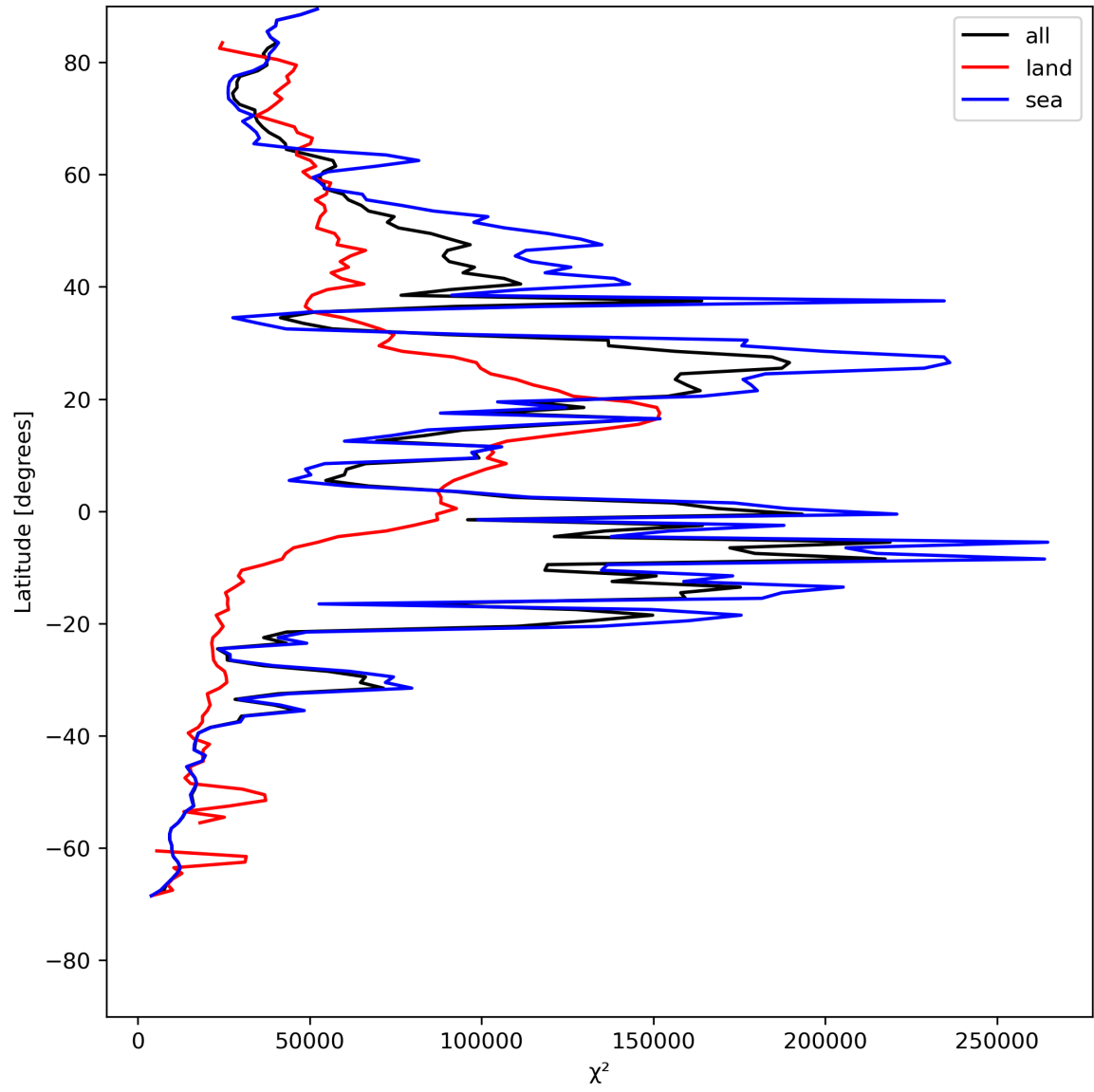
Figure 21: Zonal average of “ \chi^2 ” for 2024-07-26 to 2024-07-27.
