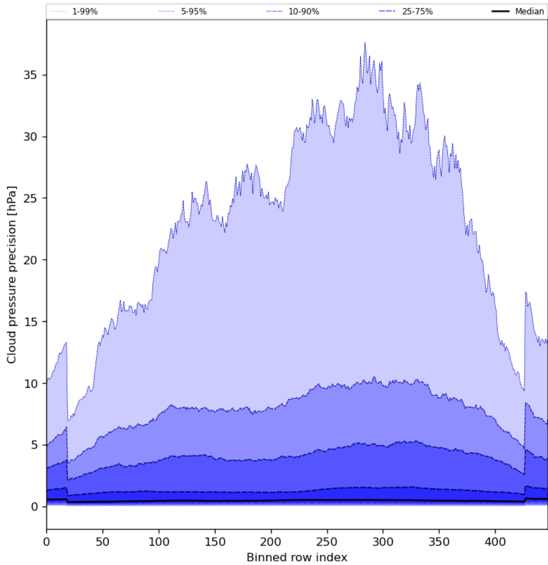
Figure 48: Along track statistics of “Cloud pressure precision” for 2024-07-26 to 2024-07-27
