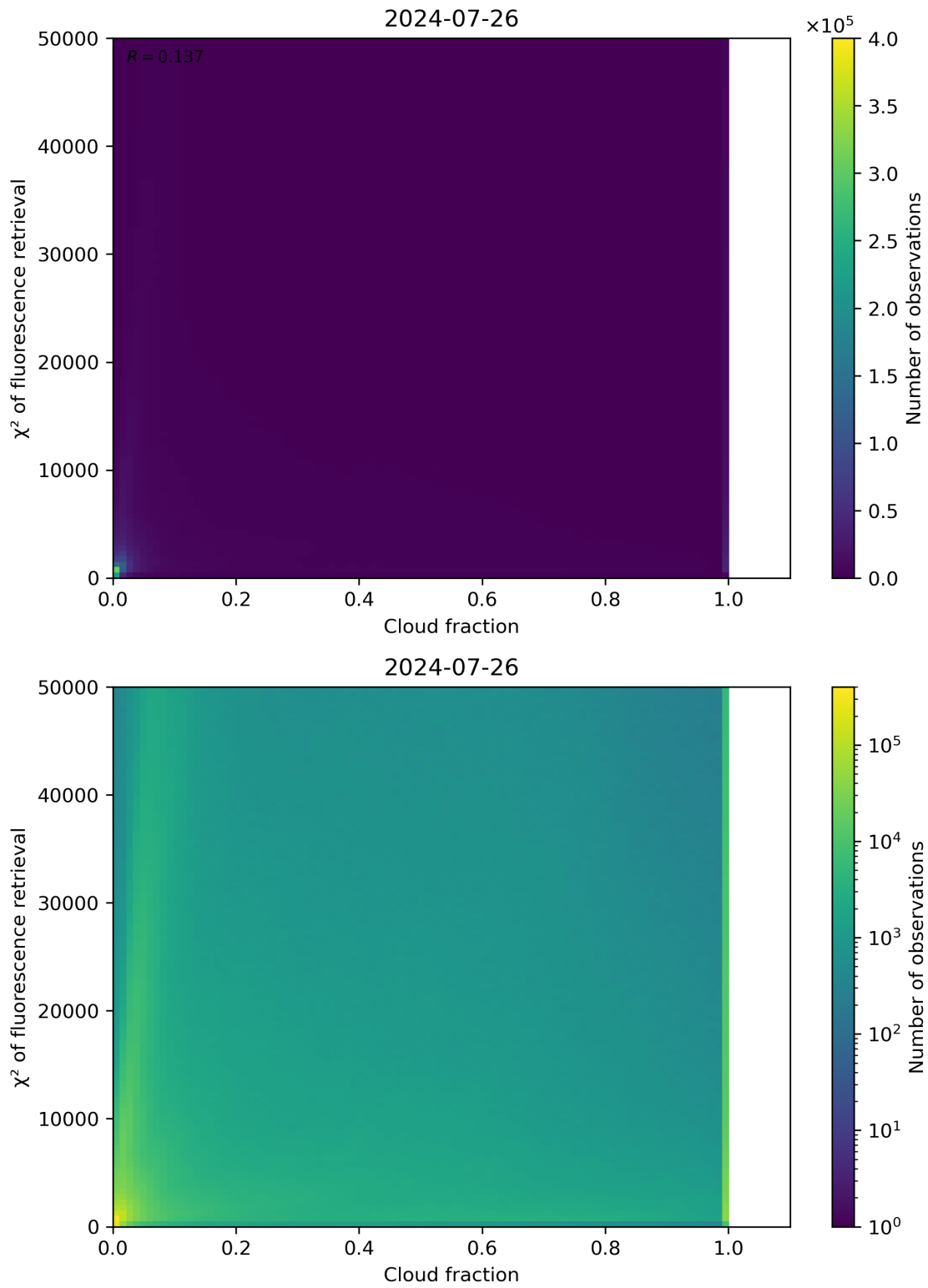
Figure 71: Scatter density plot of “Cloud fraction” against “ \chi^2 of fluorescence retrieval” for 2024-07-26 to 2024-07-27.
