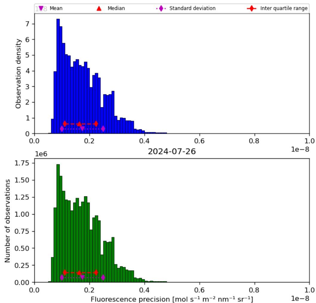
Figure 41: Histogram of “Fluorescence precision” for 2024-07-26 to 2024-07-27
