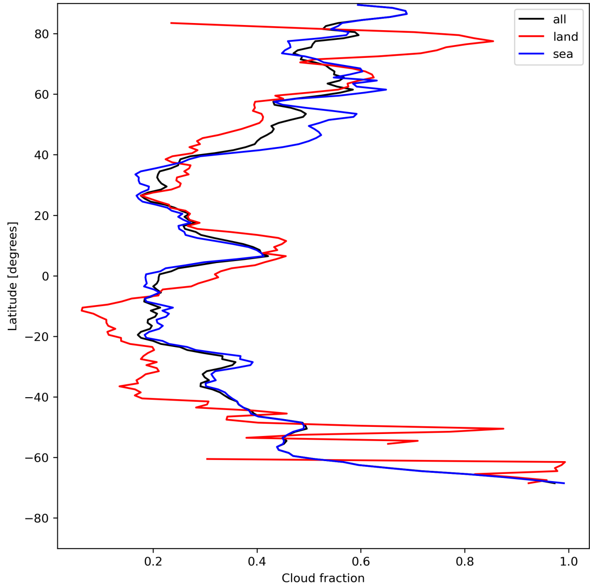
Figure 15: Zonal average of “Cloud fraction” for 2024-07-26 to 2024-07-27.
