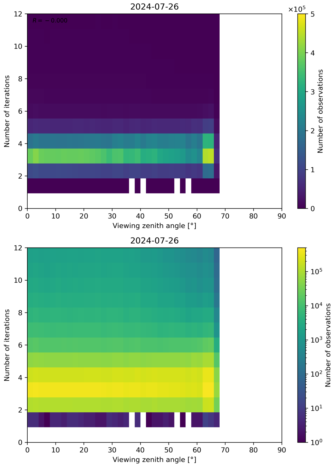
Figure 124: Scatter density plot of “Viewing zenith angle” against “Number of iterations” for 2024-07-26 to 2024-07-27.
