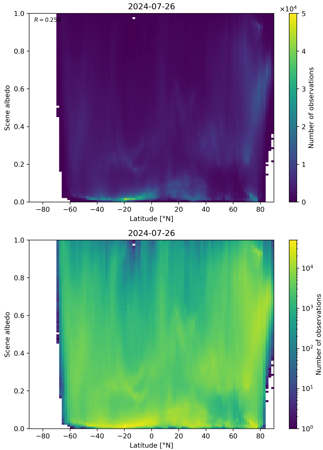
Figure 95: Scatter density plot of “Latitude” against “Scene albedo” for 2024-07-26 to 2024-07-27.
