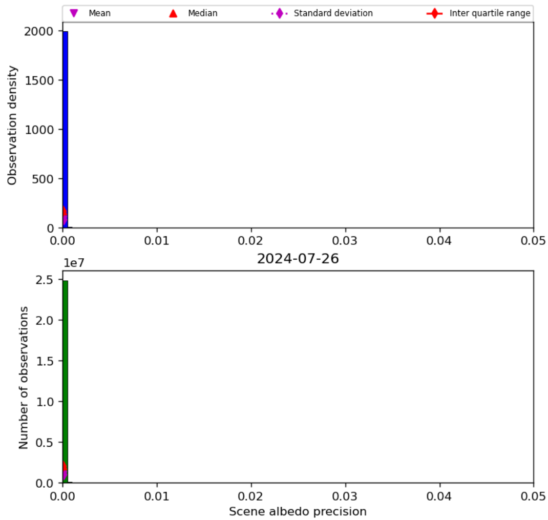
Figure 35: Histogram of “Scene albedo precision” for 2024-07-26 to 2024-07-27
