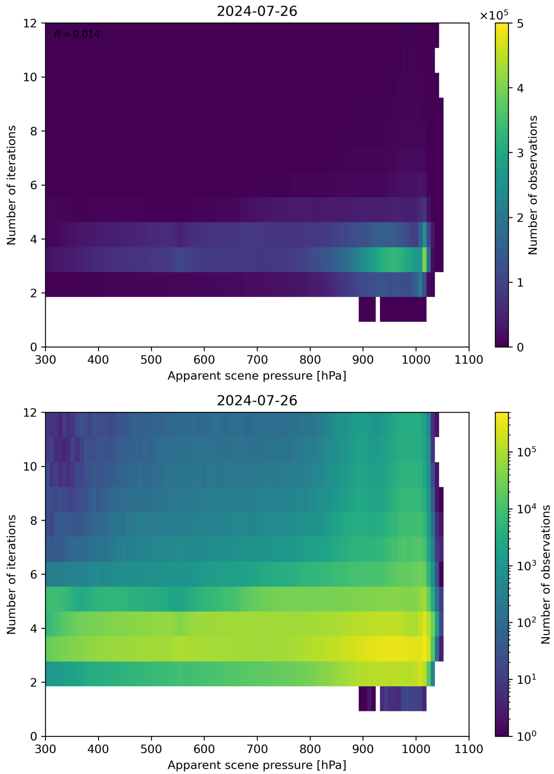
Figure 65: Scatter density plot of “Apparent scene pressure” against “Number of iterations” for 2024-07-26 to 2024-07-27.
