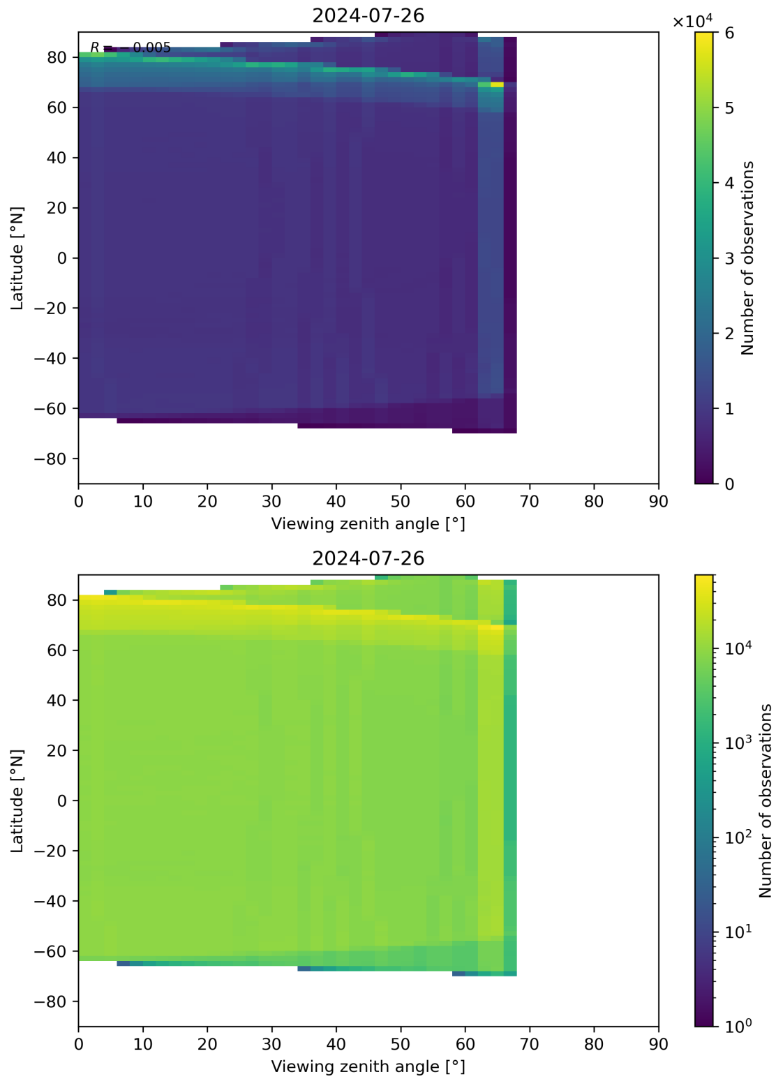
Figure 123: Scatter density plot of “Viewing zenith angle” against “Latitude” for 2024-07-26 to 2024-07-27.
