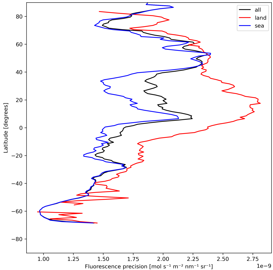
Figure 24: Zonal average of “Fluorescence precision” for 2024-07-26 to 2024-07-27.
