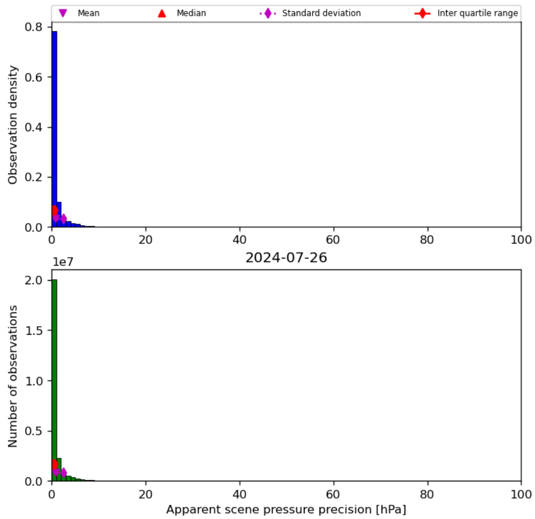
Figure 37: Histogram of “Apparent scene pressure precision” for 2024-07-26 to 2024-07-27
