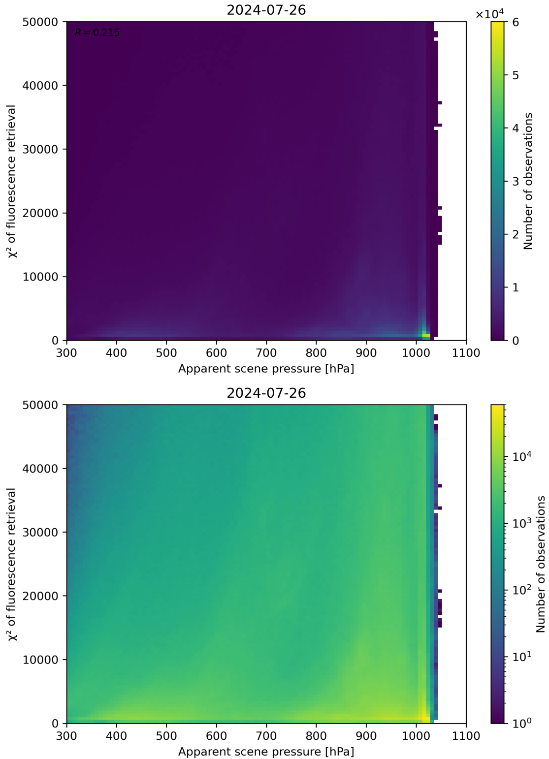
Figure 63: Scatter density plot of “Apparent scene pressure” against “ \chi^2 of fluorescence retrieval” for 2024-07-26 to 2024-07-27.
