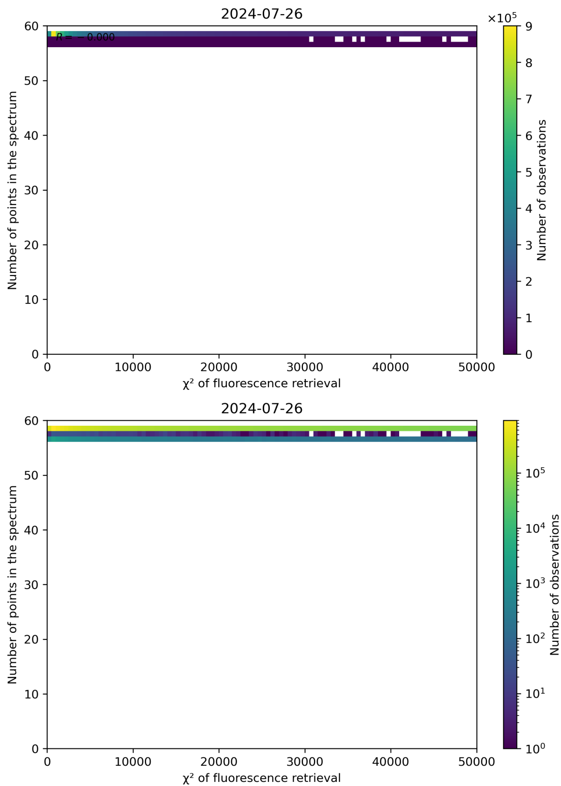
Figure 68: Scatter density plot of “ \chi^2 of fluorescence retrieval” against “Number of points in the spectrum” for 2024-07-26 to 2024-07-27.
