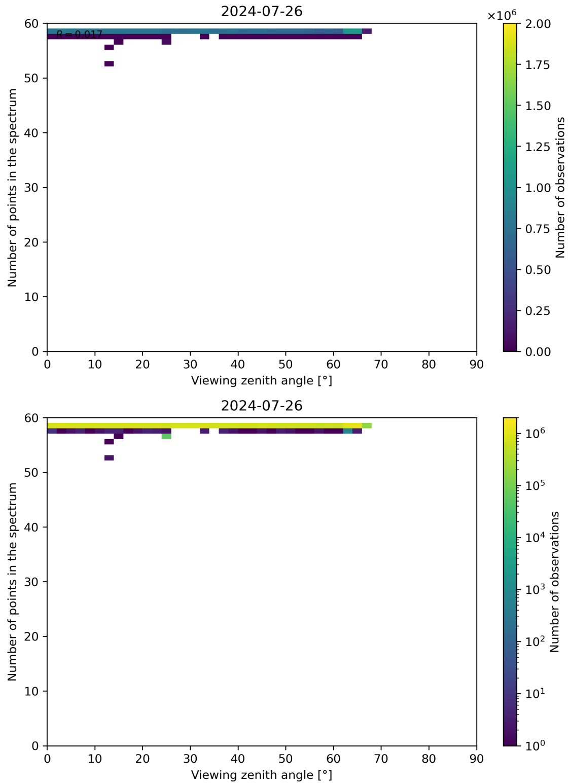
Figure 125: Scatter density plot of “Viewing zenith angle” against “Number of points in the spectrum” for 2024-07-26 to 2024-07-27.
