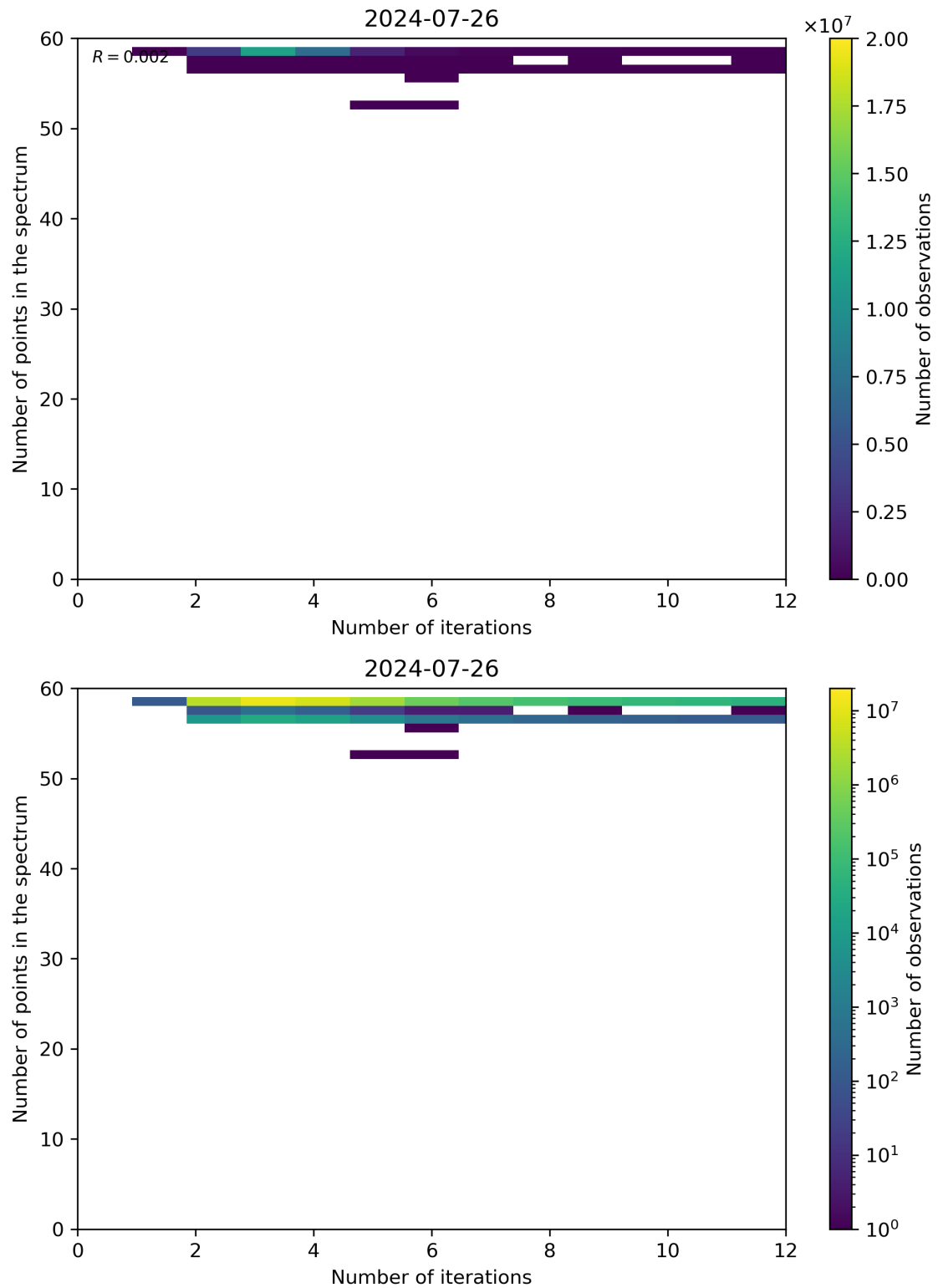
Figure 99: Scatter density plot of “Number of iterations” against “Number of points in the spectrum” for 2024-07-26 to 2024-07-27.
