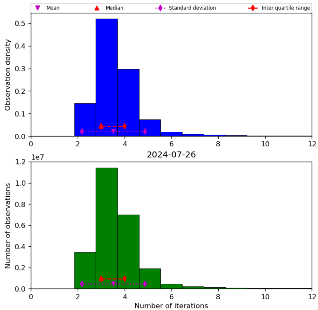
Figure 39: Histogram of “Number of iterations” for 2024-07-26 to 2024-07-27
