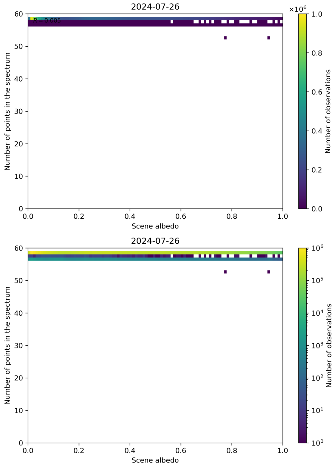
Figure 106: Scatter density plot of “Scene albedo” against “Number of points in the spectrum” for 2024-07-26 to 2024-07-27.
