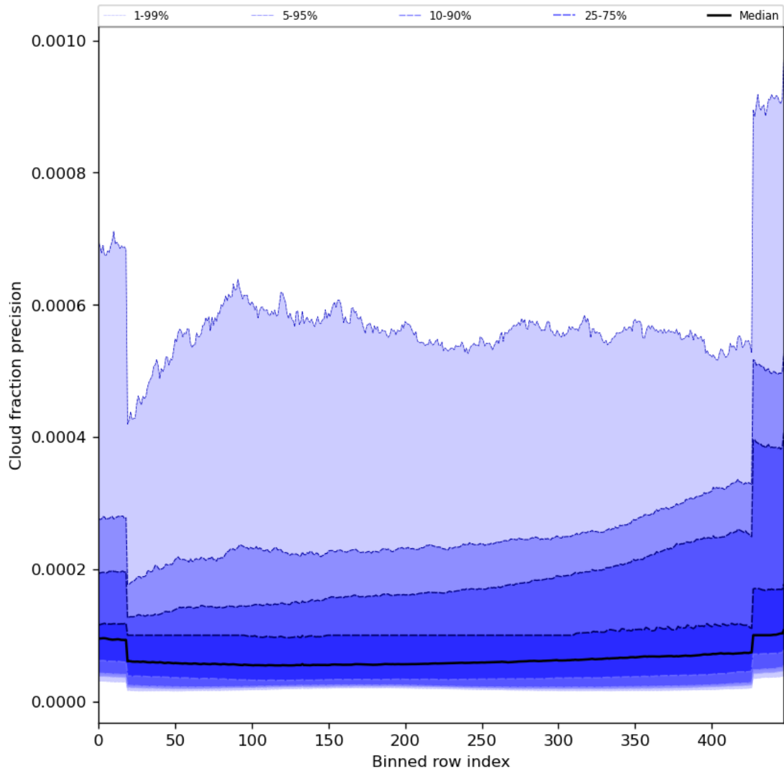
Figure 50: Along track statistics of “Cloud fraction precision” for 2024-07-26 to 2024-07-27
