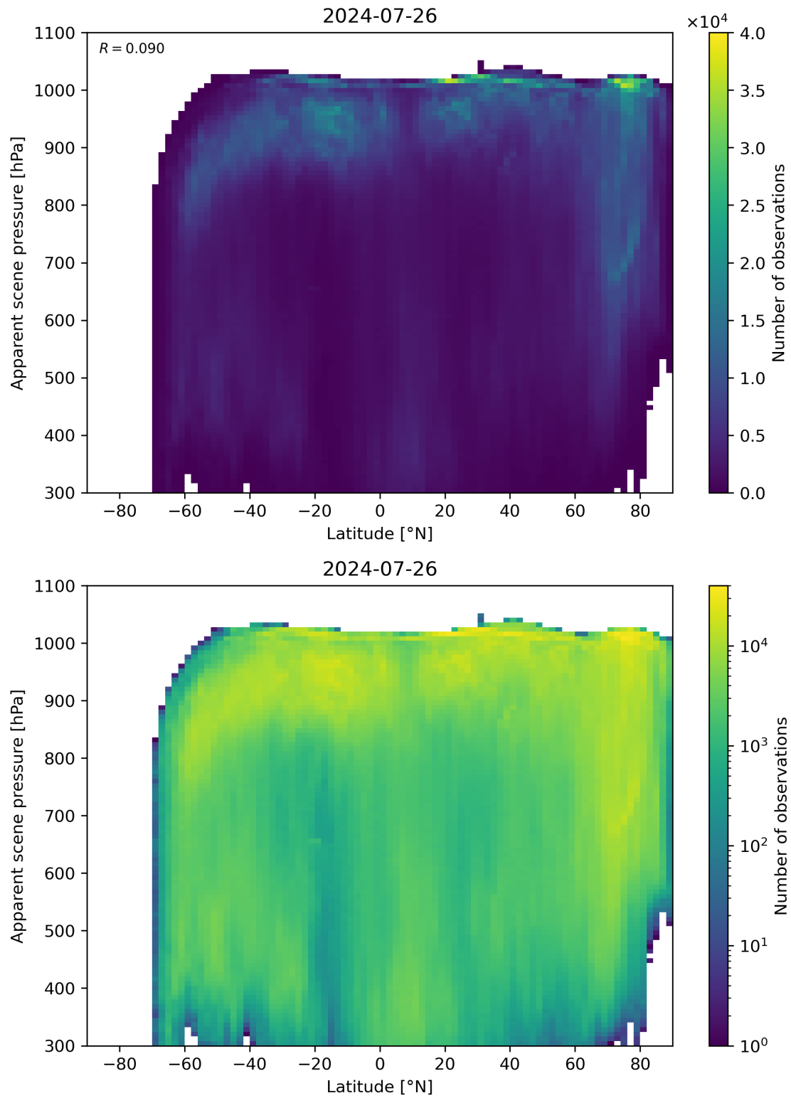
Figure 88: Scatter density plot of “Latitude” against “Apparent scene pressure” for 2024-07-26 to 2024-07-27.
