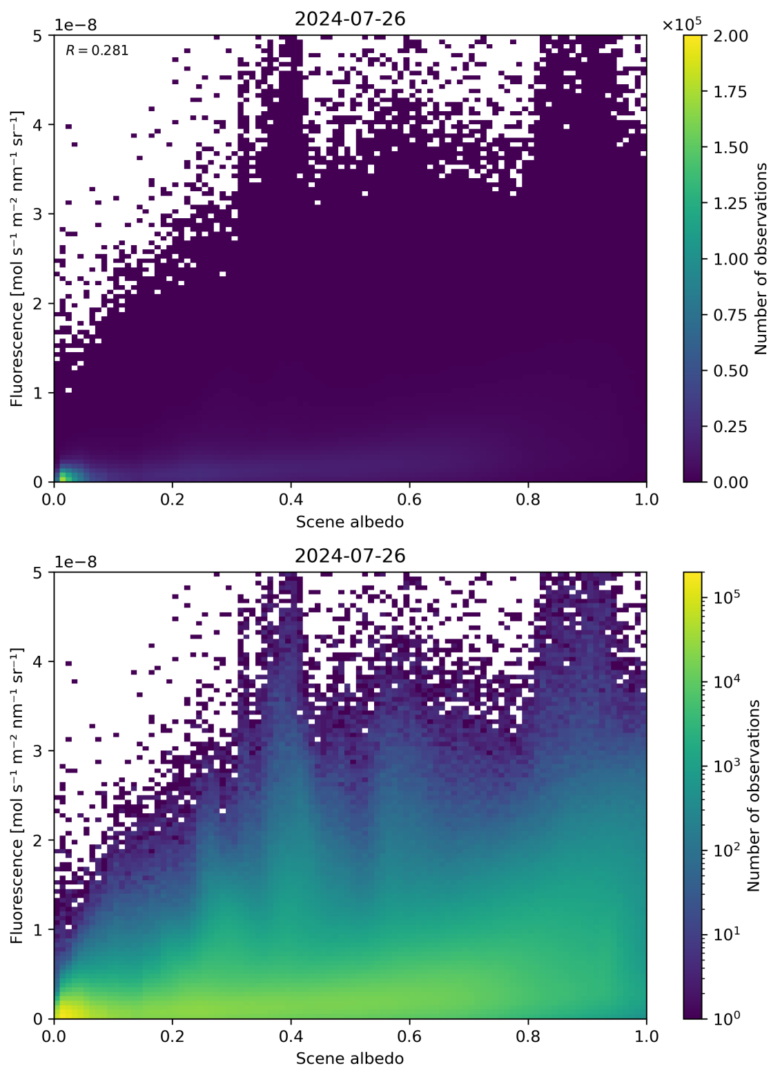
Figure 104: Scatter density plot of “Scene albedo” against “Fluorescence” for 2024-07-26 to 2024-07-27.
