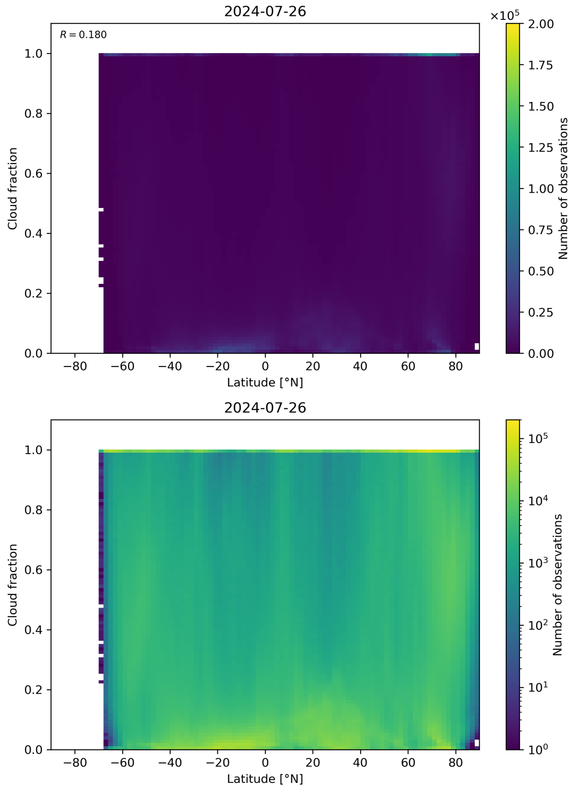
Figure 90: Scatter density plot of “Latitude” against “Cloud fraction” for 2024-07-26 to 2024-07-27.
