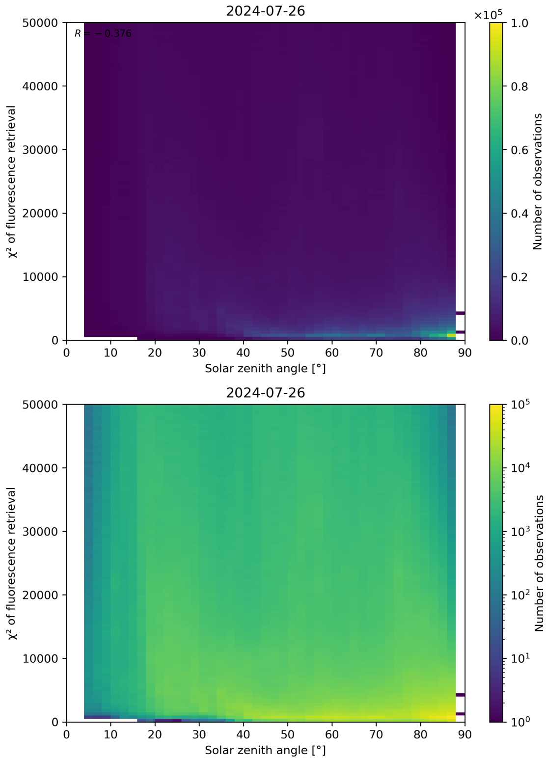
Figure 109: Scatter density plot of “Solar zenith angle” against “ \chi^2 of fluorescence retrieval” for 2024-07-26 to 2024-07-27.
