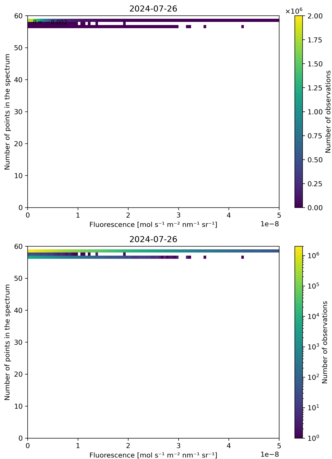
Figure 86: Scatter density plot of “Fluorescence” against “Number of points in the spectrum” for 2024-07-26 to 2024-07-27.
