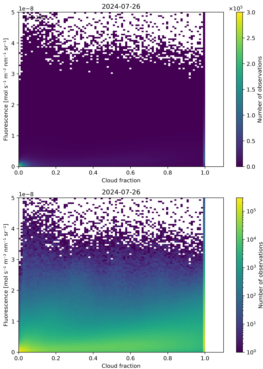
Figure 72: Scatter density plot of “Cloud fraction” against “Fluorescence” for 2024-07-26 to 2024-07-27.
