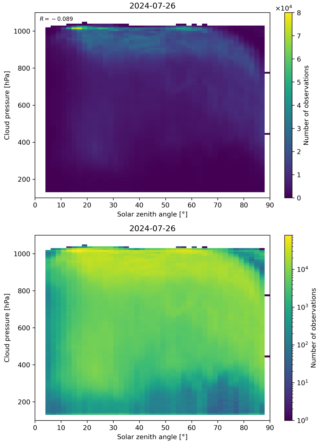
Figure 111: Scatter density plot of “Solar zenith angle” against “Cloud pressure” for 2024-07-26 to 2024-07-27.
