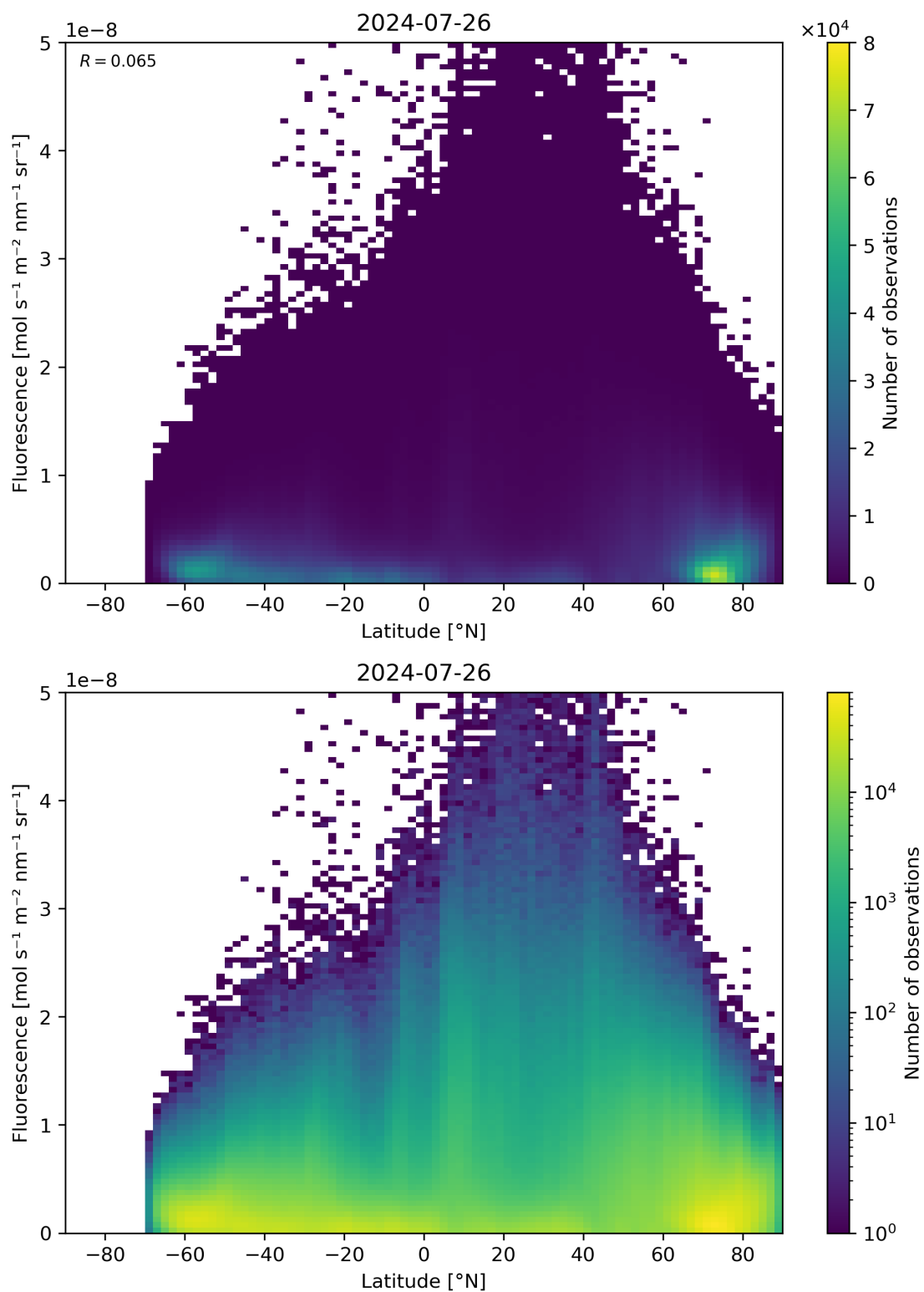
Figure 92: Scatter density plot of “Latitude” against “Fluorescence” for 2024-07-26 to 2024-07-27.
