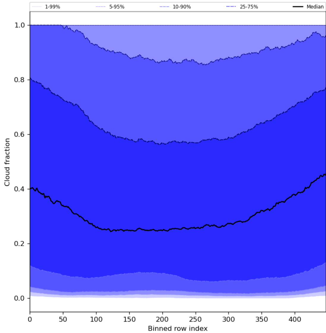
Figure 49: Along track statistics of “Cloud fraction” for 2024-07-26 to 2024-07-27
