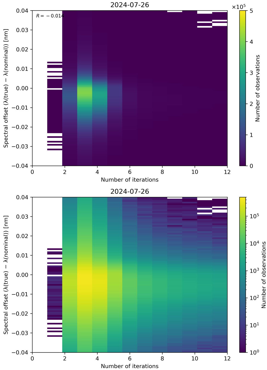
Figure 100: Scatter density plot of “Number of iterations” against “Spectral offset ( \lambda(\text{true}) - \lambda(\text{nominal}) )” for 2024-07-26 to 2024-07-27.
