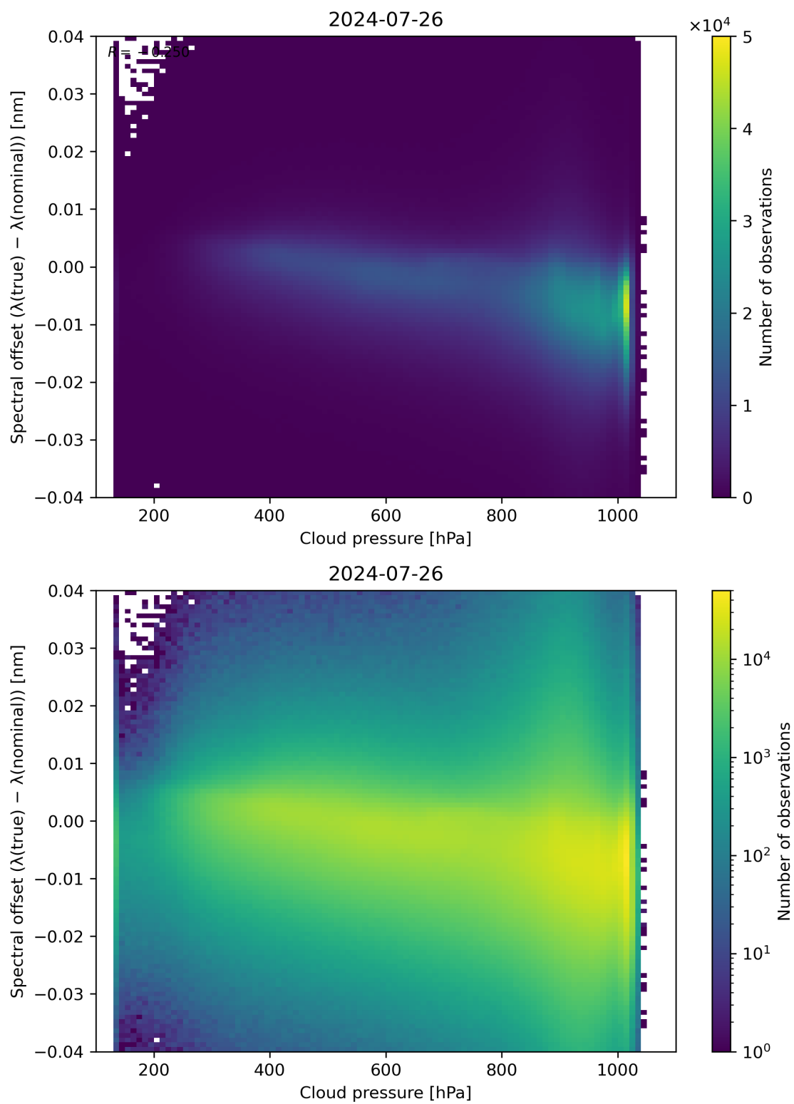
Figure 84: Scatter density plot of “Cloud pressure” against “Spectral offset ( \lambda(\text{true}) - \lambda(\text{nominal}) )” for 2024-07-26 to 2024-07-27.
