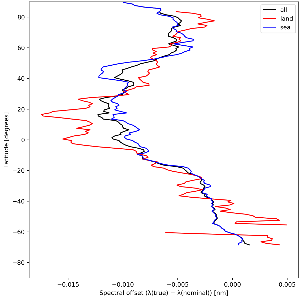
Figure 28: Zonal average of “Spectral offset ( \lambda(\text{true}) - \lambda(\text{nominal}) )” for 2024-07-26 to 2024-07-27.
