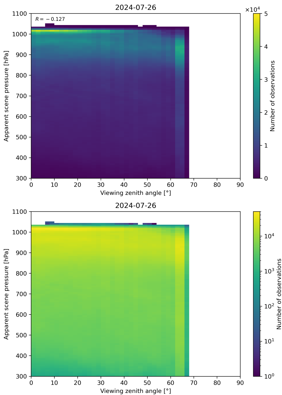
Figure 118: Scatter density plot of “Viewing zenith angle” against “Apparent scene pressure” for 2024-07-26 to 2024-07-27.
