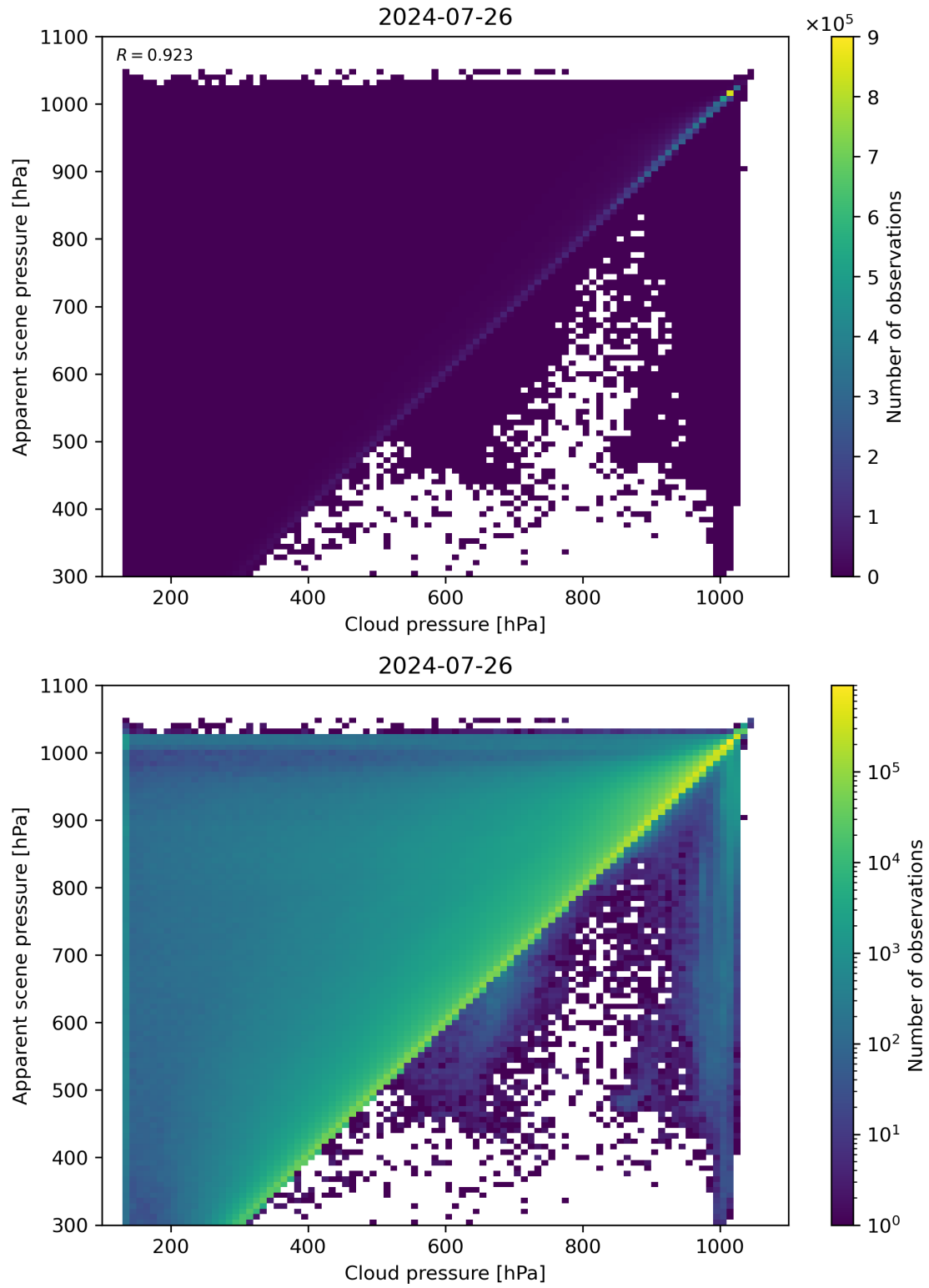
Figure 77: Scatter density plot of “Cloud pressure” against “Apparent scene pressure” for 2024-07-26 to 2024-07-27.
