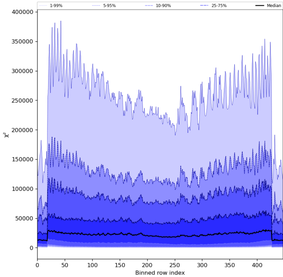
Figure 55: Along track statistics of “ \chi^2 ” for 2024-07-26 to 2024-07-27
