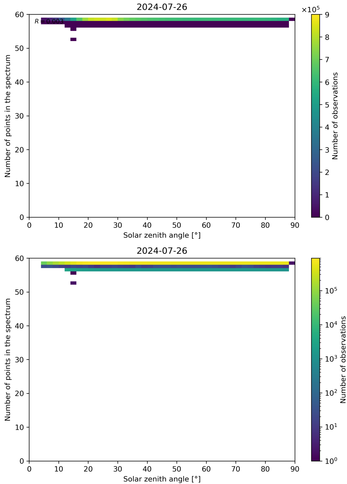
Figure 115: Scatter density plot of “Solar zenith angle” against “Number of points in the spectrum” for 2024-07-26 to 2024-07-27.
