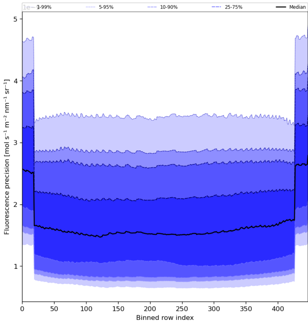
Figure 58: Along track statistics of “Fluorescence precision” for 2024-07-26 to 2024-07-27
