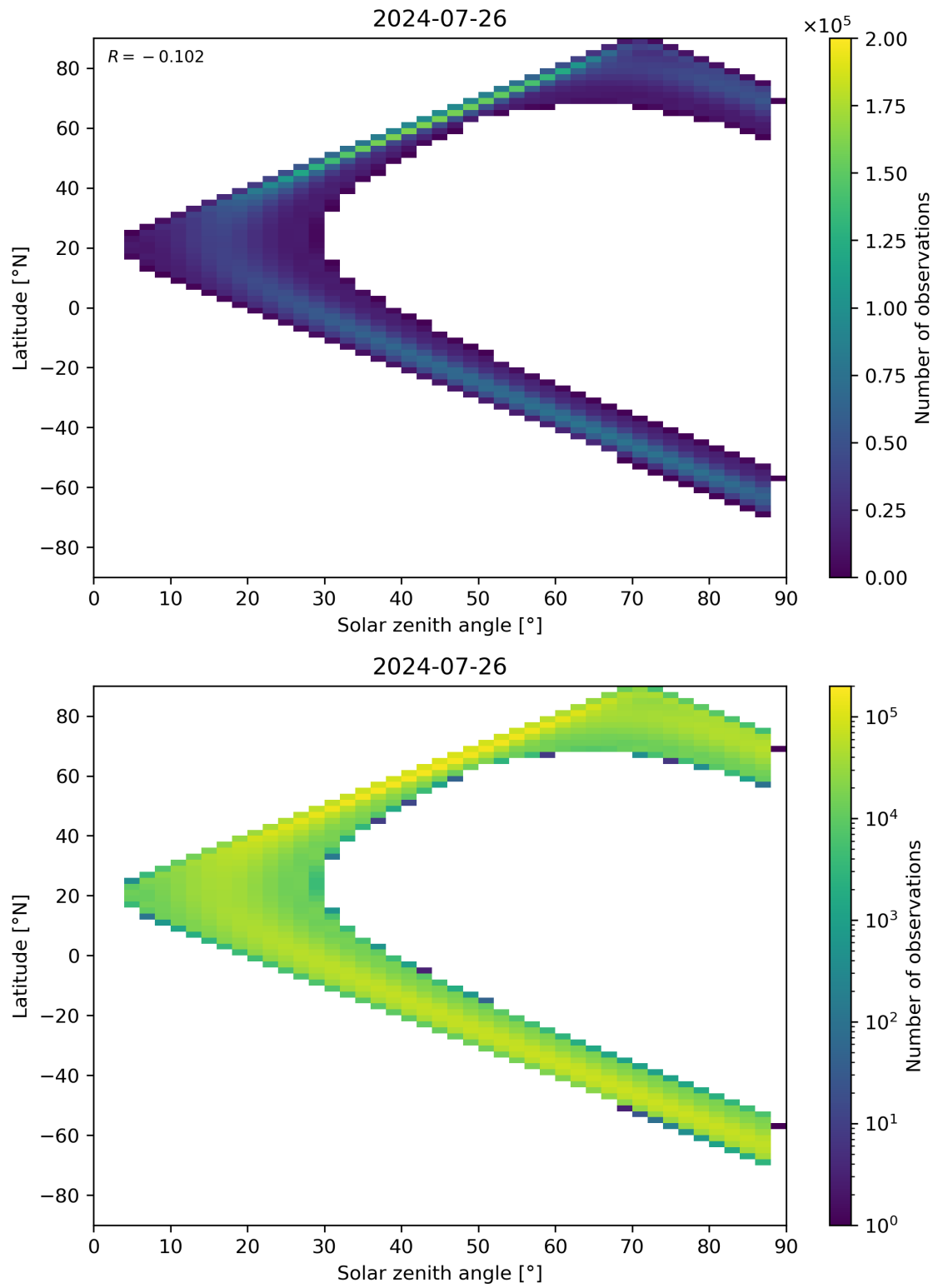
Figure 113: Scatter density plot of “Solar zenith angle” against “Latitude” for 2024-07-26 to 2024-07-27.
