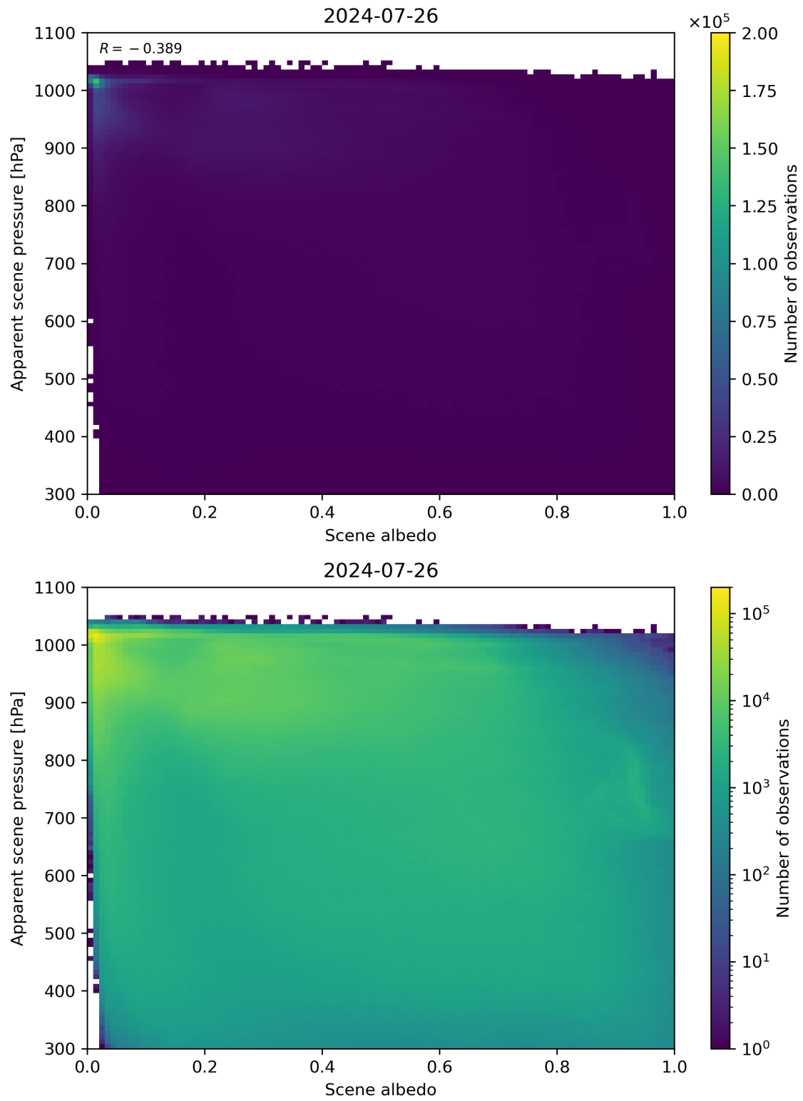
Figure 102: Scatter density plot of “Scene albedo” against “Apparent scene pressure” for 2024-07-26 to 2024-07-27.
