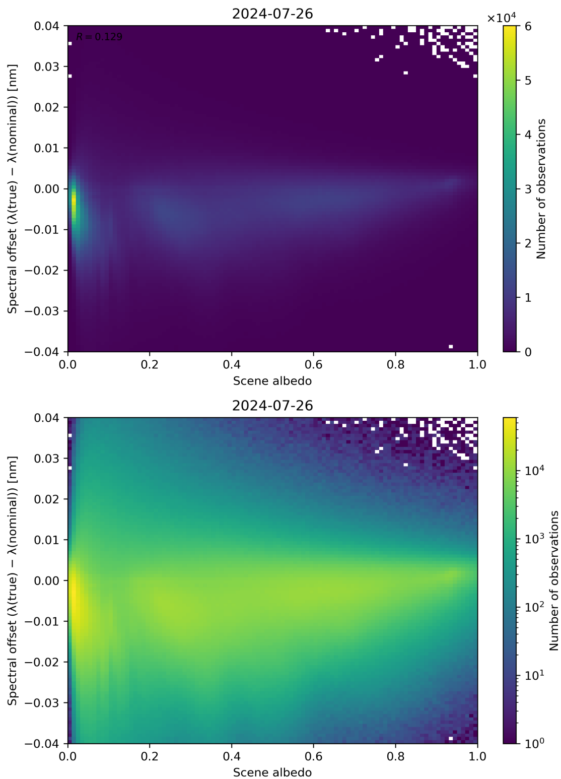
Figure 107: Scatter density plot of “Scene albedo” against “Spectral offset ( \lambda(\text{true}) - \lambda(\text{nominal}) )” for 2024-07-26 to 2024-07-27.
