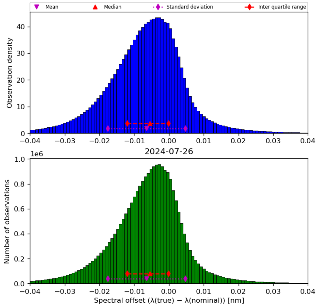
Figure 45: Histogram of “Spectral offset ( \lambda(\text{true}) - \lambda(\text{nominal}) )” for 2024-07-26 to 2024-07-27
