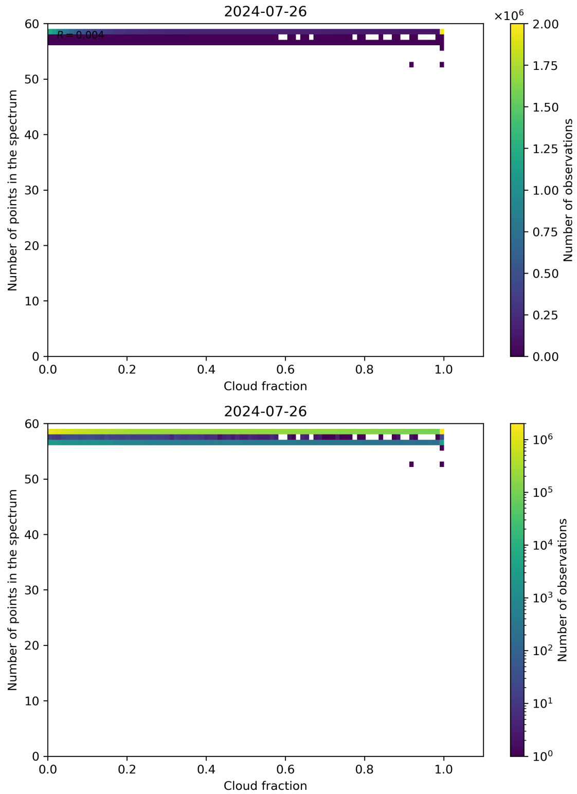
Figure 74: Scatter density plot of “Cloud fraction” against “Number of points in the spectrum” for 2024-07-26 to 2024-07-27.
