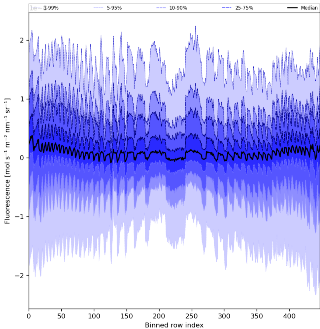
Figure 57: Along track statistics of “Fluorescence” for 2024-07-26 to 2024-07-27
