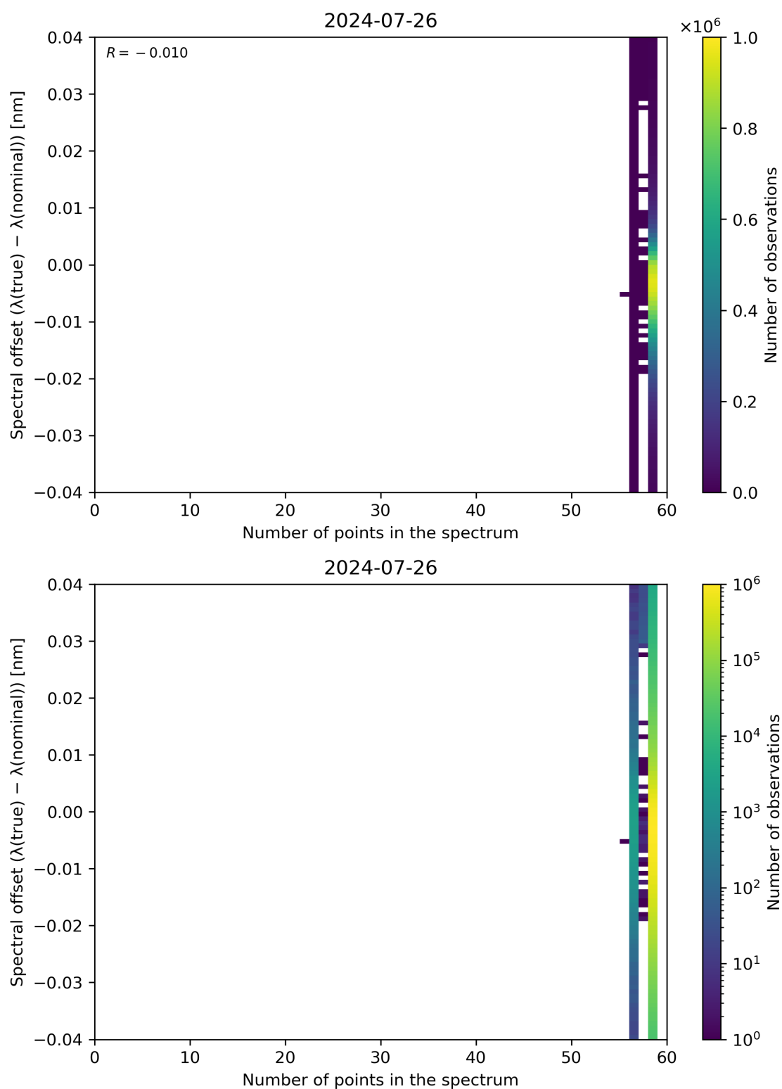
Figure 101: Scatter density plot of “Number of points in the spectrum” against “Spectral offset ( \lambda(\text{true}) - \lambda(\text{nominal}) )” for 2024-07-26 to 2024-07-27.
