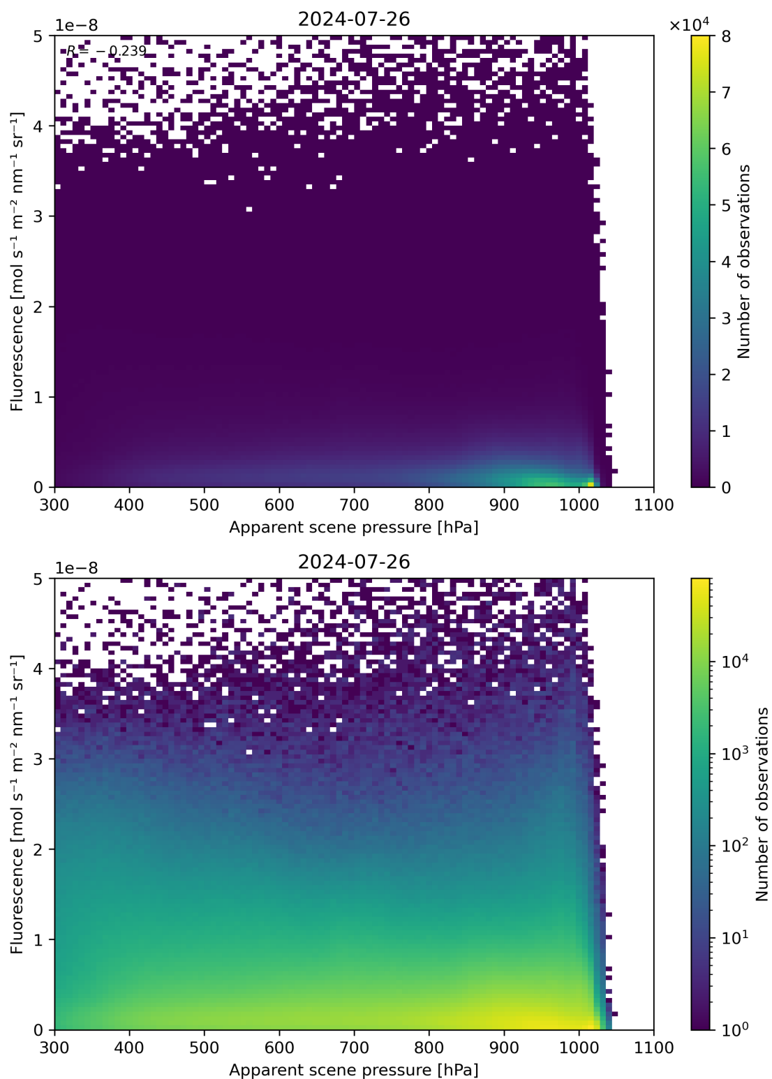
Figure 64: Scatter density plot of “Apparent scene pressure” against “Fluorescence” for 2024-07-26 to 2024-07-27.
