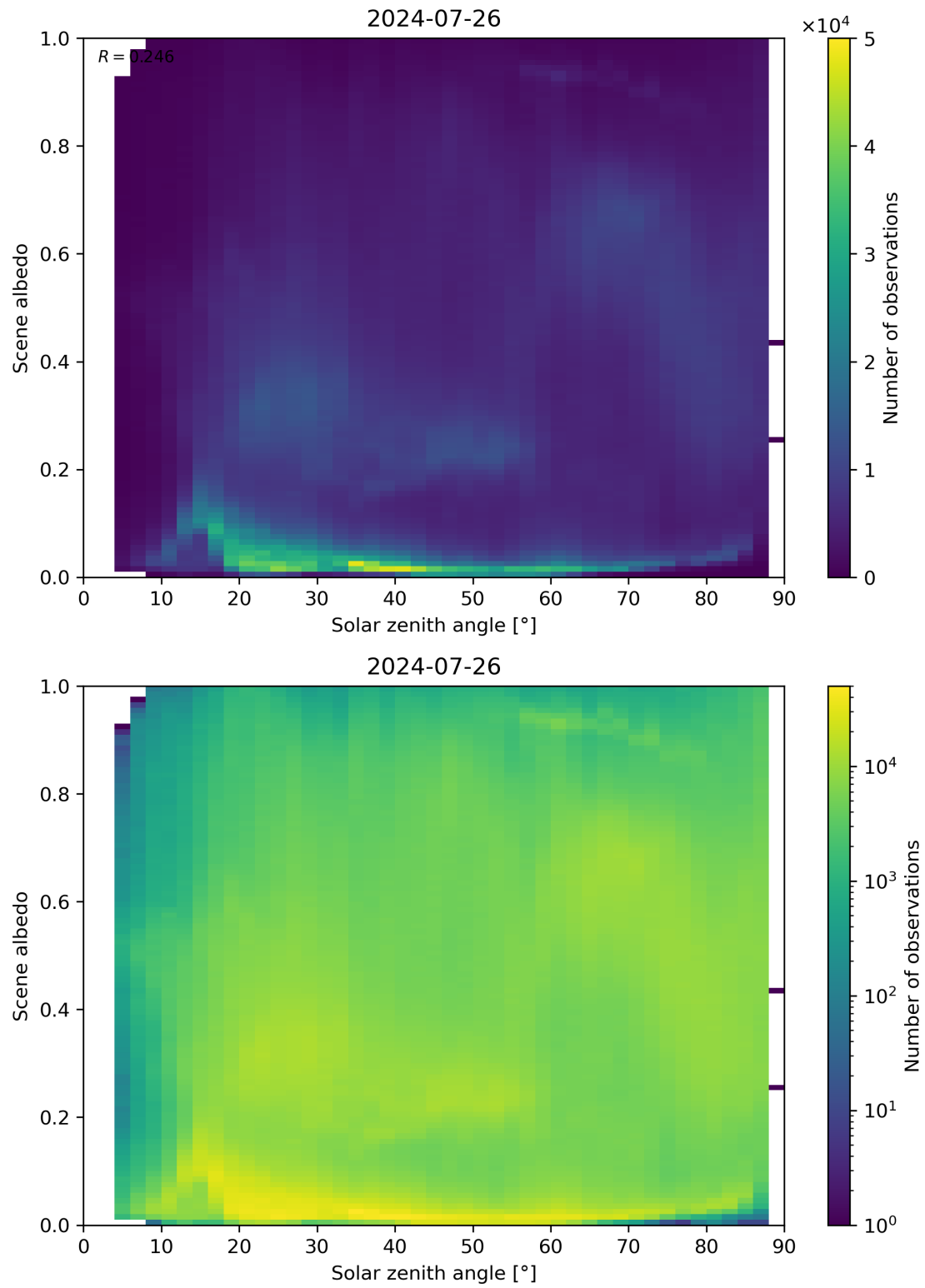
Figure 116: Scatter density plot of “Solar zenith angle” against “Scene albedo” for 2024-07-26 to 2024-07-27.
