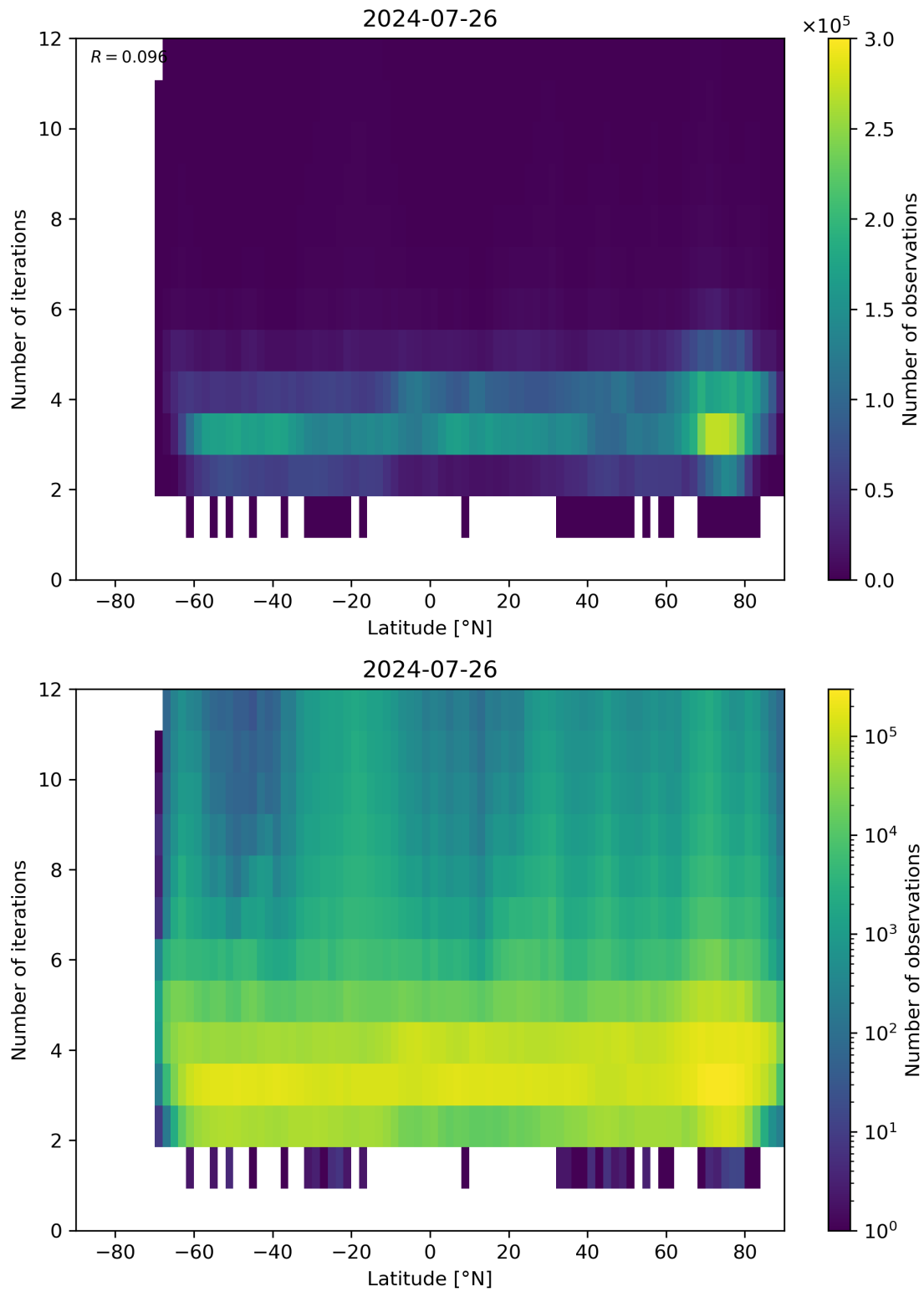
Figure 93: Scatter density plot of “Latitude” against “Number of iterations” for 2024-07-26 to 2024-07-27.
