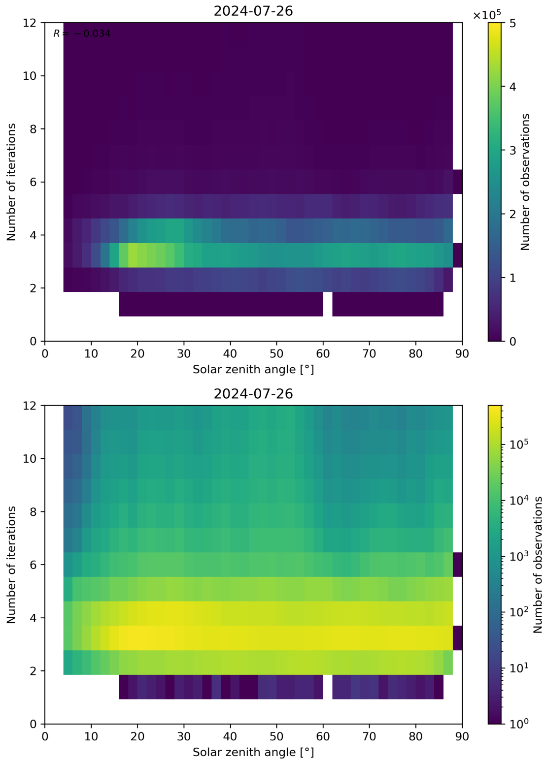
Figure 114: Scatter density plot of “Solar zenith angle” against “Number of iterations” for 2024-07-26 to 2024-07-27.
