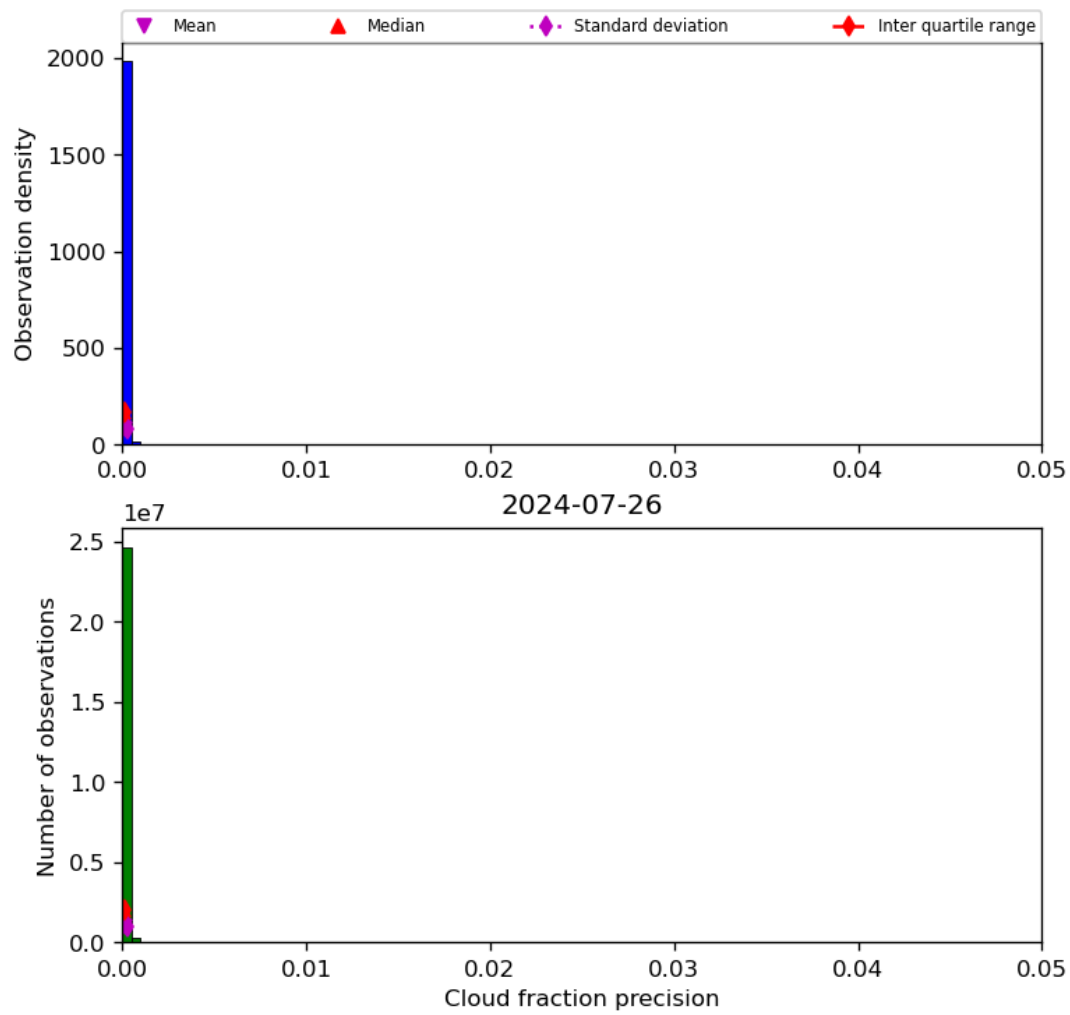
Figure 33: Histogram of “Cloud fraction precision” for 2024-07-26 to 2024-07-27
