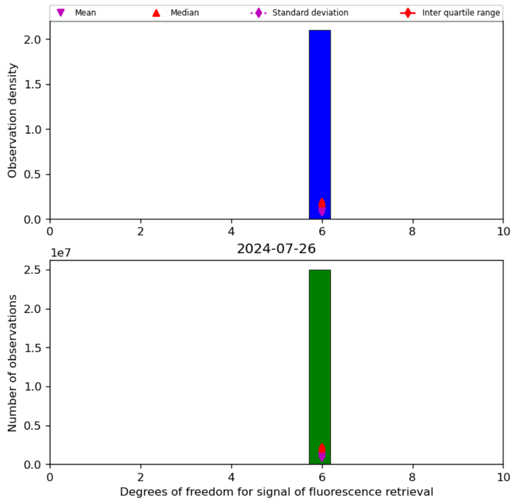
Figure 43: Histogram of “Degrees of freedom for signal of fluorescence retrieval” for 2024-07-26 to 2024-07-27
