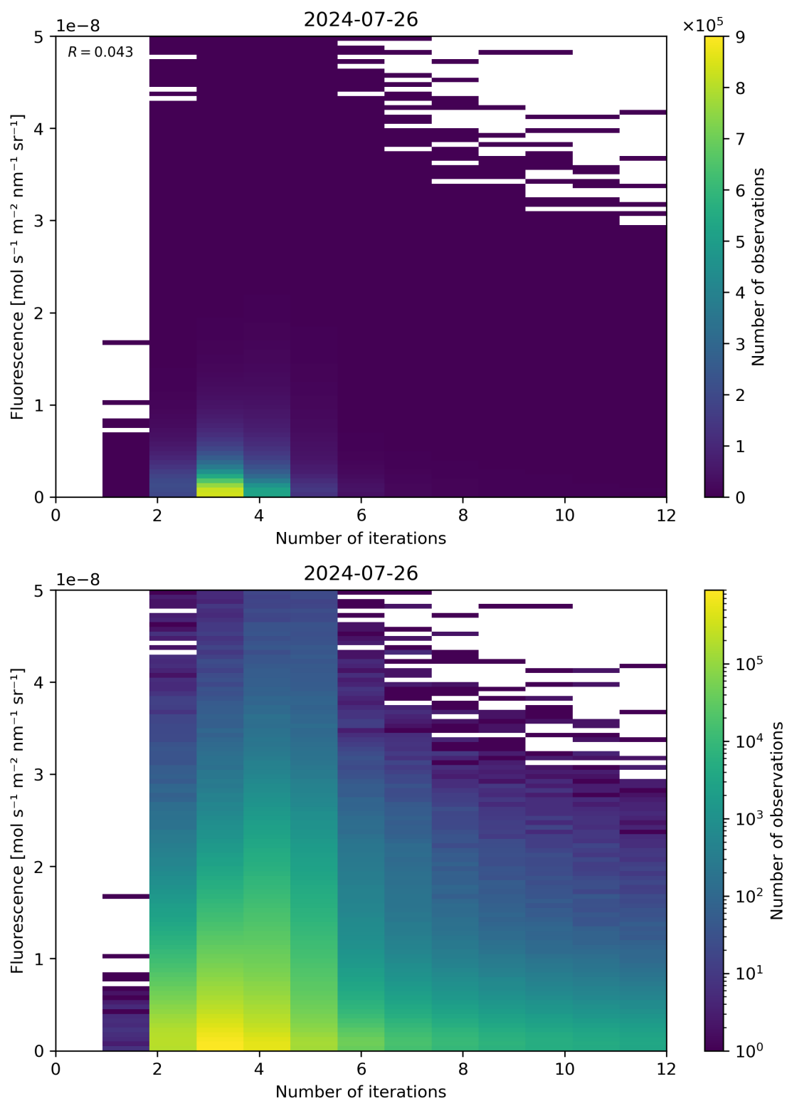
Figure 98: Scatter density plot of “Number of iterations” against “Fluorescence” for 2024-07-26 to 2024-07-27.
