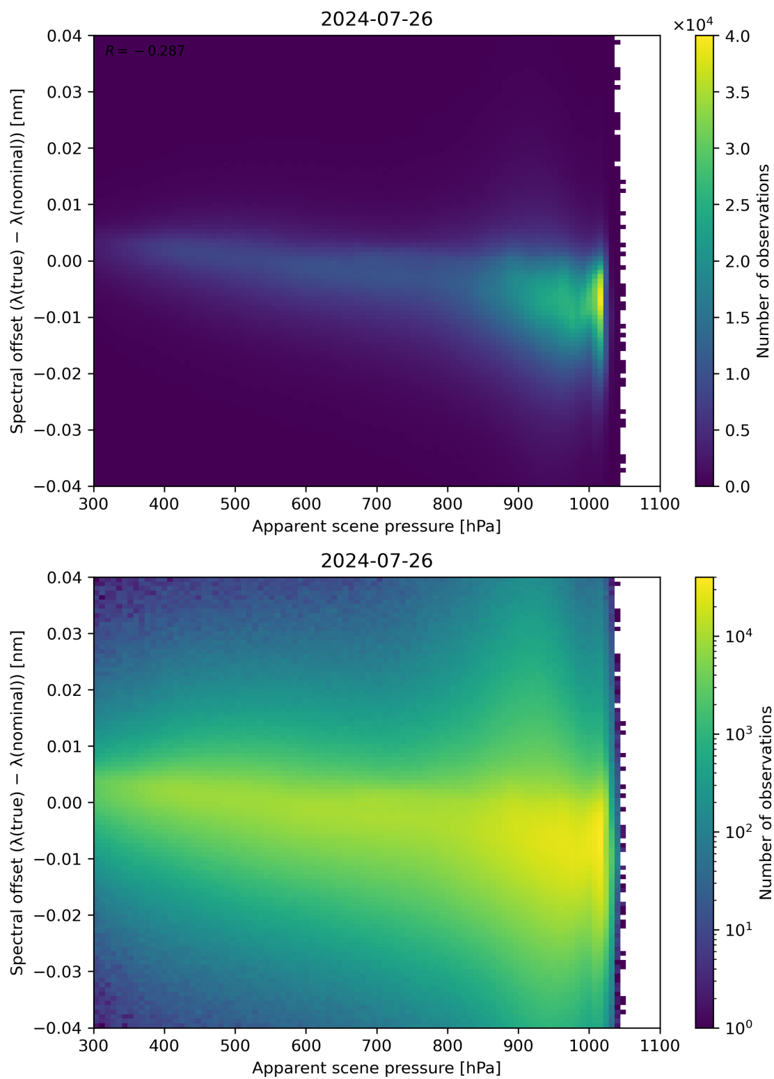
Figure 67: Scatter density plot of “Apparent scene pressure” against “Spectral offset ( \lambda(\text{true}) - \lambda(\text{nominal}) )” for 2024-07-26 to 2024-07-27.
