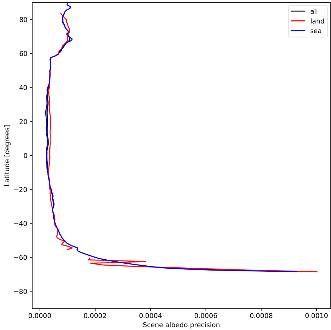
Figure 18: Zonal average of “Scene albedo precision” for 2024-07-26 to 2024-07-27.
