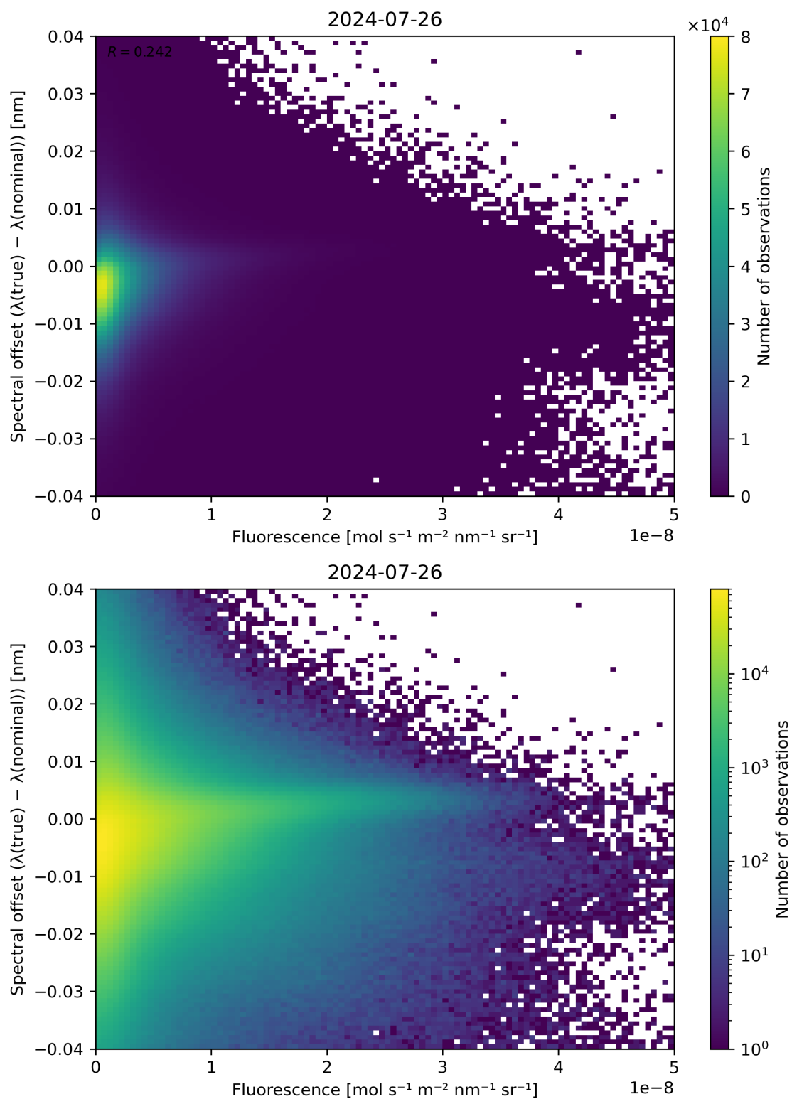
Figure 87: Scatter density plot of “Fluorescence” against “Spectral offset ( \lambda(\text{true}) - \lambda(\text{nominal}) )” for 2024-07-26 to 2024-07-27.
