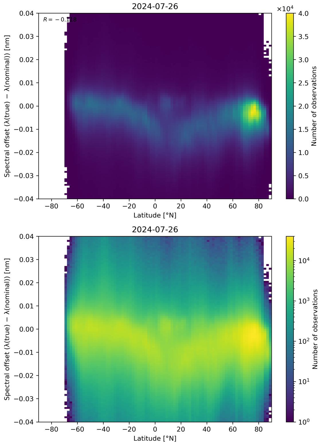
Figure 96: Scatter density plot of “Latitude” against “Spectral offset ( \lambda(\text{true}) - \lambda(\text{nominal}) )” for 2024-07-26 to 2024-07-27.
