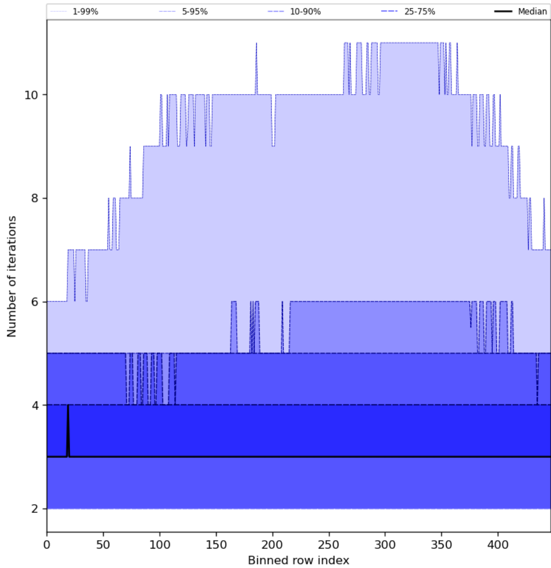
Figure 56: Along track statistics of “Number of iterations” for 2024-07-26 to 2024-07-27
