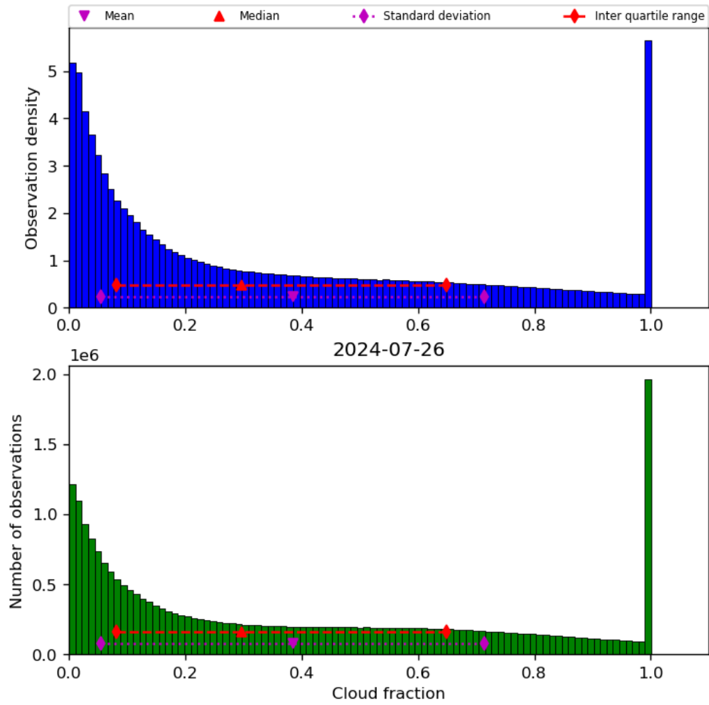
Figure 32: Histogram of “Cloud fraction” for 2024-07-26 to 2024-07-27
