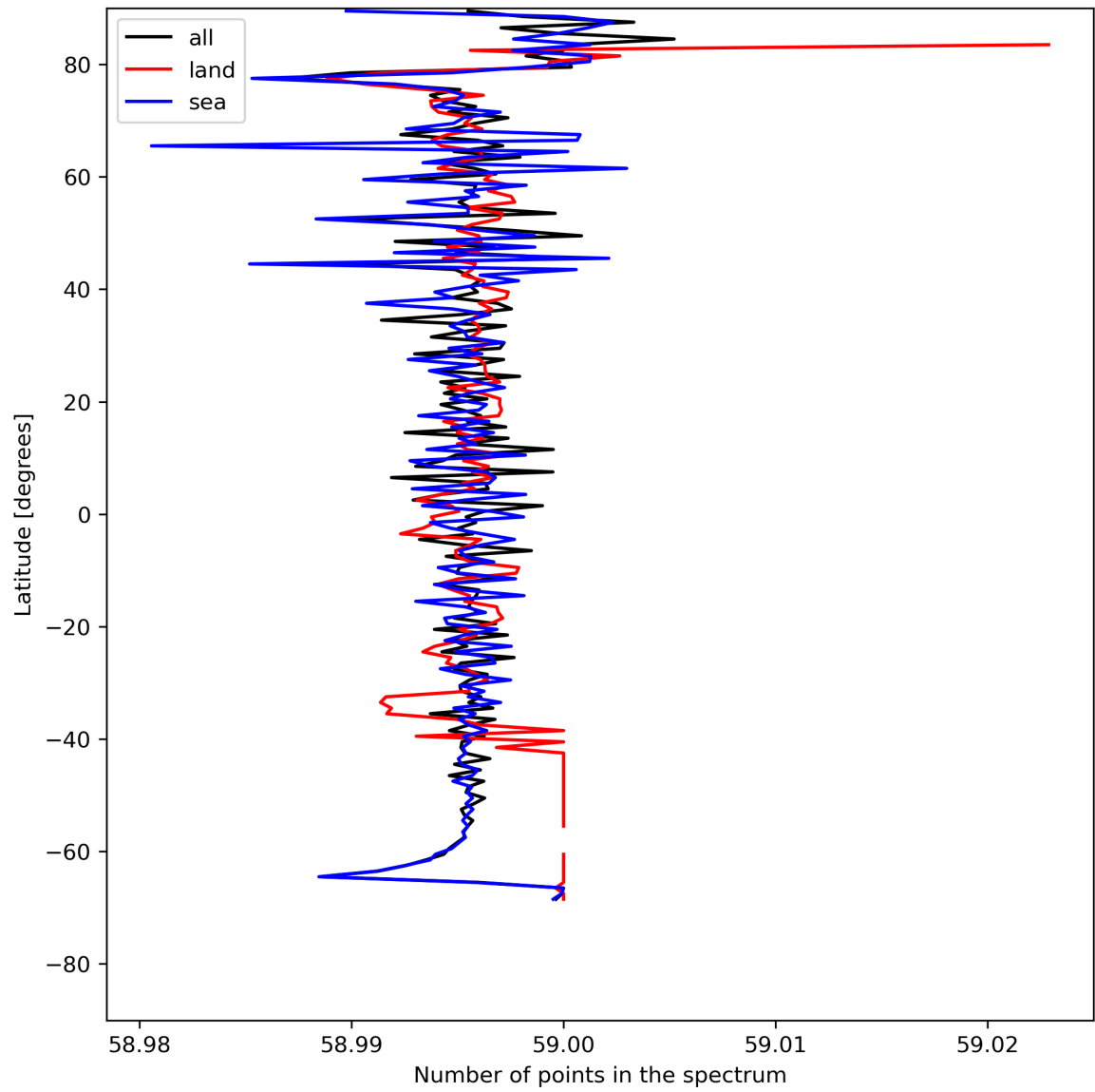
Figure 27: Zonal average of “Number of points in the spectrum” for 2024-07-26 to 2024-07-27.
