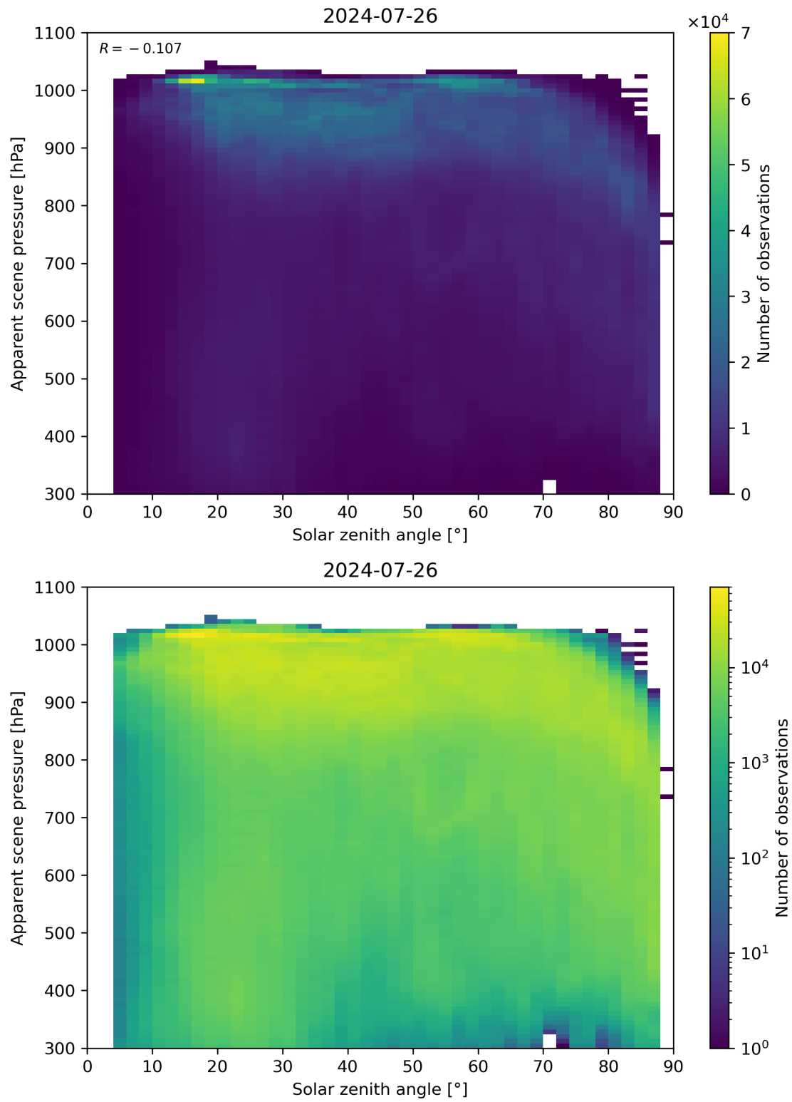
Figure 108: Scatter density plot of “Solar zenith angle” against “Apparent scene pressure” for 2024-07-26 to 2024-07-27.
