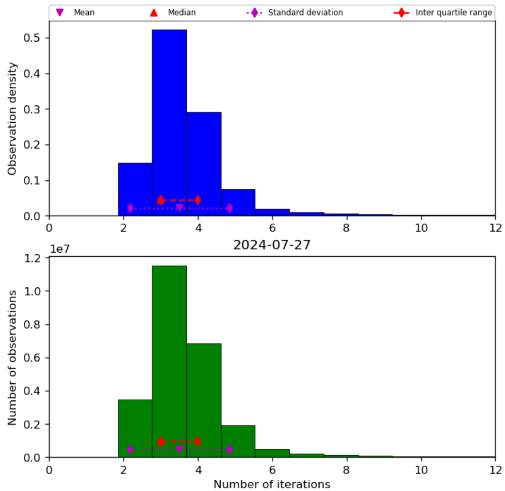
Figure 39: Histogram of “Number of iterations” for 2024-07-26 to 2024-07-28
