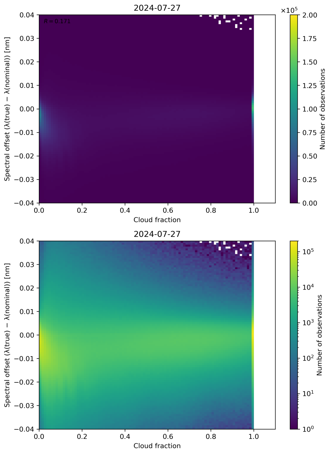
Figure 76: Scatter density plot of “Cloud fraction” against “Spectral offset ( \lambda(\text{true}) - \lambda(\text{nominal}) )” for 2024-07-26 to 2024-07-28.
