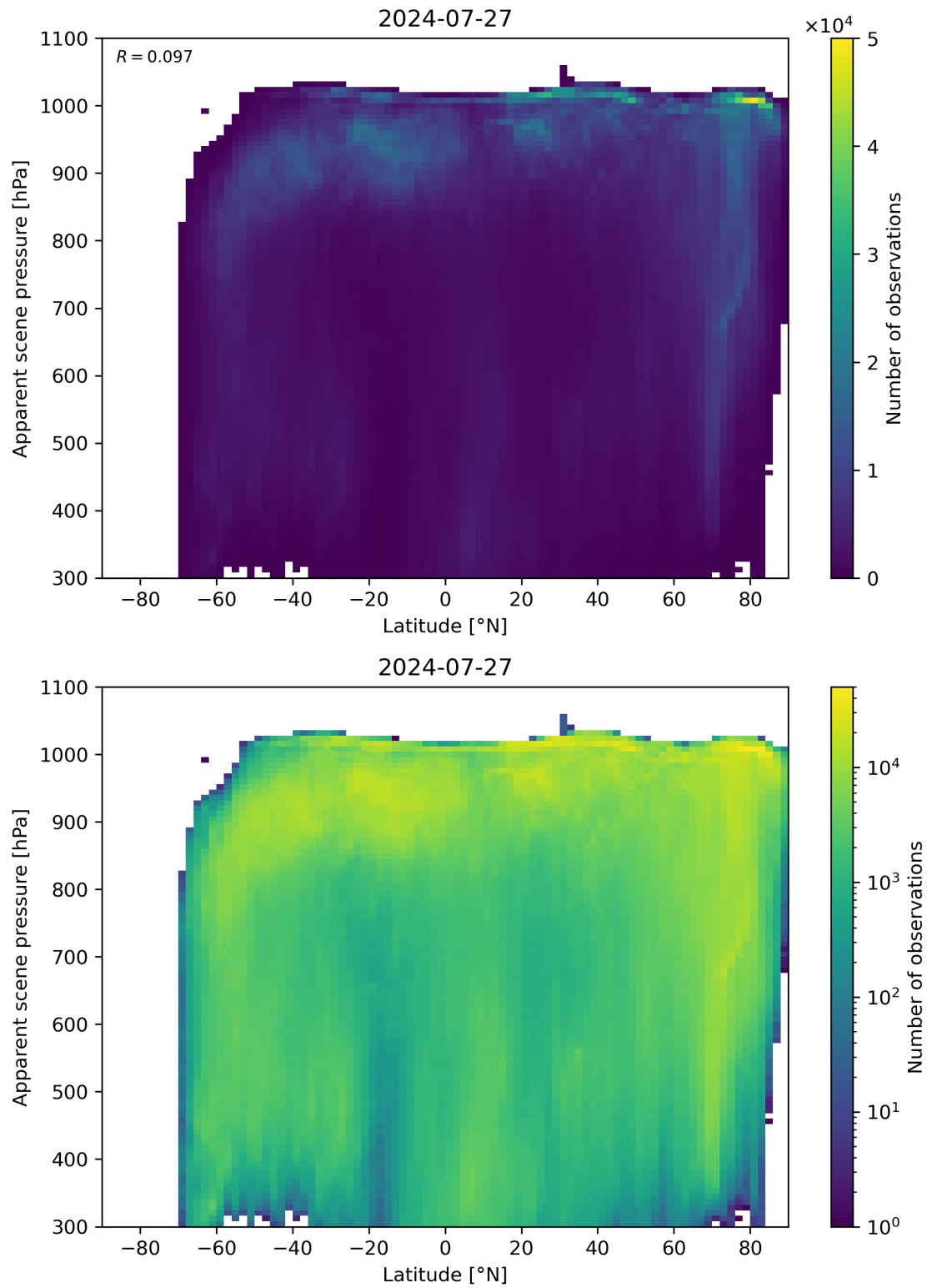
Figure 88: Scatter density plot of “Latitude” against “Apparent scene pressure” for 2024-07-26 to 2024-07-28.
