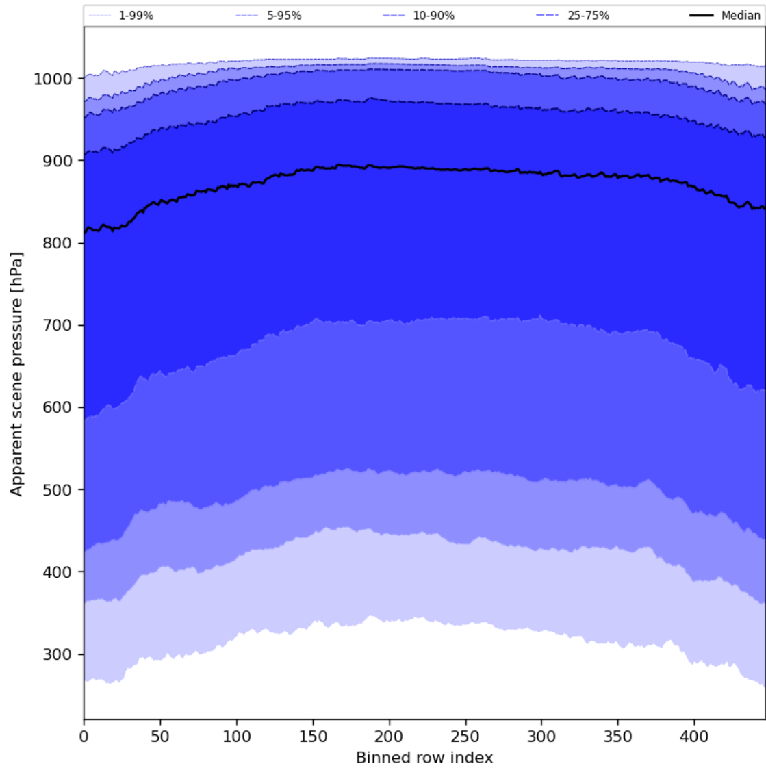
Figure 53: Along track statistics of “Apparent scene pressure” for 2024-07-26 to 2024-07-28
