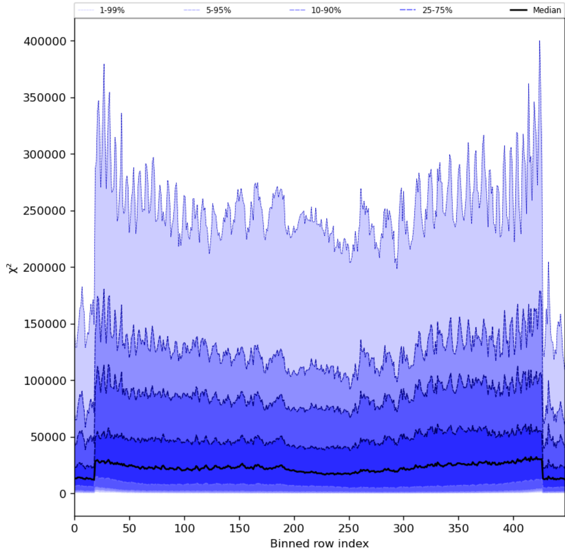
Figure 55: Along track statistics of “ \chi^2 ” for 2024-07-26 to 2024-07-28
