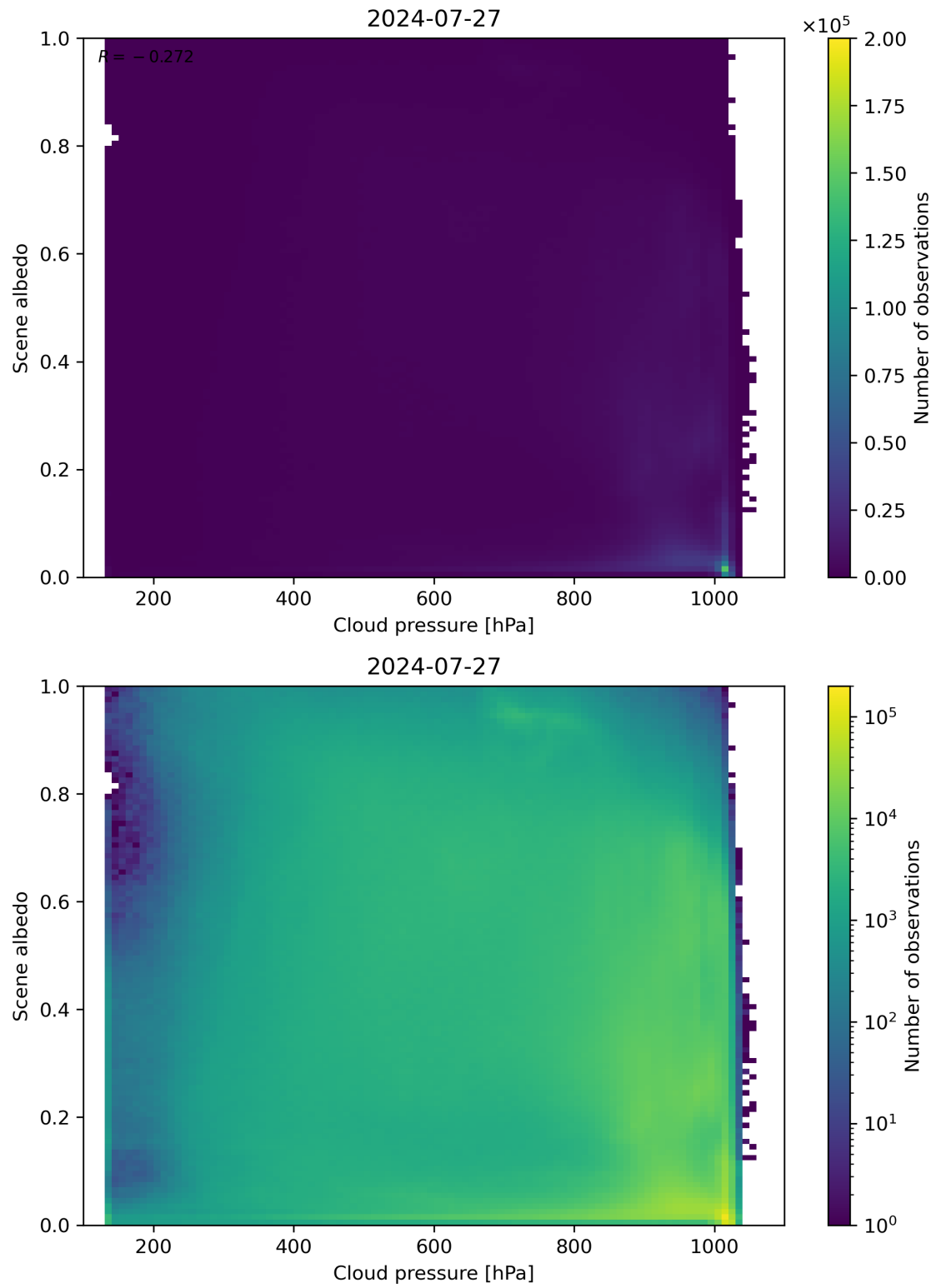
Figure 83: Scatter density plot of “Cloud pressure” against “Scene albedo” for 2024-07-26 to 2024-07-28.
