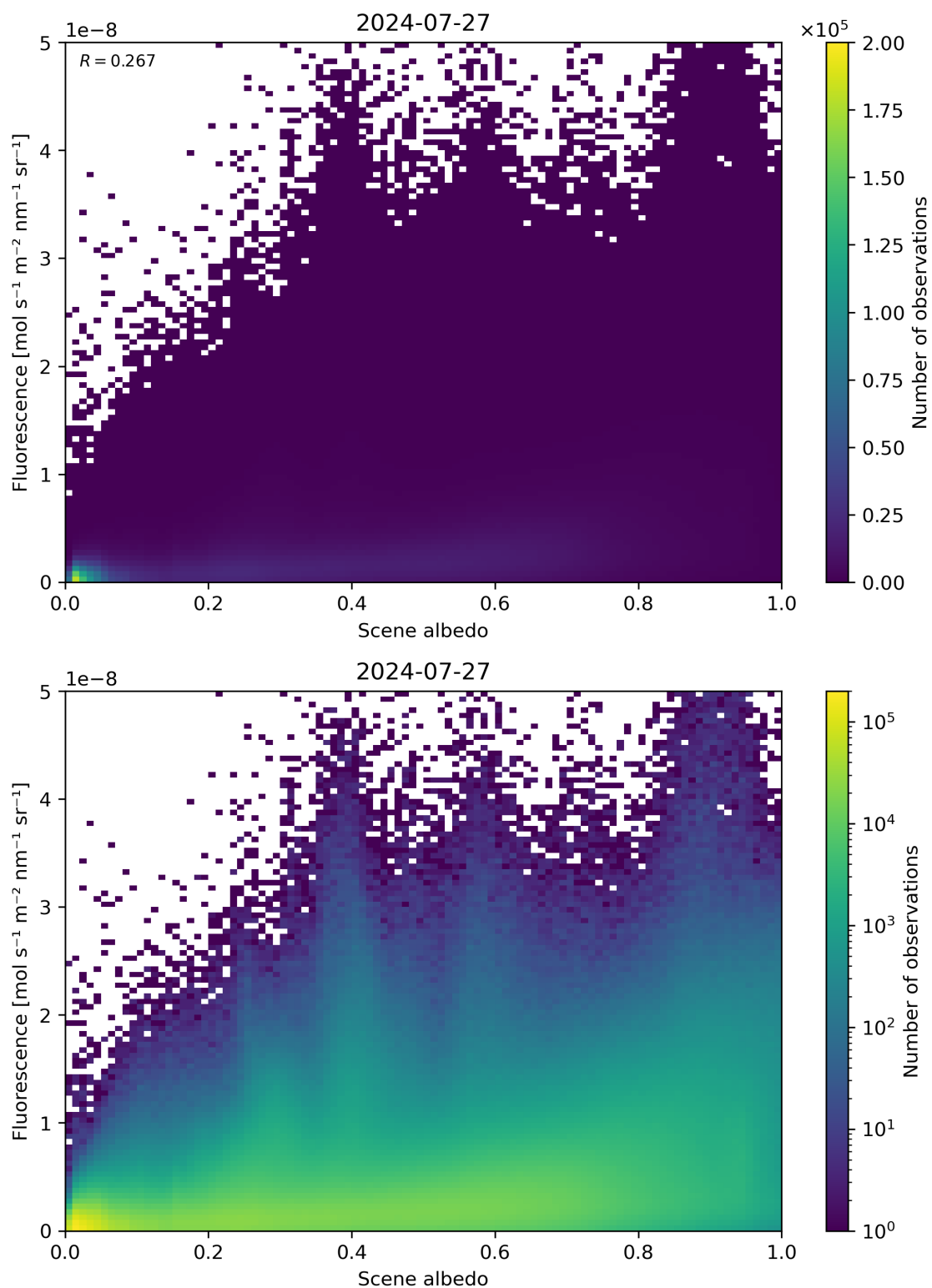
Figure 104: Scatter density plot of “Scene albedo” against “Fluorescence” for 2024-07-26 to 2024-07-28.
