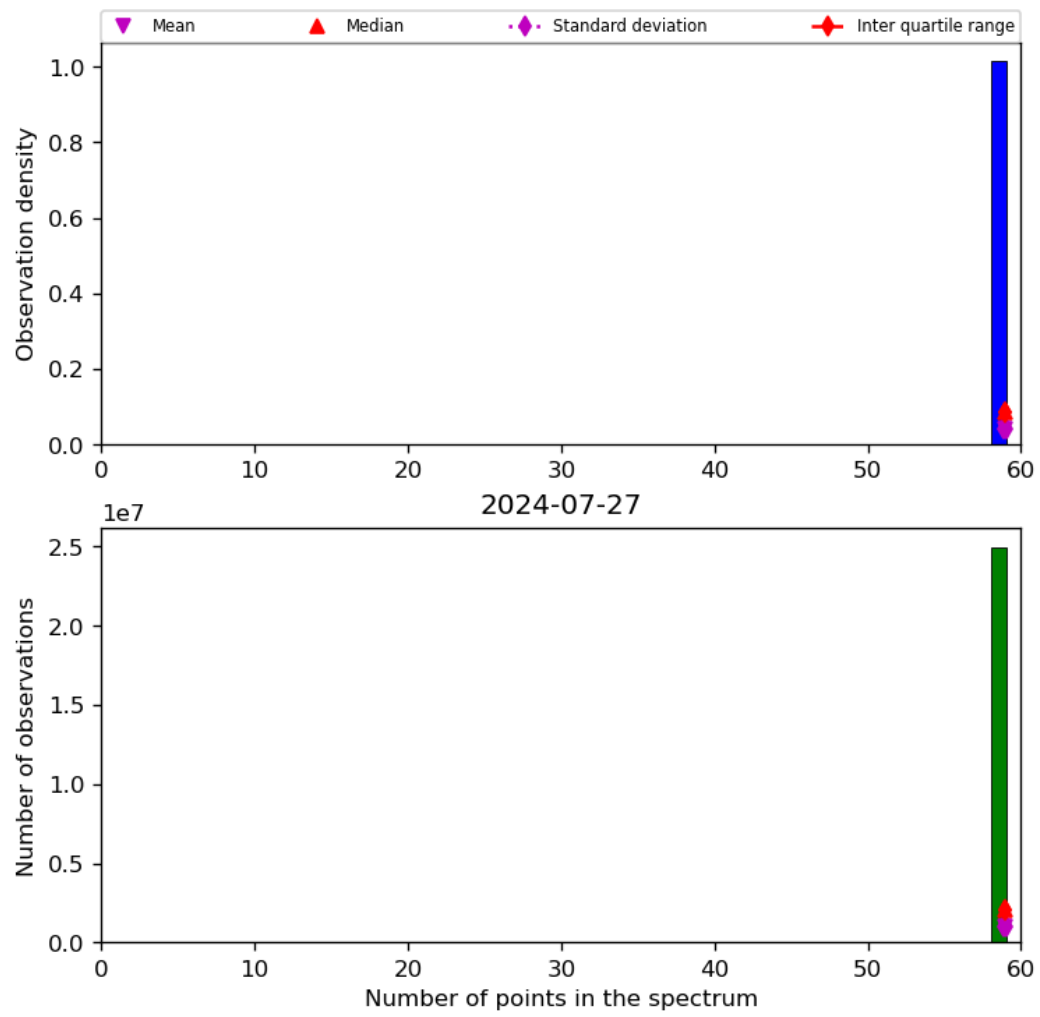
Figure 44: Histogram of “Number of points in the spectrum” for 2024-07-26 to 2024-07-28
