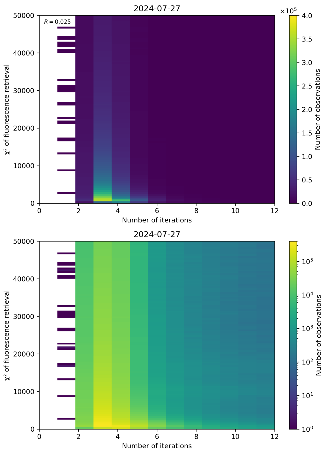
Figure 97: Scatter density plot of “Number of iterations” against “ \chi^2 of fluorescence retrieval” for 2024-07-26 to 2024-07-28.
