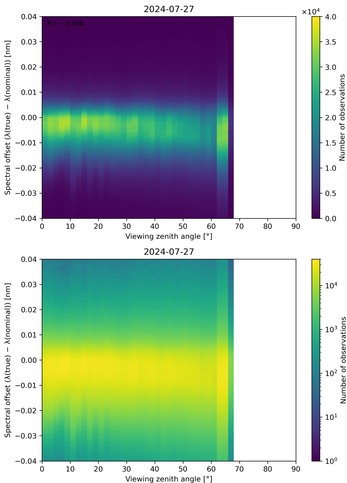
Figure 128: Scatter density plot of “Viewing zenith angle” against “Spectral offset ( \lambda(\text{true}) - \lambda(\text{nominal}) )” for 2024-07-26 to 2024-07-28.
