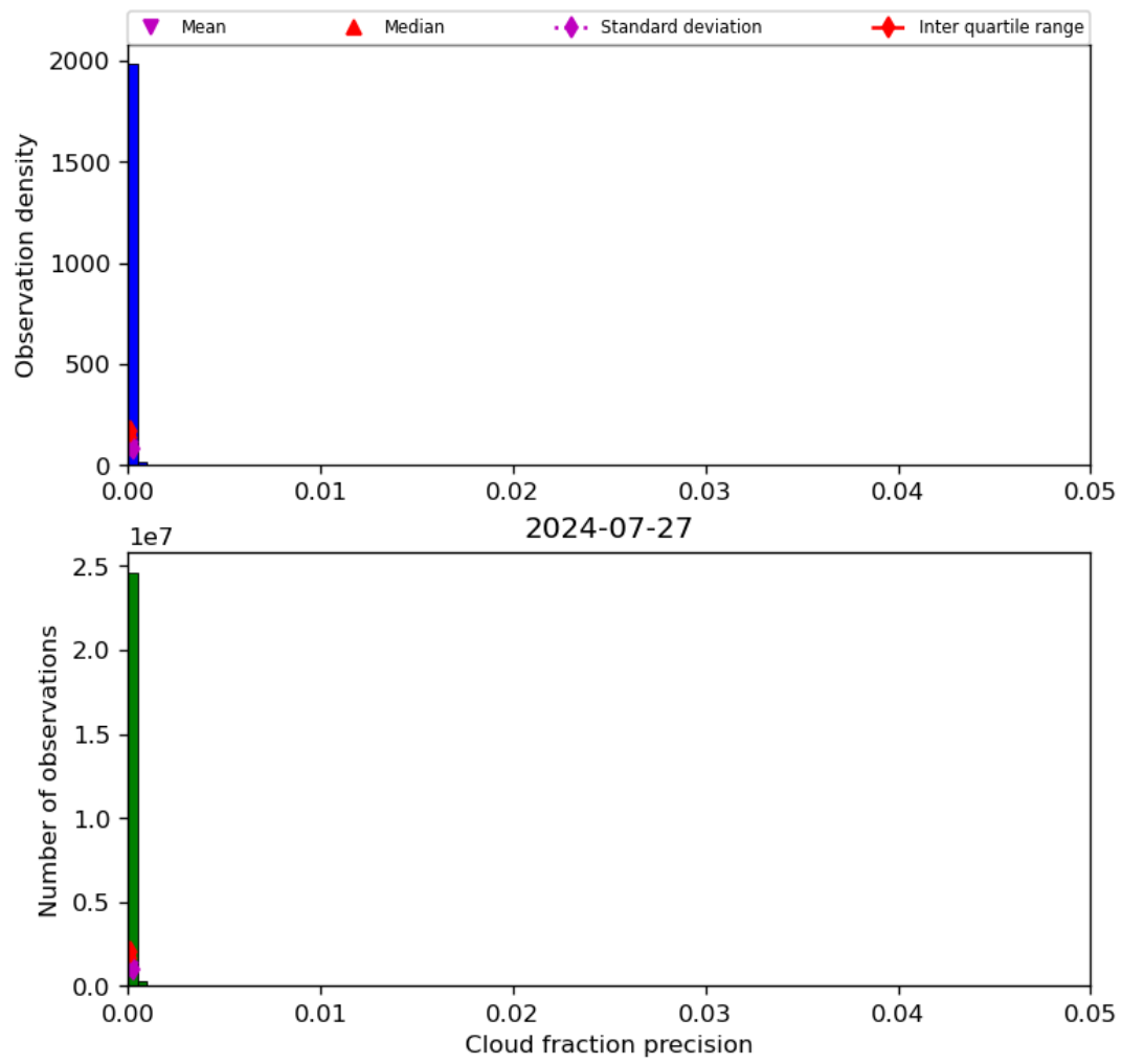
Figure 33: Histogram of “Cloud fraction precision” for 2024-07-26 to 2024-07-28
