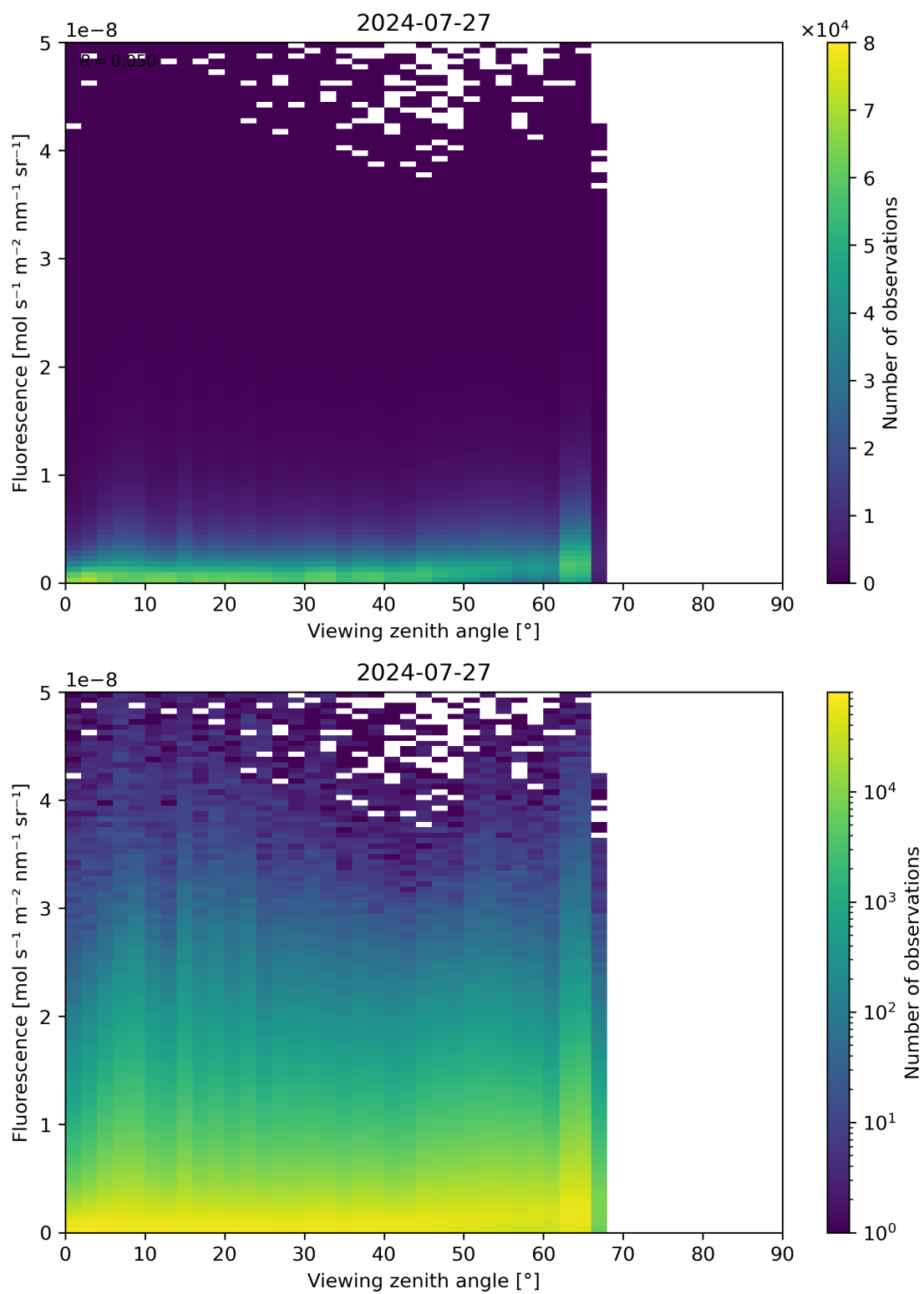
Figure 122: Scatter density plot of “Viewing zenith angle” against “Fluorescence” for 2024-07-26 to 2024-07-28.
