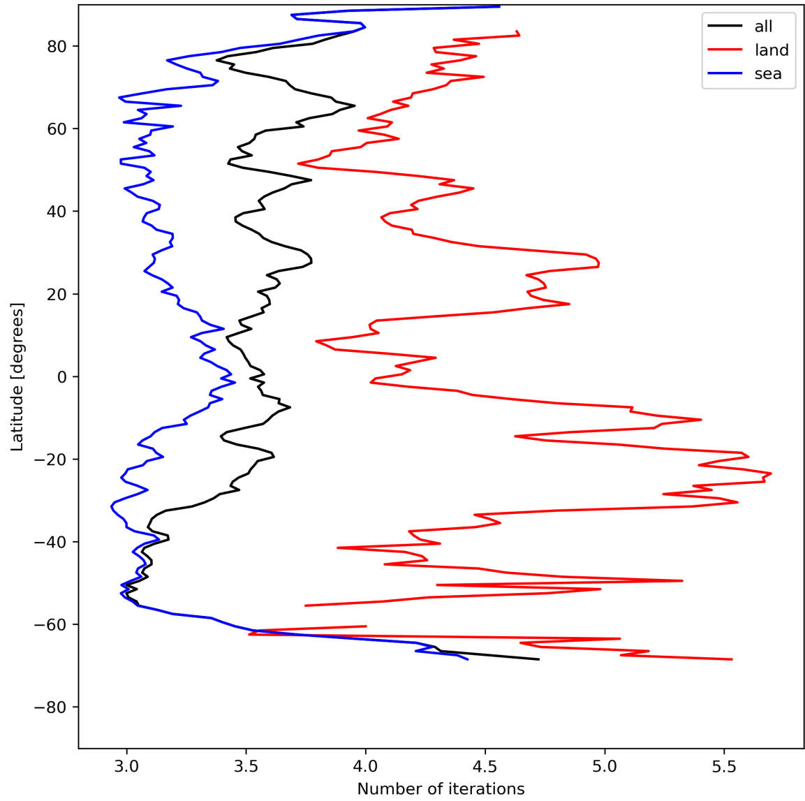
Figure 22: Zonal average of “Number of iterations” for 2024-07-26 to 2024-07-28.
