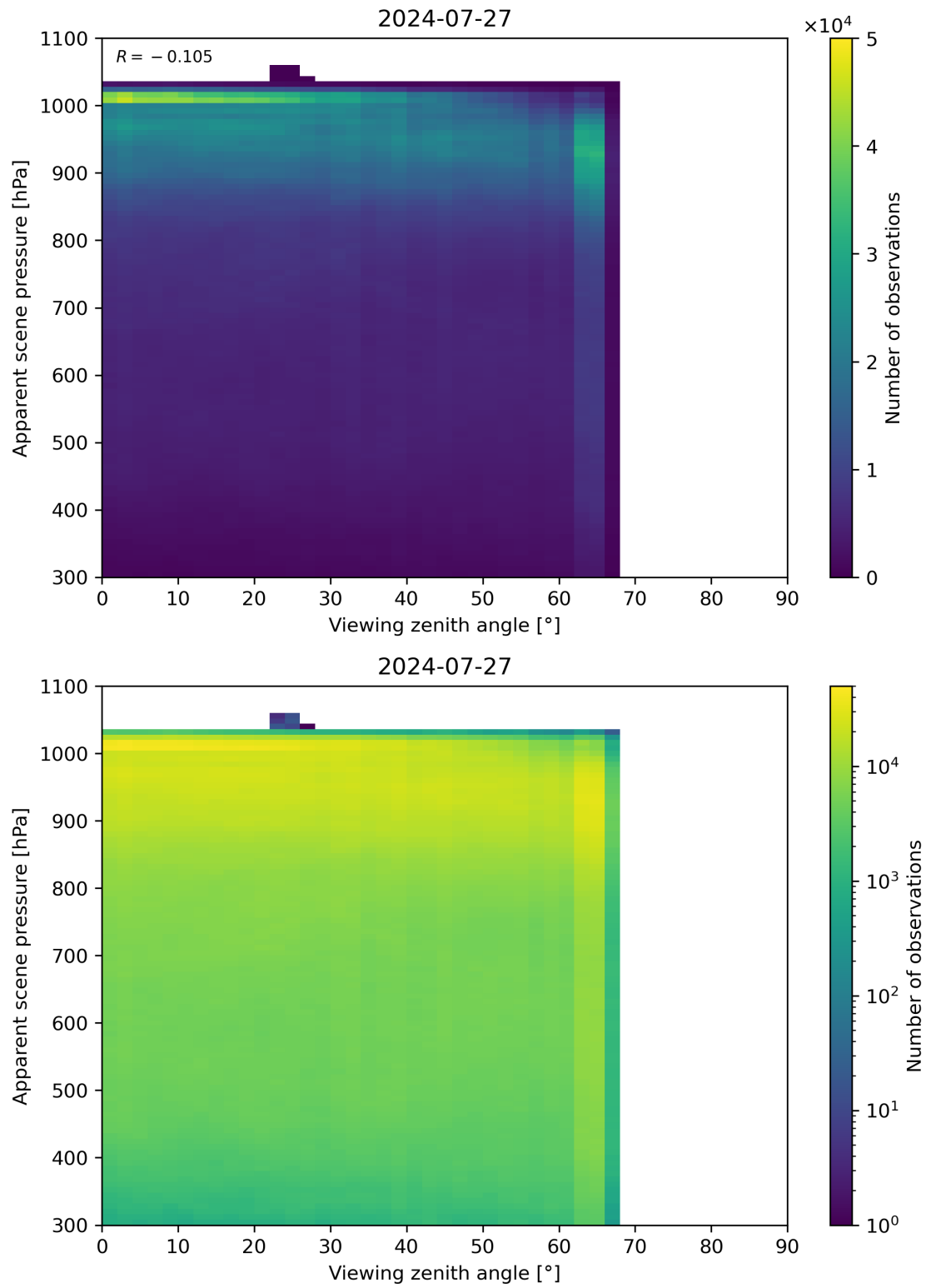
Figure 118: Scatter density plot of “Viewing zenith angle” against “Apparent scene pressure” for 2024-07-26 to 2024-07-28.
