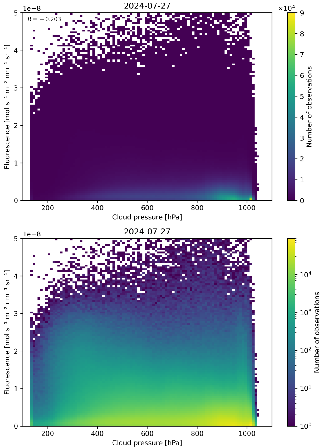
Figure 80: Scatter density plot of “Cloud pressure” against “Fluorescence” for 2024-07-26 to 2024-07-28.
