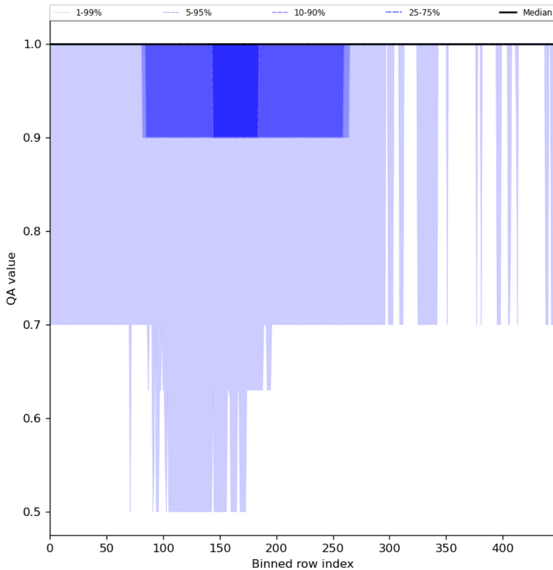
Figure 46: Along track statistics of “QA value” for 2024-07-26 to 2024-07-28
