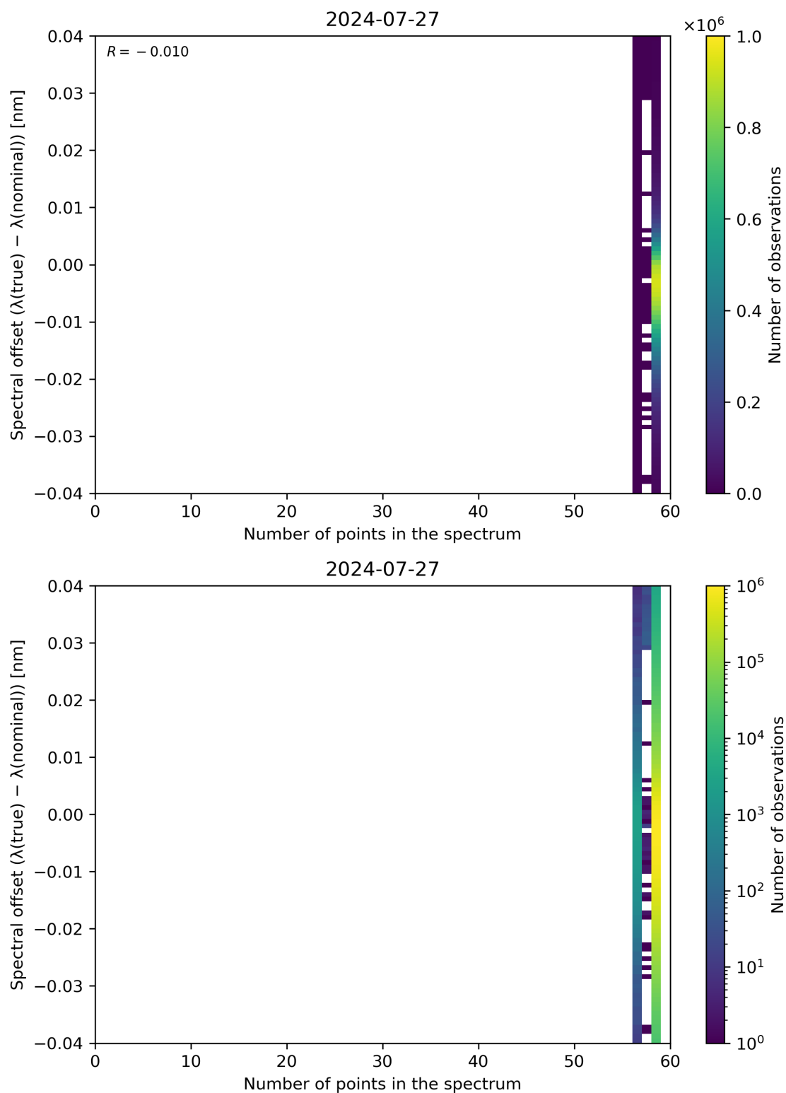
Figure 101: Scatter density plot of “Number of points in the spectrum” against “Spectral offset ( \lambda(\text{true}) - \lambda(\text{nominal}) )” for 2024-07-26 to 2024-07-28.
