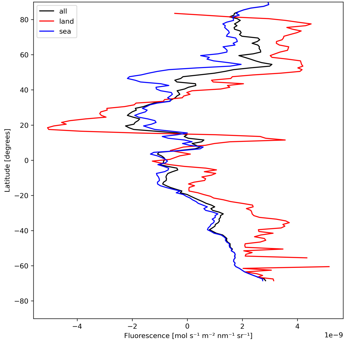
Figure 23: Zonal average of “Fluorescence” for 2024-07-26 to 2024-07-28.
