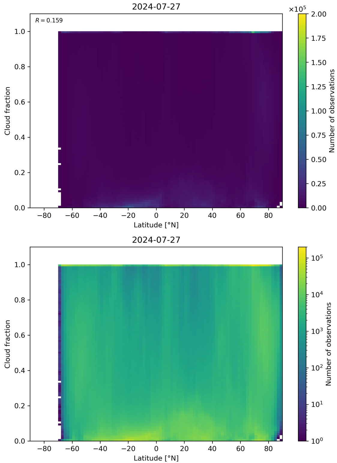
Figure 90: Scatter density plot of “Latitude” against “Cloud fraction” for 2024-07-26 to 2024-07-28.
