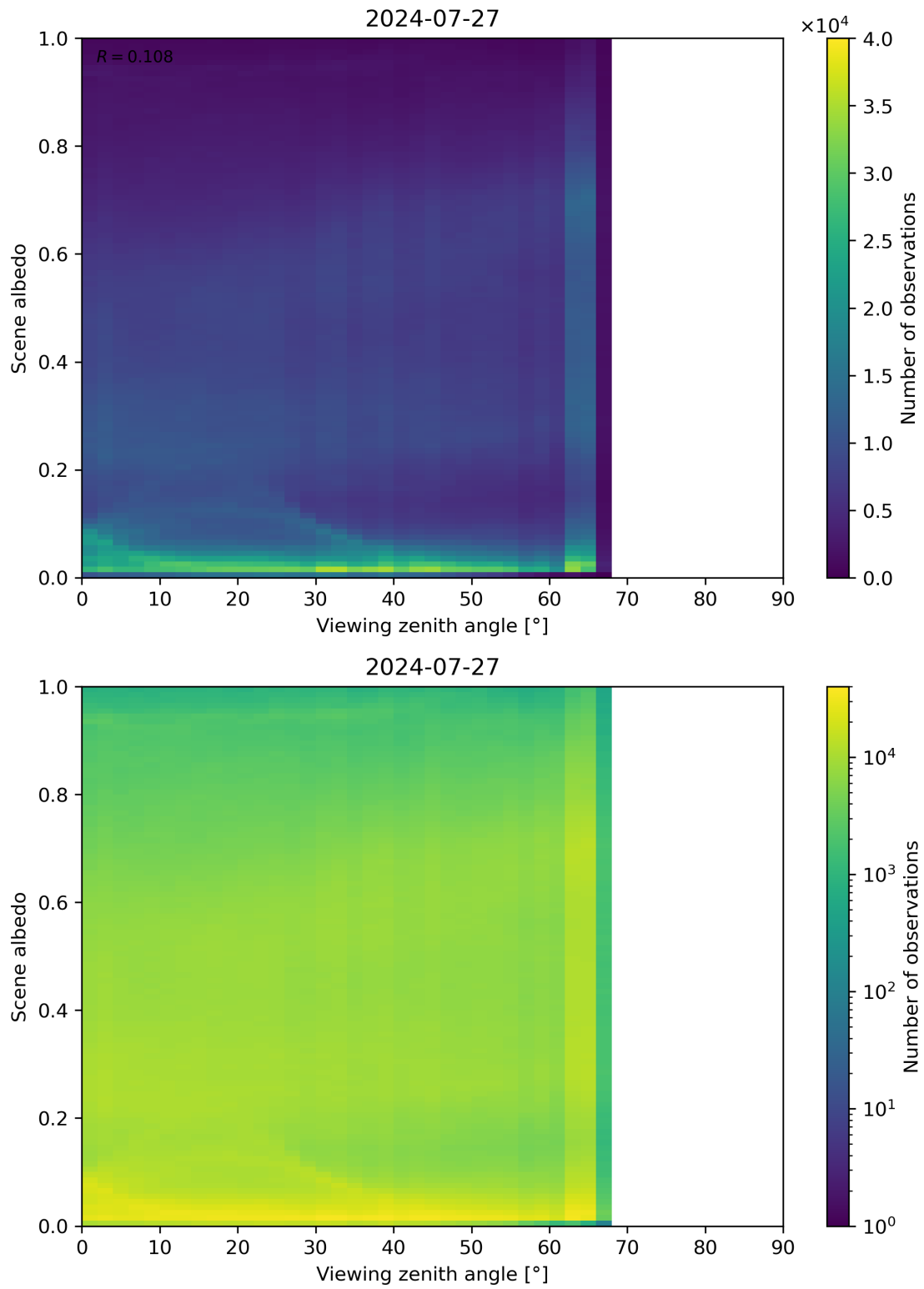
Figure 126: Scatter density plot of “Viewing zenith angle” against “Scene albedo” for 2024-07-26 to 2024-07-28.
