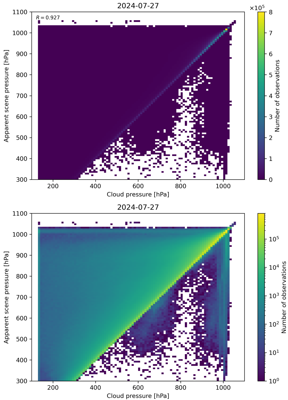
Figure 77: Scatter density plot of “Cloud pressure” against “Apparent scene pressure” for 2024-07-26 to 2024-07-28.
