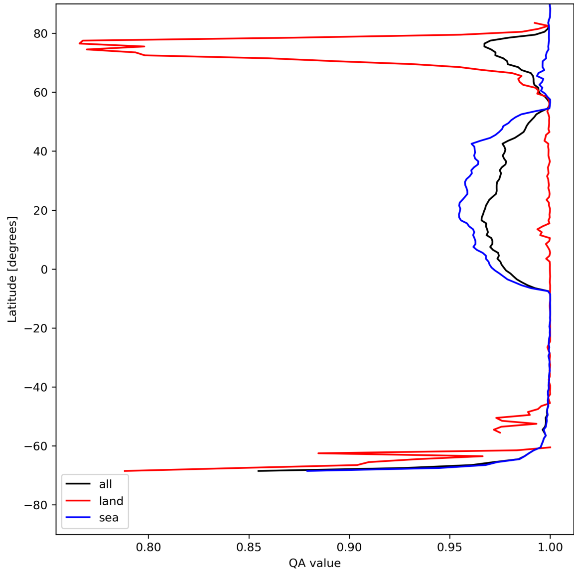
Figure 12: Zonal average of “QA value” for 2024-07-26 to 2024-07-28.
