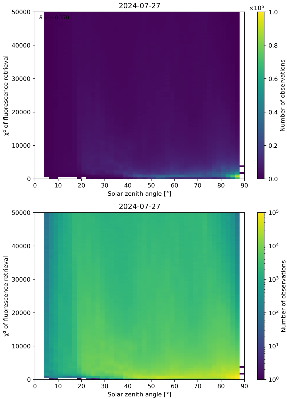
Figure 109: Scatter density plot of “Solar zenith angle” against “ \chi^2 of fluorescence retrieval” for 2024-07-26 to 2024-07-28.
