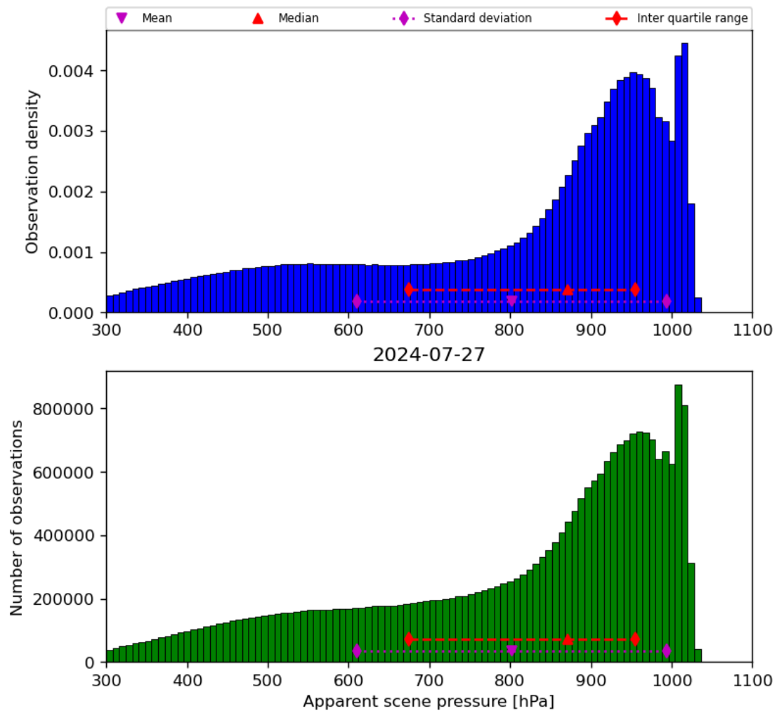
Figure 36: Histogram of “Apparent scene pressure” for 2024-07-26 to 2024-07-28
