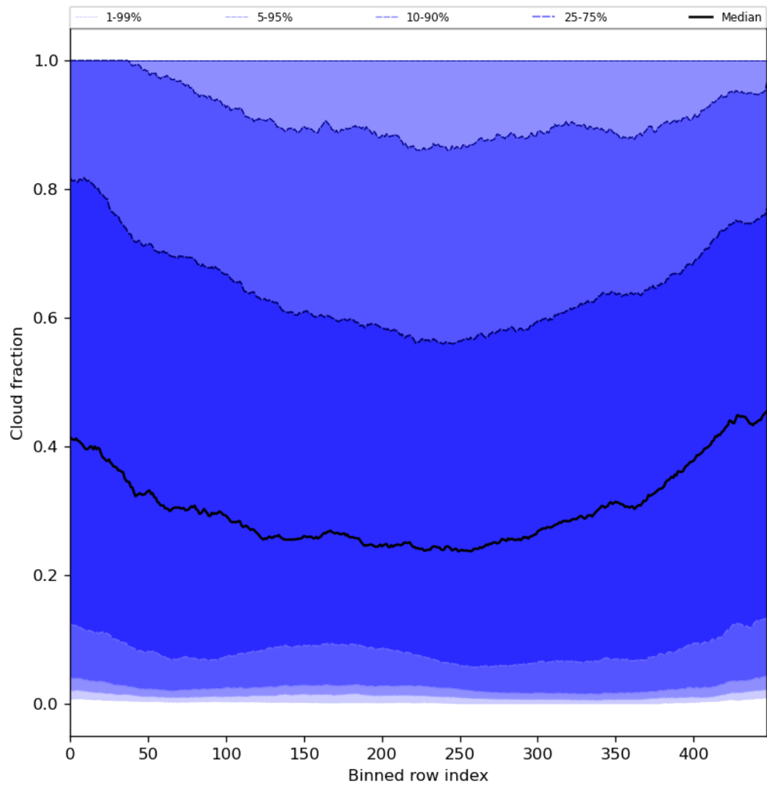
Figure 49: Along track statistics of “Cloud fraction” for 2024-07-26 to 2024-07-28
