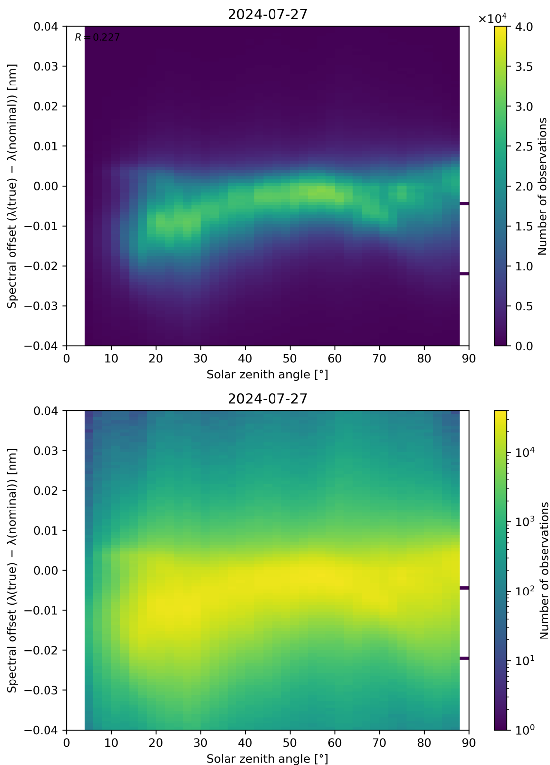
Figure 117: Scatter density plot of “Solar zenith angle” against “Spectral offset ( \lambda(\text{true}) - \lambda(\text{nominal}) )” for 2024-07-26 to 2024-07-28.
