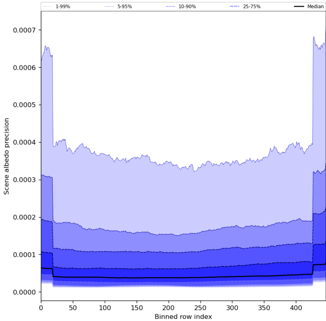
Figure 52: Along track statistics of “Scene albedo precision” for 2024-07-26 to 2024-07-28
