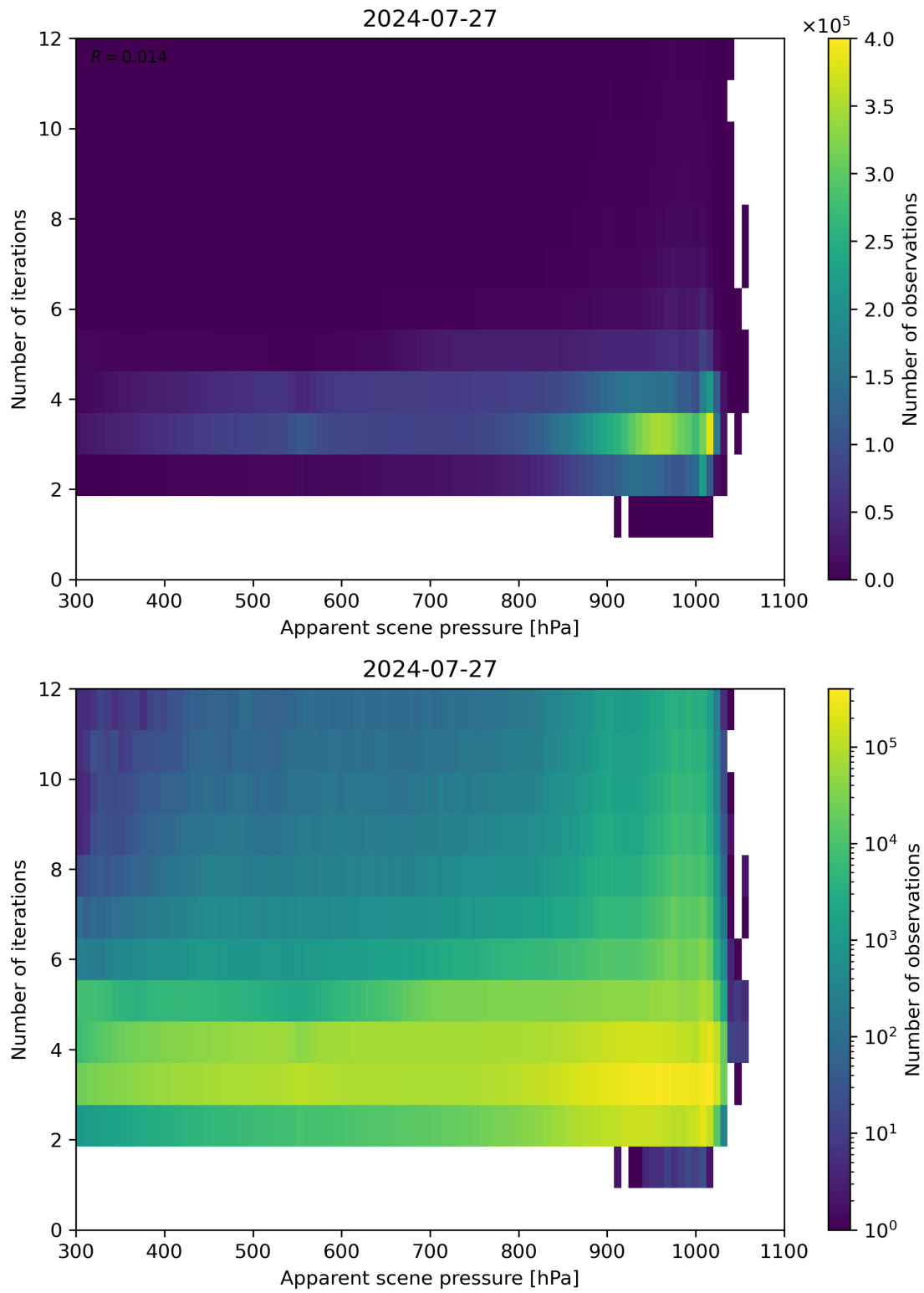
Figure 65: Scatter density plot of “Apparent scene pressure” against “Number of iterations” for 2024-07-26 to 2024-07-28.
