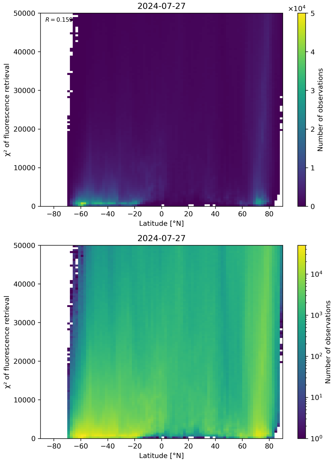
Figure 89: Scatter density plot of “Latitude” against “ \chi^2 of fluorescence retrieval” for 2024-07-26 to 2024-07-28.
