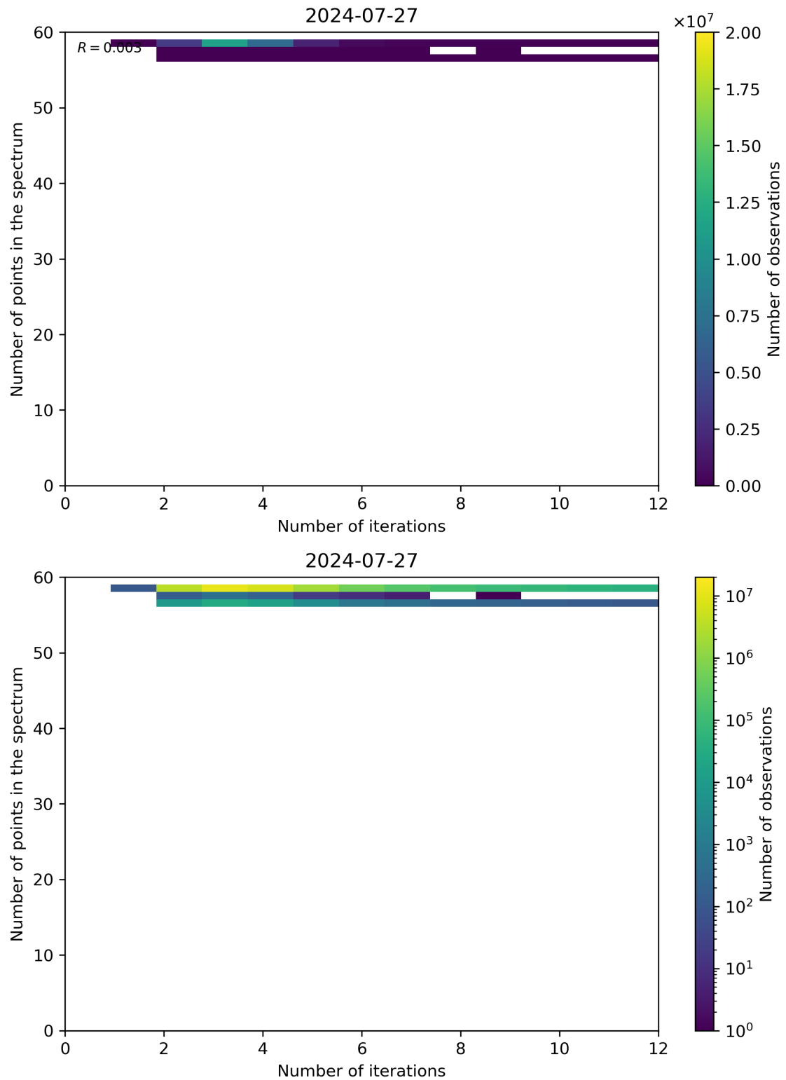
Figure 99: Scatter density plot of “Number of iterations” against “Number of points in the spectrum” for 2024-07-26 to 2024-07-28.
