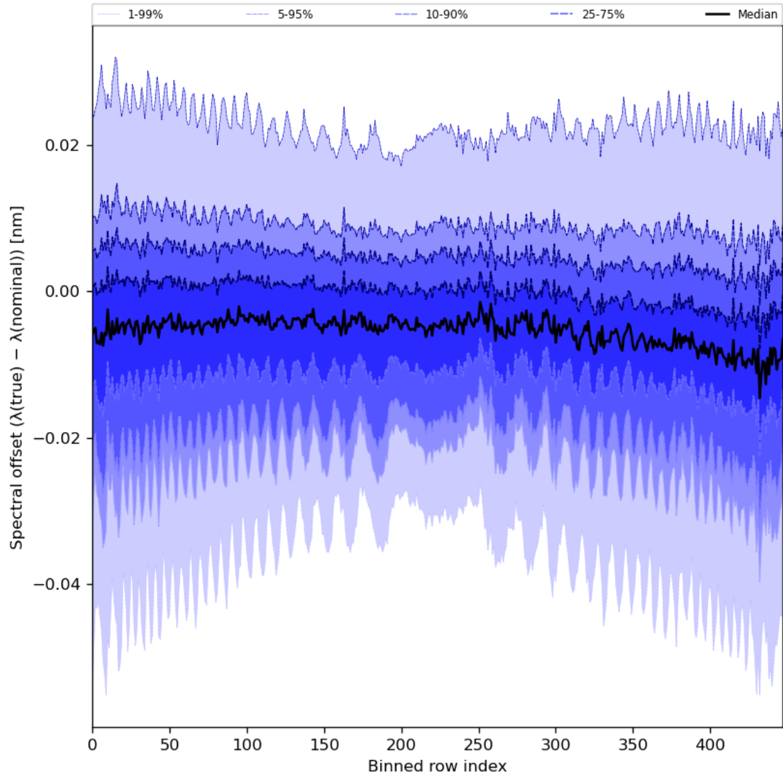
Figure 62: Along track statistics of “Spectral offset ( \lambda(\text{true}) - \lambda(\text{nominal}) )” for 2024-07-26 to 2024-07-28
