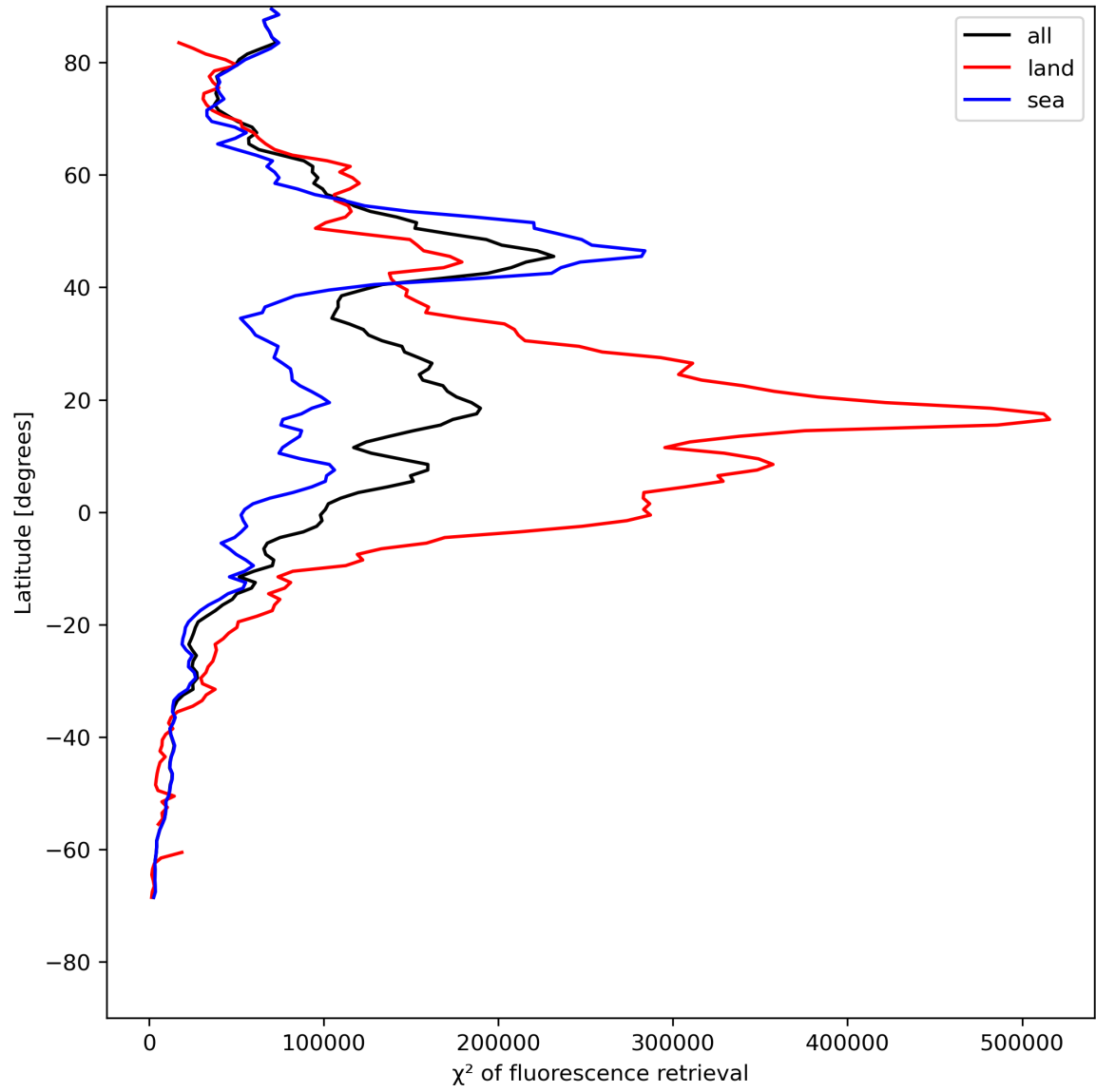
Figure 25: Zonal average of “ \chi^2 of fluorescence retrieval” for 2024-07-26 to 2024-07-28.
