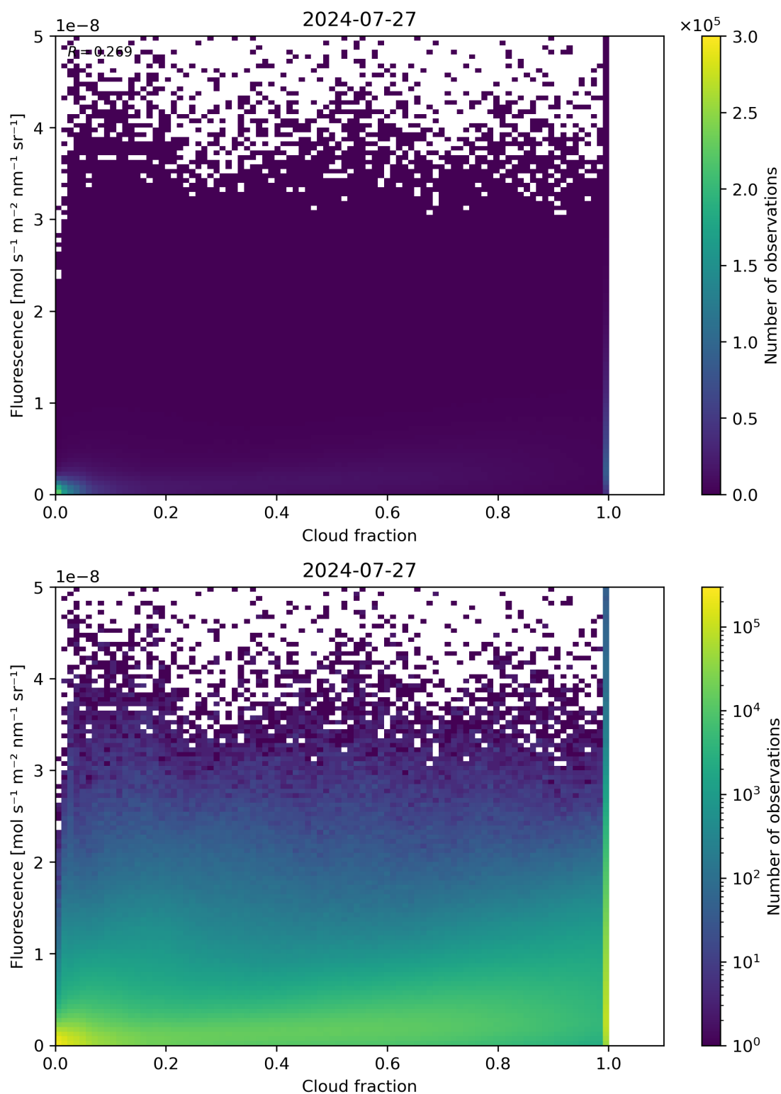
Figure 72: Scatter density plot of “Cloud fraction” against “Fluorescence” for 2024-07-26 to 2024-07-28.
