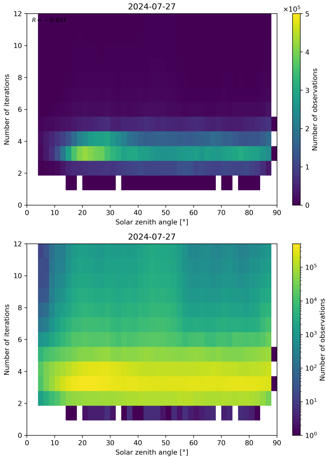
Figure 114: Scatter density plot of “Solar zenith angle” against “Number of iterations” for 2024-07-26 to 2024-07-28.
