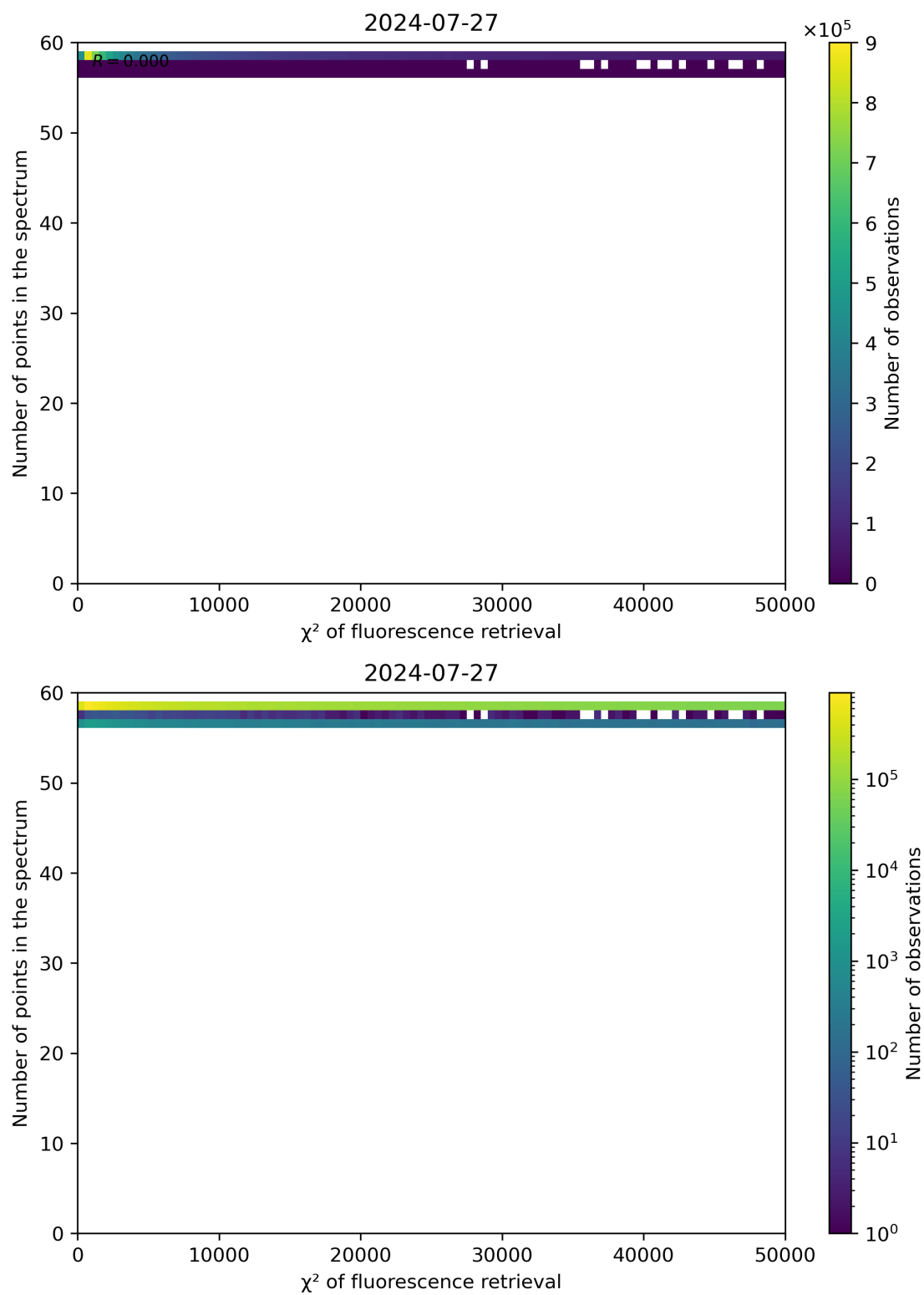
Figure 68: Scatter density plot of " \chi^2 of fluorescence retrieval" against "Number of points in the spectrum" for 2024-07-26 to 2024-07-28.
