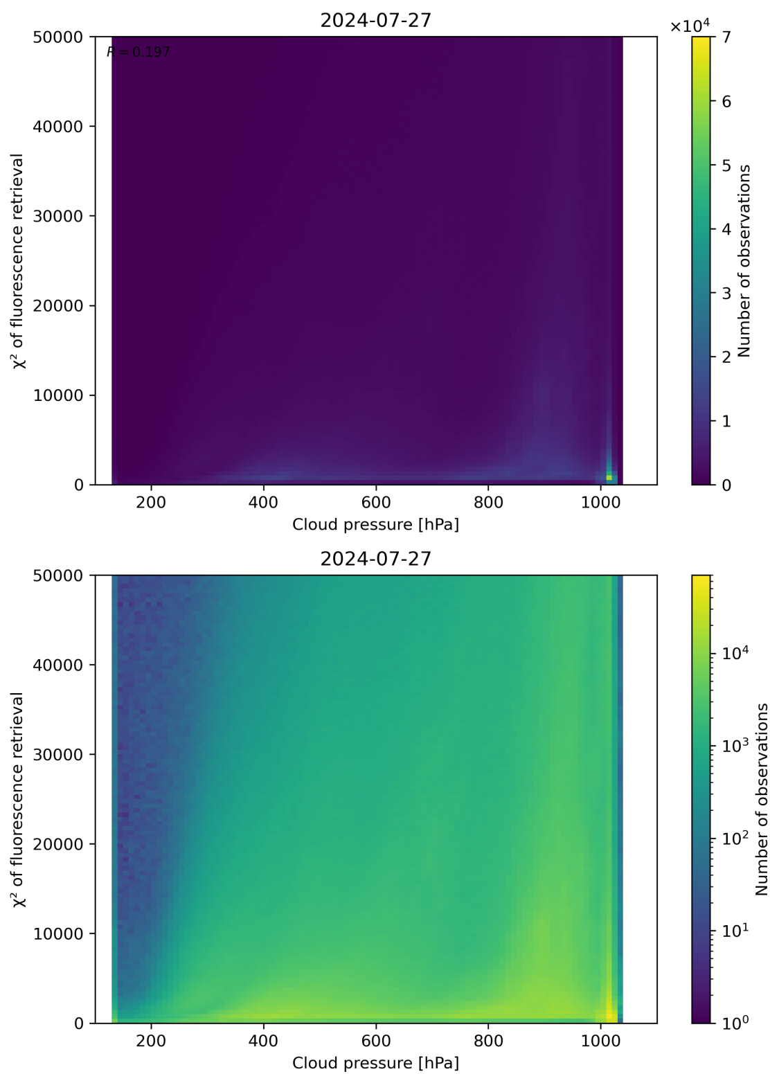
Figure 78: Scatter density plot of “Cloud pressure” against “ \chi^2 of fluorescence retrieval” for 2024-07-26 to 2024-07-28.
