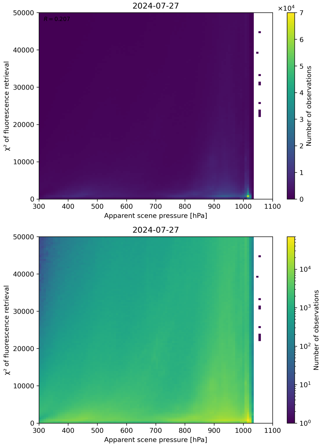
Figure 63: Scatter density plot of “Apparent scene pressure” against “ \chi^2 of fluorescence retrieval” for 2024-07-26 to 2024-07-28.
