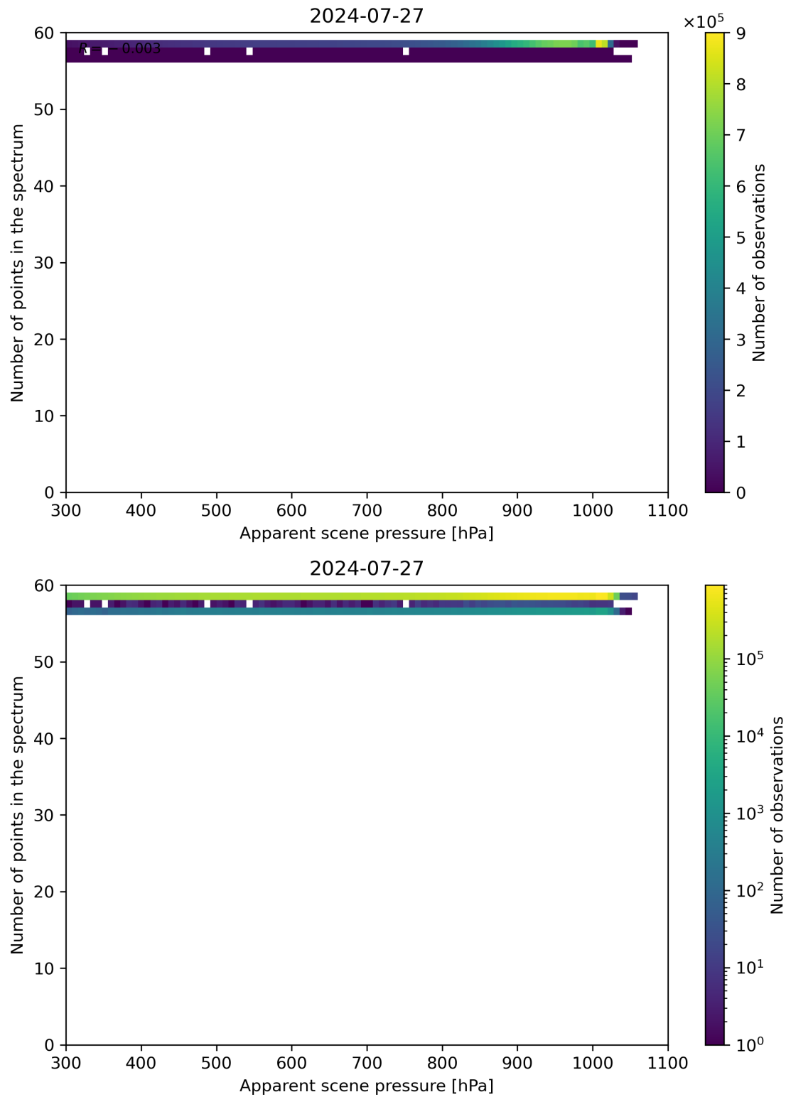
Figure 66: Scatter density plot of “Apparent scene pressure” against “Number of points in the spectrum” for 2024-07-26 to 2024-07-28.
