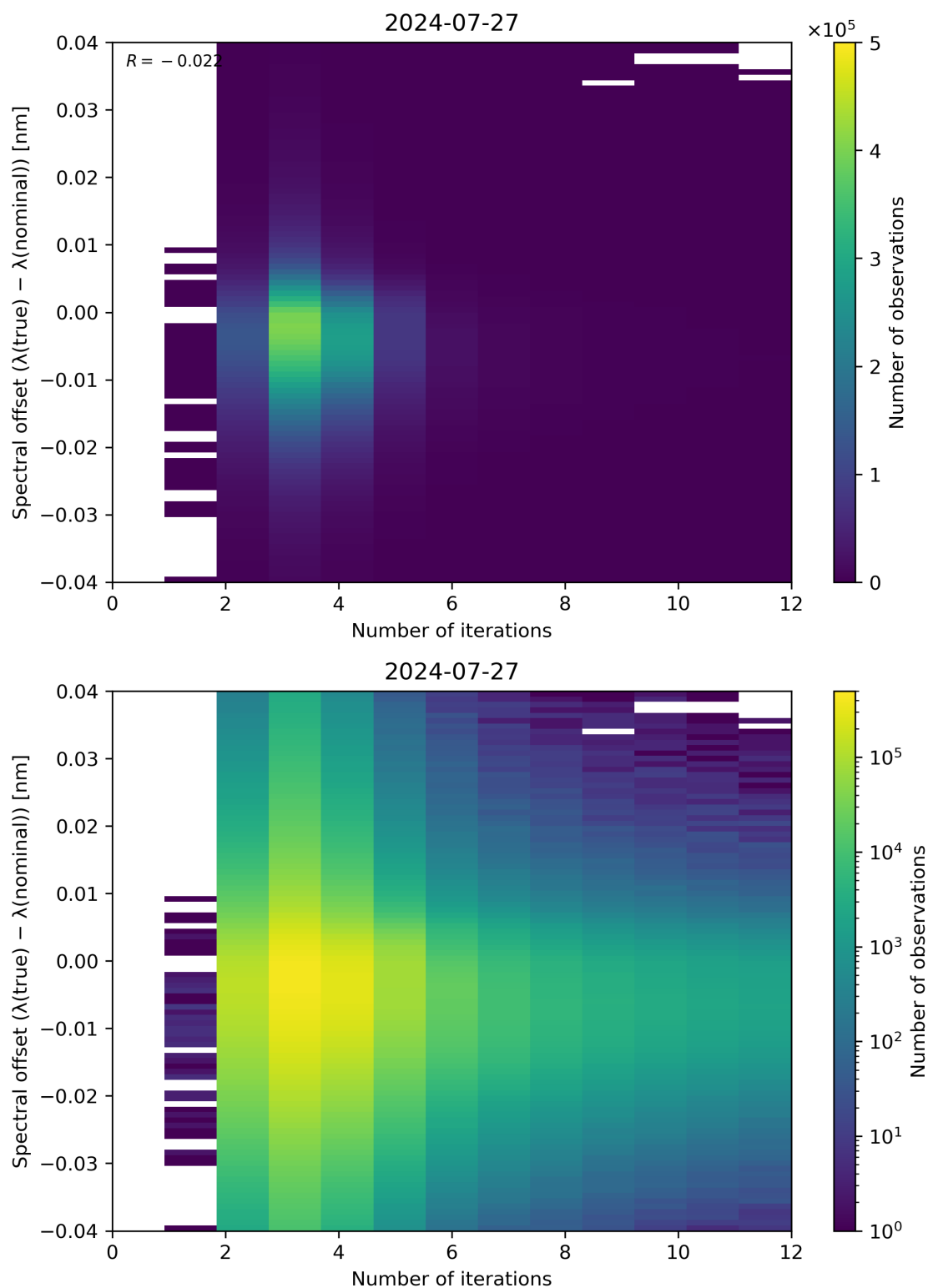
Figure 100: Scatter density plot of “Number of iterations” against “Spectral offset ( \lambda(\text{true}) - \lambda(\text{nominal}) )” for 2024-07-26 to 2024-07-28.
