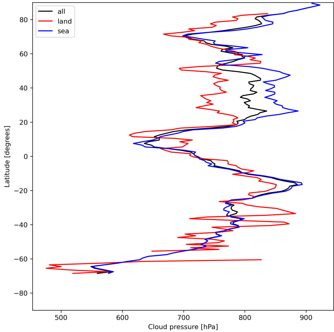
Figure 13: Zonal average of “Cloud pressure” for 2024-07-26 to 2024-07-28.
