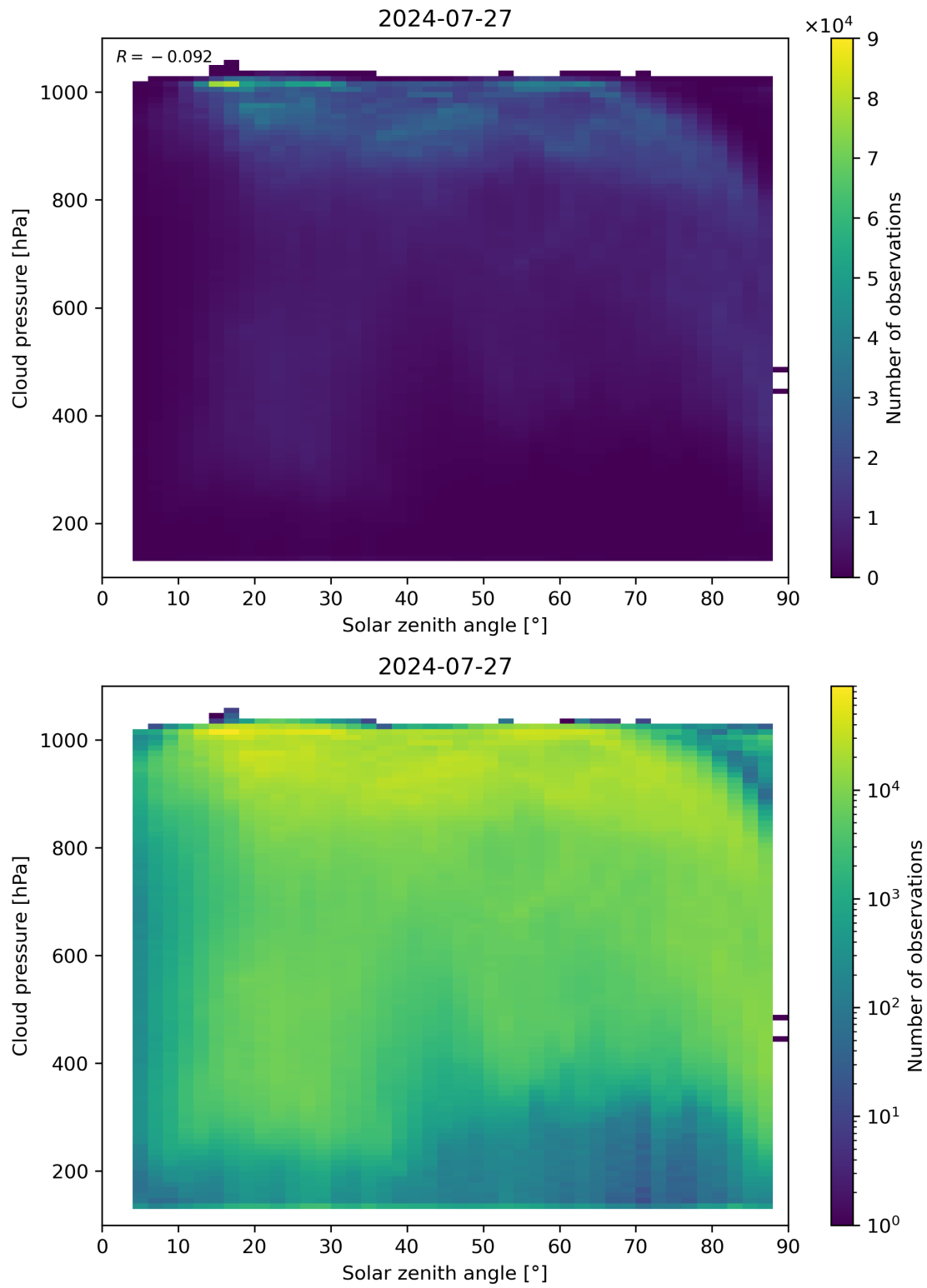
Figure 111: Scatter density plot of “Solar zenith angle” against “Cloud pressure” for 2024-07-26 to 2024-07-28.
