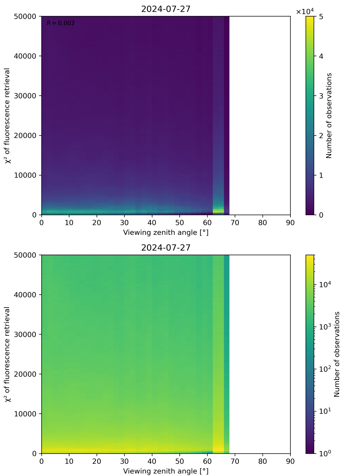
Figure 119: Scatter density plot of “Viewing zenith angle” against “ \chi^2 of fluorescence retrieval” for 2024-07-26 to 2024-07-28.
