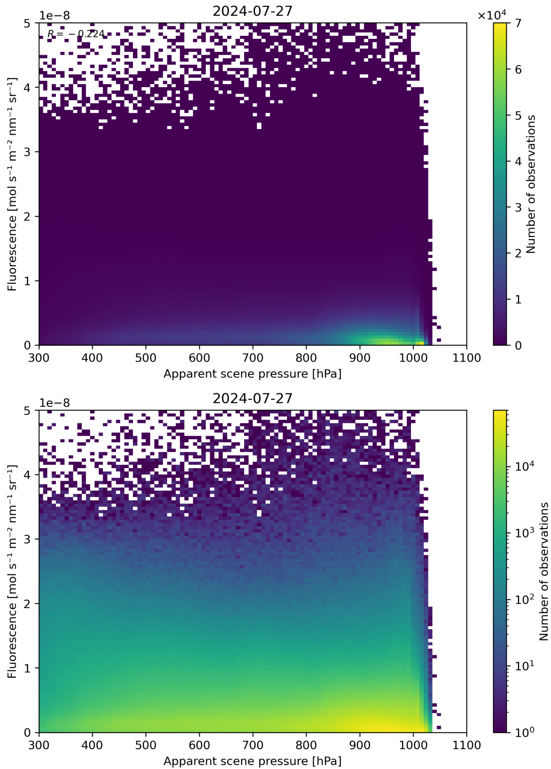
Figure 64: Scatter density plot of “Apparent scene pressure” against “Fluorescence” for 2024-07-26 to 2024-07-28.
