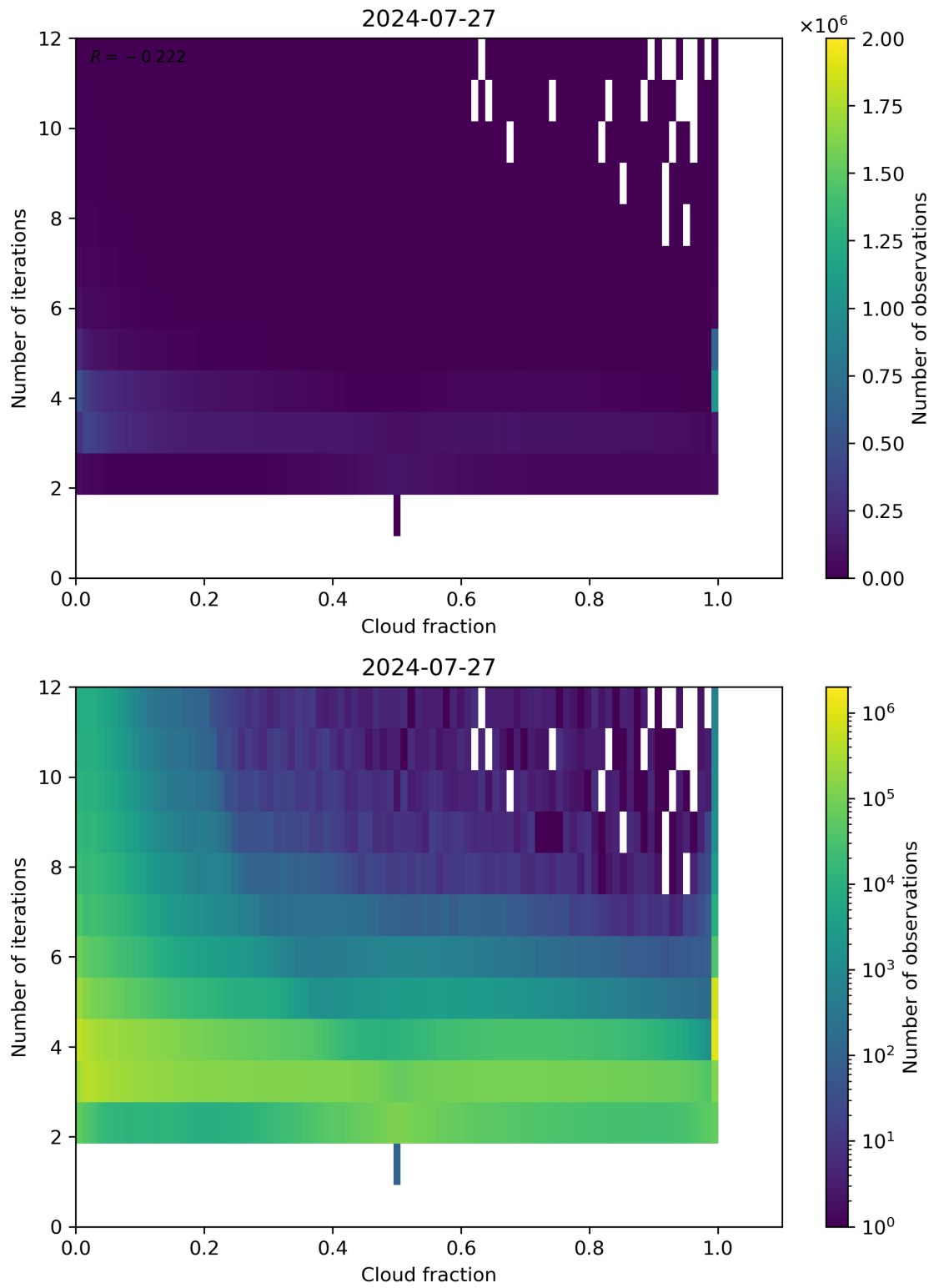
Figure 73: Scatter density plot of “Cloud fraction” against “Number of iterations” for 2024-07-26 to 2024-07-28.
