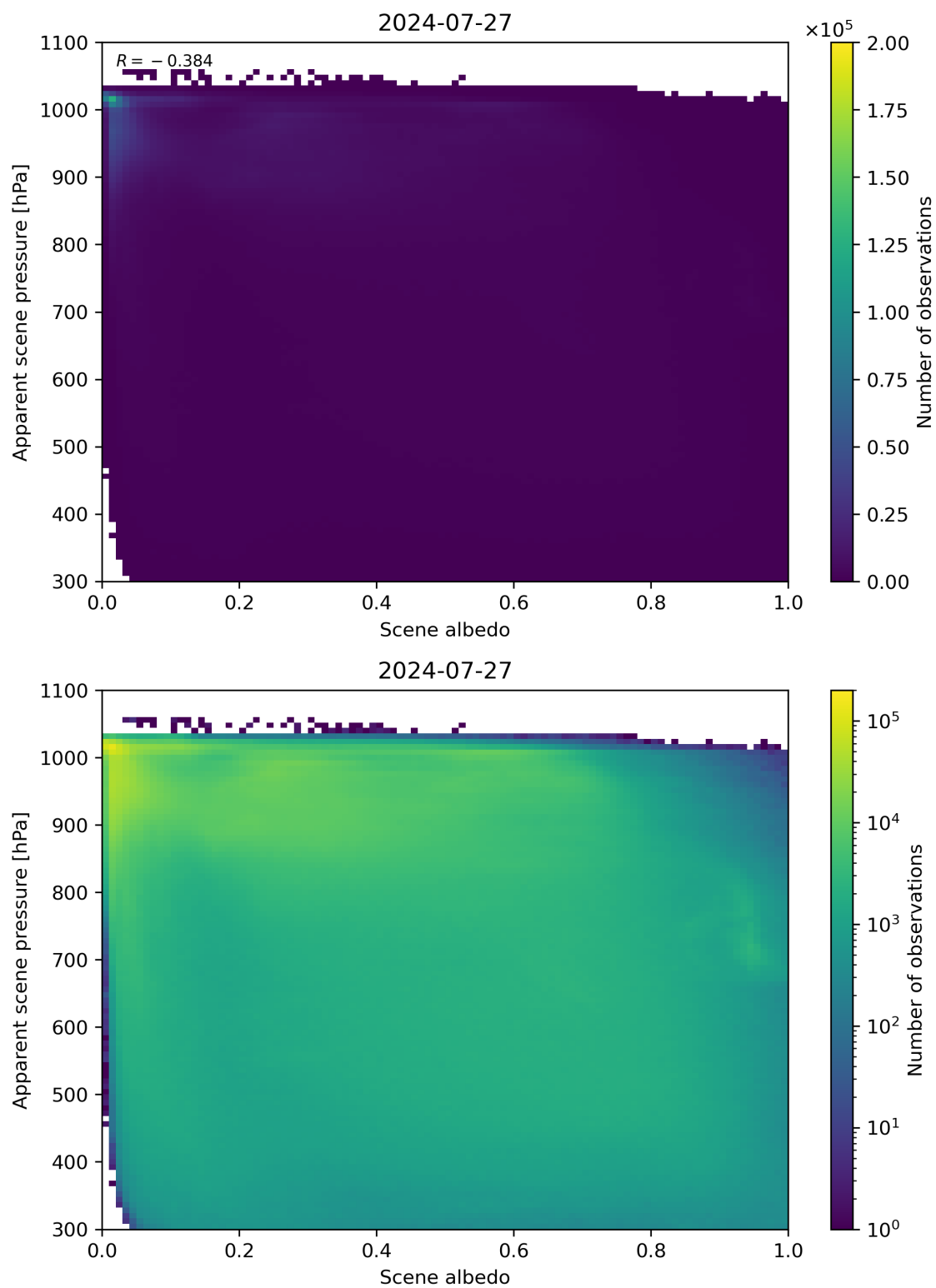
Figure 102: Scatter density plot of “Scene albedo” against “Apparent scene pressure” for 2024-07-26 to 2024-07-28.
