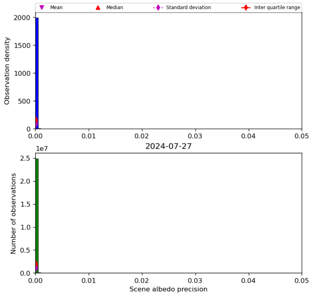
Figure 35: Histogram of “Scene albedo precision” for 2024-07-26 to 2024-07-28
