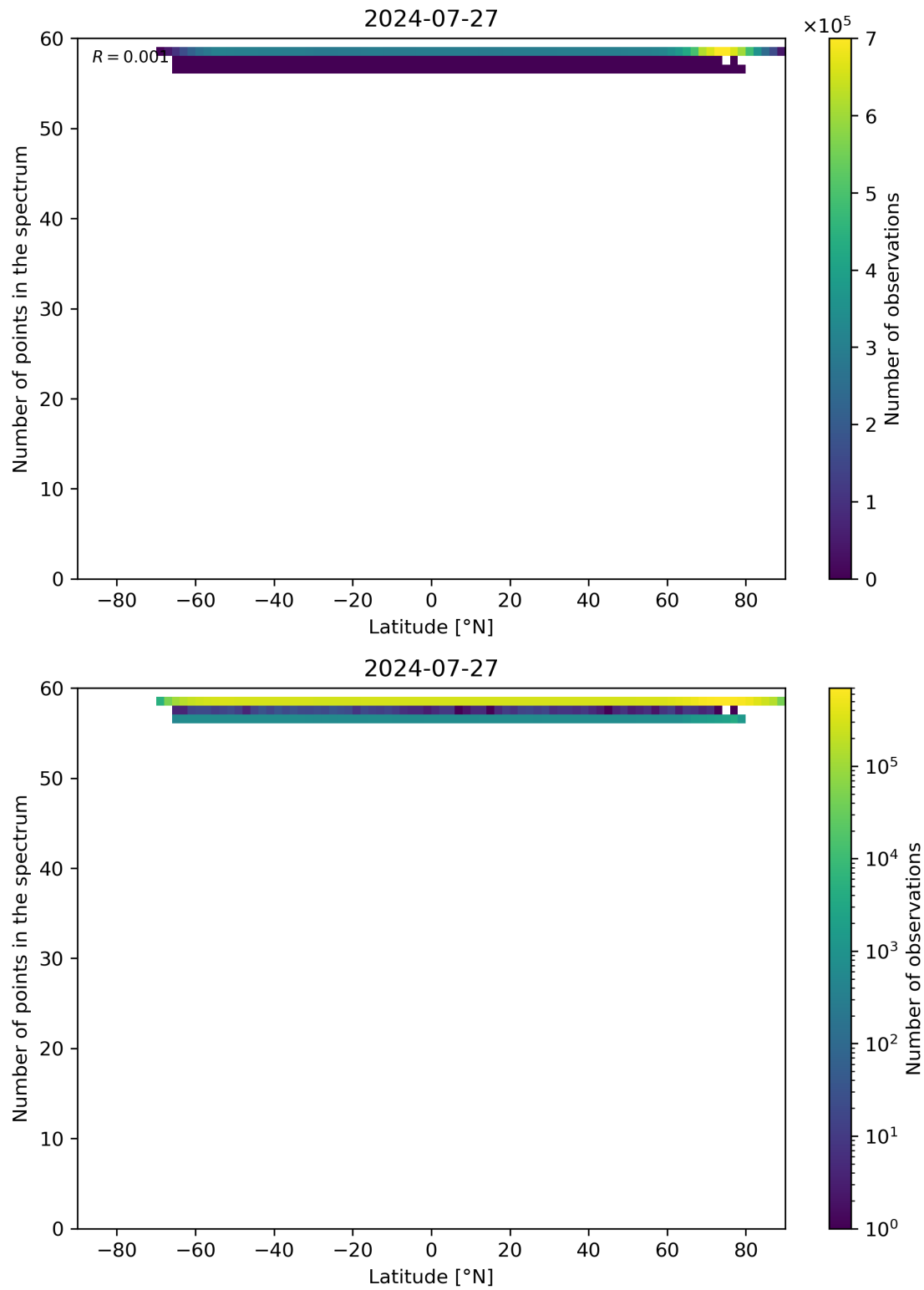
Figure 94: Scatter density plot of “Latitude” against “Number of points in the spectrum” for 2024-07-26 to 2024-07-28.
