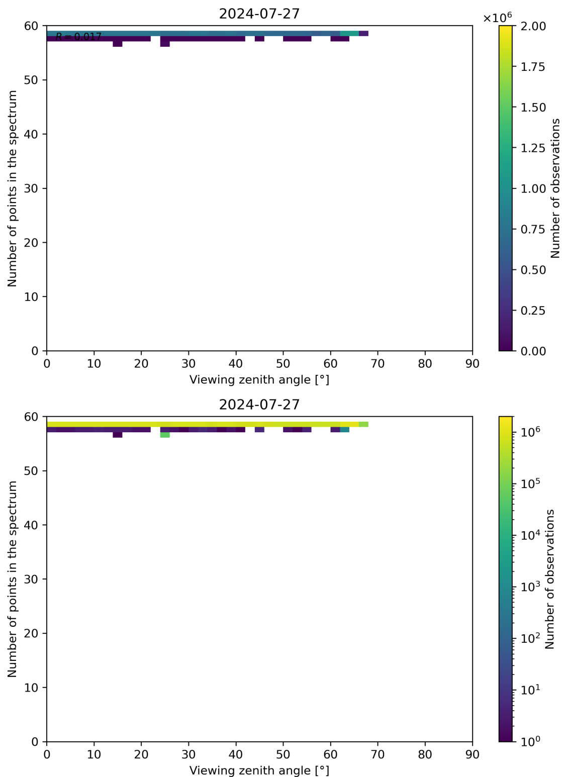
Figure 125: Scatter density plot of “Viewing zenith angle” against “Number of points in the spectrum” for 2024-07-26 to 2024-07-28.
