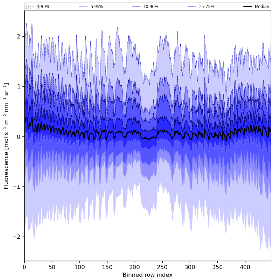
Figure 57: Along track statistics of “Fluorescence” for 2024-07-26 to 2024-07-28
