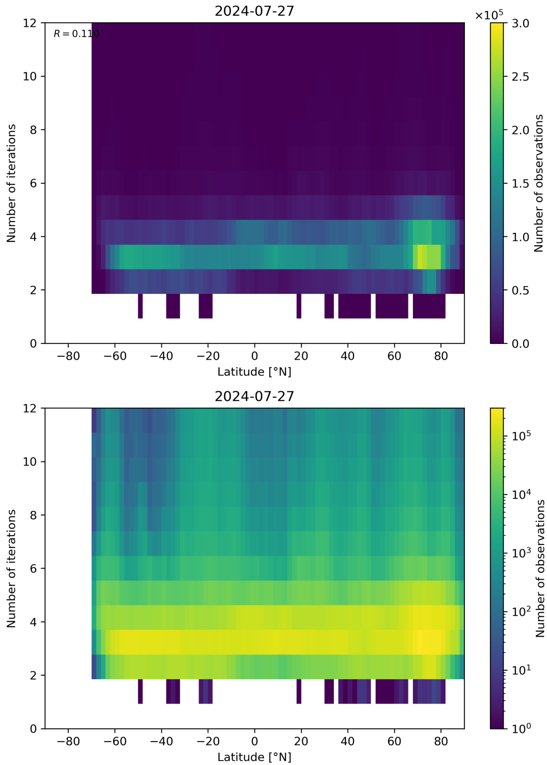
Figure 93: Scatter density plot of “Latitude” against “Number of iterations” for 2024-07-26 to 2024-07-28.
