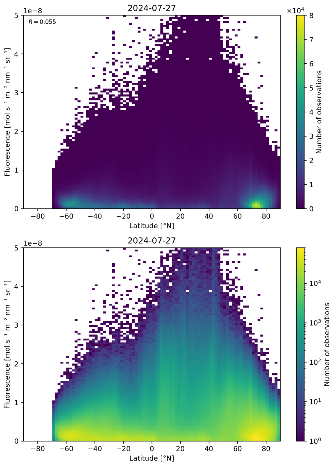
Figure 92: Scatter density plot of “Latitude” against “Fluorescence” for 2024-07-26 to 2024-07-28.
