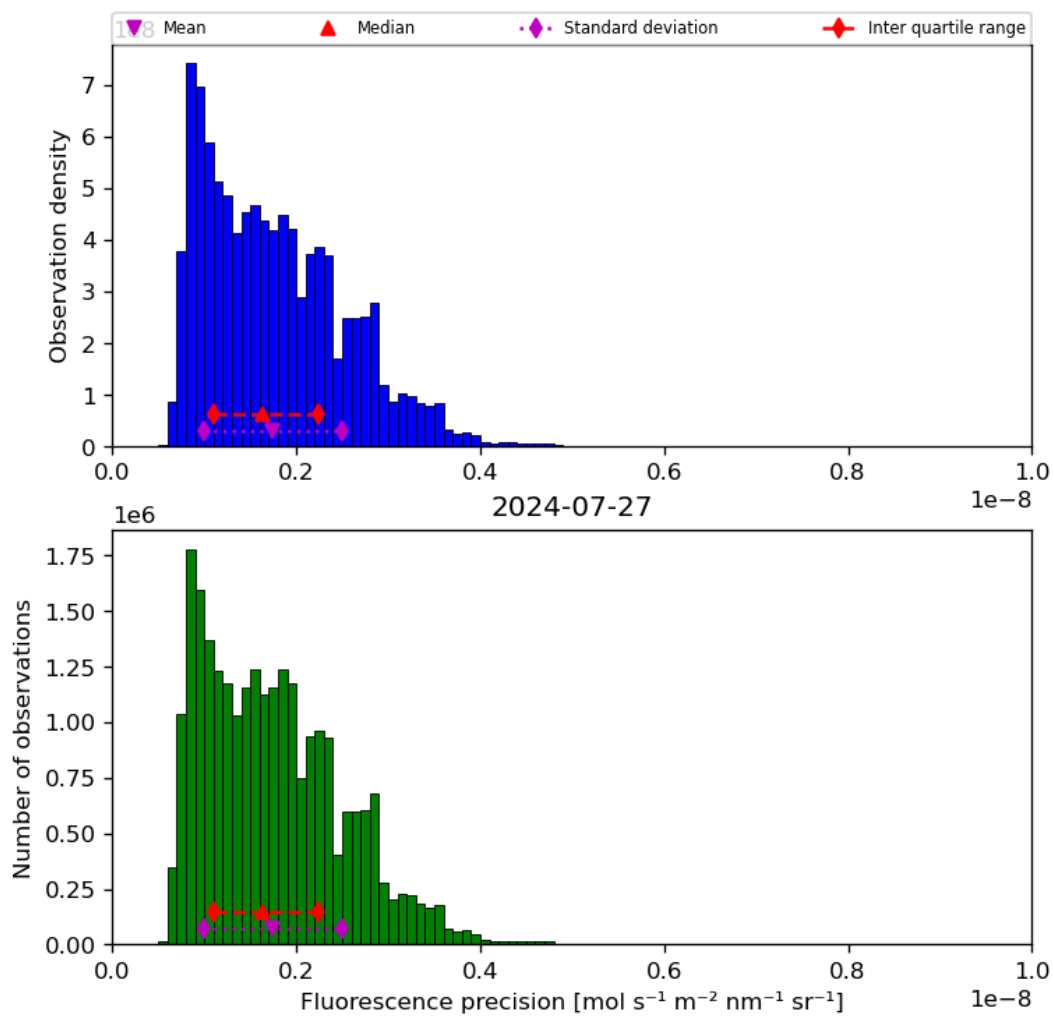
Figure 41: Histogram of “Fluorescence precision” for 2024-07-26 to 2024-07-28
