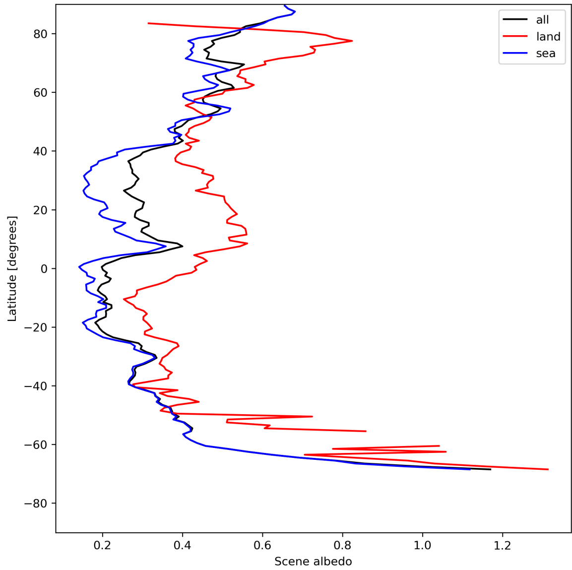
Figure 17: Zonal average of “Scene albedo” for 2024-07-26 to 2024-07-28.
