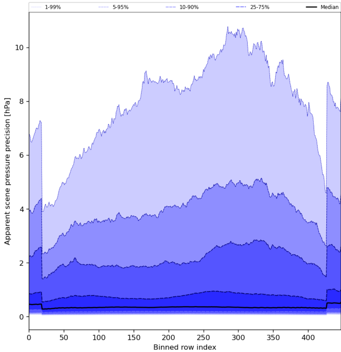
Figure 54: Along track statistics of “Apparent scene pressure precision” for 2024-07-26 to 2024-07-28
