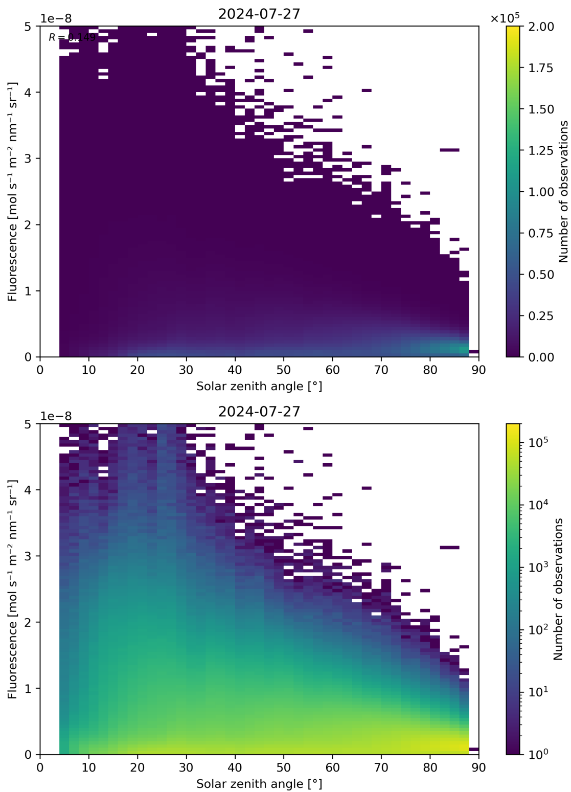
Figure 112: Scatter density plot of “Solar zenith angle” against “Fluorescence” for 2024-07-26 to 2024-07-28.
