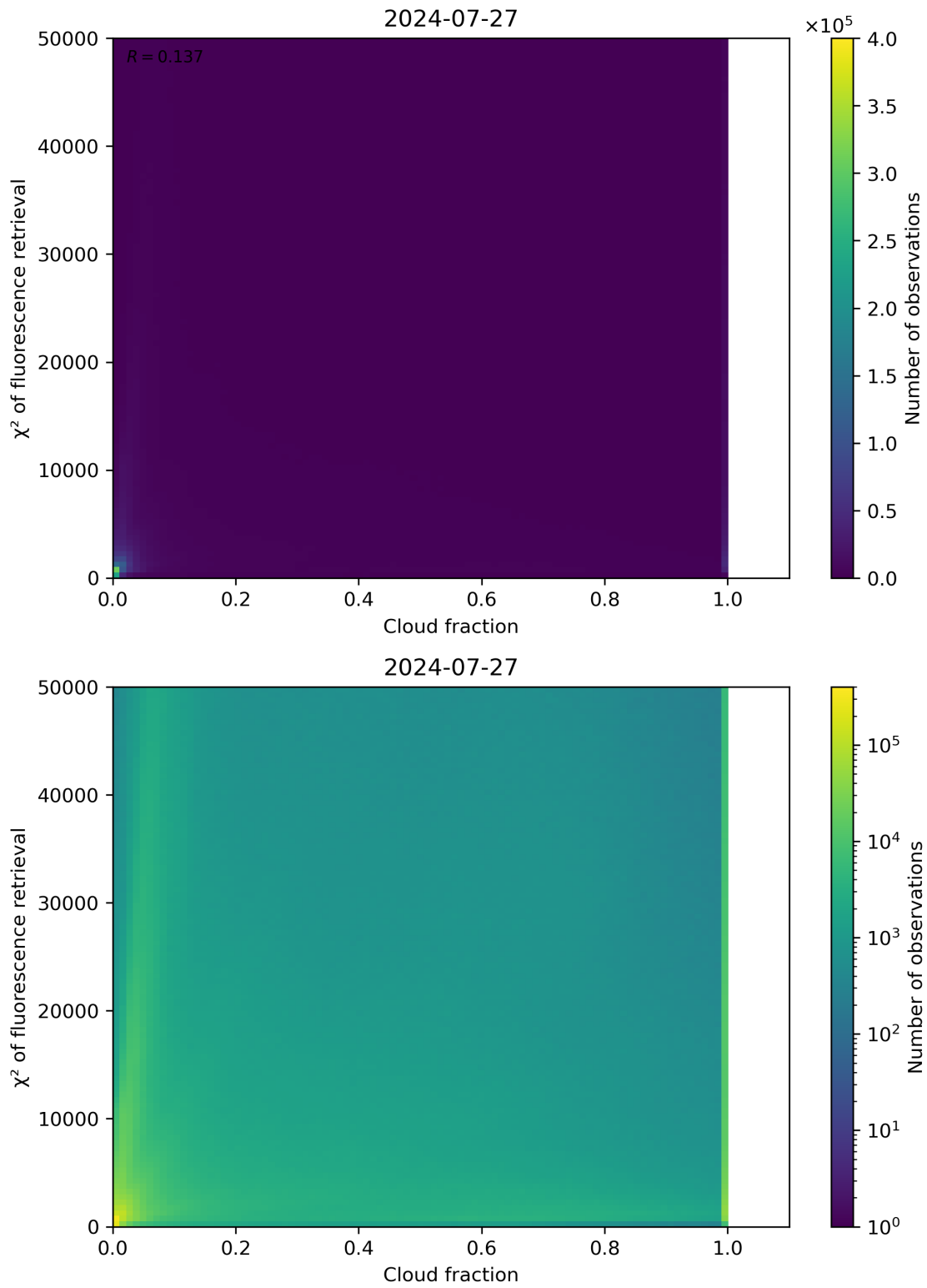
Figure 71: Scatter density plot of “Cloud fraction” against “ \chi^2 of fluorescence retrieval” for 2024-07-26 to 2024-07-28.
