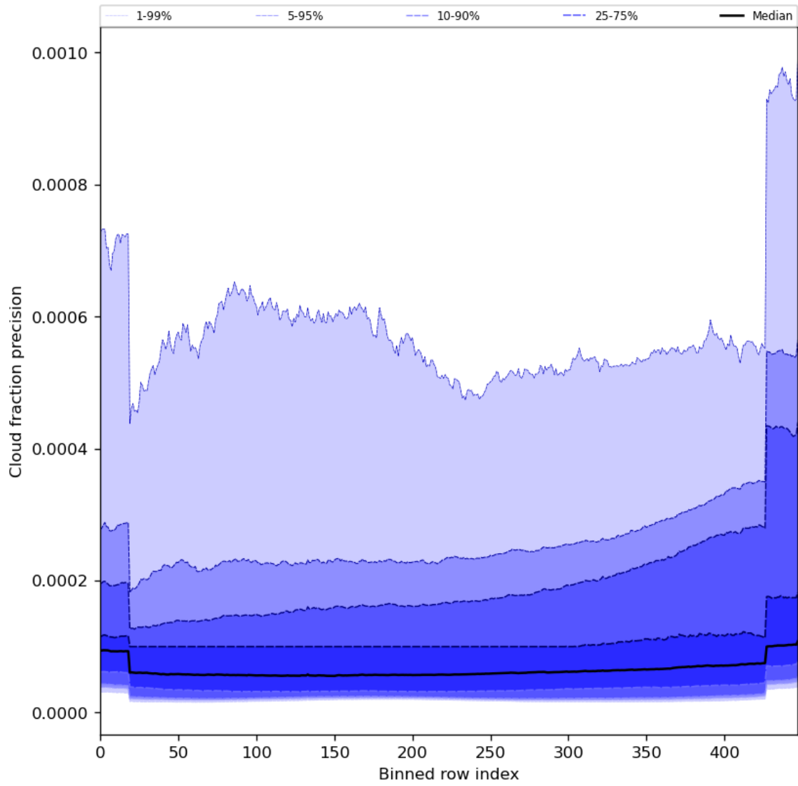
Figure 50: Along track statistics of “Cloud fraction precision” for 2024-07-26 to 2024-07-28
