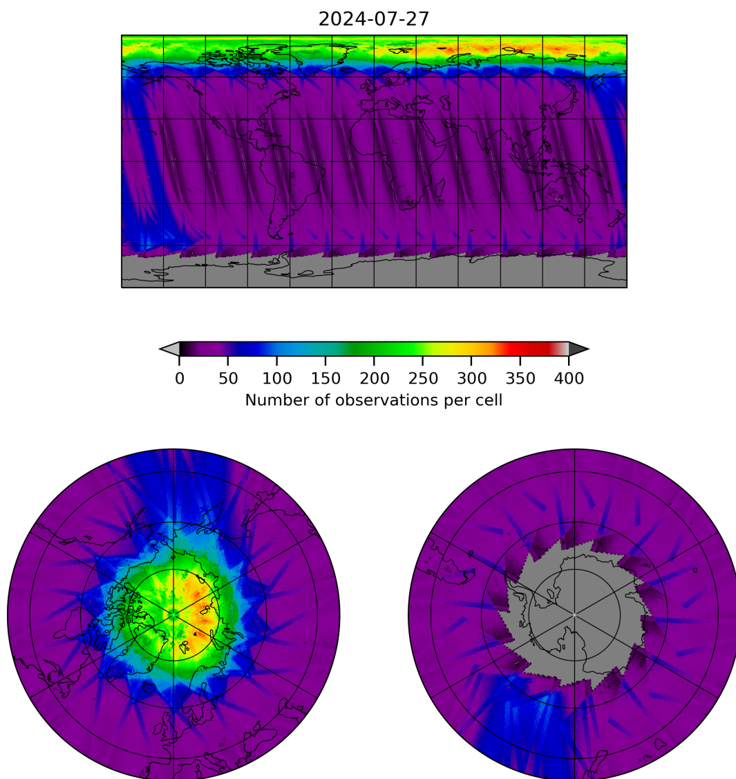
Figure 11: Map of the number of observations for 2024-07-26 to 2024-07-28
