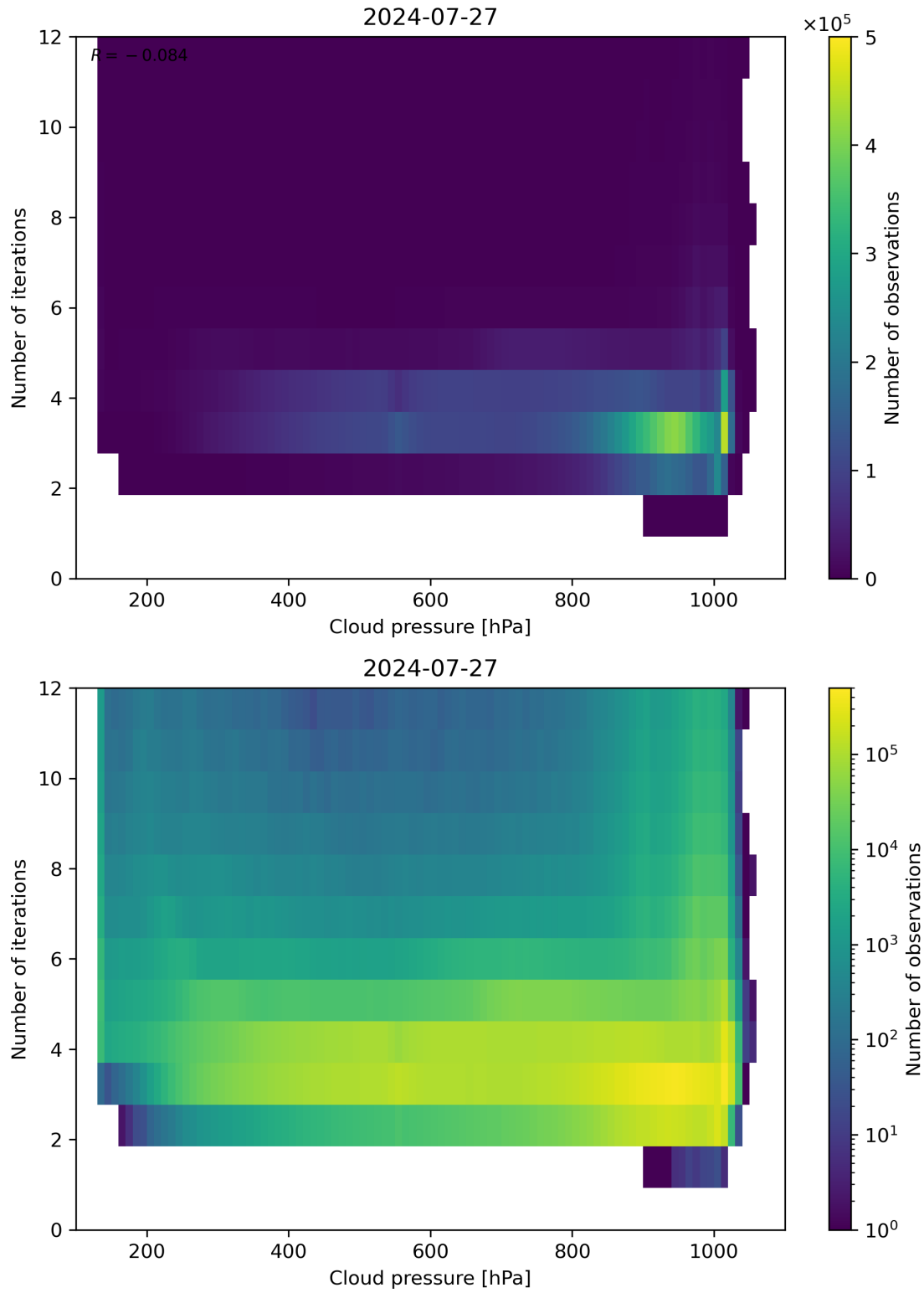
Figure 81: Scatter density plot of “Cloud pressure” against “Number of iterations” for 2024-07-26 to 2024-07-28.
