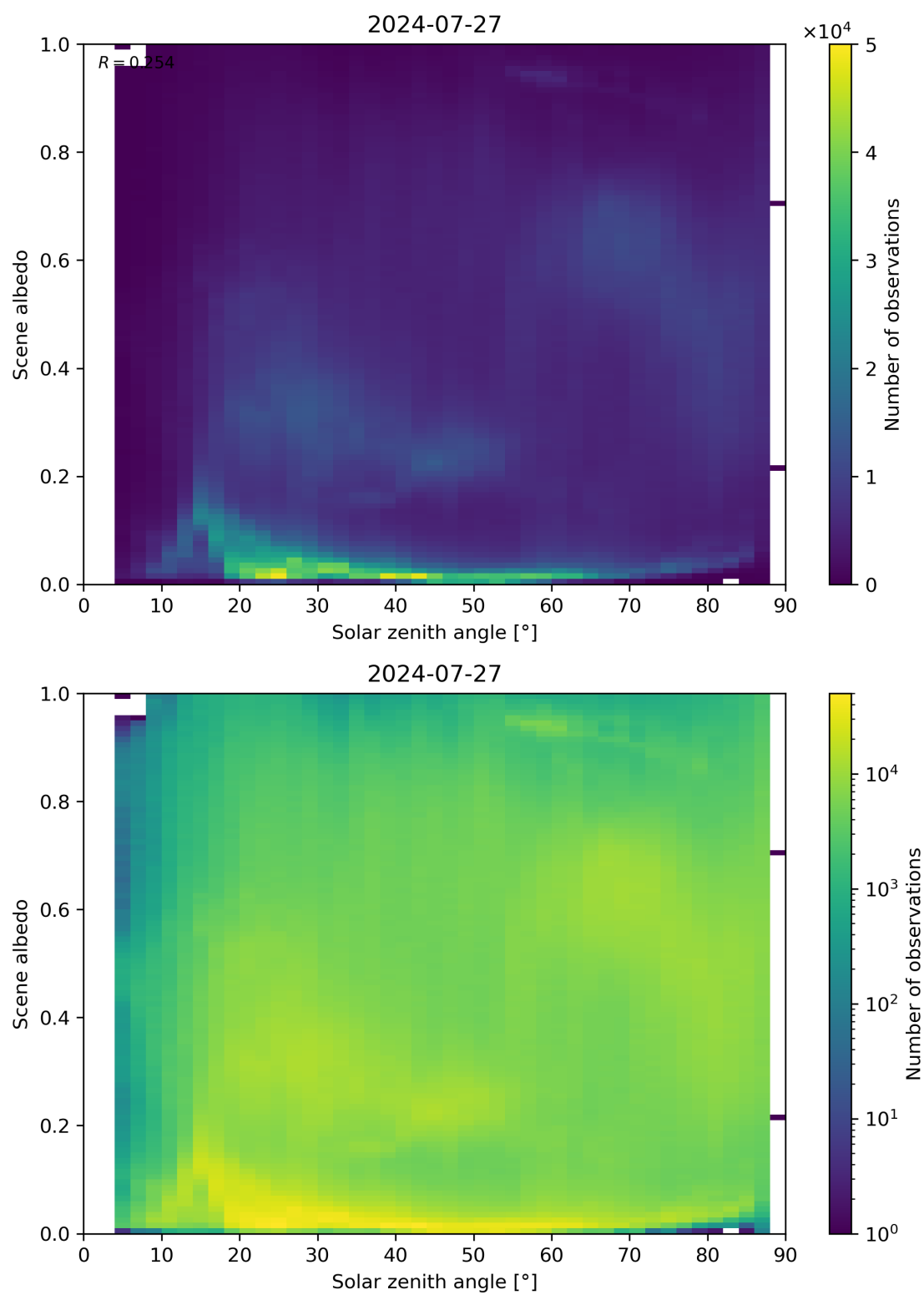
Figure 116: Scatter density plot of “Solar zenith angle” against “Scene albedo” for 2024-07-26 to 2024-07-28.
