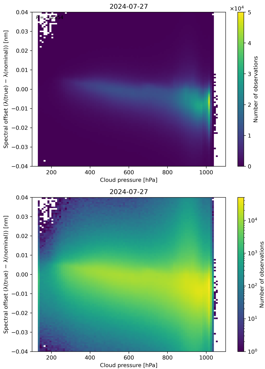
Figure 84: Scatter density plot of “Cloud pressure” against “Spectral offset ( \lambda(\text{true}) - \lambda(\text{nominal}) )” for 2024-07-26 to 2024-07-28.
