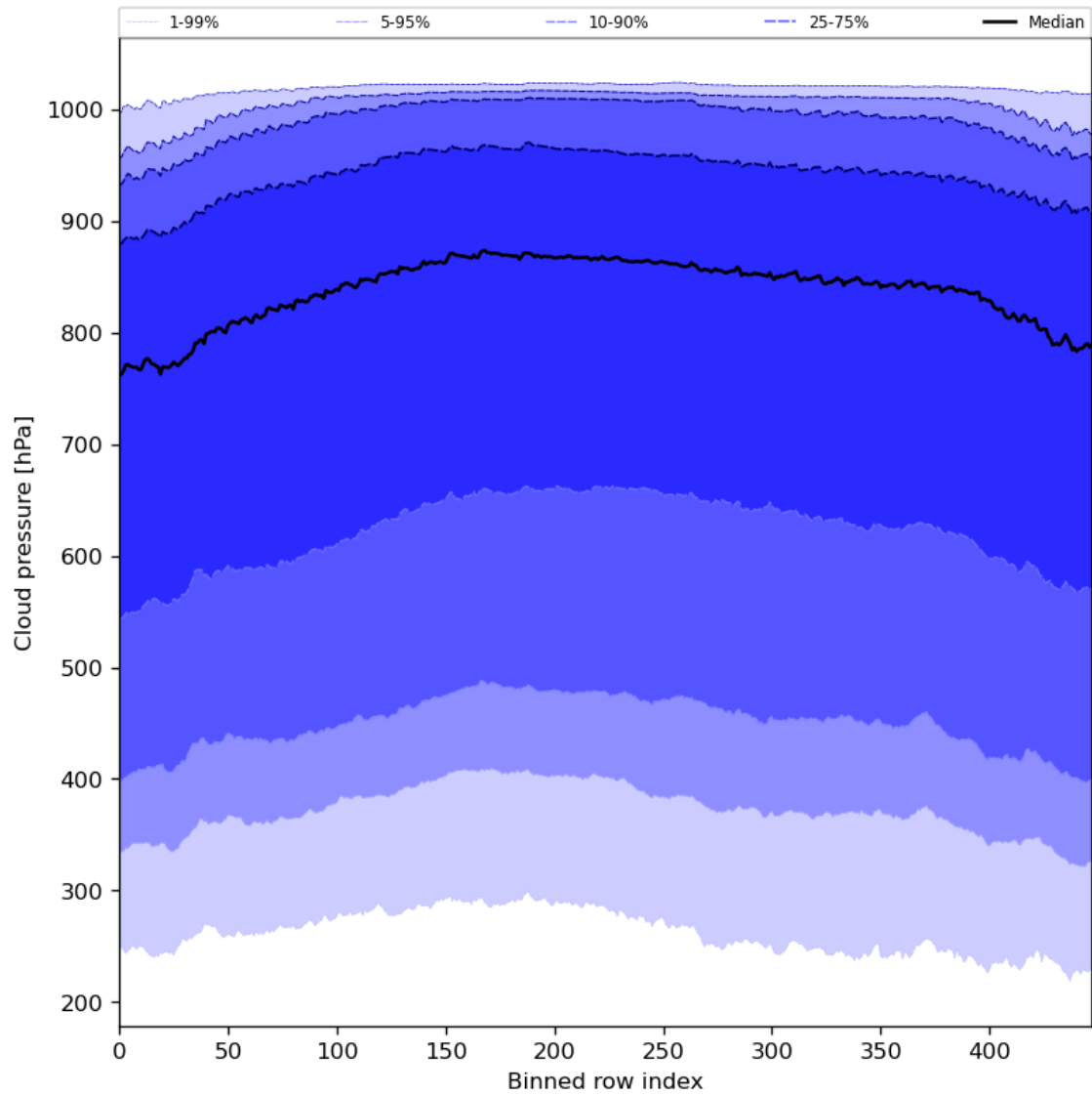
Figure 47: Along track statistics of “Cloud pressure” for 2024-07-26 to 2024-07-28
