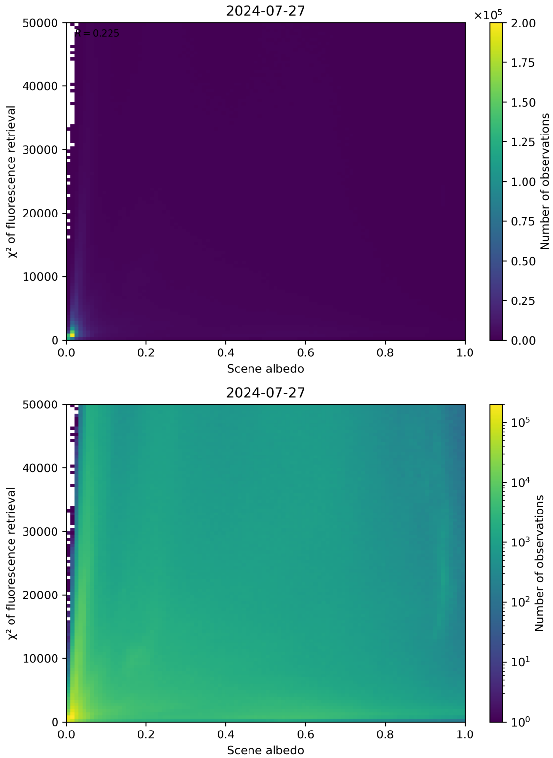
Figure 103: Scatter density plot of “Scene albedo” against “ \chi^2 of fluorescence retrieval” for 2024-07-26 to 2024-07-28.
