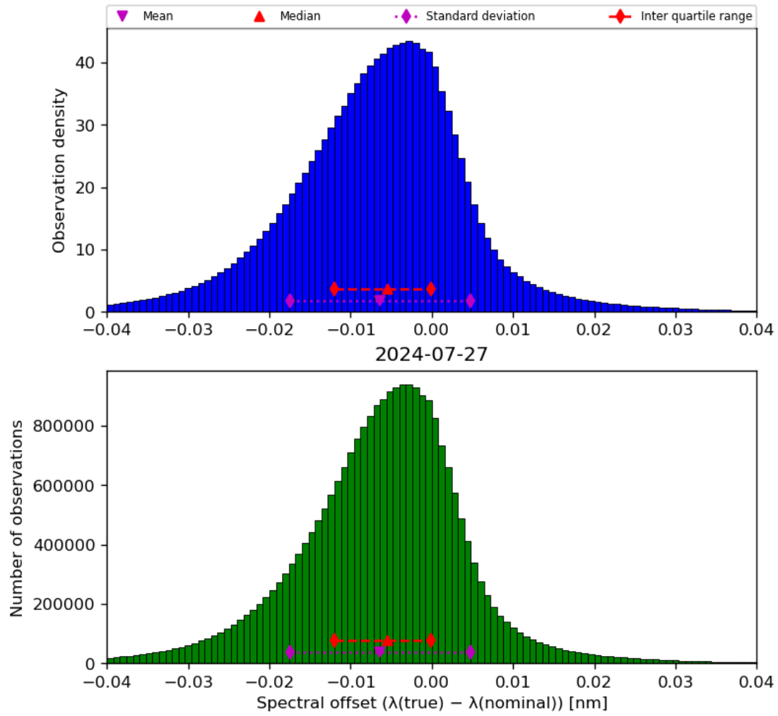
Figure 45: Histogram of “Spectral offset ( \lambda(\text{true}) - \lambda(\text{nominal}) )” for 2024-07-26 to 2024-07-28
