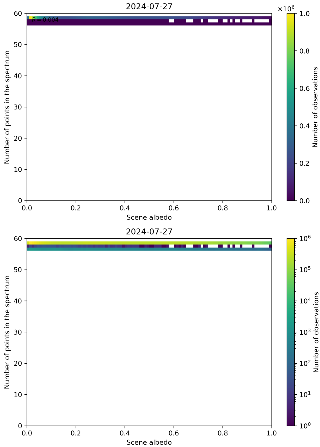
Figure 106: Scatter density plot of “Scene albedo” against “Number of points in the spectrum” for 2024-07-26 to 2024-07-28.
