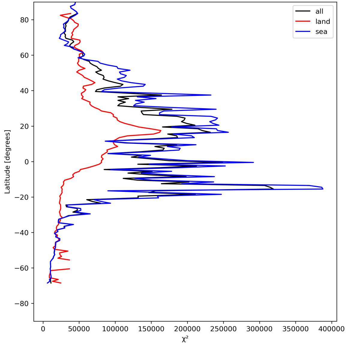
Figure 21: Zonal average of “ \chi^2 ” for 2024-07-26 to 2024-07-28.
