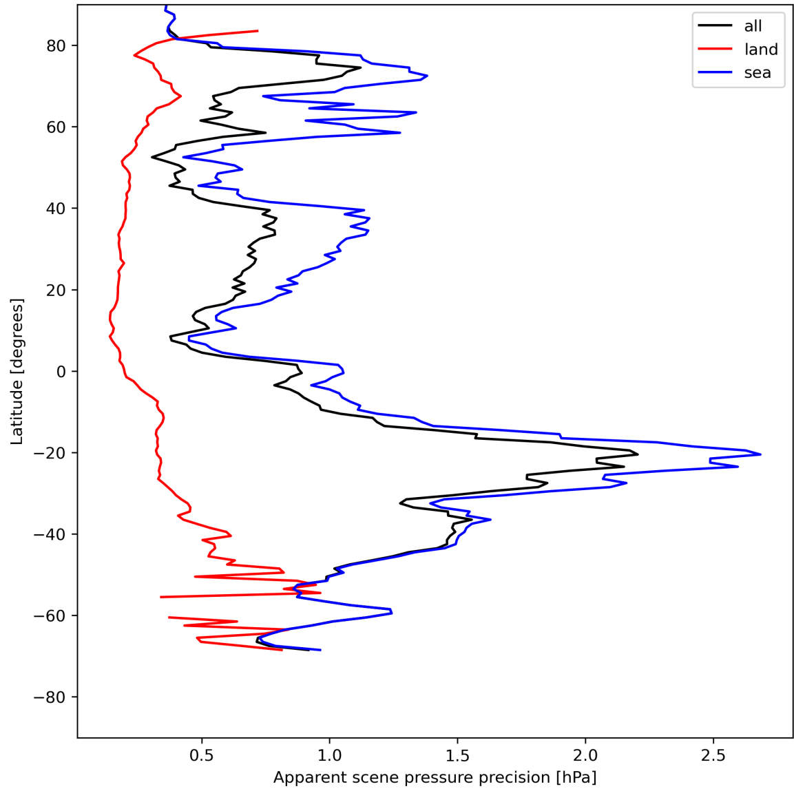
Figure 20: Zonal average of “Apparent scene pressure precision” for 2024-07-26 to 2024-07-28.
