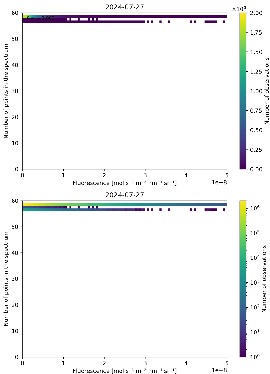
Figure 86: Scatter density plot of “Fluorescence” against “Number of points in the spectrum” for 2024-07-26 to 2024-07-28.
