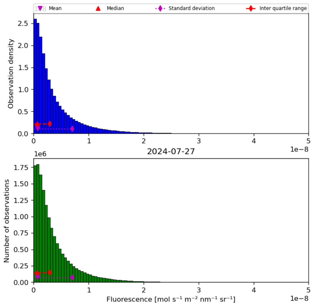
Figure 40: Histogram of “Fluorescence” for 2024-07-26 to 2024-07-28
