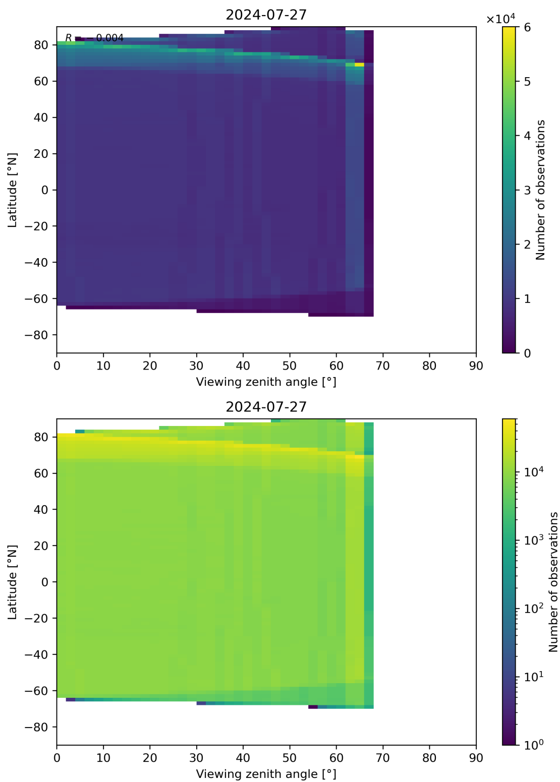
Figure 123: Scatter density plot of “Viewing zenith angle” against “Latitude” for 2024-07-26 to 2024-07-28.
