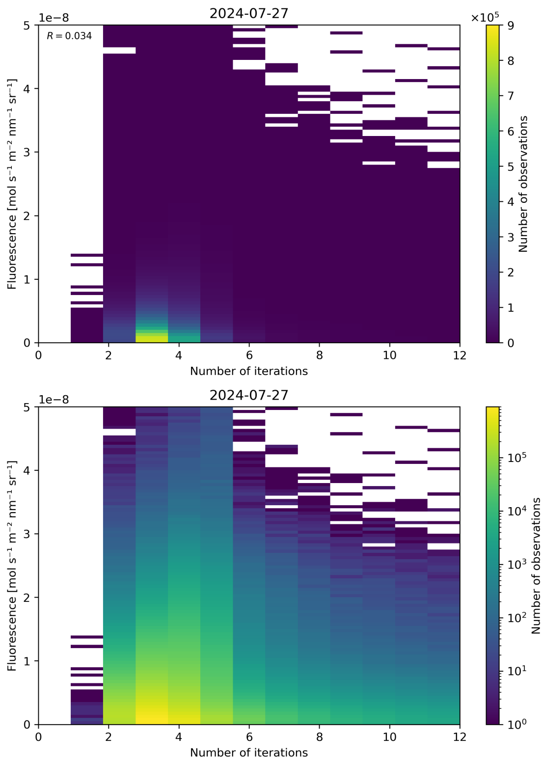
Figure 98: Scatter density plot of “Number of iterations” against “Fluorescence” for 2024-07-26 to 2024-07-28.
