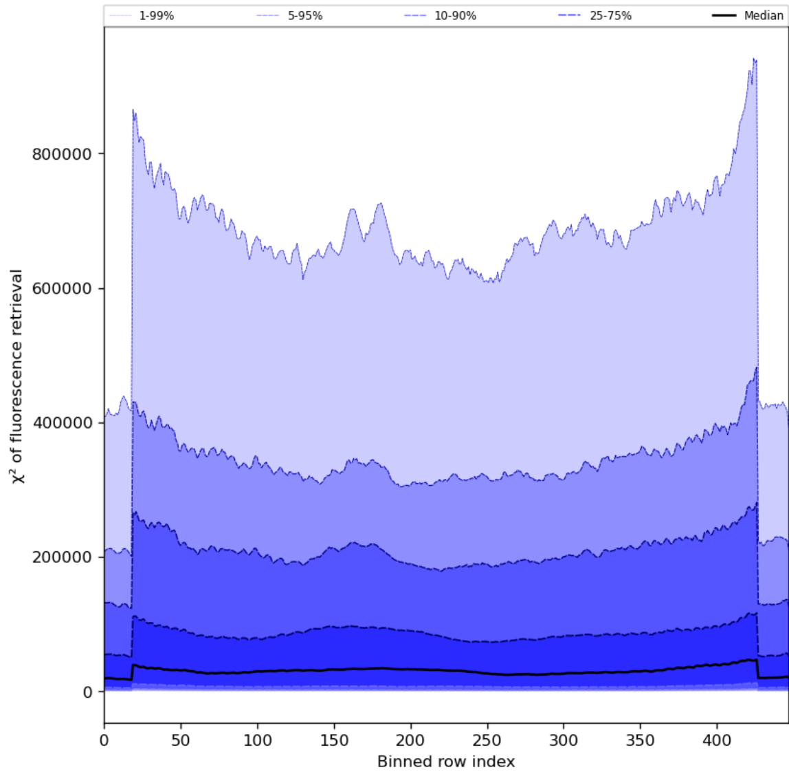
Figure 59: Along track statistics of “ \chi^2 of fluorescence retrieval” for 2024-07-26 to 2024-07-28
