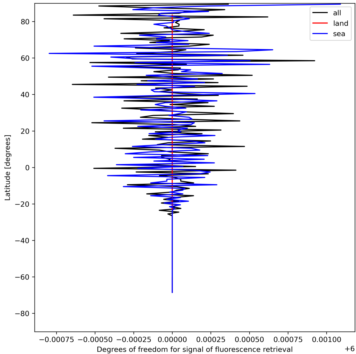
Figure 26: Zonal average of “Degrees of freedom for signal of fluorescence retrieval” for 2024-07-26 to 2024-07-28.
