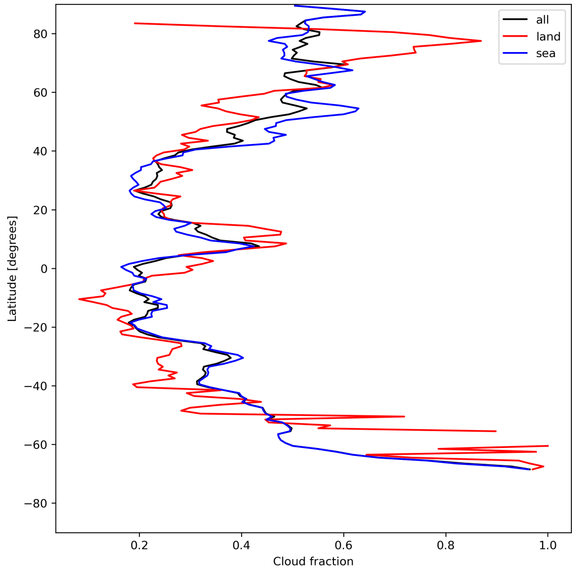
Figure 15: Zonal average of “Cloud fraction” for 2024-07-26 to 2024-07-28.
