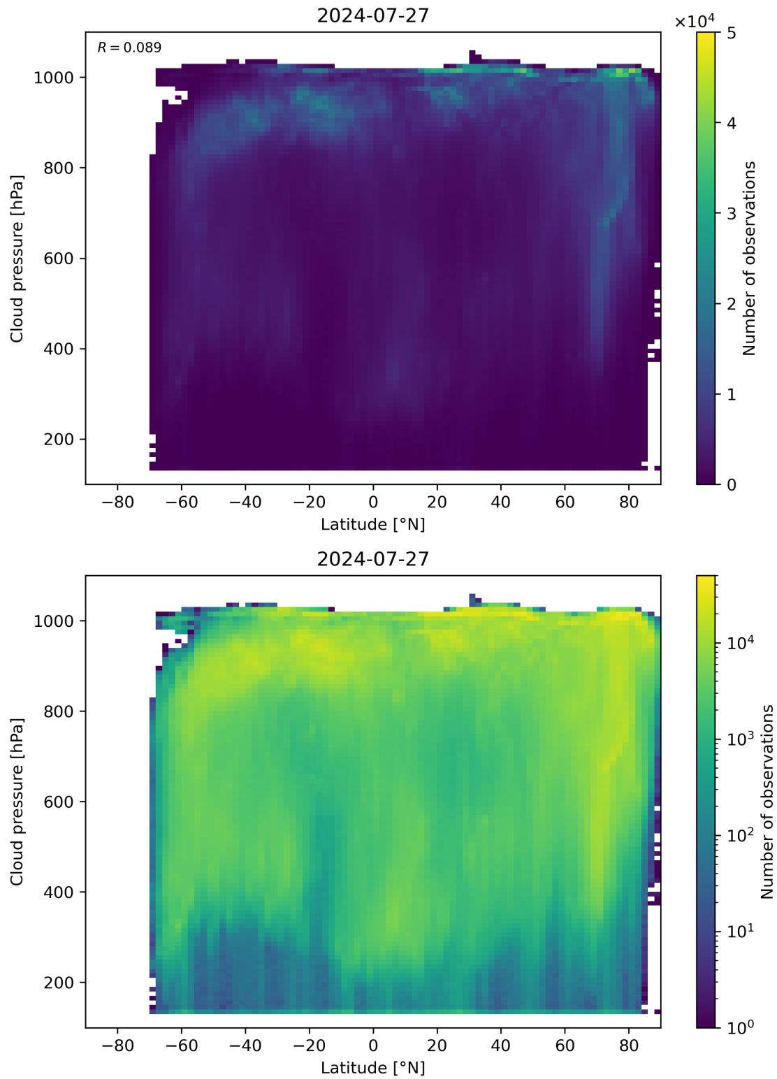
Figure 91: Scatter density plot of “Latitude” against “Cloud pressure” for 2024-07-26 to 2024-07-28.
