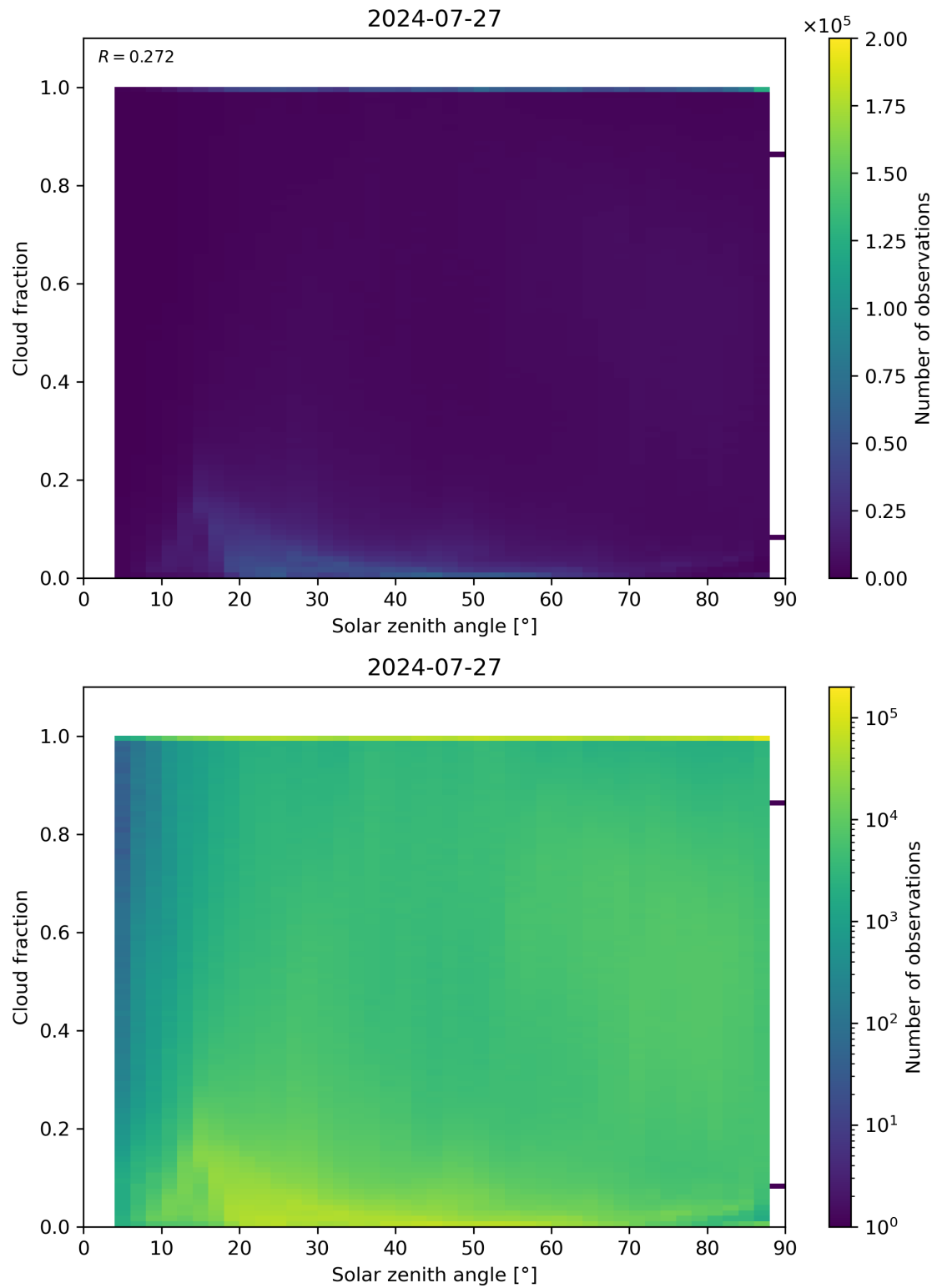
Figure 110: Scatter density plot of “Solar zenith angle” against “Cloud fraction” for 2024-07-26 to 2024-07-28.
