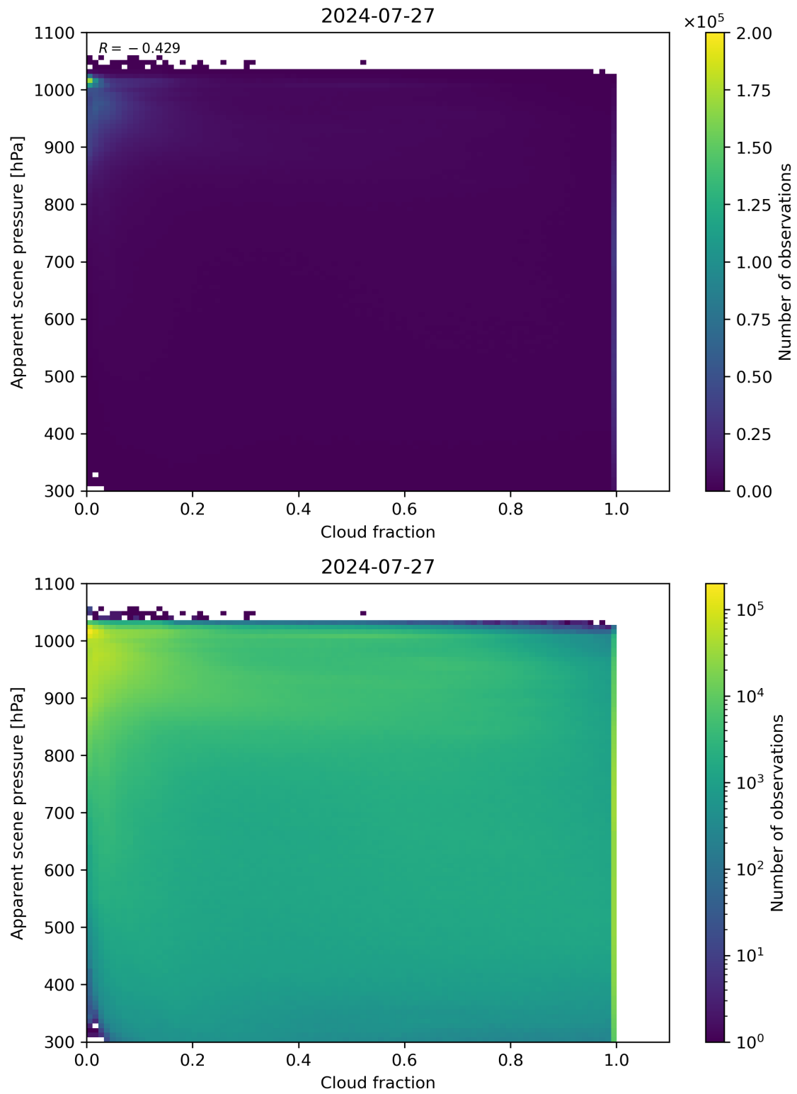
Figure 70: Scatter density plot of “Cloud fraction” against “Apparent scene pressure” for 2024-07-26 to 2024-07-28.
