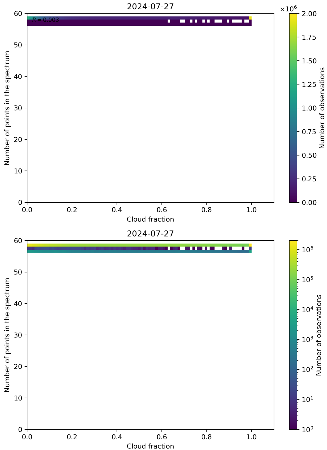
Figure 74: Scatter density plot of “Cloud fraction” against “Number of points in the spectrum” for 2024-07-26 to 2024-07-28.
