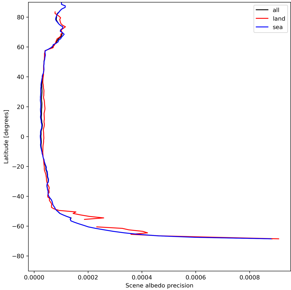
Figure 18: Zonal average of “Scene albedo precision” for 2024-07-26 to 2024-07-28.
