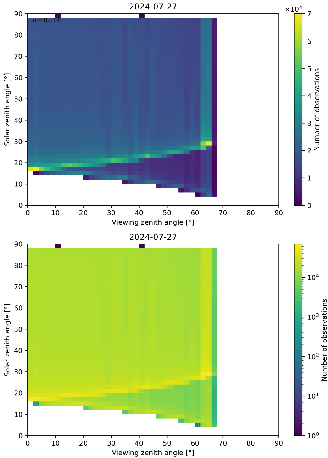
Figure 127: Scatter density plot of “Viewing zenith angle” against “Solar zenith angle” for 2024-07-26 to 2024-07-28.
