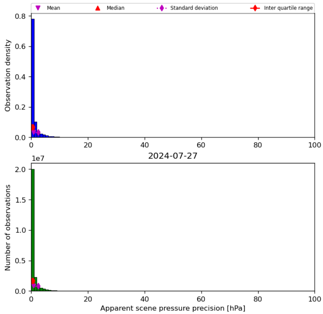
Figure 37: Histogram of “Apparent scene pressure precision” for 2024-07-26 to 2024-07-28
