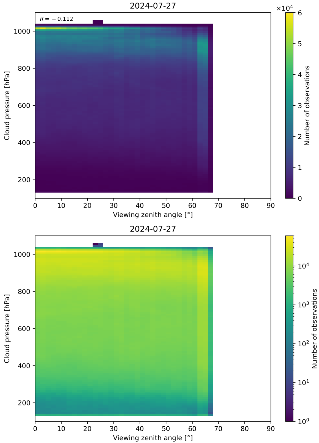
Figure 121: Scatter density plot of “Viewing zenith angle” against “Cloud pressure” for 2024-07-26 to 2024-07-28.
