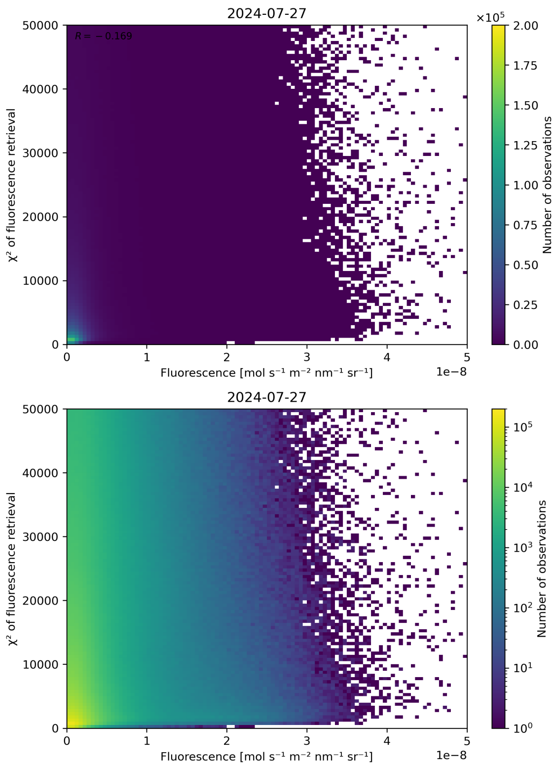
Figure 85: Scatter density plot of “Fluorescence” against “ \chi^2 of fluorescence retrieval” for 2024-07-26 to 2024-07-28.
