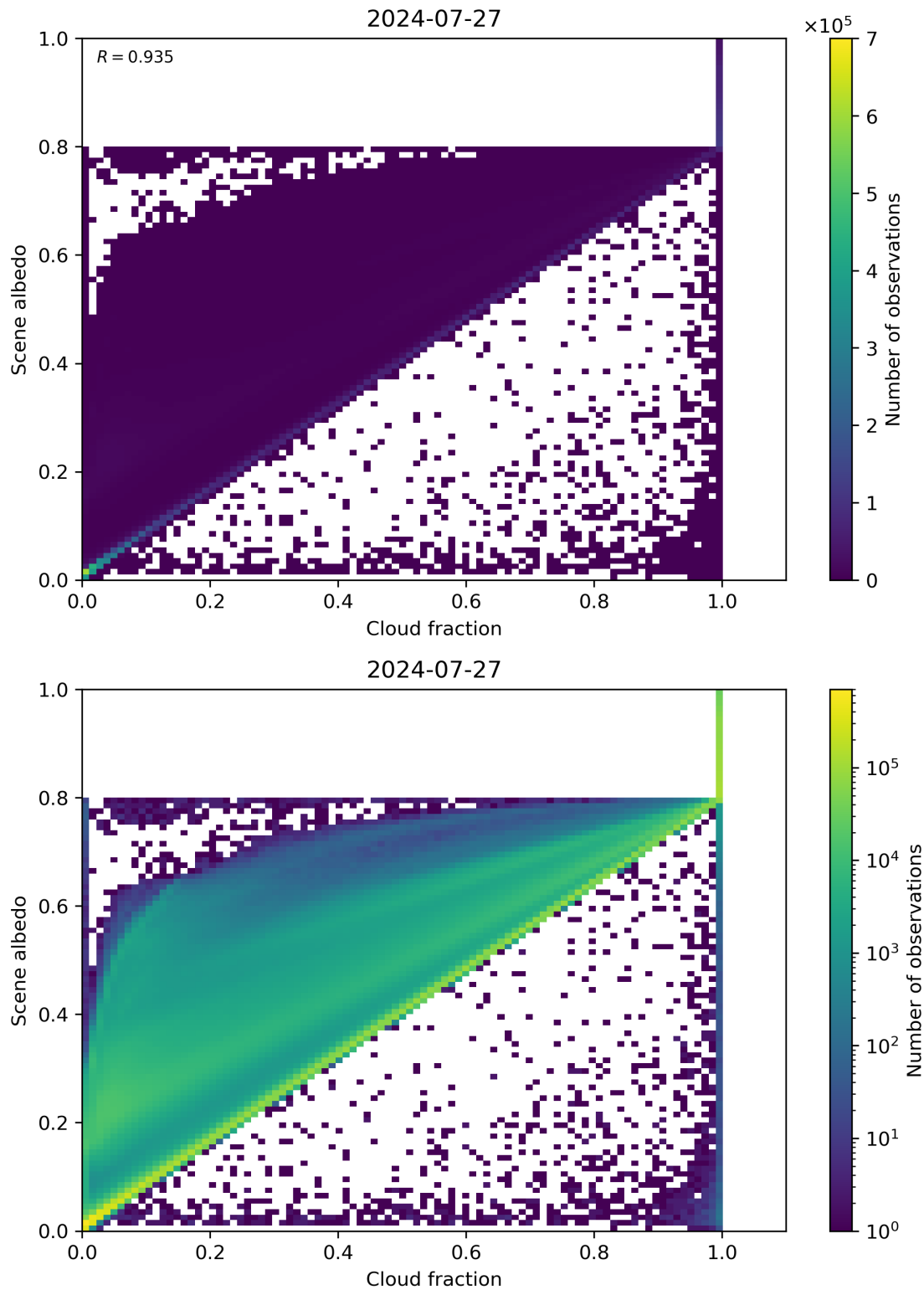
Figure 75: Scatter density plot of “Cloud fraction” against “Scene albedo” for 2024-07-26 to 2024-07-28.
