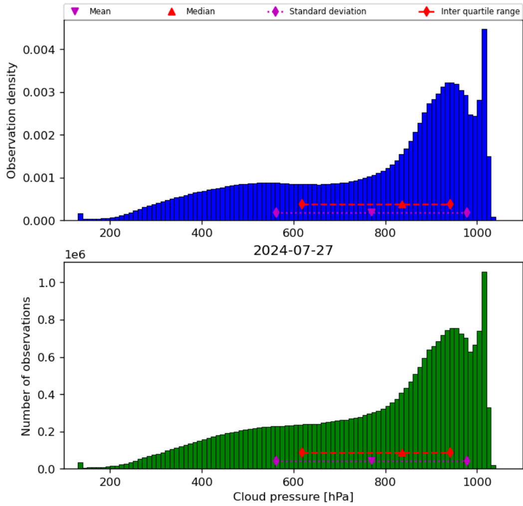
Figure 30: Histogram of “Cloud pressure” for 2024-07-26 to 2024-07-28
