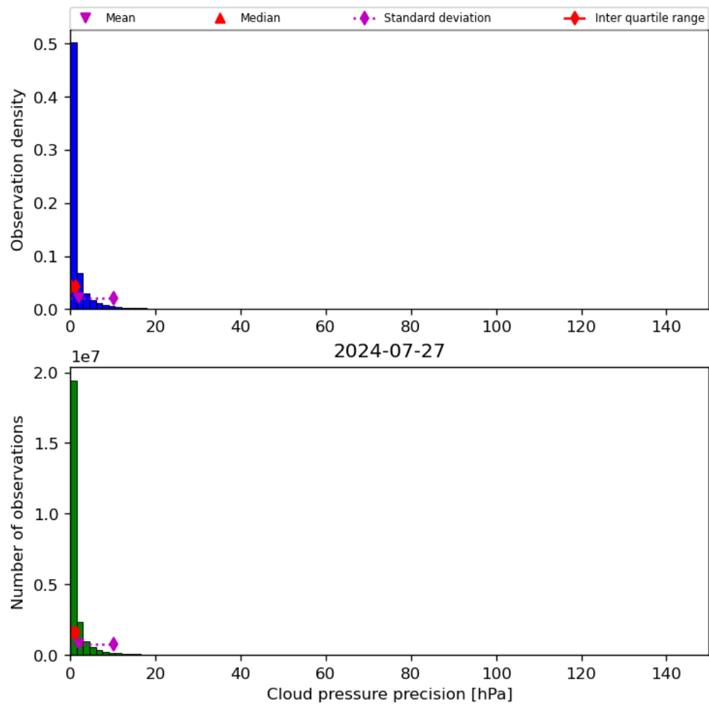
Figure 31: Histogram of “Cloud pressure precision” for 2024-07-26 to 2024-07-28
