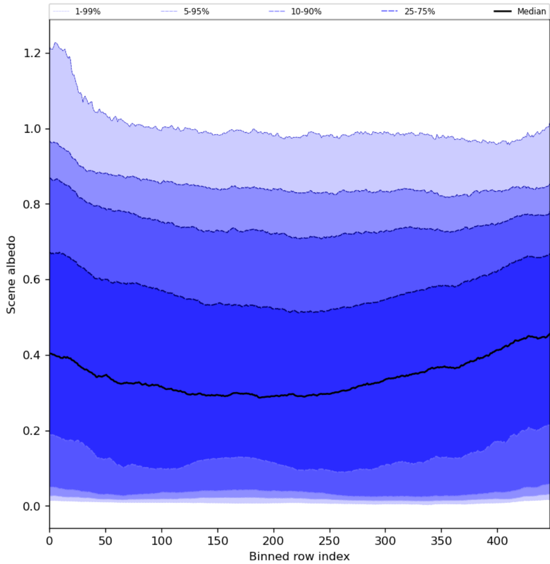
Figure 51: Along track statistics of “Scene albedo” for 2024-07-26 to 2024-07-28
