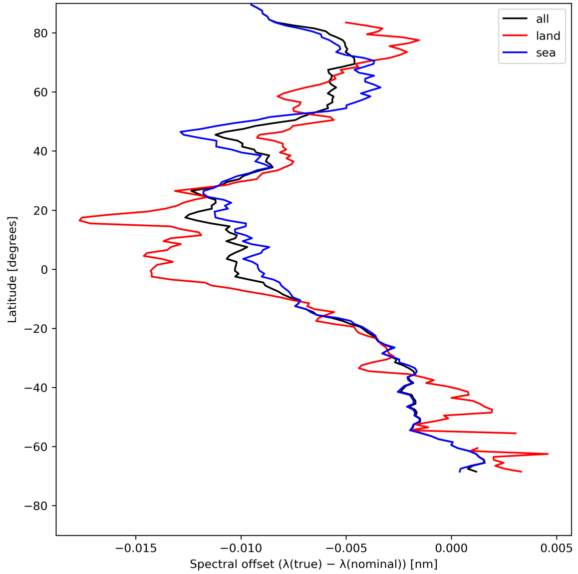
Figure 28: Zonal average of “Spectral offset ( \lambda(\text{true}) - \lambda(\text{nominal}) )” for 2024-07-26 to 2024-07-28.
