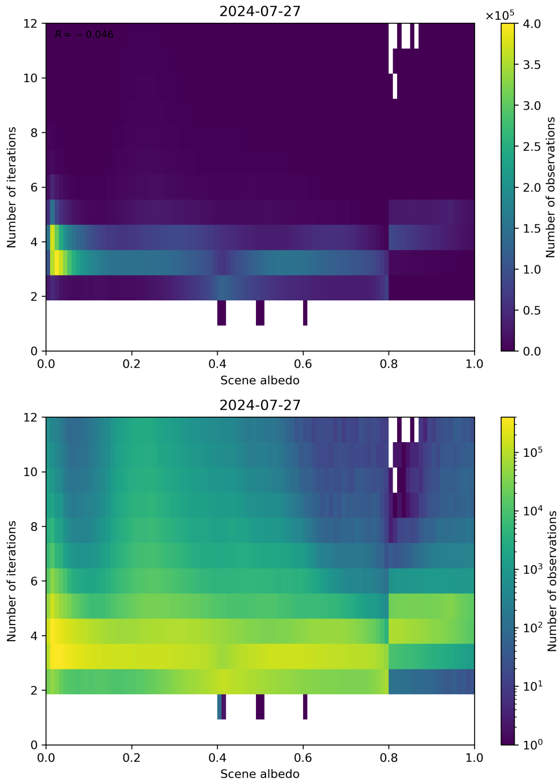
Figure 105: Scatter density plot of “Scene albedo” against “Number of iterations” for 2024-07-26 to 2024-07-28.
