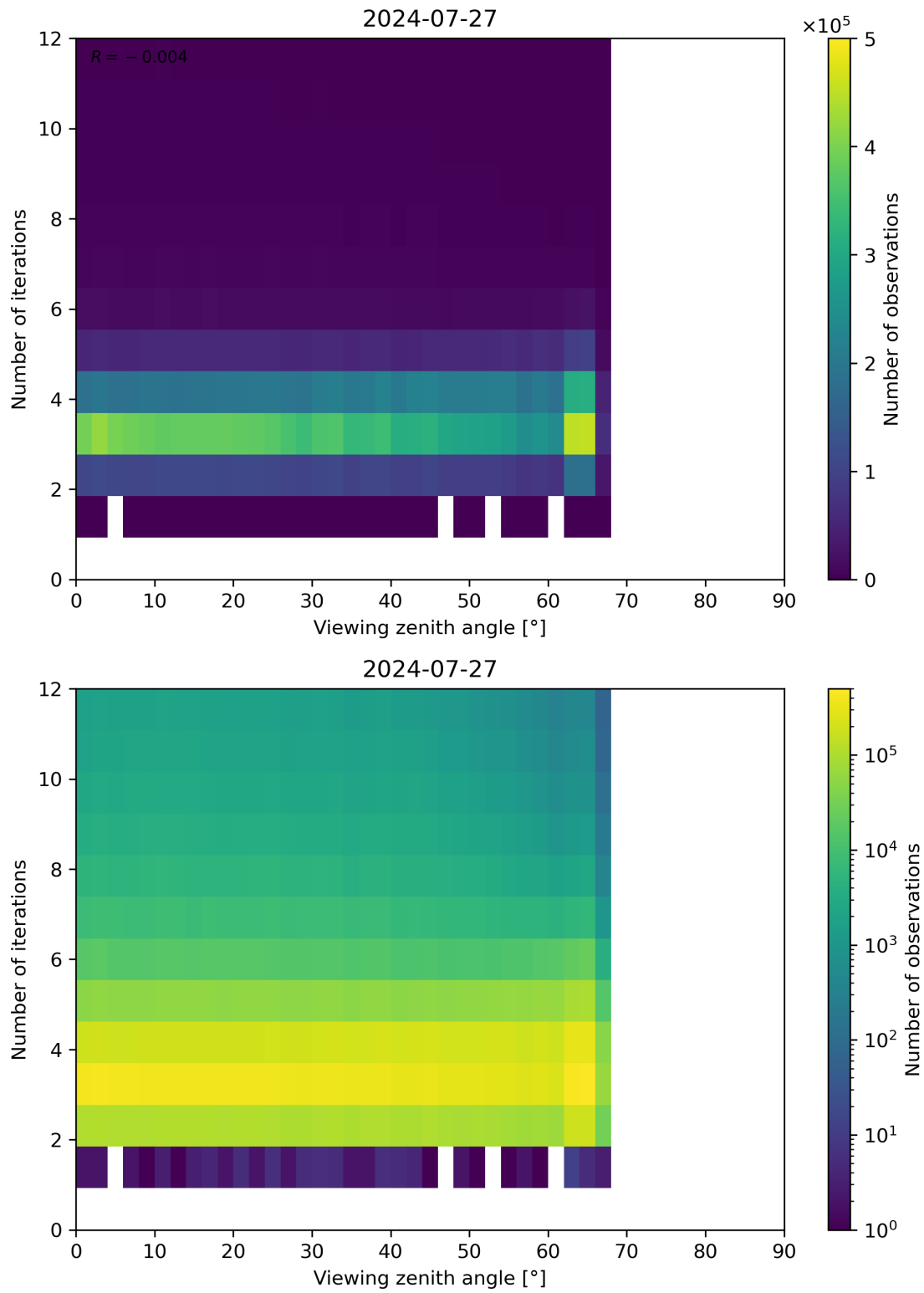
Figure 124: Scatter density plot of “Viewing zenith angle” against “Number of iterations” for 2024-07-26 to 2024-07-28.
