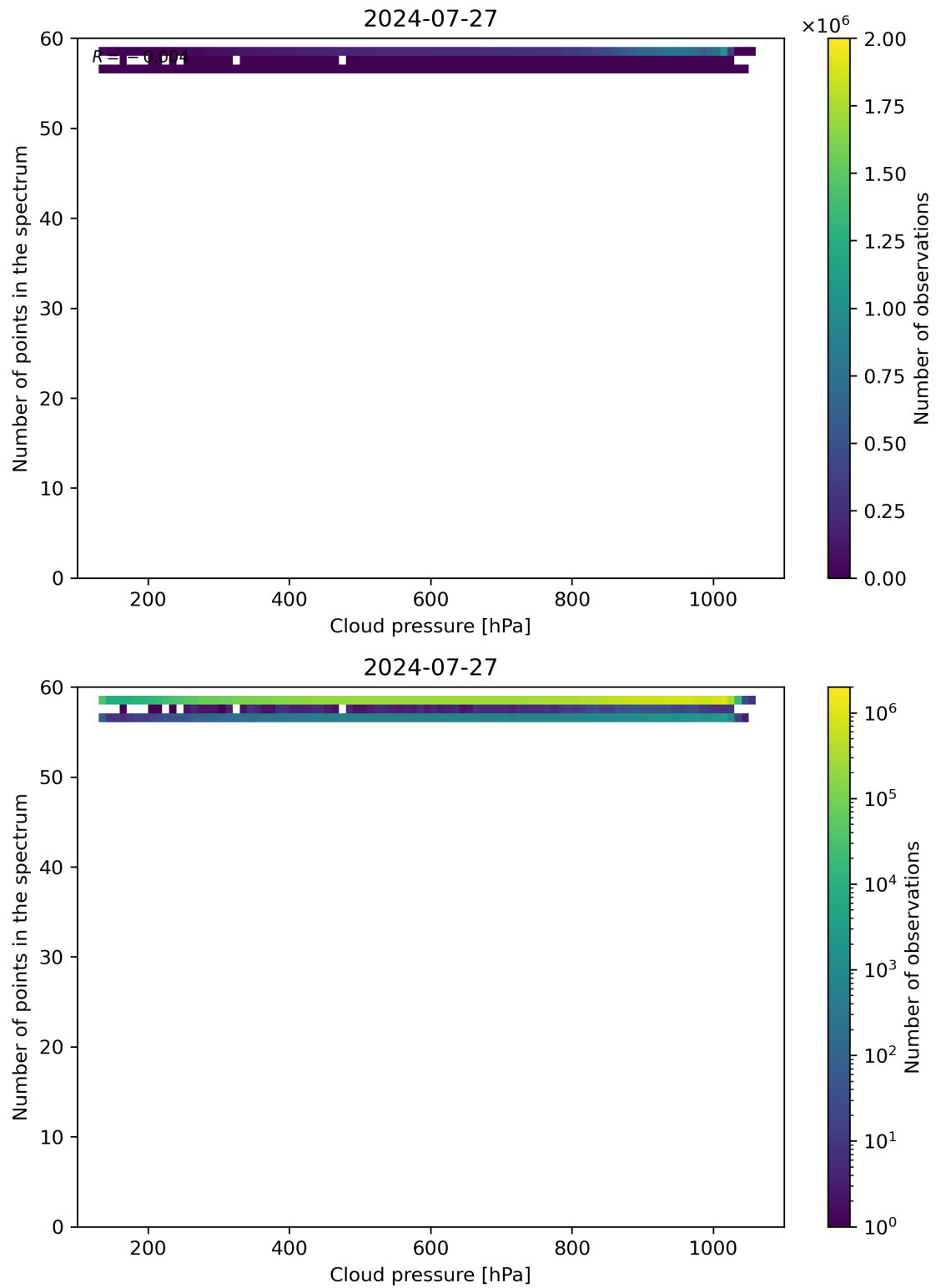
Figure 82: Scatter density plot of “Cloud pressure” against “Number of points in the spectrum” for 2024-07-26 to 2024-07-28.
