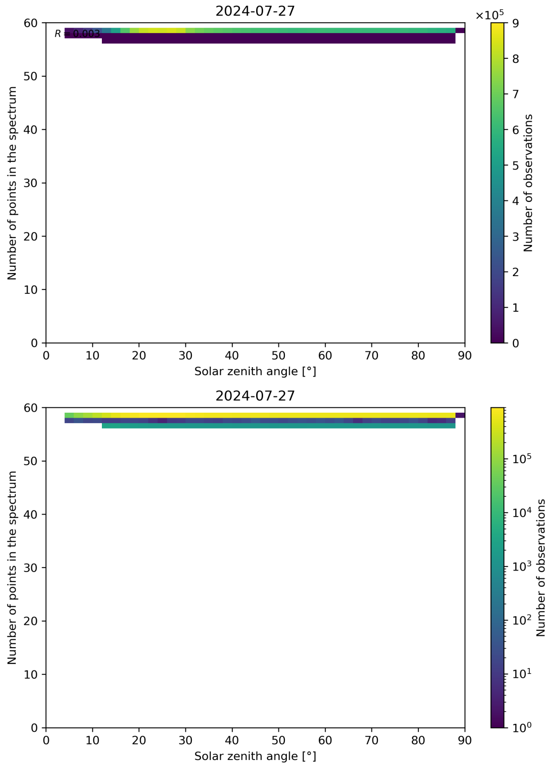
Figure 115: Scatter density plot of “Solar zenith angle” against “Number of points in the spectrum” for 2024-07-26 to 2024-07-28.
