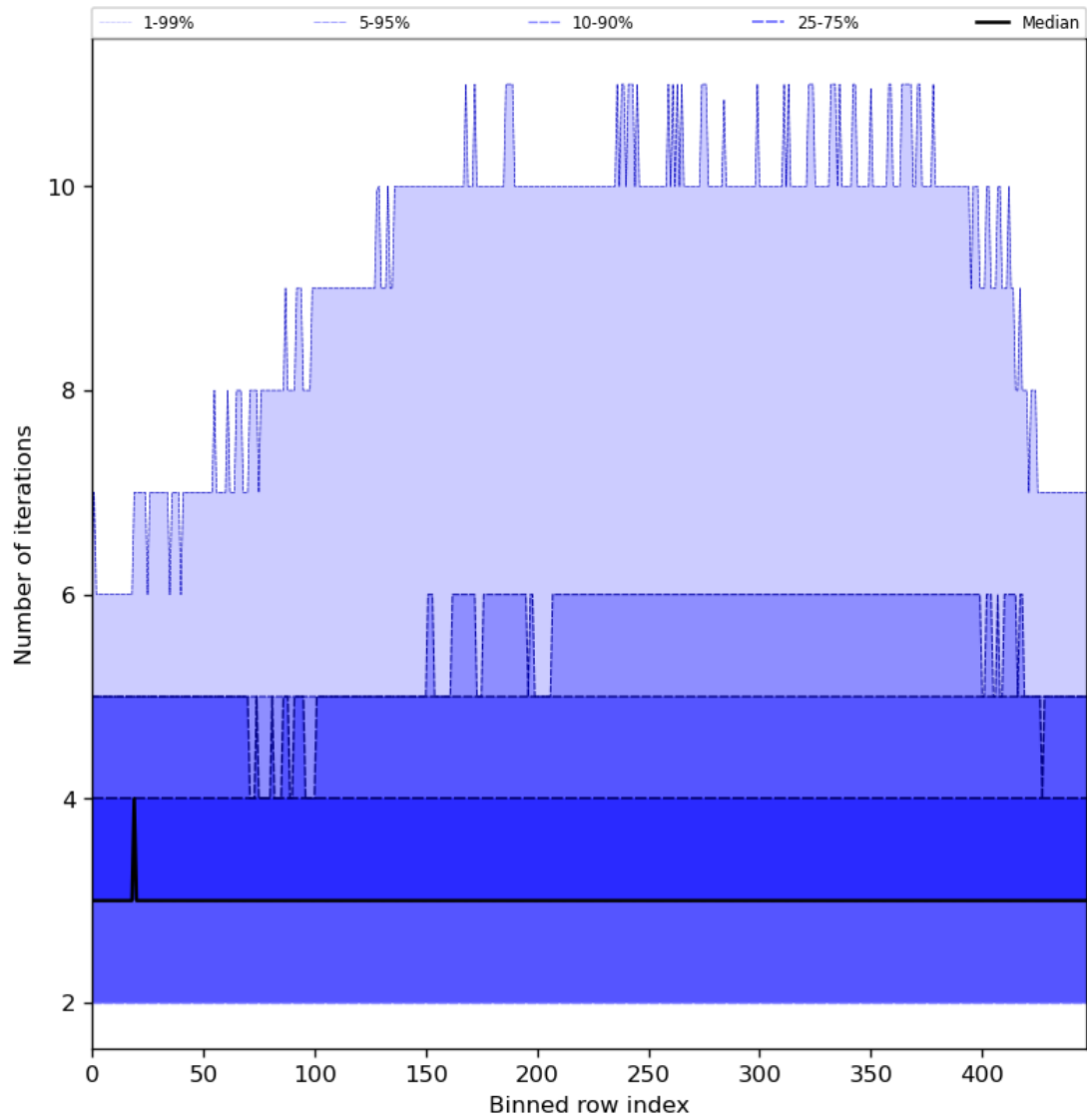
Figure 56: Along track statistics of “Number of iterations” for 2024-07-26 to 2024-07-28
