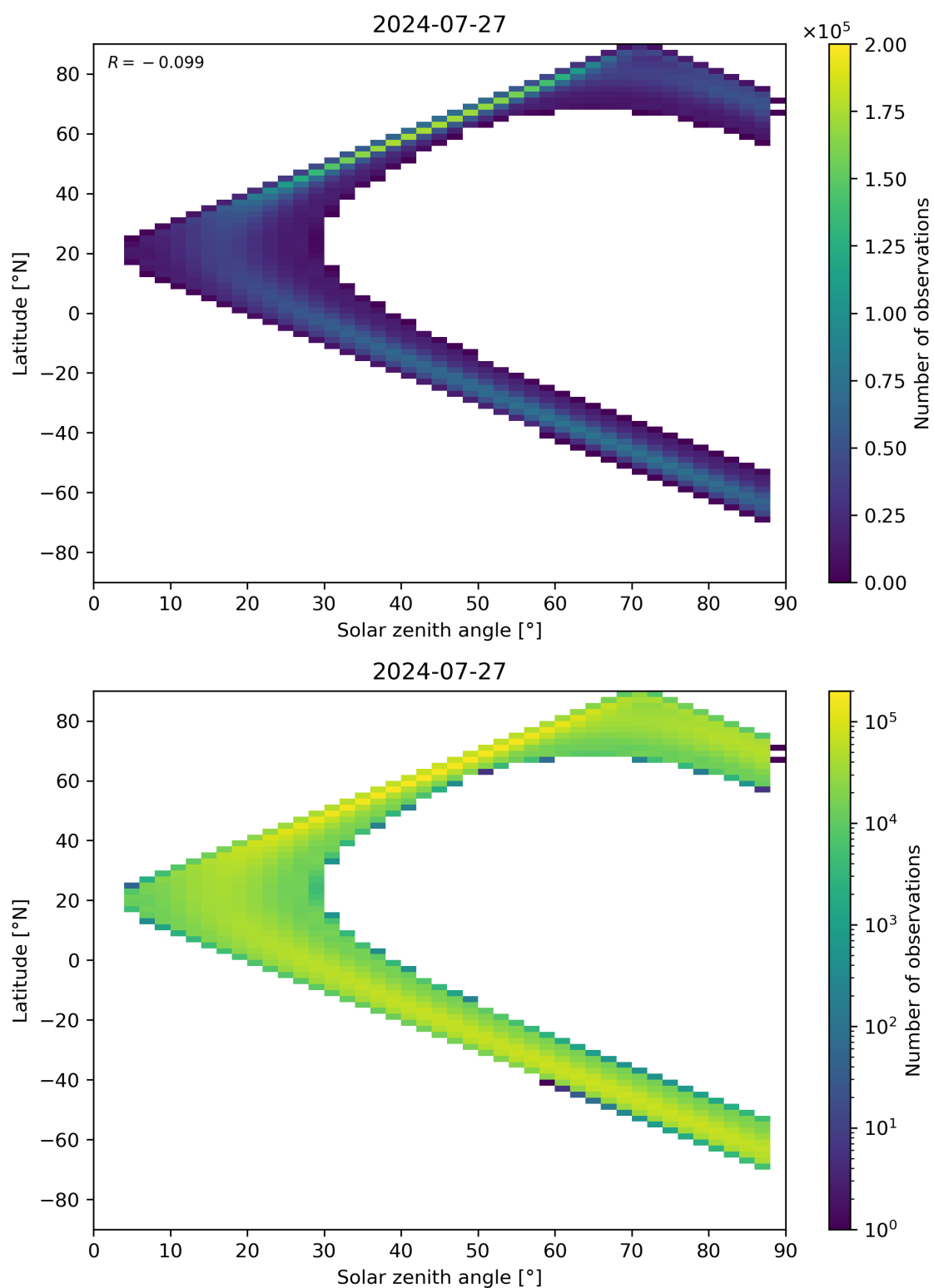
Figure 113: Scatter density plot of “Solar zenith angle” against “Latitude” for 2024-07-26 to 2024-07-28.
