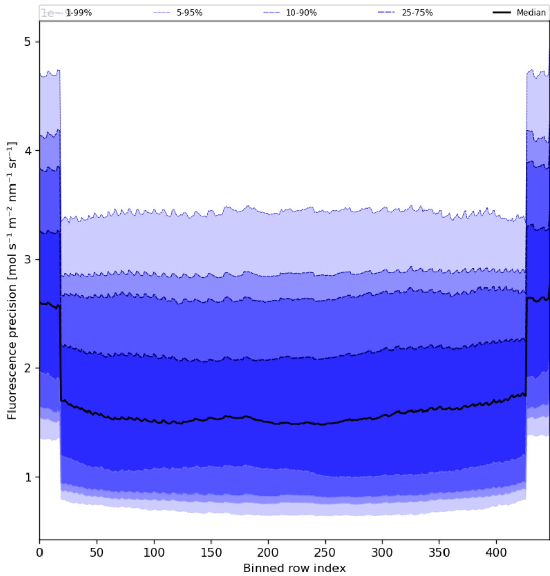
Figure 58: Along track statistics of “Fluorescence precision” for 2024-07-26 to 2024-07-28
