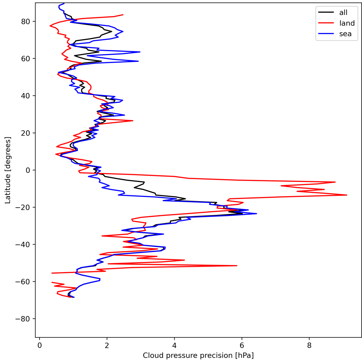
Figure 14: Zonal average of “Cloud pressure precision” for 2024-07-26 to 2024-07-28.
