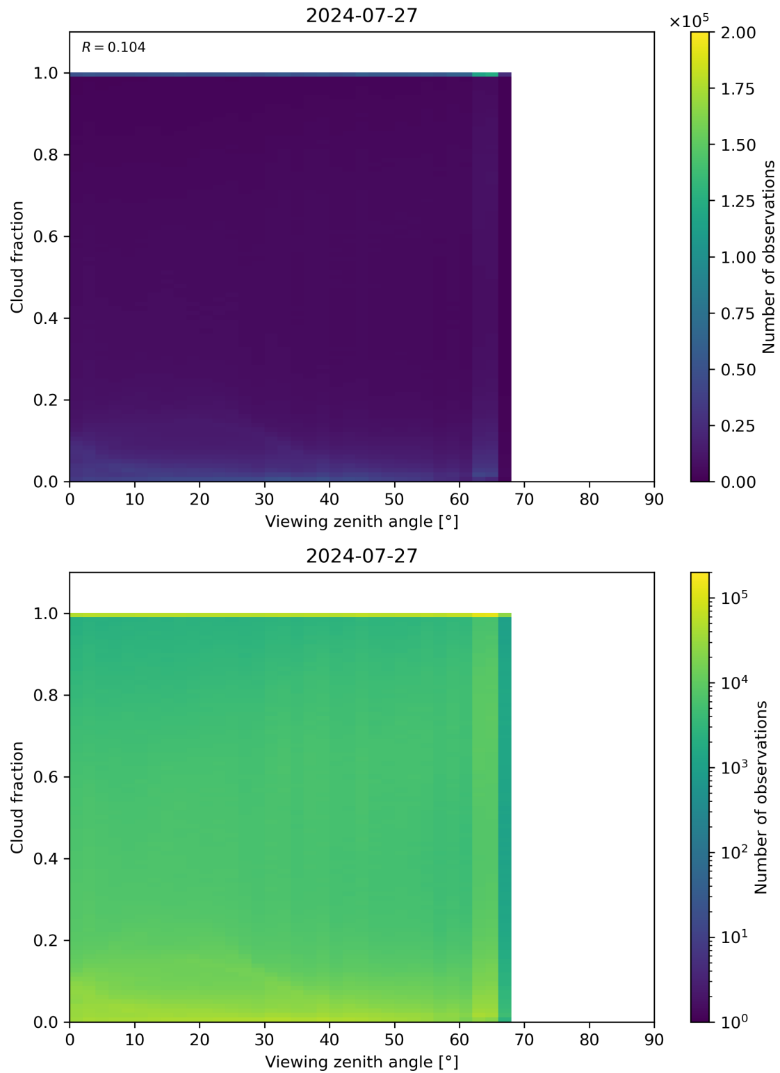
Figure 120: Scatter density plot of “Viewing zenith angle” against “Cloud fraction” for 2024-07-26 to 2024-07-28.
