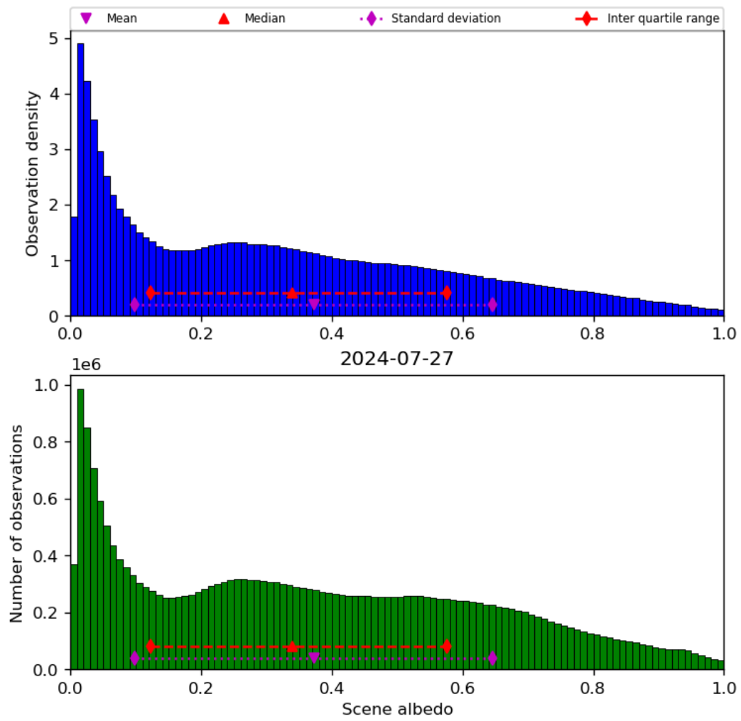
Figure 34: Histogram of “Scene albedo” for 2024-07-26 to 2024-07-28
