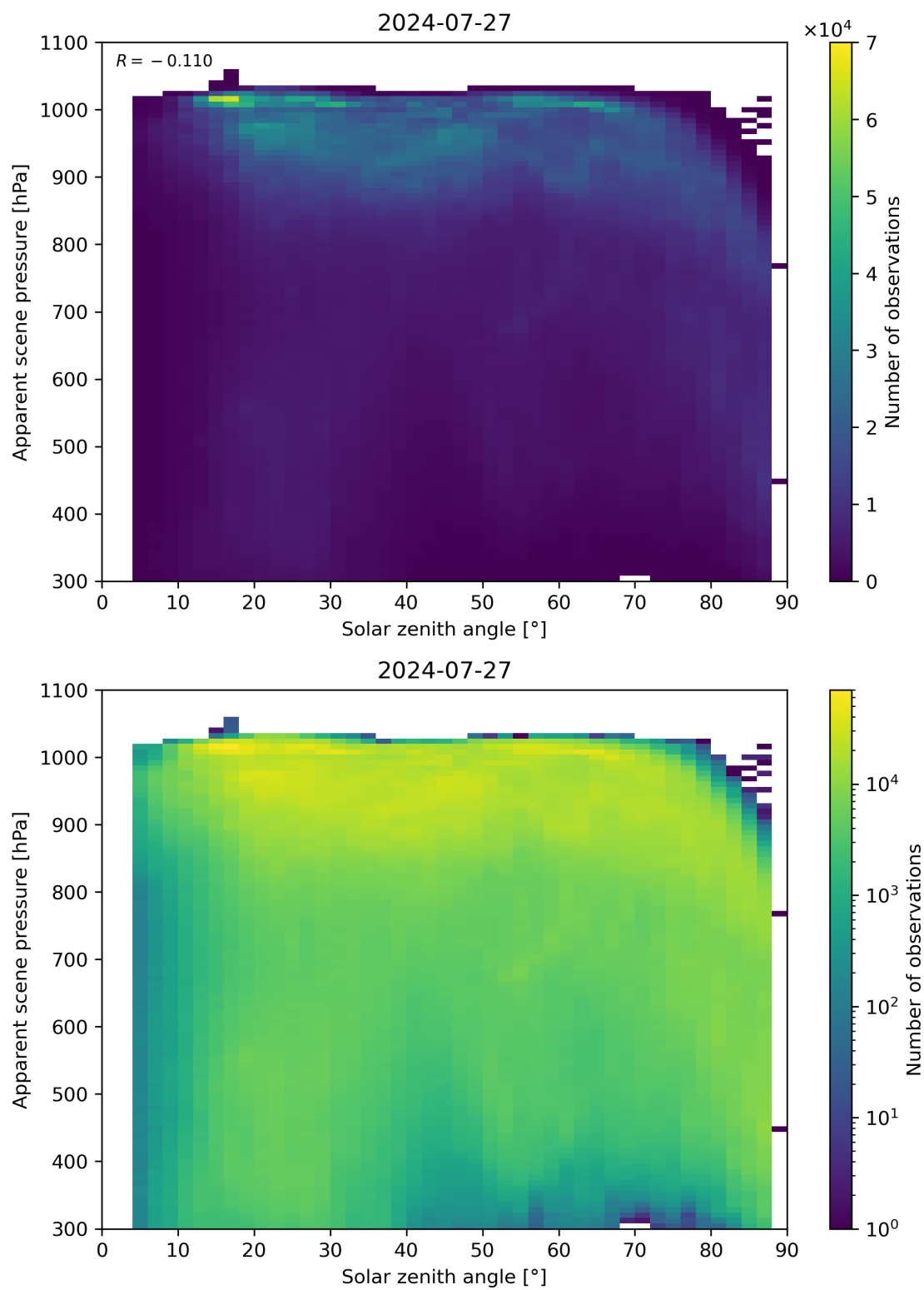
Figure 108: Scatter density plot of “Solar zenith angle” against “Apparent scene pressure” for 2024-07-26 to 2024-07-28.
