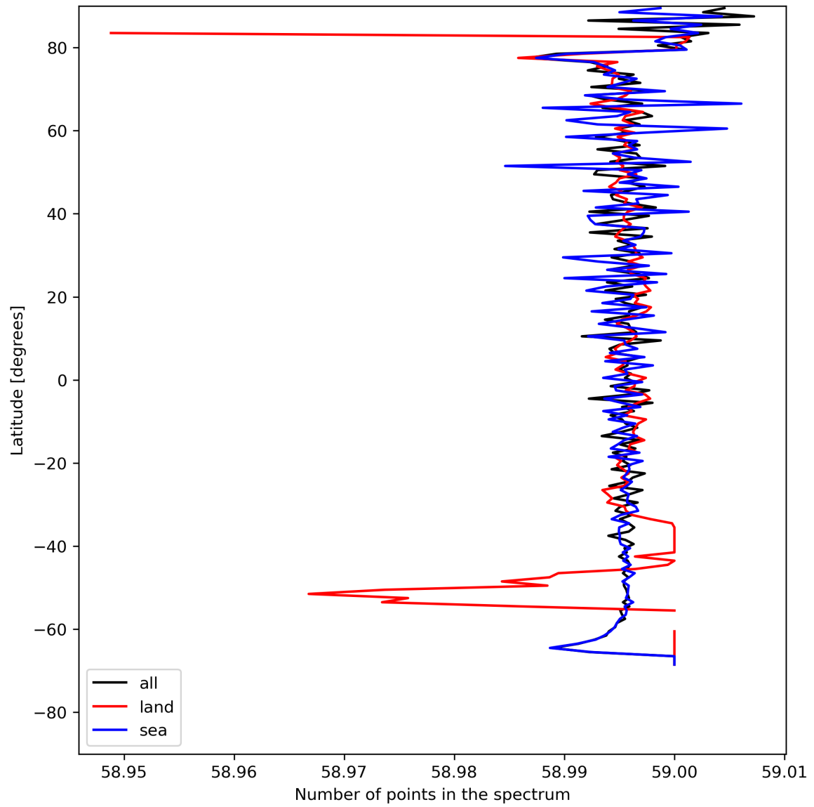
Figure 27: Zonal average of “Number of points in the spectrum” for 2024-07-26 to 2024-07-28.
