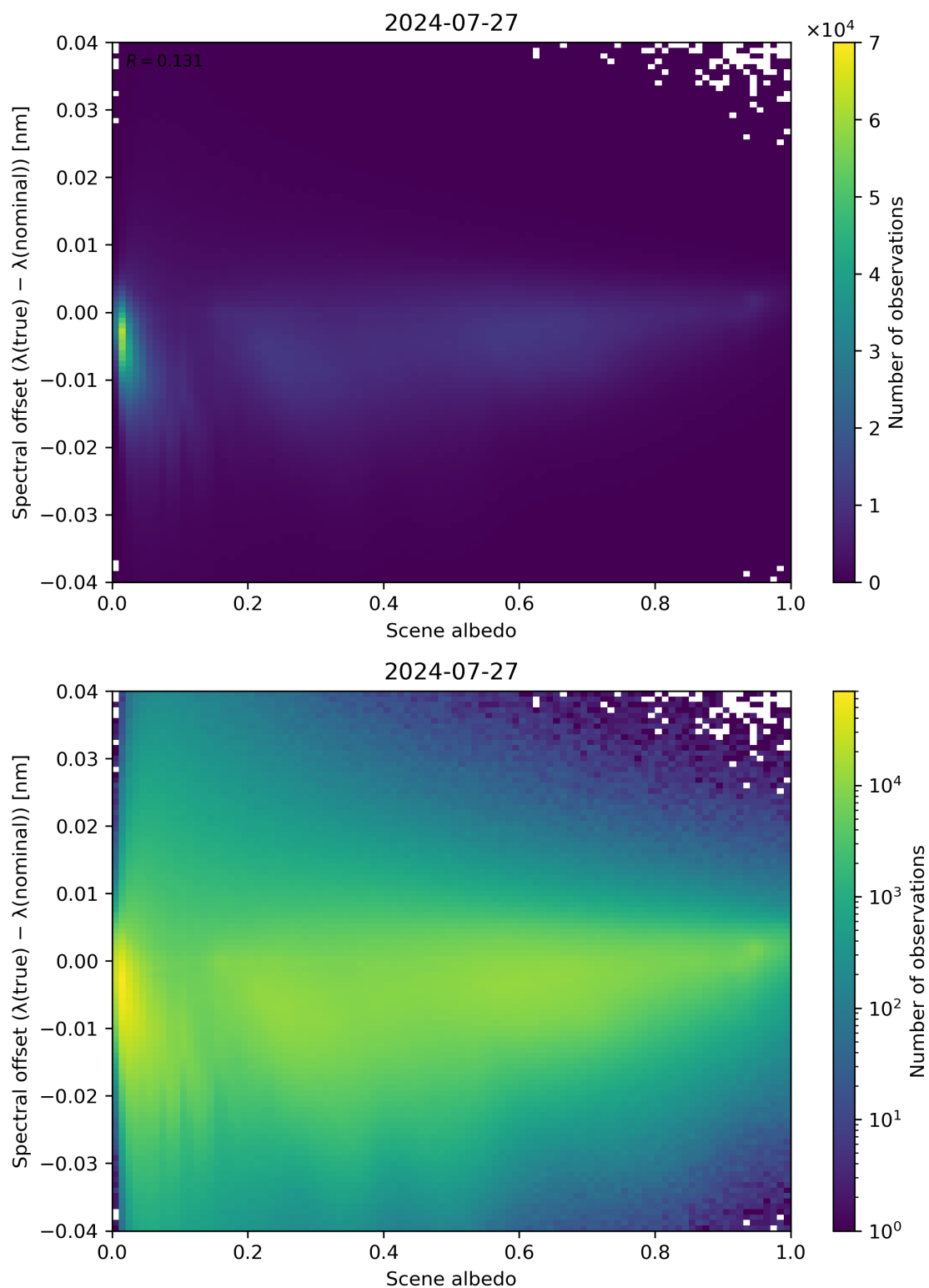
Figure 107: Scatter density plot of “Scene albedo” against “Spectral offset ( \lambda(\text{true}) - \lambda(\text{nominal}) )” for 2024-07-26 to 2024-07-28.
