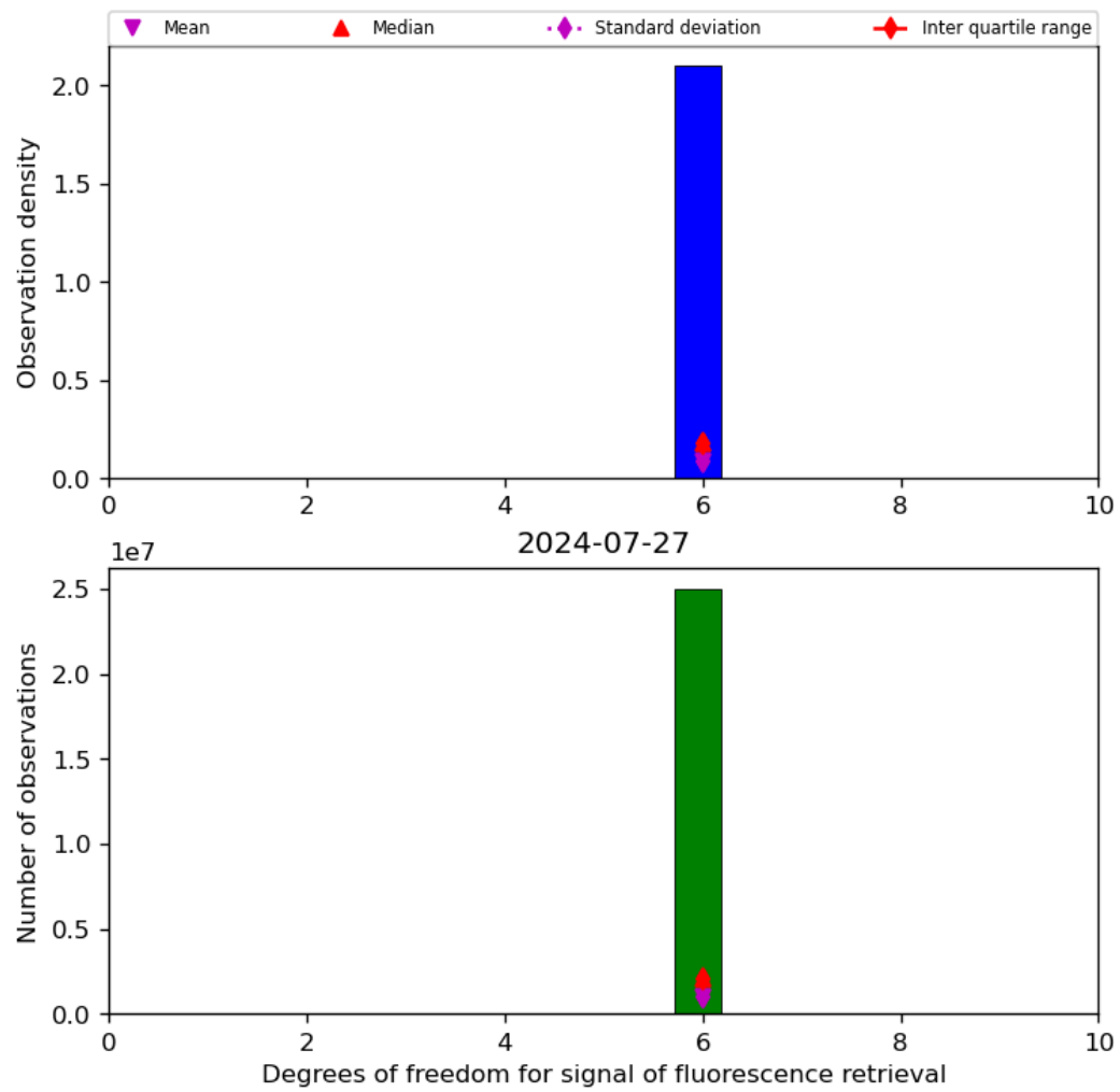
Figure 43: Histogram of “Degrees of freedom for signal of fluorescence retrieval” for 2024-07-26 to 2024-07-28
