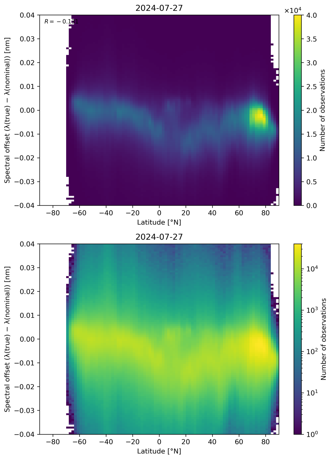
Figure 96: Scatter density plot of “Latitude” against “Spectral offset ( \lambda(\text{true}) - \lambda(\text{nominal}) )” for 2024-07-26 to 2024-07-28.
