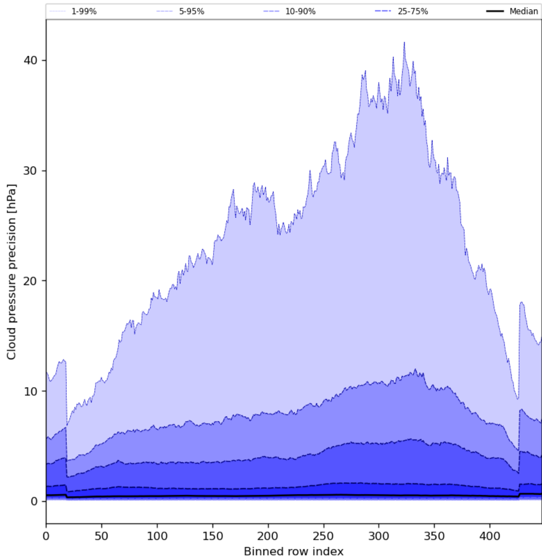
Figure 48: Along track statistics of “Cloud pressure precision” for 2024-07-26 to 2024-07-28
