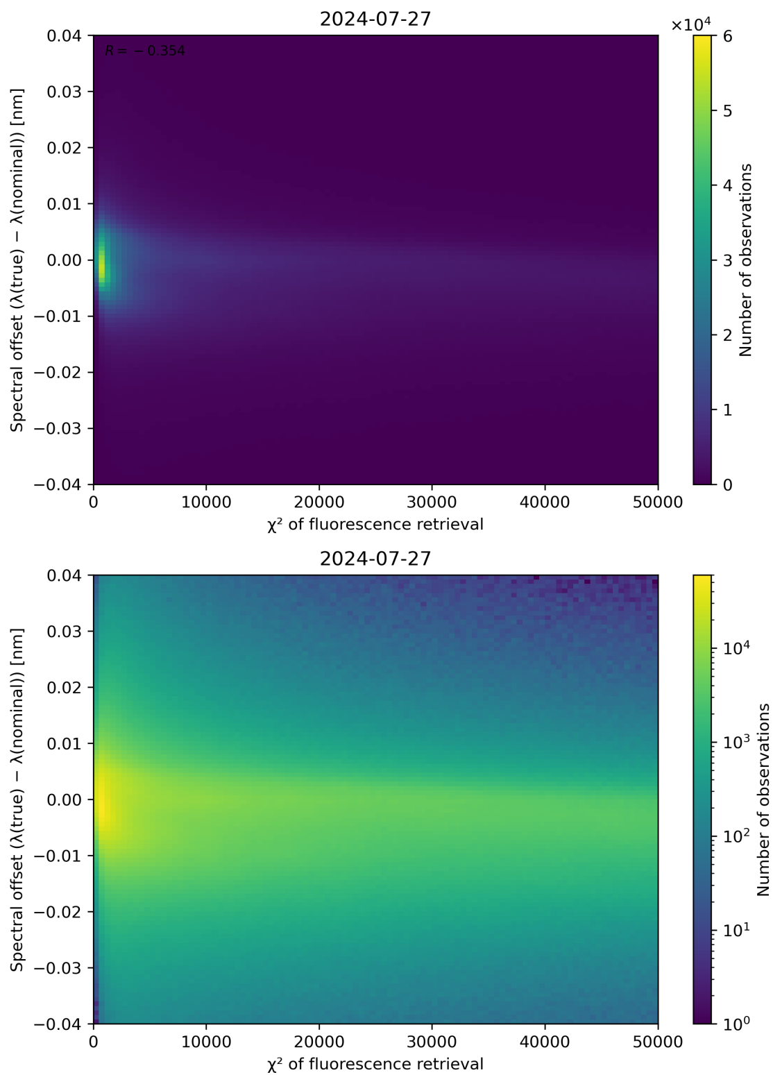
Figure 69: Scatter density plot of " \chi^2 of fluorescence retrieval" against "Spectral offset ( \lambda(\text{true}) - \lambda(\text{nominal})) " for 2024-07-26 to 2024-07-28.
