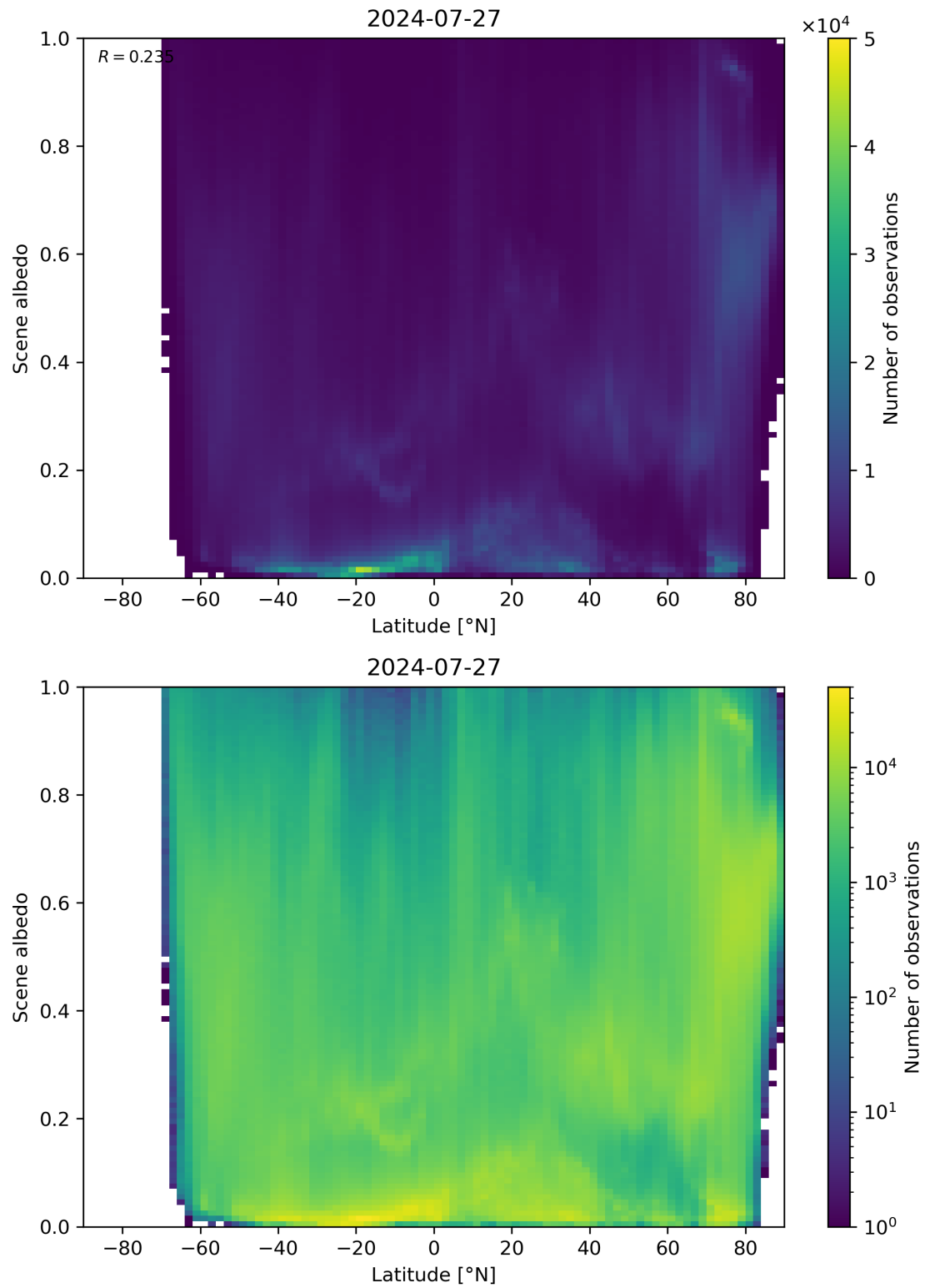
Figure 95: Scatter density plot of “Latitude” against “Scene albedo” for 2024-07-26 to 2024-07-28.
