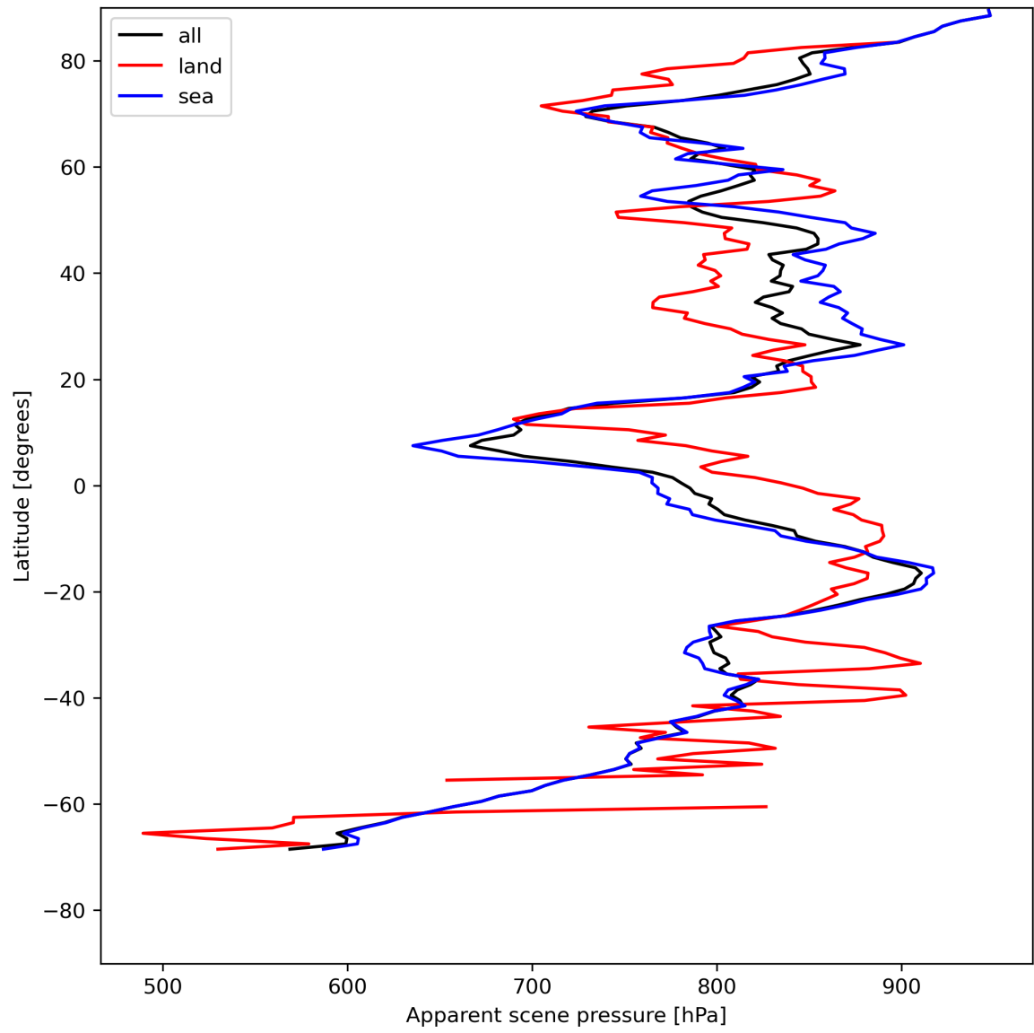
Figure 19: Zonal average of “Apparent scene pressure” for 2024-07-26 to 2024-07-28.
