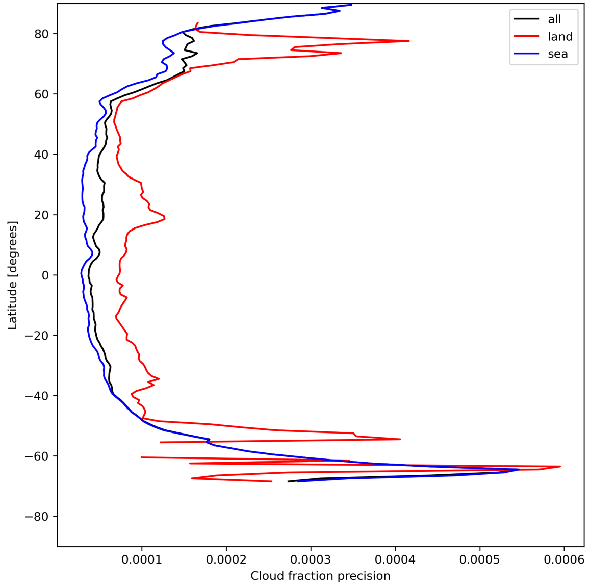
Figure 16: Zonal average of “Cloud fraction precision” for 2024-07-26 to 2024-07-28.
