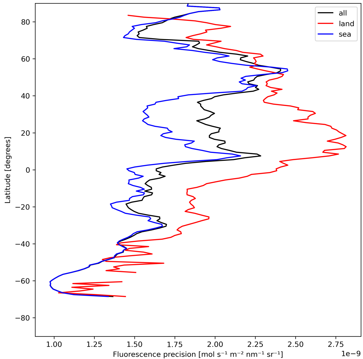
Figure 24: Zonal average of “Fluorescence precision” for 2024-07-26 to 2024-07-28.
