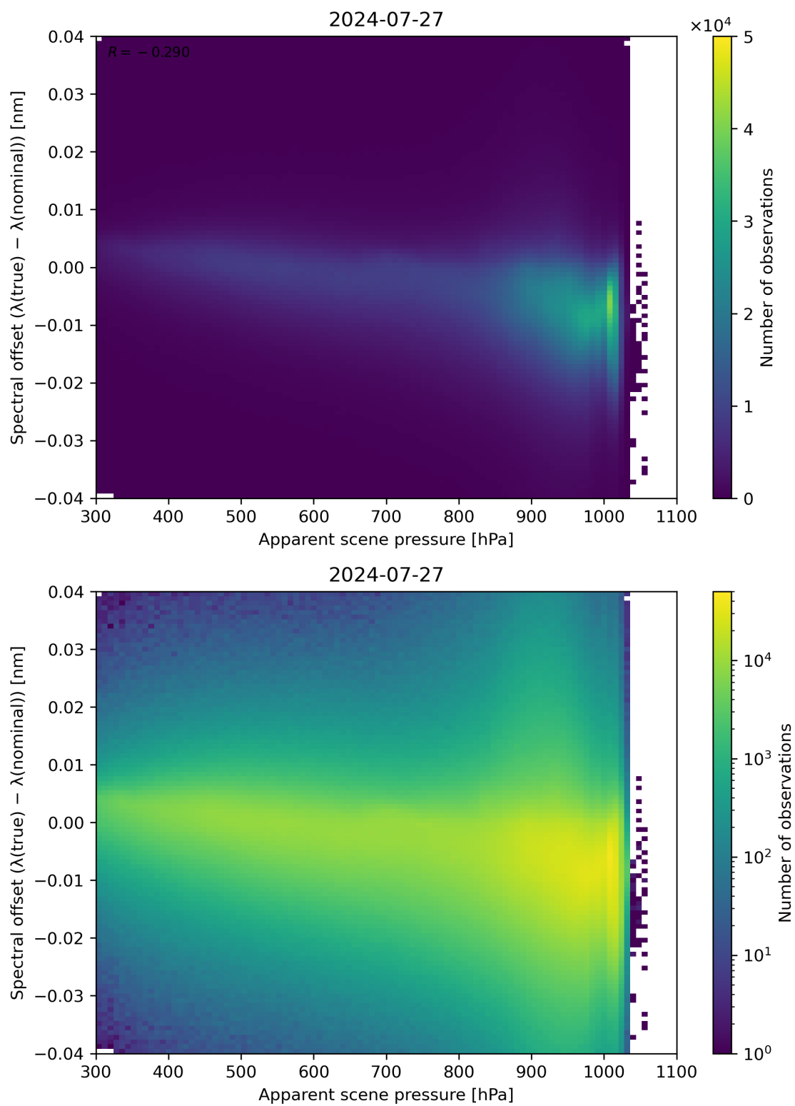
Figure 67: Scatter density plot of “Apparent scene pressure” against “Spectral offset ( \lambda(\text{true}) - \lambda(\text{nominal}) )” for 2024-07-26 to 2024-07-28.
