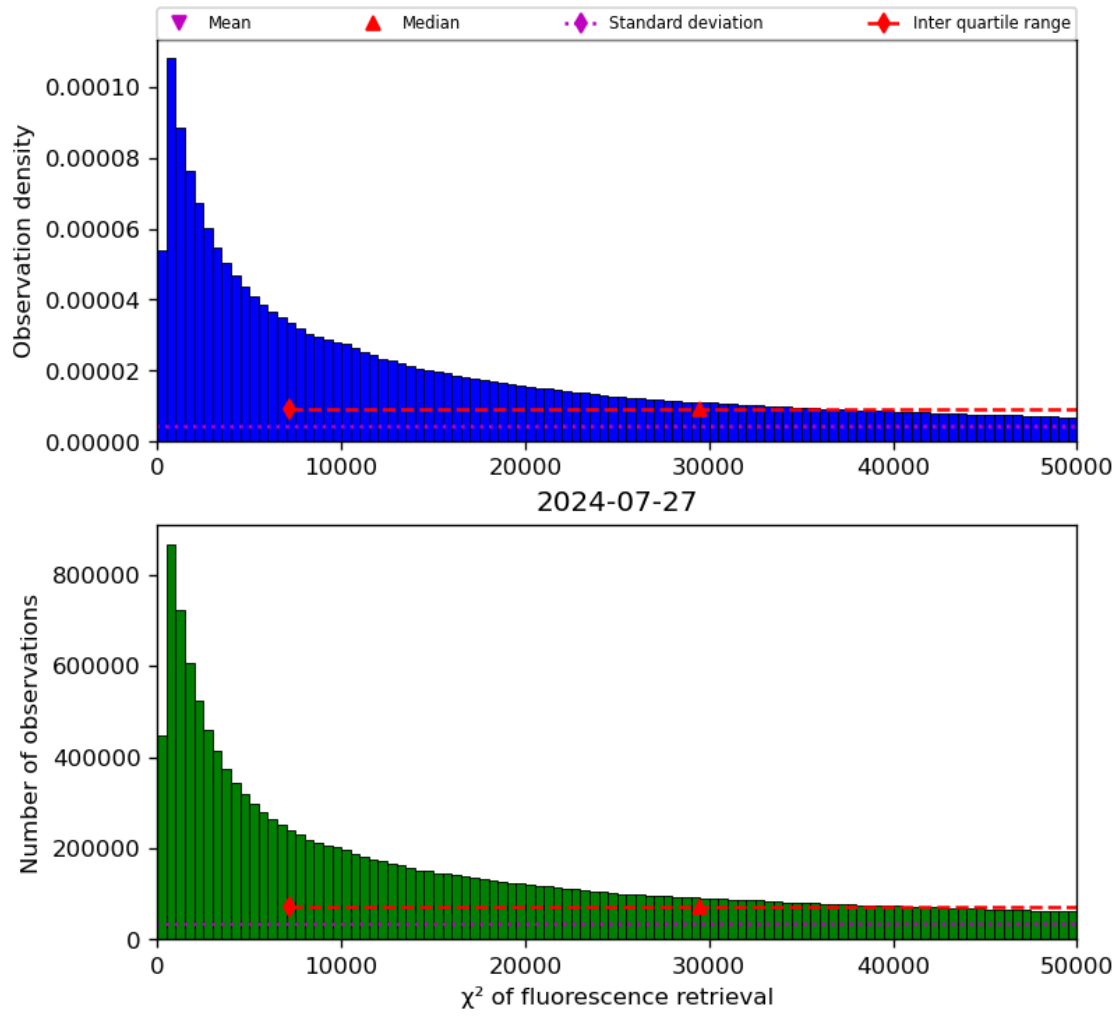
Figure 42: Histogram of “ \chi^2 of fluorescence retrieval” for 2024-07-26 to 2024-07-28
