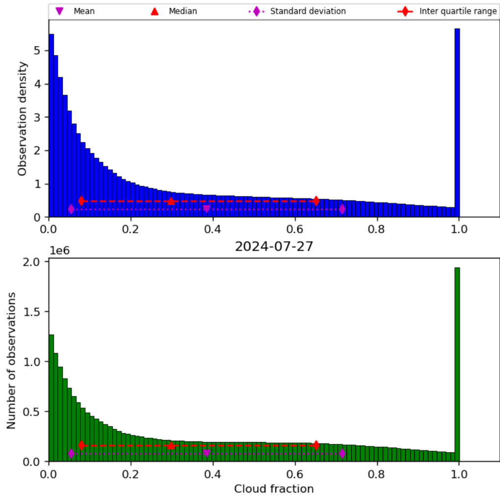
Figure 32: Histogram of “Cloud fraction” for 2024-07-26 to 2024-07-28
