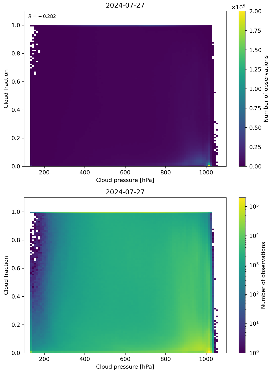
Figure 79: Scatter density plot of “Cloud pressure” against “Cloud fraction” for 2024-07-26 to 2024-07-28.
