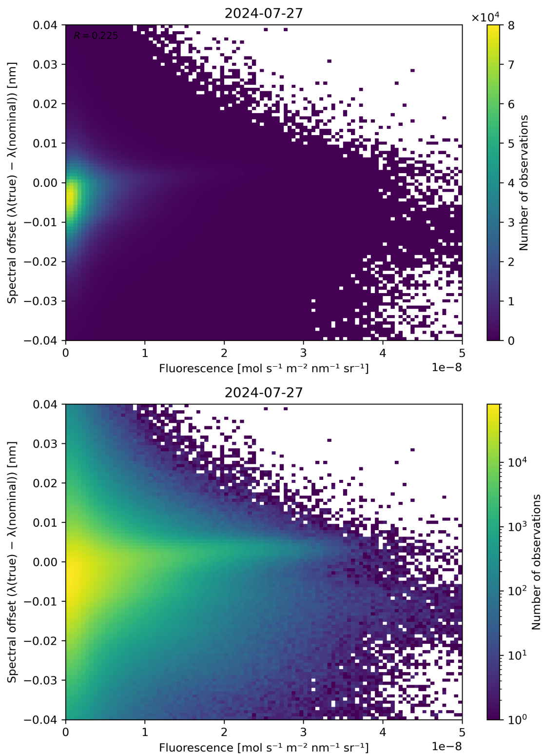
Figure 87: Scatter density plot of “Fluorescence” against “Spectral offset ( \lambda(\text{true}) - \lambda(\text{nominal}) )” for 2024-07-26 to 2024-07-28.
