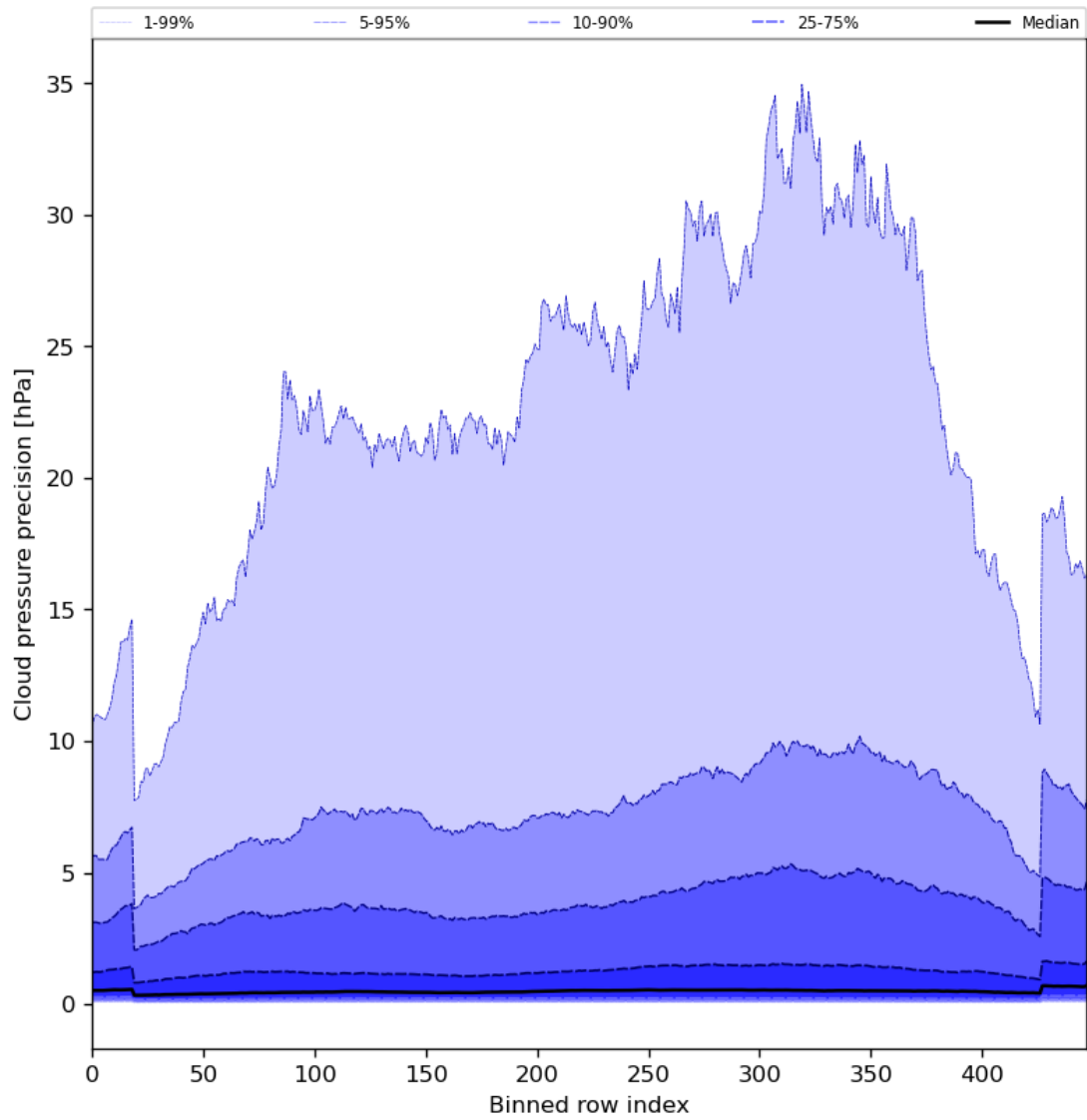
Figure 48: Along track statistics of “Cloud pressure precision” for 2024-07-27 to 2024-07-29
