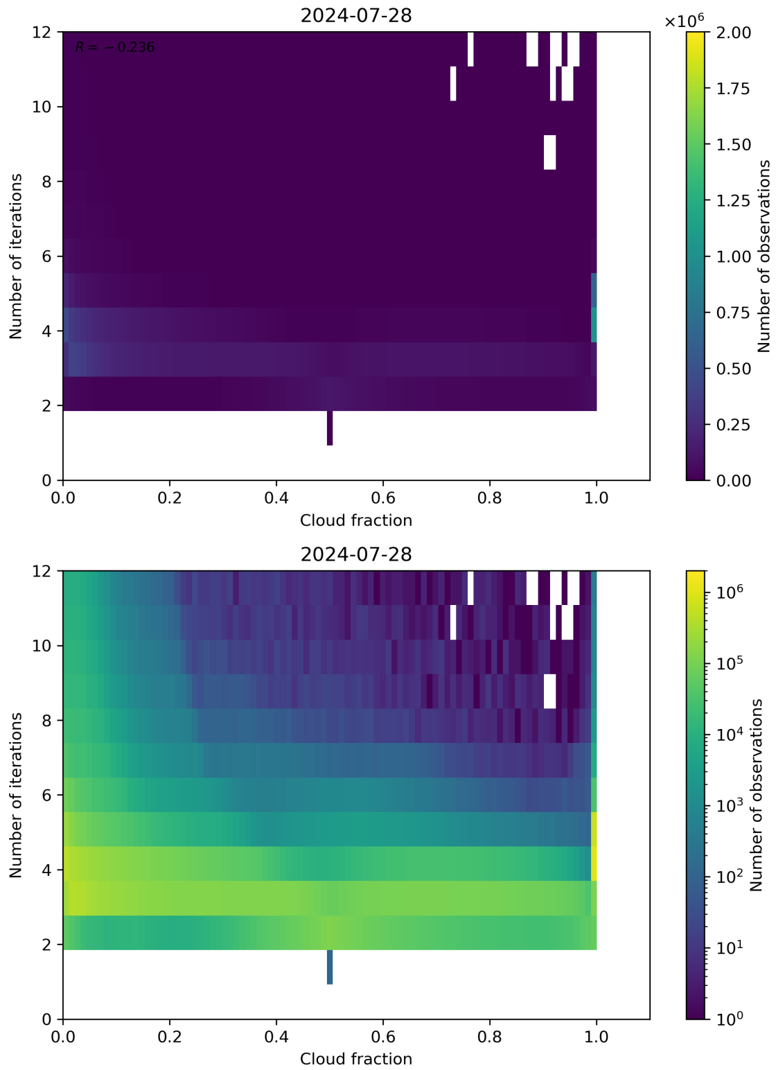
Figure 73: Scatter density plot of “Cloud fraction” against “Number of iterations” for 2024-07-27 to 2024-07-29.
