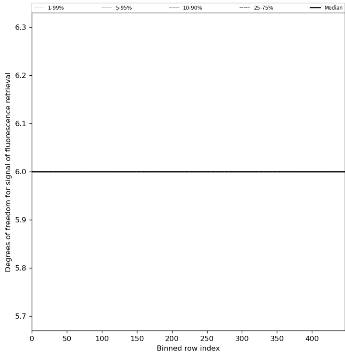
Figure 60: Along track statistics of “Degrees of freedom for signal of fluorescence retrieval” for 2024-07-27 to 2024-07-29
