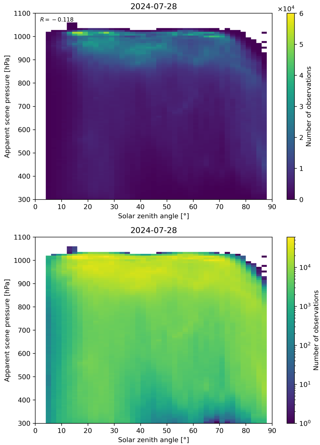
Figure 108: Scatter density plot of “Solar zenith angle” against “Apparent scene pressure” for 2024-07-27 to 2024-07-29.
