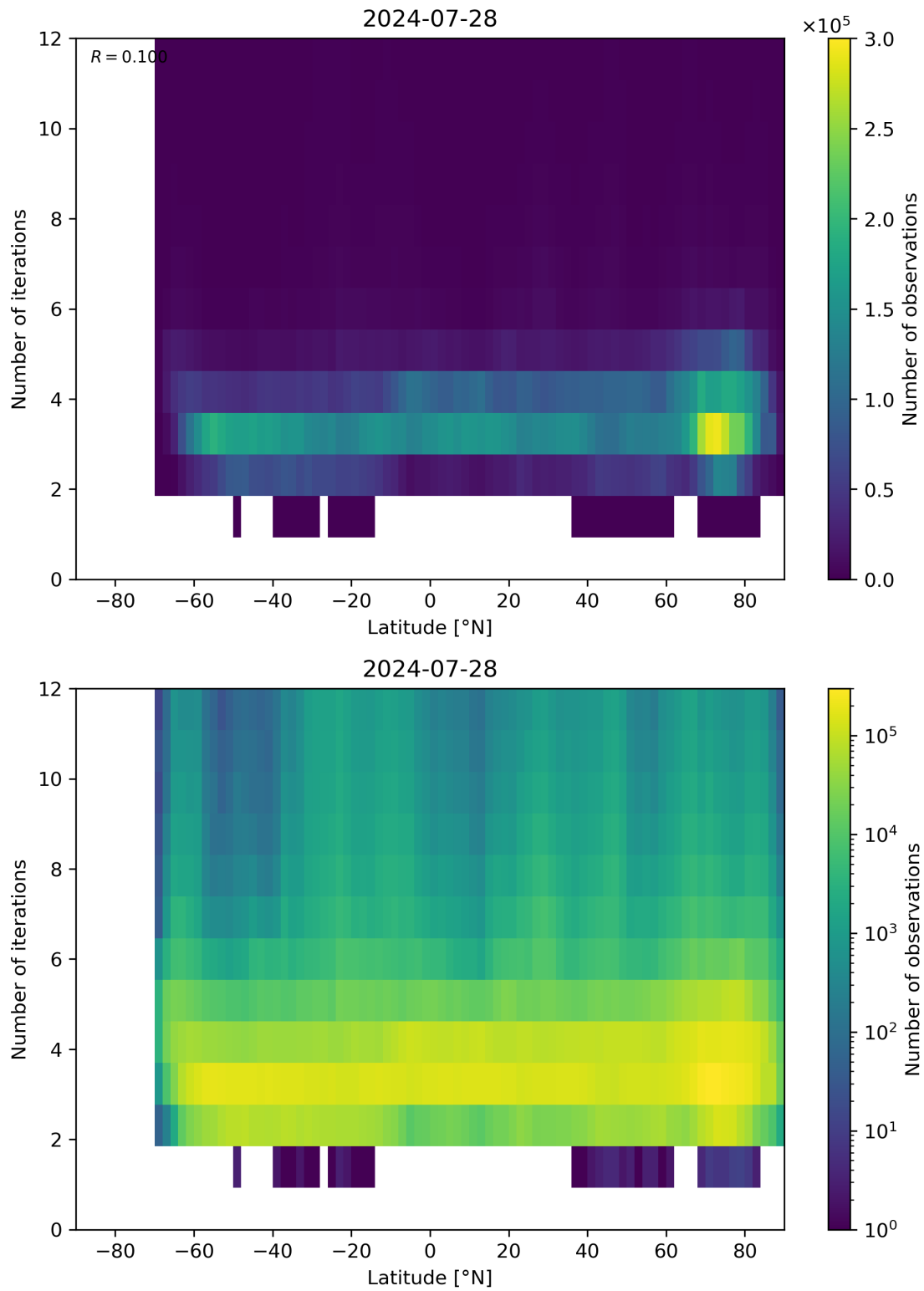
Figure 93: Scatter density plot of “Latitude” against “Number of iterations” for 2024-07-27 to 2024-07-29.
