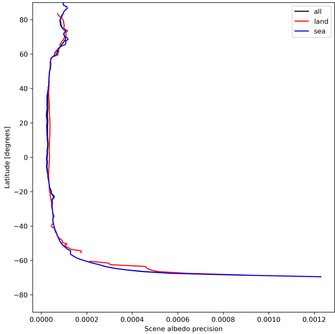
Figure 18: Zonal average of “Scene albedo precision” for 2024-07-27 to 2024-07-29.
