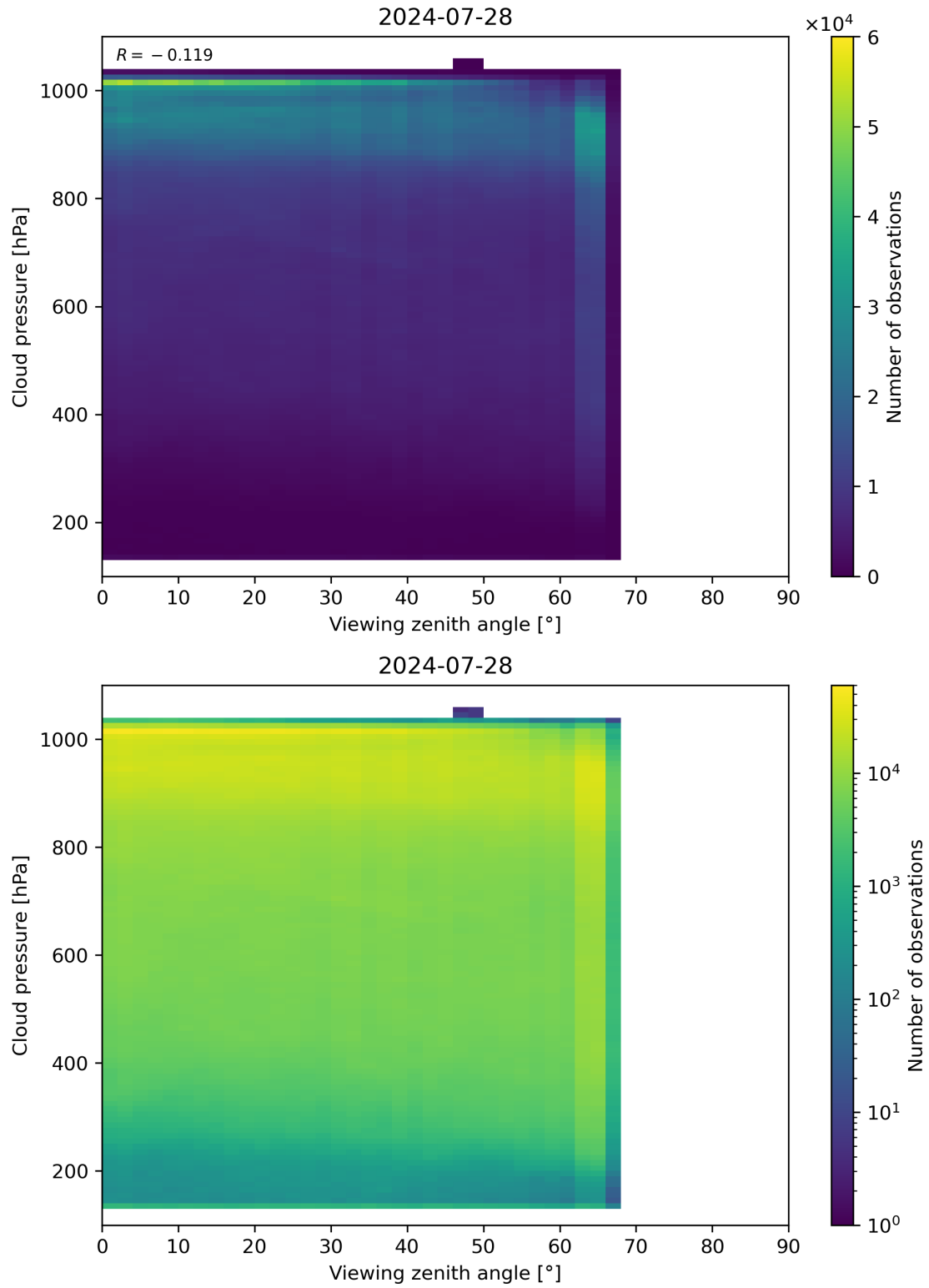
Figure 121: Scatter density plot of “Viewing zenith angle” against “Cloud pressure” for 2024-07-27 to 2024-07-29.
