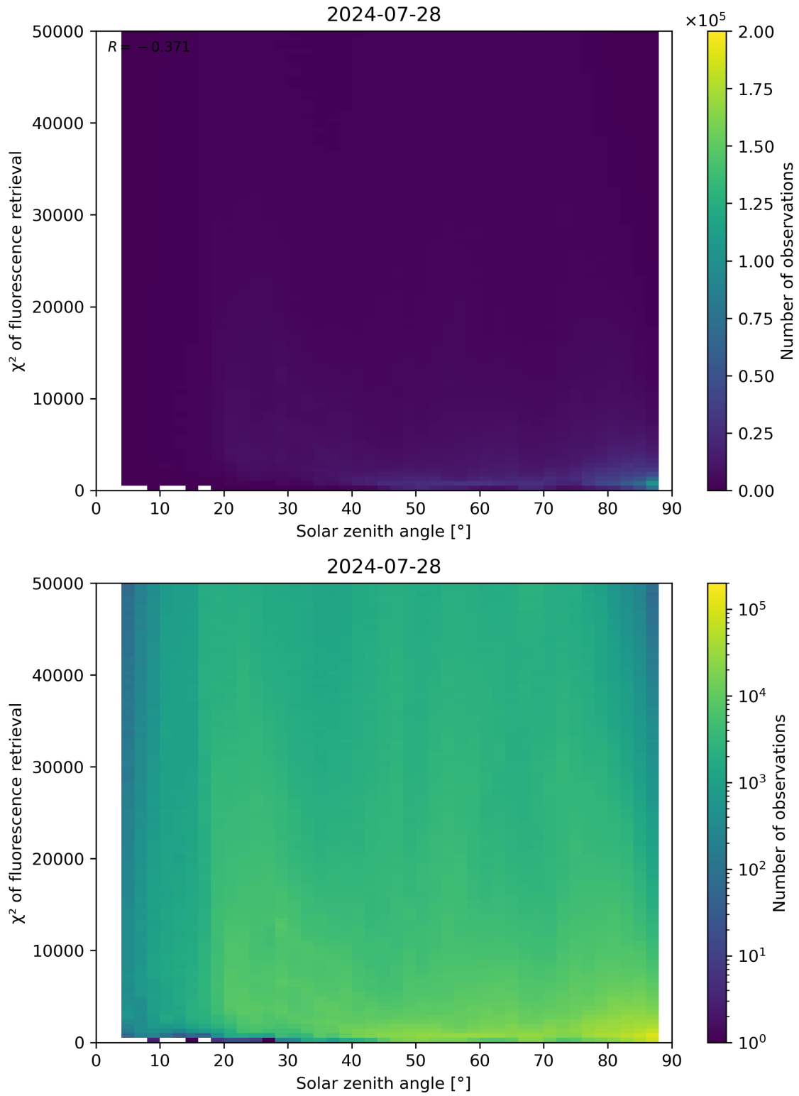
Figure 109: Scatter density plot of “Solar zenith angle” against “ \chi^2 of fluorescence retrieval” for 2024-07-27 to 2024-07-29.
