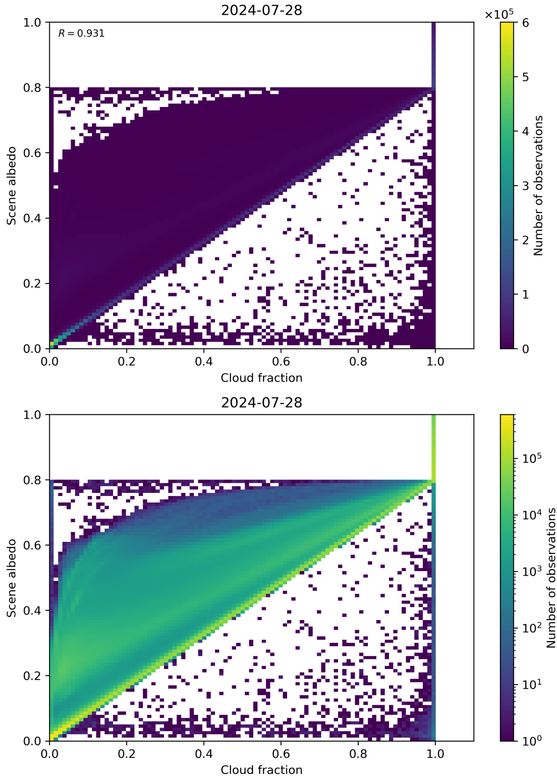
Figure 75: Scatter density plot of “Cloud fraction” against “Scene albedo” for 2024-07-27 to 2024-07-29.
