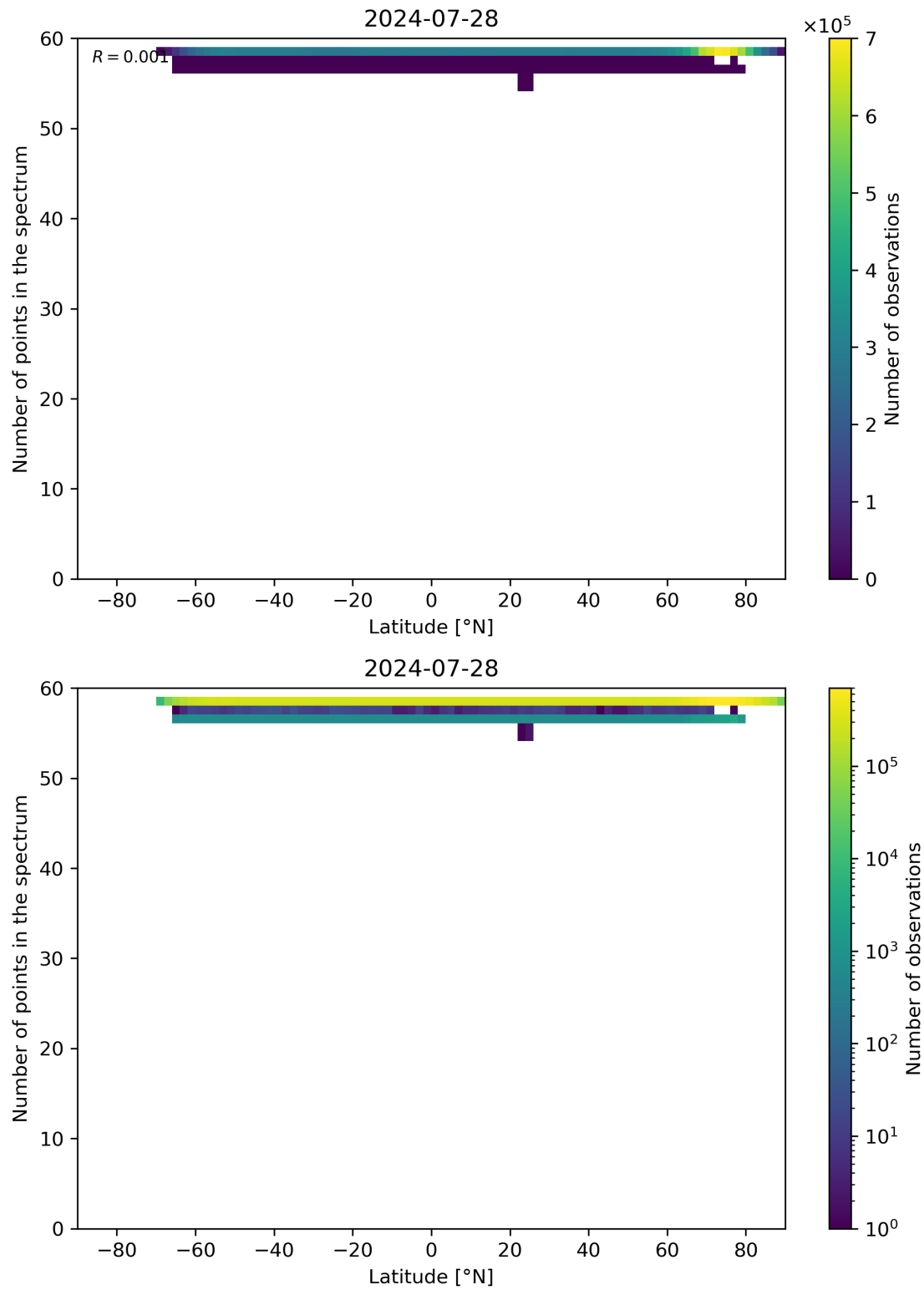
Figure 94: Scatter density plot of “Latitude” against “Number of points in the spectrum” for 2024-07-27 to 2024-07-29.
