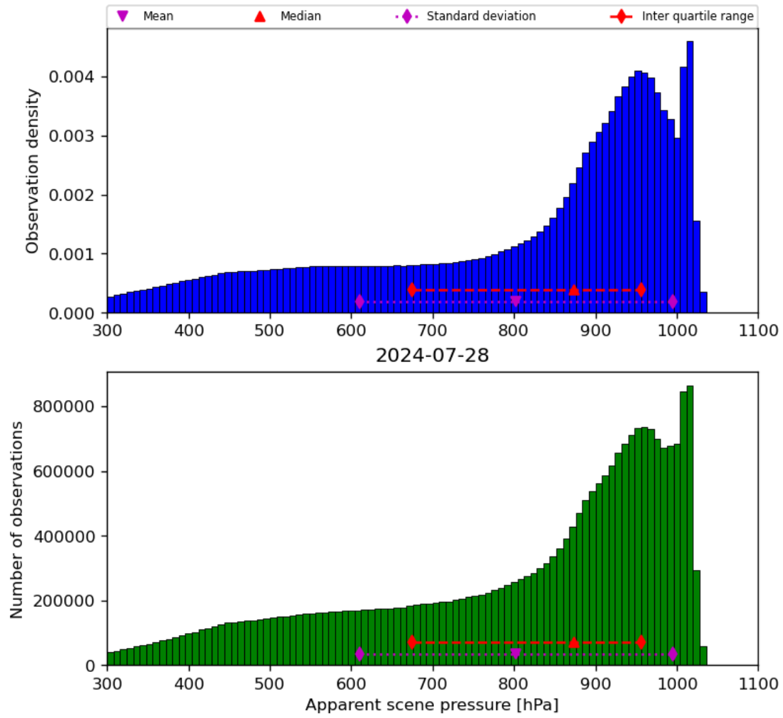
Figure 36: Histogram of “Apparent scene pressure” for 2024-07-27 to 2024-07-29
