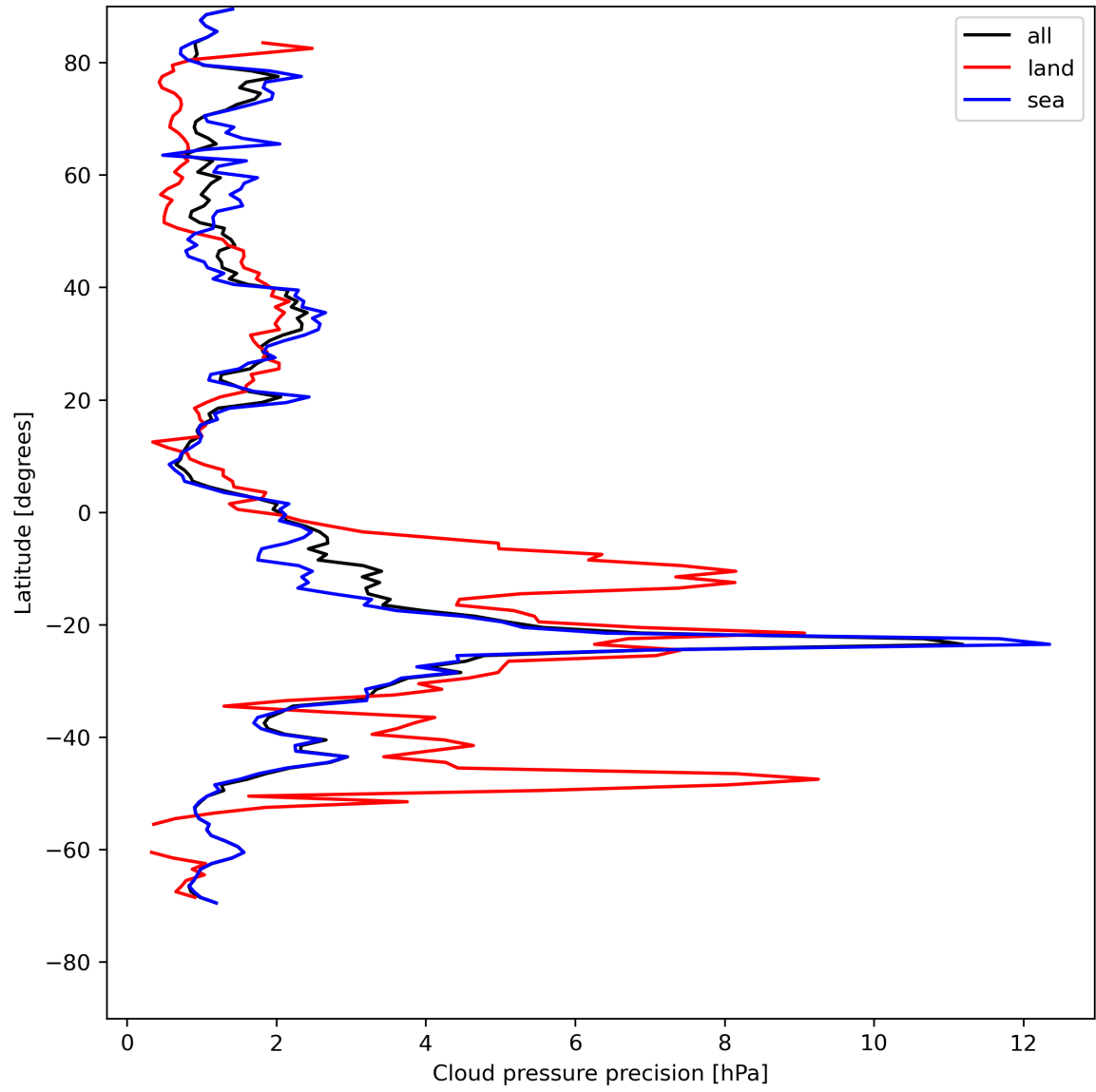
Figure 14: Zonal average of “Cloud pressure precision” for 2024-07-27 to 2024-07-29.
