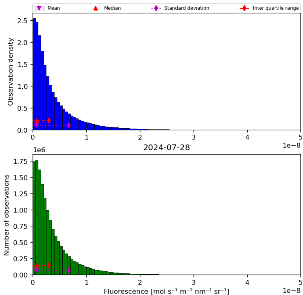
Figure 40: Histogram of “Fluorescence” for 2024-07-27 to 2024-07-29
