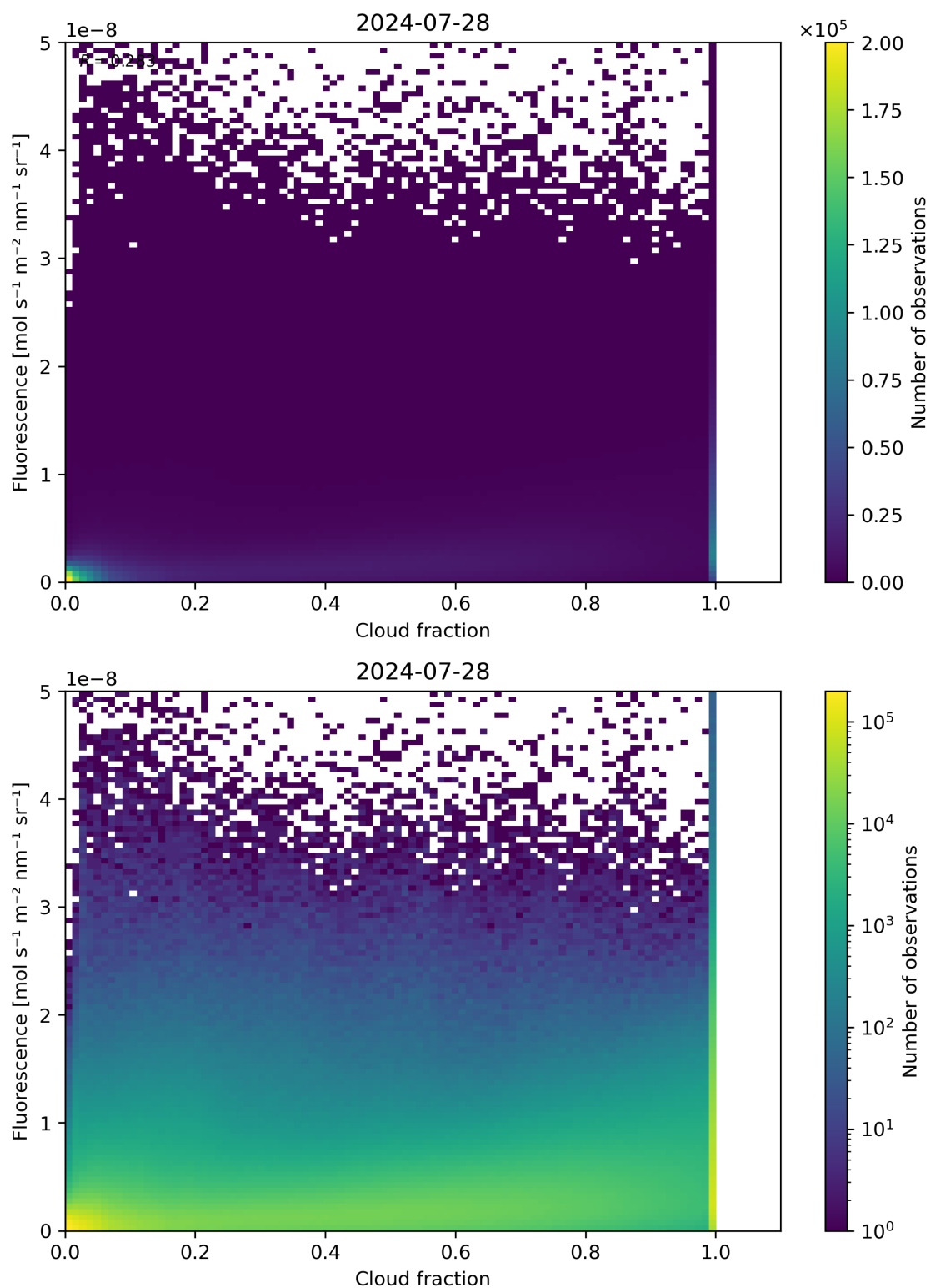
Figure 72: Scatter density plot of “Cloud fraction” against “Fluorescence” for 2024-07-27 to 2024-07-29.
