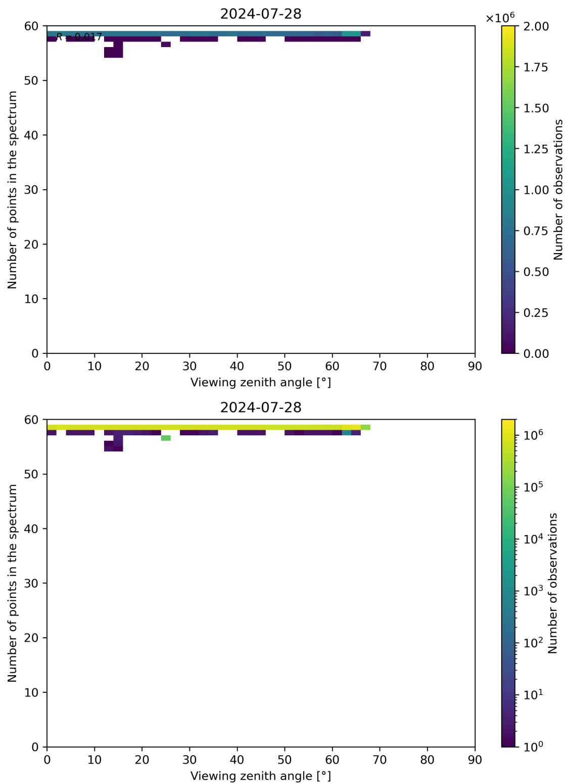
Figure 125: Scatter density plot of “Viewing zenith angle” against “Number of points in the spectrum” for 2024-07-27 to 2024-07-29.
