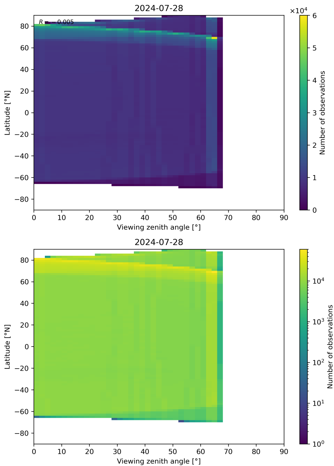
Figure 123: Scatter density plot of “Viewing zenith angle” against “Latitude” for 2024-07-27 to 2024-07-29.
