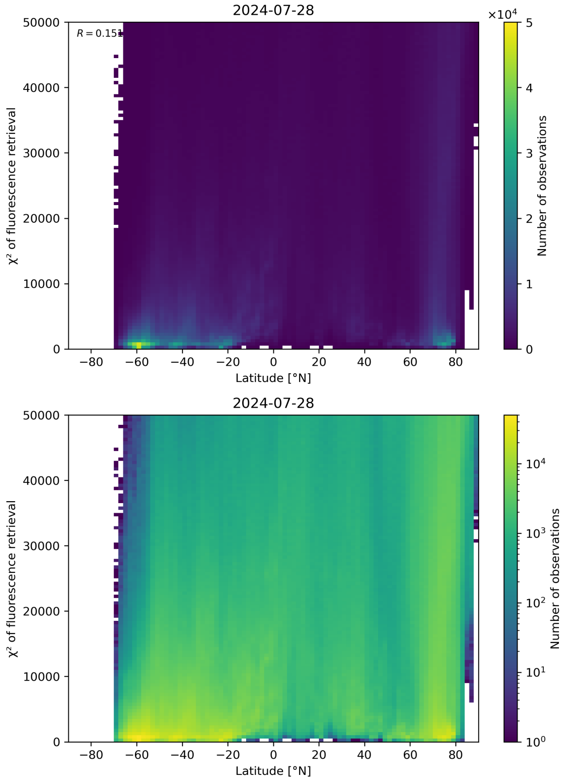
Figure 89: Scatter density plot of “Latitude” against “ \chi^2 of fluorescence retrieval” for 2024-07-27 to 2024-07-29.
