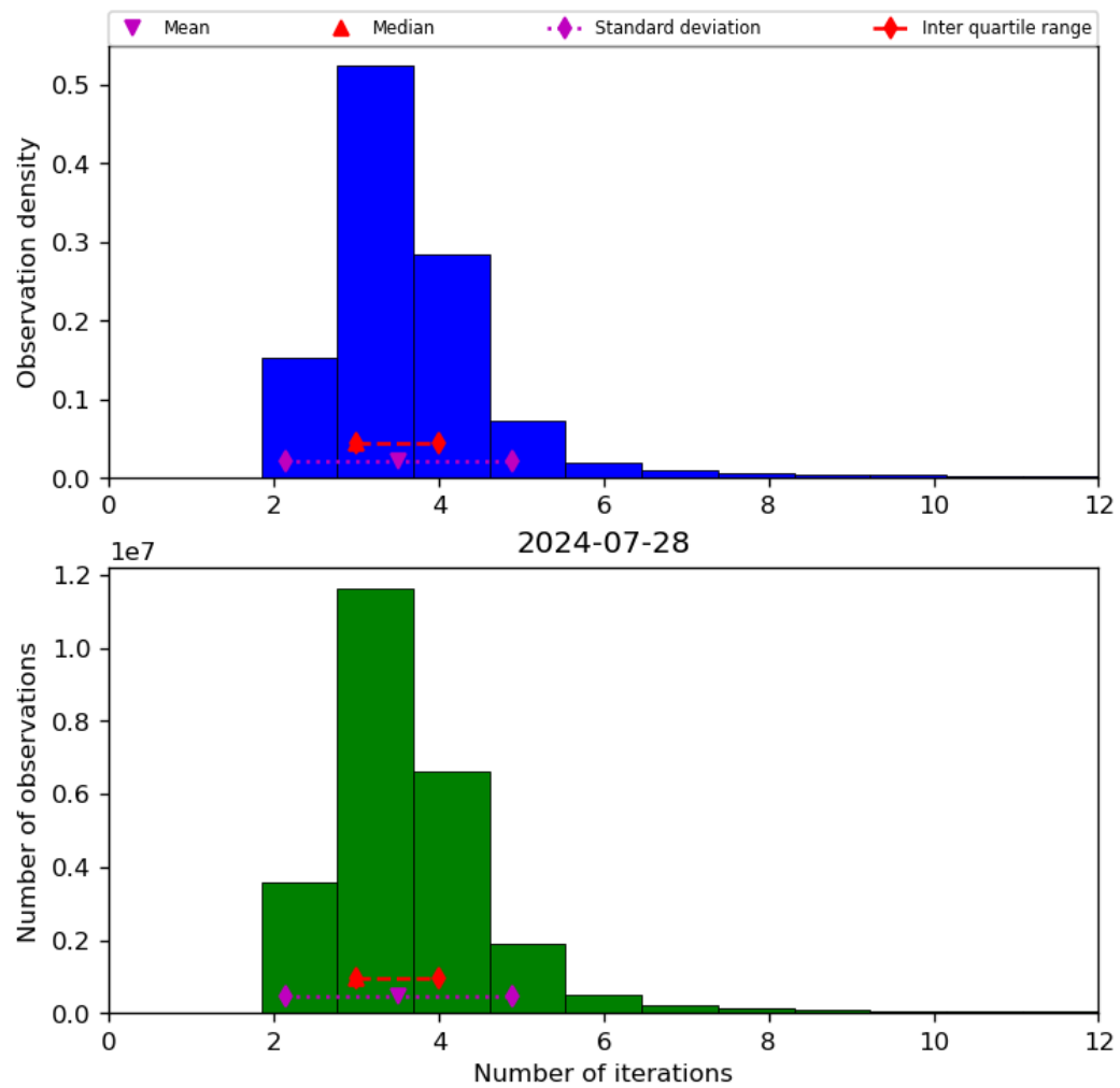
Figure 39: Histogram of “Number of iterations” for 2024-07-27 to 2024-07-29
