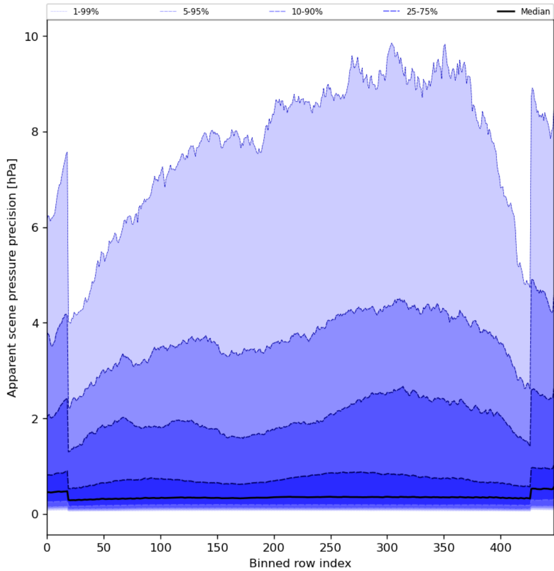
Figure 54: Along track statistics of “Apparent scene pressure precision” for 2024-07-27 to 2024-07-29
