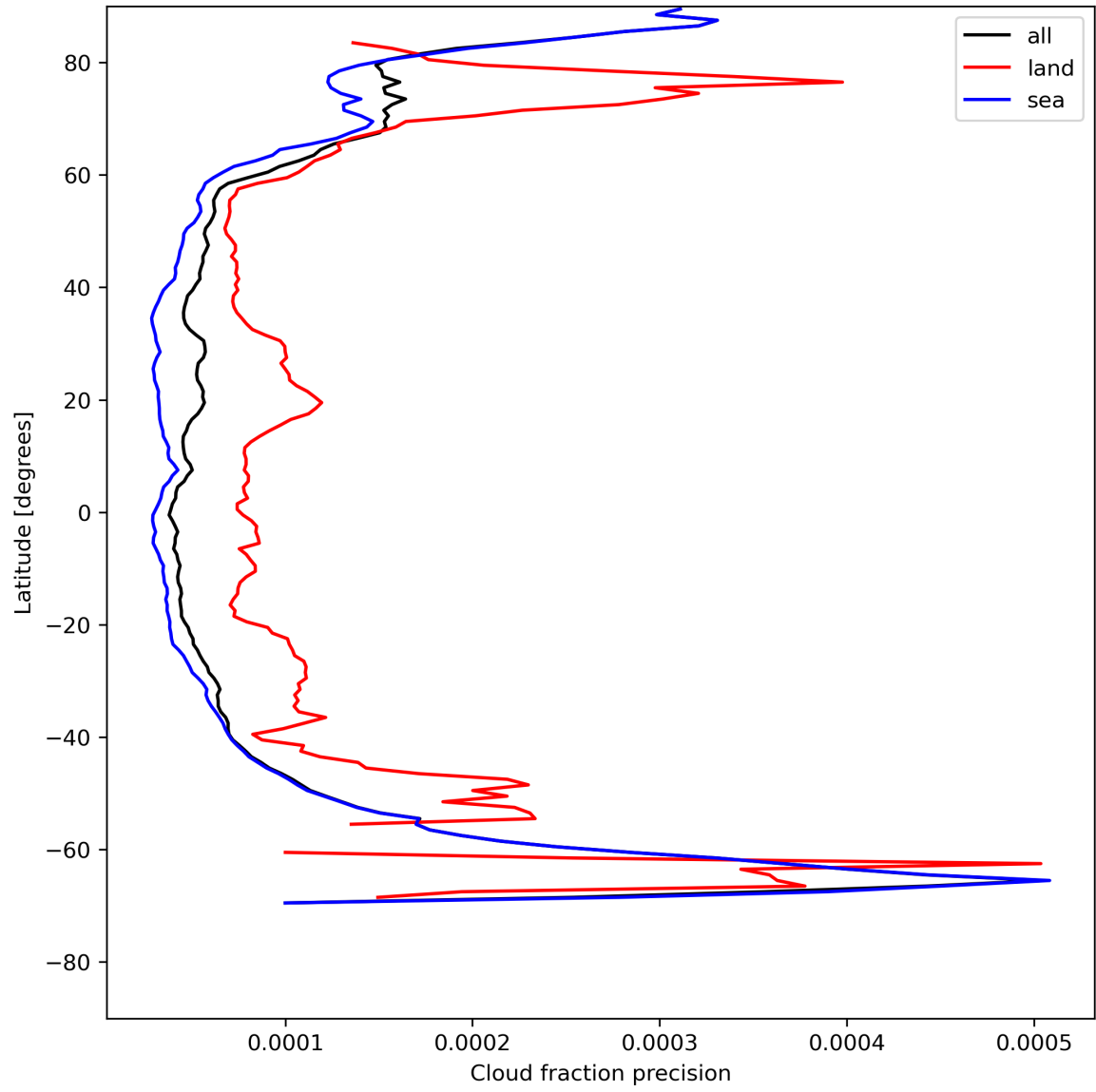
Figure 16: Zonal average of “Cloud fraction precision” for 2024-07-27 to 2024-07-29.
