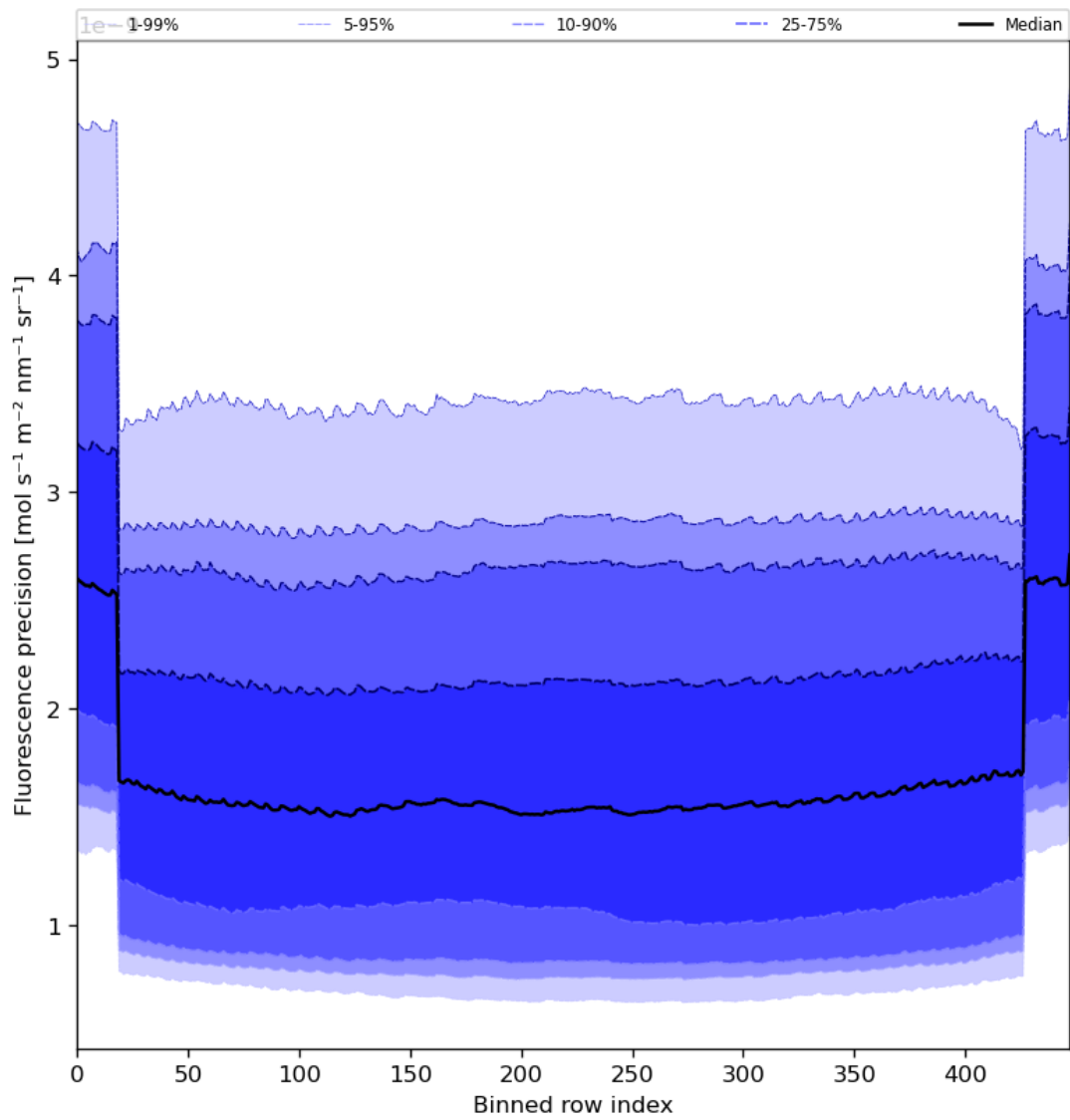
Figure 58: Along track statistics of “Fluorescence precision” for 2024-07-27 to 2024-07-29
