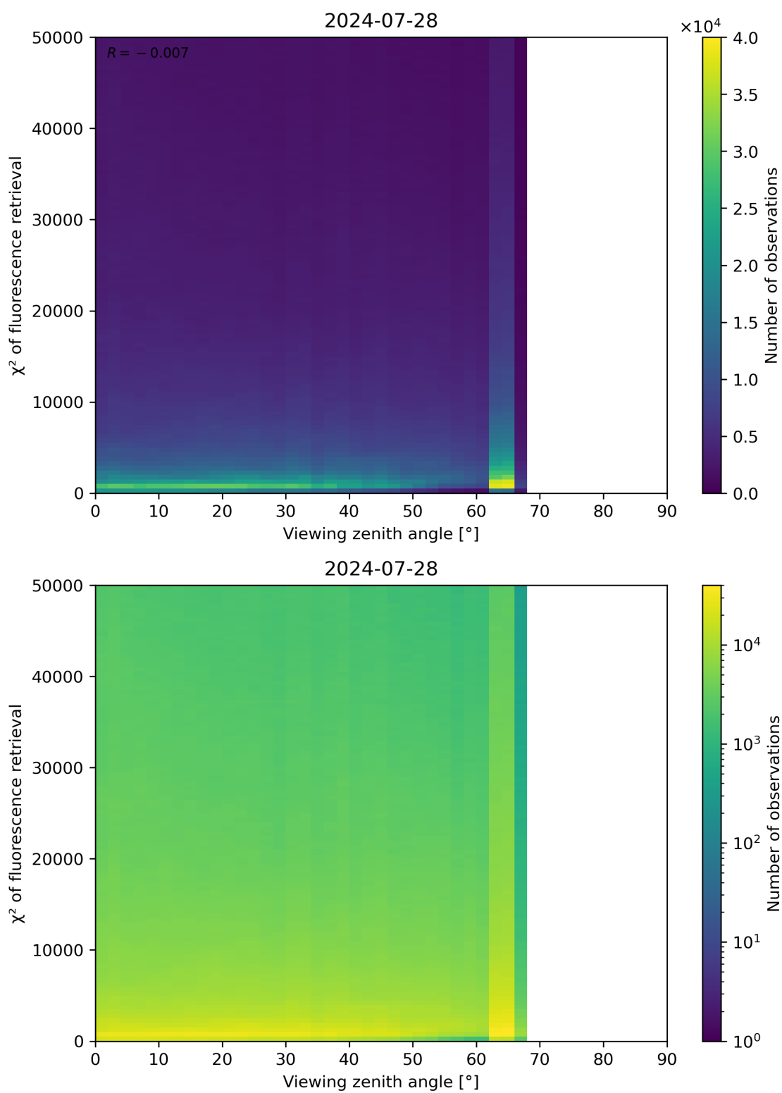
Figure 119: Scatter density plot of “Viewing zenith angle” against “ \chi^2 of fluorescence retrieval” for 2024-07-27 to 2024-07-29.
