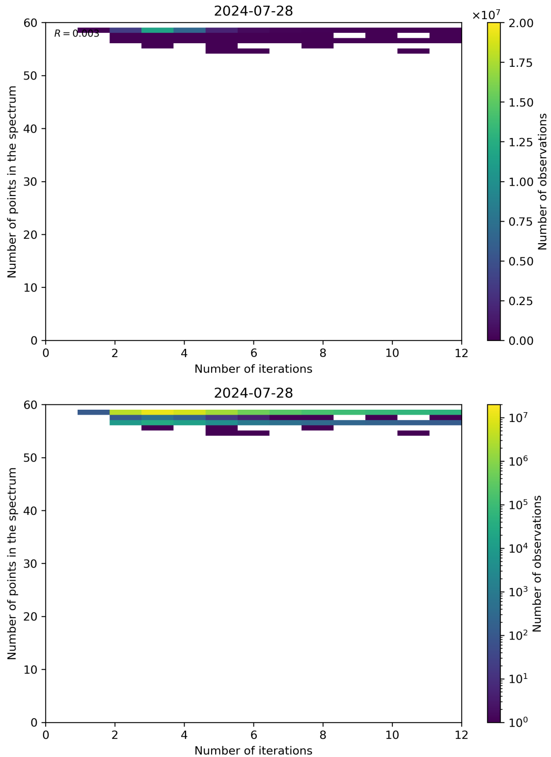
Figure 99: Scatter density plot of “Number of iterations” against “Number of points in the spectrum” for 2024-07-27 to 2024-07-29.
