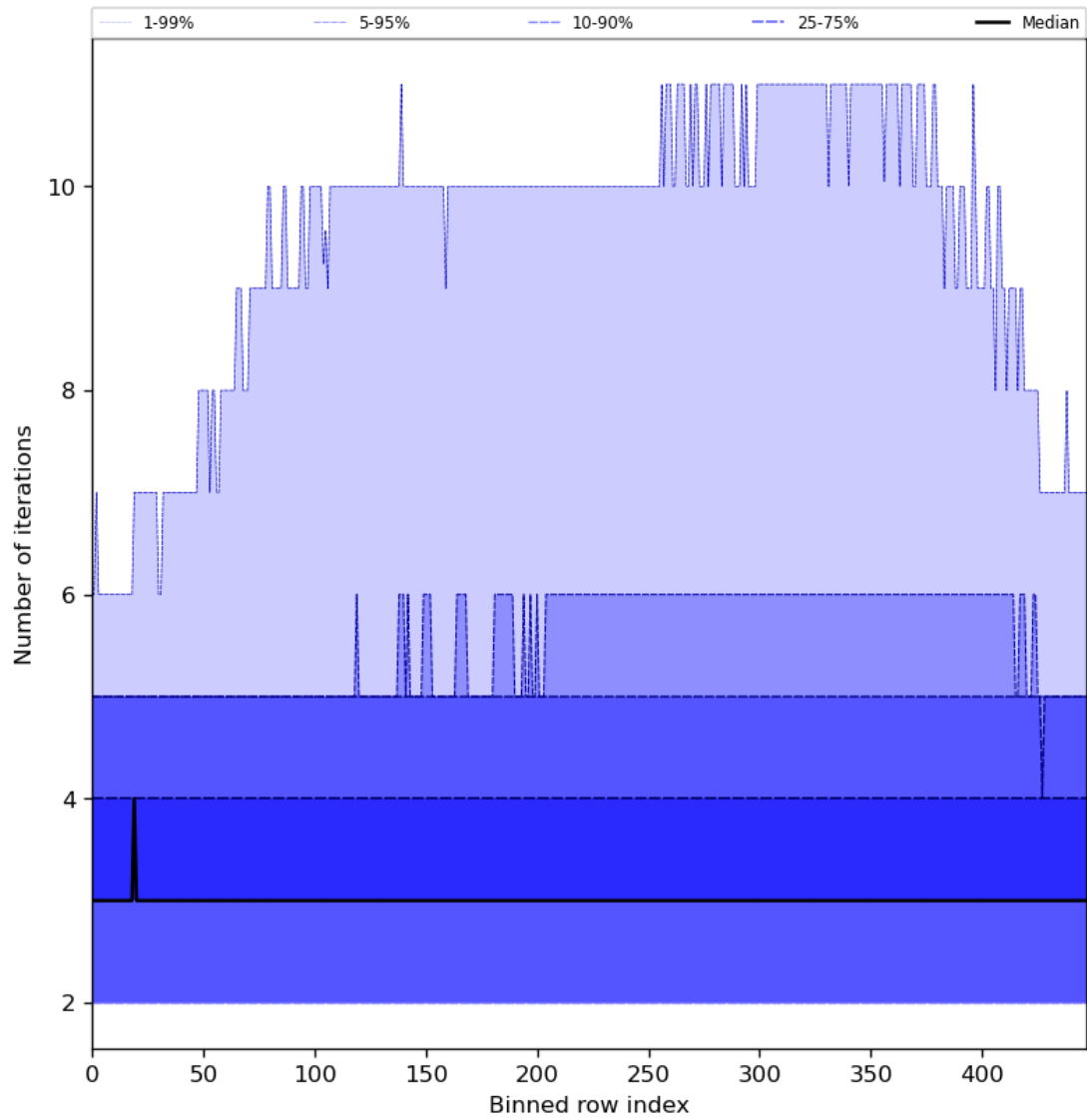
Figure 56: Along track statistics of “Number of iterations” for 2024-07-27 to 2024-07-29
