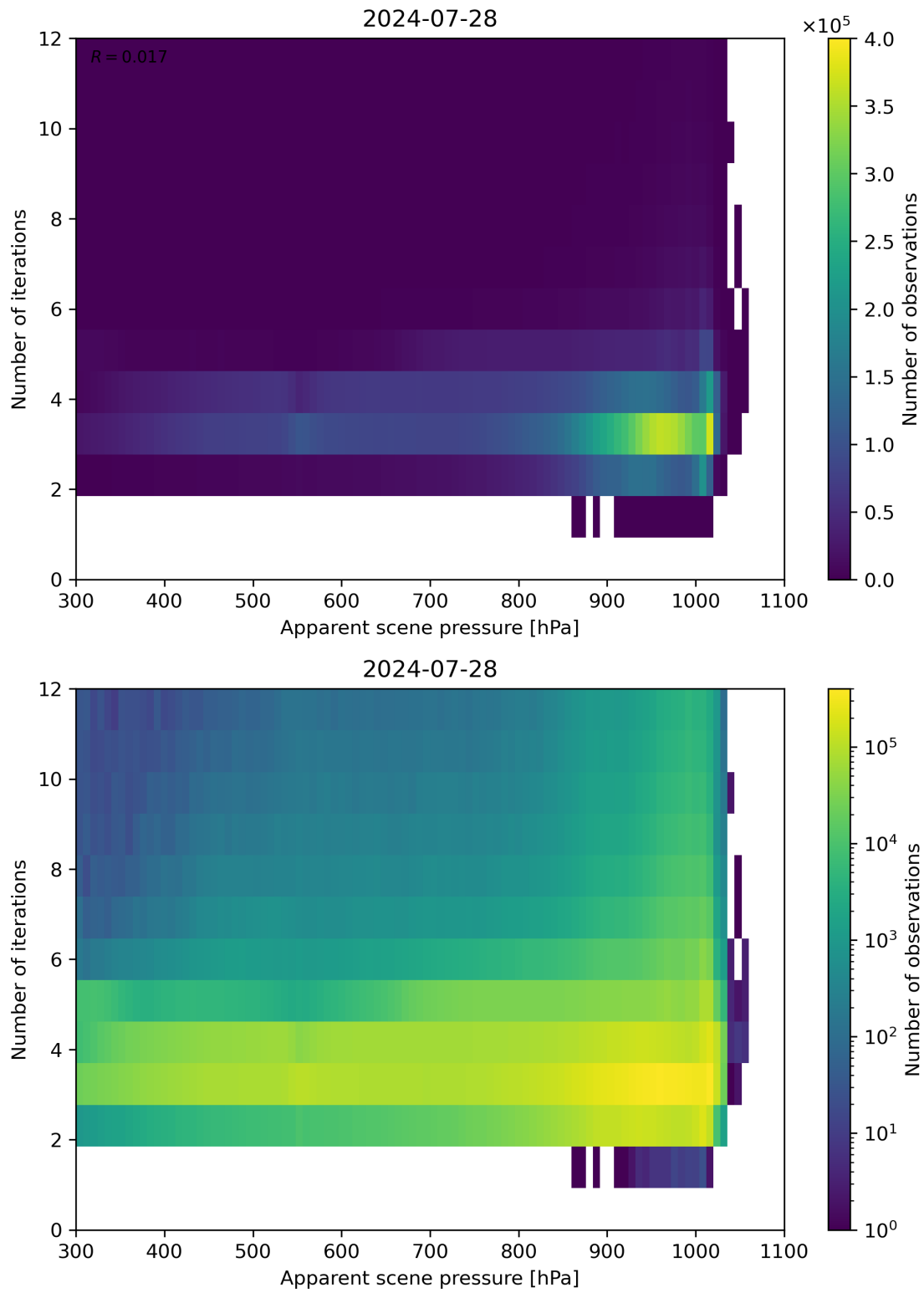
Figure 65: Scatter density plot of “Apparent scene pressure” against “Number of iterations” for 2024-07-27 to 2024-07-29.
