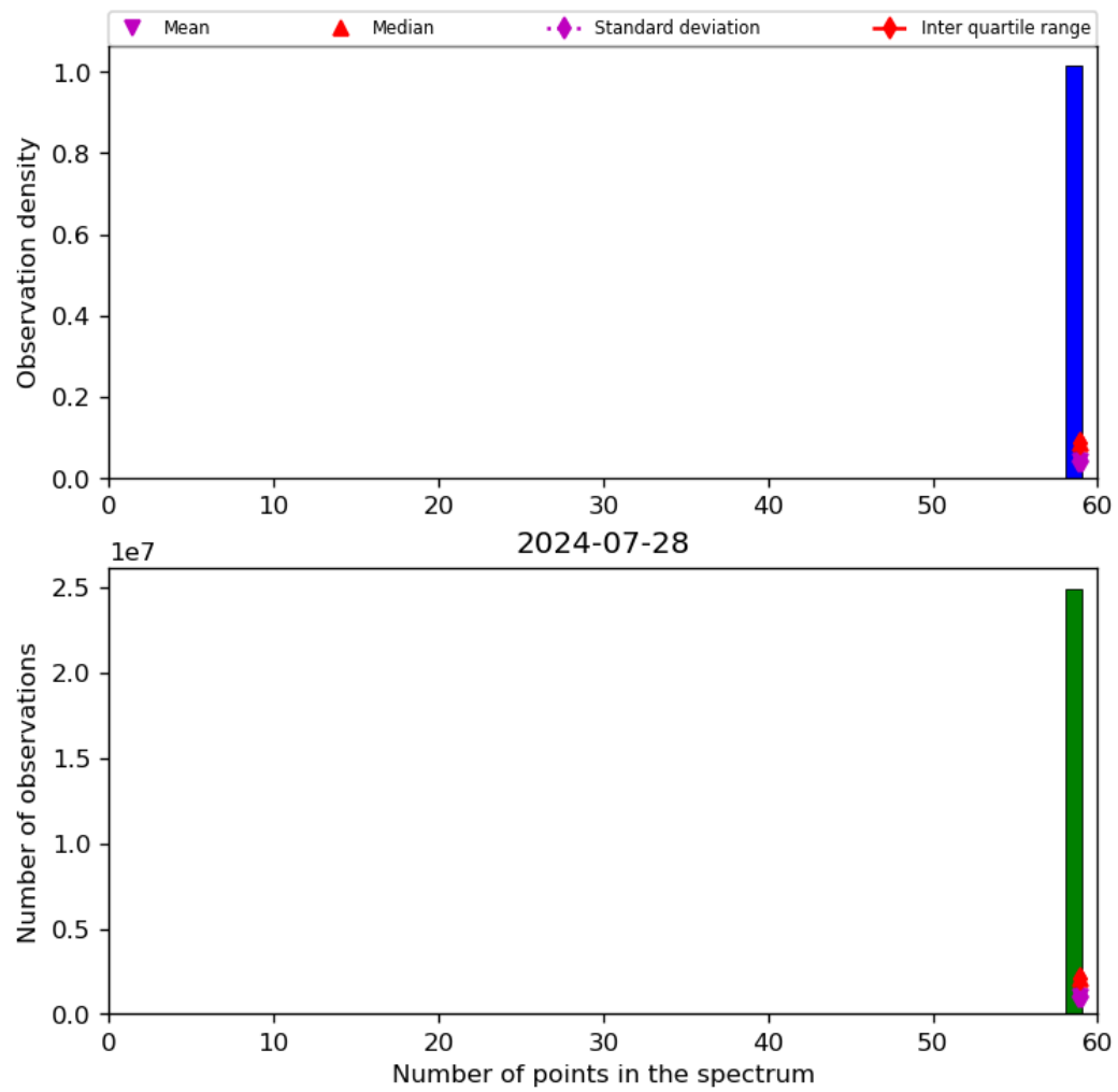
Figure 44: Histogram of “Number of points in the spectrum” for 2024-07-27 to 2024-07-29
