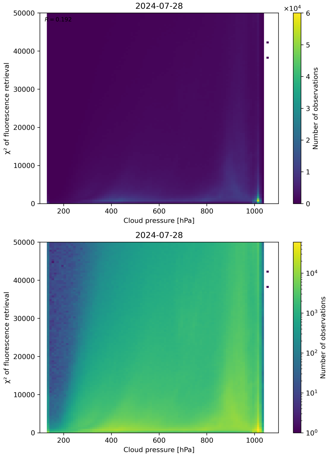
Figure 78: Scatter density plot of “Cloud pressure” against “ \chi^2 of fluorescence retrieval” for 2024-07-27 to 2024-07-29.
