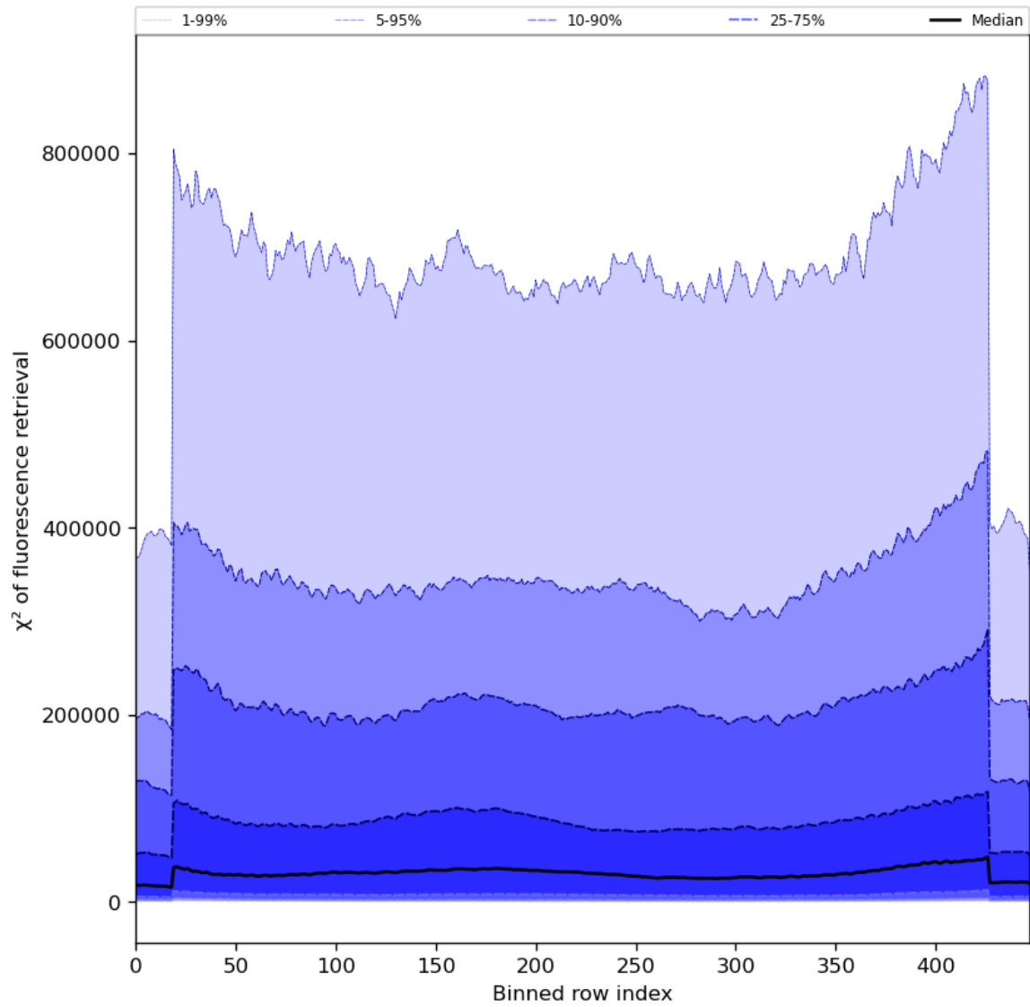
Figure 59: Along track statistics of “ \chi^2 of fluorescence retrieval” for 2024-07-27 to 2024-07-29
