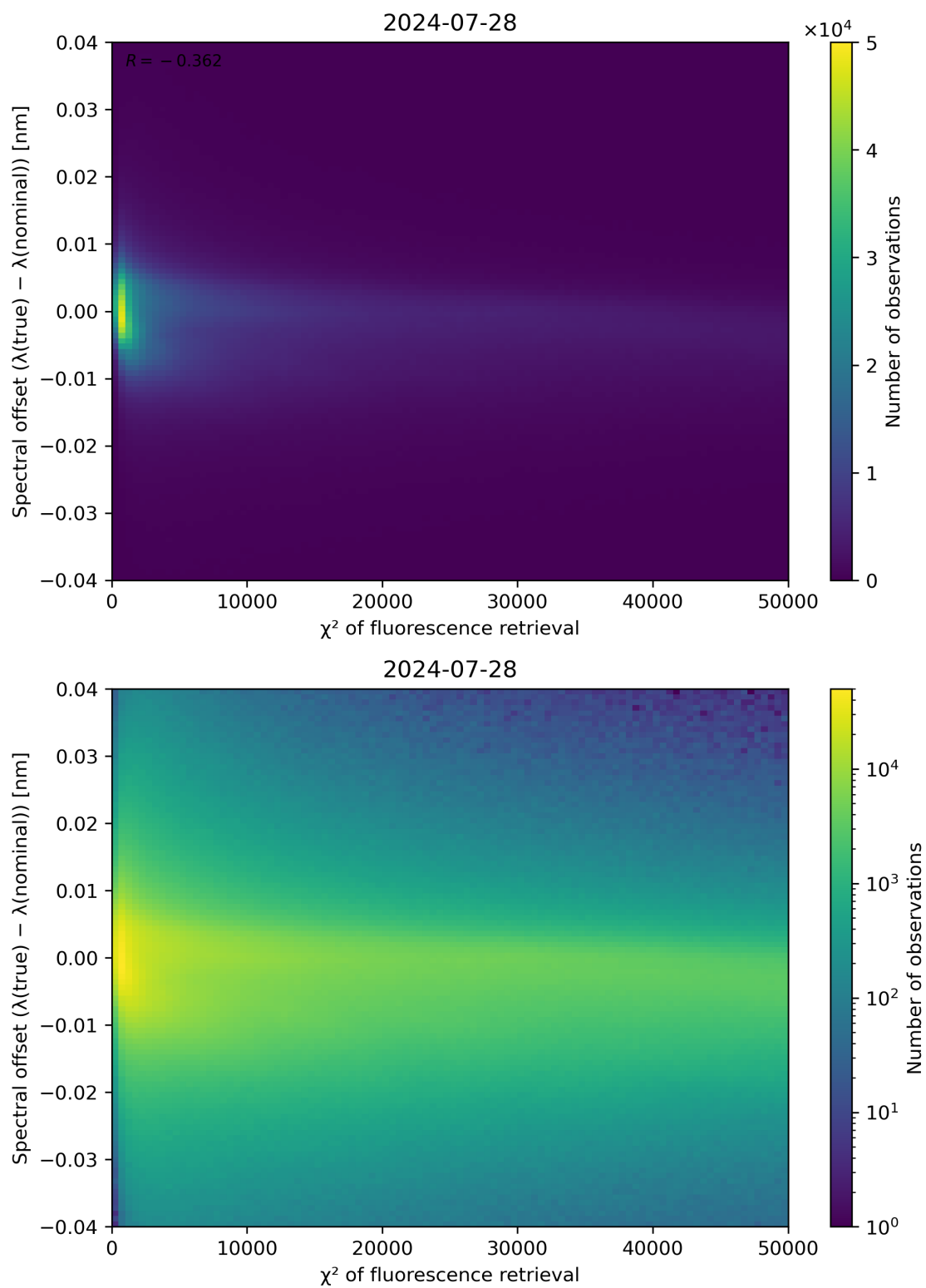
Figure 69: Scatter density plot of “ \chi^2 of fluorescence retrieval” against “Spectral offset ( \lambda(\text{true}) - \lambda(\text{nominal}) )” for 2024-07-27 to 2024-07-29.
