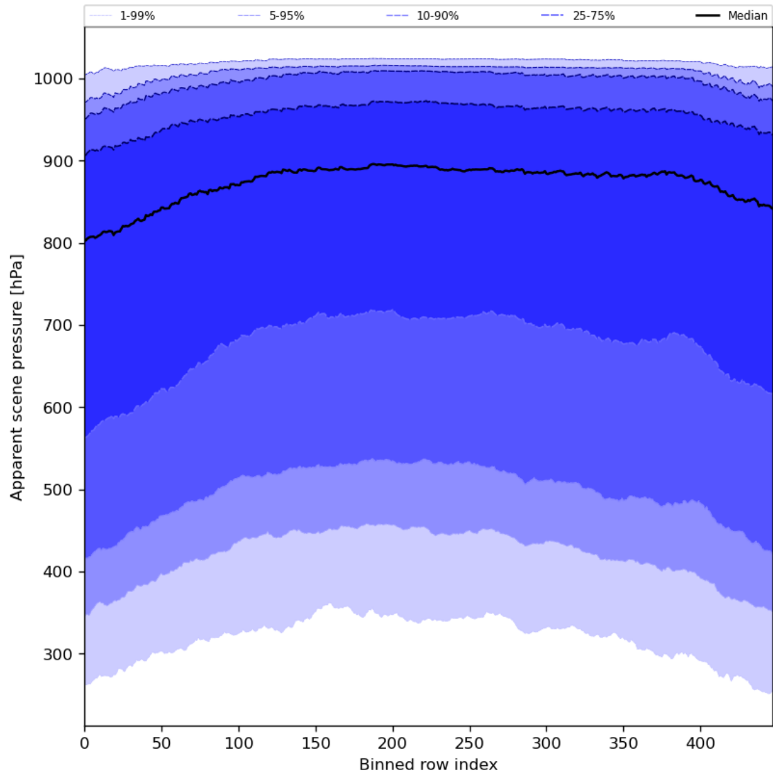
Figure 53: Along track statistics of “Apparent scene pressure” for 2024-07-27 to 2024-07-29
