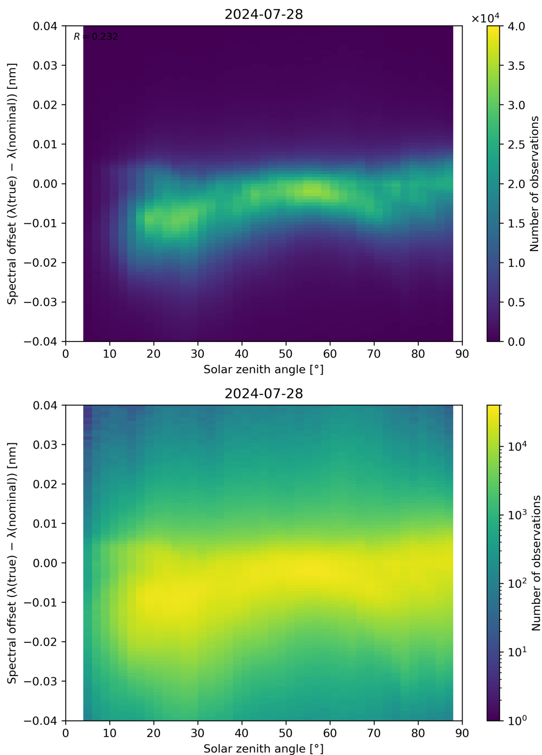
Figure 117: Scatter density plot of “Solar zenith angle” against “Spectral offset ( \lambda(\text{true}) - \lambda(\text{nominal}) )” for 2024-07-27 to 2024-07-29.
