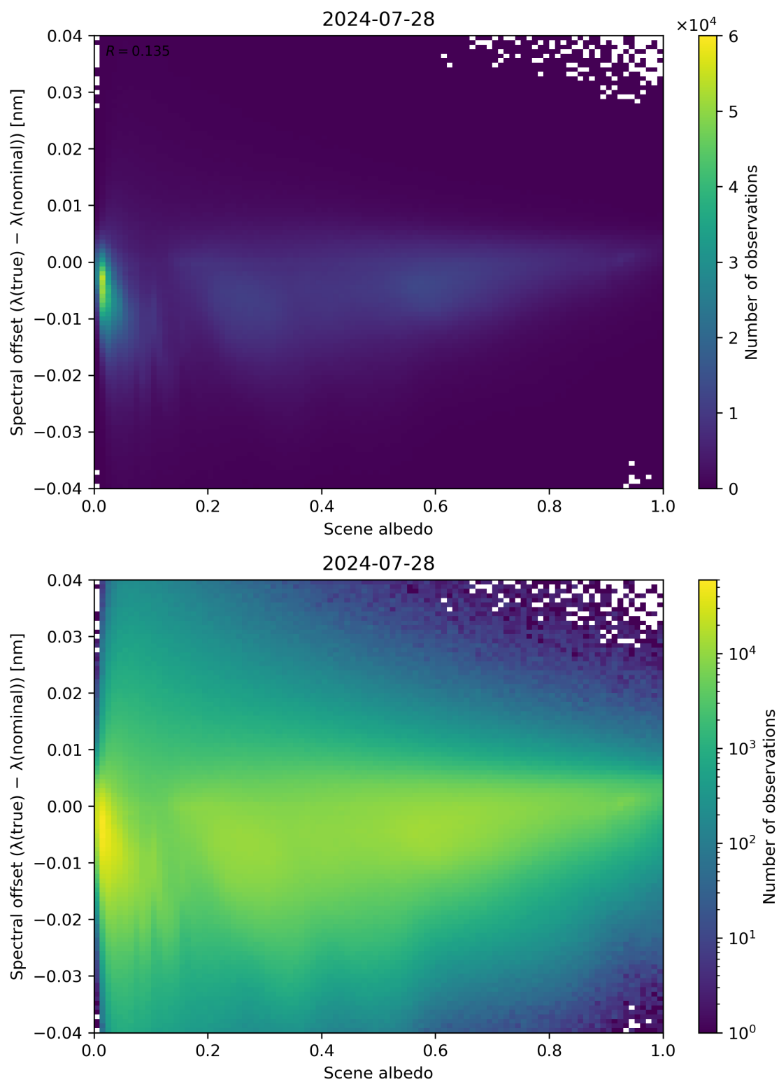
Figure 107: Scatter density plot of “Scene albedo” against “Spectral offset ( \lambda(\text{true}) - \lambda(\text{nominal}) )” for 2024-07-27 to 2024-07-29.
