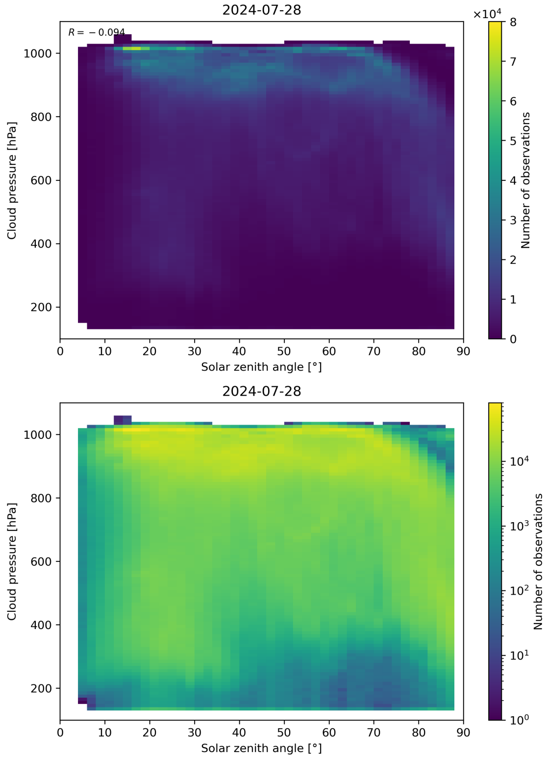
Figure 111: Scatter density plot of “Solar zenith angle” against “Cloud pressure” for 2024-07-27 to 2024-07-29.
