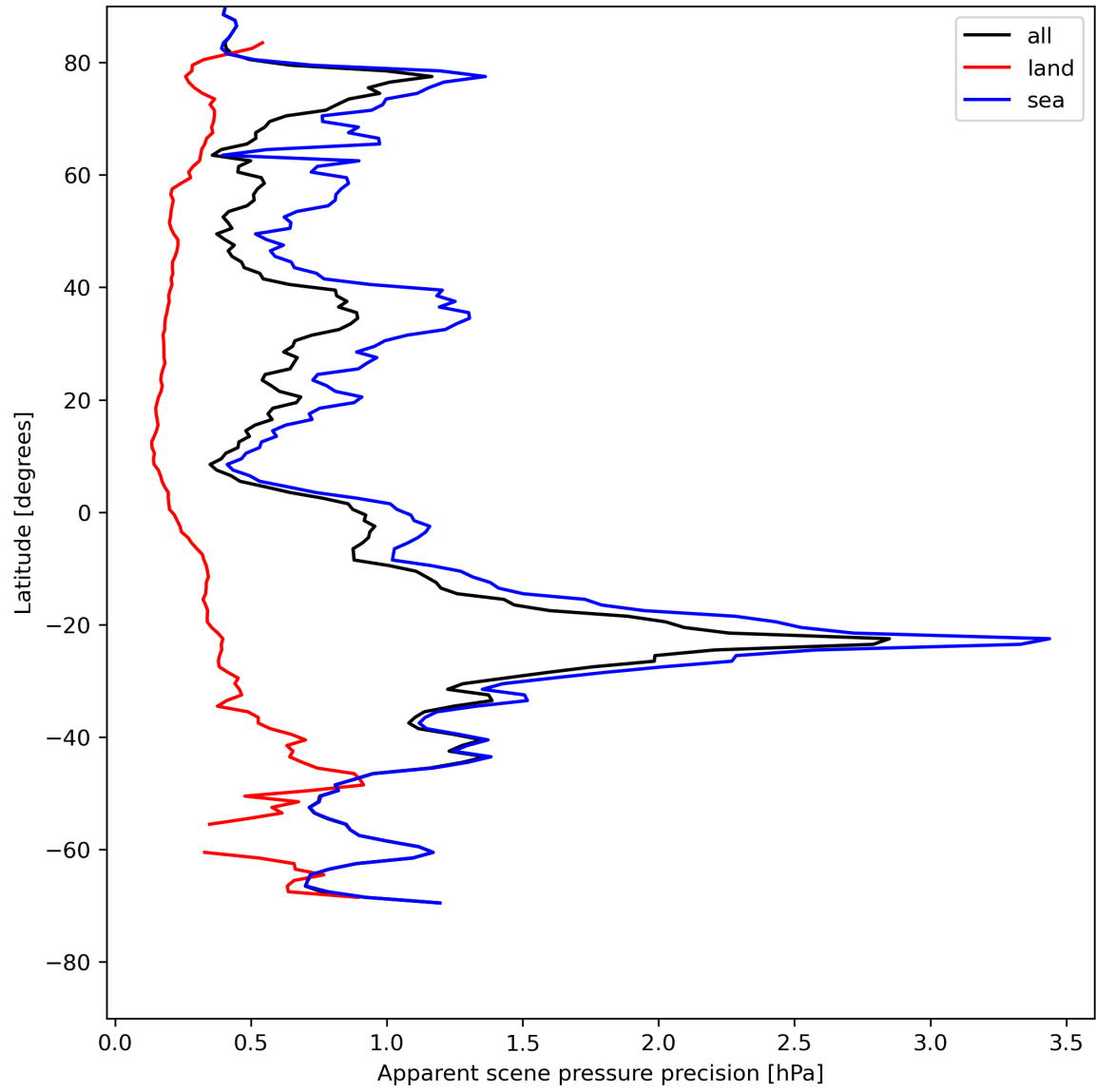
Figure 20: Zonal average of “Apparent scene pressure precision” for 2024-07-27 to 2024-07-29.
