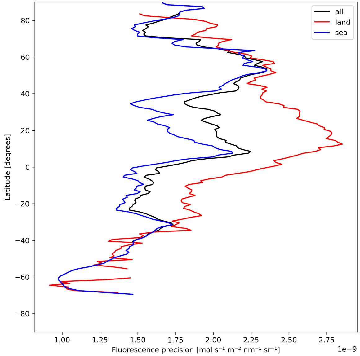
Figure 24: Zonal average of “Fluorescence precision” for 2024-07-27 to 2024-07-29.
