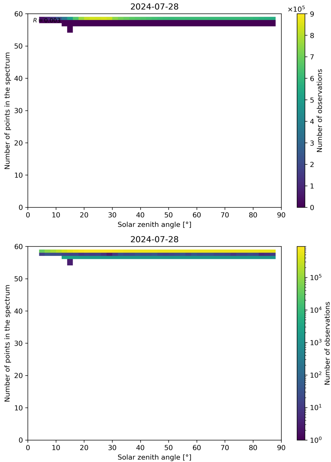
Figure 115: Scatter density plot of “Solar zenith angle” against “Number of points in the spectrum” for 2024-07-27 to 2024-07-29.
