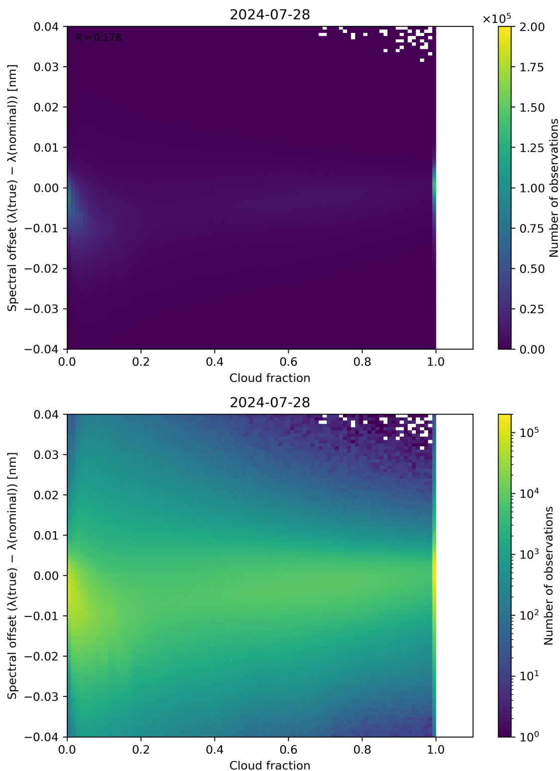
Figure 76: Scatter density plot of “Cloud fraction” against “Spectral offset ( \lambda(\text{true}) - \lambda(\text{nominal}) )” for 2024-07-27 to 2024-07-29.
