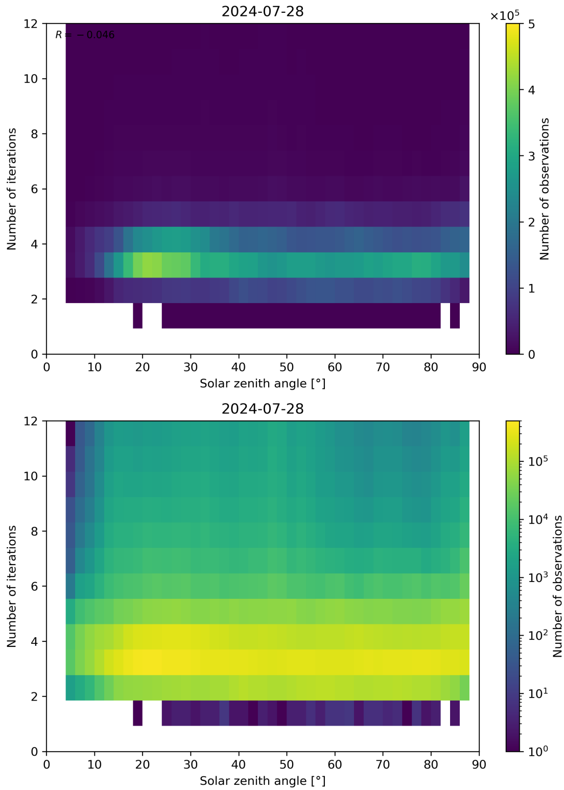
Figure 114: Scatter density plot of “Solar zenith angle” against “Number of iterations” for 2024-07-27 to 2024-07-29.
