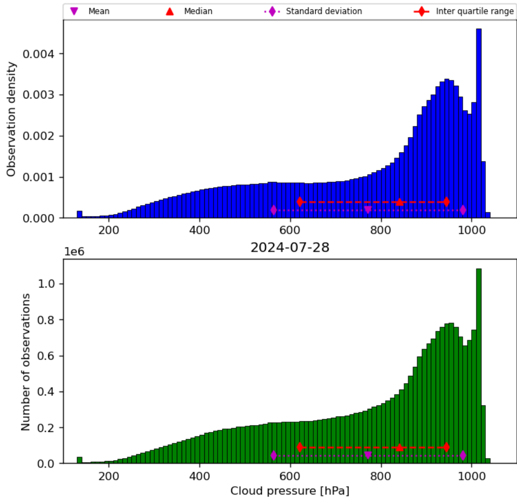
Figure 30: Histogram of “Cloud pressure” for 2024-07-27 to 2024-07-29
