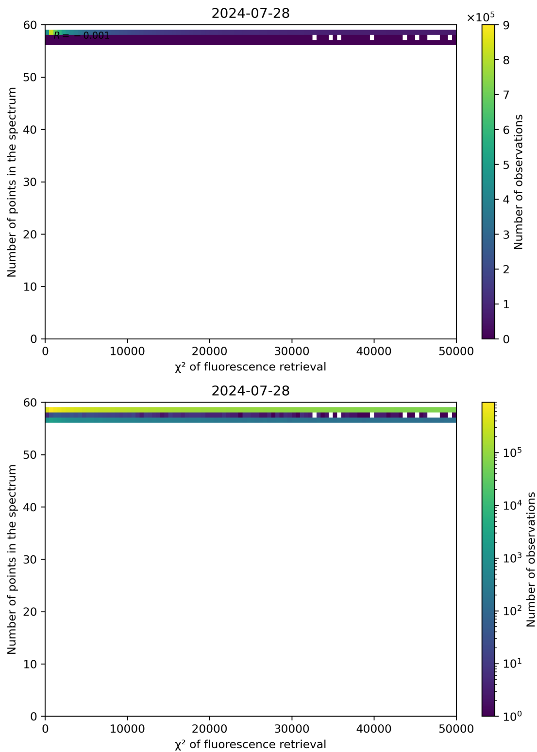
Figure 68: Scatter density plot of " \chi^2 of fluorescence retrieval" against "Number of points in the spectrum" for 2024-07-27 to 2024-07-29.
