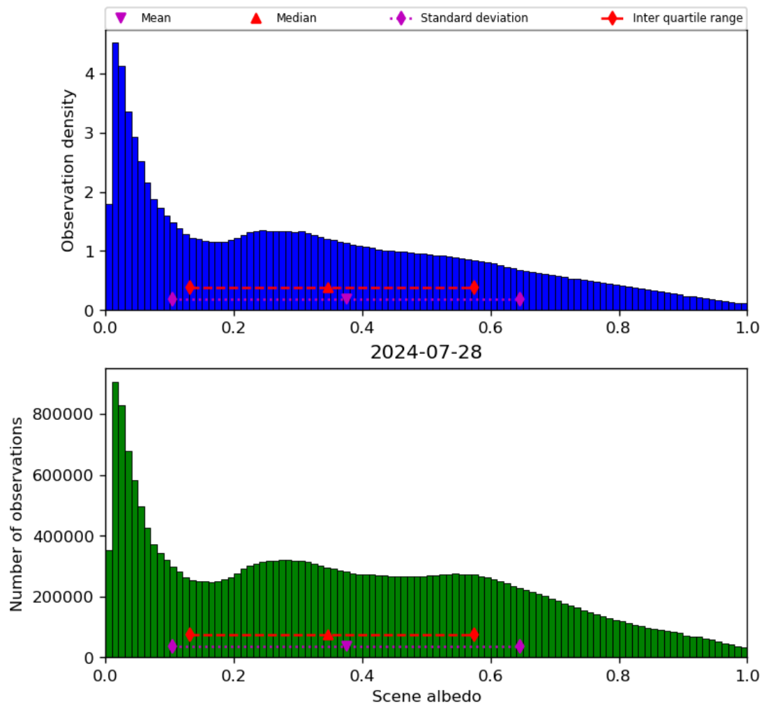
Figure 34: Histogram of “Scene albedo” for 2024-07-27 to 2024-07-29
