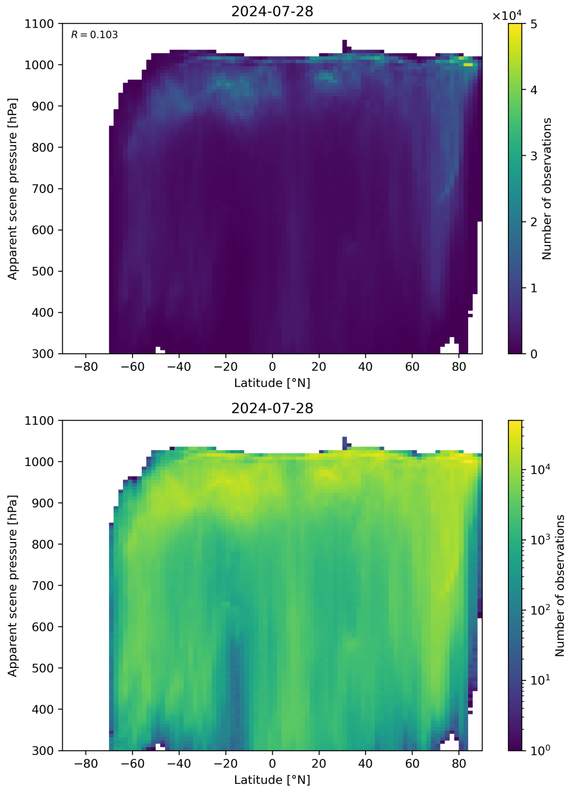
Figure 88: Scatter density plot of “Latitude” against “Apparent scene pressure” for 2024-07-27 to 2024-07-29.
