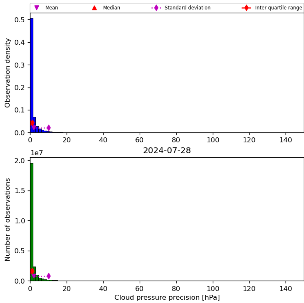
Figure 31: Histogram of “Cloud pressure precision” for 2024-07-27 to 2024-07-29
