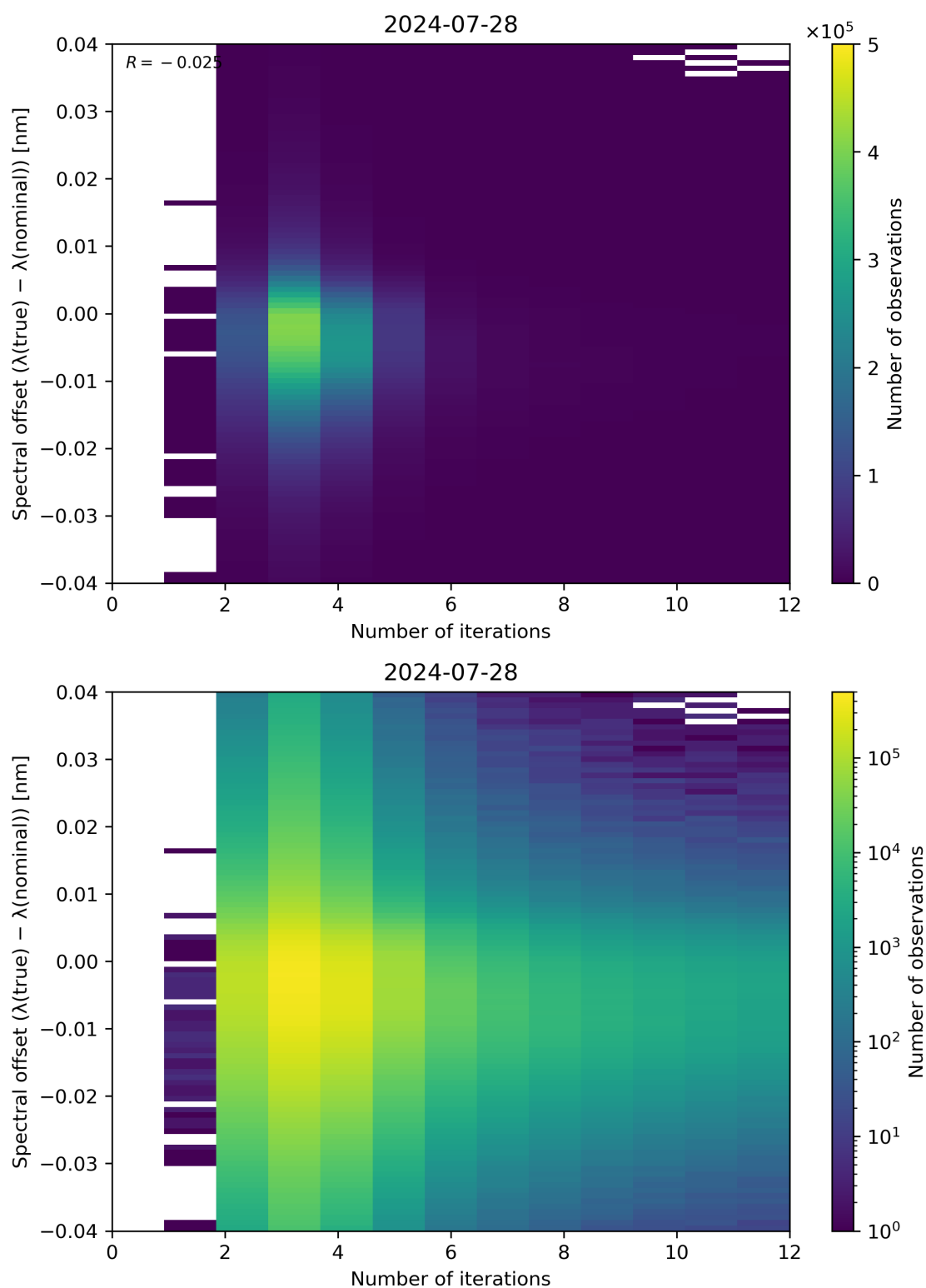
Figure 100: Scatter density plot of “Number of iterations” against “Spectral offset ( \lambda(\text{true}) - \lambda(\text{nominal}) )” for 2024-07-27 to 2024-07-29.
