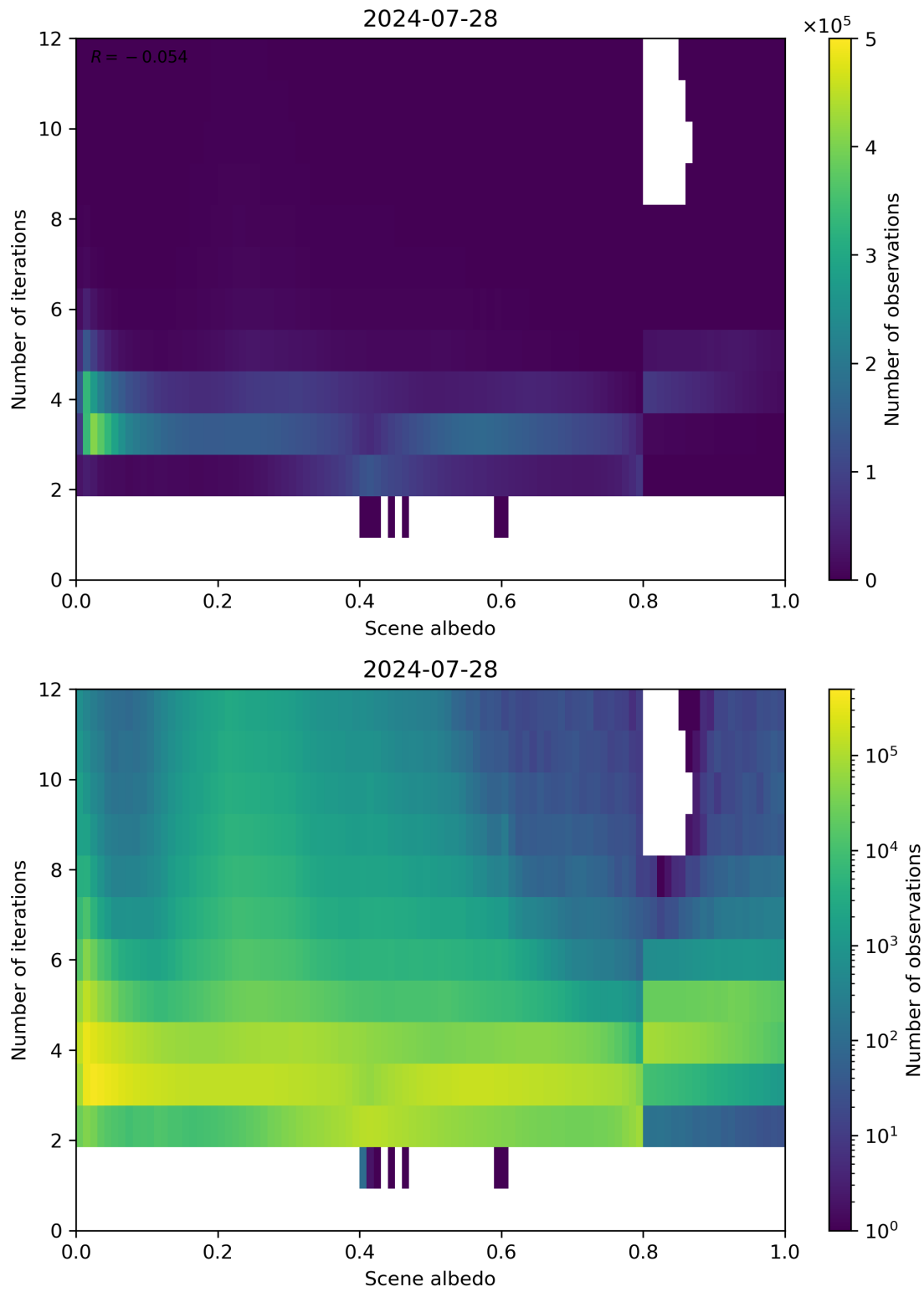
Figure 105: Scatter density plot of “Scene albedo” against “Number of iterations” for 2024-07-27 to 2024-07-29.
