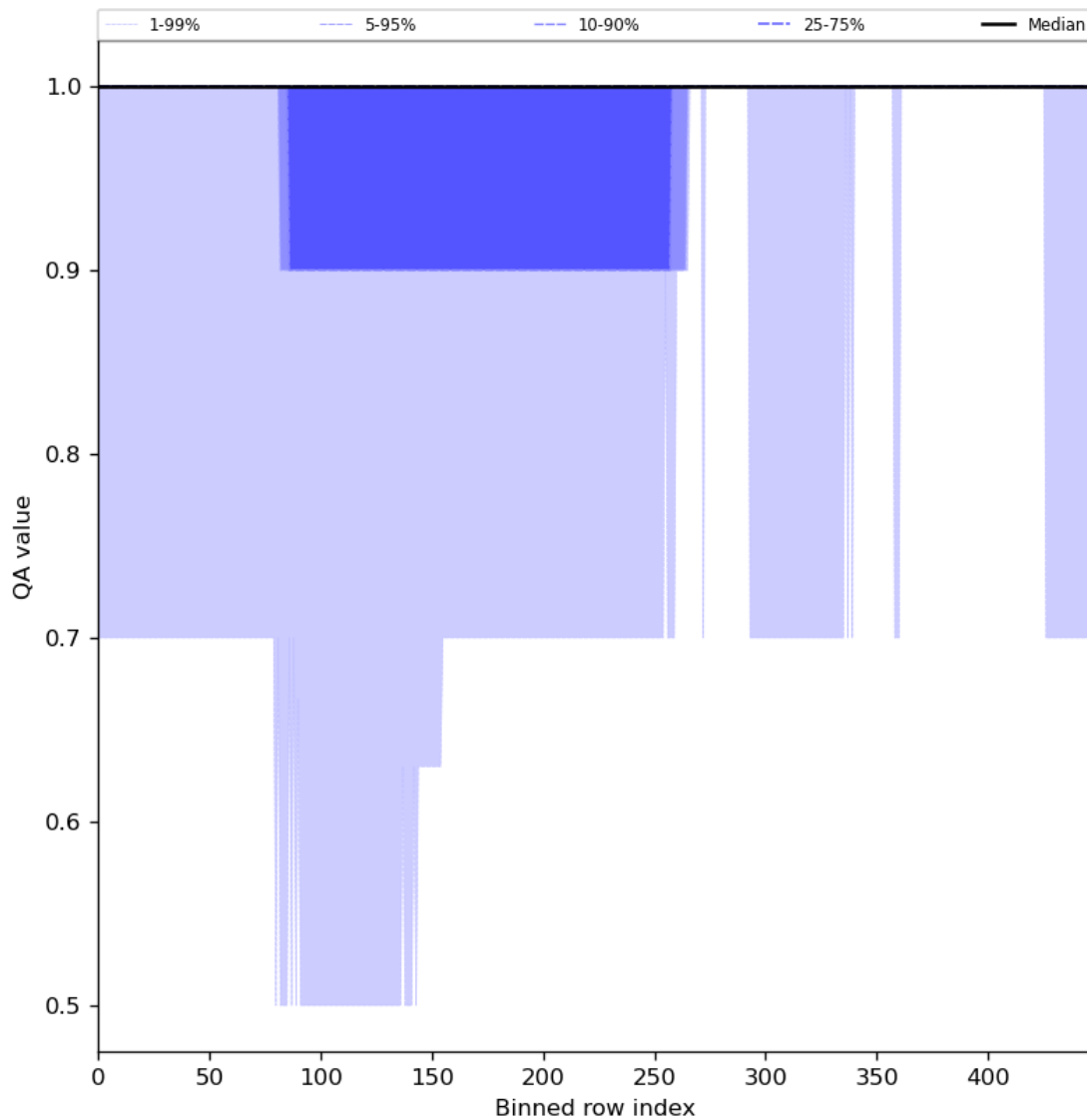
Figure 46: Along track statistics of “QA value” for 2024-07-27 to 2024-07-29
