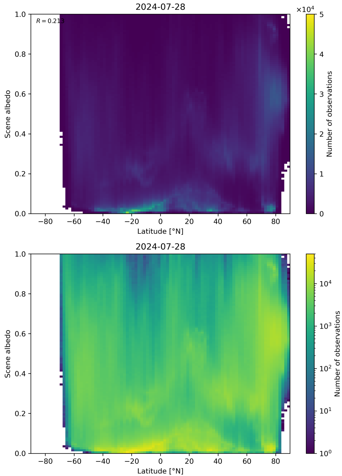
Figure 95: Scatter density plot of “Latitude” against “Scene albedo” for 2024-07-27 to 2024-07-29.
