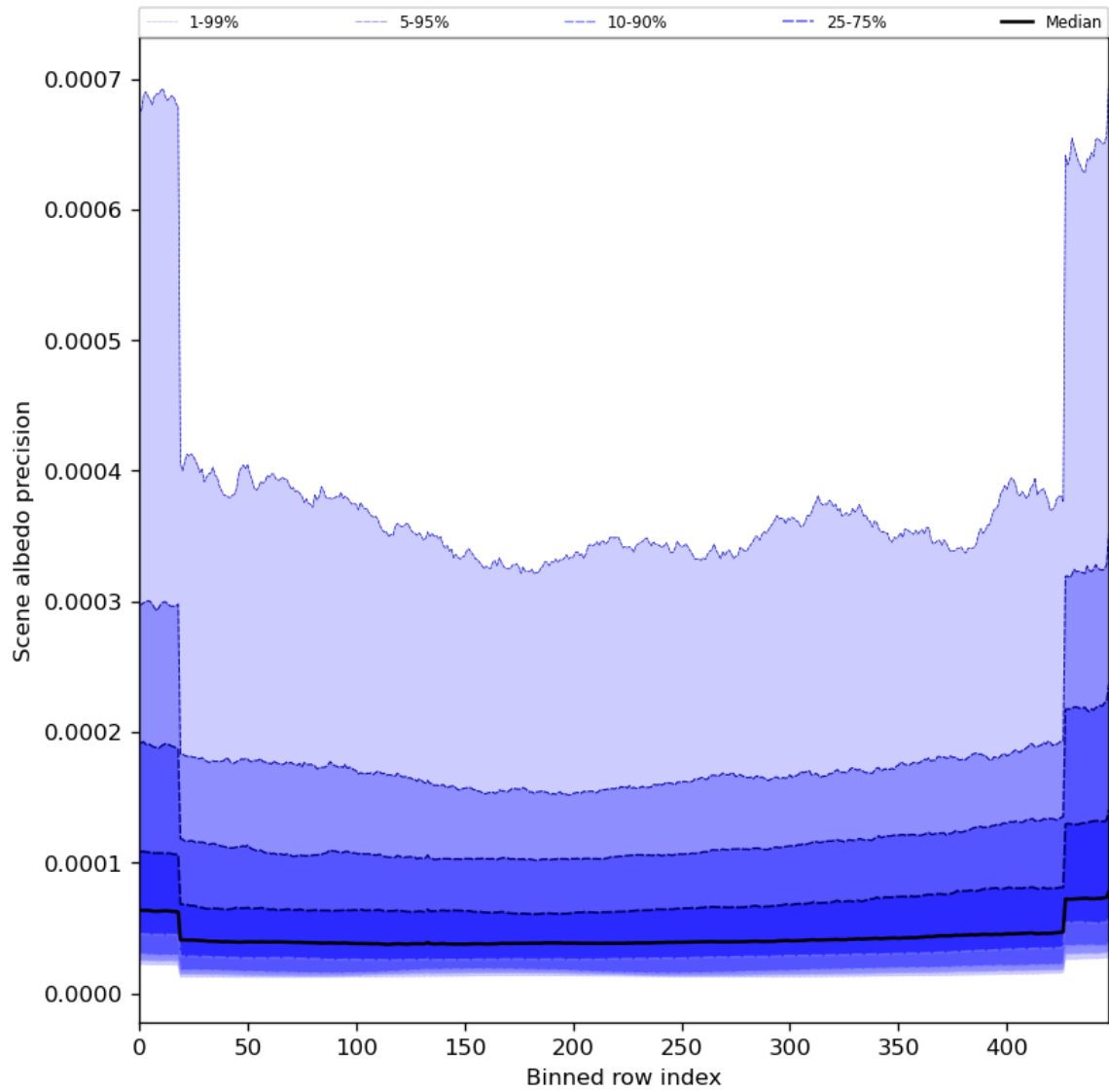
Figure 52: Along track statistics of “Scene albedo precision” for 2024-07-27 to 2024-07-29
