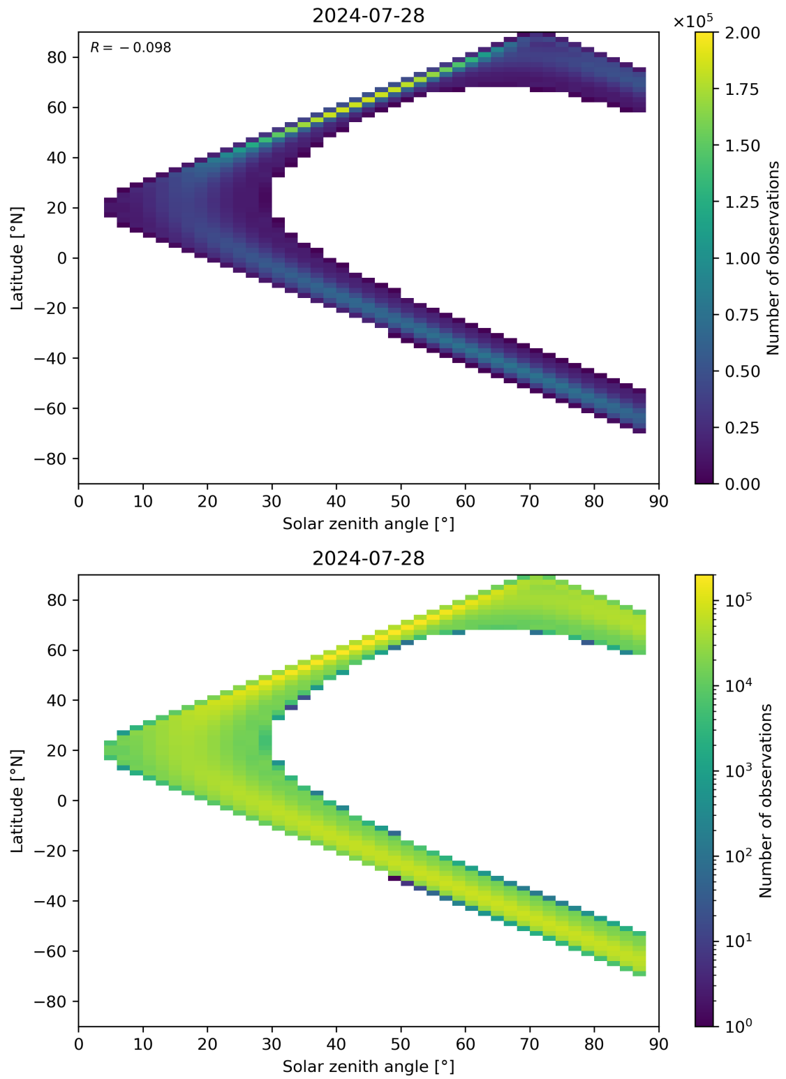
Figure 113: Scatter density plot of “Solar zenith angle” against “Latitude” for 2024-07-27 to 2024-07-29.
