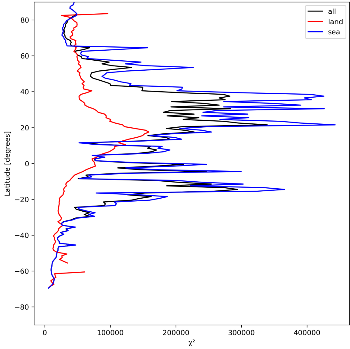
Figure 21: Zonal average of “ \chi^2 ” for 2024-07-27 to 2024-07-29.
