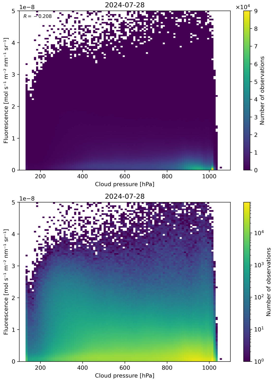
Figure 80: Scatter density plot of “Cloud pressure” against “Fluorescence” for 2024-07-27 to 2024-07-29.
