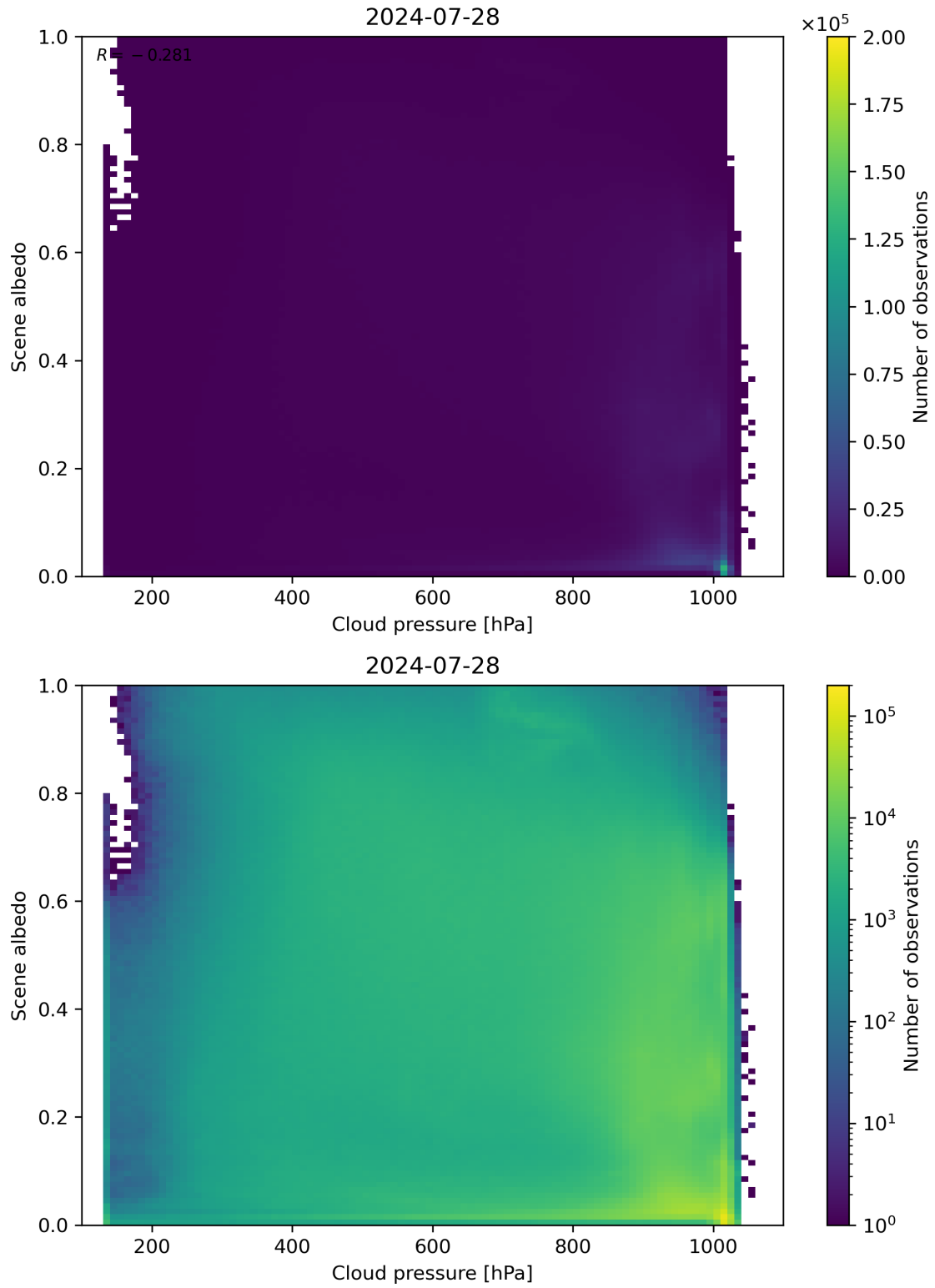
Figure 83: Scatter density plot of “Cloud pressure” against “Scene albedo” for 2024-07-27 to 2024-07-29.
