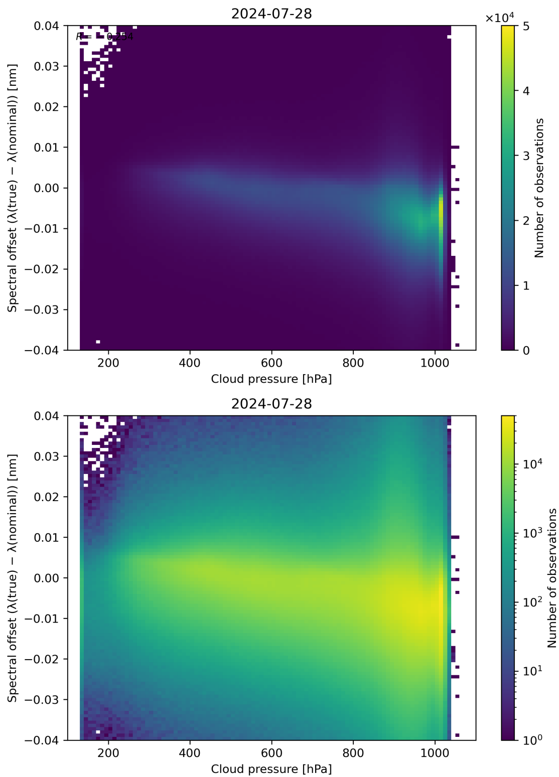
Figure 84: Scatter density plot of “Cloud pressure” against “Spectral offset ( \lambda(\text{true}) - \lambda(\text{nominal}) )” for 2024-07-27 to 2024-07-29.
