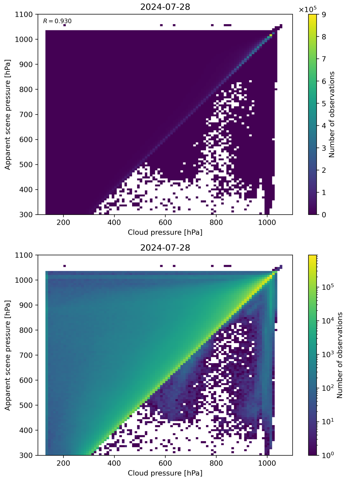
Figure 77: Scatter density plot of “Cloud pressure” against “Apparent scene pressure” for 2024-07-27 to 2024-07-29.
