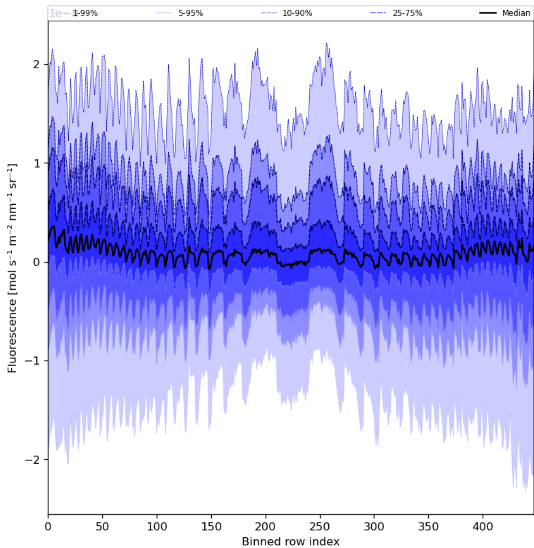
Figure 57: Along track statistics of “Fluorescence” for 2024-07-27 to 2024-07-29
