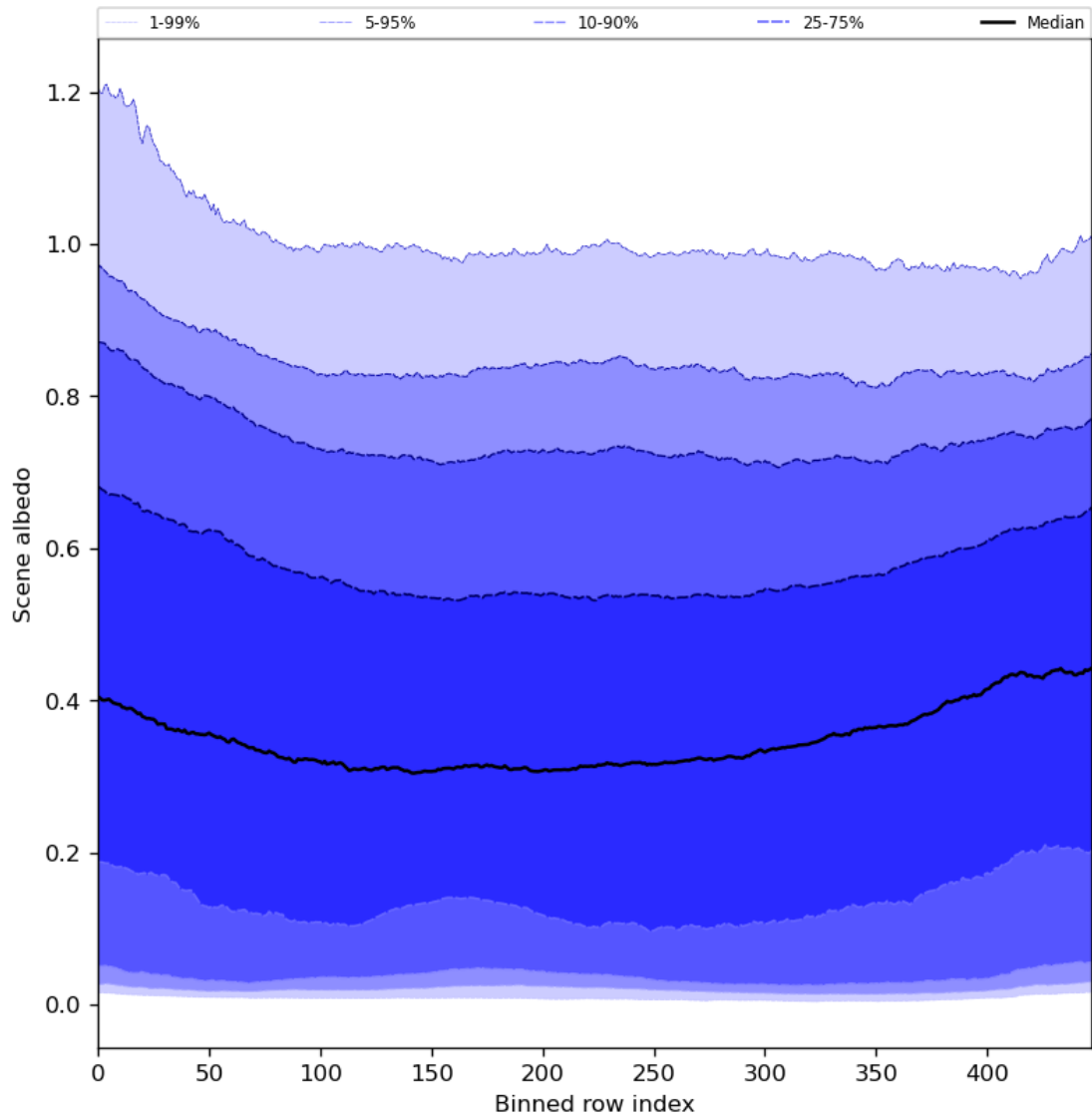
Figure 51: Along track statistics of “Scene albedo” for 2024-07-27 to 2024-07-29
