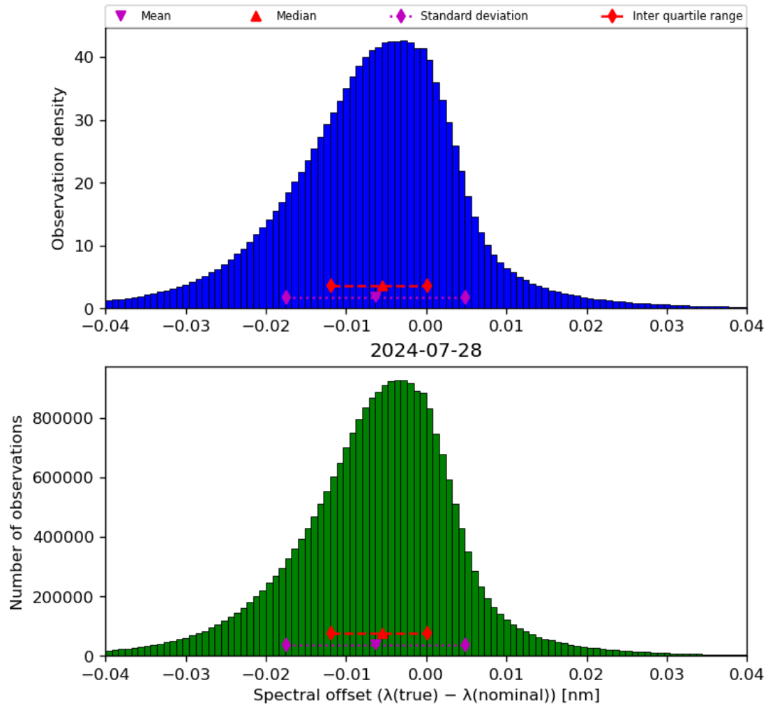
Figure 45: Histogram of “Spectral offset ( \lambda(\text{true}) - \lambda(\text{nominal}) )” for 2024-07-27 to 2024-07-29
