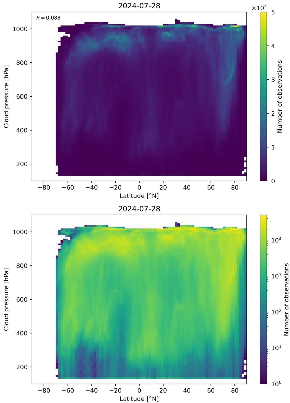
Figure 91: Scatter density plot of “Latitude” against “Cloud pressure” for 2024-07-27 to 2024-07-29.
