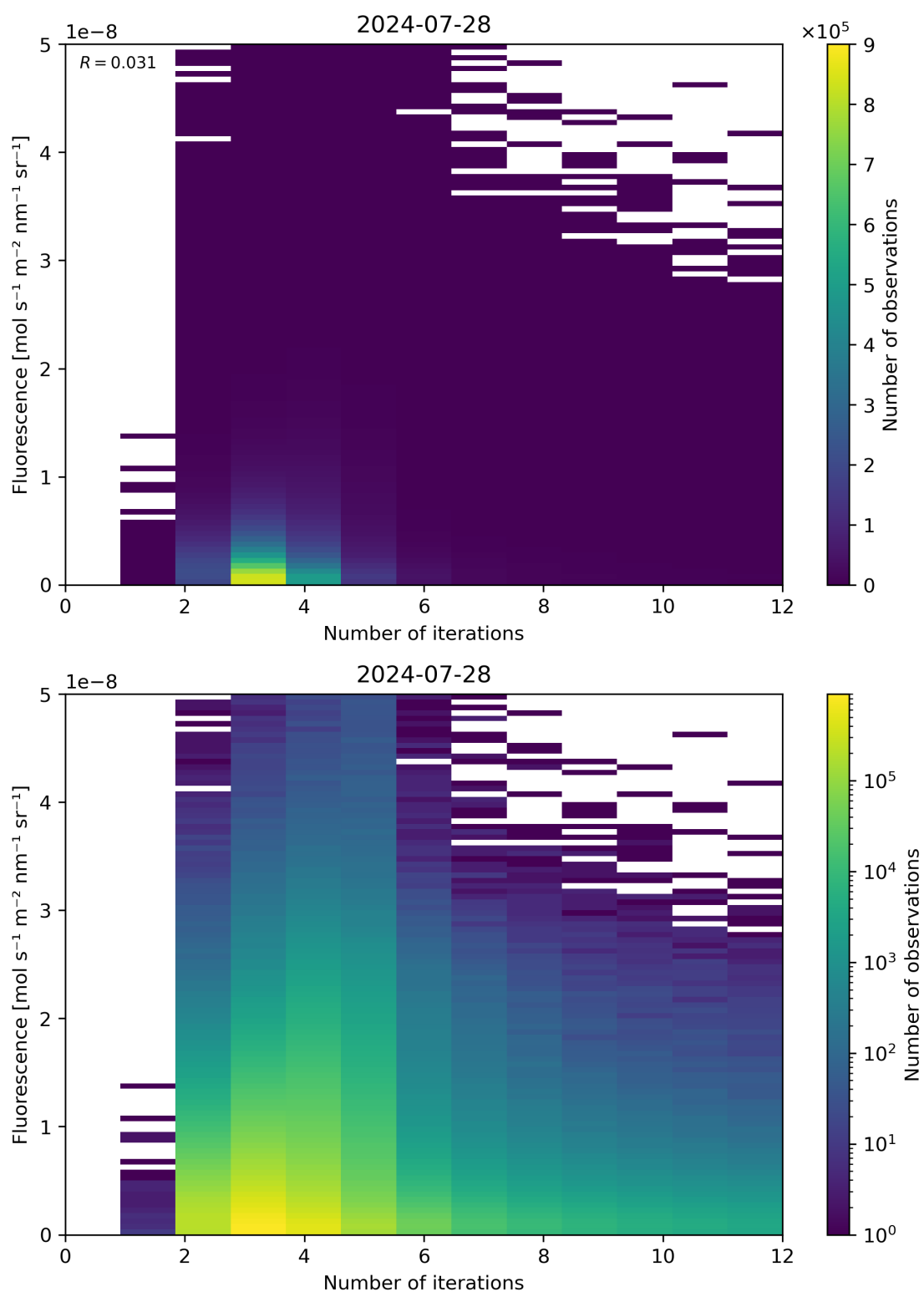
Figure 98: Scatter density plot of “Number of iterations” against “Fluorescence” for 2024-07-27 to 2024-07-29.
