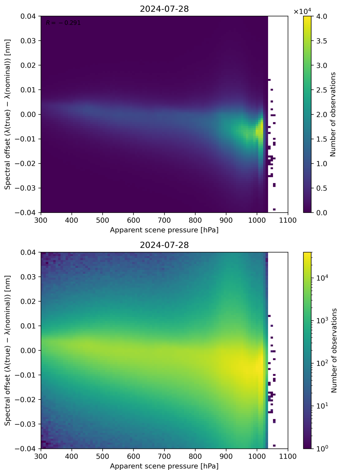
Figure 67: Scatter density plot of “Apparent scene pressure” against “Spectral offset ( \lambda(\text{true}) - \lambda(\text{nominal}) )” for 2024-07-27 to 2024-07-29.
