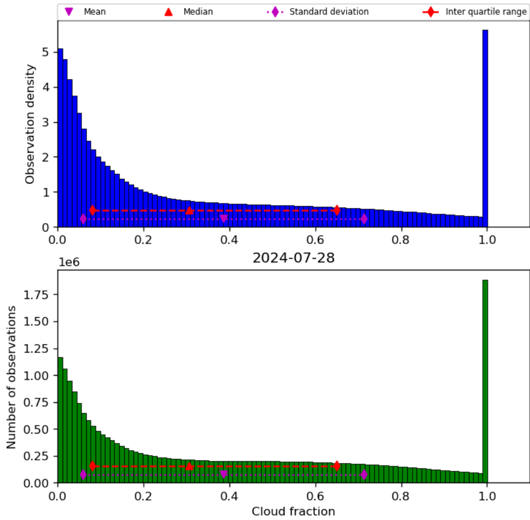
Figure 32: Histogram of “Cloud fraction” for 2024-07-27 to 2024-07-29
