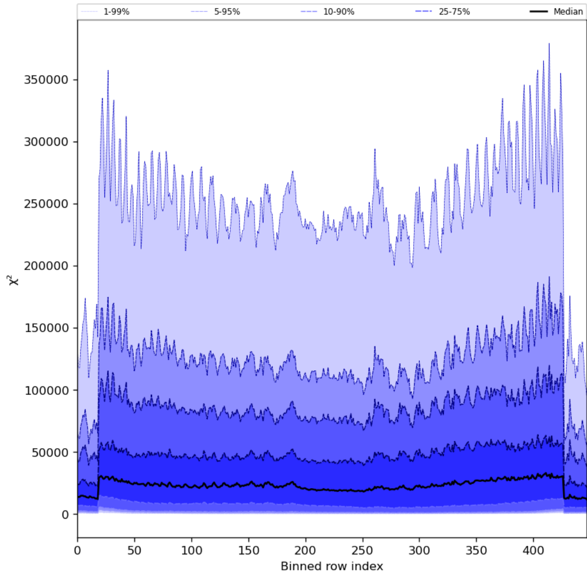
Figure 55: Along track statistics of “ \chi^2 ” for 2024-07-27 to 2024-07-29
