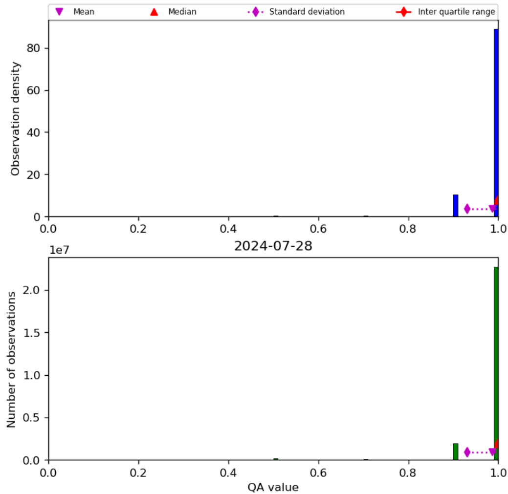
Figure 29: Histogram of “QA value” for 2024-07-27 to 2024-07-29
