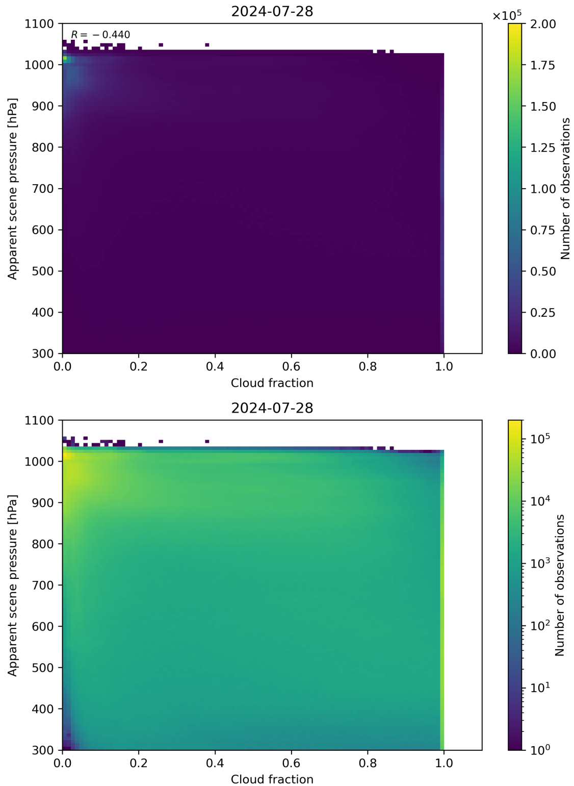
Figure 70: Scatter density plot of “Cloud fraction” against “Apparent scene pressure” for 2024-07-27 to 2024-07-29.
