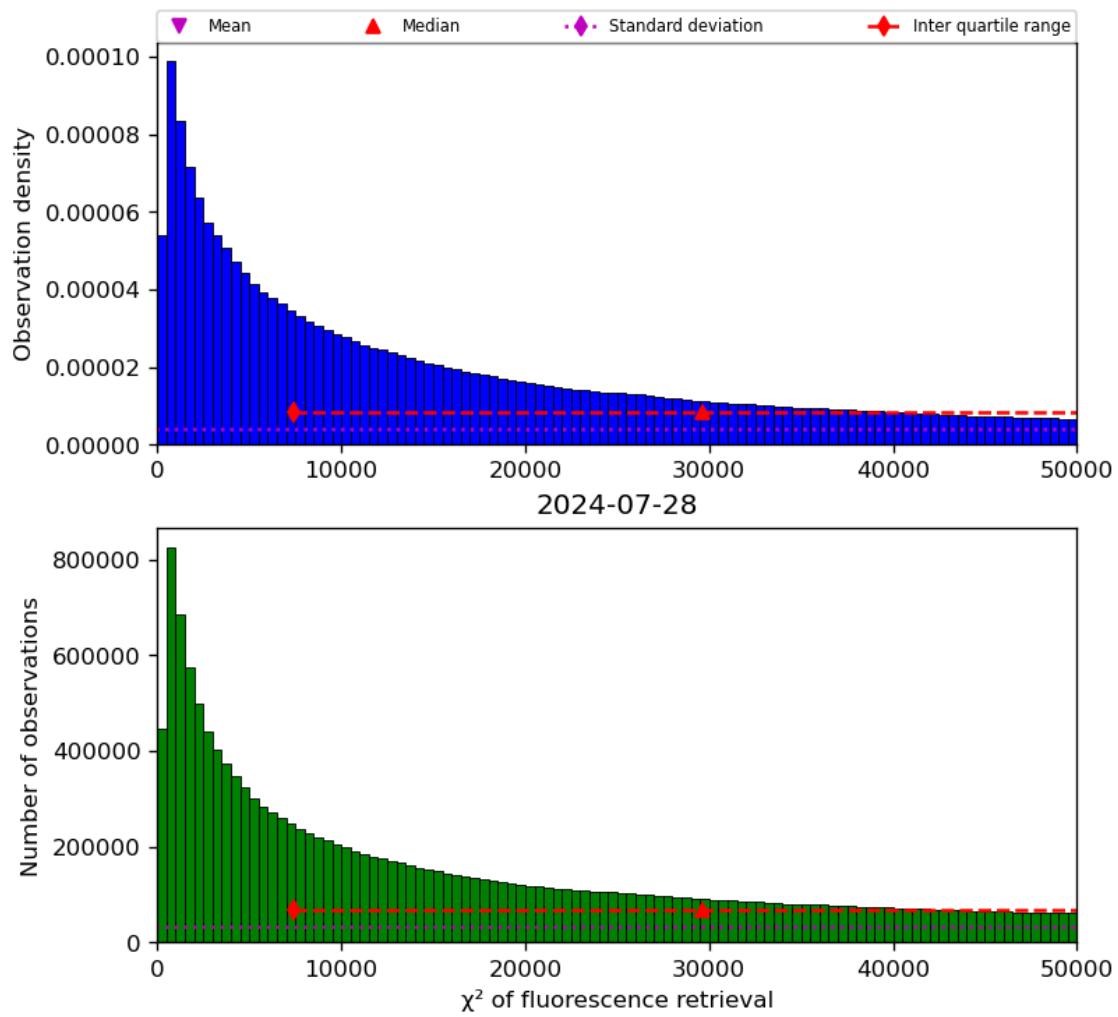
Figure 42: Histogram of “ \chi^2 of fluorescence retrieval” for 2024-07-27 to 2024-07-29
