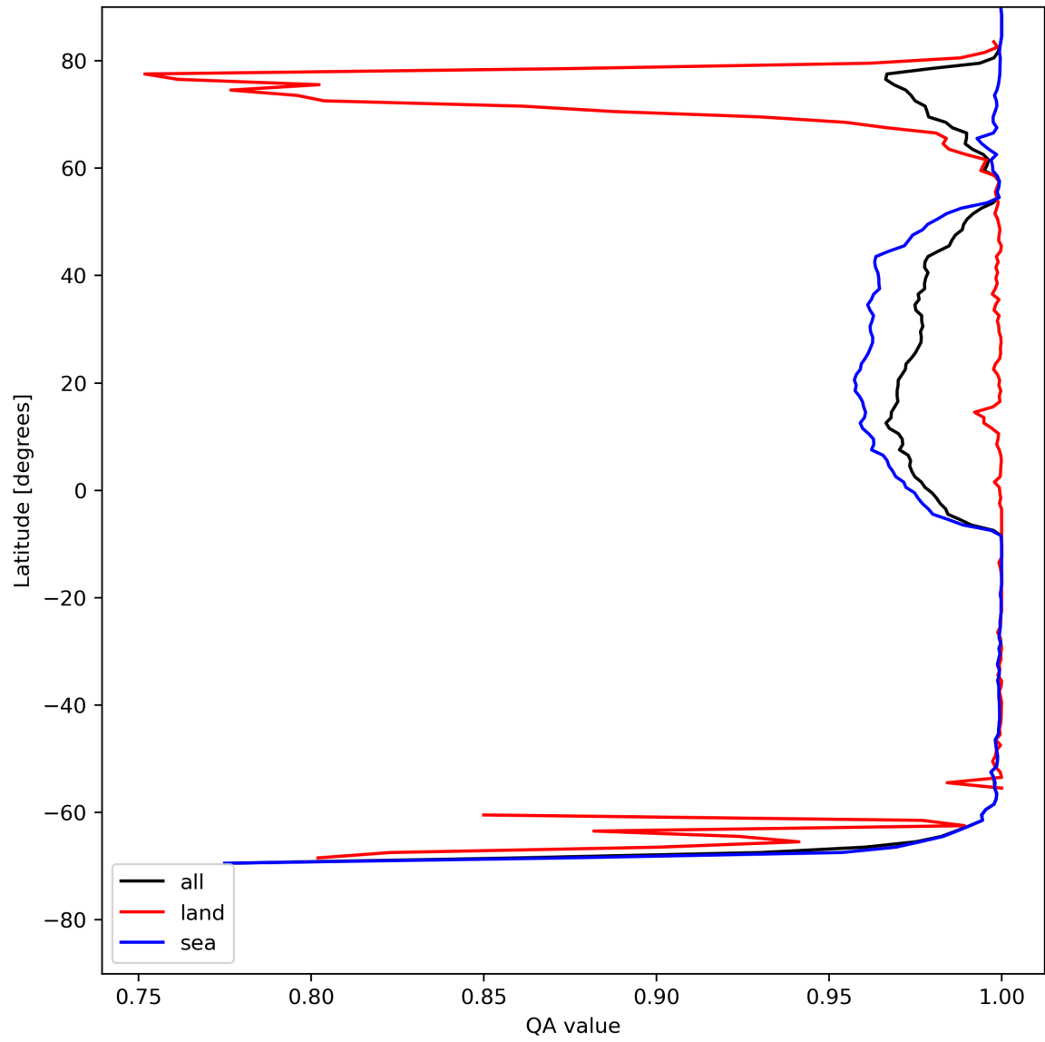
Figure 12: Zonal average of “QA value” for 2024-07-27 to 2024-07-29.
