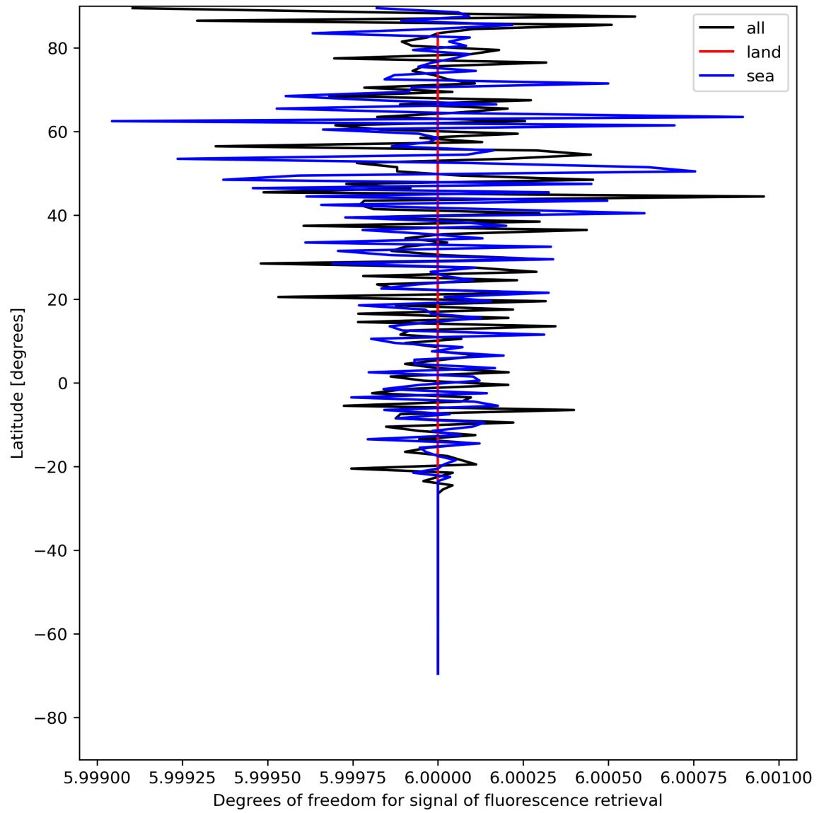
Figure 26: Zonal average of “Degrees of freedom for signal of fluorescence retrieval” for 2024-07-27 to 2024-07-29.
