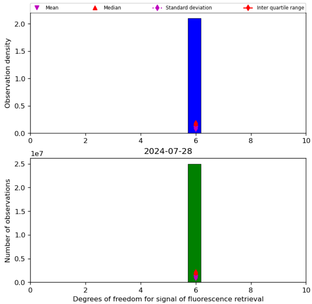
Figure 43: Histogram of “Degrees of freedom for signal of fluorescence retrieval” for 2024-07-27 to 2024-07-29
