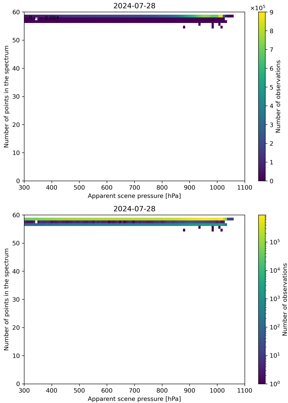
Figure 66: Scatter density plot of “Apparent scene pressure” against “Number of points in the spectrum” for 2024-07-27 to 2024-07-29.
