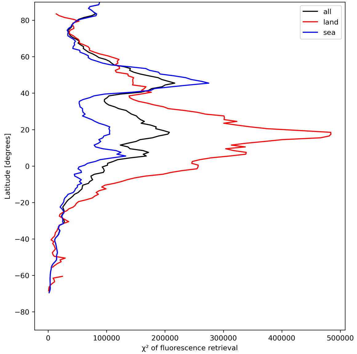
Figure 25: Zonal average of “ \chi^2 of fluorescence retrieval” for 2024-07-27 to 2024-07-29.
