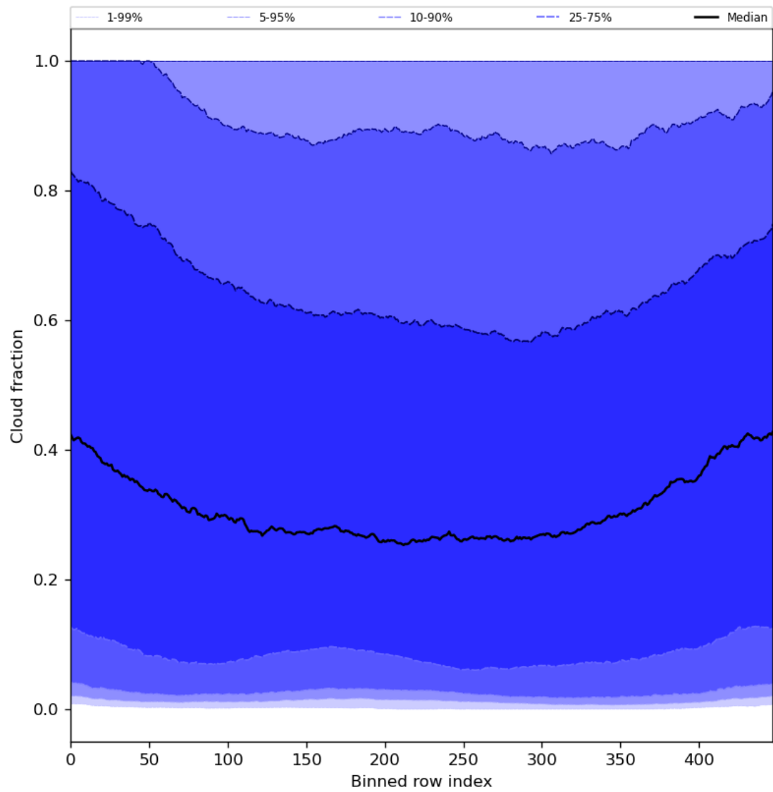
Figure 49: Along track statistics of “Cloud fraction” for 2024-07-27 to 2024-07-29
