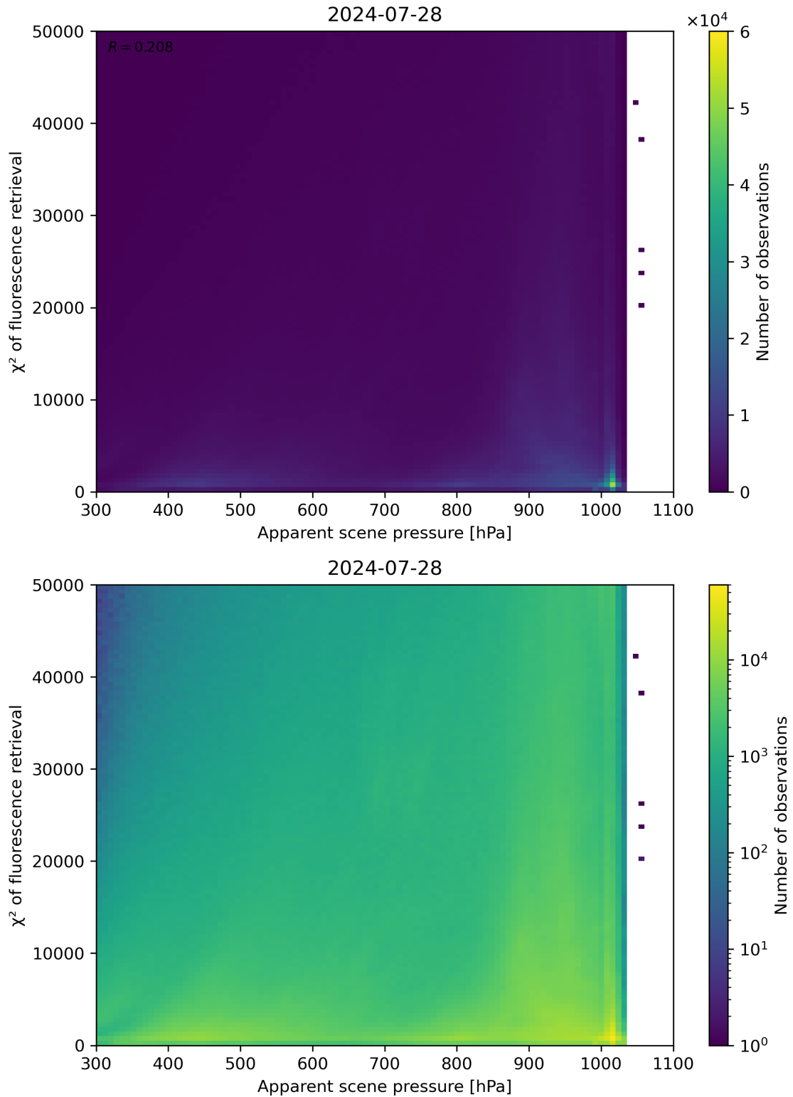
Figure 63: Scatter density plot of “Apparent scene pressure” against “ \chi^2 of fluorescence retrieval” for 2024-07-27 to 2024-07-29.
