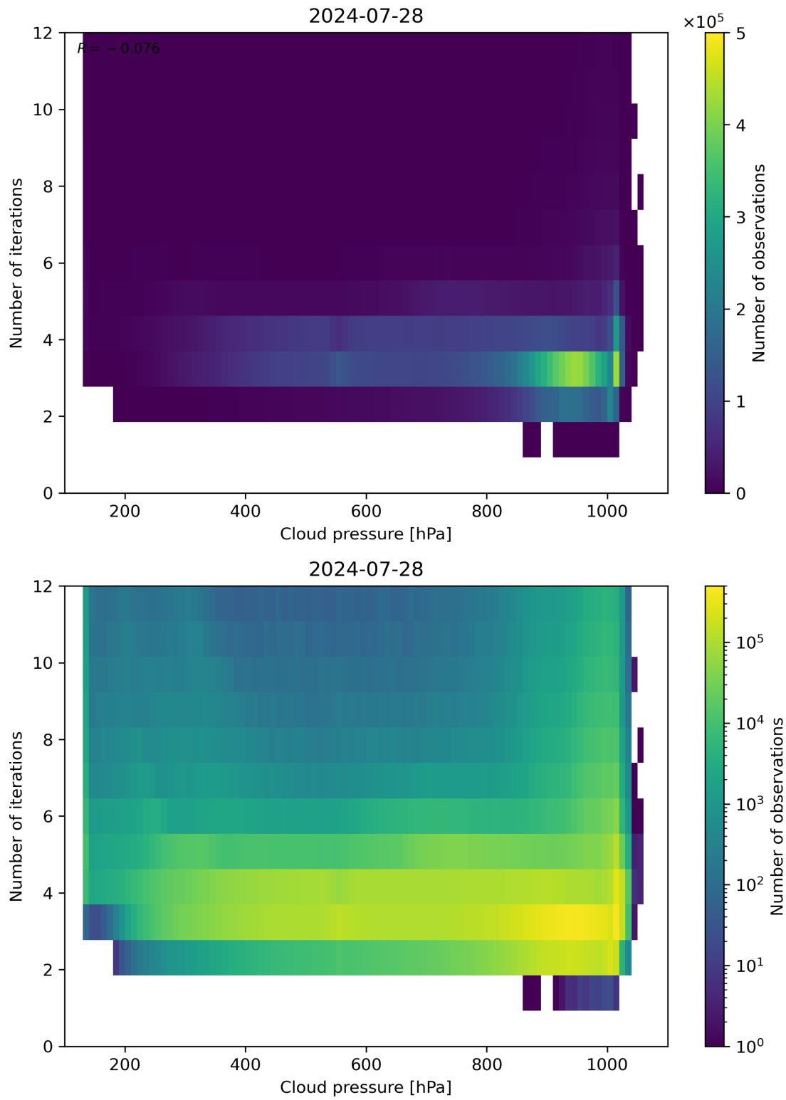
Figure 81: Scatter density plot of “Cloud pressure” against “Number of iterations” for 2024-07-27 to 2024-07-29.
