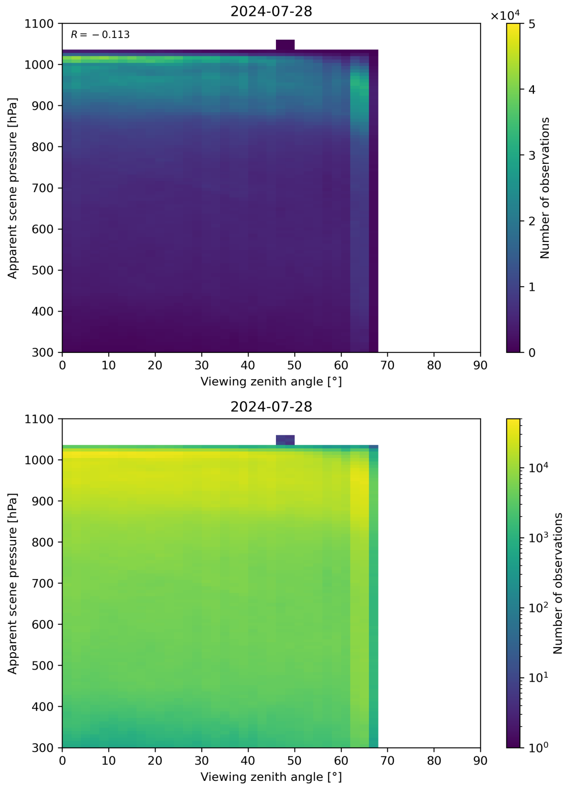
Figure 118: Scatter density plot of “Viewing zenith angle” against “Apparent scene pressure” for 2024-07-27 to 2024-07-29.
