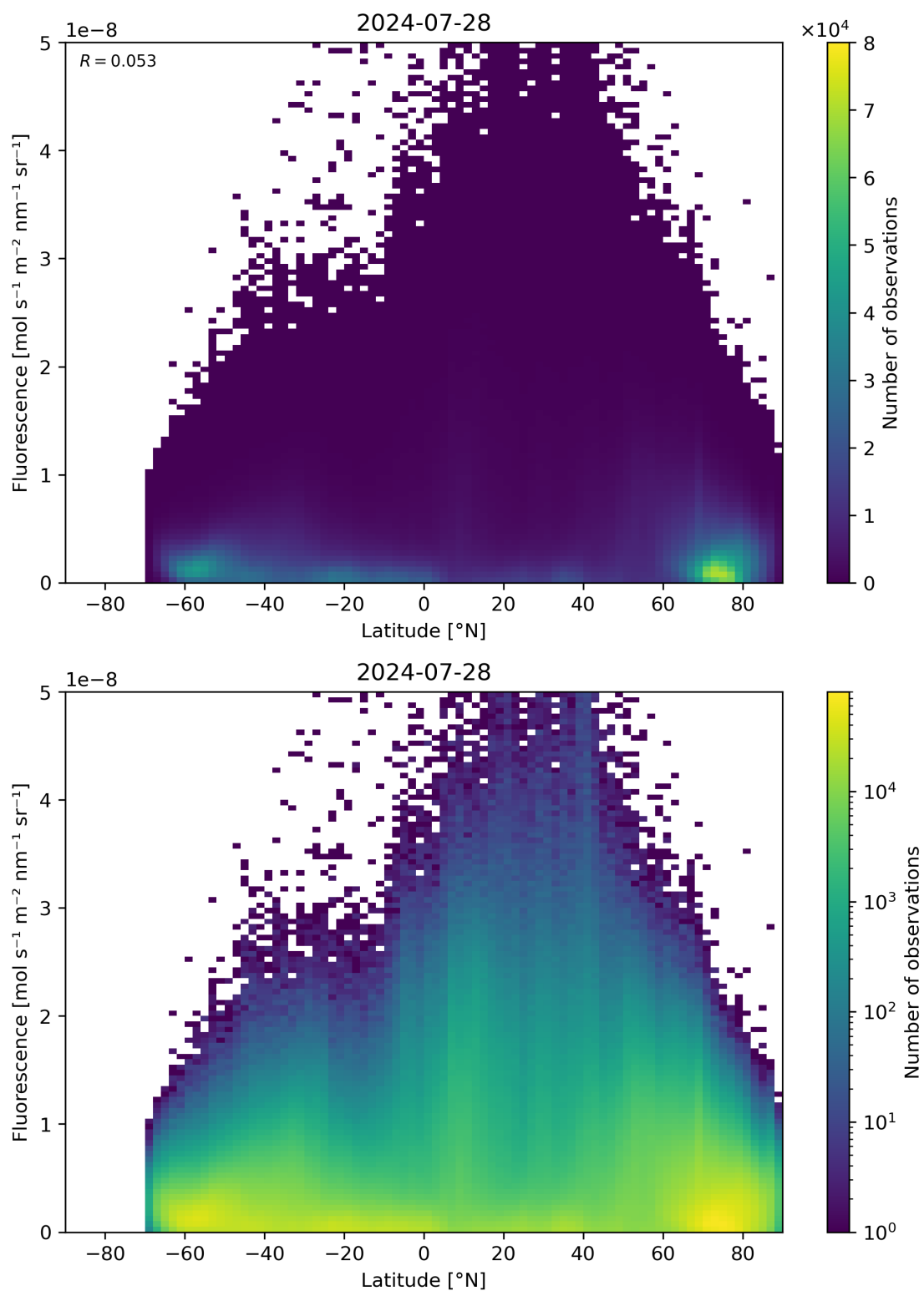
Figure 92: Scatter density plot of “Latitude” against “Fluorescence” for 2024-07-27 to 2024-07-29.
