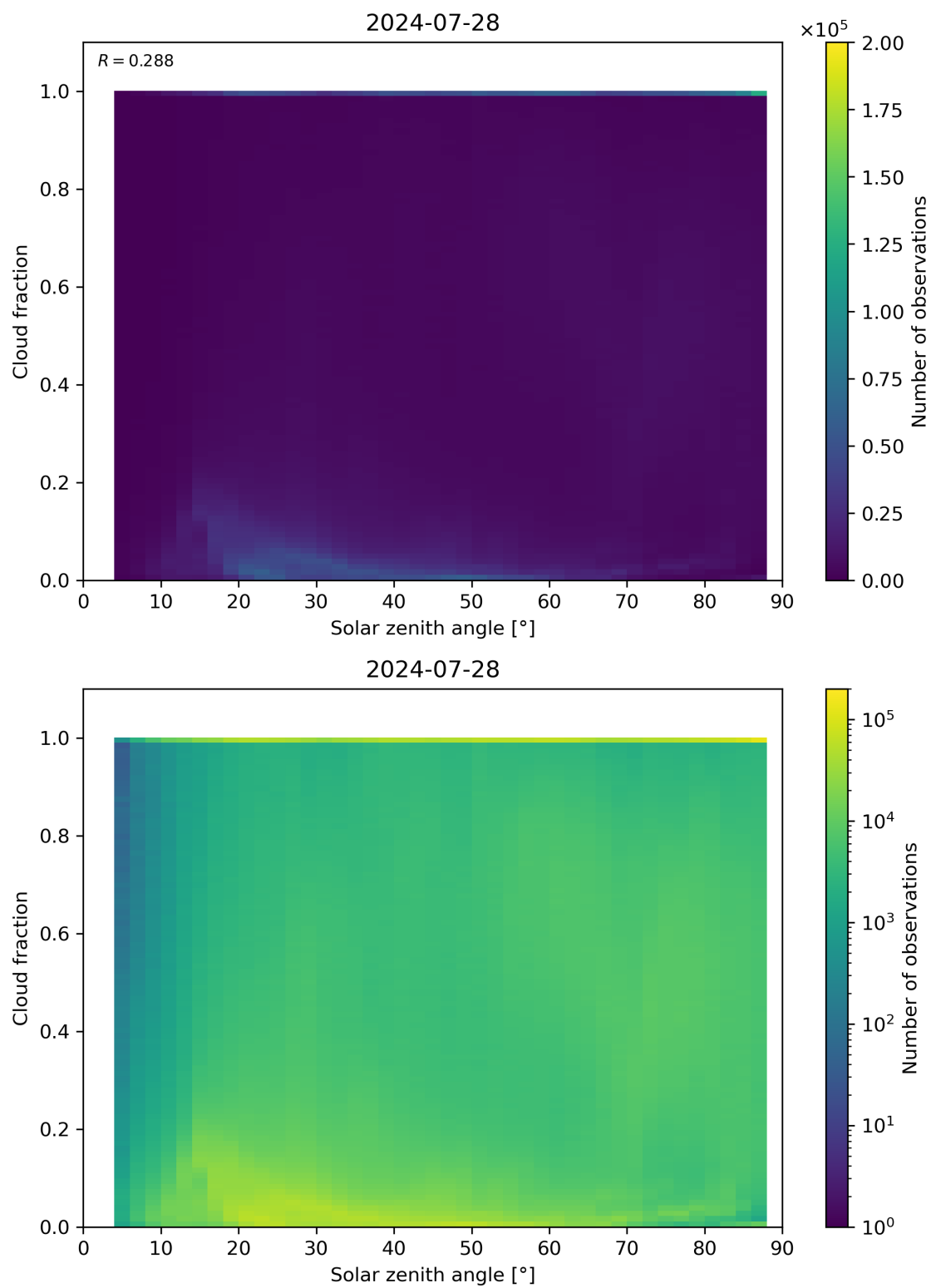
Figure 110: Scatter density plot of “Solar zenith angle” against “Cloud fraction” for 2024-07-27 to 2024-07-29.
