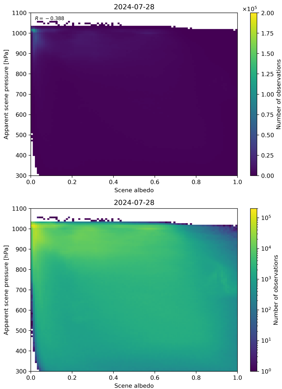
Figure 102: Scatter density plot of “Scene albedo” against “Apparent scene pressure” for 2024-07-27 to 2024-07-29.
