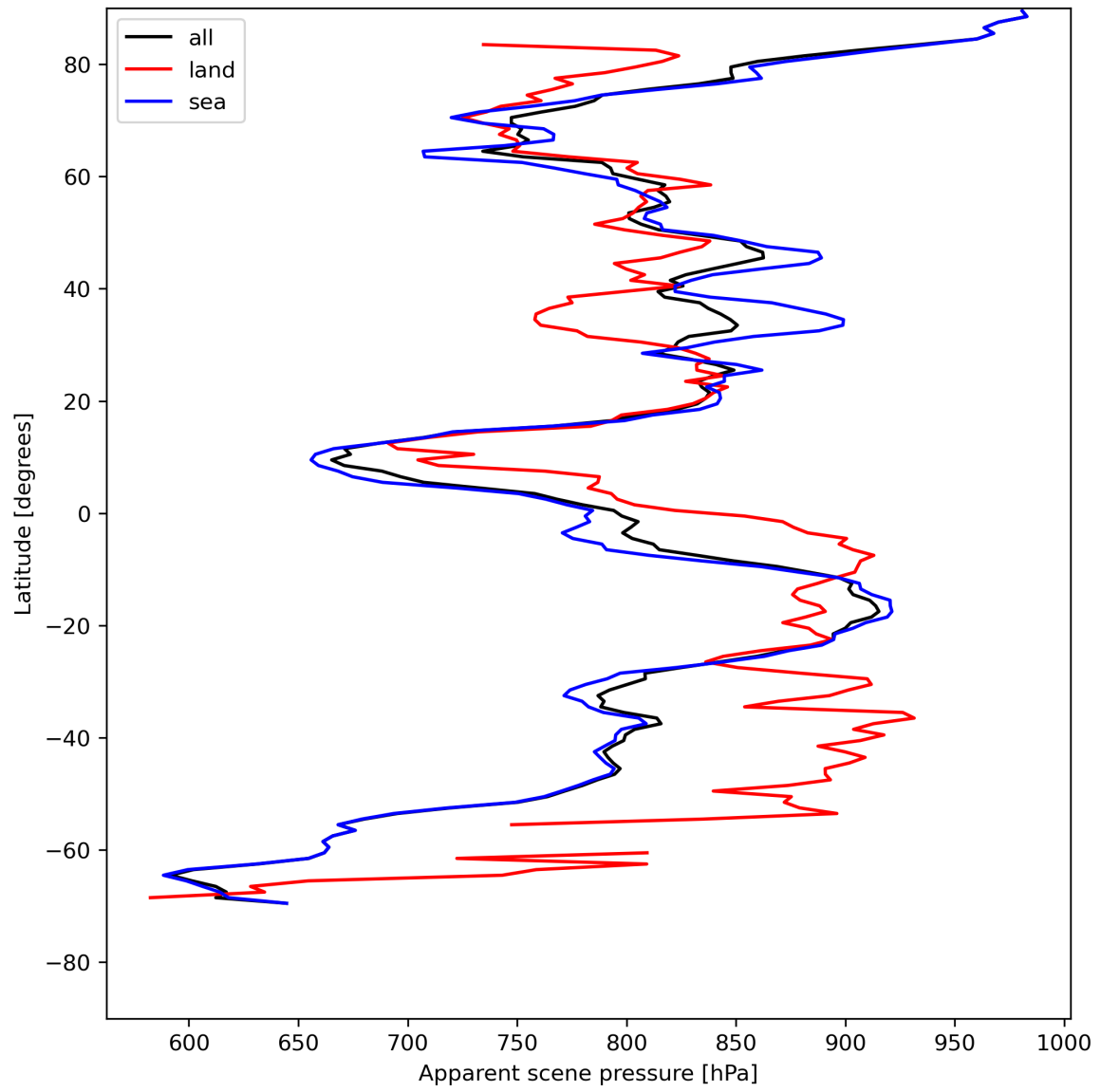
Figure 19: Zonal average of “Apparent scene pressure” for 2024-07-27 to 2024-07-29.
