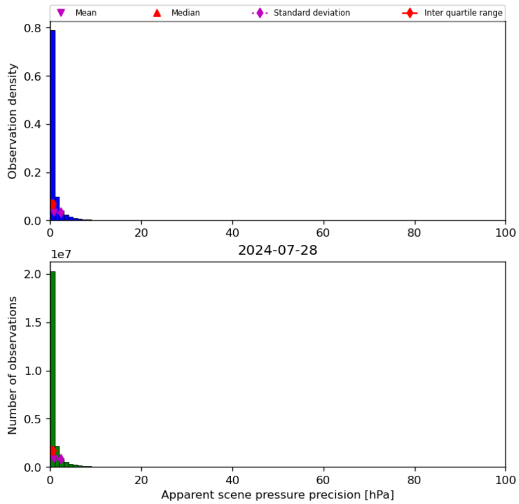
Figure 37: Histogram of “Apparent scene pressure precision” for 2024-07-27 to 2024-07-29
