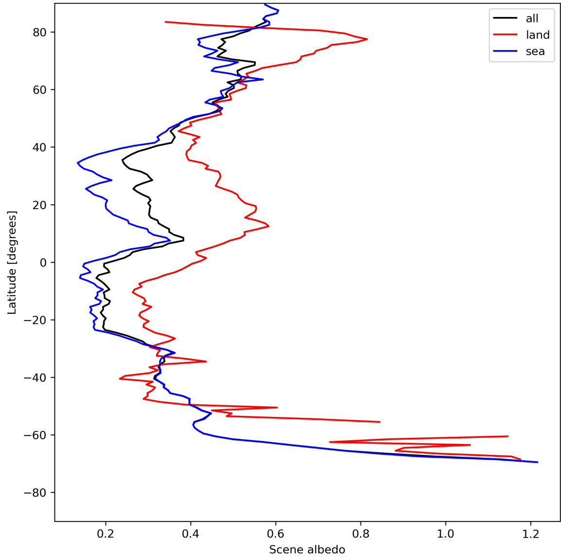
Figure 17: Zonal average of “Scene albedo” for 2024-07-27 to 2024-07-29.
