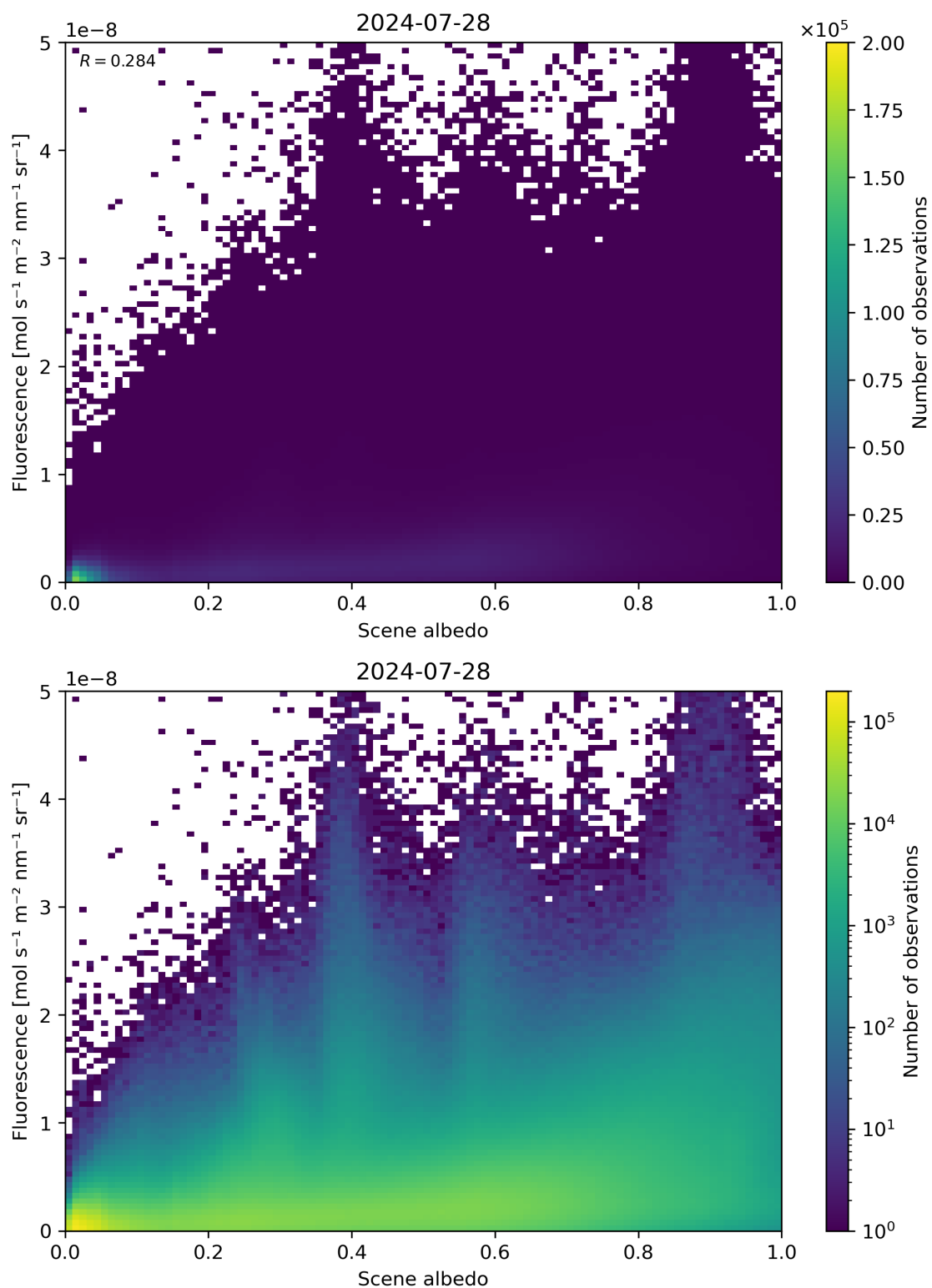
Figure 104: Scatter density plot of “Scene albedo” against “Fluorescence” for 2024-07-27 to 2024-07-29.
