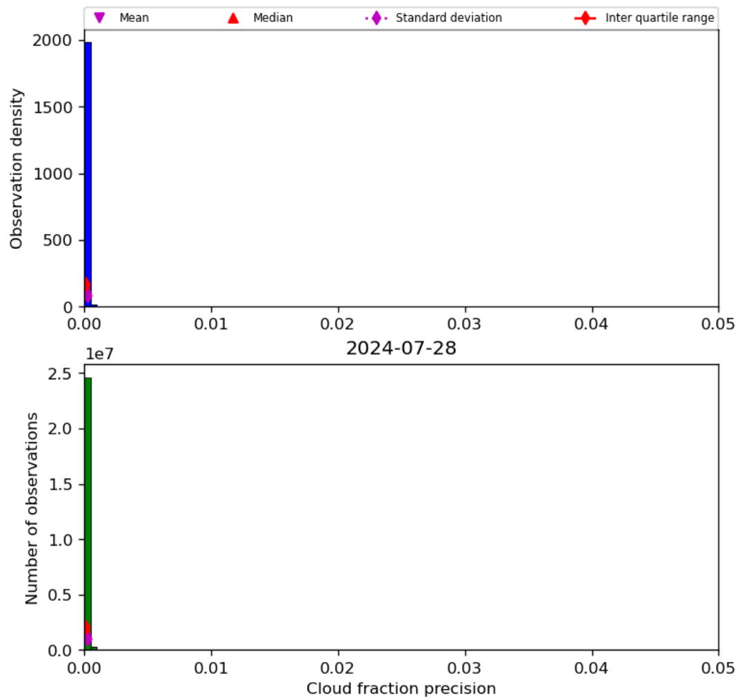
Figure 33: Histogram of “Cloud fraction precision” for 2024-07-27 to 2024-07-29
