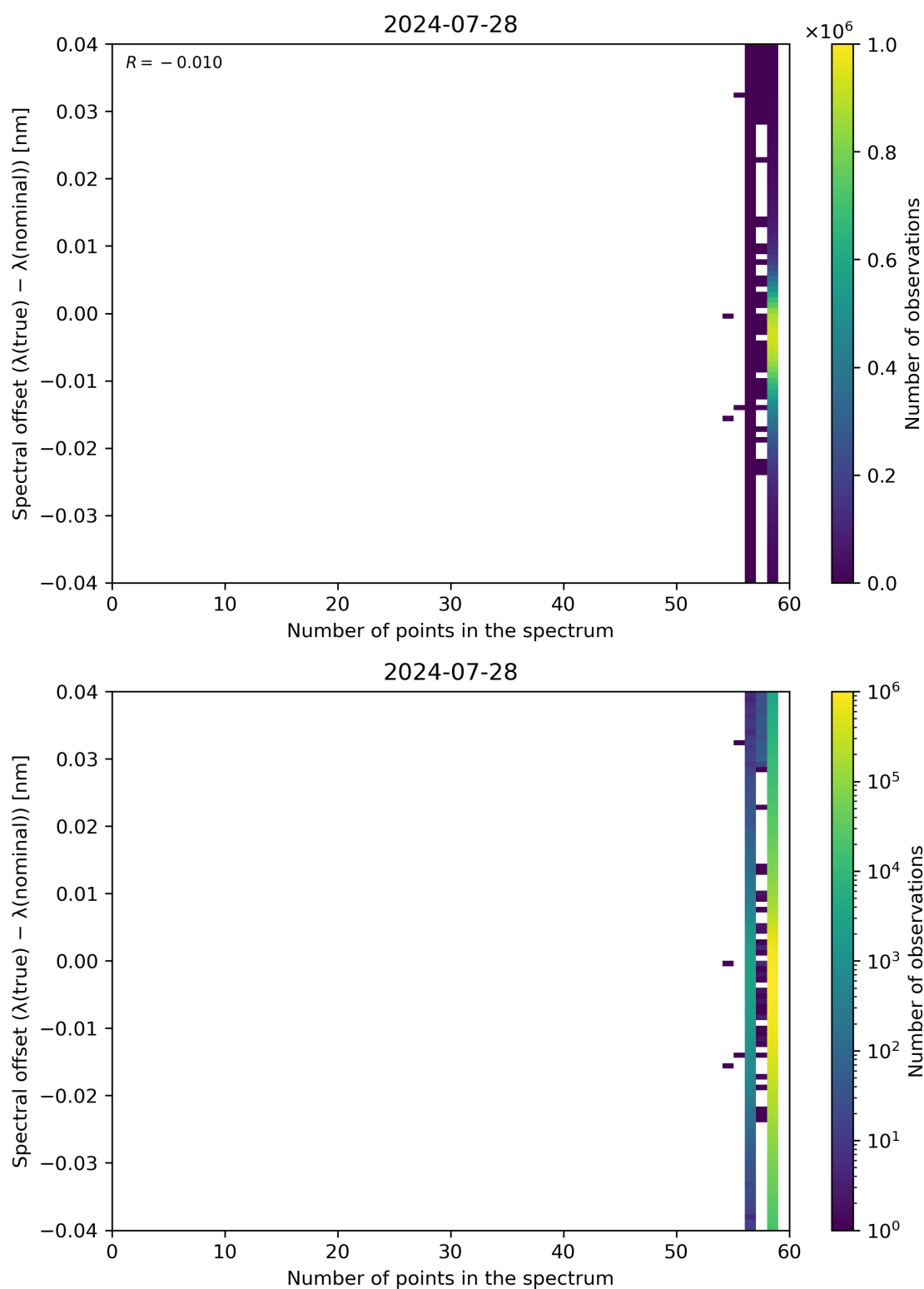
Figure 101: Scatter density plot of “Number of points in the spectrum” against “Spectral offset ( \lambda(\text{true}) - \lambda(\text{nominal}) )” for 2024-07-27 to 2024-07-29.
