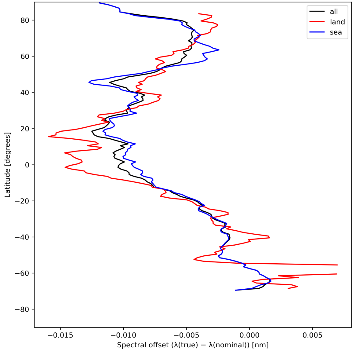
Figure 28: Zonal average of “Spectral offset ( \lambda(\text{true}) - \lambda(\text{nominal}) )” for 2024-07-27 to 2024-07-29.
