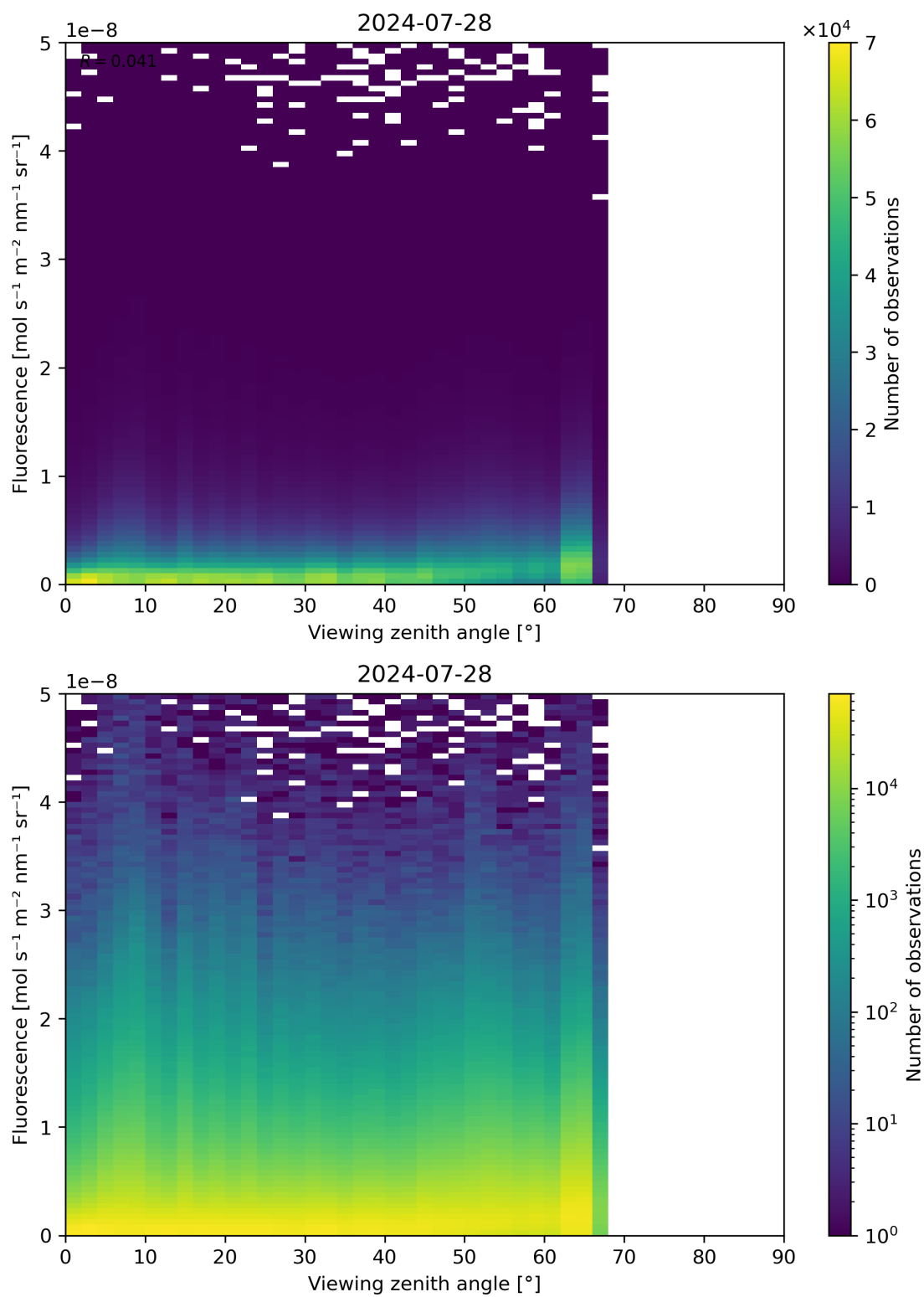
Figure 122: Scatter density plot of “Viewing zenith angle” against “Fluorescence” for 2024-07-27 to 2024-07-29.
