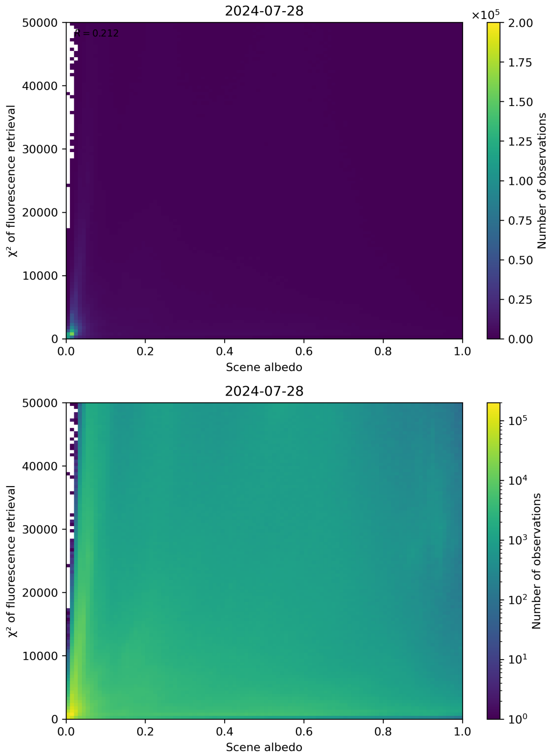
Figure 103: Scatter density plot of “Scene albedo” against “ \chi^2 of fluorescence retrieval” for 2024-07-27 to 2024-07-29.
