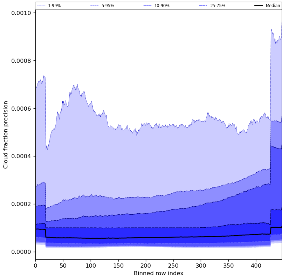
Figure 50: Along track statistics of “Cloud fraction precision” for 2024-07-27 to 2024-07-29
