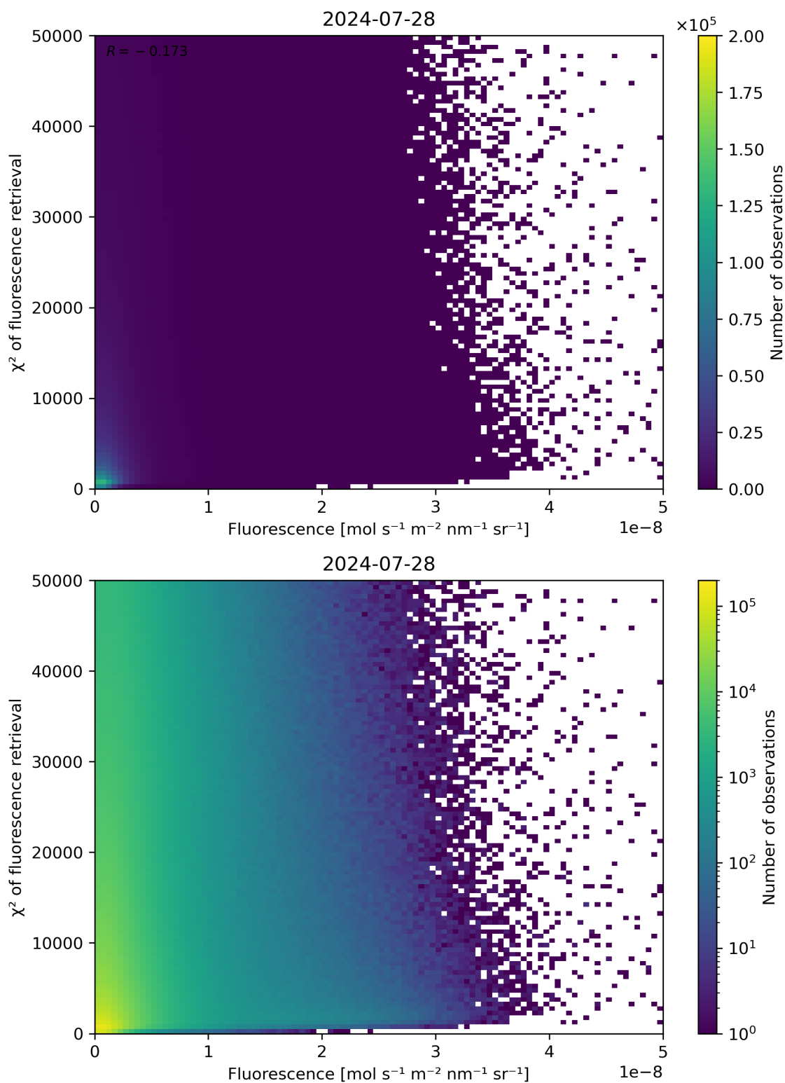
Figure 85: Scatter density plot of “Fluorescence” against “ \chi^2 of fluorescence retrieval” for 2024-07-27 to 2024-07-29.
