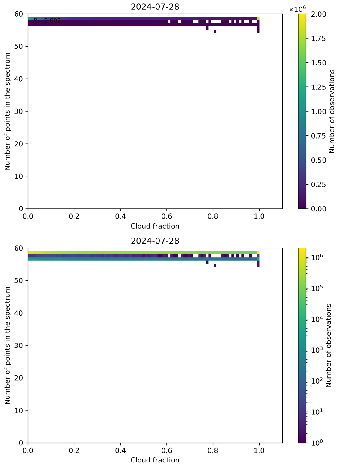
Figure 74: Scatter density plot of “Cloud fraction” against “Number of points in the spectrum” for 2024-07-27 to 2024-07-29.
