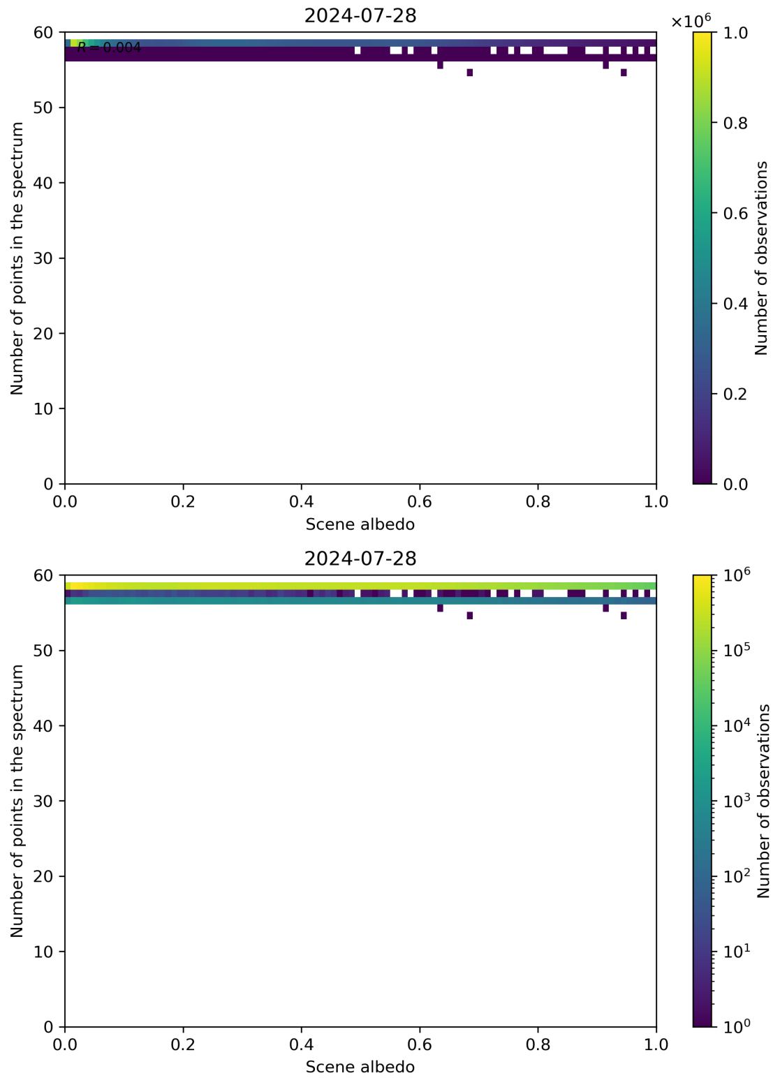
Figure 106: Scatter density plot of “Scene albedo” against “Number of points in the spectrum” for 2024-07-27 to 2024-07-29.
