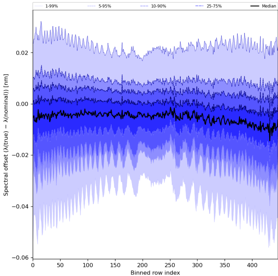
Figure 62: Along track statistics of “Spectral offset ( \lambda(\text{true}) - \lambda(\text{nominal}) )” for 2024-07-27 to 2024-07-29
