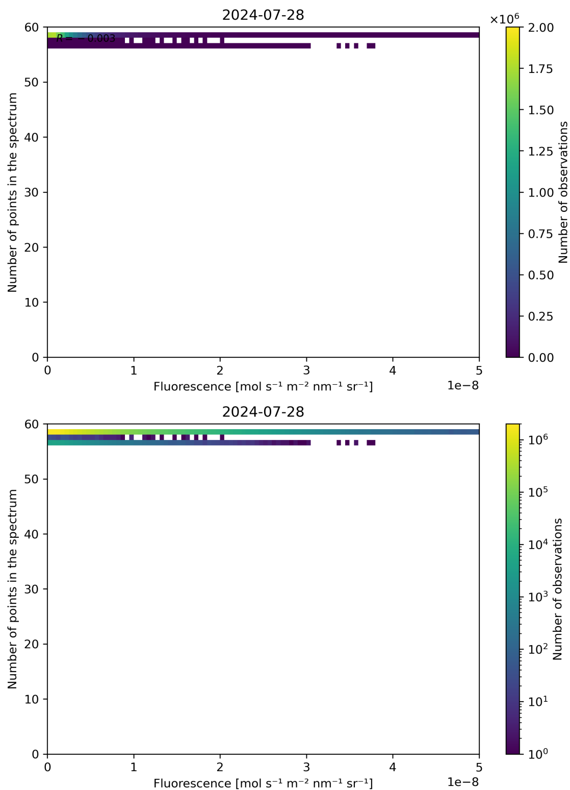
Figure 86: Scatter density plot of “Fluorescence” against “Number of points in the spectrum” for 2024-07-27 to 2024-07-29.
