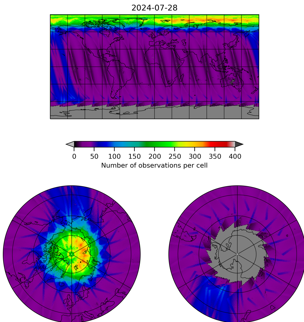
Figure 11: Map of the number of observations for 2024-07-27 to 2024-07-29
