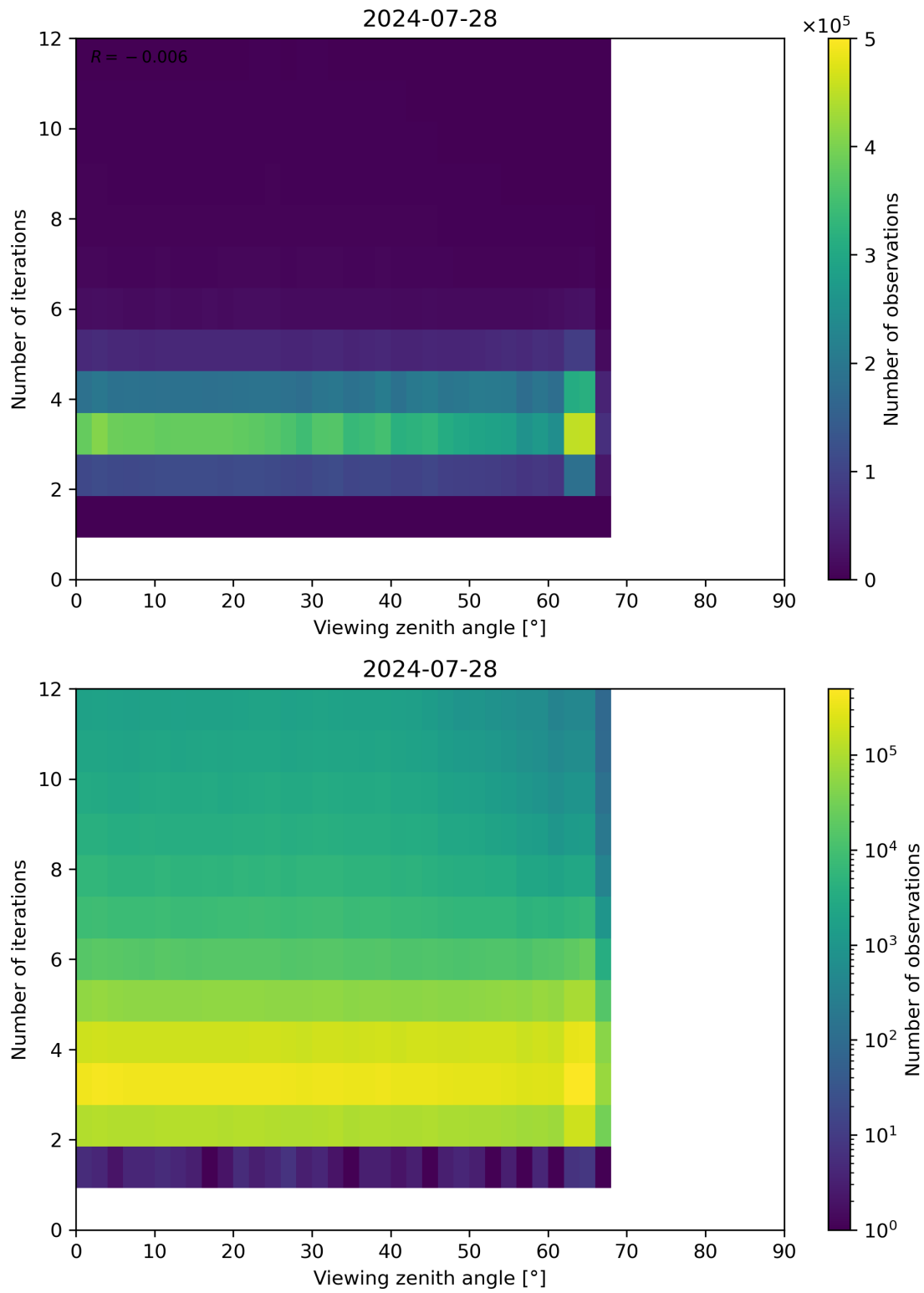
Figure 124: Scatter density plot of “Viewing zenith angle” against “Number of iterations” for 2024-07-27 to 2024-07-29.
