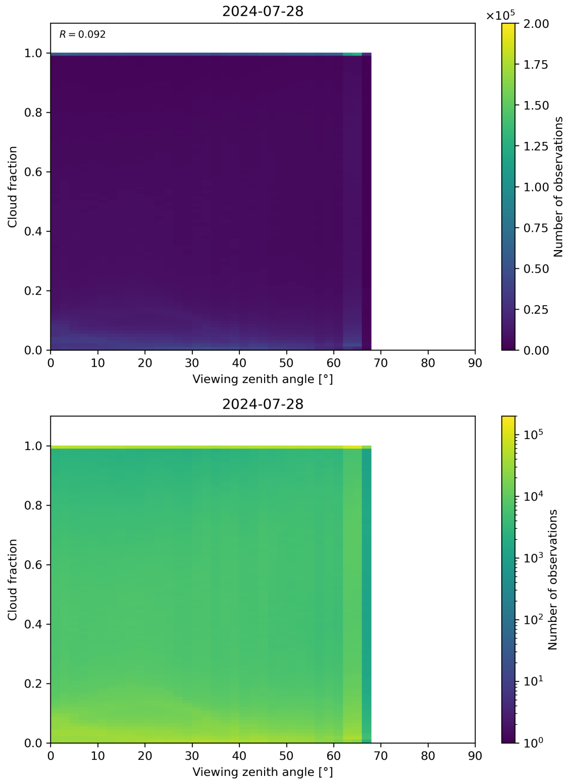
Figure 120: Scatter density plot of “Viewing zenith angle” against “Cloud fraction” for 2024-07-27 to 2024-07-29.
