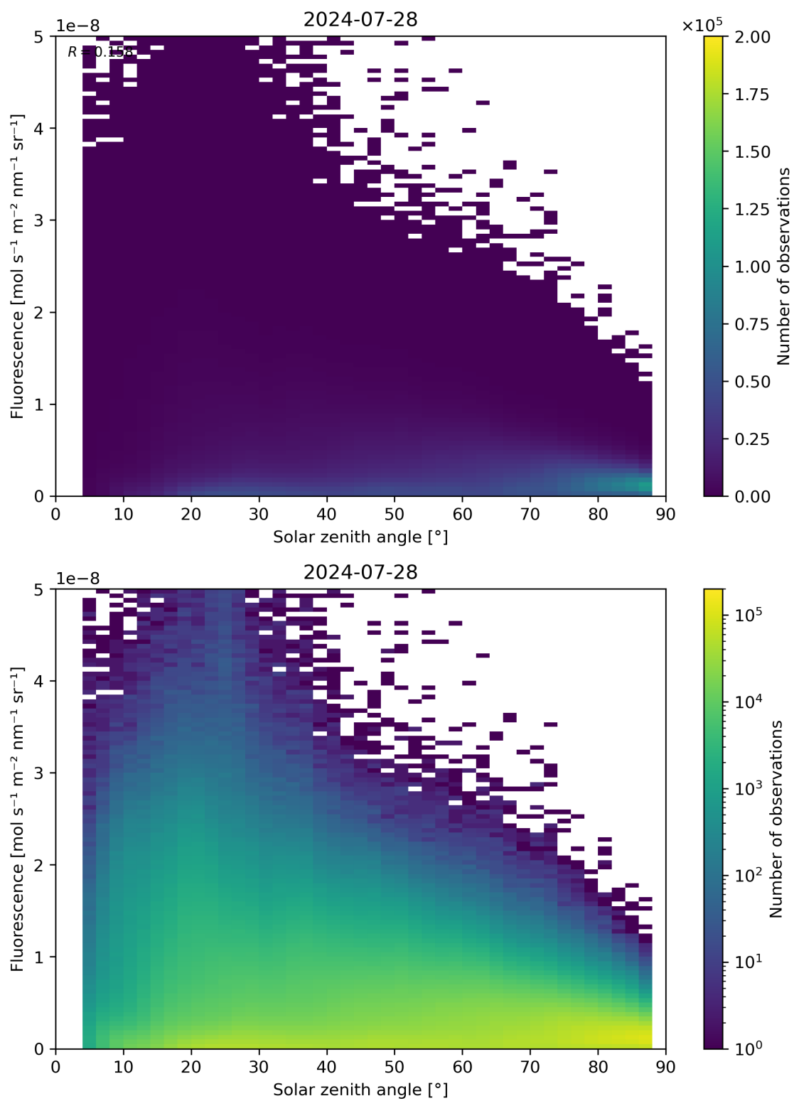
Figure 112: Scatter density plot of “Solar zenith angle” against “Fluorescence” for 2024-07-27 to 2024-07-29.
