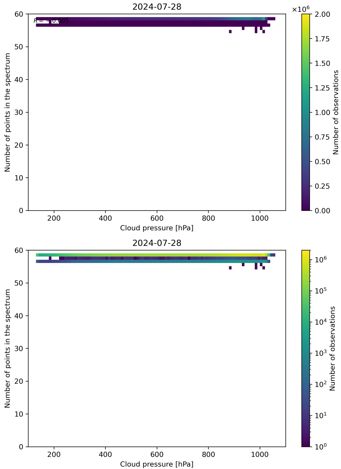
Figure 82: Scatter density plot of “Cloud pressure” against “Number of points in the spectrum” for 2024-07-27 to 2024-07-29.
