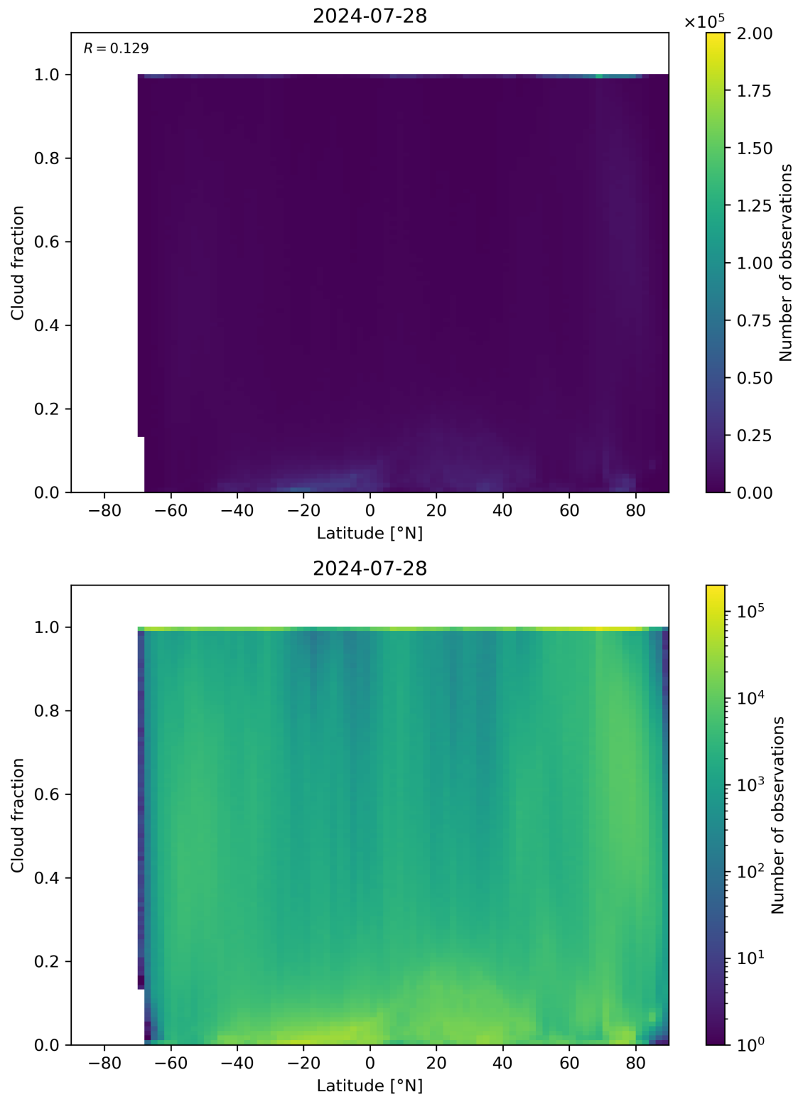
Figure 90: Scatter density plot of “Latitude” against “Cloud fraction” for 2024-07-27 to 2024-07-29.
