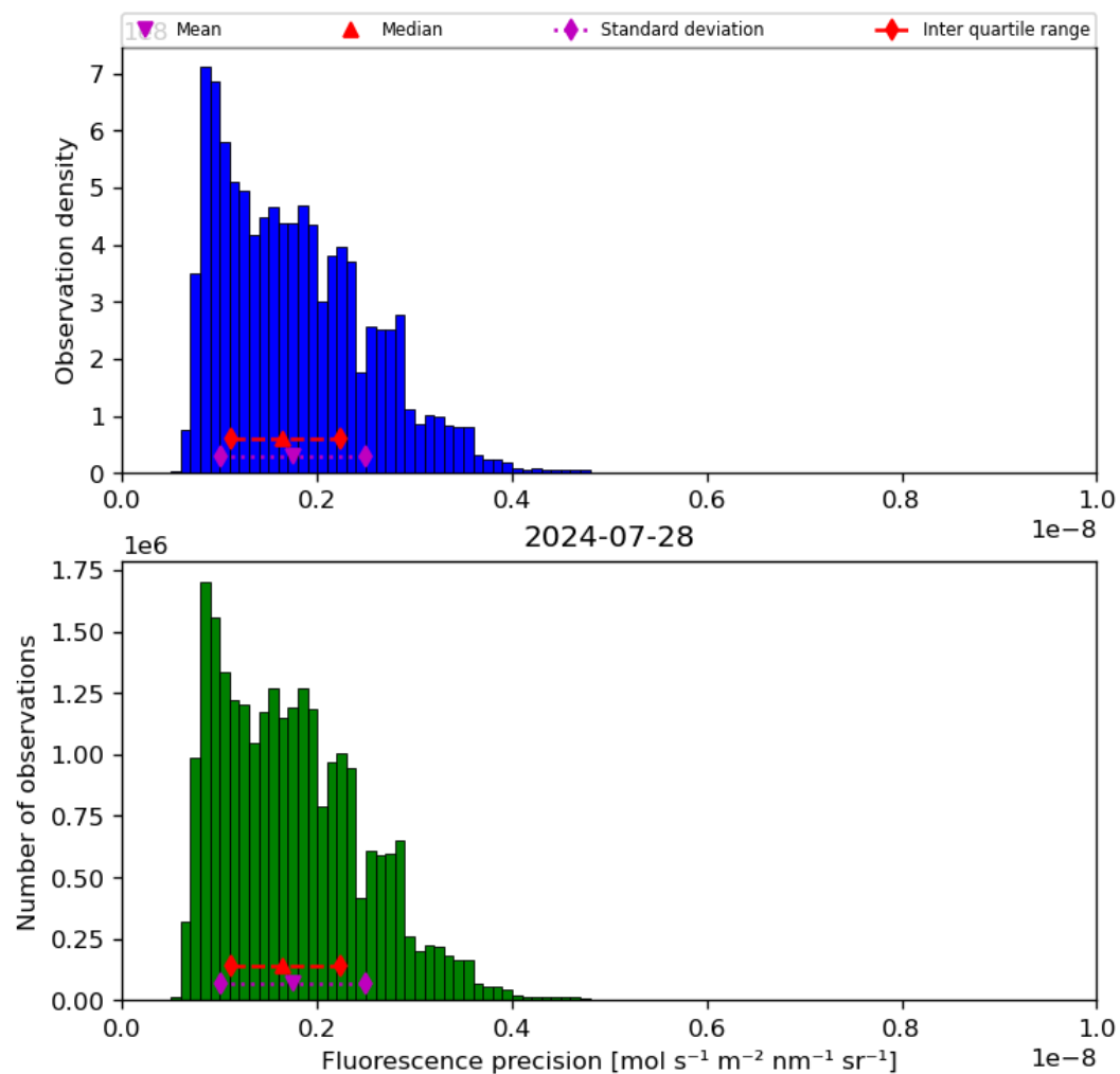
Figure 41: Histogram of “Fluorescence precision” for 2024-07-27 to 2024-07-29
