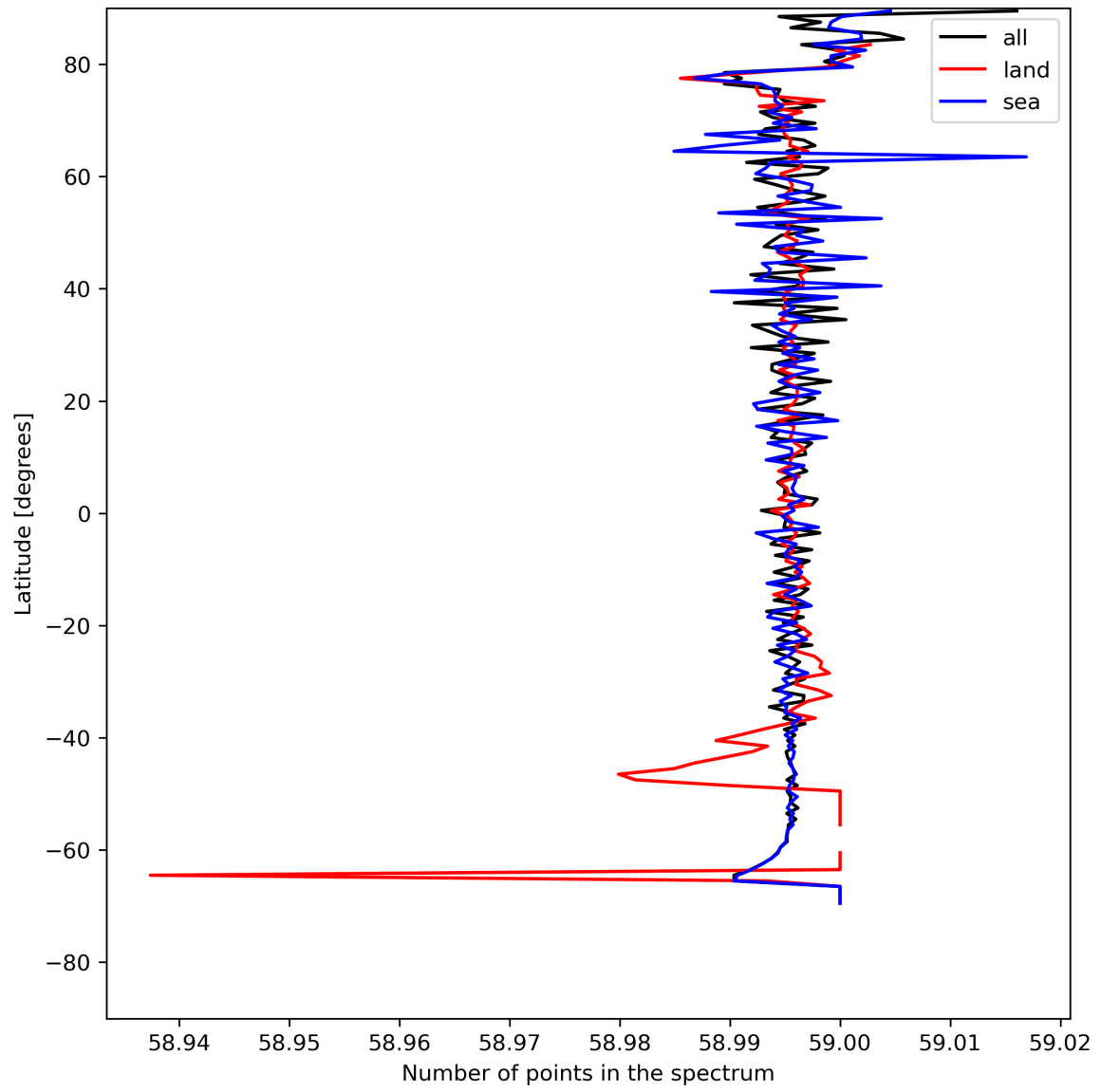
Figure 27: Zonal average of “Number of points in the spectrum” for 2024-07-27 to 2024-07-29.
