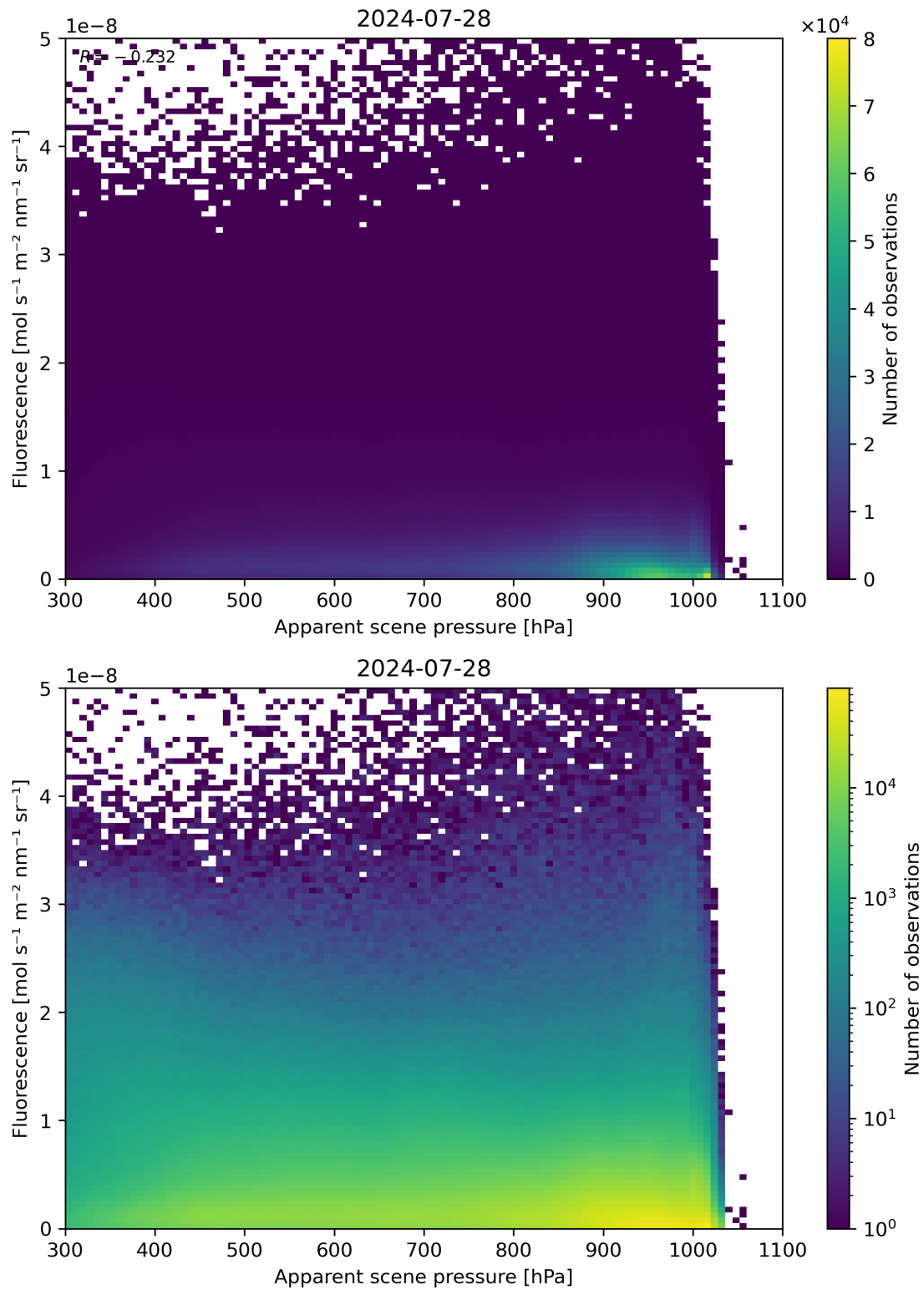
Figure 64: Scatter density plot of “Apparent scene pressure” against “Fluorescence” for 2024-07-27 to 2024-07-29.
