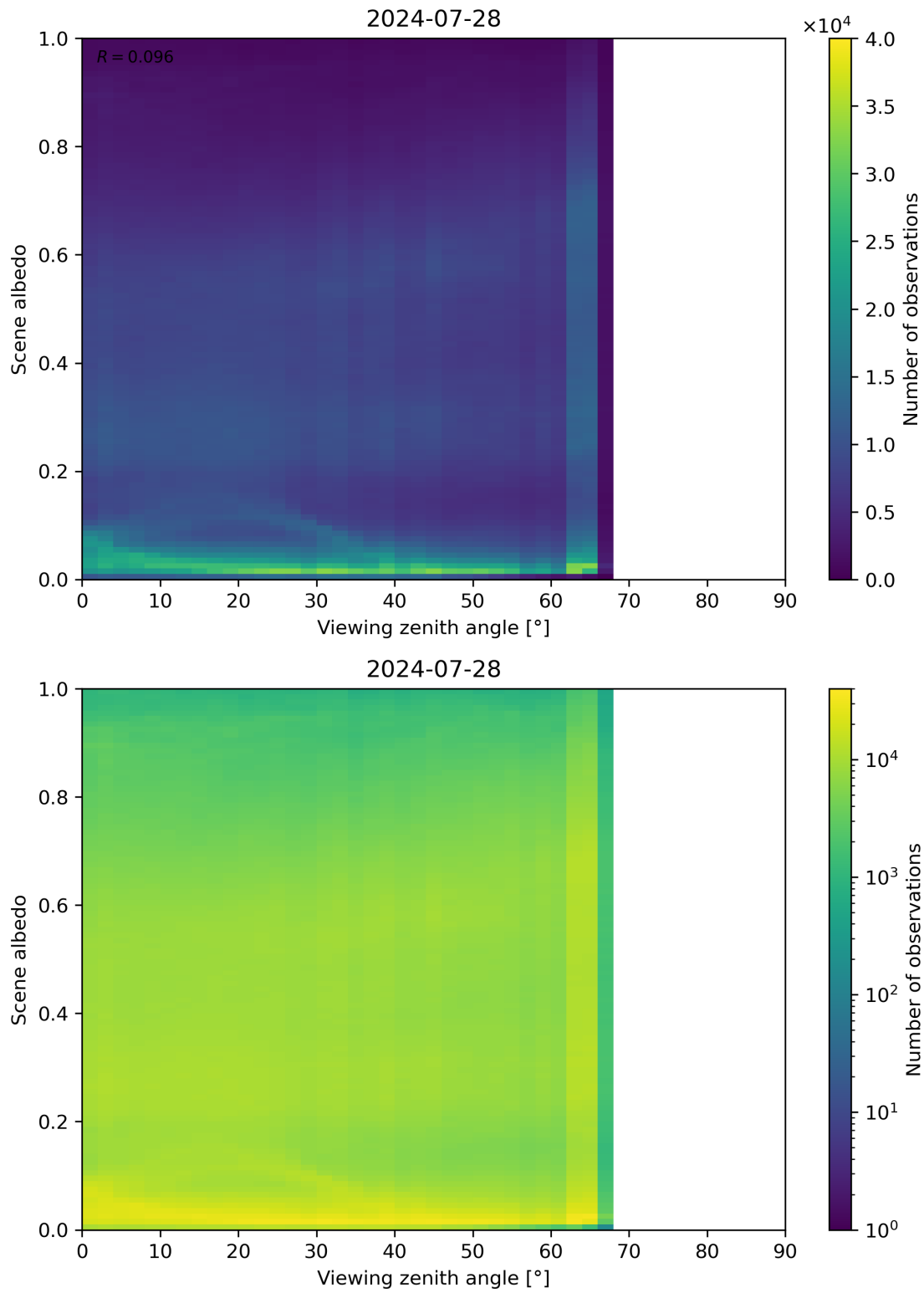
Figure 126: Scatter density plot of “Viewing zenith angle” against “Scene albedo” for 2024-07-27 to 2024-07-29.
