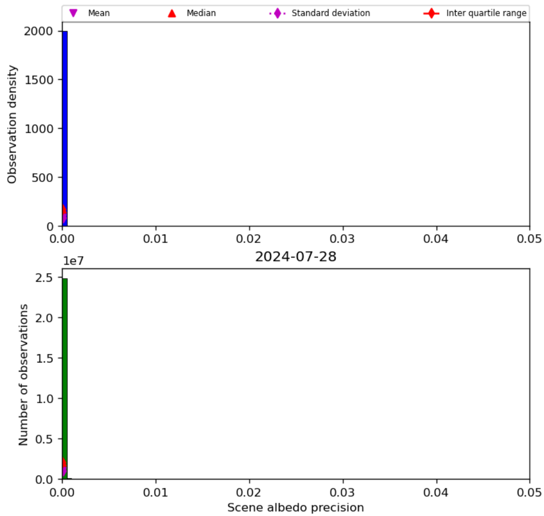
Figure 35: Histogram of “Scene albedo precision” for 2024-07-27 to 2024-07-29
