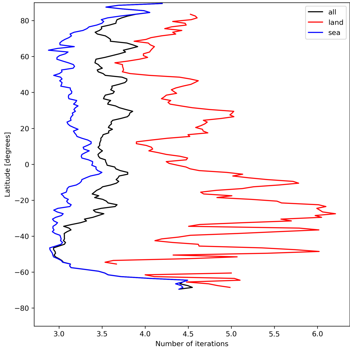
Figure 22: Zonal average of “Number of iterations” for 2024-07-27 to 2024-07-29.
