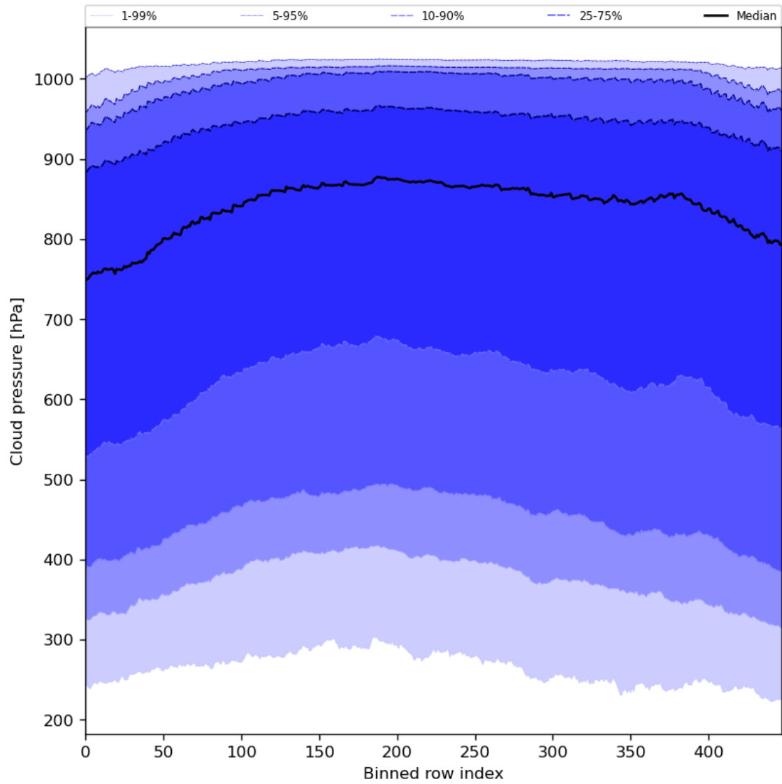
Figure 47: Along track statistics of “Cloud pressure” for 2024-07-27 to 2024-07-29
