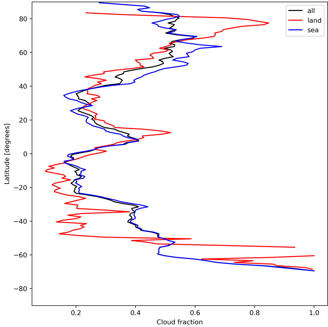
Figure 15: Zonal average of “Cloud fraction” for 2024-07-27 to 2024-07-29.
