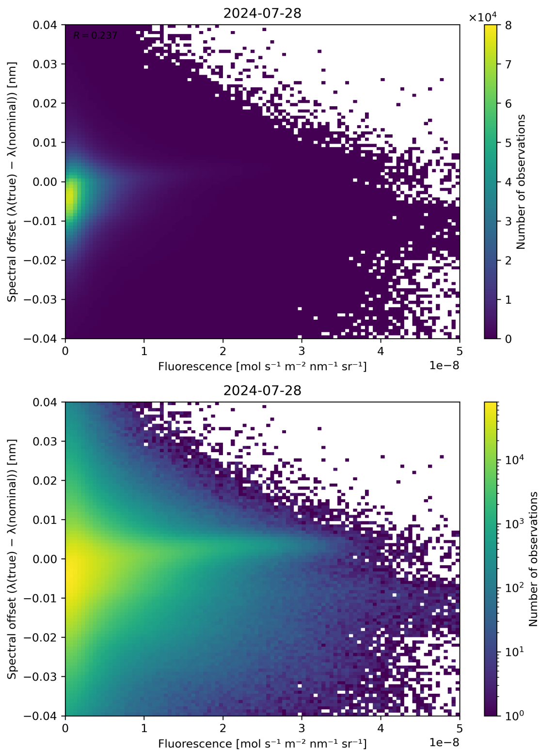
Figure 87: Scatter density plot of “Fluorescence” against “Spectral offset ( \lambda(\text{true}) - \lambda(\text{nominal}) )” for 2024-07-27 to 2024-07-29.
