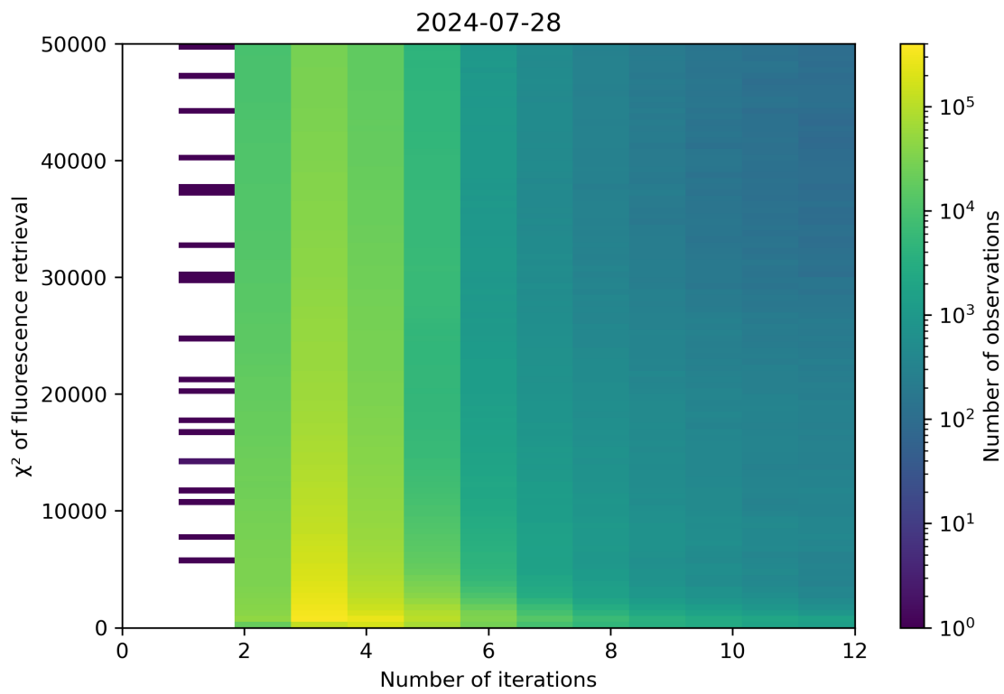
Figure 97: Scatter density plot of “Number of iterations” against “ \chi^2 of fluorescence retrieval” for 2024-07-27 to 2024-07-29.
