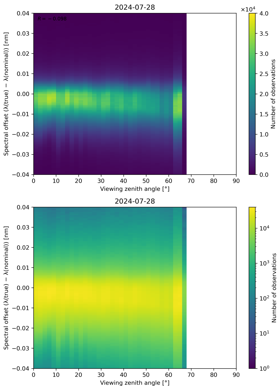
Figure 128: Scatter density plot of “Viewing zenith angle” against “Spectral offset ( \lambda(\text{true}) - \lambda(\text{nominal}) )” for 2024-07-27 to 2024-07-29.
