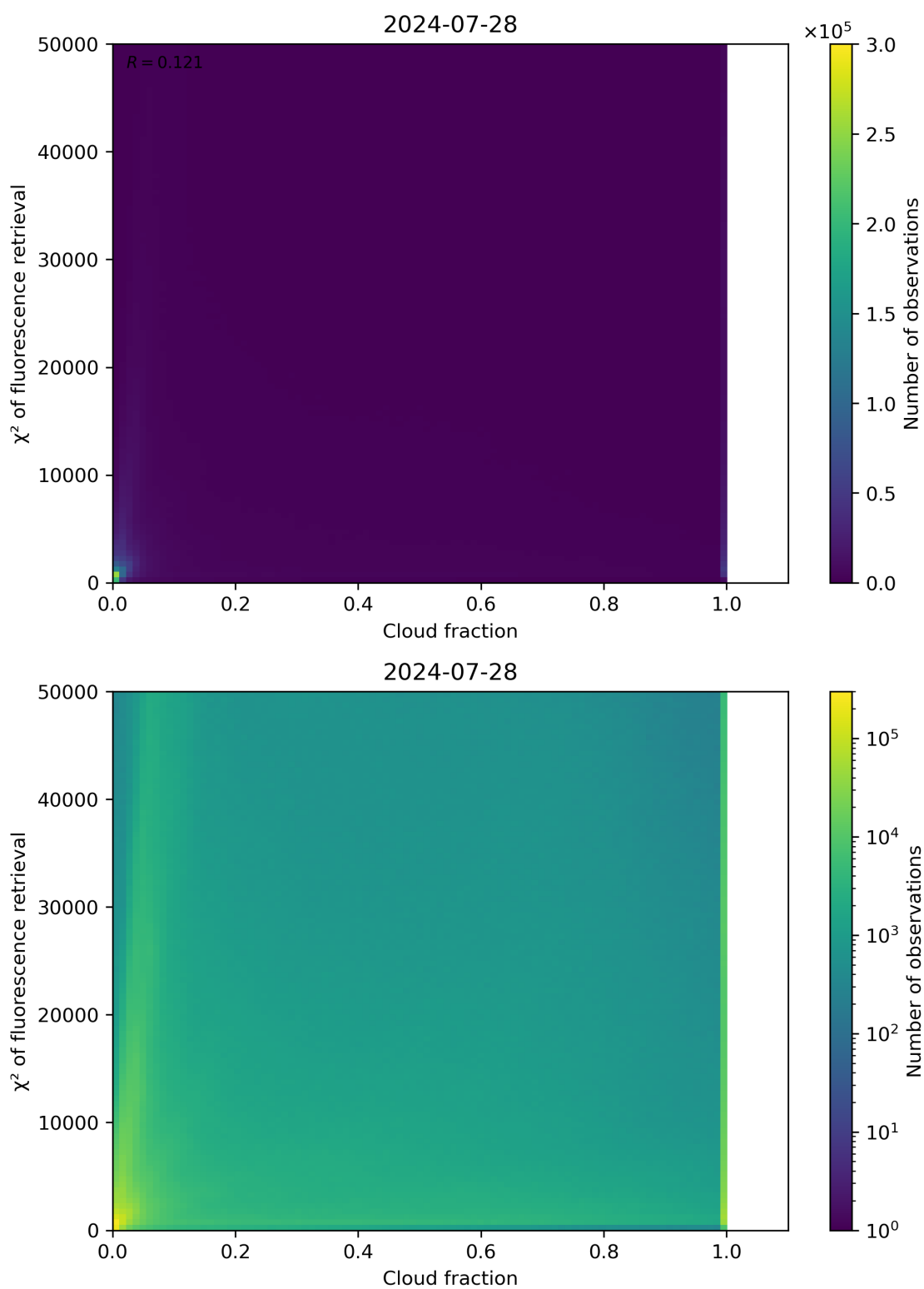
Figure 71: Scatter density plot of “Cloud fraction” against “ \chi^2 of fluorescence retrieval” for 2024-07-27 to 2024-07-29.
