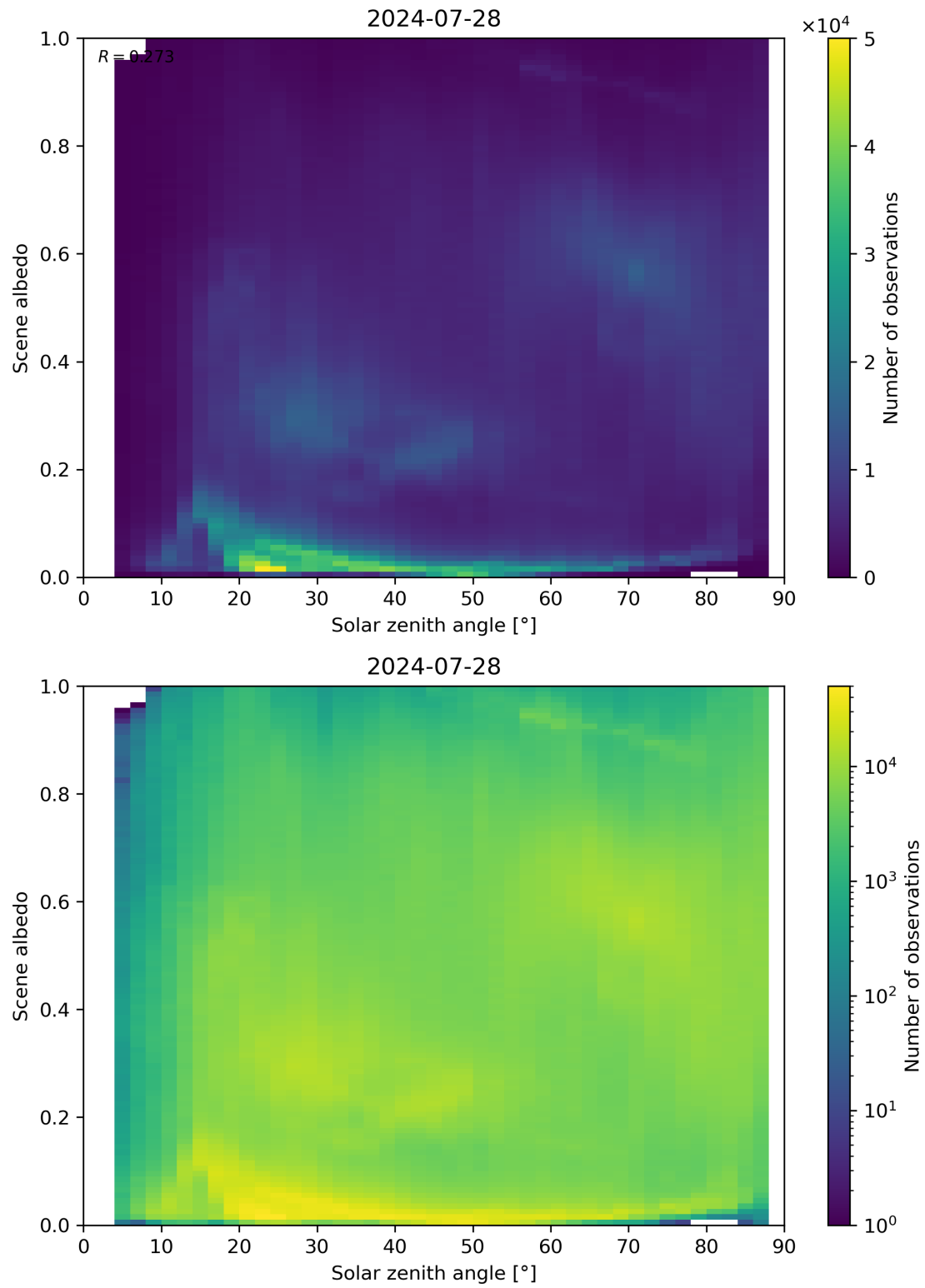
Figure 116: Scatter density plot of “Solar zenith angle” against “Scene albedo” for 2024-07-27 to 2024-07-29.
