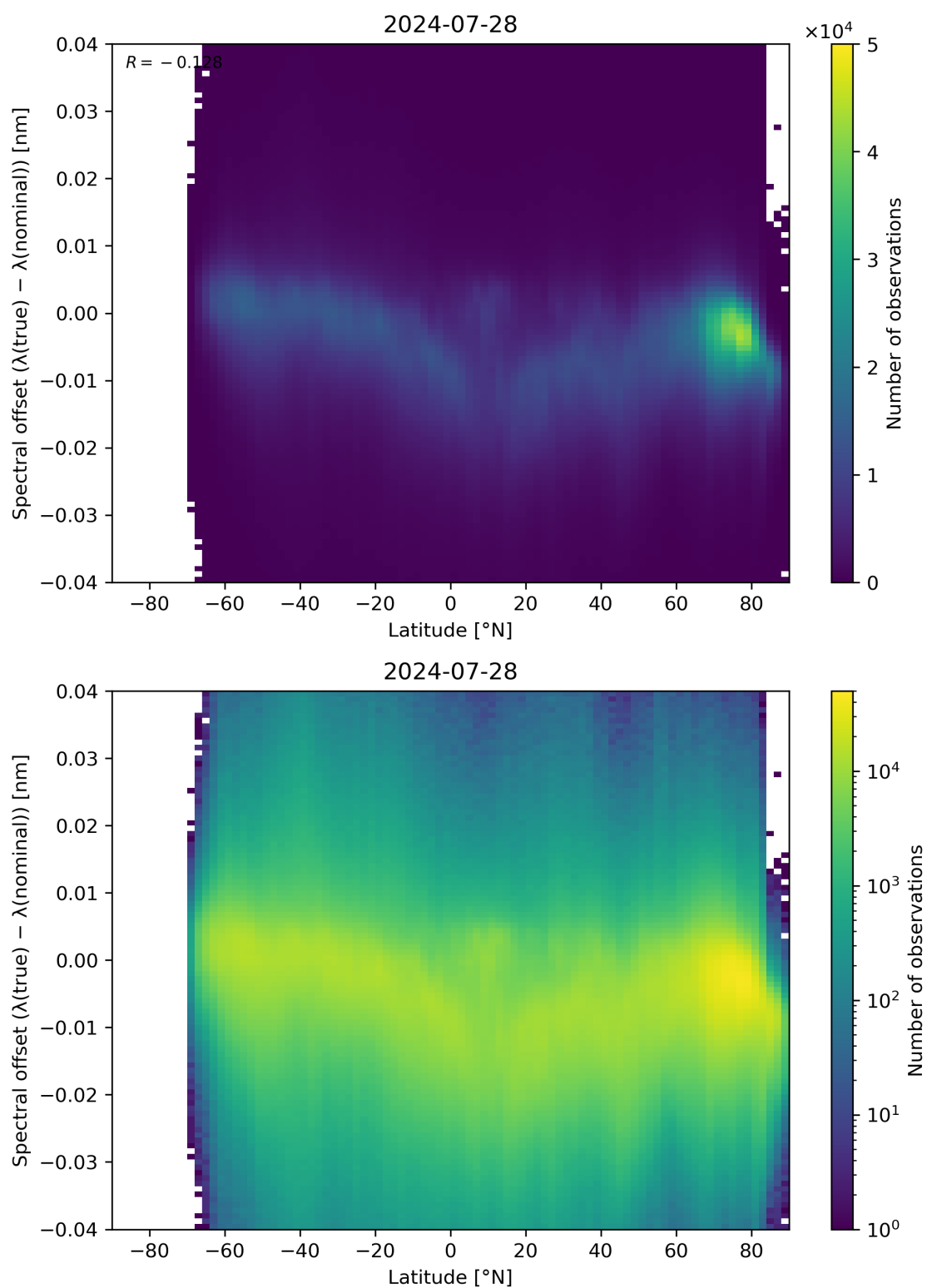
Figure 96: Scatter density plot of “Latitude” against “Spectral offset ( \lambda(\text{true}) - \lambda(\text{nominal}) )” for 2024-07-27 to 2024-07-29.
