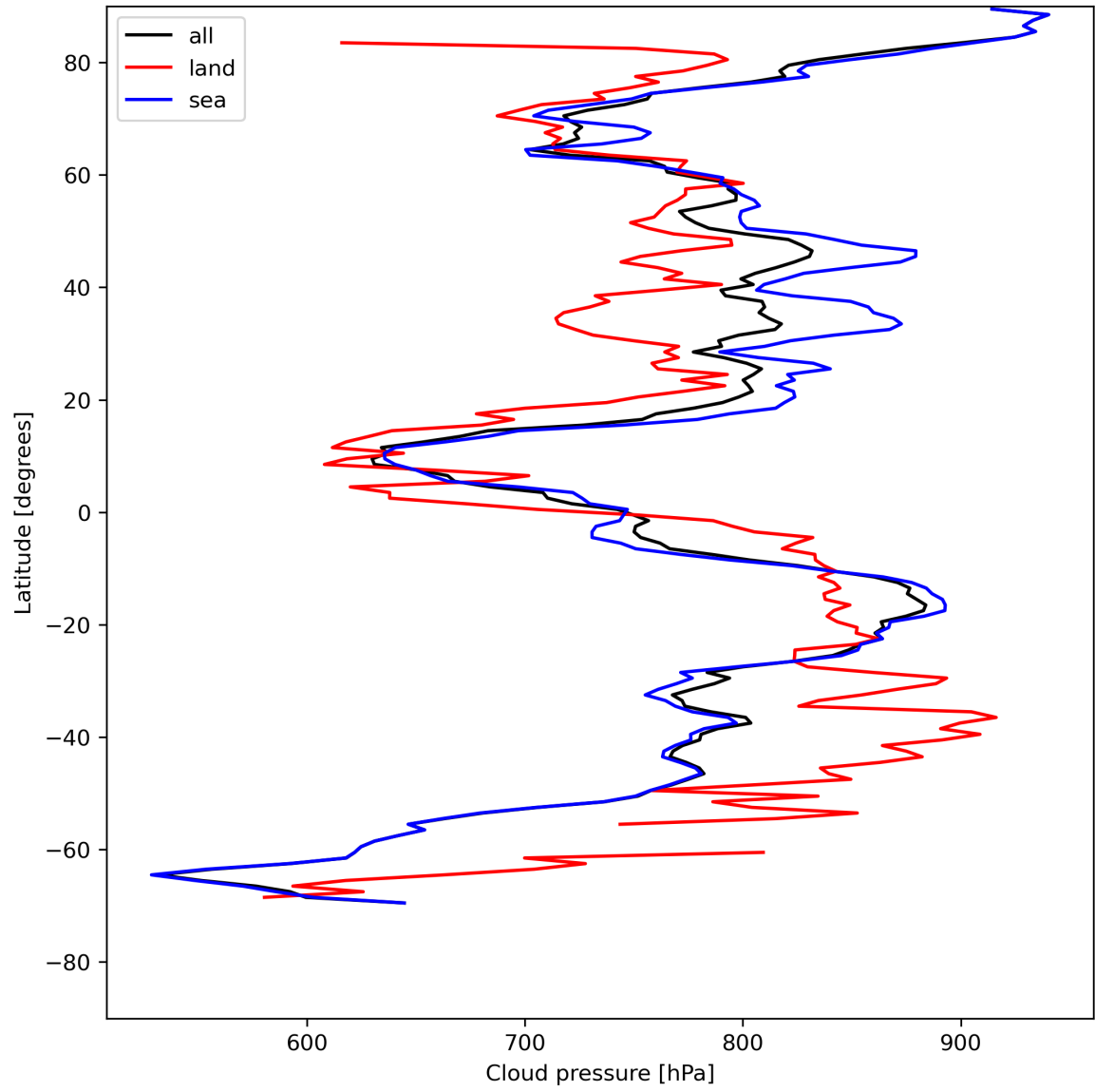
Figure 13: Zonal average of “Cloud pressure” for 2024-07-27 to 2024-07-29.
