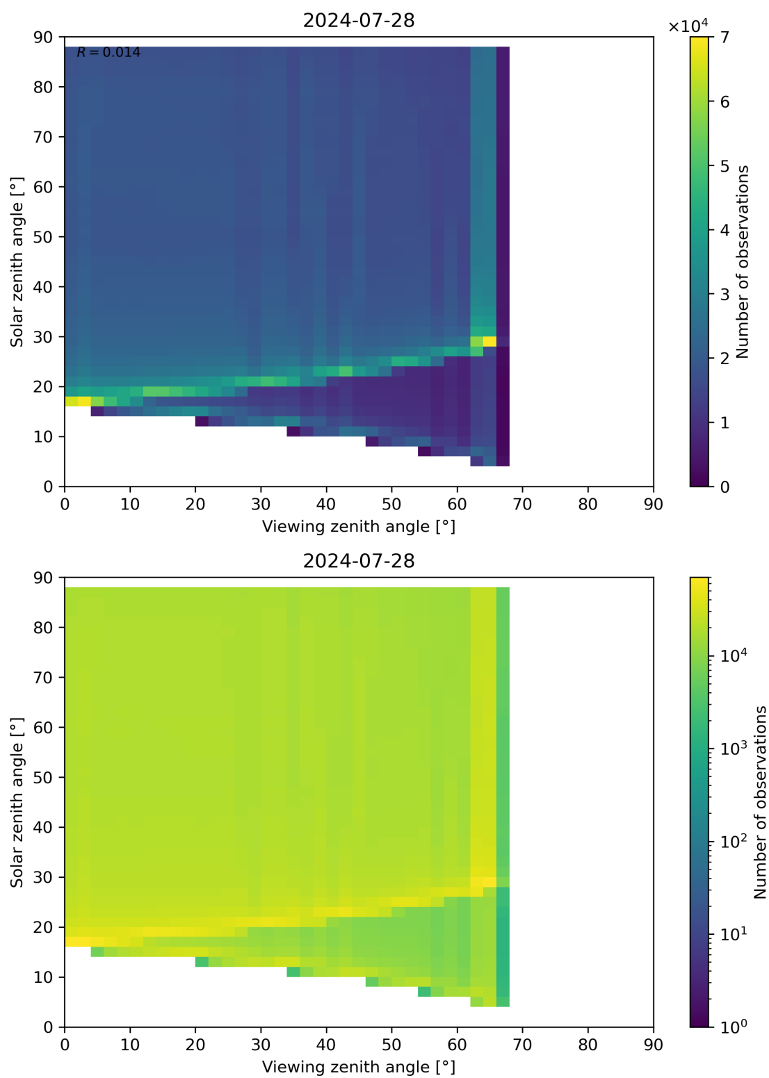
Figure 127: Scatter density plot of “Viewing zenith angle” against “Solar zenith angle” for 2024-07-27 to 2024-07-29.
