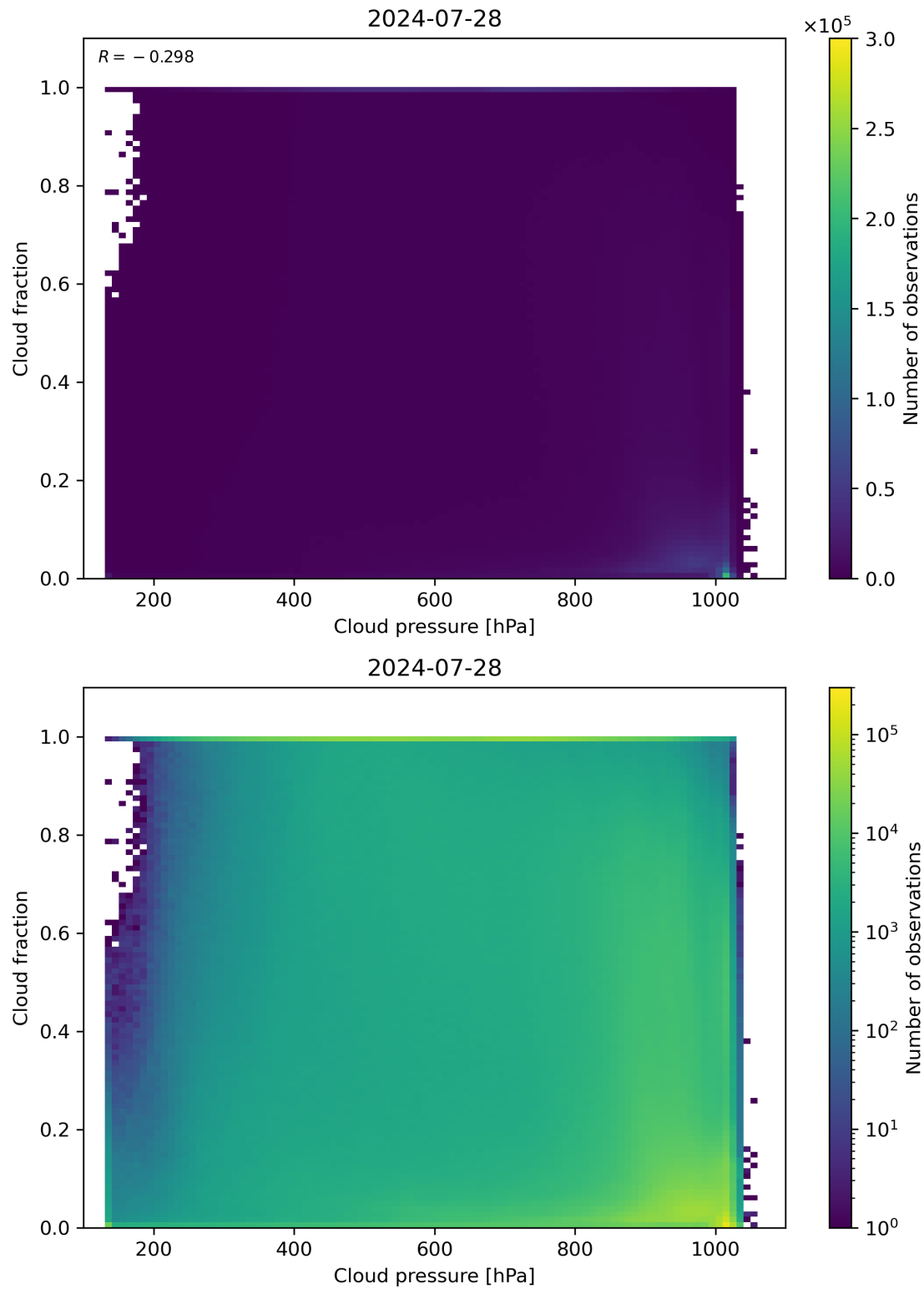
Figure 79: Scatter density plot of “Cloud pressure” against “Cloud fraction” for 2024-07-27 to 2024-07-29.
