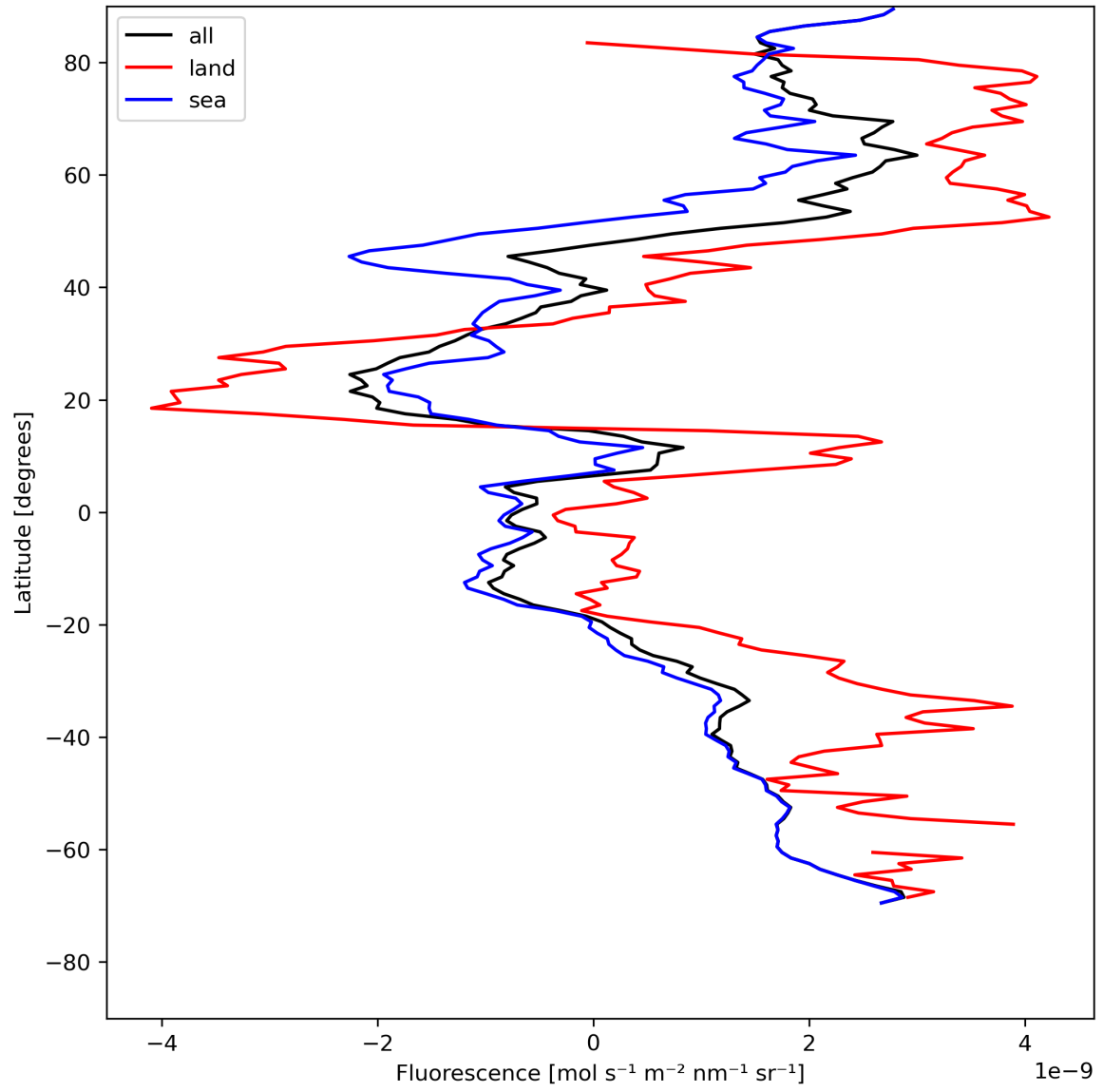
Figure 23: Zonal average of “Fluorescence” for 2024-07-27 to 2024-07-29.
