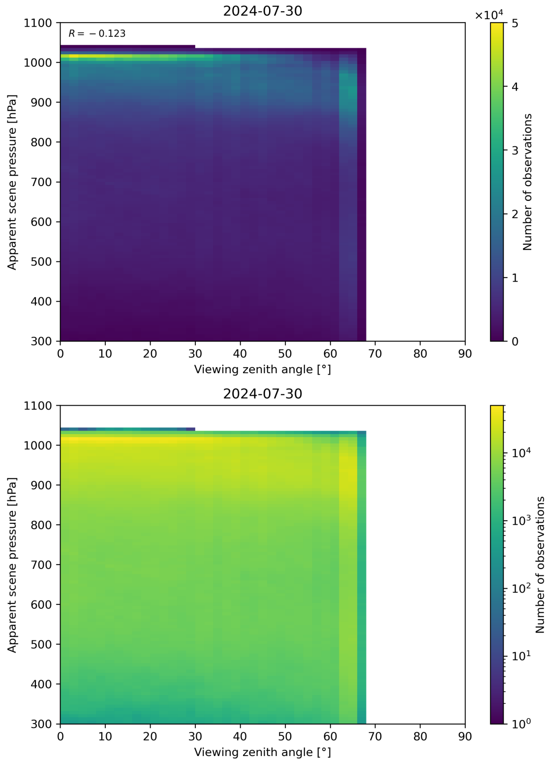
Figure 118: Scatter density plot of “Viewing zenith angle” against “Apparent scene pressure” for 2024-07-29 to 2024-07-31.
