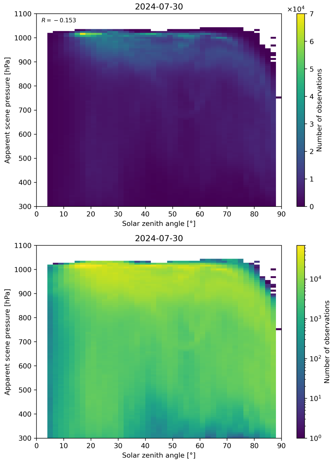
Figure 108: Scatter density plot of “Solar zenith angle” against “Apparent scene pressure” for 2024-07-29 to 2024-07-31.
