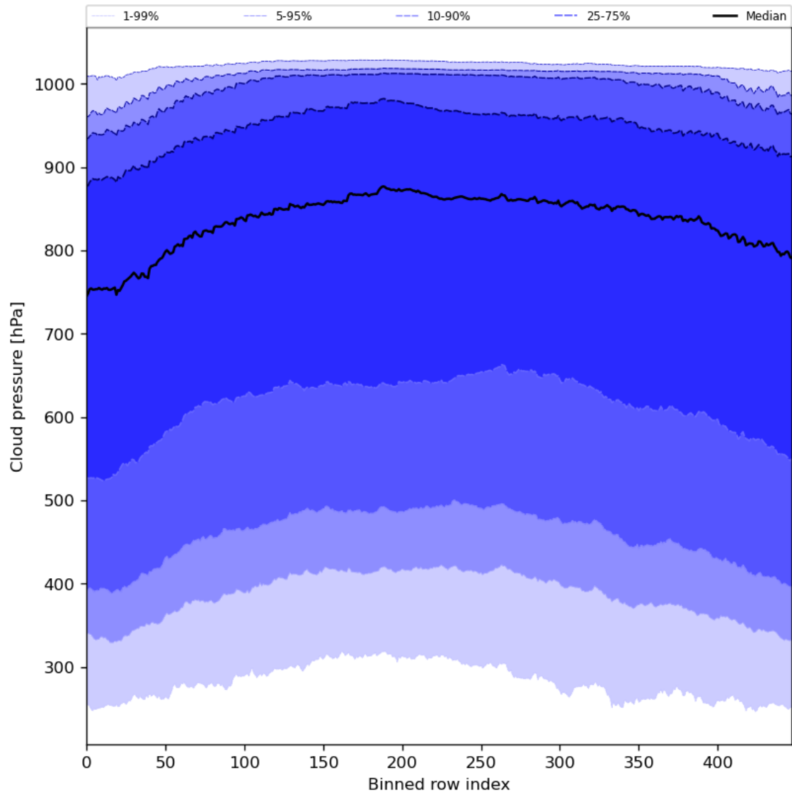
Figure 47: Along track statistics of “Cloud pressure” for 2024-07-29 to 2024-07-31
