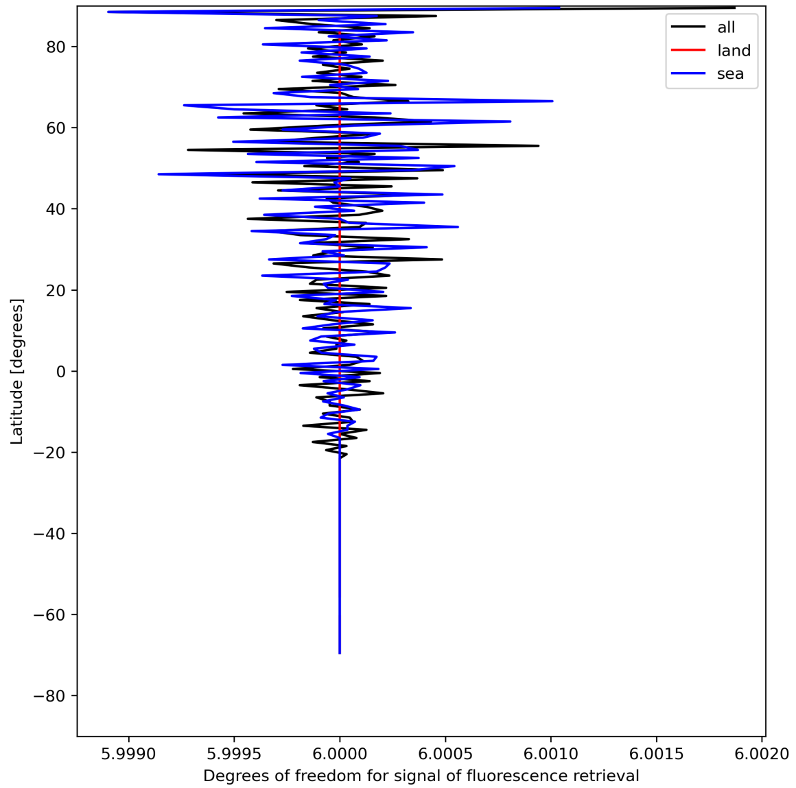
Figure 26: Zonal average of “Degrees of freedom for signal of fluorescence retrieval” for 2024-07-29 to 2024-07-31.
