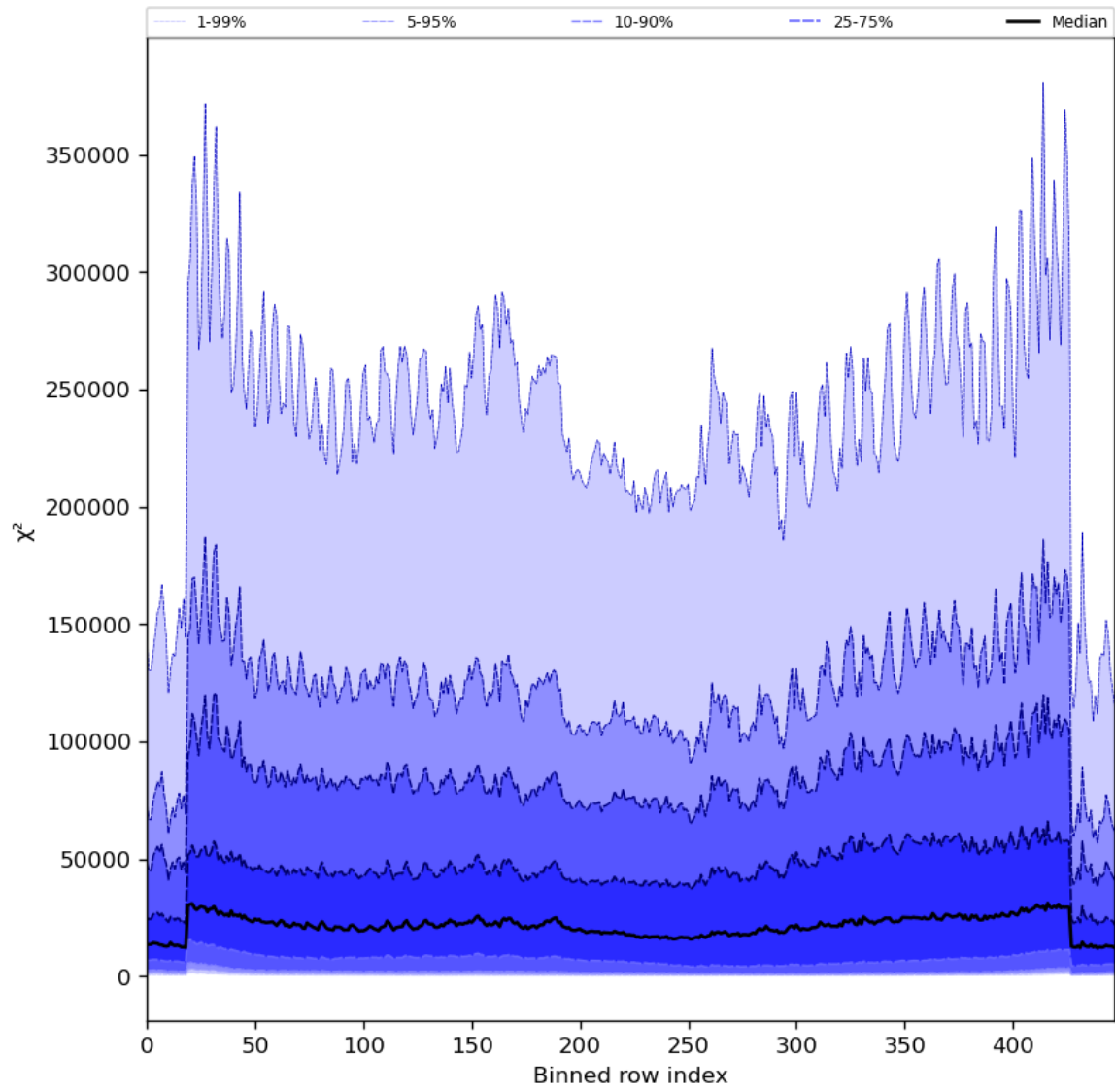
Figure 55: Along track statistics of “ \chi^2 ” for 2024-07-29 to 2024-07-31
