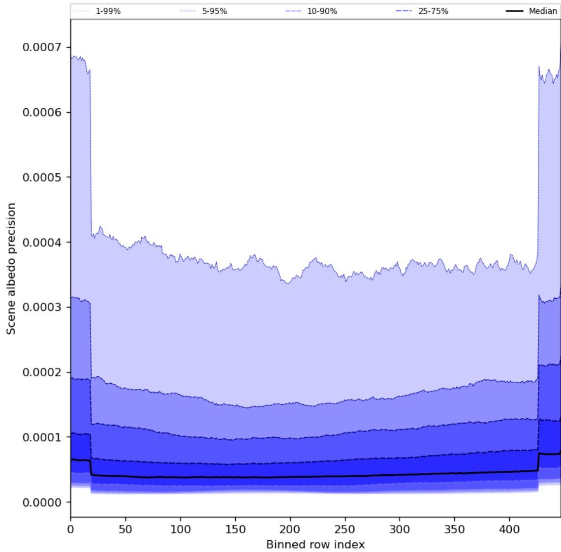
Figure 52: Along track statistics of “Scene albedo precision” for 2024-07-29 to 2024-07-31
