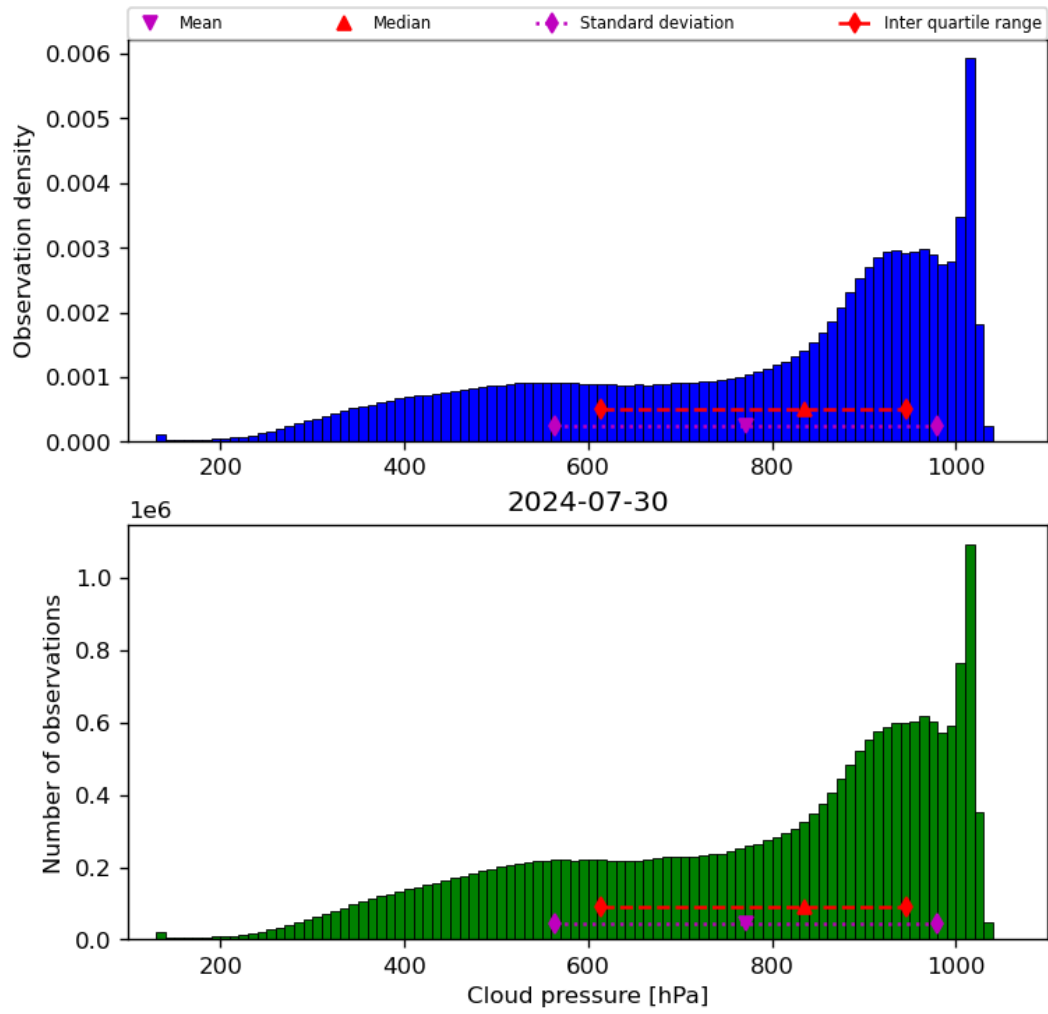
Figure 30: Histogram of “Cloud pressure” for 2024-07-29 to 2024-07-31
