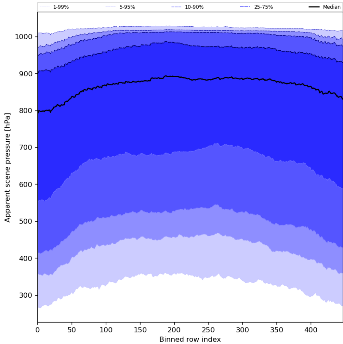
Figure 53: Along track statistics of “Apparent scene pressure” for 2024-07-29 to 2024-07-31
