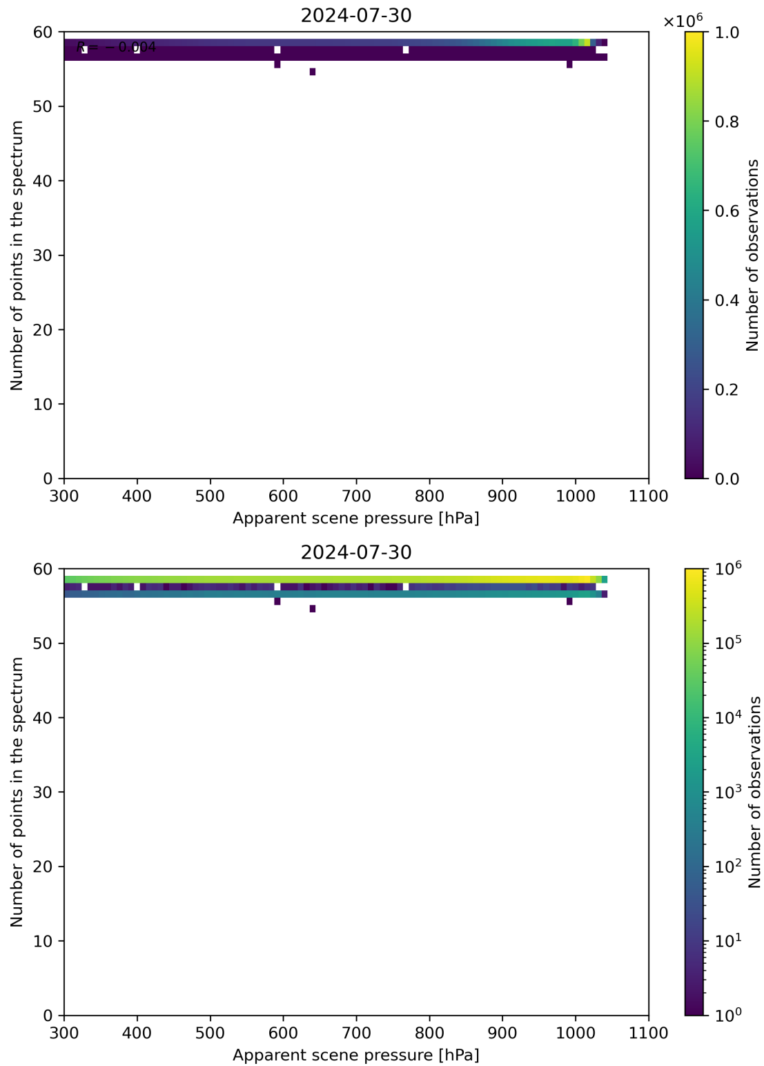
Figure 66: Scatter density plot of “Apparent scene pressure” against “Number of points in the spectrum” for 2024-07-29 to 2024-07-31.
