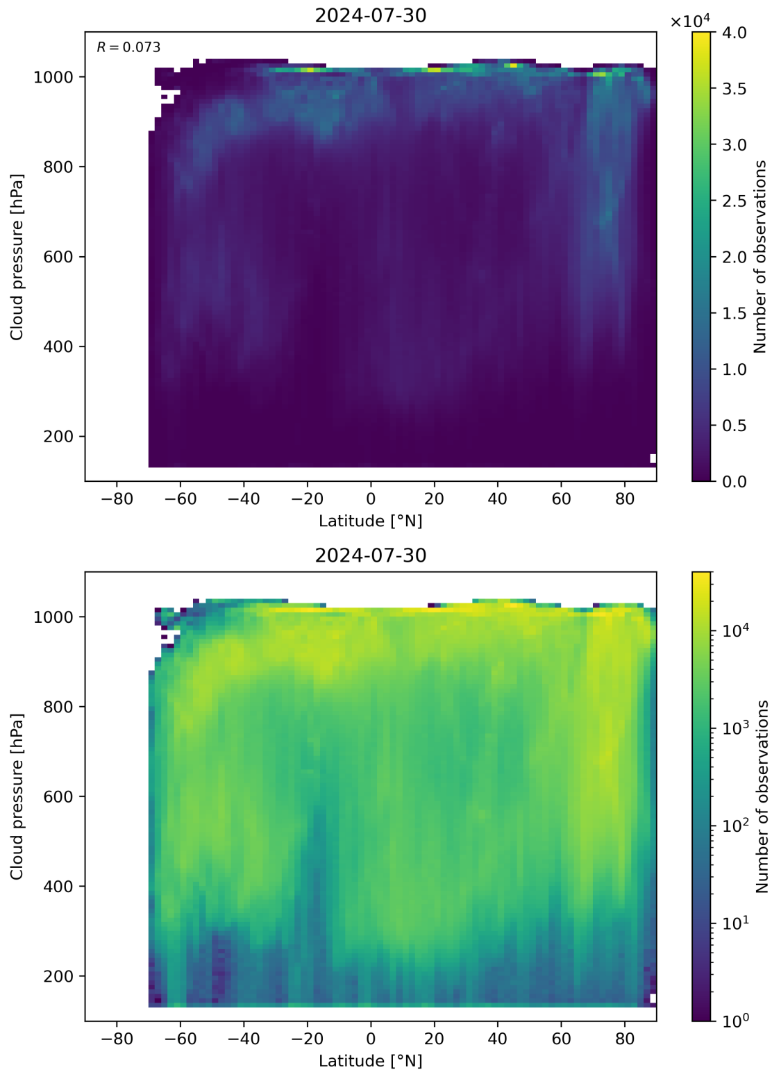
Figure 91: Scatter density plot of “Latitude” against “Cloud pressure” for 2024-07-29 to 2024-07-31.
