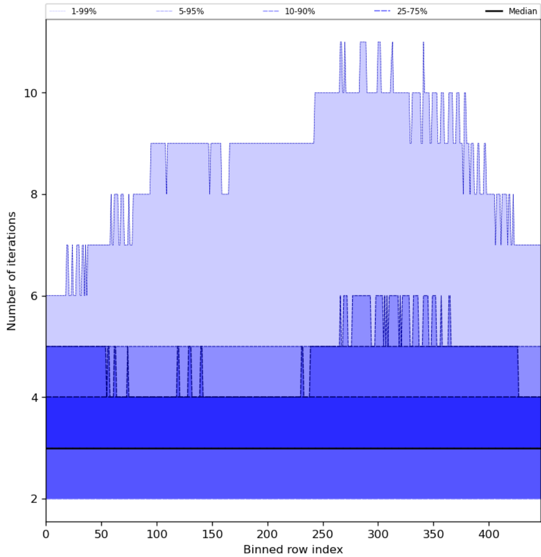
Figure 56: Along track statistics of “Number of iterations” for 2024-07-29 to 2024-07-31
