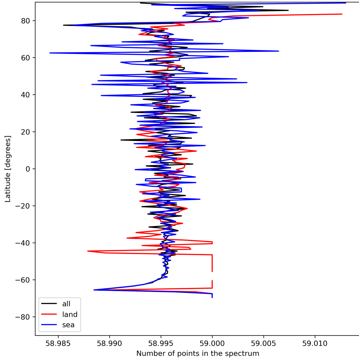
Figure 27: Zonal average of “Number of points in the spectrum” for 2024-07-29 to 2024-07-31.
