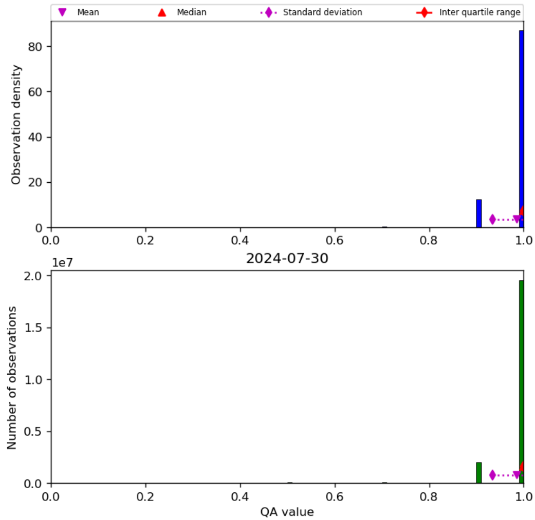
Figure 29: Histogram of “QA value” for 2024-07-29 to 2024-07-31
