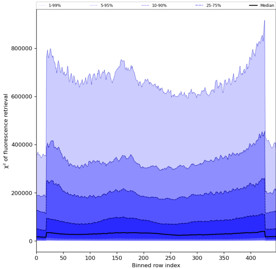
Figure 59: Along track statistics of “ \chi^2 of fluorescence retrieval” for 2024-07-29 to 2024-07-31
