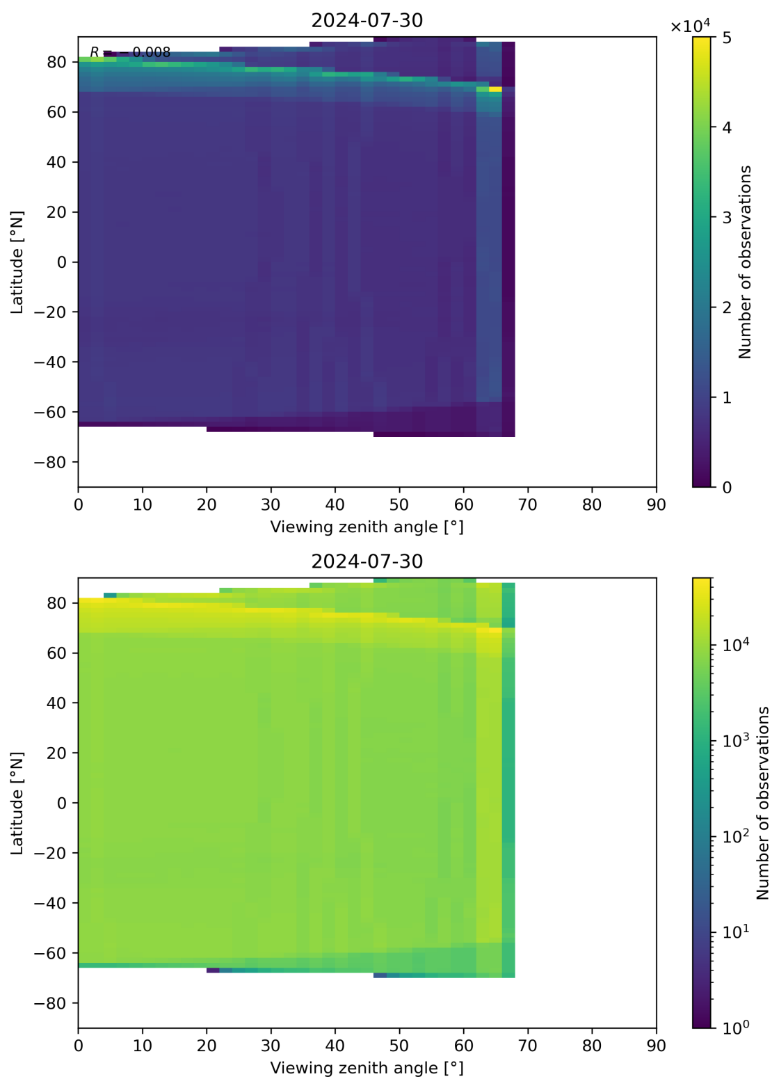
Figure 123: Scatter density plot of “Viewing zenith angle” against “Latitude” for 2024-07-29 to 2024-07-31.
