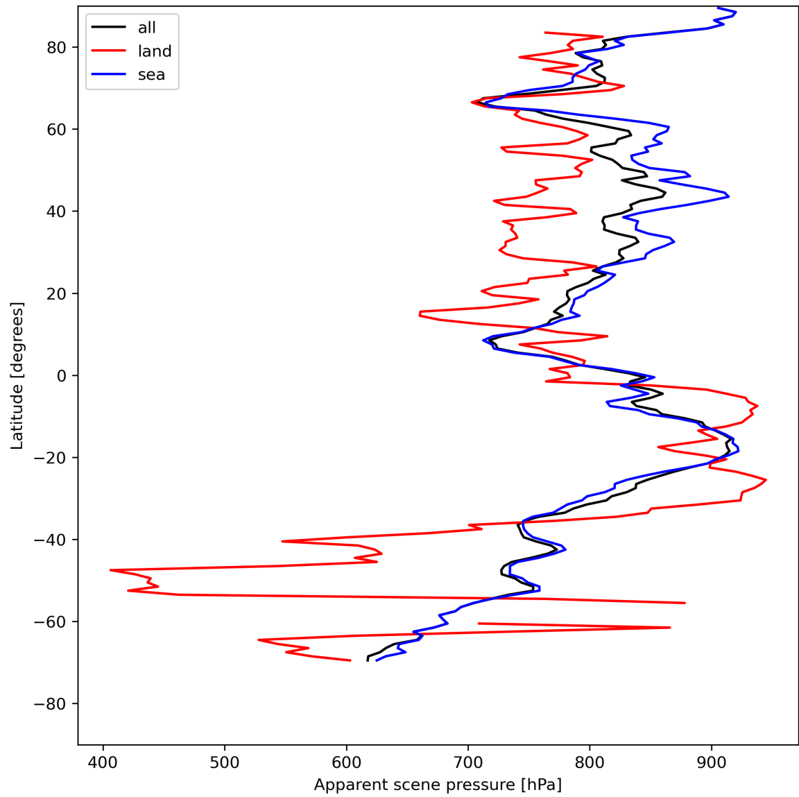
Figure 19: Zonal average of “Apparent scene pressure” for 2024-07-29 to 2024-07-31.
