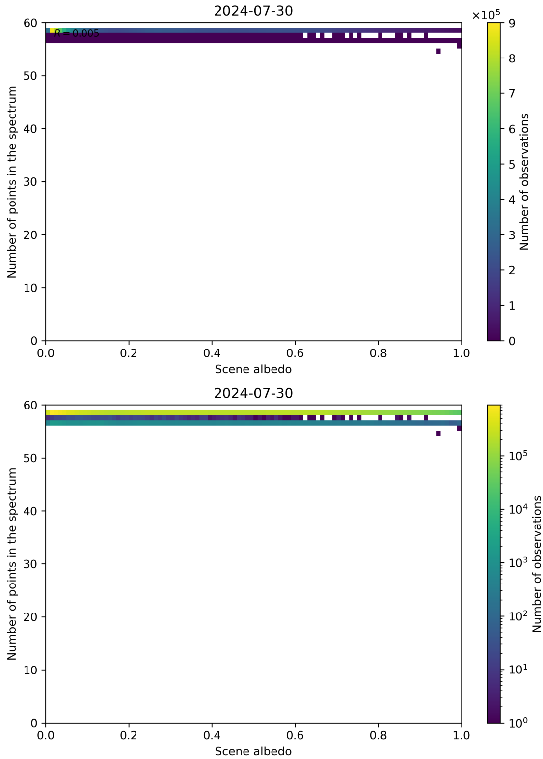
Figure 106: Scatter density plot of “Scene albedo” against “Number of points in the spectrum” for 2024-07-29 to 2024-07-31.
