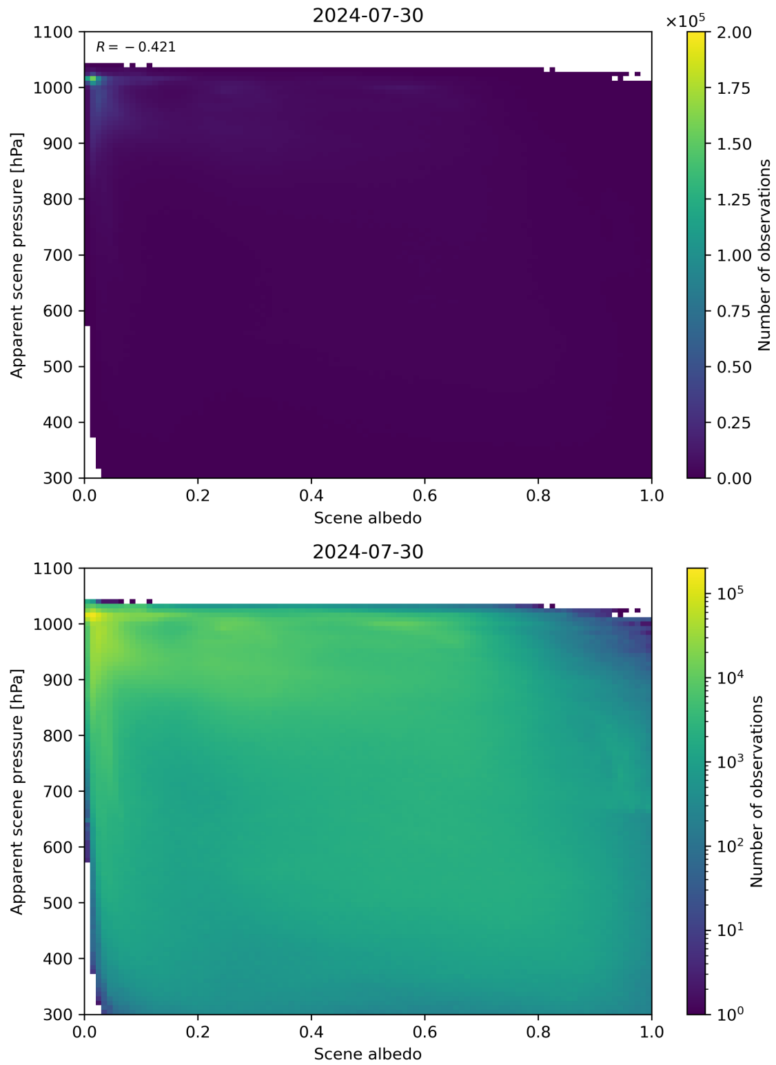
Figure 102: Scatter density plot of “Scene albedo” against “Apparent scene pressure” for 2024-07-29 to 2024-07-31.
