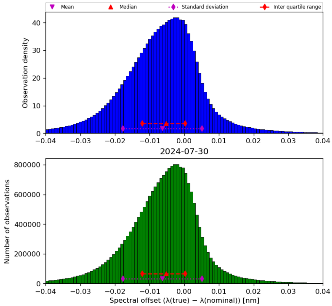
Figure 45: Histogram of “Spectral offset ( \lambda(\text{true}) - \lambda(\text{nominal}) )” for 2024-07-29 to 2024-07-31
