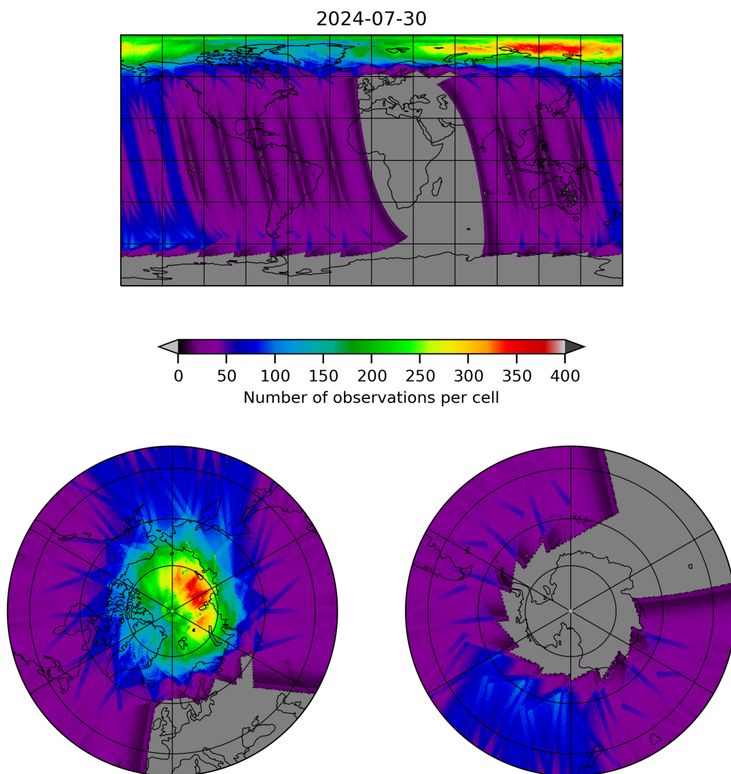
Figure 11: Map of the number of observations for 2024-07-29 to 2024-07-31
