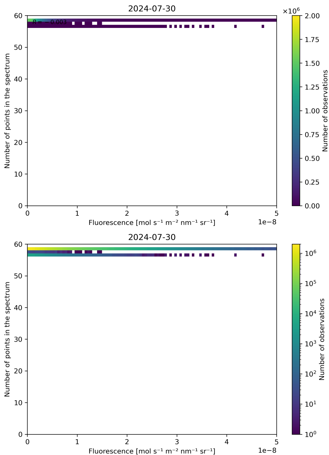
Figure 86: Scatter density plot of “Fluorescence” against “Number of points in the spectrum” for 2024-07-29 to 2024-07-31.
