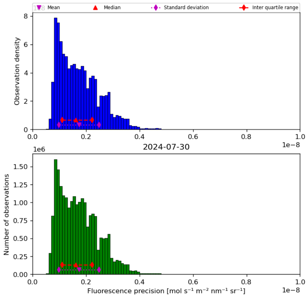
Figure 41: Histogram of “Fluorescence precision” for 2024-07-29 to 2024-07-31
