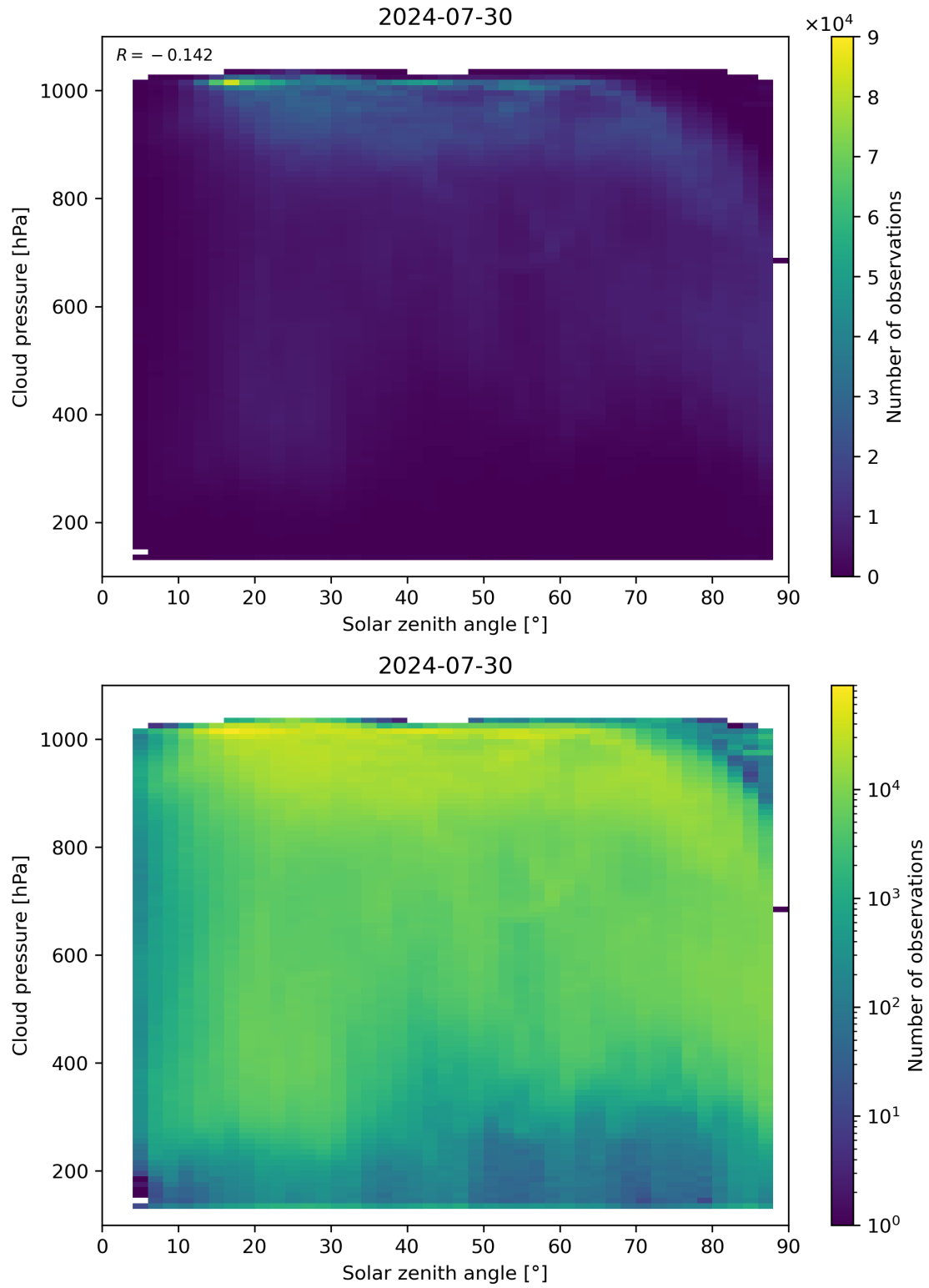
Figure 111: Scatter density plot of “Solar zenith angle” against “Cloud pressure” for 2024-07-29 to 2024-07-31.
