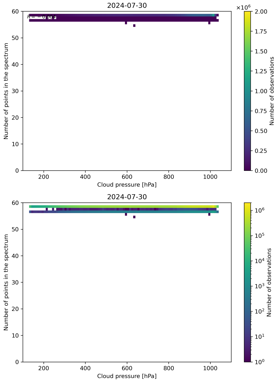
Figure 82: Scatter density plot of “Cloud pressure” against “Number of points in the spectrum” for 2024-07-29 to 2024-07-31.
