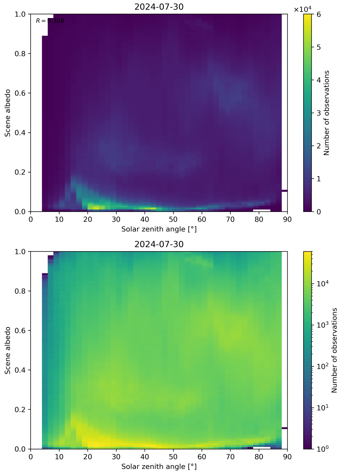
Figure 116: Scatter density plot of “Solar zenith angle” against “Scene albedo” for 2024-07-29 to 2024-07-31.
