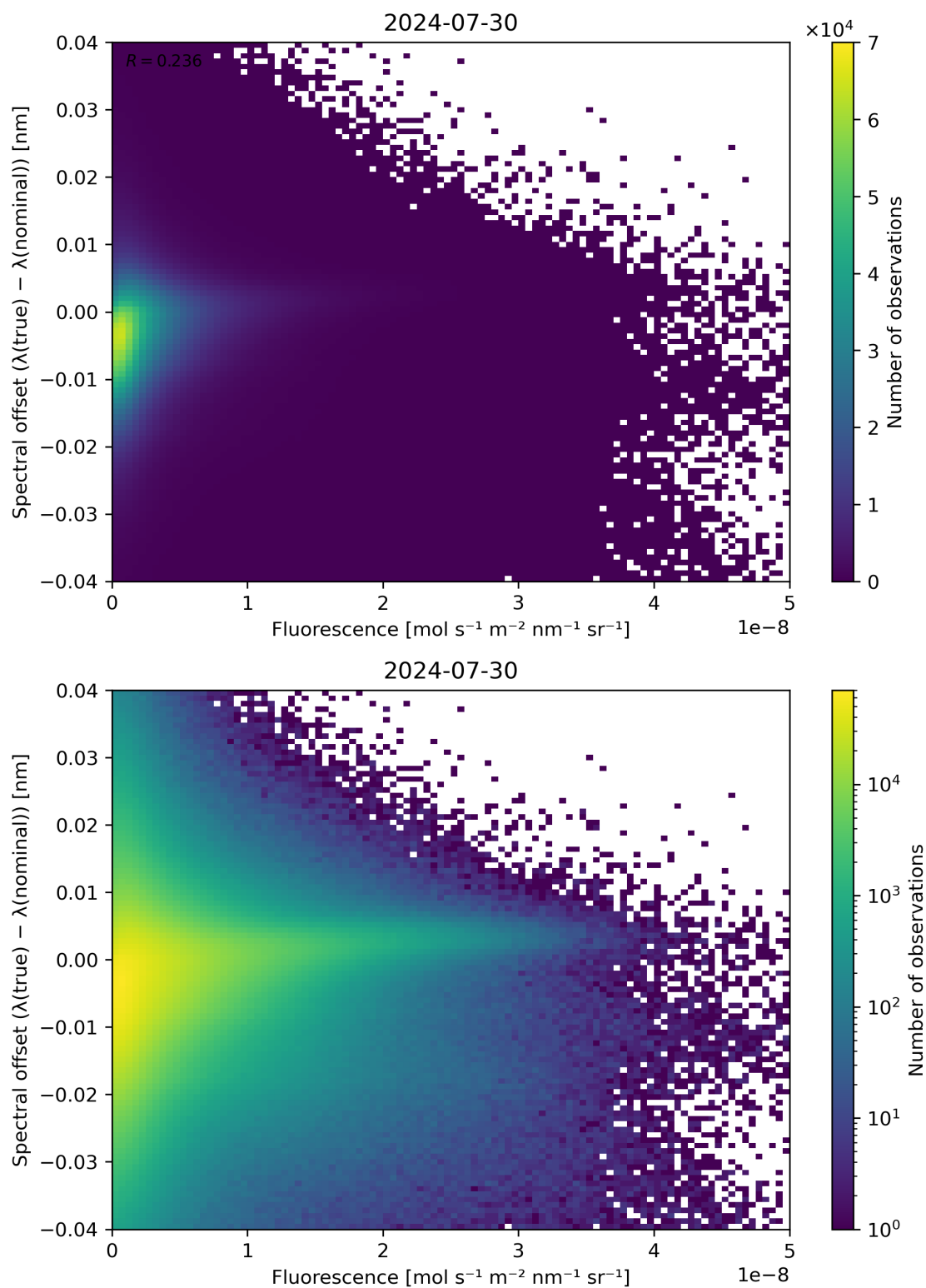
Figure 87: Scatter density plot of “Fluorescence” against “Spectral offset ( \lambda(\text{true}) - \lambda(\text{nominal}) )” for 2024-07-29 to 2024-07-31.
