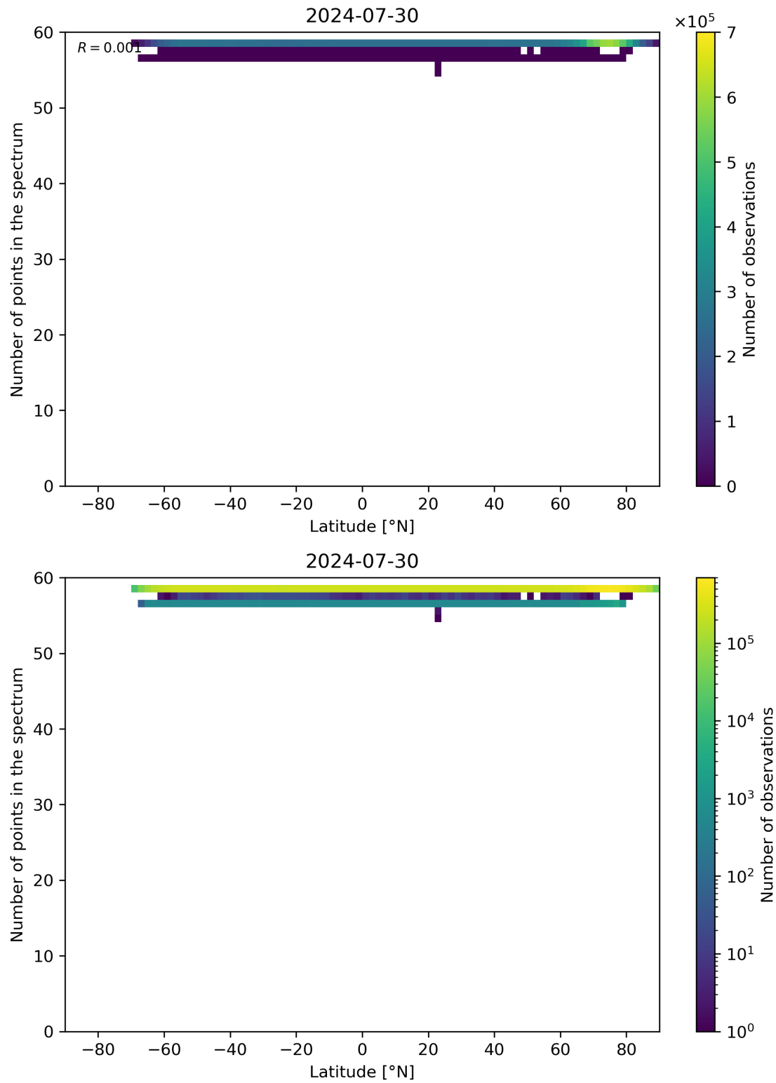
Figure 94: Scatter density plot of “Latitude” against “Number of points in the spectrum” for 2024-07-29 to 2024-07-31.
