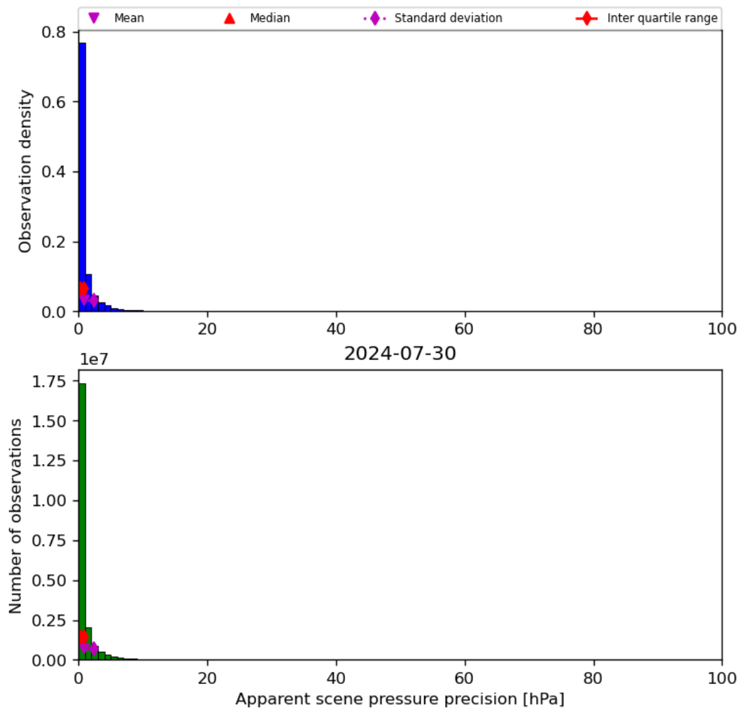
Figure 37: Histogram of “Apparent scene pressure precision” for 2024-07-29 to 2024-07-31
