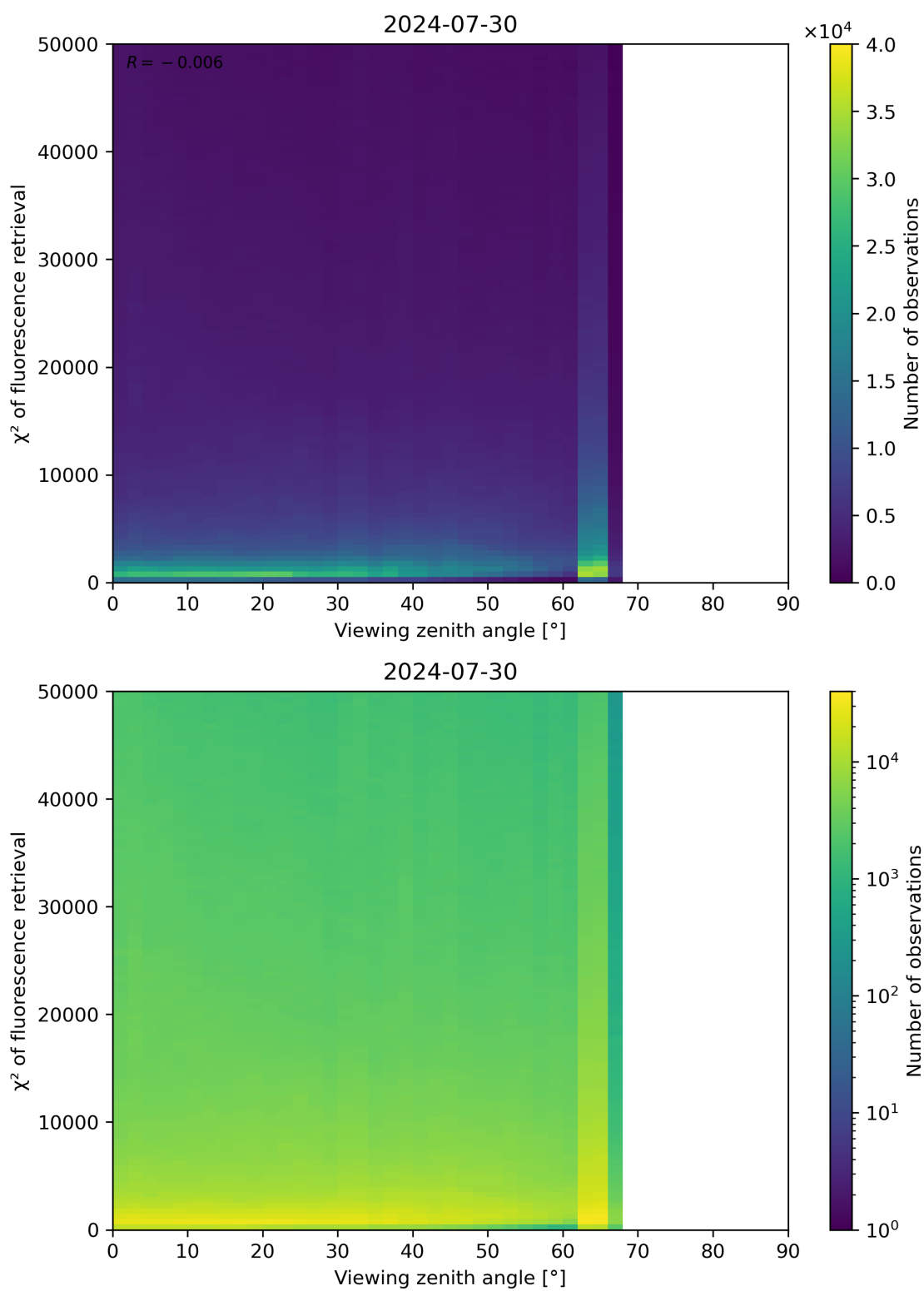
Figure 119: Scatter density plot of “Viewing zenith angle” against “ \chi^2 of fluorescence retrieval” for 2024-07-29 to 2024-07-31.
