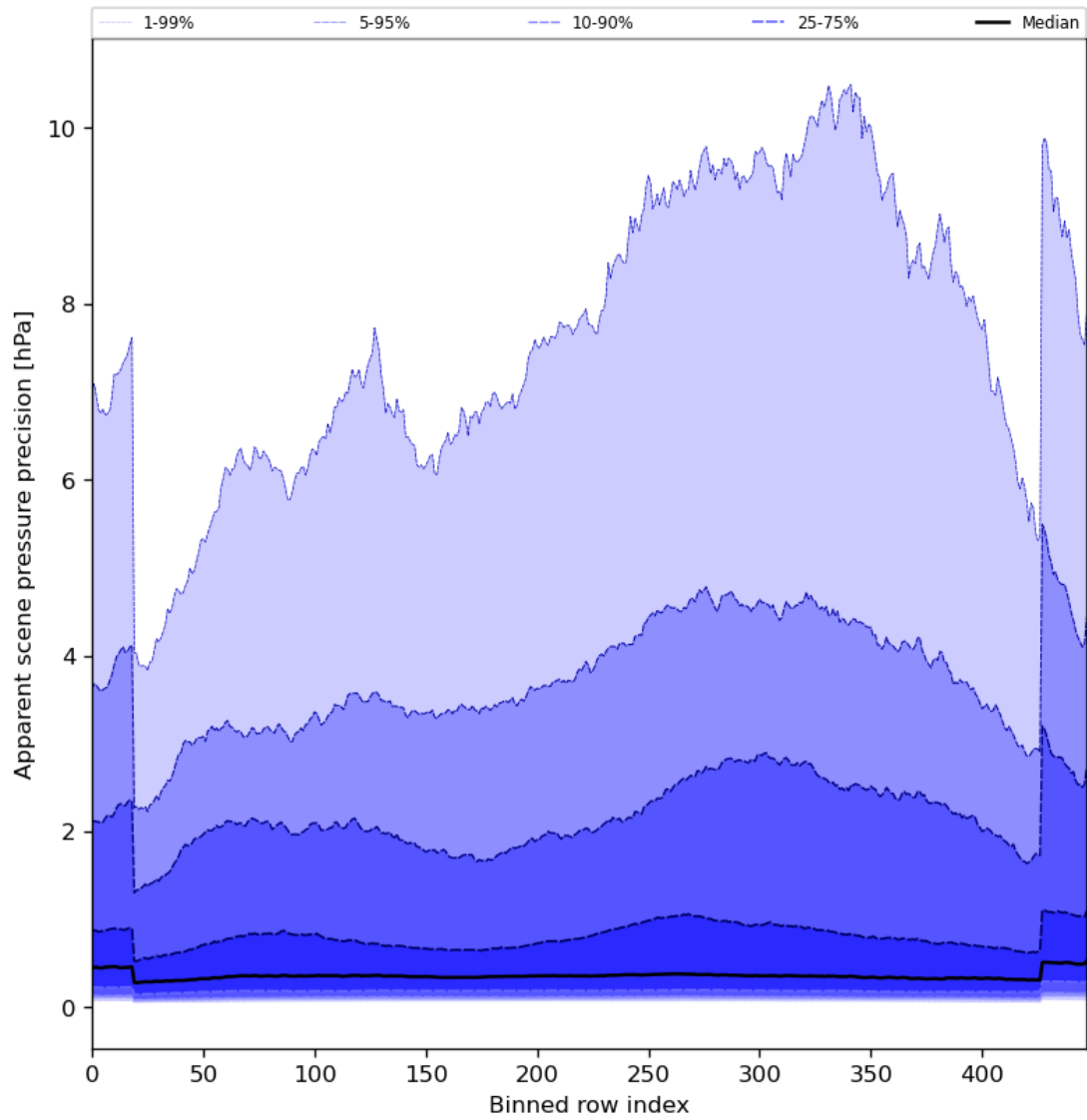
Figure 54: Along track statistics of “Apparent scene pressure precision” for 2024-07-29 to 2024-07-31
