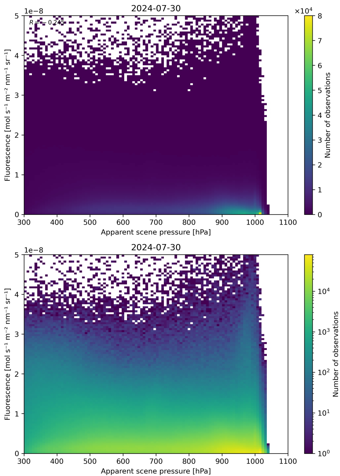
Figure 64: Scatter density plot of “Apparent scene pressure” against “Fluorescence” for 2024-07-29 to 2024-07-31.
