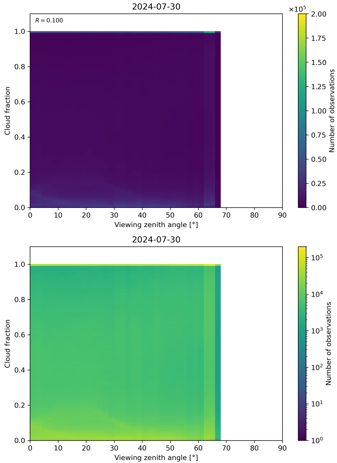
Figure 120: Scatter density plot of “Viewing zenith angle” against “Cloud fraction” for 2024-07-29 to 2024-07-31.
