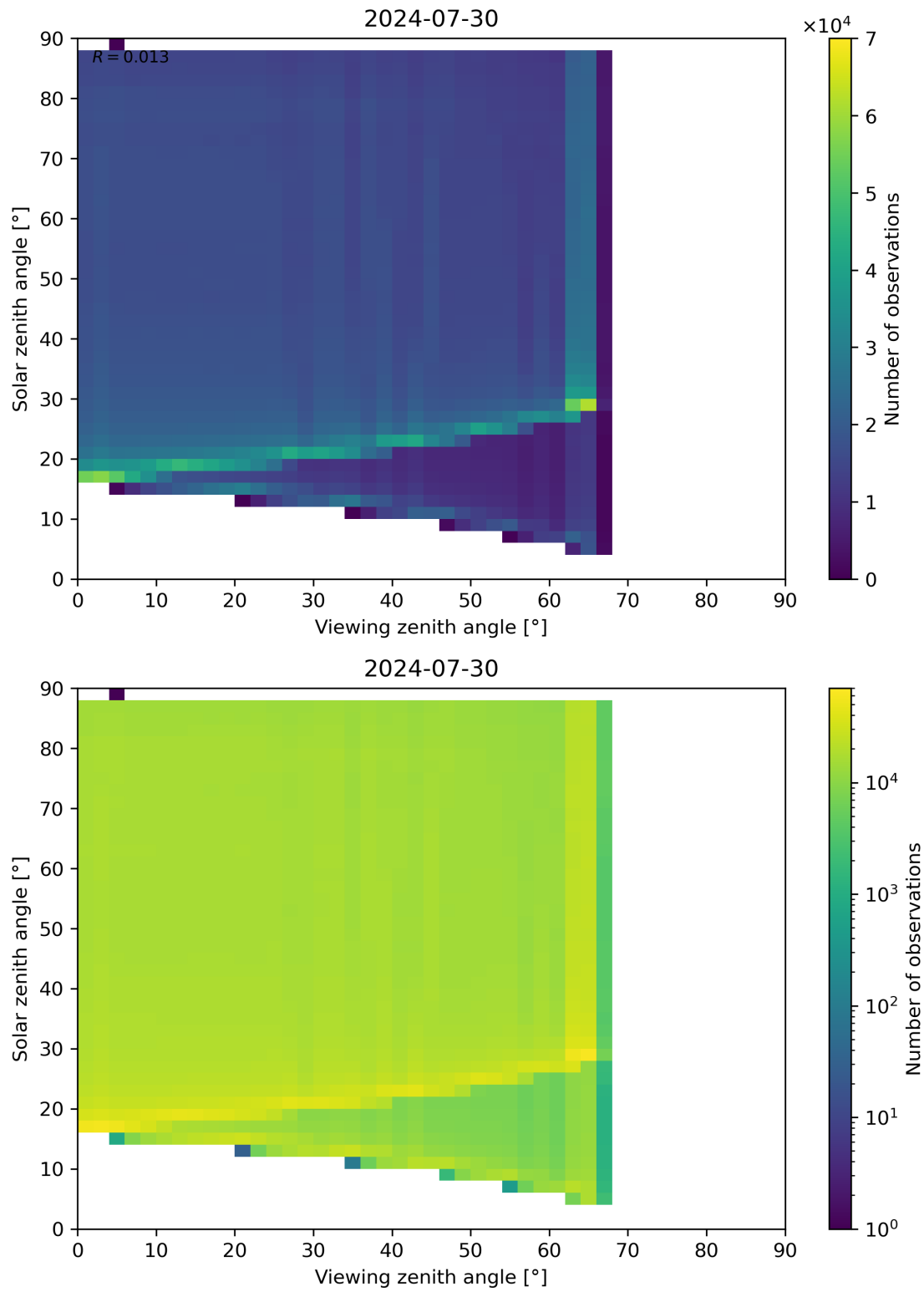
Figure 127: Scatter density plot of “Viewing zenith angle” against “Solar zenith angle” for 2024-07-29 to 2024-07-31.
