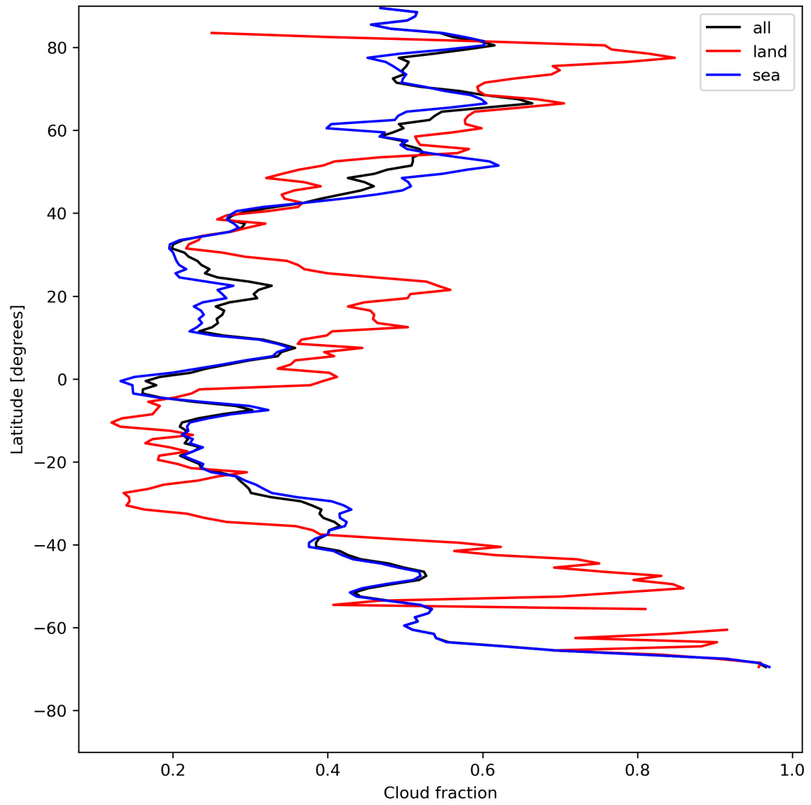
Figure 15: Zonal average of “Cloud fraction” for 2024-07-29 to 2024-07-31.
