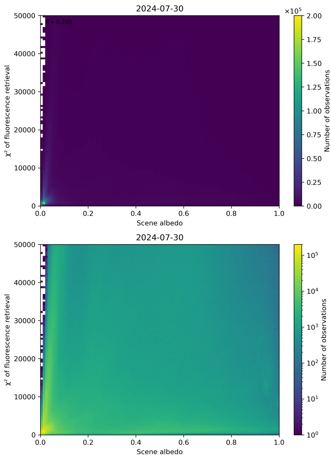
Figure 103: Scatter density plot of “Scene albedo” against “ \chi^2 of fluorescence retrieval” for 2024-07-29 to 2024-07-31.
