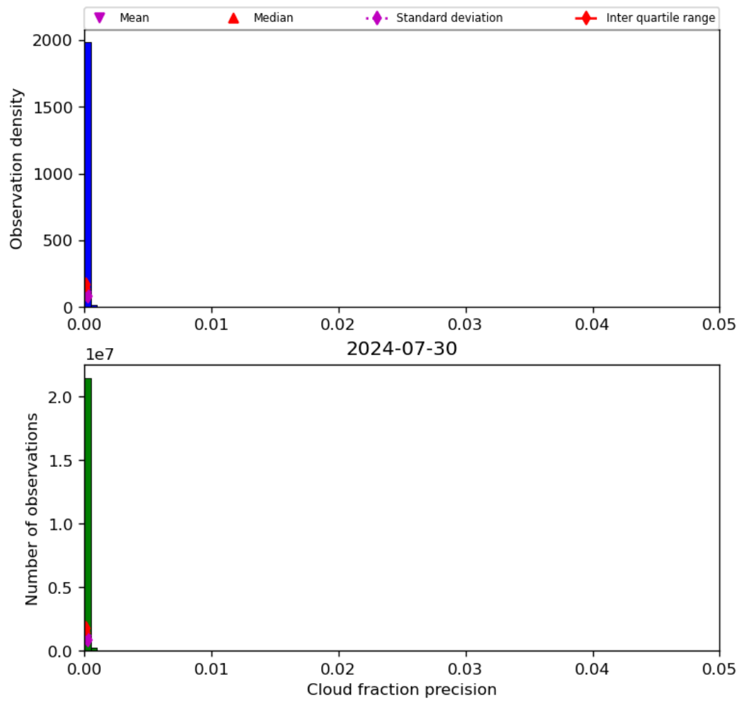
Figure 33: Histogram of “Cloud fraction precision” for 2024-07-29 to 2024-07-31
