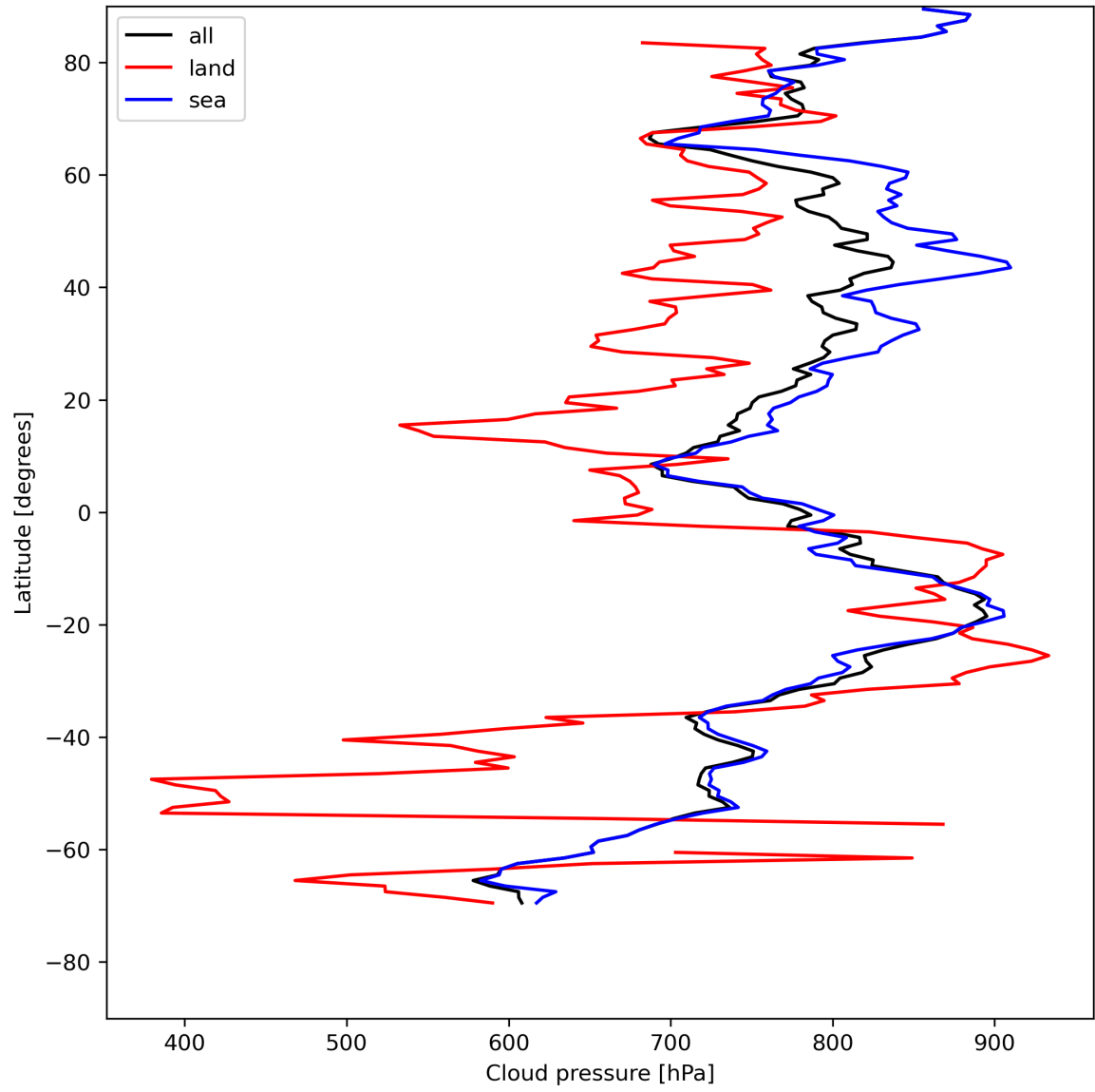
Figure 13: Zonal average of “Cloud pressure” for 2024-07-29 to 2024-07-31.
