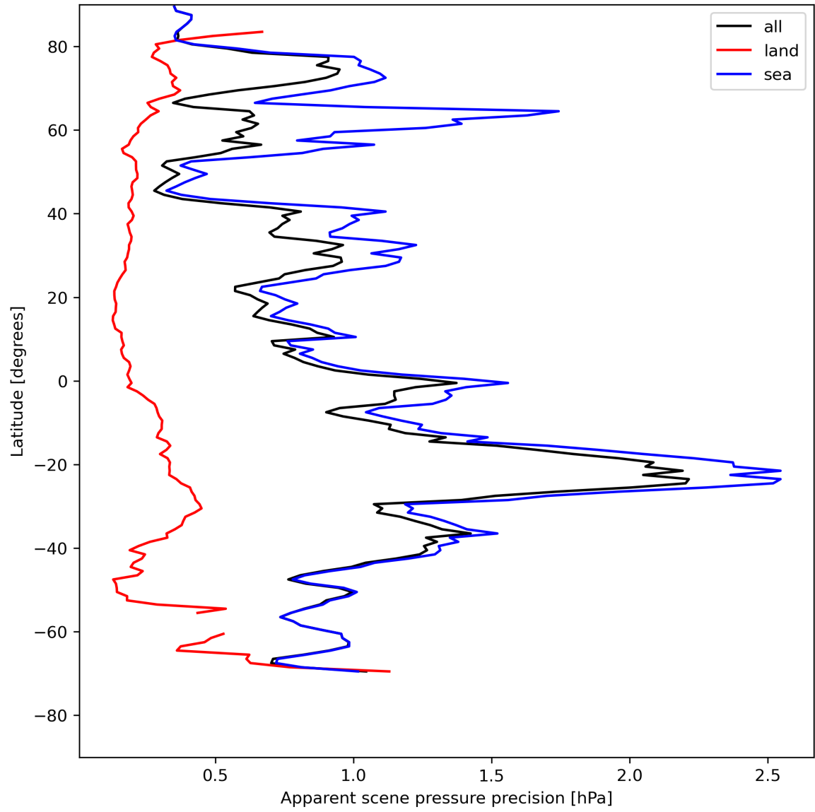
Figure 20: Zonal average of “Apparent scene pressure precision” for 2024-07-29 to 2024-07-31.
