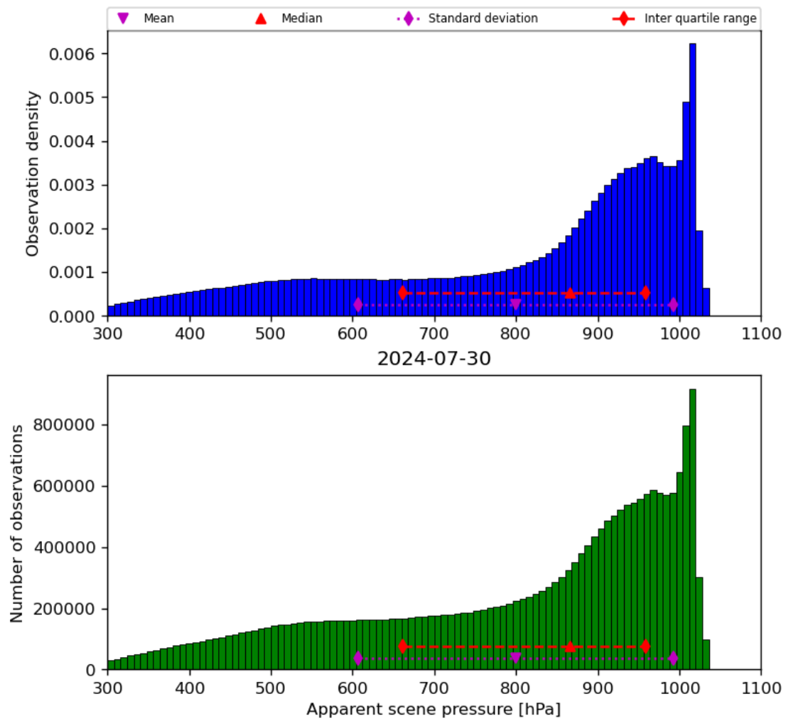
Figure 36: Histogram of “Apparent scene pressure” for 2024-07-29 to 2024-07-31
