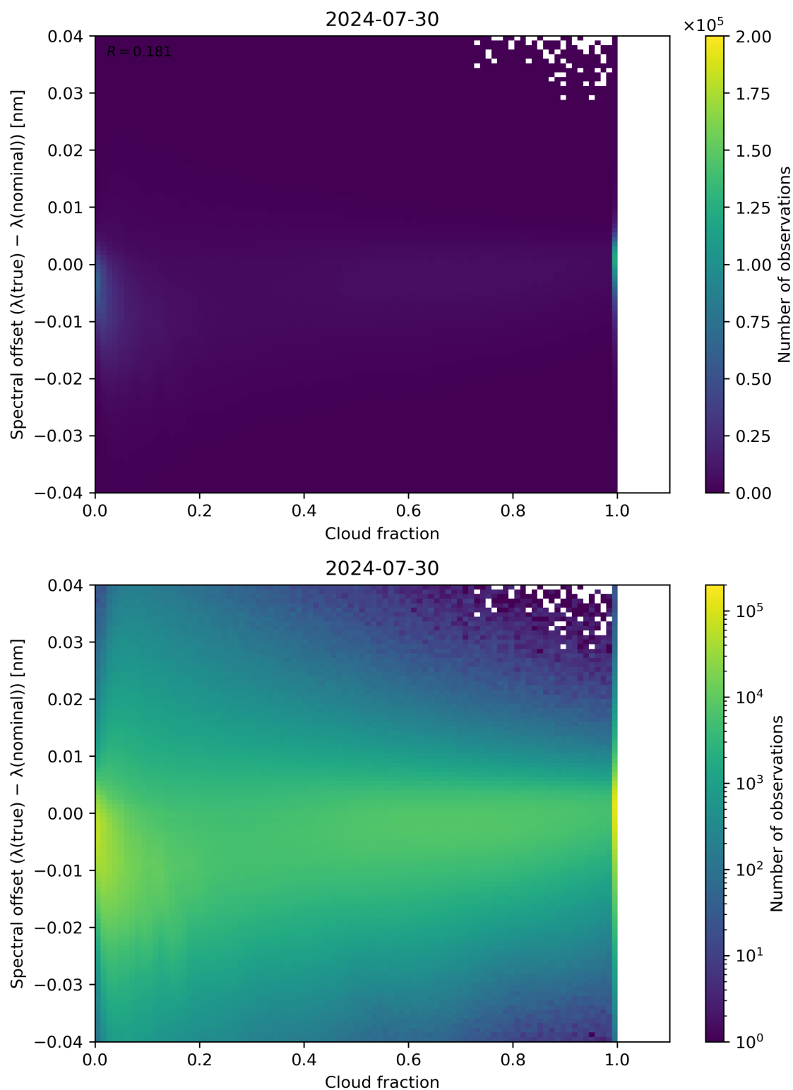
Figure 76: Scatter density plot of “Cloud fraction” against “Spectral offset ( \lambda(\text{true}) - \lambda(\text{nominal}) )” for 2024-07-29 to 2024-07-31.
