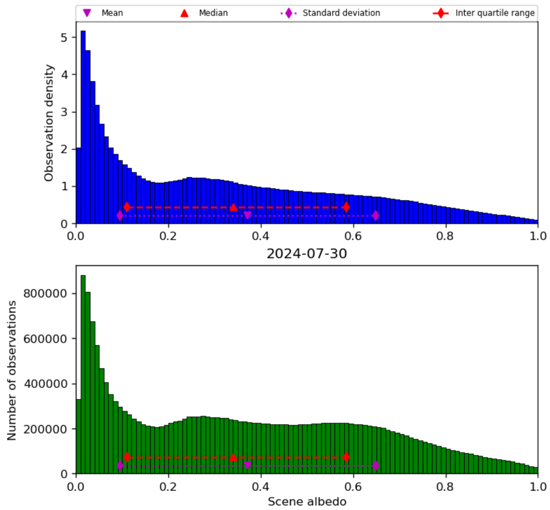
Figure 34: Histogram of “Scene albedo” for 2024-07-29 to 2024-07-31
