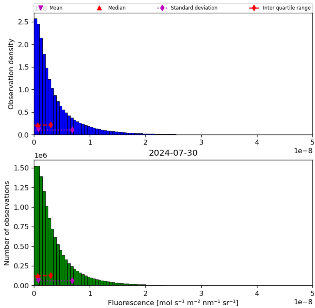
Figure 40: Histogram of “Fluorescence” for 2024-07-29 to 2024-07-31
