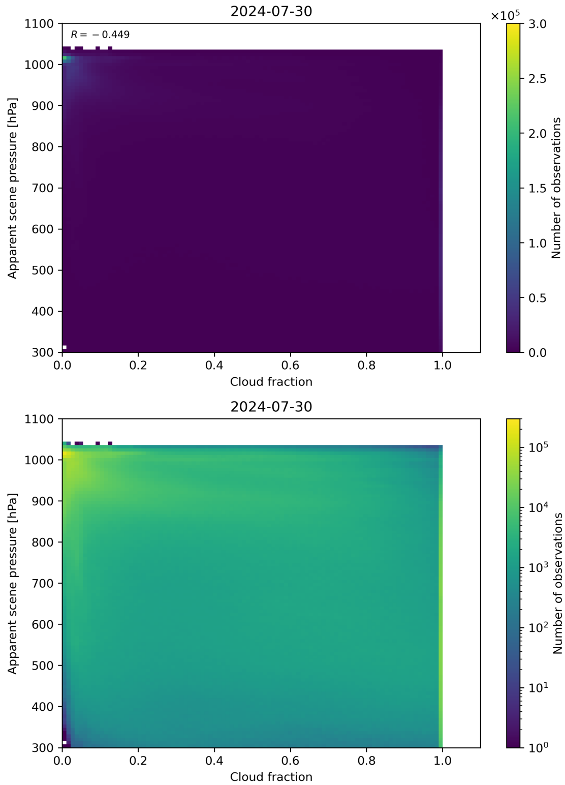
Figure 70: Scatter density plot of “Cloud fraction” against “Apparent scene pressure” for 2024-07-29 to 2024-07-31.
