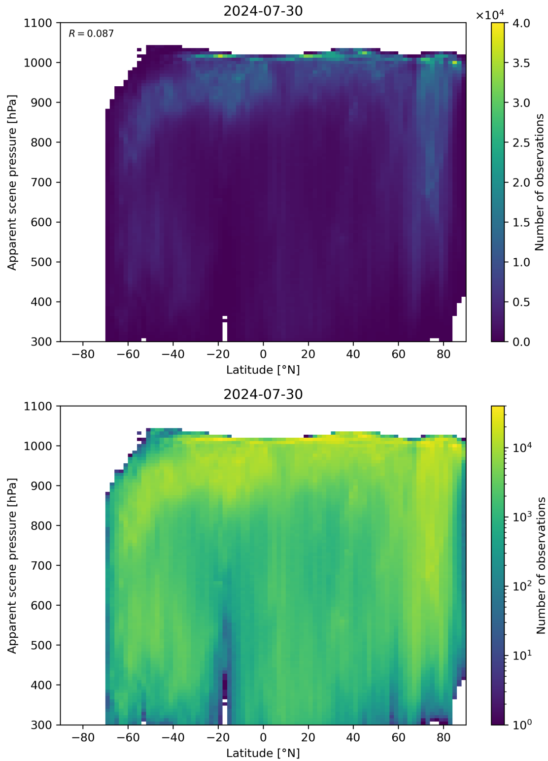
Figure 88: Scatter density plot of “Latitude” against “Apparent scene pressure” for 2024-07-29 to 2024-07-31.
