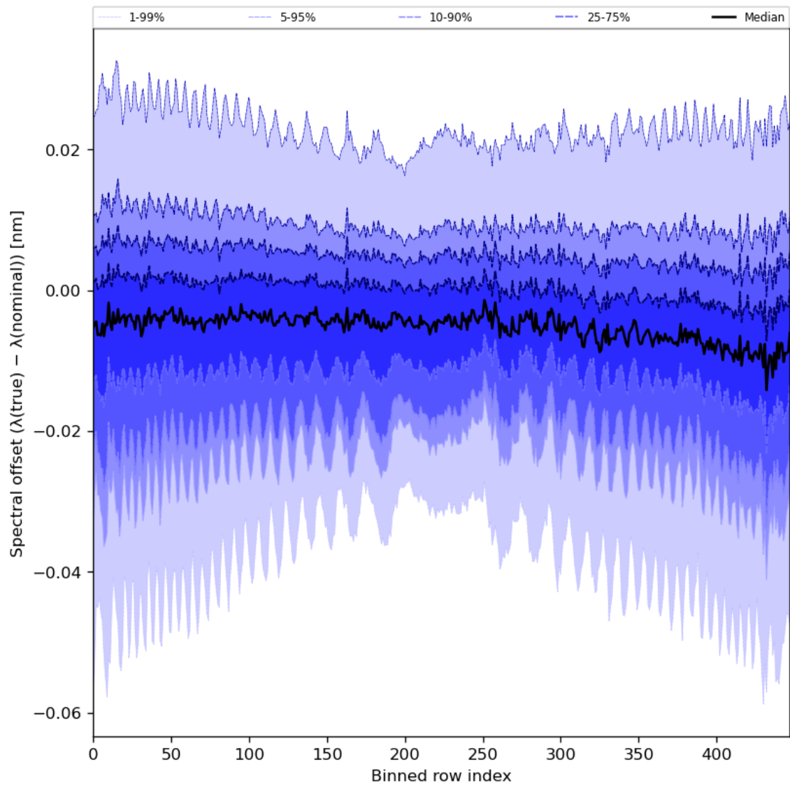
Figure 62: Along track statistics of “Spectral offset ( \lambda(\text{true}) - \lambda(\text{nominal}) )” for 2024-07-29 to 2024-07-31
