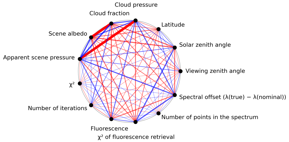
Figure 1: Map of correlation graph for 2024-07-29 to 2024-07-31.
