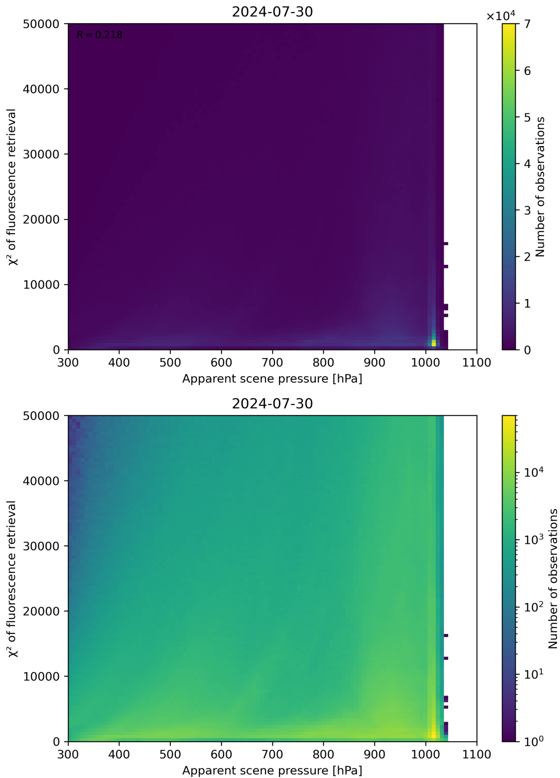
Figure 63: Scatter density plot of “Apparent scene pressure” against “ \chi^2 of fluorescence retrieval” for 2024-07-29 to 2024-07-31.
