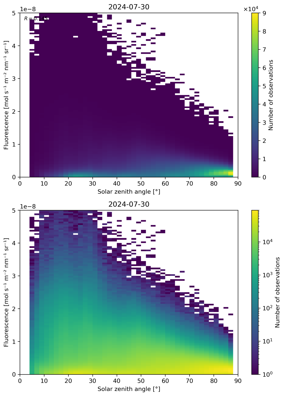
Figure 112: Scatter density plot of “Solar zenith angle” against “Fluorescence” for 2024-07-29 to 2024-07-31.
