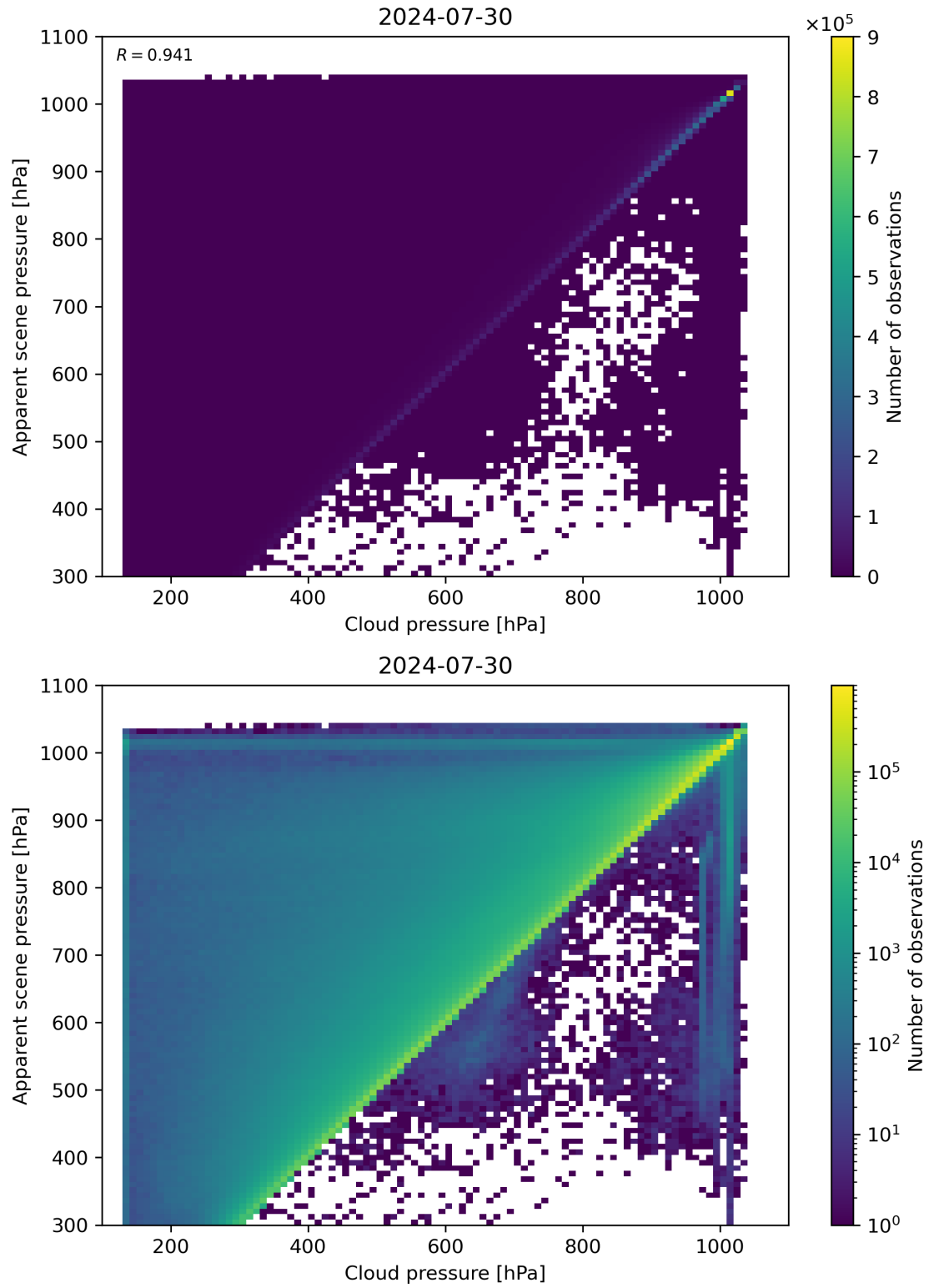
Figure 77: Scatter density plot of “Cloud pressure” against “Apparent scene pressure” for 2024-07-29 to 2024-07-31.
