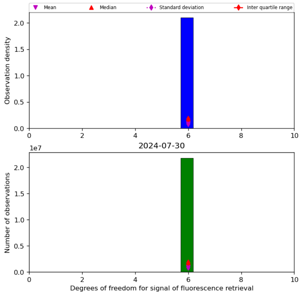
Figure 43: Histogram of “Degrees of freedom for signal of fluorescence retrieval” for 2024-07-29 to 2024-07-31
