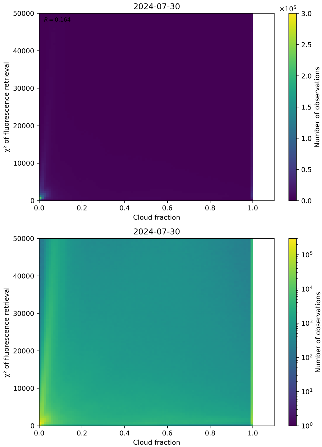
Figure 71: Scatter density plot of “Cloud fraction” against “ \chi^2 of fluorescence retrieval” for 2024-07-29 to 2024-07-31.
