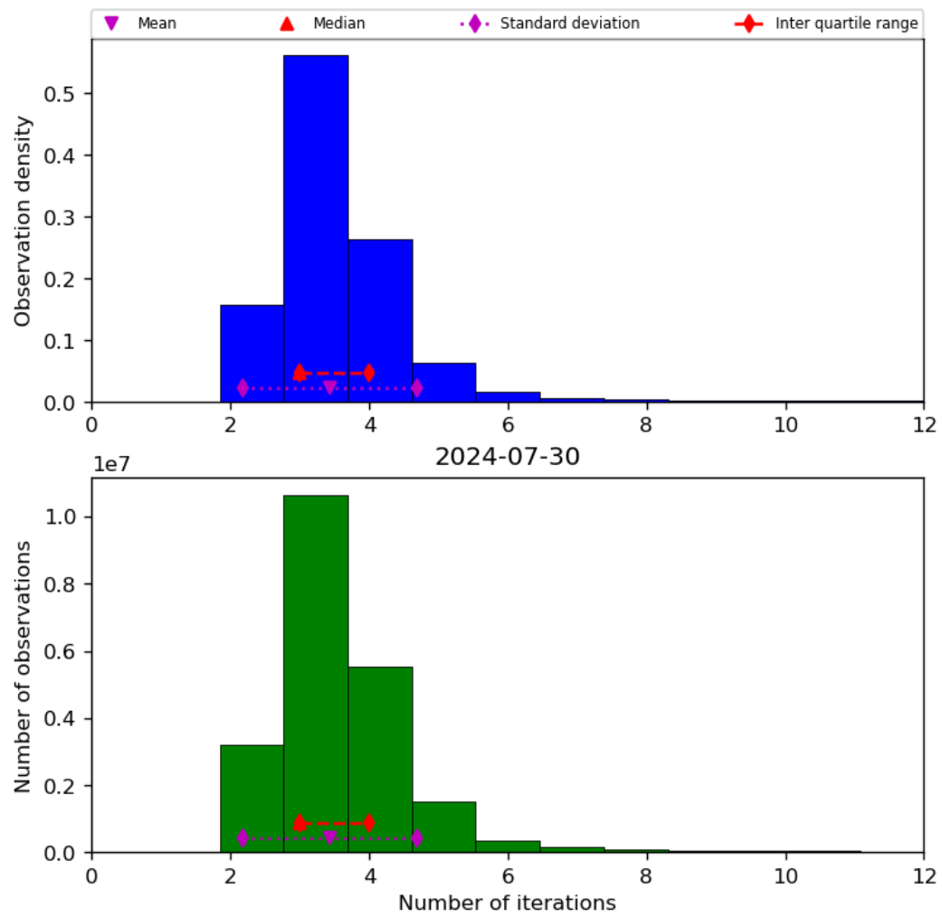
Figure 39: Histogram of “Number of iterations” for 2024-07-29 to 2024-07-31
