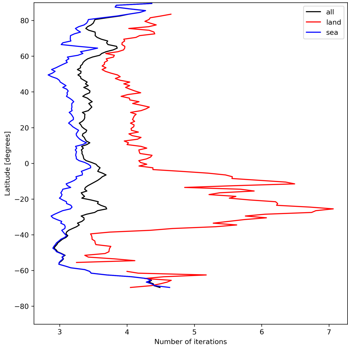
Figure 22: Zonal average of “Number of iterations” for 2024-07-29 to 2024-07-31.
