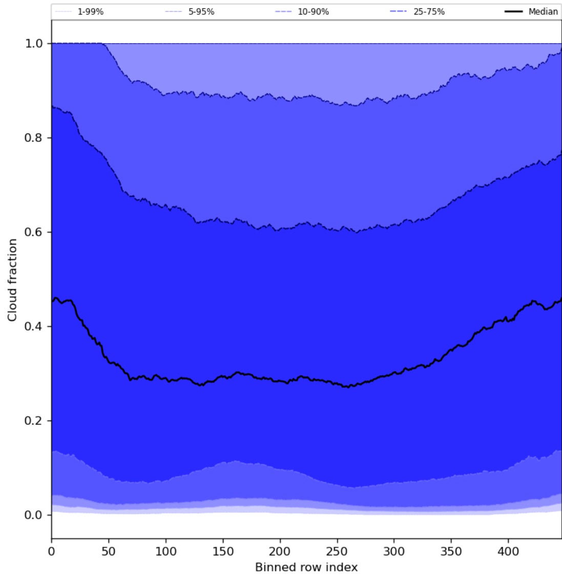
Figure 49: Along track statistics of “Cloud fraction” for 2024-07-29 to 2024-07-31
