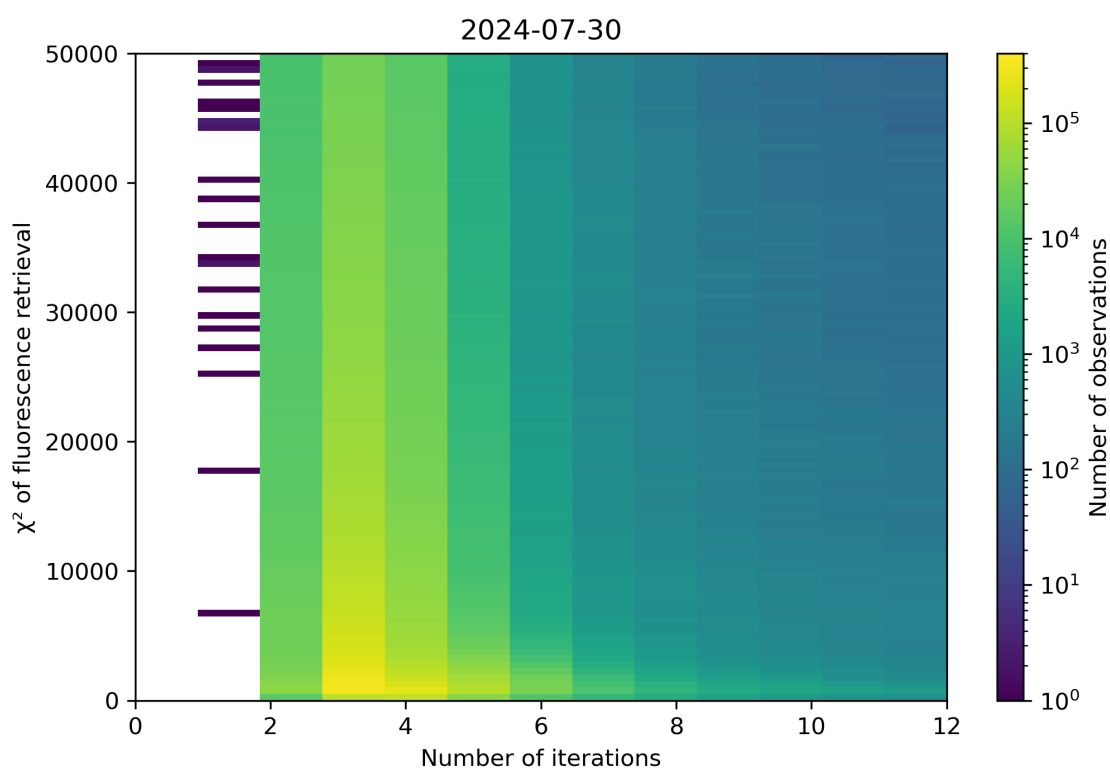
Figure 97: Scatter density plot of “Number of iterations” against “ \chi^2 of fluorescence retrieval” for 2024-07-29 to 2024-07-31.
