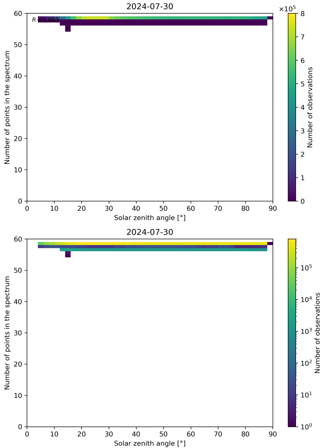
Figure 115: Scatter density plot of “Solar zenith angle” against “Number of points in the spectrum” for 2024-07-29 to 2024-07-31.
