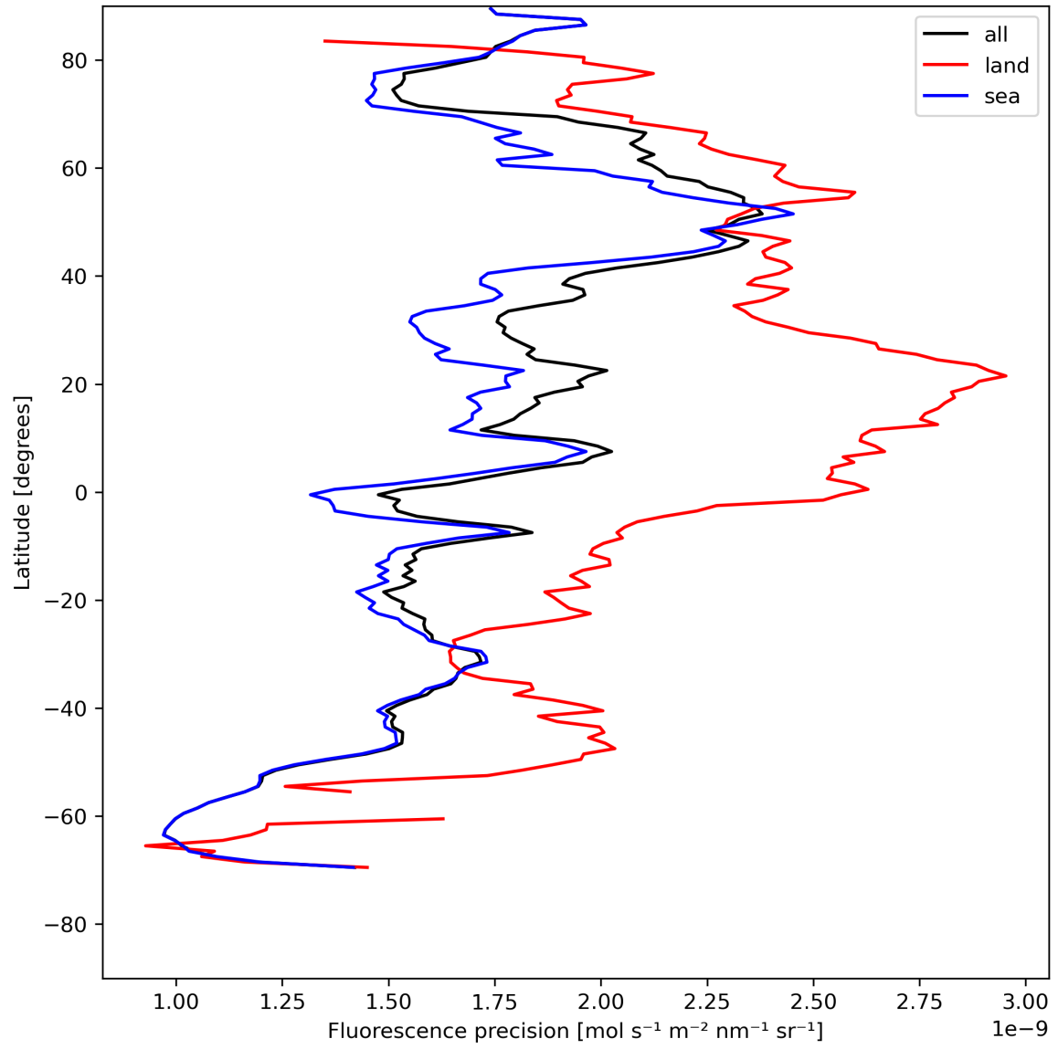
Figure 24: Zonal average of “Fluorescence precision” for 2024-07-29 to 2024-07-31.
