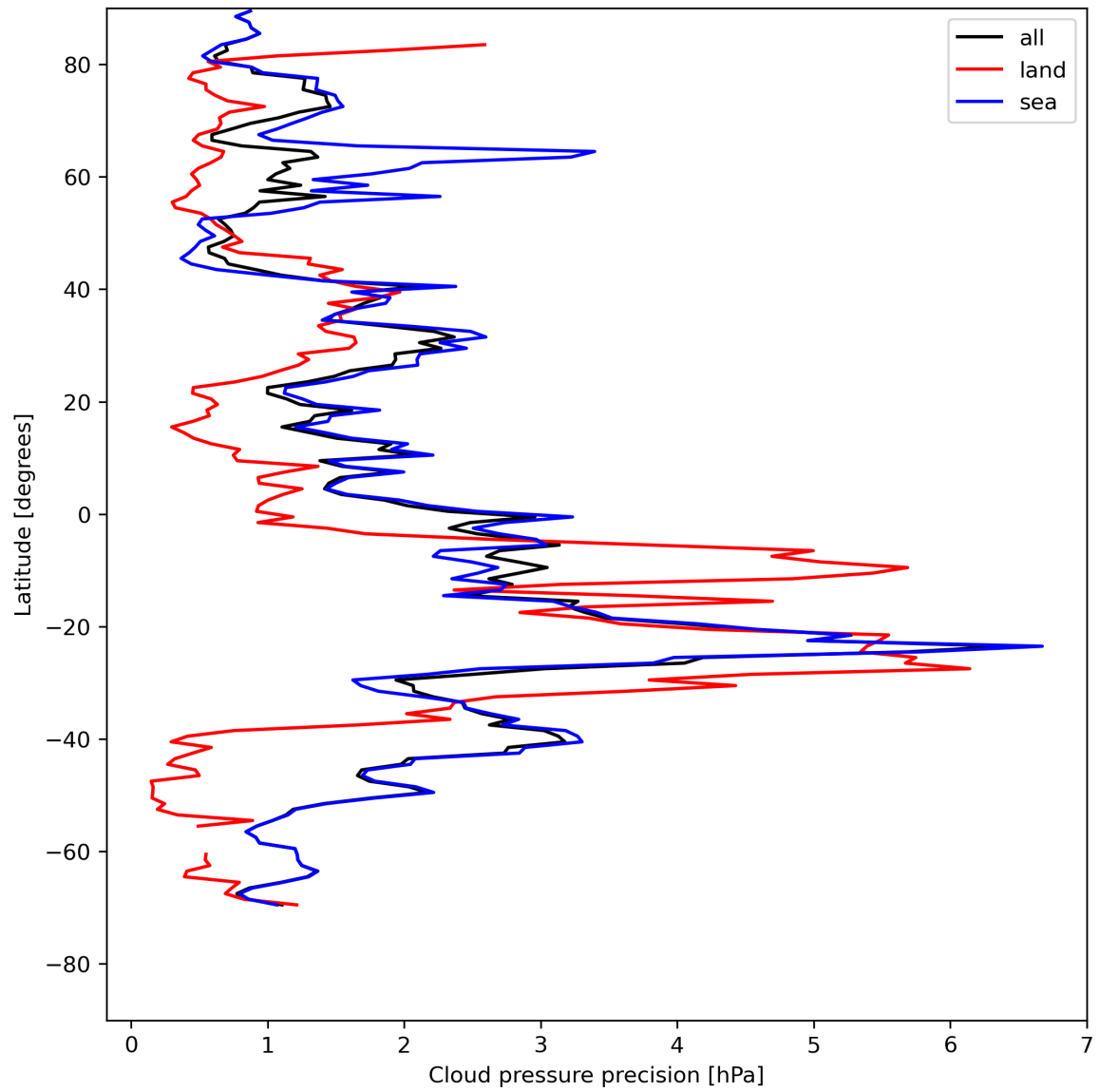
Figure 14: Zonal average of “Cloud pressure precision” for 2024-07-29 to 2024-07-31.
