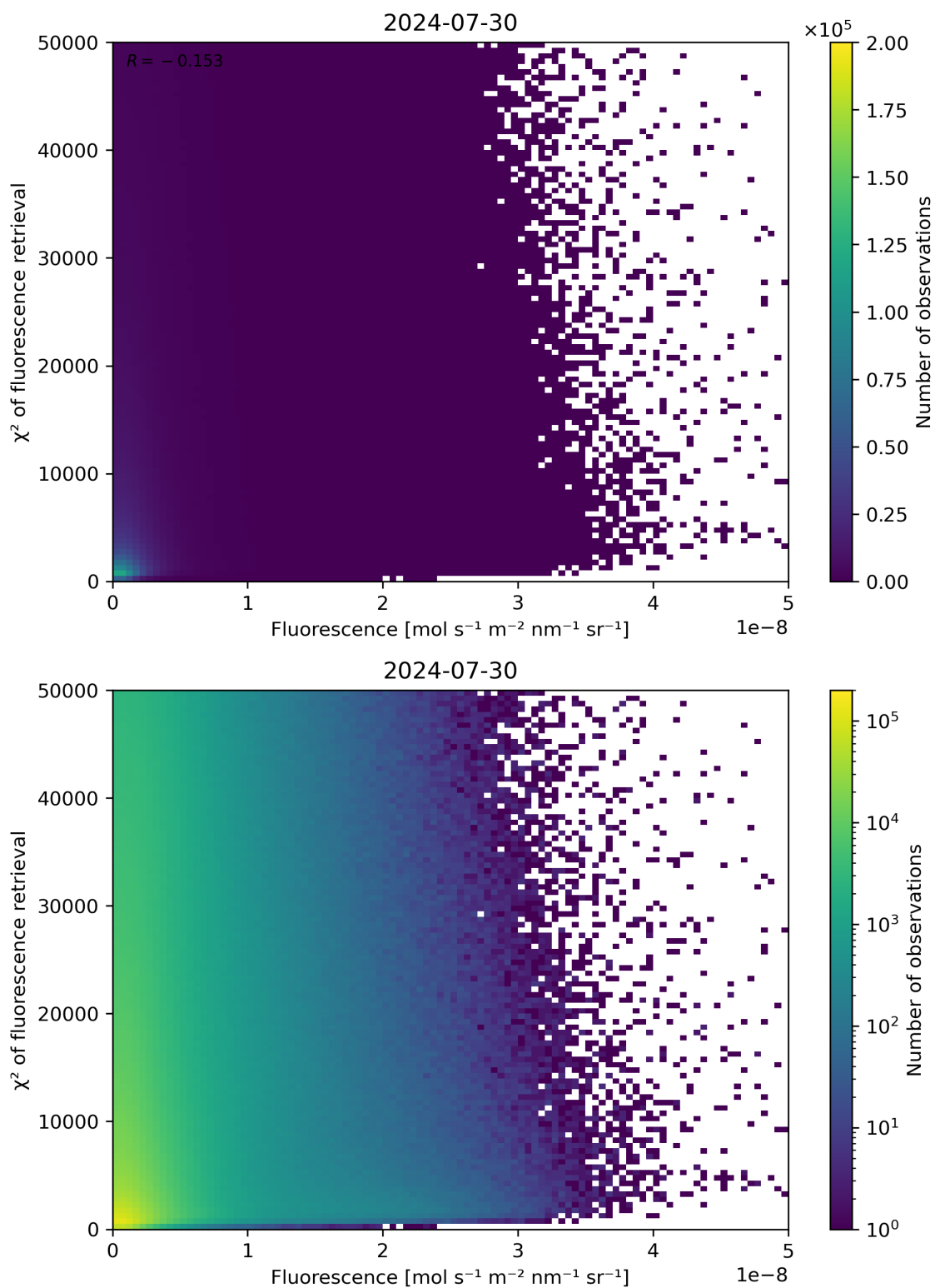
Figure 85: Scatter density plot of “Fluorescence” against “ \chi^2 of fluorescence retrieval” for 2024-07-29 to 2024-07-31.
