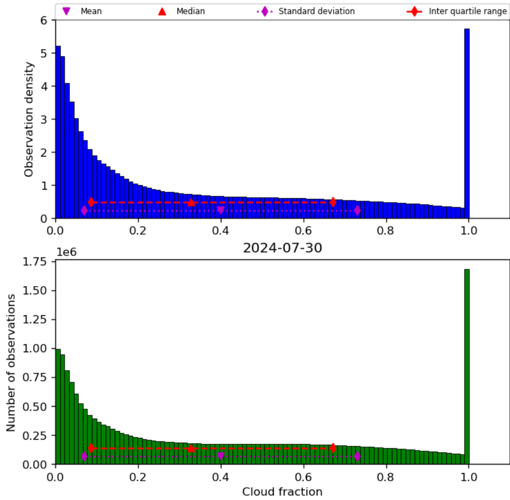
Figure 32: Histogram of “Cloud fraction” for 2024-07-29 to 2024-07-31
