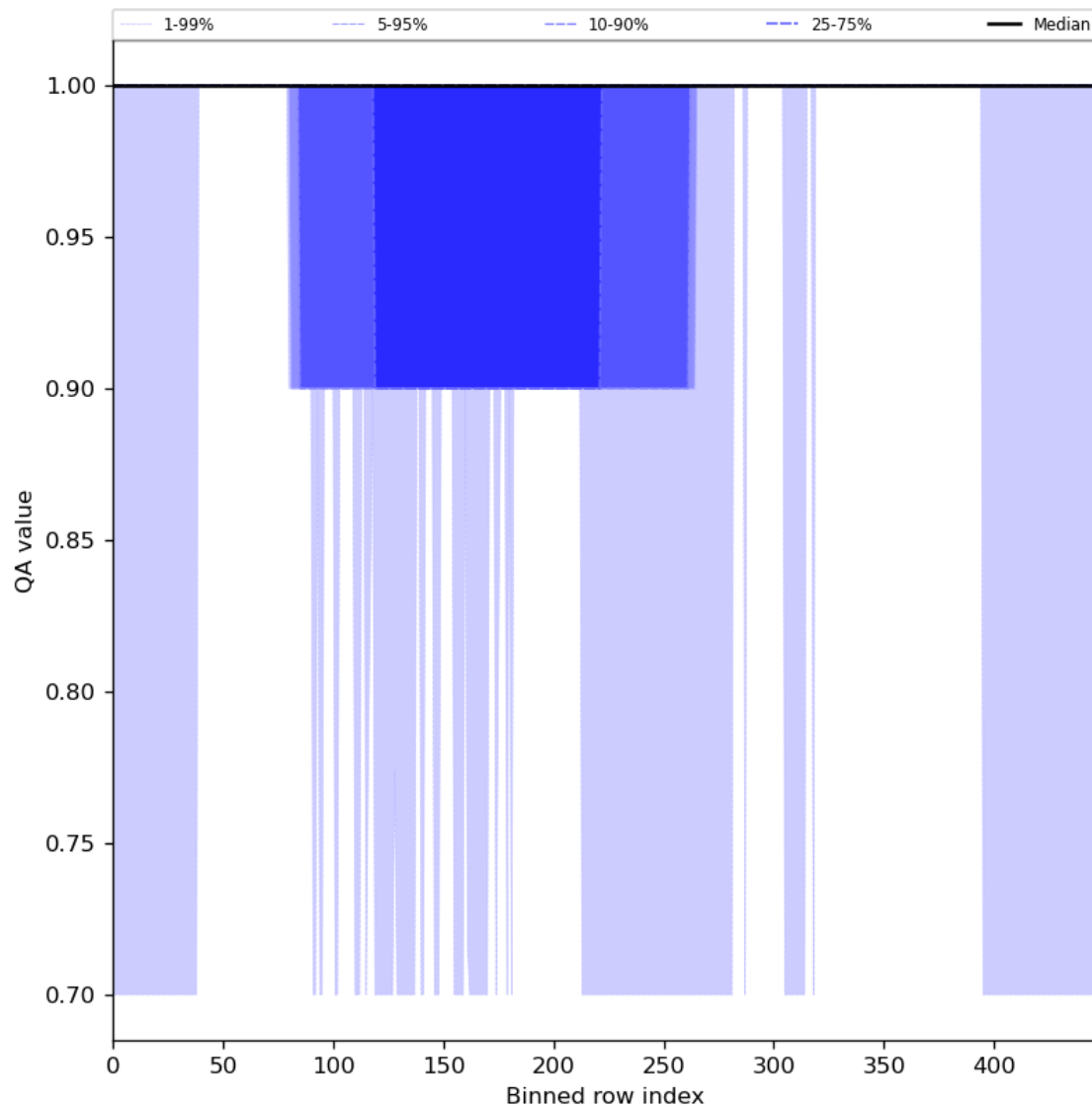
Figure 46: Along track statistics of “QA value” for 2024-07-29 to 2024-07-31
