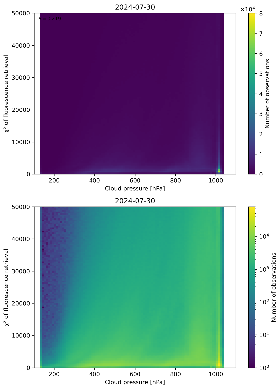
Figure 78: Scatter density plot of “Cloud pressure” against “ \chi^2 of fluorescence retrieval” for 2024-07-29 to 2024-07-31.
