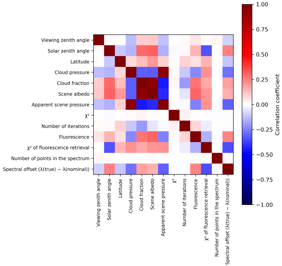
Figure 2: Map of correlation matrix for 2024-07-29 to 2024-07-31.
