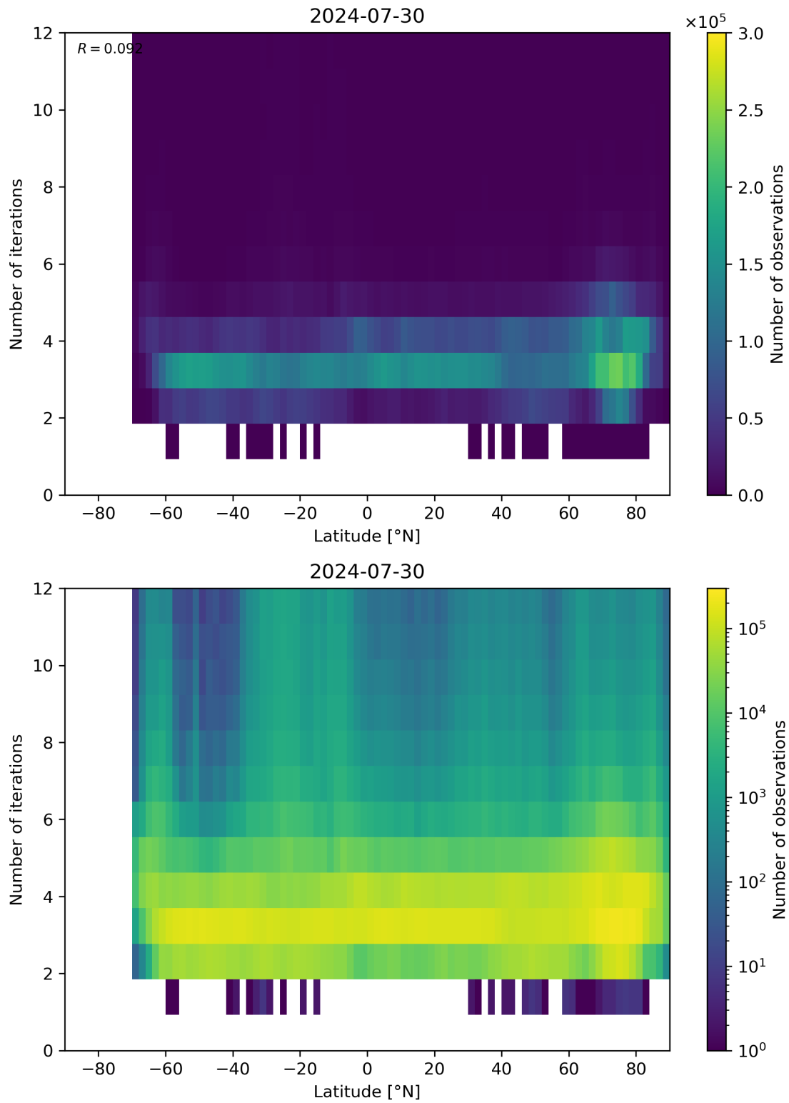
Figure 93: Scatter density plot of “Latitude” against “Number of iterations” for 2024-07-29 to 2024-07-31.
