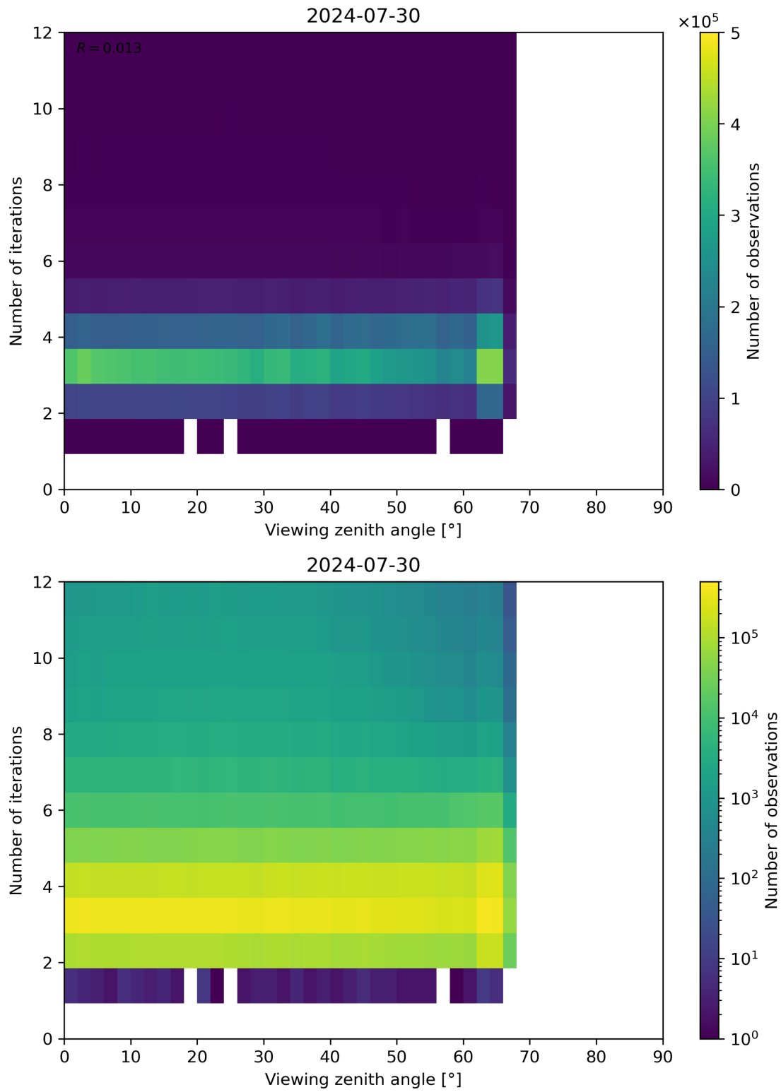
Figure 124: Scatter density plot of “Viewing zenith angle” against “Number of iterations” for 2024-07-29 to 2024-07-31.
