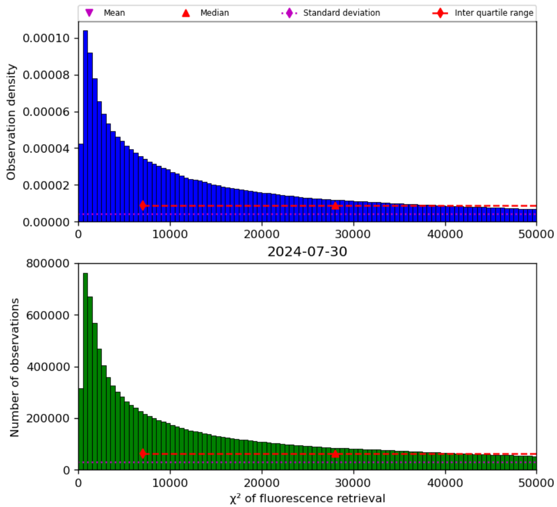
Figure 42: Histogram of “ \chi^2 of fluorescence retrieval” for 2024-07-29 to 2024-07-31
