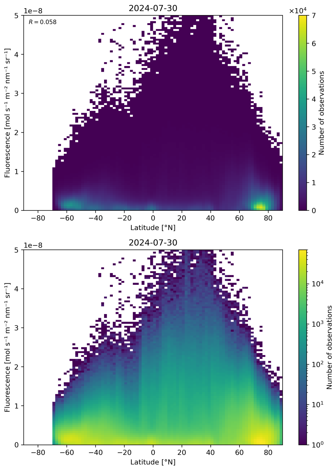
Figure 92: Scatter density plot of “Latitude” against “Fluorescence” for 2024-07-29 to 2024-07-31.
