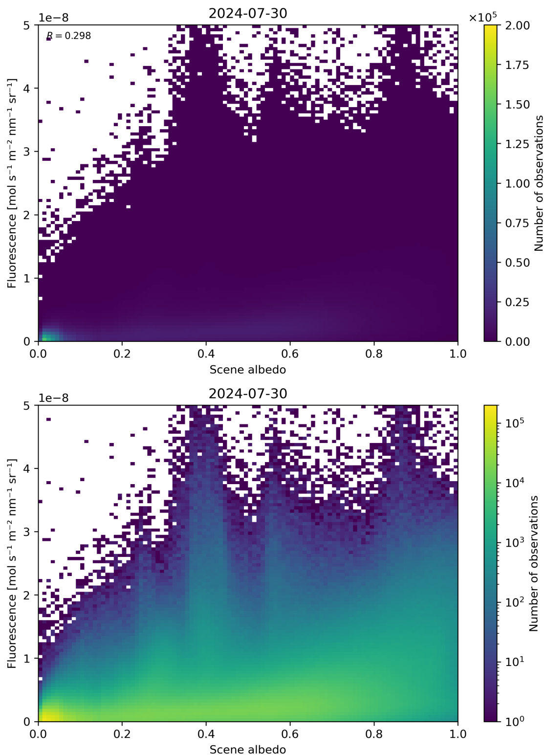
Figure 104: Scatter density plot of “Scene albedo” against “Fluorescence” for 2024-07-29 to 2024-07-31.
