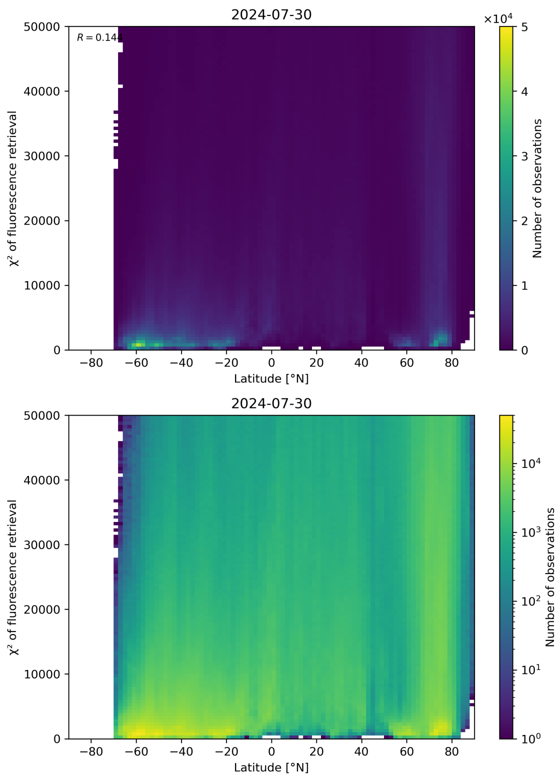
Figure 89: Scatter density plot of “Latitude” against “ \chi^2 of fluorescence retrieval” for 2024-07-29 to 2024-07-31.
