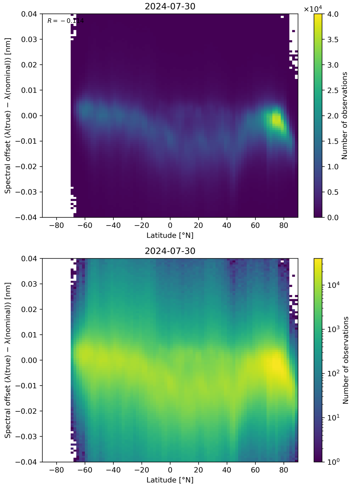
Figure 96: Scatter density plot of “Latitude” against “Spectral offset ( \lambda(\text{true}) - \lambda(\text{nominal}) )” for 2024-07-29 to 2024-07-31.
