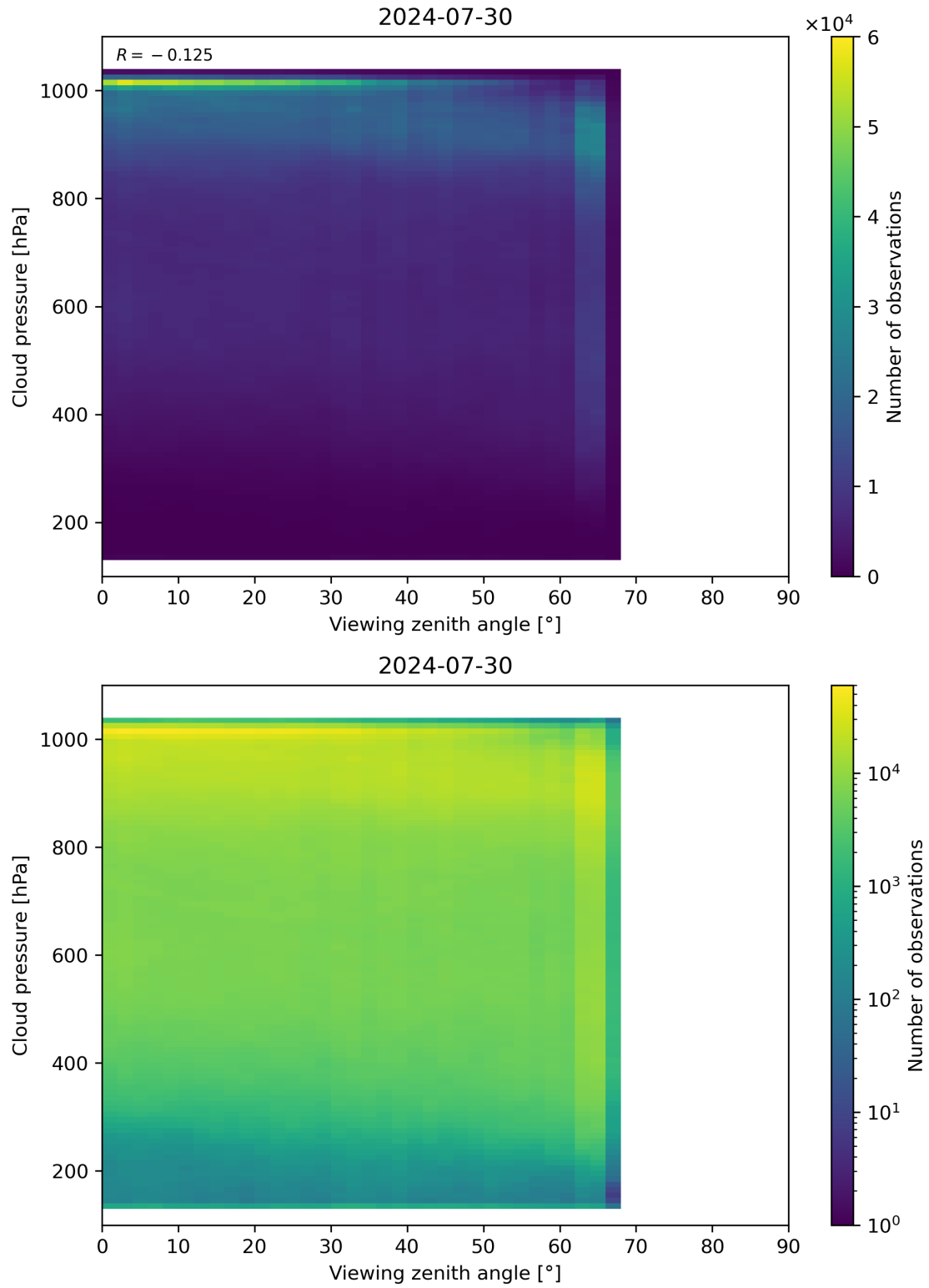
Figure 121: Scatter density plot of “Viewing zenith angle” against “Cloud pressure” for 2024-07-29 to 2024-07-31.
