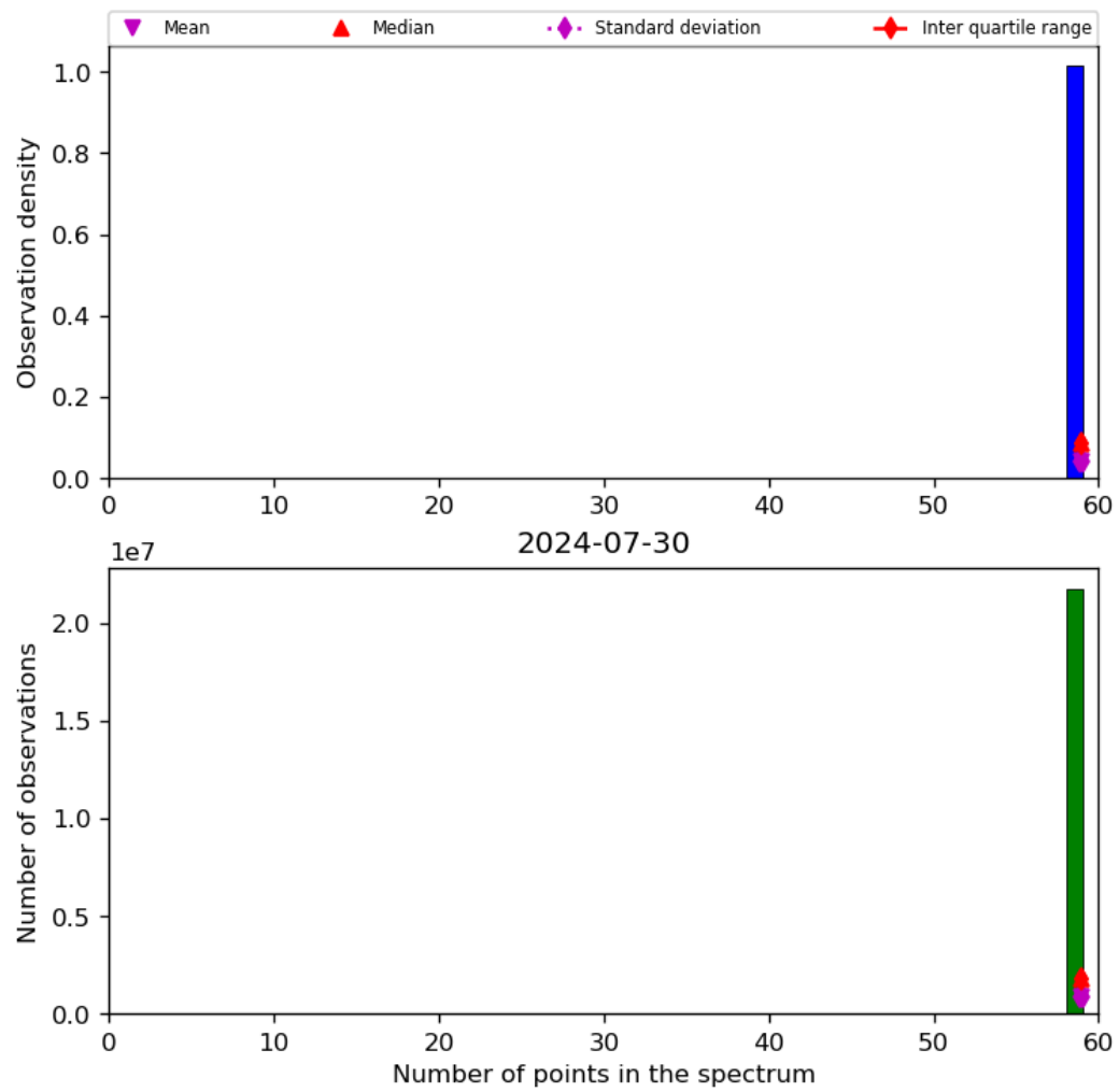
Figure 44: Histogram of “Number of points in the spectrum” for 2024-07-29 to 2024-07-31
