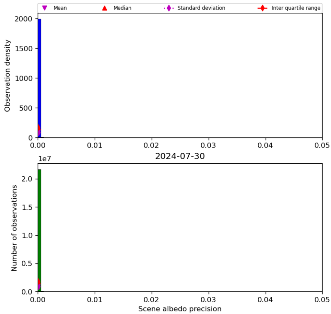
Figure 35: Histogram of “Scene albedo precision” for 2024-07-29 to 2024-07-31
