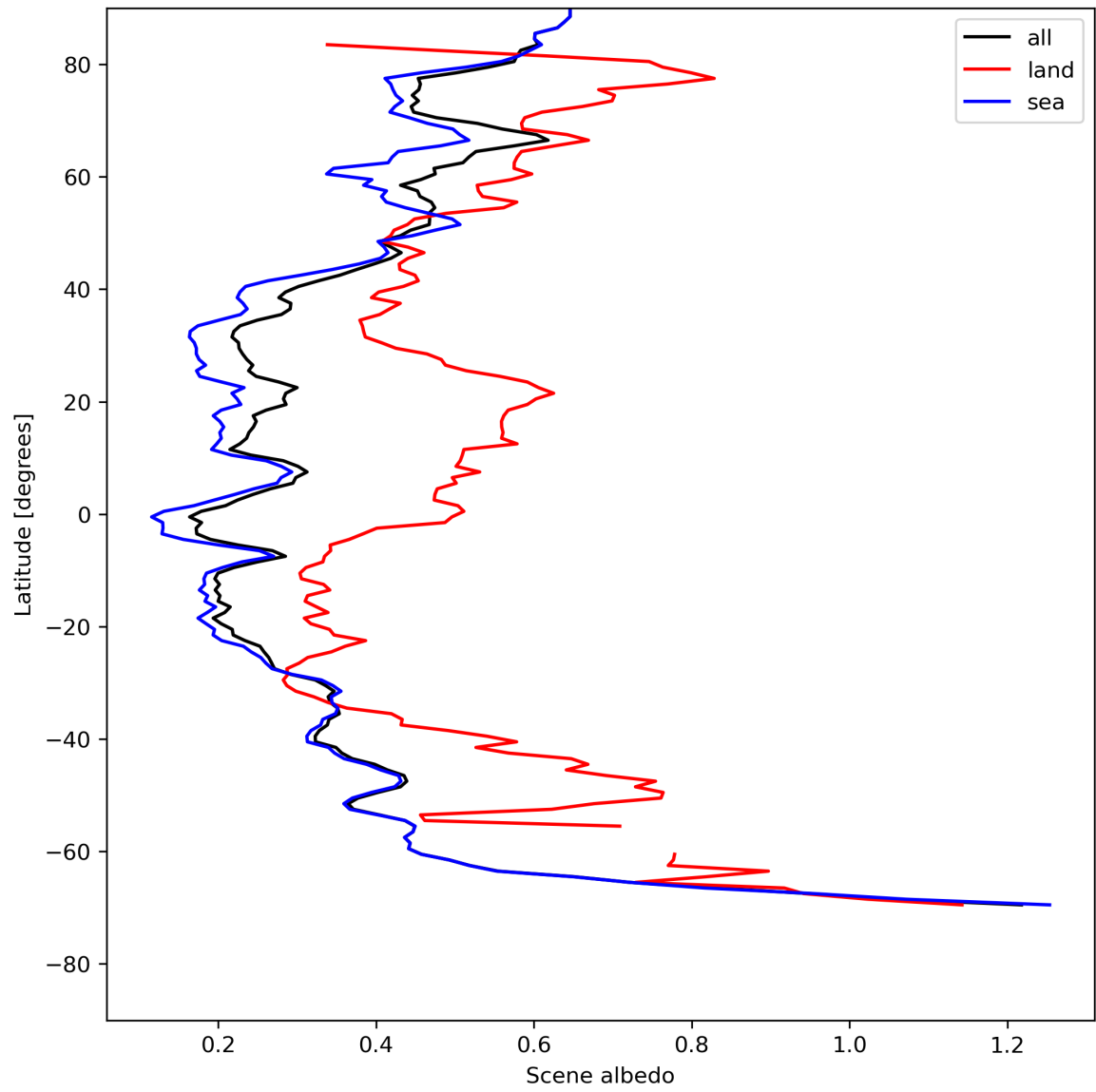
Figure 17: Zonal average of “Scene albedo” for 2024-07-29 to 2024-07-31.
