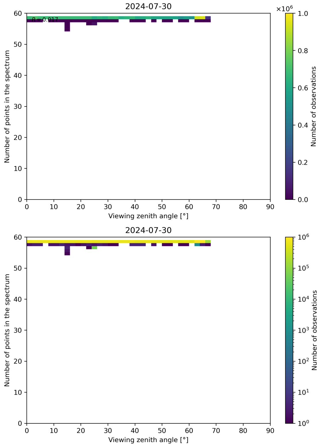
Figure 125: Scatter density plot of “Viewing zenith angle” against “Number of points in the spectrum” for 2024-07-29 to 2024-07-31.
