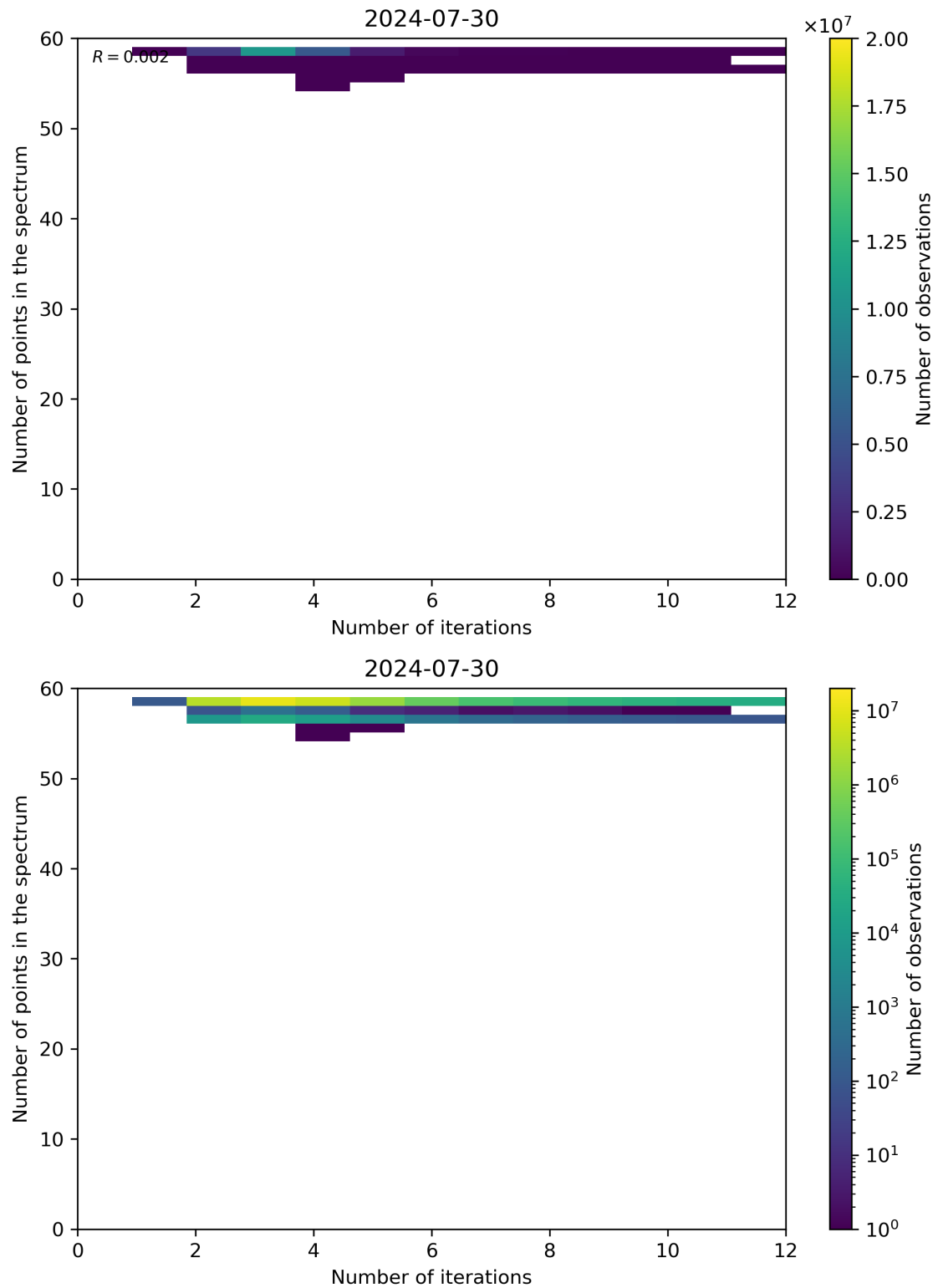
Figure 99: Scatter density plot of “Number of iterations” against “Number of points in the spectrum” for 2024-07-29 to 2024-07-31.
