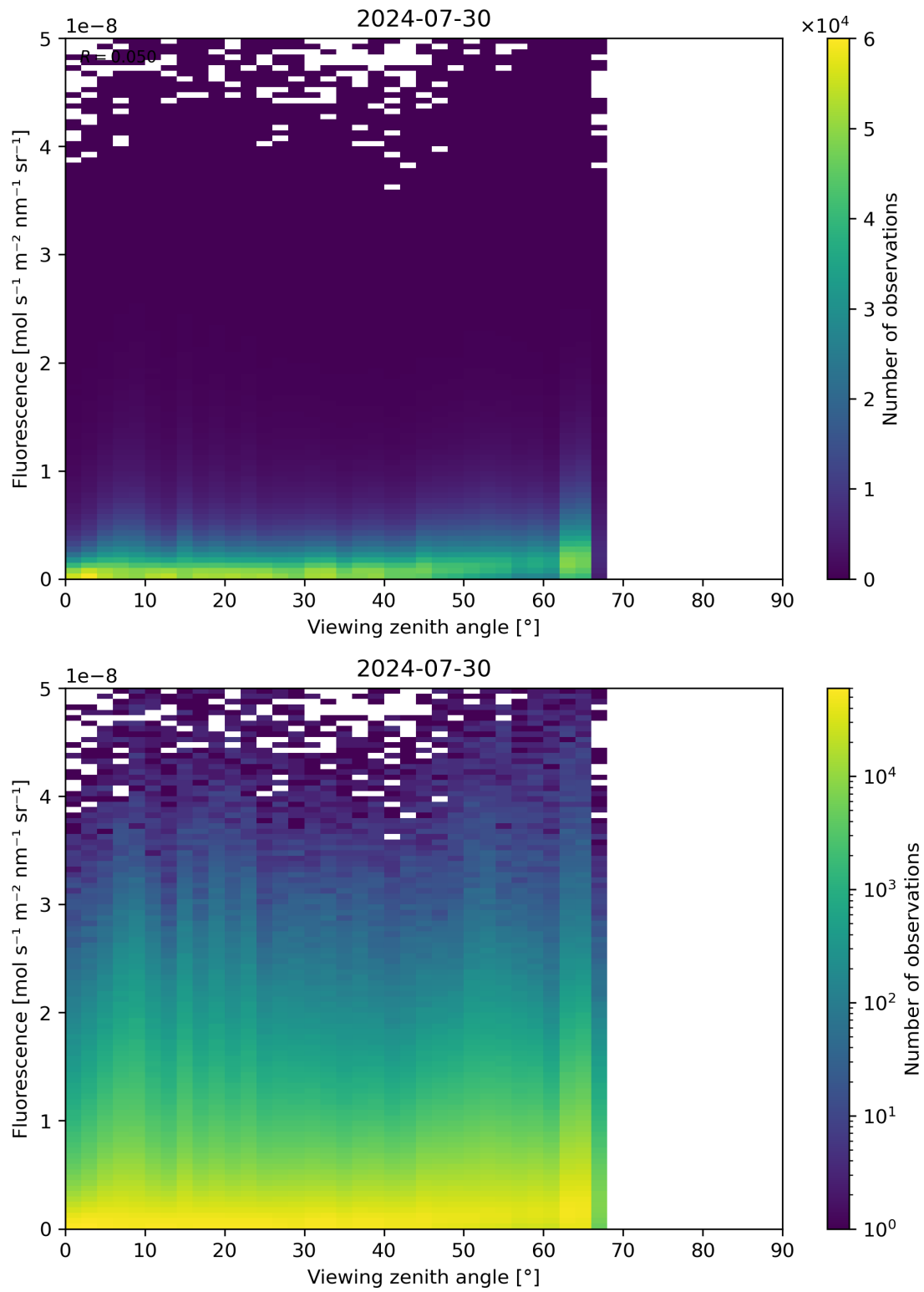
Figure 122: Scatter density plot of “Viewing zenith angle” against “Fluorescence” for 2024-07-29 to 2024-07-31.
