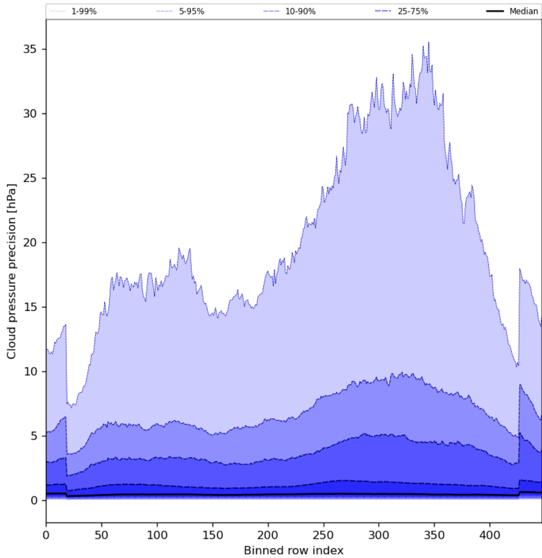
Figure 48: Along track statistics of “Cloud pressure precision” for 2024-07-29 to 2024-07-31
