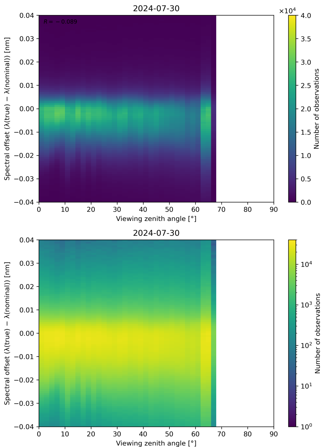
Figure 128: Scatter density plot of “Viewing zenith angle” against “Spectral offset ( \lambda(\text{true}) - \lambda(\text{nominal}) )” for 2024-07-29 to 2024-07-31.
