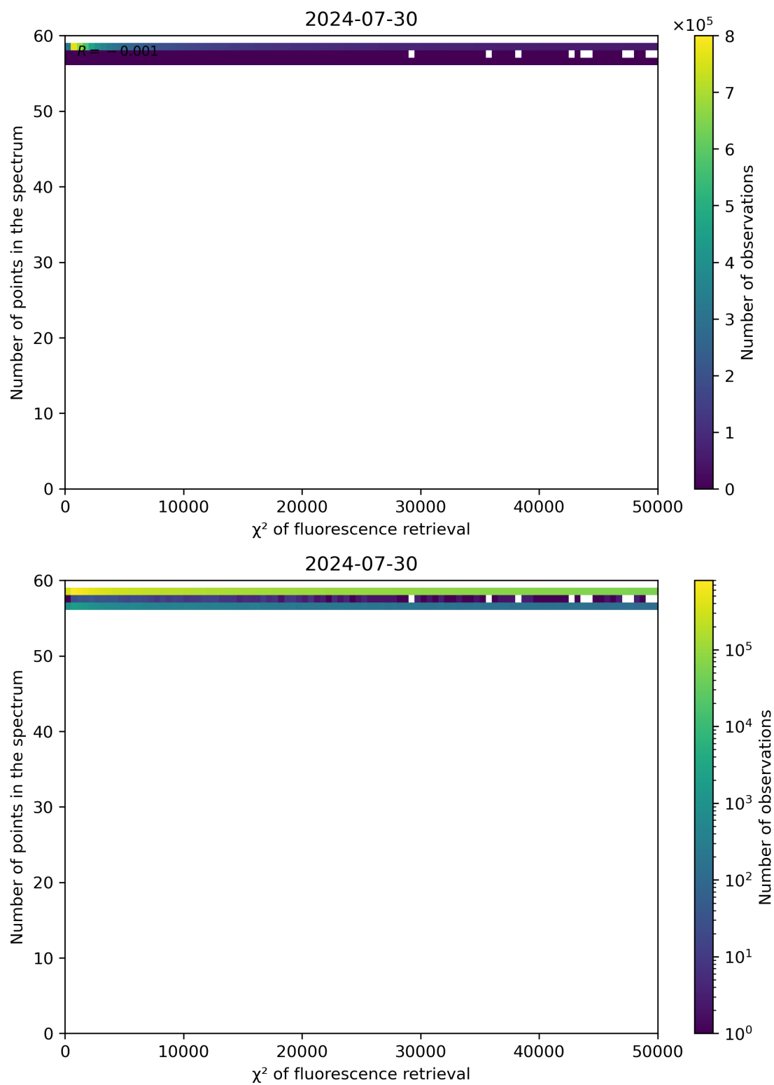
Figure 68: Scatter density plot of " \chi^2 of fluorescence retrieval" against "Number of points in the spectrum" for 2024-07-29 to 2024-07-31.
