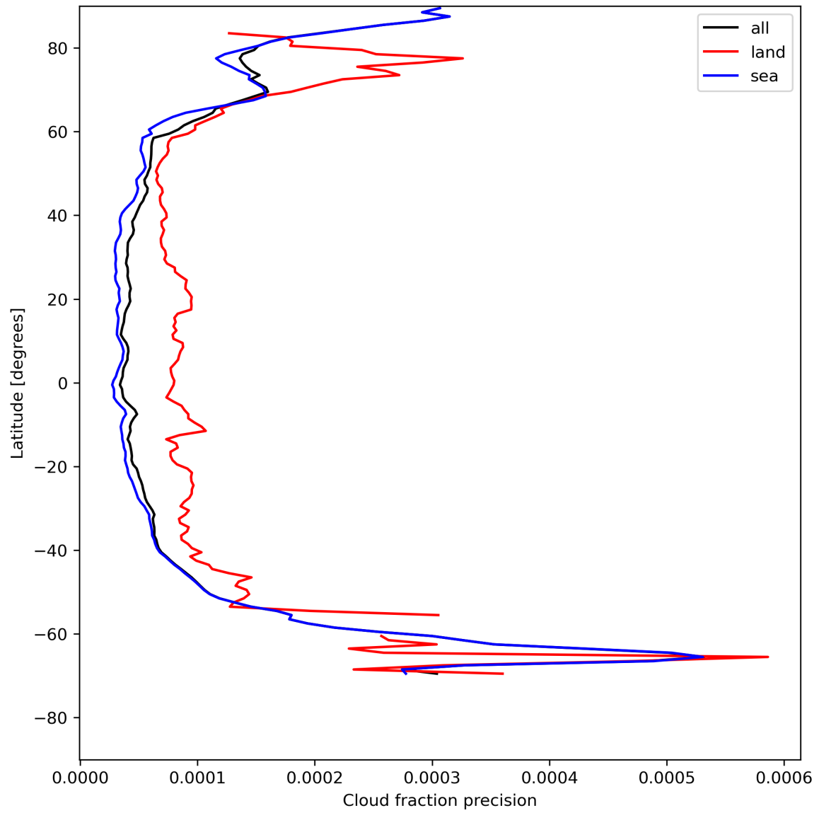
Figure 16: Zonal average of “Cloud fraction precision” for 2024-07-29 to 2024-07-31.
