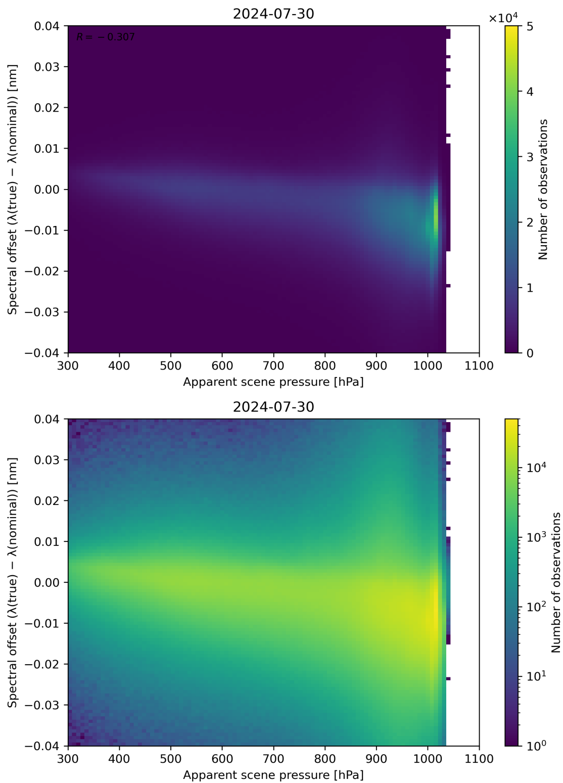
Figure 67: Scatter density plot of “Apparent scene pressure” against “Spectral offset ( \lambda(\text{true}) - \lambda(\text{nominal}) )” for 2024-07-29 to 2024-07-31.
