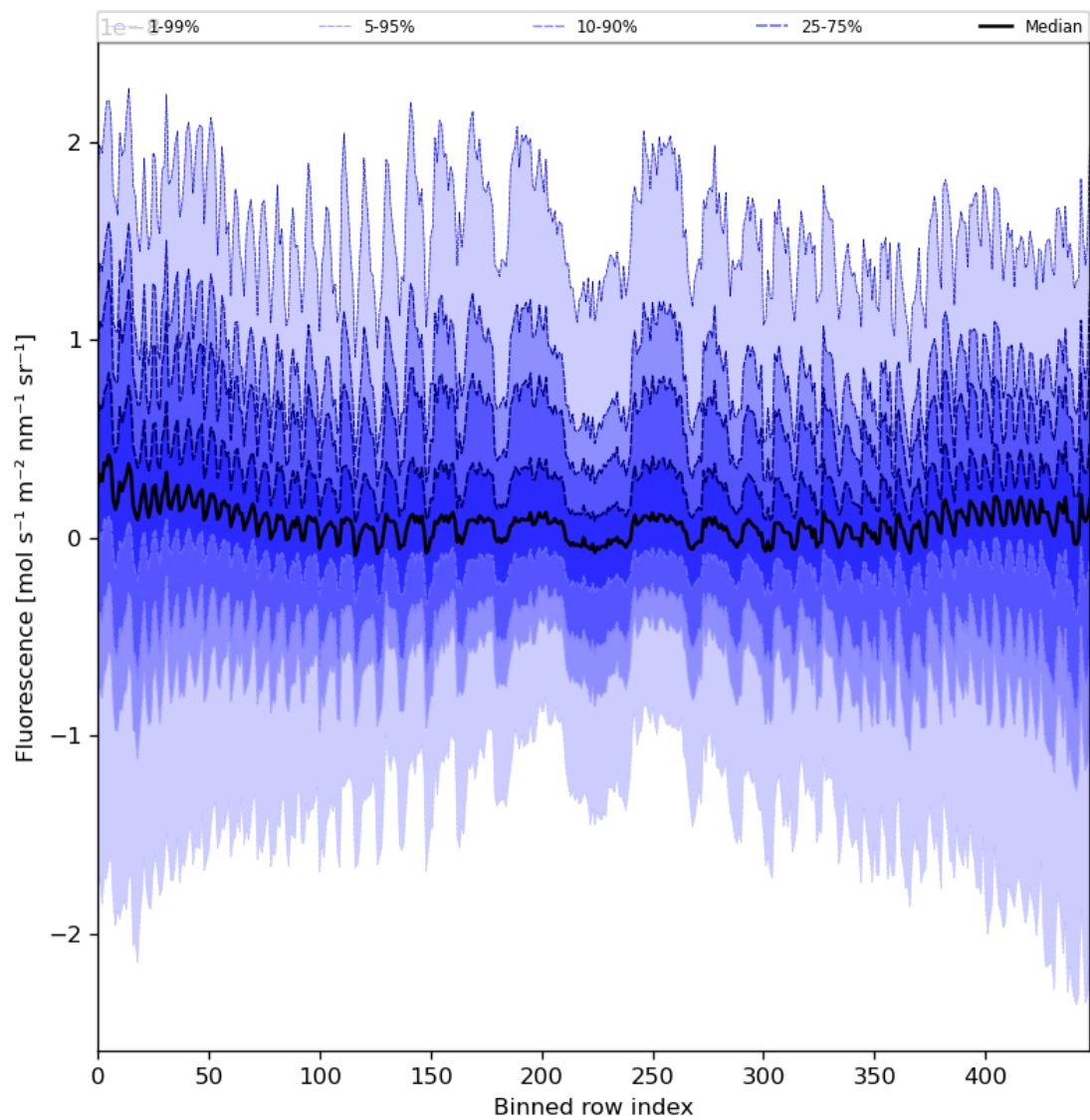
Figure 57: Along track statistics of “Fluorescence” for 2024-07-29 to 2024-07-31
