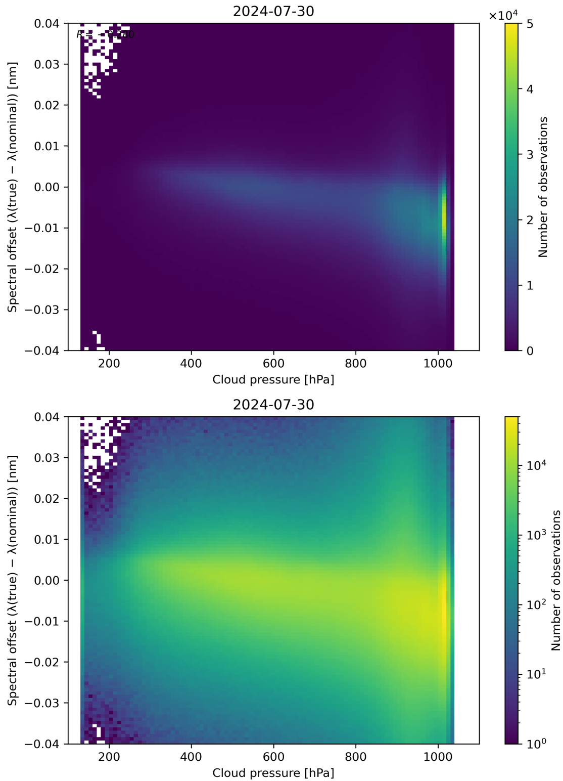
Figure 84: Scatter density plot of “Cloud pressure” against “Spectral offset ( \lambda(\text{true}) - \lambda(\text{nominal}) )” for 2024-07-29 to 2024-07-31.
