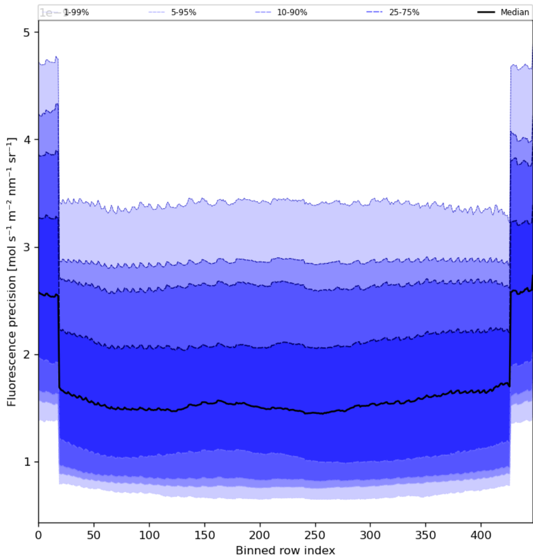
Figure 58: Along track statistics of “Fluorescence precision” for 2024-07-29 to 2024-07-31
