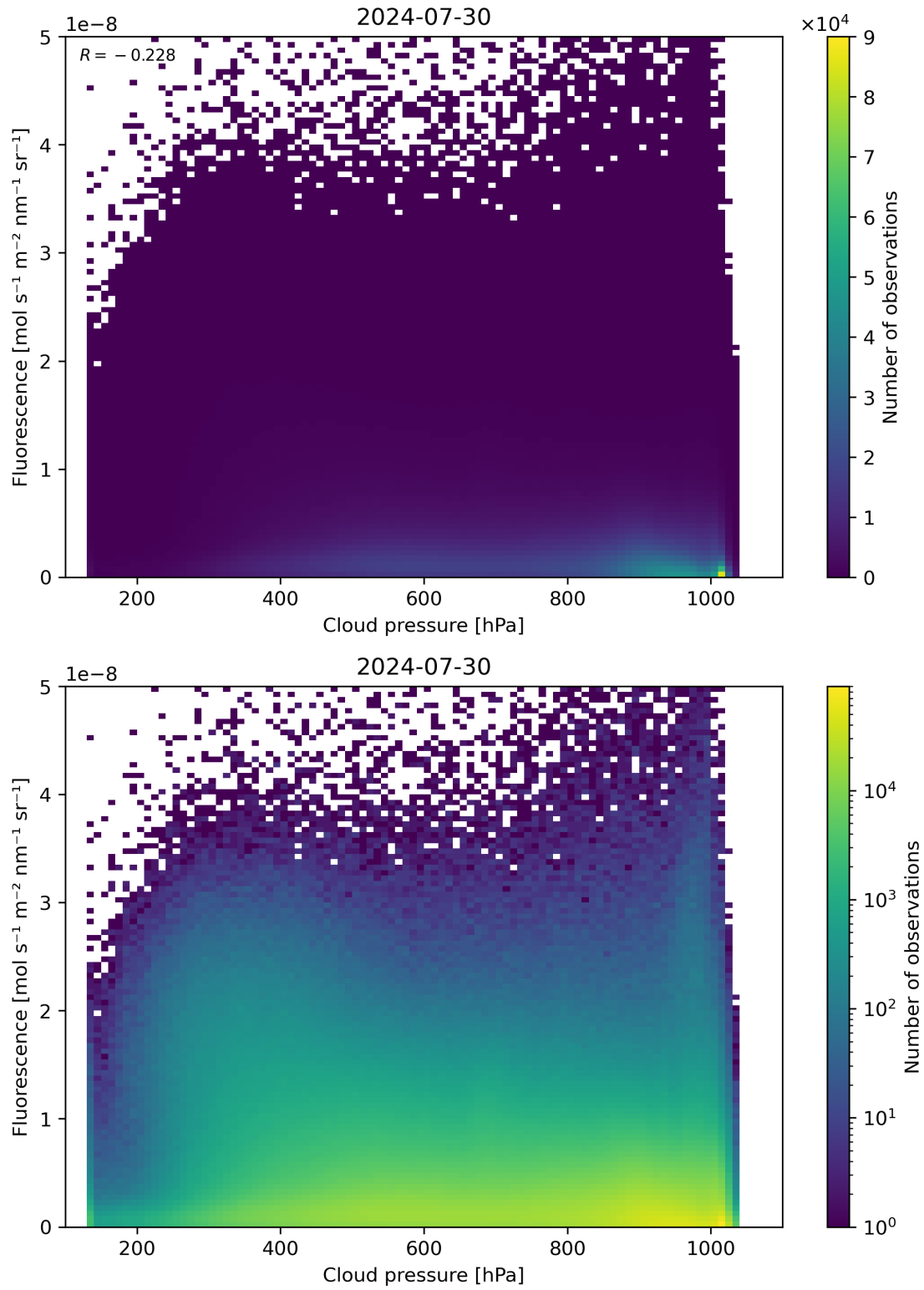
Figure 80: Scatter density plot of “Cloud pressure” against “Fluorescence” for 2024-07-29 to 2024-07-31.
