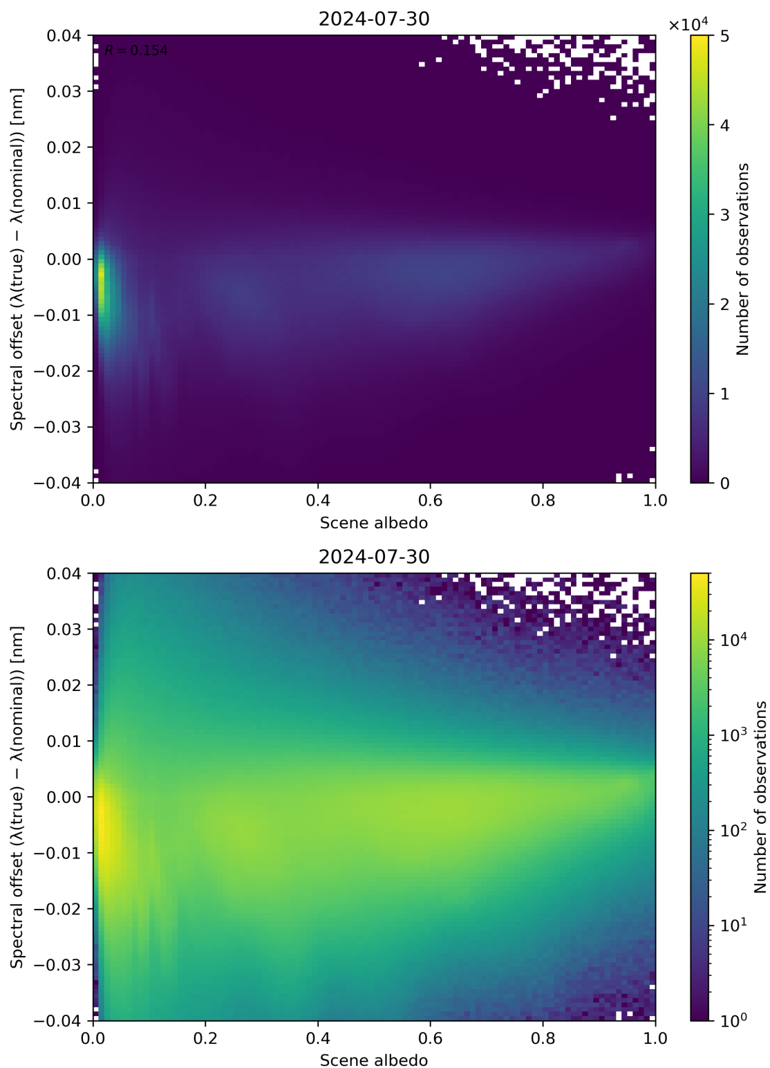
Figure 107: Scatter density plot of “Scene albedo” against “Spectral offset ( \lambda(\text{true}) - \lambda(\text{nominal}) )” for 2024-07-29 to 2024-07-31.
