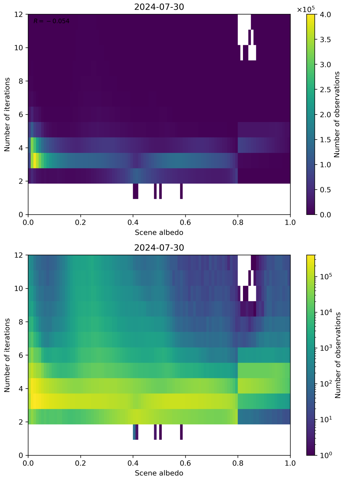
Figure 105: Scatter density plot of “Scene albedo” against “Number of iterations” for 2024-07-29 to 2024-07-31.
