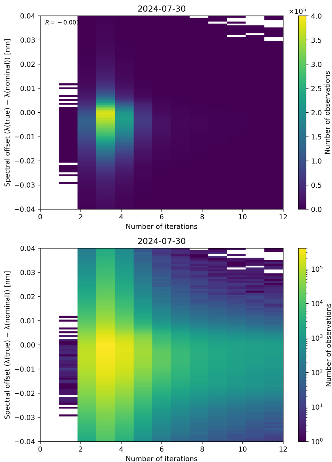
Figure 100: Scatter density plot of “Number of iterations” against “Spectral offset ( \lambda(\text{true}) - \lambda(\text{nominal}) )” for 2024-07-29 to 2024-07-31.
