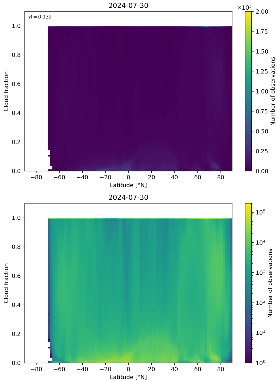
Figure 90: Scatter density plot of “Latitude” against “Cloud fraction” for 2024-07-29 to 2024-07-31.
