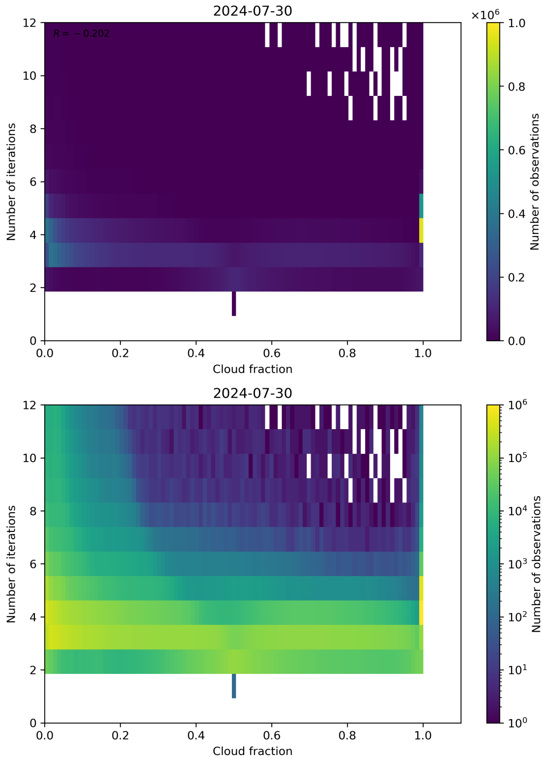
Figure 73: Scatter density plot of “Cloud fraction” against “Number of iterations” for 2024-07-29 to 2024-07-31.
