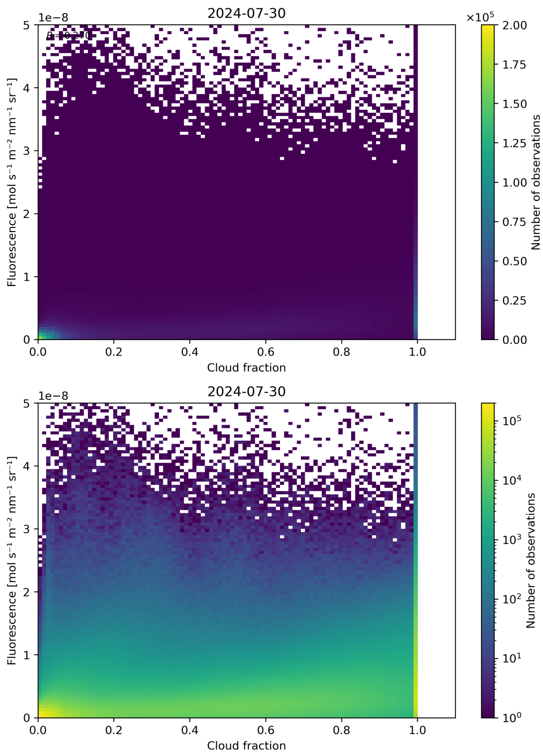
Figure 72: Scatter density plot of “Cloud fraction” against “Fluorescence” for 2024-07-29 to 2024-07-31.
