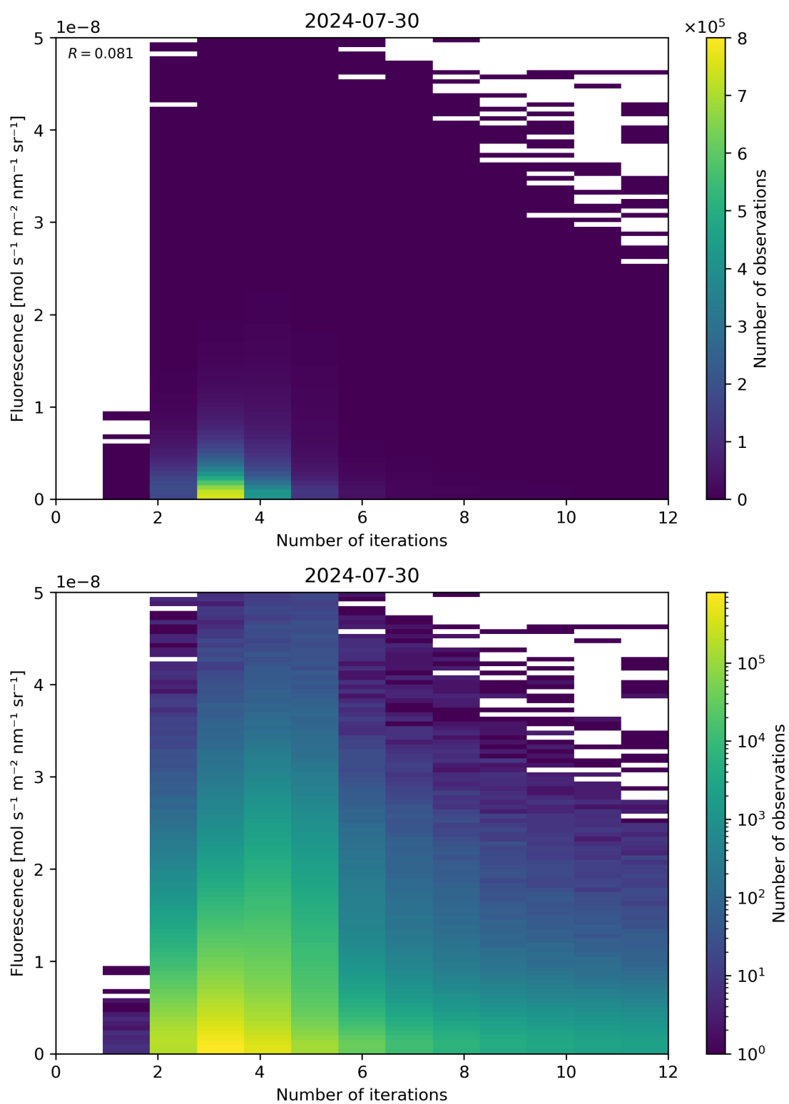
Figure 98: Scatter density plot of “Number of iterations” against “Fluorescence” for 2024-07-29 to 2024-07-31.
