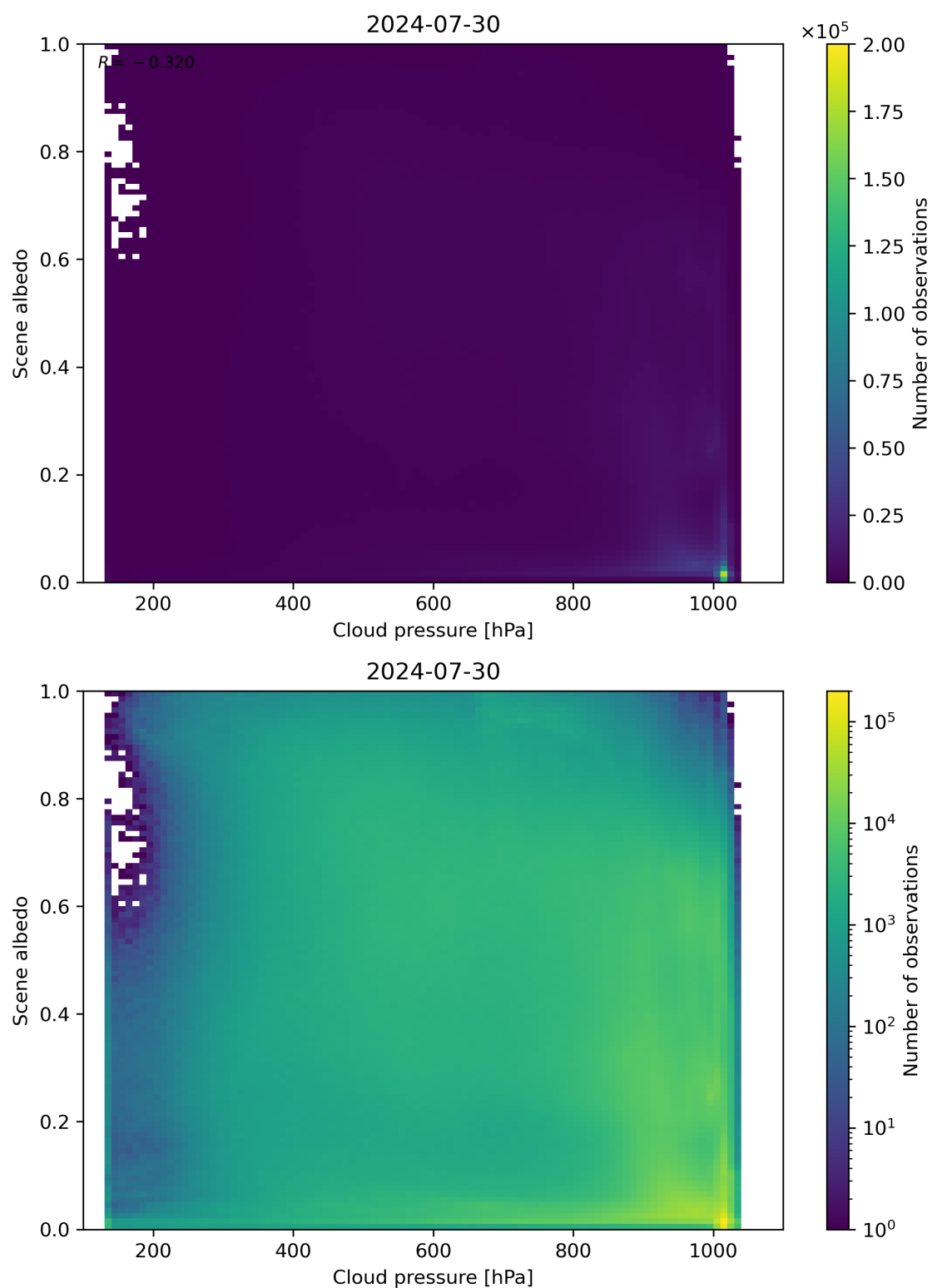
Figure 83: Scatter density plot of “Cloud pressure” against “Scene albedo” for 2024-07-29 to 2024-07-31.
