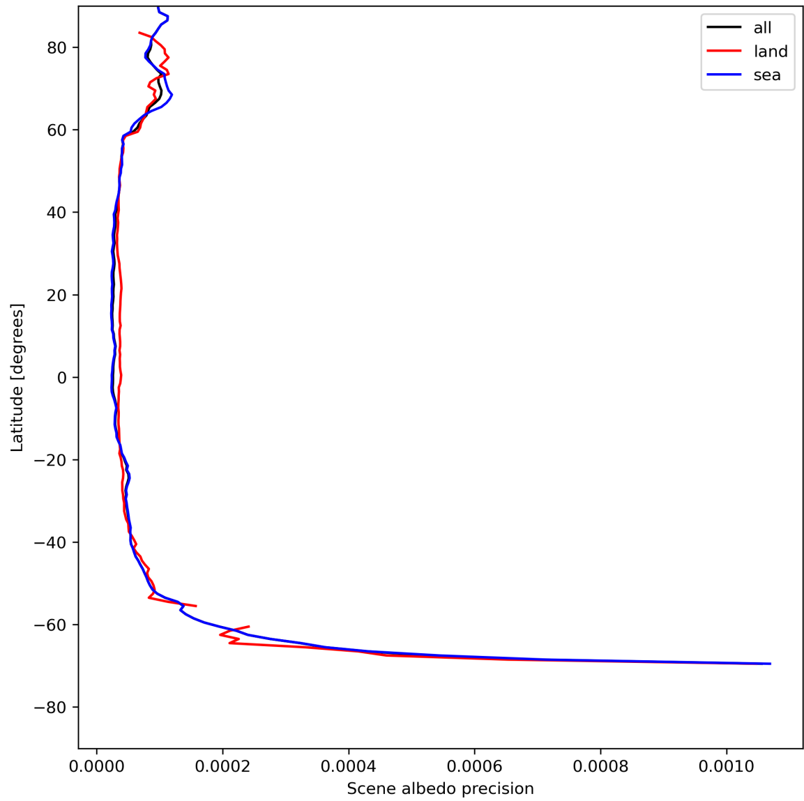
Figure 18: Zonal average of “Scene albedo precision” for 2024-07-29 to 2024-07-31.
