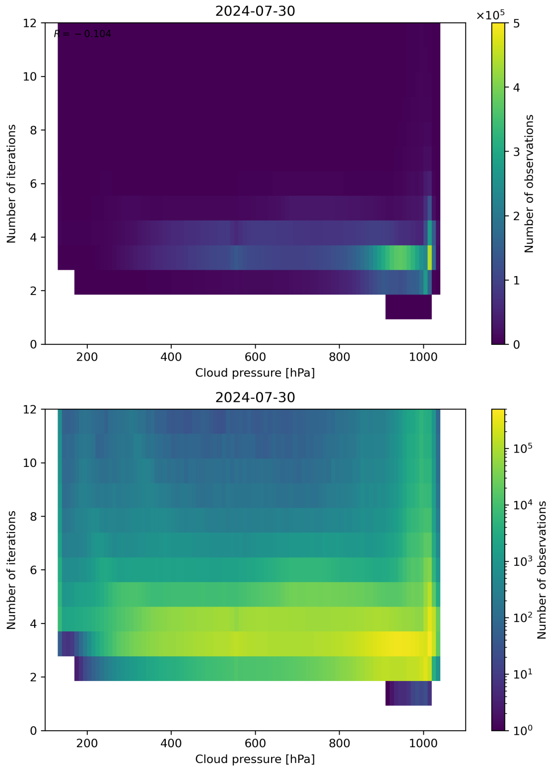
Figure 81: Scatter density plot of “Cloud pressure” against “Number of iterations” for 2024-07-29 to 2024-07-31.
