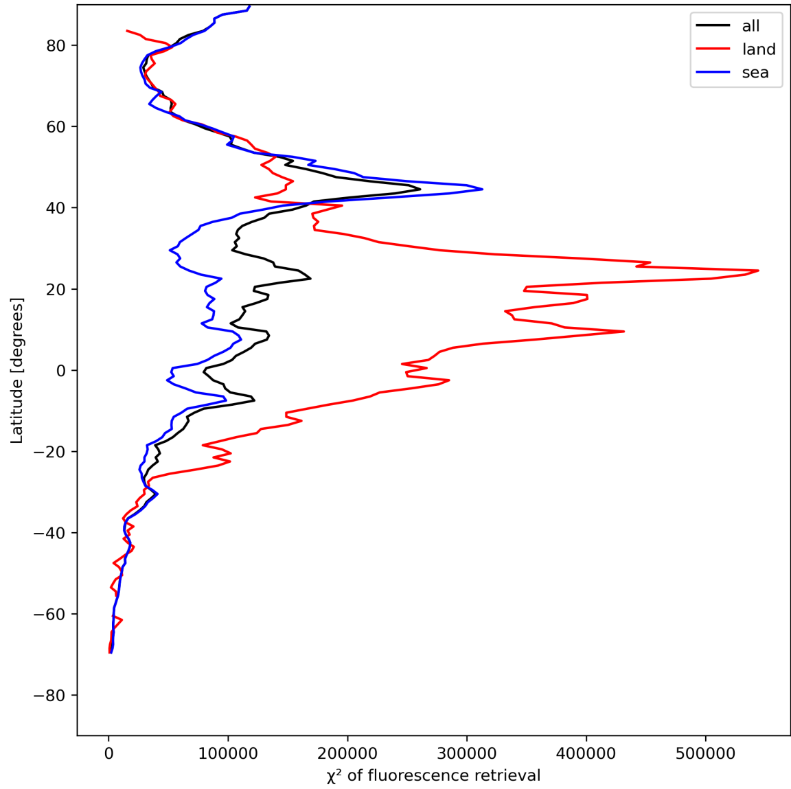
Figure 25: Zonal average of “ \chi^2 of fluorescence retrieval” for 2024-07-29 to 2024-07-31.
