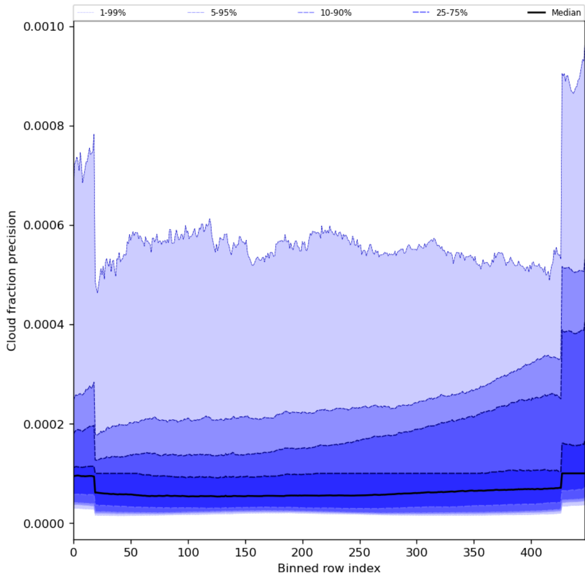
Figure 50: Along track statistics of “Cloud fraction precision” for 2024-07-29 to 2024-07-31
