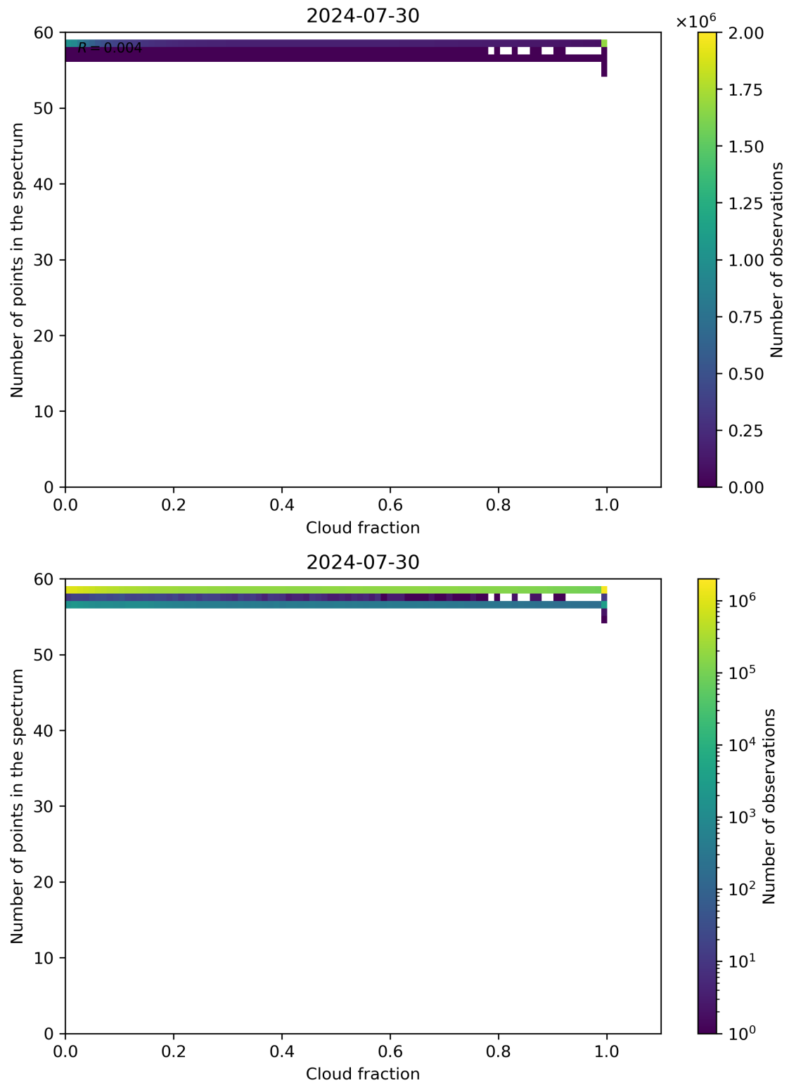
Figure 74: Scatter density plot of “Cloud fraction” against “Number of points in the spectrum” for 2024-07-29 to 2024-07-31.
