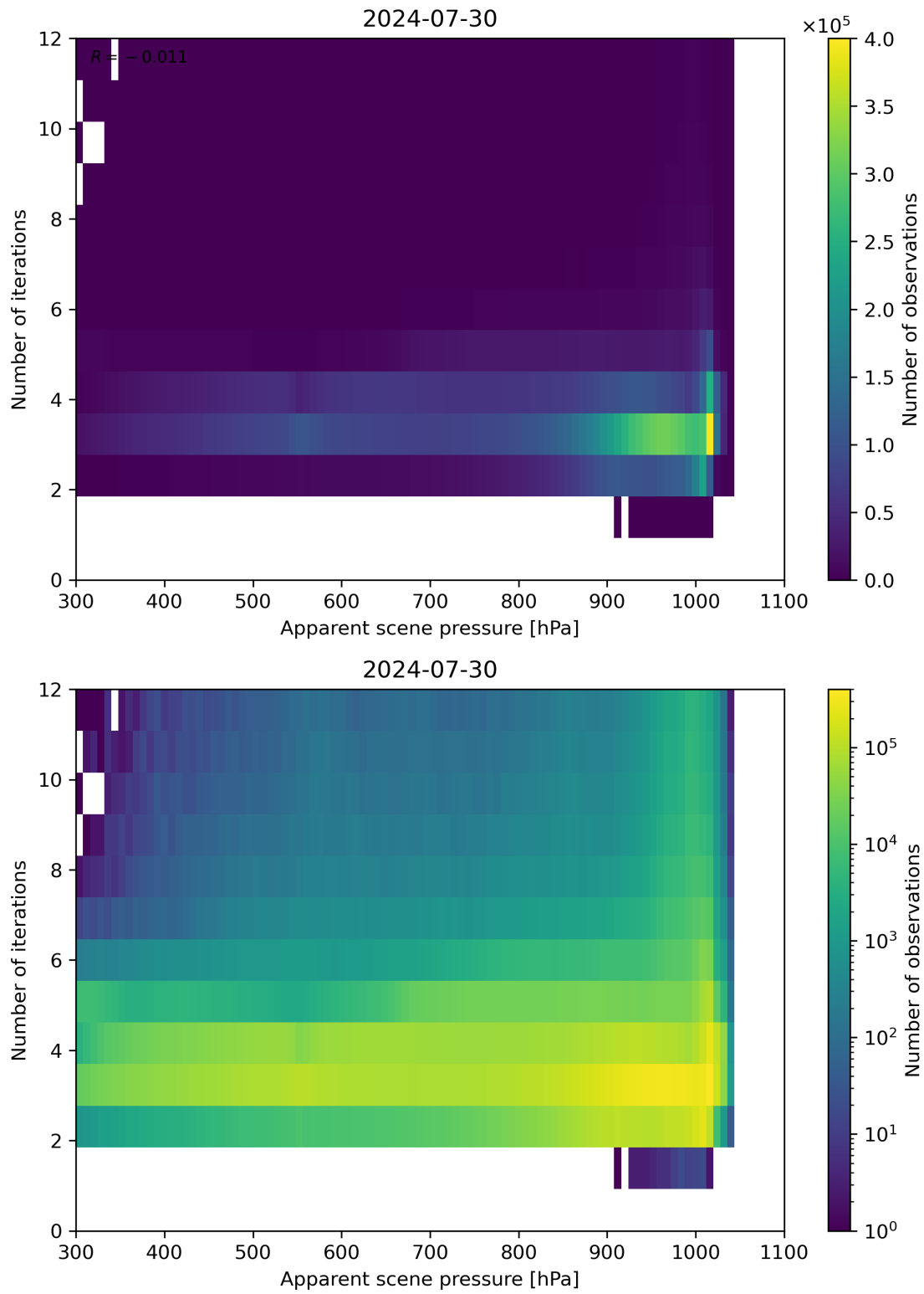
Figure 65: Scatter density plot of “Apparent scene pressure” against “Number of iterations” for 2024-07-29 to 2024-07-31.
