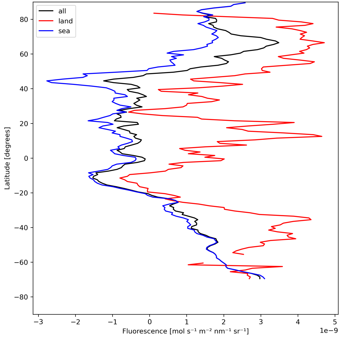
Figure 23: Zonal average of “Fluorescence” for 2024-07-29 to 2024-07-31.
