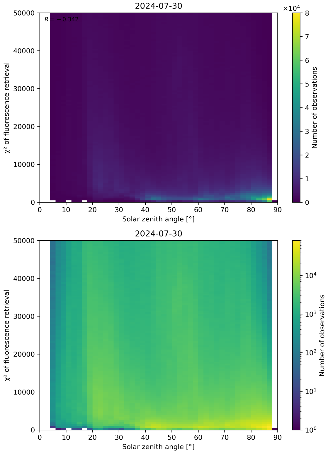
Figure 109: Scatter density plot of “Solar zenith angle” against “ \chi^2 of fluorescence retrieval” for 2024-07-29 to 2024-07-31.
