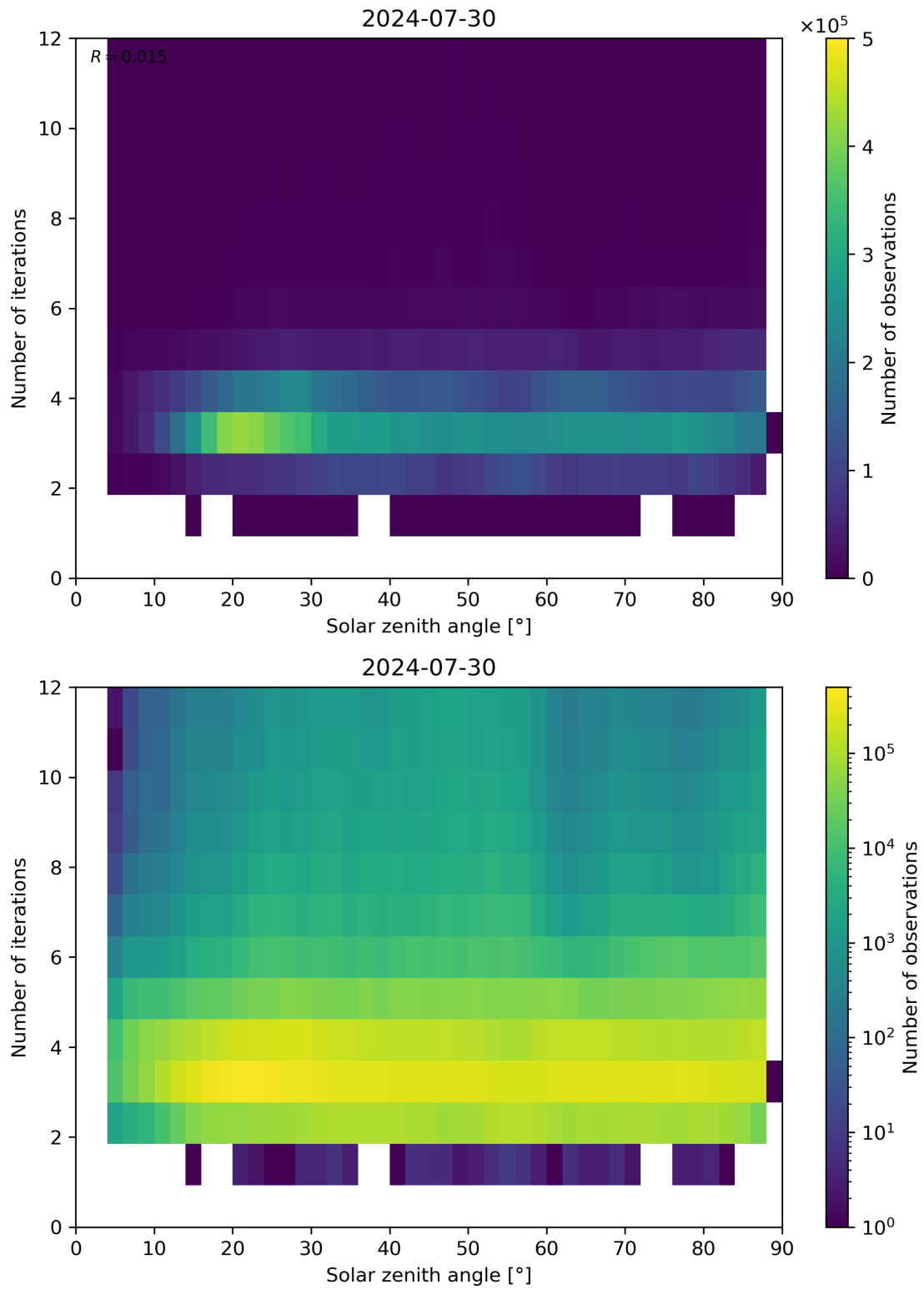
Figure 114: Scatter density plot of “Solar zenith angle” against “Number of iterations” for 2024-07-29 to 2024-07-31.
