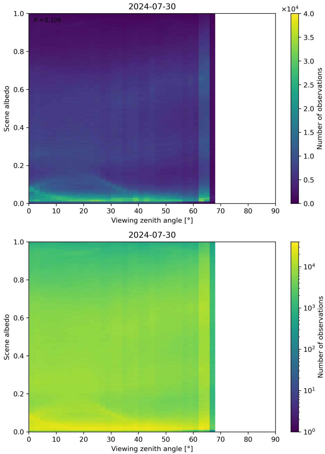
Figure 126: Scatter density plot of “Viewing zenith angle” against “Scene albedo” for 2024-07-29 to 2024-07-31.
