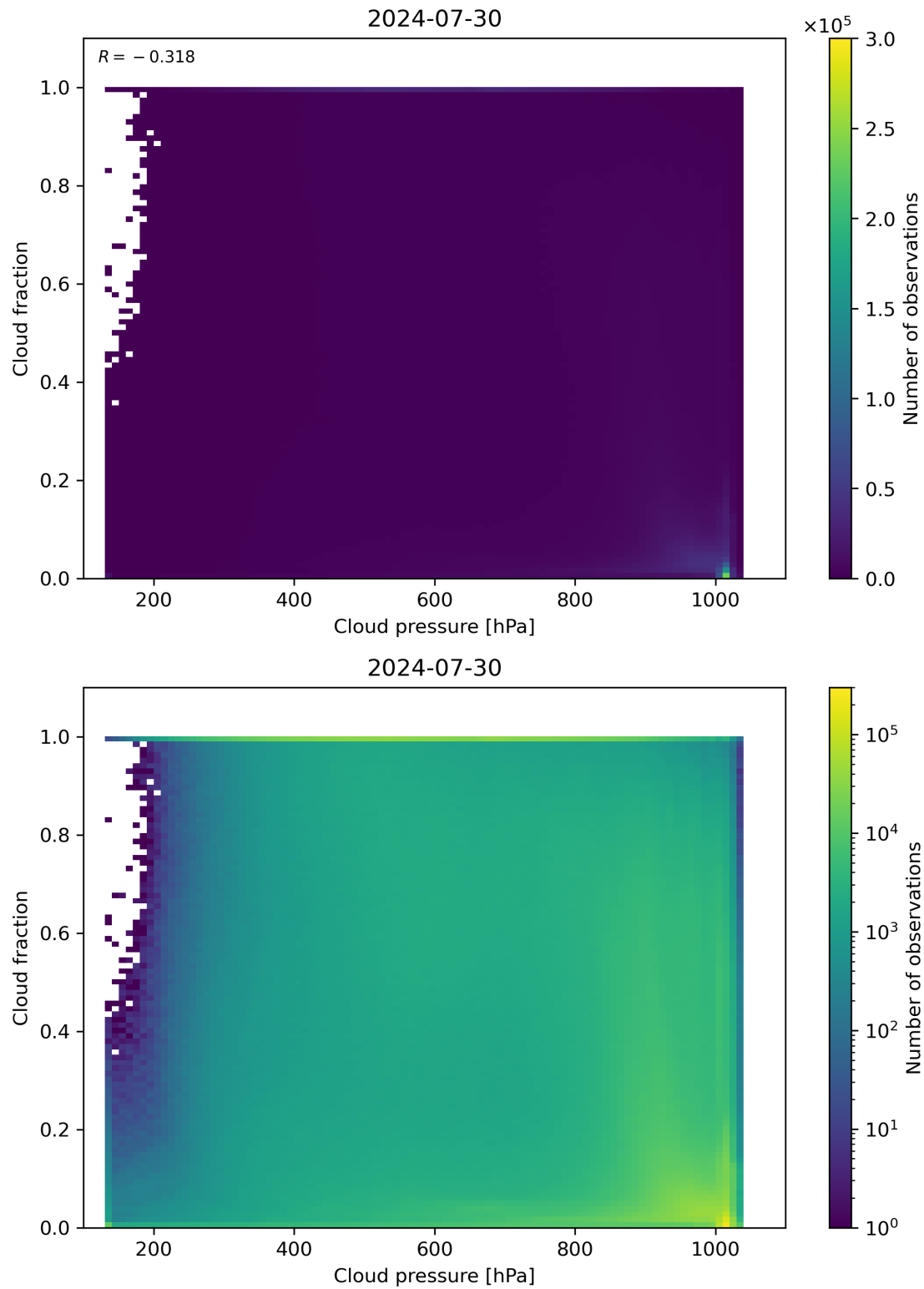
Figure 79: Scatter density plot of “Cloud pressure” against “Cloud fraction” for 2024-07-29 to 2024-07-31.
