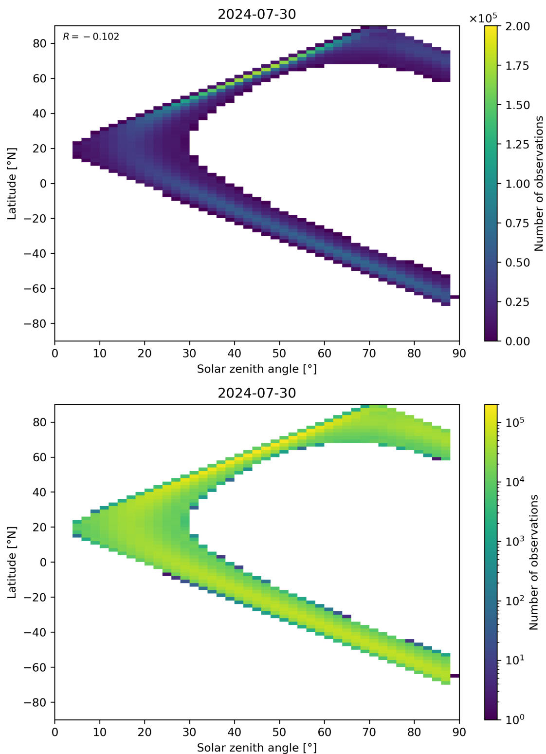
Figure 113: Scatter density plot of “Solar zenith angle” against “Latitude” for 2024-07-29 to 2024-07-31.
