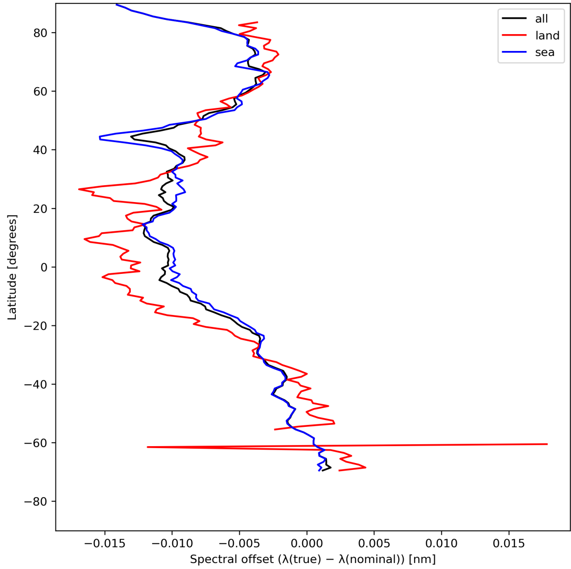
Figure 28: Zonal average of “Spectral offset ( \lambda(\text{true}) - \lambda(\text{nominal}) )” for 2024-07-29 to 2024-07-31.
