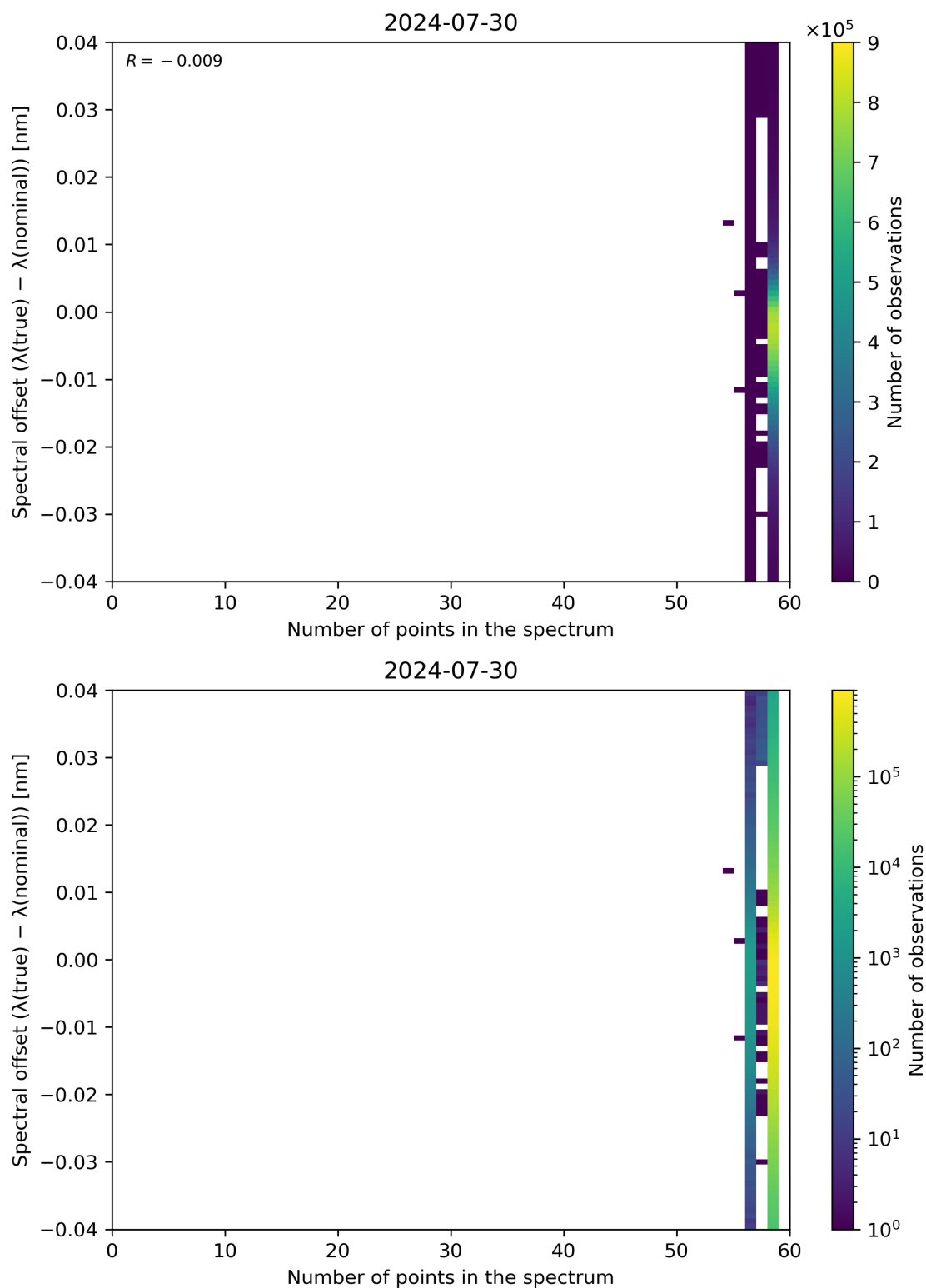
Figure 101: Scatter density plot of “Number of points in the spectrum” against “Spectral offset ( \lambda(\text{true}) - \lambda(\text{nominal}) )” for 2024-07-29 to 2024-07-31.
