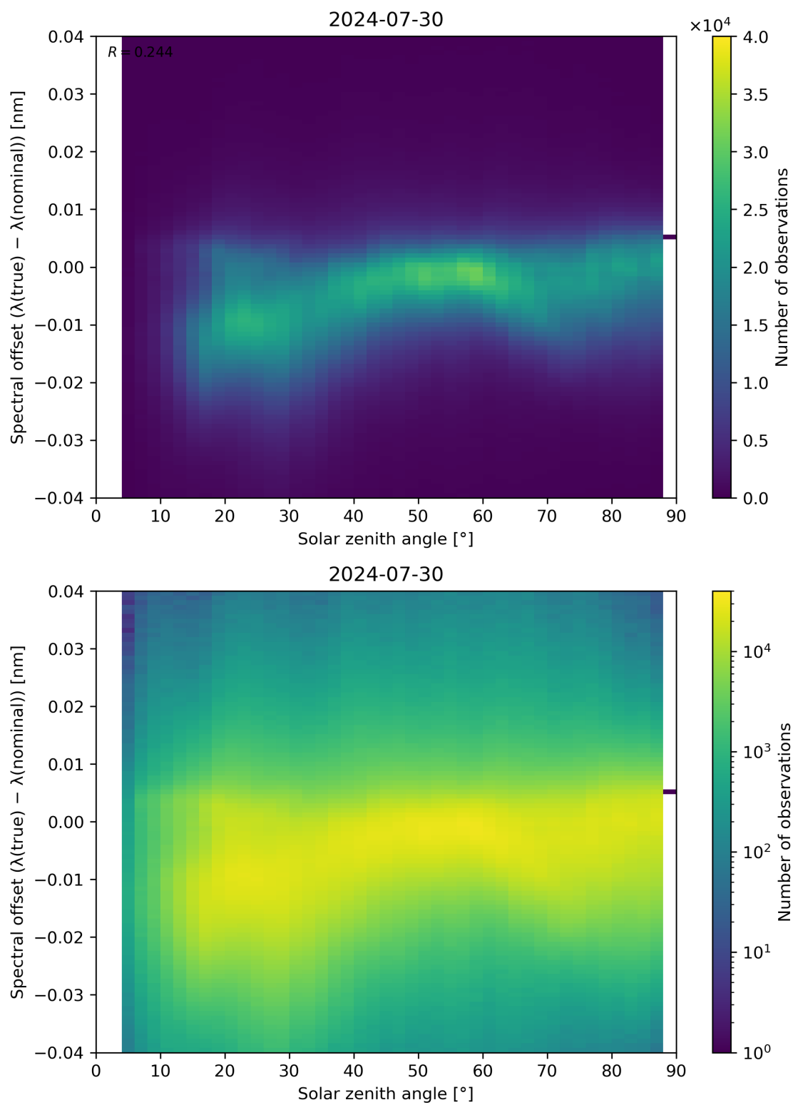
Figure 117: Scatter density plot of “Solar zenith angle” against “Spectral offset ( \lambda(\text{true}) - \lambda(\text{nominal}) )” for 2024-07-29 to 2024-07-31.
