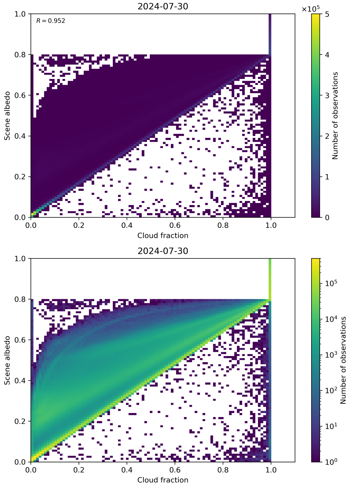
Figure 75: Scatter density plot of “Cloud fraction” against “Scene albedo” for 2024-07-29 to 2024-07-31.
