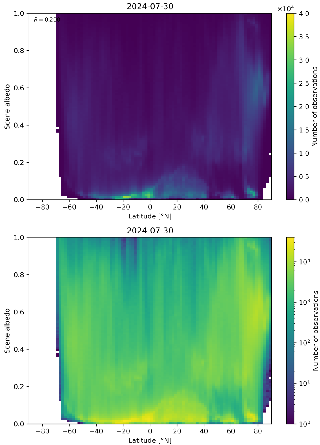
Figure 95: Scatter density plot of “Latitude” against “Scene albedo” for 2024-07-29 to 2024-07-31.
