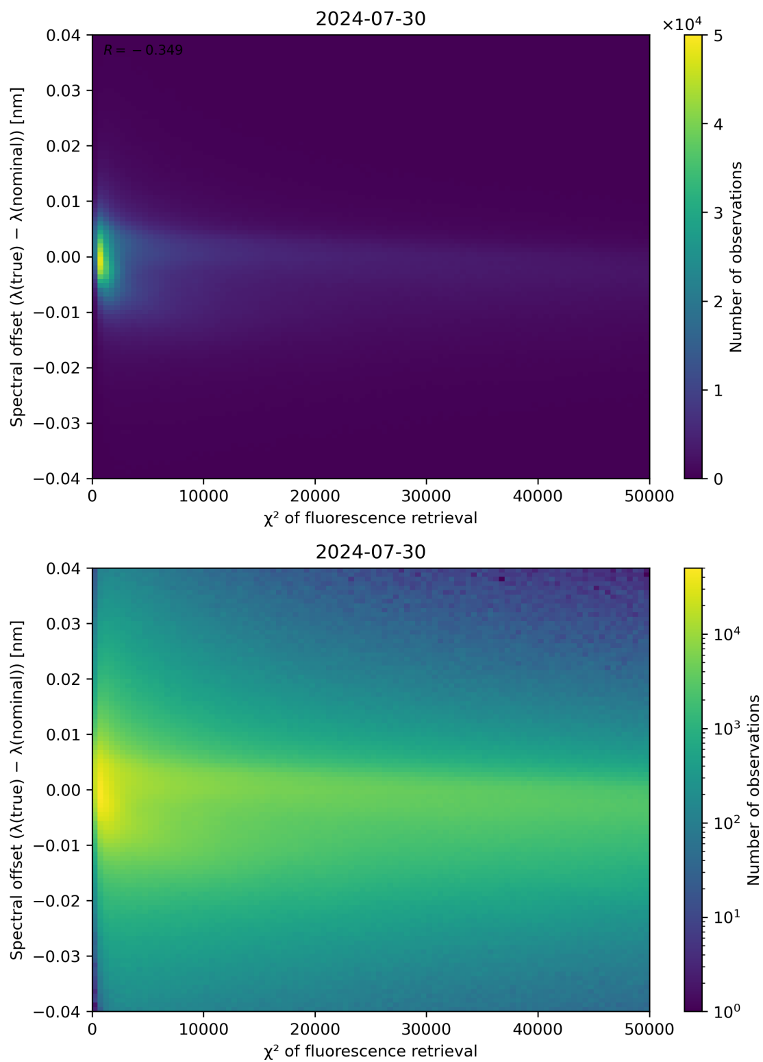
Figure 69: Scatter density plot of " \chi^2 of fluorescence retrieval" against "Spectral offset ( \lambda(\text{true}) - \lambda(\text{nominal})) " for 2024-07-29 to 2024-07-31.
