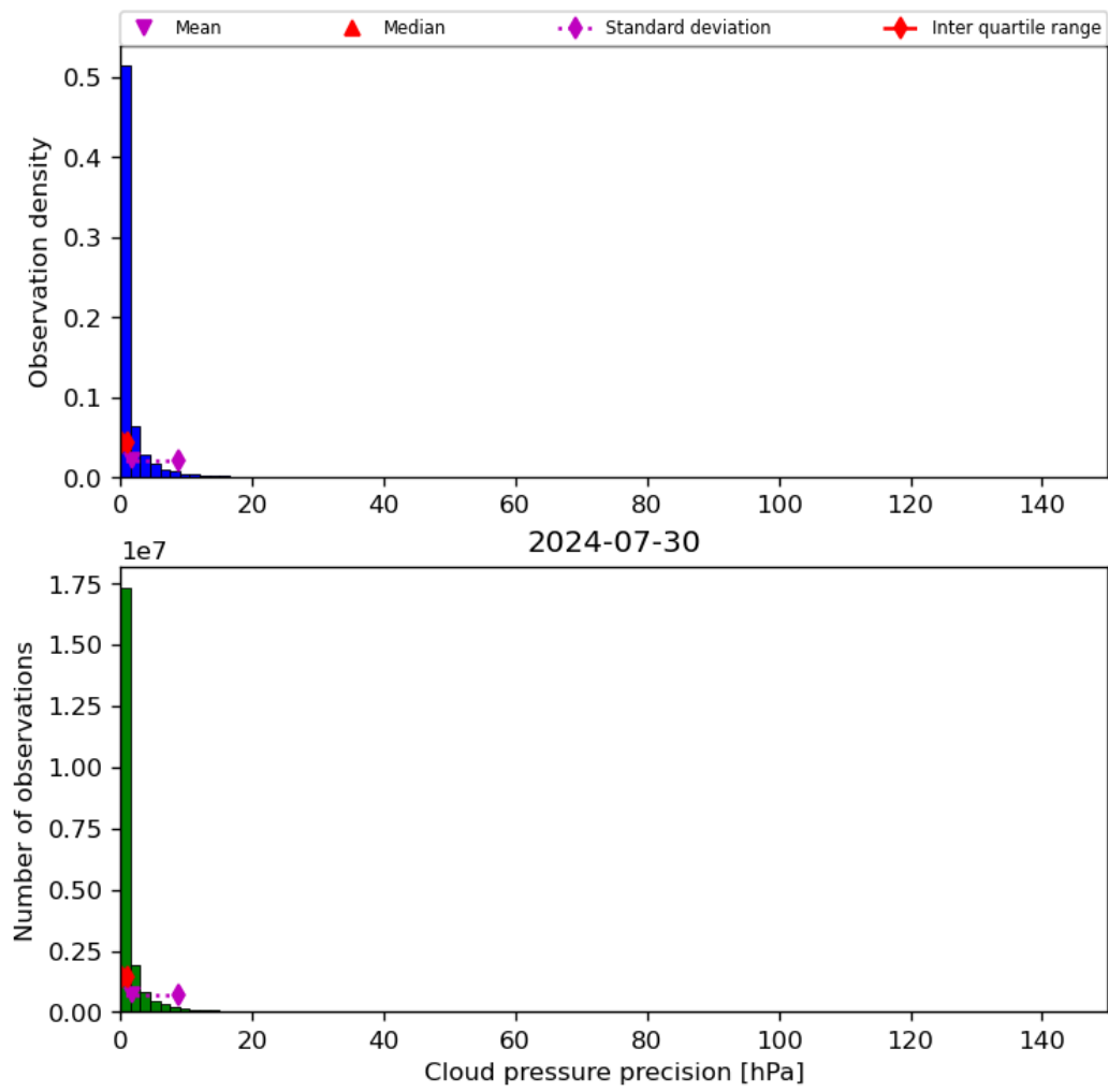
Figure 31: Histogram of “Cloud pressure precision” for 2024-07-29 to 2024-07-31
