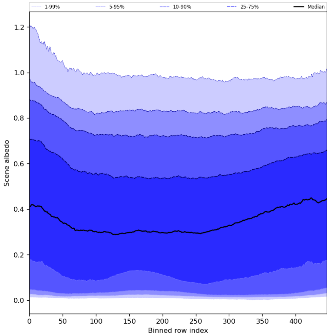
Figure 51: Along track statistics of “Scene albedo” for 2024-07-29 to 2024-07-31
