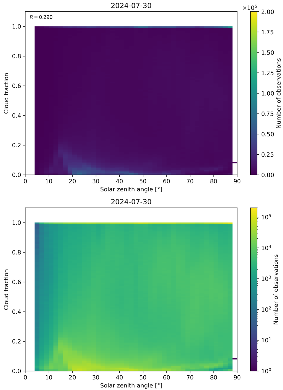
Figure 110: Scatter density plot of “Solar zenith angle” against “Cloud fraction” for 2024-07-29 to 2024-07-31.
