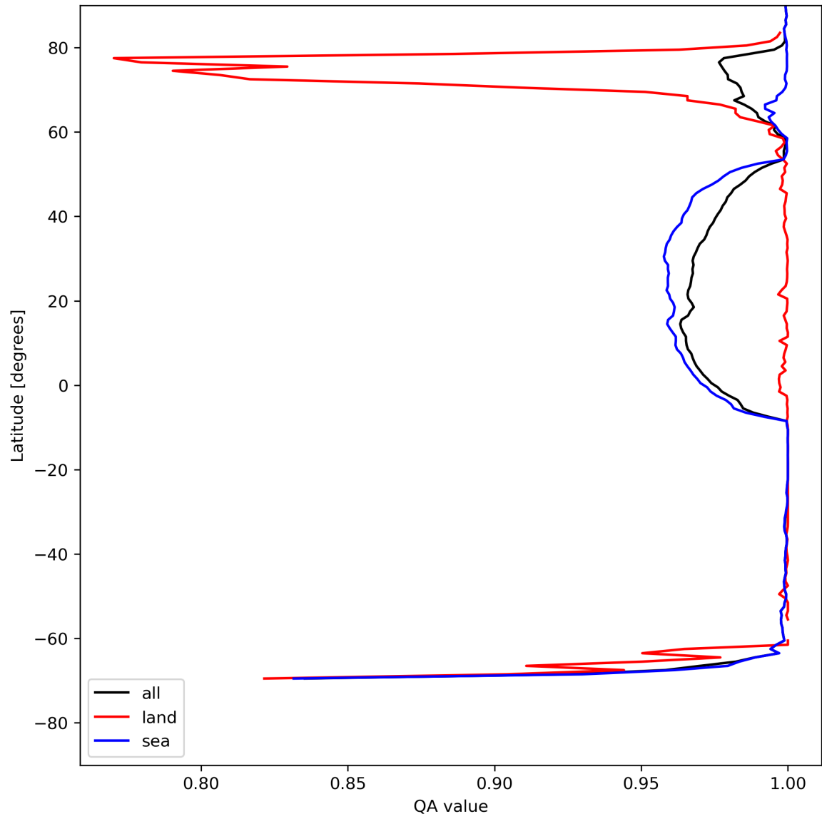
Figure 12: Zonal average of “QA value” for 2024-07-29 to 2024-07-31.
