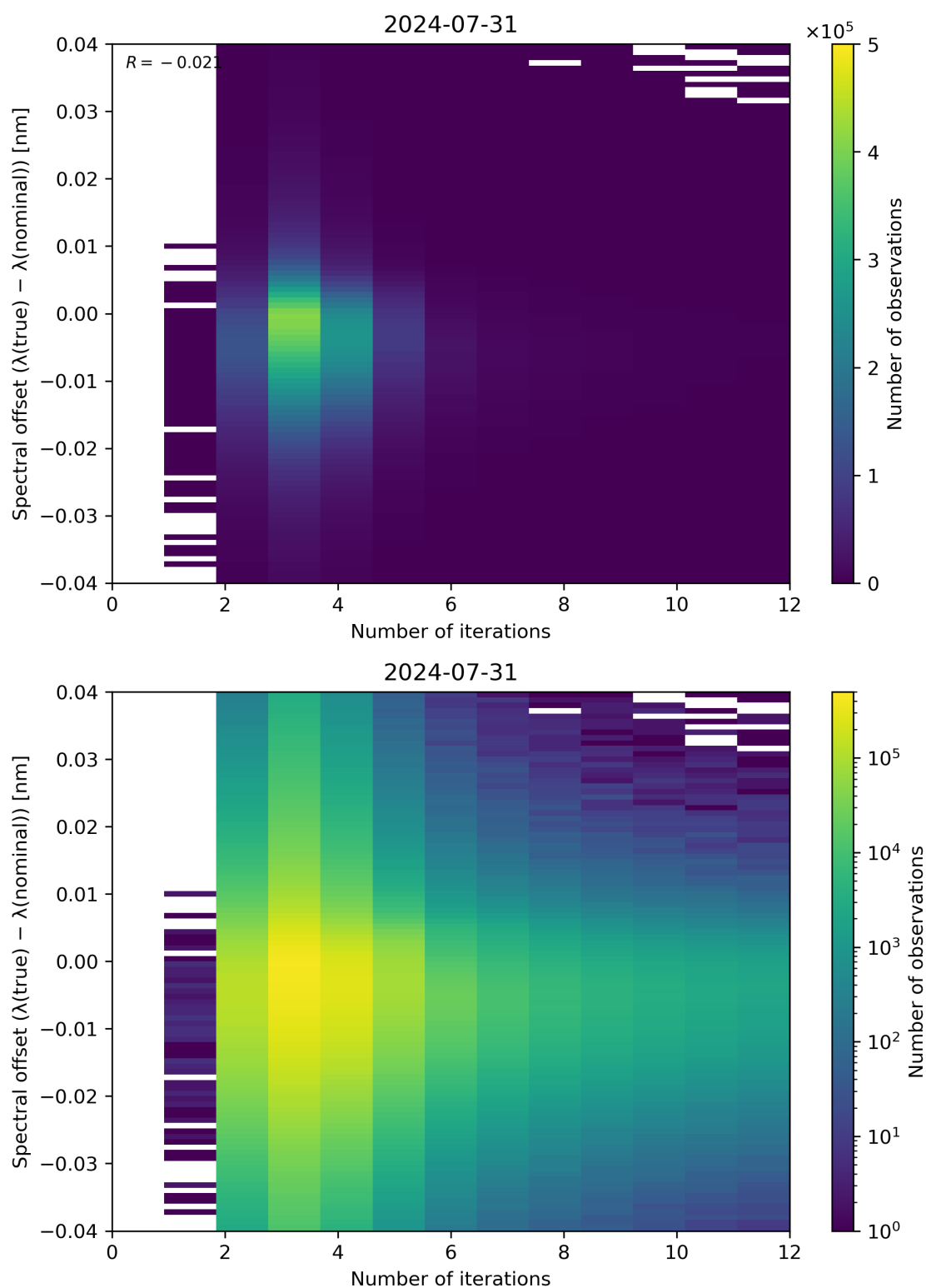
Figure 100: Scatter density plot of “Number of iterations” against “Spectral offset ( \lambda(\text{true}) - \lambda(\text{nominal}) )” for 2024-07-31 to 2024-08-01.
