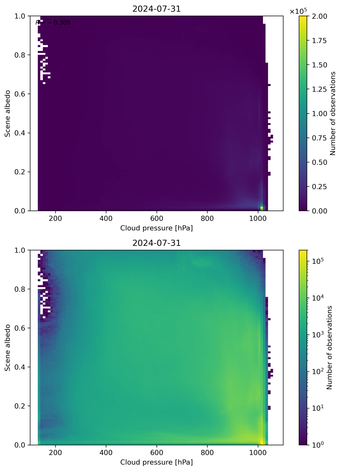
Figure 83: Scatter density plot of “Cloud pressure” against “Scene albedo” for 2024-07-31 to 2024-08-01.
