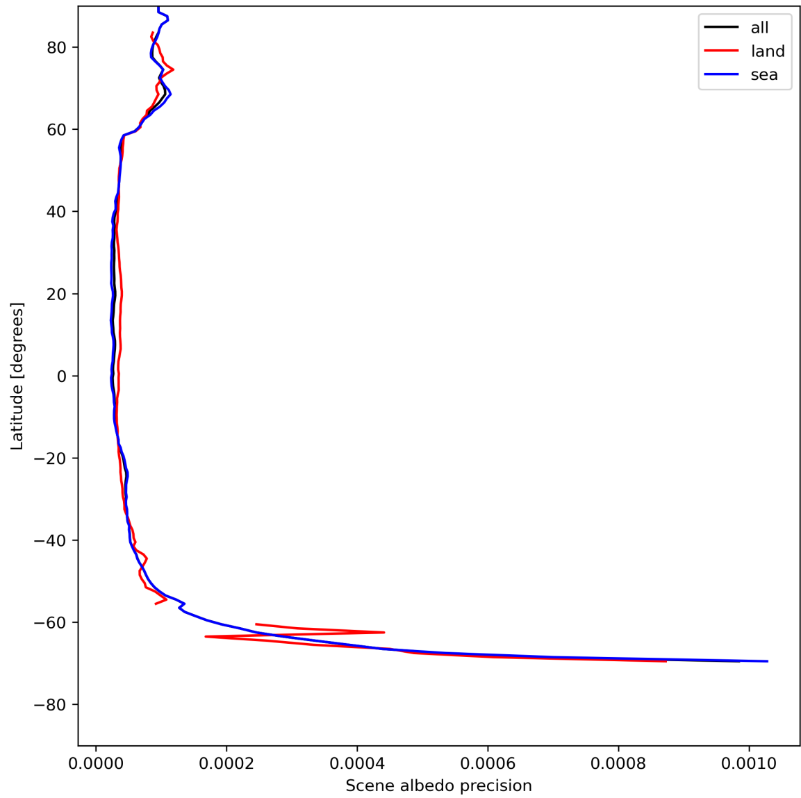
Figure 18: Zonal average of “Scene albedo precision” for 2024-07-31 to 2024-08-01.
