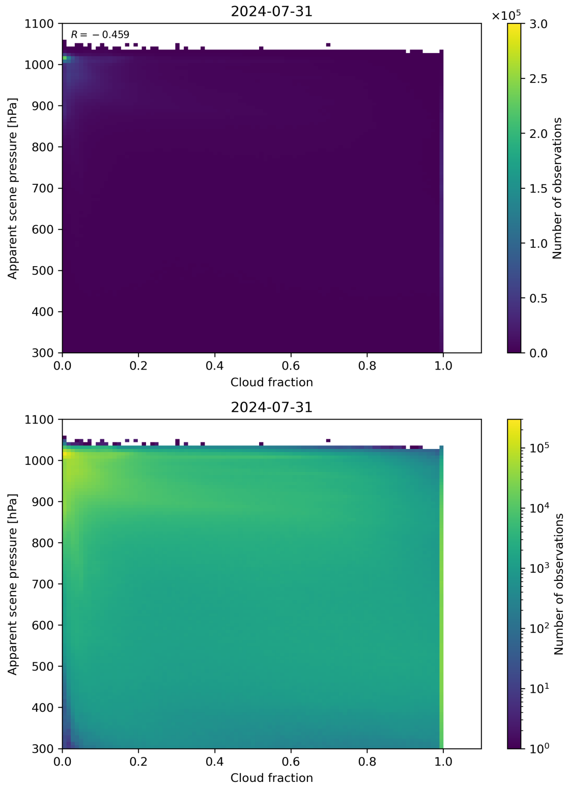
Figure 70: Scatter density plot of “Cloud fraction” against “Apparent scene pressure” for 2024-07-31 to 2024-08-01.
