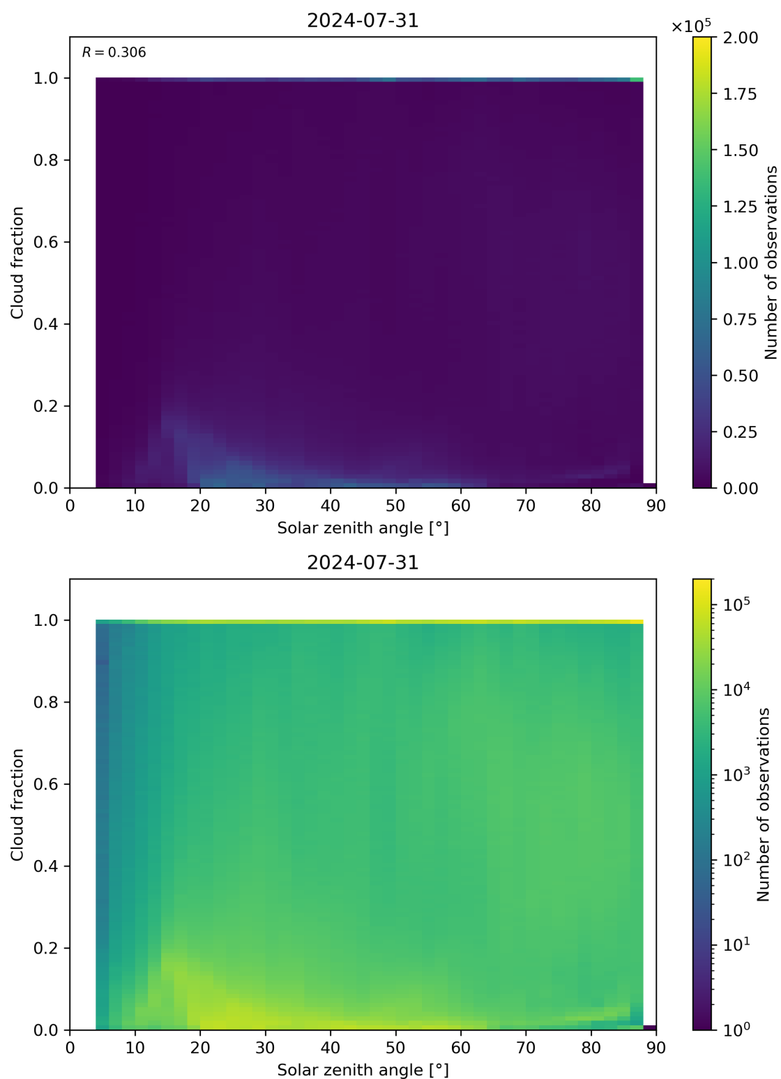
Figure 110: Scatter density plot of “Solar zenith angle” against “Cloud fraction” for 2024-07-31 to 2024-08-01.
