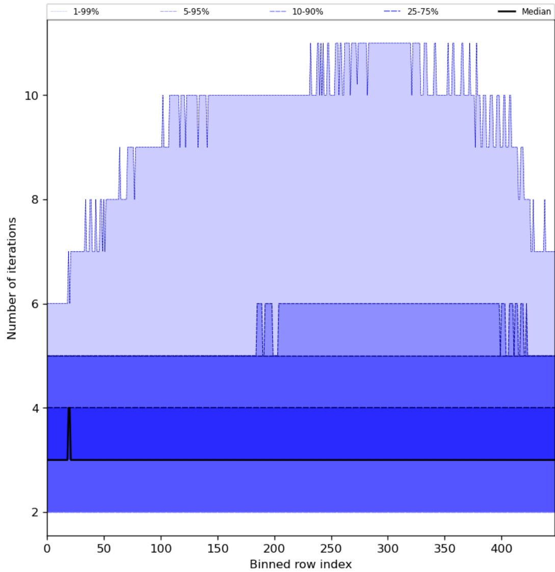
Figure 56: Along track statistics of “Number of iterations” for 2024-07-31 to 2024-08-01
