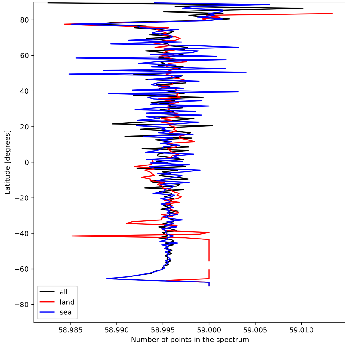
Figure 27: Zonal average of “Number of points in the spectrum” for 2024-07-31 to 2024-08-01.
