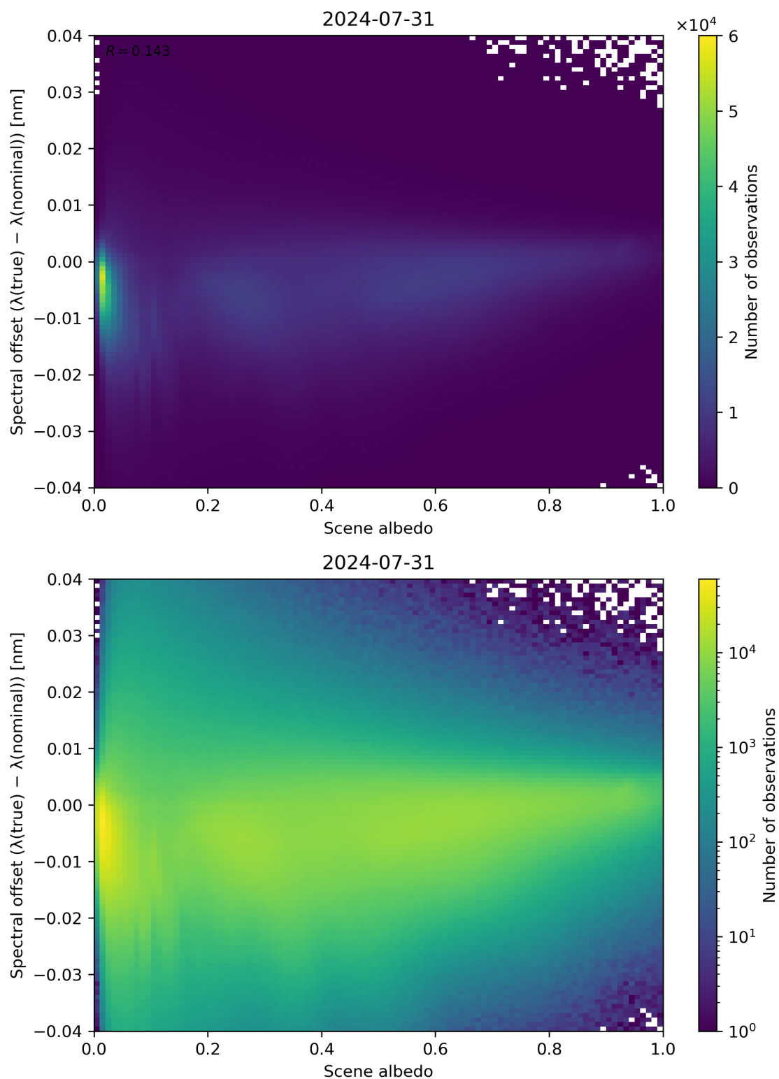
Figure 107: Scatter density plot of “Scene albedo” against “Spectral offset ( \lambda(\text{true}) - \lambda(\text{nominal}) )” for 2024-07-31 to 2024-08-01.
