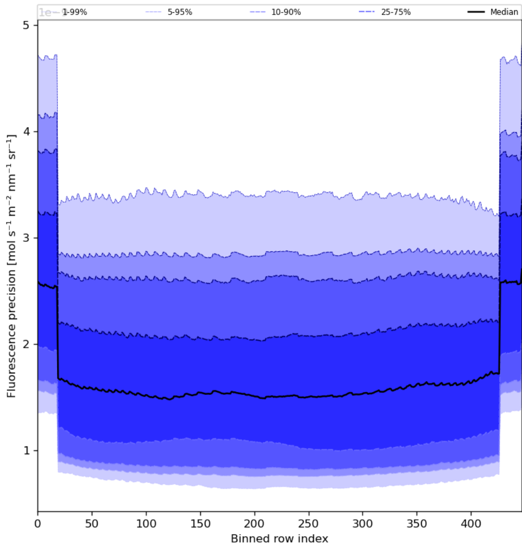
Figure 58: Along track statistics of “Fluorescence precision” for 2024-07-31 to 2024-08-01
