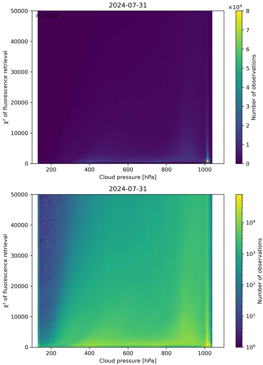
Figure 78: Scatter density plot of “Cloud pressure” against “ \chi^2 of fluorescence retrieval” for 2024-07-31 to 2024-08-01.
