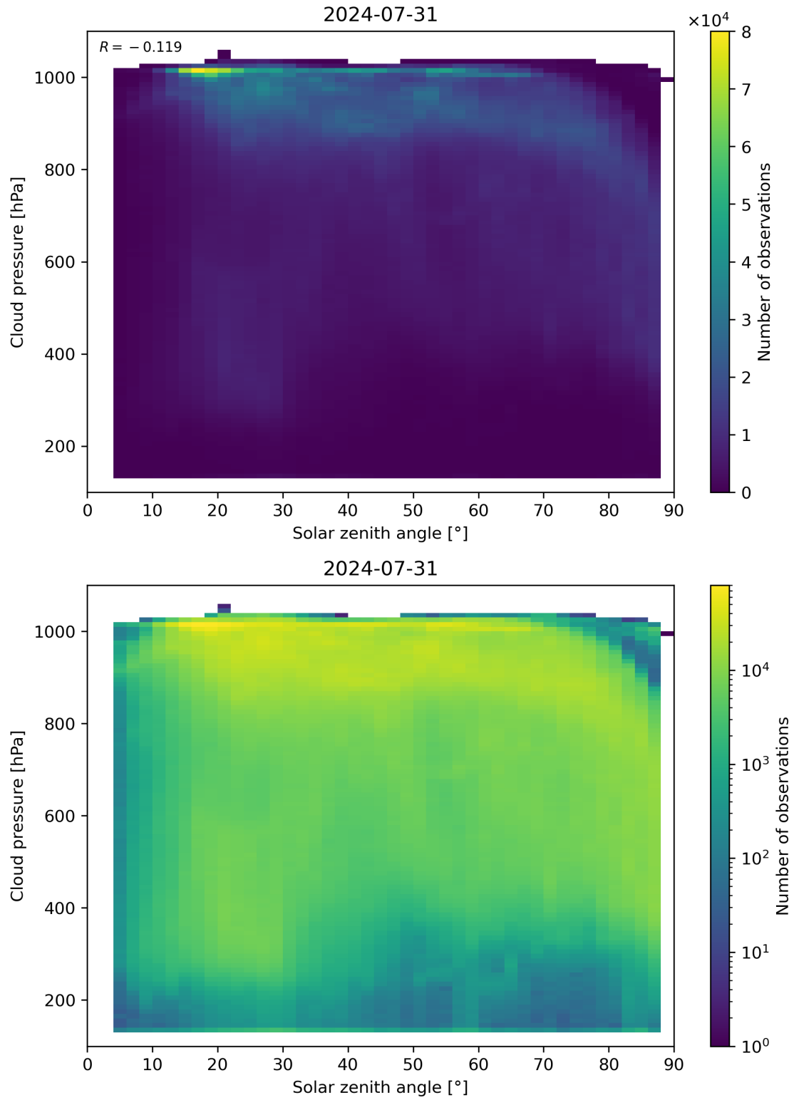
Figure 111: Scatter density plot of “Solar zenith angle” against “Cloud pressure” for 2024-07-31 to 2024-08-01.
