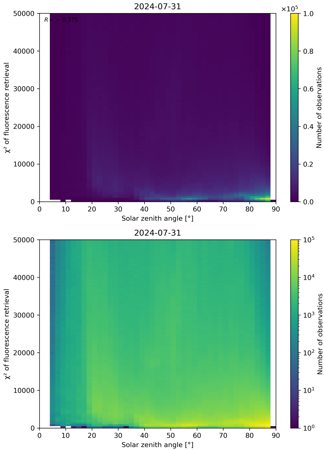
Figure 109: Scatter density plot of “Solar zenith angle” against “ \chi^2 of fluorescence retrieval” for 2024-07-31 to 2024-08-01.
