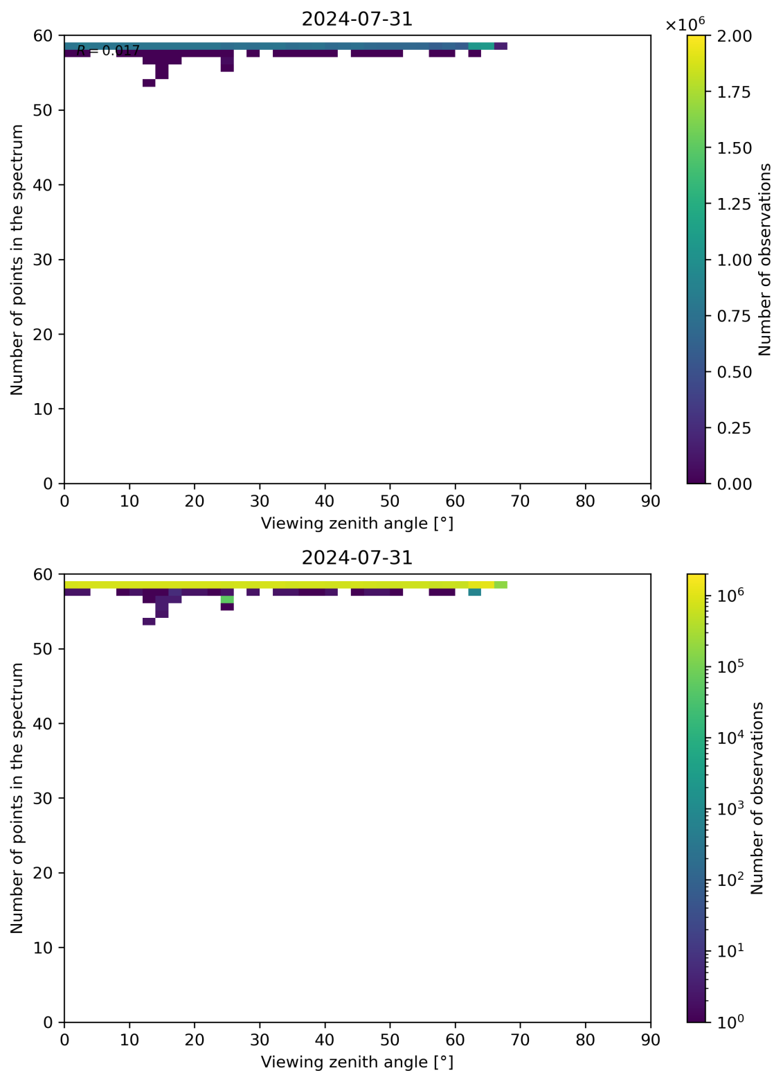
Figure 125: Scatter density plot of “Viewing zenith angle” against “Number of points in the spectrum” for 2024-07-31 to 2024-08-01.
