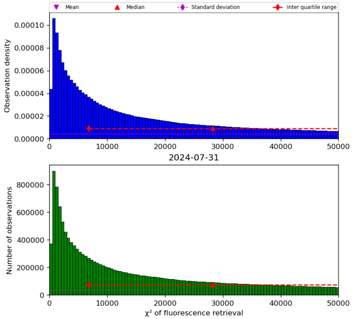
Figure 42: Histogram of “ \chi^2 of fluorescence retrieval” for 2024-07-31 to 2024-08-01
