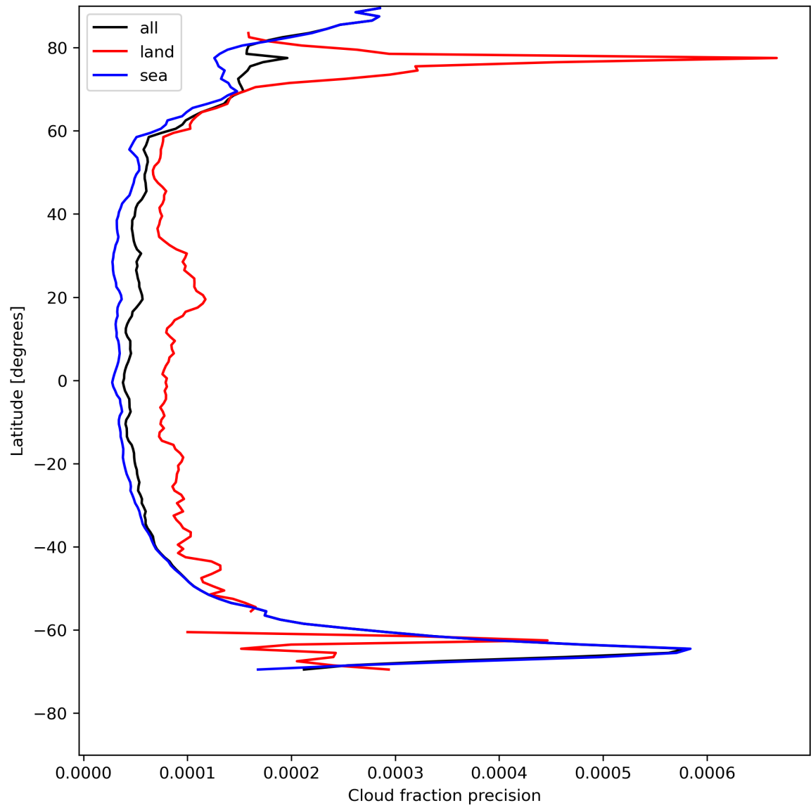
Figure 16: Zonal average of “Cloud fraction precision” for 2024-07-31 to 2024-08-01.
