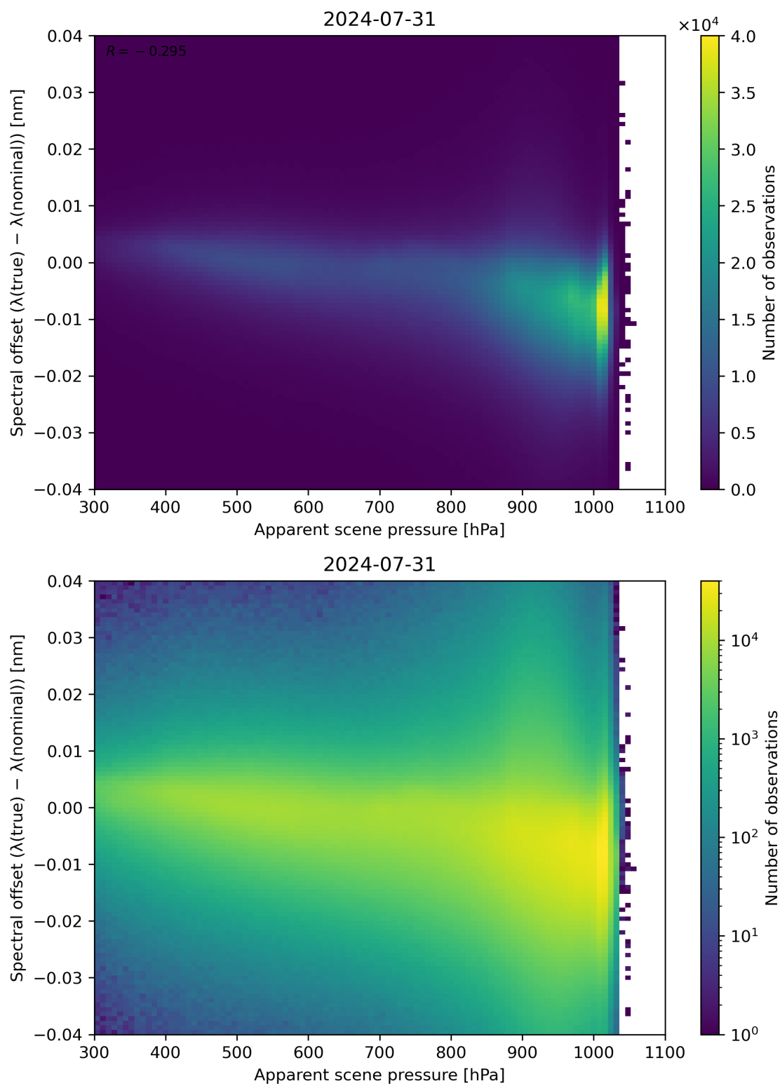
Figure 67: Scatter density plot of “Apparent scene pressure” against “Spectral offset ( \lambda(\text{true}) - \lambda(\text{nominal}) )” for 2024-07-31 to 2024-08-01.
