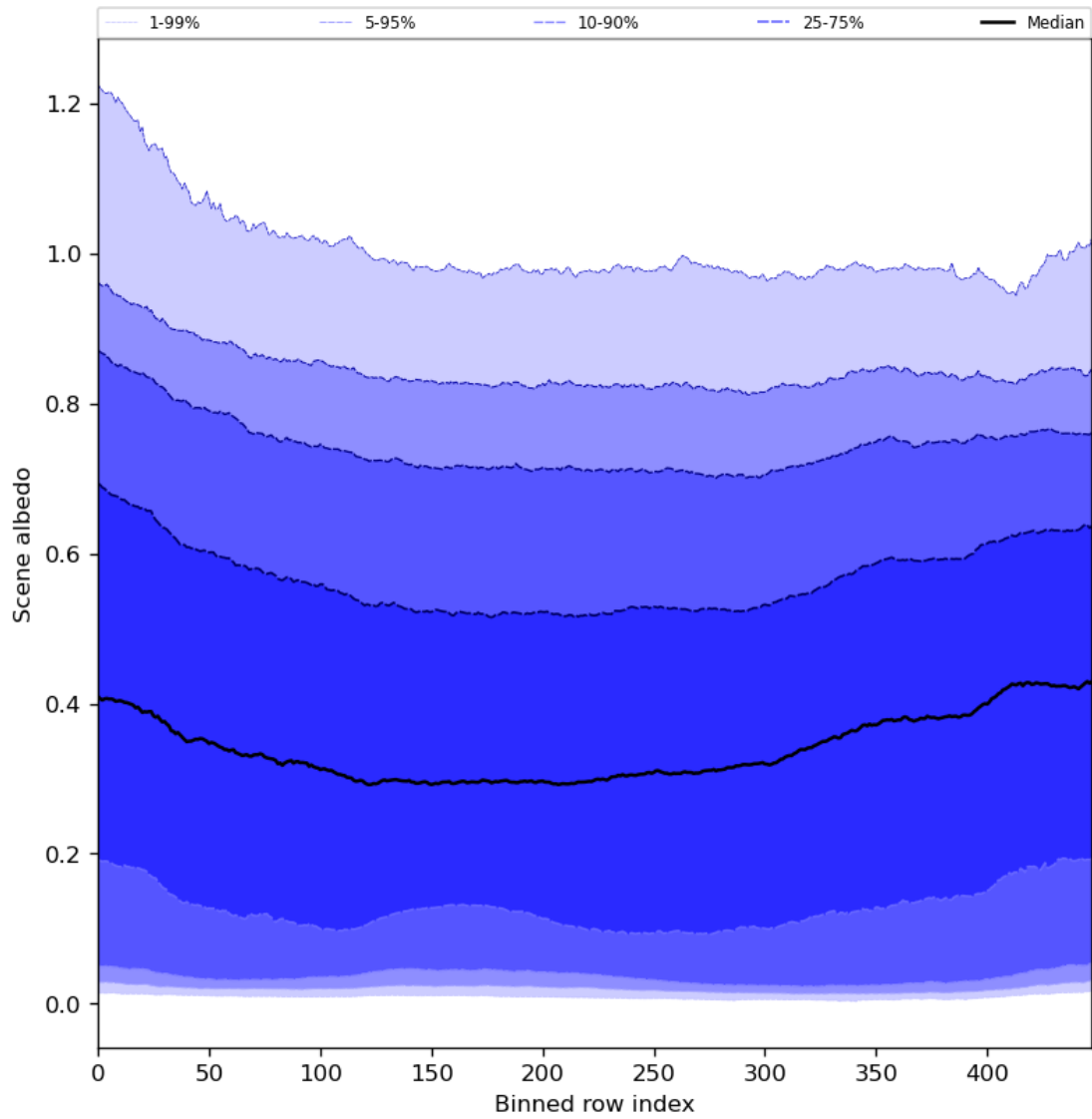
Figure 51: Along track statistics of “Scene albedo” for 2024-07-31 to 2024-08-01
