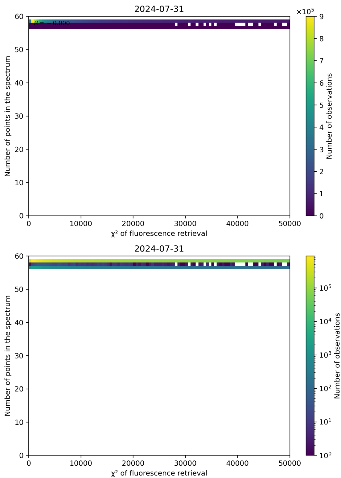
Figure 68: Scatter density plot of " \chi^2 of fluorescence retrieval" against "Number of points in the spectrum" for 2024-07-31 to 2024-08-01.
