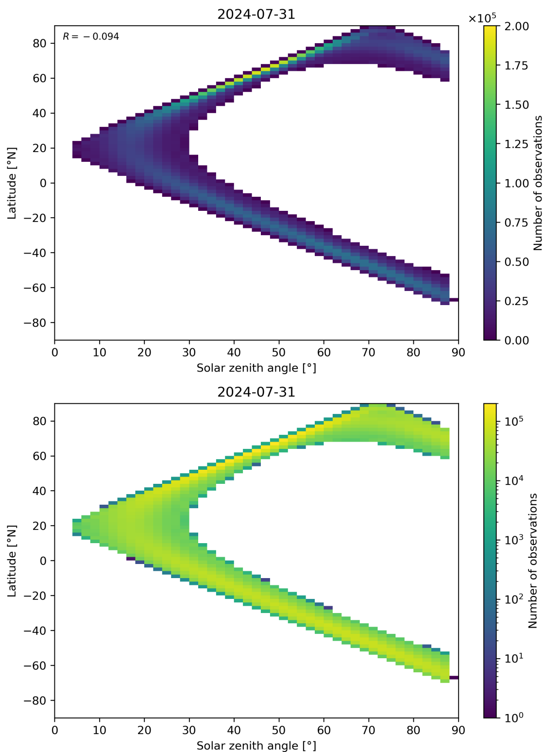
Figure 113: Scatter density plot of “Solar zenith angle” against “Latitude” for 2024-07-31 to 2024-08-01.
