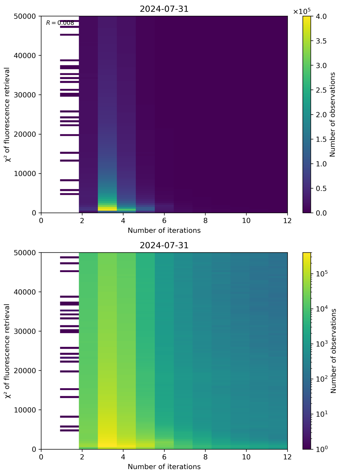
Figure 97: Scatter density plot of “Number of iterations” against “ \chi^2 of fluorescence retrieval” for 2024-07-31 to 2024-08-01.
