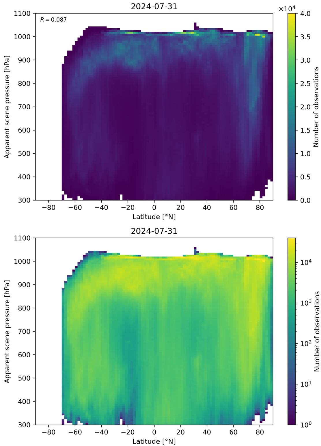
Figure 88: Scatter density plot of “Latitude” against “Apparent scene pressure” for 2024-07-31 to 2024-08-01.
