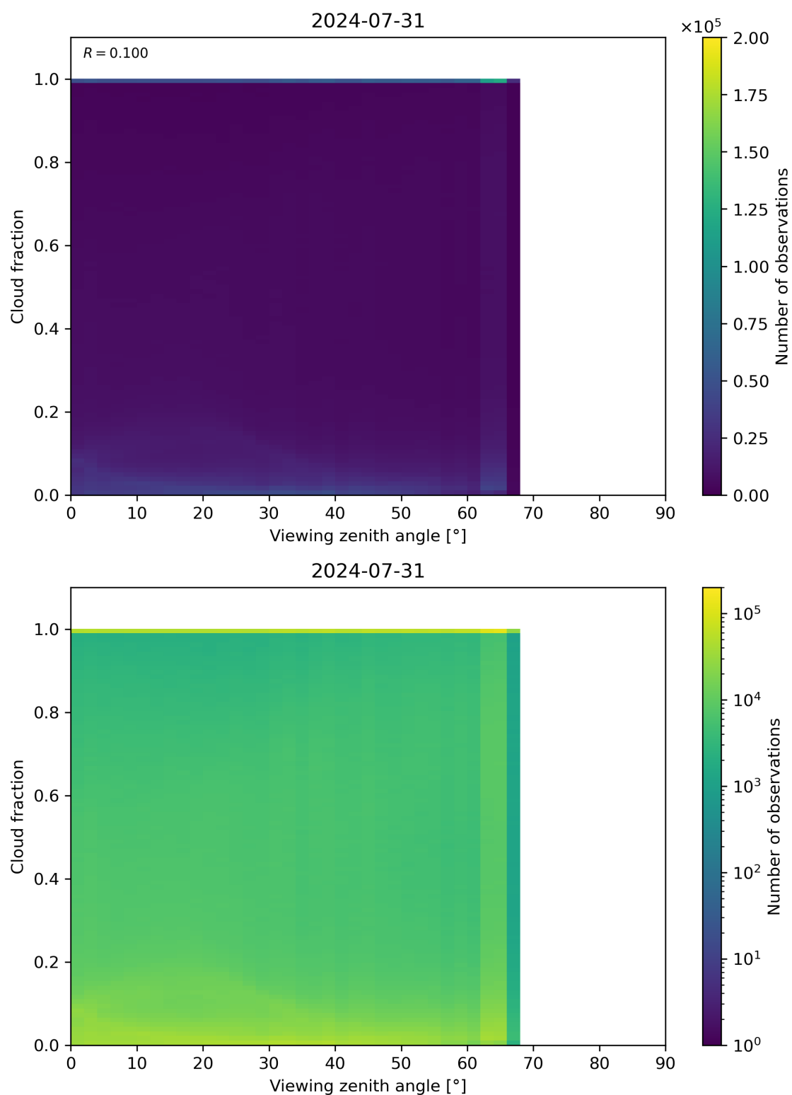
Figure 120: Scatter density plot of “Viewing zenith angle” against “Cloud fraction” for 2024-07-31 to 2024-08-01.
