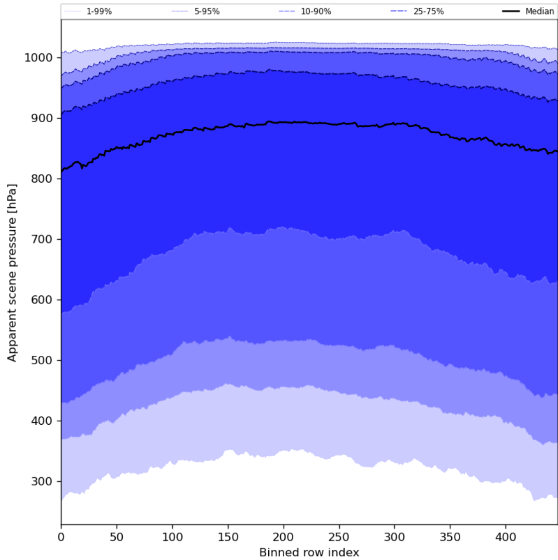
Figure 53: Along track statistics of “Apparent scene pressure” for 2024-07-31 to 2024-08-01
