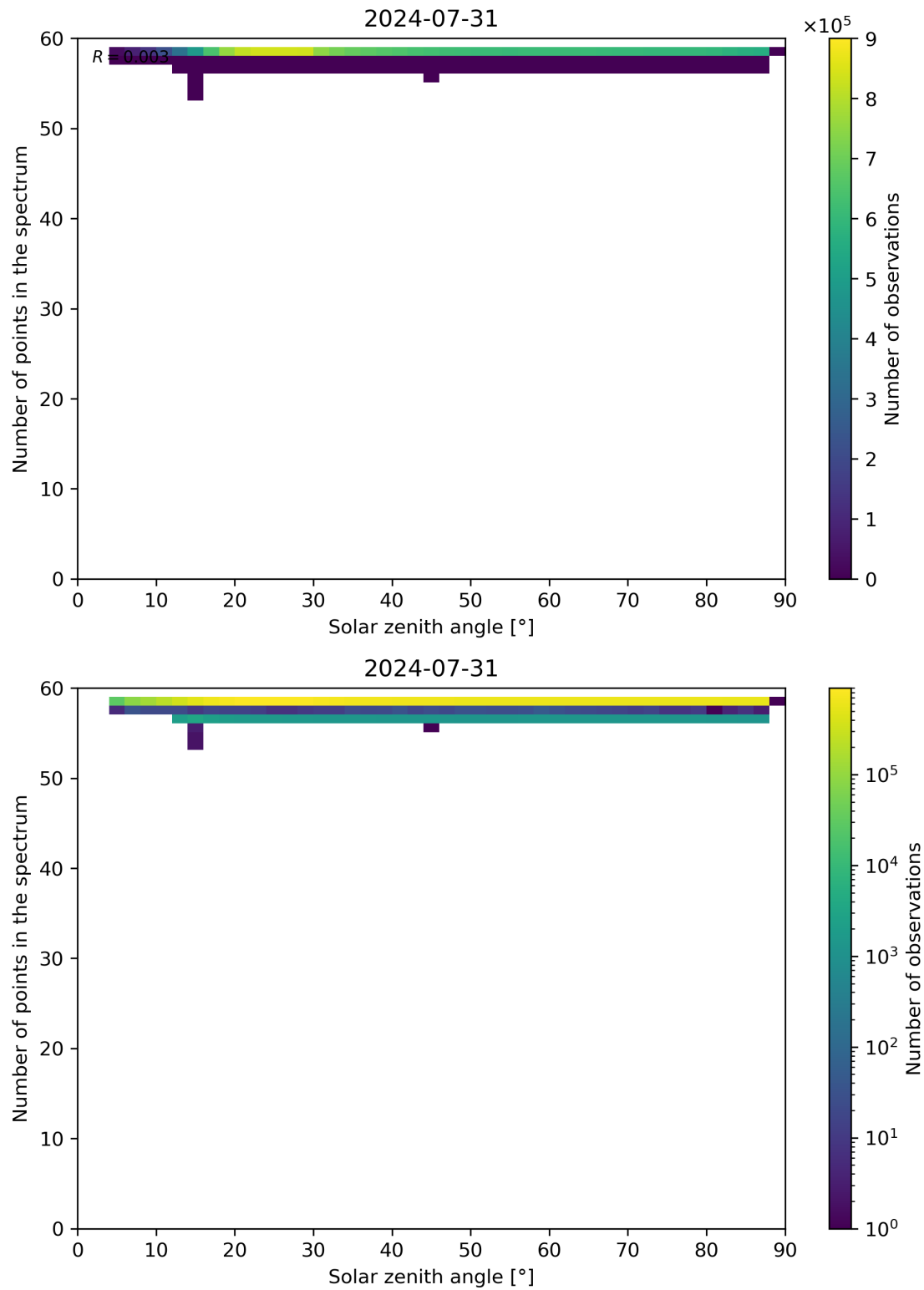
Figure 115: Scatter density plot of “Solar zenith angle” against “Number of points in the spectrum” for 2024-07-31 to 2024-08-01.
