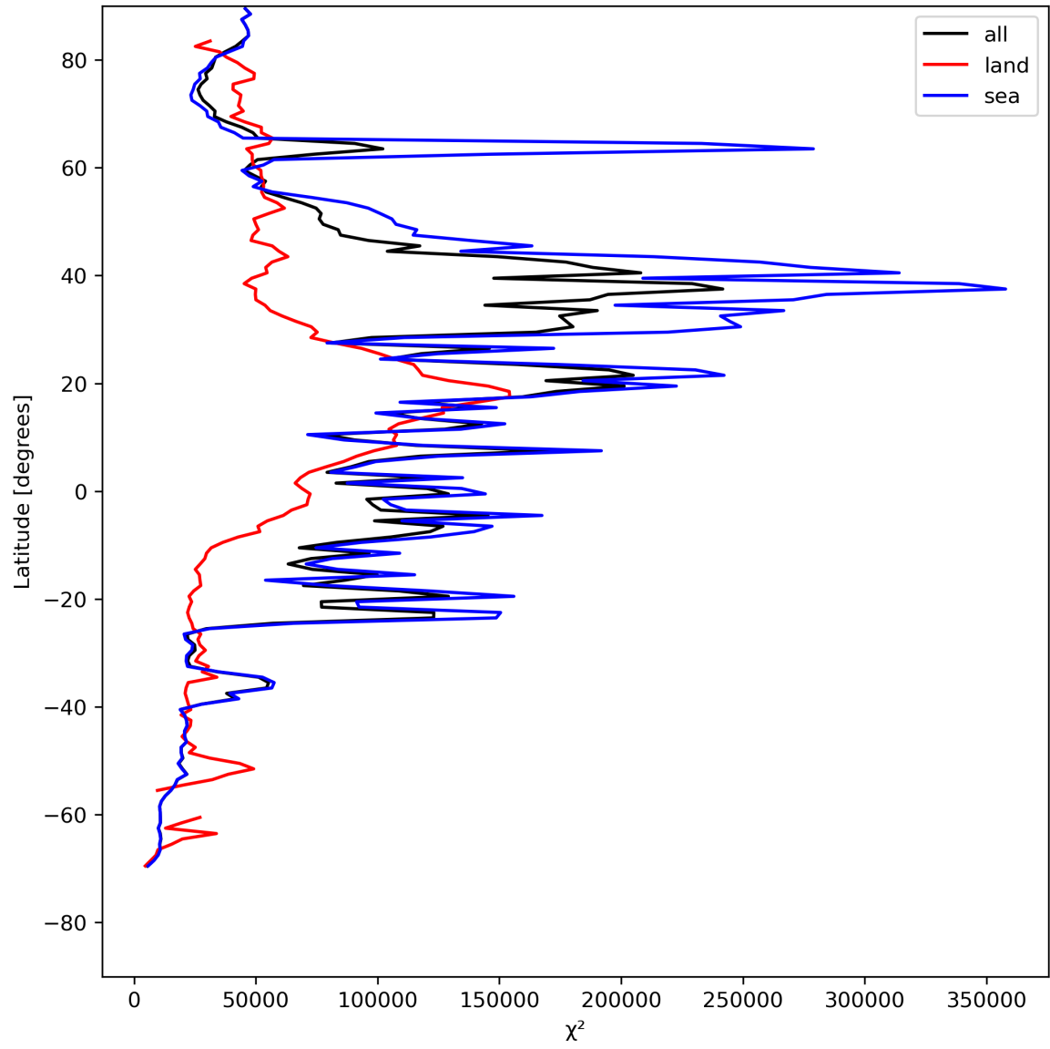
Figure 21: Zonal average of “ \chi^2 ” for 2024-07-31 to 2024-08-01.
