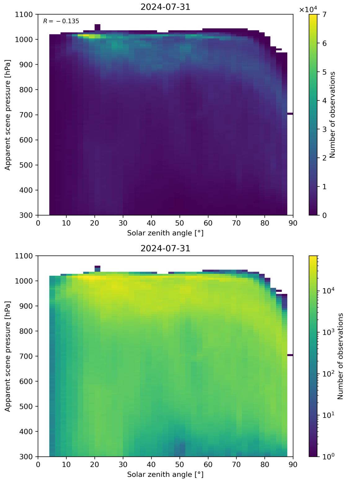
Figure 108: Scatter density plot of “Solar zenith angle” against “Apparent scene pressure” for 2024-07-31 to 2024-08-01.
