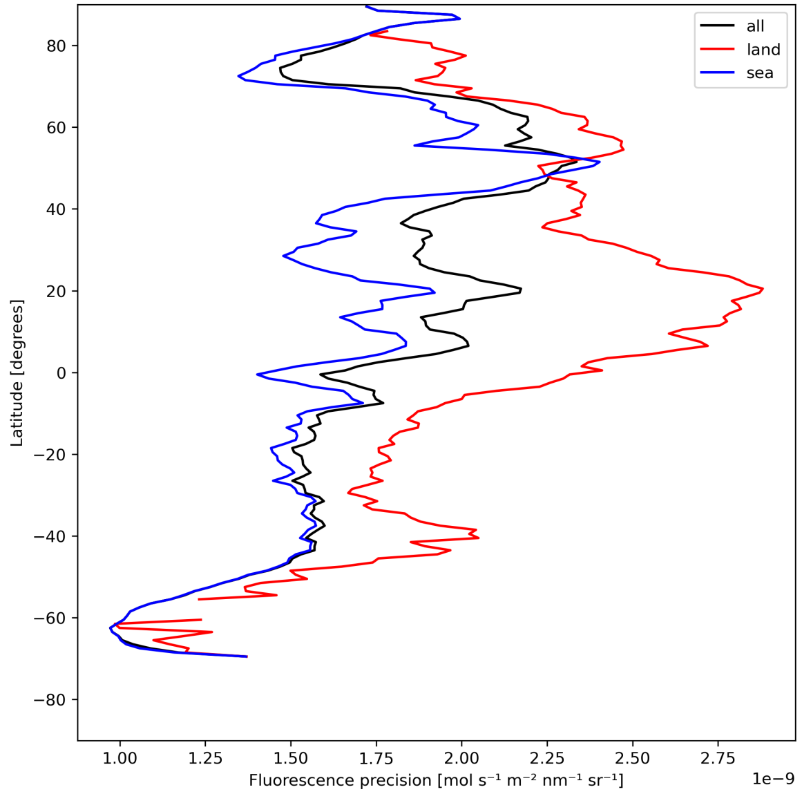
Figure 24: Zonal average of “Fluorescence precision” for 2024-07-31 to 2024-08-01.
