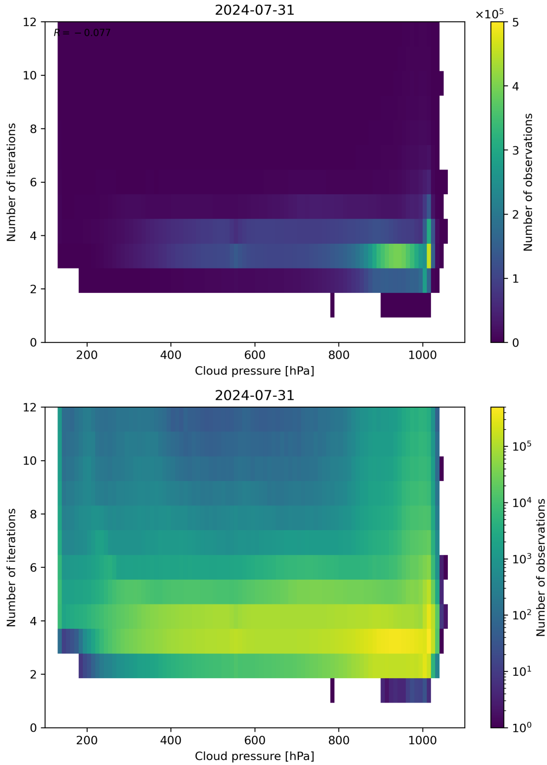
Figure 81: Scatter density plot of “Cloud pressure” against “Number of iterations” for 2024-07-31 to 2024-08-01.
