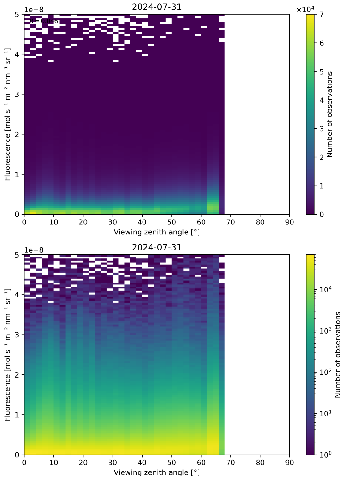
Figure 122: Scatter density plot of “Viewing zenith angle” against “Fluorescence” for 2024-07-31 to 2024-08-01.
