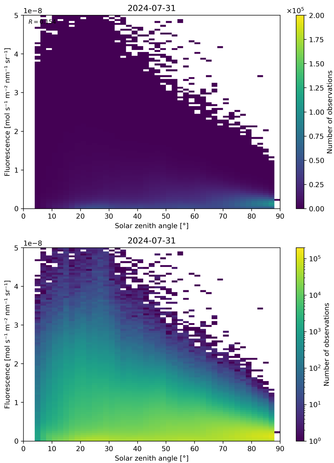
Figure 112: Scatter density plot of “Solar zenith angle” against “Fluorescence” for 2024-07-31 to 2024-08-01.
