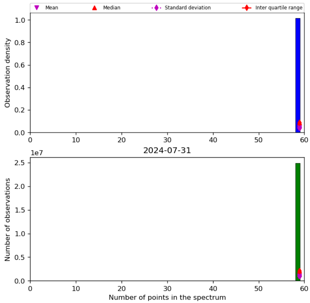
Figure 44: Histogram of “Number of points in the spectrum” for 2024-07-31 to 2024-08-01
