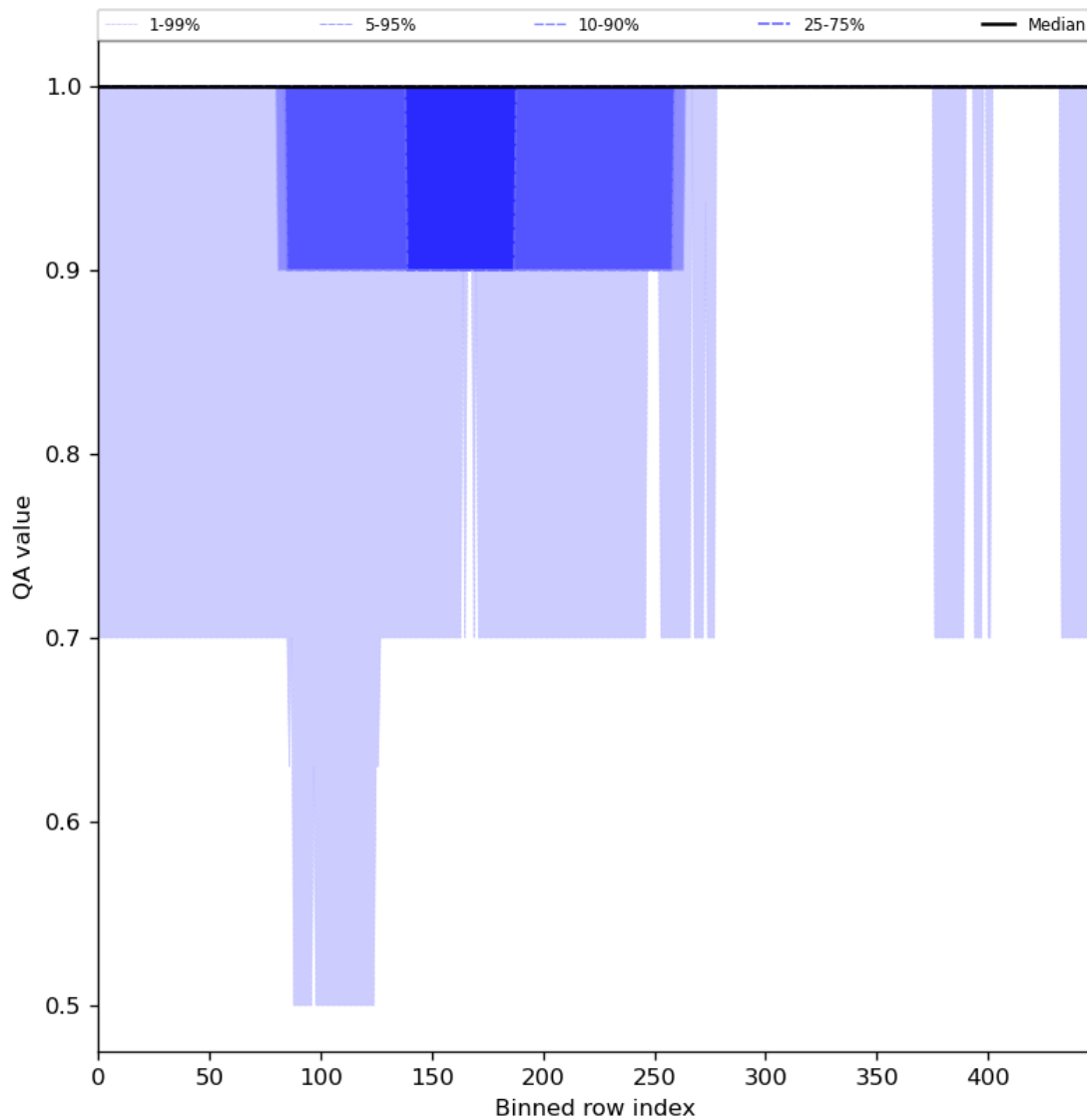
Figure 46: Along track statistics of “QA value” for 2024-07-31 to 2024-08-01
