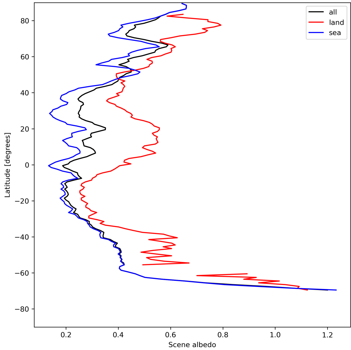
Figure 17: Zonal average of “Scene albedo” for 2024-07-31 to 2024-08-01.
