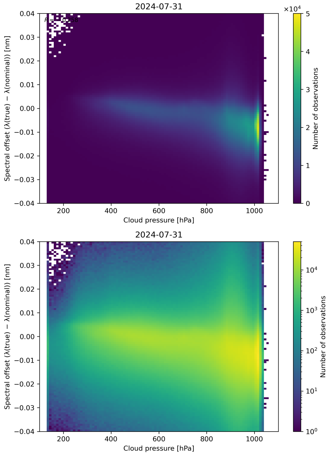
Figure 84: Scatter density plot of “Cloud pressure” against “Spectral offset ( \lambda(\text{true}) - \lambda(\text{nominal}) )” for 2024-07-31 to 2024-08-01.
