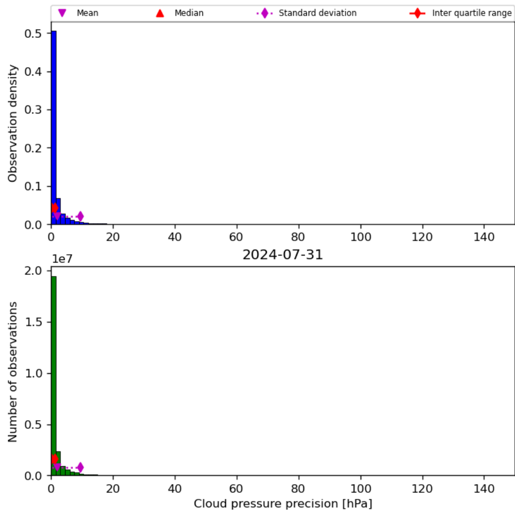
Figure 31: Histogram of “Cloud pressure precision” for 2024-07-31 to 2024-08-01
