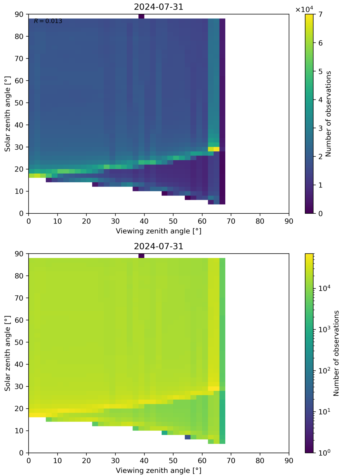
Figure 127: Scatter density plot of “Viewing zenith angle” against “Solar zenith angle” for 2024-07-31 to 2024-08-01.
