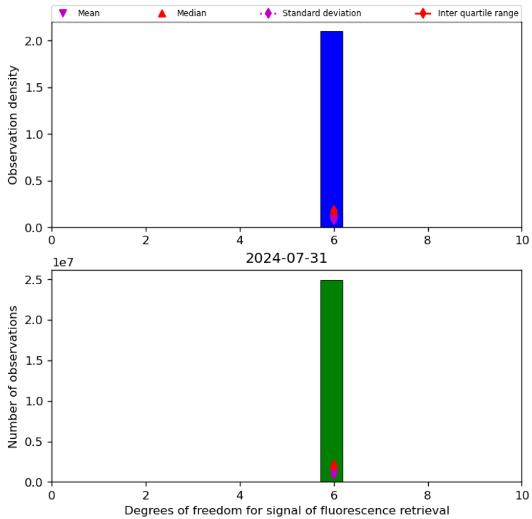
Figure 43: Histogram of “Degrees of freedom for signal of fluorescence retrieval” for 2024-07-31 to 2024-08-01
