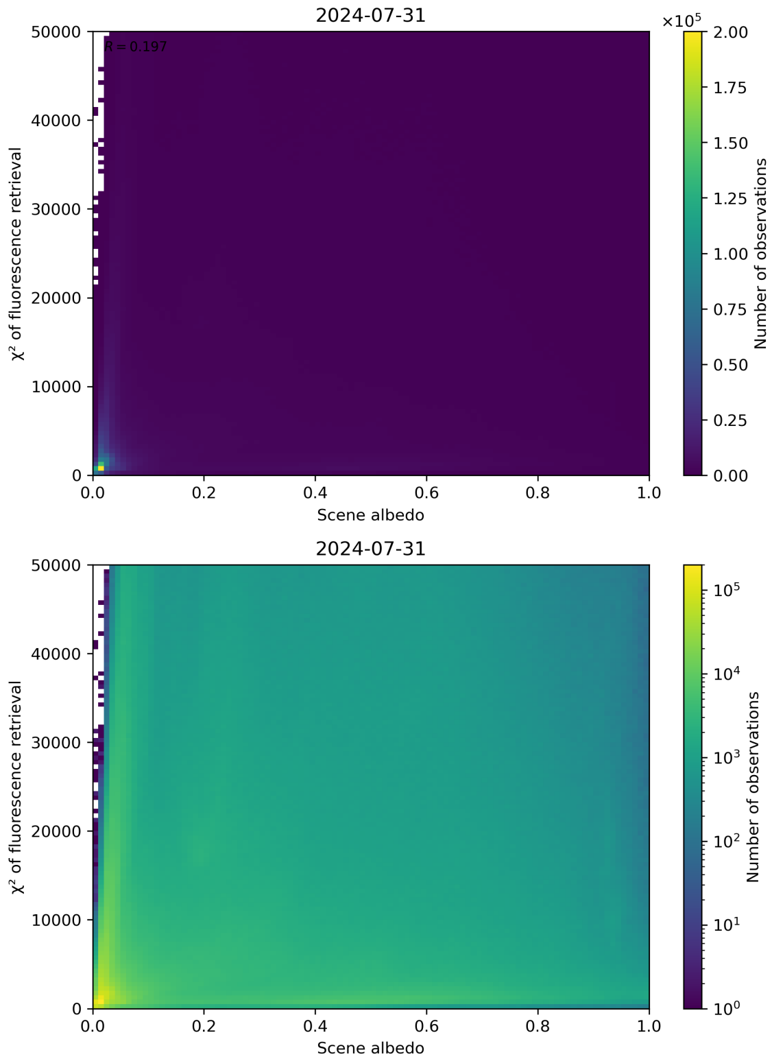
Figure 103: Scatter density plot of “Scene albedo” against “ \chi^2 of fluorescence retrieval” for 2024-07-31 to 2024-08-01.
