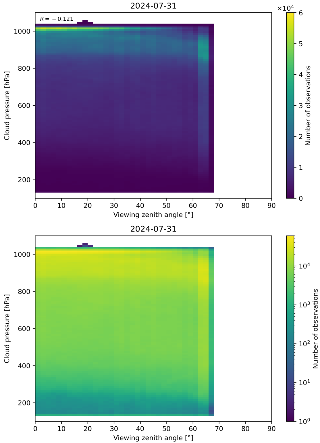
Figure 121: Scatter density plot of “Viewing zenith angle” against “Cloud pressure” for 2024-07-31 to 2024-08-01.
