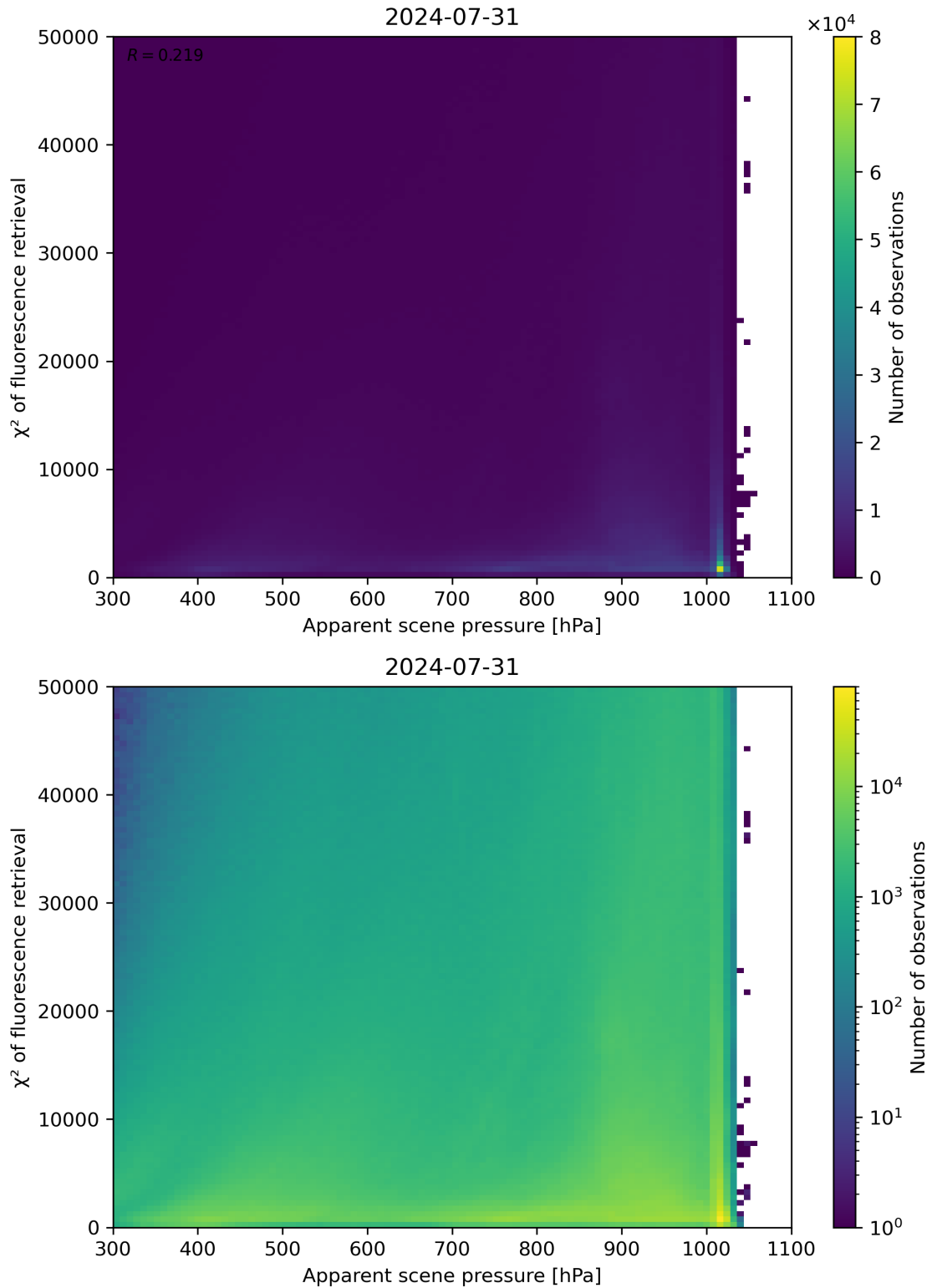
Figure 63: Scatter density plot of “Apparent scene pressure” against “ \chi^2 of fluorescence retrieval” for 2024-07-31 to 2024-08-01.
