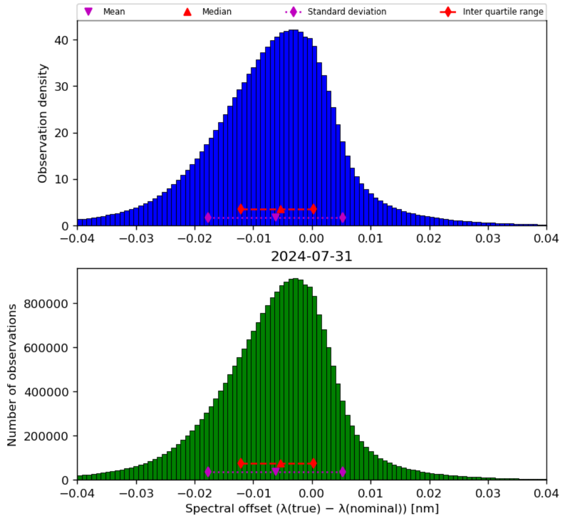
Figure 45: Histogram of “Spectral offset ( \lambda(\text{true}) - \lambda(\text{nominal}) )” for 2024-07-31 to 2024-08-01
