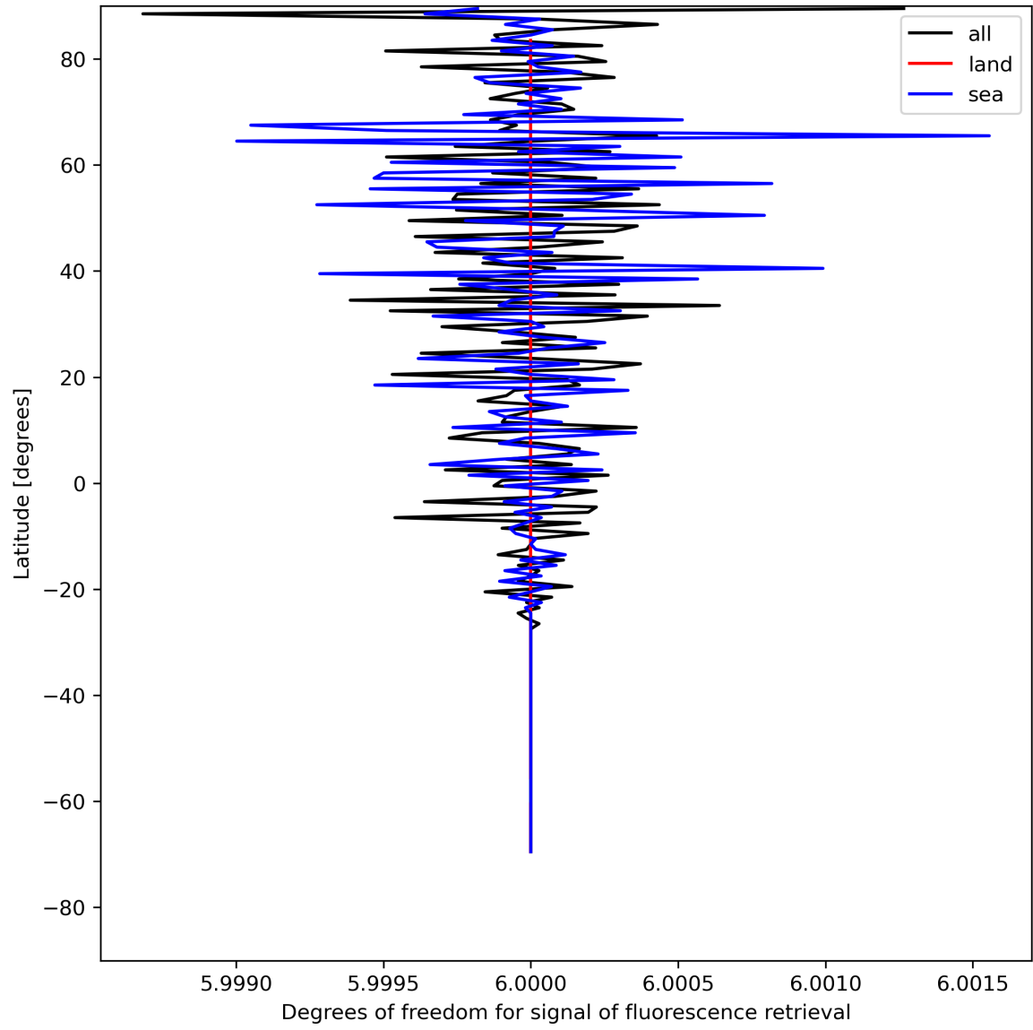
Figure 26: Zonal average of “Degrees of freedom for signal of fluorescence retrieval” for 2024-07-31 to 2024-08-01.
