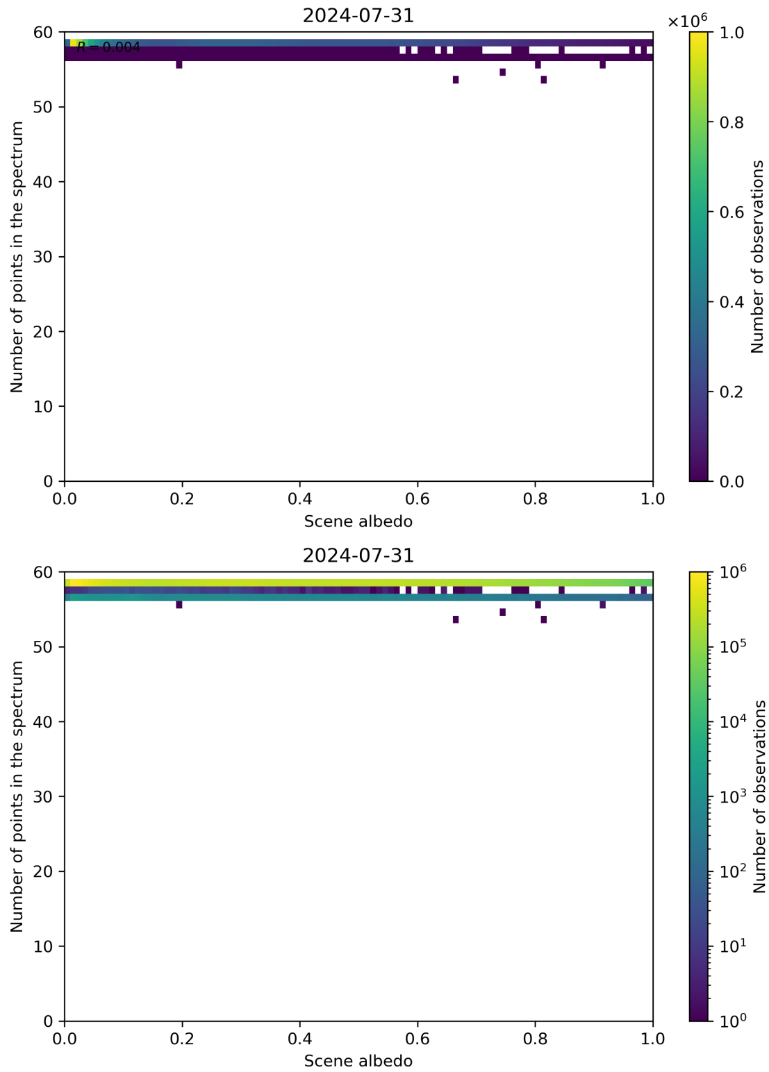
Figure 106: Scatter density plot of “Scene albedo” against “Number of points in the spectrum” for 2024-07-31 to 2024-08-01.
