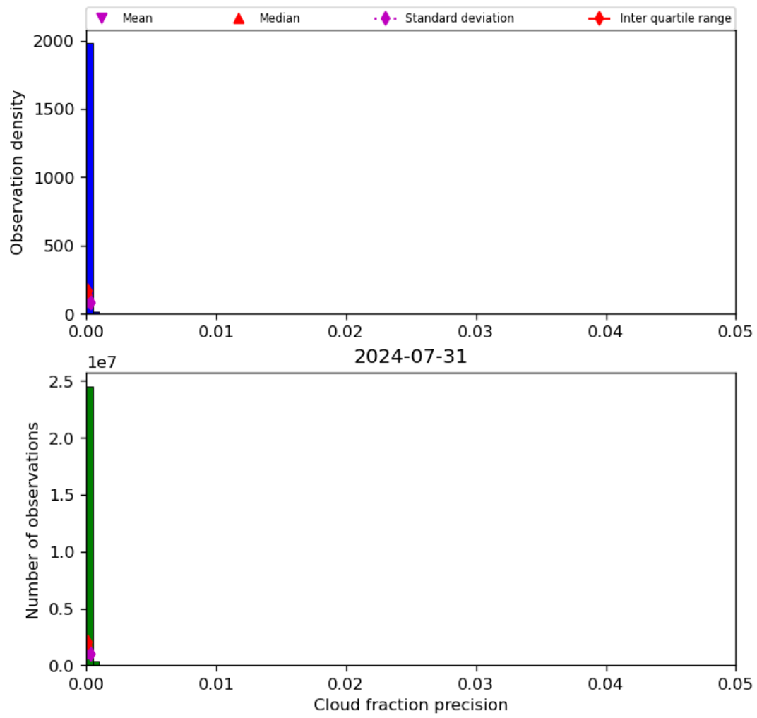
Figure 33: Histogram of “Cloud fraction precision” for 2024-07-31 to 2024-08-01
