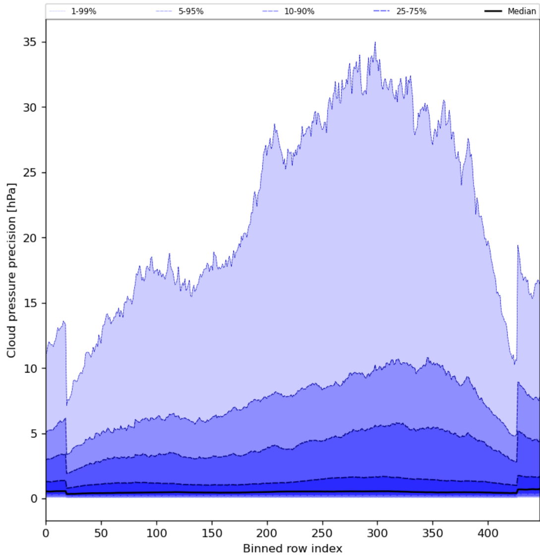
Figure 48: Along track statistics of “Cloud pressure precision” for 2024-07-31 to 2024-08-01
