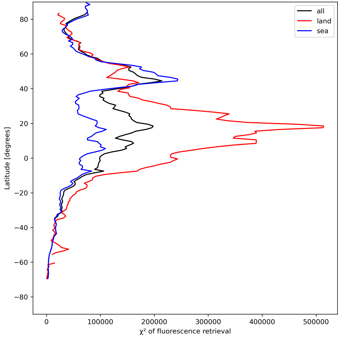
Figure 25: Zonal average of “ \chi^2 of fluorescence retrieval” for 2024-07-31 to 2024-08-01.
