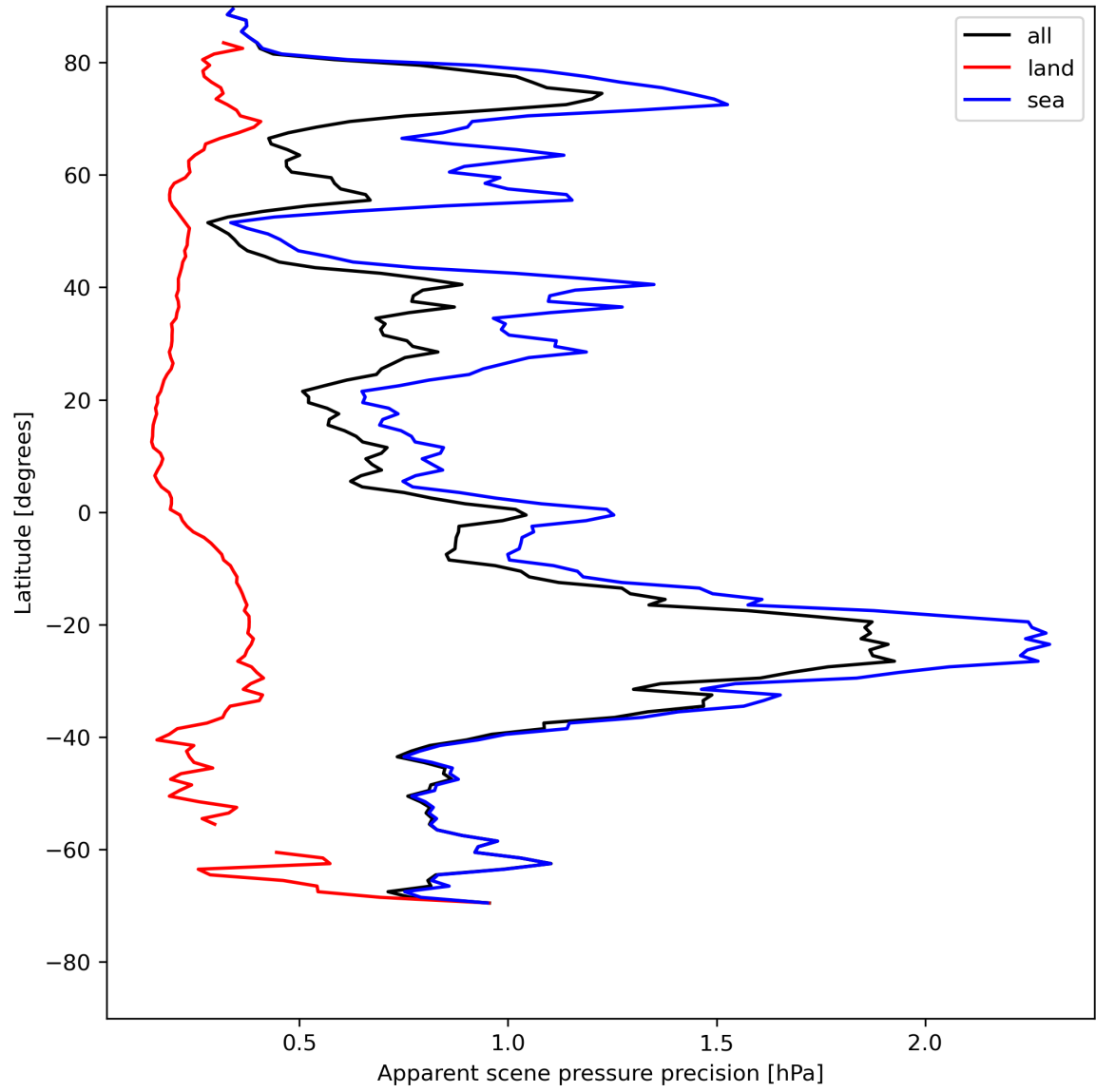
Figure 20: Zonal average of “Apparent scene pressure precision” for 2024-07-31 to 2024-08-01.
