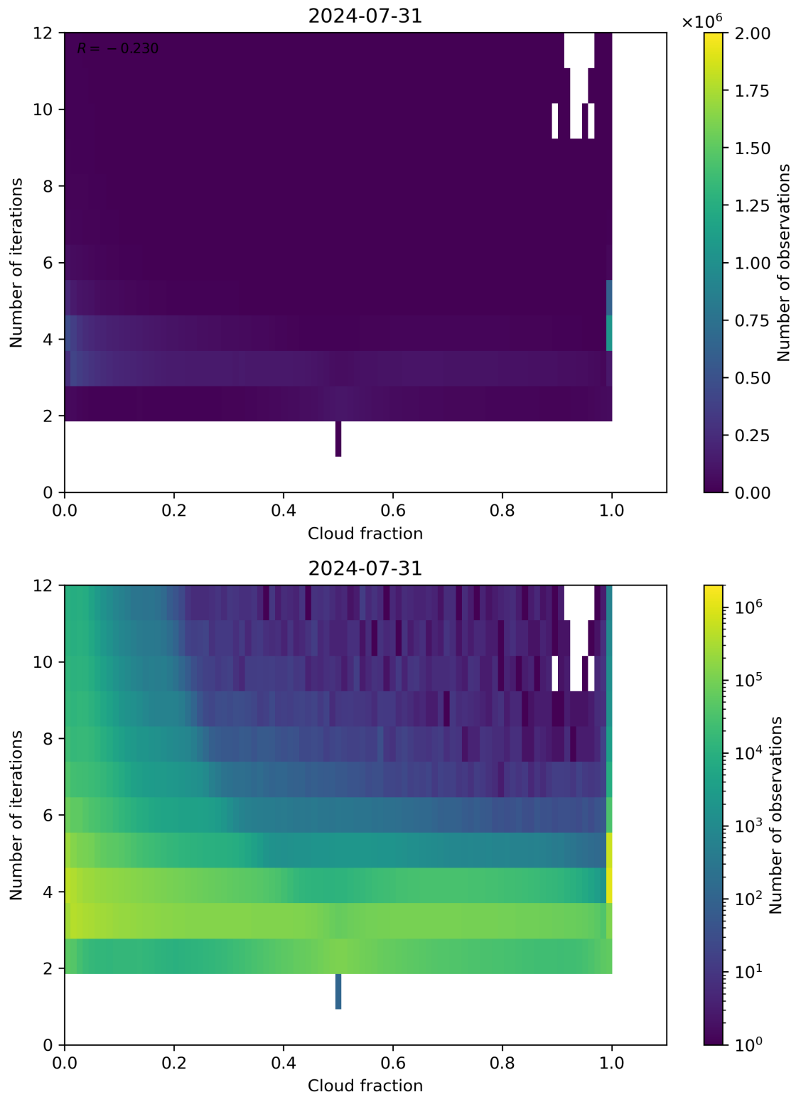
Figure 73: Scatter density plot of “Cloud fraction” against “Number of iterations” for 2024-07-31 to 2024-08-01.
