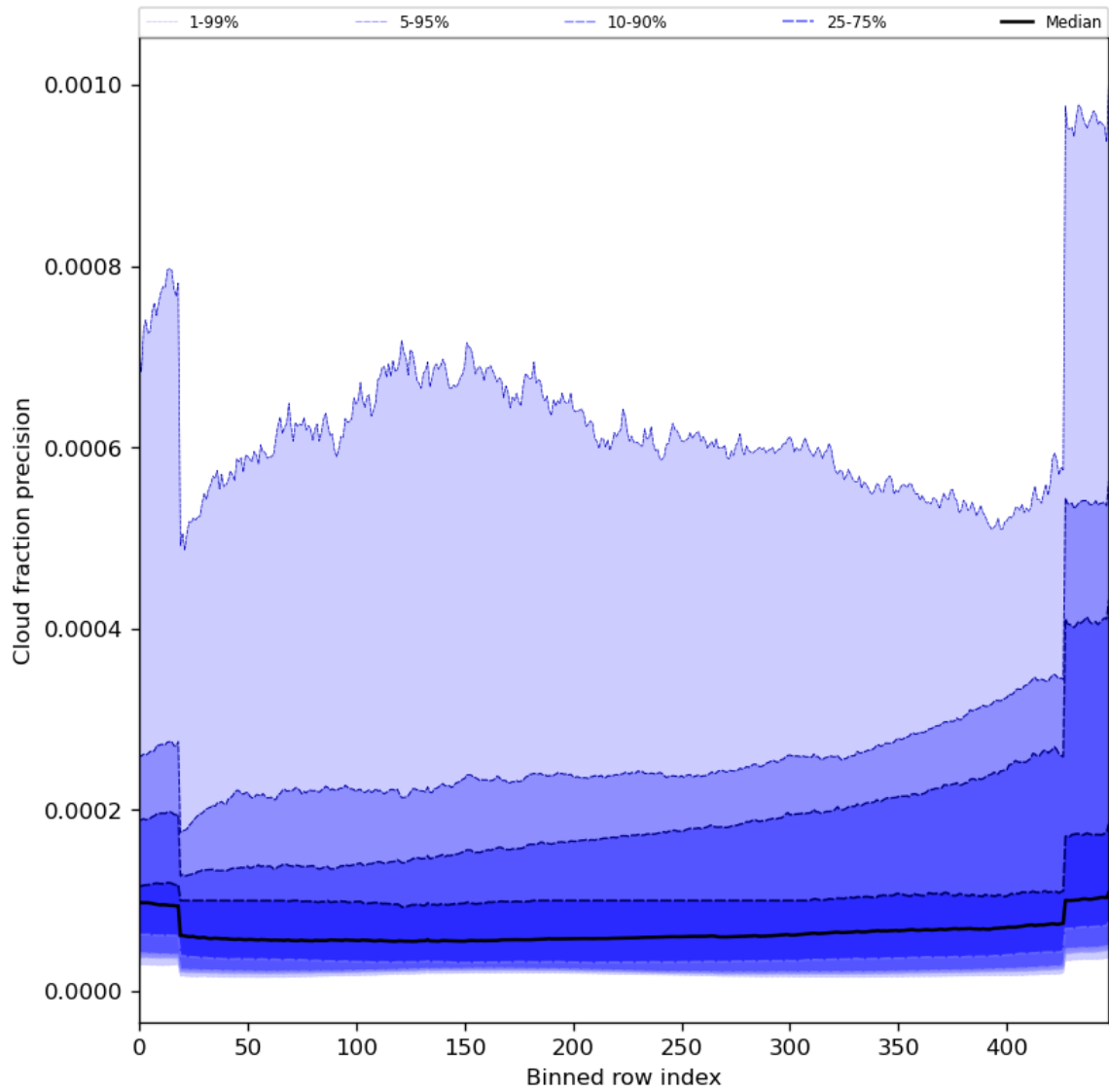
Figure 50: Along track statistics of “Cloud fraction precision” for 2024-07-31 to 2024-08-01
