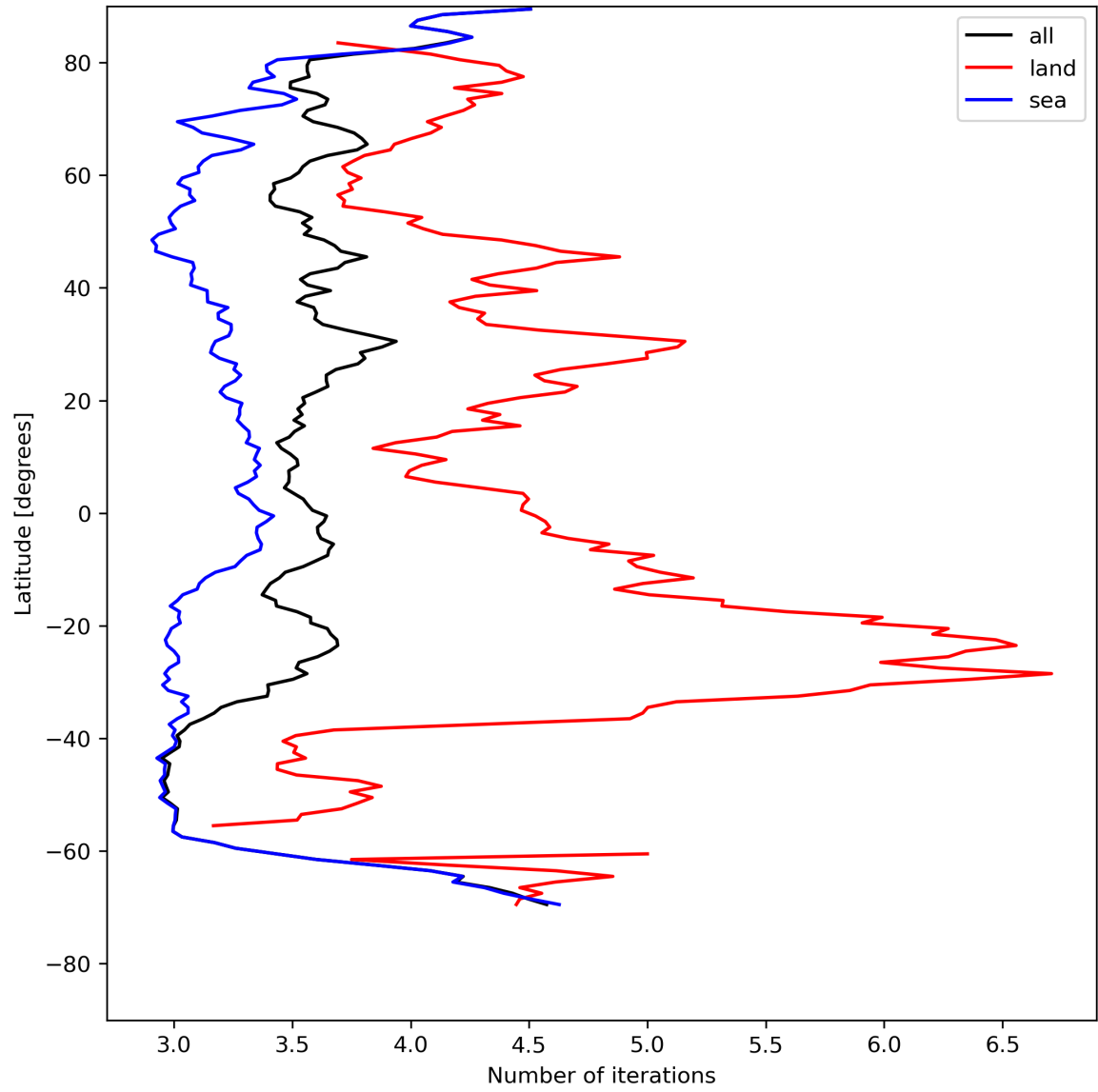
Figure 22: Zonal average of “Number of iterations” for 2024-07-31 to 2024-08-01.
