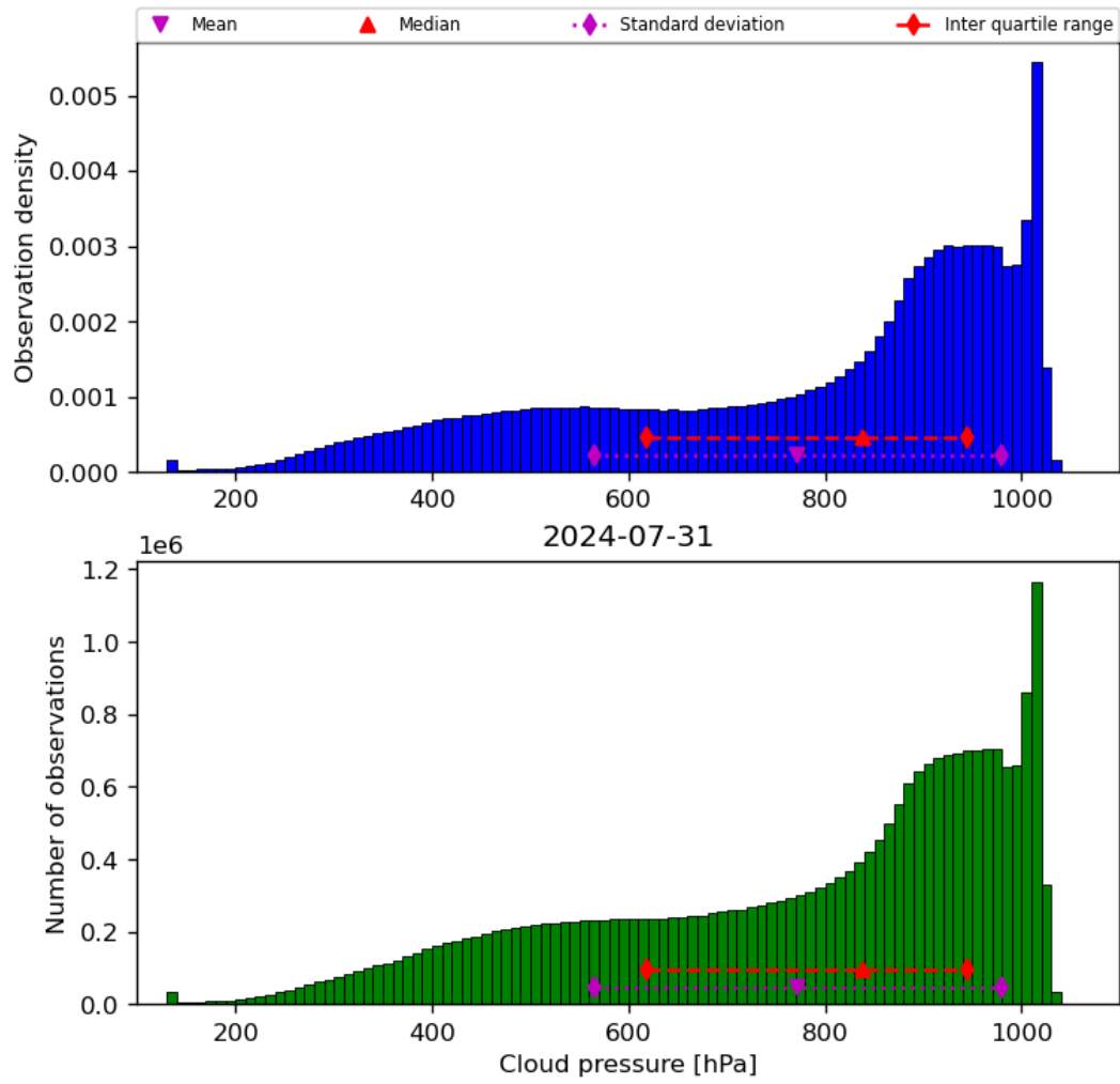
Figure 30: Histogram of “Cloud pressure” for 2024-07-31 to 2024-08-01
