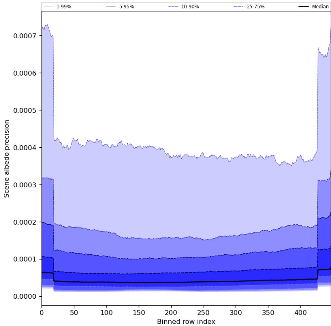
Figure 52: Along track statistics of “Scene albedo precision” for 2024-07-31 to 2024-08-01
