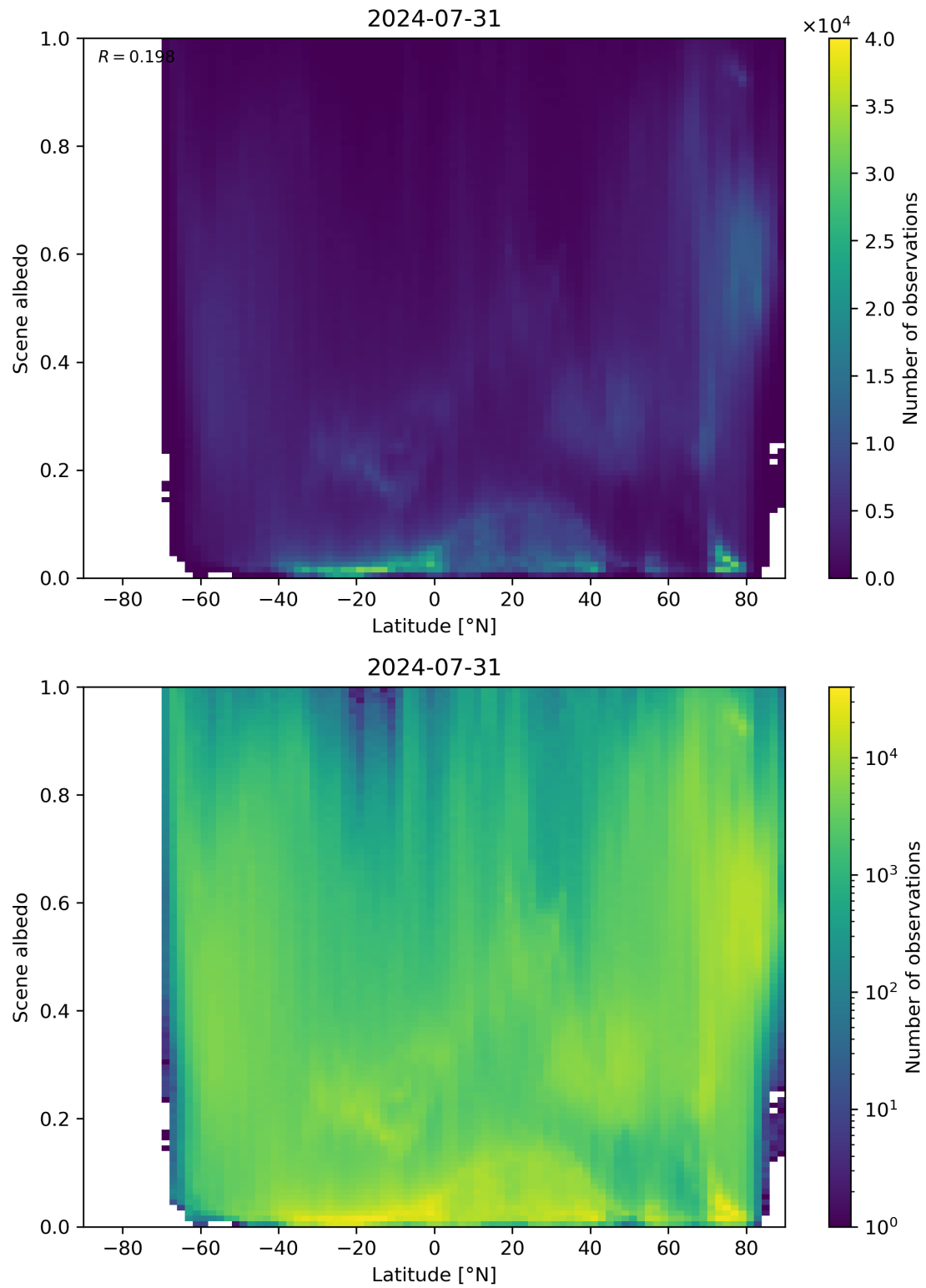
Figure 95: Scatter density plot of “Latitude” against “Scene albedo” for 2024-07-31 to 2024-08-01.
