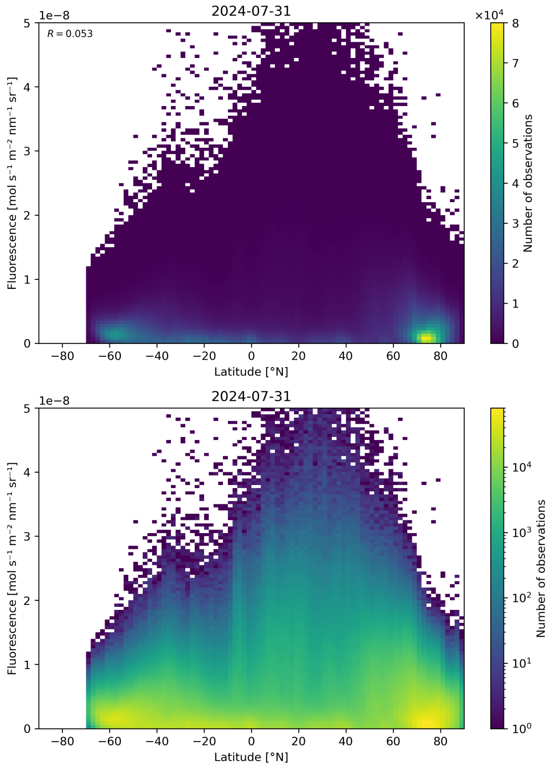
Figure 92: Scatter density plot of “Latitude” against “Fluorescence” for 2024-07-31 to 2024-08-01.
