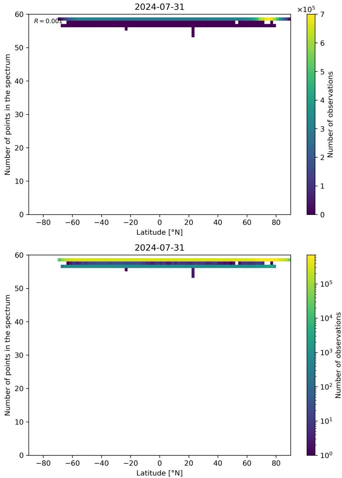
Figure 94: Scatter density plot of “Latitude” against “Number of points in the spectrum” for 2024-07-31 to 2024-08-01.
