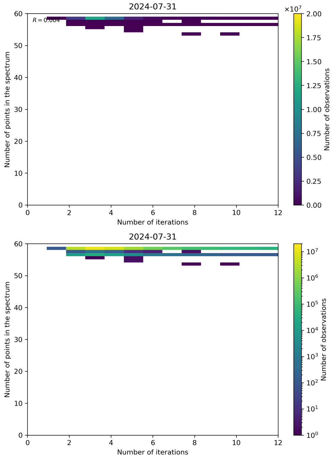
Figure 99: Scatter density plot of “Number of iterations” against “Number of points in the spectrum” for 2024-07-31 to 2024-08-01.
