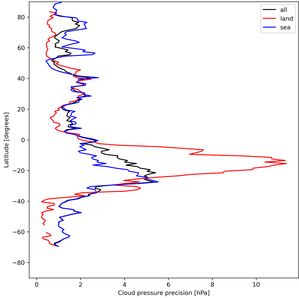
Figure 14: Zonal average of “Cloud pressure precision” for 2024-07-31 to 2024-08-01.
