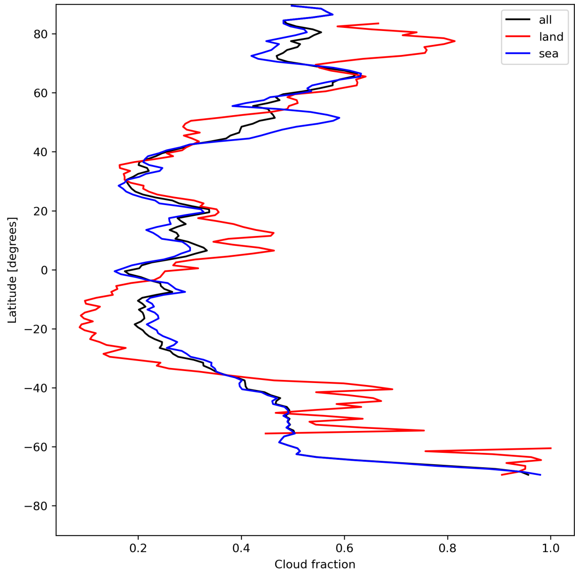
Figure 15: Zonal average of “Cloud fraction” for 2024-07-31 to 2024-08-01.
