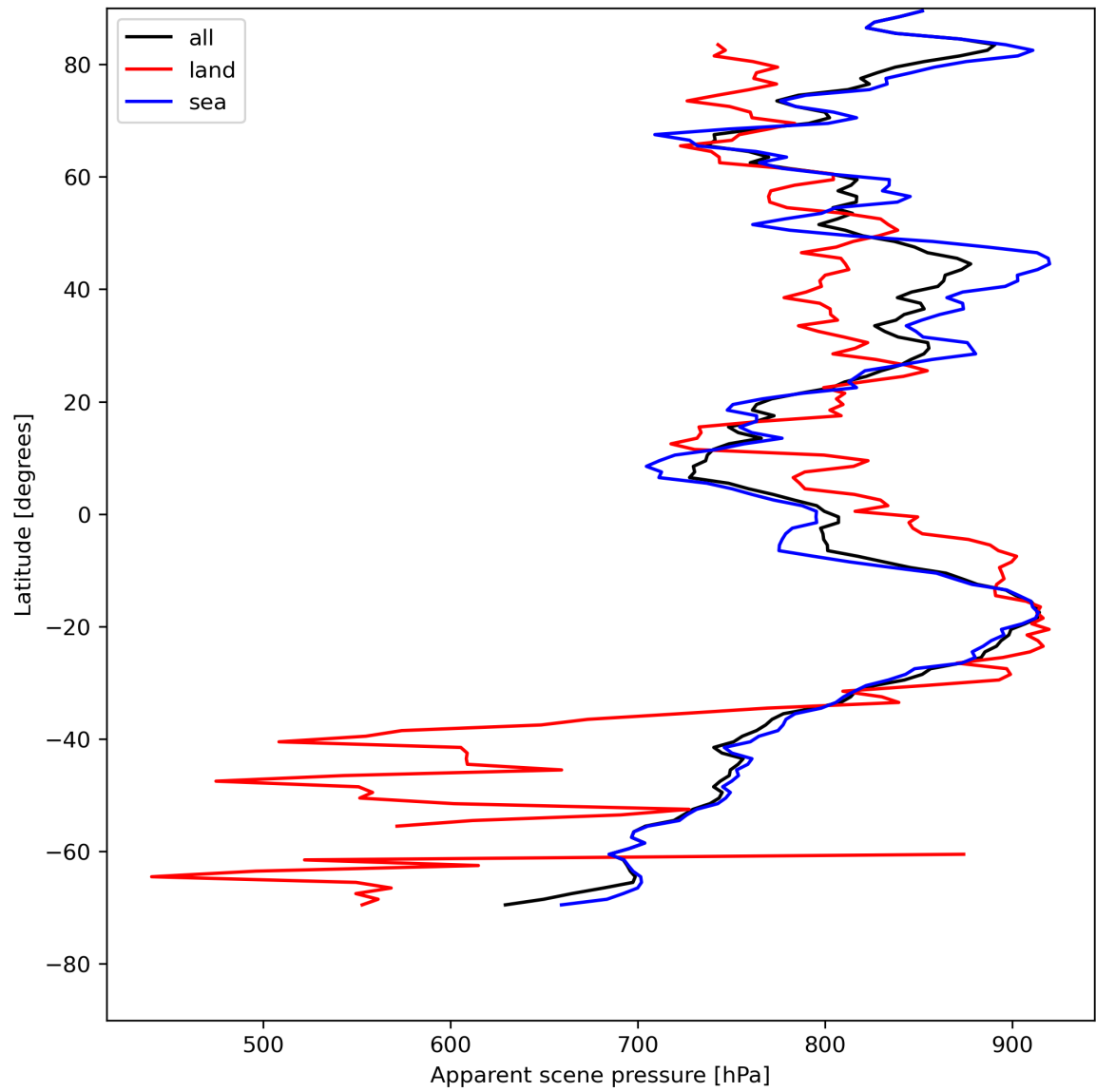
Figure 19: Zonal average of “Apparent scene pressure” for 2024-07-31 to 2024-08-01.
