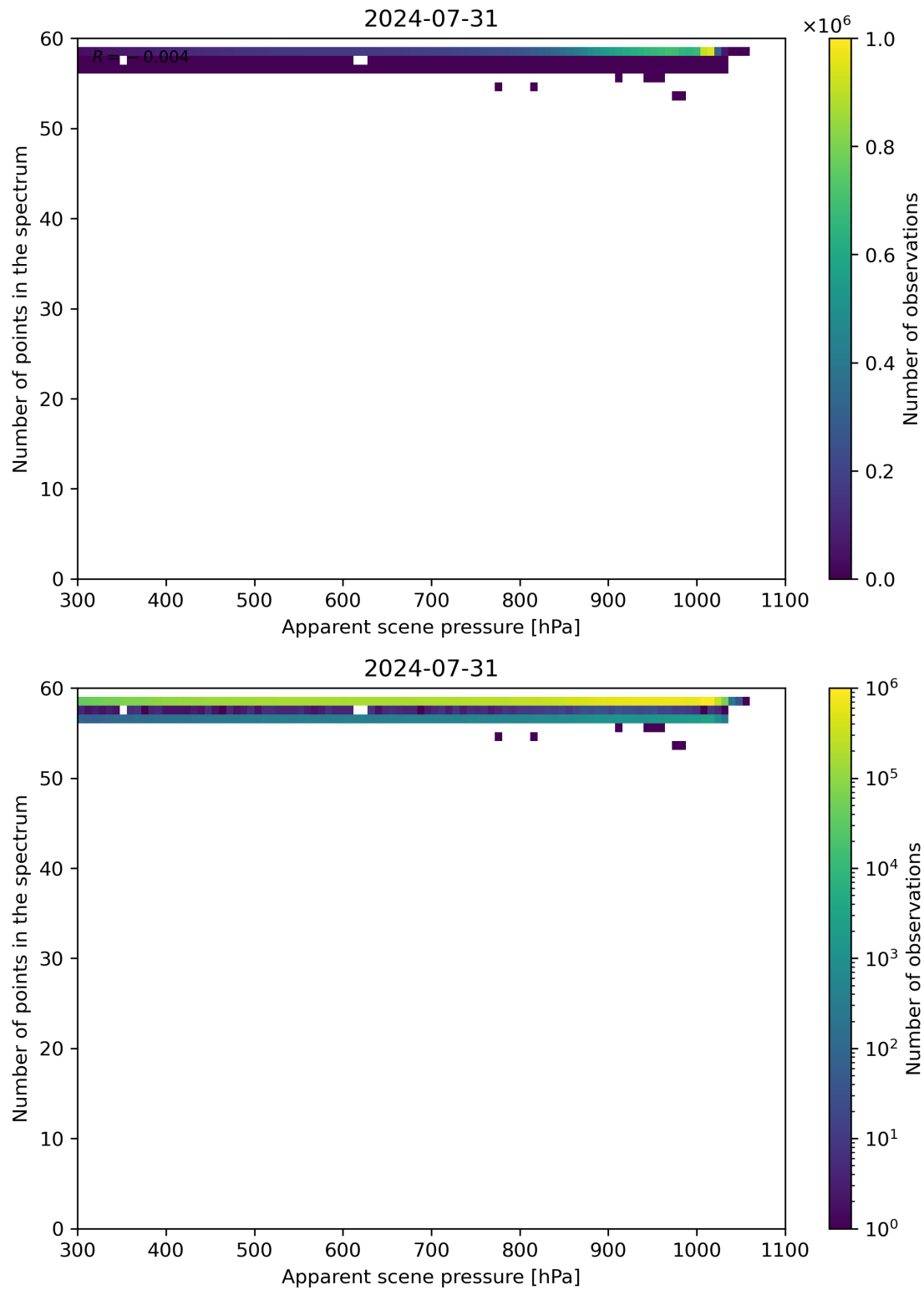
Figure 66: Scatter density plot of “Apparent scene pressure” against “Number of points in the spectrum” for 2024-07-31 to 2024-08-01.
