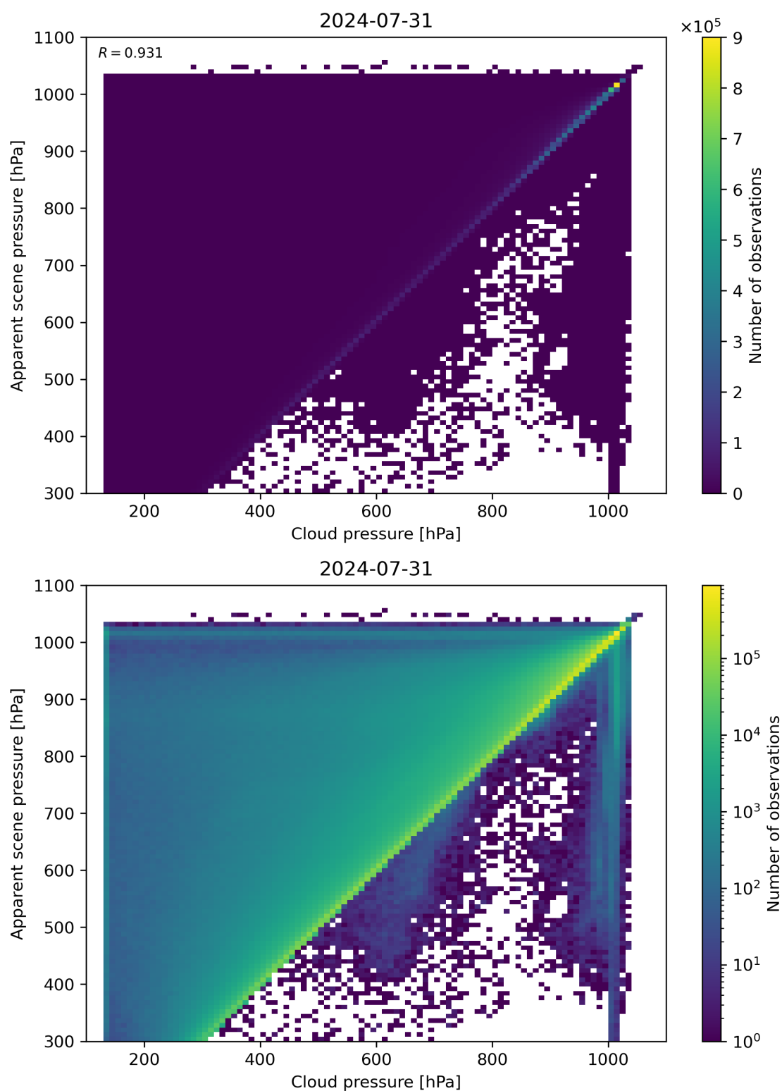
Figure 77: Scatter density plot of “Cloud pressure” against “Apparent scene pressure” for 2024-07-31 to 2024-08-01.
