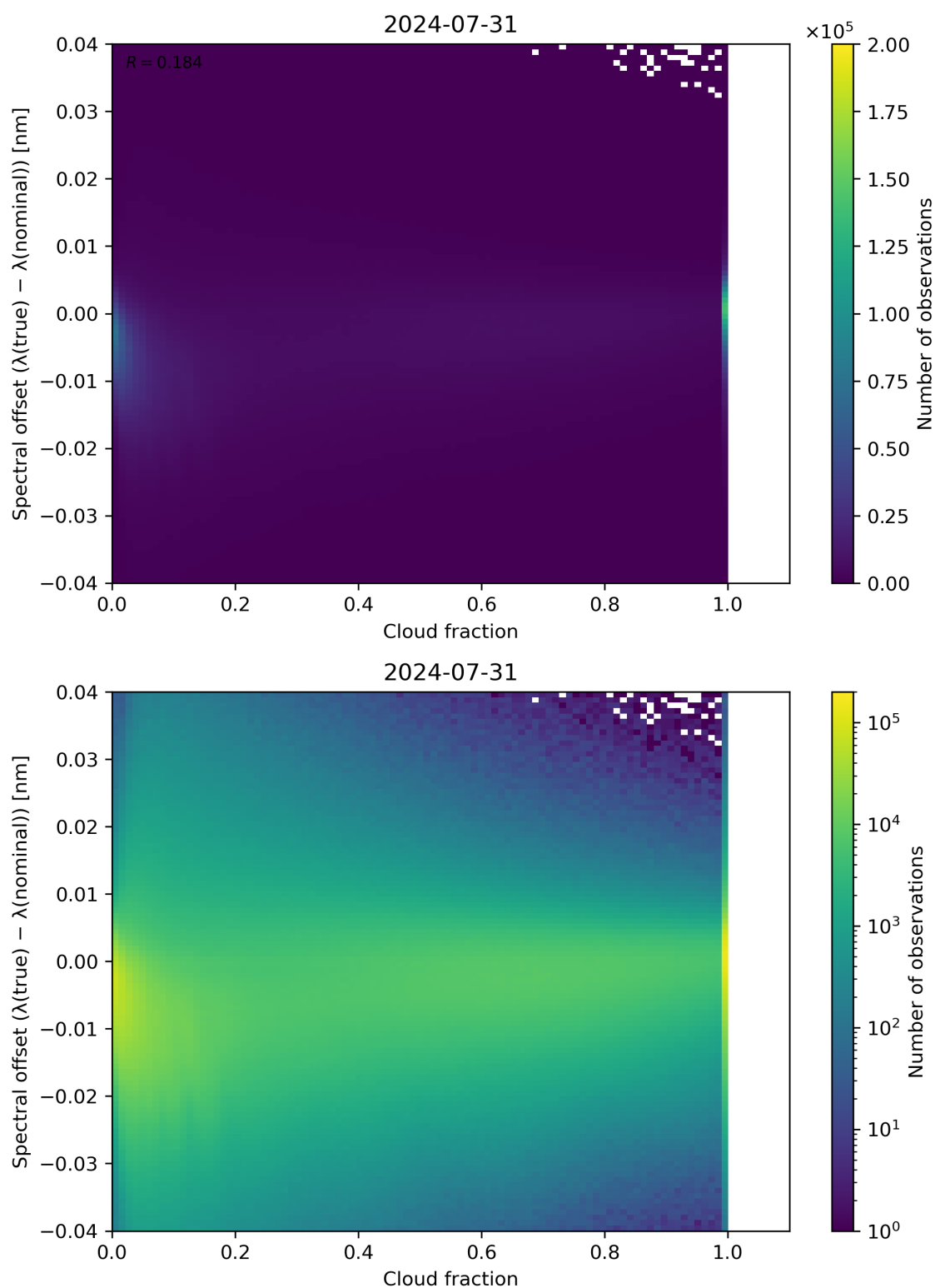
Figure 76: Scatter density plot of “Cloud fraction” against “Spectral offset ( \lambda(\text{true}) - \lambda(\text{nominal}) )” for 2024-07-31 to 2024-08-01.
