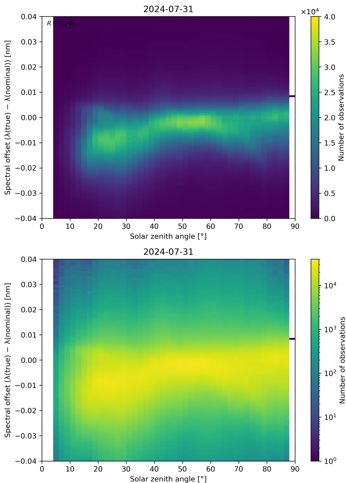
Figure 117: Scatter density plot of “Solar zenith angle” against “Spectral offset ( \lambda(\text{true}) - \lambda(\text{nominal}) )” for 2024-07-31 to 2024-08-01.
