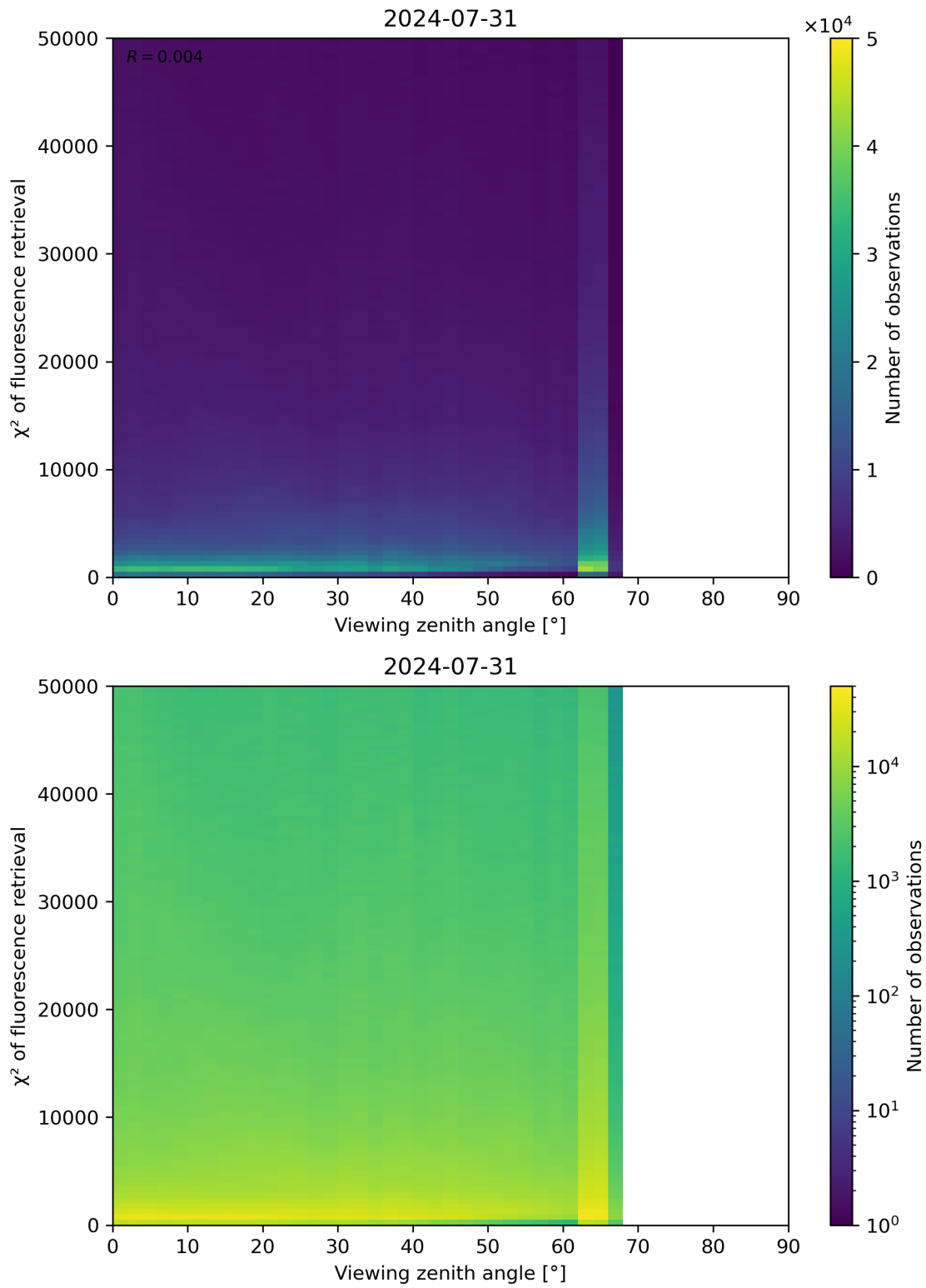
Figure 119: Scatter density plot of “Viewing zenith angle” against “ \chi^2 of fluorescence retrieval” for 2024-07-31 to 2024-08-01.
