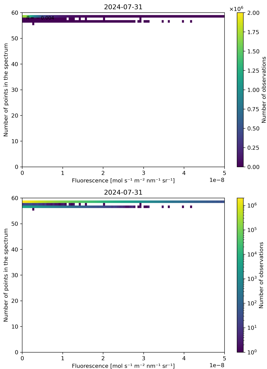
Figure 86: Scatter density plot of “Fluorescence” against “Number of points in the spectrum” for 2024-07-31 to 2024-08-01.
