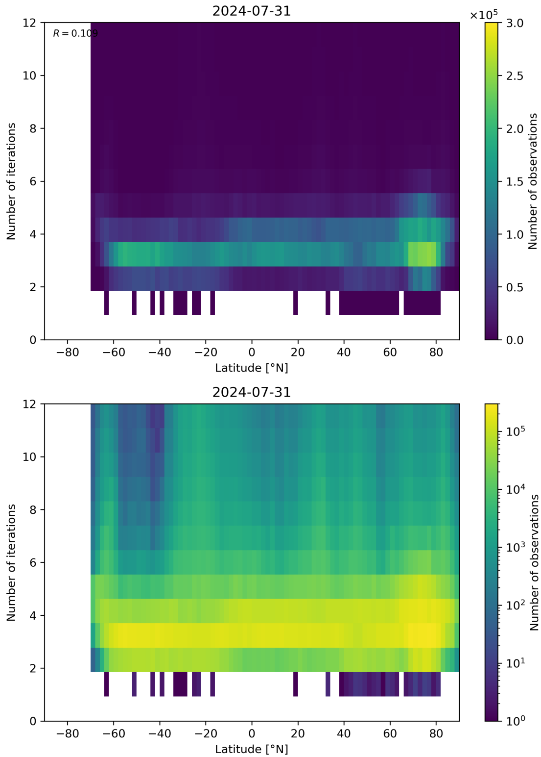
Figure 93: Scatter density plot of “Latitude” against “Number of iterations” for 2024-07-31 to 2024-08-01.
