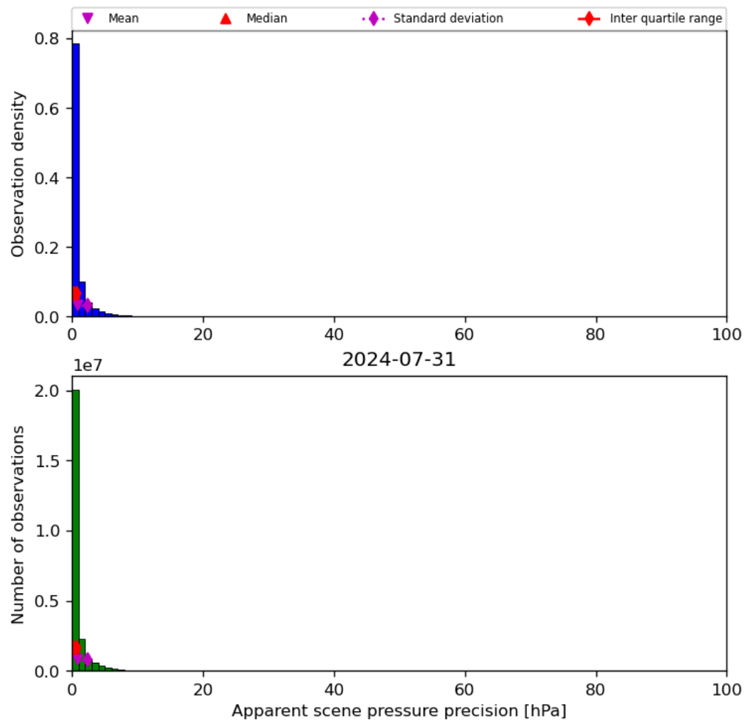
Figure 37: Histogram of “Apparent scene pressure precision” for 2024-07-31 to 2024-08-01
