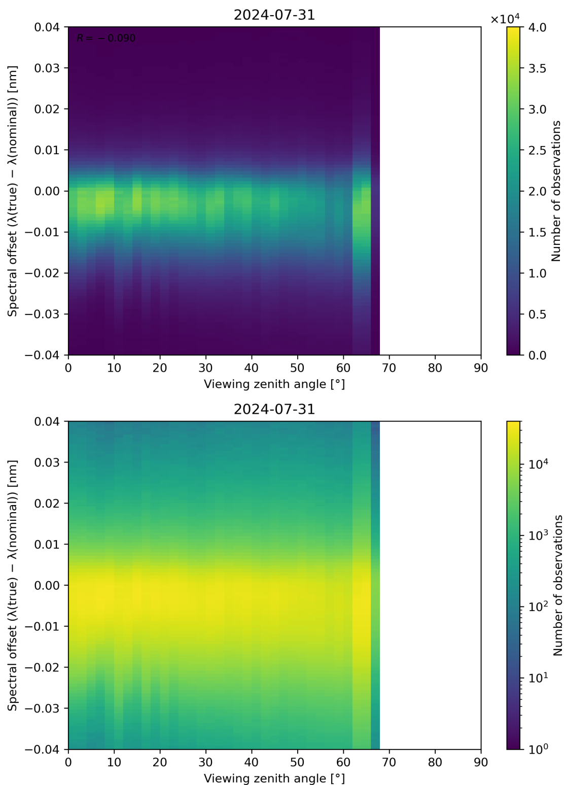
Figure 128: Scatter density plot of “Viewing zenith angle” against “Spectral offset ( \lambda(\text{true}) - \lambda(\text{nominal}) )” for 2024-07-31 to 2024-08-01.
