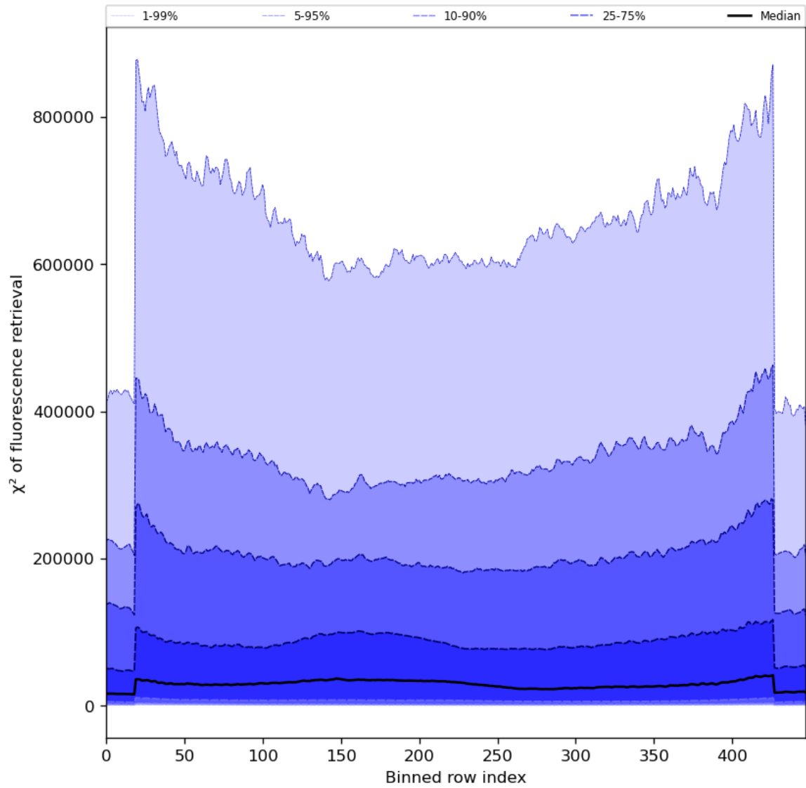
Figure 59: Along track statistics of “ \chi^2 of fluorescence retrieval” for 2024-07-31 to 2024-08-01
