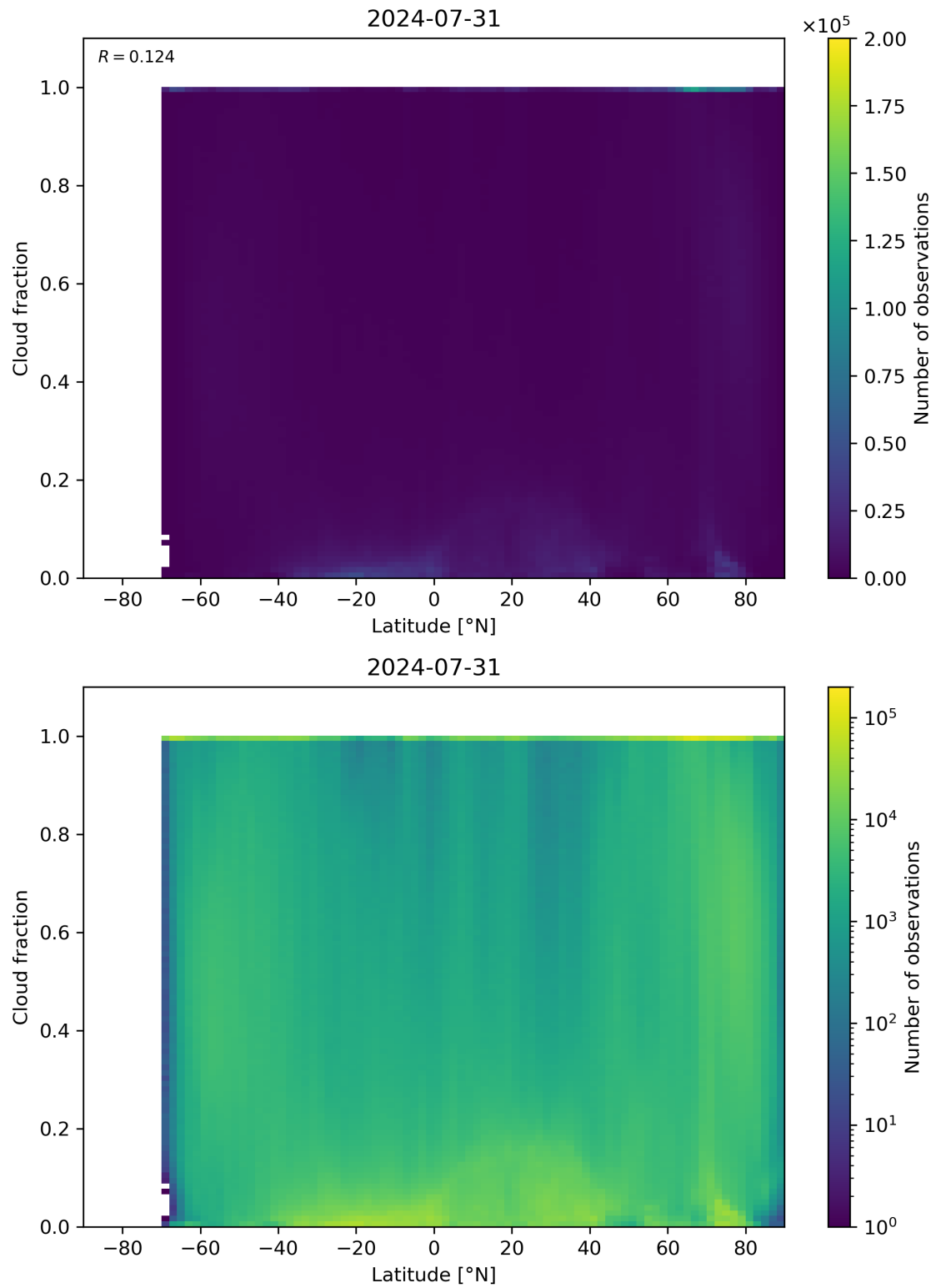
Figure 90: Scatter density plot of “Latitude” against “Cloud fraction” for 2024-07-31 to 2024-08-01.
