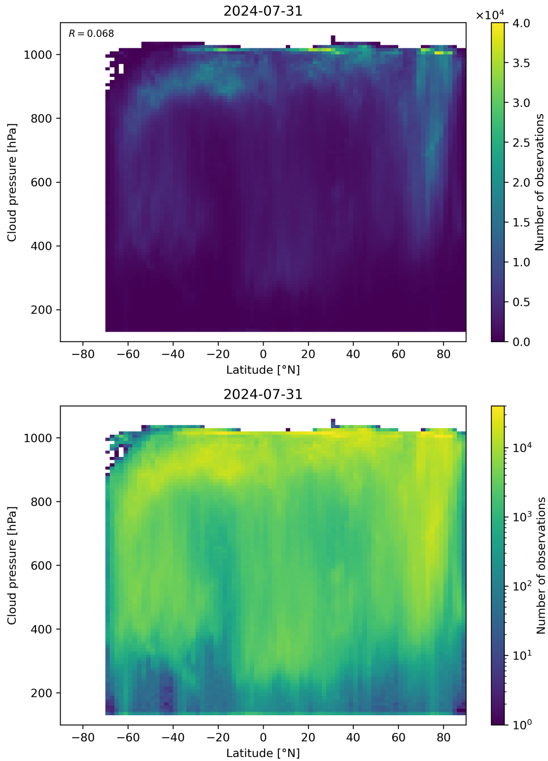
Figure 91: Scatter density plot of “Latitude” against “Cloud pressure” for 2024-07-31 to 2024-08-01.
