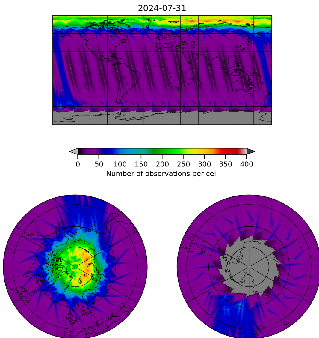
Figure 11: Map of the number of observations for 2024-07-31 to 2024-08-01
