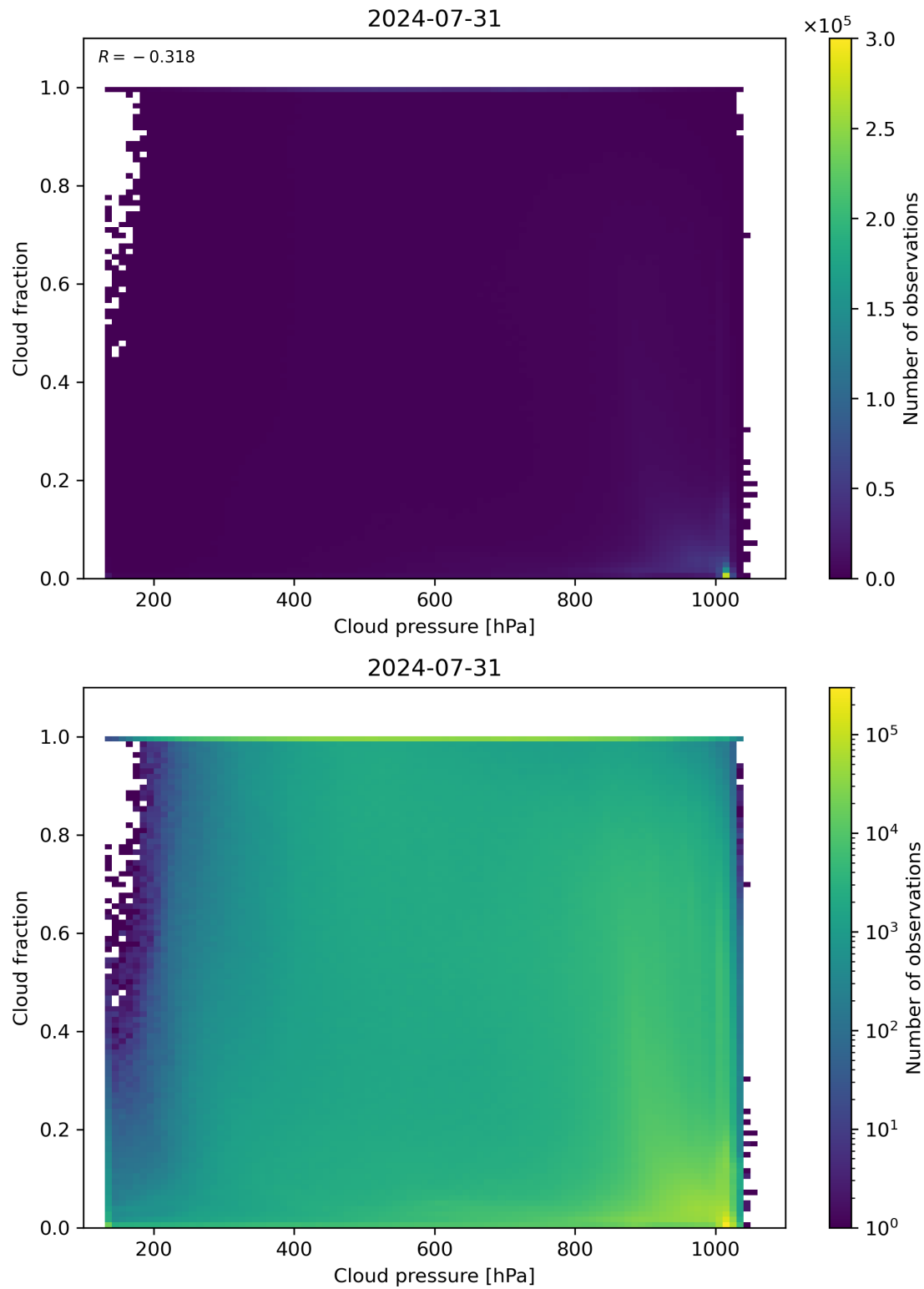
Figure 79: Scatter density plot of “Cloud pressure” against “Cloud fraction” for 2024-07-31 to 2024-08-01.
