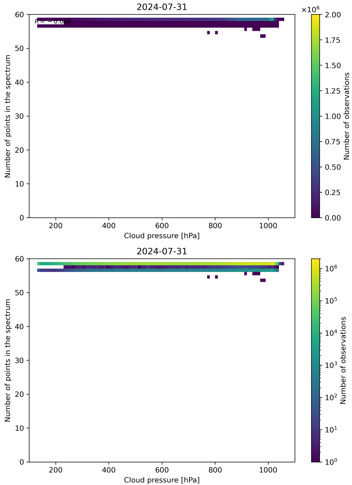
Figure 82: Scatter density plot of “Cloud pressure” against “Number of points in the spectrum” for 2024-07-31 to 2024-08-01.
