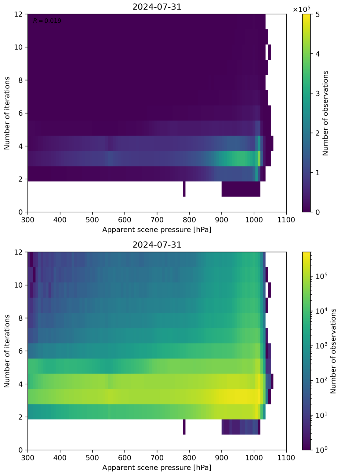
Figure 65: Scatter density plot of “Apparent scene pressure” against “Number of iterations” for 2024-07-31 to 2024-08-01.
