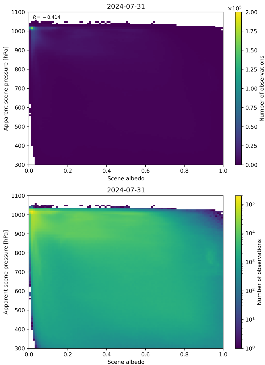
Figure 102: Scatter density plot of “Scene albedo” against “Apparent scene pressure” for 2024-07-31 to 2024-08-01.
