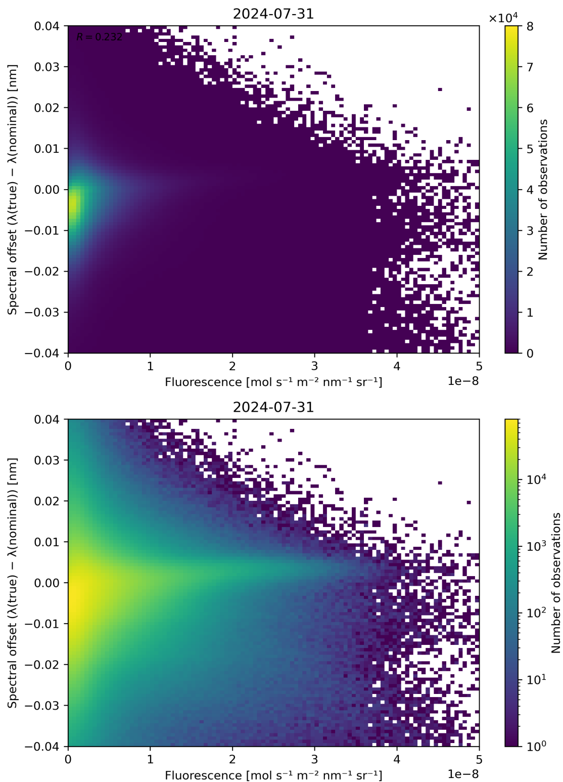
Figure 87: Scatter density plot of “Fluorescence” against “Spectral offset ( \lambda(\text{true}) - \lambda(\text{nominal}) )” for 2024-07-31 to 2024-08-01.
