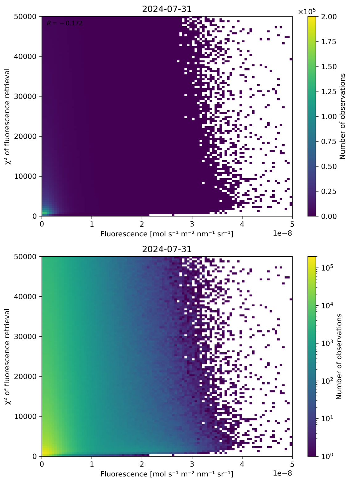
Figure 85: Scatter density plot of “Fluorescence” against “ \chi^2 of fluorescence retrieval” for 2024-07-31 to 2024-08-01.
