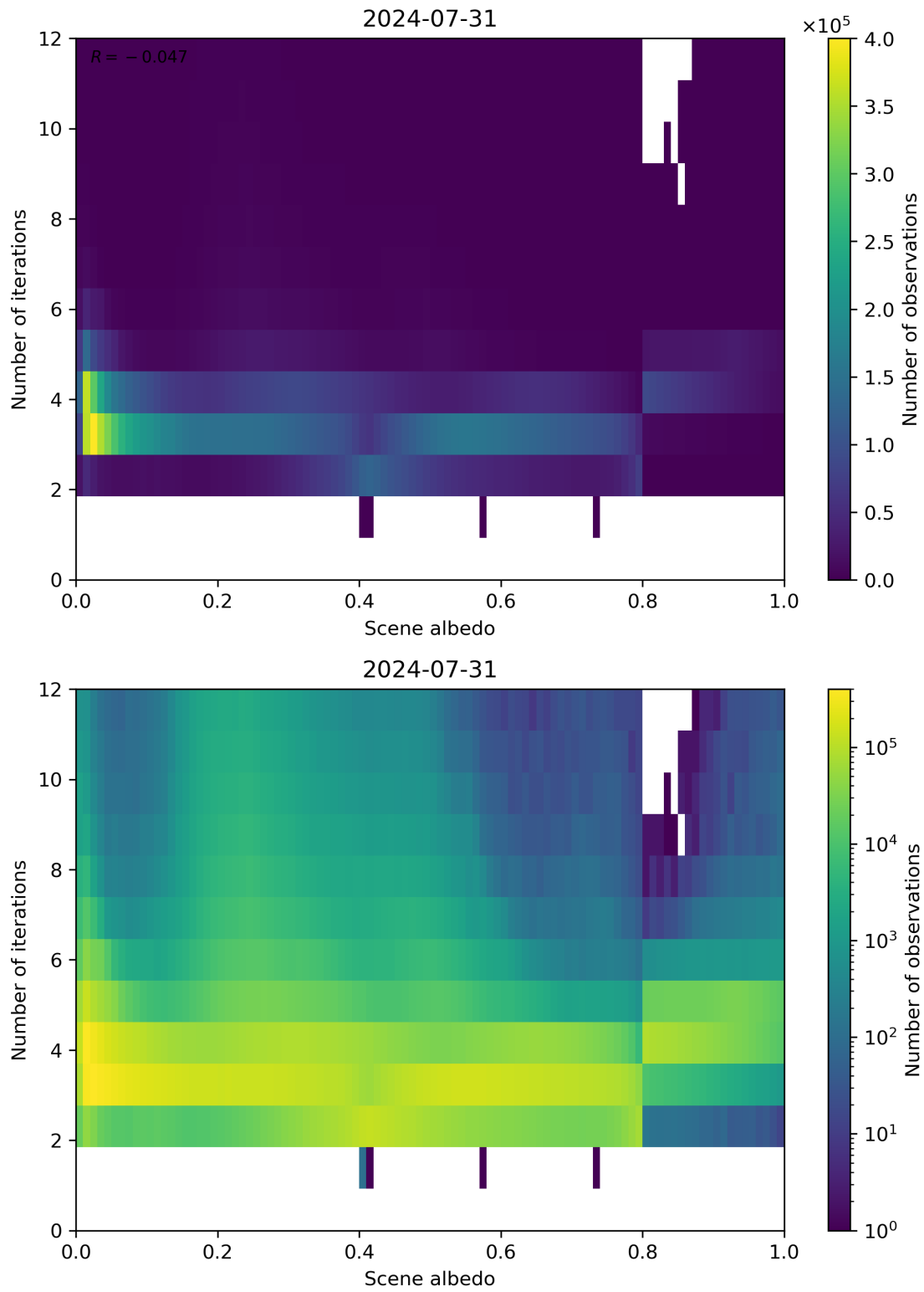
Figure 105: Scatter density plot of “Scene albedo” against “Number of iterations” for 2024-07-31 to 2024-08-01.
