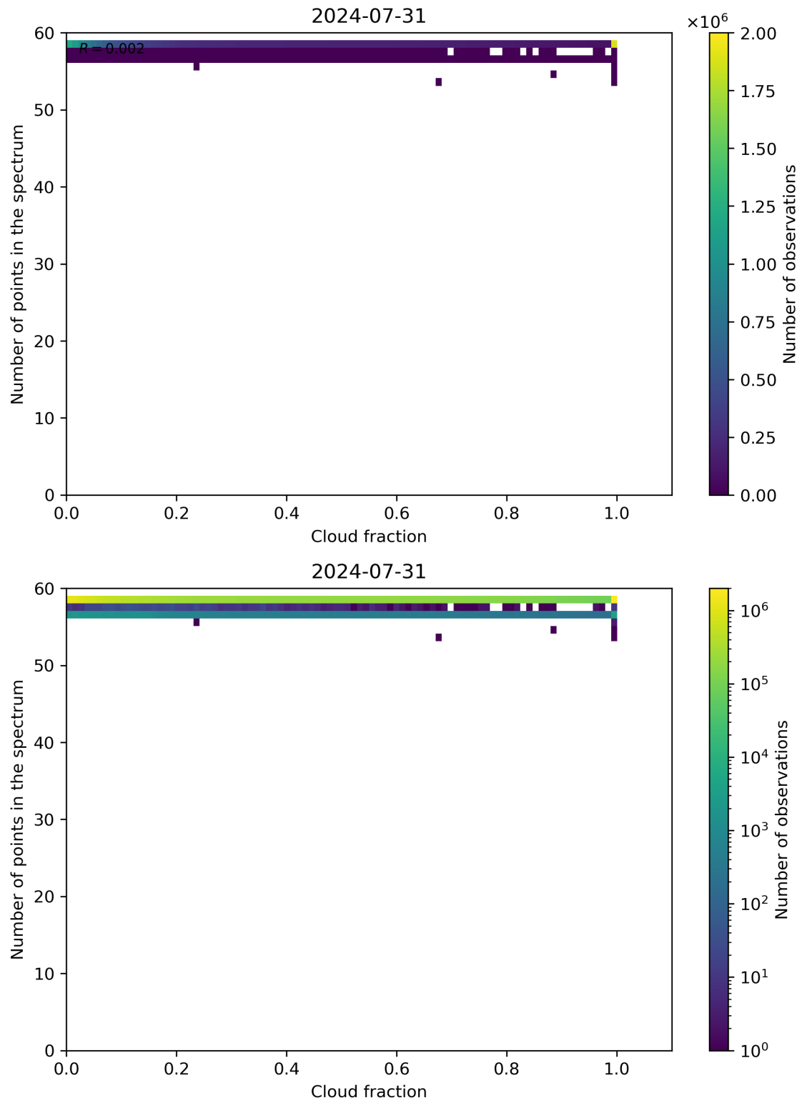
Figure 74: Scatter density plot of “Cloud fraction” against “Number of points in the spectrum” for 2024-07-31 to 2024-08-01.
