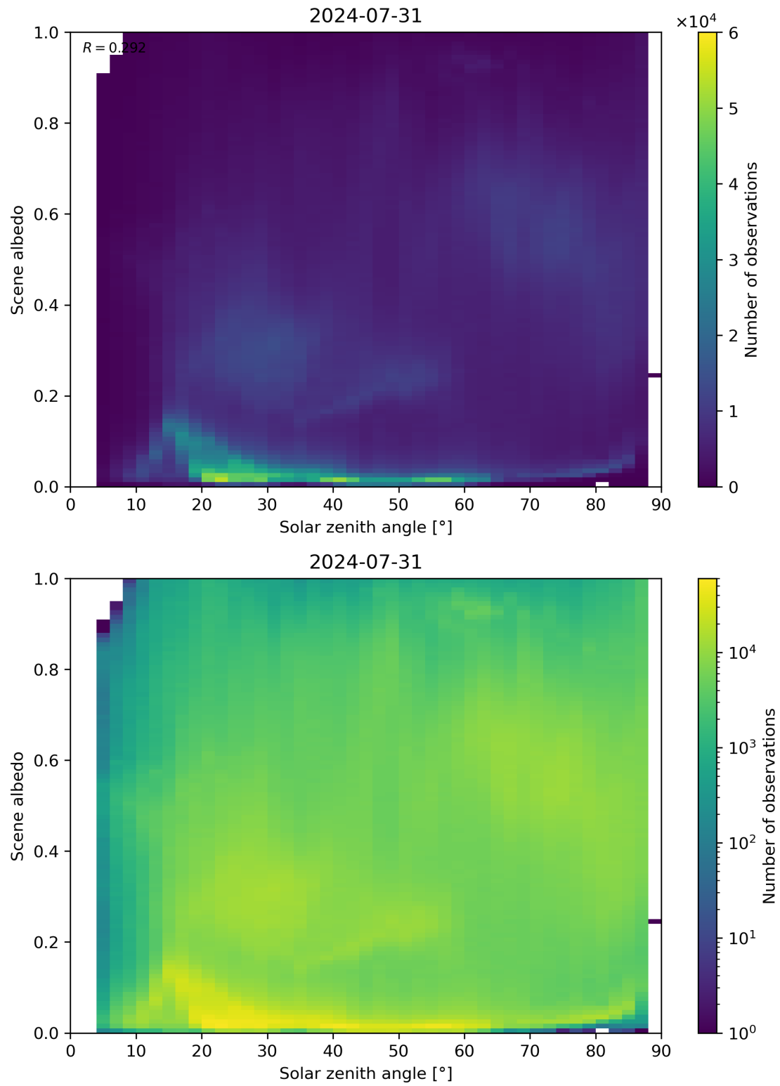
Figure 116: Scatter density plot of “Solar zenith angle” against “Scene albedo” for 2024-07-31 to 2024-08-01.
