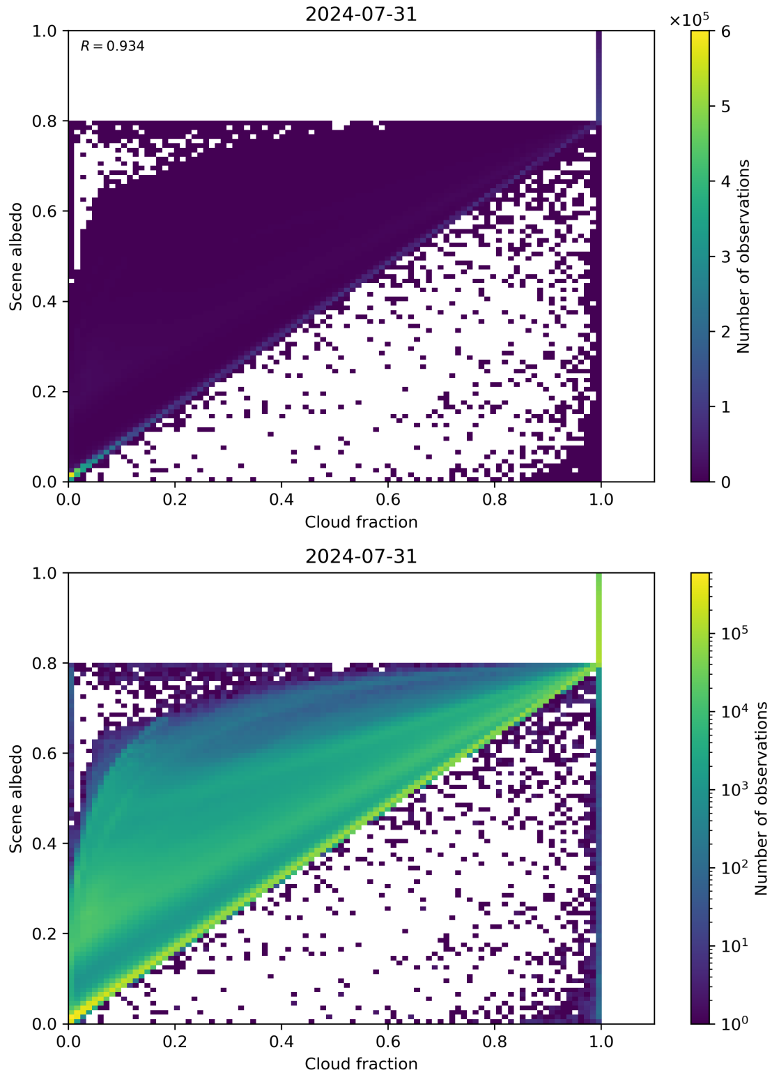
Figure 75: Scatter density plot of “Cloud fraction” against “Scene albedo” for 2024-07-31 to 2024-08-01.
