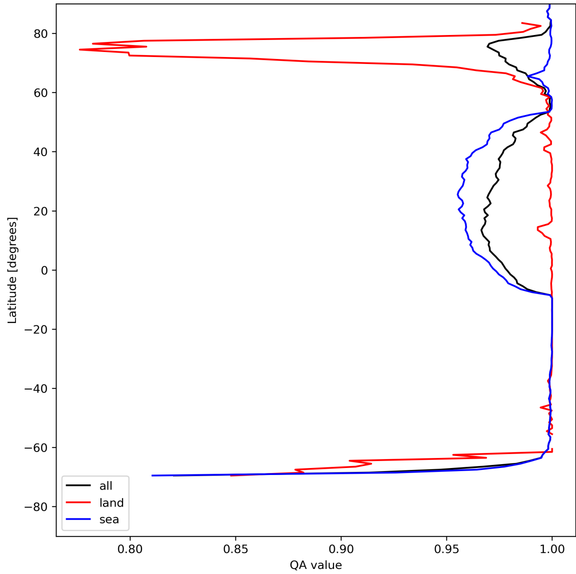
Figure 12: Zonal average of “QA value” for 2024-07-31 to 2024-08-01.
