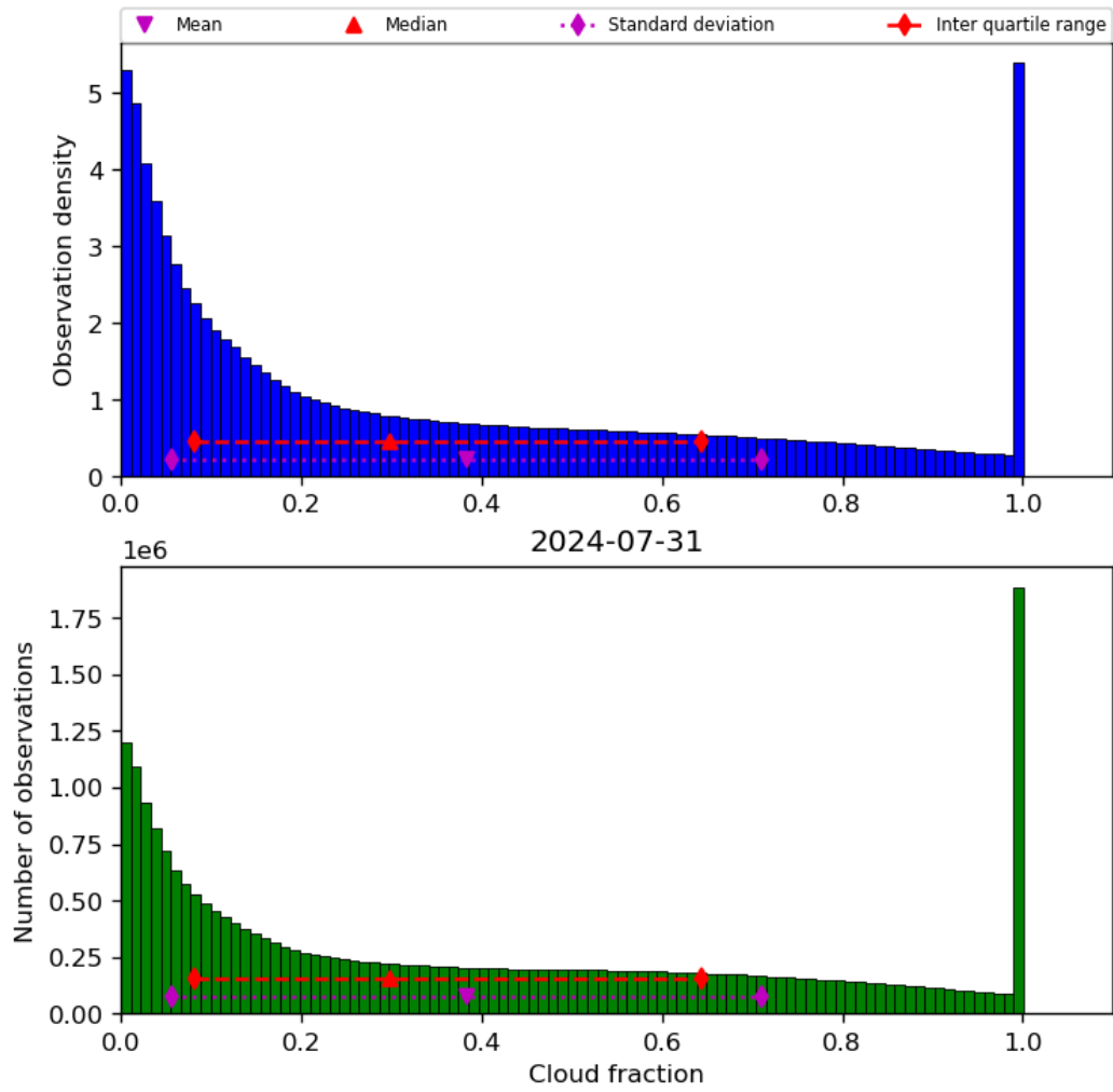
Figure 32: Histogram of “Cloud fraction” for 2024-07-31 to 2024-08-01
