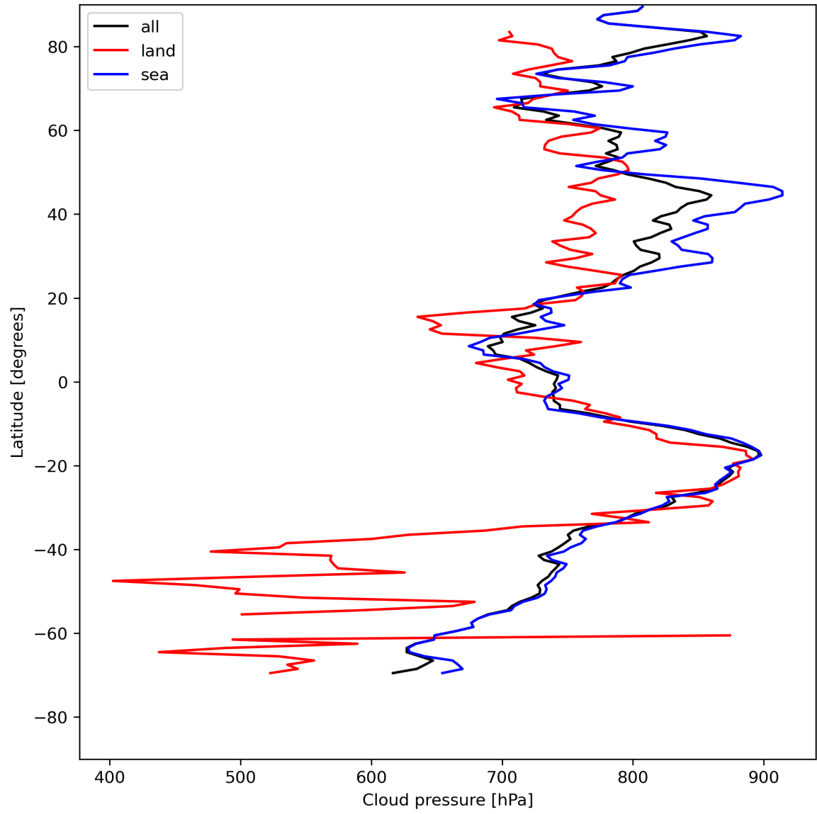
Figure 13: Zonal average of “Cloud pressure” for 2024-07-31 to 2024-08-01.
