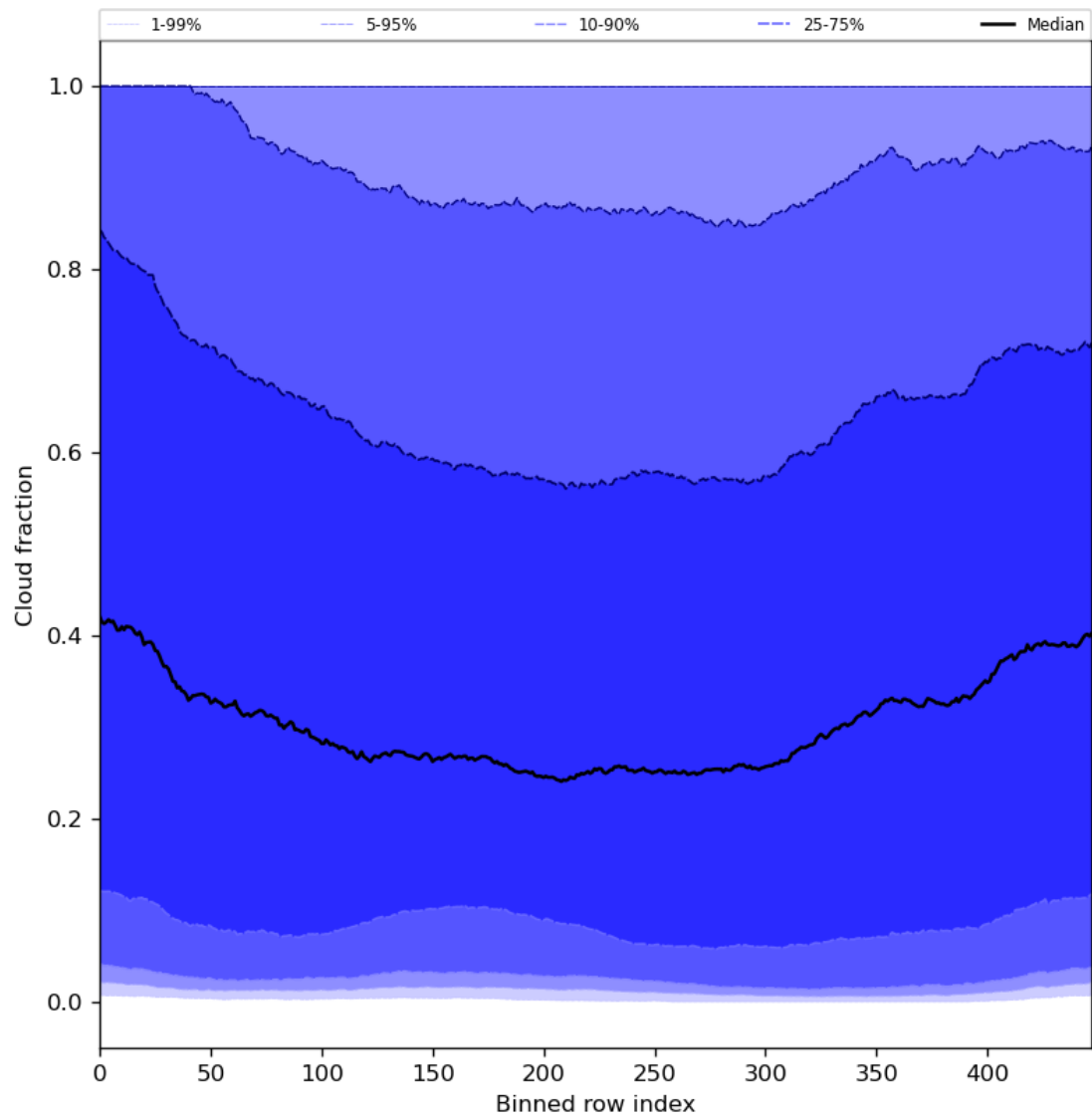
Figure 49: Along track statistics of “Cloud fraction” for 2024-07-31 to 2024-08-01
