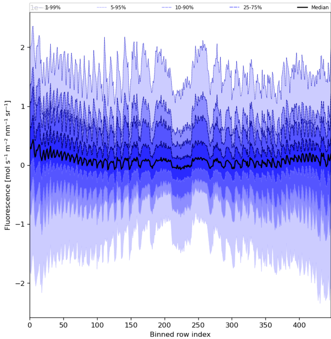
Figure 57: Along track statistics of “Fluorescence” for 2024-07-31 to 2024-08-01
