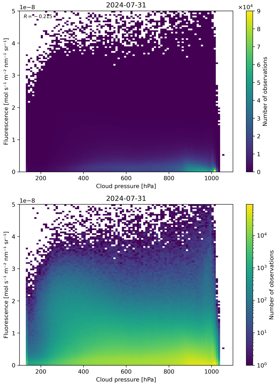
Figure 80: Scatter density plot of “Cloud pressure” against “Fluorescence” for 2024-07-31 to 2024-08-01.
