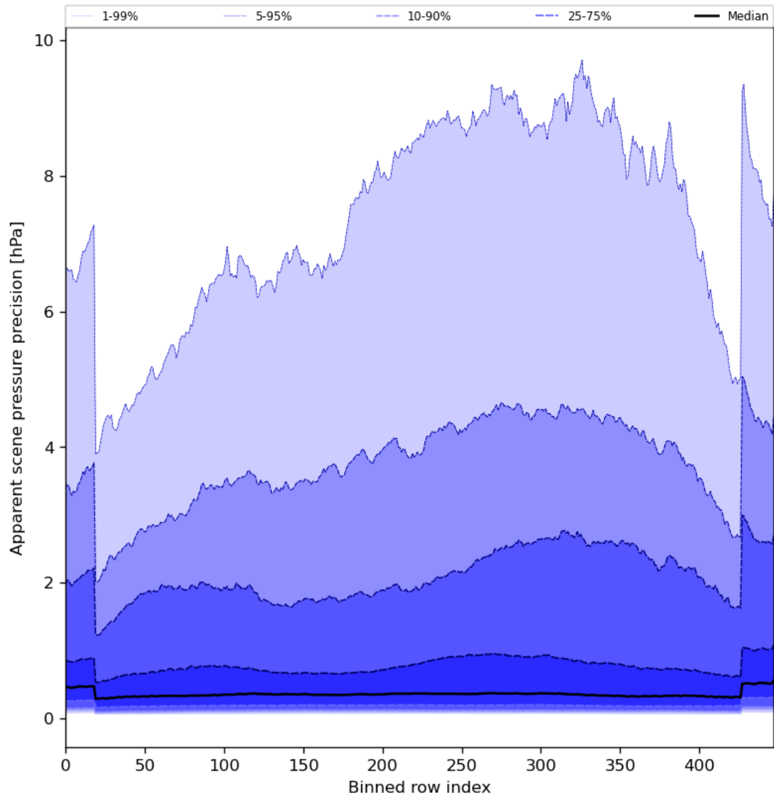
Figure 54: Along track statistics of “Apparent scene pressure precision” for 2024-07-31 to 2024-08-01
