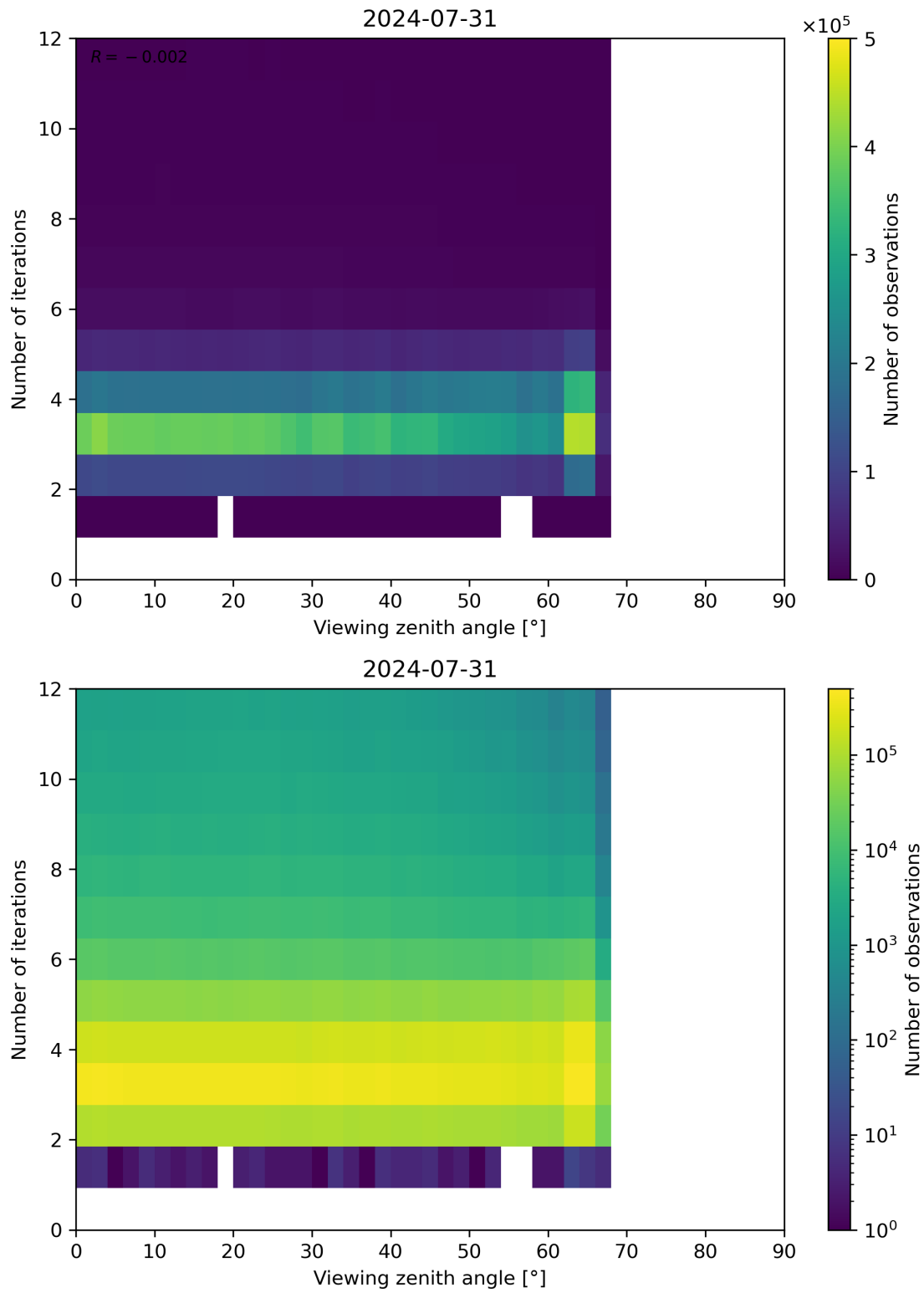
Figure 124: Scatter density plot of “Viewing zenith angle” against “Number of iterations” for 2024-07-31 to 2024-08-01.
