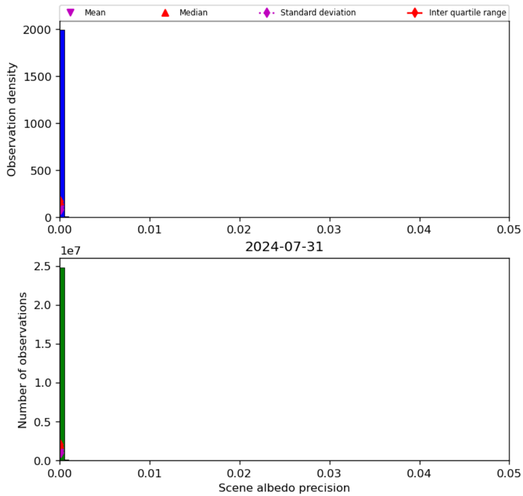
Figure 35: Histogram of “Scene albedo precision” for 2024-07-31 to 2024-08-01
