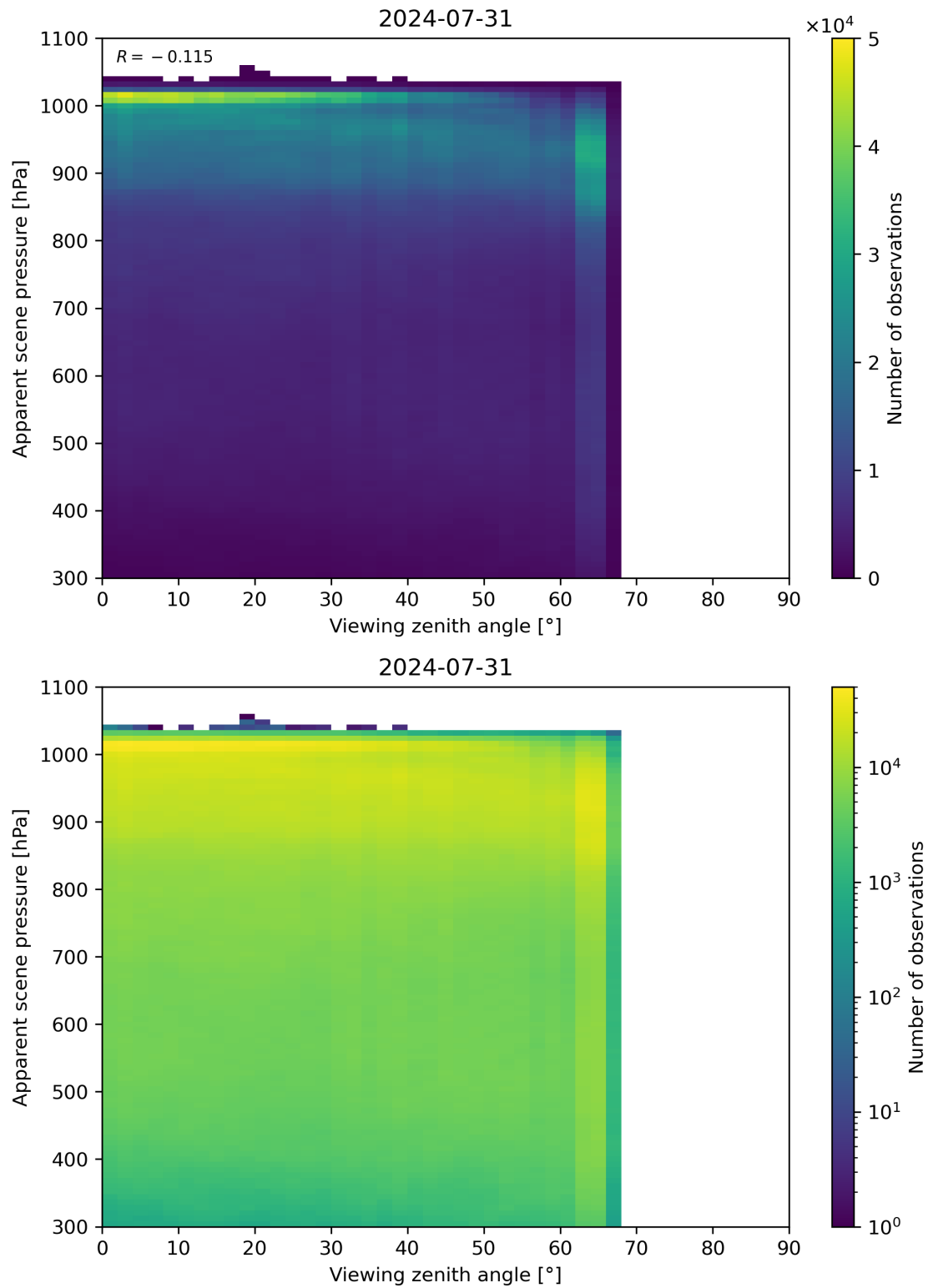
Figure 118: Scatter density plot of “Viewing zenith angle” against “Apparent scene pressure” for 2024-07-31 to 2024-08-01.
