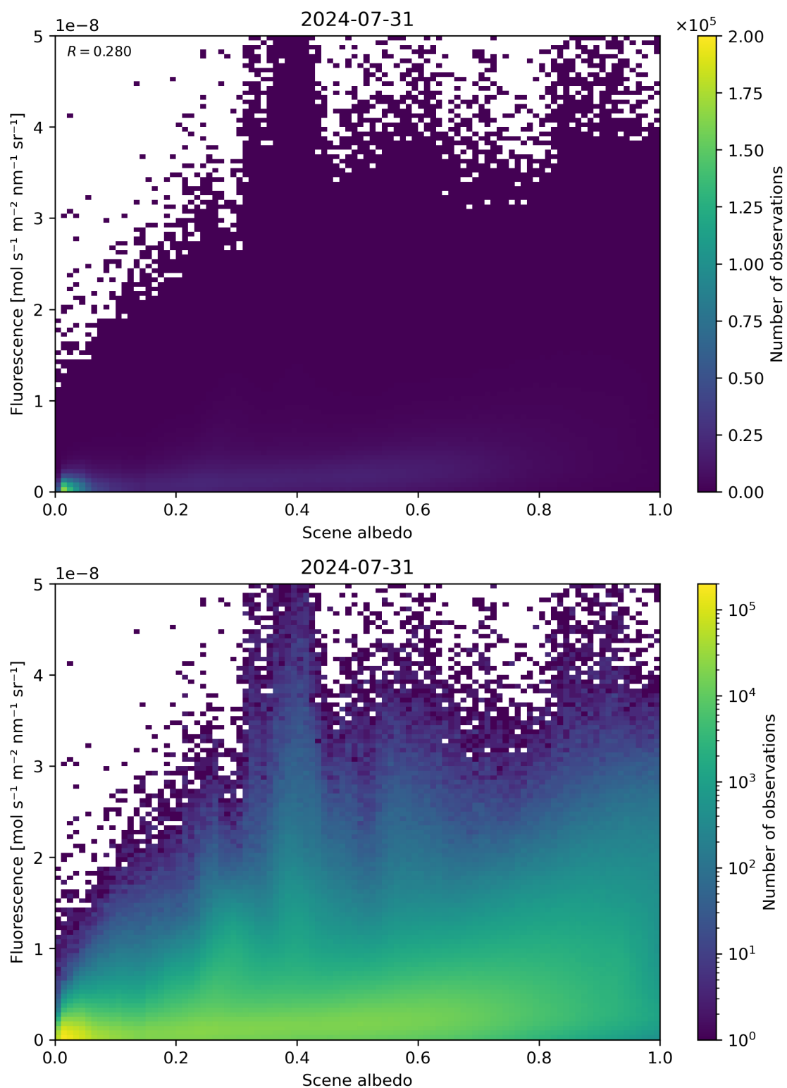
Figure 104: Scatter density plot of “Scene albedo” against “Fluorescence” for 2024-07-31 to 2024-08-01.
