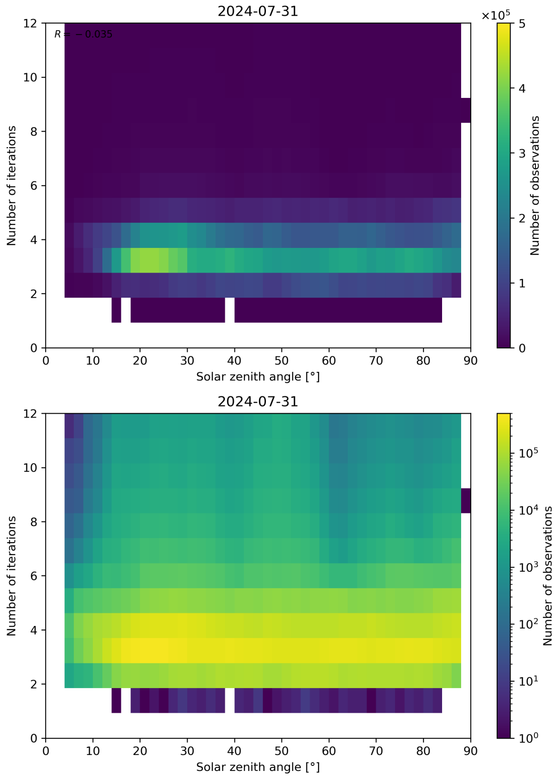
Figure 114: Scatter density plot of “Solar zenith angle” against “Number of iterations” for 2024-07-31 to 2024-08-01.
