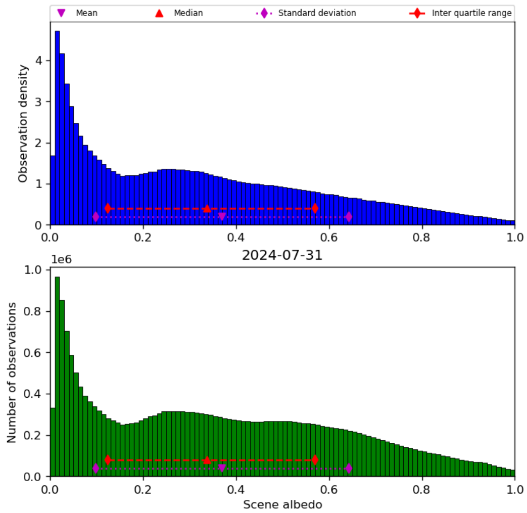
Figure 34: Histogram of “Scene albedo” for 2024-07-31 to 2024-08-01
