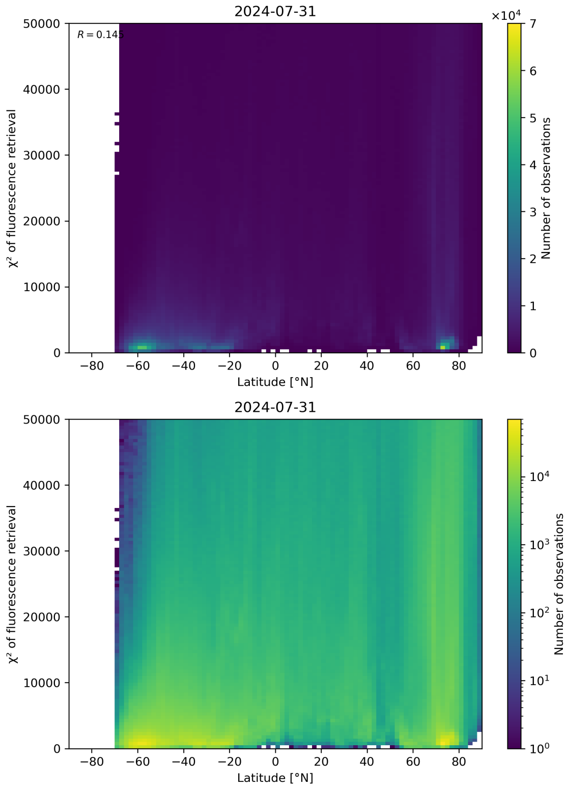
Figure 89: Scatter density plot of “Latitude” against “ \chi^2 of fluorescence retrieval” for 2024-07-31 to 2024-08-01.
