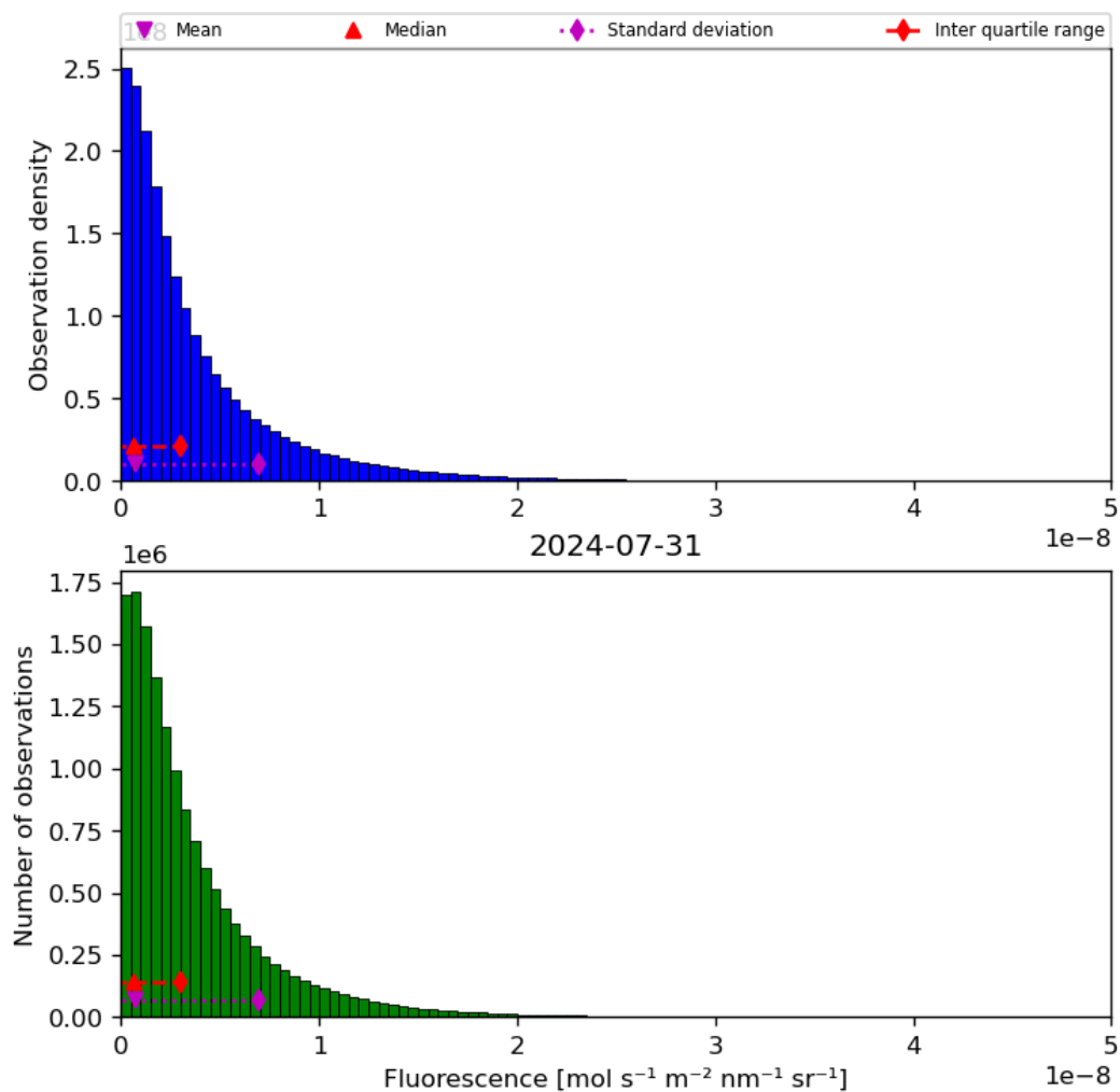
Figure 40: Histogram of “Fluorescence” for 2024-07-31 to 2024-08-01
