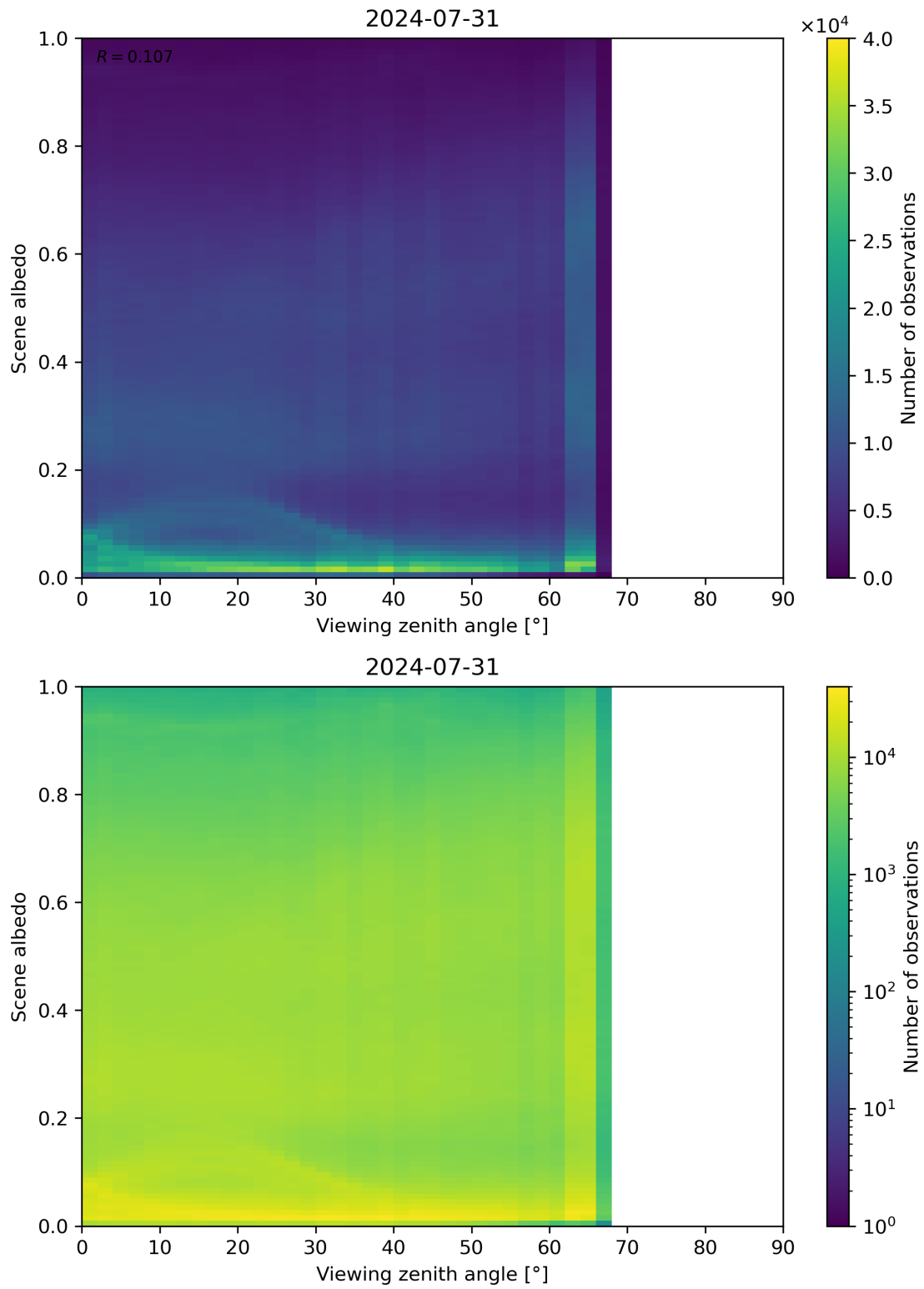
Figure 126: Scatter density plot of “Viewing zenith angle” against “Scene albedo” for 2024-07-31 to 2024-08-01.
