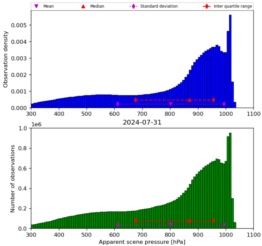
Figure 36: Histogram of “Apparent scene pressure” for 2024-07-31 to 2024-08-01
