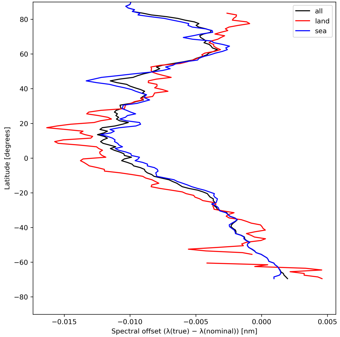
Figure 28: Zonal average of “Spectral offset ( \lambda(\text{true}) - \lambda(\text{nominal}) )” for 2024-07-31 to 2024-08-01.
