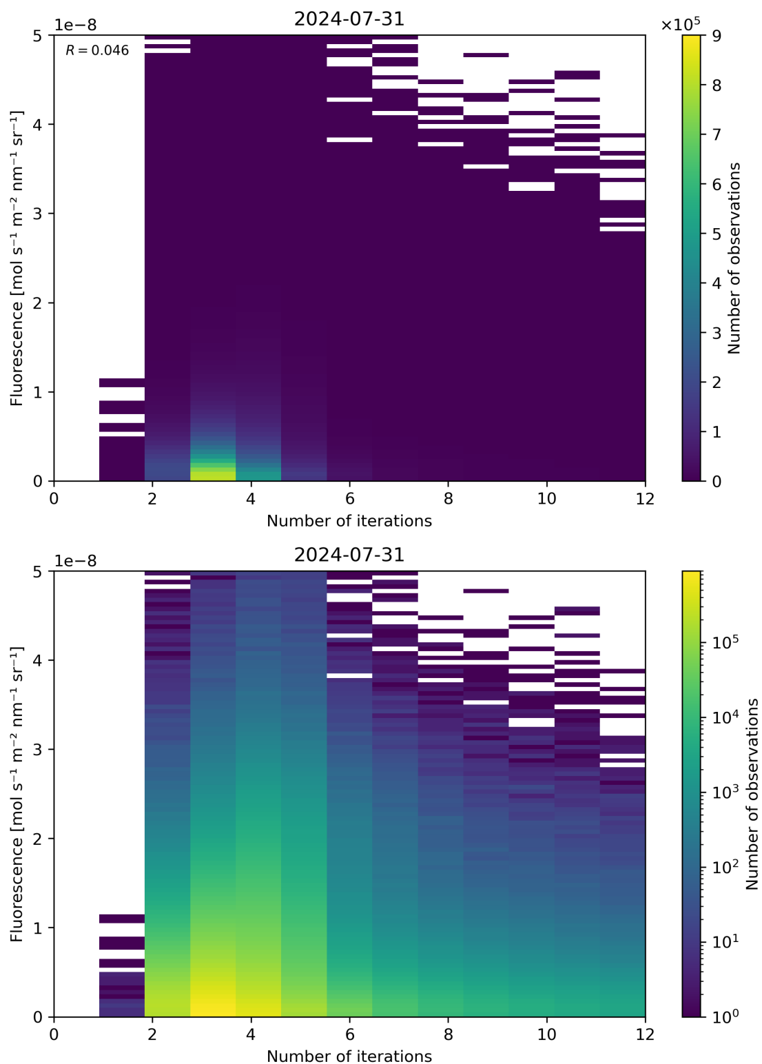
Figure 98: Scatter density plot of “Number of iterations” against “Fluorescence” for 2024-07-31 to 2024-08-01.
