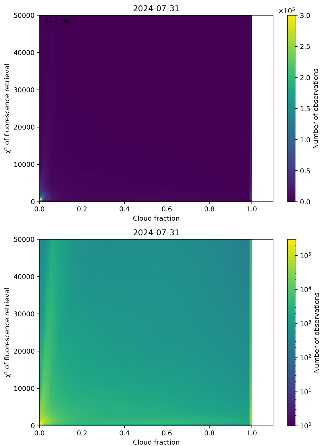
Figure 71: Scatter density plot of “Cloud fraction” against “ \chi^2 of fluorescence retrieval” for 2024-07-31 to 2024-08-01.
