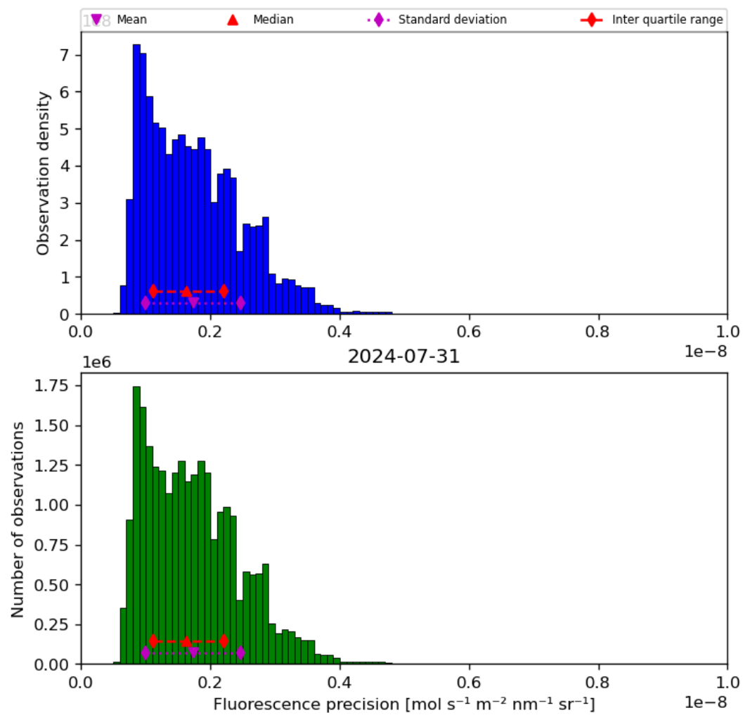
Figure 41: Histogram of “Fluorescence precision” for 2024-07-31 to 2024-08-01
