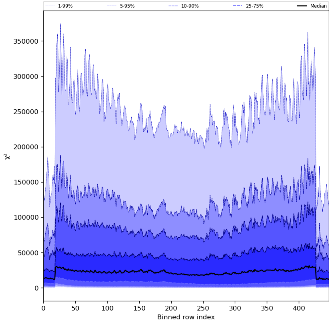
Figure 55: Along track statistics of “ \chi^2 ” for 2024-07-31 to 2024-08-01
