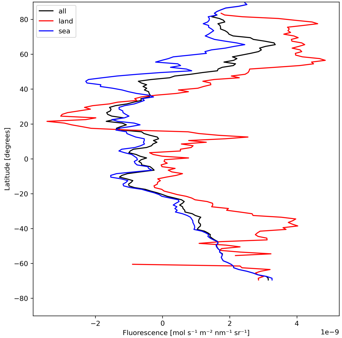
Figure 23: Zonal average of “Fluorescence” for 2024-07-31 to 2024-08-01.
