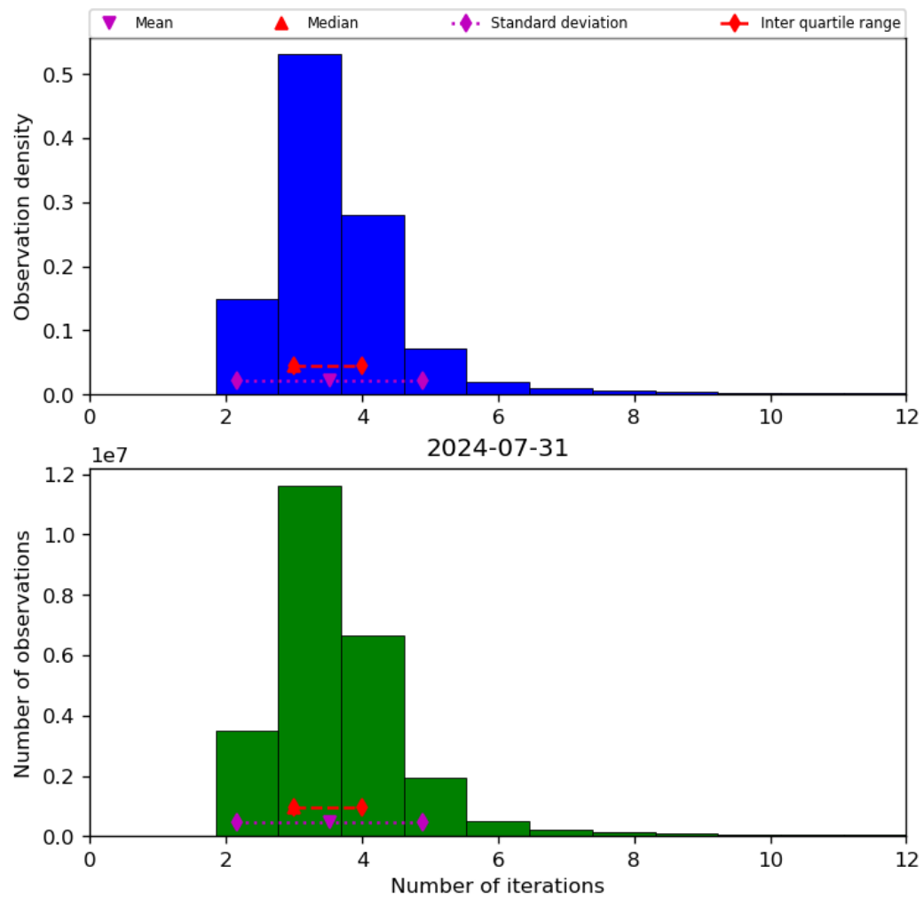
Figure 39: Histogram of “Number of iterations” for 2024-07-31 to 2024-08-01
