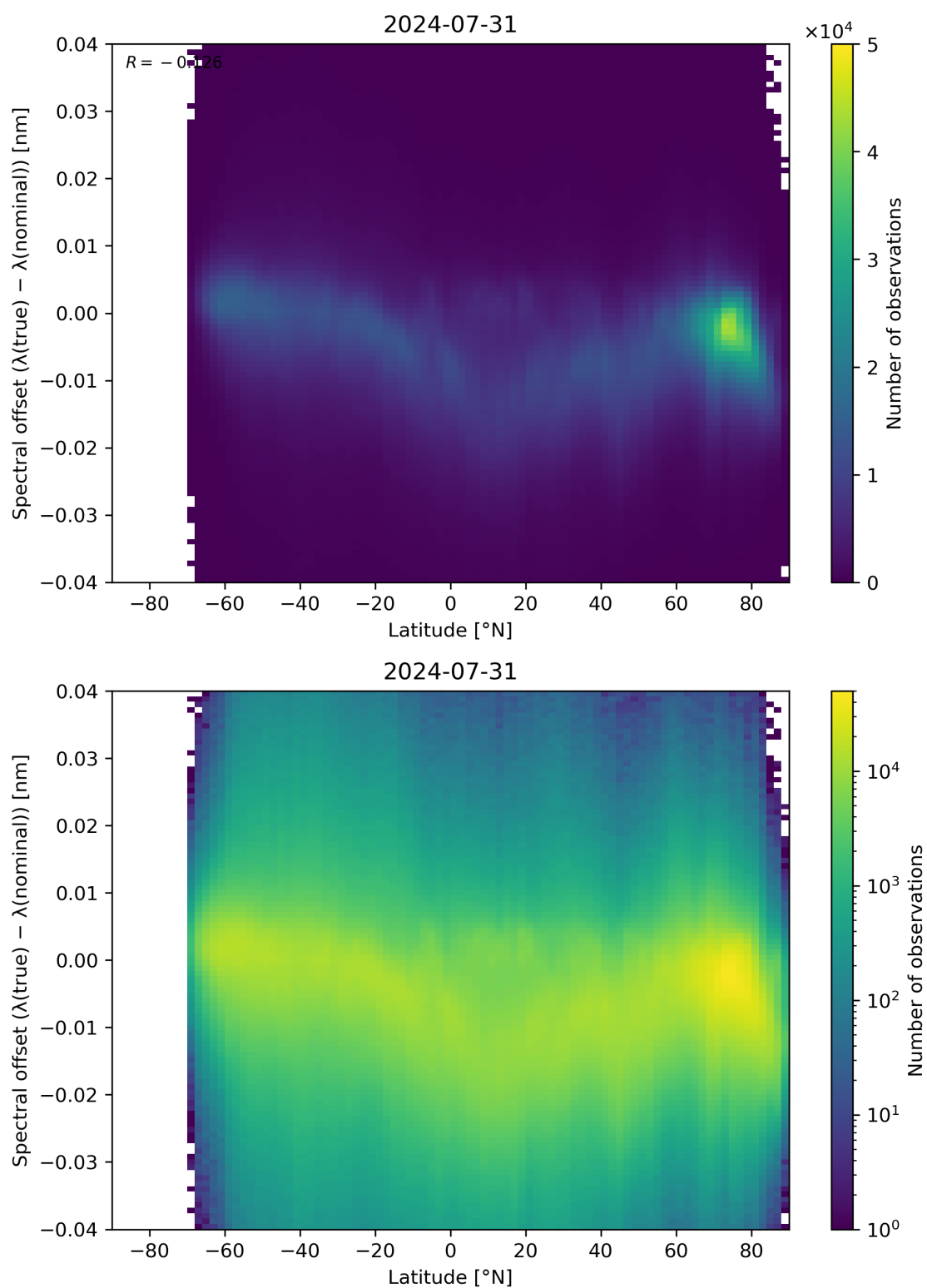
Figure 96: Scatter density plot of “Latitude” against “Spectral offset ( \lambda(\text{true}) - \lambda(\text{nominal}) )” for 2024-07-31 to 2024-08-01.
