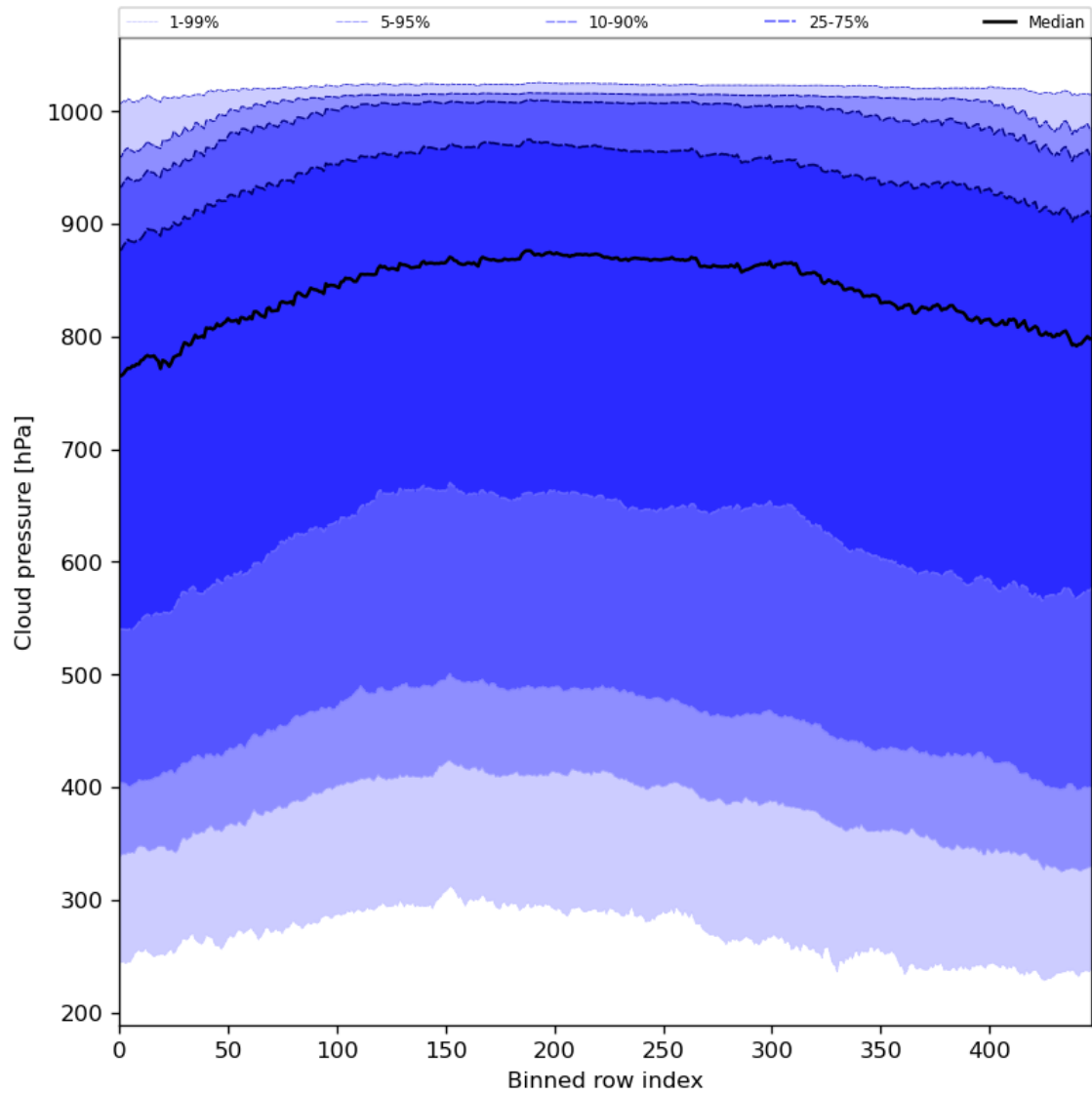
Figure 47: Along track statistics of “Cloud pressure” for 2024-07-31 to 2024-08-01
