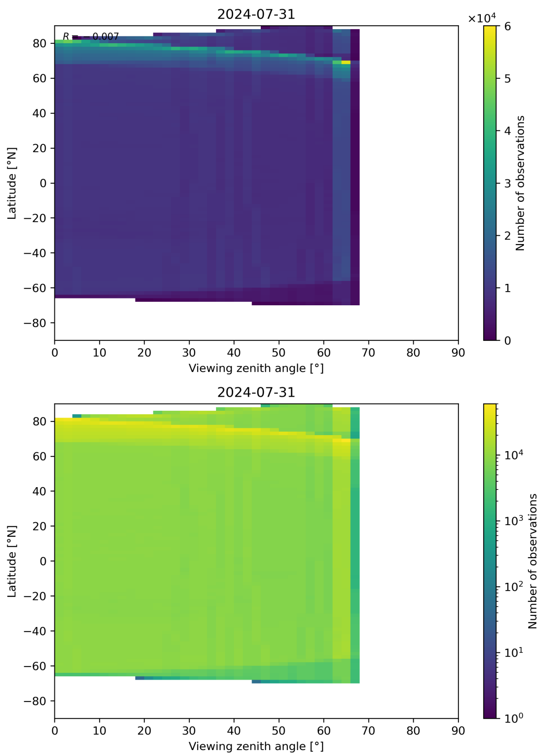
Figure 123: Scatter density plot of “Viewing zenith angle” against “Latitude” for 2024-07-31 to 2024-08-01.
