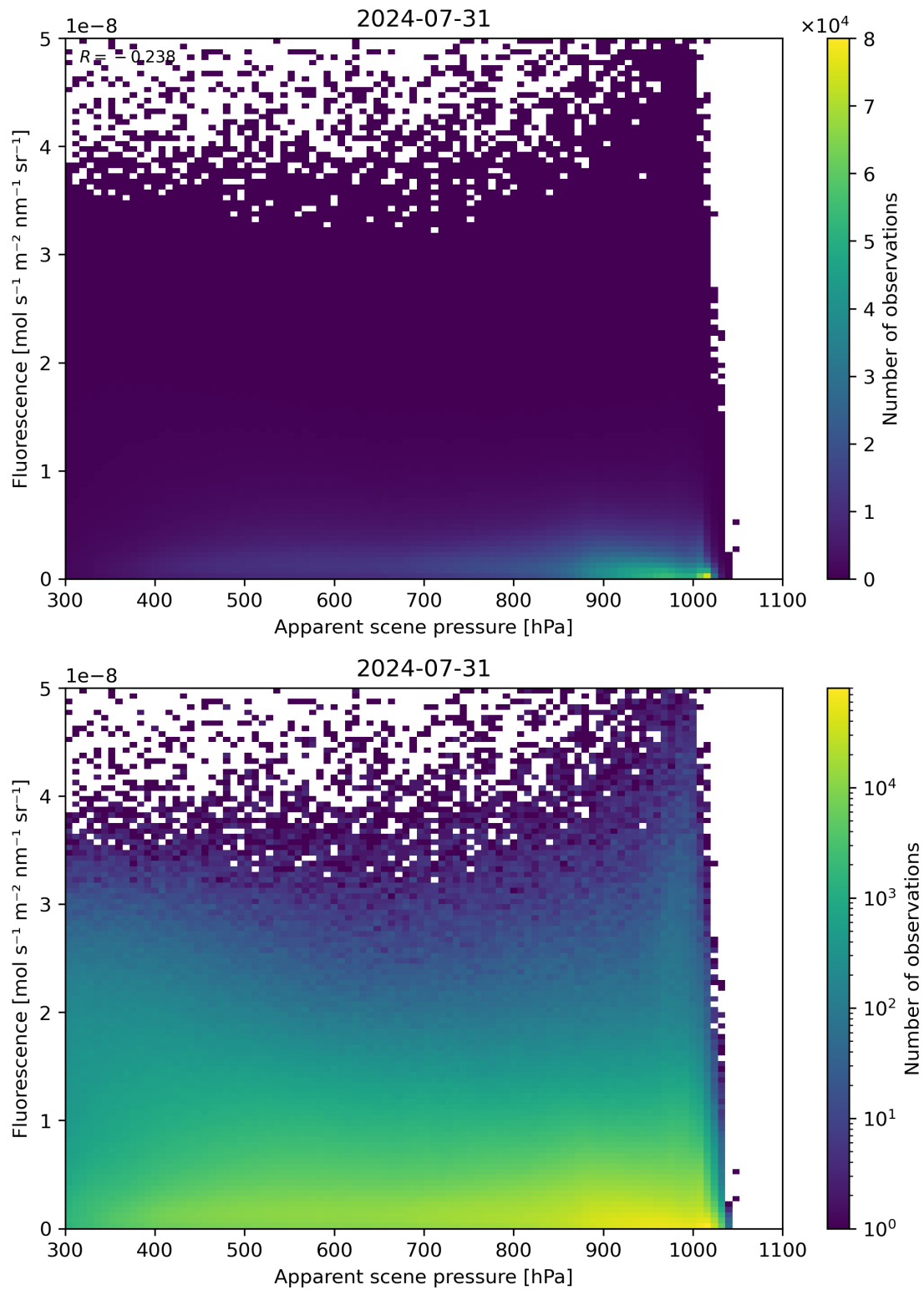
Figure 64: Scatter density plot of “Apparent scene pressure” against “Fluorescence” for 2024-07-31 to 2024-08-01.
