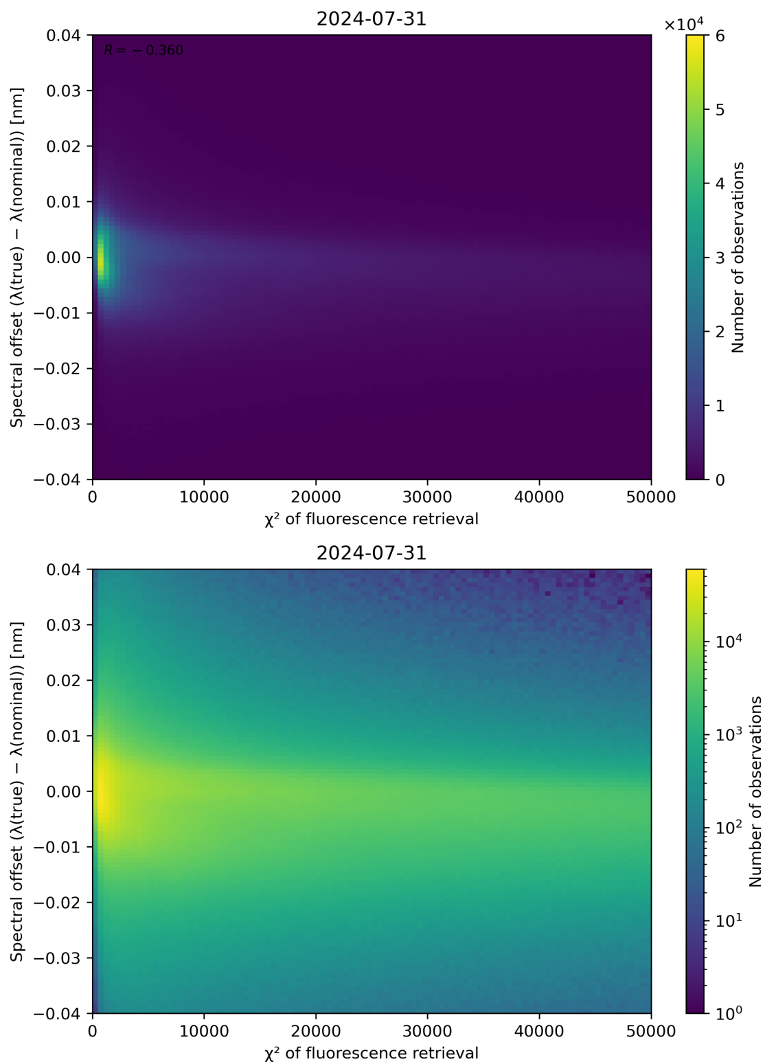
Figure 69: Scatter density plot of " \chi^2 of fluorescence retrieval" against "Spectral offset ( \lambda(\text{true}) - \lambda(\text{nominal}) )" for 2024-07-31 to 2024-08-01.
