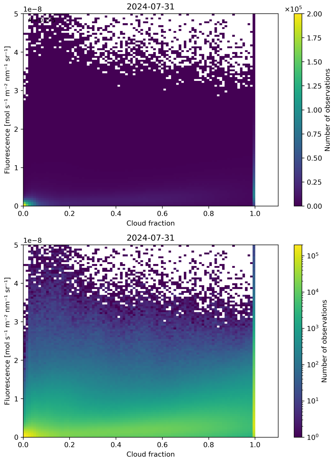
Figure 72: Scatter density plot of “Cloud fraction” against “Fluorescence” for 2024-07-31 to 2024-08-01.
