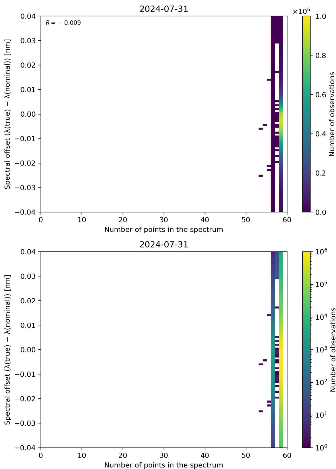
Figure 101: Scatter density plot of “Number of points in the spectrum” against “Spectral offset ( \lambda(\text{true}) - \lambda(\text{nominal}) )” for 2024-07-31 to 2024-08-01.
