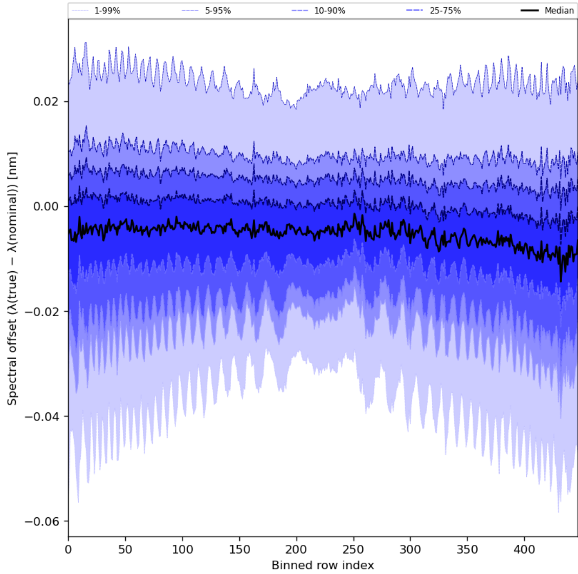
Figure 62: Along track statistics of “Spectral offset ( \lambda(\text{true}) - \lambda(\text{nominal}) )” for 2024-07-31 to 2024-08-01
