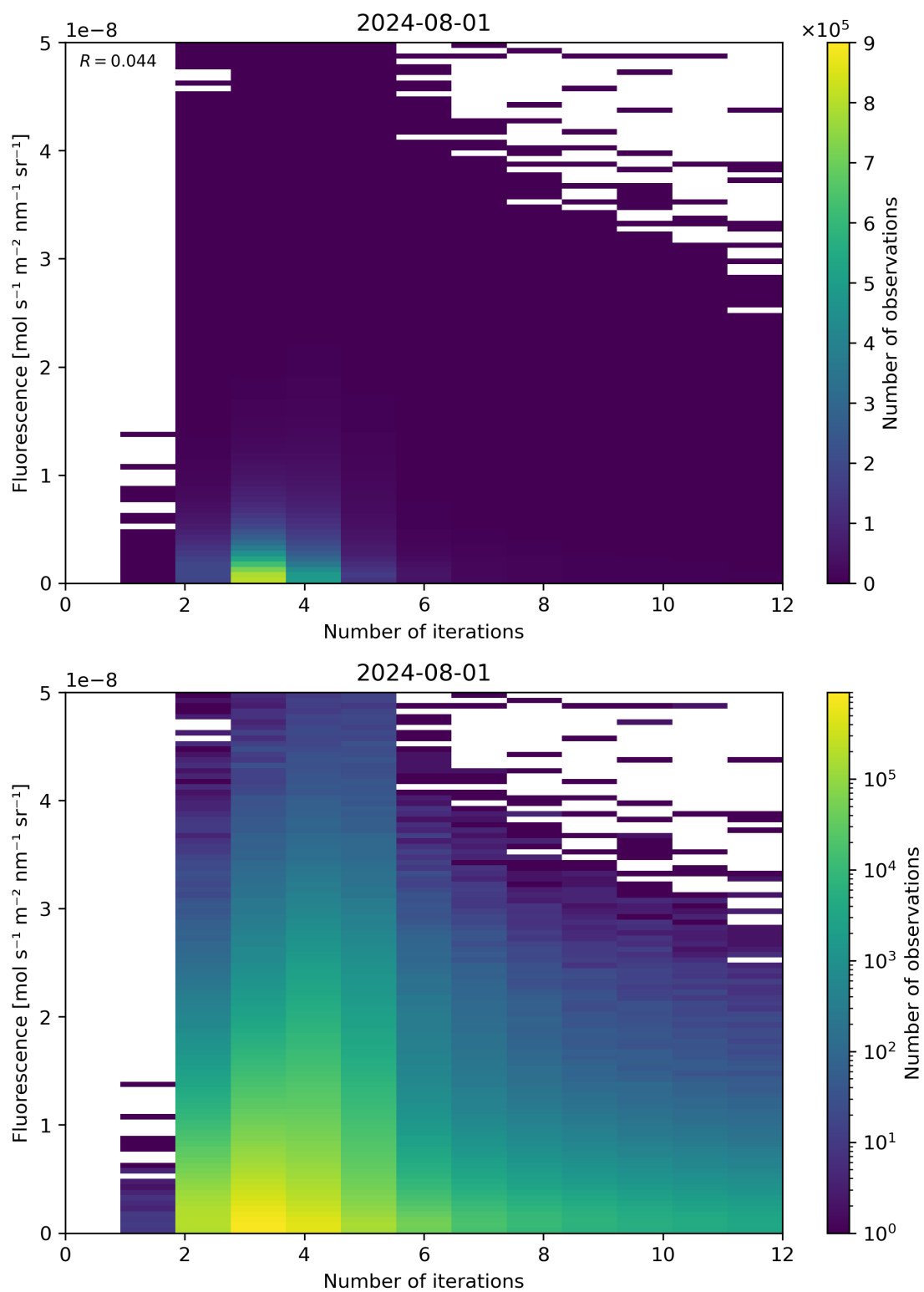
Figure 98: Scatter density plot of "Number of iterations" against "Fluorescence" for 2024-07-31 to 2024-08-02.
