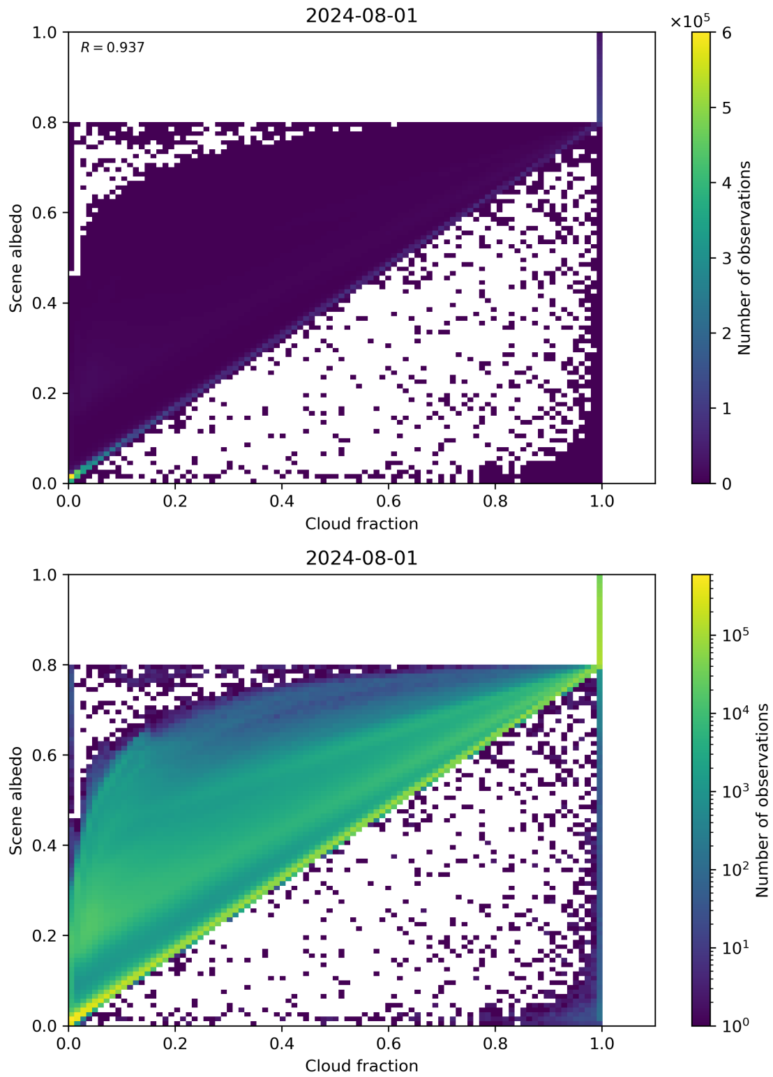
Figure 75: Scatter density plot of “Cloud fraction” against “Scene albedo” for 2024-07-31 to 2024-08-02.
