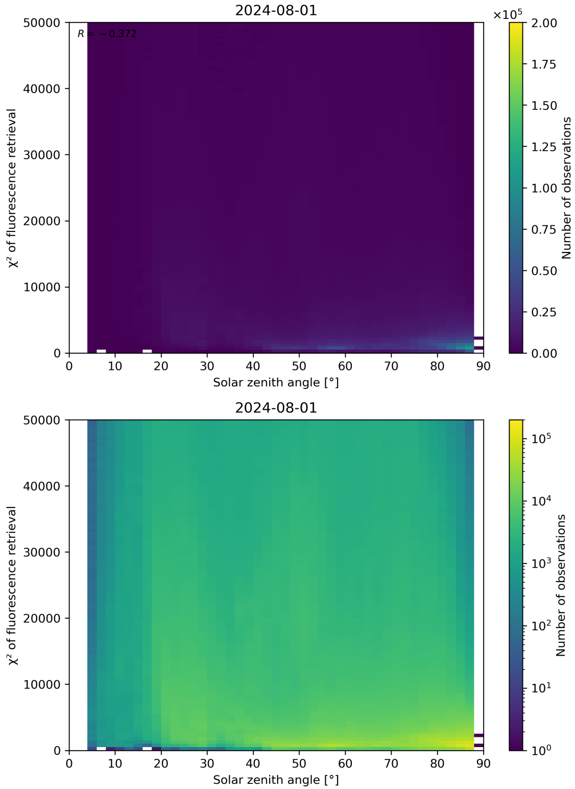
Figure 109: Scatter density plot of “Solar zenith angle” against “ \chi^2 of fluorescence retrieval” for 2024-07-31 to 2024-08-02.
