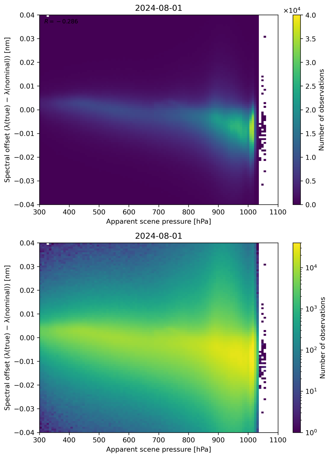
Figure 67: Scatter density plot of “Apparent scene pressure” against “Spectral offset ( \lambda(\text{true}) - \lambda(\text{nominal}) )” for 2024-07-31 to 2024-08-02.
