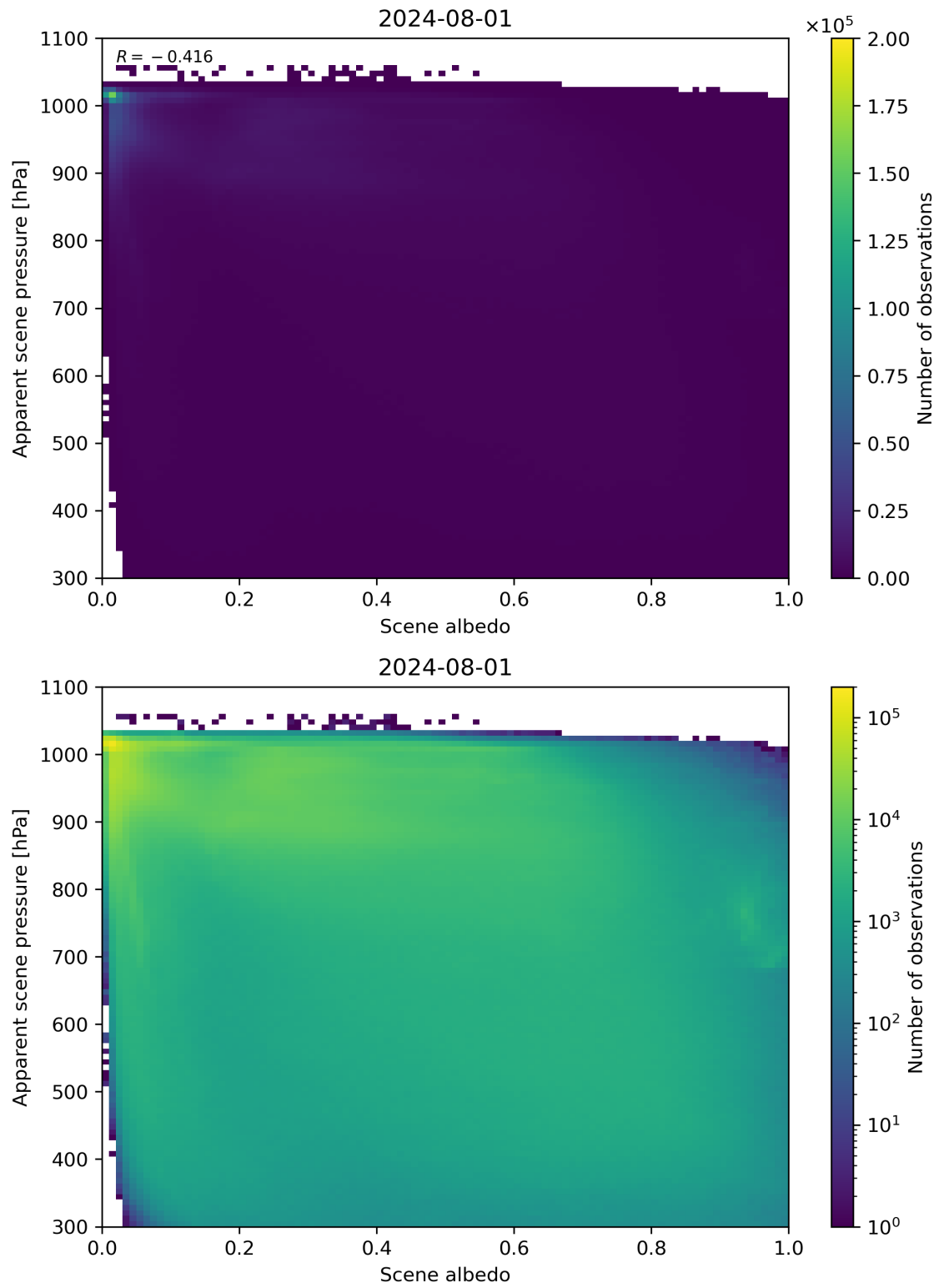
Figure 102: Scatter density plot of “Scene albedo” against “Apparent scene pressure” for 2024-07-31 to 2024-08-02.
