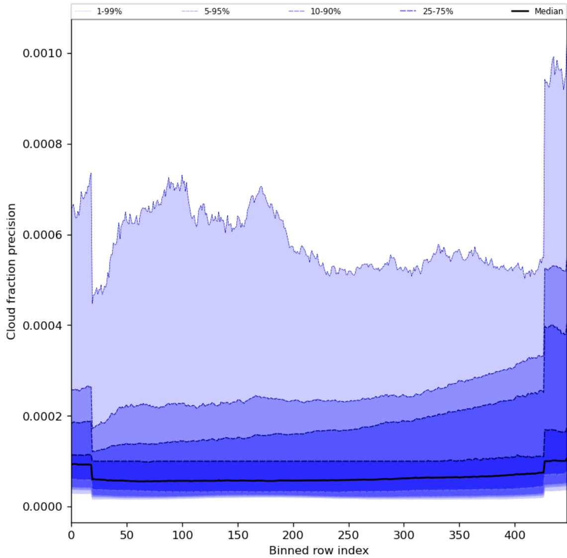
Figure 50: Along track statistics of “Cloud fraction precision” for 2024-07-31 to 2024-08-02
