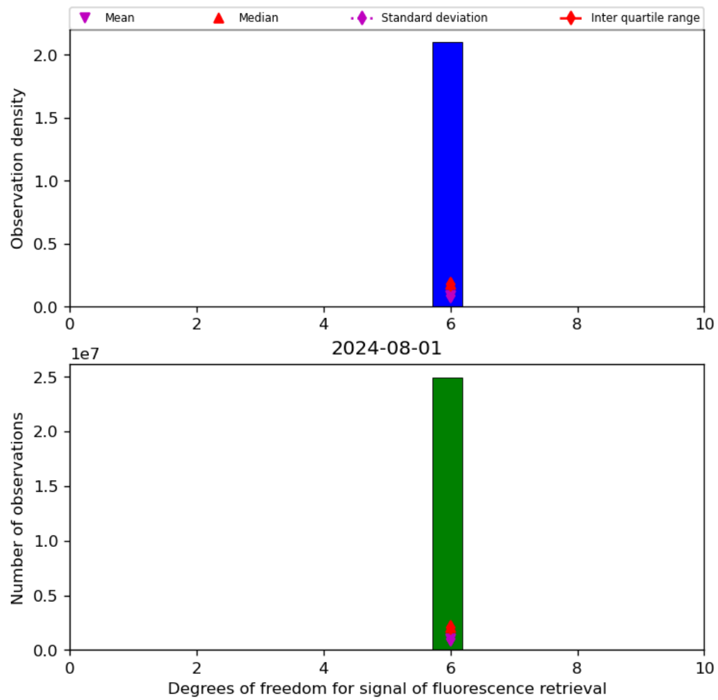
Figure 43: Histogram of “Degrees of freedom for signal of fluorescence retrieval” for 2024-07-31 to 2024-08-02
