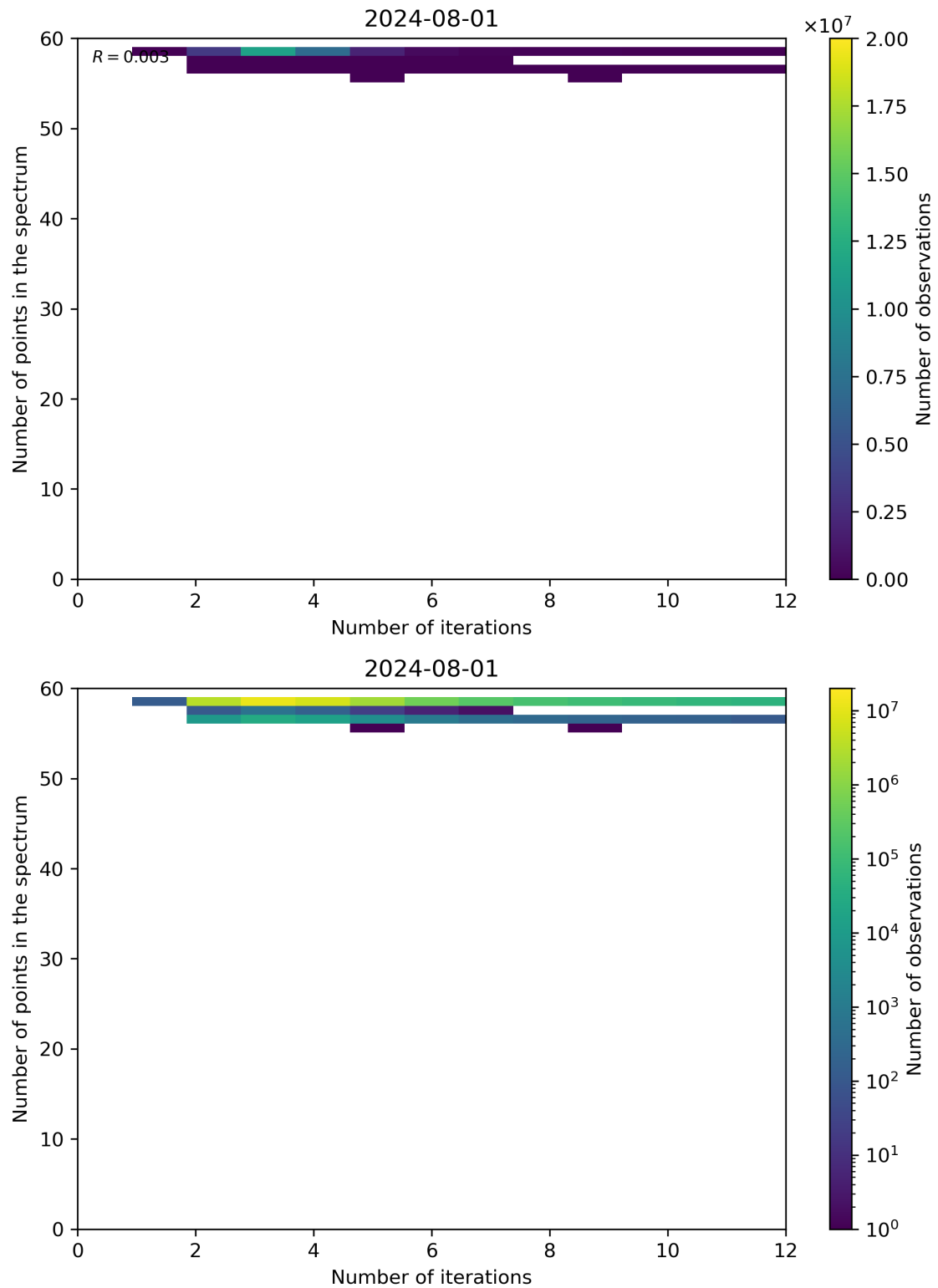
Figure 99: Scatter density plot of “Number of iterations” against “Number of points in the spectrum” for 2024-07-31 to 2024-08-02.
