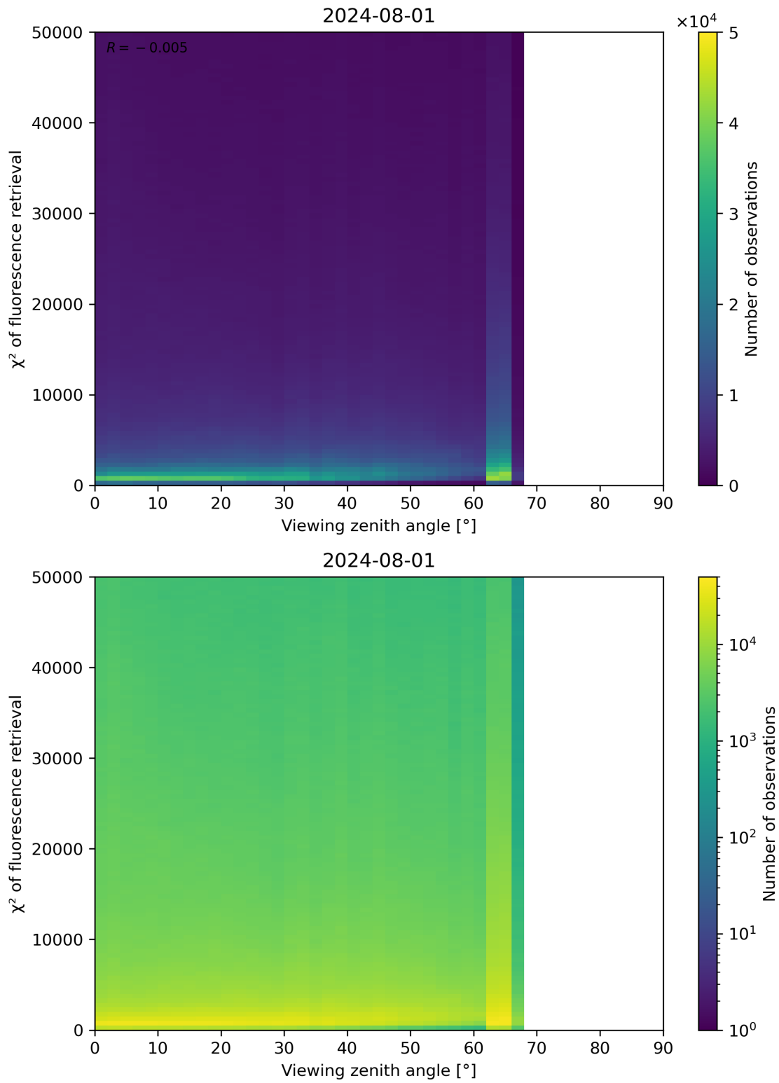
Figure 119: Scatter density plot of “Viewing zenith angle” against “ \chi^2 of fluorescence retrieval” for 2024-07-31 to 2024-08-02.
