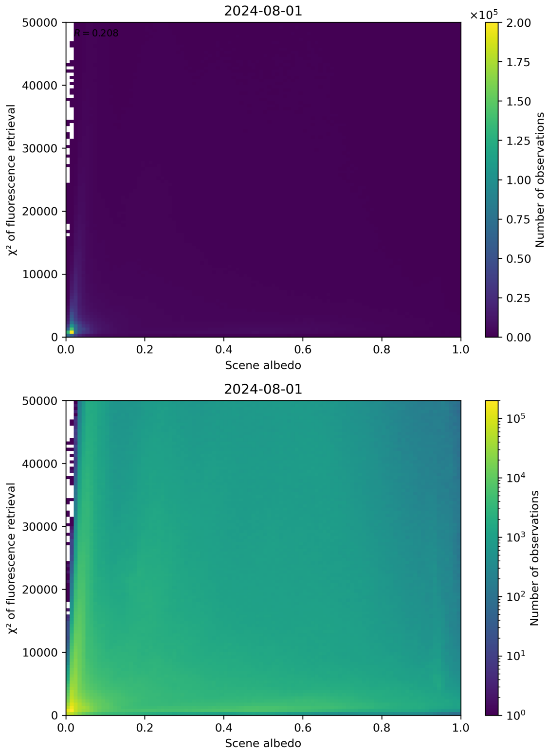
Figure 103: Scatter density plot of “Scene albedo” against “ \chi^2 of fluorescence retrieval” for 2024-07-31 to 2024-08-02.
