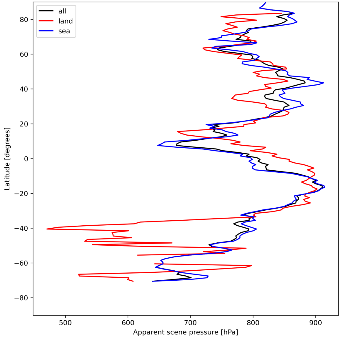
Figure 19: Zonal average of “Apparent scene pressure” for 2024-07-31 to 2024-08-02.
