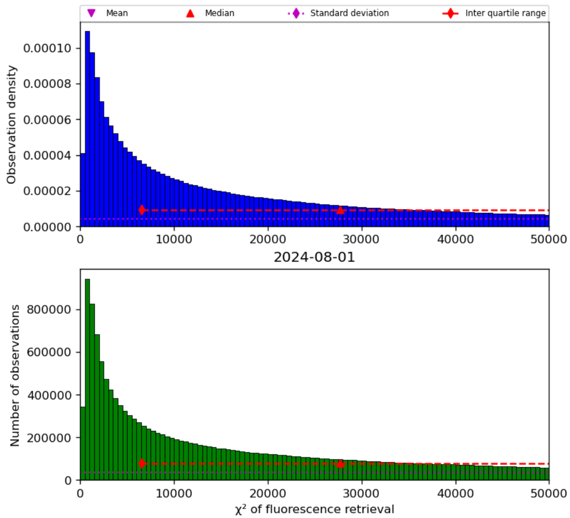
Figure 42: Histogram of “ \chi^2 of fluorescence retrieval” for 2024-07-31 to 2024-08-02
