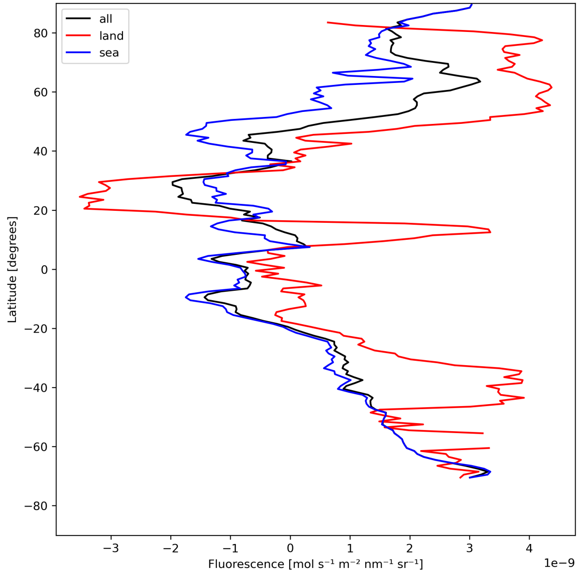
Figure 23: Zonal average of “Fluorescence” for 2024-07-31 to 2024-08-02.
