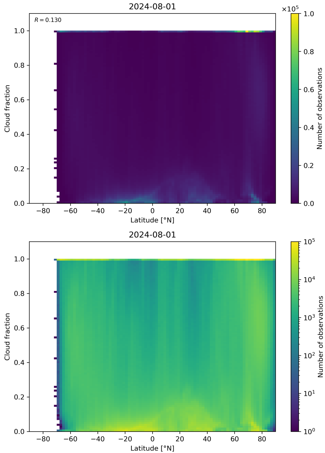
Figure 90: Scatter density plot of “Latitude” against “Cloud fraction” for 2024-07-31 to 2024-08-02.
