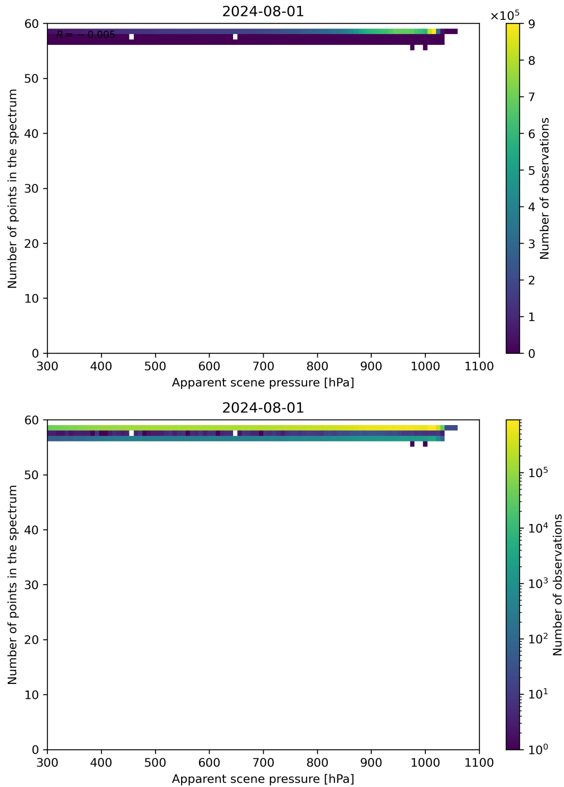
Figure 66: Scatter density plot of “Apparent scene pressure” against “Number of points in the spectrum” for 2024-07-31 to 2024-08-02.
