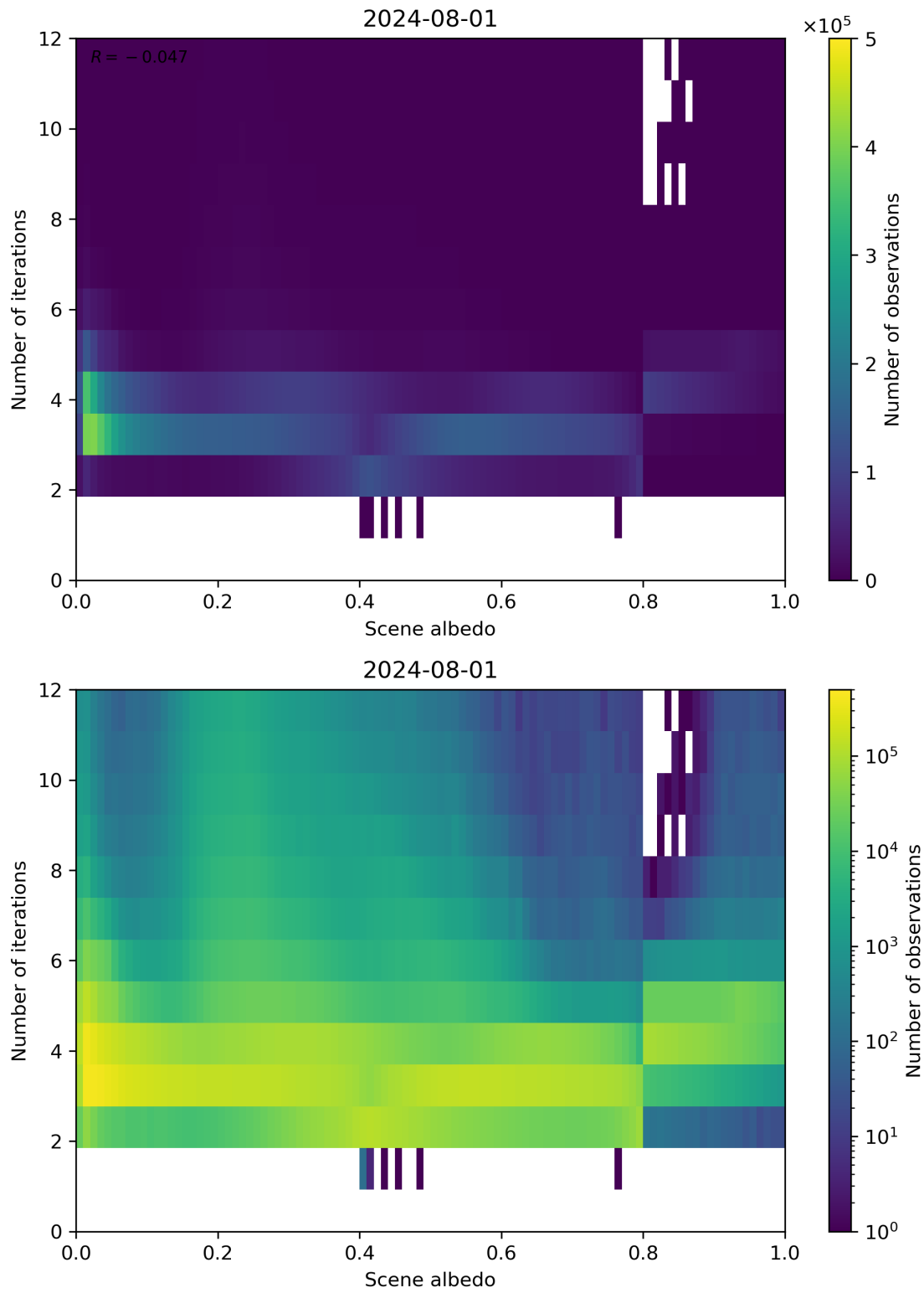
Figure 105: Scatter density plot of “Scene albedo” against “Number of iterations” for 2024-07-31 to 2024-08-02.
