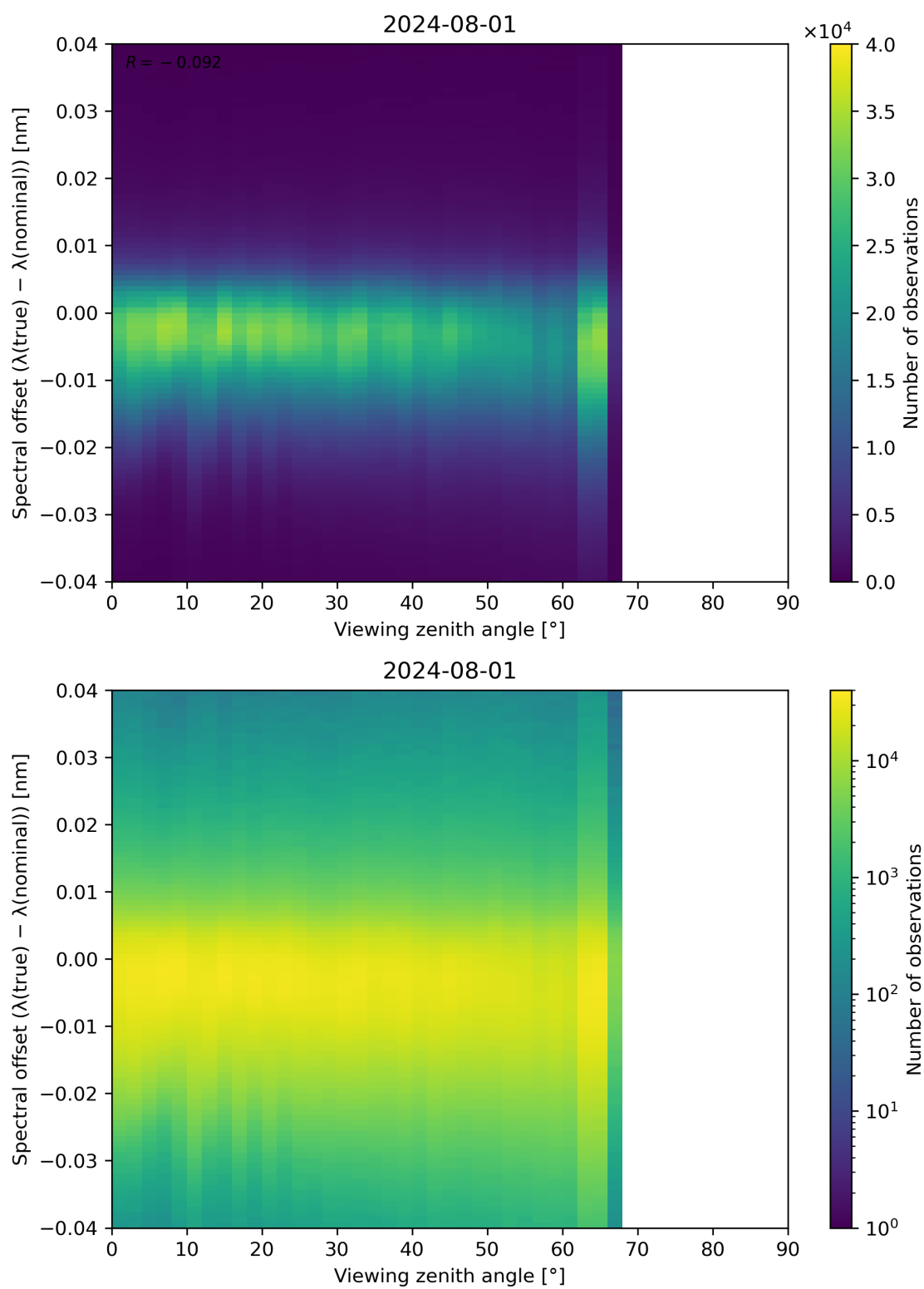
Figure 128: Scatter density plot of “Viewing zenith angle” against “Spectral offset ( \lambda(\text{true}) - \lambda(\text{nominal}) )” for 2024-07-31 to 2024-08-02.
