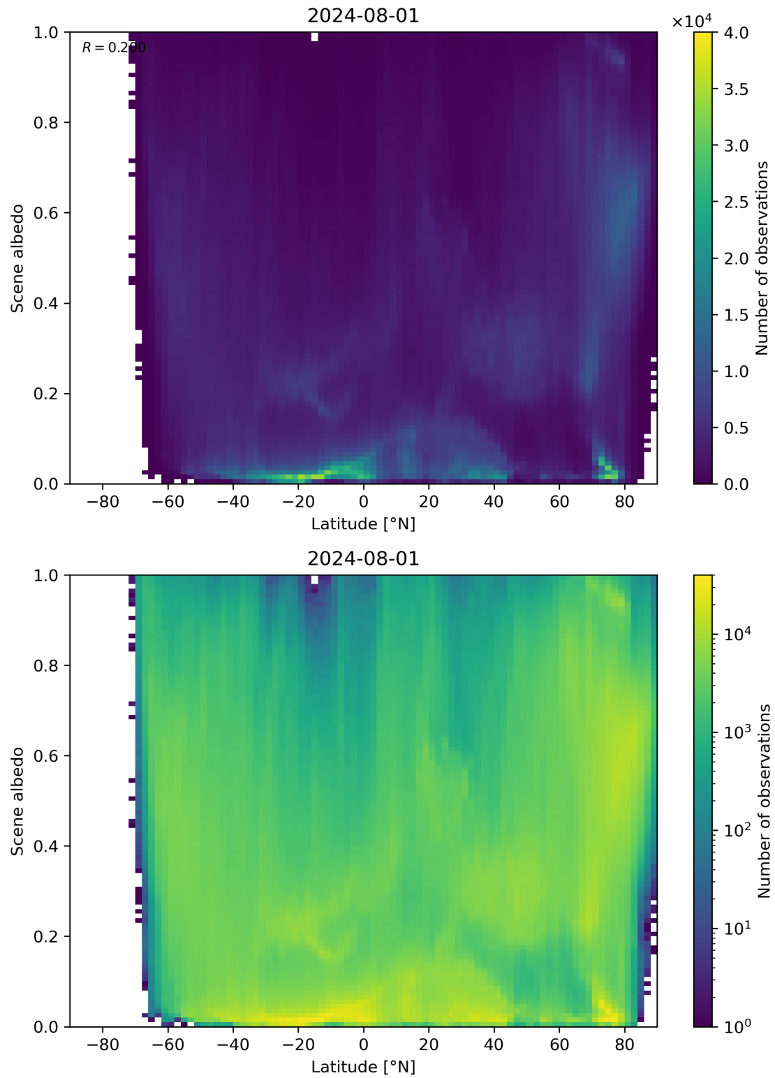
Figure 95: Scatter density plot of “Latitude” against “Scene albedo” for 2024-07-31 to 2024-08-02.
