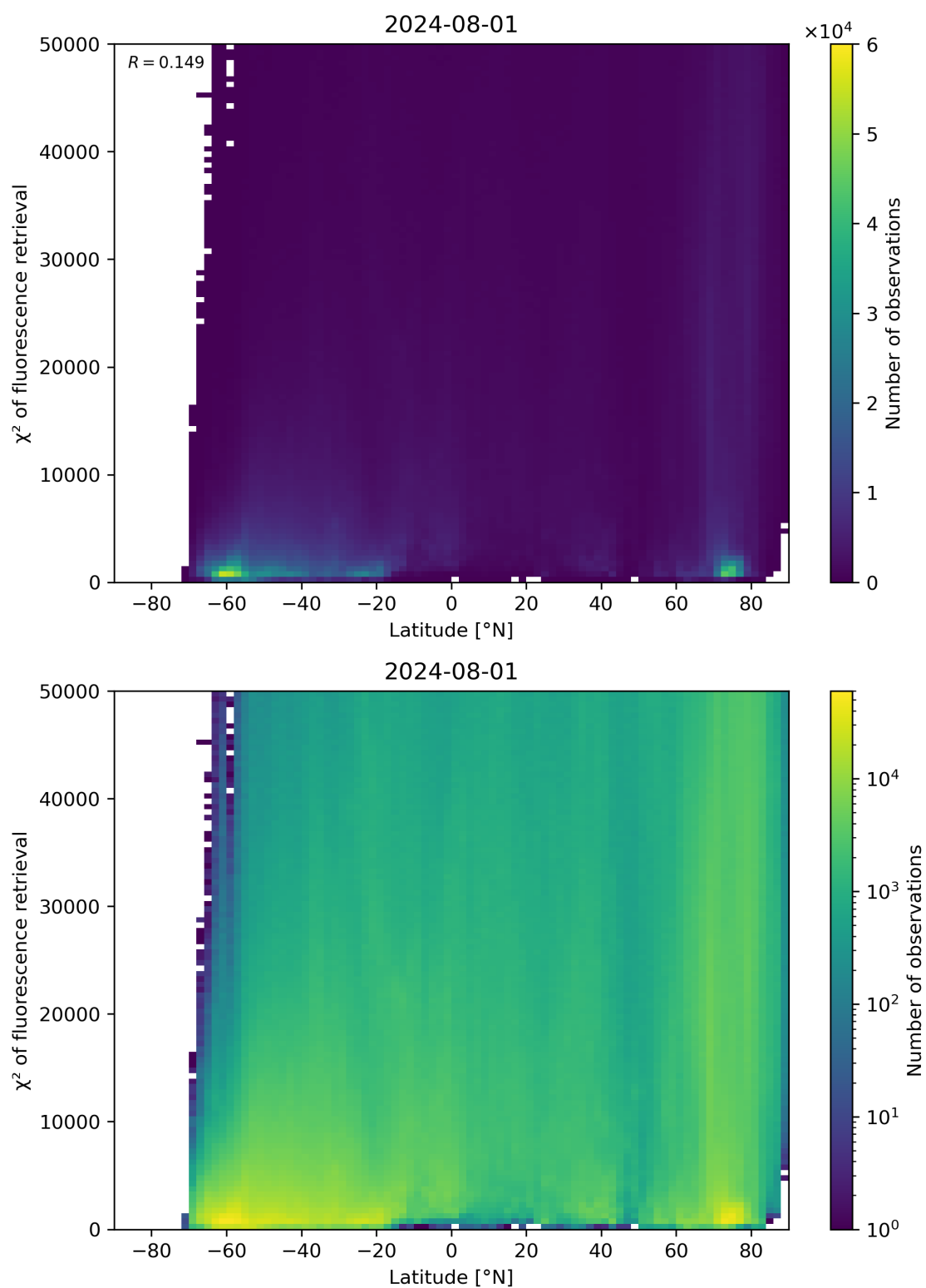
Figure 89: Scatter density plot of “Latitude” against “ \chi^2 of fluorescence retrieval” for 2024-07-31 to 2024-08-02.
