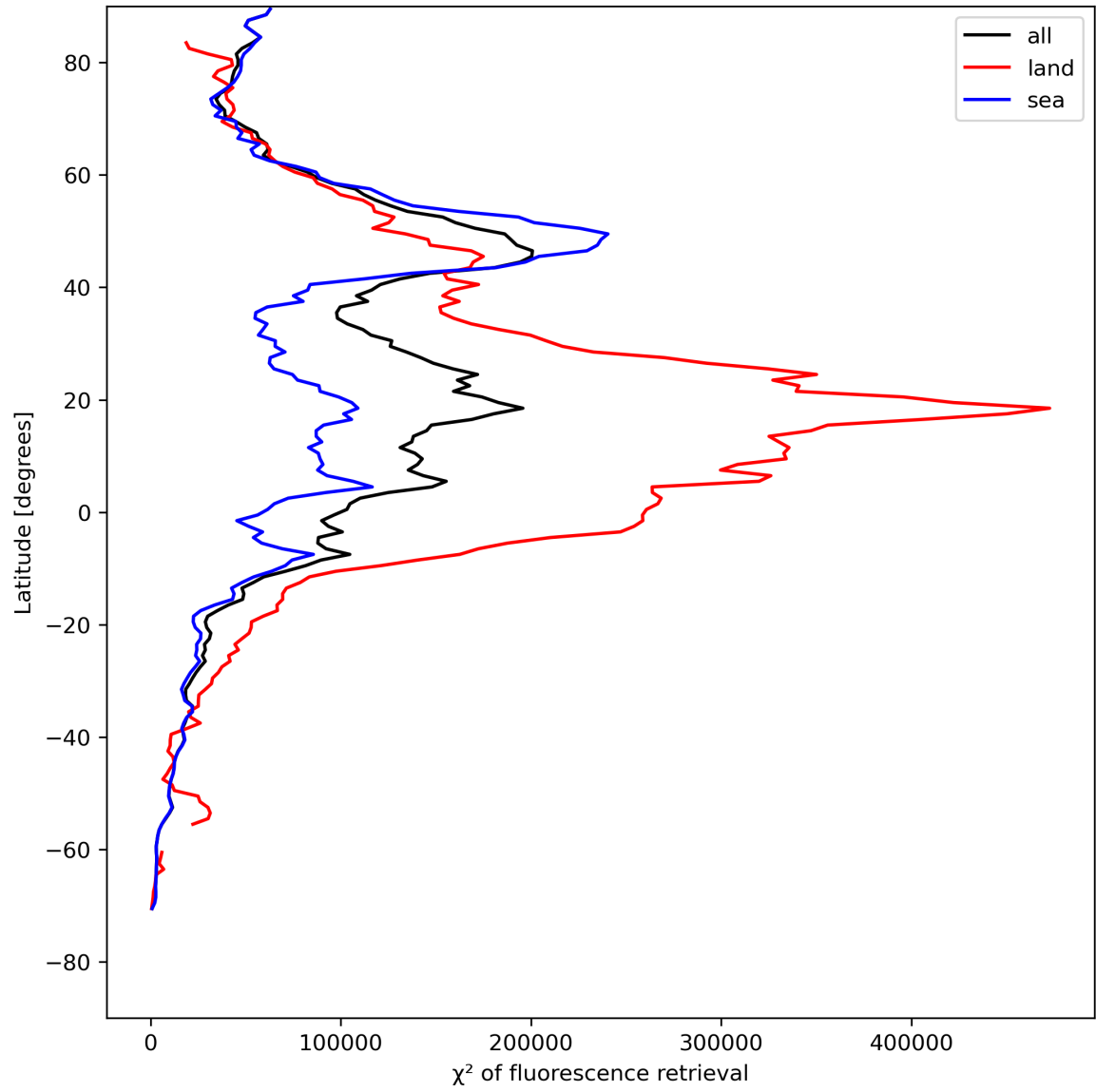
Figure 25: Zonal average of “ \chi^2 of fluorescence retrieval” for 2024-07-31 to 2024-08-02.
