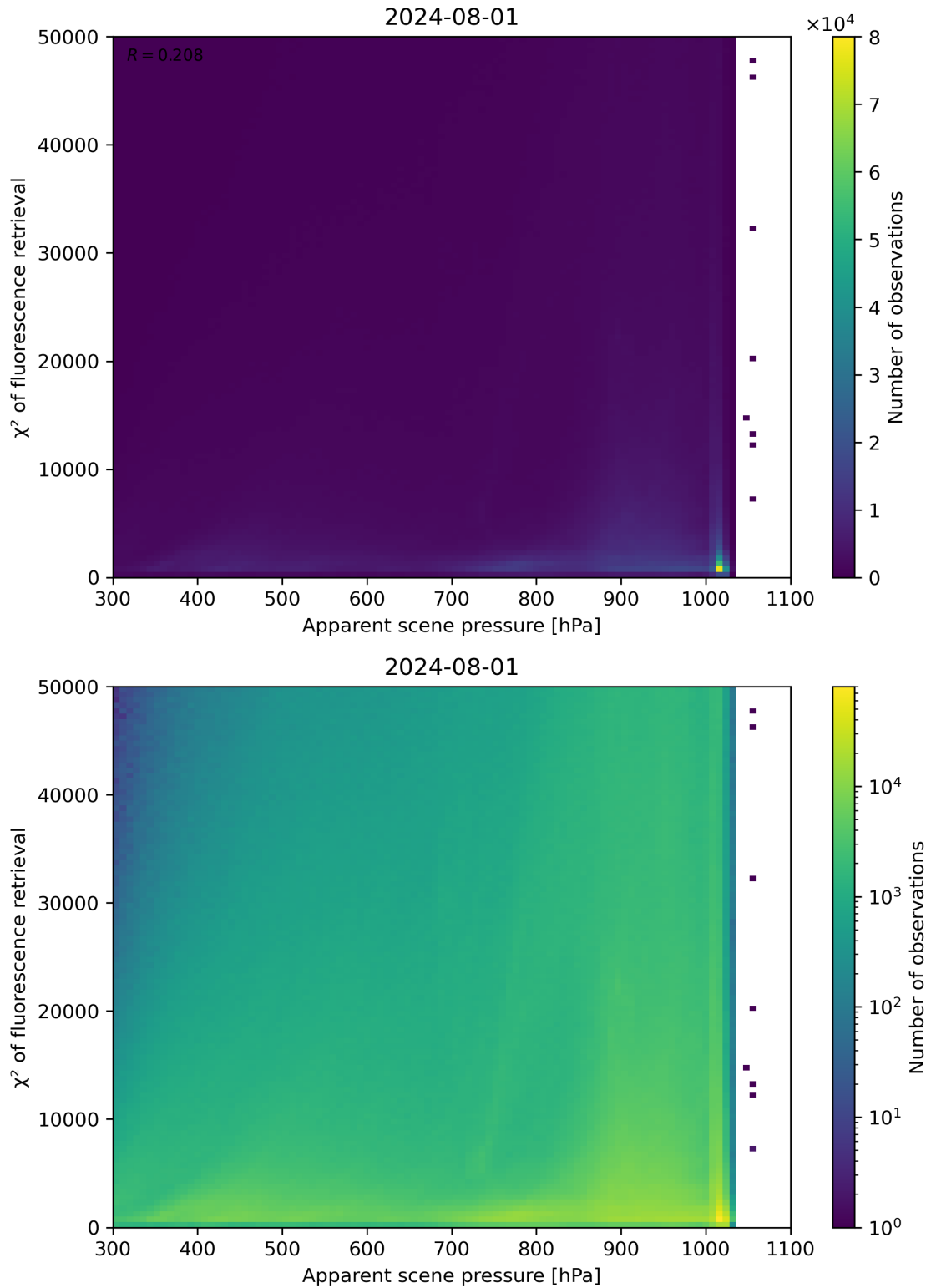
Figure 63: Scatter density plot of “Apparent scene pressure” against “ \chi^2 of fluorescence retrieval” for 2024-07-31 to 2024-08-02.
