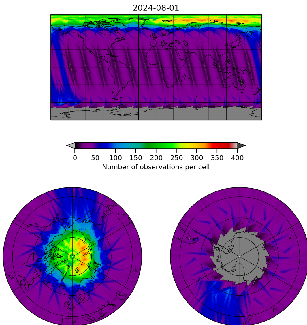
Figure 11: Map of the number of observations for 2024-07-31 to 2024-08-02
