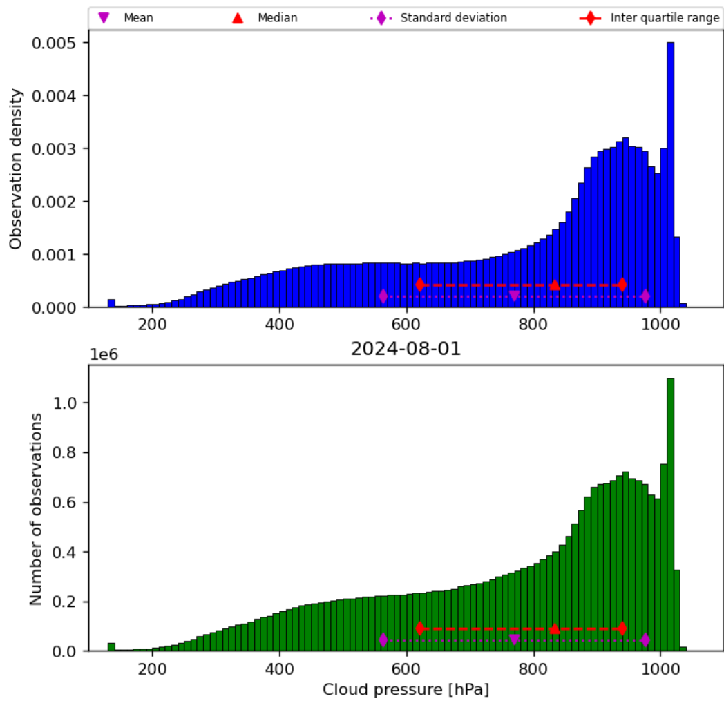
Figure 30: Histogram of “Cloud pressure” for 2024-07-31 to 2024-08-02
