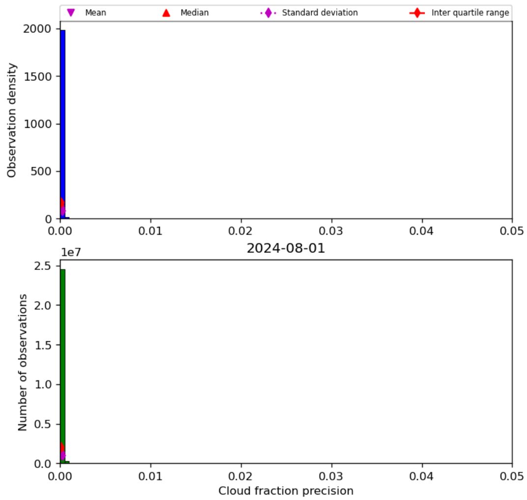
Figure 33: Histogram of “Cloud fraction precision” for 2024-07-31 to 2024-08-02
