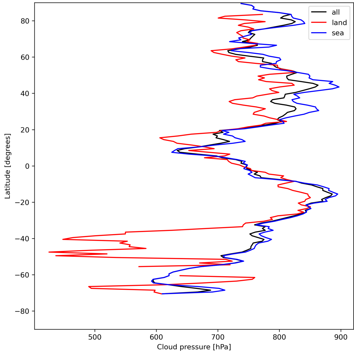
Figure 13: Zonal average of “Cloud pressure” for 2024-07-31 to 2024-08-02.
