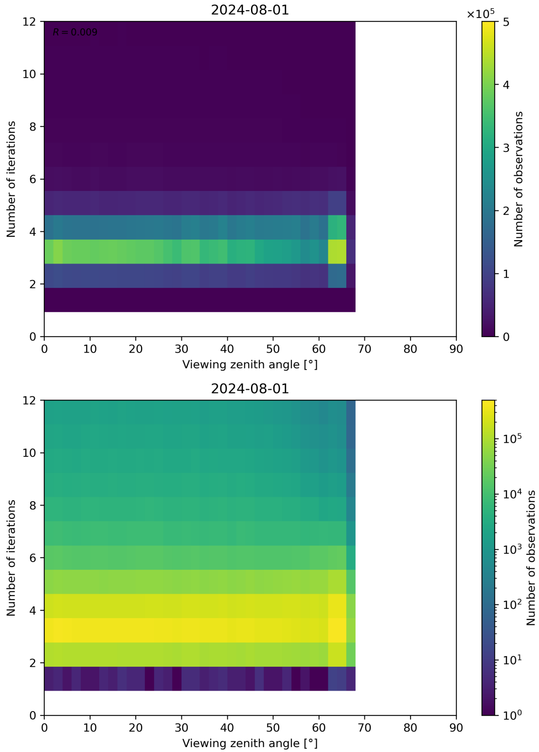
Figure 124: Scatter density plot of “Viewing zenith angle” against “Number of iterations” for 2024-07-31 to 2024-08-02.
