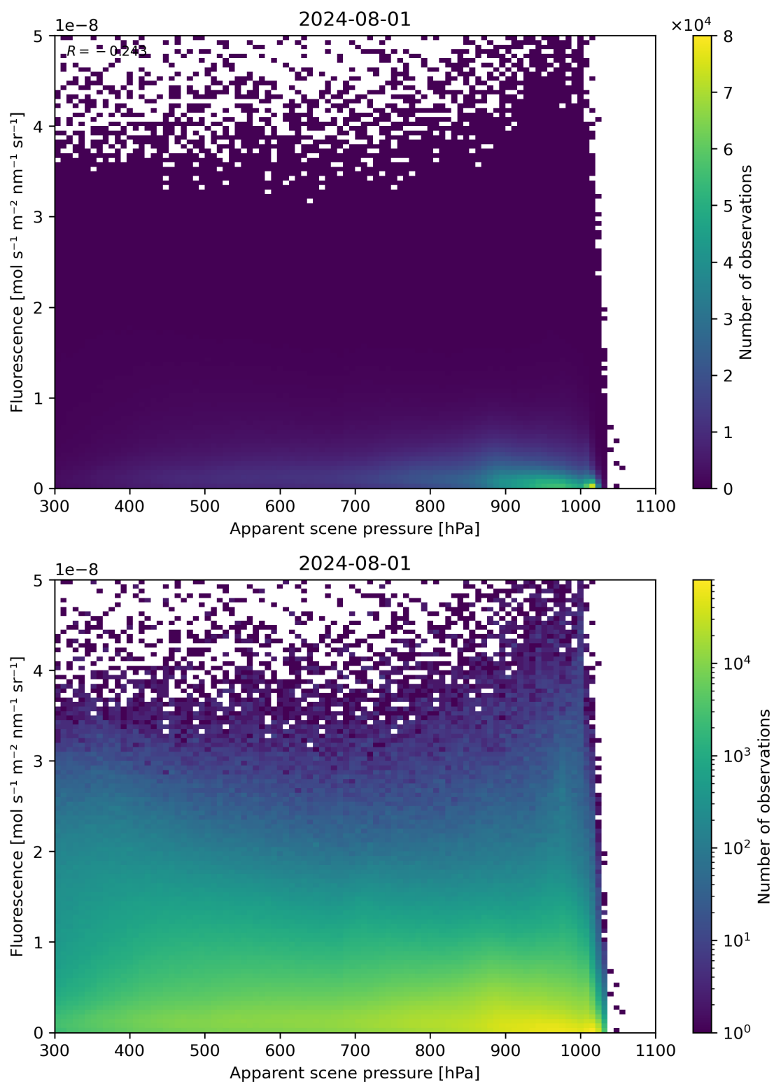
Figure 64: Scatter density plot of “Apparent scene pressure” against “Fluorescence” for 2024-07-31 to 2024-08-02.
