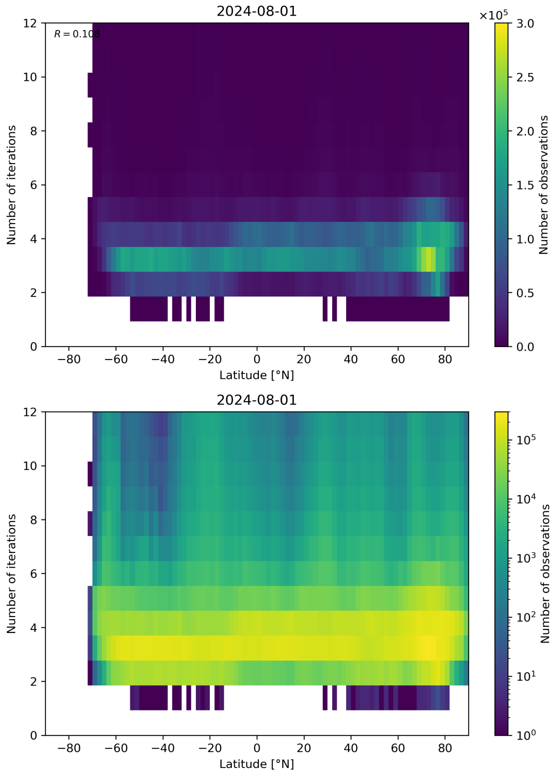
Figure 93: Scatter density plot of “Latitude” against “Number of iterations” for 2024-07-31 to 2024-08-02.
