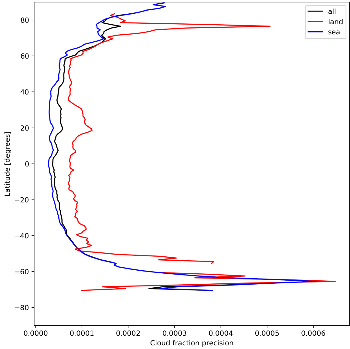
Figure 16: Zonal average of “Cloud fraction precision” for 2024-07-31 to 2024-08-02.
