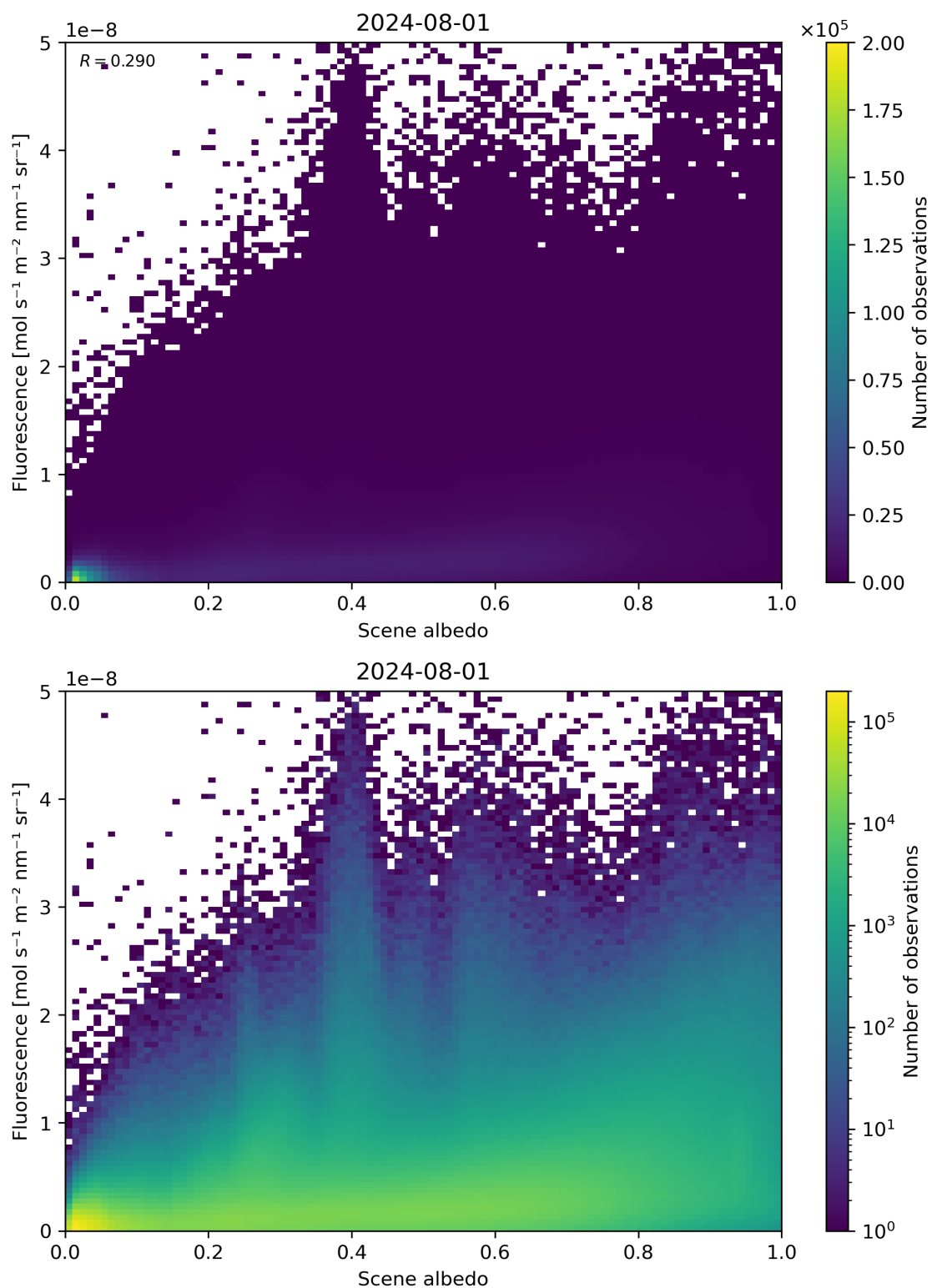
Figure 104: Scatter density plot of “Scene albedo” against “Fluorescence” for 2024-07-31 to 2024-08-02.
