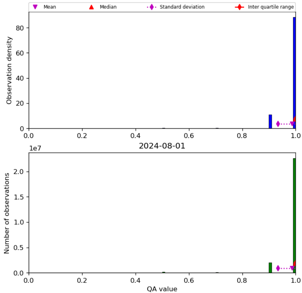
Figure 29: Histogram of “QA value” for 2024-07-31 to 2024-08-02
