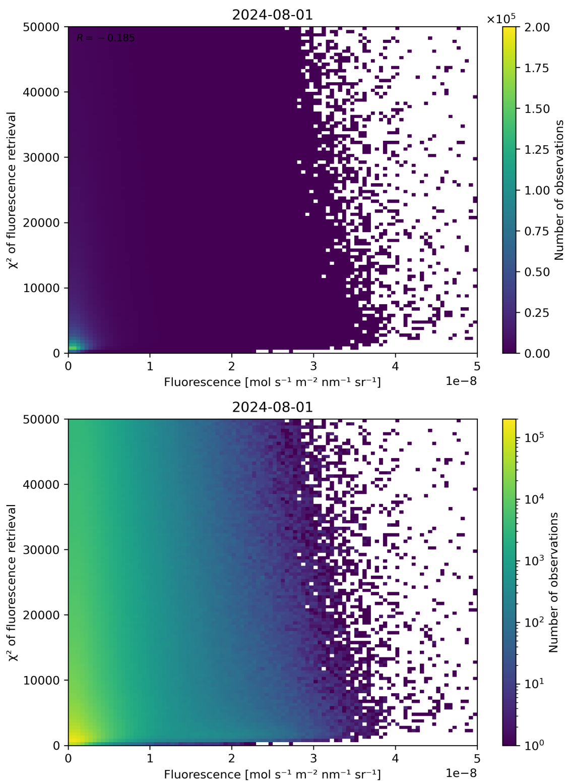
Figure 85: Scatter density plot of “Fluorescence” against “ \chi^2 of fluorescence retrieval” for 2024-07-31 to 2024-08-02.
