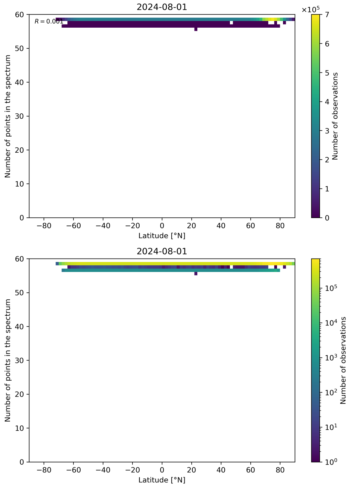
Figure 94: Scatter density plot of “Latitude” against “Number of points in the spectrum” for 2024-07-31 to 2024-08-02.
