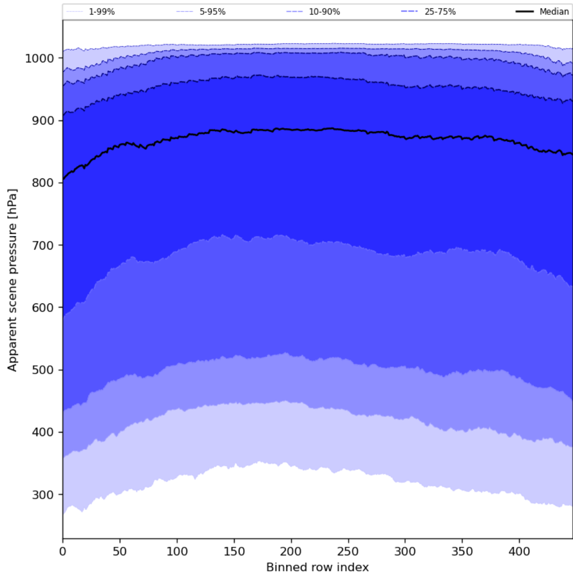
Figure 53: Along track statistics of “Apparent scene pressure” for 2024-07-31 to 2024-08-02
