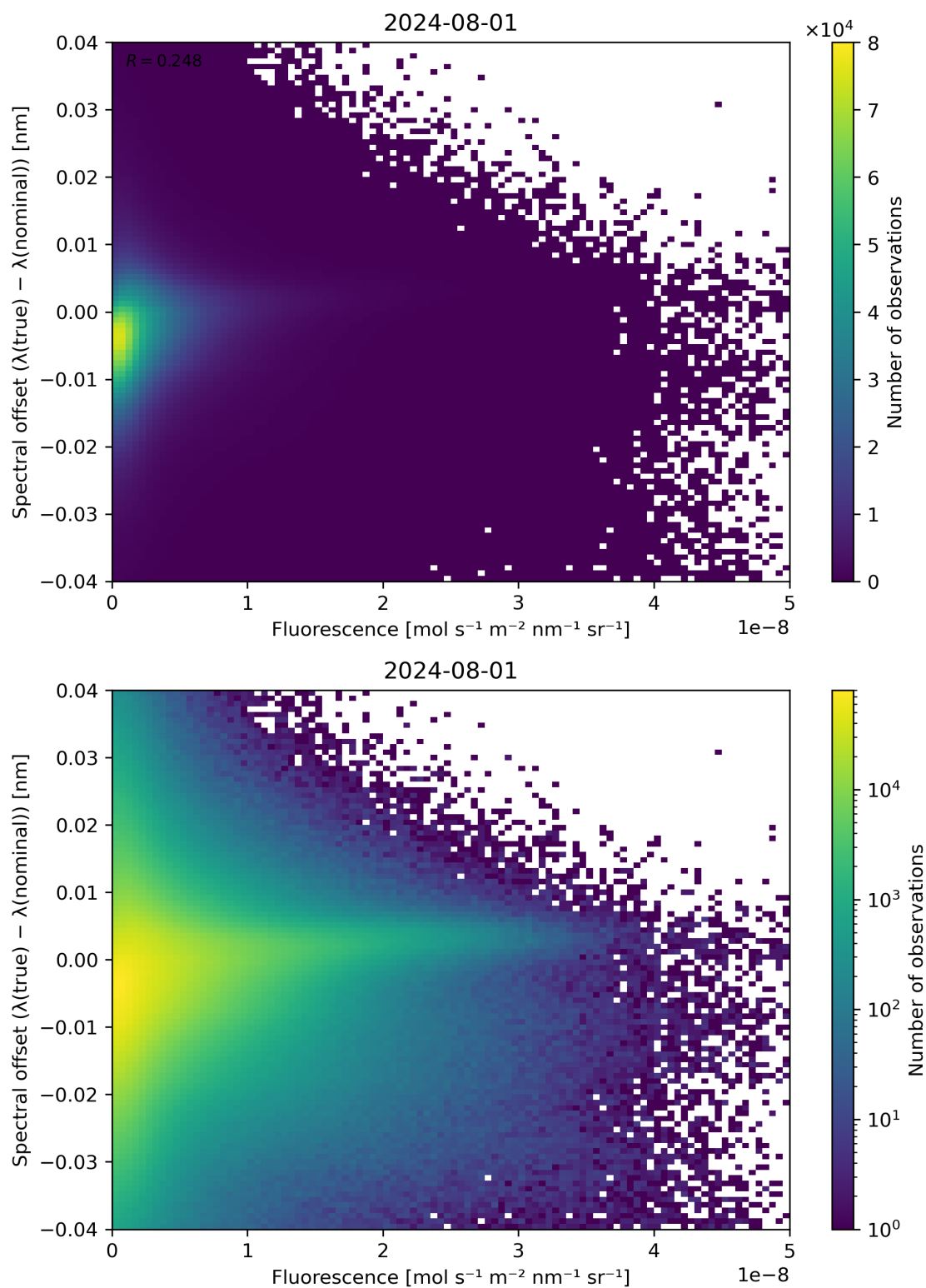
Figure 87: Scatter density plot of “Fluorescence” against “Spectral offset ( \lambda(\text{true}) - \lambda(\text{nominal}) )” for 2024-07-31 to 2024-08-02.
