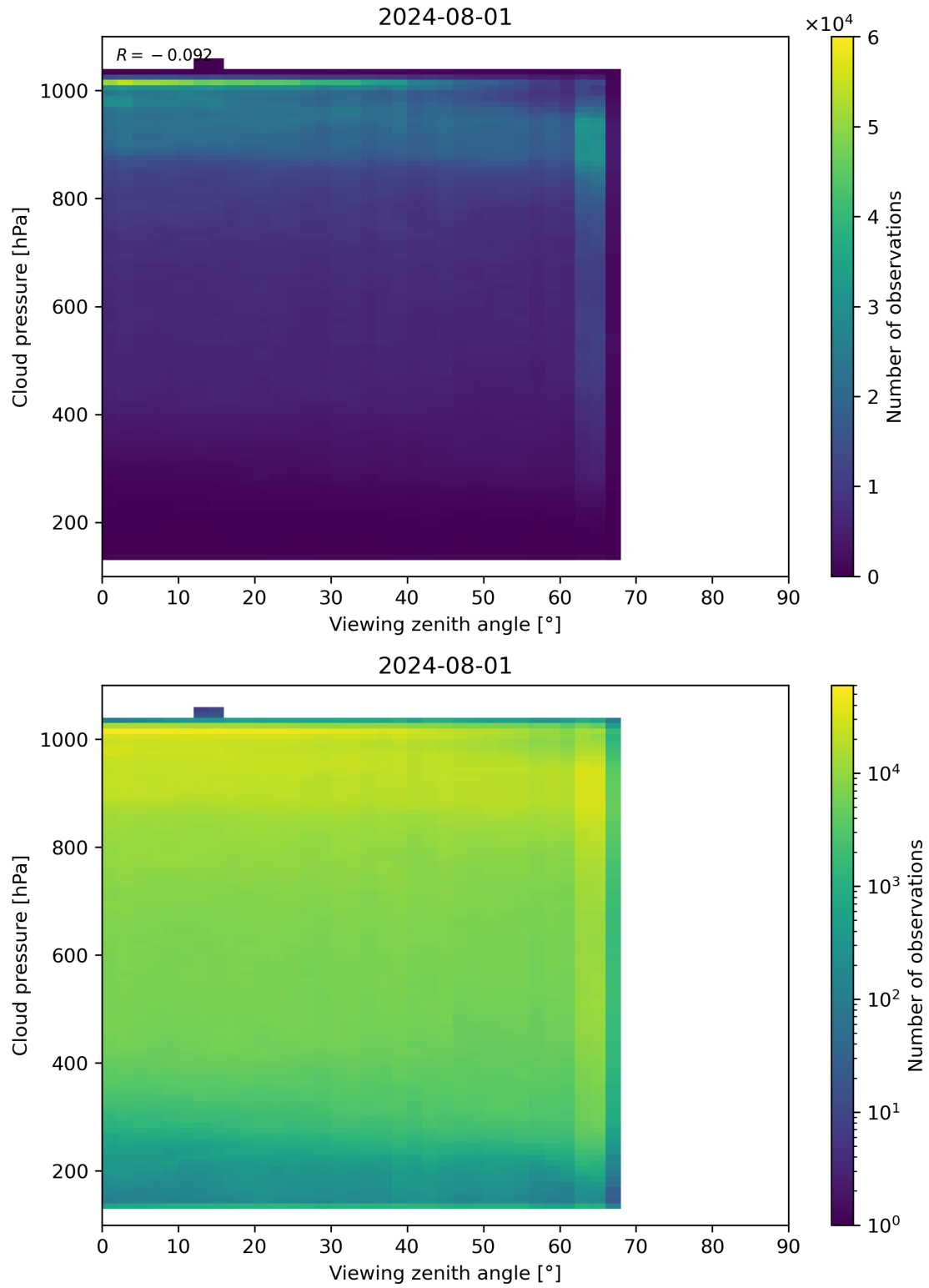
Figure 121: Scatter density plot of “Viewing zenith angle” against “Cloud pressure” for 2024-07-31 to 2024-08-02.
