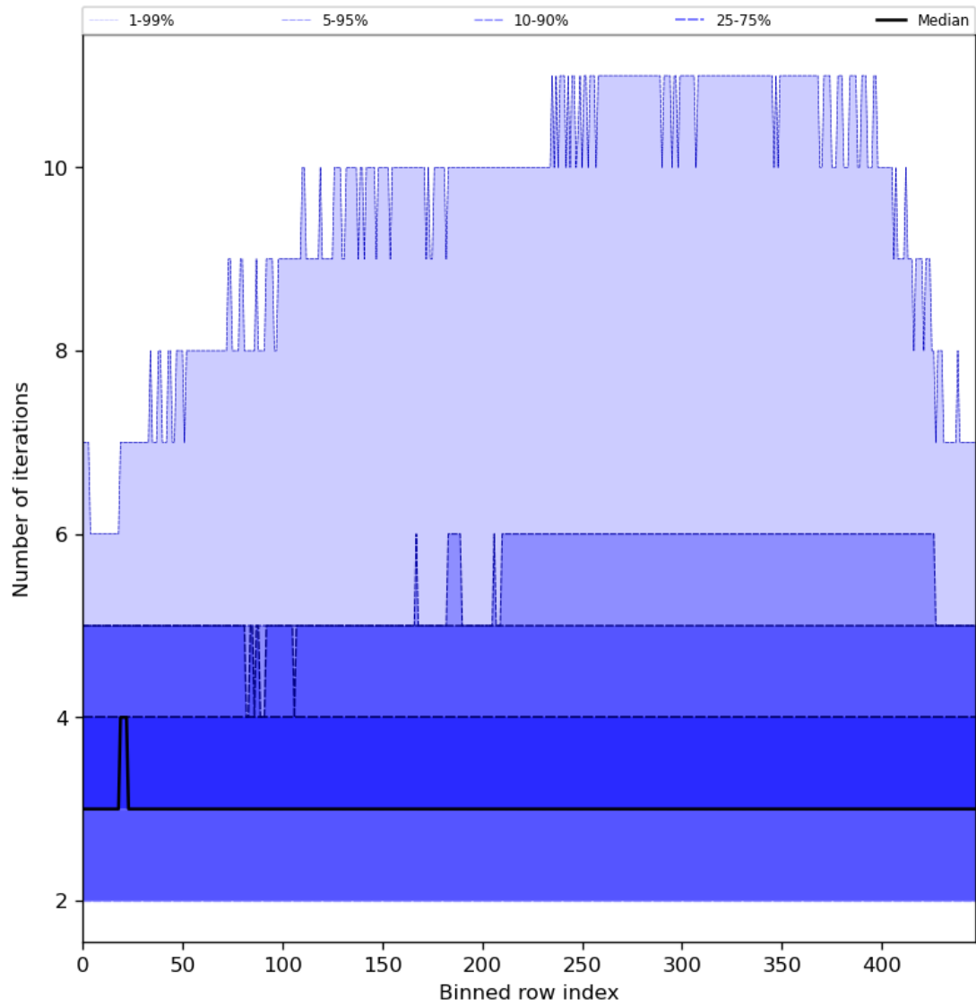
Figure 56: Along track statistics of “Number of iterations” for 2024-07-31 to 2024-08-02
