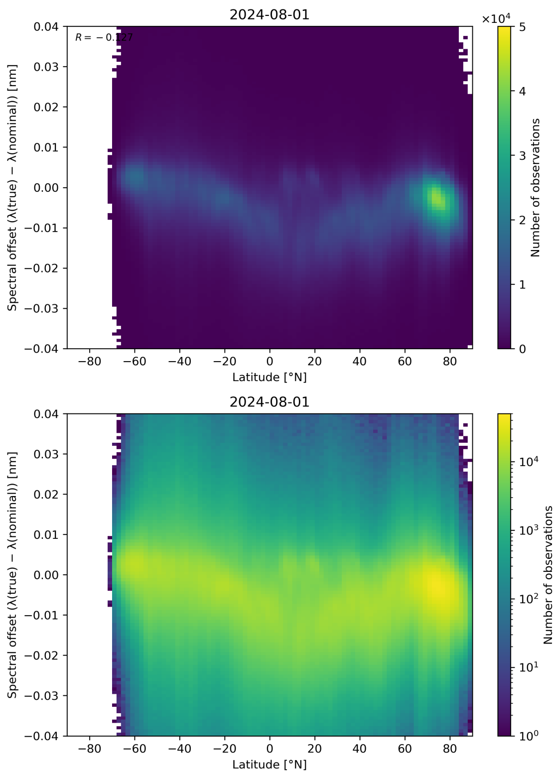
Figure 96: Scatter density plot of “Latitude” against “Spectral offset ( \lambda(\text{true}) - \lambda(\text{nominal}) )” for 2024-07-31 to 2024-08-02.
