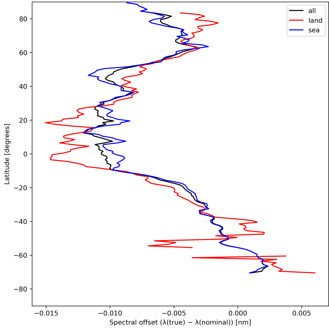
Figure 28: Zonal average of “Spectral offset ( \lambda(\text{true}) - \lambda(\text{nominal}) )” for 2024-07-31 to 2024-08-02.
