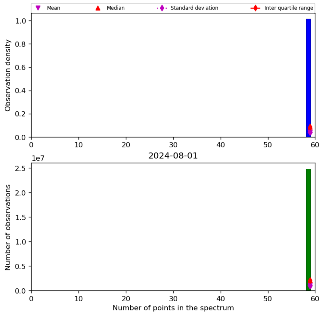
Figure 44: Histogram of “Number of points in the spectrum” for 2024-07-31 to 2024-08-02
