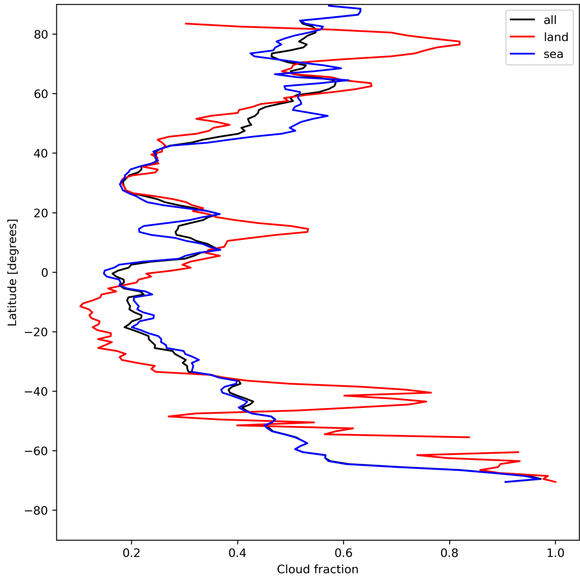
Figure 15: Zonal average of “Cloud fraction” for 2024-07-31 to 2024-08-02.
