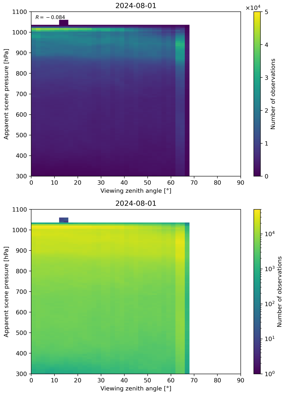
Figure 118: Scatter density plot of “Viewing zenith angle” against “Apparent scene pressure” for 2024-07-31 to 2024-08-02.
