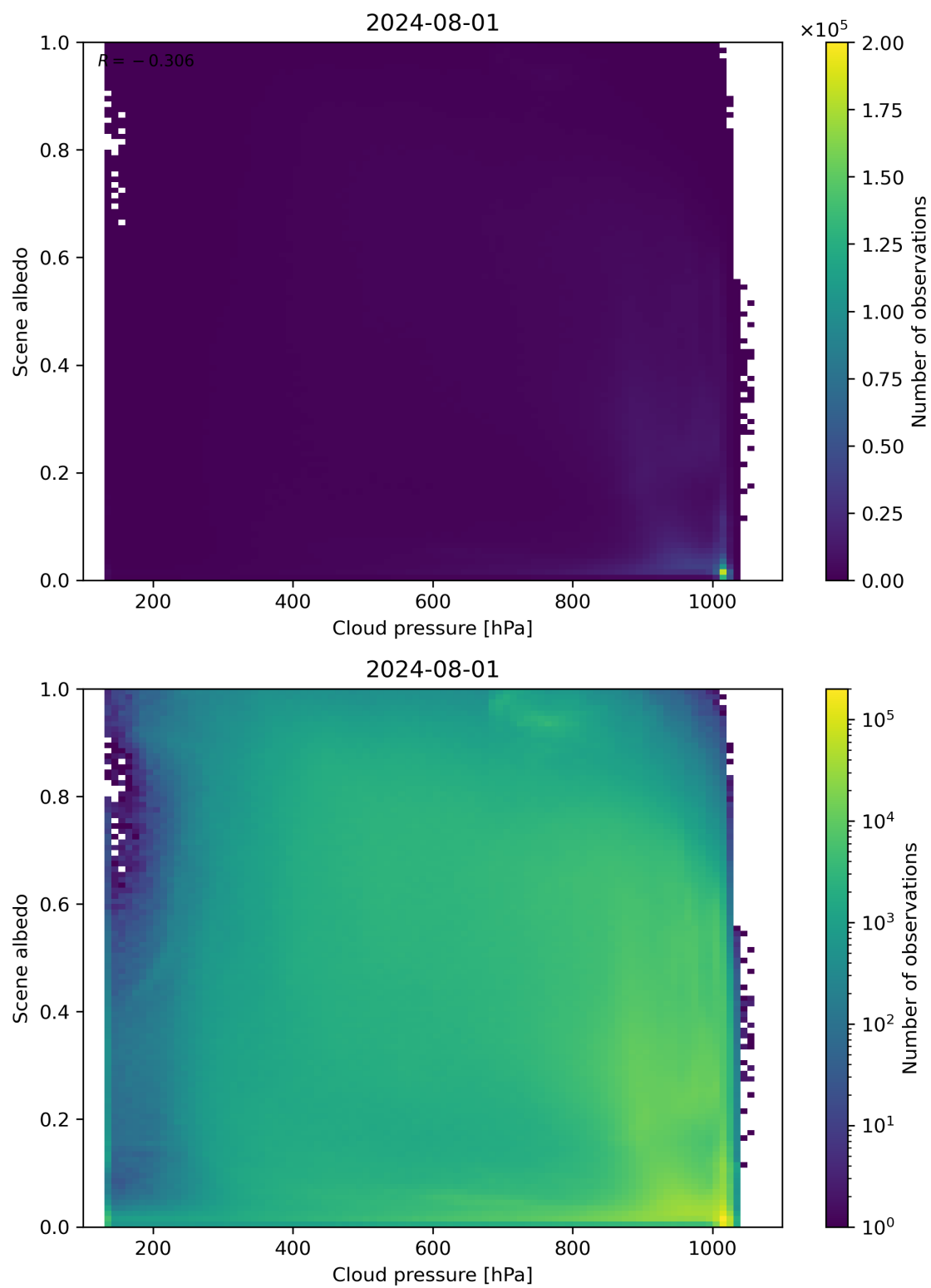
Figure 83: Scatter density plot of “Cloud pressure” against “Scene albedo” for 2024-07-31 to 2024-08-02.
