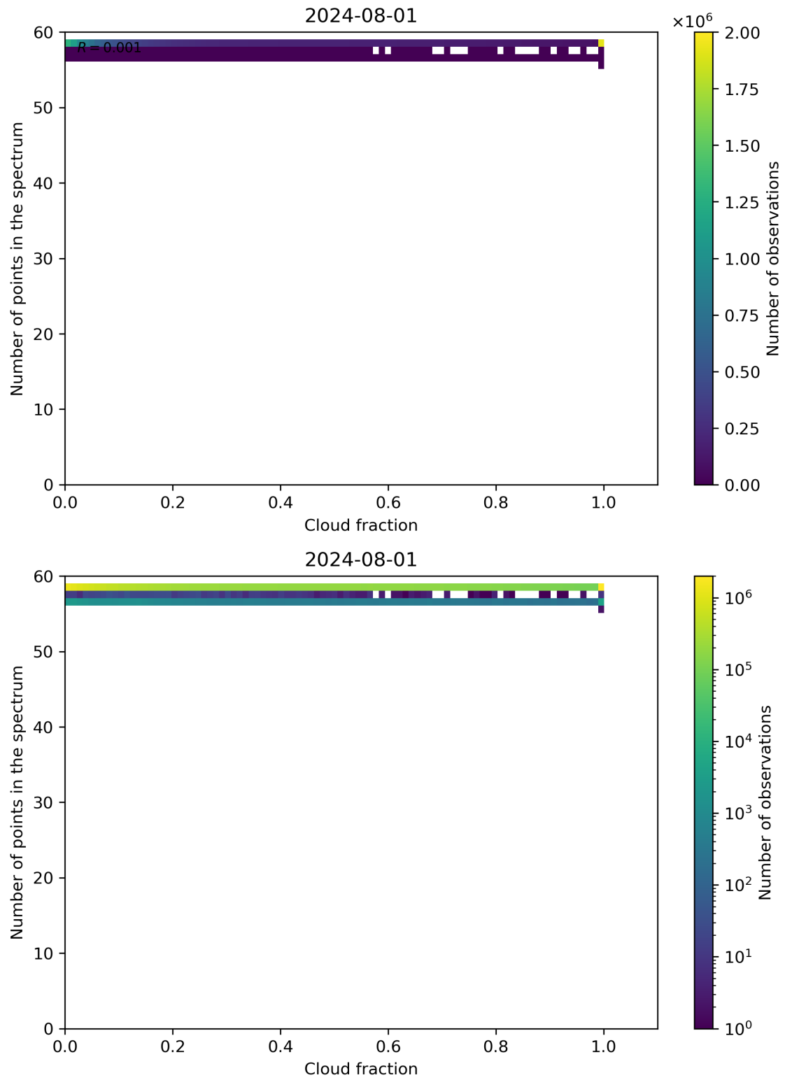
Figure 74: Scatter density plot of “Cloud fraction” against “Number of points in the spectrum” for 2024-07-31 to 2024-08-02.
