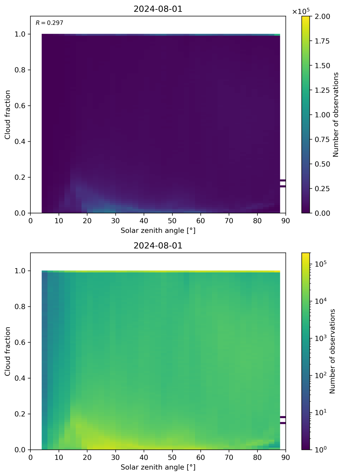
Figure 110: Scatter density plot of “Solar zenith angle” against “Cloud fraction” for 2024-07-31 to 2024-08-02.
