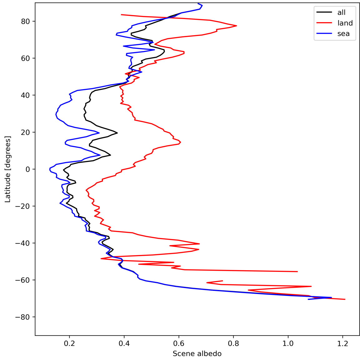
Figure 17: Zonal average of “Scene albedo” for 2024-07-31 to 2024-08-02.
