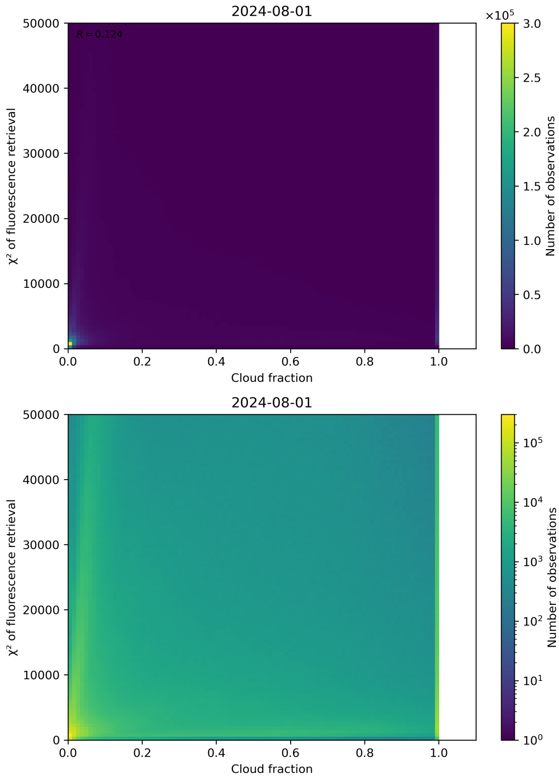
Figure 71: Scatter density plot of “Cloud fraction” against “ \chi^2 of fluorescence retrieval” for 2024-07-31 to 2024-08-02.
