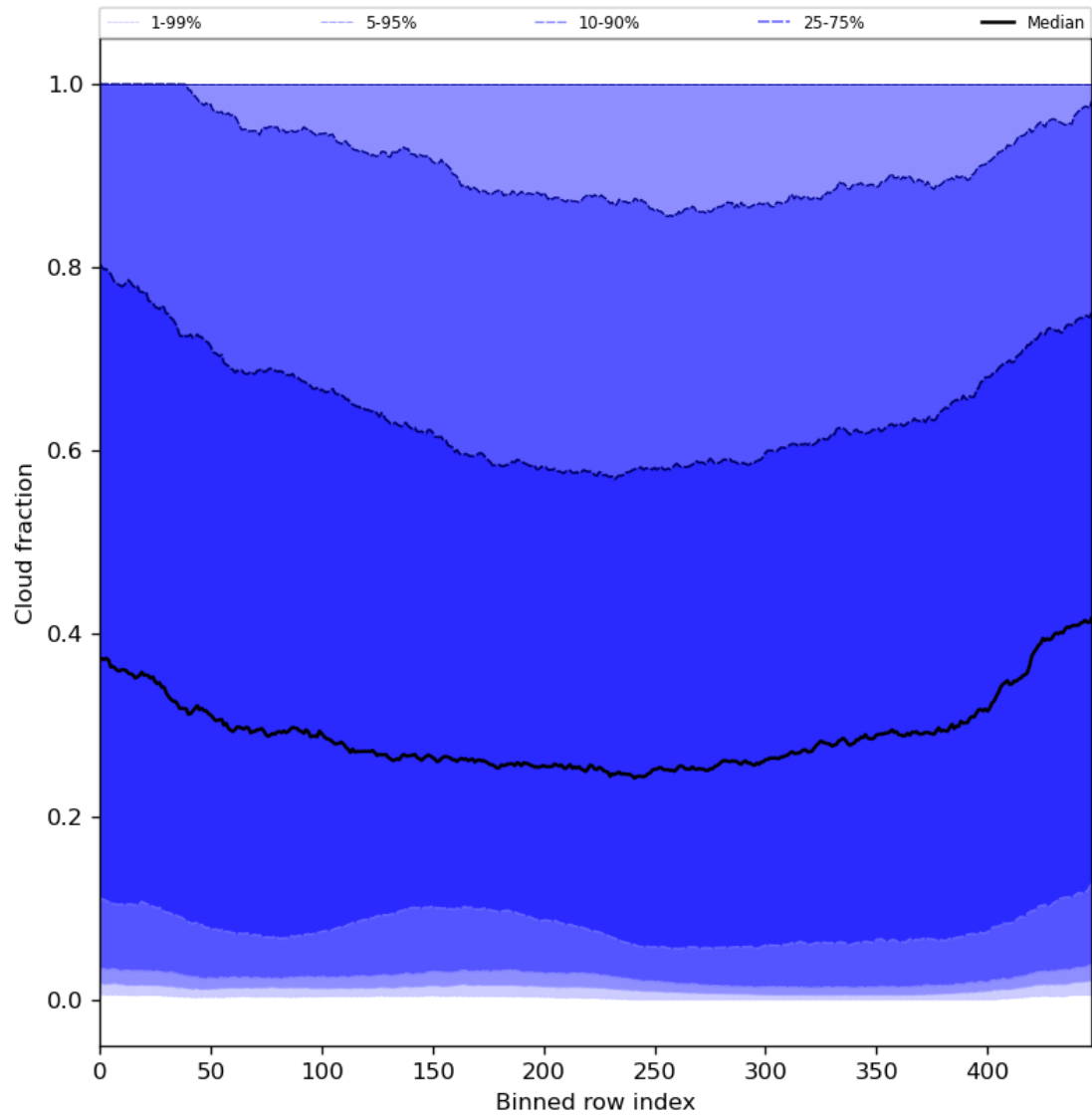
Figure 49: Along track statistics of “Cloud fraction” for 2024-07-31 to 2024-08-02
