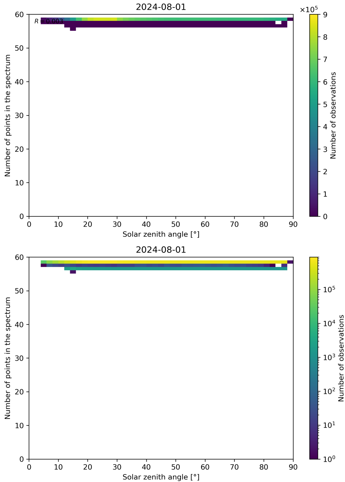
Figure 115: Scatter density plot of “Solar zenith angle” against “Number of points in the spectrum” for 2024-07-31 to 2024-08-02.
