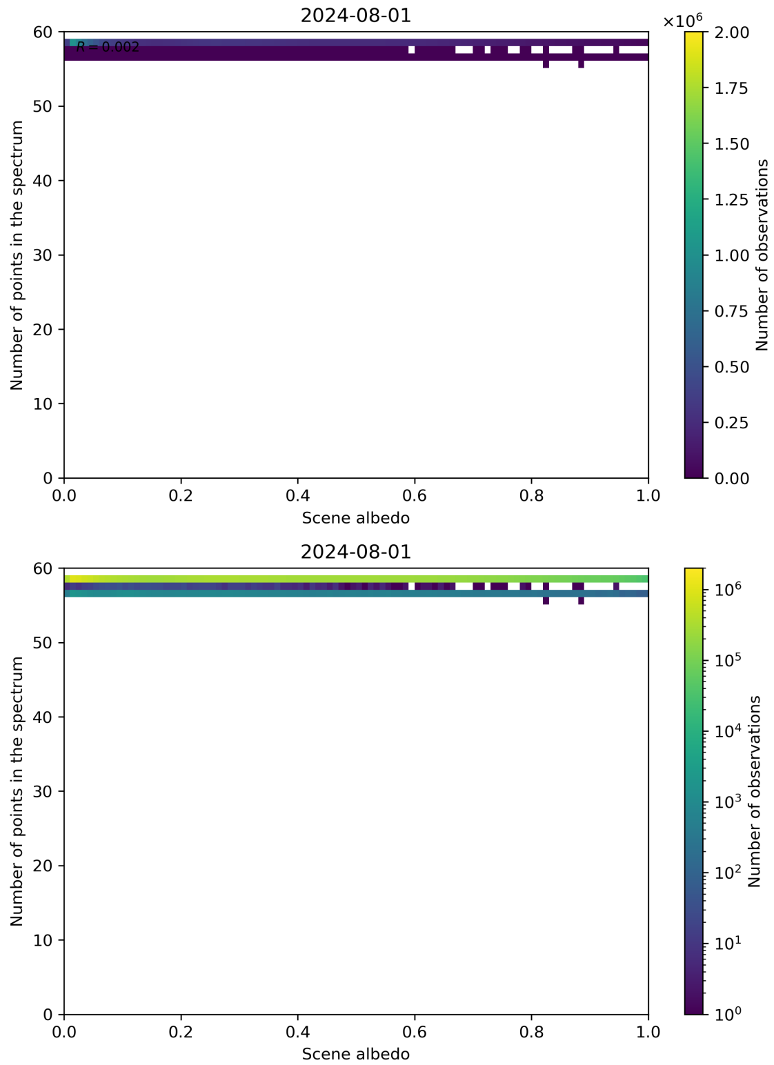
Figure 106: Scatter density plot of “Scene albedo” against “Number of points in the spectrum” for 2024-07-31 to 2024-08-02.
