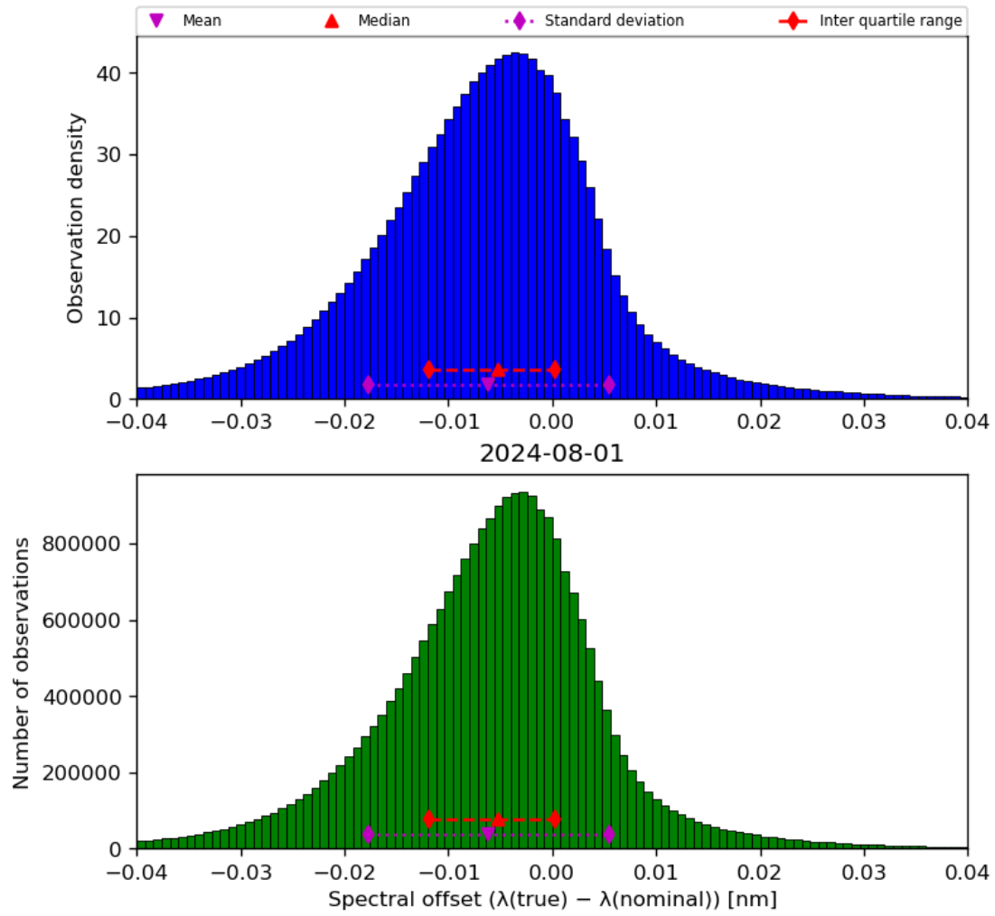
Figure 45: Histogram of “Spectral offset ( \lambda(\text{true}) - \lambda(\text{nominal}) )” for 2024-07-31 to 2024-08-02
