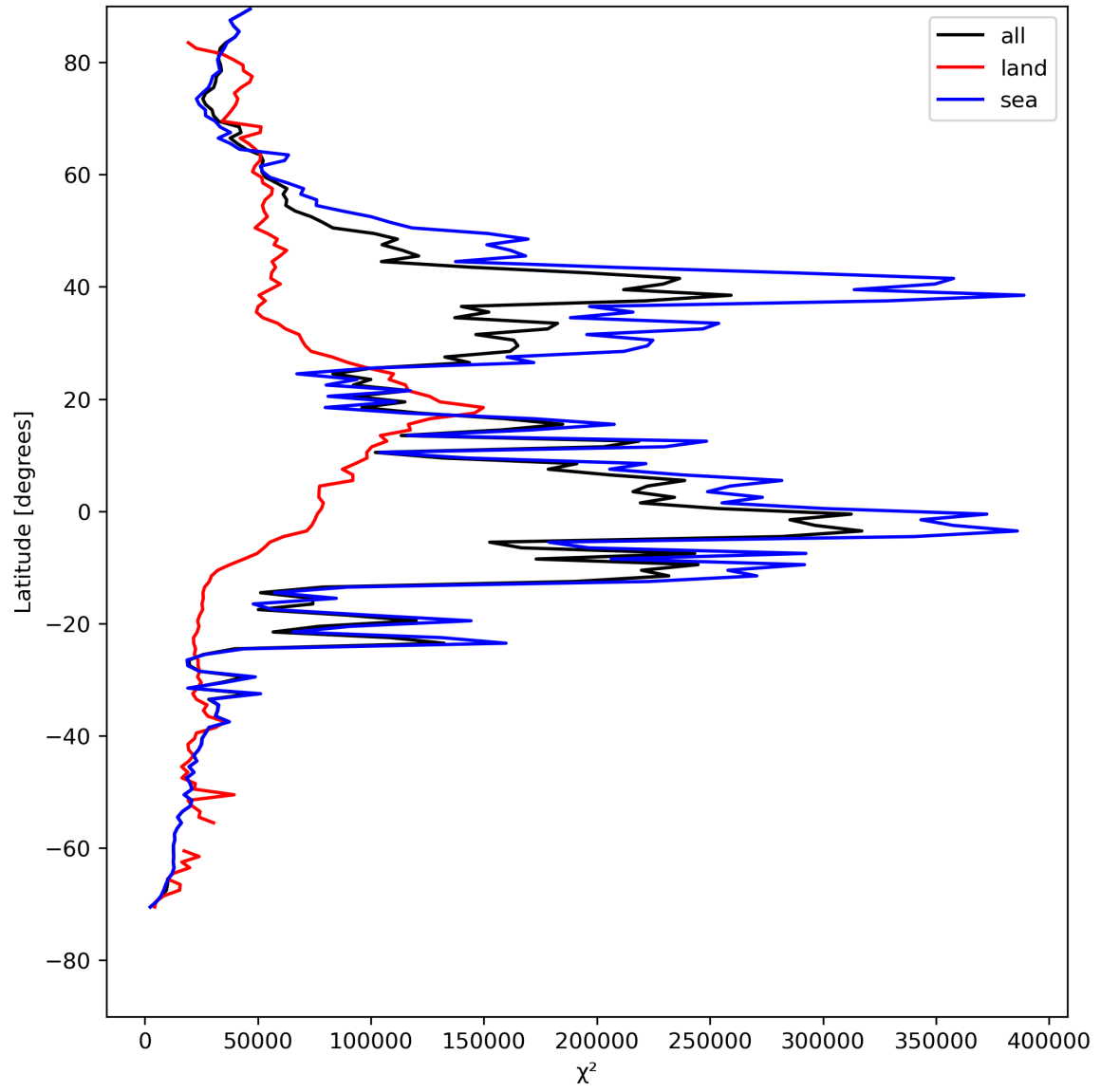
Figure 21: Zonal average of “ \chi^2 ” for 2024-07-31 to 2024-08-02.
