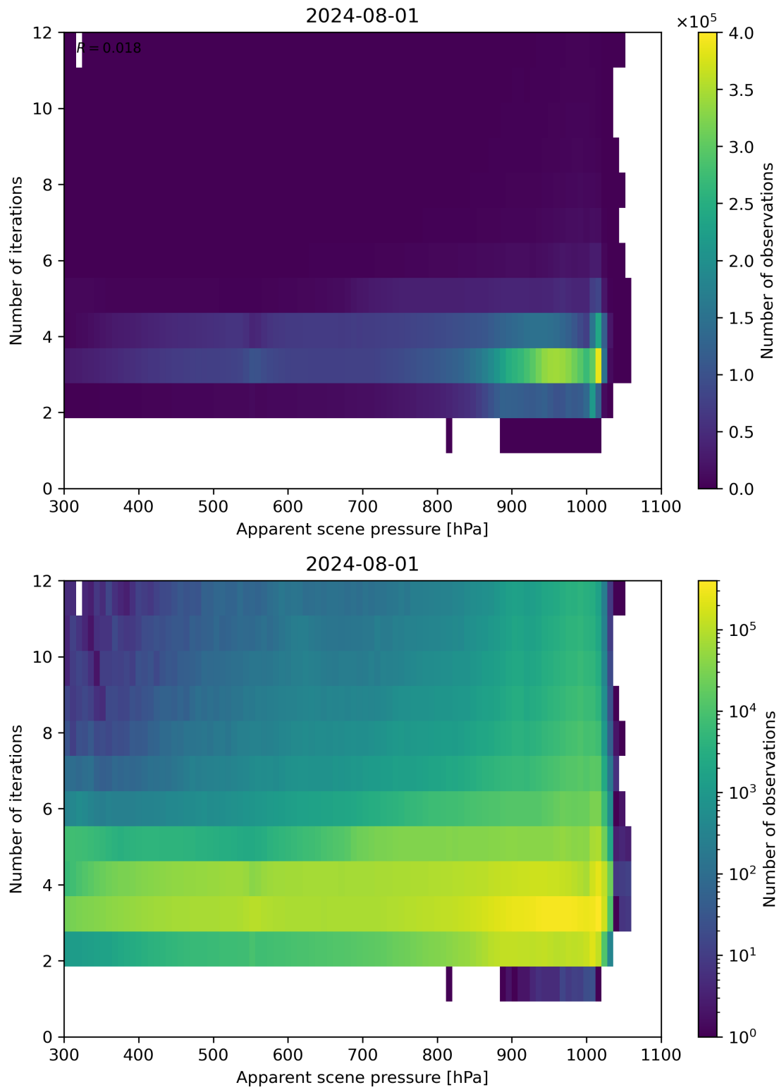
Figure 65: Scatter density plot of “Apparent scene pressure” against “Number of iterations” for 2024-07-31 to 2024-08-02.
