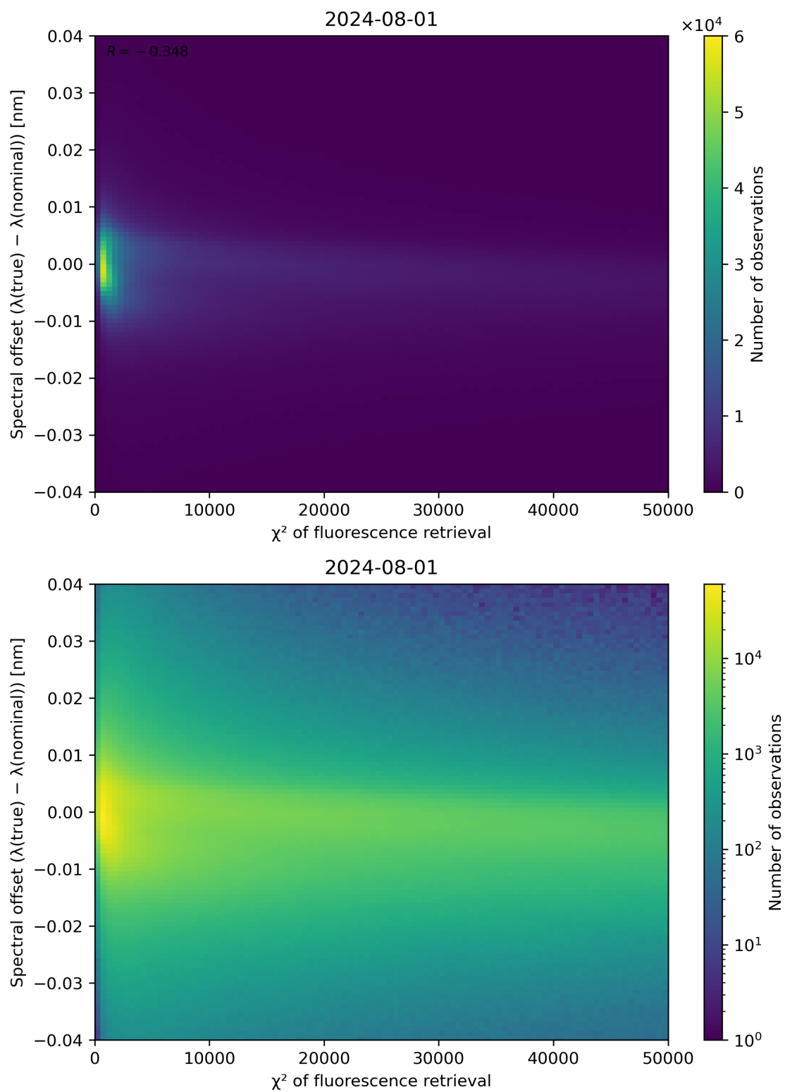
Figure 69: Scatter density plot of " \chi^2 of fluorescence retrieval" against "Spectral offset ( \lambda(\text{true}) - \lambda(\text{nominal}) )" for 2024-07-31 to 2024-08-02.
