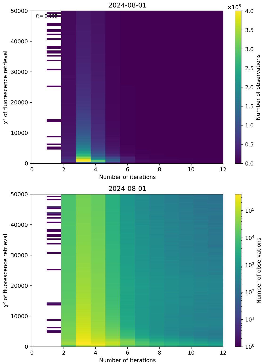
Figure 97: Scatter density plot of “Number of iterations” against “ \chi^2 of fluorescence retrieval” for 2024-07-31 to 2024-08-02.
