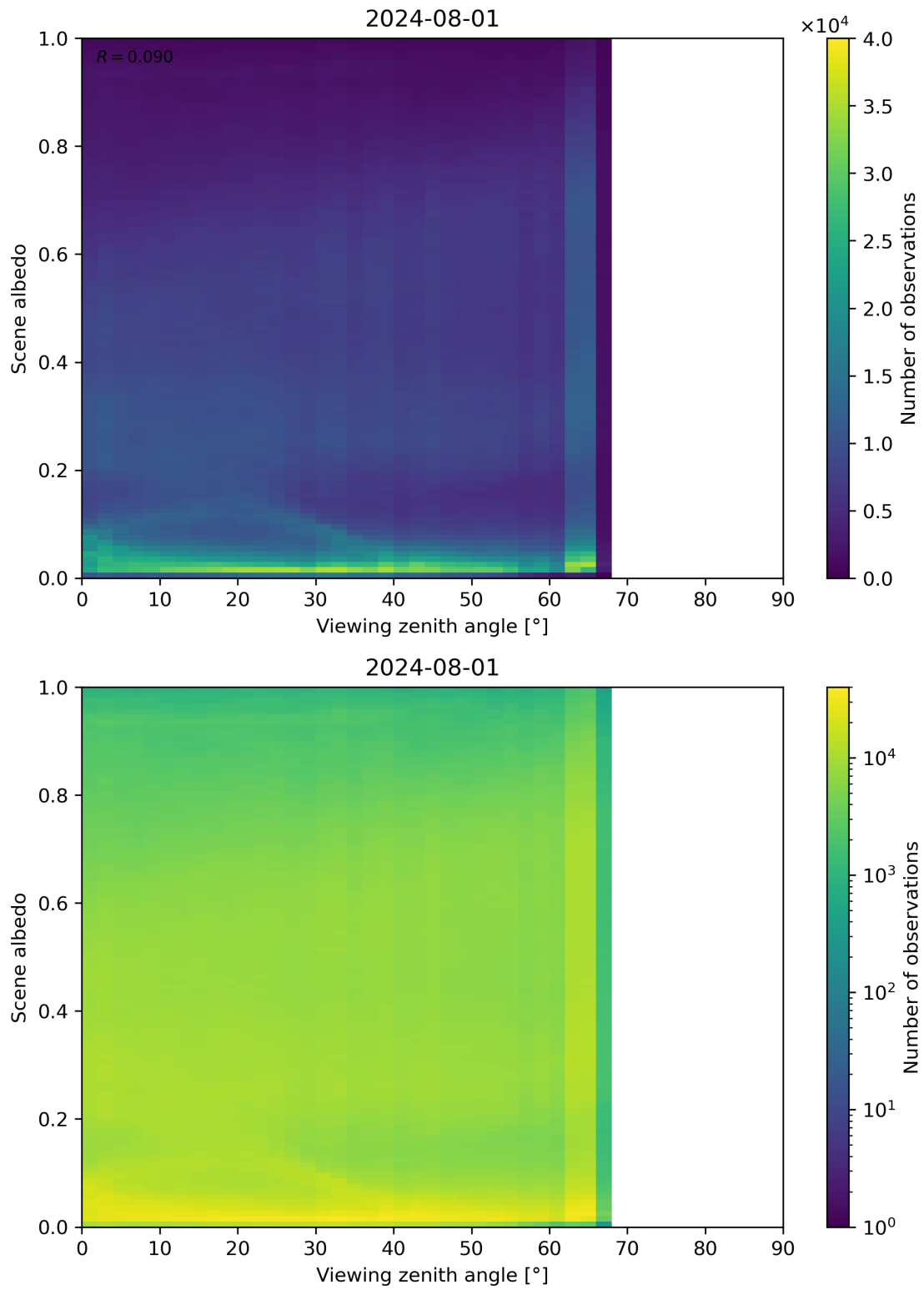
Figure 126: Scatter density plot of “Viewing zenith angle” against “Scene albedo” for 2024-07-31 to 2024-08-02.
