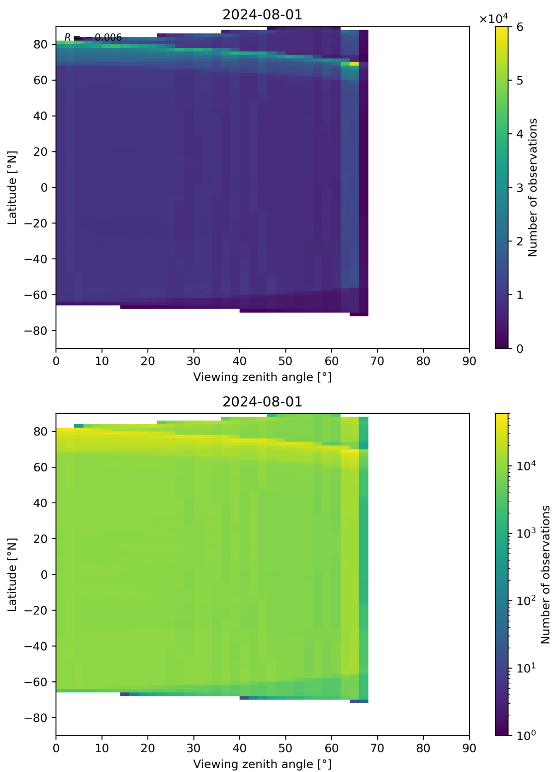
Figure 123: Scatter density plot of “Viewing zenith angle” against “Latitude” for 2024-07-31 to 2024-08-02.
