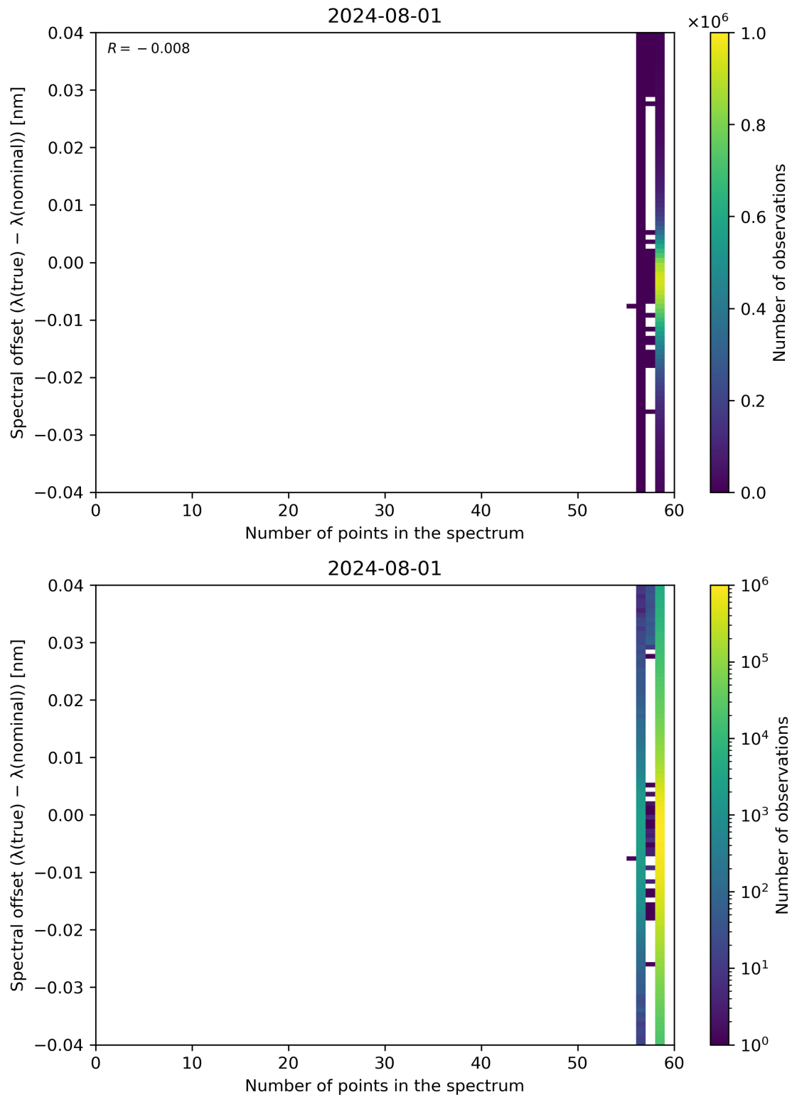
Figure 101: Scatter density plot of “Number of points in the spectrum” against “Spectral offset ( \lambda(\text{true}) - \lambda(\text{nominal}) )” for 2024-07-31 to 2024-08-02.
