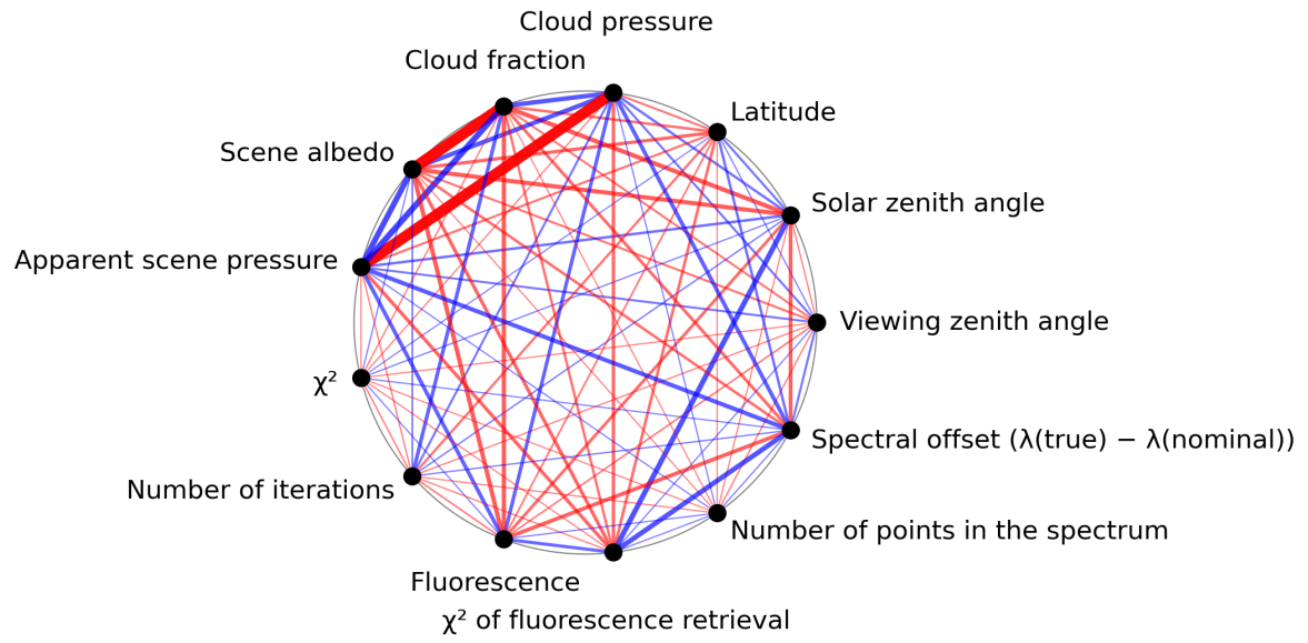
Figure 1: Map of correlation graph for 2024-07-31 to 2024-08-02.
