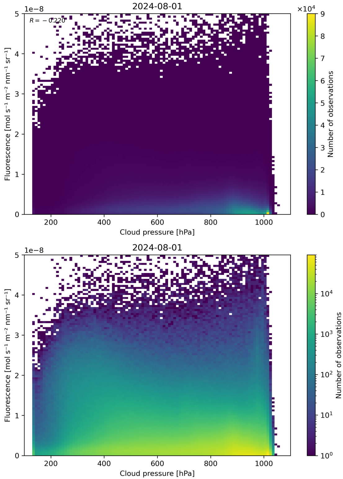
Figure 80: Scatter density plot of “Cloud pressure” against “Fluorescence” for 2024-07-31 to 2024-08-02.
