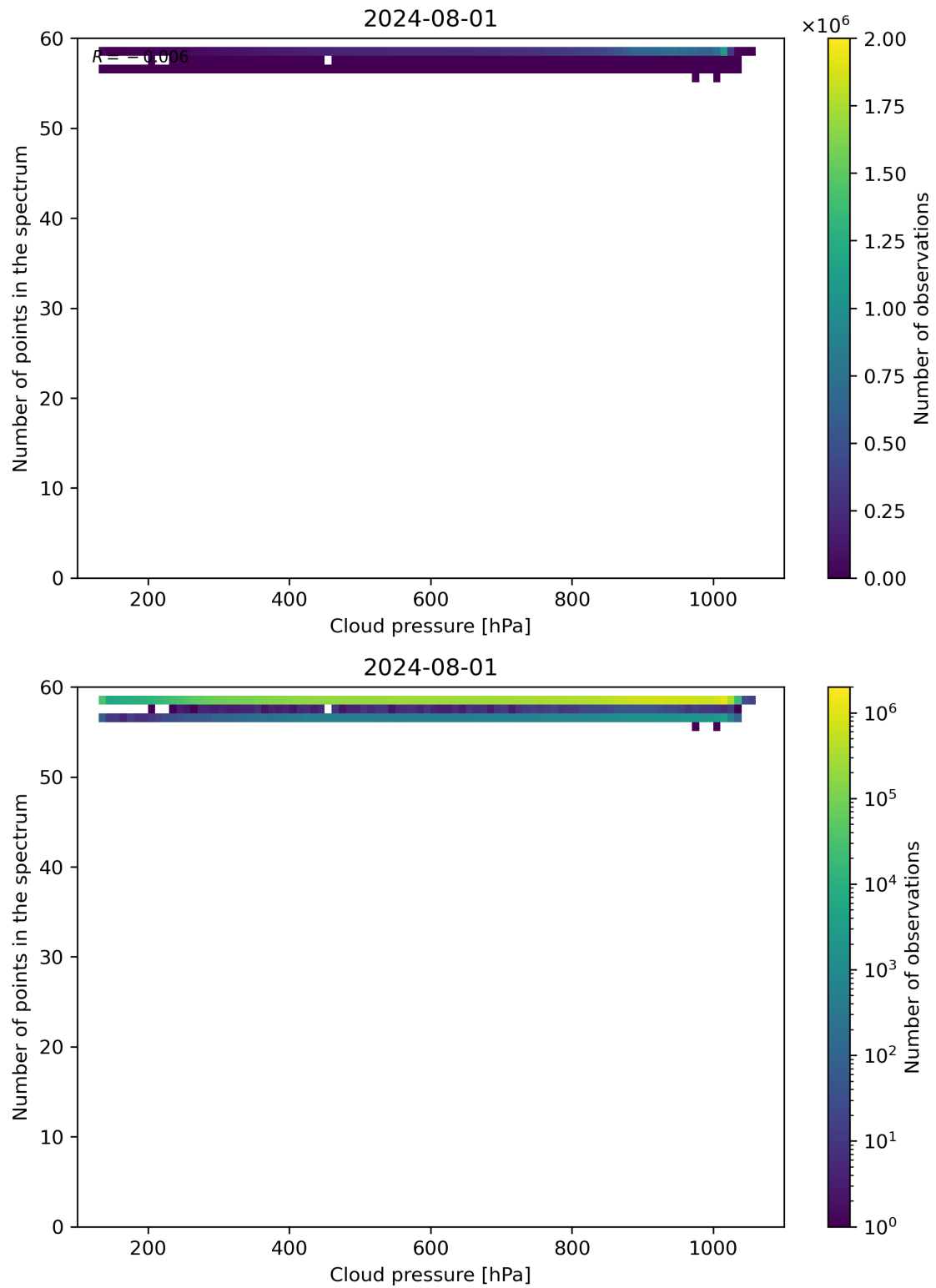
Figure 82: Scatter density plot of “Cloud pressure” against “Number of points in the spectrum” for 2024-07-31 to 2024-08-02.
