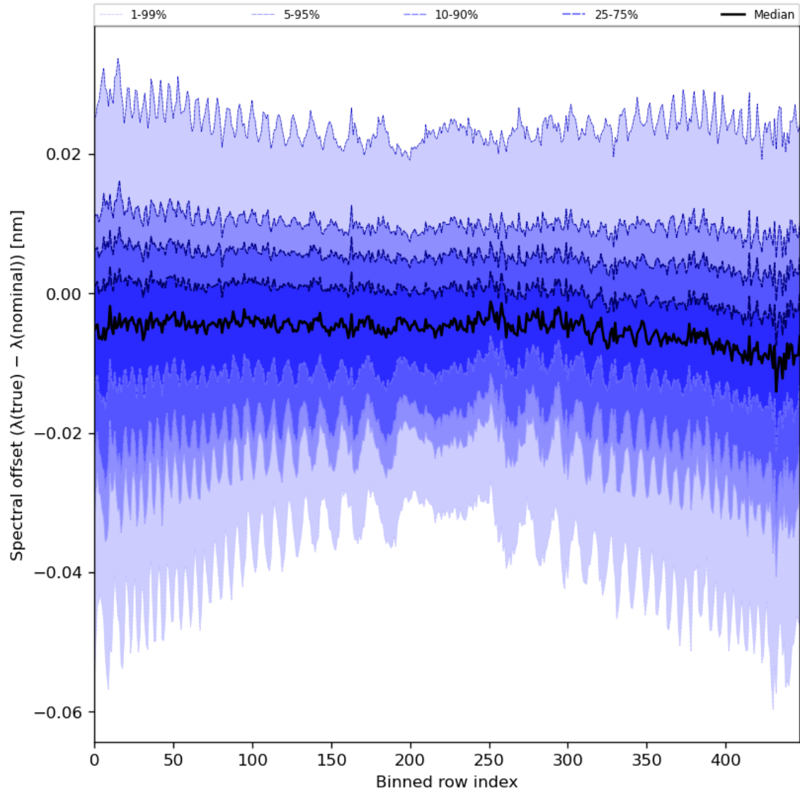
Figure 62: Along track statistics of “Spectral offset ( \lambda(\text{true}) - \lambda(\text{nominal}) )” for 2024-07-31 to 2024-08-02
