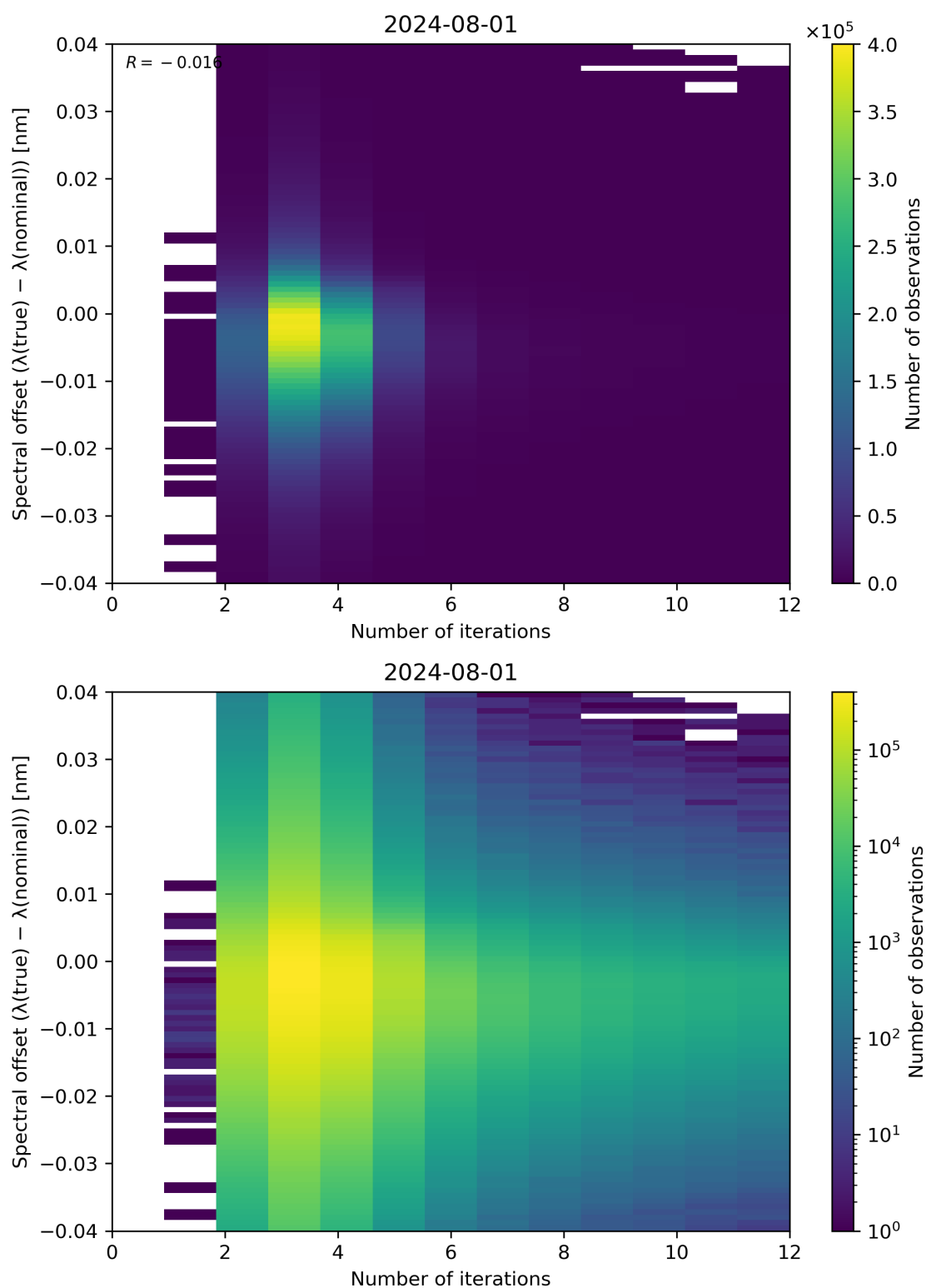
Figure 100: Scatter density plot of “Number of iterations” against “Spectral offset ( \lambda(\text{true}) - \lambda(\text{nominal}) )” for 2024-07-31 to 2024-08-02.
