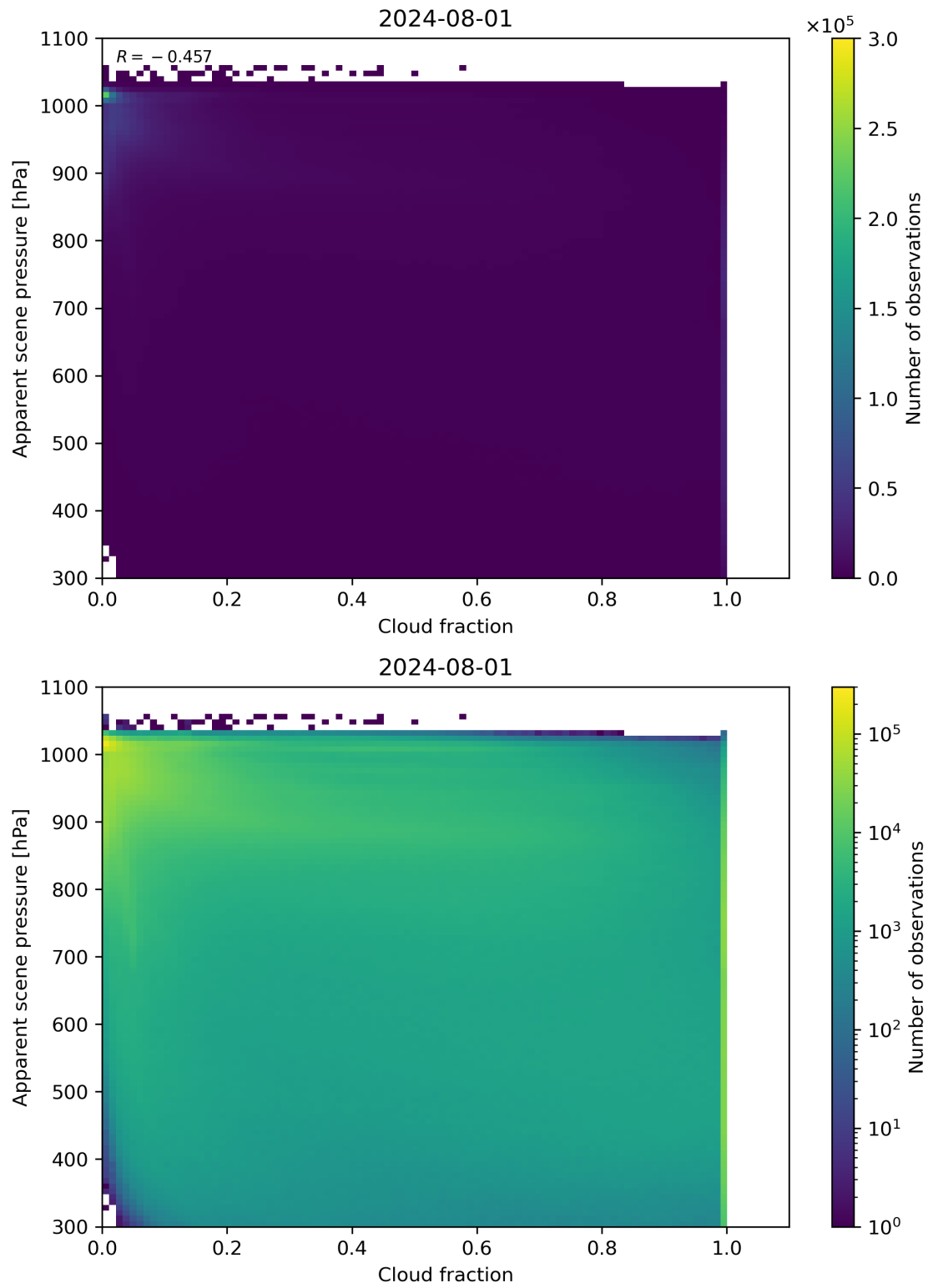
Figure 70: Scatter density plot of “Cloud fraction” against “Apparent scene pressure” for 2024-07-31 to 2024-08-02.
