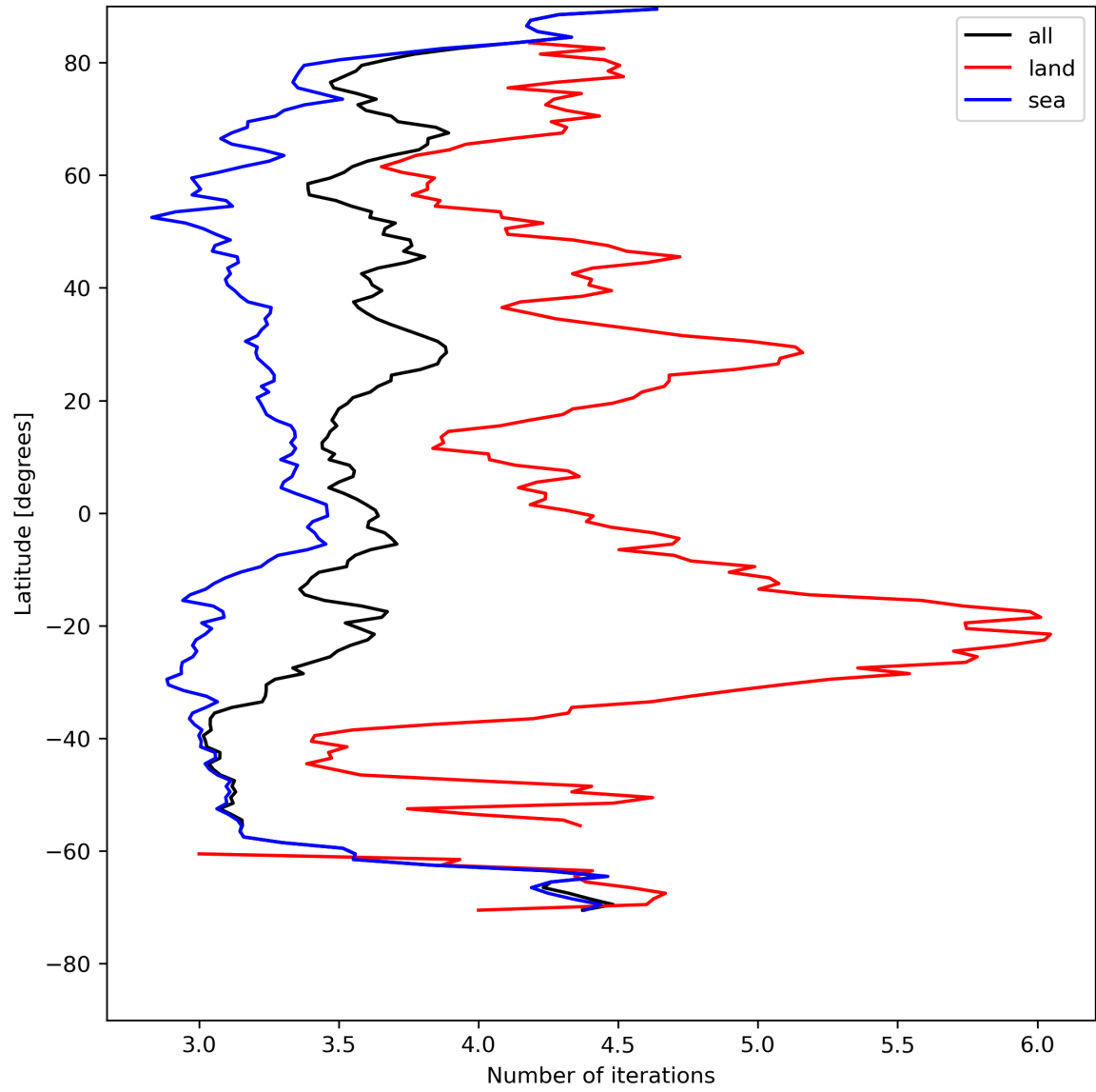
Figure 22: Zonal average of “Number of iterations” for 2024-07-31 to 2024-08-02.
