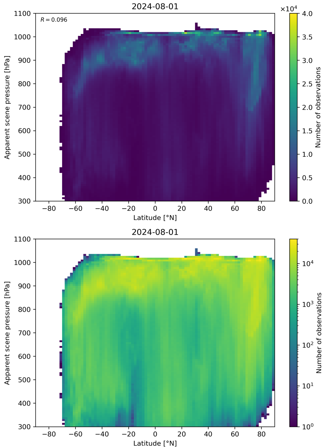
Figure 88: Scatter density plot of “Latitude” against “Apparent scene pressure” for 2024-07-31 to 2024-08-02.
