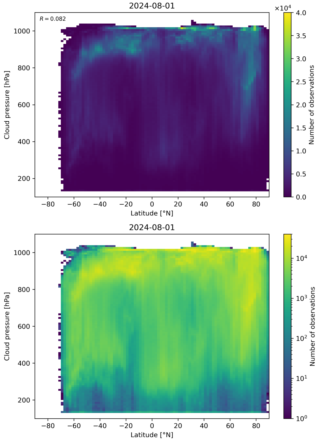
Figure 91: Scatter density plot of “Latitude” against “Cloud pressure” for 2024-07-31 to 2024-08-02.
