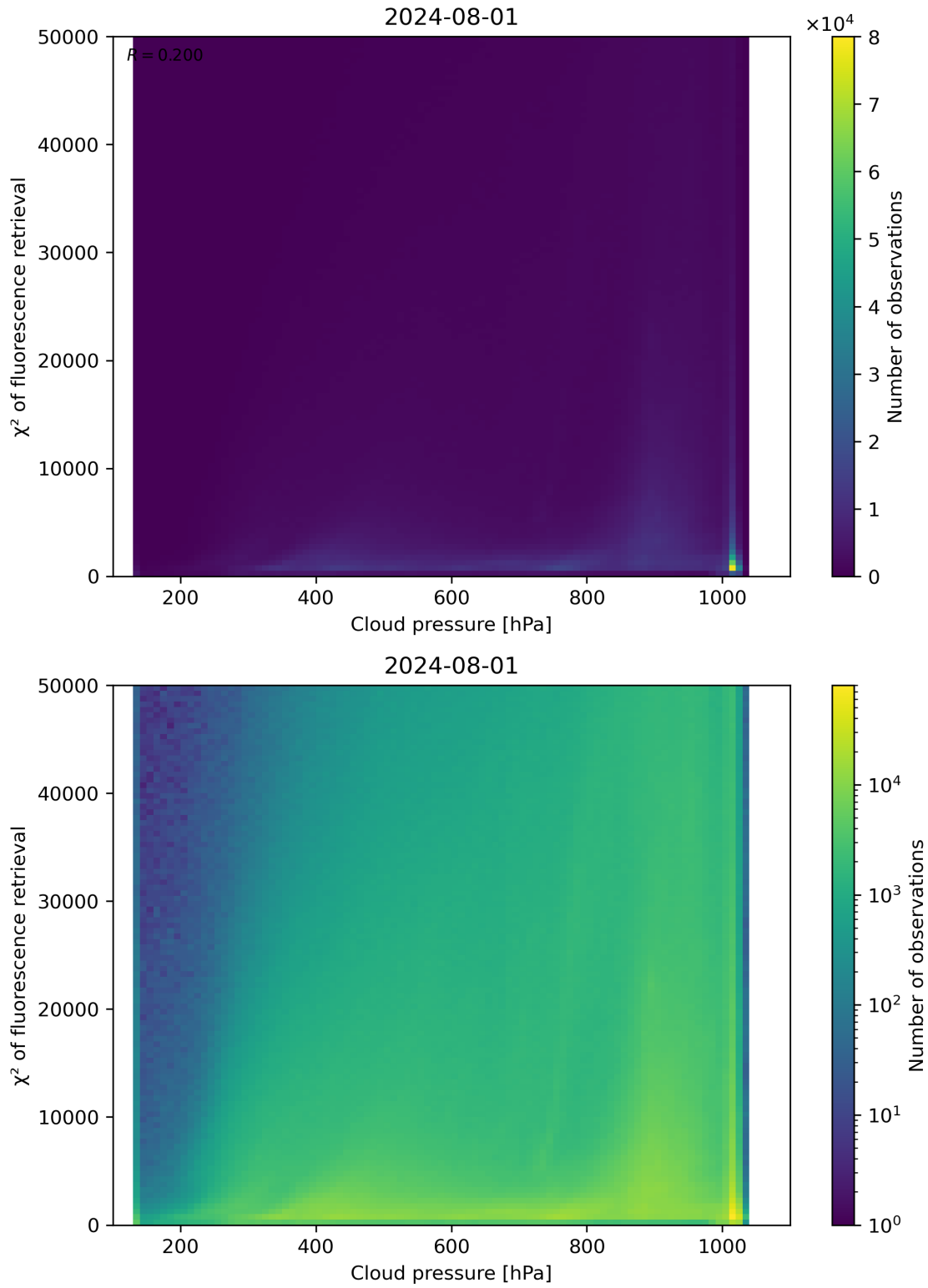
Figure 78: Scatter density plot of “Cloud pressure” against “ \chi^2 of fluorescence retrieval” for 2024-07-31 to 2024-08-02.
