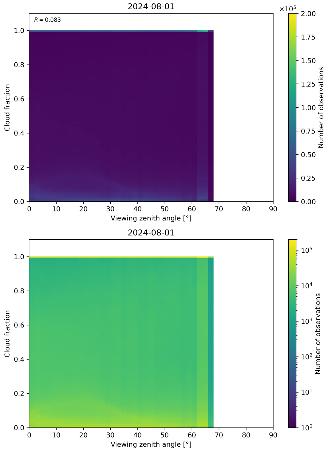
Figure 120: Scatter density plot of “Viewing zenith angle” against “Cloud fraction” for 2024-07-31 to 2024-08-02.
