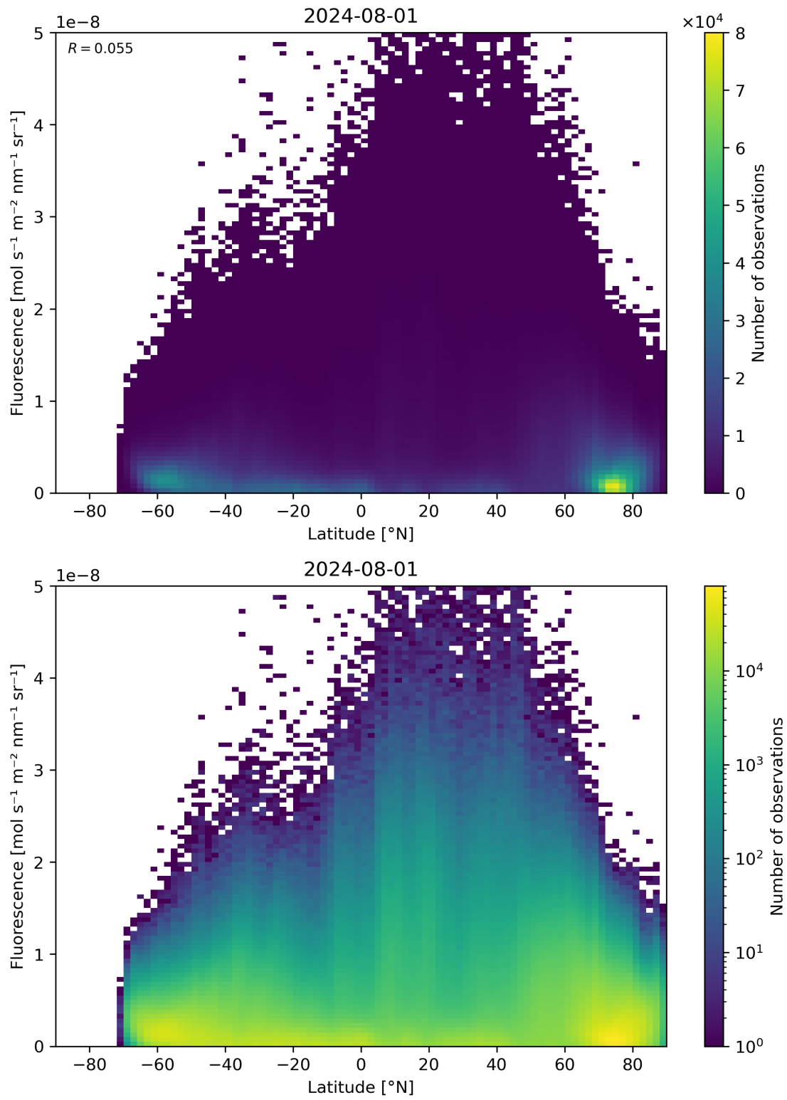
Figure 92: Scatter density plot of “Latitude” against “Fluorescence” for 2024-07-31 to 2024-08-02.
