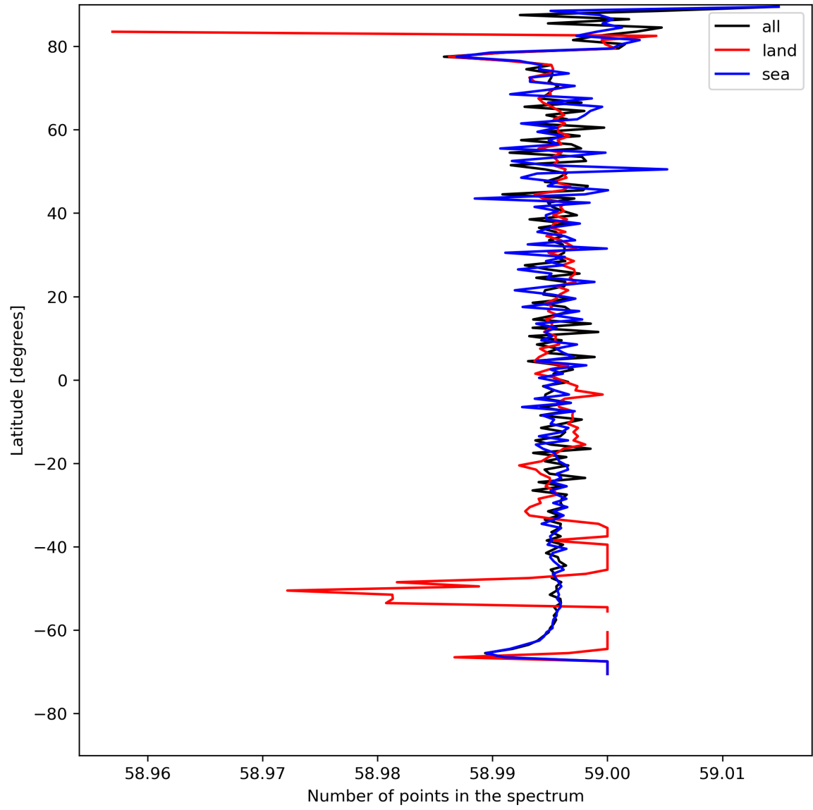
Figure 27: Zonal average of “Number of points in the spectrum” for 2024-07-31 to 2024-08-02.
