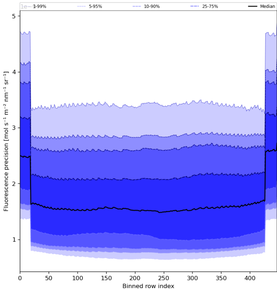
Figure 58: Along track statistics of “Fluorescence precision” for 2024-07-31 to 2024-08-02
