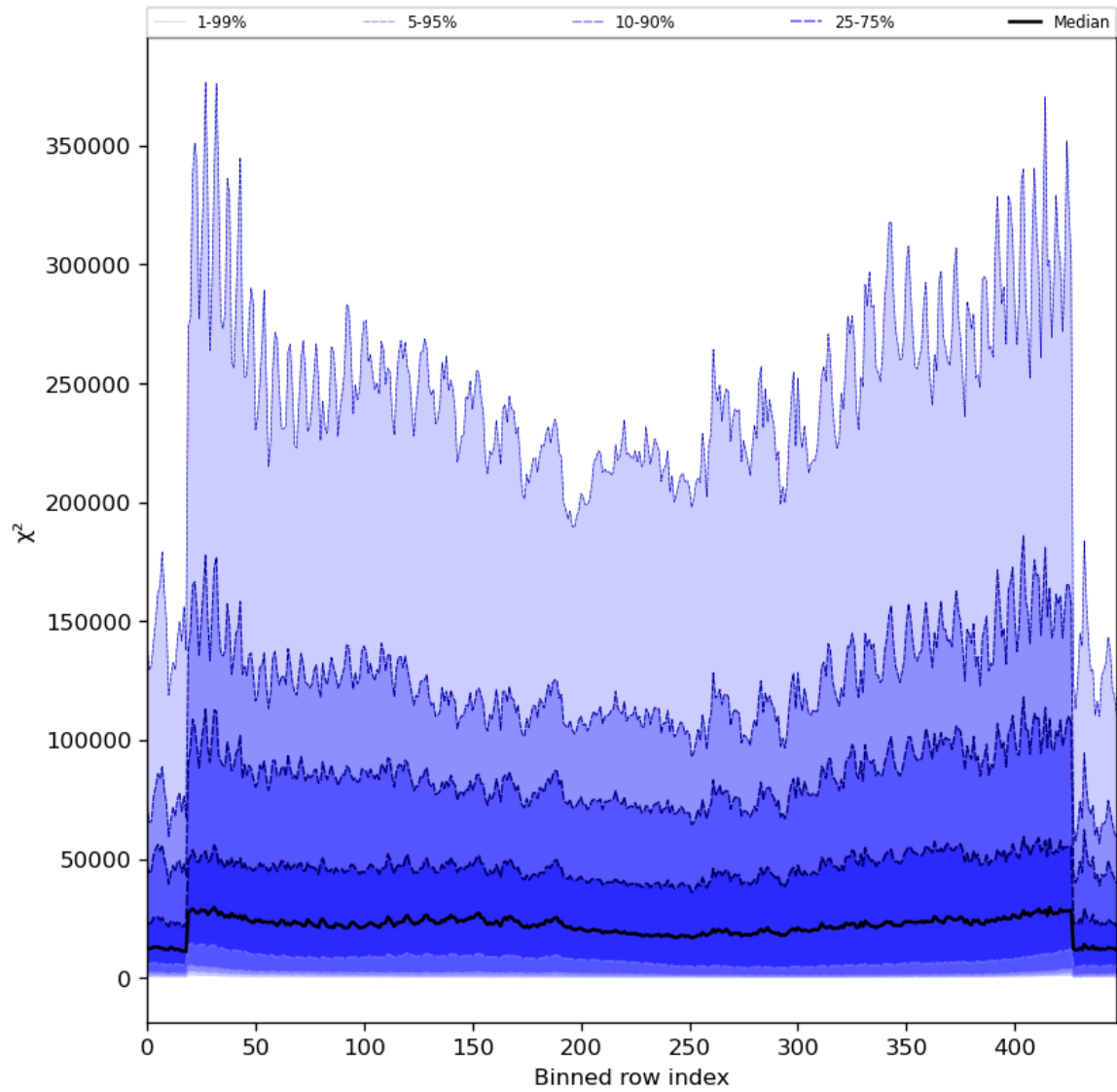
Figure 55: Along track statistics of “ \chi^2 ” for 2024-07-31 to 2024-08-02
