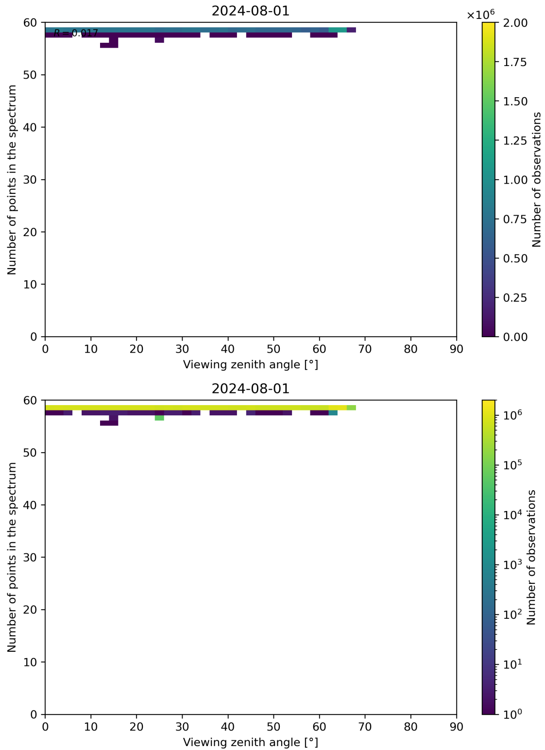
Figure 125: Scatter density plot of “Viewing zenith angle” against “Number of points in the spectrum” for 2024-07-31 to 2024-08-02.
