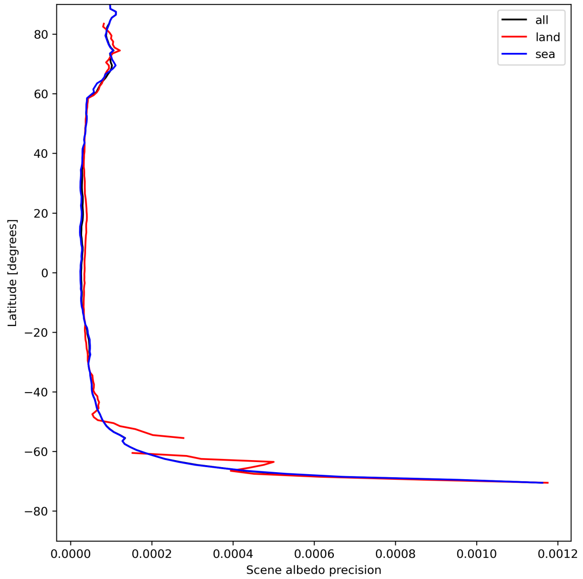
Figure 18: Zonal average of “Scene albedo precision” for 2024-07-31 to 2024-08-02.
