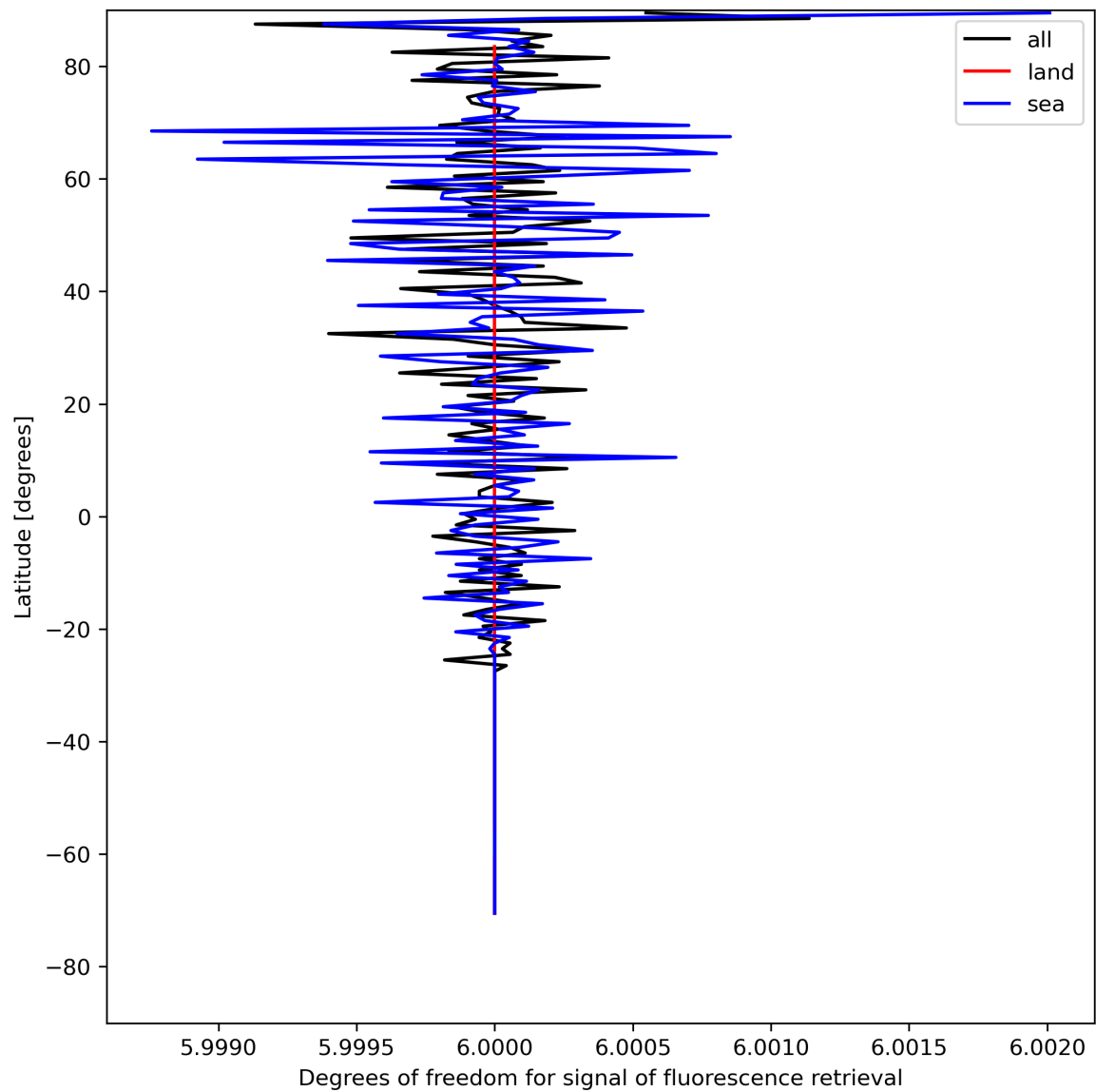
Figure 26: Zonal average of “Degrees of freedom for signal of fluorescence retrieval” for 2024-07-31 to 2024-08-02.
