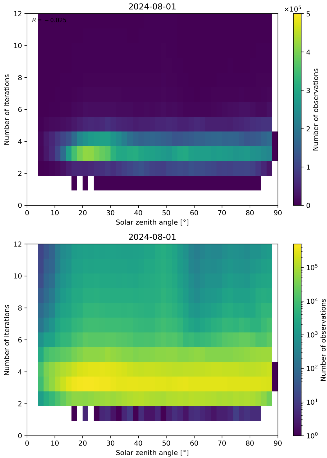
Figure 114: Scatter density plot of “Solar zenith angle” against “Number of iterations” for 2024-07-31 to 2024-08-02.
