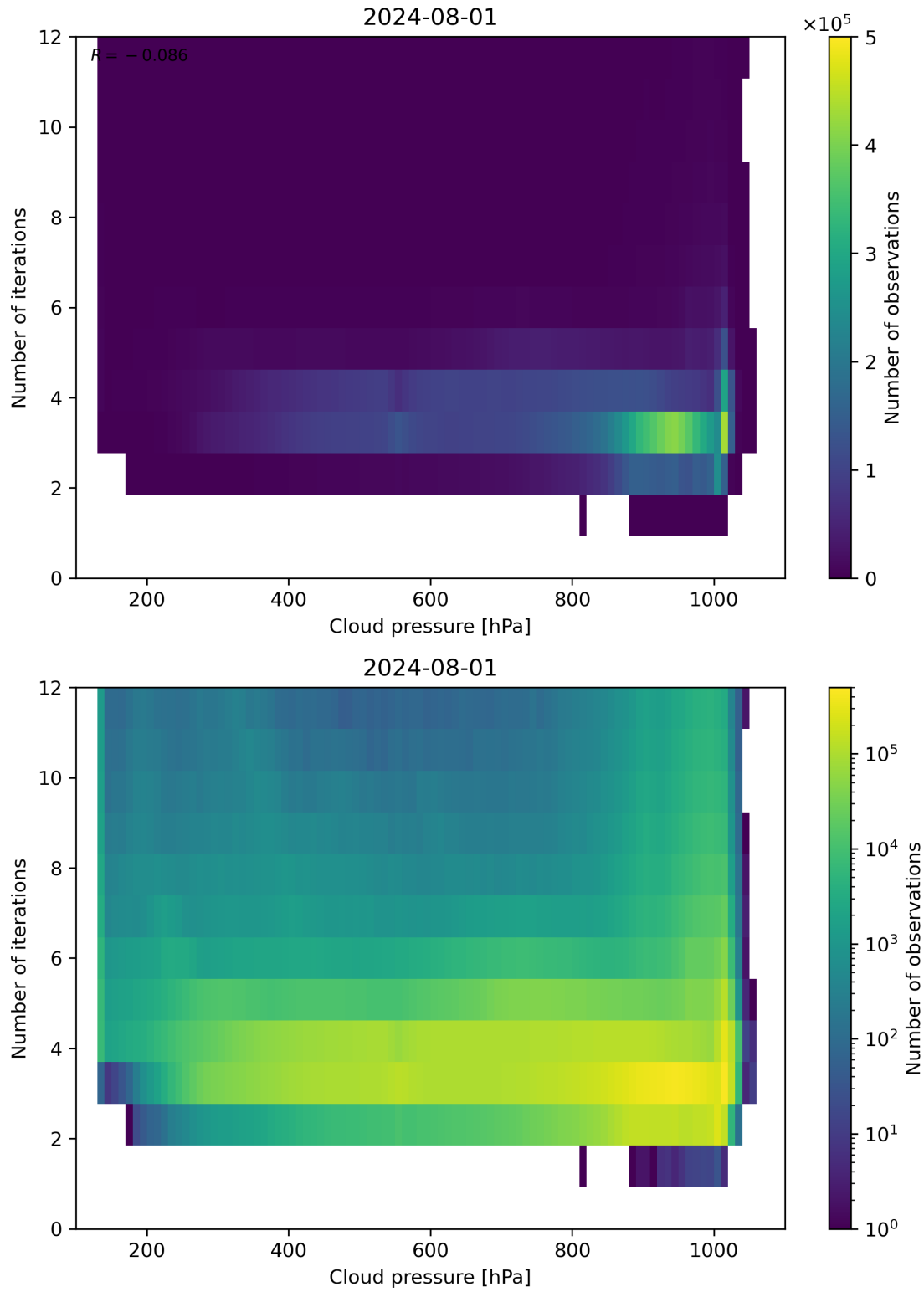
Figure 81: Scatter density plot of “Cloud pressure” against “Number of iterations” for 2024-07-31 to 2024-08-02.
