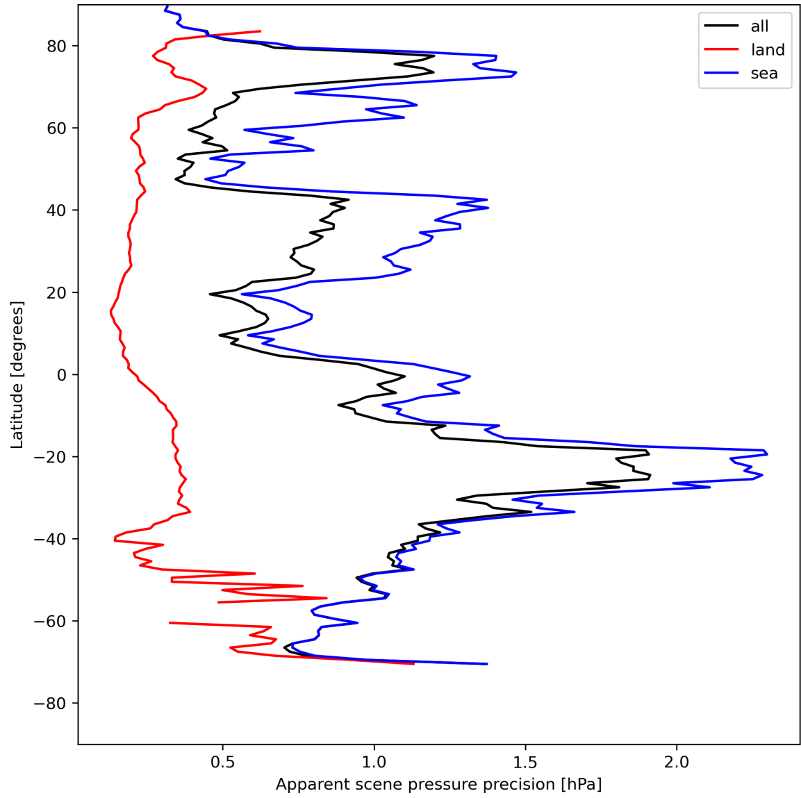
Figure 20: Zonal average of “Apparent scene pressure precision” for 2024-07-31 to 2024-08-02.
