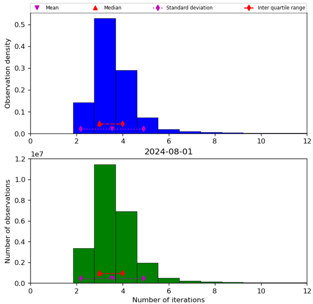
Figure 39: Histogram of “Number of iterations” for 2024-07-31 to 2024-08-02
