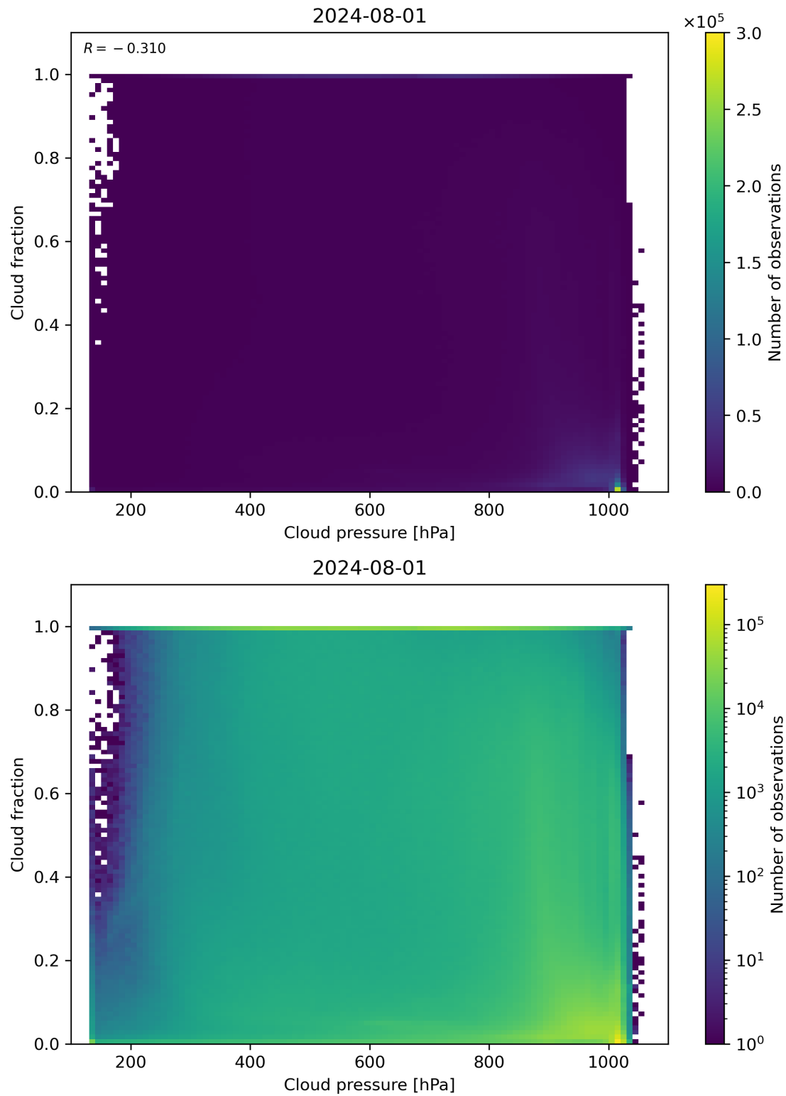
Figure 79: Scatter density plot of “Cloud pressure” against “Cloud fraction” for 2024-07-31 to 2024-08-02.
