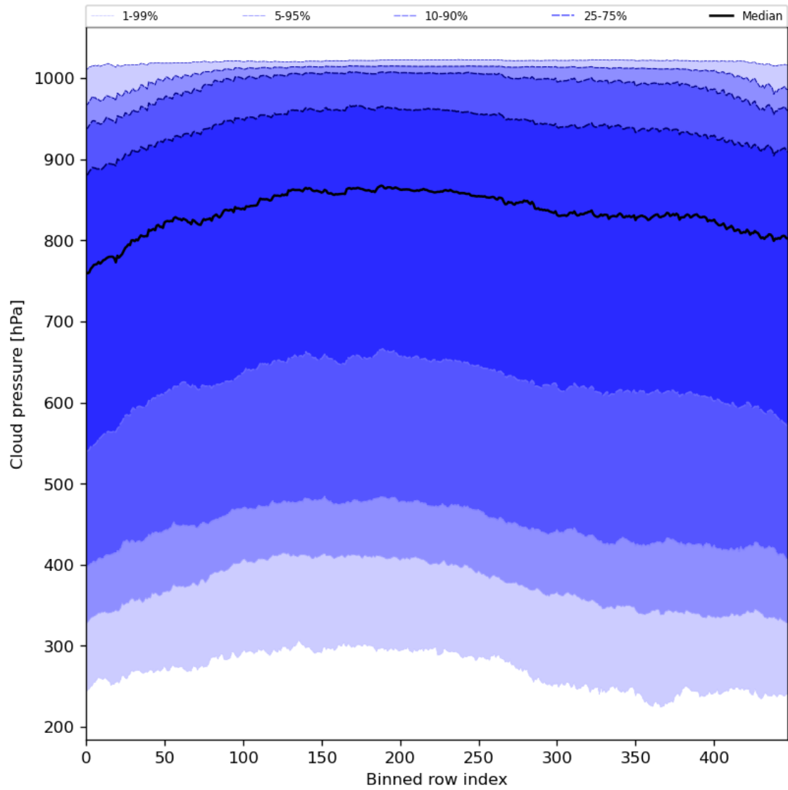
Figure 47: Along track statistics of “Cloud pressure” for 2024-07-31 to 2024-08-02
