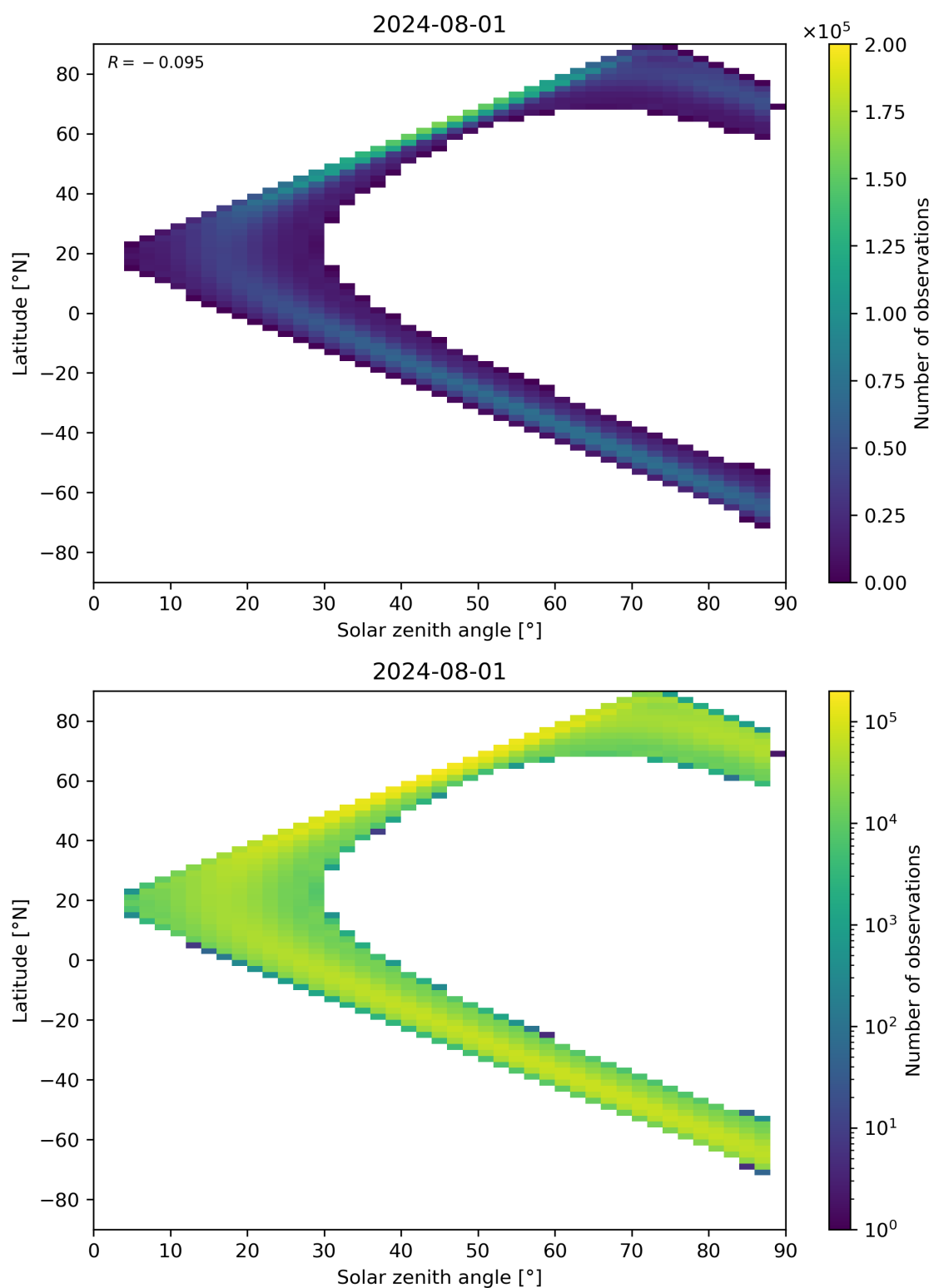
Figure 113: Scatter density plot of “Solar zenith angle” against “Latitude” for 2024-07-31 to 2024-08-02.
