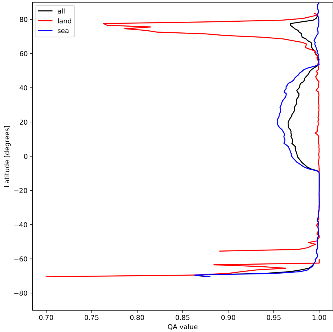
Figure 12: Zonal average of “QA value” for 2024-07-31 to 2024-08-02.
