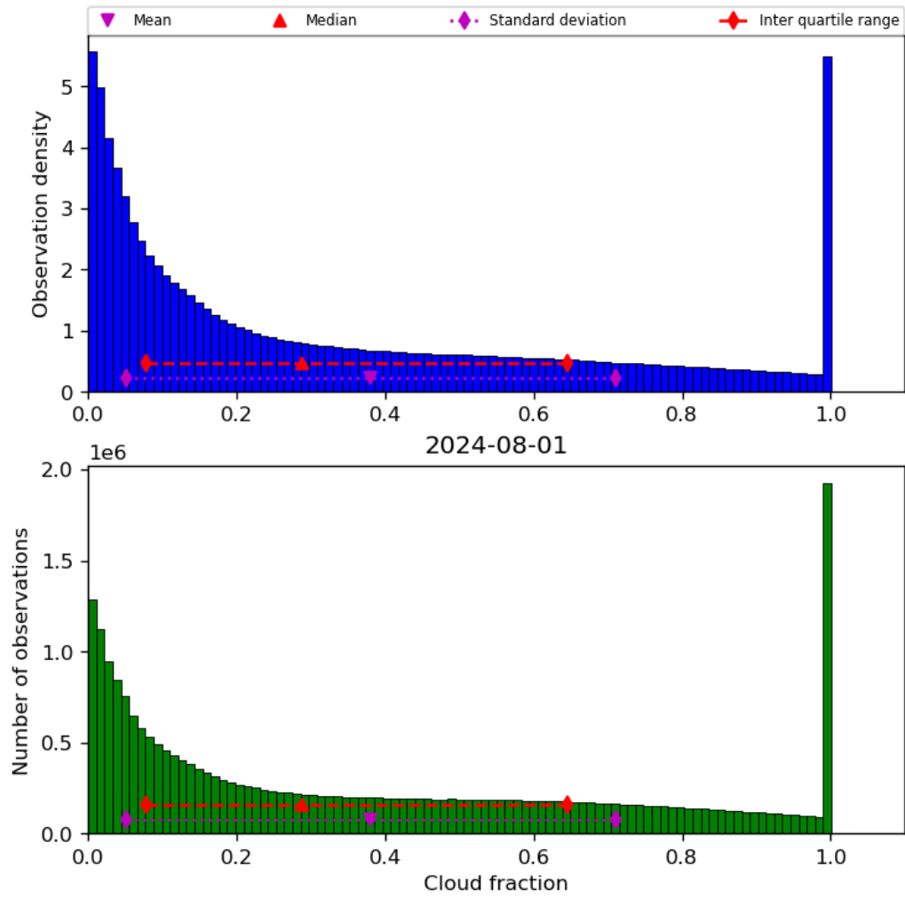
Figure 32: Histogram of “Cloud fraction” for 2024-07-31 to 2024-08-02
