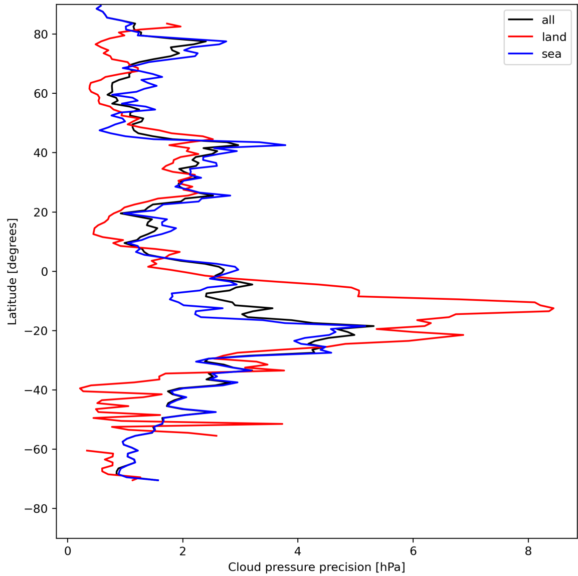
Figure 14: Zonal average of “Cloud pressure precision” for 2024-07-31 to 2024-08-02.
