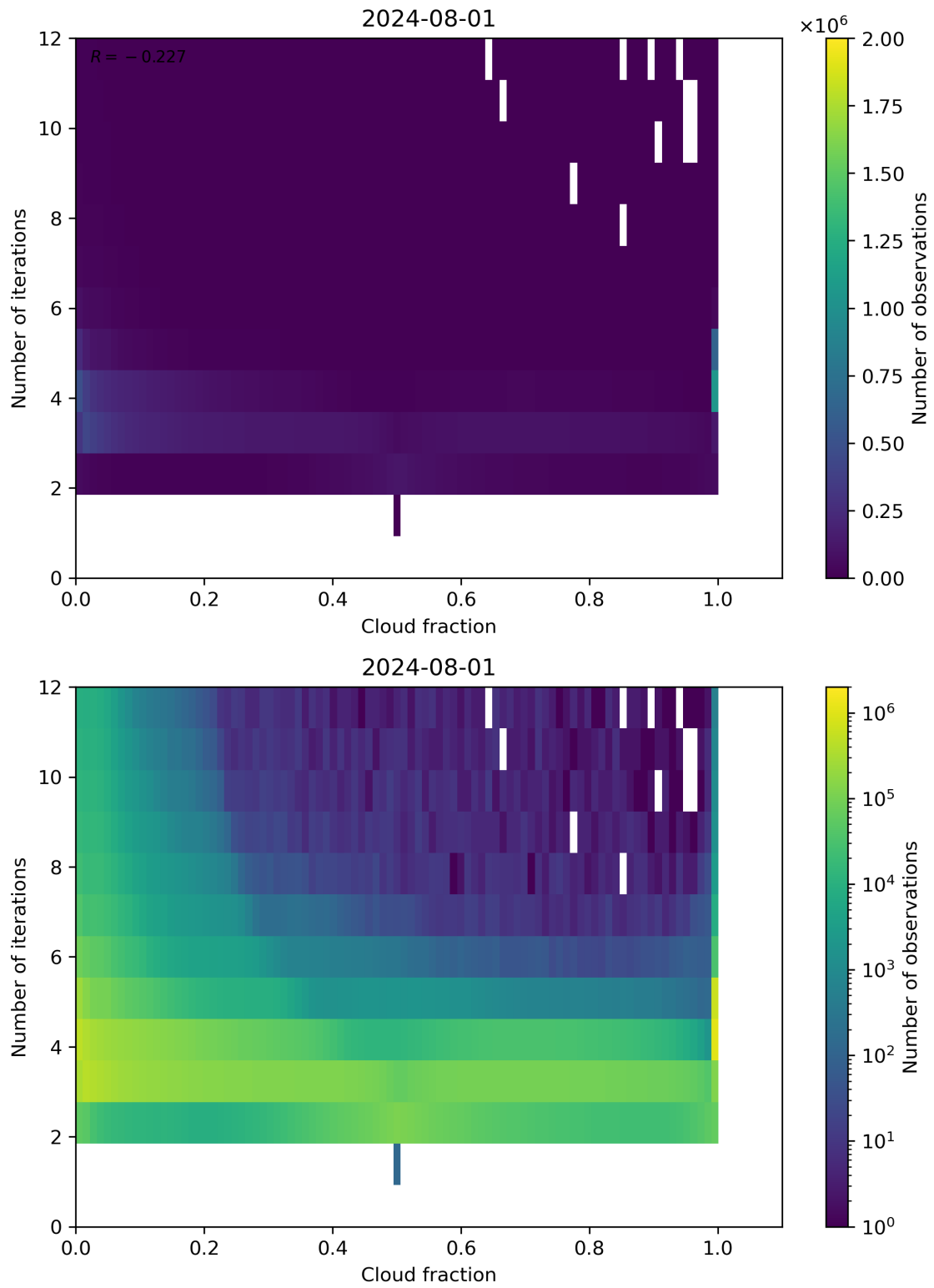
Figure 73: Scatter density plot of “Cloud fraction” against “Number of iterations” for 2024-07-31 to 2024-08-02.
