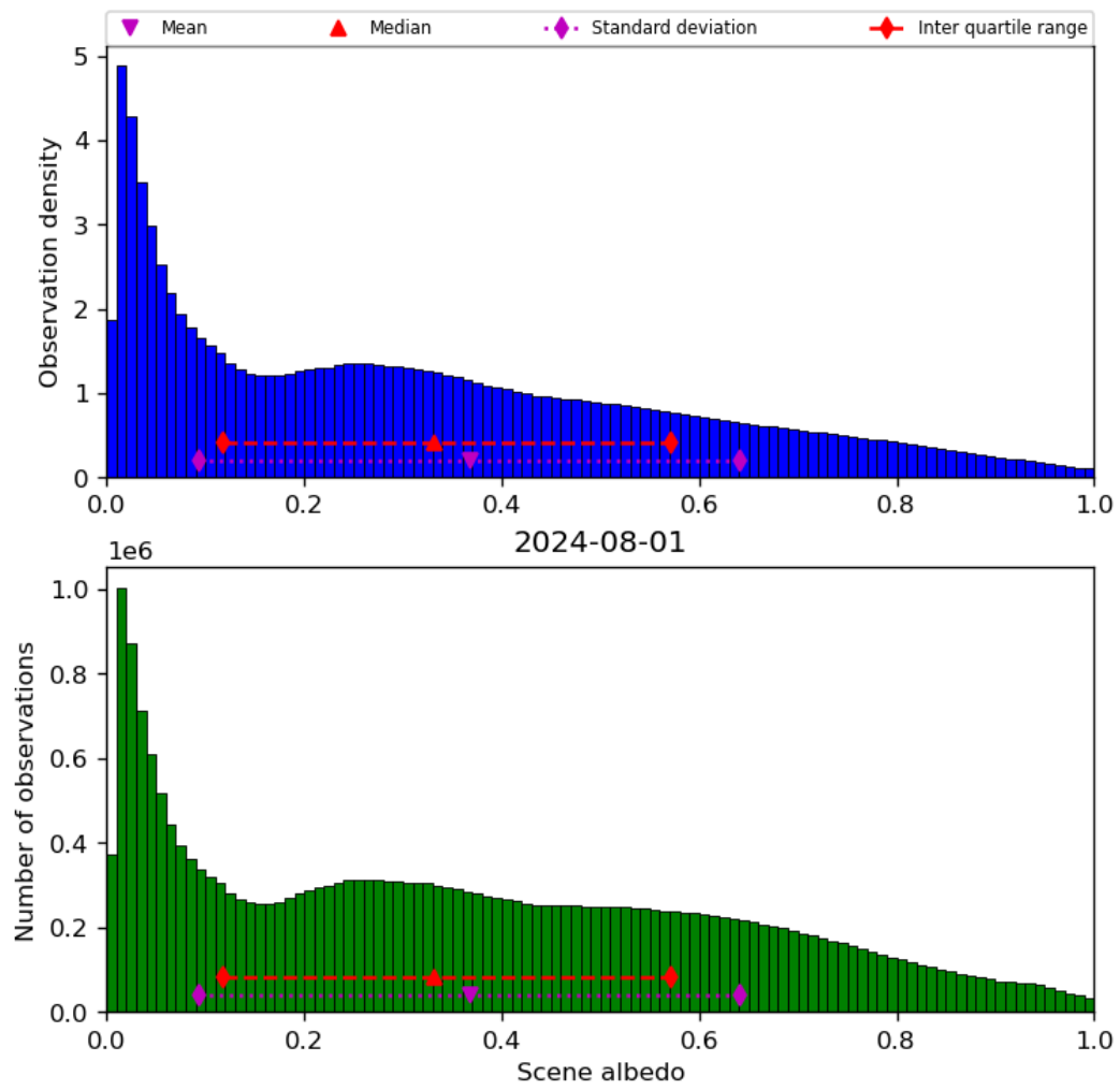
Figure 34: Histogram of “Scene albedo” for 2024-07-31 to 2024-08-02
