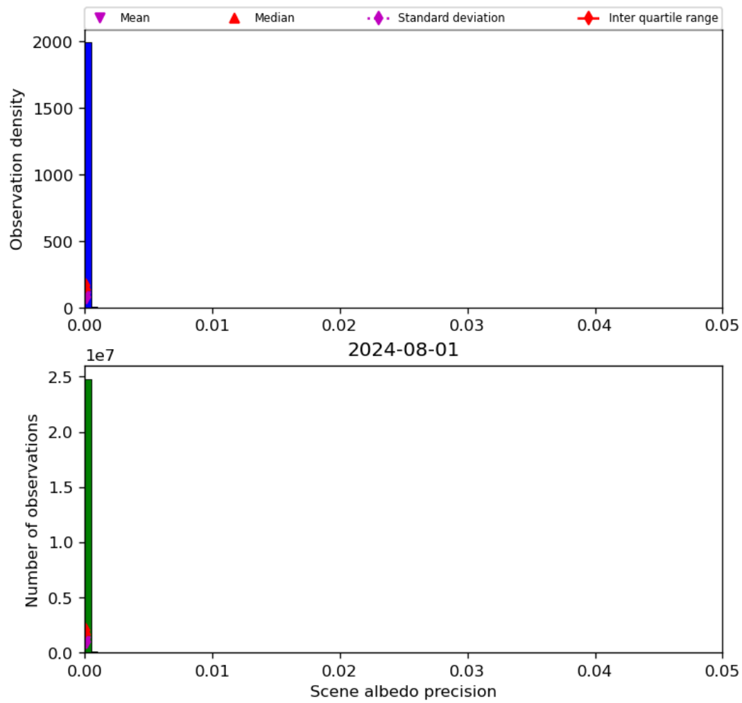
Figure 35: Histogram of “Scene albedo precision” for 2024-07-31 to 2024-08-02
