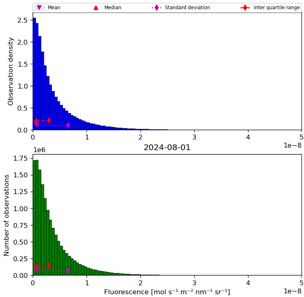
Figure 40: Histogram of “Fluorescence” for 2024-07-31 to 2024-08-02
