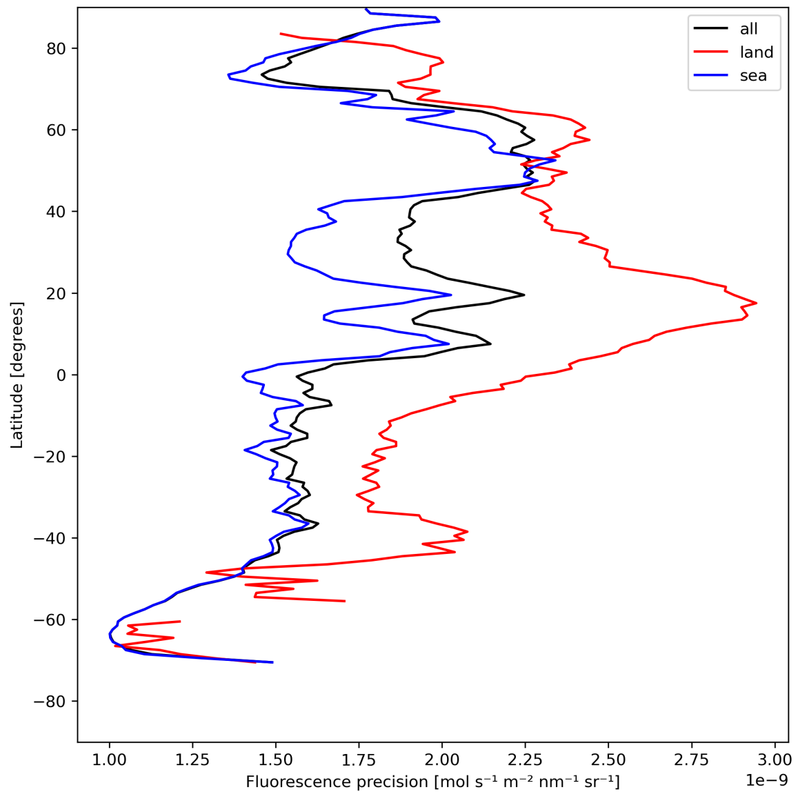
Figure 24: Zonal average of “Fluorescence precision” for 2024-07-31 to 2024-08-02.
