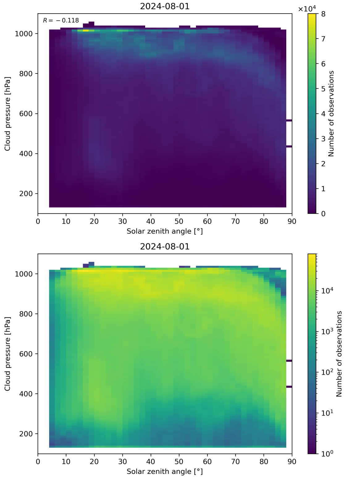
Figure 111: Scatter density plot of “Solar zenith angle” against “Cloud pressure” for 2024-07-31 to 2024-08-02.
