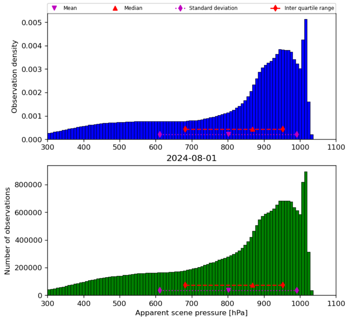
Figure 36: Histogram of “Apparent scene pressure” for 2024-07-31 to 2024-08-02
