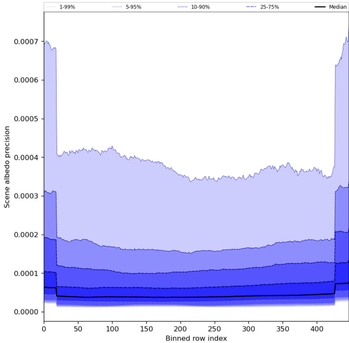
Figure 52: Along track statistics of “Scene albedo precision” for 2024-07-31 to 2024-08-02
