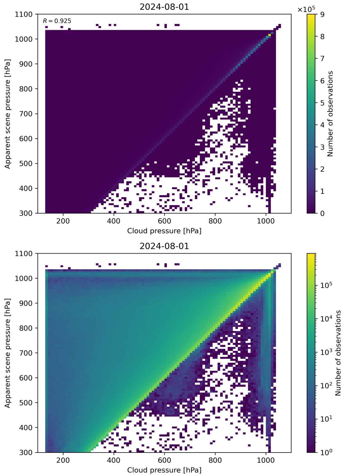
Figure 77: Scatter density plot of “Cloud pressure” against “Apparent scene pressure” for 2024-07-31 to 2024-08-02.
