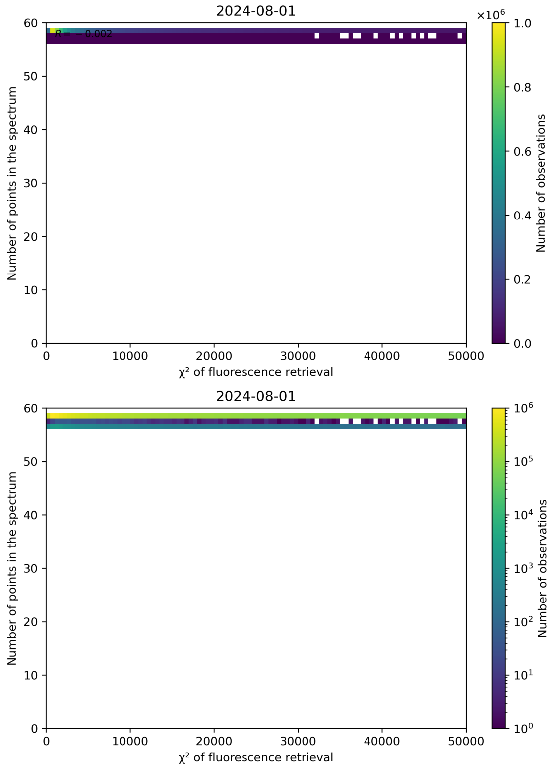
Figure 68: Scatter density plot of “ \chi^2 of fluorescence retrieval” against “Number of points in the spectrum” for 2024-07-31 to 2024-08-02.
