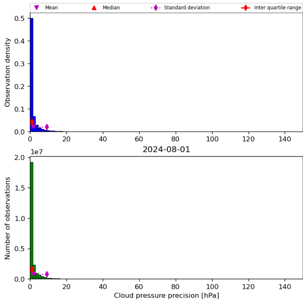
Figure 31: Histogram of “Cloud pressure precision” for 2024-07-31 to 2024-08-02
