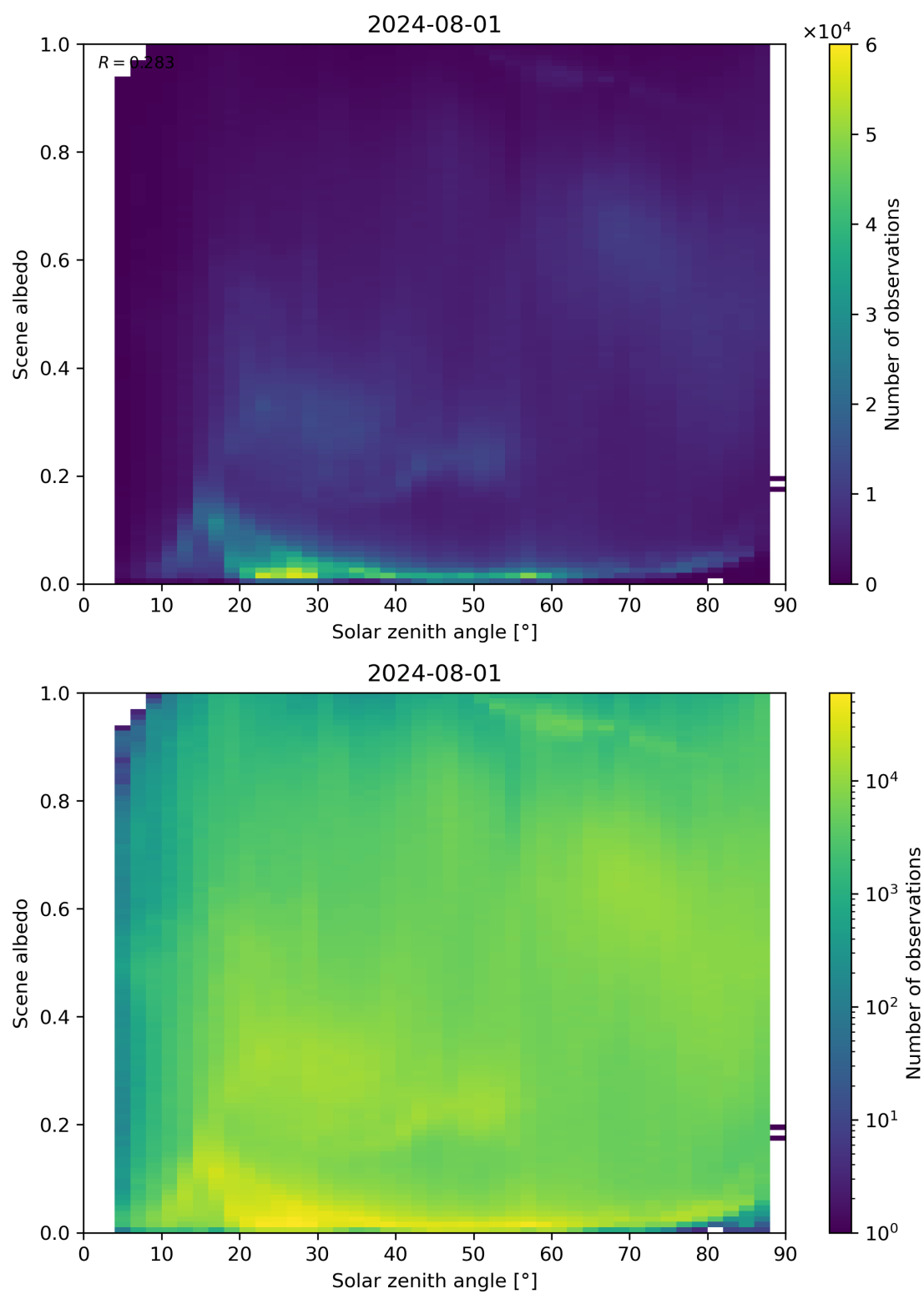
Figure 116: Scatter density plot of “Solar zenith angle” against “Scene albedo” for 2024-07-31 to 2024-08-02.
