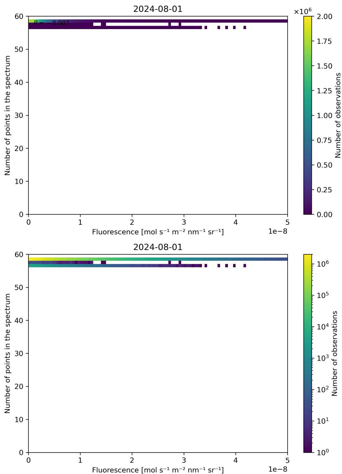
Figure 86: Scatter density plot of “Fluorescence” against “Number of points in the spectrum” for 2024-07-31 to 2024-08-02.
