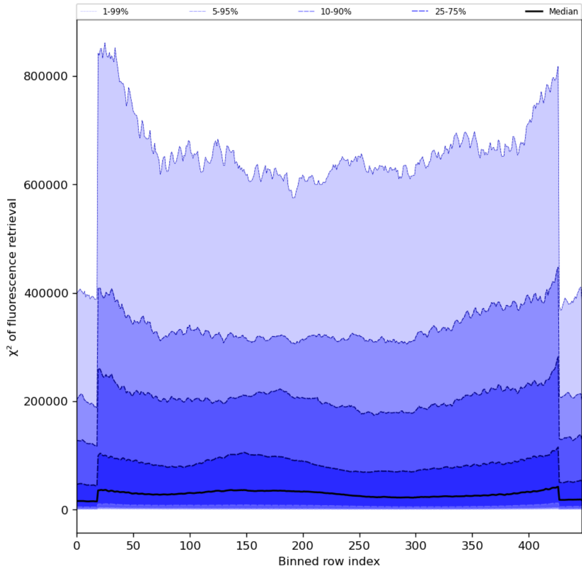
Figure 59: Along track statistics of “ \chi^2 of fluorescence retrieval” for 2024-07-31 to 2024-08-02
