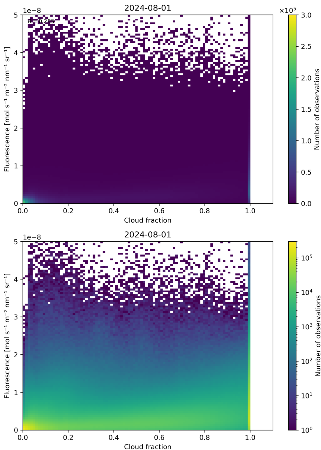
Figure 72: Scatter density plot of “Cloud fraction” against “Fluorescence” for 2024-07-31 to 2024-08-02.
