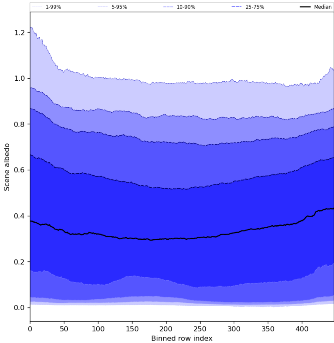
Figure 51: Along track statistics of “Scene albedo” for 2024-07-31 to 2024-08-02
