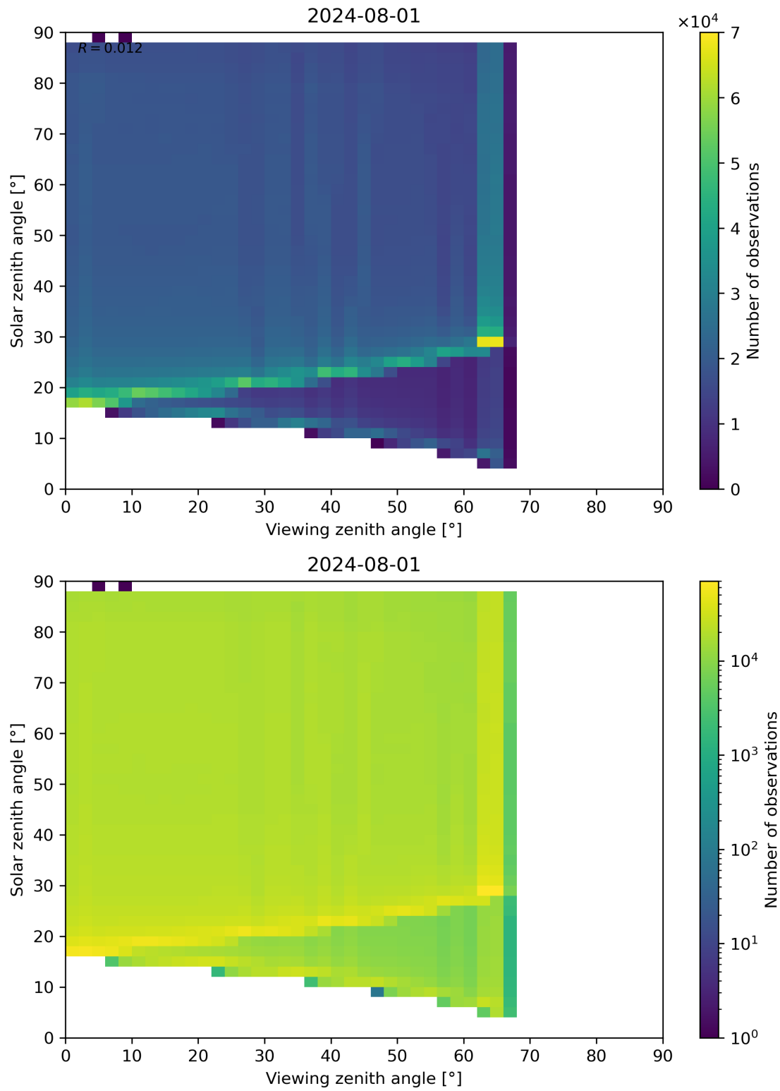
Figure 127: Scatter density plot of “Viewing zenith angle” against “Solar zenith angle” for 2024-07-31 to 2024-08-02.
