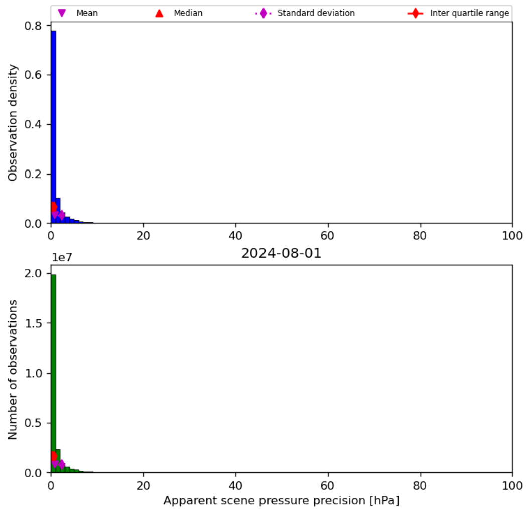
Figure 37: Histogram of “Apparent scene pressure precision” for 2024-07-31 to 2024-08-02
