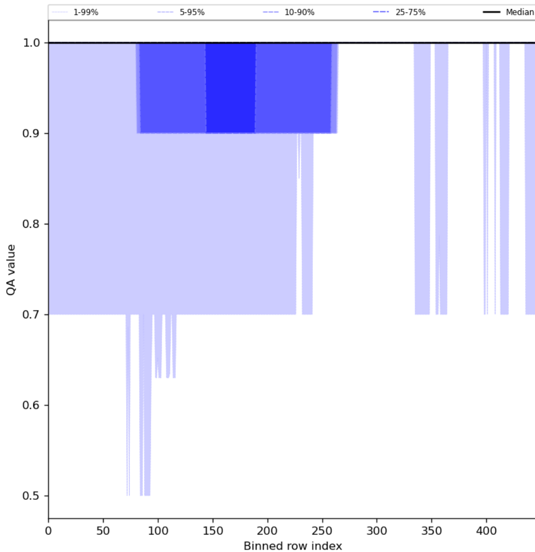
Figure 46: Along track statistics of “QA value” for 2024-07-31 to 2024-08-02
