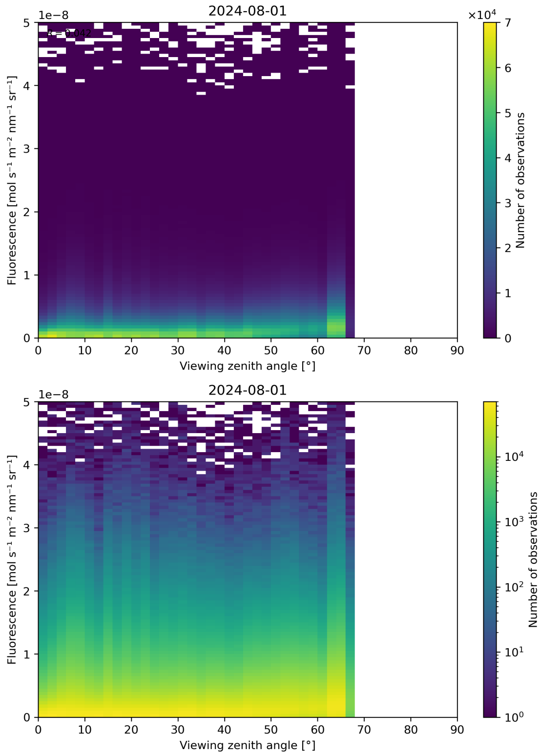
Figure 122: Scatter density plot of “Viewing zenith angle” against “Fluorescence” for 2024-07-31 to 2024-08-02.
