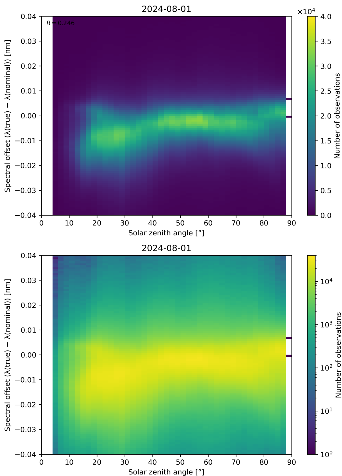
Figure 117: Scatter density plot of “Solar zenith angle” against “Spectral offset ( \lambda(\text{true}) - \lambda(\text{nominal}) )” for 2024-07-31 to 2024-08-02.
