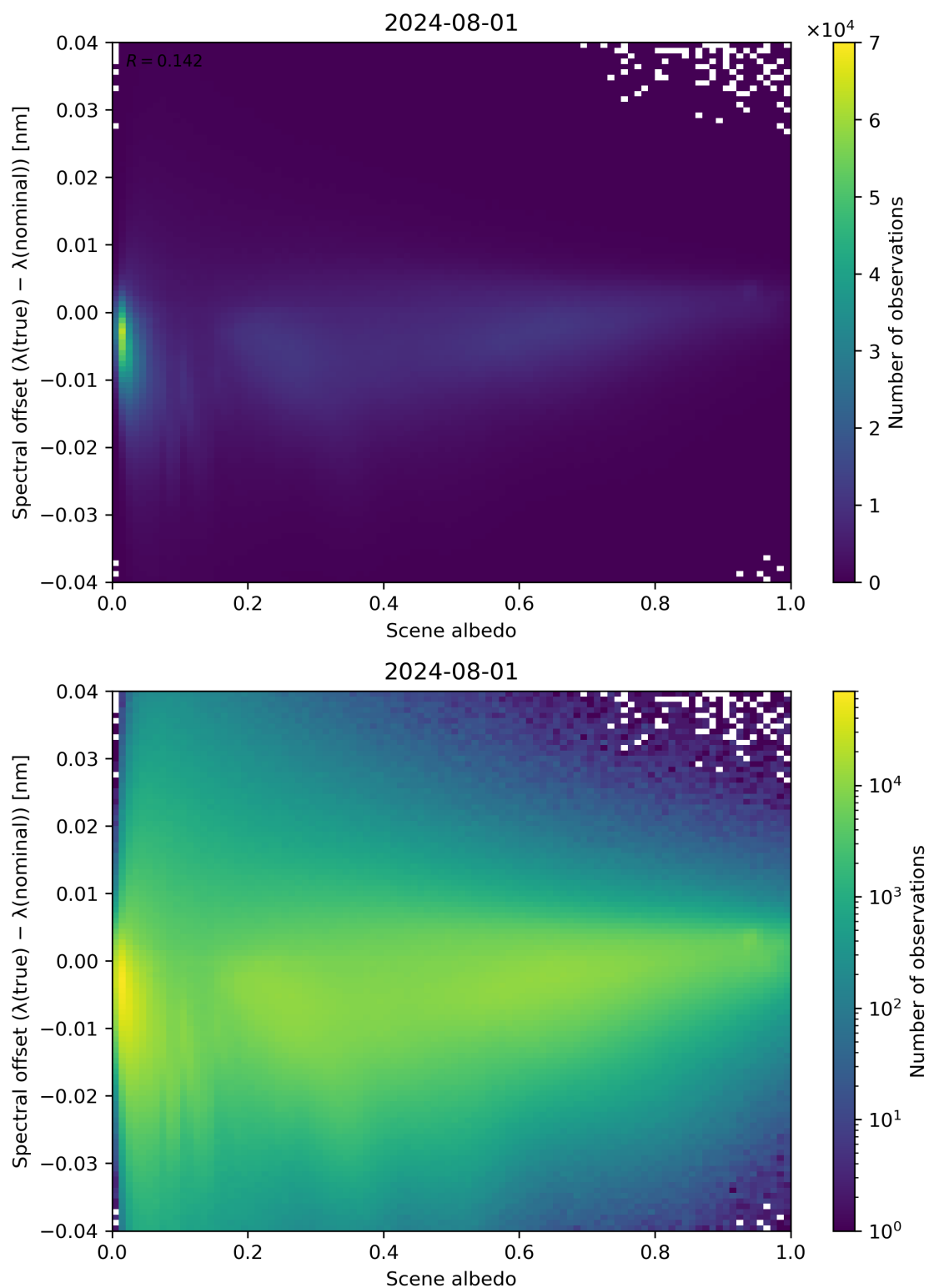
Figure 107: Scatter density plot of “Scene albedo” against “Spectral offset ( \lambda(\text{true}) - \lambda(\text{nominal}) )” for 2024-07-31 to 2024-08-02.
