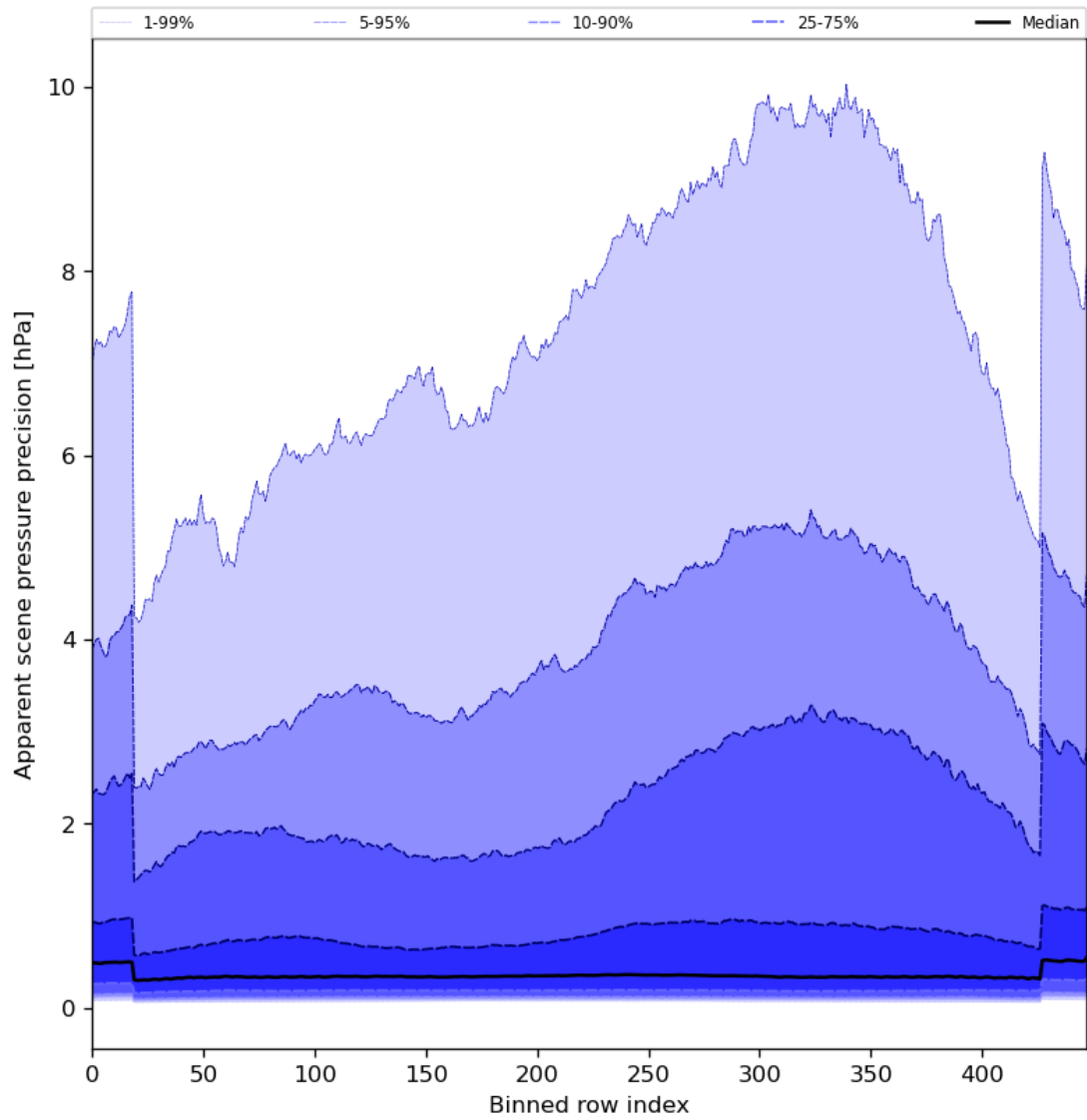
Figure 54: Along track statistics of “Apparent scene pressure precision” for 2024-07-31 to 2024-08-02
