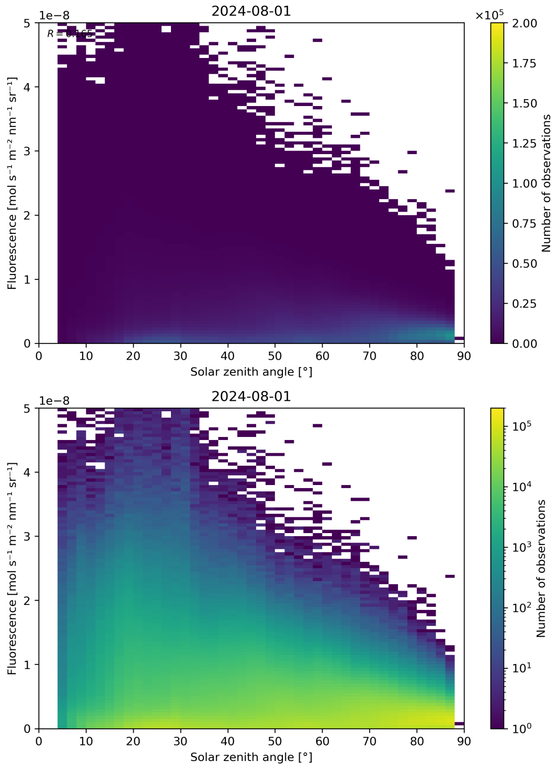
Figure 112: Scatter density plot of “Solar zenith angle” against “Fluorescence” for 2024-07-31 to 2024-08-02.
