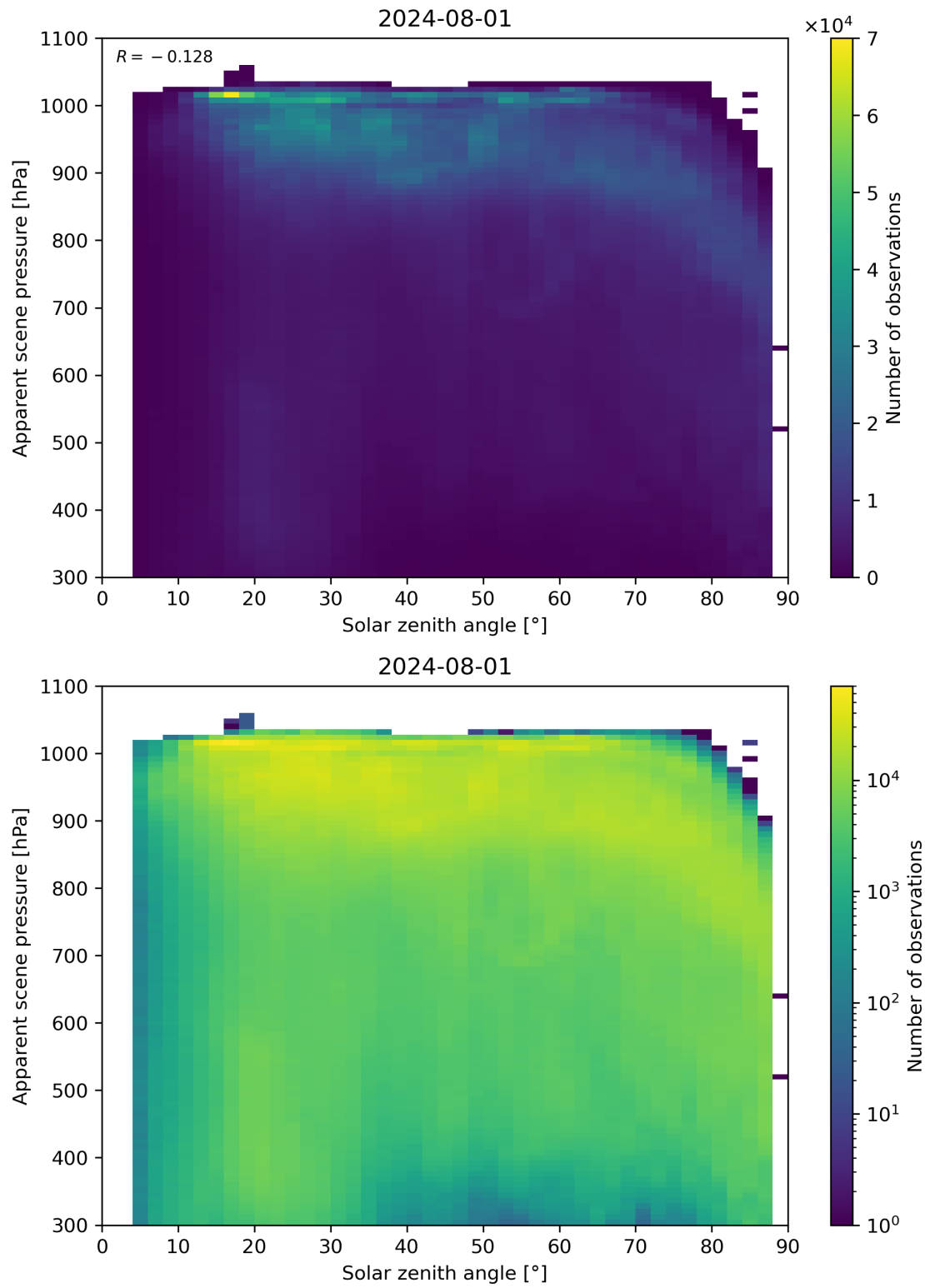
Figure 108: Scatter density plot of “Solar zenith angle” against “Apparent scene pressure” for 2024-07-31 to 2024-08-02.
