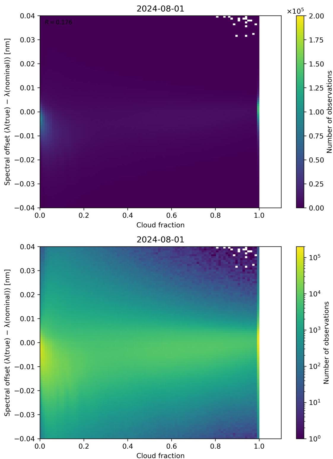
Figure 76: Scatter density plot of “Cloud fraction” against “Spectral offset ( \lambda(\text{true}) - \lambda(\text{nominal}) )” for 2024-07-31 to 2024-08-02.
