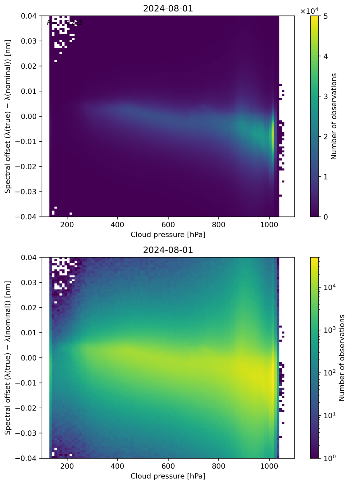
Figure 84: Scatter density plot of “Cloud pressure” against “Spectral offset ( \lambda(\text{true}) - \lambda(\text{nominal}) )” for 2024-07-31 to 2024-08-02.
