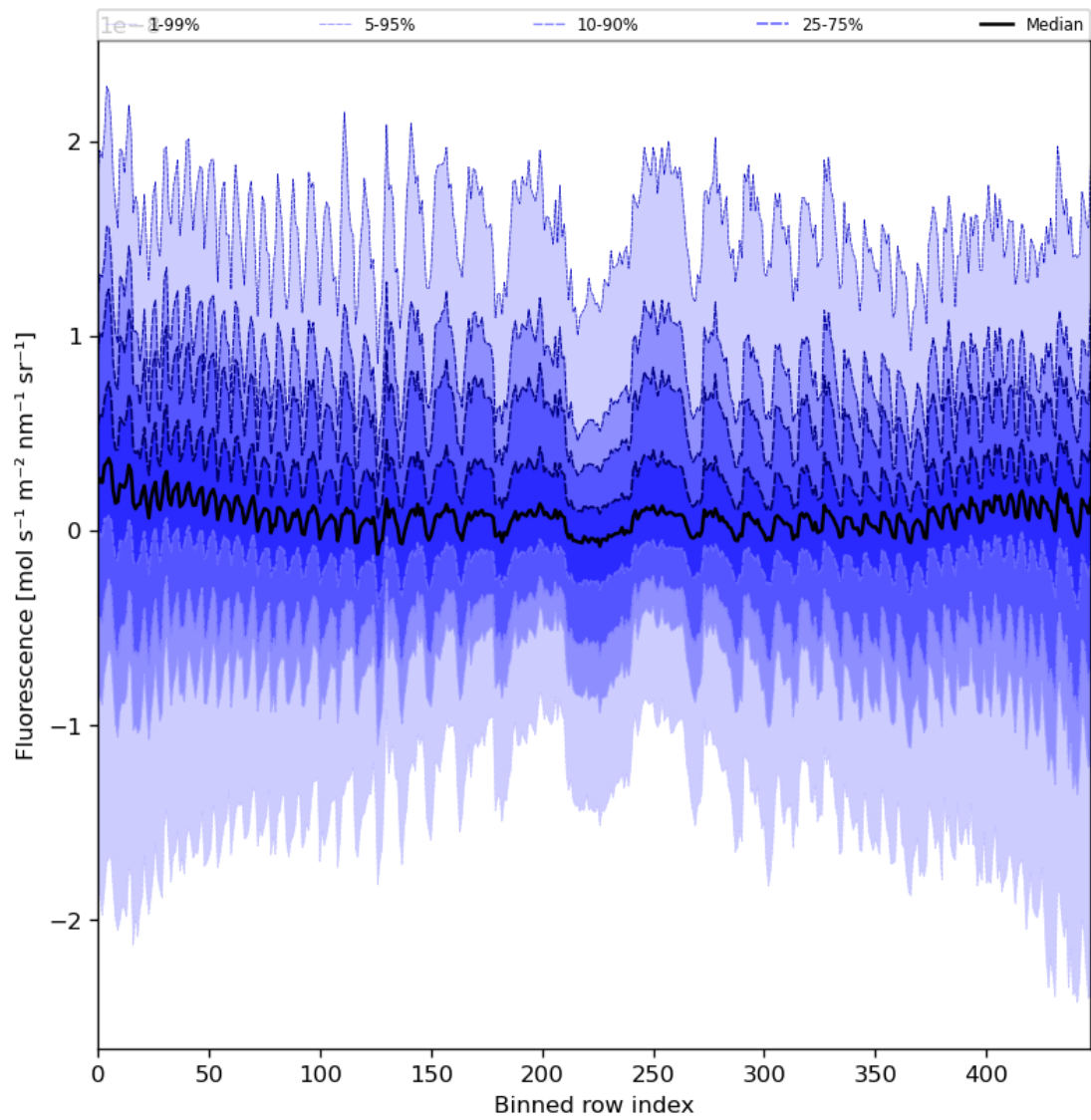
Figure 57: Along track statistics of “Fluorescence” for 2024-07-31 to 2024-08-02
