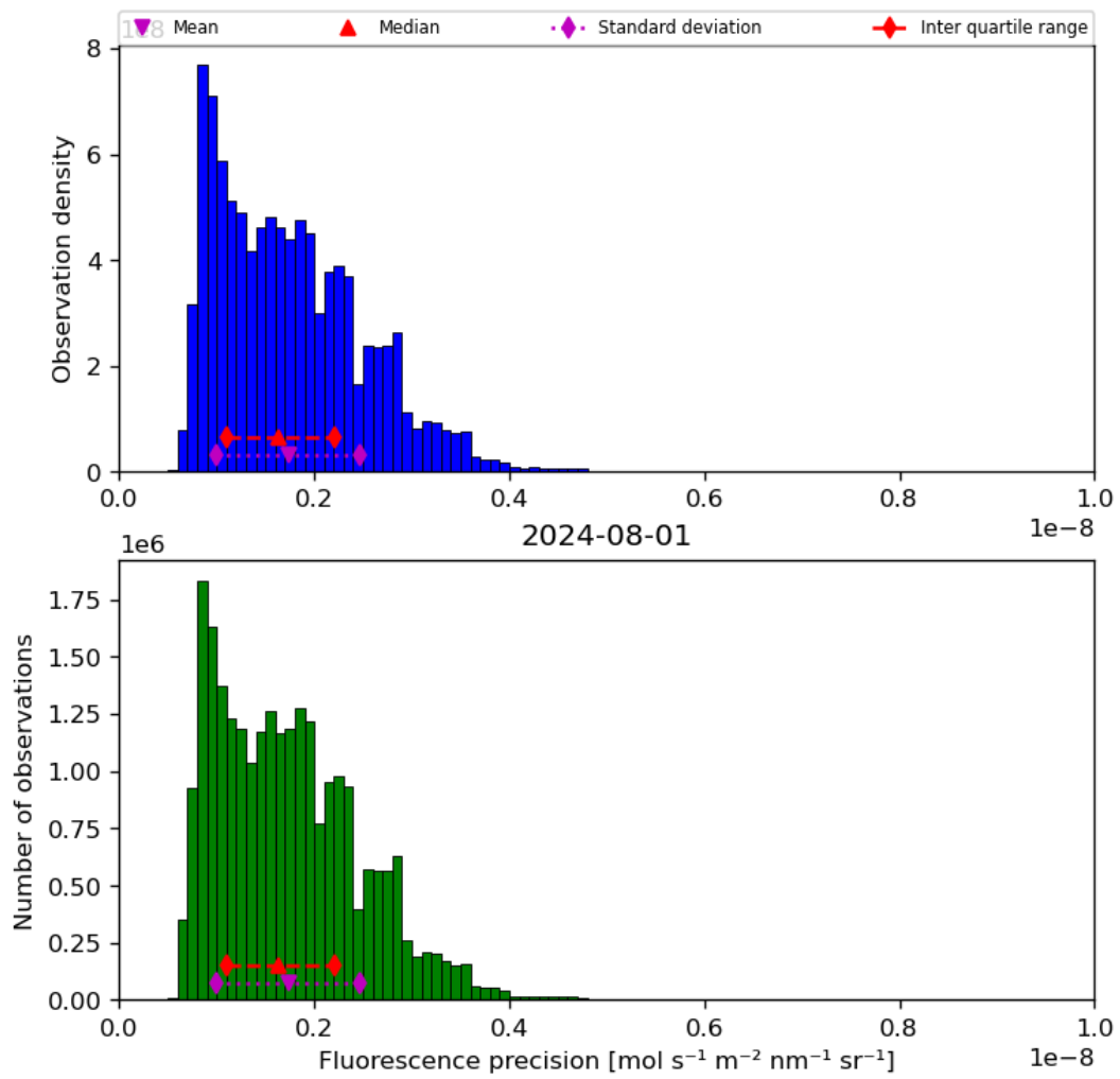
Figure 41: Histogram of “Fluorescence precision” for 2024-07-31 to 2024-08-02
