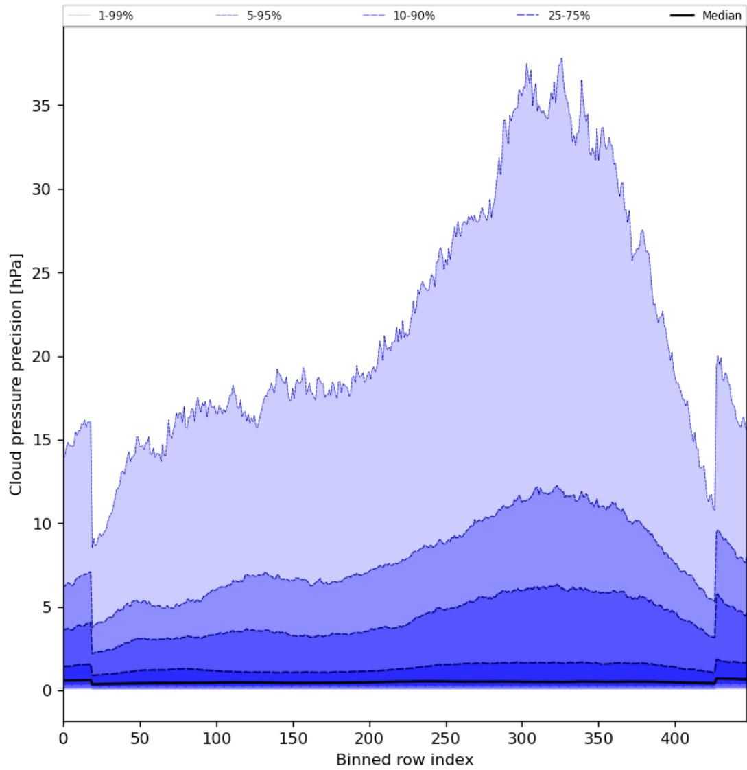
Figure 48: Along track statistics of “Cloud pressure precision” for 2024-07-31 to 2024-08-02
