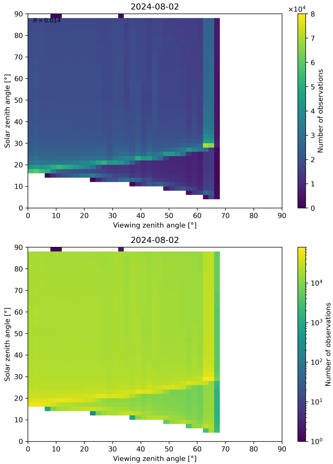
Figure 127: Scatter density plot of “Viewing zenith angle” against “Solar zenith angle” for 2024-08-01 to 2024-08-03.
