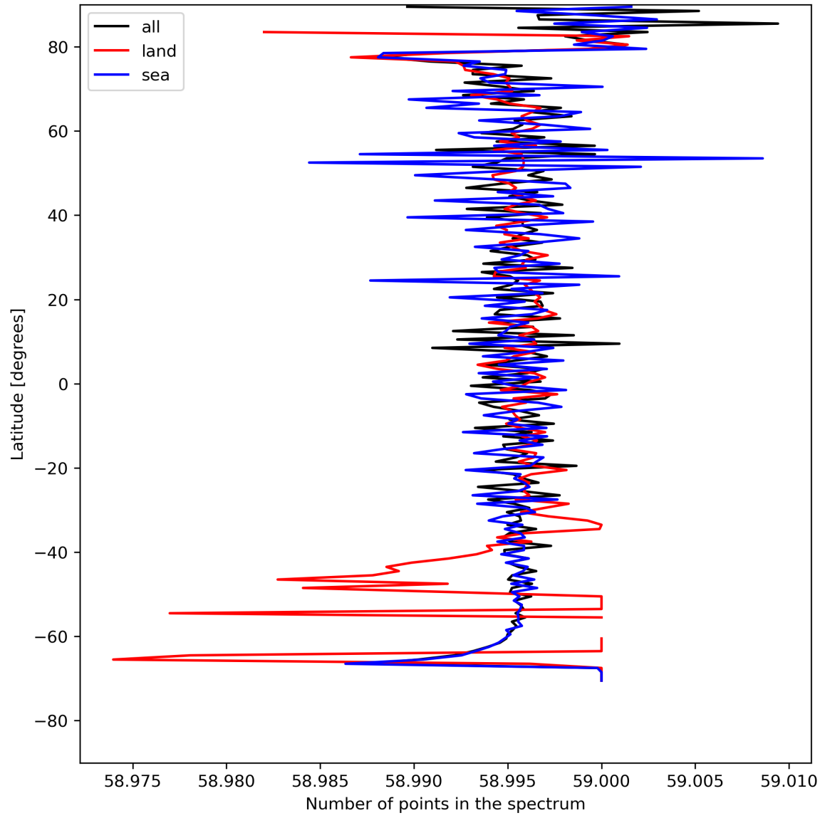
Figure 27: Zonal average of “Number of points in the spectrum” for 2024-08-01 to 2024-08-03.
