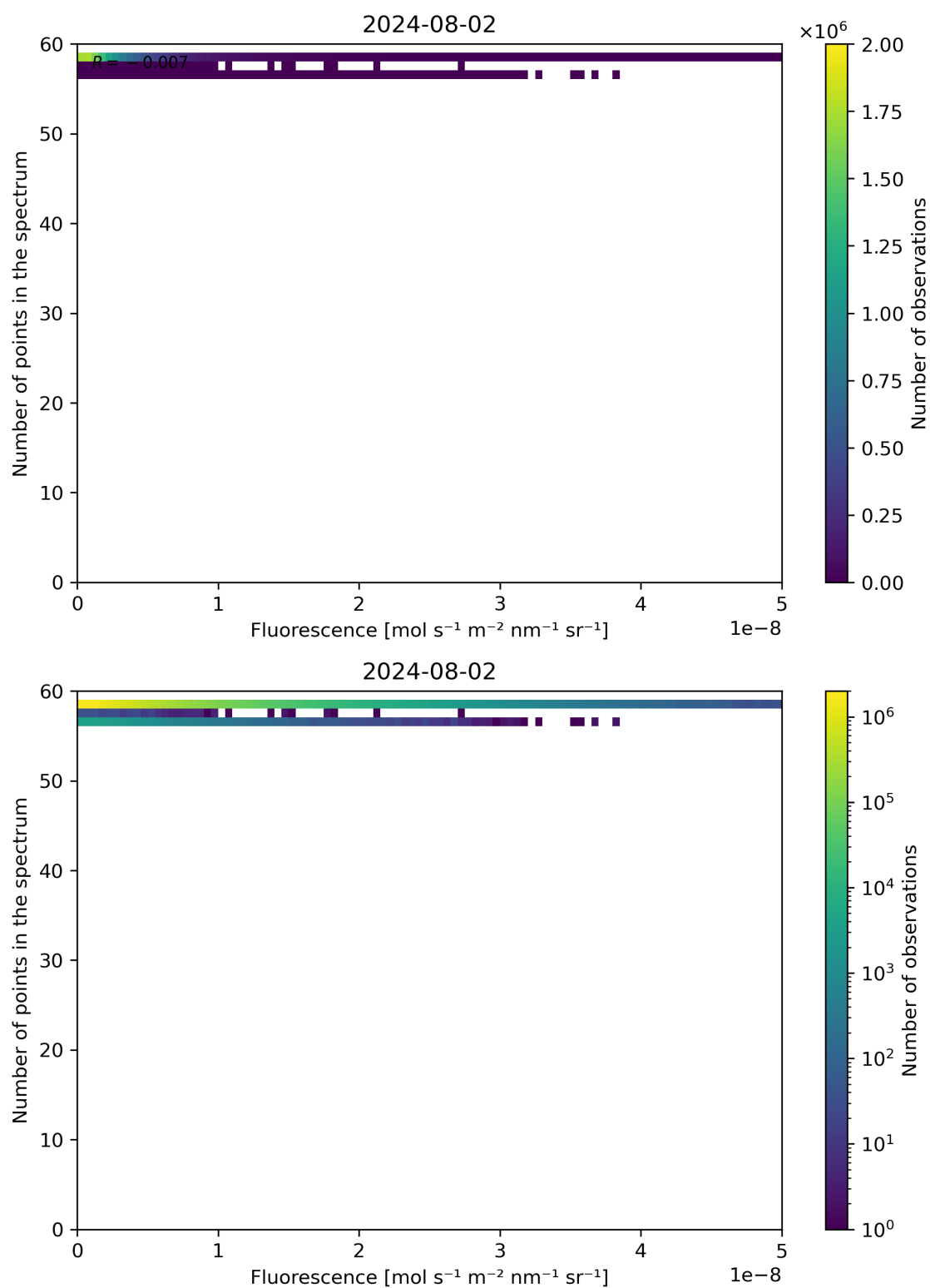
Figure 86: Scatter density plot of “Fluorescence” against “Number of points in the spectrum” for 2024-08-01 to 2024-08-03.
