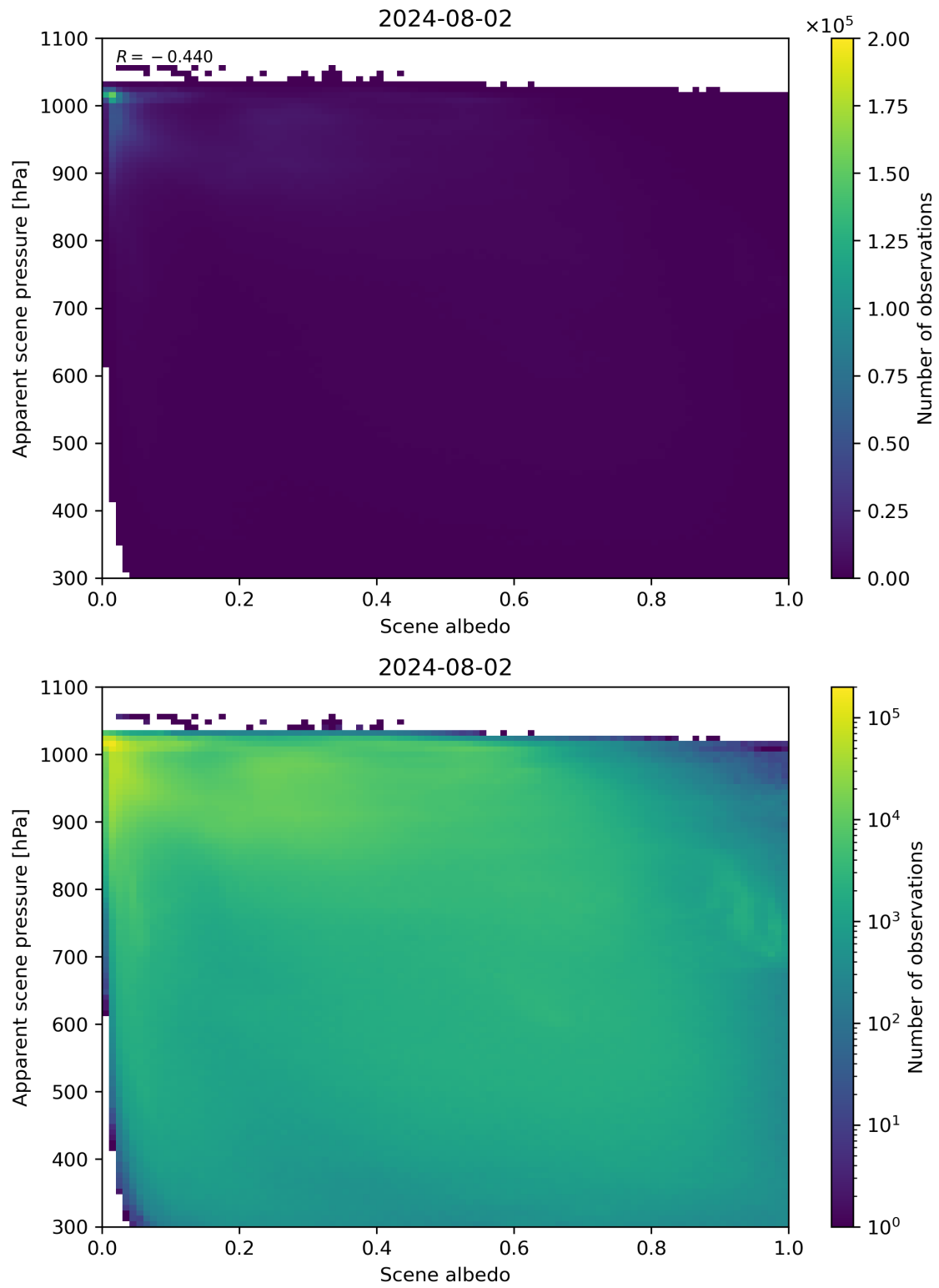
Figure 102: Scatter density plot of “Scene albedo” against “Apparent scene pressure” for 2024-08-01 to 2024-08-03.
