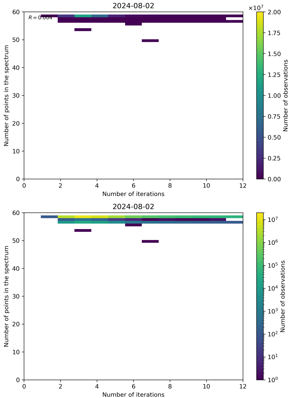
Figure 99: Scatter density plot of “Number of iterations” against “Number of points in the spectrum” for 2024-08-01 to 2024-08-03.
