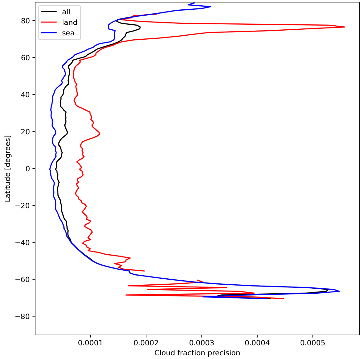
Figure 16: Zonal average of “Cloud fraction precision” for 2024-08-01 to 2024-08-03.
