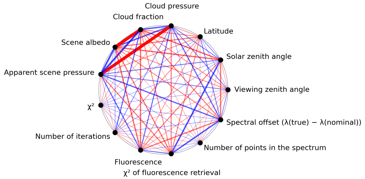
Figure 1: Map of correlation graph for 2024-08-01 to 2024-08-03.
