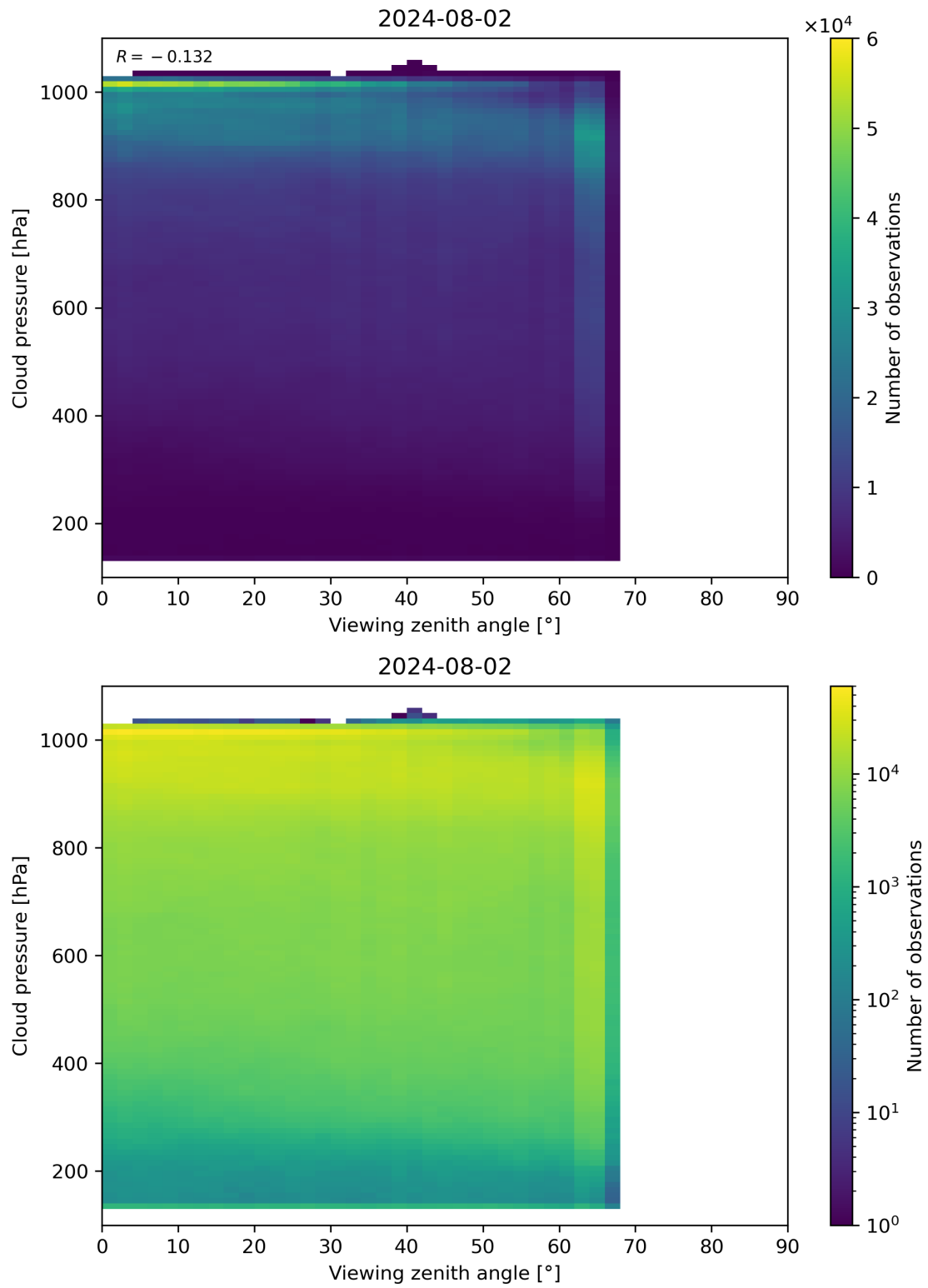
Figure 121: Scatter density plot of “Viewing zenith angle” against “Cloud pressure” for 2024-08-01 to 2024-08-03.
