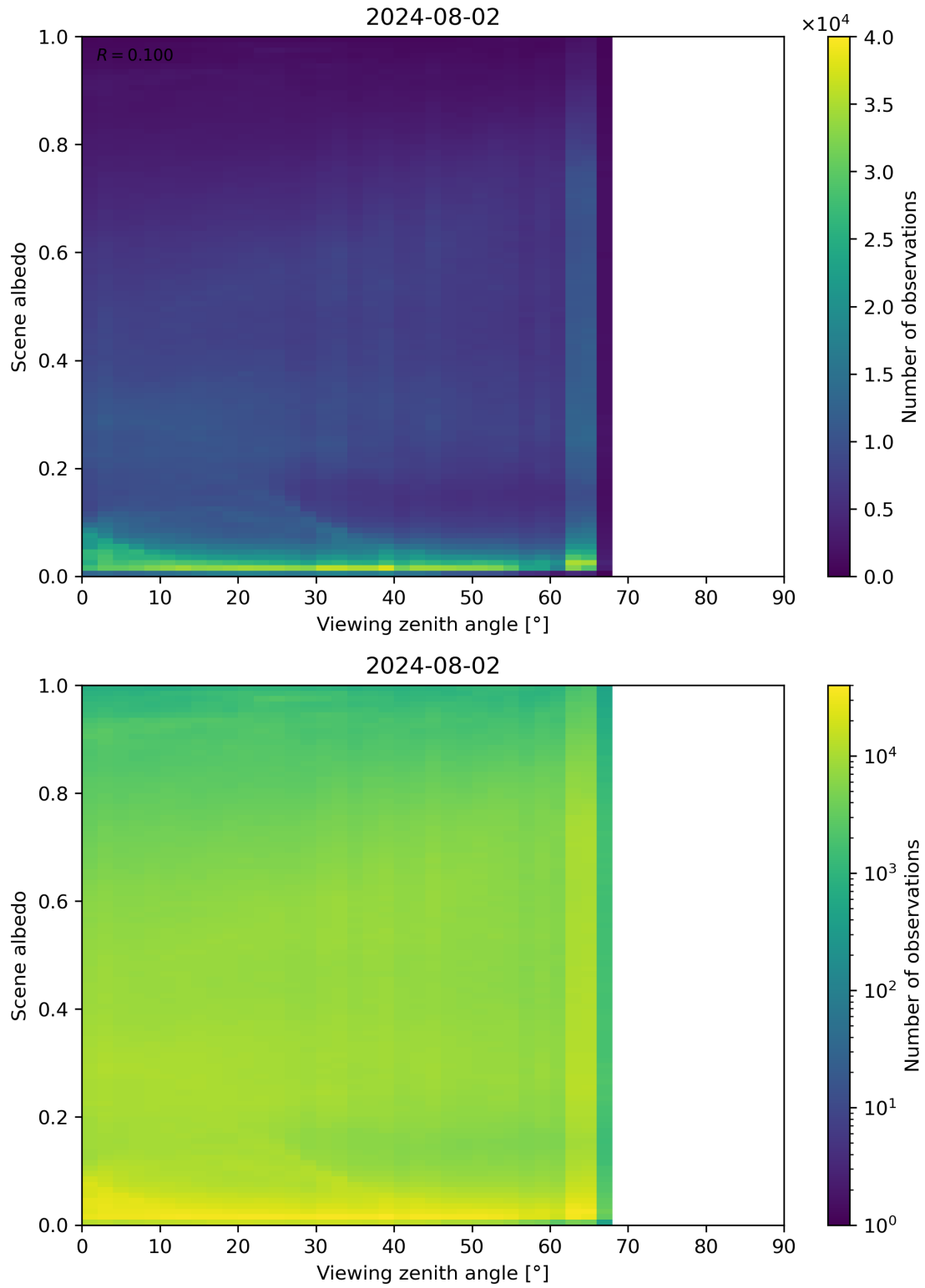
Figure 126: Scatter density plot of “Viewing zenith angle” against “Scene albedo” for 2024-08-01 to 2024-08-03.
