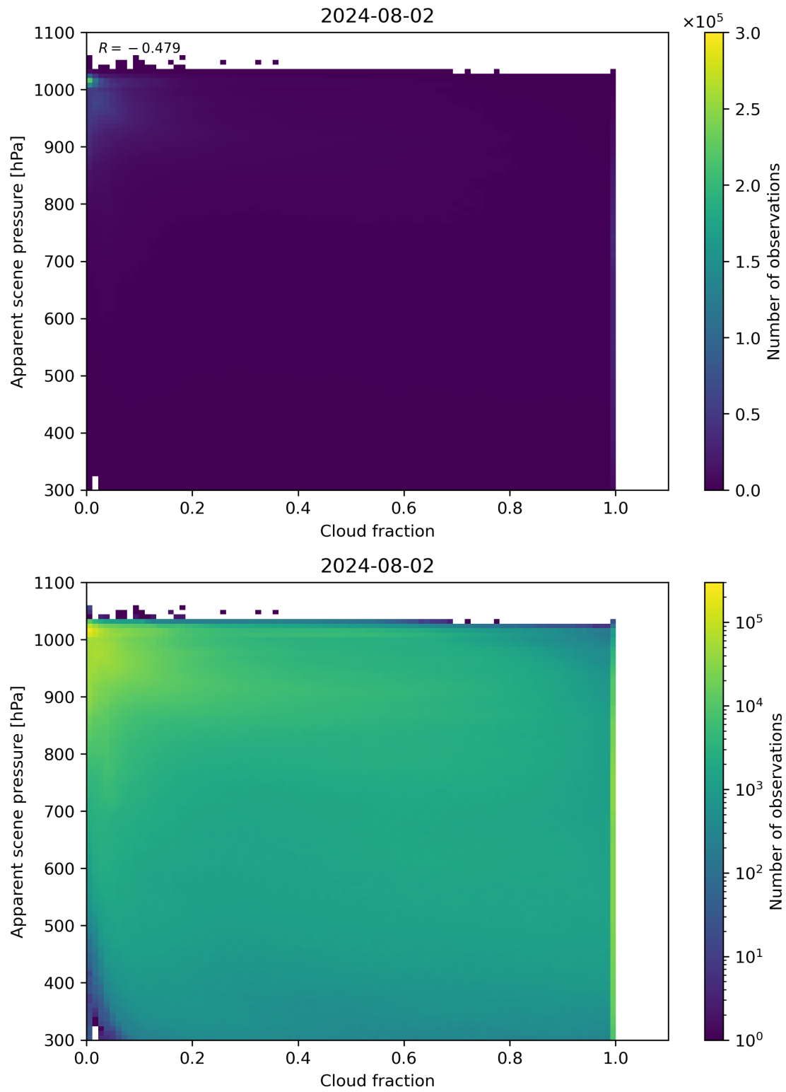
Figure 70: Scatter density plot of “Cloud fraction” against “Apparent scene pressure” for 2024-08-01 to 2024-08-03.
