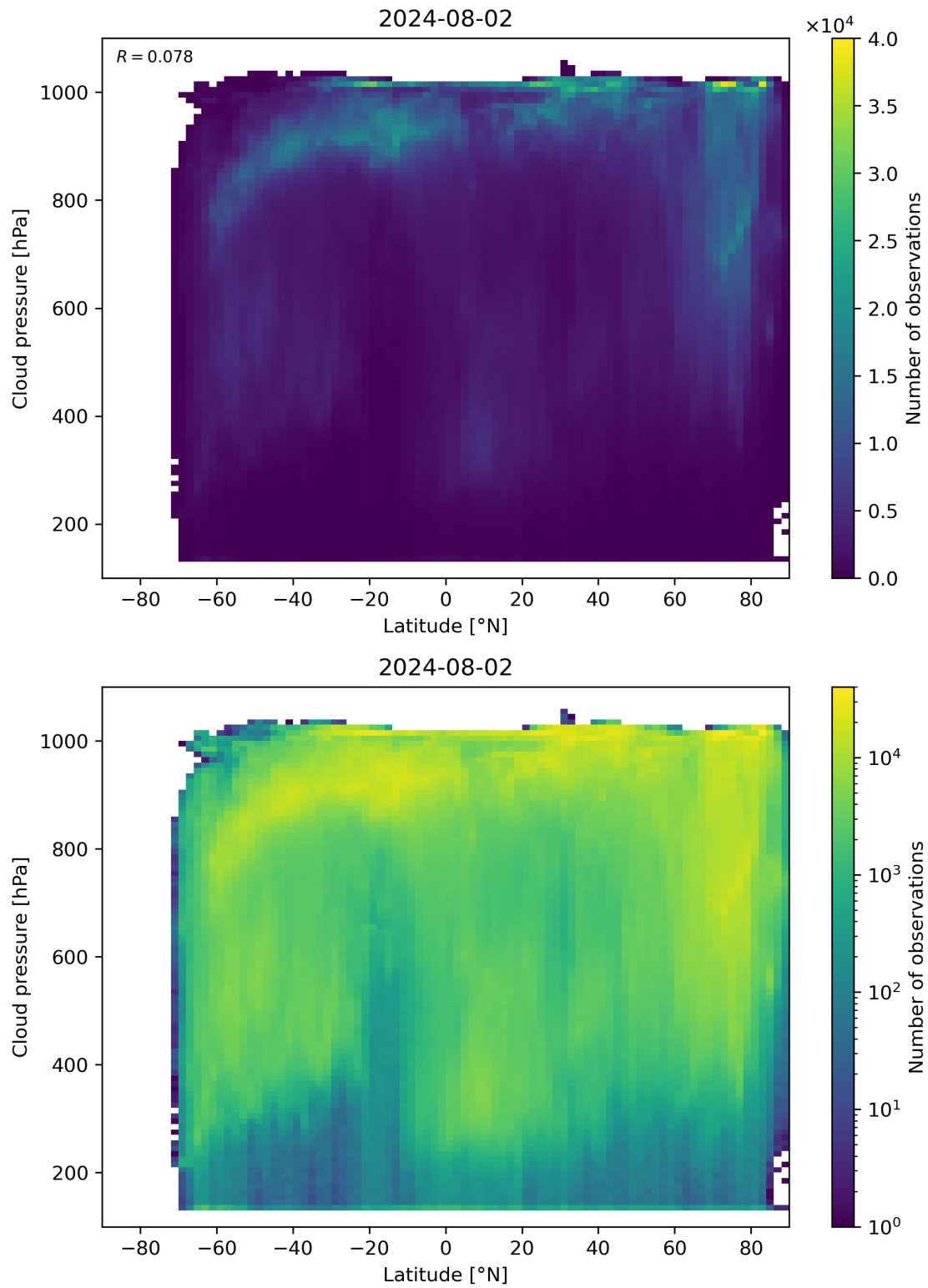
Figure 91: Scatter density plot of “Latitude” against “Cloud pressure” for 2024-08-01 to 2024-08-03.
