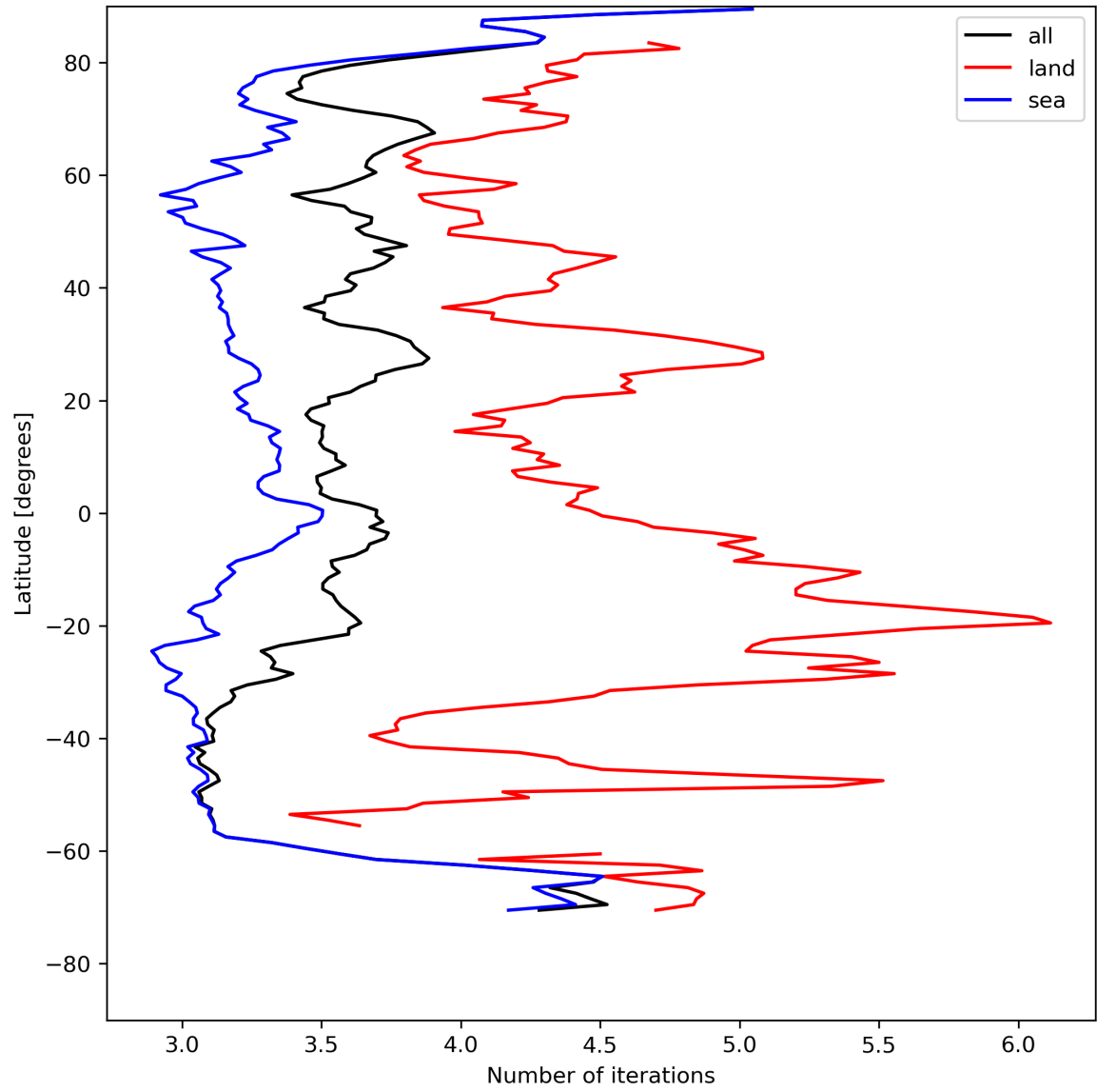
Figure 22: Zonal average of “Number of iterations” for 2024-08-01 to 2024-08-03.
