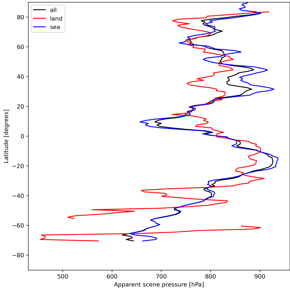
Figure 19: Zonal average of “Apparent scene pressure” for 2024-08-01 to 2024-08-03.
