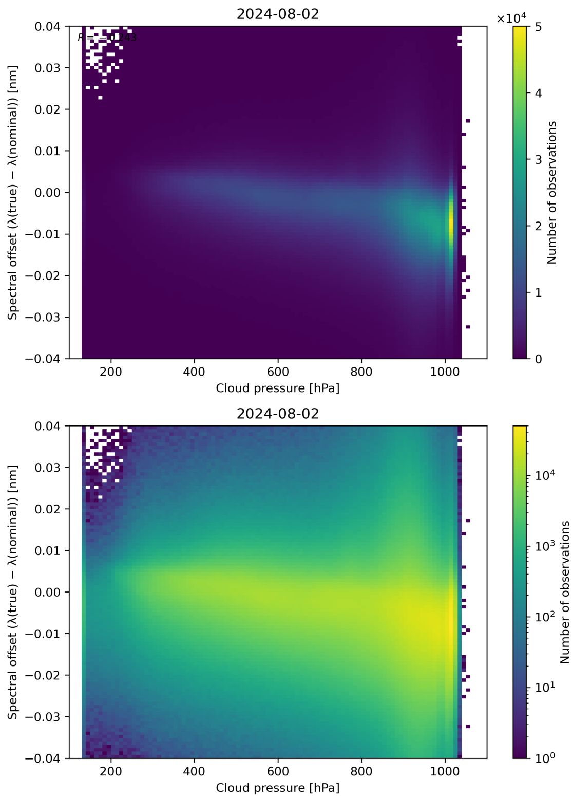
Figure 84: Scatter density plot of “Cloud pressure” against “Spectral offset ( \lambda(\text{true}) - \lambda(\text{nominal}) )” for 2024-08-01 to 2024-08-03.
