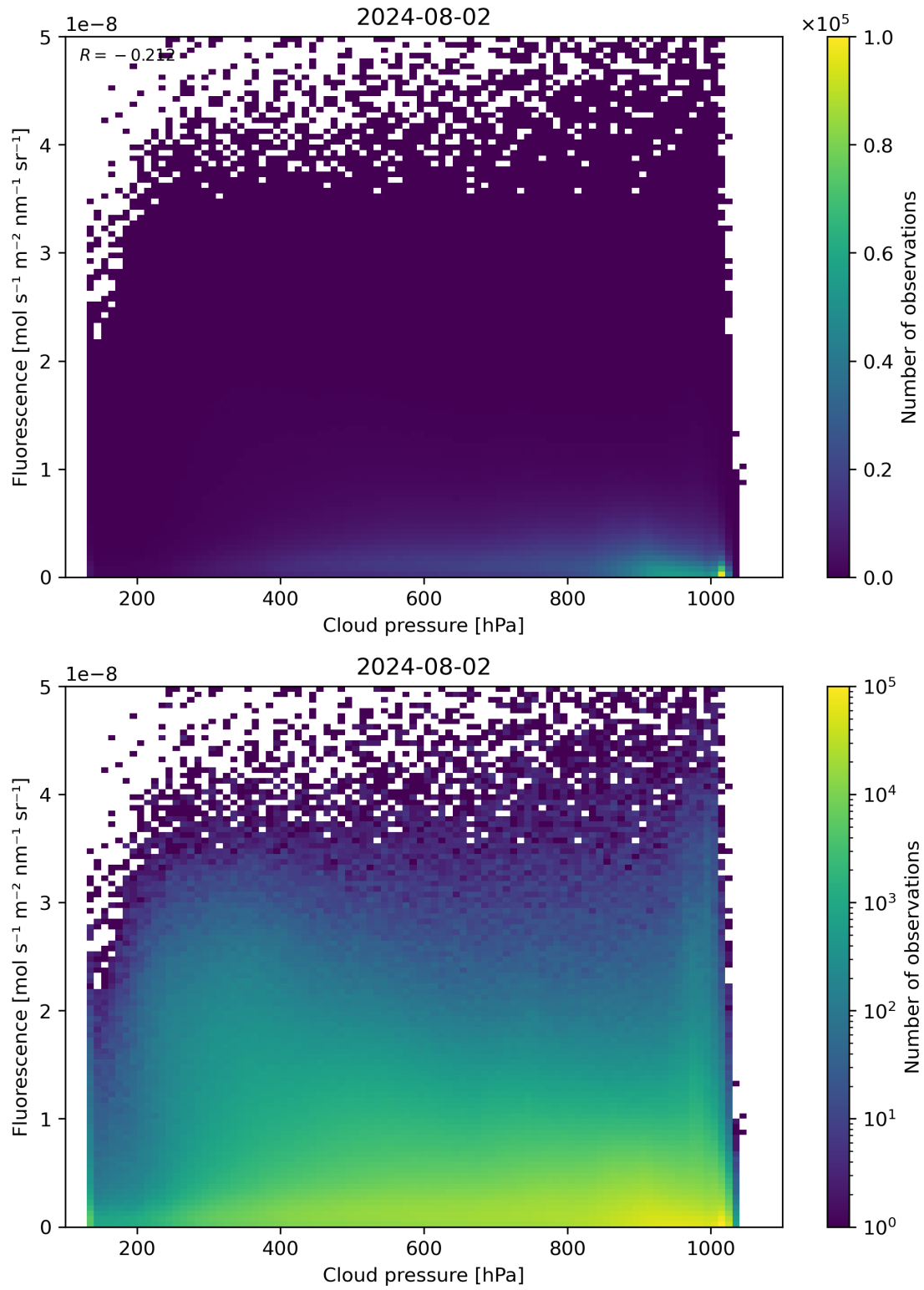
Figure 80: Scatter density plot of “Cloud pressure” against “Fluorescence” for 2024-08-01 to 2024-08-03.
