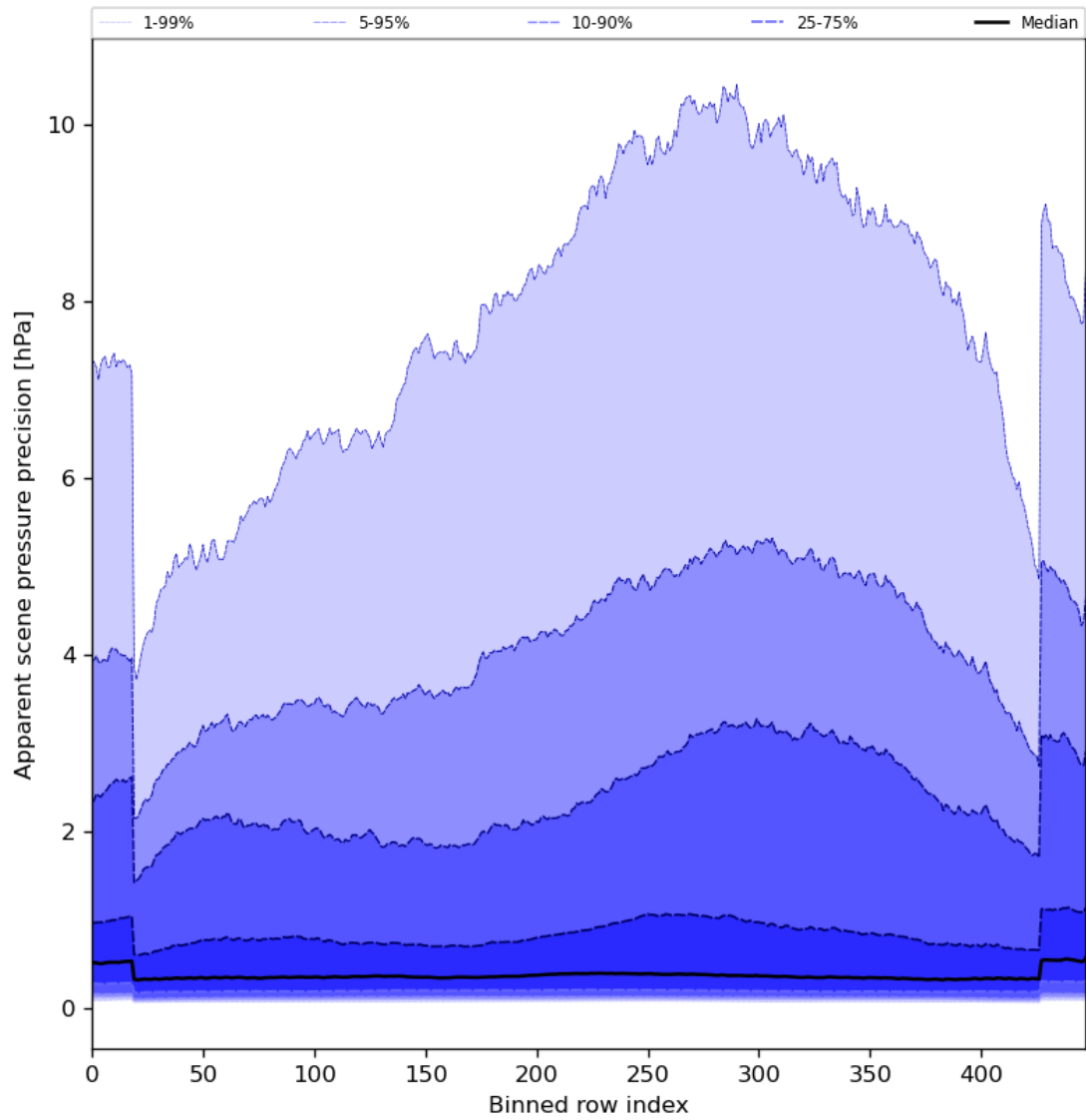
Figure 54: Along track statistics of “Apparent scene pressure precision” for 2024-08-01 to 2024-08-03
