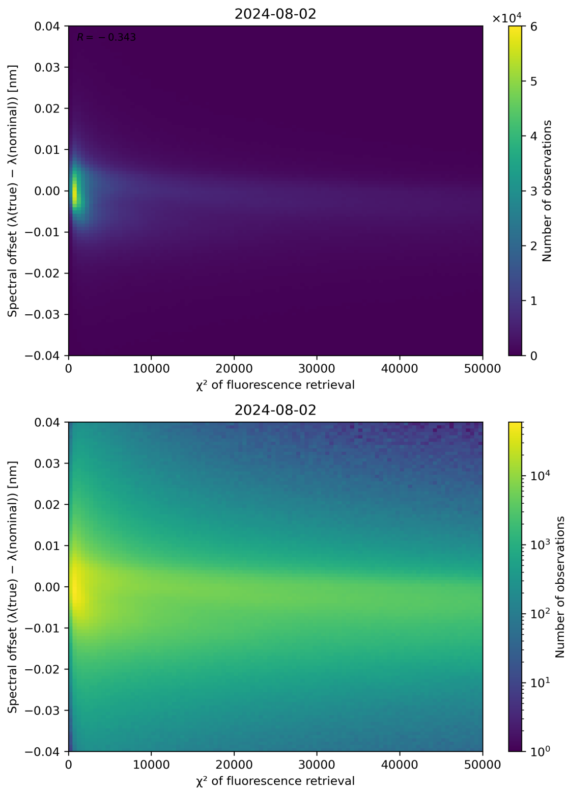
Figure 69: Scatter density plot of " \chi^2 of fluorescence retrieval" against "Spectral offset ( \lambda(\text{true}) - \lambda(\text{nominal})) " for 2024-08-01 to 2024-08-03.
