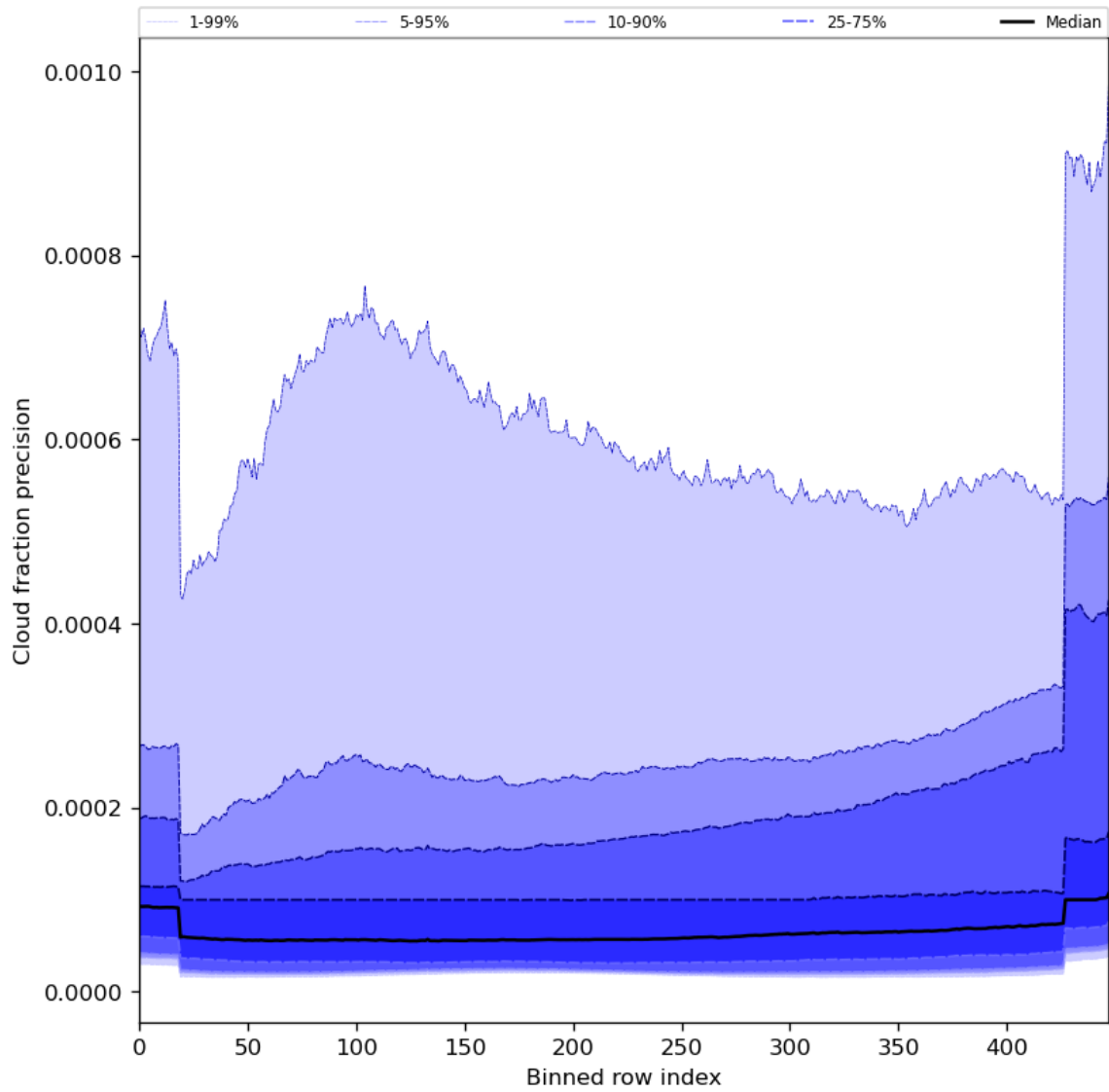
Figure 50: Along track statistics of “Cloud fraction precision” for 2024-08-01 to 2024-08-03
