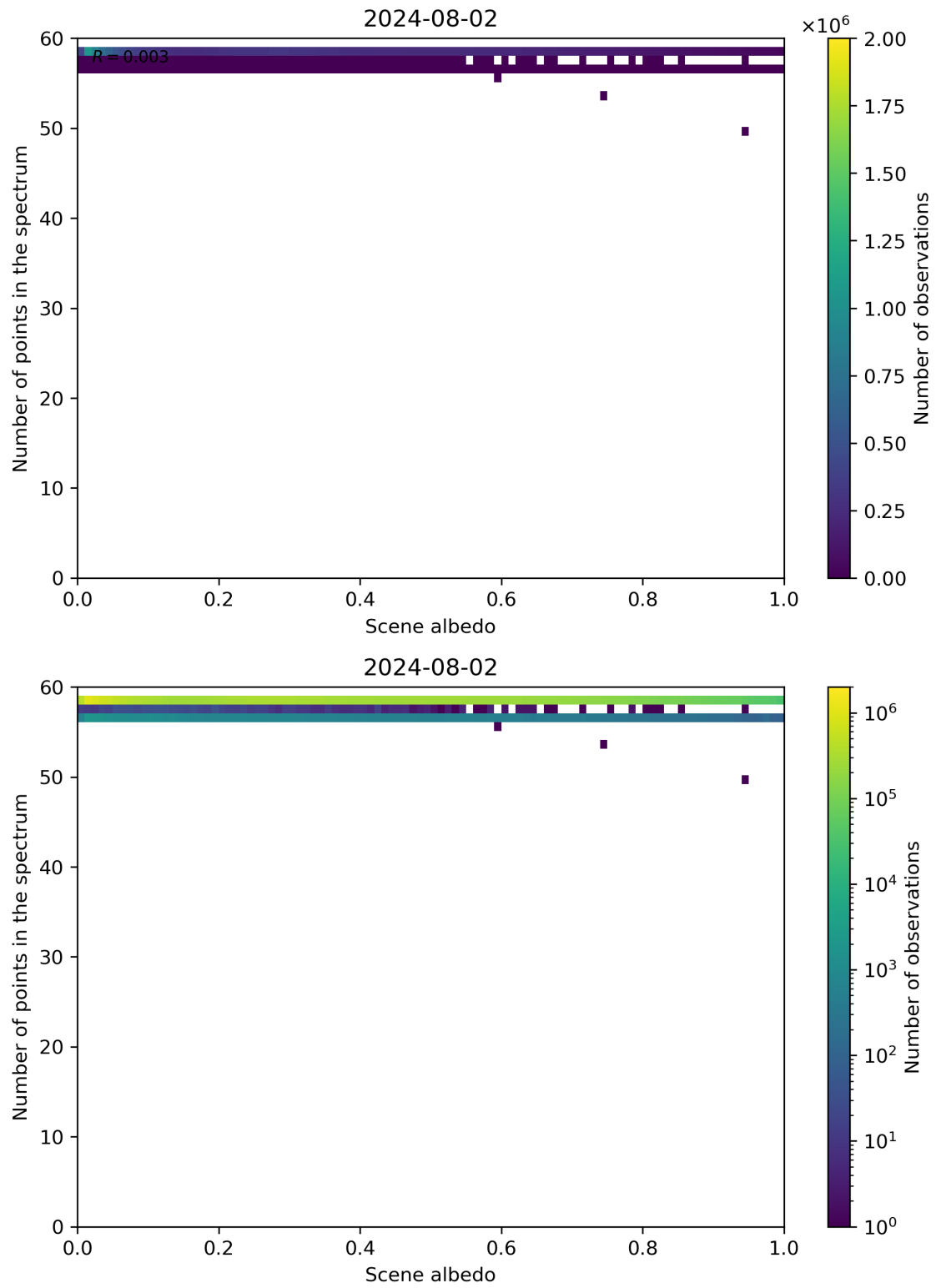
Figure 106: Scatter density plot of “Scene albedo” against “Number of points in the spectrum” for 2024-08-01 to 2024-08-03.
