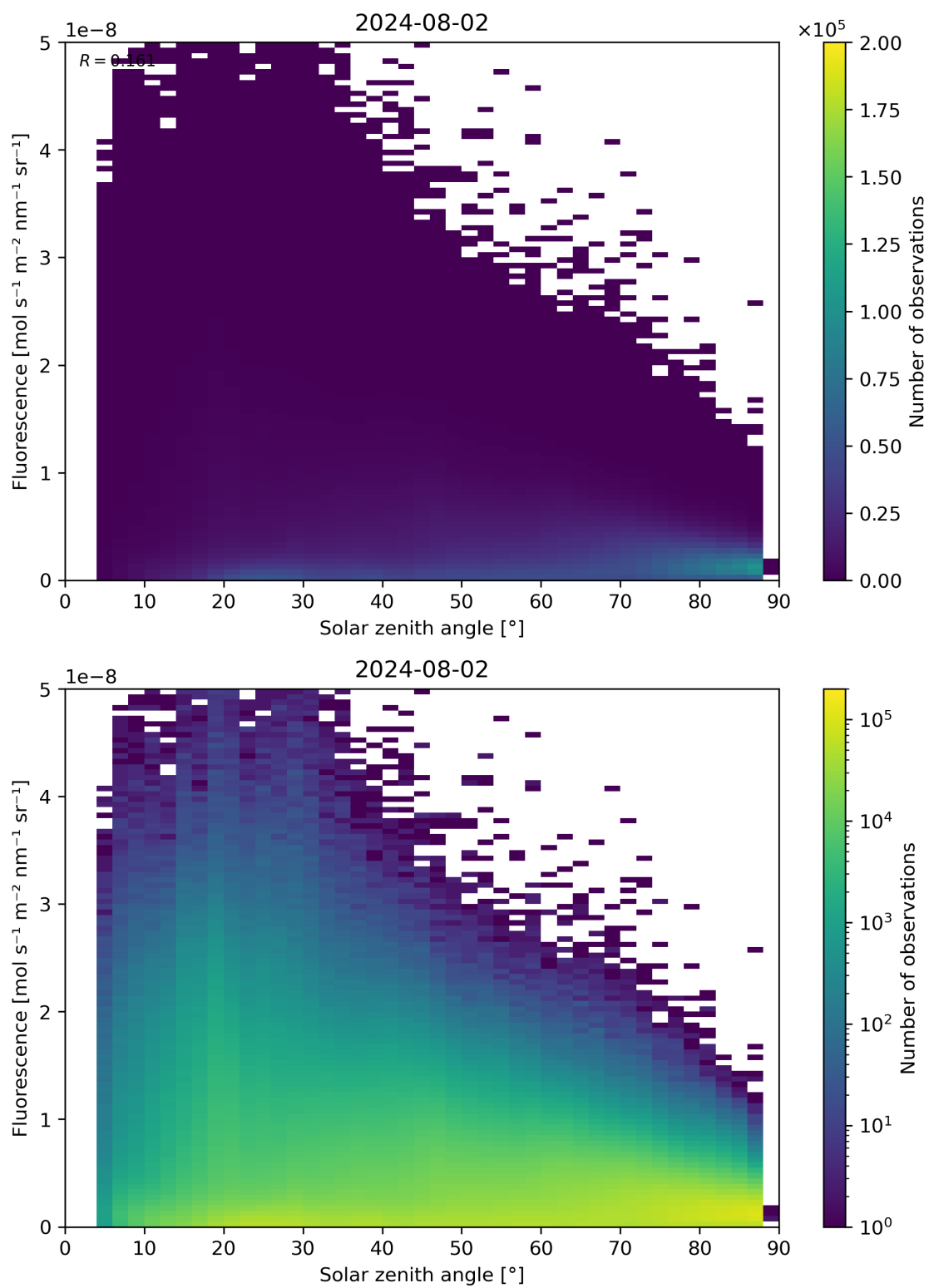
Figure 112: Scatter density plot of “Solar zenith angle” against “Fluorescence” for 2024-08-01 to 2024-08-03.
