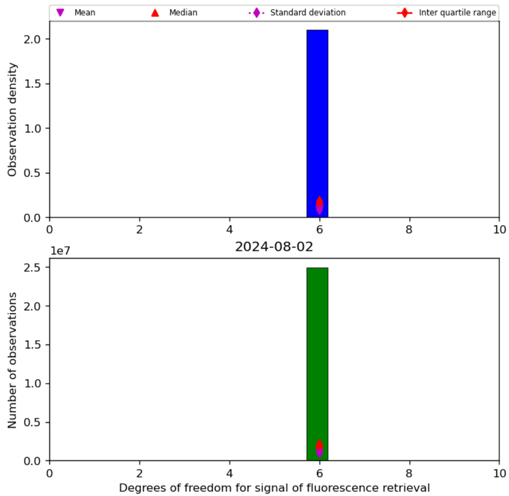
Figure 43: Histogram of “Degrees of freedom for signal of fluorescence retrieval” for 2024-08-01 to 2024-08-03
