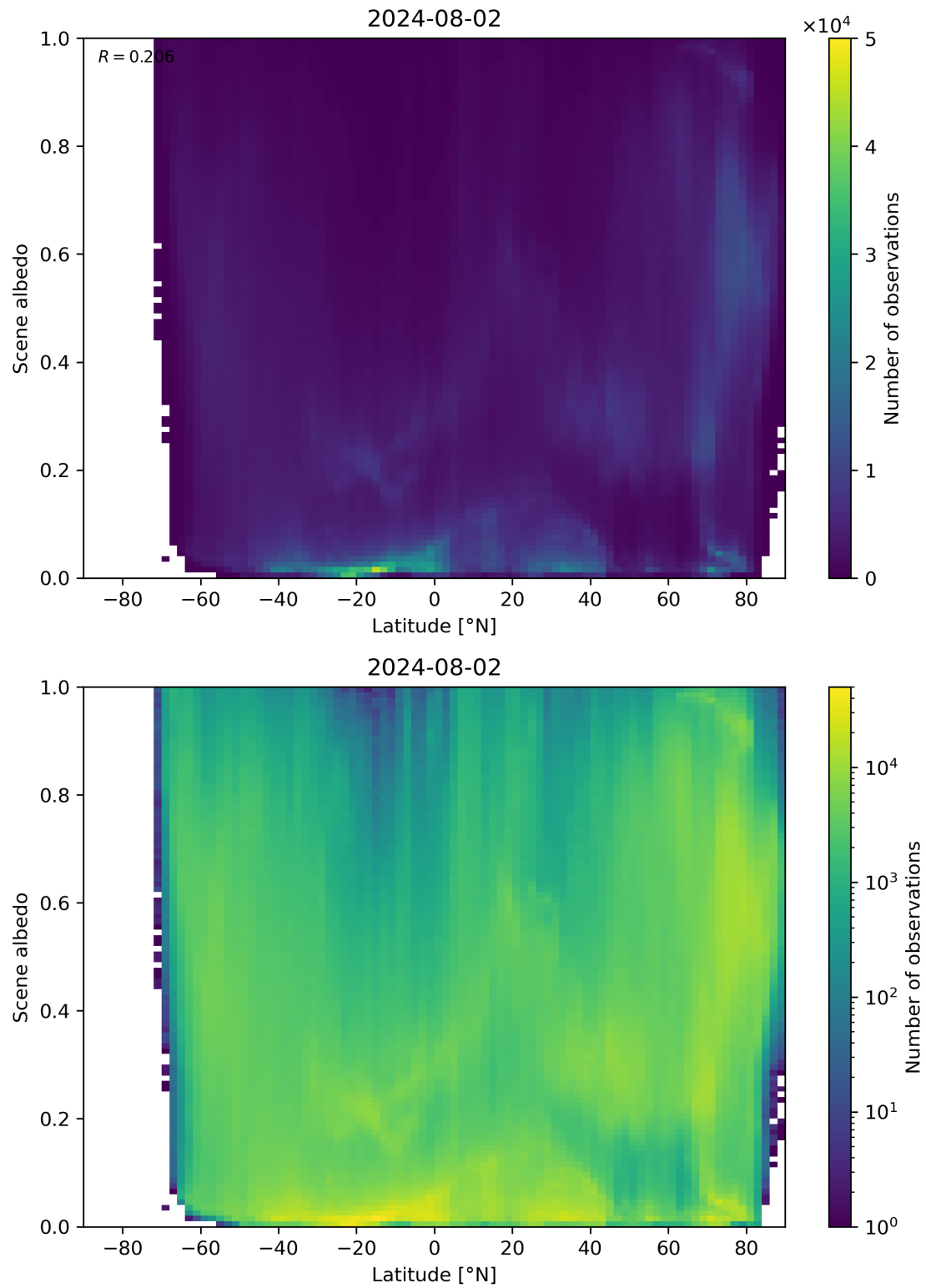
Figure 95: Scatter density plot of “Latitude” against “Scene albedo” for 2024-08-01 to 2024-08-03.
