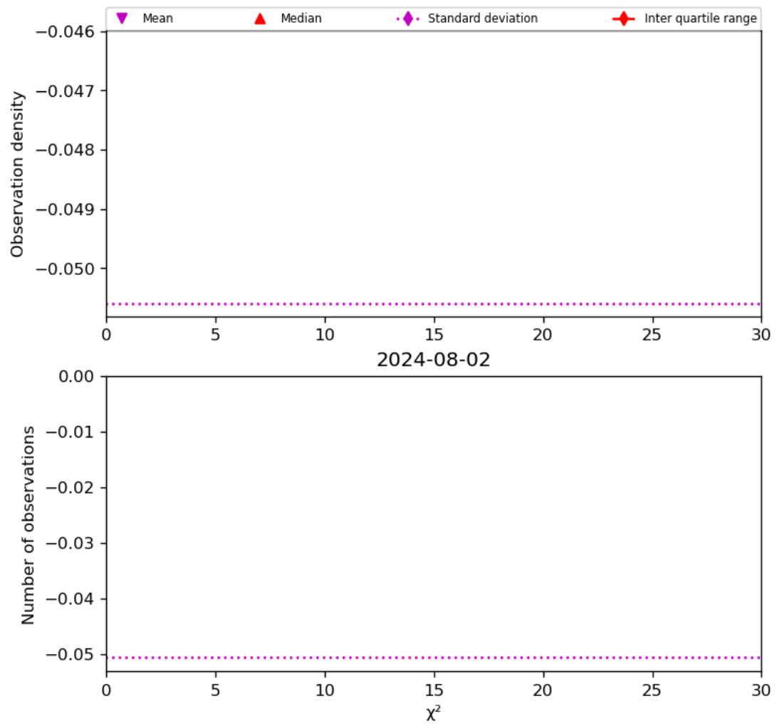
Figure 38: Histogram of “ \chi^2 ” for 2024-08-01 to 2024-08-03
