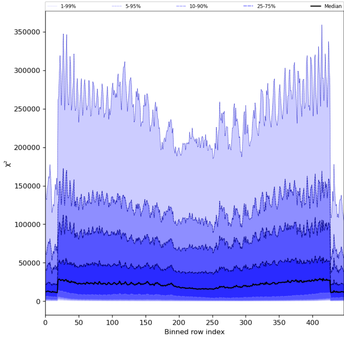
Figure 55: Along track statistics of “ \chi^2 ” for 2024-08-01 to 2024-08-03
