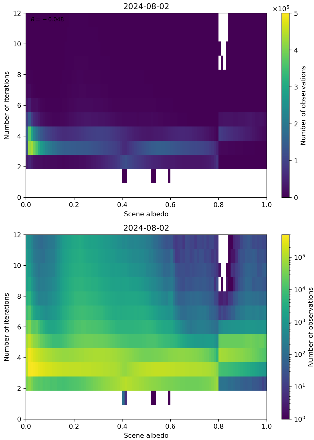
Figure 105: Scatter density plot of “Scene albedo” against “Number of iterations” for 2024-08-01 to 2024-08-03.
