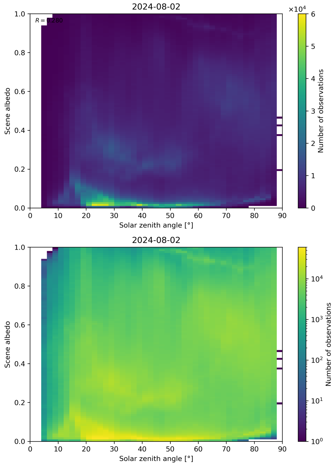
Figure 116: Scatter density plot of “Solar zenith angle” against “Scene albedo” for 2024-08-01 to 2024-08-03.
