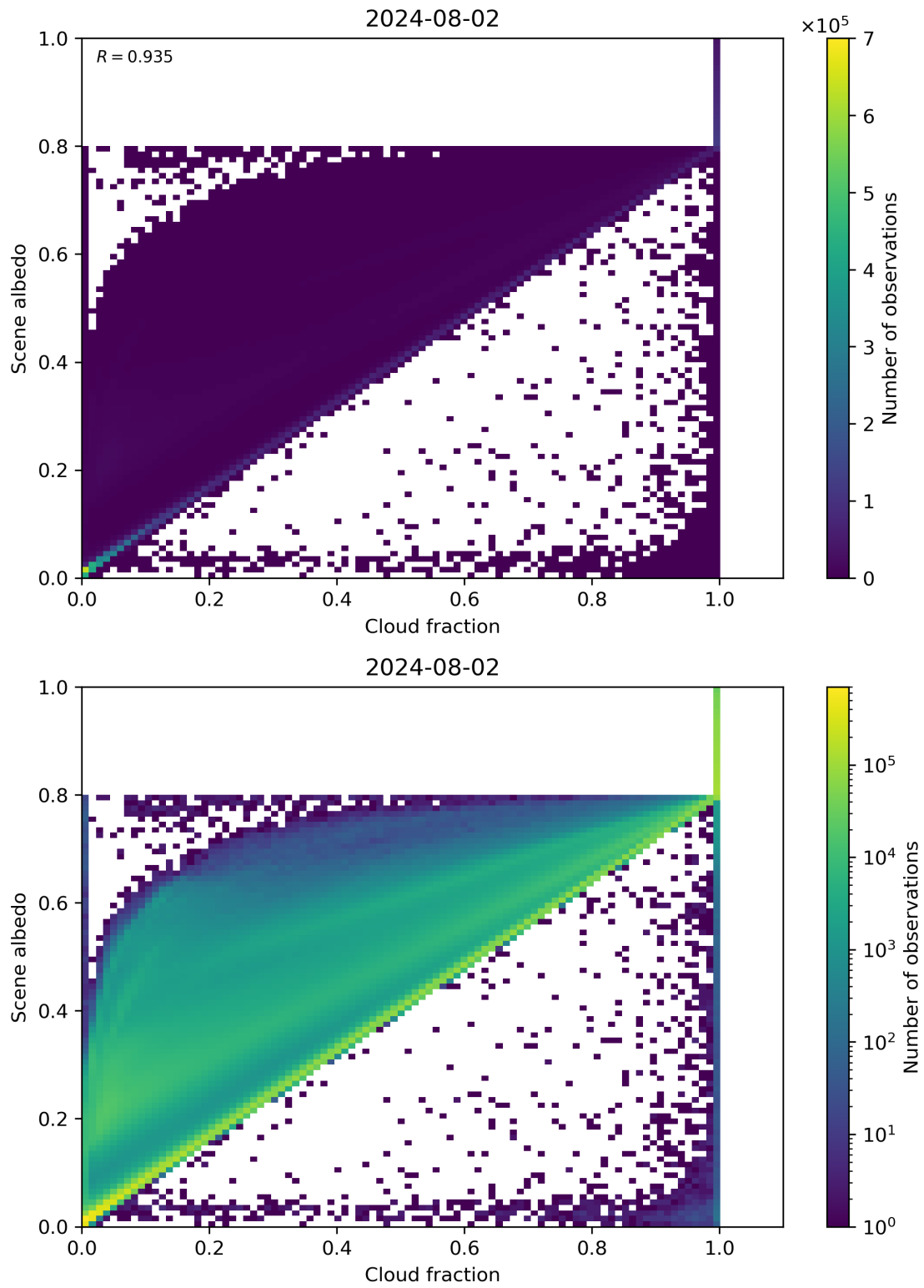
Figure 75: Scatter density plot of “Cloud fraction” against “Scene albedo” for 2024-08-01 to 2024-08-03.
