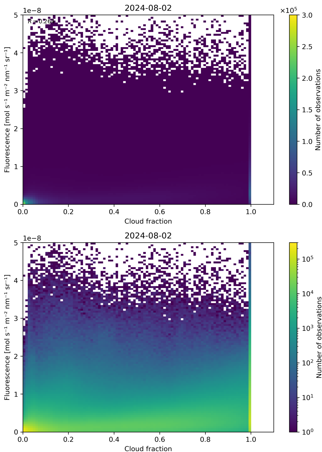
Figure 72: Scatter density plot of “Cloud fraction” against “Fluorescence” for 2024-08-01 to 2024-08-03.
