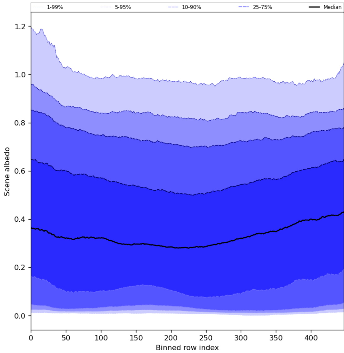
Figure 51: Along track statistics of “Scene albedo” for 2024-08-01 to 2024-08-03
