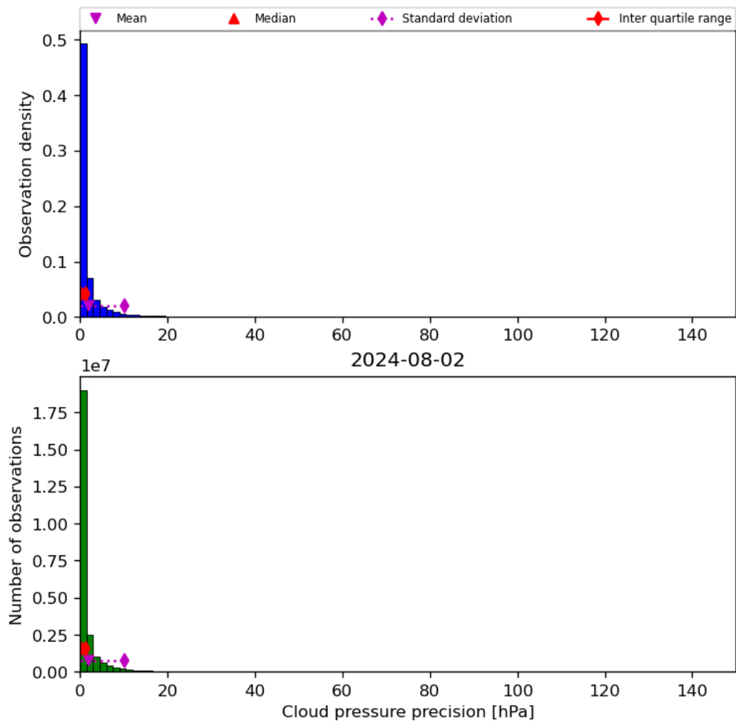
Figure 31: Histogram of “Cloud pressure precision” for 2024-08-01 to 2024-08-03
