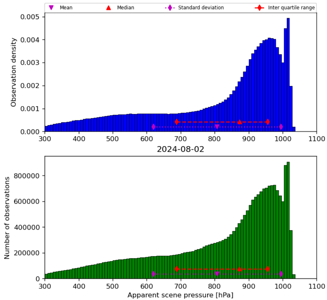
Figure 36: Histogram of “Apparent scene pressure” for 2024-08-01 to 2024-08-03
