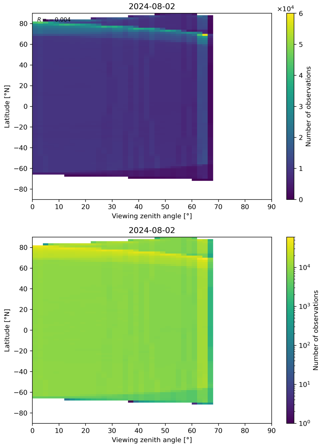
Figure 123: Scatter density plot of “Viewing zenith angle” against “Latitude” for 2024-08-01 to 2024-08-03.
