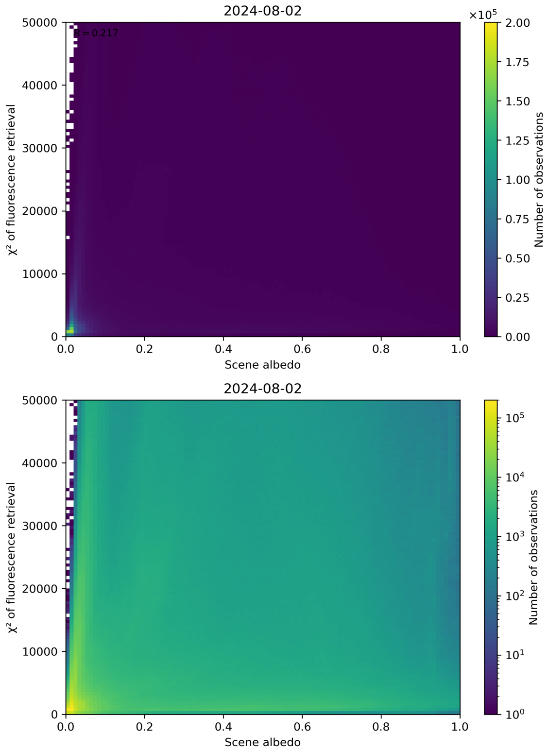
Figure 103: Scatter density plot of “Scene albedo” against “ \chi^2 of fluorescence retrieval” for 2024-08-01 to 2024-08-03.
