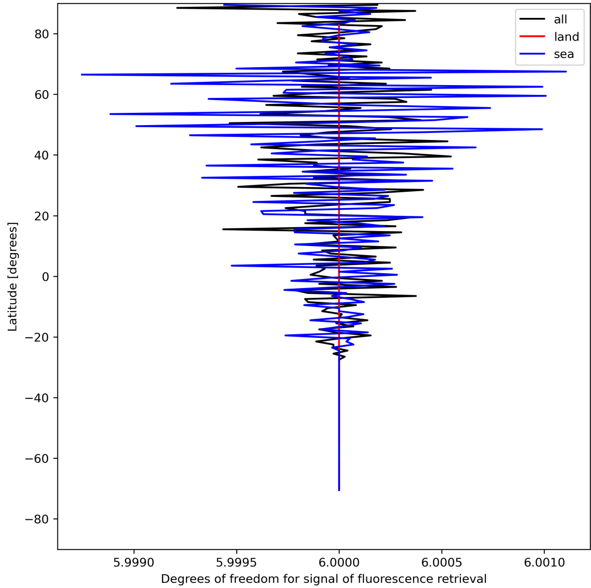
Figure 26: Zonal average of “Degrees of freedom for signal of fluorescence retrieval” for 2024-08-01 to 2024-08-03.
