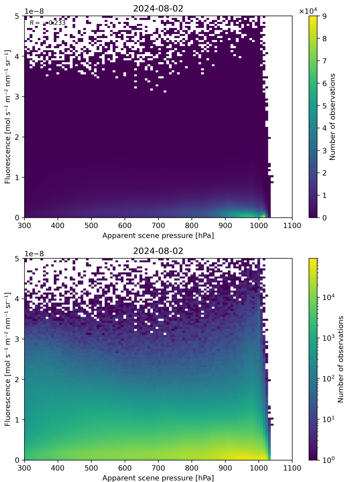
Figure 64: Scatter density plot of “Apparent scene pressure” against “Fluorescence” for 2024-08-01 to 2024-08-03.
