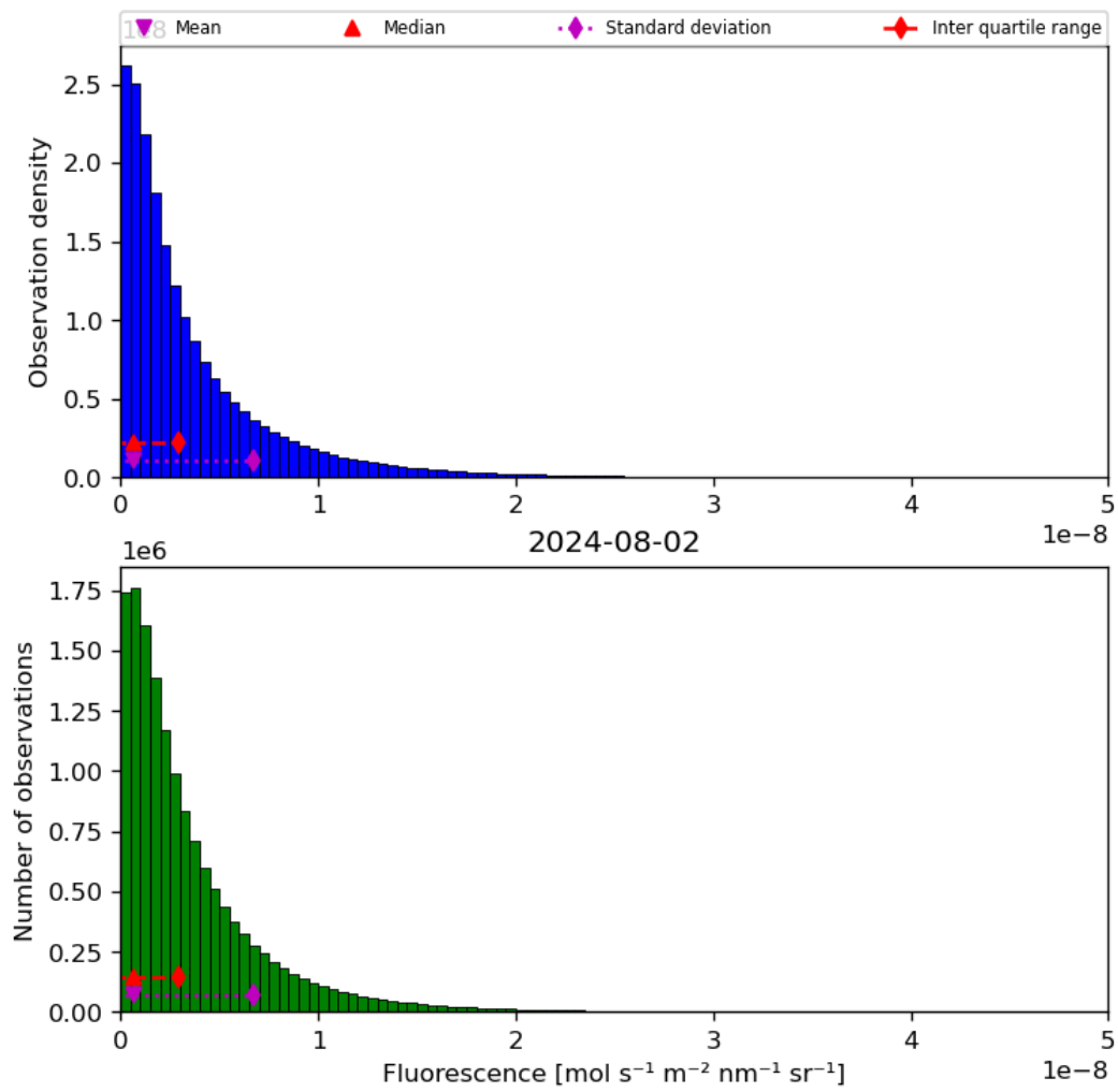
Figure 40: Histogram of “Fluorescence” for 2024-08-01 to 2024-08-03
