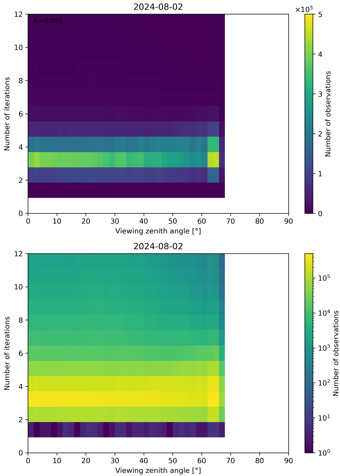
Figure 124: Scatter density plot of “Viewing zenith angle” against “Number of iterations” for 2024-08-01 to 2024-08-03.
