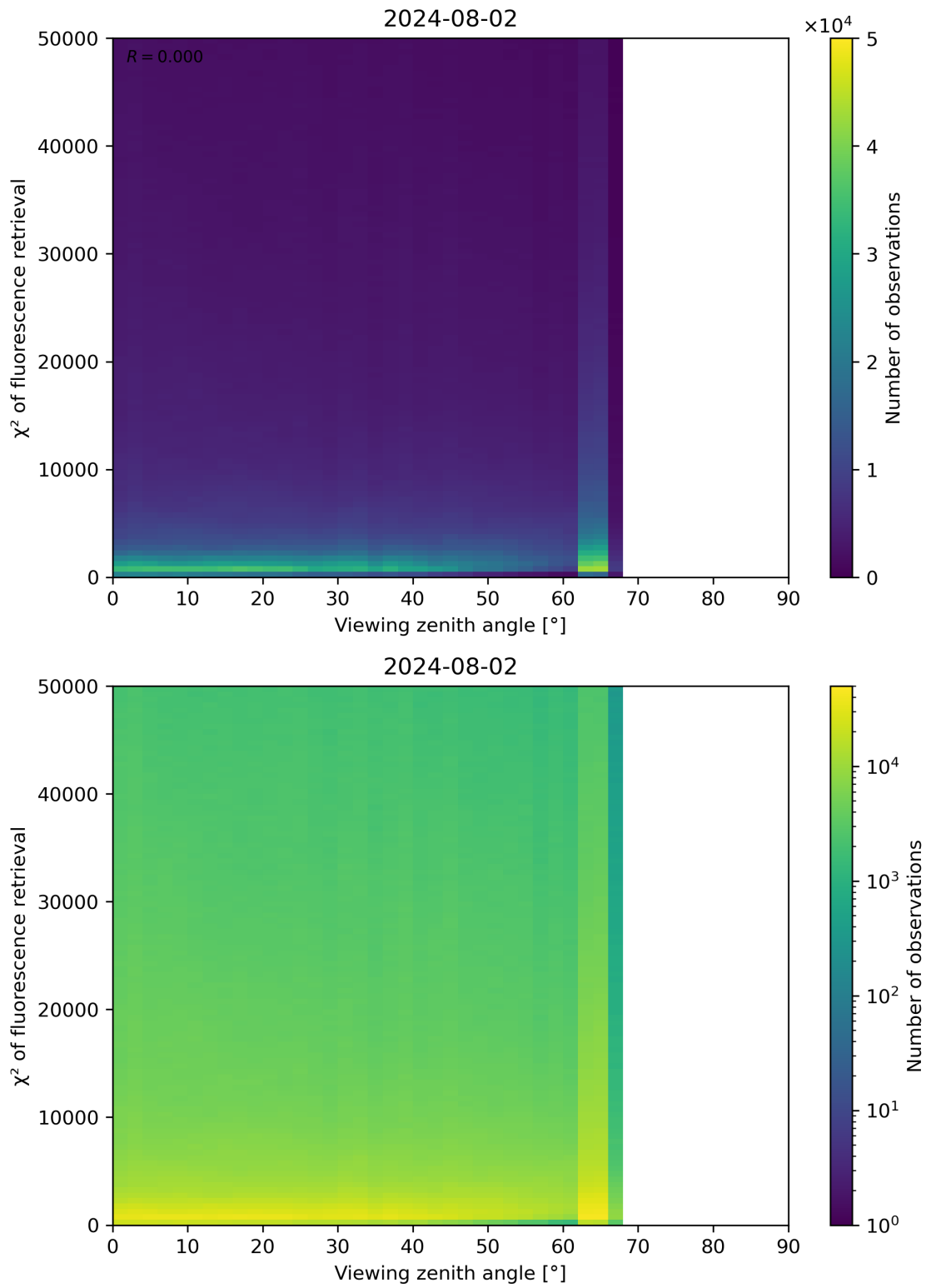
Figure 119: Scatter density plot of “Viewing zenith angle” against “ \chi^2 of fluorescence retrieval” for 2024-08-01 to 2024-08-03.
