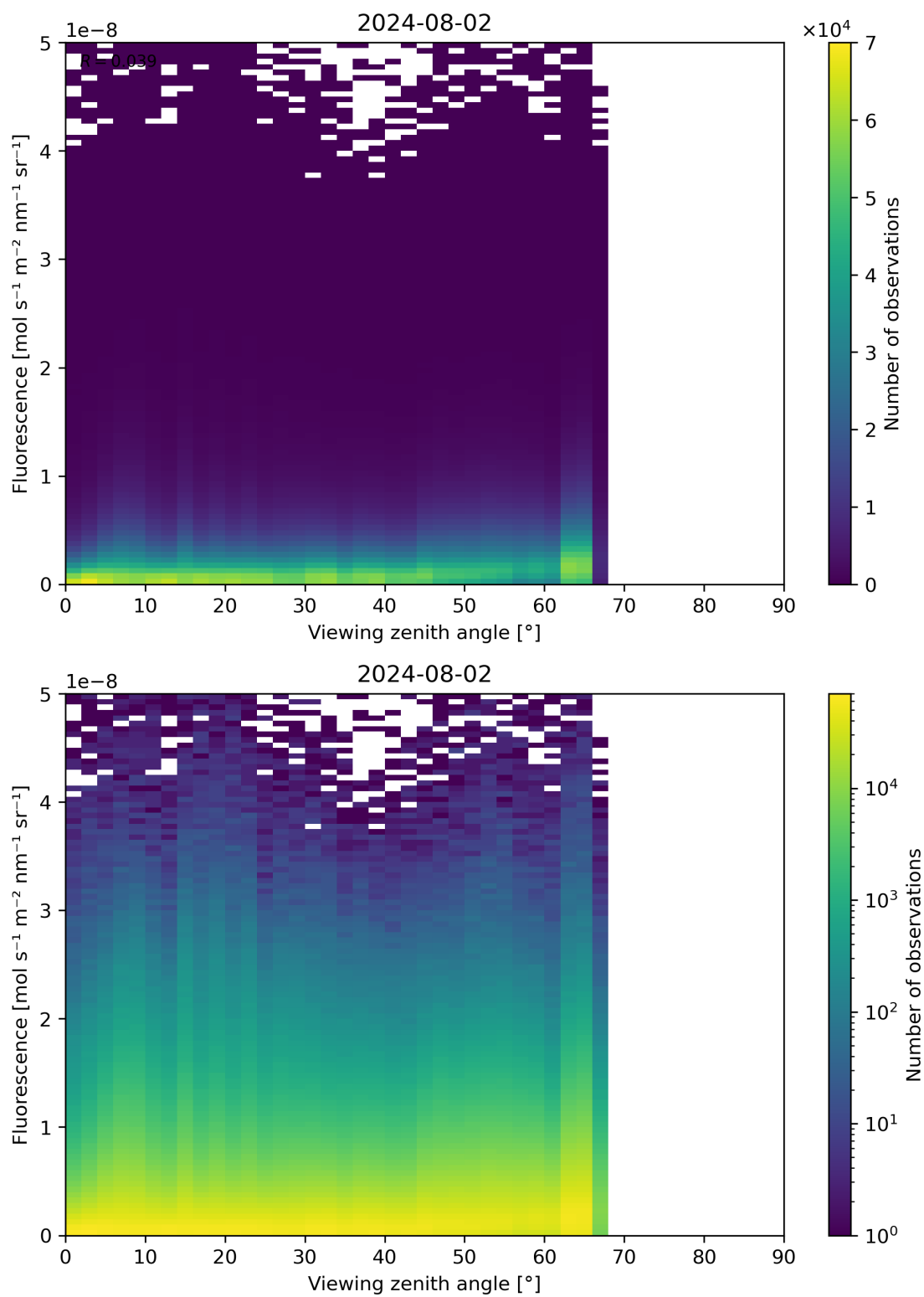
Figure 122: Scatter density plot of “Viewing zenith angle” against “Fluorescence” for 2024-08-01 to 2024-08-03.
