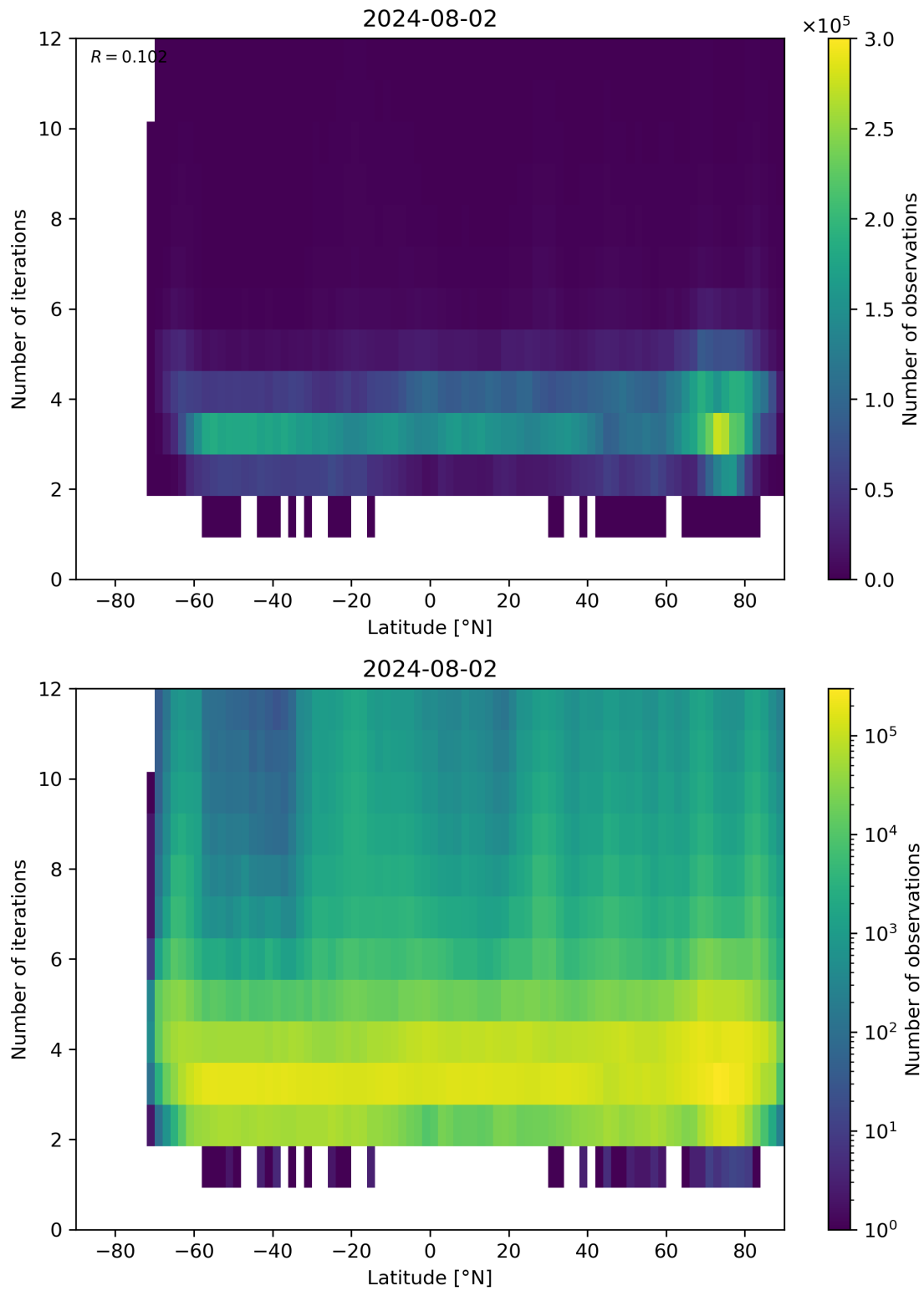
Figure 93: Scatter density plot of “Latitude” against “Number of iterations” for 2024-08-01 to 2024-08-03.
