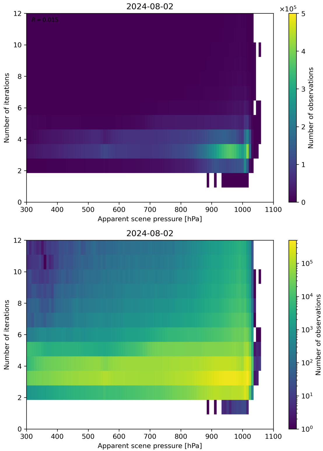
Figure 65: Scatter density plot of “Apparent scene pressure” against “Number of iterations” for 2024-08-01 to 2024-08-03.
