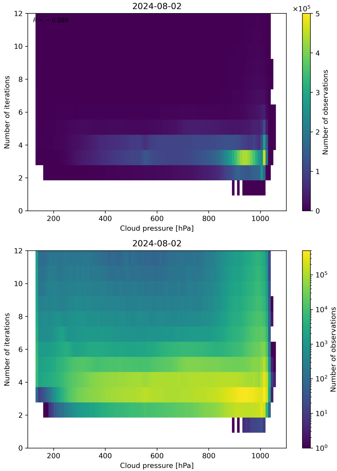
Figure 81: Scatter density plot of “Cloud pressure” against “Number of iterations” for 2024-08-01 to 2024-08-03.
