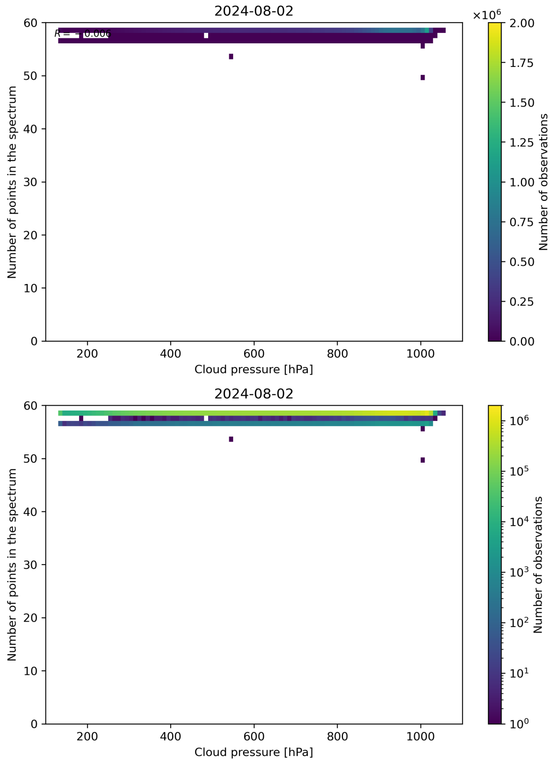
Figure 82: Scatter density plot of “Cloud pressure” against “Number of points in the spectrum” for 2024-08-01 to 2024-08-03.
