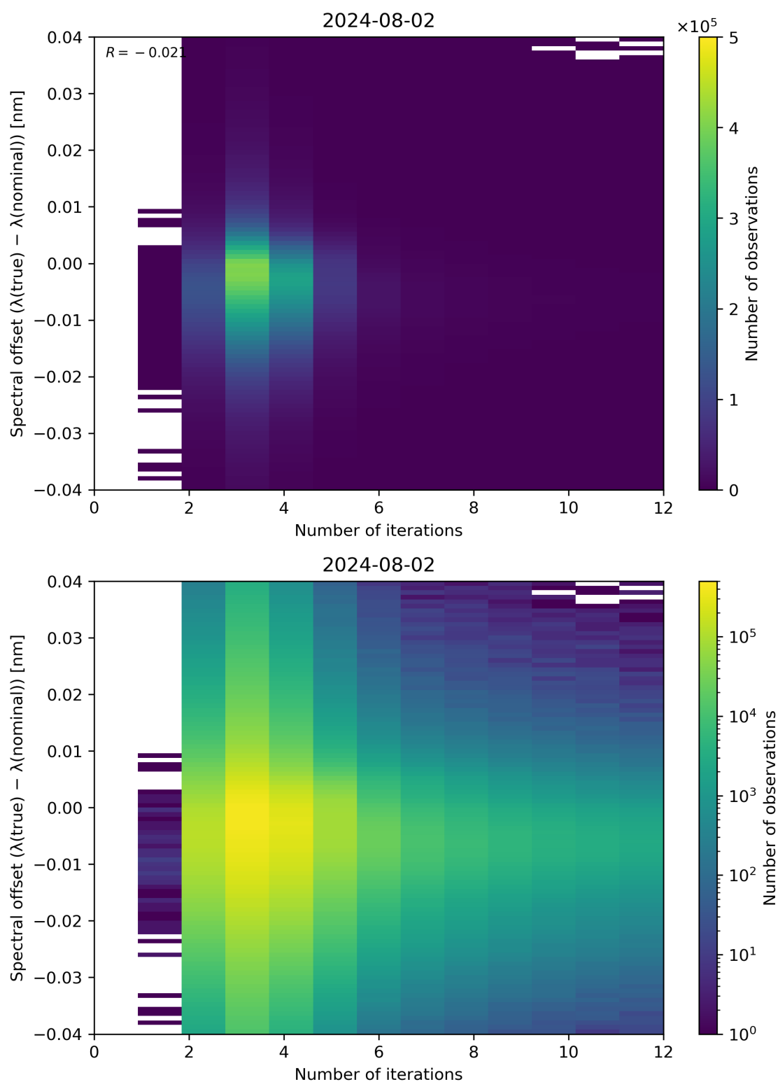
Figure 100: Scatter density plot of “Number of iterations” against “Spectral offset ( \lambda(\text{true}) - \lambda(\text{nominal}) )” for 2024-08-01 to 2024-08-03.
