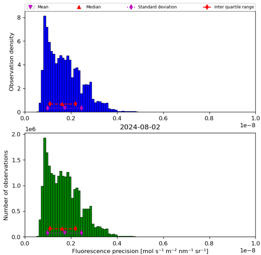
Figure 41: Histogram of “Fluorescence precision” for 2024-08-01 to 2024-08-03
