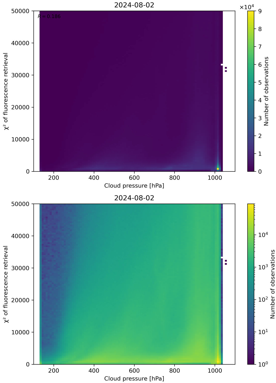
Figure 78: Scatter density plot of “Cloud pressure” against “ \chi^2 of fluorescence retrieval” for 2024-08-01 to 2024-08-03.
