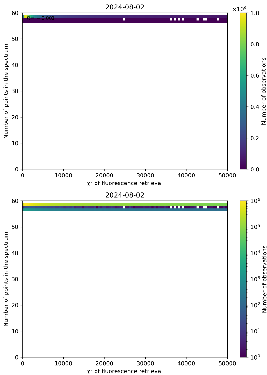
Figure 68: Scatter density plot of “ \chi^2 of fluorescence retrieval” against “Number of points in the spectrum” for 2024-08-01 to 2024-08-03.
