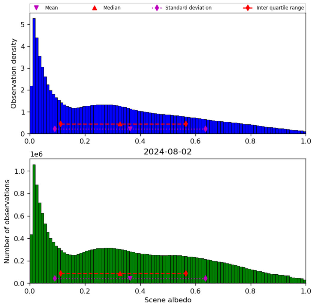
Figure 34: Histogram of “Scene albedo” for 2024-08-01 to 2024-08-03
