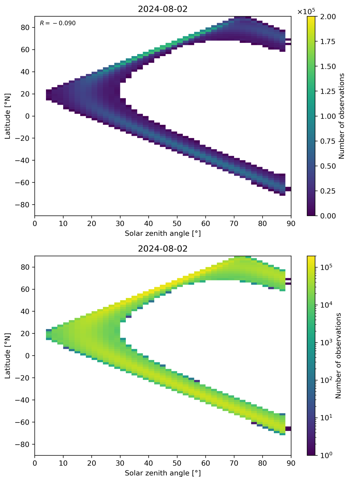
Figure 113: Scatter density plot of “Solar zenith angle” against “Latitude” for 2024-08-01 to 2024-08-03.
