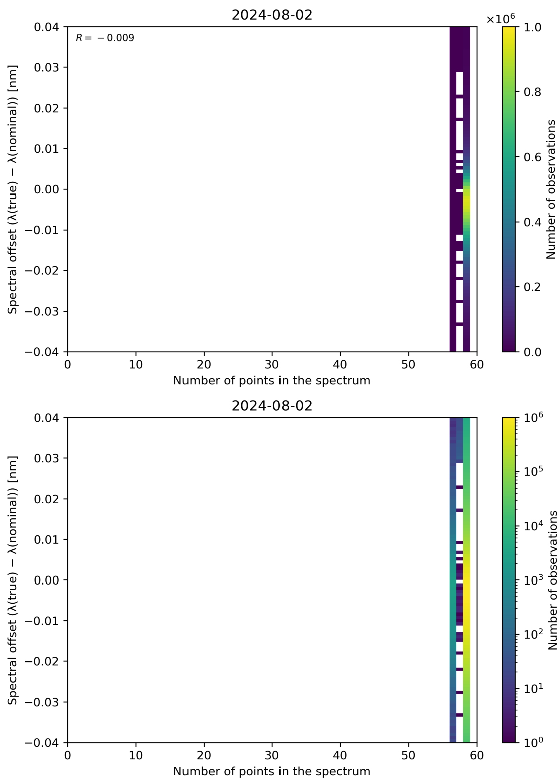
Figure 101: Scatter density plot of “Number of points in the spectrum” against “Spectral offset ( \lambda(\text{true}) - \lambda(\text{nominal}) )” for 2024-08-01 to 2024-08-03.
