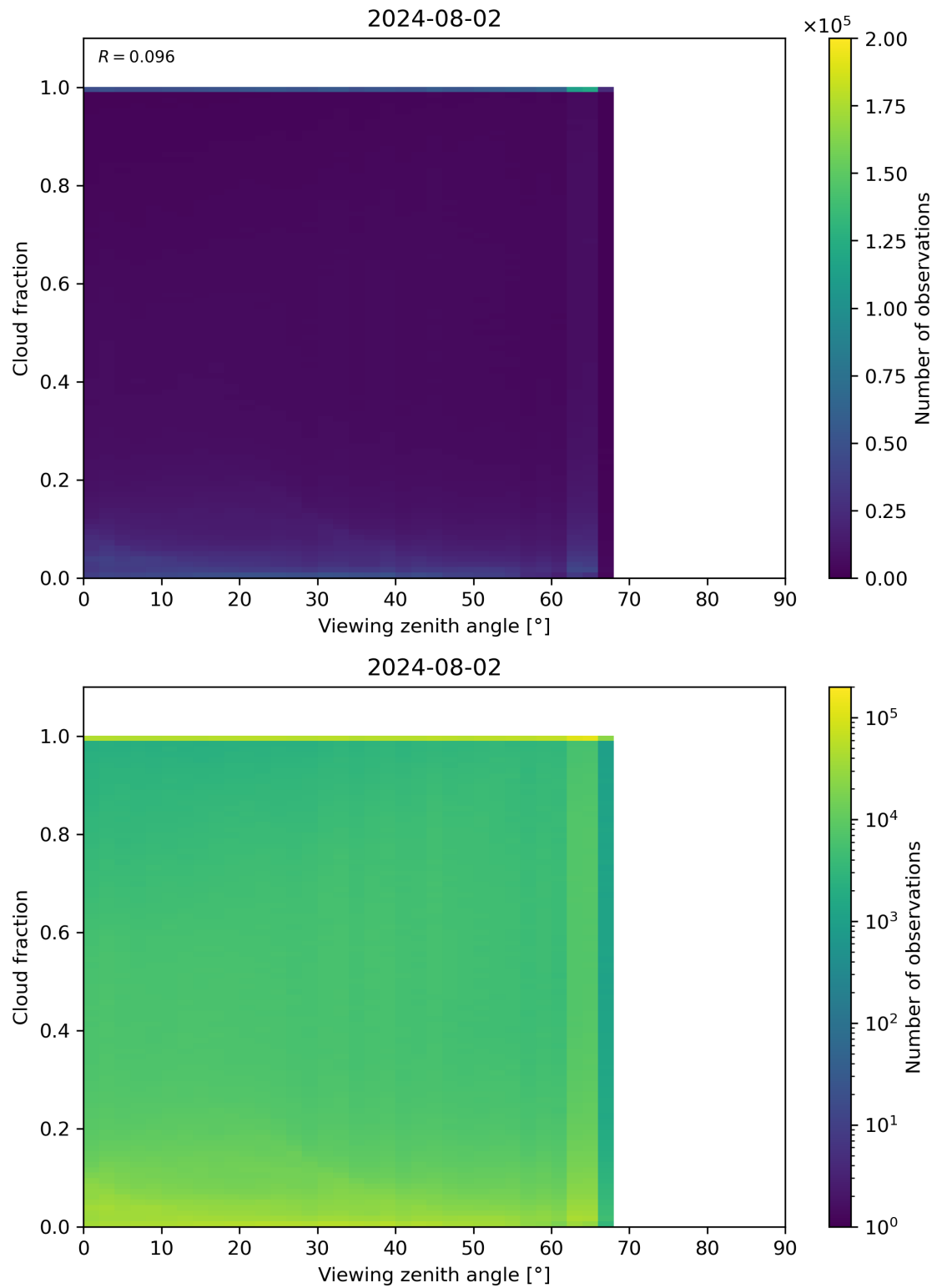
Figure 120: Scatter density plot of “Viewing zenith angle” against “Cloud fraction” for 2024-08-01 to 2024-08-03.
