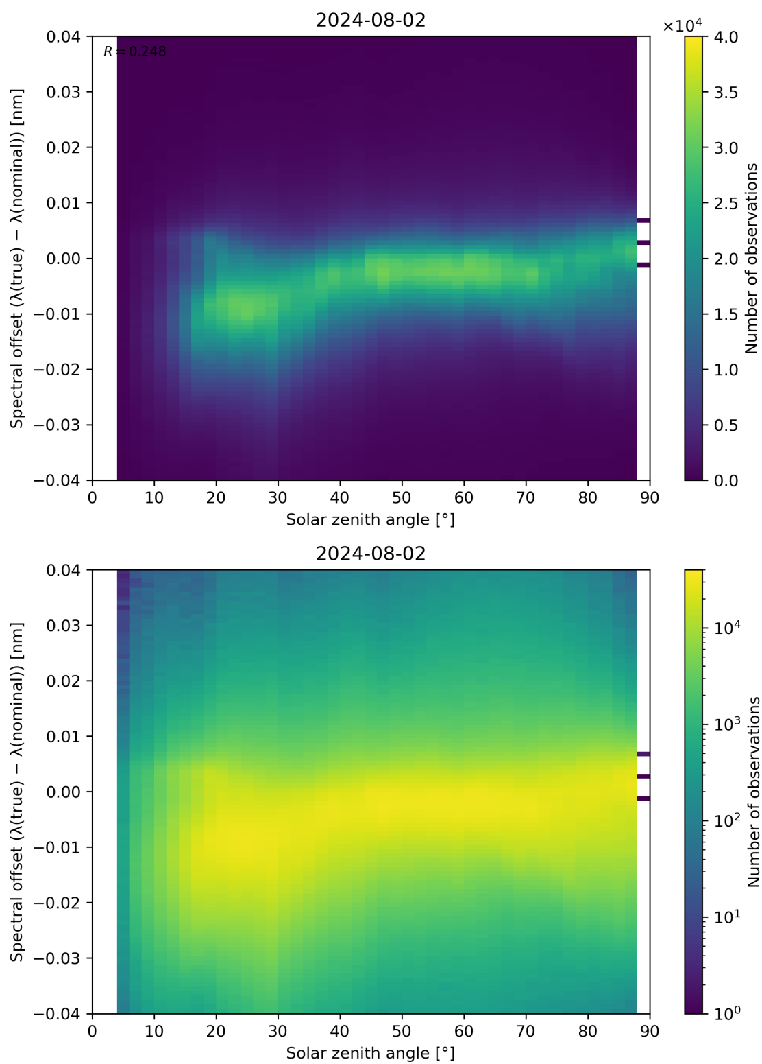
Figure 117: Scatter density plot of “Solar zenith angle” against “Spectral offset ( \lambda(\text{true}) - \lambda(\text{nominal}) )” for 2024-08-01 to 2024-08-03.
