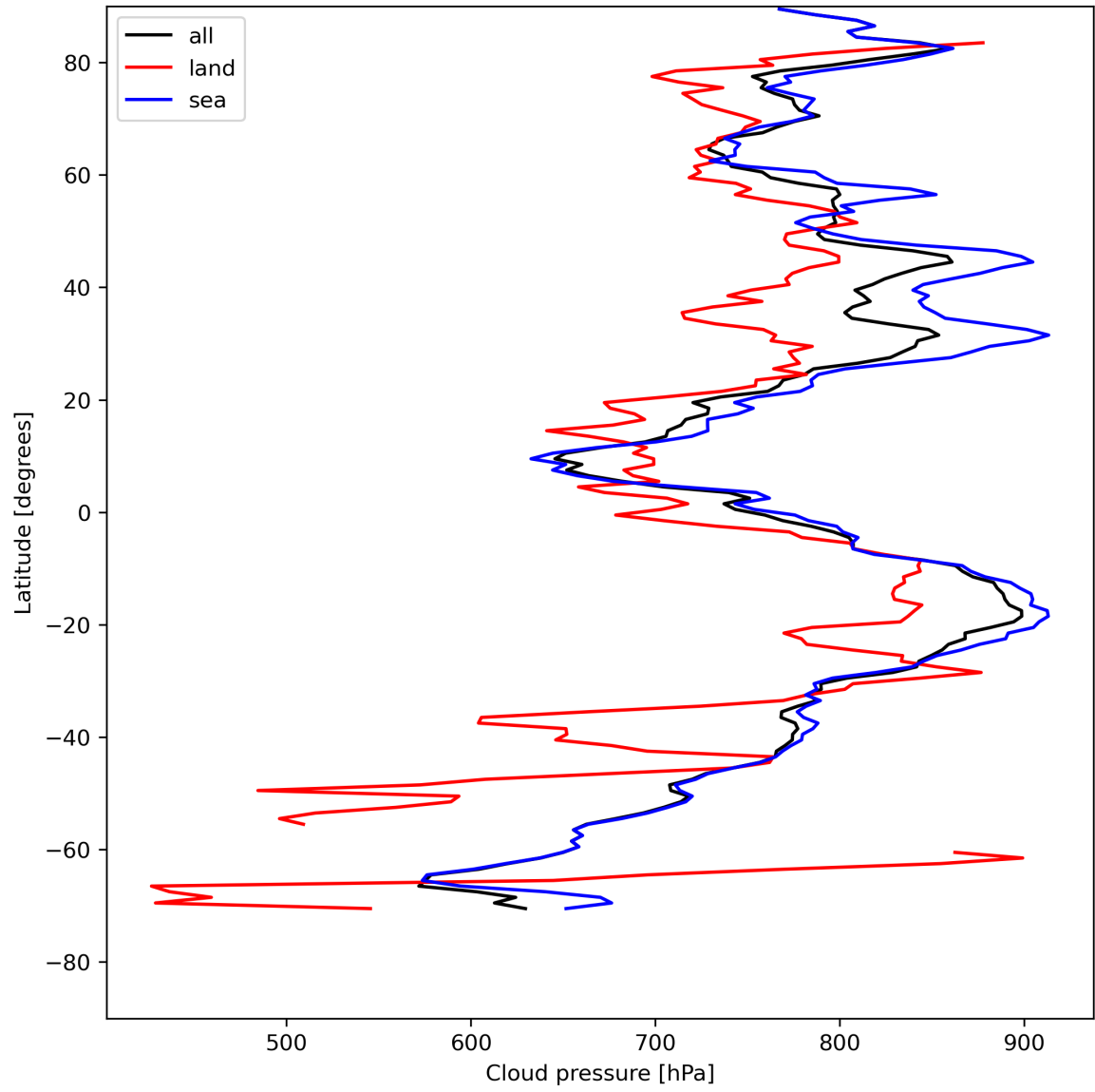
Figure 13: Zonal average of “Cloud pressure” for 2024-08-01 to 2024-08-03.
