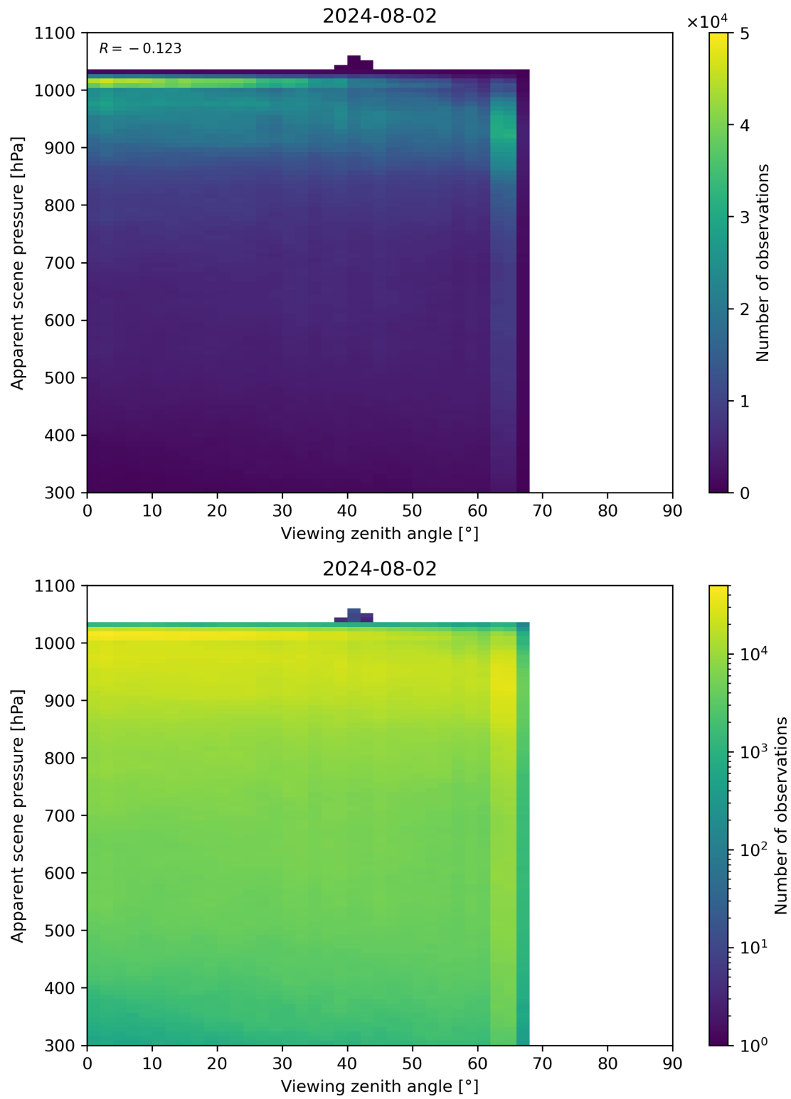
Figure 118: Scatter density plot of “Viewing zenith angle” against “Apparent scene pressure” for 2024-08-01 to 2024-08-03.
