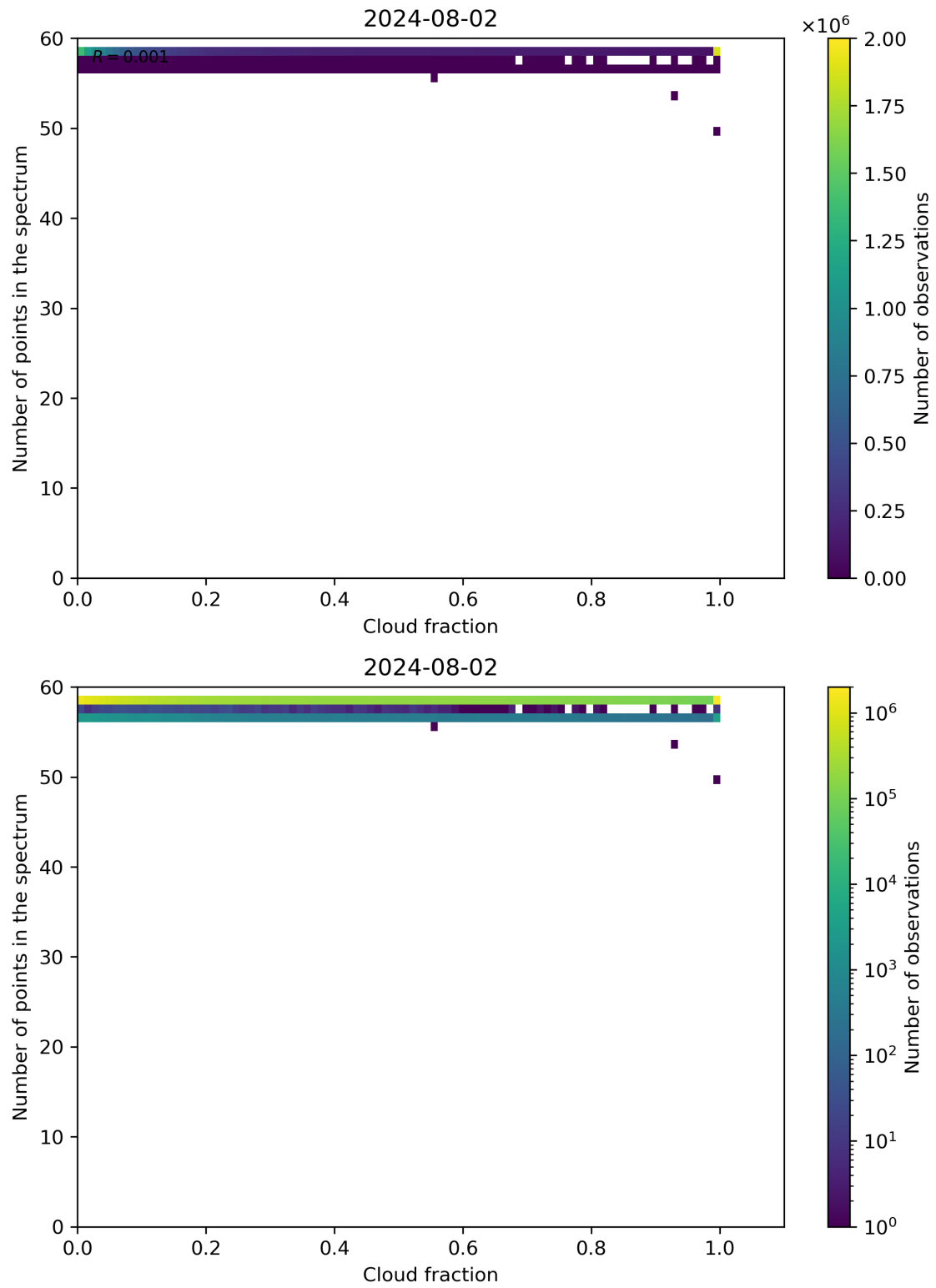
Figure 74: Scatter density plot of “Cloud fraction” against “Number of points in the spectrum” for 2024-08-01 to 2024-08-03.
