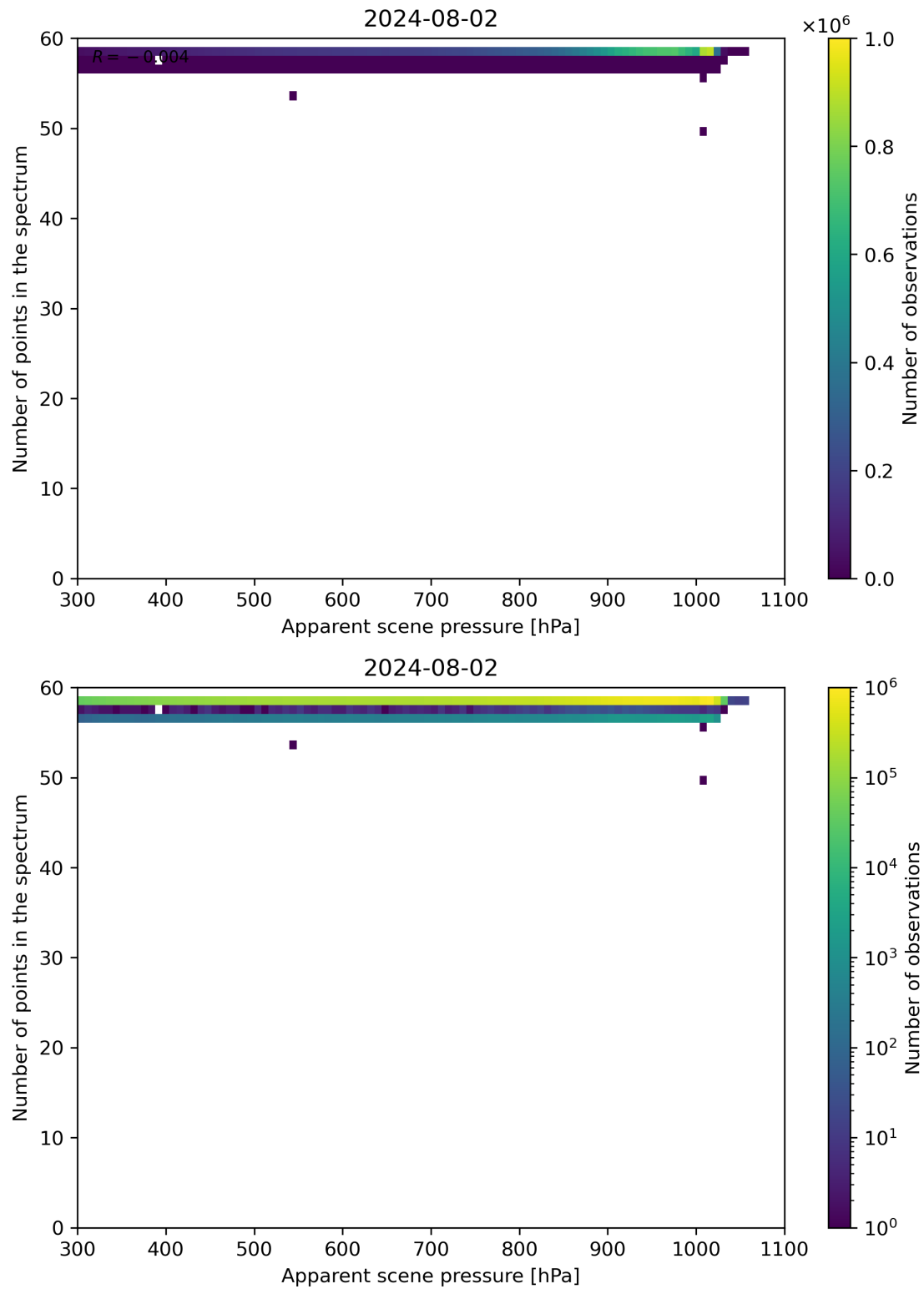
Figure 66: Scatter density plot of “Apparent scene pressure” against “Number of points in the spectrum” for 2024-08-01 to 2024-08-03.
