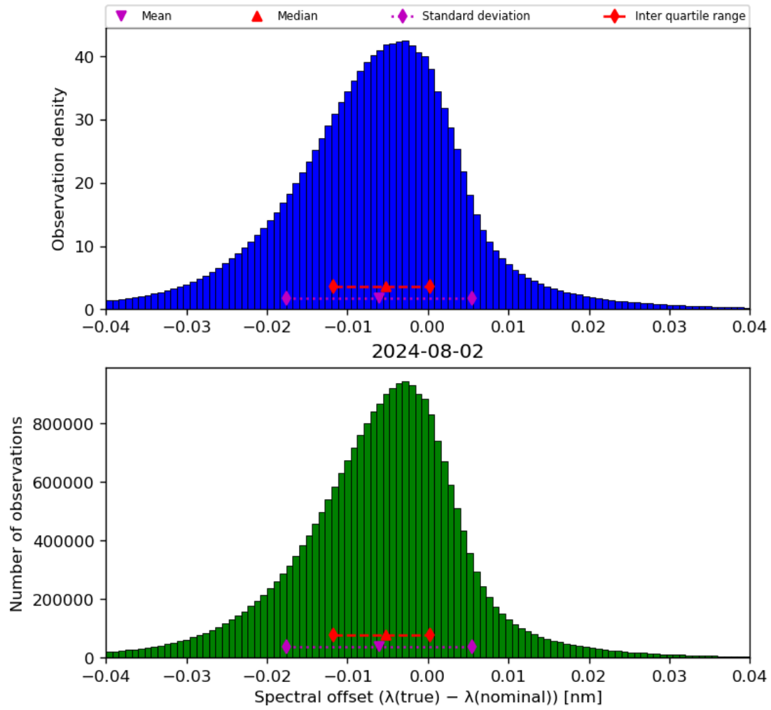
Figure 45: Histogram of “Spectral offset ( \lambda(\text{true}) - \lambda(\text{nominal}) )” for 2024-08-01 to 2024-08-03
