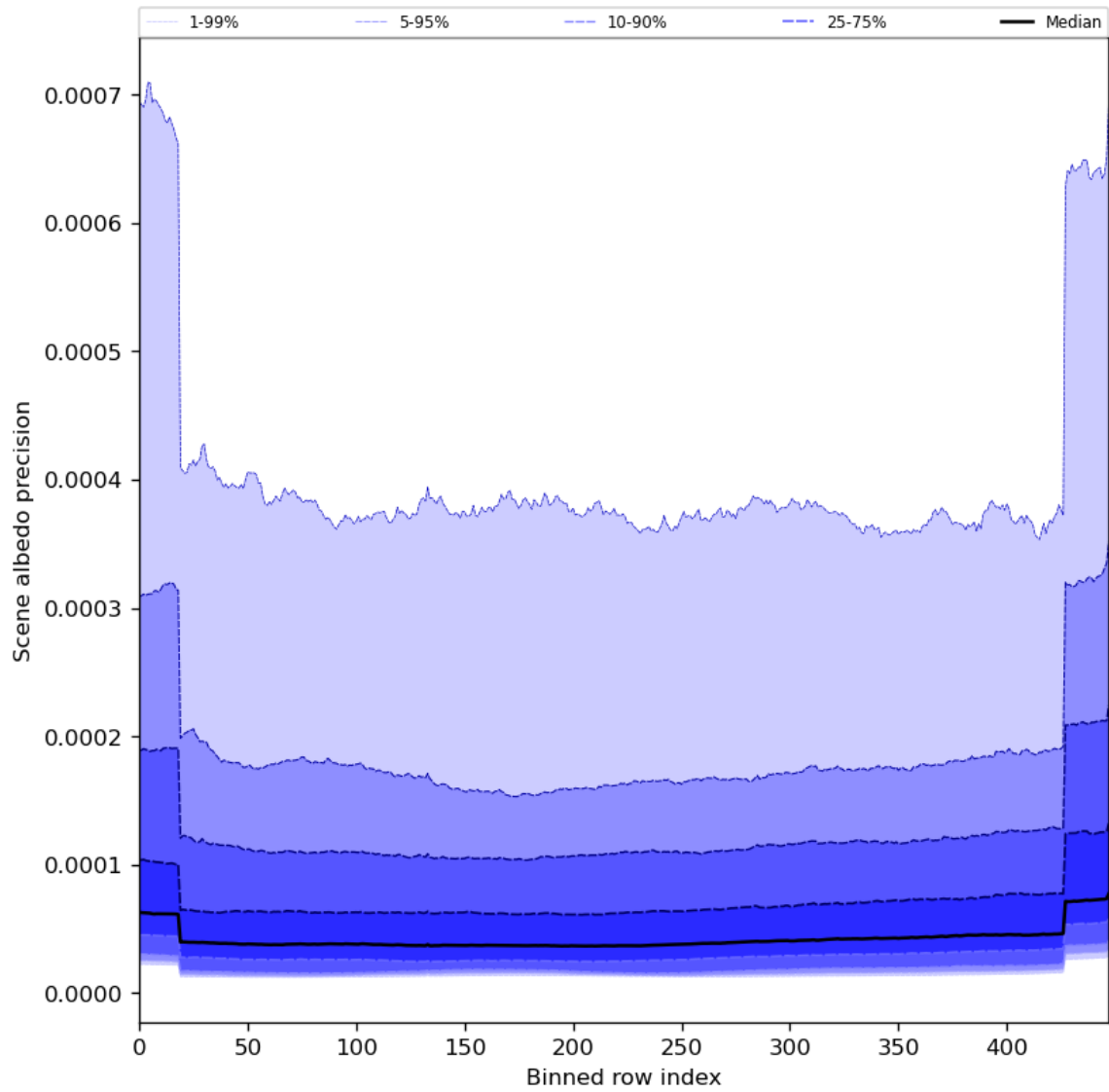
Figure 52: Along track statistics of “Scene albedo precision” for 2024-08-01 to 2024-08-03
