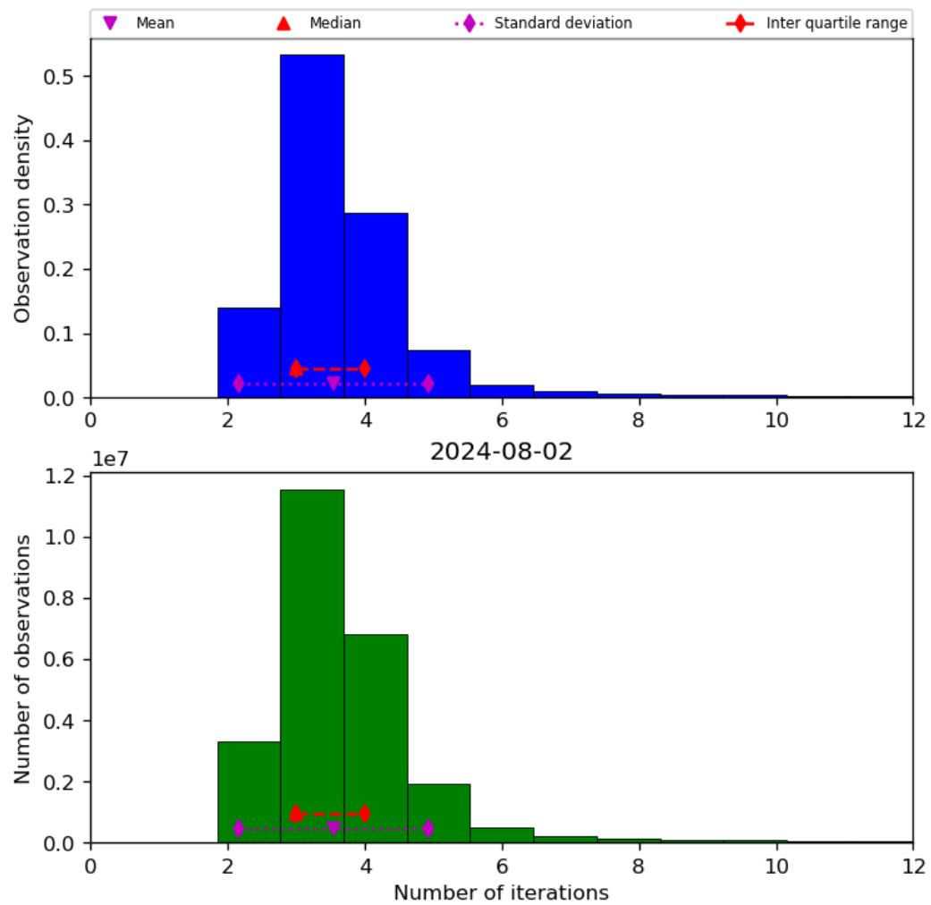
Figure 39: Histogram of “Number of iterations” for 2024-08-01 to 2024-08-03
