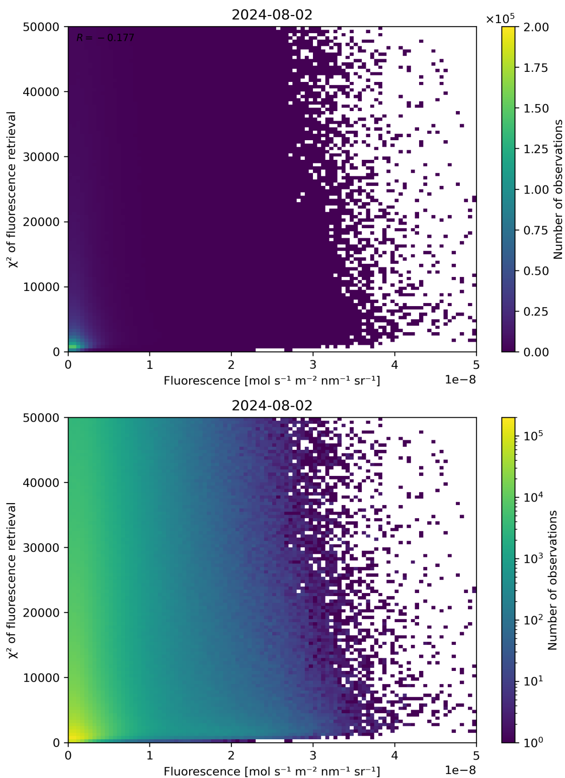
Figure 85: Scatter density plot of “Fluorescence” against “ \chi^2 of fluorescence retrieval” for 2024-08-01 to 2024-08-03.
