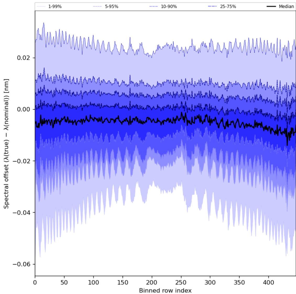
Figure 62: Along track statistics of “Spectral offset ( \lambda(\text{true}) - \lambda(\text{nominal}) )” for 2024-08-01 to 2024-08-03
