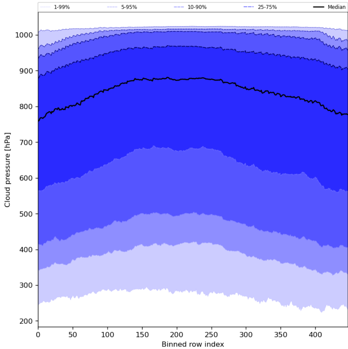
Figure 47: Along track statistics of “Cloud pressure” for 2024-08-01 to 2024-08-03
