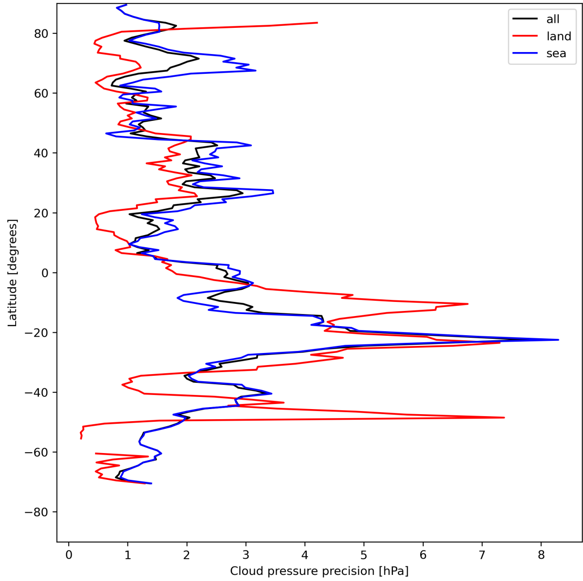
Figure 14: Zonal average of “Cloud pressure precision” for 2024-08-01 to 2024-08-03.
