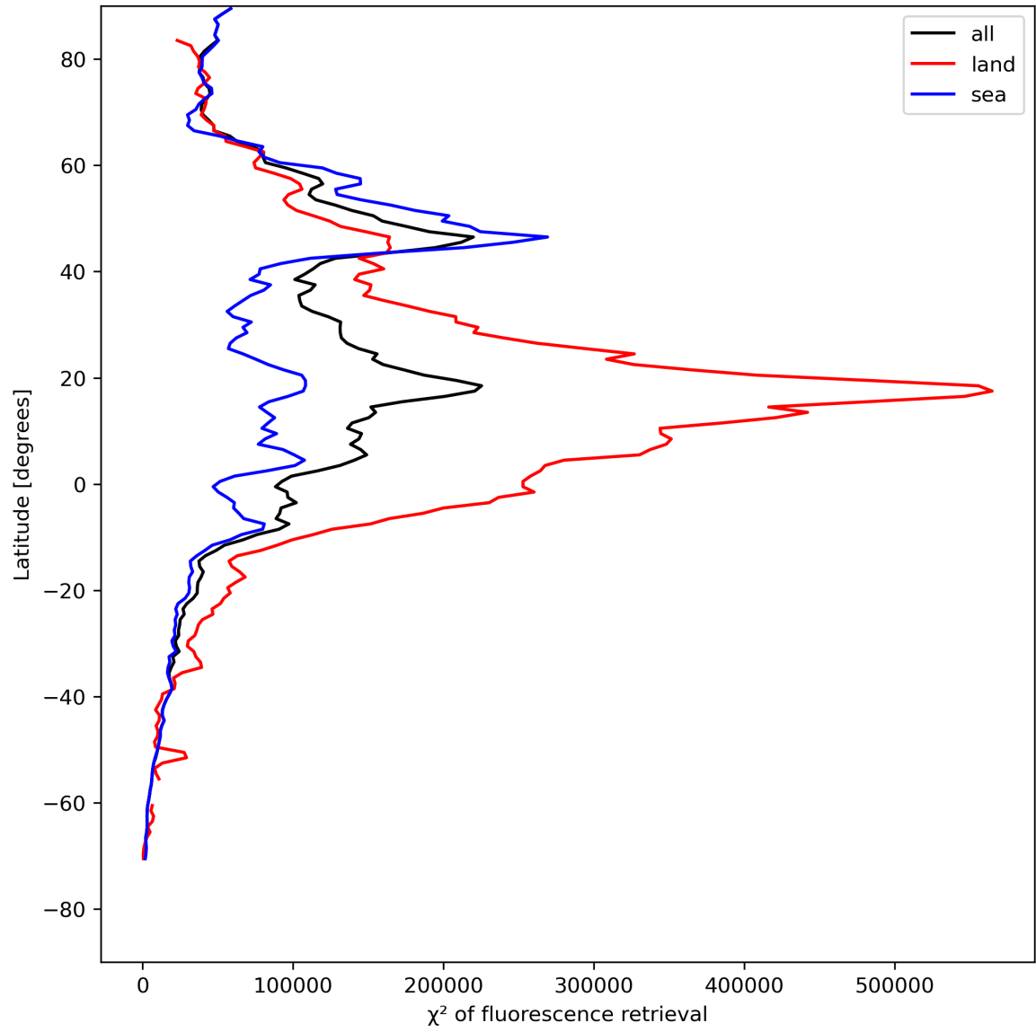
Figure 25: Zonal average of “ \chi^2 of fluorescence retrieval” for 2024-08-01 to 2024-08-03.
