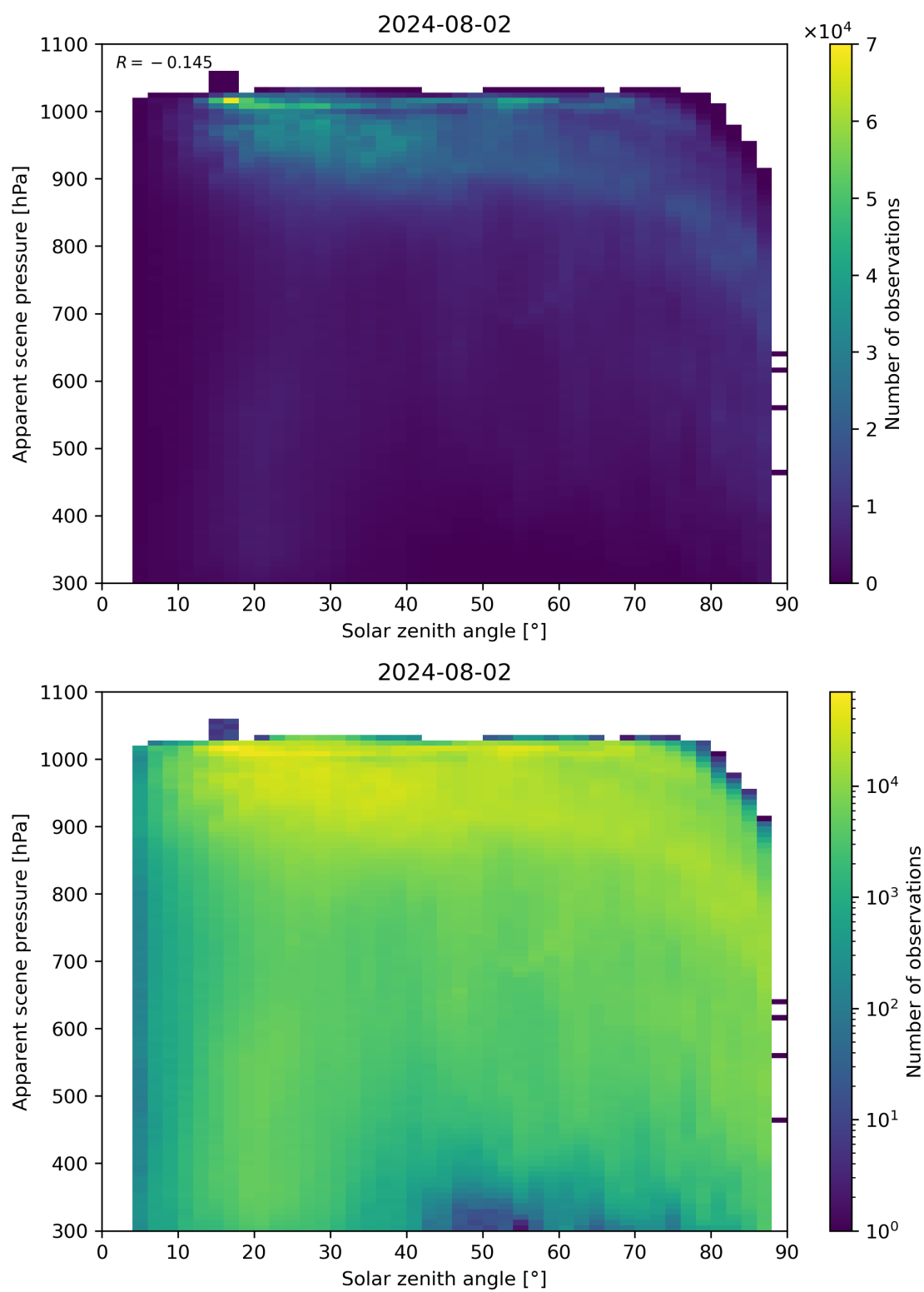
Figure 108: Scatter density plot of “Solar zenith angle” against “Apparent scene pressure” for 2024-08-01 to 2024-08-03.
