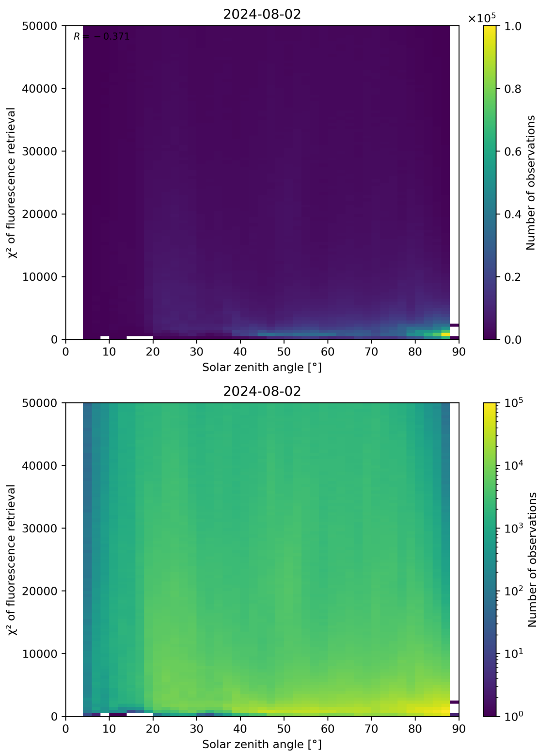
Figure 109: Scatter density plot of “Solar zenith angle” against “ \chi^2 of fluorescence retrieval” for 2024-08-01 to 2024-08-03.
