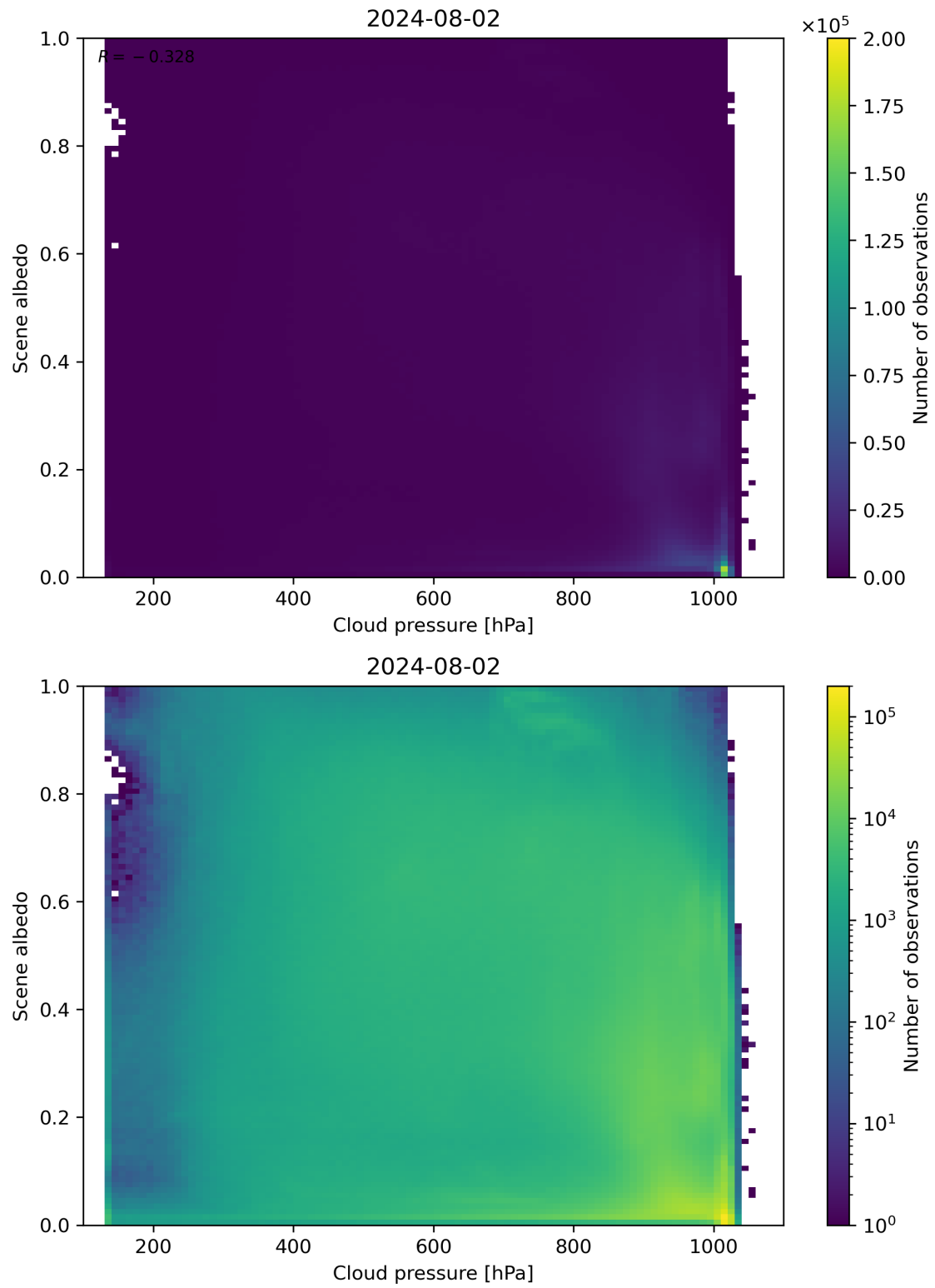
Figure 83: Scatter density plot of “Cloud pressure” against “Scene albedo” for 2024-08-01 to 2024-08-03.
