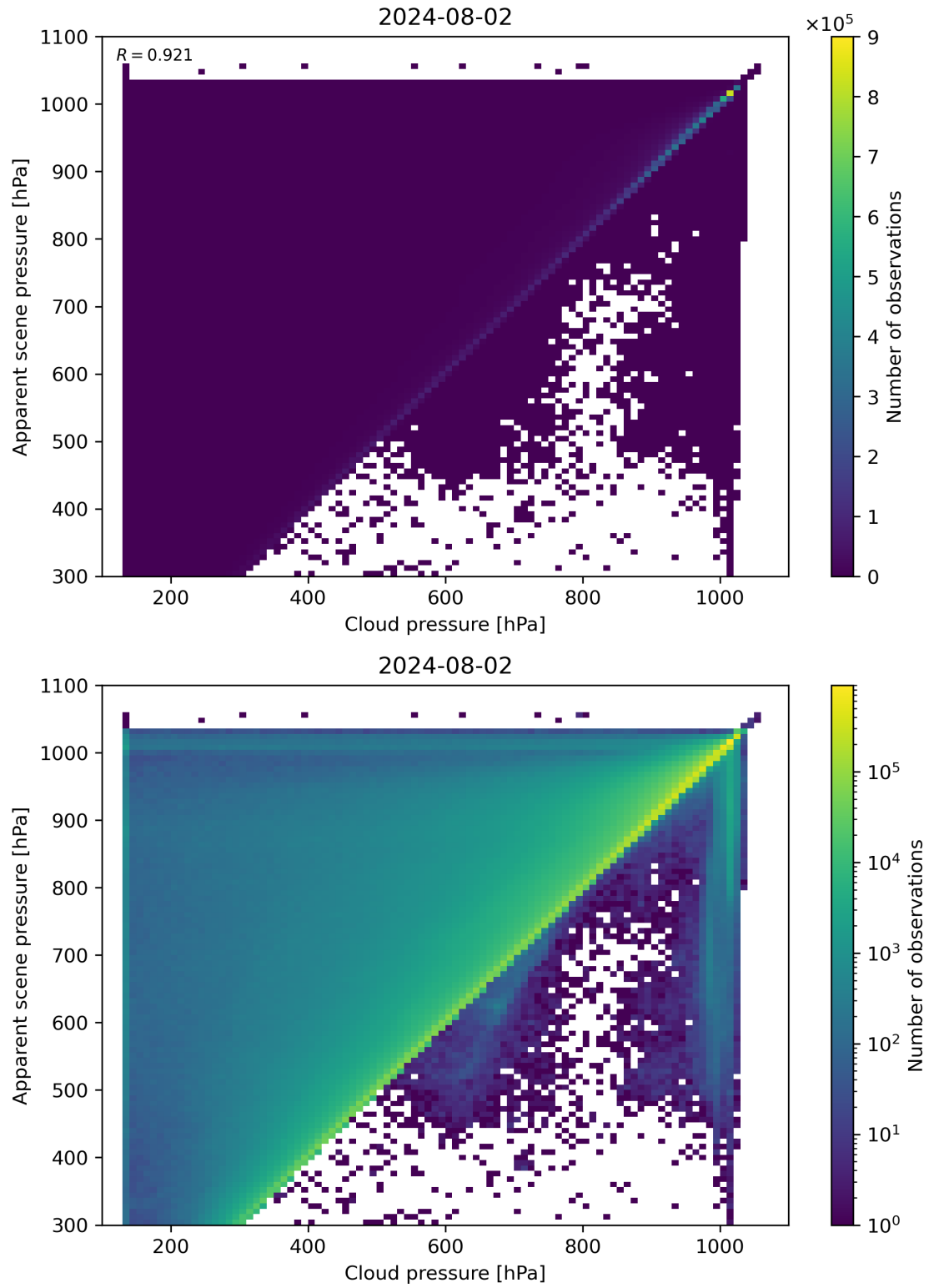
Figure 77: Scatter density plot of “Cloud pressure” against “Apparent scene pressure” for 2024-08-01 to 2024-08-03.
