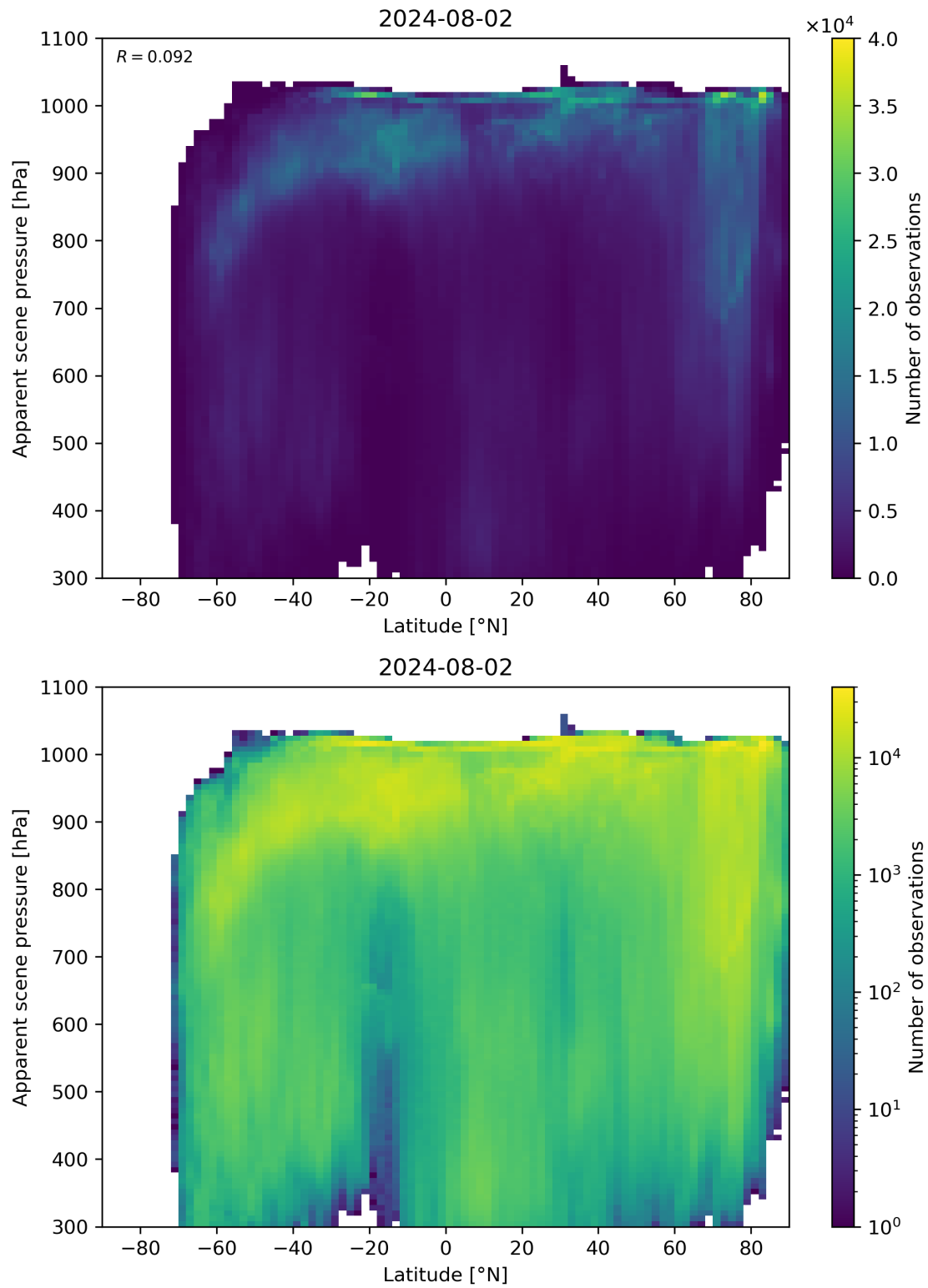
Figure 88: Scatter density plot of “Latitude” against “Apparent scene pressure” for 2024-08-01 to 2024-08-03.
