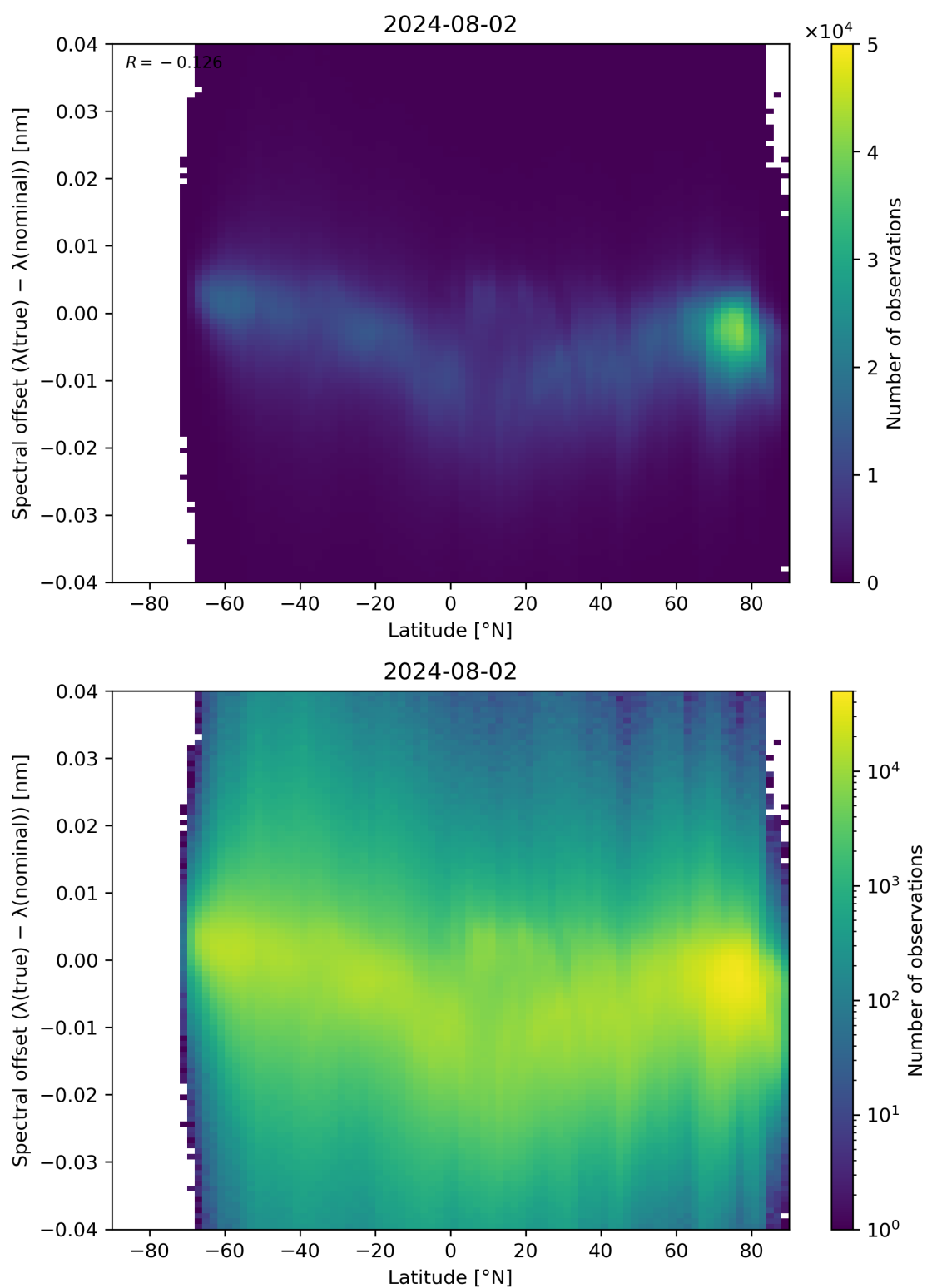
Figure 96: Scatter density plot of “Latitude” against “Spectral offset ( \lambda(\text{true}) - \lambda(\text{nominal}) )” for 2024-08-01 to 2024-08-03.
