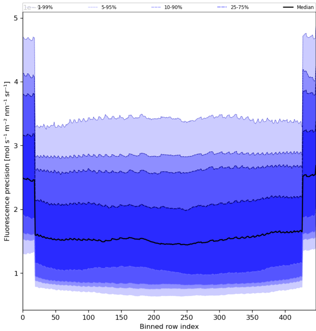
Figure 58: Along track statistics of “Fluorescence precision” for 2024-08-01 to 2024-08-03
