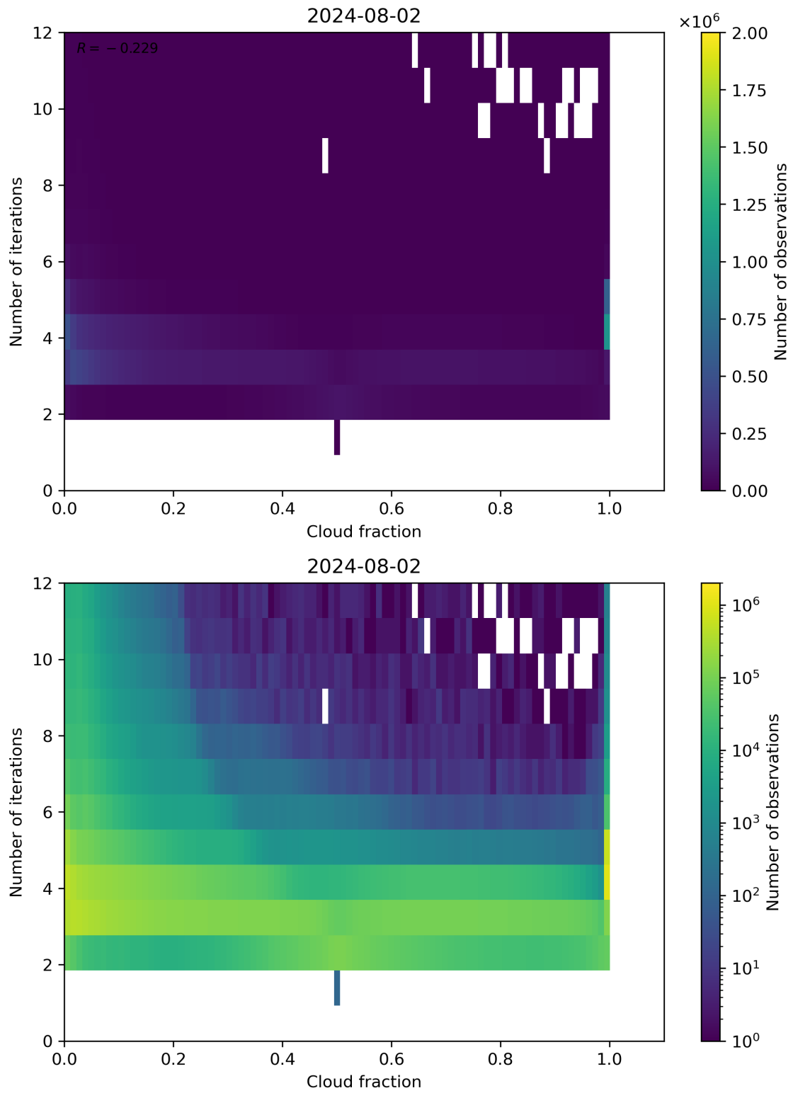
Figure 73: Scatter density plot of “Cloud fraction” against “Number of iterations” for 2024-08-01 to 2024-08-03.
