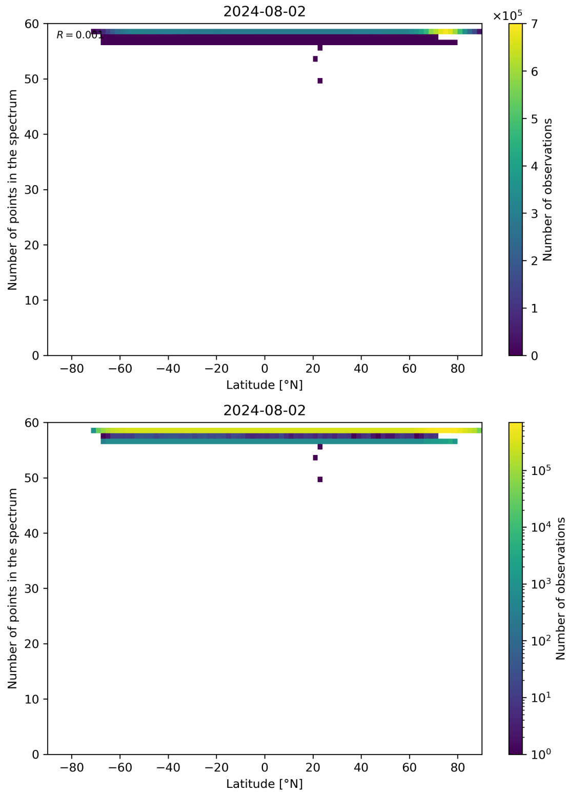
Figure 94: Scatter density plot of “Latitude” against “Number of points in the spectrum” for 2024-08-01 to 2024-08-03.
