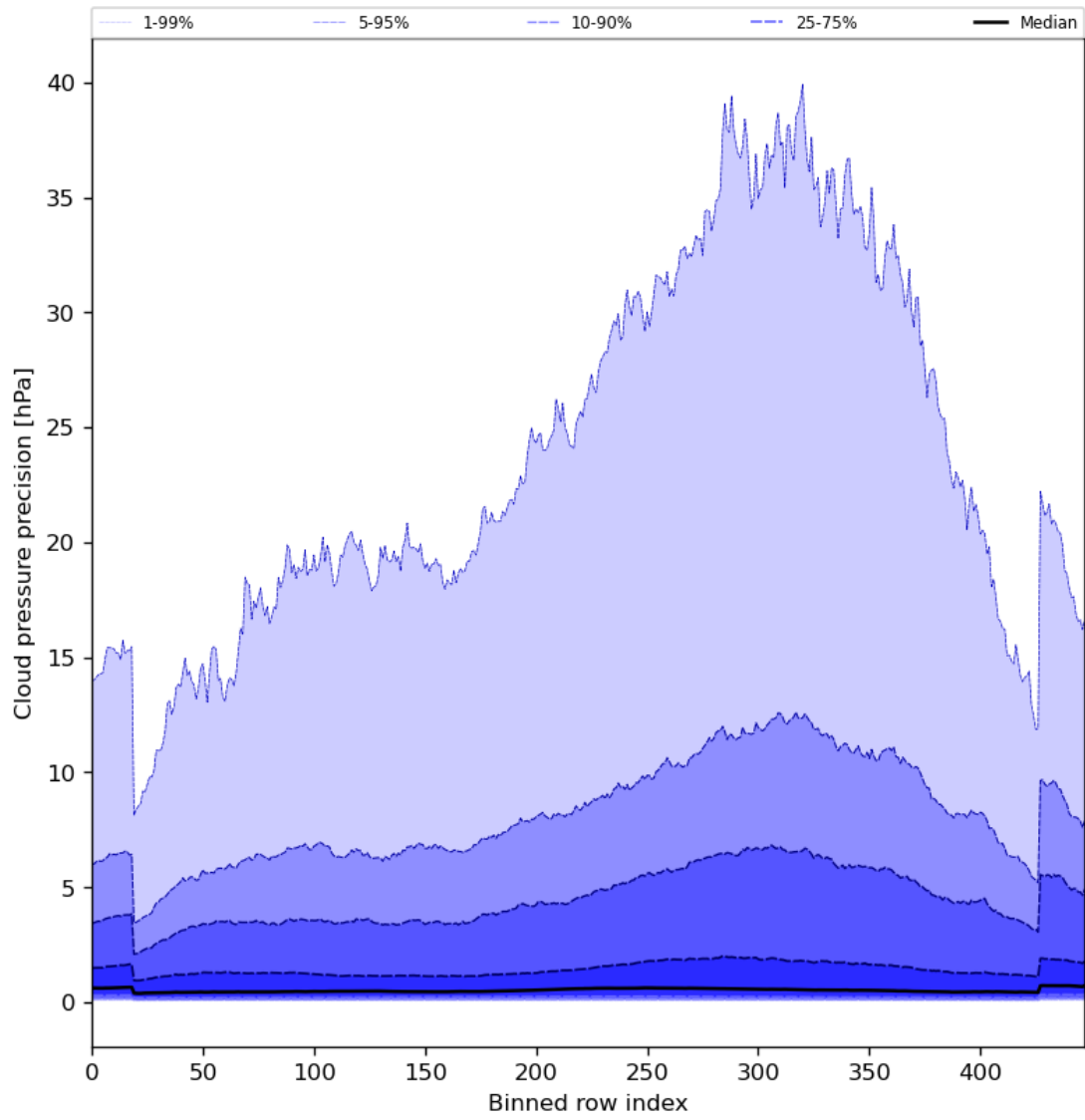
Figure 48: Along track statistics of “Cloud pressure precision” for 2024-08-01 to 2024-08-03
