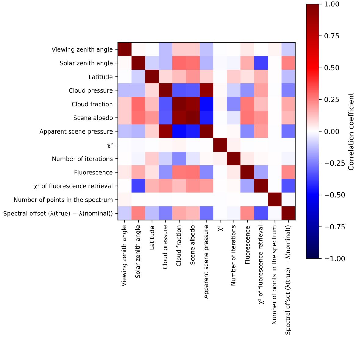
Figure 2: Map of correlation matrix for 2024-08-01 to 2024-08-03.
