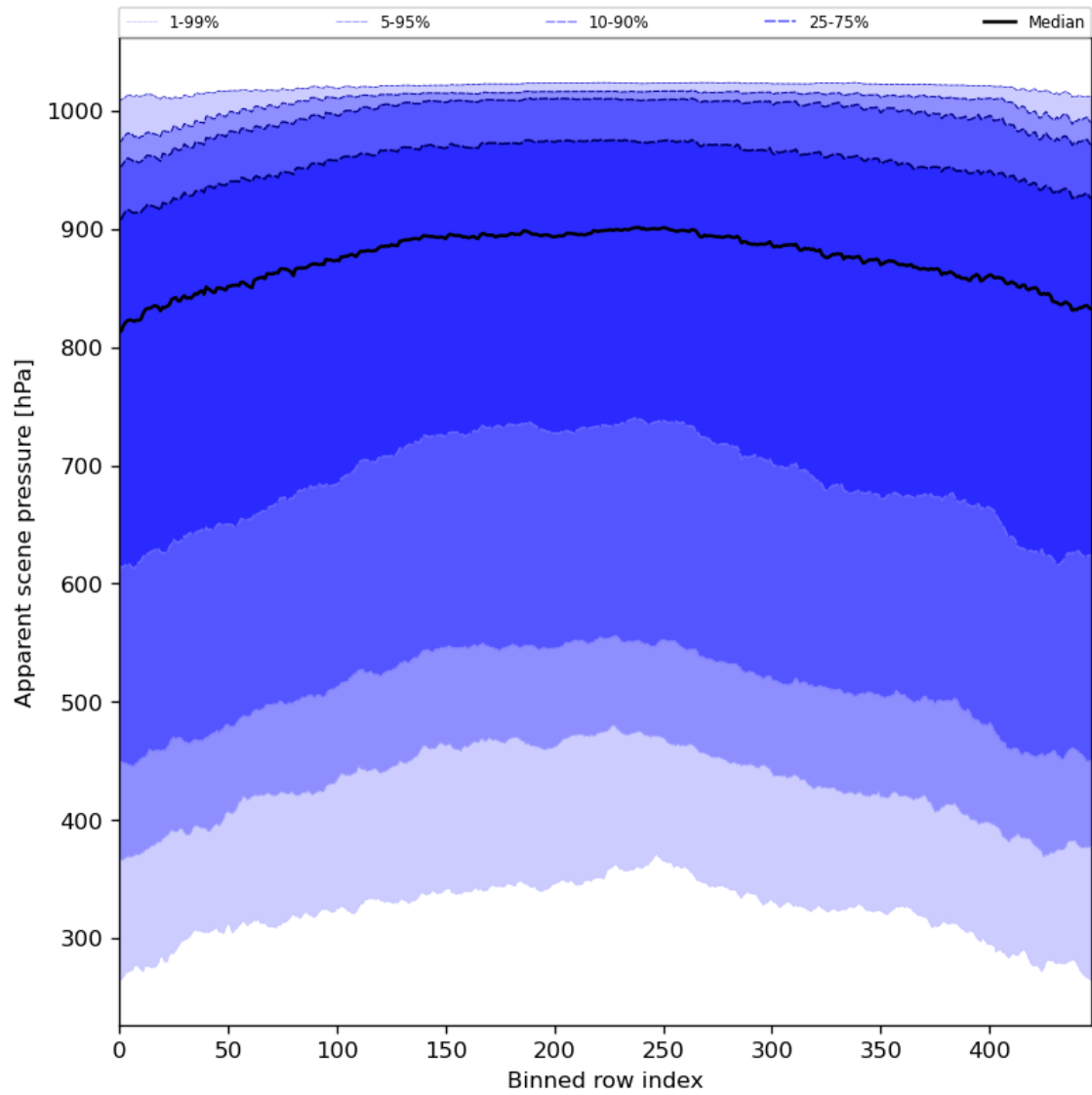
Figure 53: Along track statistics of “Apparent scene pressure” for 2024-08-01 to 2024-08-03
