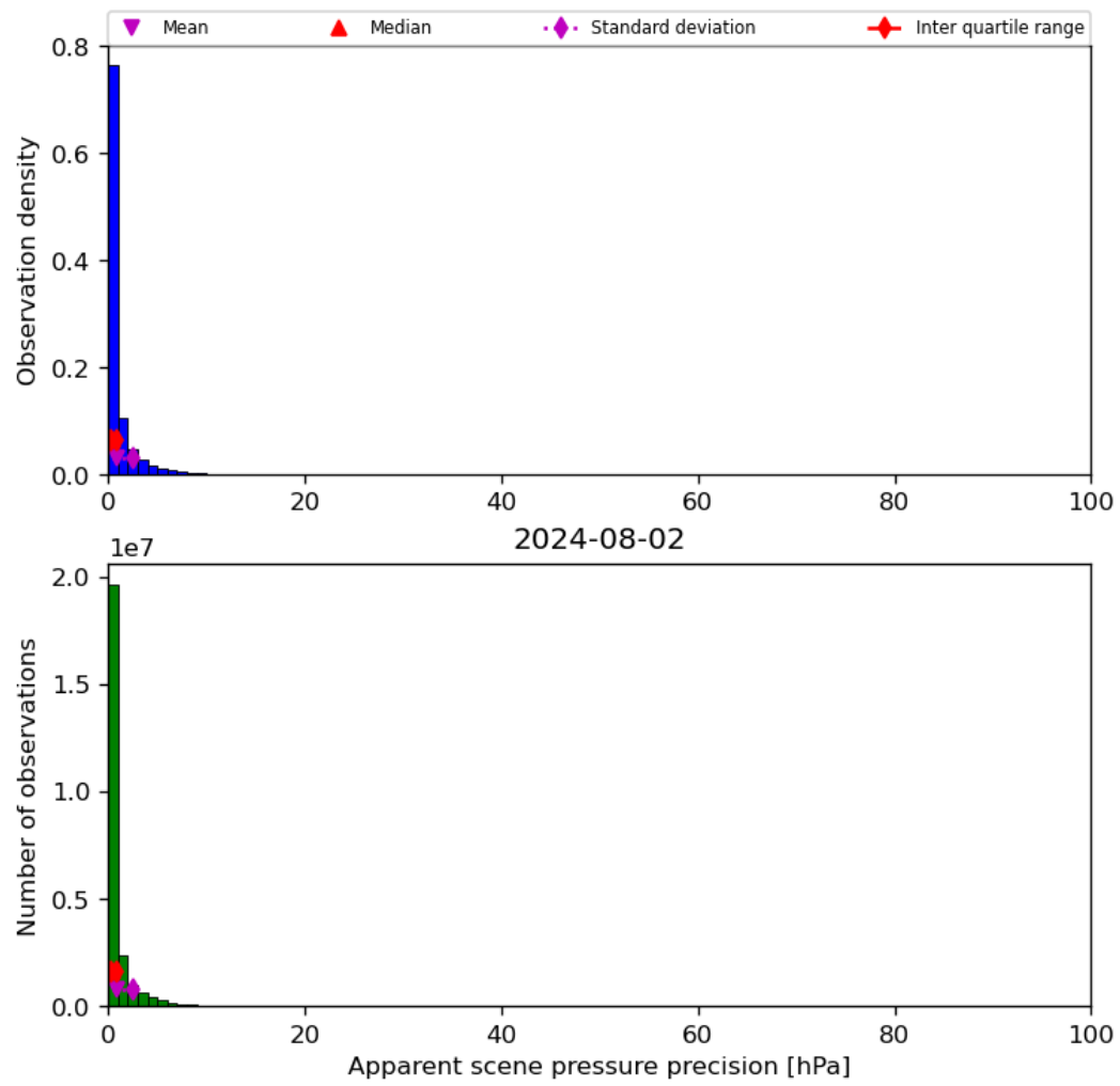
Figure 37: Histogram of “Apparent scene pressure precision” for 2024-08-01 to 2024-08-03
