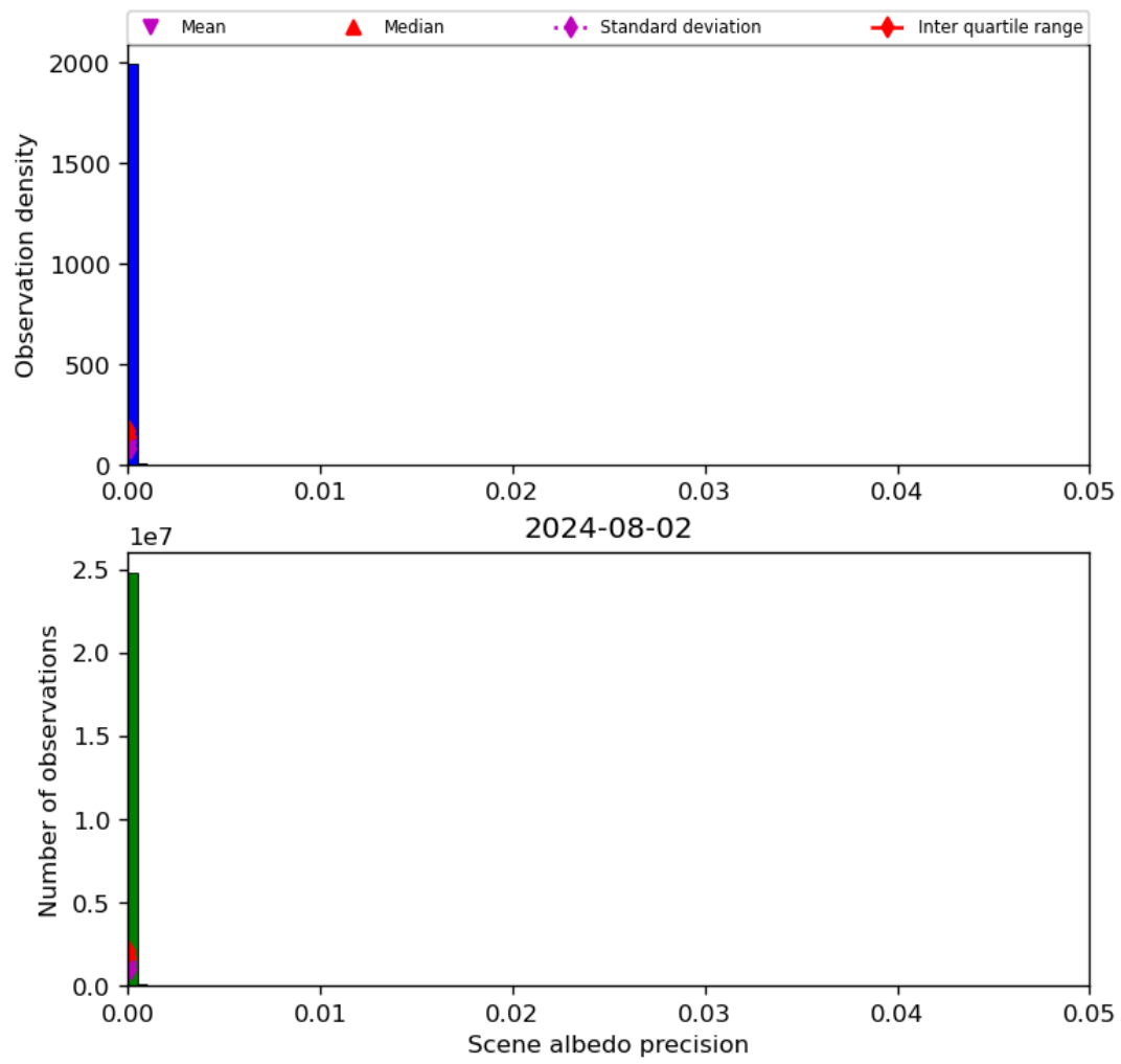
Figure 35: Histogram of “Scene albedo precision” for 2024-08-01 to 2024-08-03
