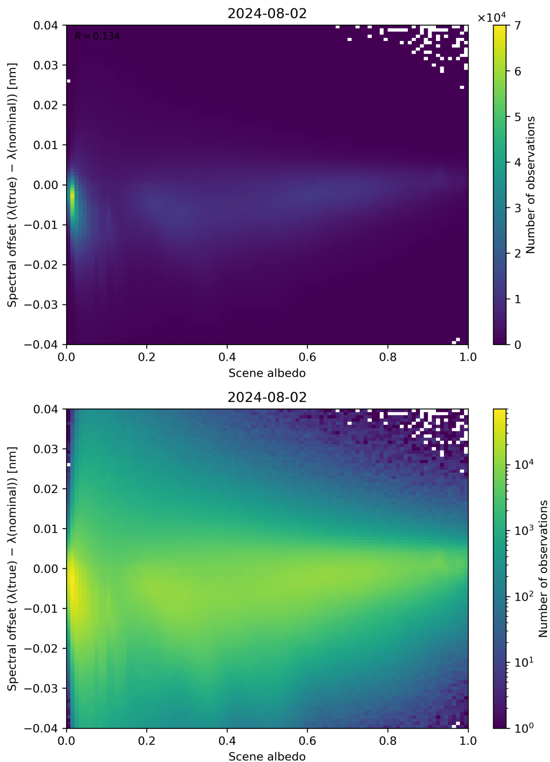
Figure 107: Scatter density plot of “Scene albedo” against “Spectral offset ( \lambda(\text{true}) - \lambda(\text{nominal}) )” for 2024-08-01 to 2024-08-03.
