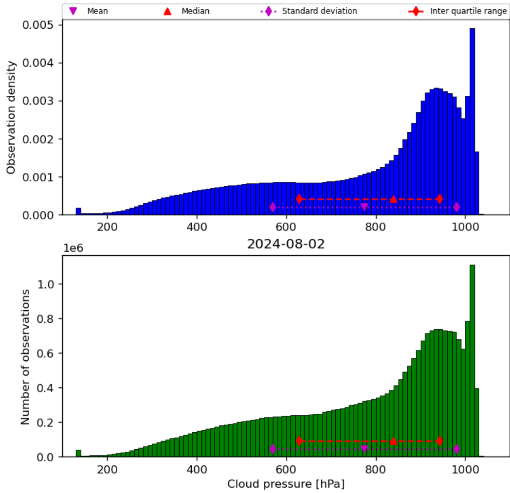
Figure 30: Histogram of “Cloud pressure” for 2024-08-01 to 2024-08-03
