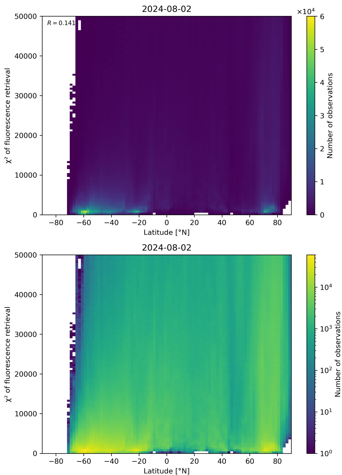
Figure 89: Scatter density plot of “Latitude” against “ \chi^2 of fluorescence retrieval” for 2024-08-01 to 2024-08-03.
