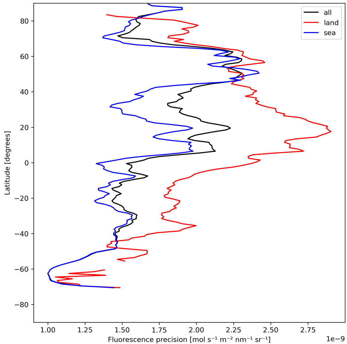
Figure 24: Zonal average of “Fluorescence precision” for 2024-08-01 to 2024-08-03.
