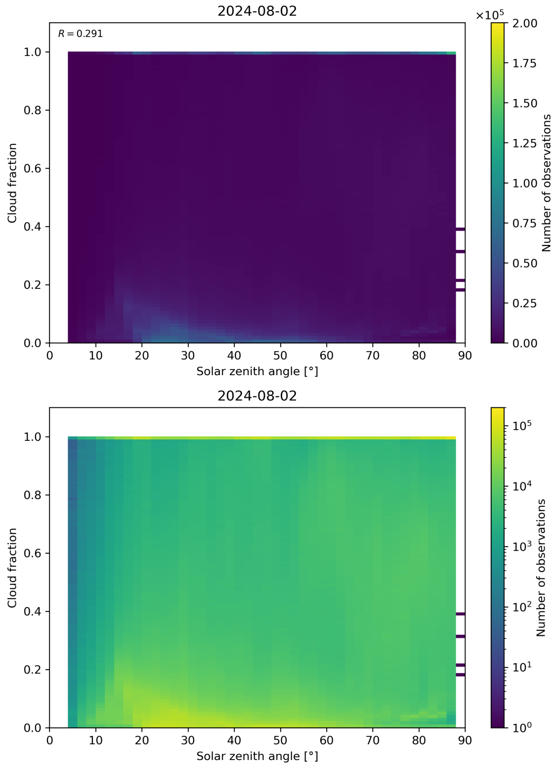
Figure 110: Scatter density plot of “Solar zenith angle” against “Cloud fraction” for 2024-08-01 to 2024-08-03.
