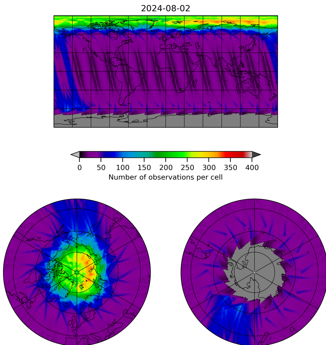
Figure 11: Map of the number of observations for 2024-08-01 to 2024-08-03
