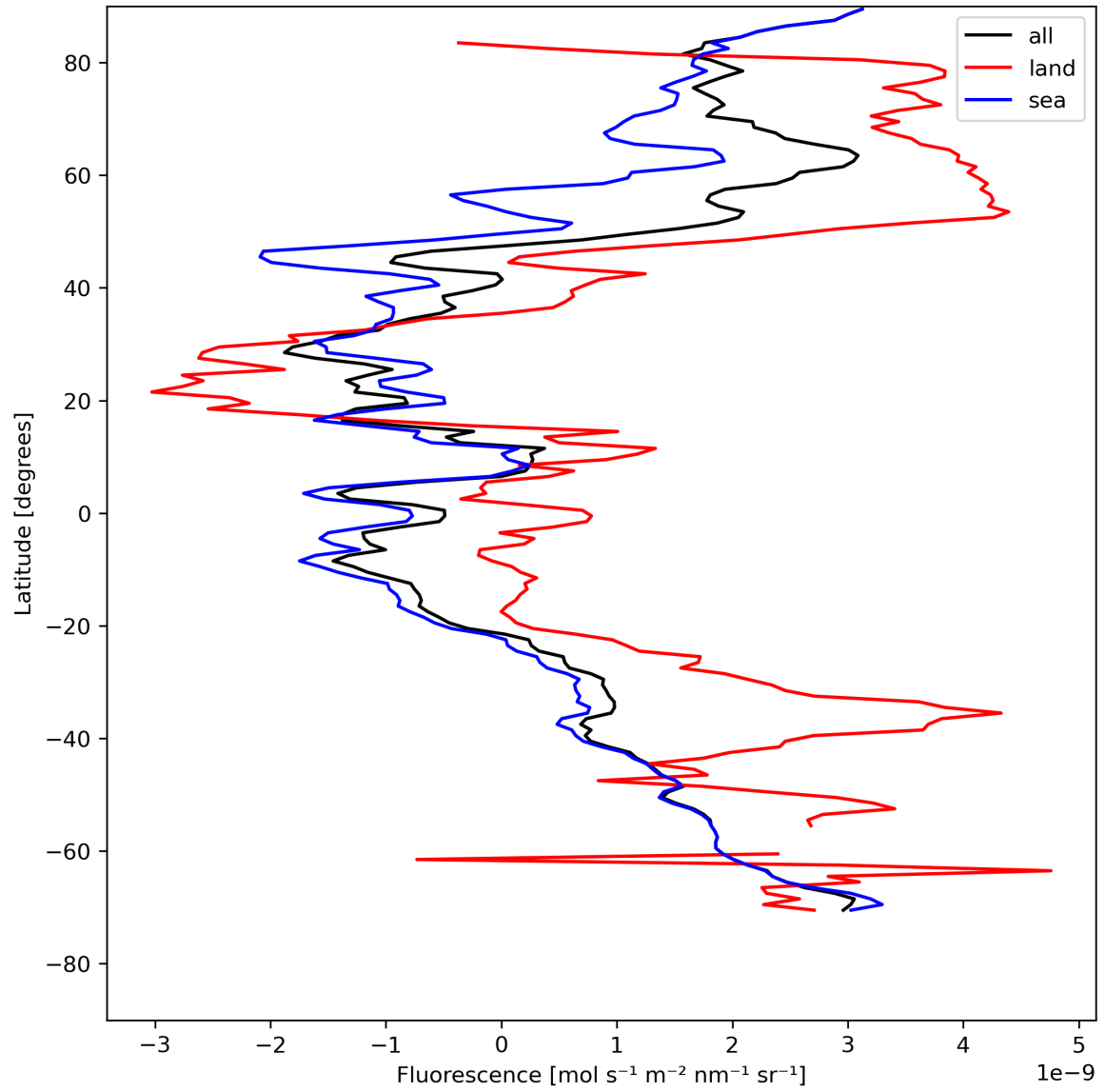
Figure 23: Zonal average of “Fluorescence” for 2024-08-01 to 2024-08-03.
