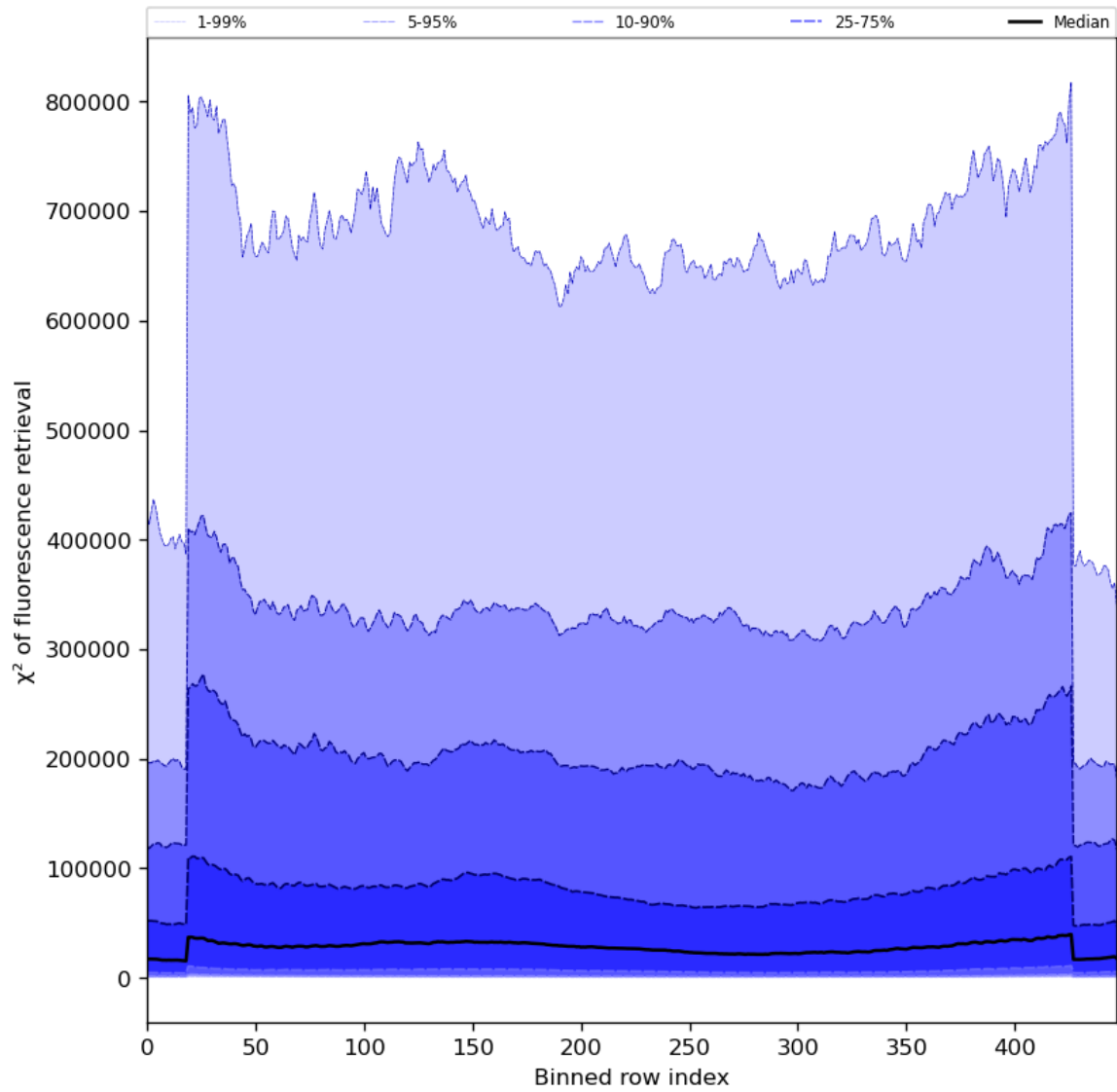
Figure 59: Along track statistics of “ \chi^2 of fluorescence retrieval” for 2024-08-01 to 2024-08-03
