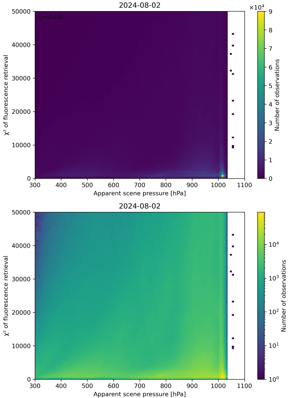
Figure 63: Scatter density plot of “Apparent scene pressure” against “ \chi^2 of fluorescence retrieval” for 2024-08-01 to 2024-08-03.
