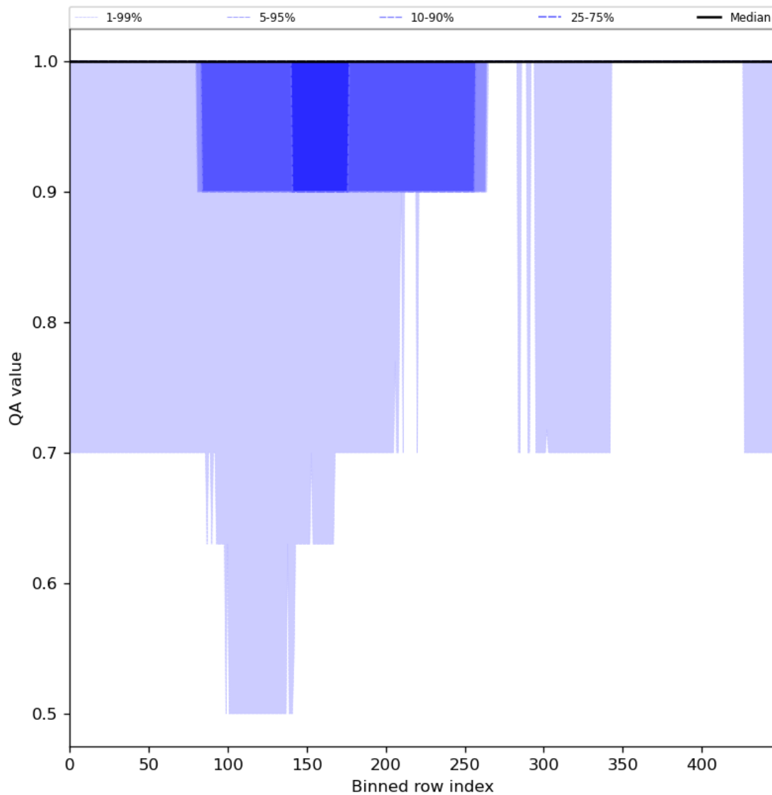
Figure 46: Along track statistics of “QA value” for 2024-08-01 to 2024-08-03
