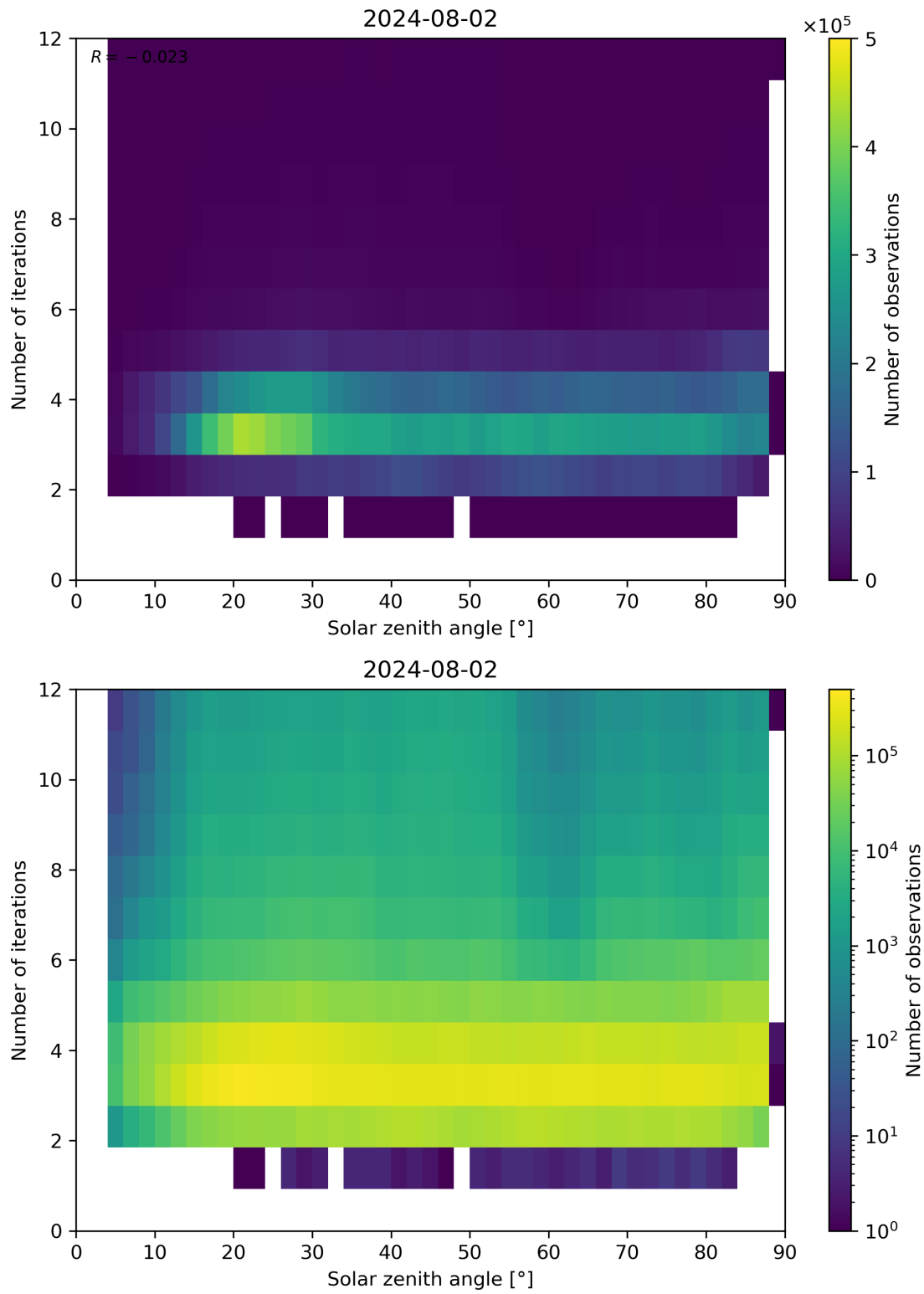
Figure 114: Scatter density plot of “Solar zenith angle” against “Number of iterations” for 2024-08-01 to 2024-08-03.
