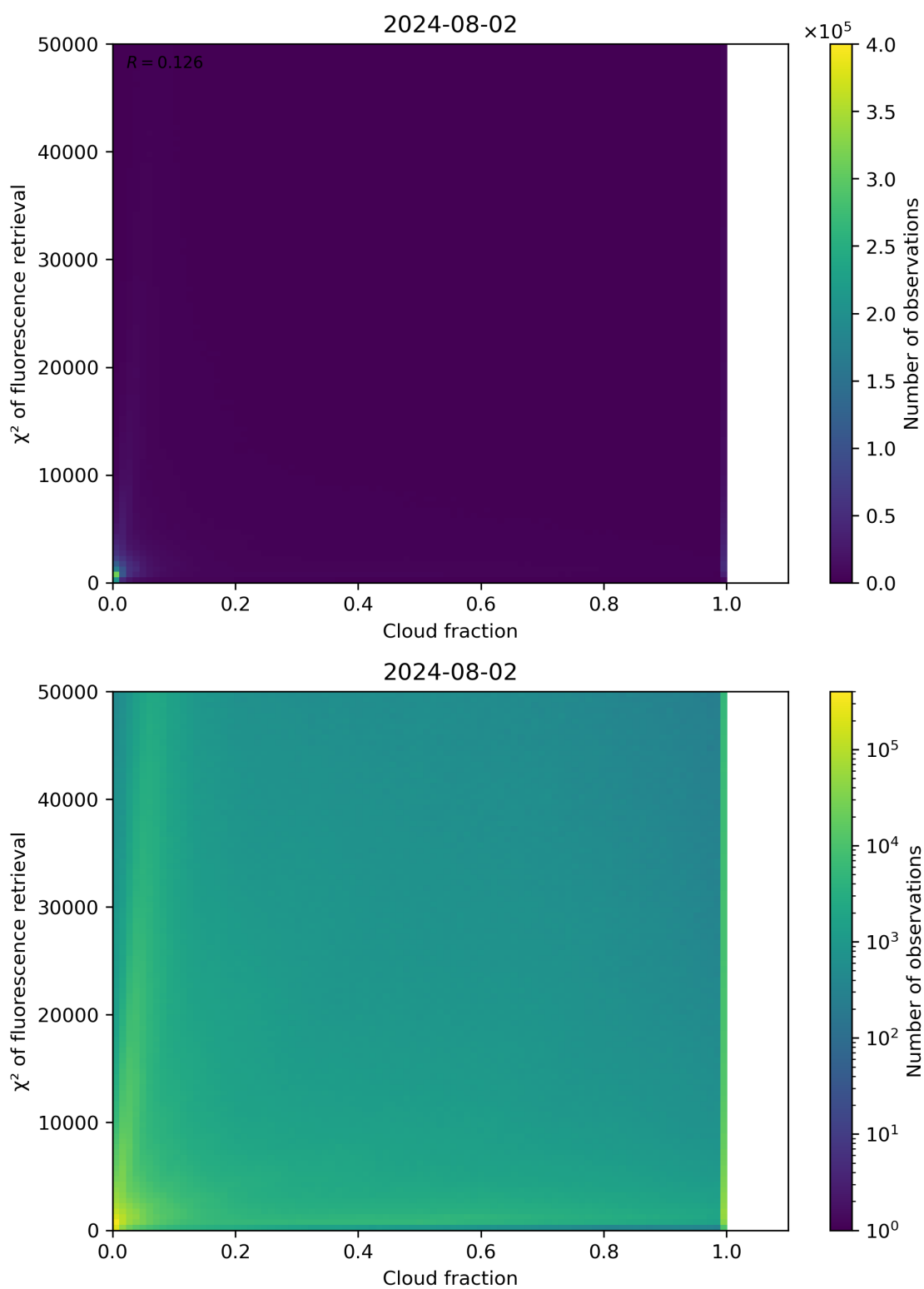
Figure 71: Scatter density plot of “Cloud fraction” against “ \chi^2 of fluorescence retrieval” for 2024-08-01 to 2024-08-03.
