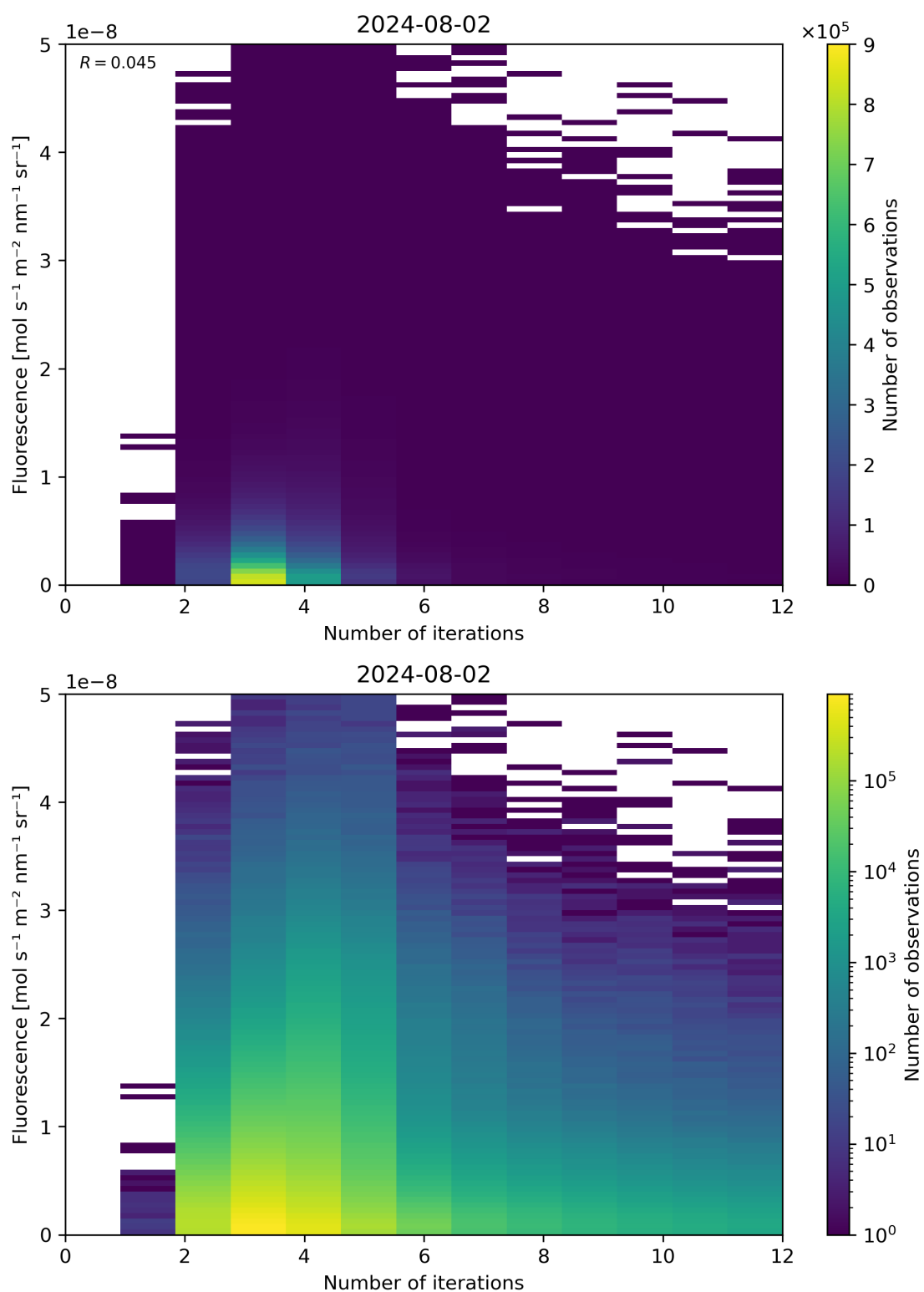
Figure 98: Scatter density plot of “Number of iterations” against “Fluorescence” for 2024-08-01 to 2024-08-03.
