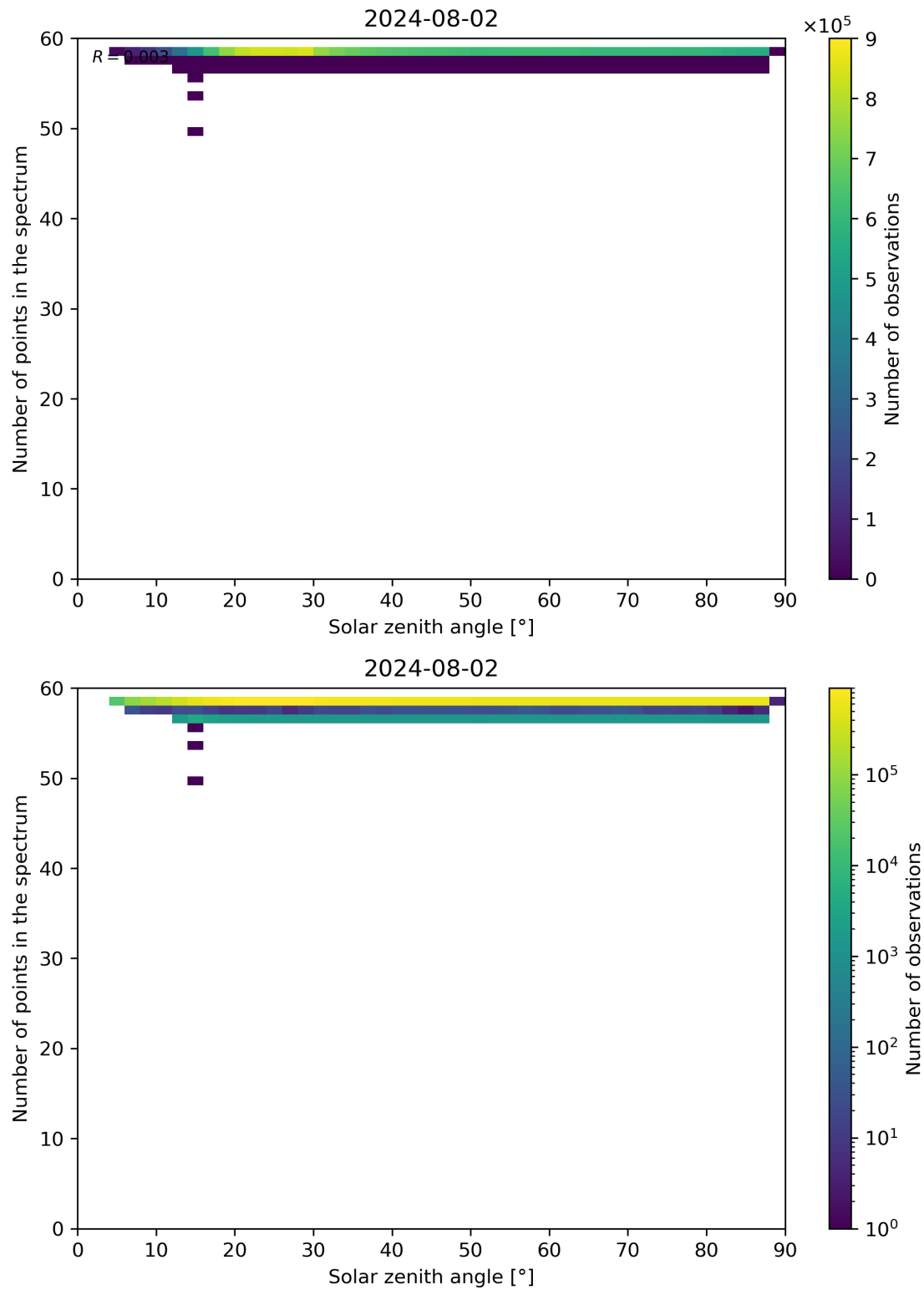
Figure 115: Scatter density plot of “Solar zenith angle” against “Number of points in the spectrum” for 2024-08-01 to 2024-08-03.
