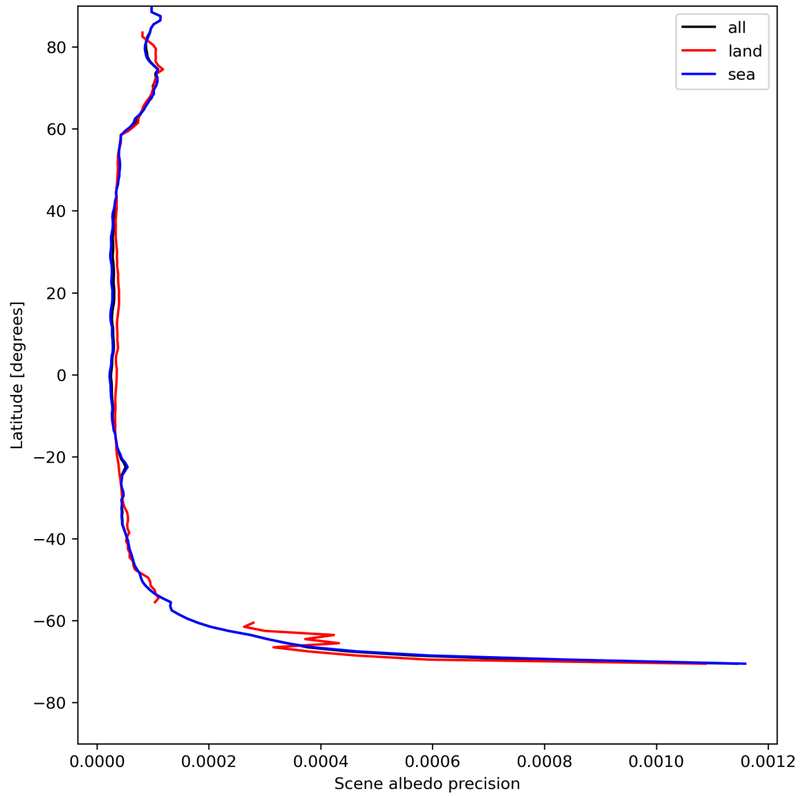
Figure 18: Zonal average of “Scene albedo precision” for 2024-08-01 to 2024-08-03.
