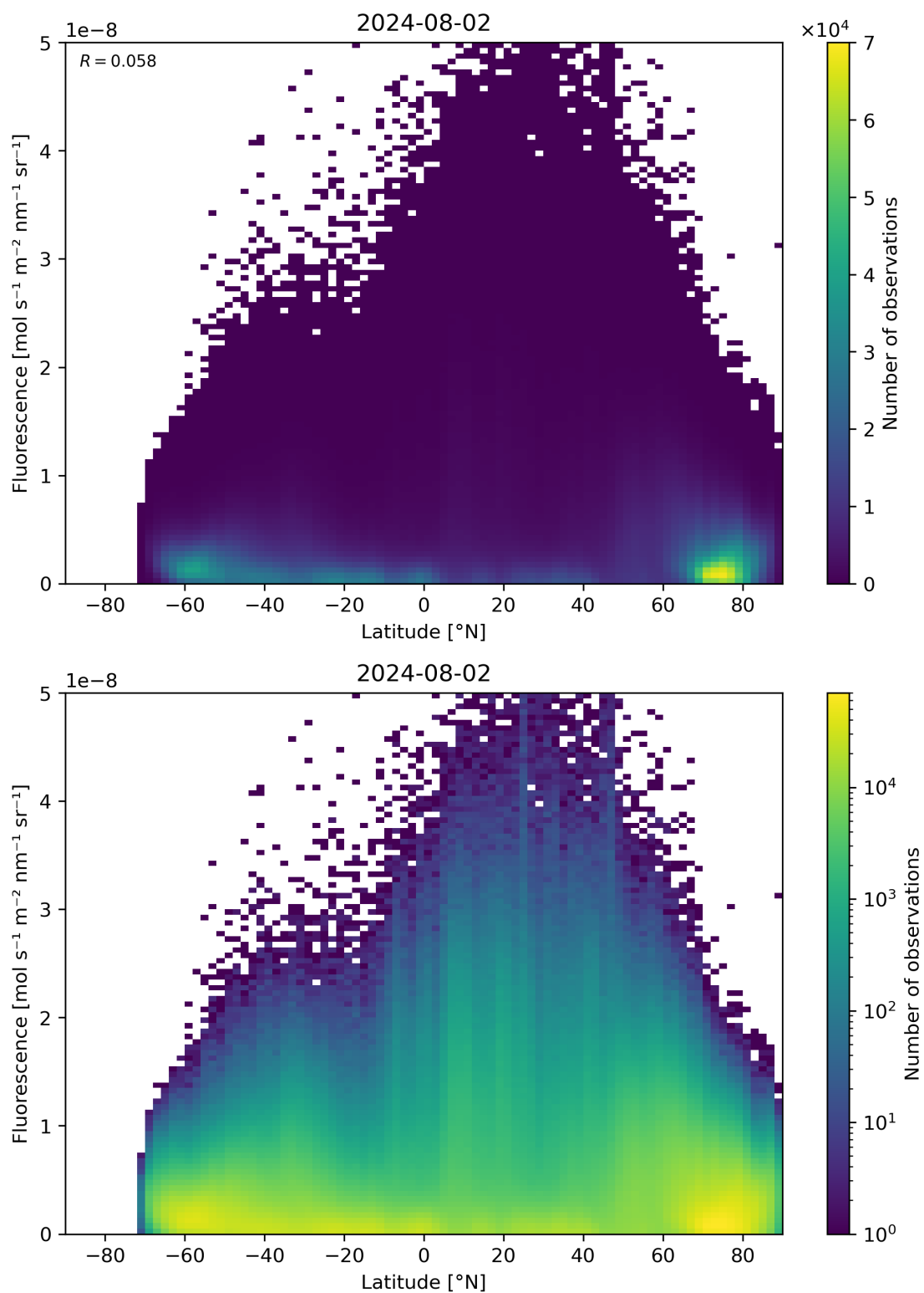
Figure 92: Scatter density plot of “Latitude” against “Fluorescence” for 2024-08-01 to 2024-08-03.
