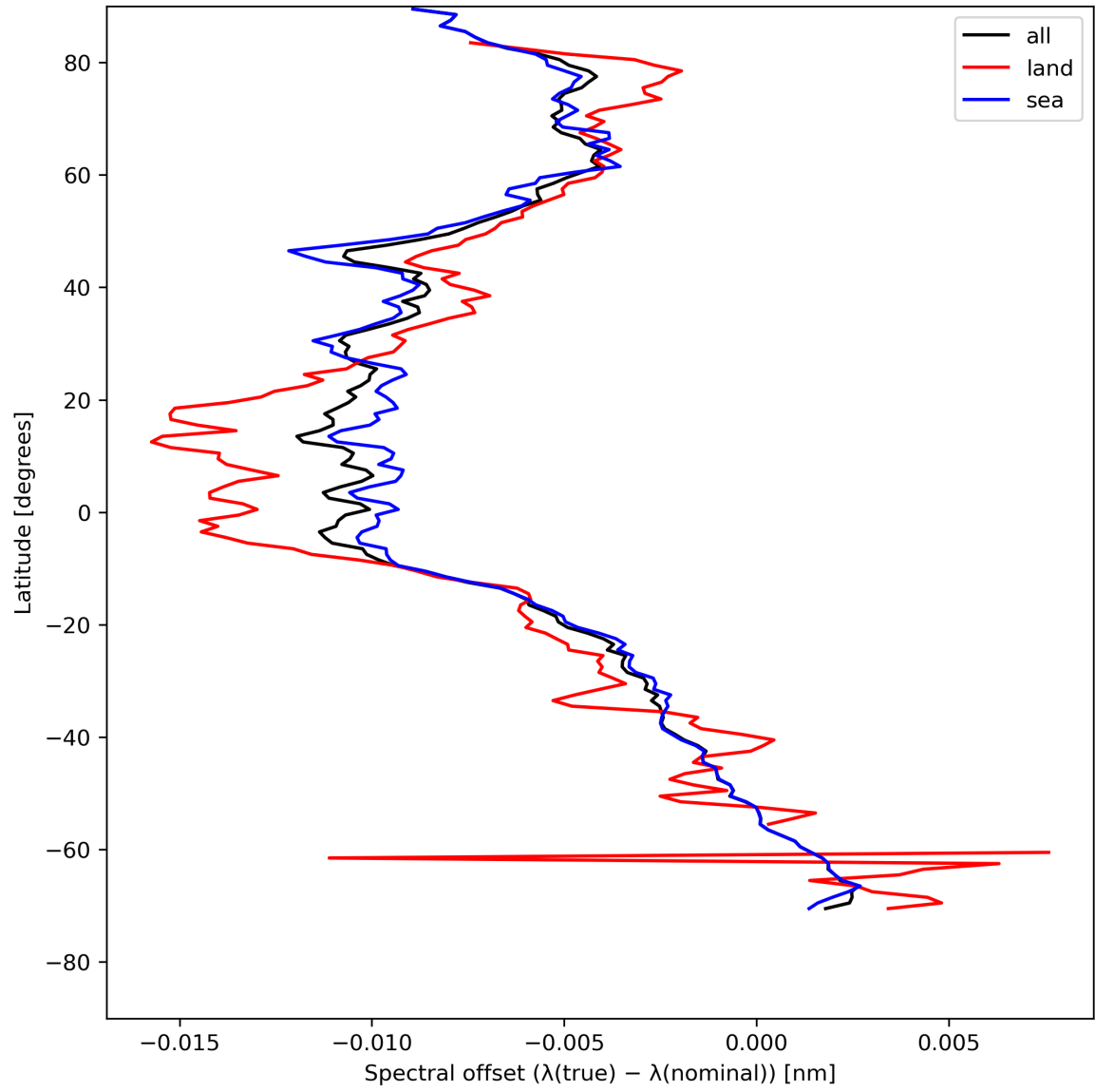
Figure 28: Zonal average of “Spectral offset ( \lambda(\text{true}) - \lambda(\text{nominal}) )” for 2024-08-01 to 2024-08-03.
