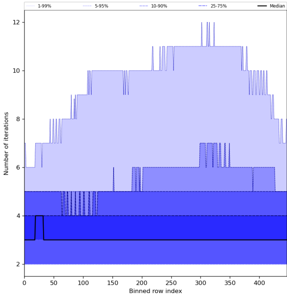
Figure 56: Along track statistics of “Number of iterations” for 2024-08-01 to 2024-08-03
