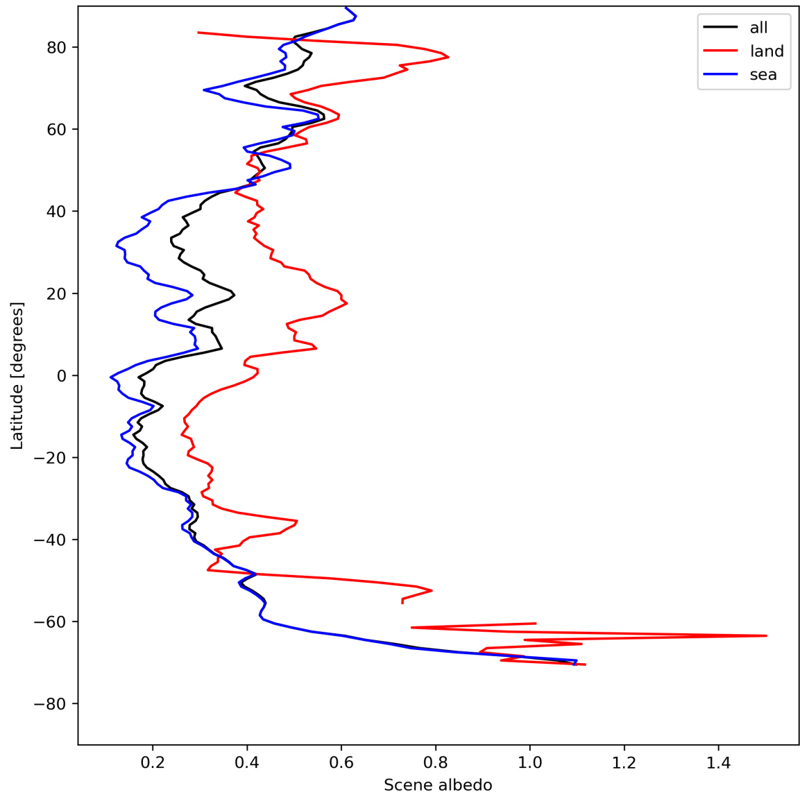
Figure 17: Zonal average of “Scene albedo” for 2024-08-01 to 2024-08-03.
