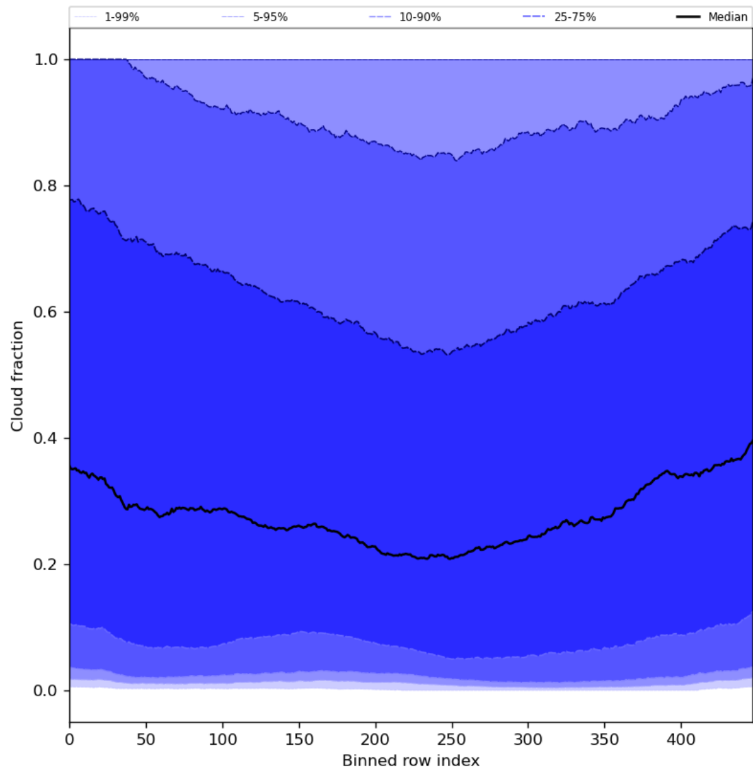
Figure 49: Along track statistics of “Cloud fraction” for 2024-08-01 to 2024-08-03
