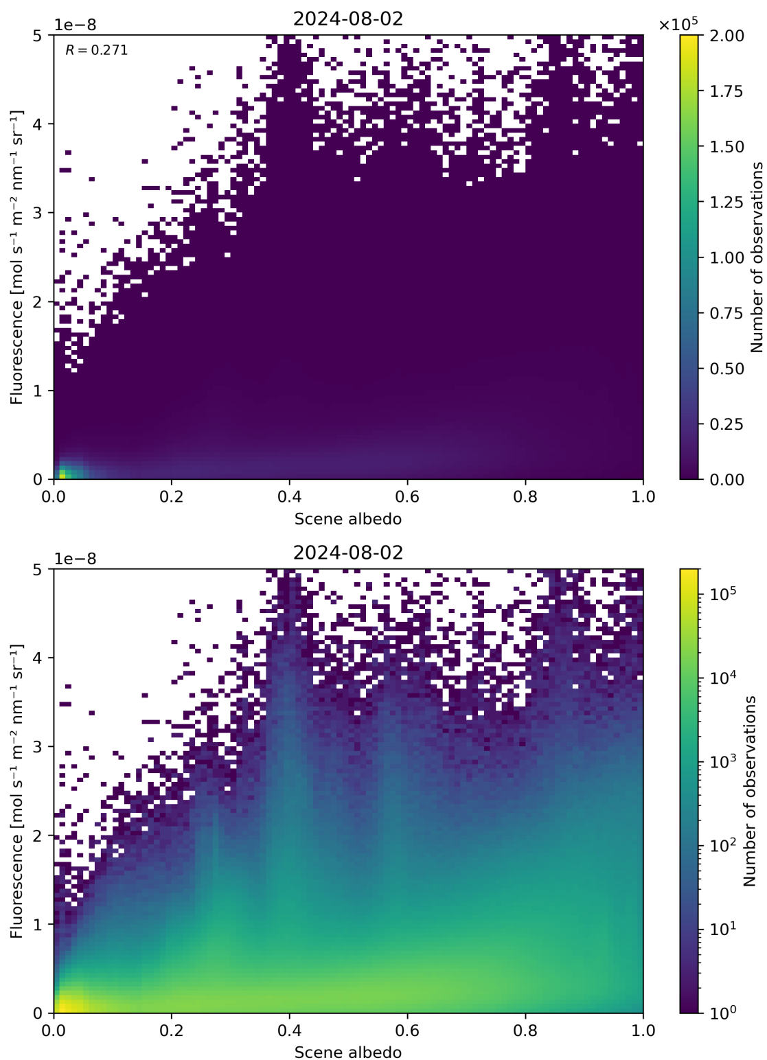
Figure 104: Scatter density plot of “Scene albedo” against “Fluorescence” for 2024-08-01 to 2024-08-03.
