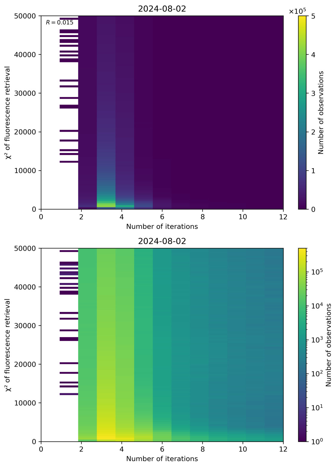
Figure 97: Scatter density plot of “Number of iterations” against “ \chi^2 of fluorescence retrieval” for 2024-08-01 to 2024-08-03.
