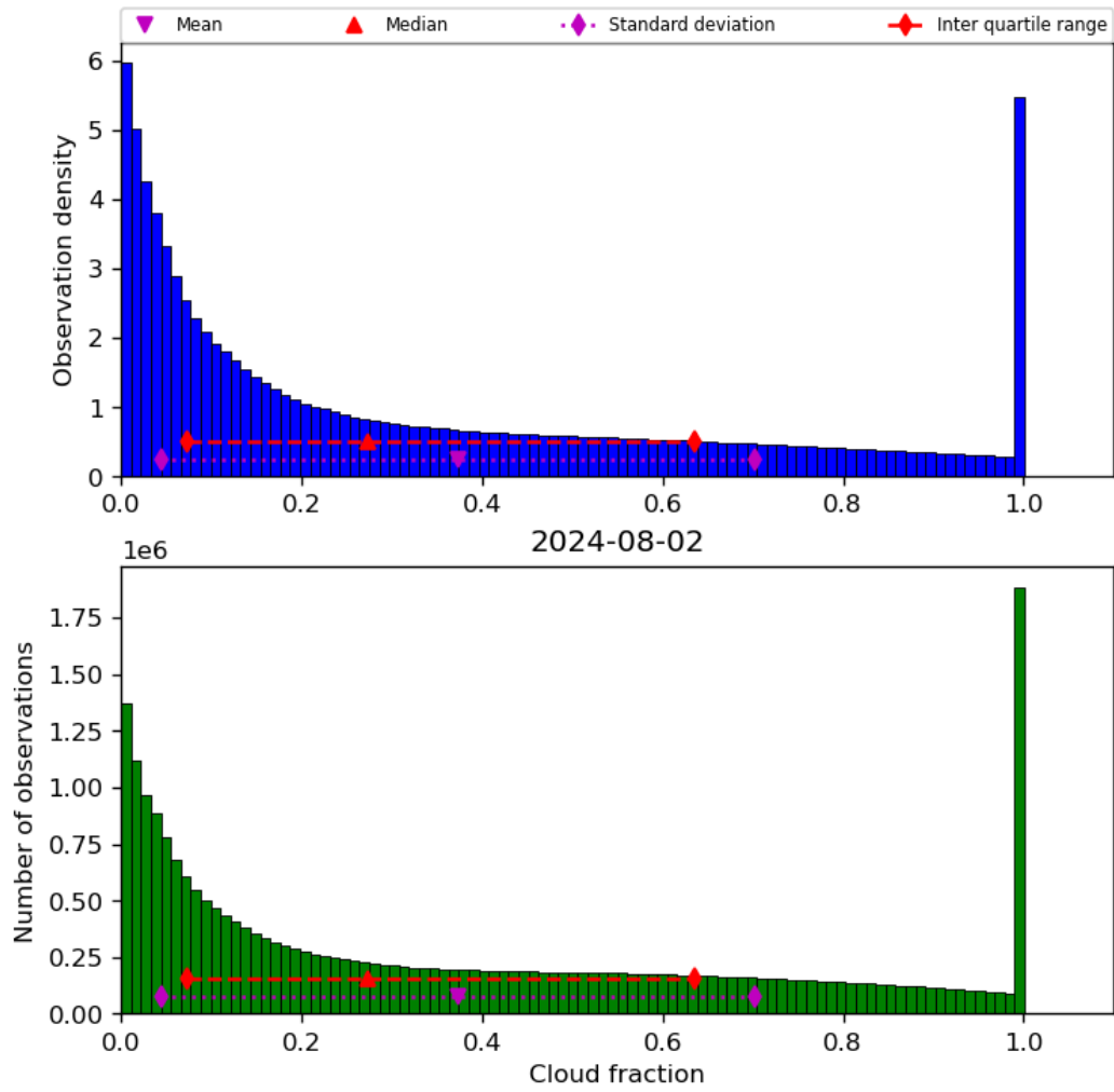
Figure 32: Histogram of “Cloud fraction” for 2024-08-01 to 2024-08-03
