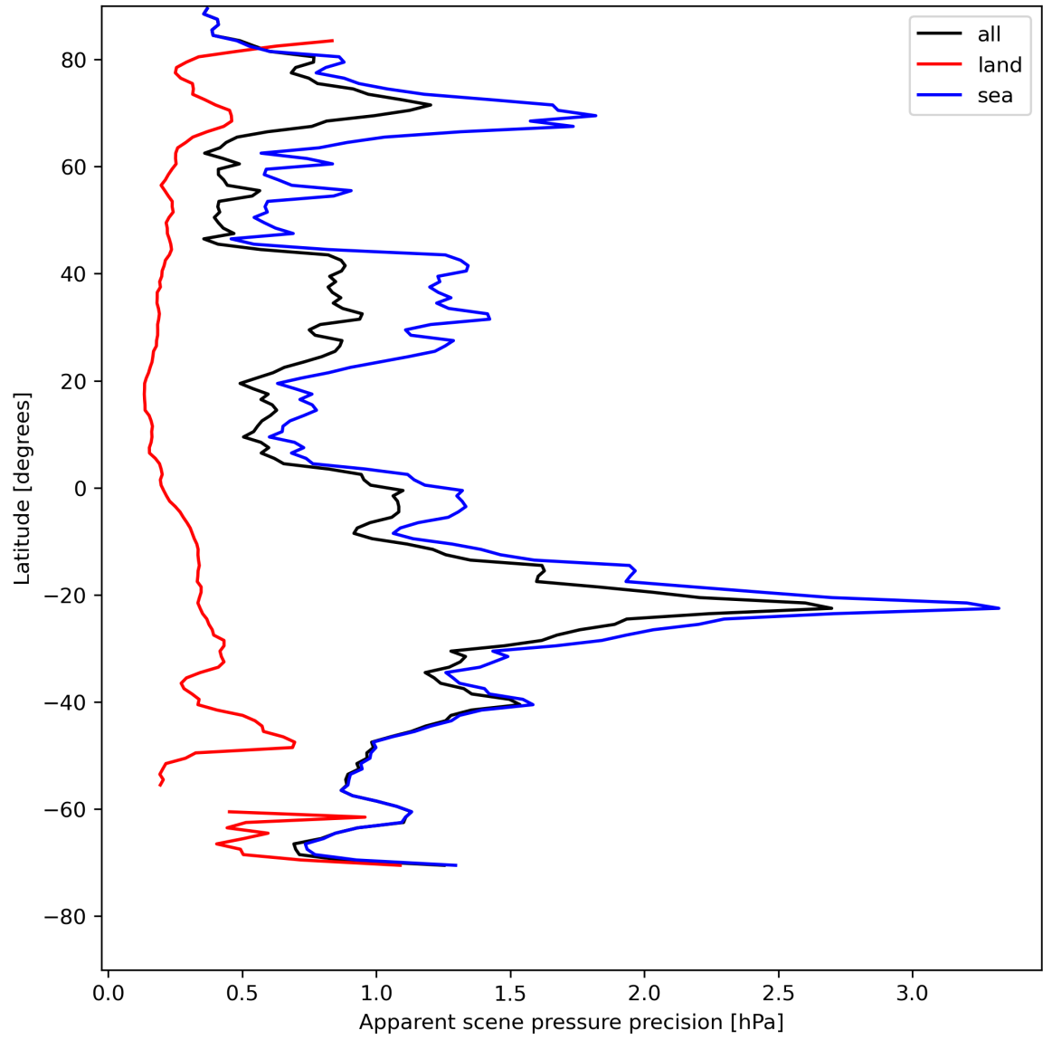
Figure 20: Zonal average of “Apparent scene pressure precision” for 2024-08-01 to 2024-08-03.
