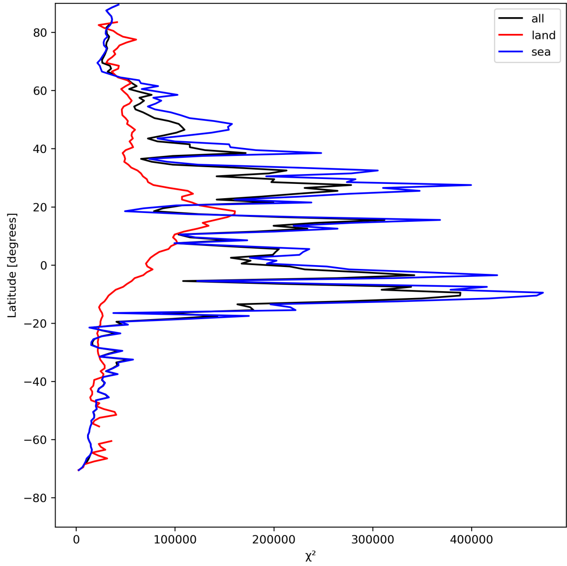
Figure 21: Zonal average of “ \chi^2 ” for 2024-08-01 to 2024-08-03.
