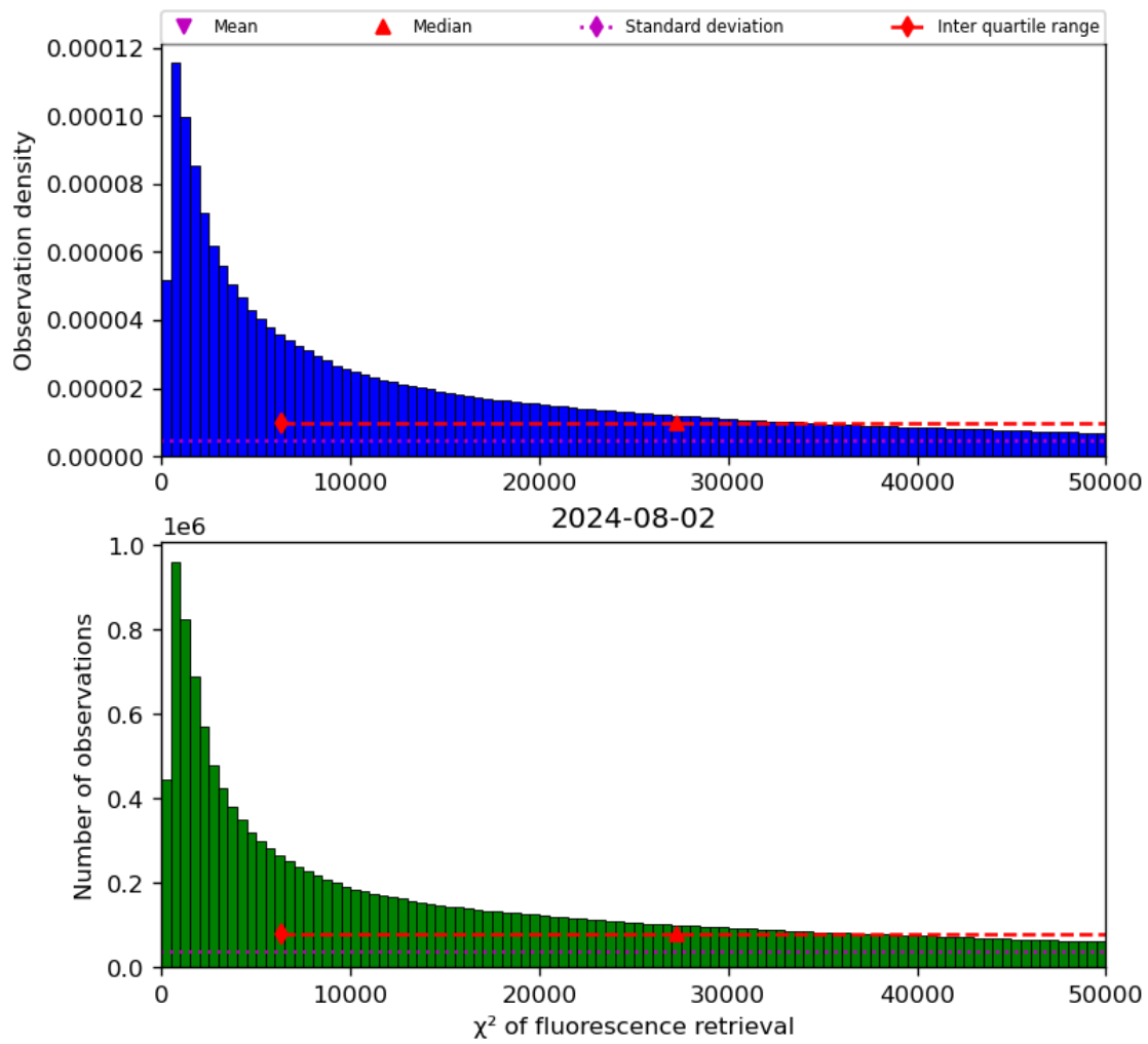
Figure 42: Histogram of “ \chi^2 of fluorescence retrieval” for 2024-08-01 to 2024-08-03
