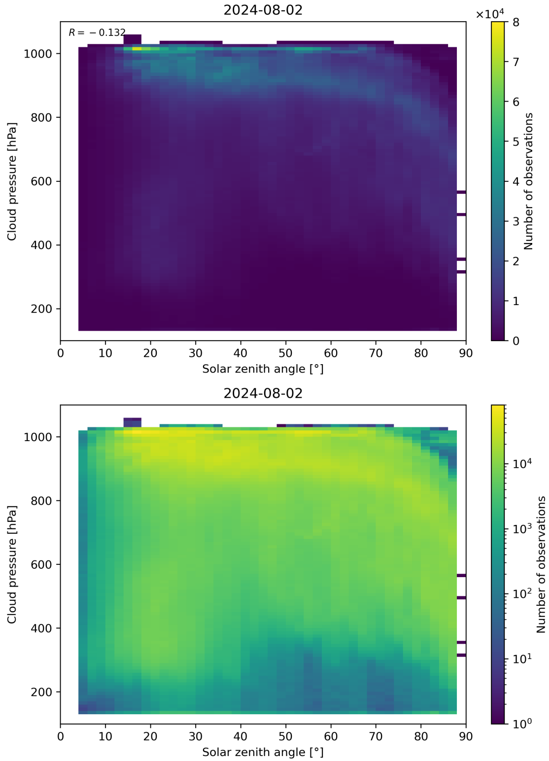
Figure 111: Scatter density plot of “Solar zenith angle” against “Cloud pressure” for 2024-08-01 to 2024-08-03.
