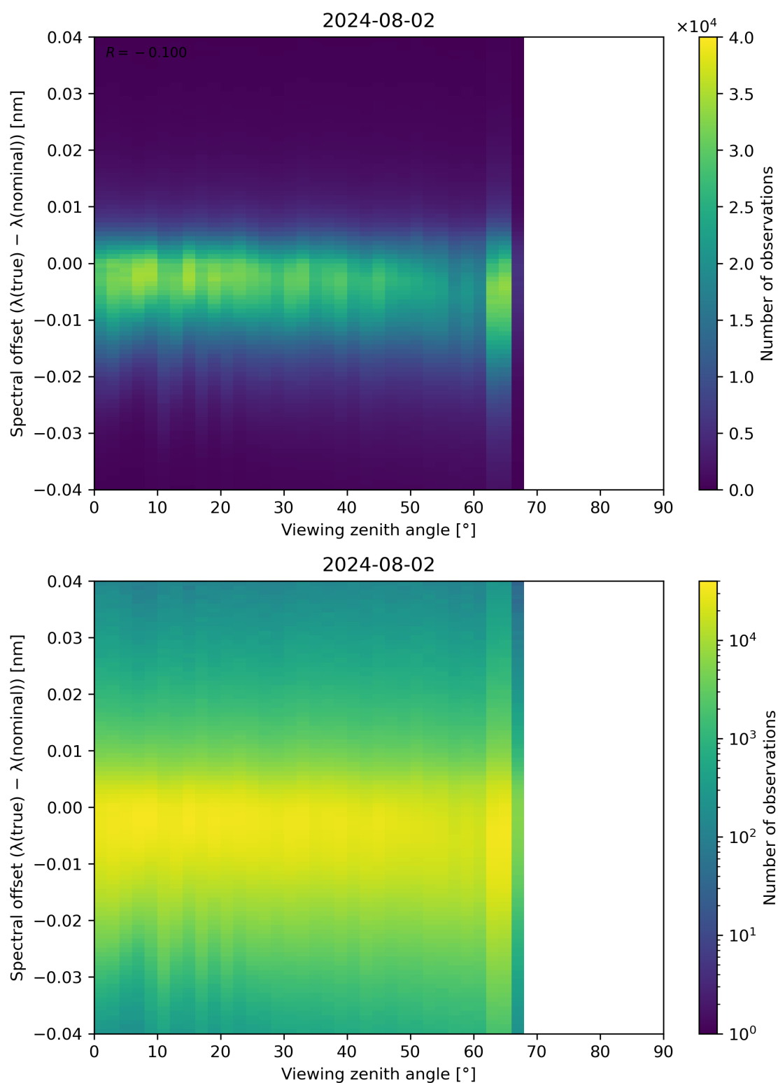
Figure 128: Scatter density plot of “Viewing zenith angle” against “Spectral offset ( \lambda(\text{true}) - \lambda(\text{nominal}) )” for 2024-08-01 to 2024-08-03.
