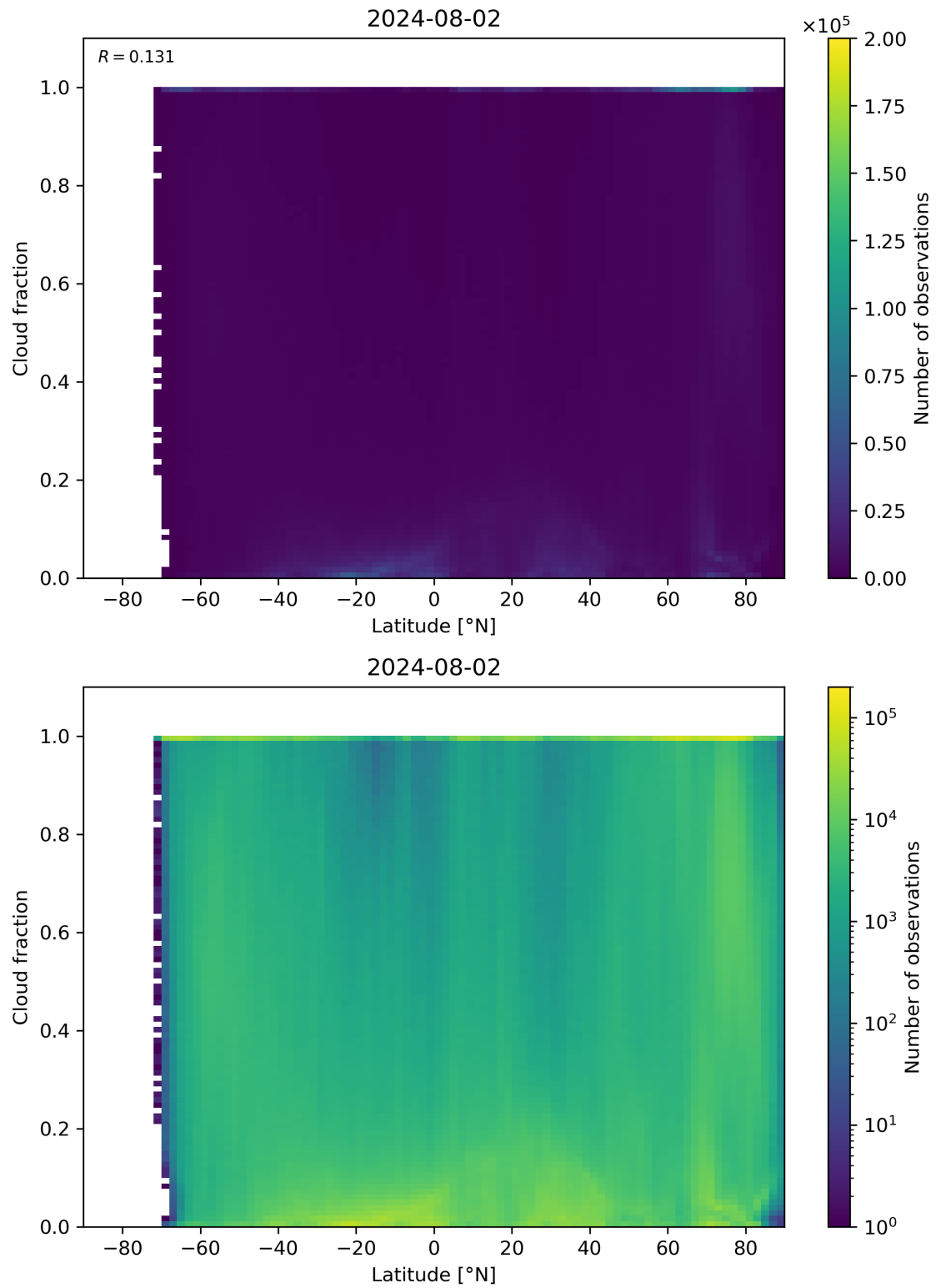
Figure 90: Scatter density plot of “Latitude” against “Cloud fraction” for 2024-08-01 to 2024-08-03.
