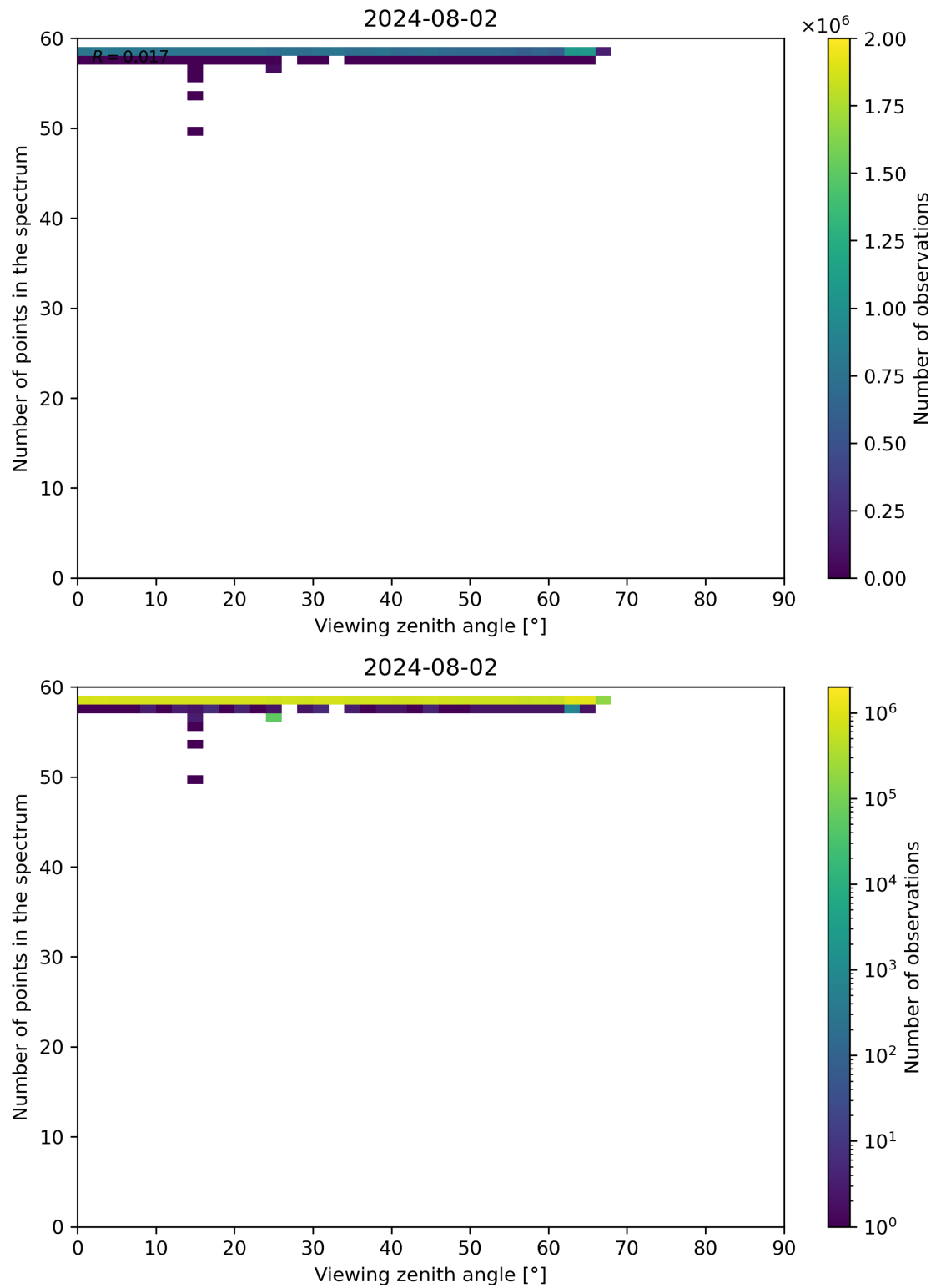
Figure 125: Scatter density plot of “Viewing zenith angle” against “Number of points in the spectrum” for 2024-08-01 to 2024-08-03.
