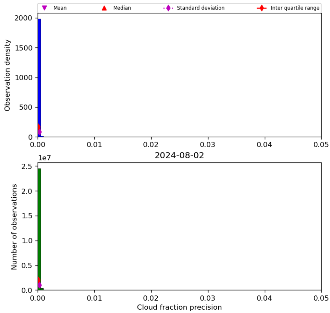
Figure 33: Histogram of “Cloud fraction precision” for 2024-08-01 to 2024-08-03
