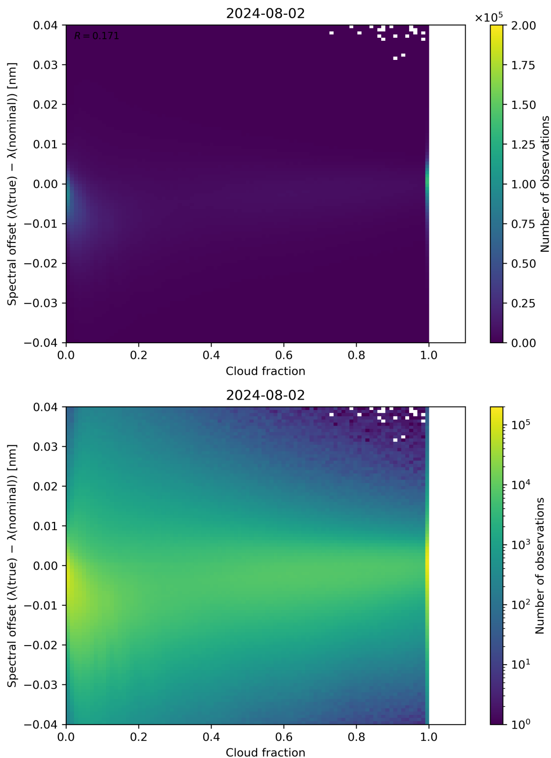
Figure 76: Scatter density plot of “Cloud fraction” against “Spectral offset ( \lambda(\text{true}) - \lambda(\text{nominal}) )” for 2024-08-01 to 2024-08-03.
