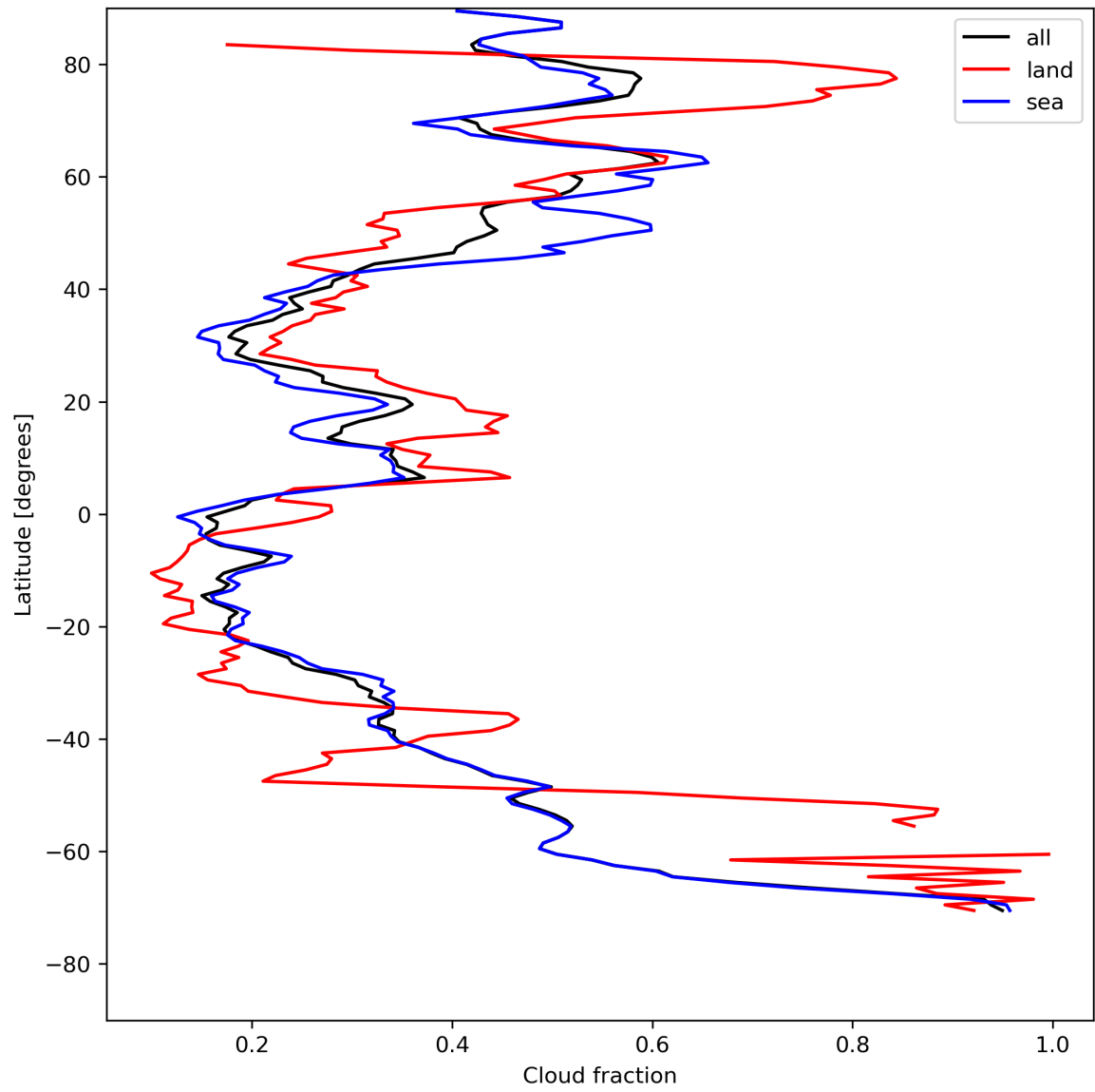
Figure 15: Zonal average of “Cloud fraction” for 2024-08-01 to 2024-08-03.
