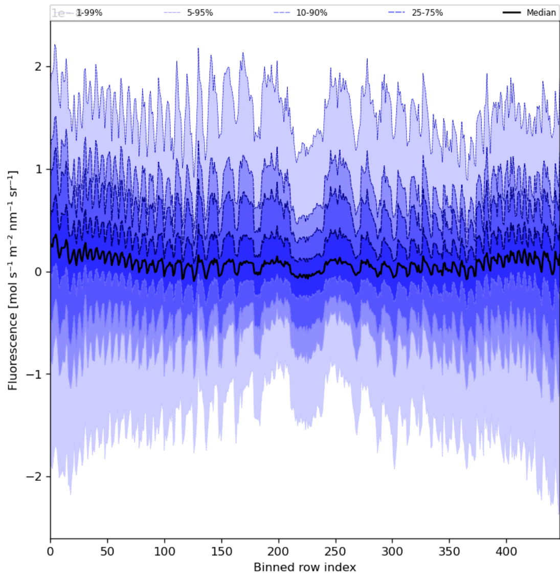
Figure 57: Along track statistics of “Fluorescence” for 2024-08-01 to 2024-08-03
