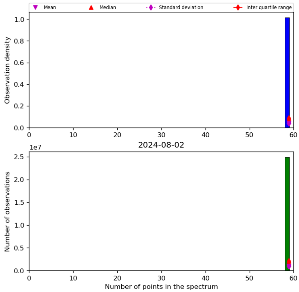
Figure 44: Histogram of “Number of points in the spectrum” for 2024-08-01 to 2024-08-03
