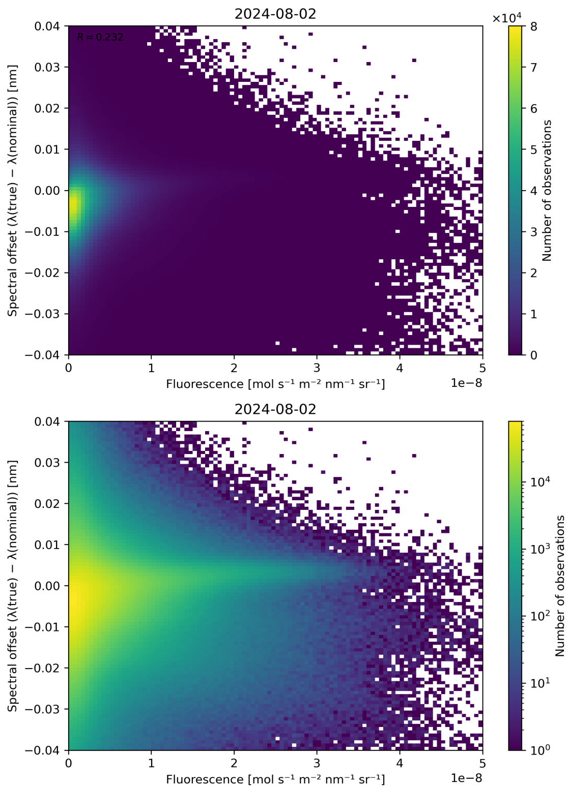
Figure 87: Scatter density plot of “Fluorescence” against “Spectral offset ( \lambda(\text{true}) - \lambda(\text{nominal}) )” for 2024-08-01 to 2024-08-03.
