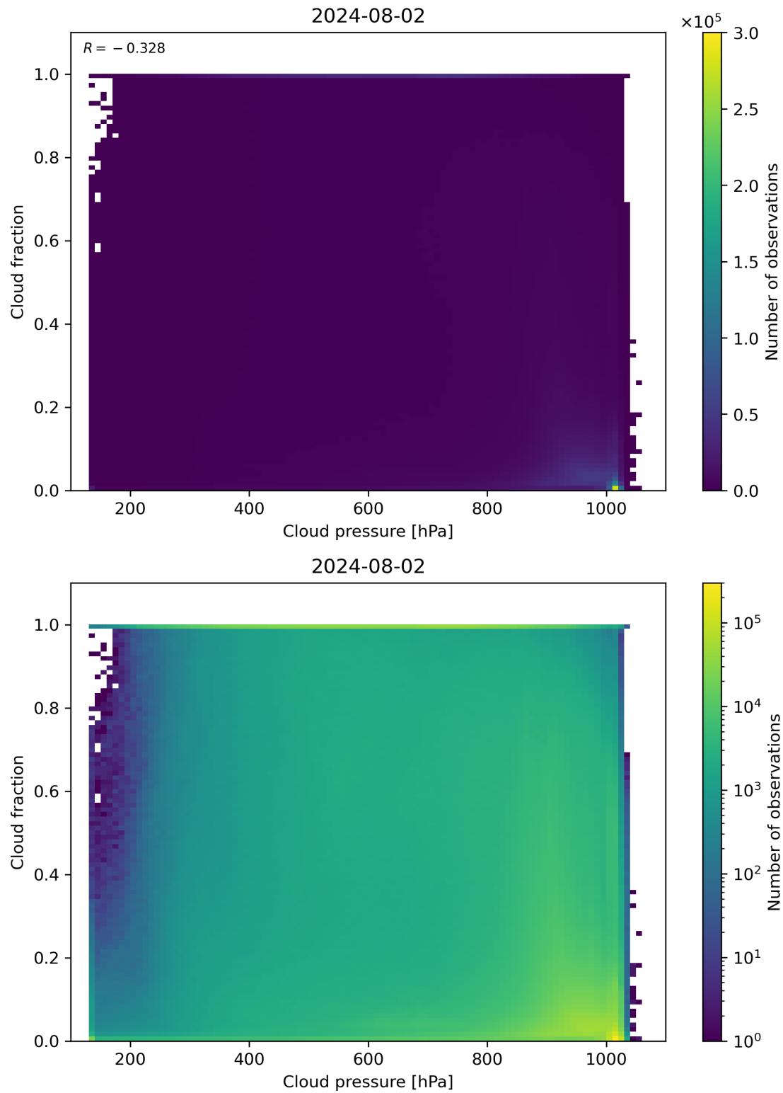
Figure 79: Scatter density plot of “Cloud pressure” against “Cloud fraction” for 2024-08-01 to 2024-08-03.
