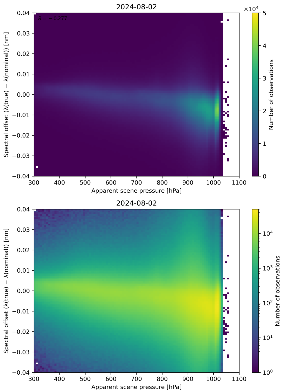
Figure 67: Scatter density plot of “Apparent scene pressure” against “Spectral offset ( \lambda(\text{true}) - \lambda(\text{nominal}) )” for 2024-08-01 to 2024-08-03.
