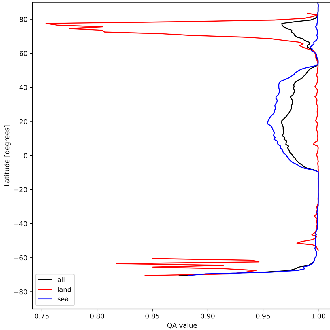
Figure 12: Zonal average of “QA value” for 2024-08-01 to 2024-08-03.
