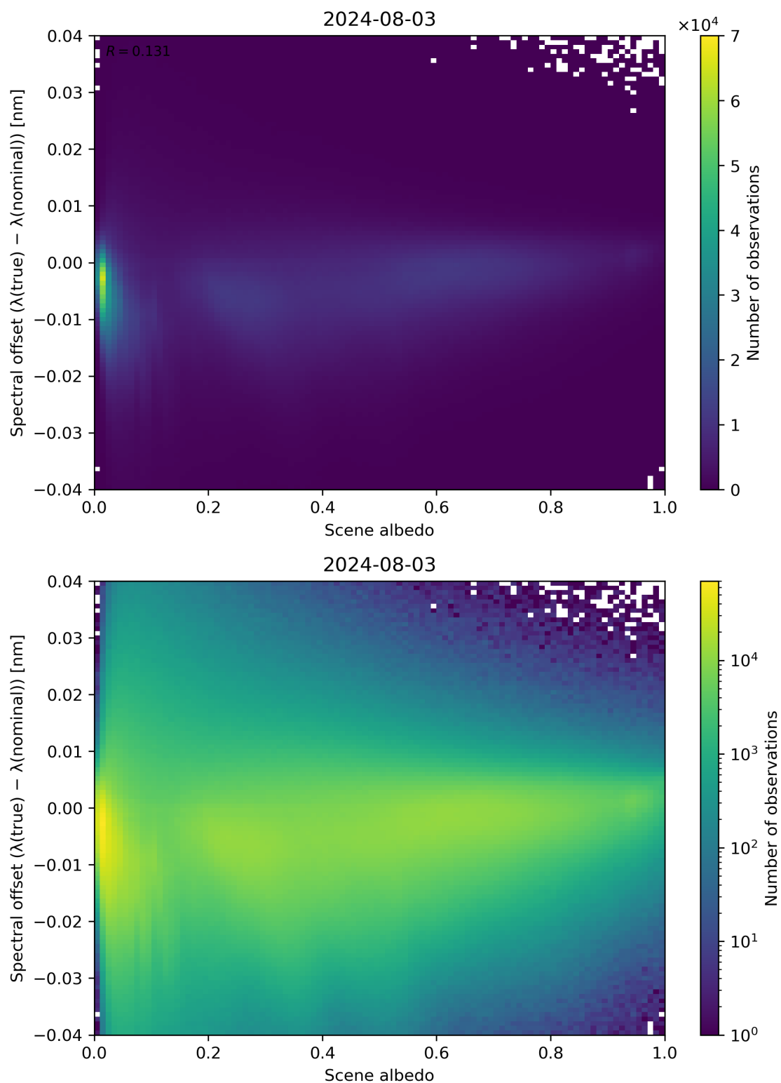
Figure 107: Scatter density plot of “Scene albedo” against “Spectral offset ( \lambda(\text{true}) - \lambda(\text{nominal}) )” for 2024-08-02 to 2024-08-04.
