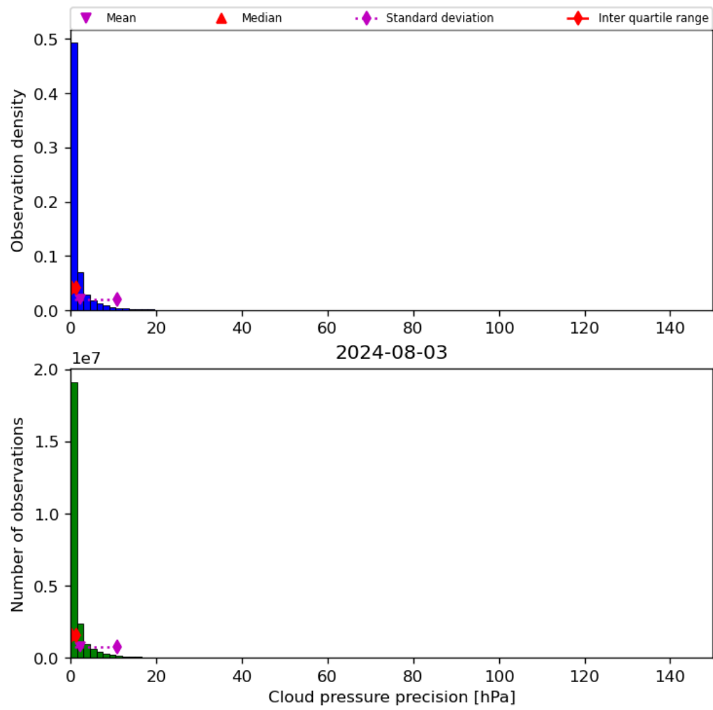
Figure 31: Histogram of “Cloud pressure precision” for 2024-08-02 to 2024-08-04
