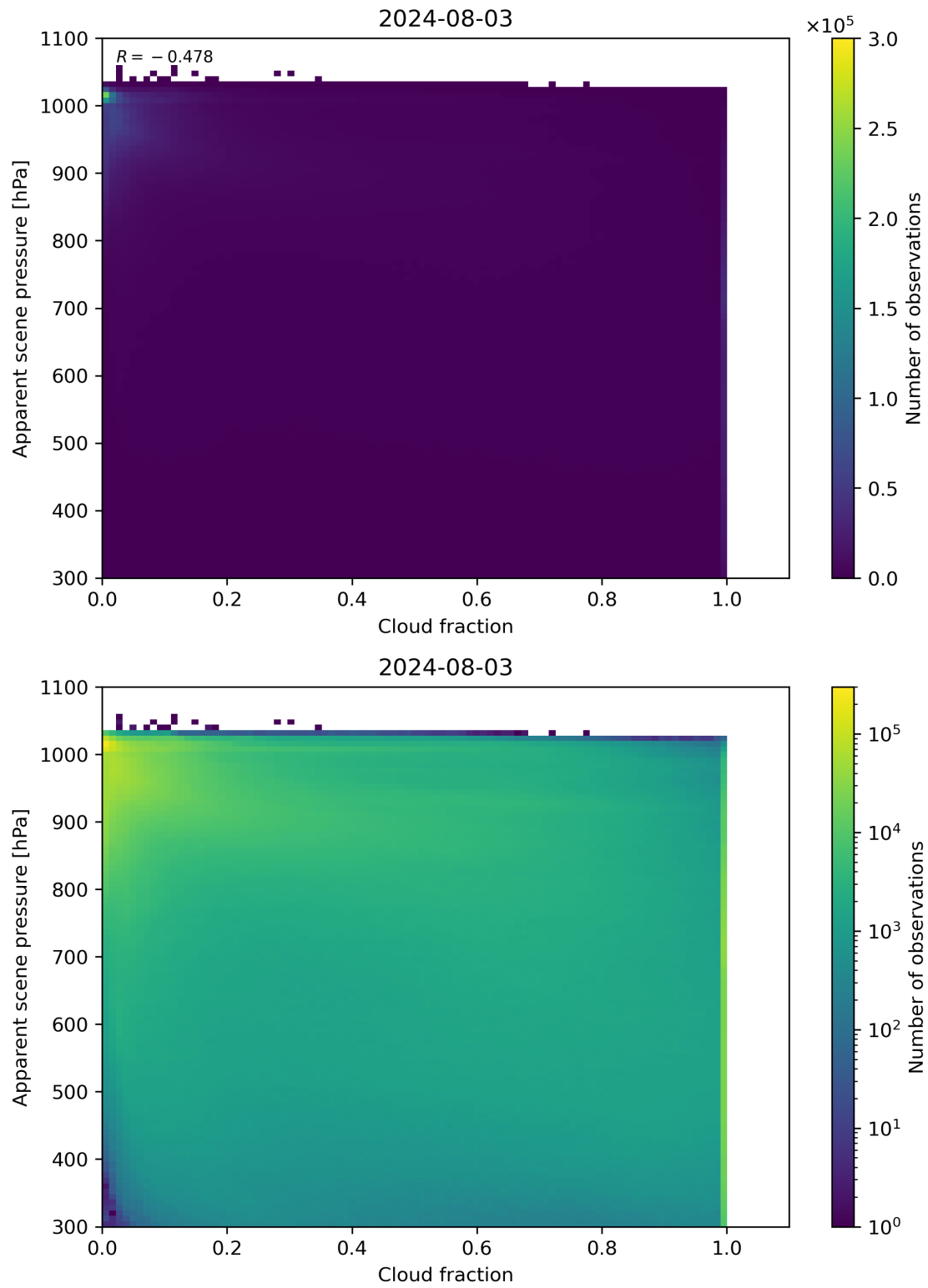
Figure 70: Scatter density plot of “Cloud fraction” against “Apparent scene pressure” for 2024-08-02 to 2024-08-04.
