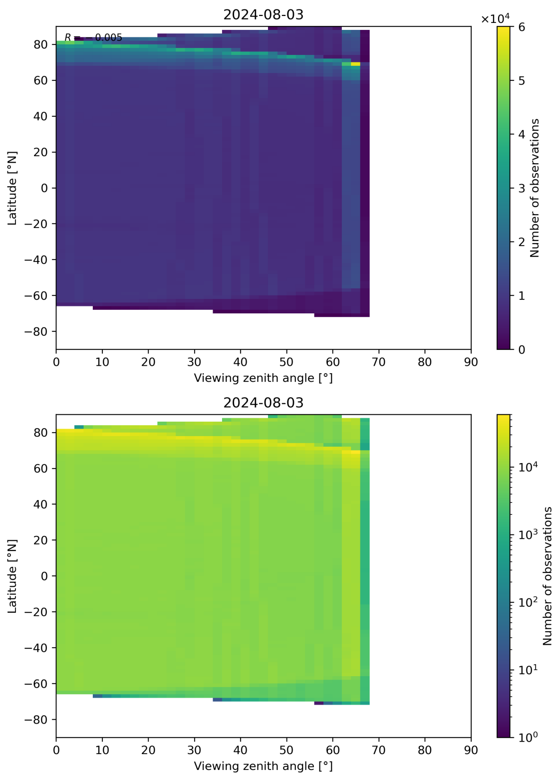
Figure 123: Scatter density plot of “Viewing zenith angle” against “Latitude” for 2024-08-02 to 2024-08-04.
