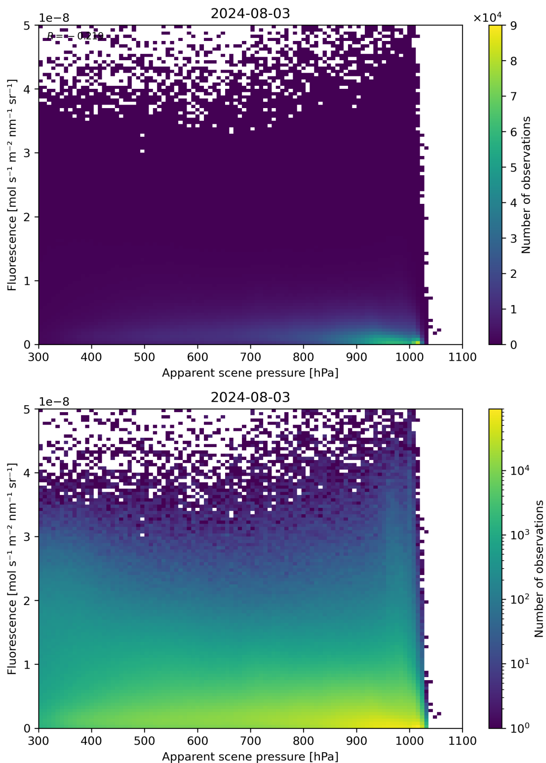
Figure 64: Scatter density plot of “Apparent scene pressure” against “Fluorescence” for 2024-08-02 to 2024-08-04.
