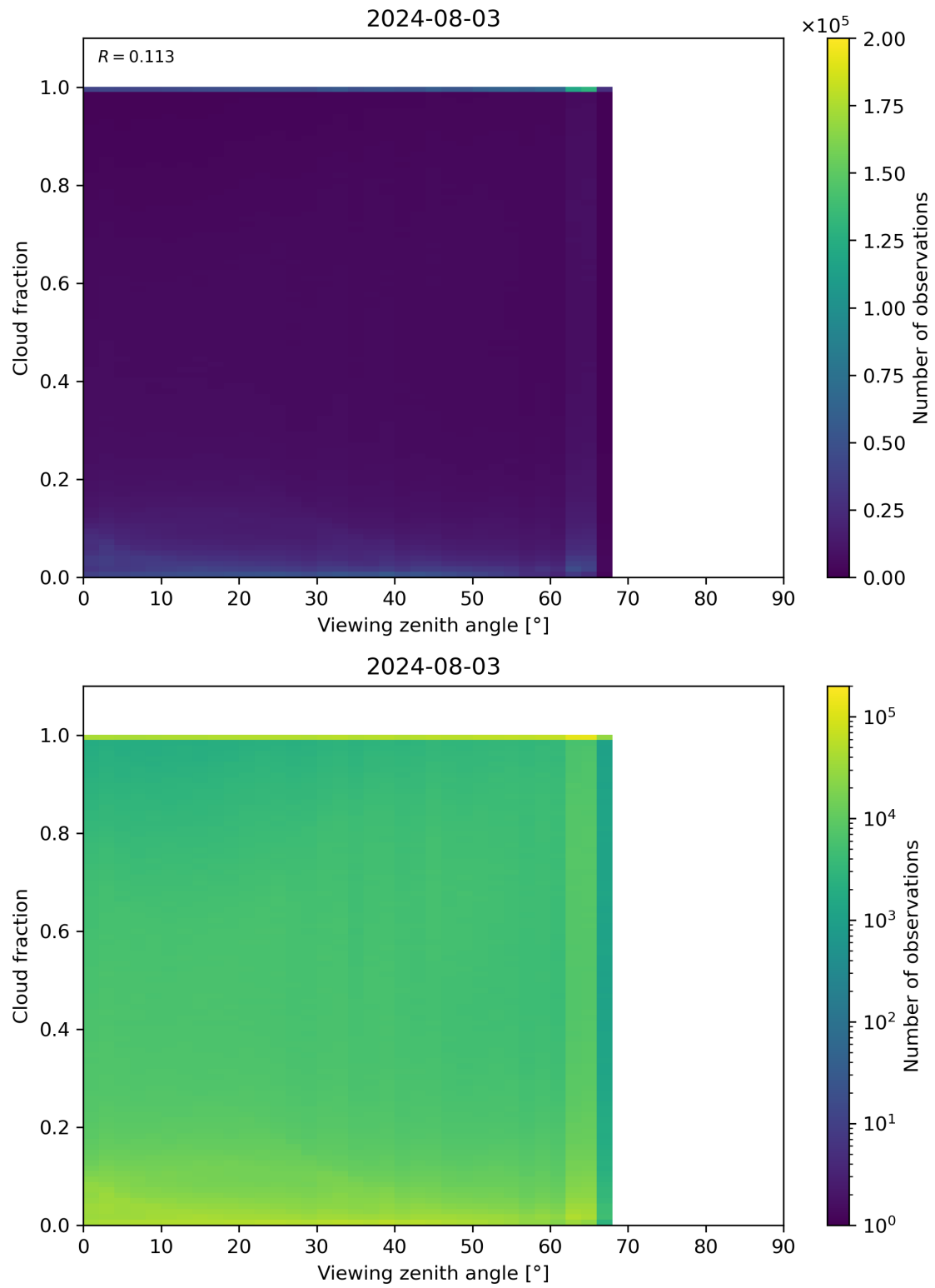
Figure 120: Scatter density plot of “Viewing zenith angle” against “Cloud fraction” for 2024-08-02 to 2024-08-04.
