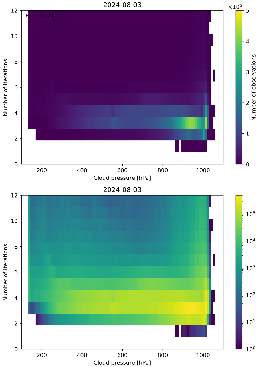
Figure 81: Scatter density plot of “Cloud pressure” against “Number of iterations” for 2024-08-02 to 2024-08-04.
