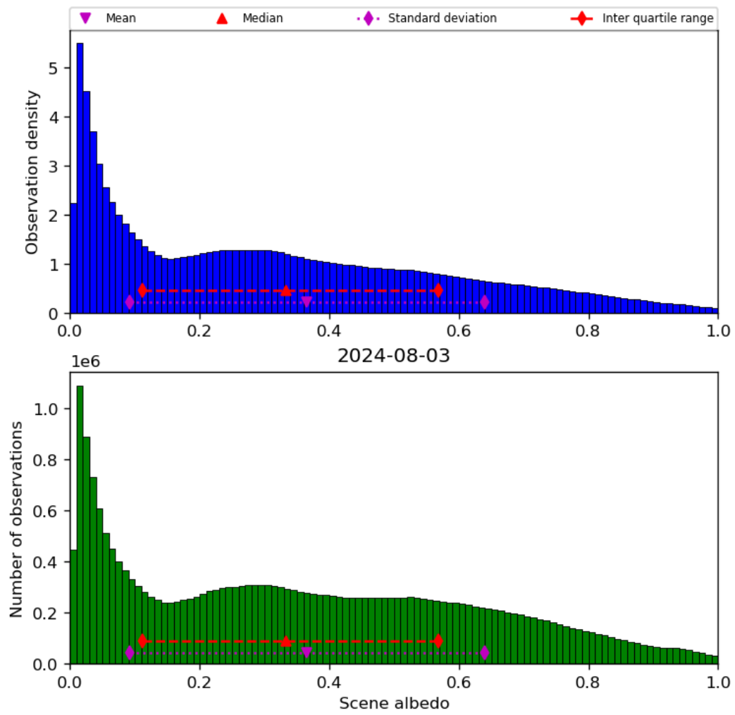
Figure 34: Histogram of “Scene albedo” for 2024-08-02 to 2024-08-04
