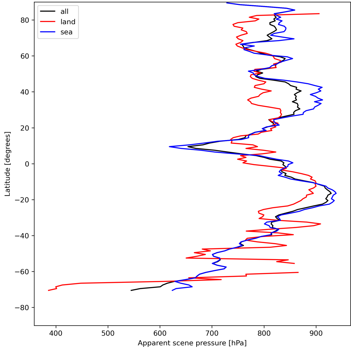
Figure 19: Zonal average of “Apparent scene pressure” for 2024-08-02 to 2024-08-04.
