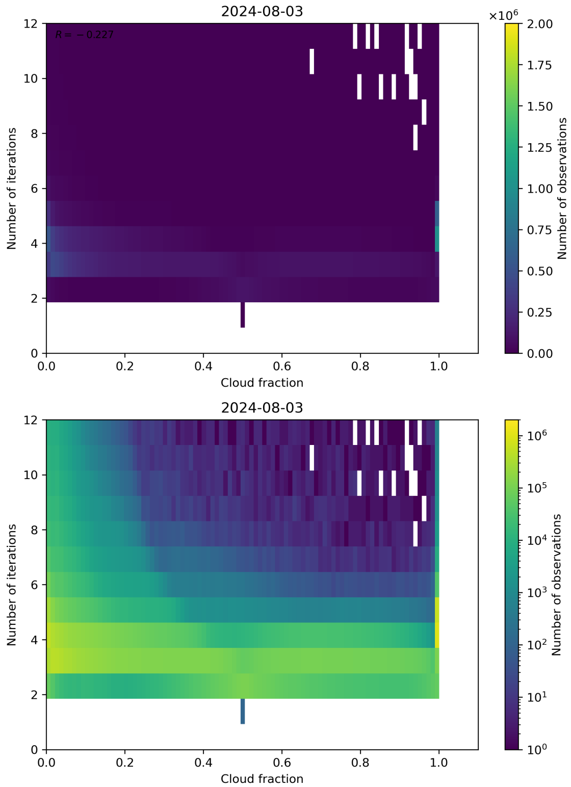
Figure 73: Scatter density plot of “Cloud fraction” against “Number of iterations” for 2024-08-02 to 2024-08-04.
