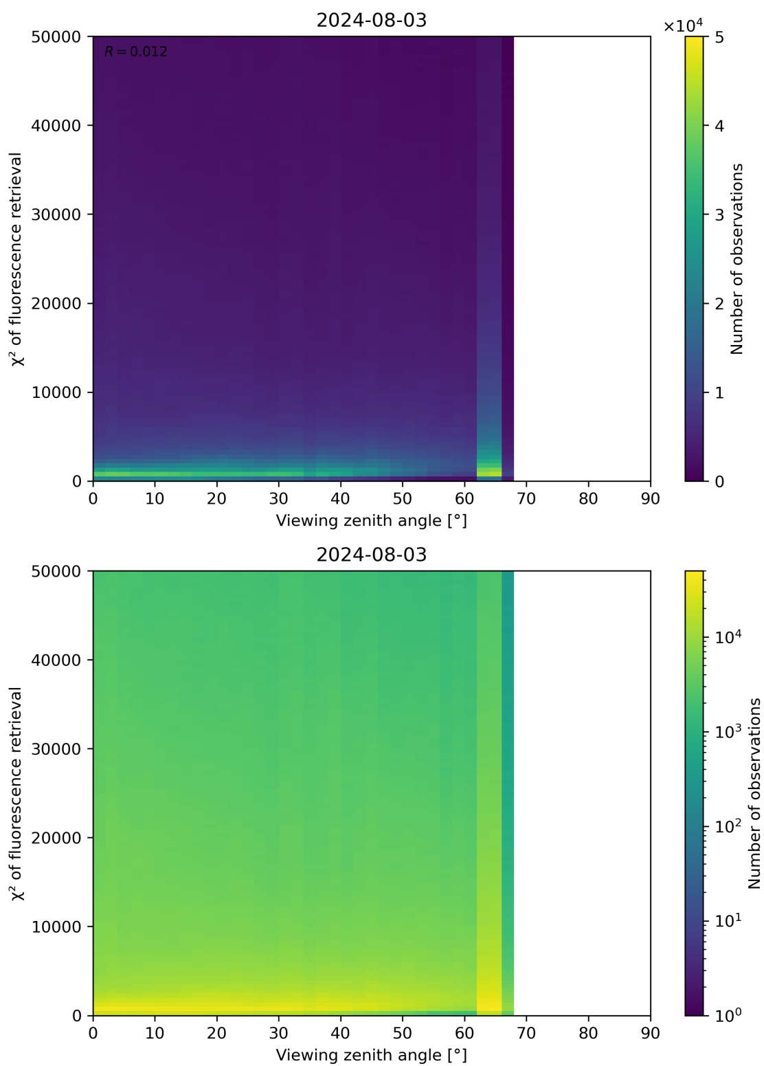
Figure 119: Scatter density plot of “Viewing zenith angle” against “ \chi^2 of fluorescence retrieval” for 2024-08-02 to 2024-08-04.
