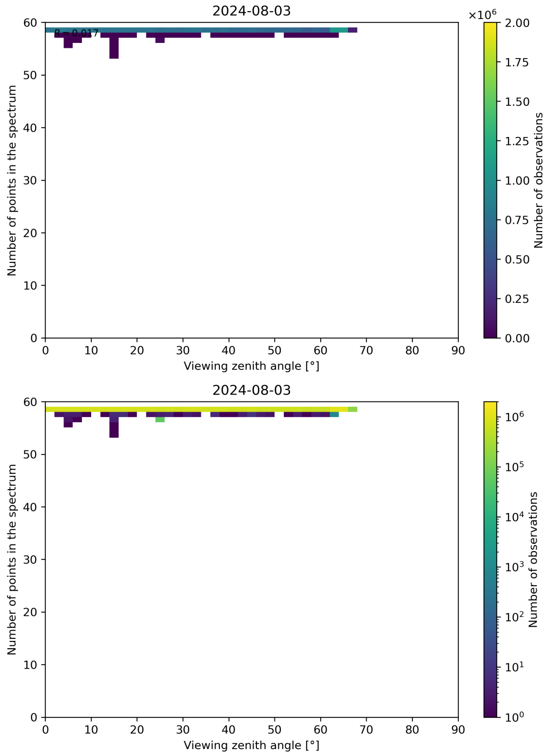
Figure 125: Scatter density plot of “Viewing zenith angle” against “Number of points in the spectrum” for 2024-08-02 to 2024-08-04.
