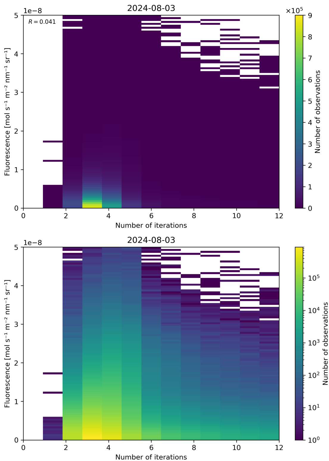
Figure 98: Scatter density plot of “Number of iterations” against “Fluorescence” for 2024-08-02 to 2024-08-04.
