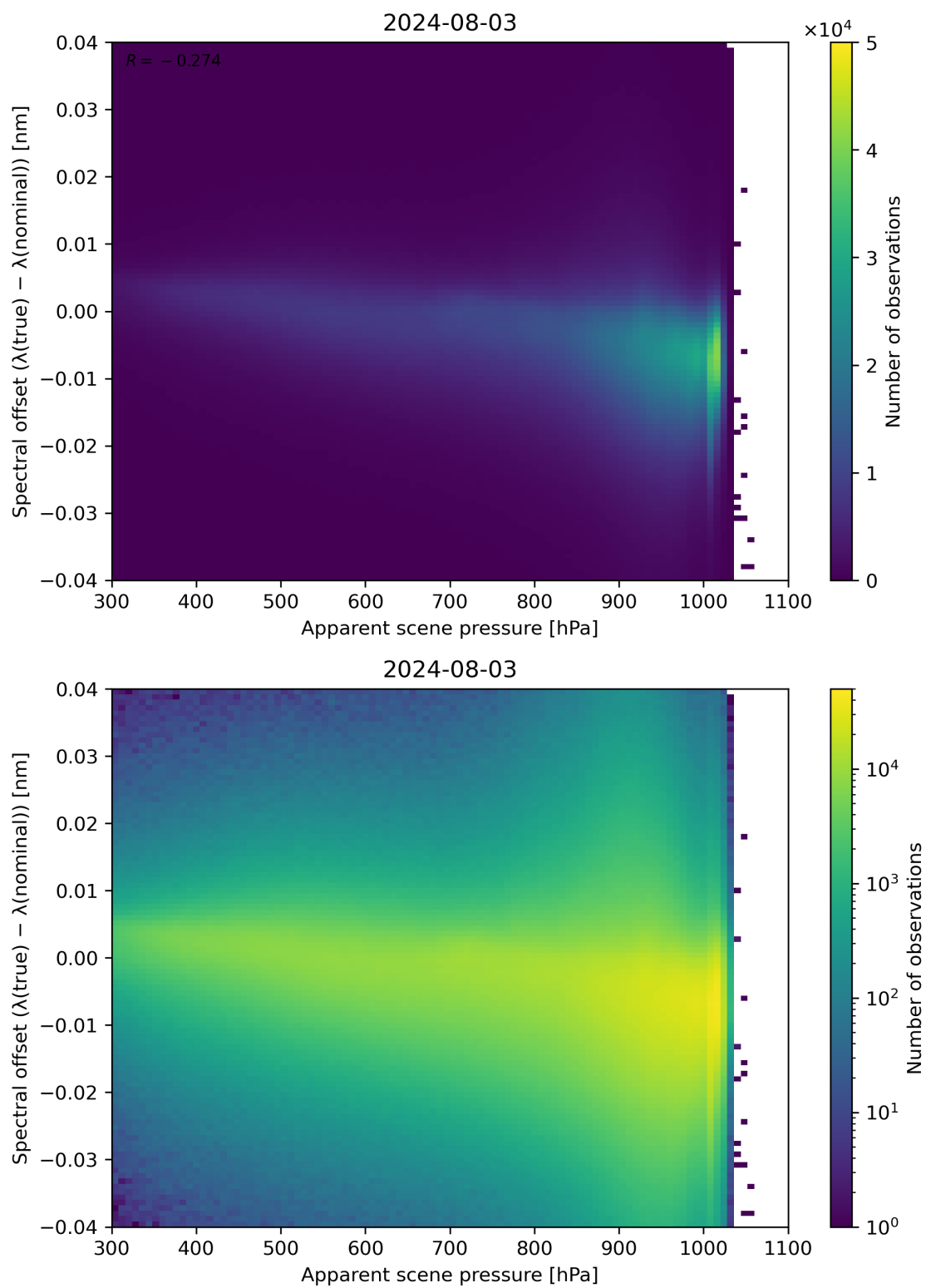
Figure 67: Scatter density plot of “Apparent scene pressure” against “Spectral offset ( \lambda(\text{true}) - \lambda(\text{nominal}) )” for 2024-08-02 to 2024-08-04.
