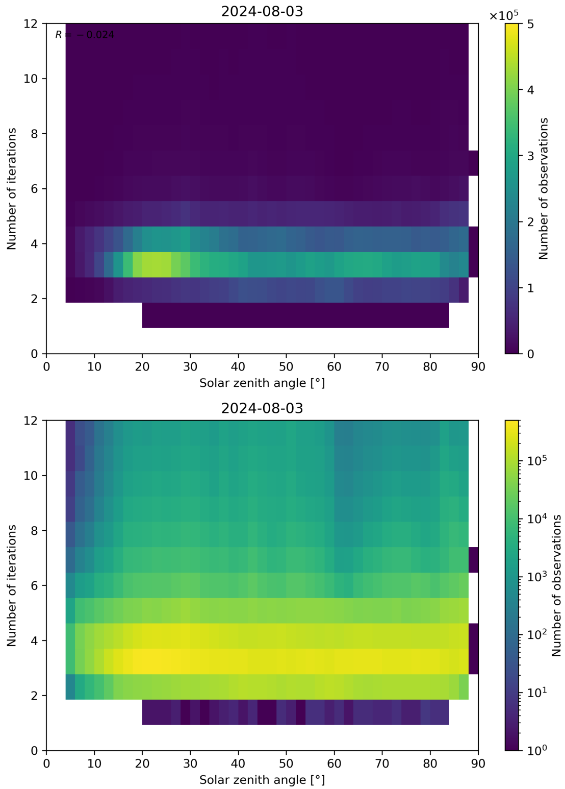
Figure 114: Scatter density plot of “Solar zenith angle” against “Number of iterations” for 2024-08-02 to 2024-08-04.
