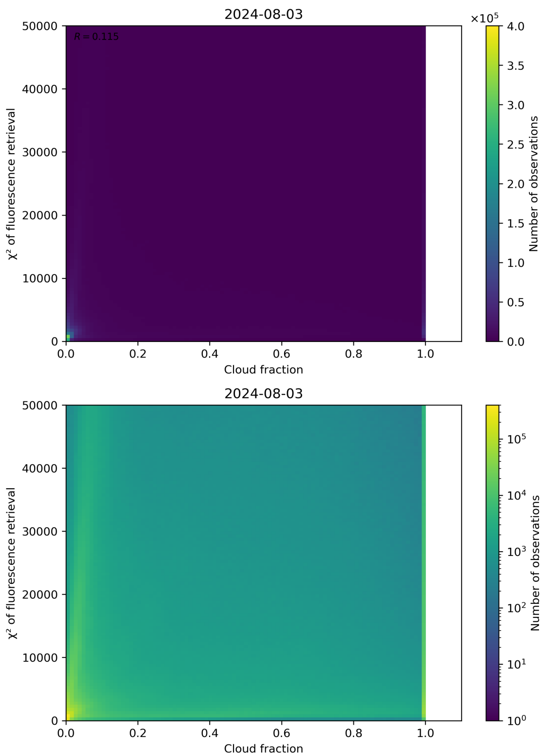
Figure 71: Scatter density plot of “Cloud fraction” against “ \chi^2 of fluorescence retrieval” for 2024-08-02 to 2024-08-04.
