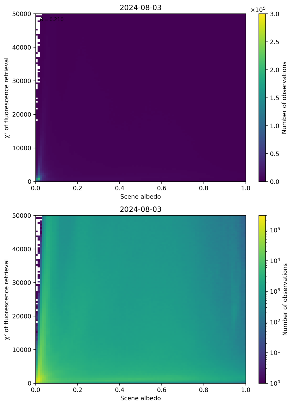
Figure 103: Scatter density plot of “Scene albedo” against “ \chi^2 of fluorescence retrieval” for 2024-08-02 to 2024-08-04.
