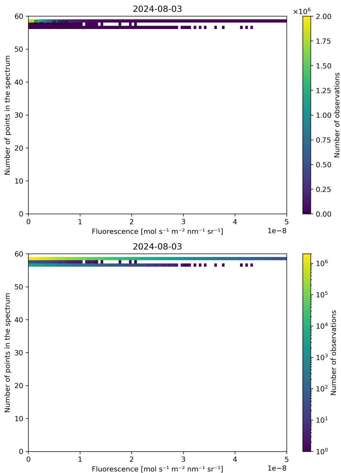
Figure 86: Scatter density plot of “Fluorescence” against “Number of points in the spectrum” for 2024-08-02 to 2024-08-04.
