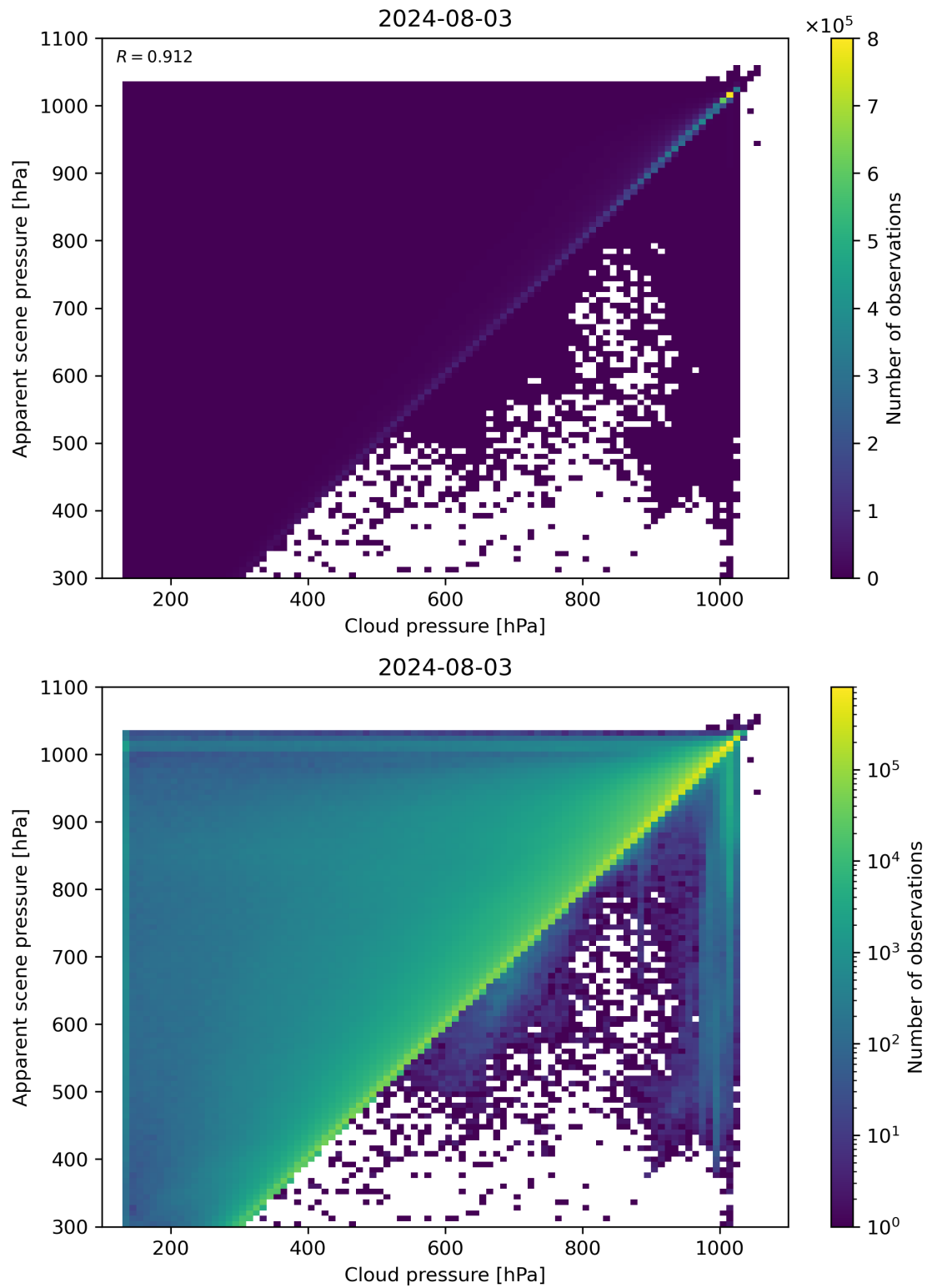
Figure 77: Scatter density plot of “Cloud pressure” against “Apparent scene pressure” for 2024-08-02 to 2024-08-04.
