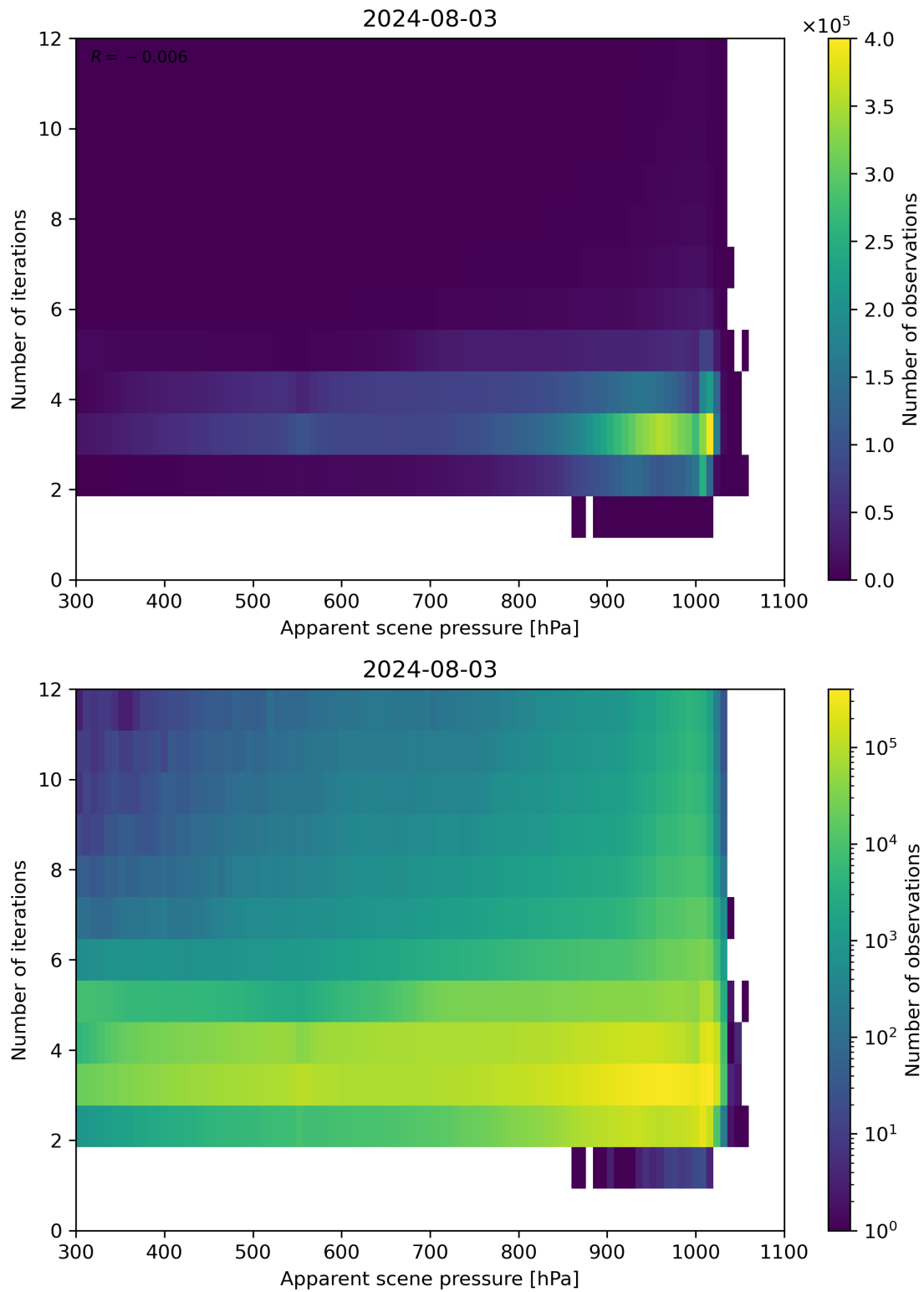
Figure 65: Scatter density plot of “Apparent scene pressure” against “Number of iterations” for 2024-08-02 to 2024-08-04.
