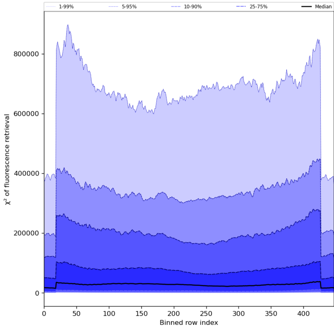
Figure 59: Along track statistics of “ \chi^2 of fluorescence retrieval” for 2024-08-02 to 2024-08-04
