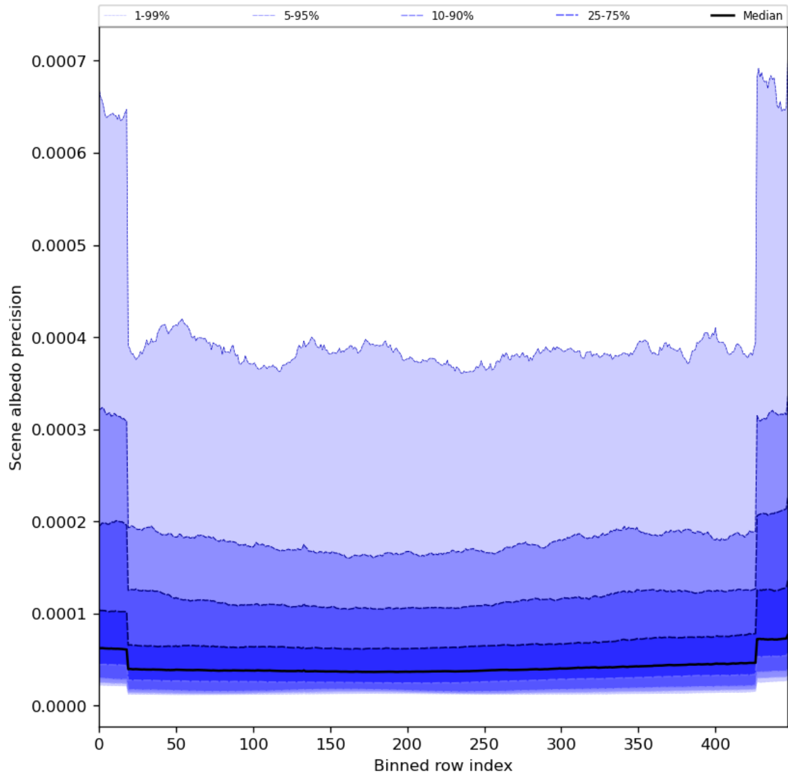
Figure 52: Along track statistics of “Scene albedo precision” for 2024-08-02 to 2024-08-04
