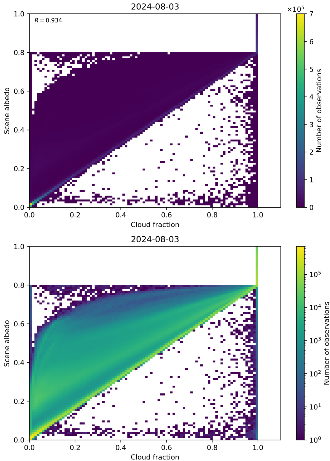
Figure 75: Scatter density plot of “Cloud fraction” against “Scene albedo” for 2024-08-02 to 2024-08-04.
