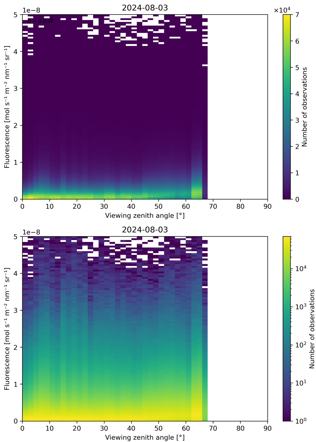
Figure 122: Scatter density plot of “Viewing zenith angle” against “Fluorescence” for 2024-08-02 to 2024-08-04.
