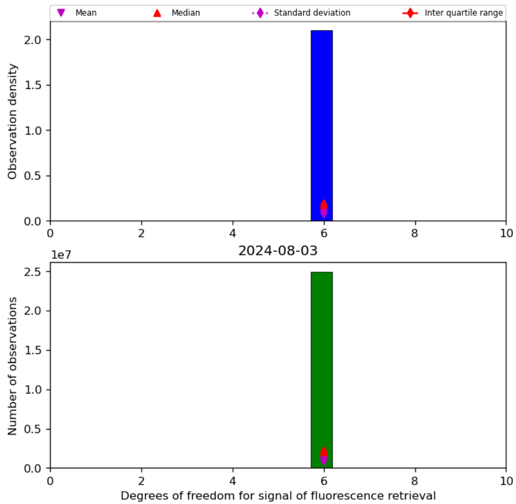
Figure 43: Histogram of “Degrees of freedom for signal of fluorescence retrieval” for 2024-08-02 to 2024-08-04
