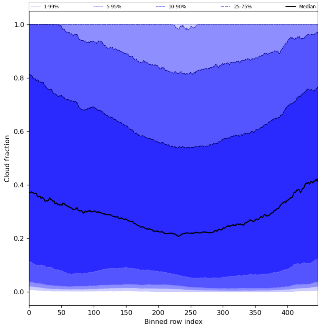
Figure 49: Along track statistics of “Cloud fraction” for 2024-08-02 to 2024-08-04
