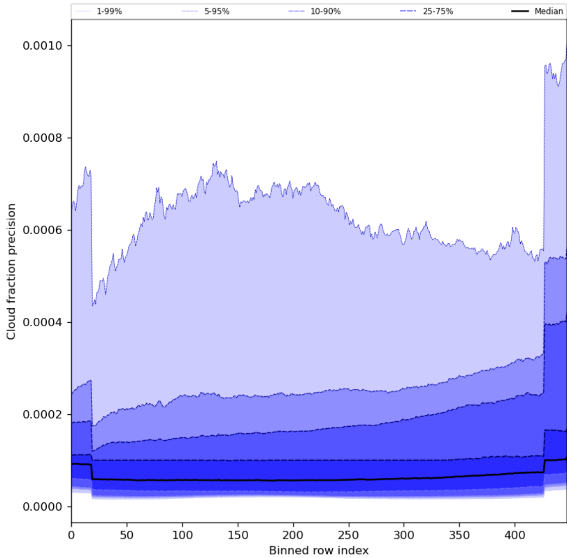
Figure 50: Along track statistics of “Cloud fraction precision” for 2024-08-02 to 2024-08-04
