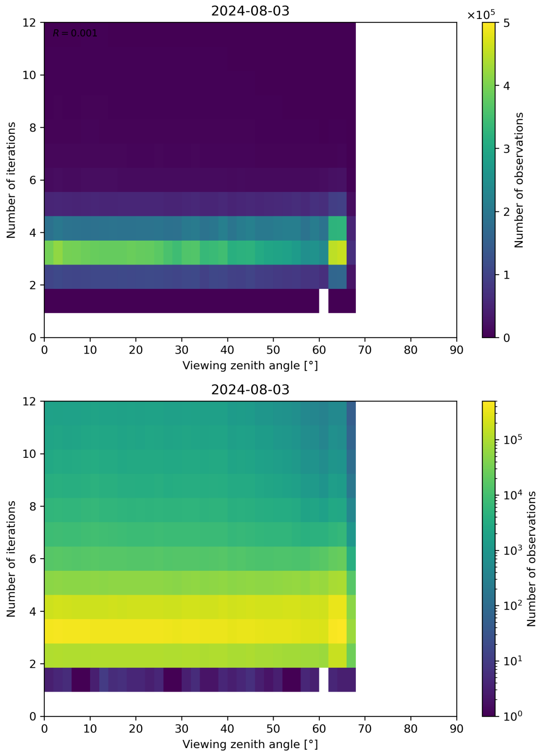
Figure 124: Scatter density plot of “Viewing zenith angle” against “Number of iterations” for 2024-08-02 to 2024-08-04.
