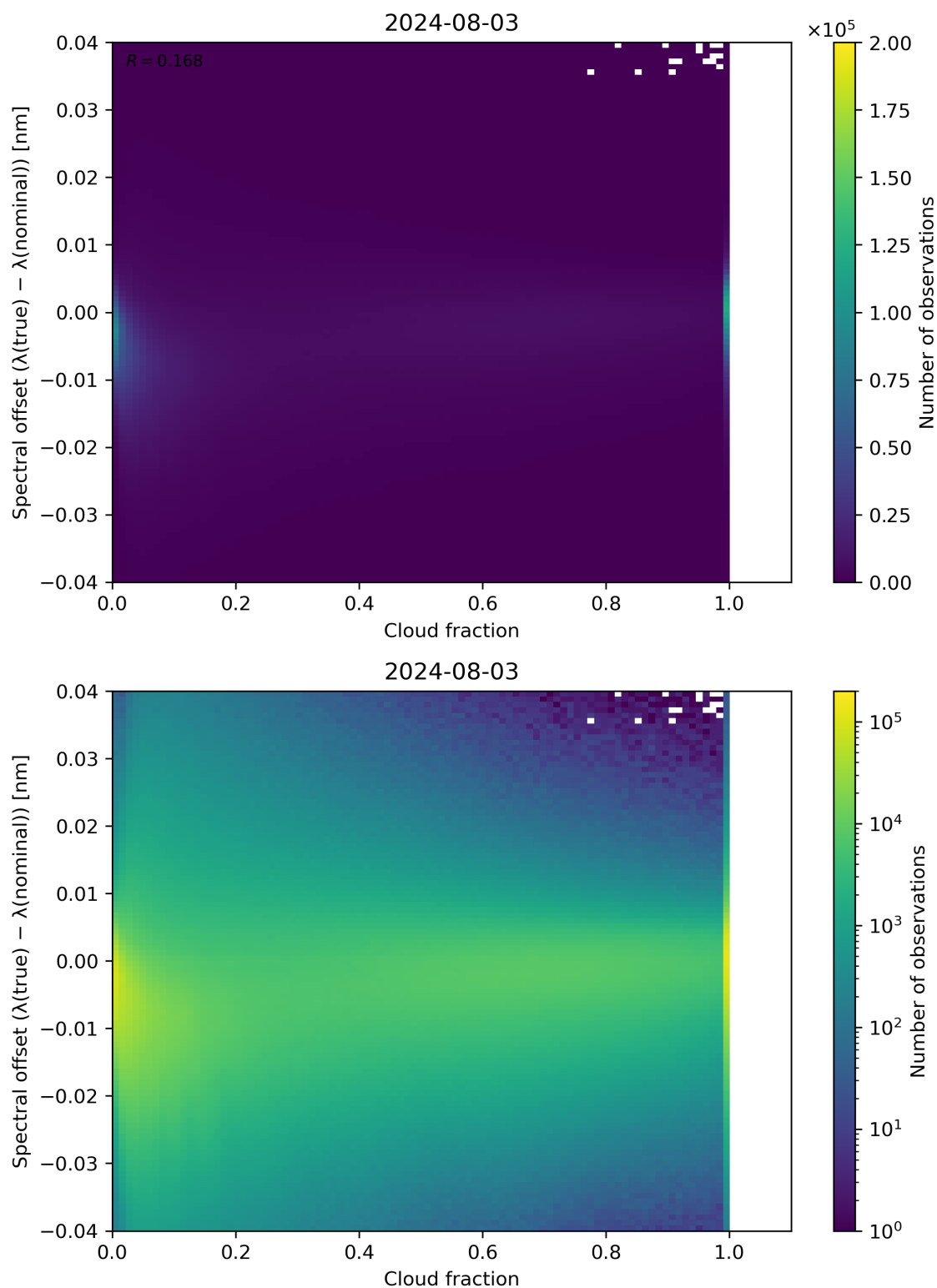
Figure 76: Scatter density plot of “Cloud fraction” against “Spectral offset ( \lambda(\text{true}) - \lambda(\text{nominal}) )” for 2024-08-02 to 2024-08-04.
