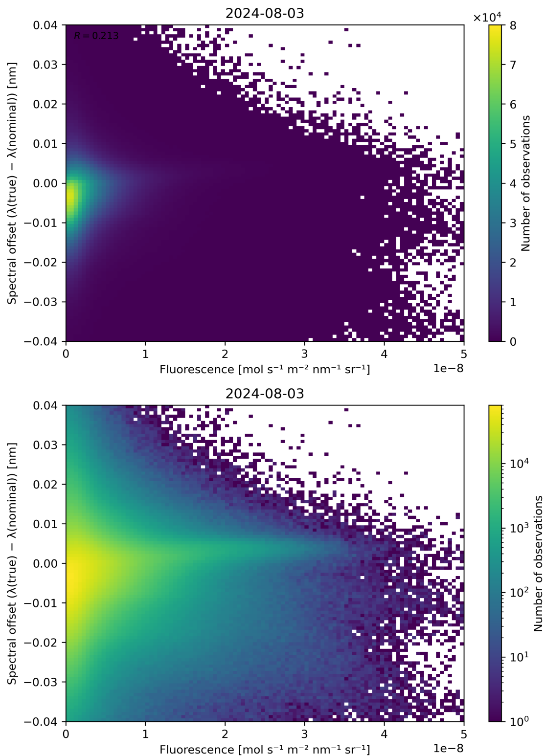
Figure 87: Scatter density plot of “Fluorescence” against “Spectral offset ( \lambda(\text{true}) - \lambda(\text{nominal}) )” for 2024-08-02 to 2024-08-04.
