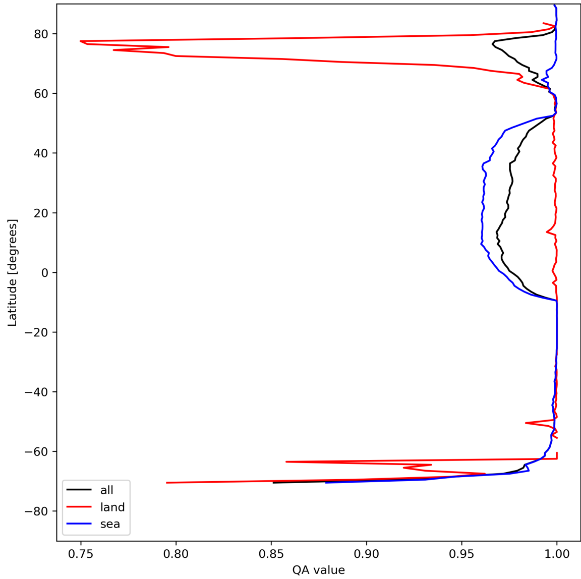
Figure 12: Zonal average of “QA value” for 2024-08-02 to 2024-08-04.
