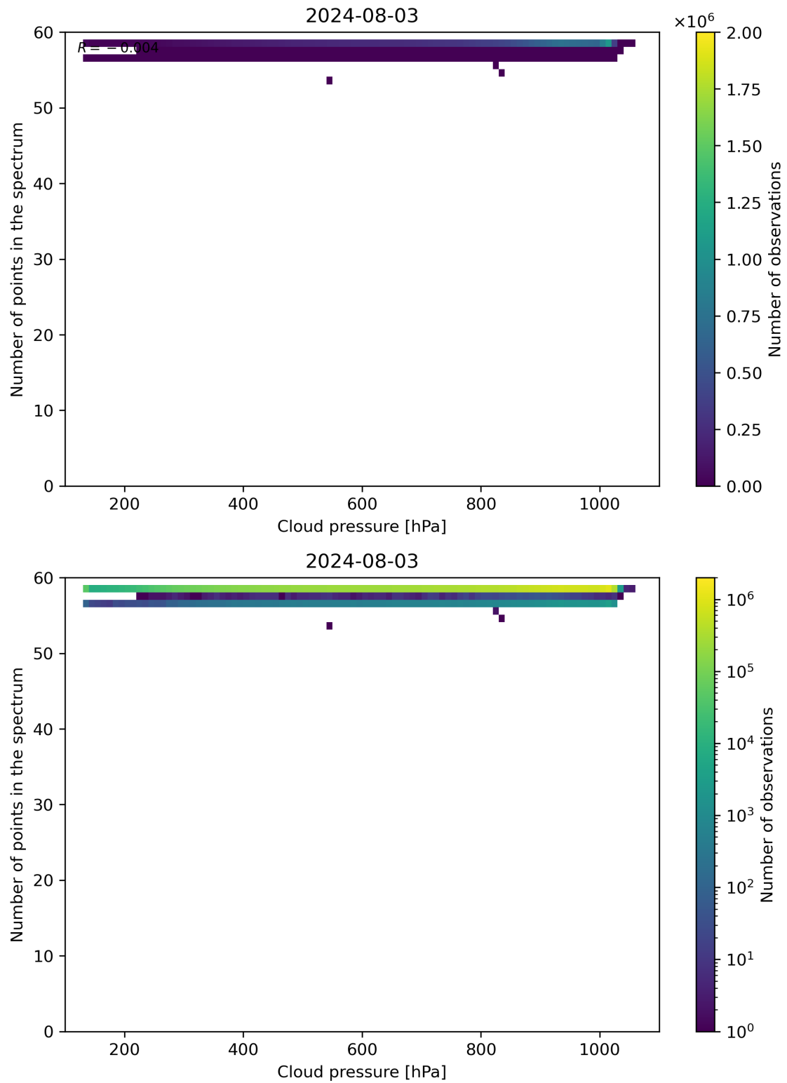
Figure 82: Scatter density plot of “Cloud pressure” against “Number of points in the spectrum” for 2024-08-02 to 2024-08-04.
