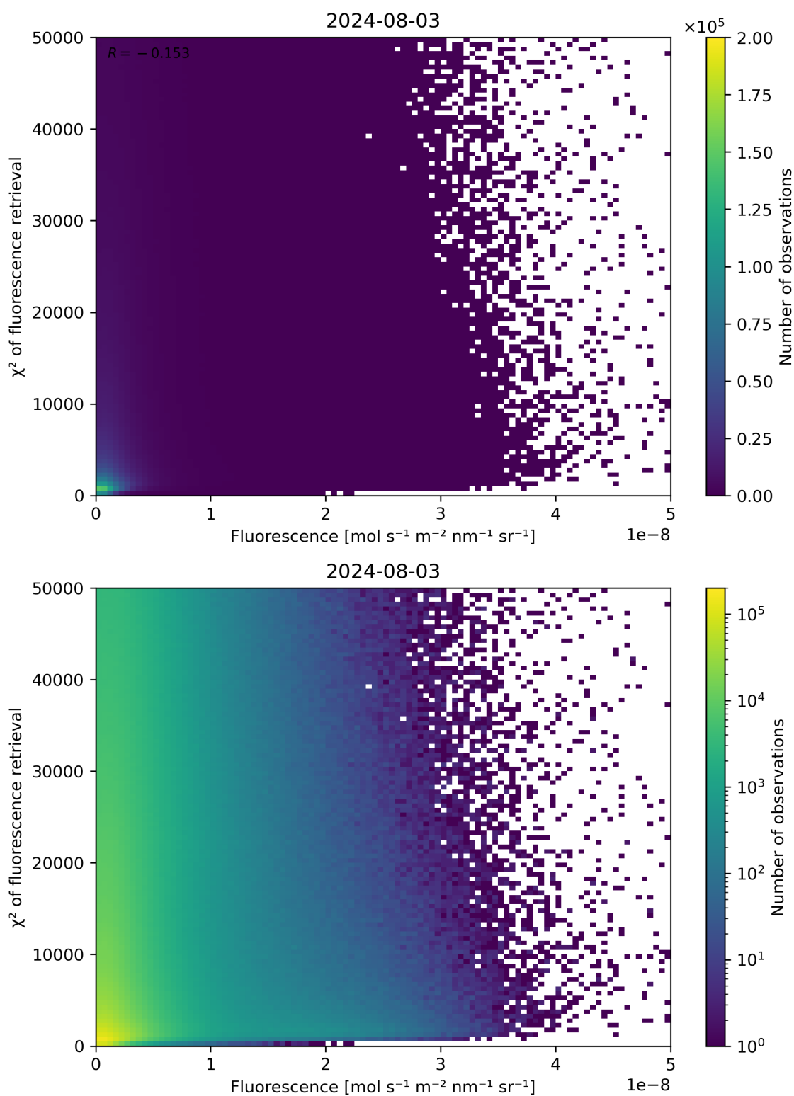
Figure 85: Scatter density plot of “Fluorescence” against “ \chi^2 of fluorescence retrieval” for 2024-08-02 to 2024-08-04.
