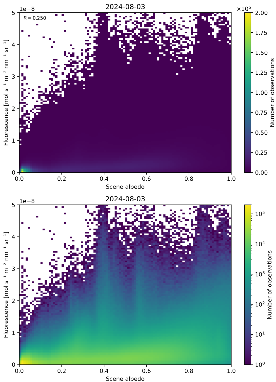
Figure 104: Scatter density plot of “Scene albedo” against “Fluorescence” for 2024-08-02 to 2024-08-04.
