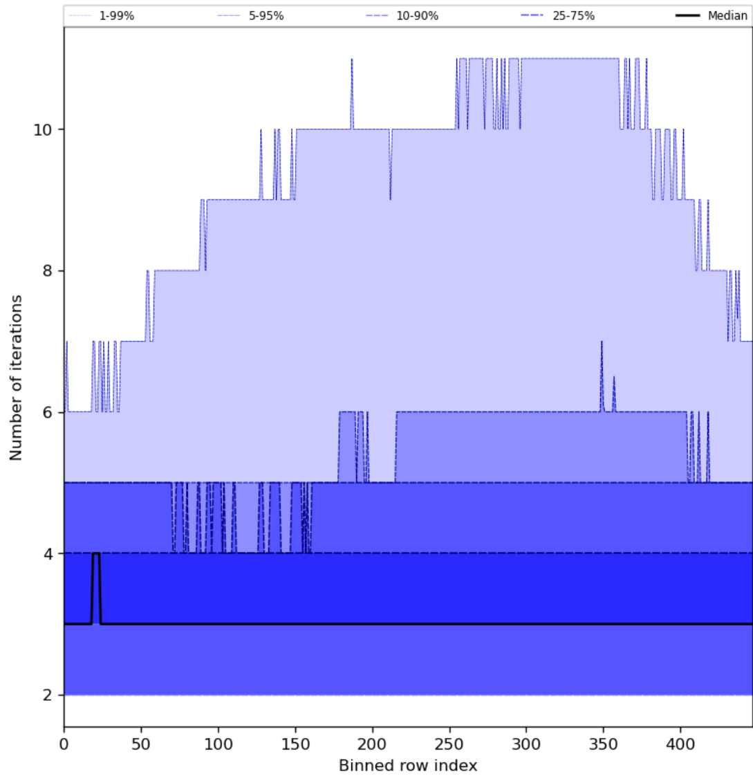
Figure 56: Along track statistics of “Number of iterations” for 2024-08-02 to 2024-08-04
