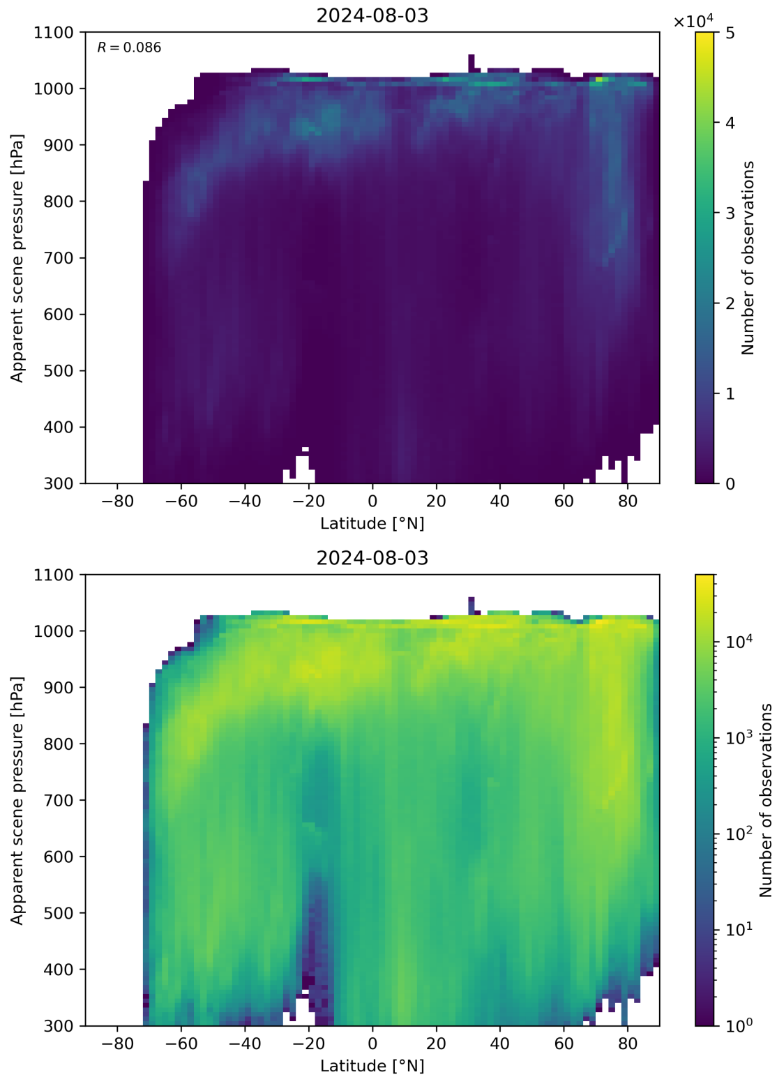
Figure 88: Scatter density plot of “Latitude” against “Apparent scene pressure” for 2024-08-02 to 2024-08-04.
