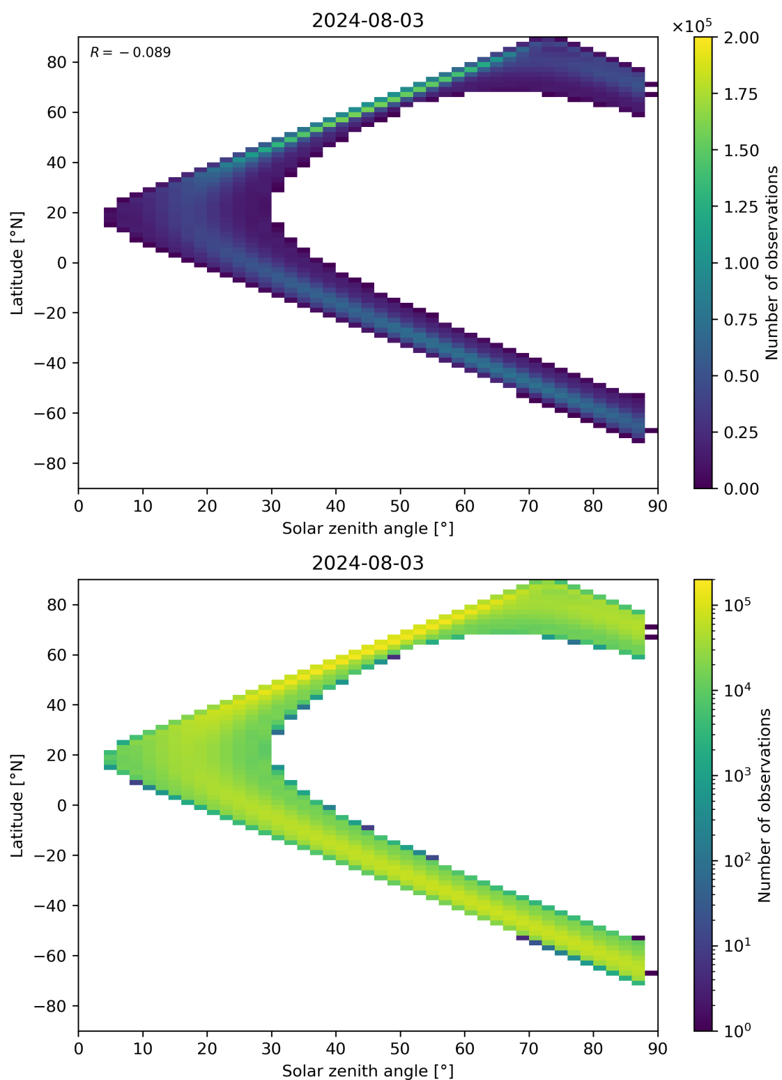
Figure 113: Scatter density plot of “Solar zenith angle” against “Latitude” for 2024-08-02 to 2024-08-04.
