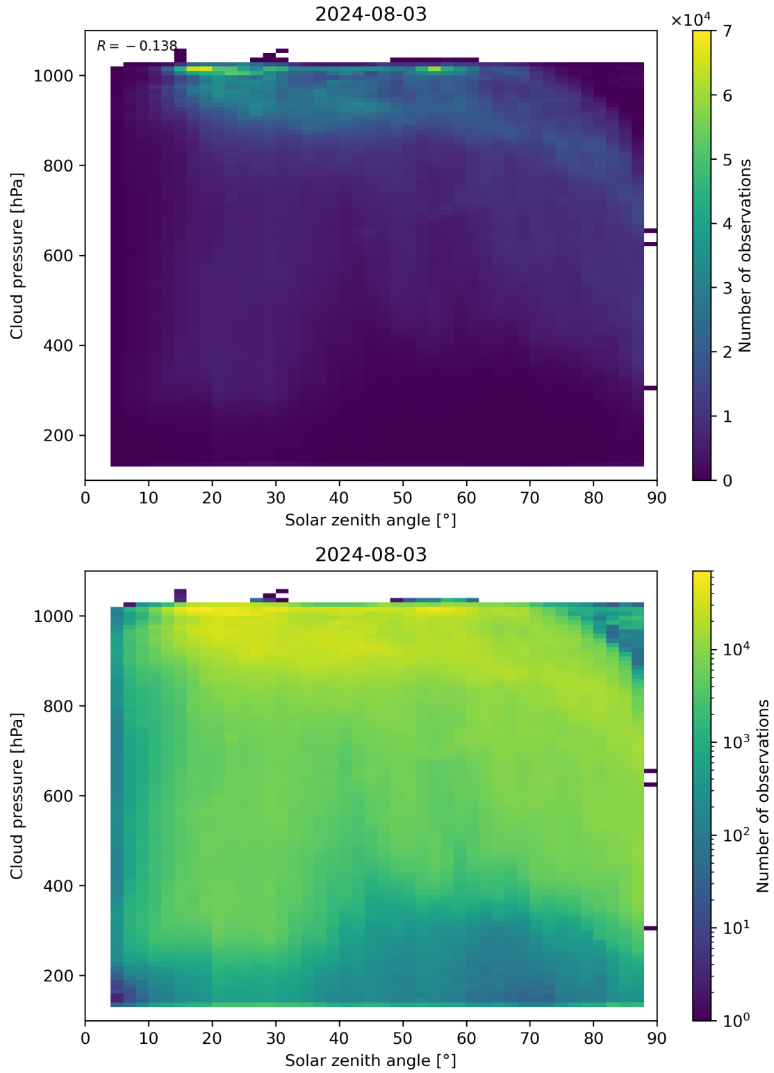
Figure 111: Scatter density plot of “Solar zenith angle” against “Cloud pressure” for 2024-08-02 to 2024-08-04.
