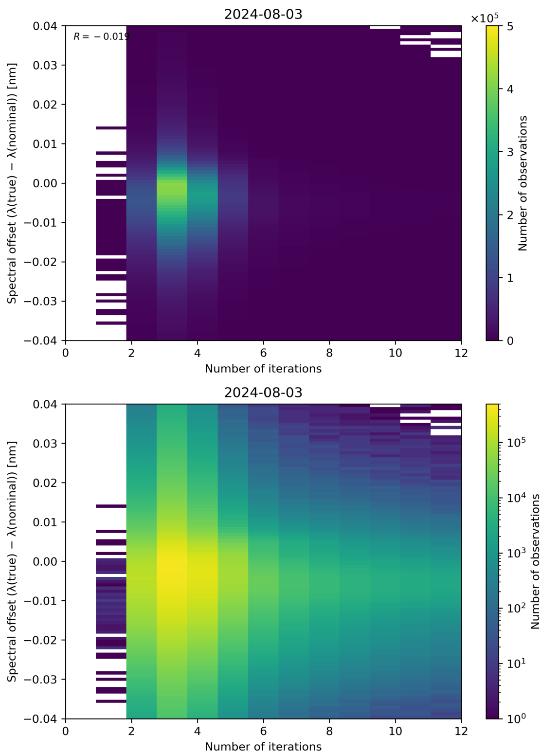
Figure 100: Scatter density plot of “Number of iterations” against “Spectral offset ( \lambda(\text{true}) - \lambda(\text{nominal}) )” for 2024-08-02 to 2024-08-04.
