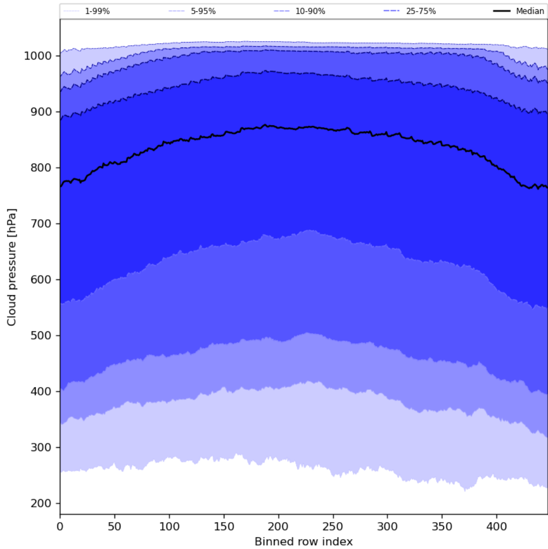
Figure 47: Along track statistics of “Cloud pressure” for 2024-08-02 to 2024-08-04
