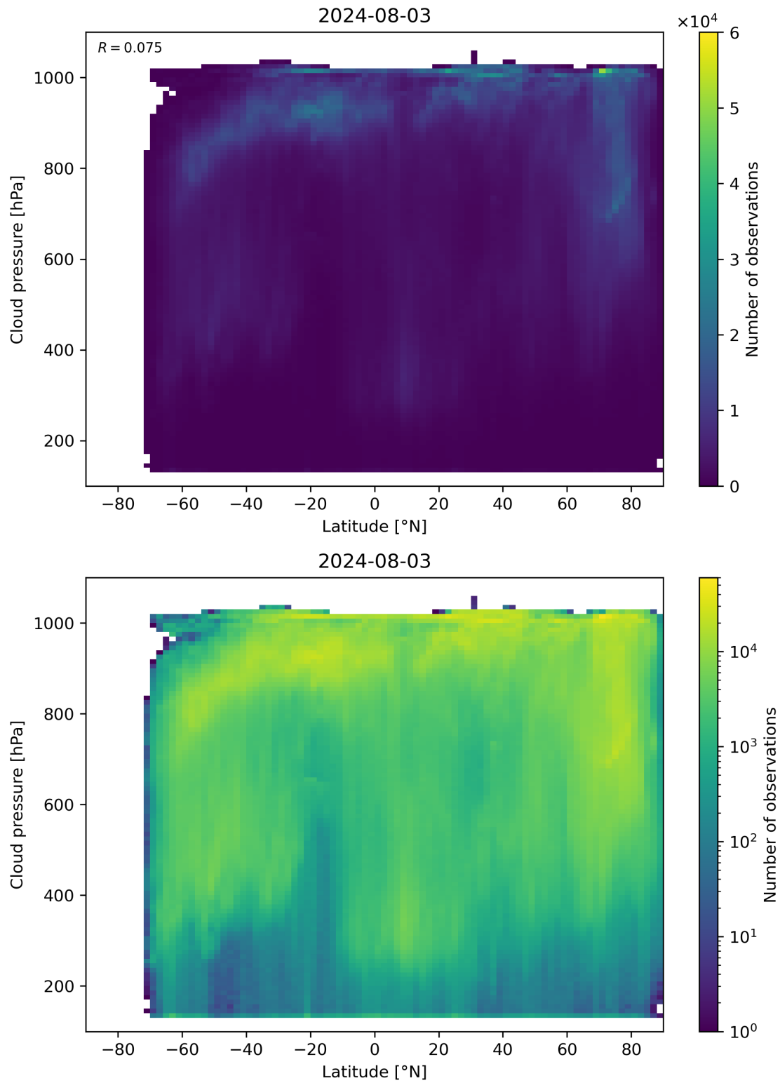
Figure 91: Scatter density plot of “Latitude” against “Cloud pressure” for 2024-08-02 to 2024-08-04.
