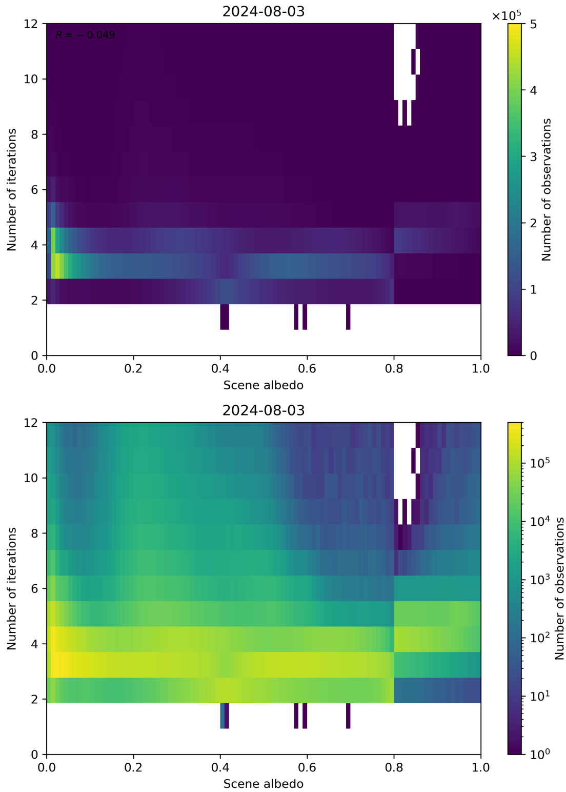
Figure 105: Scatter density plot of “Scene albedo” against “Number of iterations” for 2024-08-02 to 2024-08-04.
