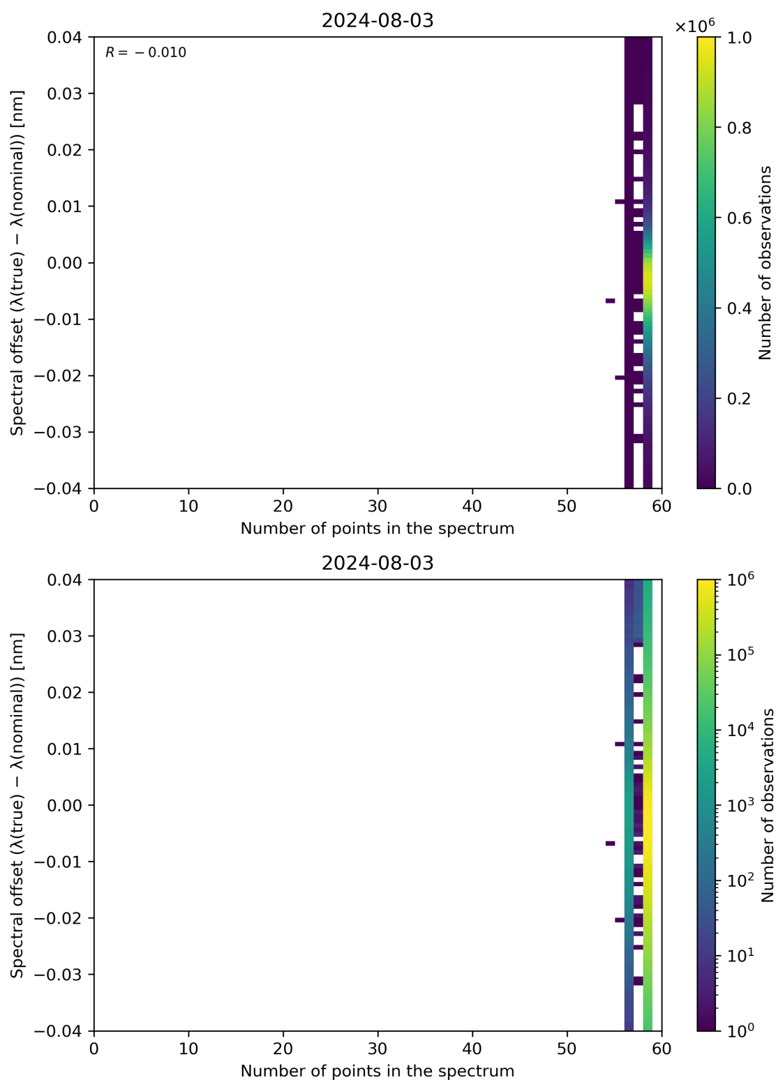
Figure 101: Scatter density plot of “Number of points in the spectrum” against “Spectral offset ( \lambda(\text{true}) - \lambda(\text{nominal}) )” for 2024-08-02 to 2024-08-04.
