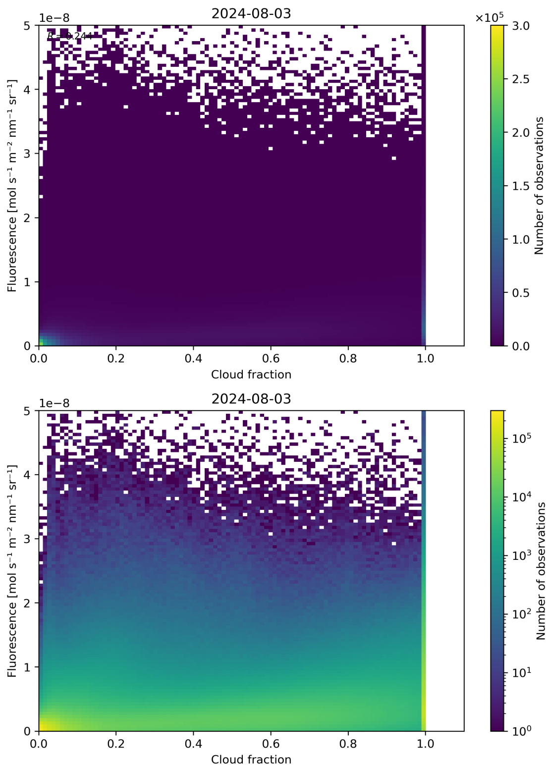
Figure 72: Scatter density plot of “Cloud fraction” against “Fluorescence” for 2024-08-02 to 2024-08-04.
