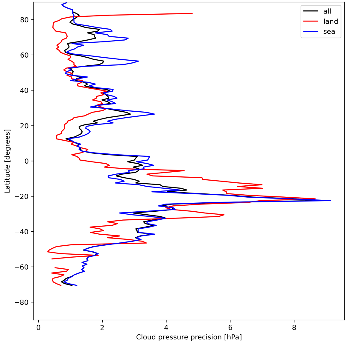
Figure 14: Zonal average of “Cloud pressure precision” for 2024-08-02 to 2024-08-04.
