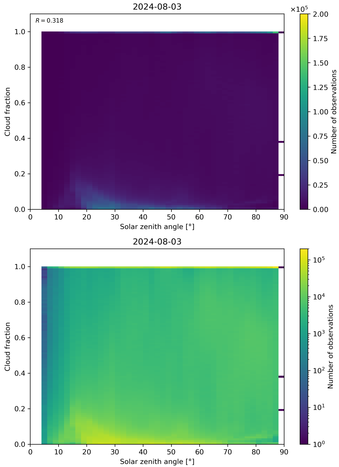
Figure 110: Scatter density plot of “Solar zenith angle” against “Cloud fraction” for 2024-08-02 to 2024-08-04.
