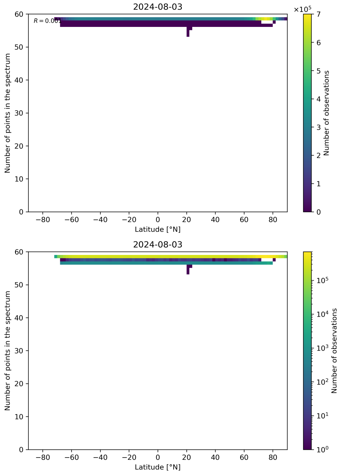
Figure 94: Scatter density plot of “Latitude” against “Number of points in the spectrum” for 2024-08-02 to 2024-08-04.
