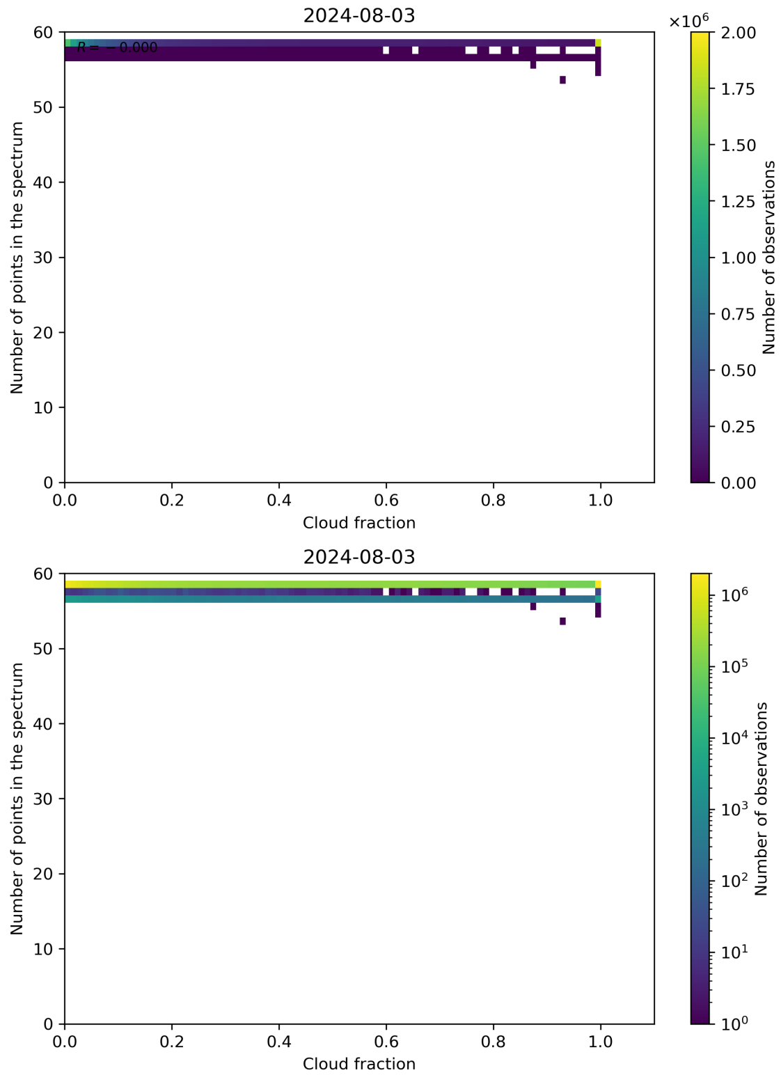
Figure 74: Scatter density plot of “Cloud fraction” against “Number of points in the spectrum” for 2024-08-02 to 2024-08-04.
