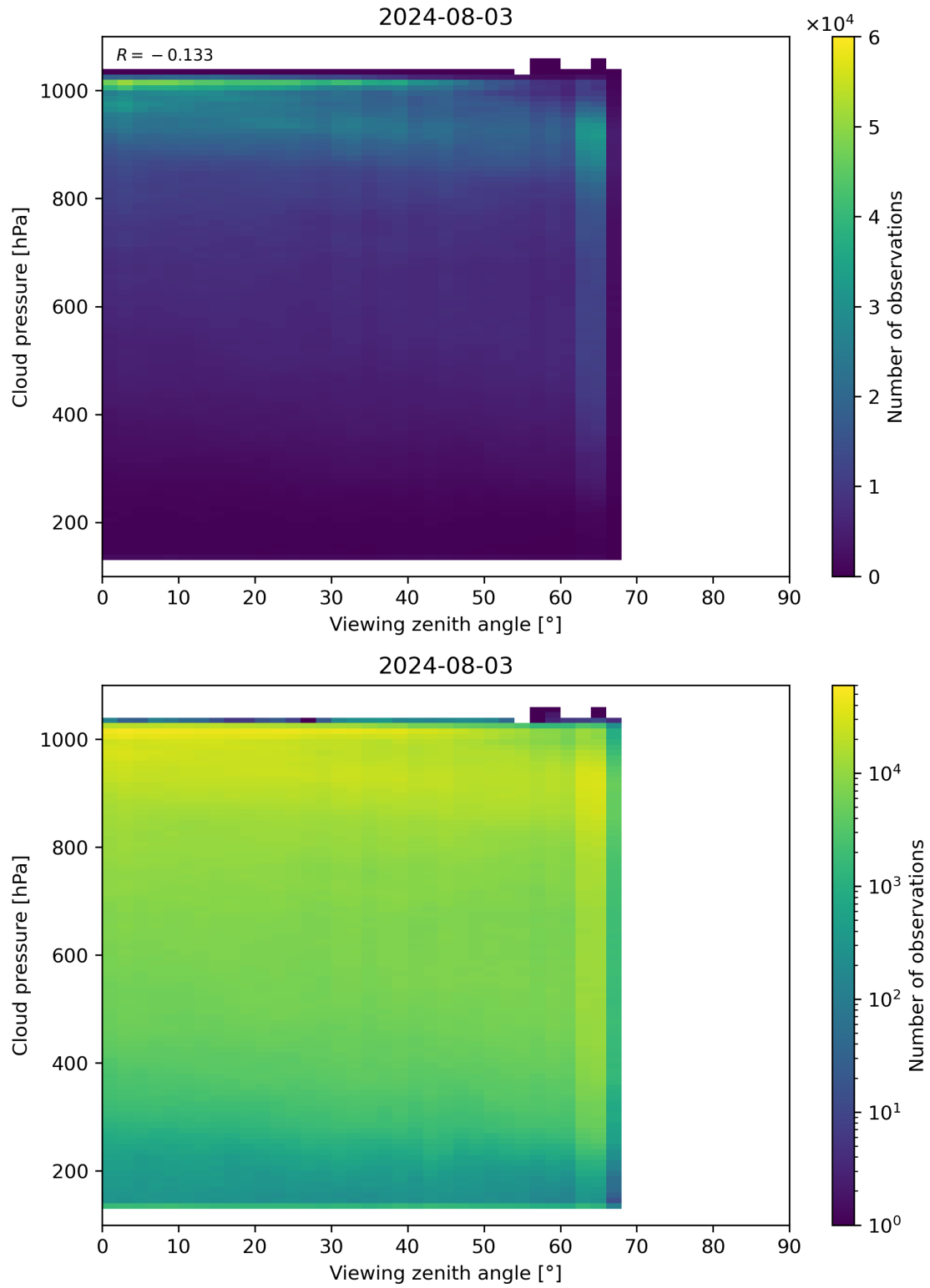
Figure 121: Scatter density plot of “Viewing zenith angle” against “Cloud pressure” for 2024-08-02 to 2024-08-04.
