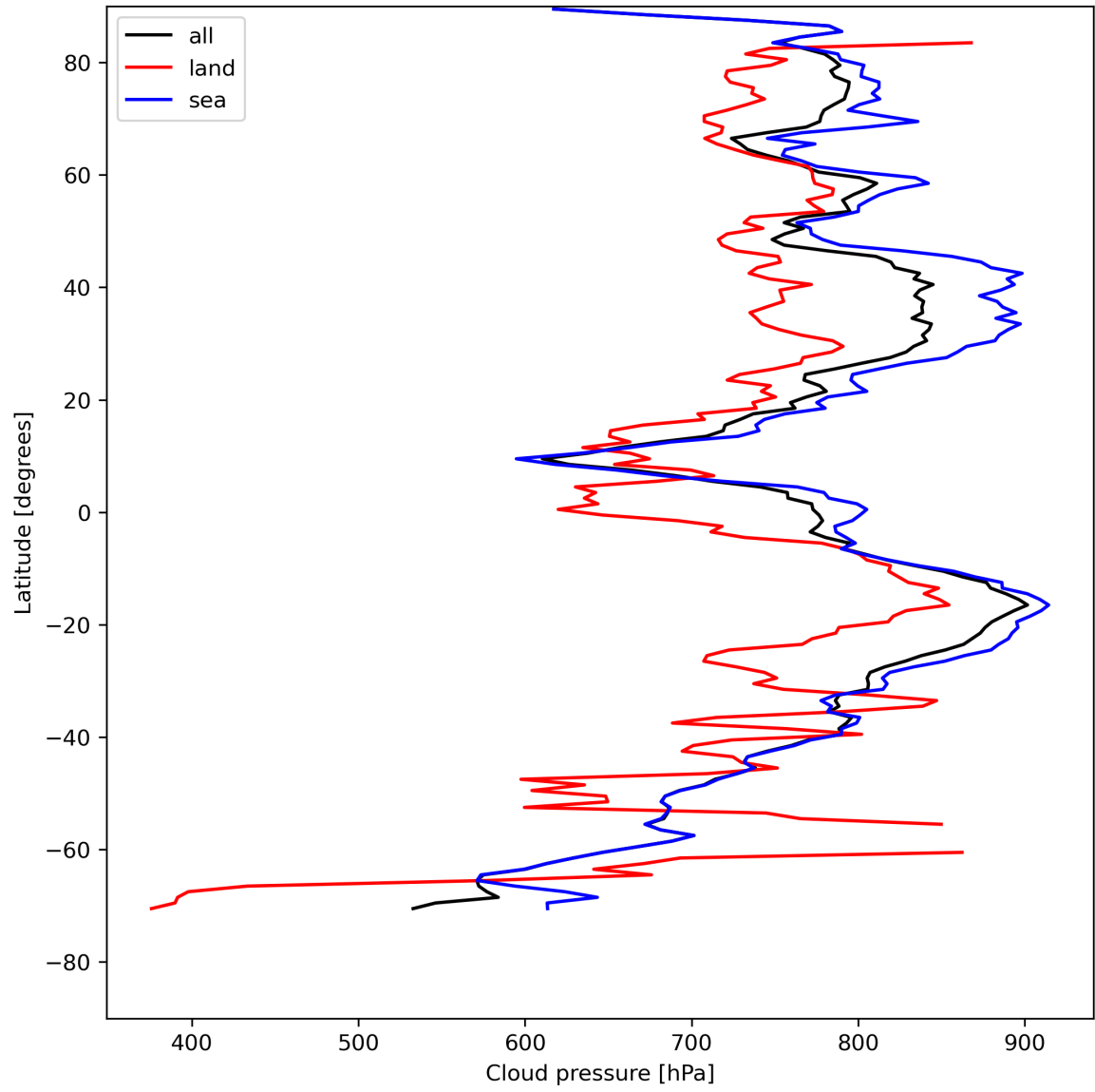
Figure 13: Zonal average of “Cloud pressure” for 2024-08-02 to 2024-08-04.
