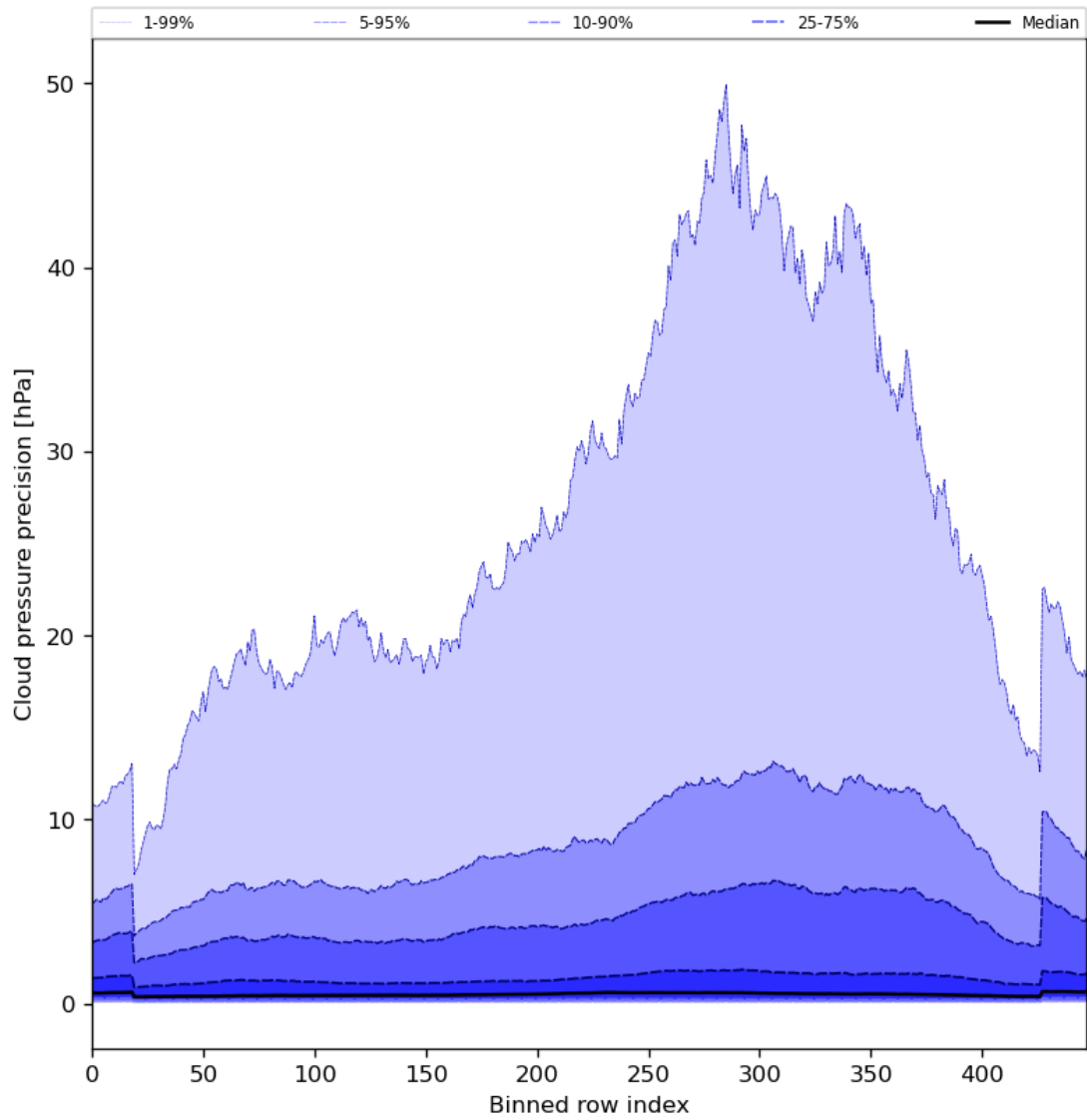
Figure 48: Along track statistics of “Cloud pressure precision” for 2024-08-02 to 2024-08-04
