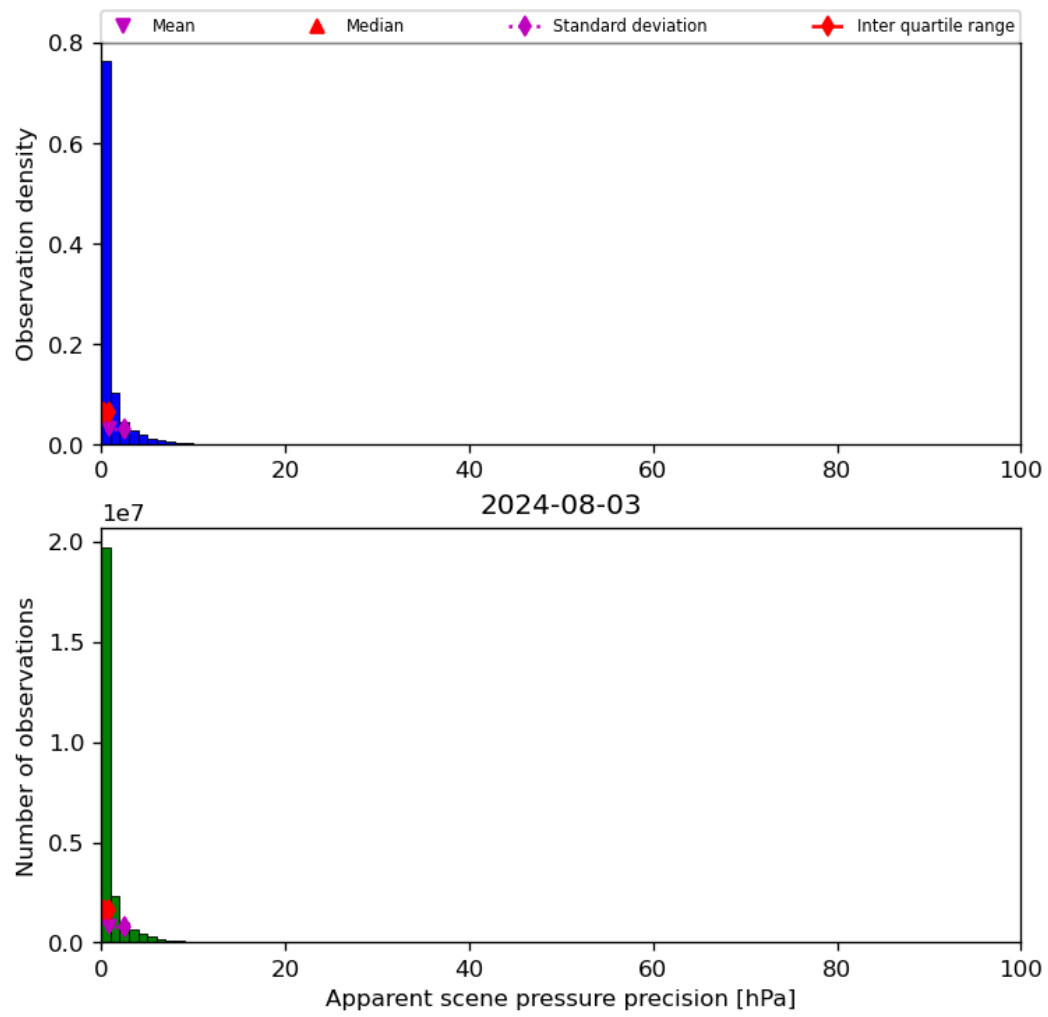
Figure 37: Histogram of “Apparent scene pressure precision” for 2024-08-02 to 2024-08-04
