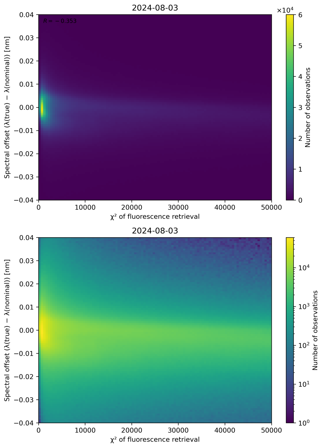
Figure 69: Scatter density plot of " \chi^2 of fluorescence retrieval" against "Spectral offset ( \lambda(\text{true}) - \lambda(\text{nominal})) " for 2024-08-02 to 2024-08-04.
