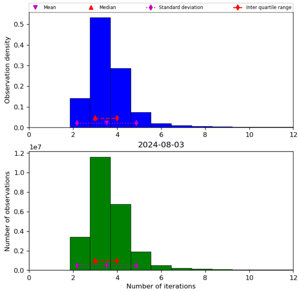
Figure 39: Histogram of “Number of iterations” for 2024-08-02 to 2024-08-04
