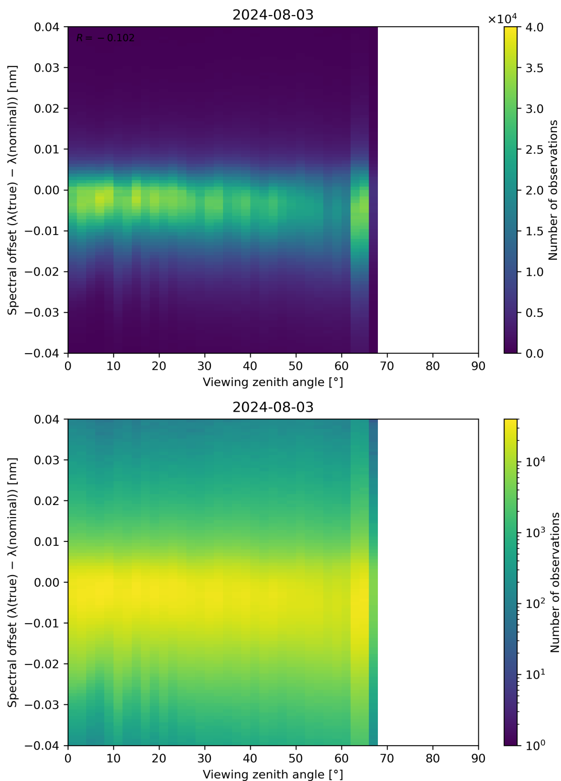
Figure 128: Scatter density plot of “Viewing zenith angle” against “Spectral offset ( \lambda(\text{true}) - \lambda(\text{nominal}) )” for 2024-08-02 to 2024-08-04.
