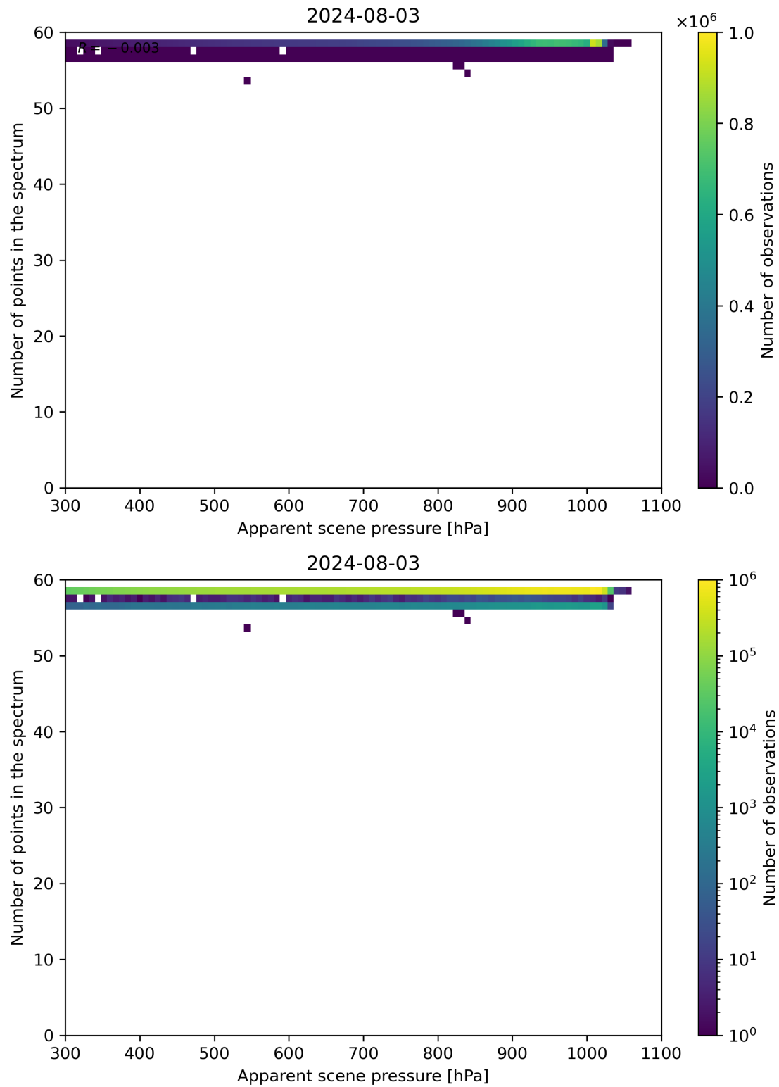
Figure 66: Scatter density plot of “Apparent scene pressure” against “Number of points in the spectrum” for 2024-08-02 to 2024-08-04.
