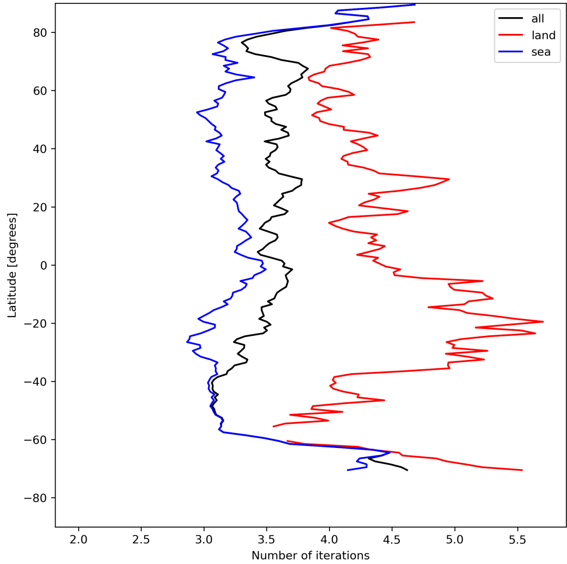
Figure 22: Zonal average of “Number of iterations” for 2024-08-02 to 2024-08-04.
