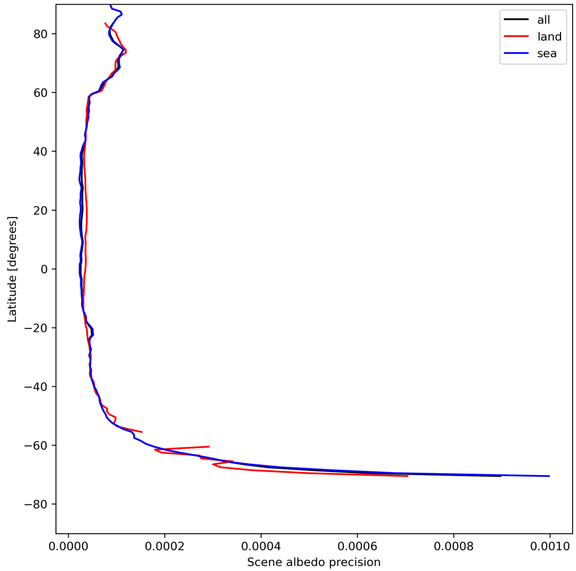
Figure 18: Zonal average of “Scene albedo precision” for 2024-08-02 to 2024-08-04.
