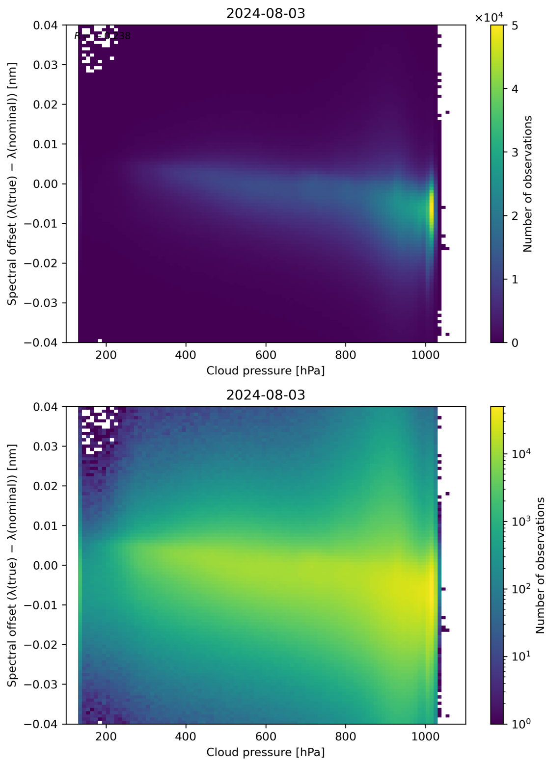
Figure 84: Scatter density plot of “Cloud pressure” against “Spectral offset ( \lambda(\text{true}) - \lambda(\text{nominal}) )” for 2024-08-02 to 2024-08-04.
