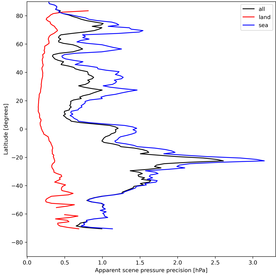
Figure 20: Zonal average of “Apparent scene pressure precision” for 2024-08-02 to 2024-08-04.
