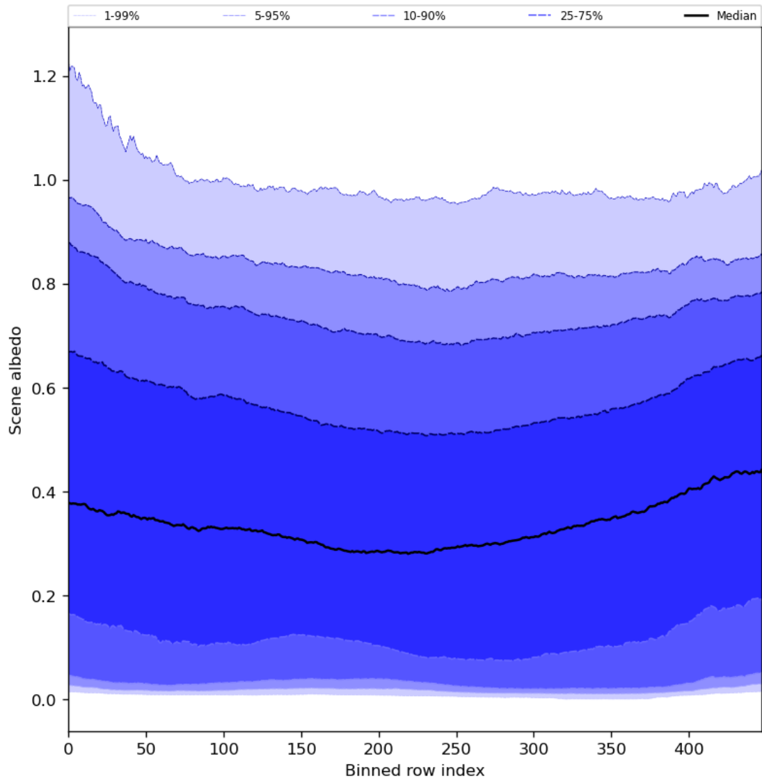
Figure 51: Along track statistics of “Scene albedo” for 2024-08-02 to 2024-08-04
