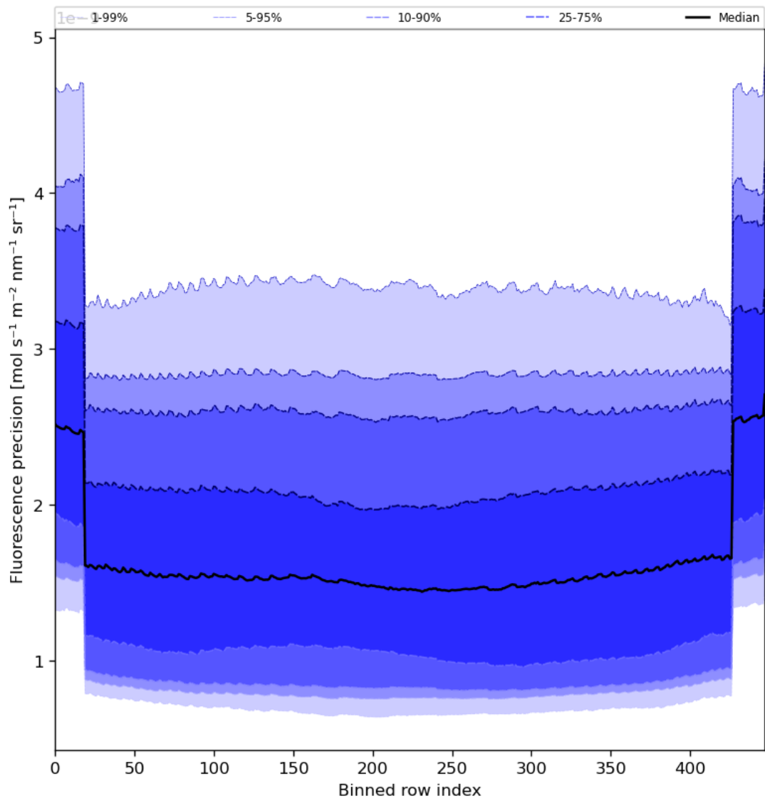
Figure 58: Along track statistics of “Fluorescence precision” for 2024-08-02 to 2024-08-04
