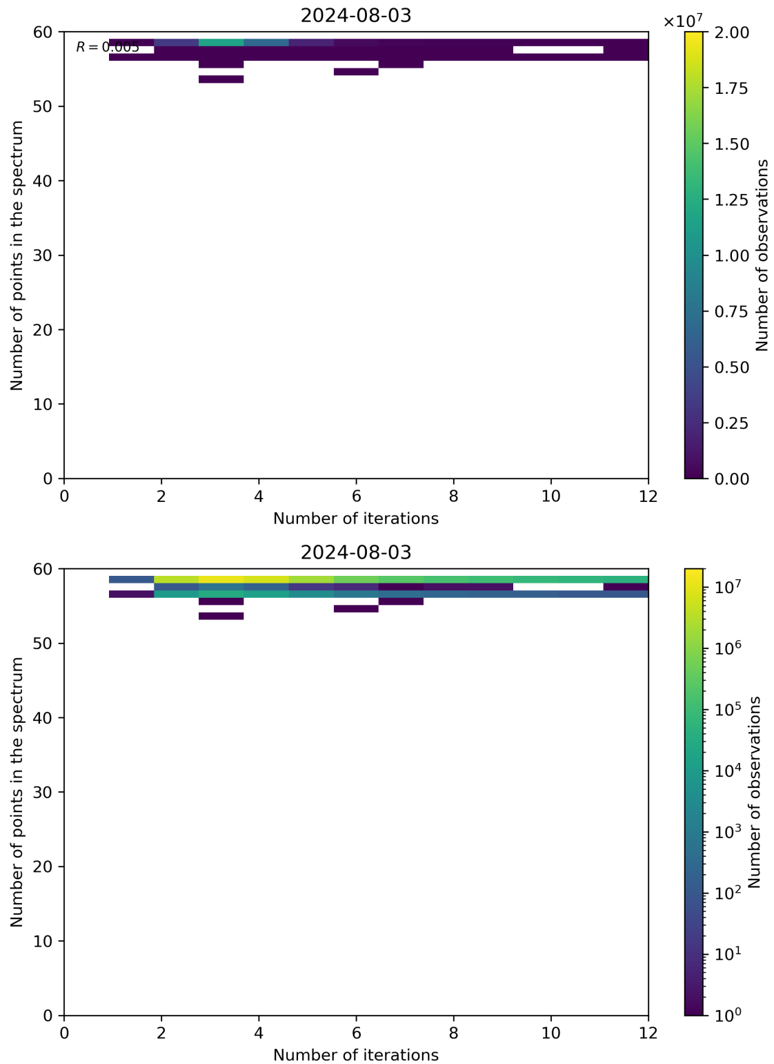
Figure 99: Scatter density plot of “Number of iterations” against “Number of points in the spectrum” for 2024-08-02 to 2024-08-04.
