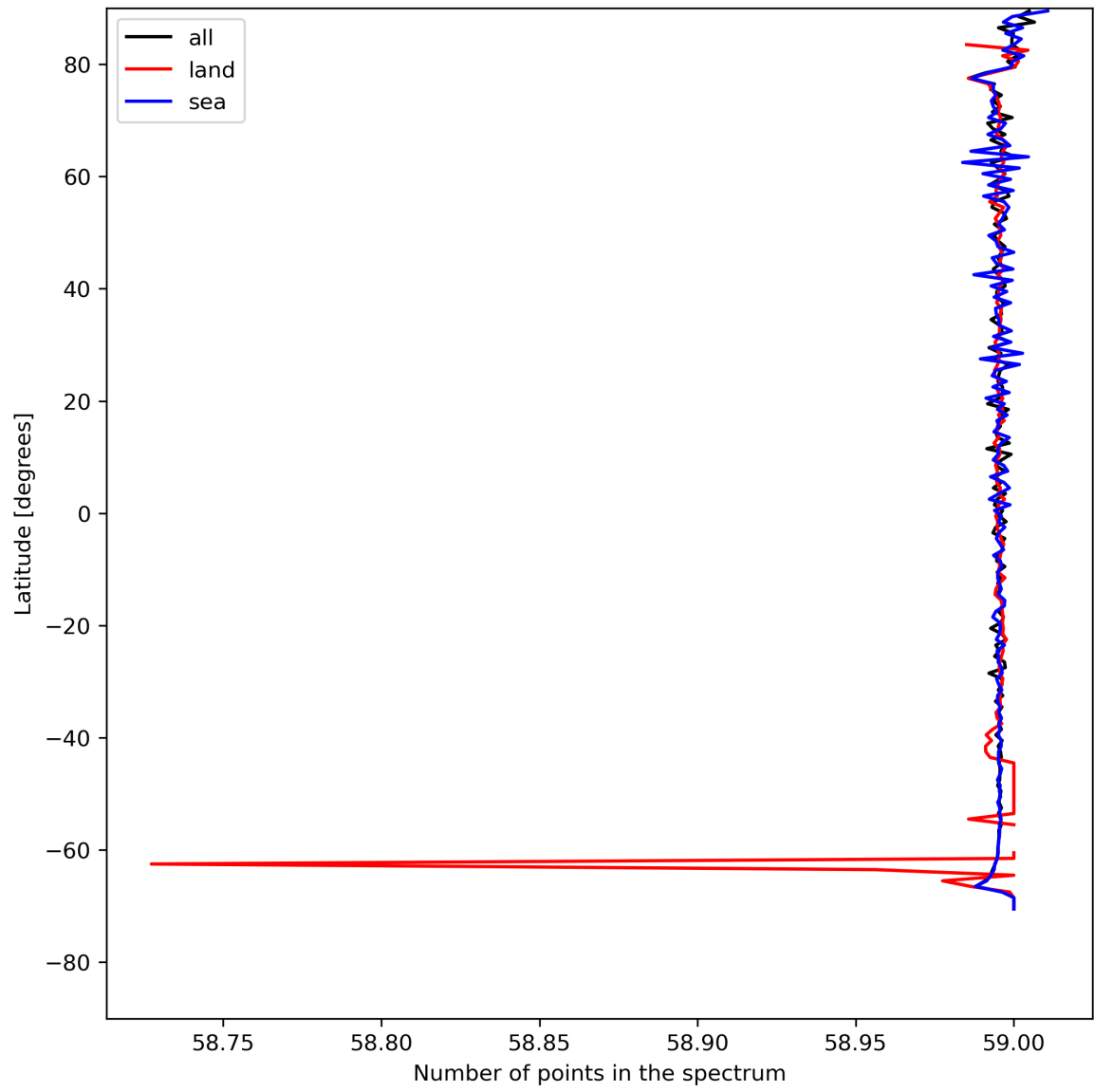
Figure 27: Zonal average of “Number of points in the spectrum” for 2024-08-02 to 2024-08-04.
