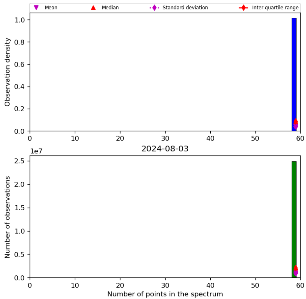
Figure 44: Histogram of “Number of points in the spectrum” for 2024-08-02 to 2024-08-04
