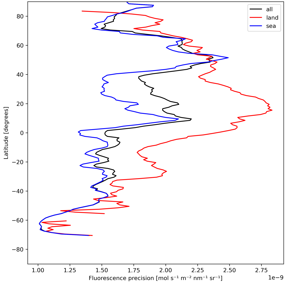
Figure 24: Zonal average of “Fluorescence precision” for 2024-08-02 to 2024-08-04.
