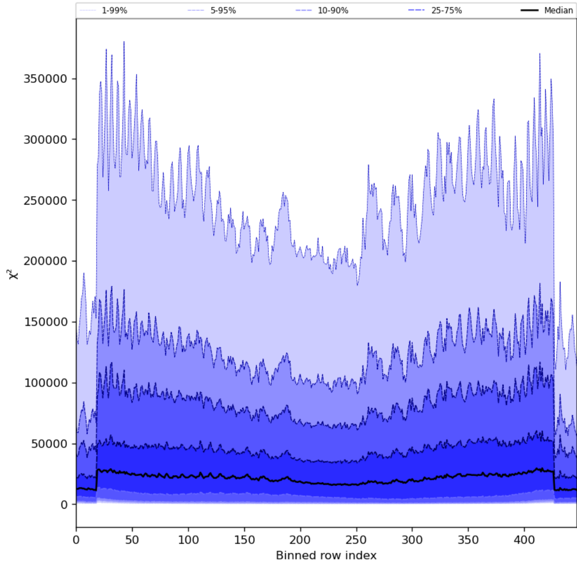
Figure 55: Along track statistics of “ \chi^2 ” for 2024-08-02 to 2024-08-04
