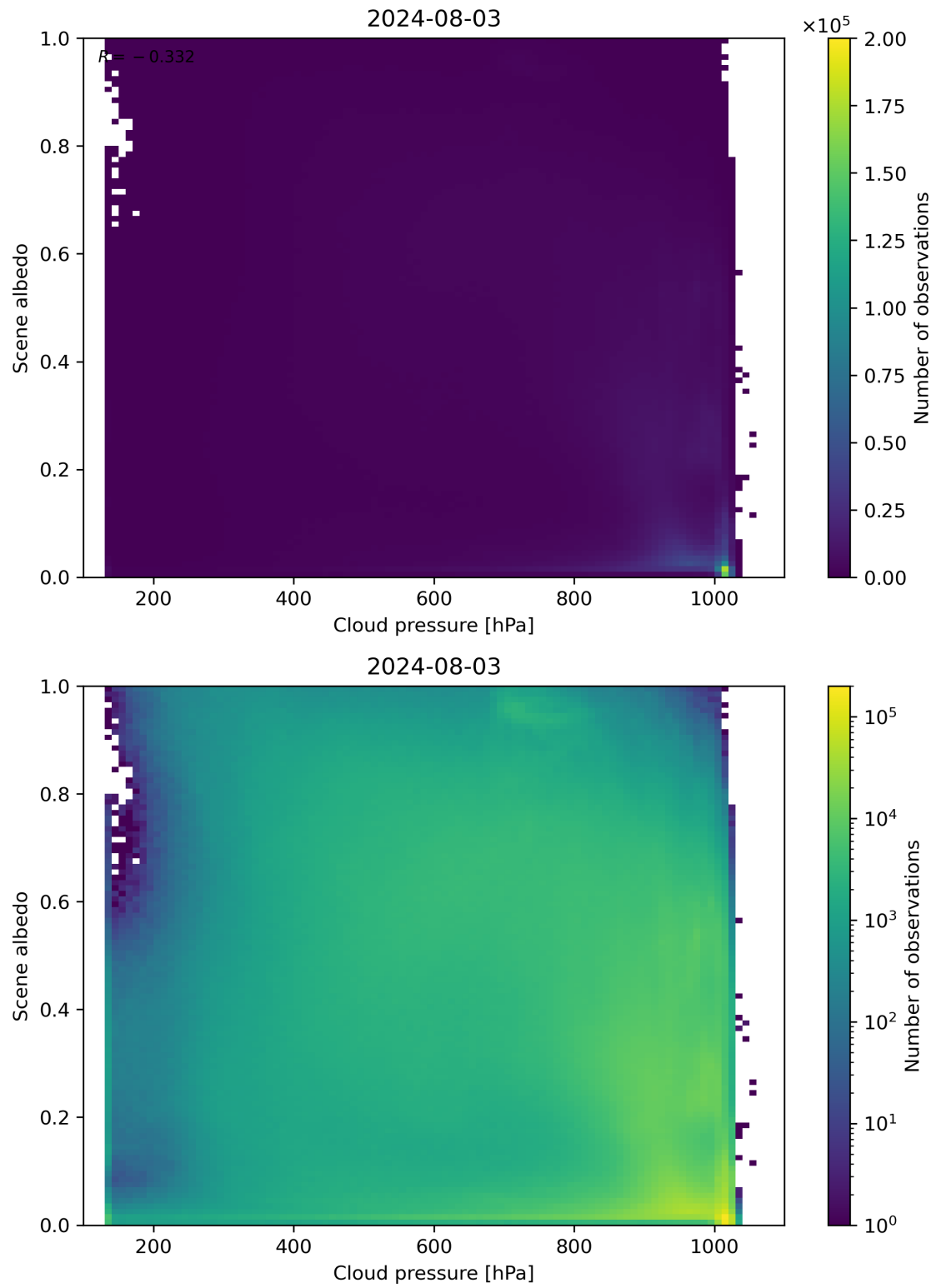
Figure 83: Scatter density plot of “Cloud pressure” against “Scene albedo” for 2024-08-02 to 2024-08-04.
