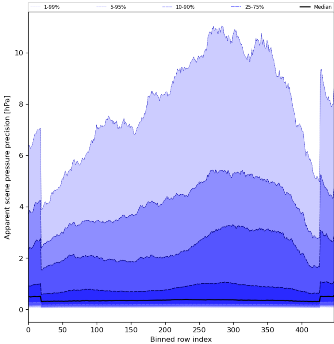
Figure 54: Along track statistics of “Apparent scene pressure precision” for 2024-08-02 to 2024-08-04
