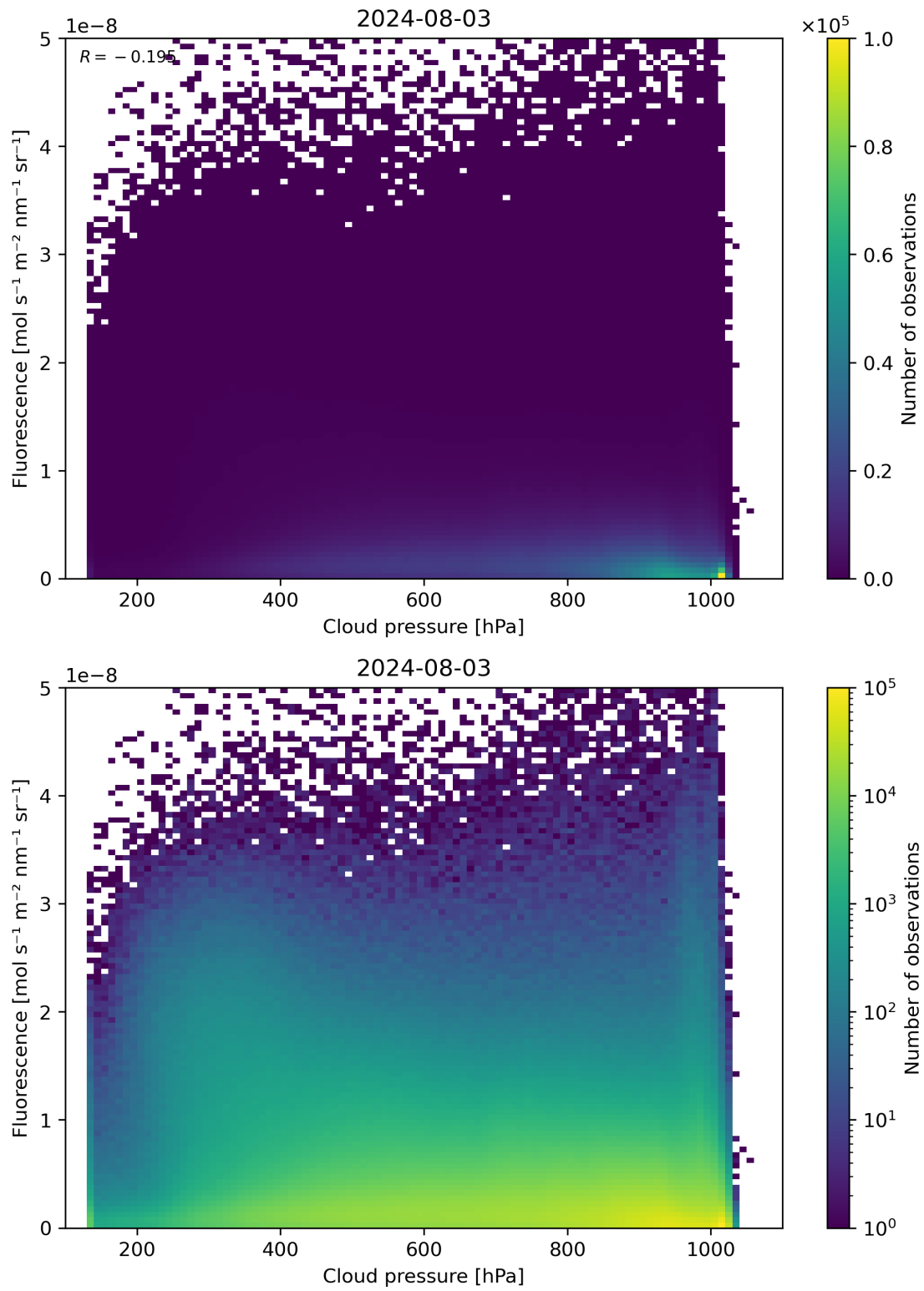
Figure 80: Scatter density plot of “Cloud pressure” against “Fluorescence” for 2024-08-02 to 2024-08-04.
