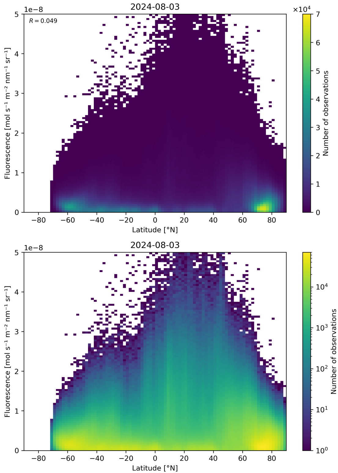
Figure 92: Scatter density plot of “Latitude” against “Fluorescence” for 2024-08-02 to 2024-08-04.
