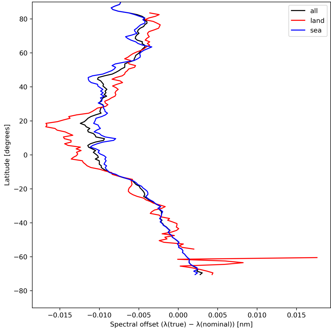
Figure 28: Zonal average of “Spectral offset ( \lambda(\text{true}) - \lambda(\text{nominal}) )” for 2024-08-02 to 2024-08-04.
