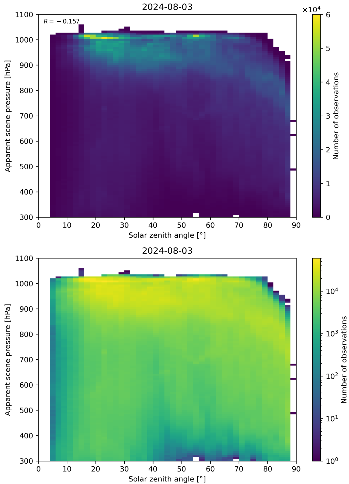
Figure 108: Scatter density plot of “Solar zenith angle” against “Apparent scene pressure” for 2024-08-02 to 2024-08-04.
