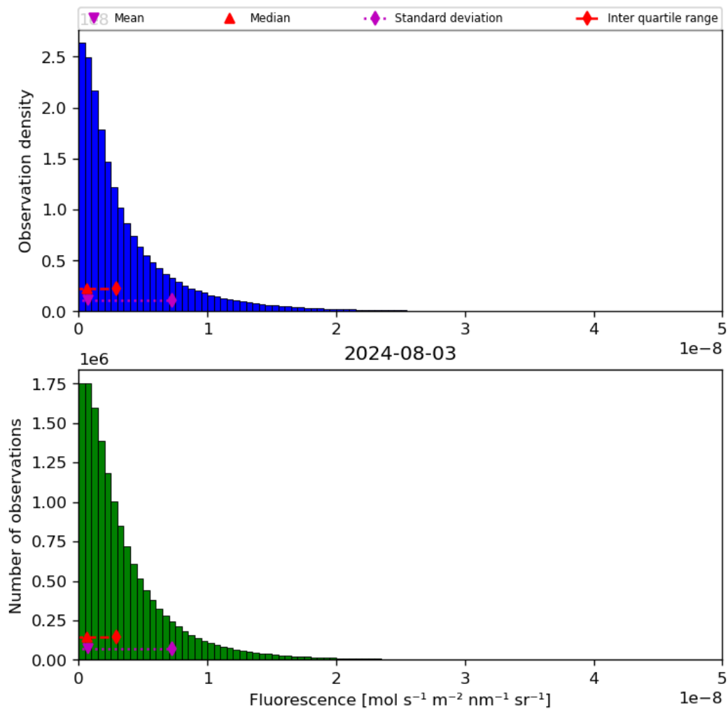
Figure 40: Histogram of “Fluorescence” for 2024-08-02 to 2024-08-04
