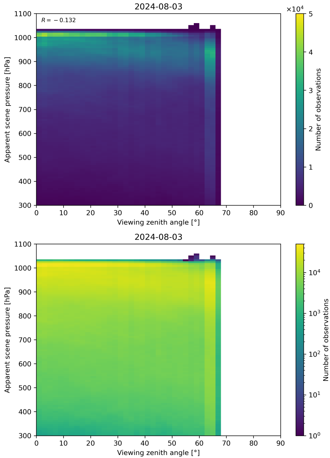
Figure 118: Scatter density plot of “Viewing zenith angle” against “Apparent scene pressure” for 2024-08-02 to 2024-08-04.
