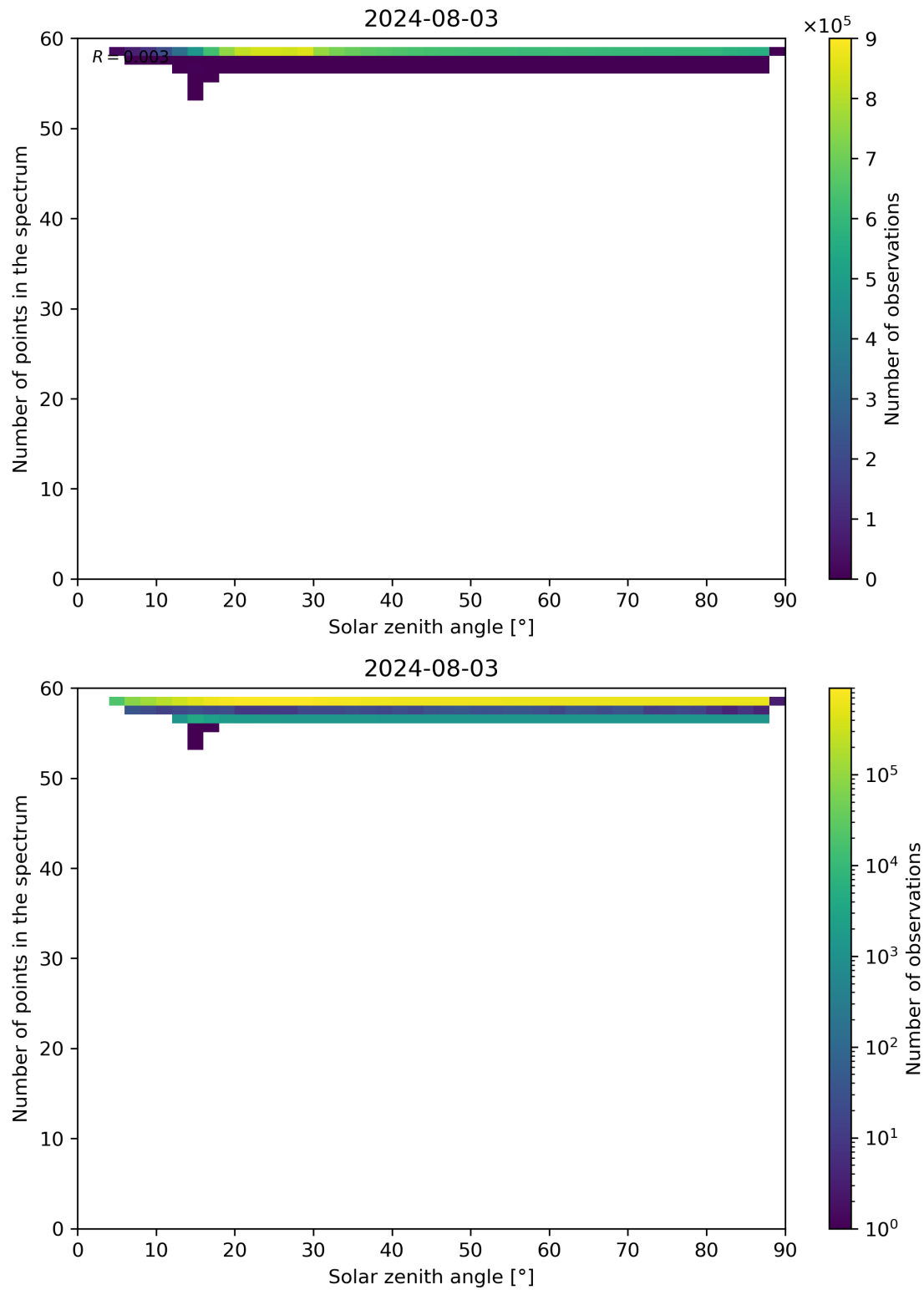
Figure 115: Scatter density plot of “Solar zenith angle” against “Number of points in the spectrum” for 2024-08-02 to 2024-08-04.
