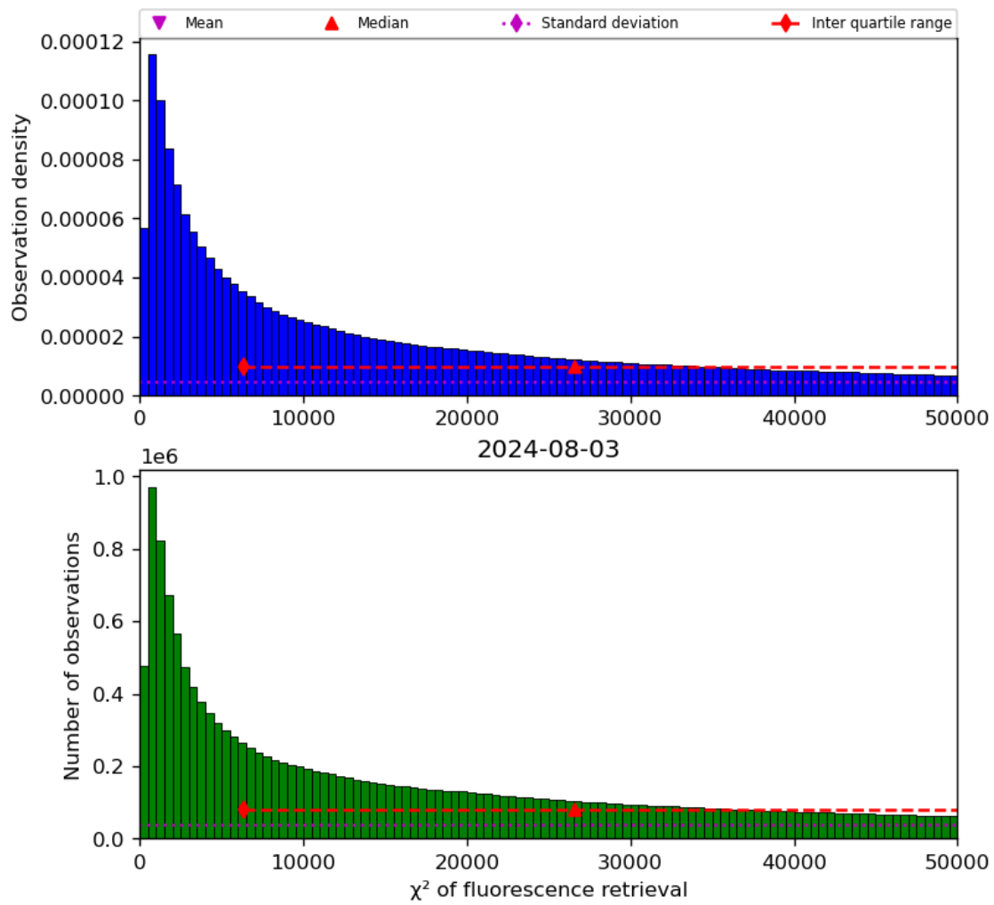
Figure 42: Histogram of “ \chi^2 of fluorescence retrieval” for 2024-08-02 to 2024-08-04
