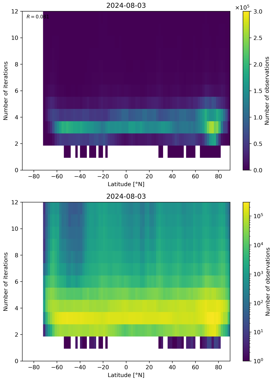
Figure 93: Scatter density plot of “Latitude” against “Number of iterations” for 2024-08-02 to 2024-08-04.
