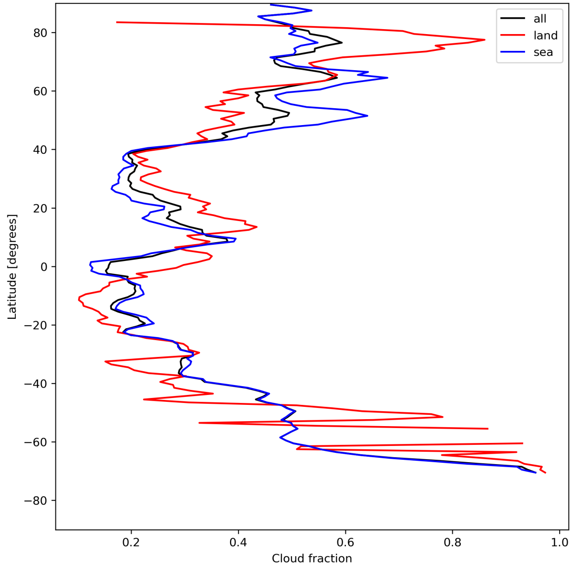
Figure 15: Zonal average of “Cloud fraction” for 2024-08-02 to 2024-08-04.
