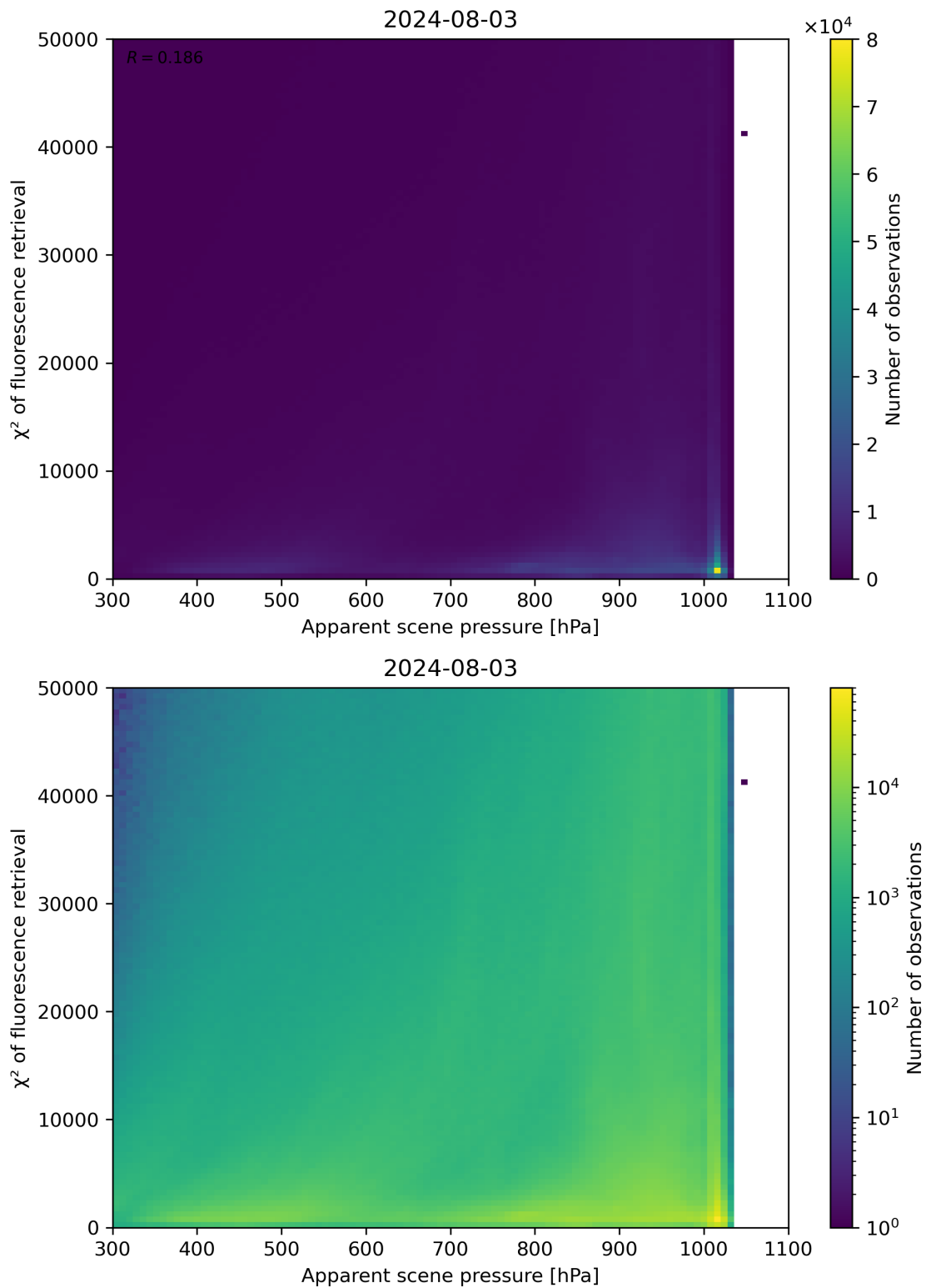
Figure 63: Scatter density plot of “Apparent scene pressure” against “ \chi^2 of fluorescence retrieval” for 2024-08-02 to 2024-08-04.
