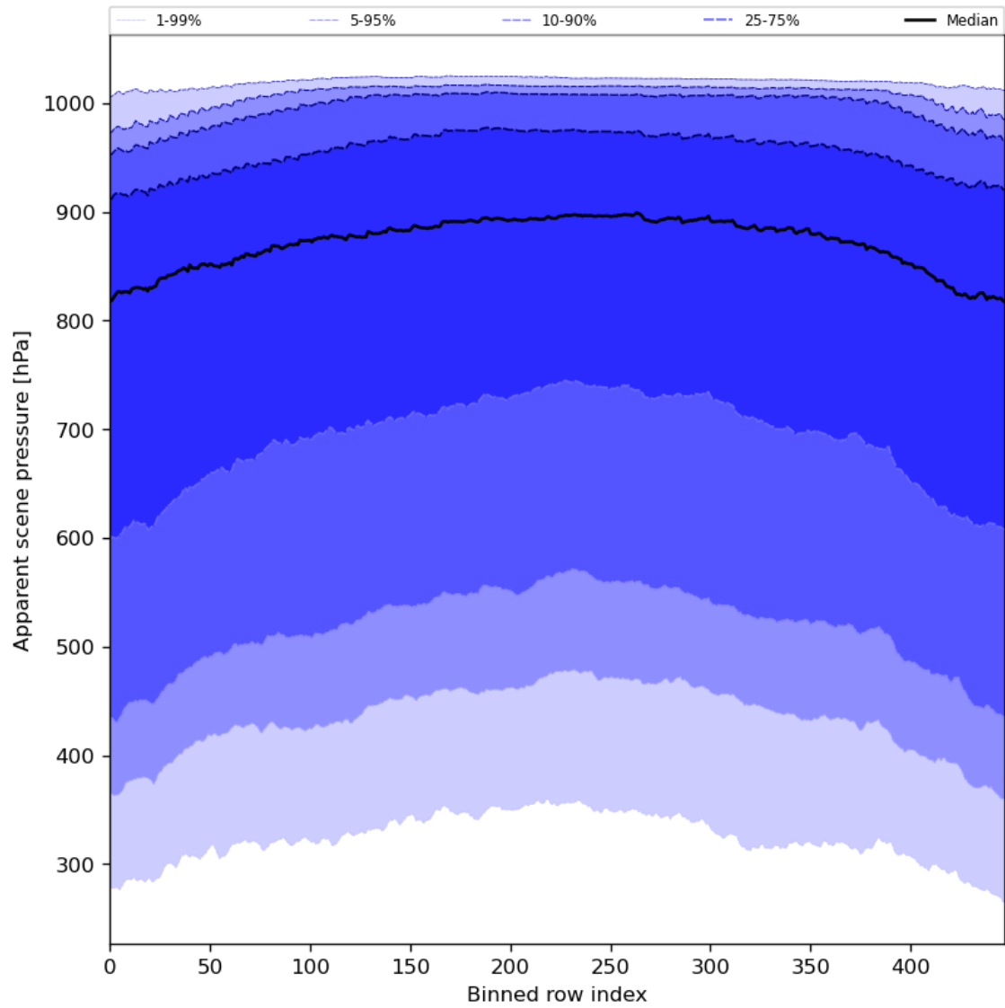
Figure 53: Along track statistics of “Apparent scene pressure” for 2024-08-02 to 2024-08-04
