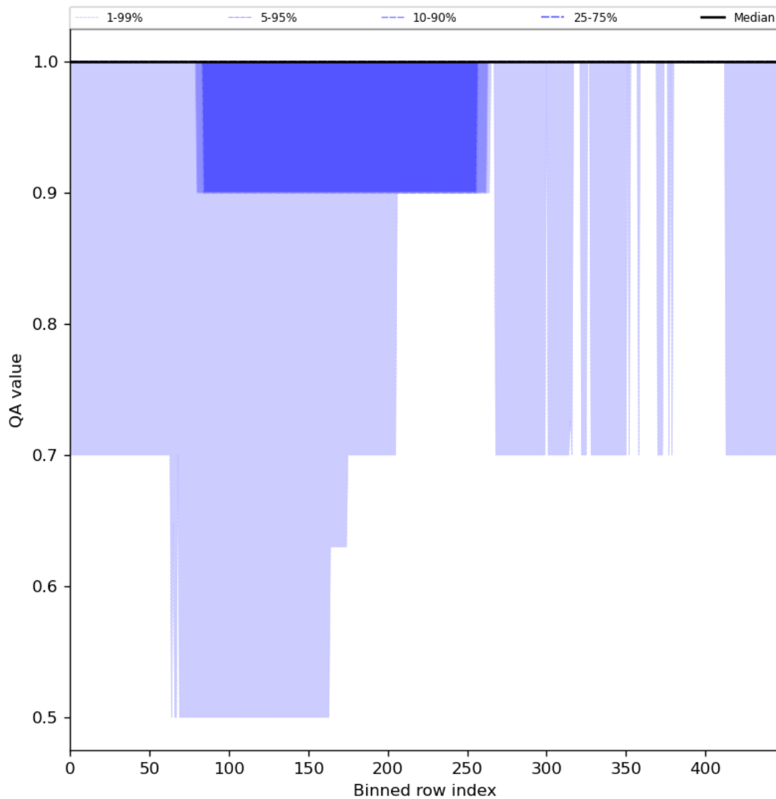
Figure 46: Along track statistics of “QA value” for 2024-08-02 to 2024-08-04
