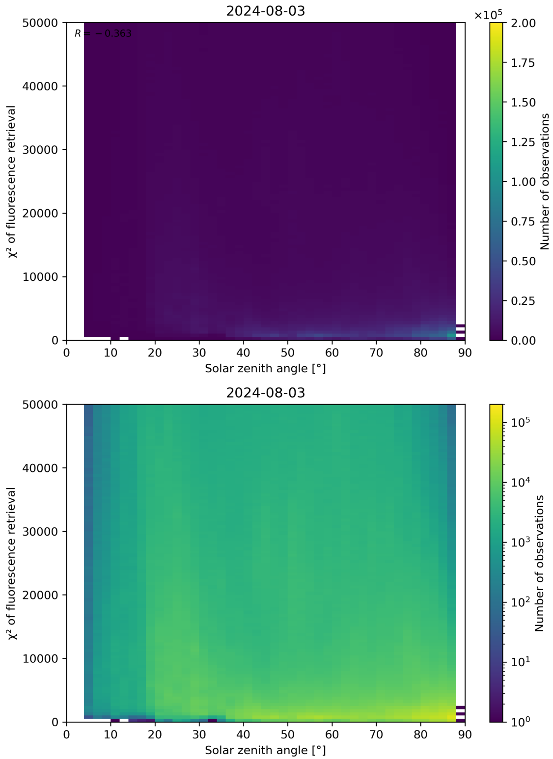
Figure 109: Scatter density plot of “Solar zenith angle” against “ \chi^2 of fluorescence retrieval” for 2024-08-02 to 2024-08-04.
