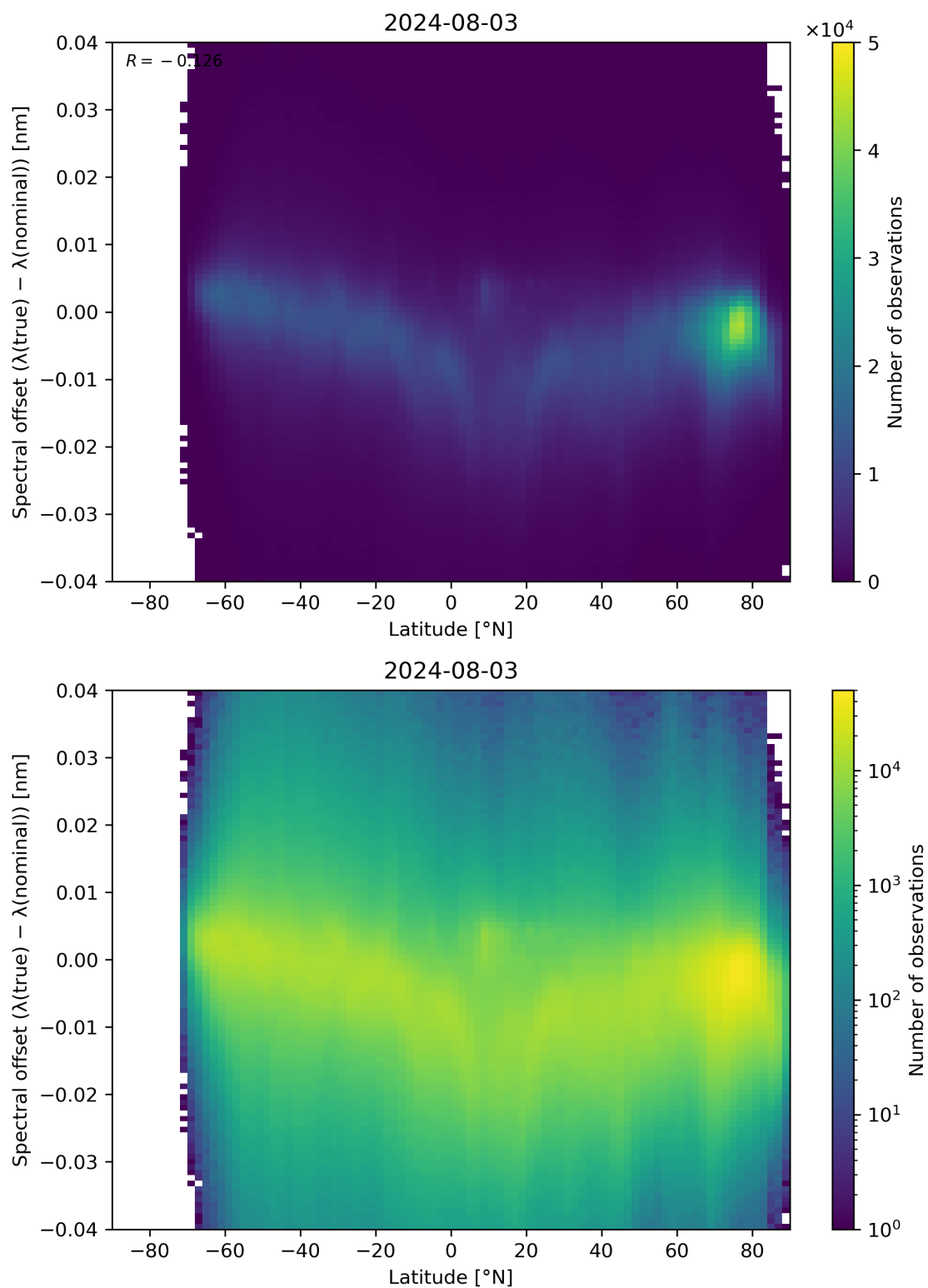
Figure 96: Scatter density plot of “Latitude” against “Spectral offset ( \lambda(\text{true}) - \lambda(\text{nominal}) )” for 2024-08-02 to 2024-08-04.
