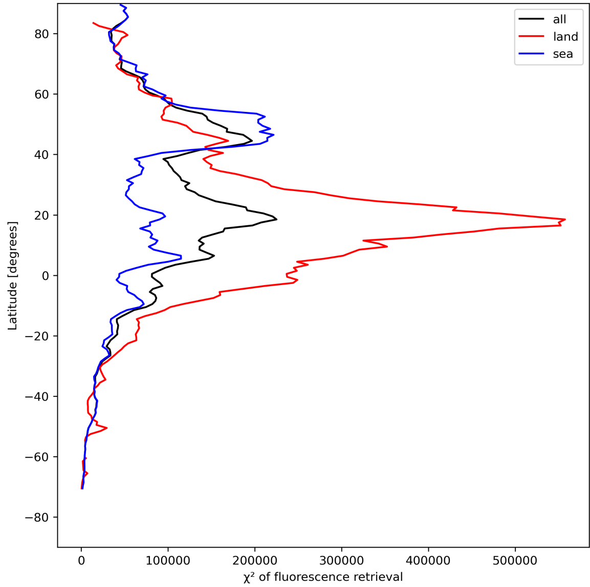
Figure 25: Zonal average of “ \chi^2 of fluorescence retrieval” for 2024-08-02 to 2024-08-04.
