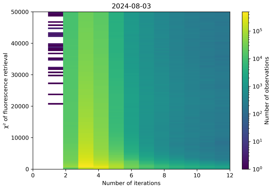
Figure 97: Scatter density plot of “Number of iterations” against “ \chi^2 of fluorescence retrieval” for 2024-08-02 to 2024-08-04.
