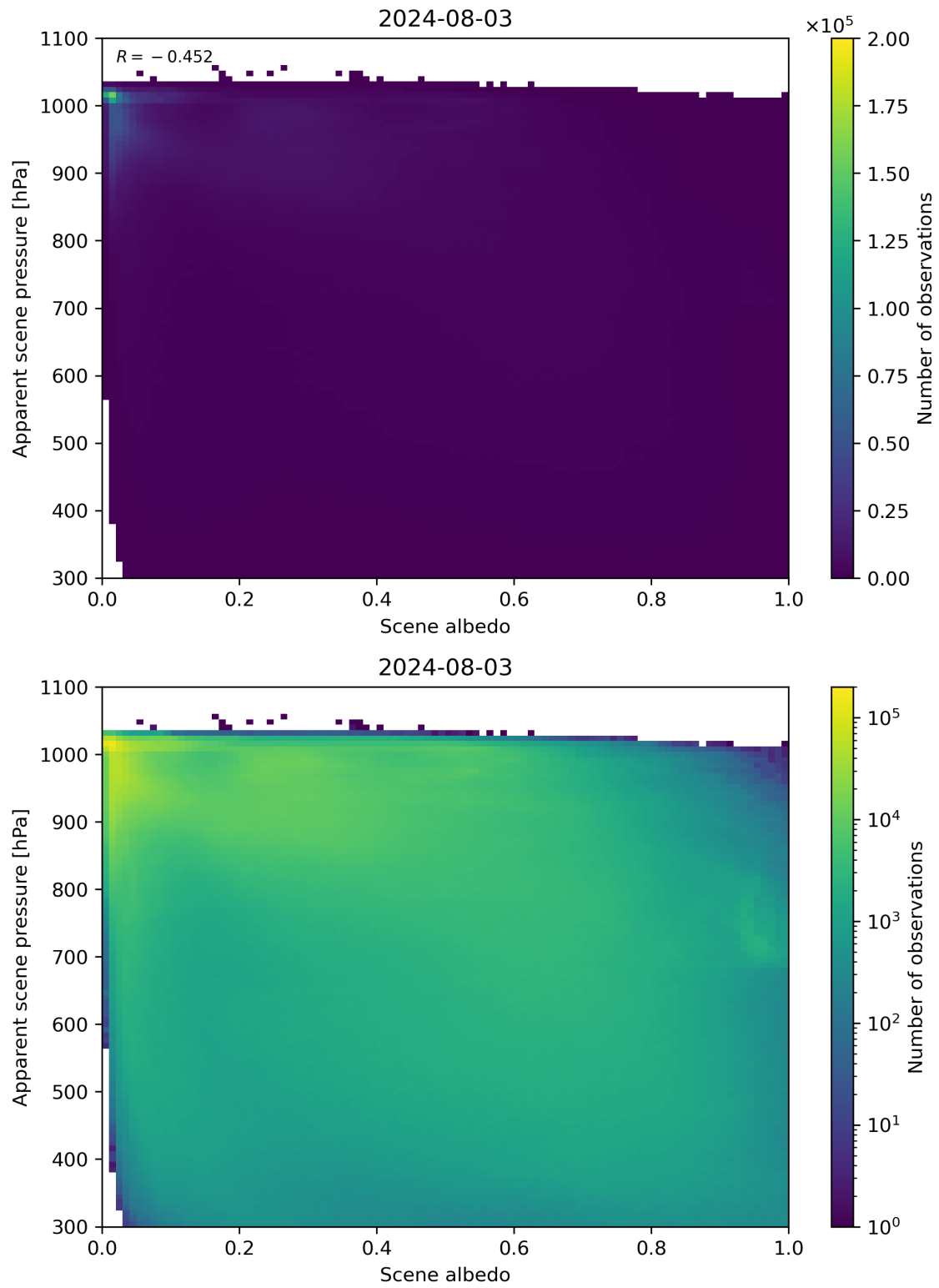
Figure 102: Scatter density plot of “Scene albedo” against “Apparent scene pressure” for 2024-08-02 to 2024-08-04.
