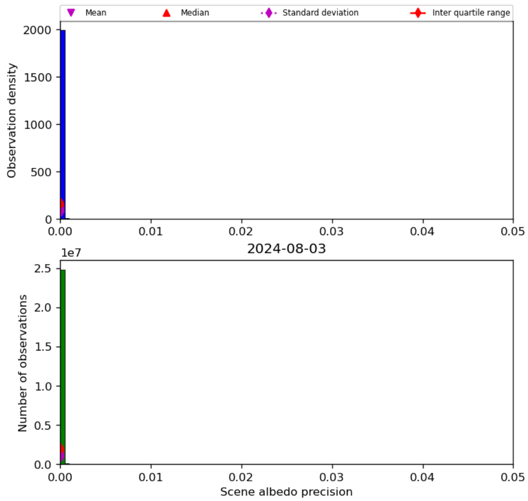
Figure 35: Histogram of “Scene albedo precision” for 2024-08-02 to 2024-08-04
