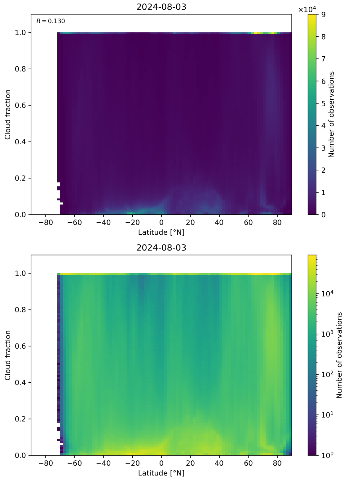
Figure 90: Scatter density plot of “Latitude” against “Cloud fraction” for 2024-08-02 to 2024-08-04.
