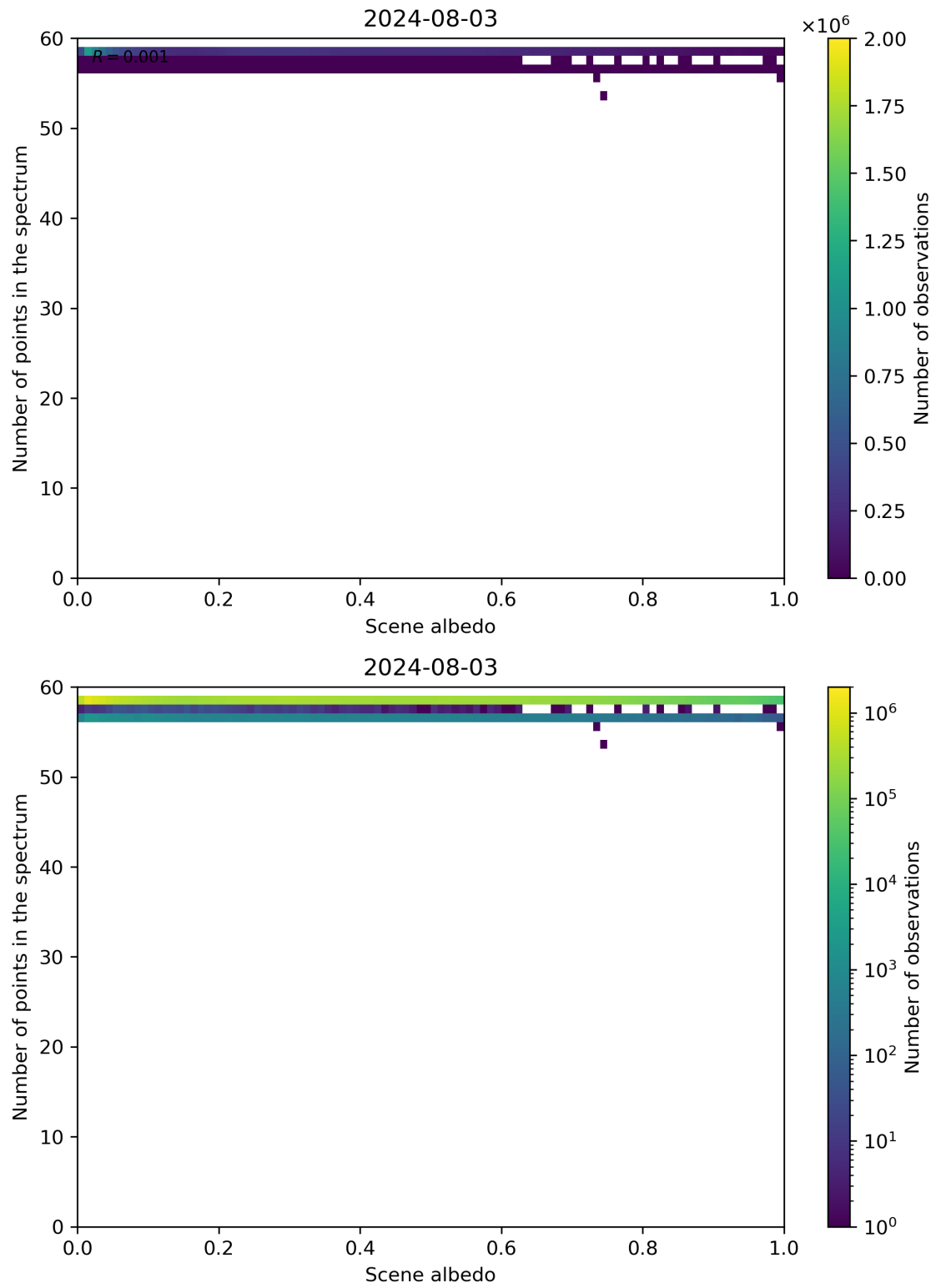
Figure 106: Scatter density plot of “Scene albedo” against “Number of points in the spectrum” for 2024-08-02 to 2024-08-04.
