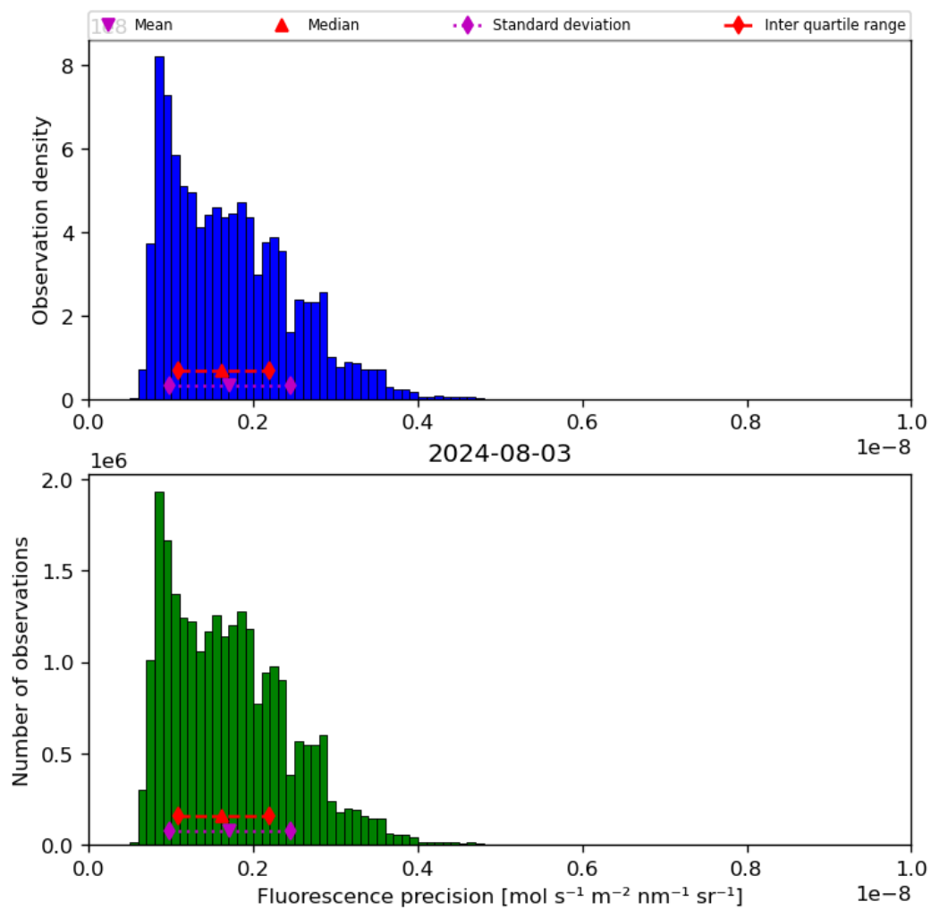
Figure 41: Histogram of “Fluorescence precision” for 2024-08-02 to 2024-08-04
