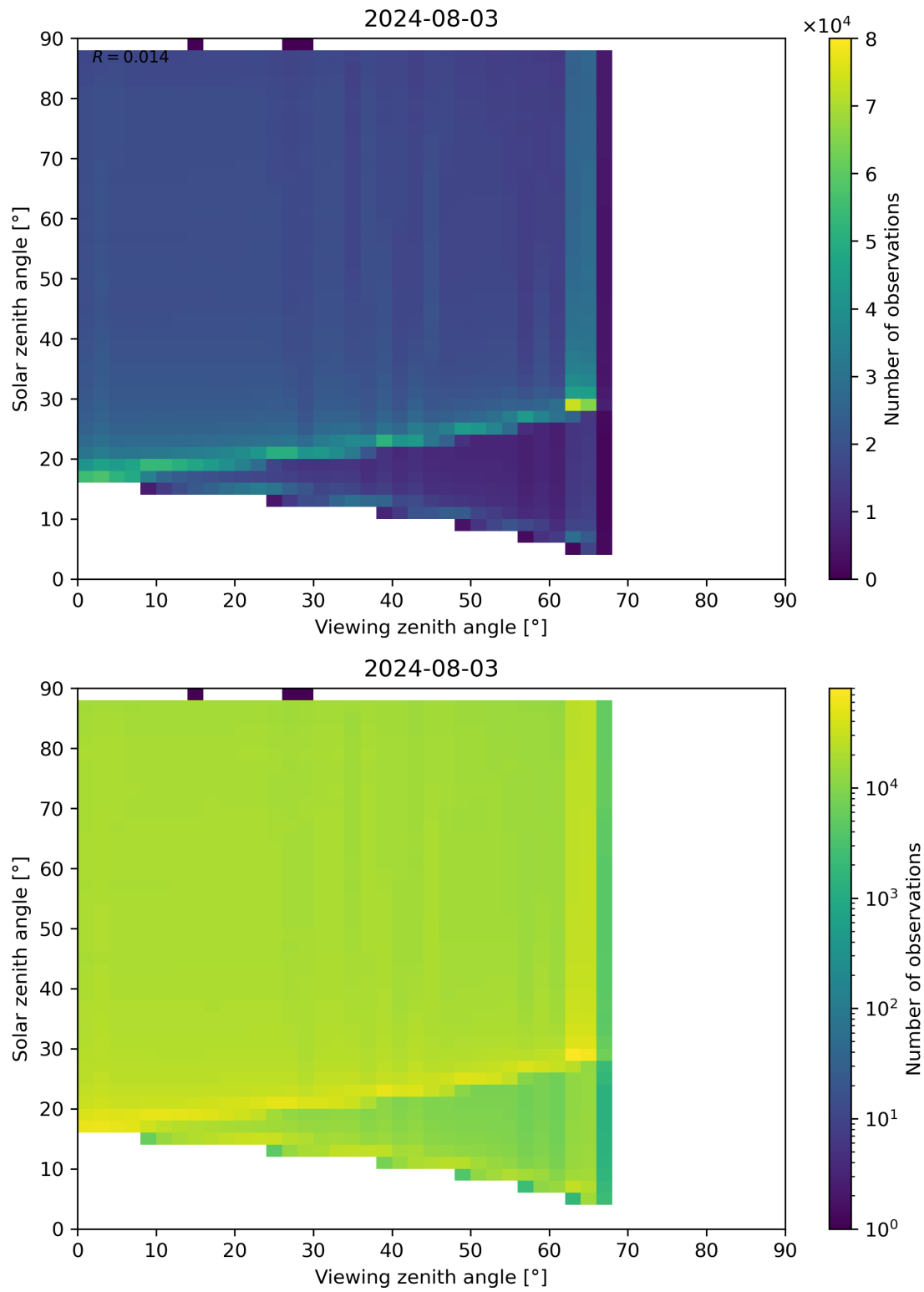
Figure 127: Scatter density plot of “Viewing zenith angle” against “Solar zenith angle” for 2024-08-02 to 2024-08-04.
