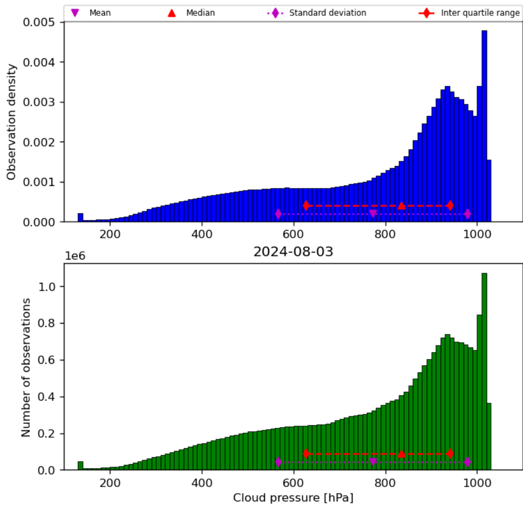
Figure 30: Histogram of “Cloud pressure” for 2024-08-02 to 2024-08-04
