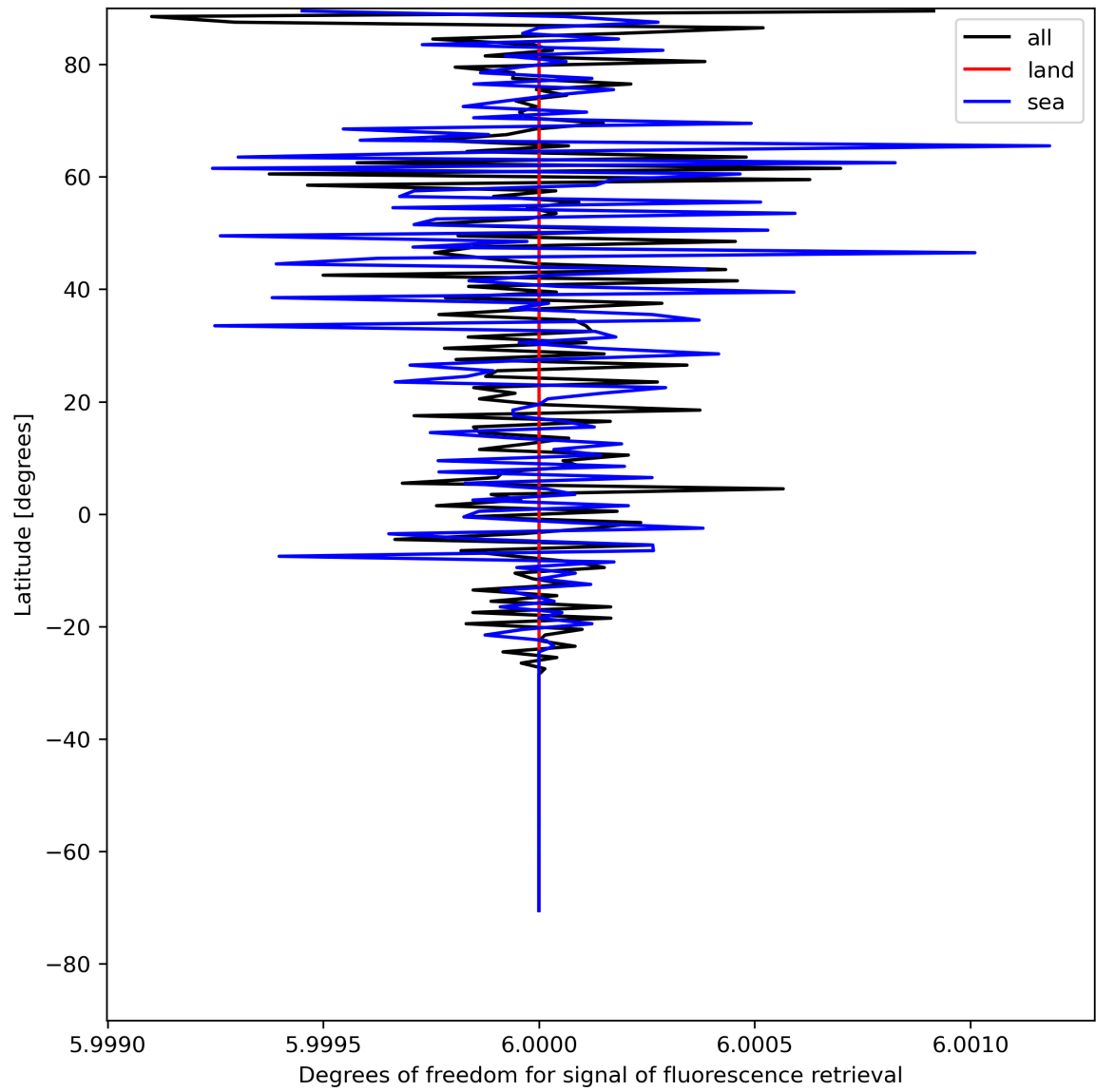
Figure 26: Zonal average of “Degrees of freedom for signal of fluorescence retrieval” for 2024-08-02 to 2024-08-04.
