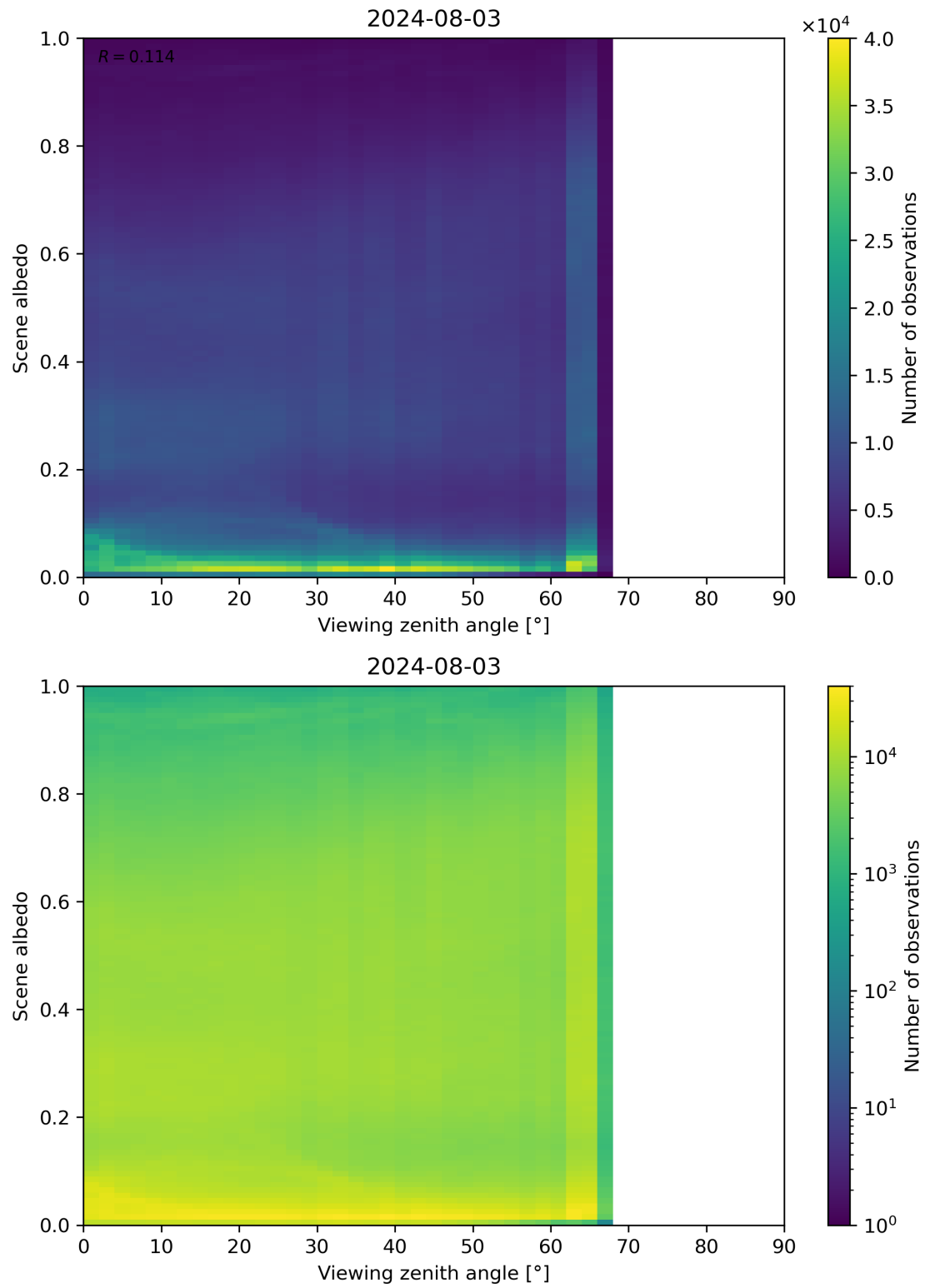
Figure 126: Scatter density plot of “Viewing zenith angle” against “Scene albedo” for 2024-08-02 to 2024-08-04.
