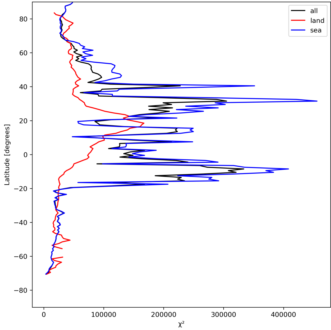
Figure 21: Zonal average of “ \chi^2 ” for 2024-08-02 to 2024-08-04.
