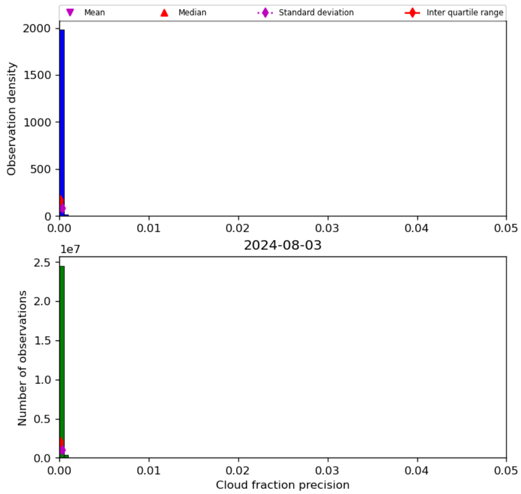
Figure 33: Histogram of “Cloud fraction precision” for 2024-08-02 to 2024-08-04
