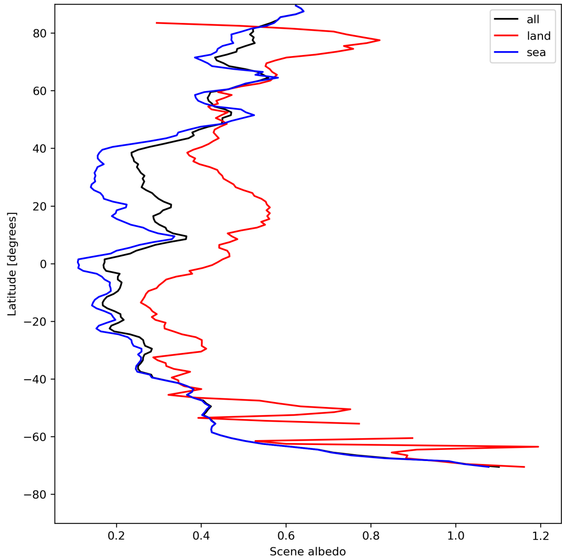
Figure 17: Zonal average of “Scene albedo” for 2024-08-02 to 2024-08-04.
