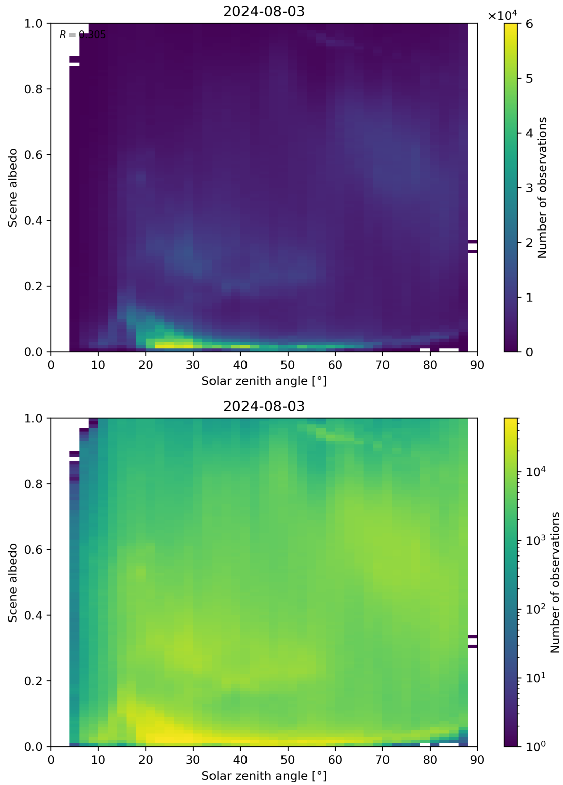
Figure 116: Scatter density plot of “Solar zenith angle” against “Scene albedo” for 2024-08-02 to 2024-08-04.
