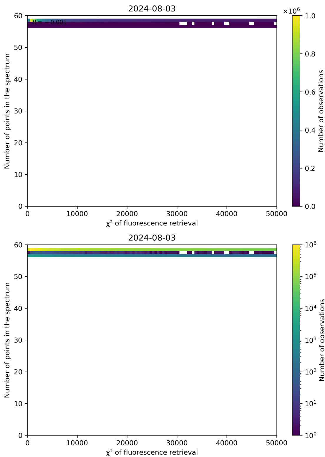
Figure 68: Scatter density plot of " \chi^2 of fluorescence retrieval" against "Number of points in the spectrum" for 2024-08-02 to 2024-08-04.
