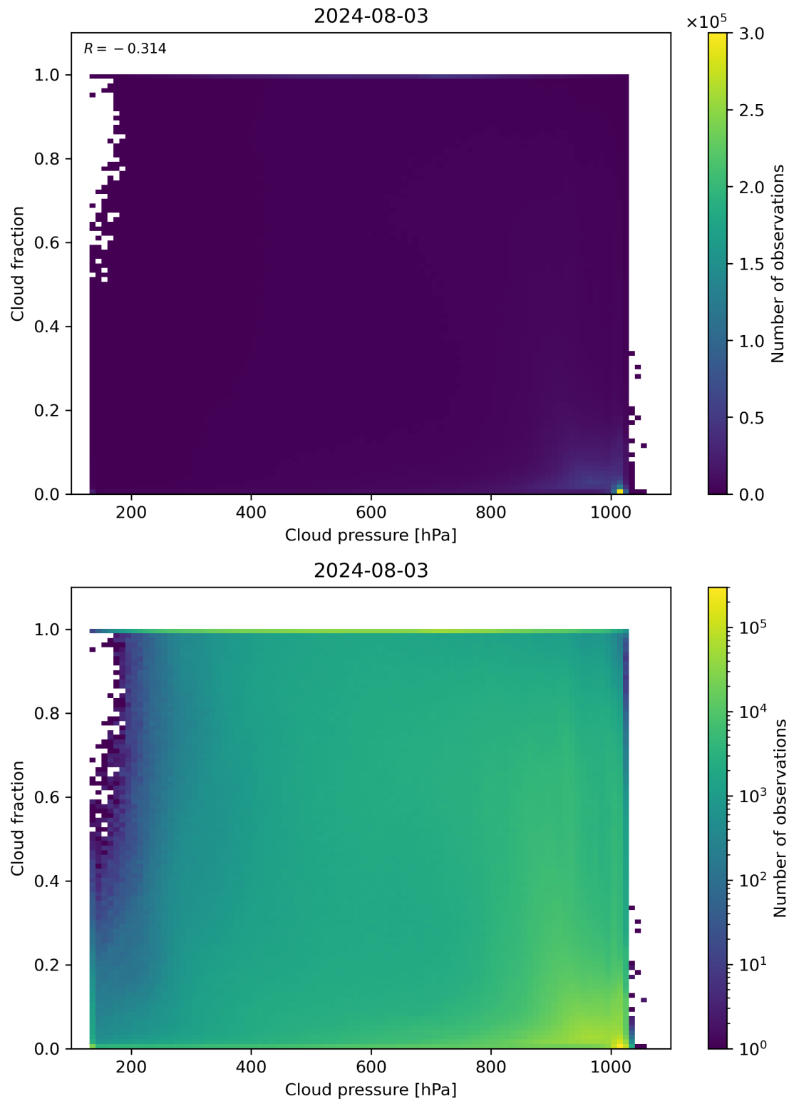
Figure 79: Scatter density plot of “Cloud pressure” against “Cloud fraction” for 2024-08-02 to 2024-08-04.
