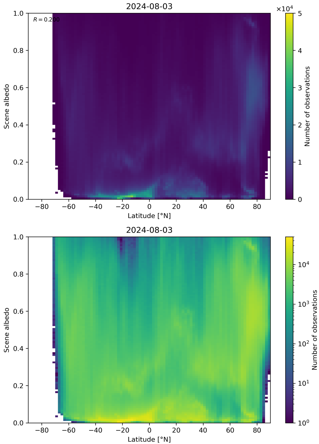
Figure 95: Scatter density plot of “Latitude” against “Scene albedo” for 2024-08-02 to 2024-08-04.
