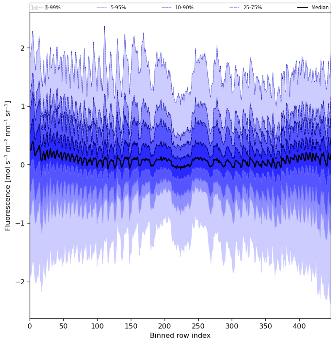
Figure 57: Along track statistics of “Fluorescence” for 2024-08-02 to 2024-08-04
