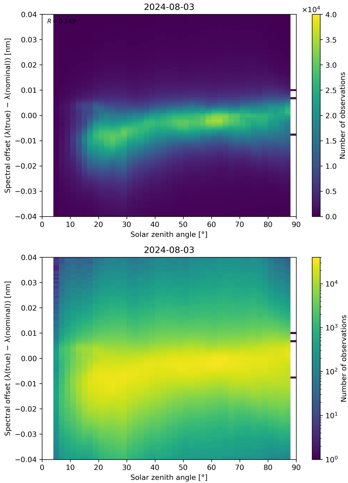
Figure 117: Scatter density plot of “Solar zenith angle” against “Spectral offset ( \lambda(\text{true}) - \lambda(\text{nominal}) )” for 2024-08-02 to 2024-08-04.
