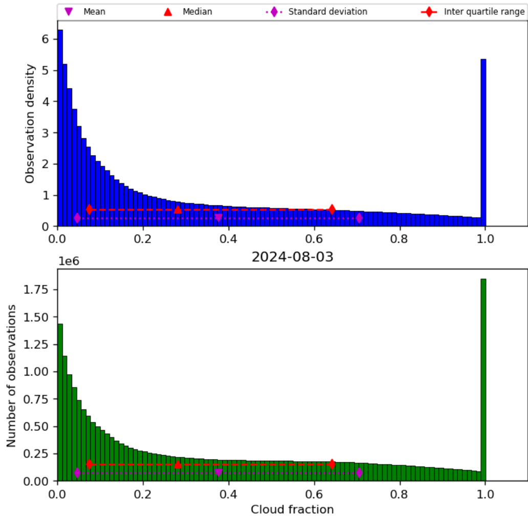
Figure 32: Histogram of “Cloud fraction” for 2024-08-02 to 2024-08-04
