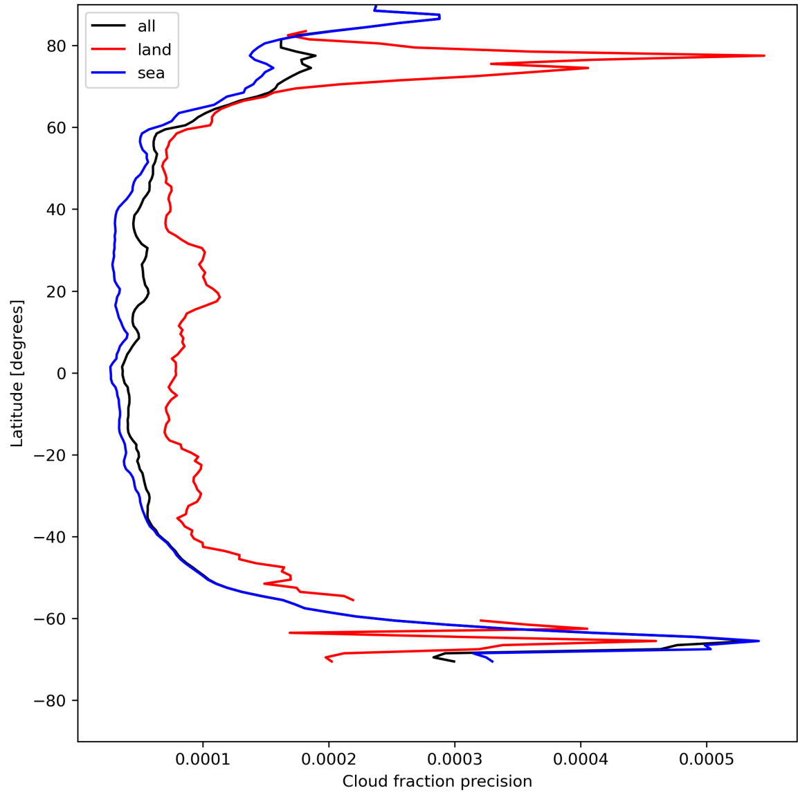
Figure 16: Zonal average of “Cloud fraction precision” for 2024-08-02 to 2024-08-04.
