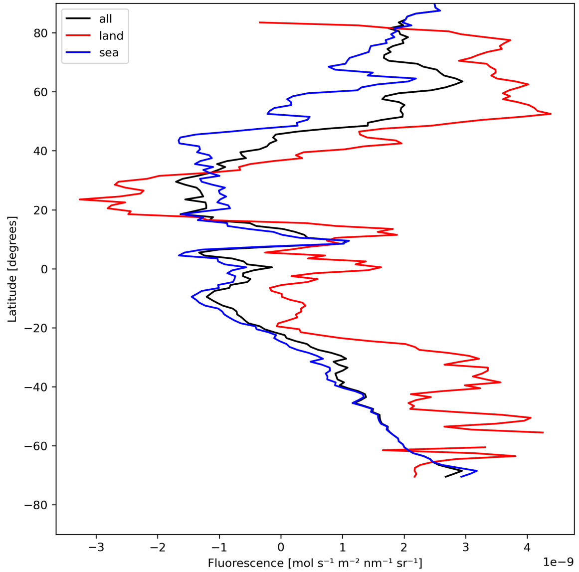
Figure 23: Zonal average of “Fluorescence” for 2024-08-02 to 2024-08-04.
