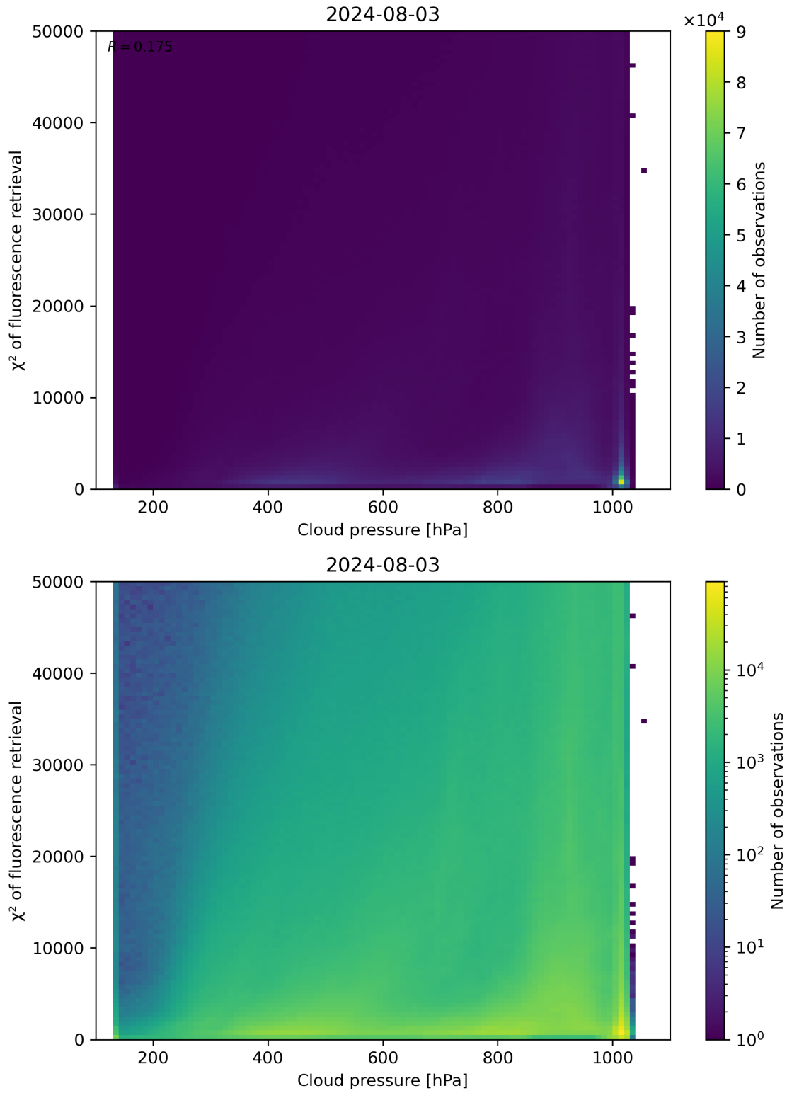
Figure 78: Scatter density plot of “Cloud pressure” against “ \chi^2 of fluorescence retrieval” for 2024-08-02 to 2024-08-04.
