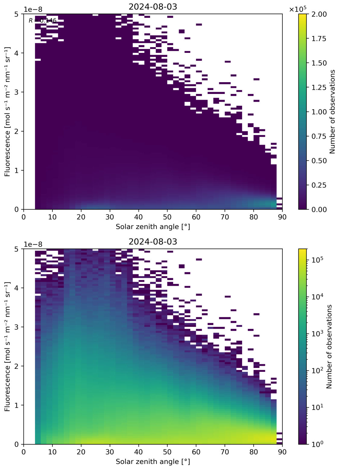
Figure 112: Scatter density plot of “Solar zenith angle” against “Fluorescence” for 2024-08-02 to 2024-08-04.
