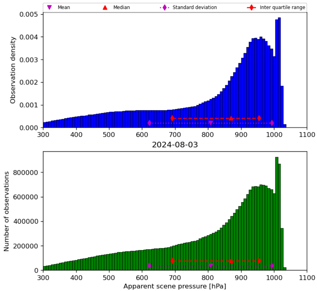
Figure 36: Histogram of “Apparent scene pressure” for 2024-08-02 to 2024-08-04
