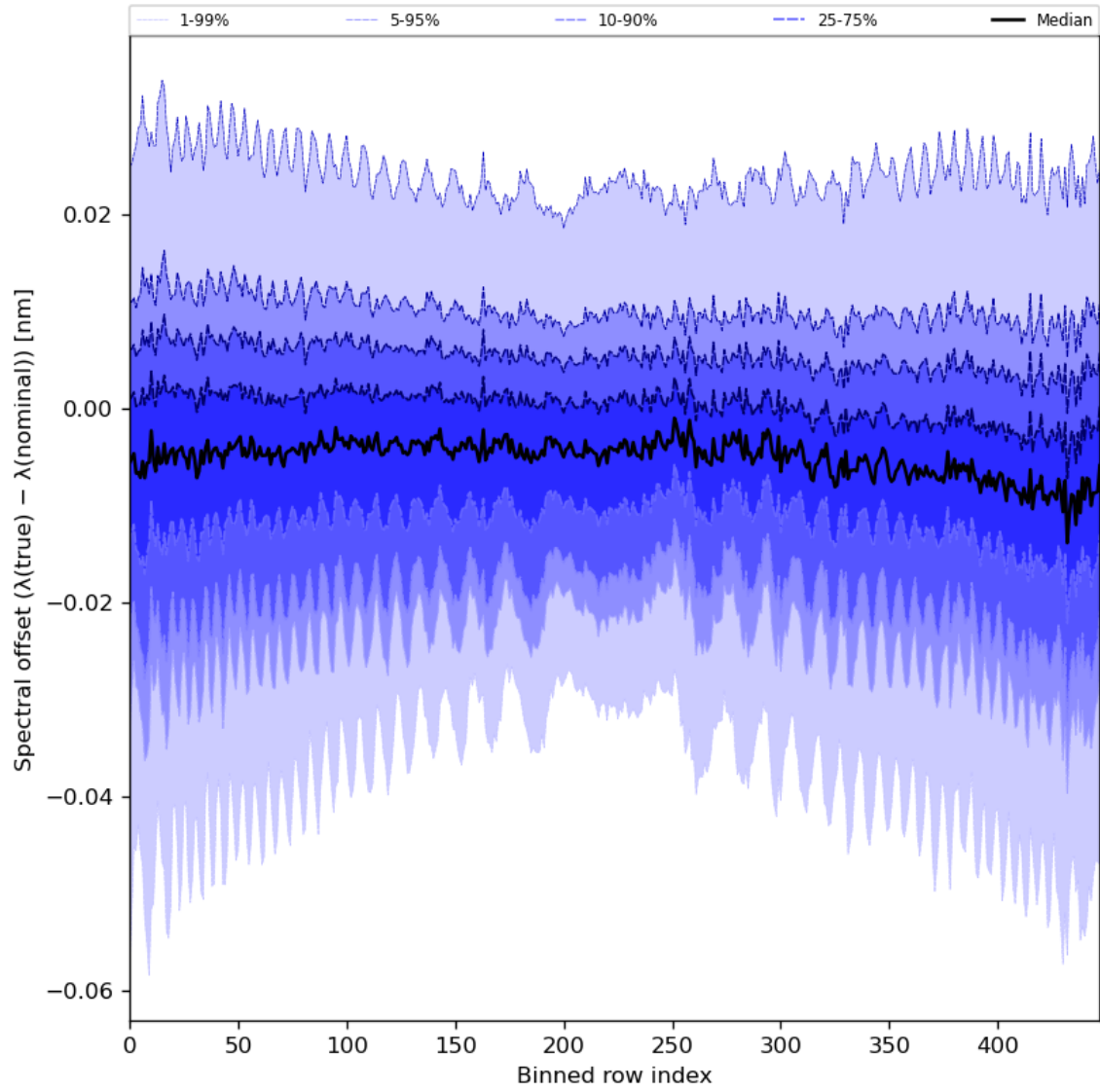
Figure 62: Along track statistics of “Spectral offset ( \lambda(\text{true}) - \lambda(\text{nominal}) )” for 2024-08-02 to 2024-08-04
