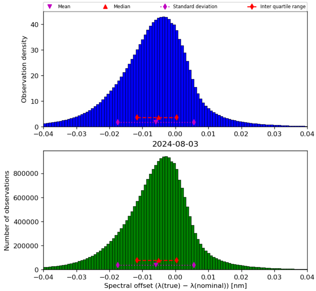
Figure 45: Histogram of “Spectral offset ( \lambda(\text{true}) - \lambda(\text{nominal}) )” for 2024-08-02 to 2024-08-04
