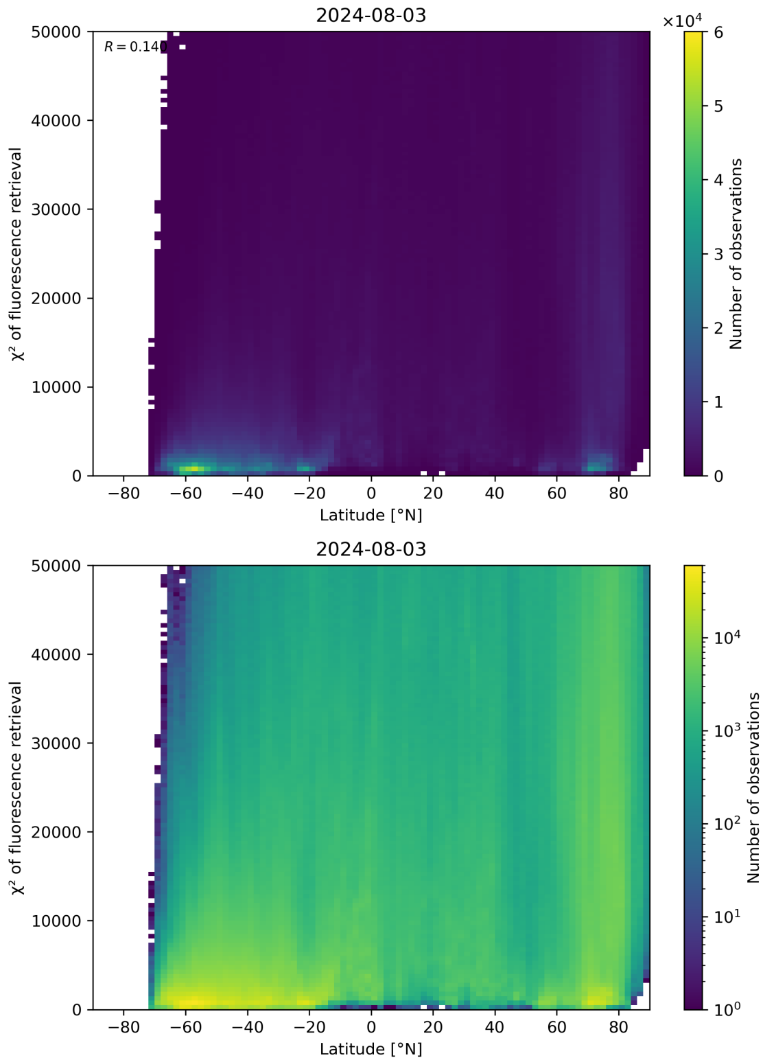
Figure 89: Scatter density plot of “Latitude” against “ \chi^2 of fluorescence retrieval” for 2024-08-02 to 2024-08-04.
