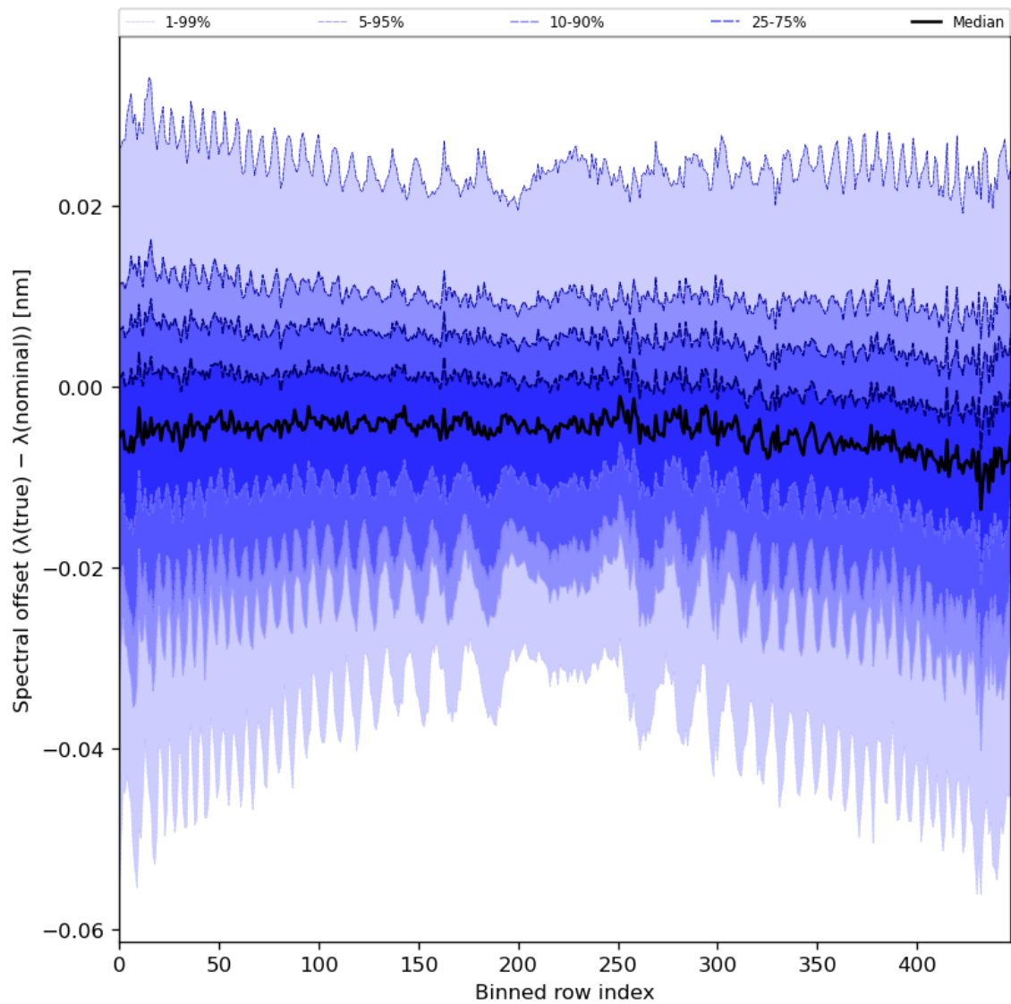
Figure 62: Along track statistics of “Spectral offset ( \lambda(\text{true}) - \lambda(\text{nominal}) )” for 2024-08-03 to 2024-08-05
