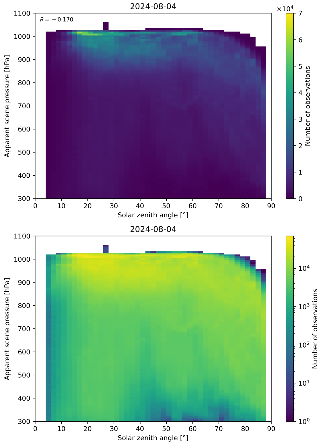
Figure 108: Scatter density plot of “Solar zenith angle” against “Apparent scene pressure” for 2024-08-03 to 2024-08-05.
