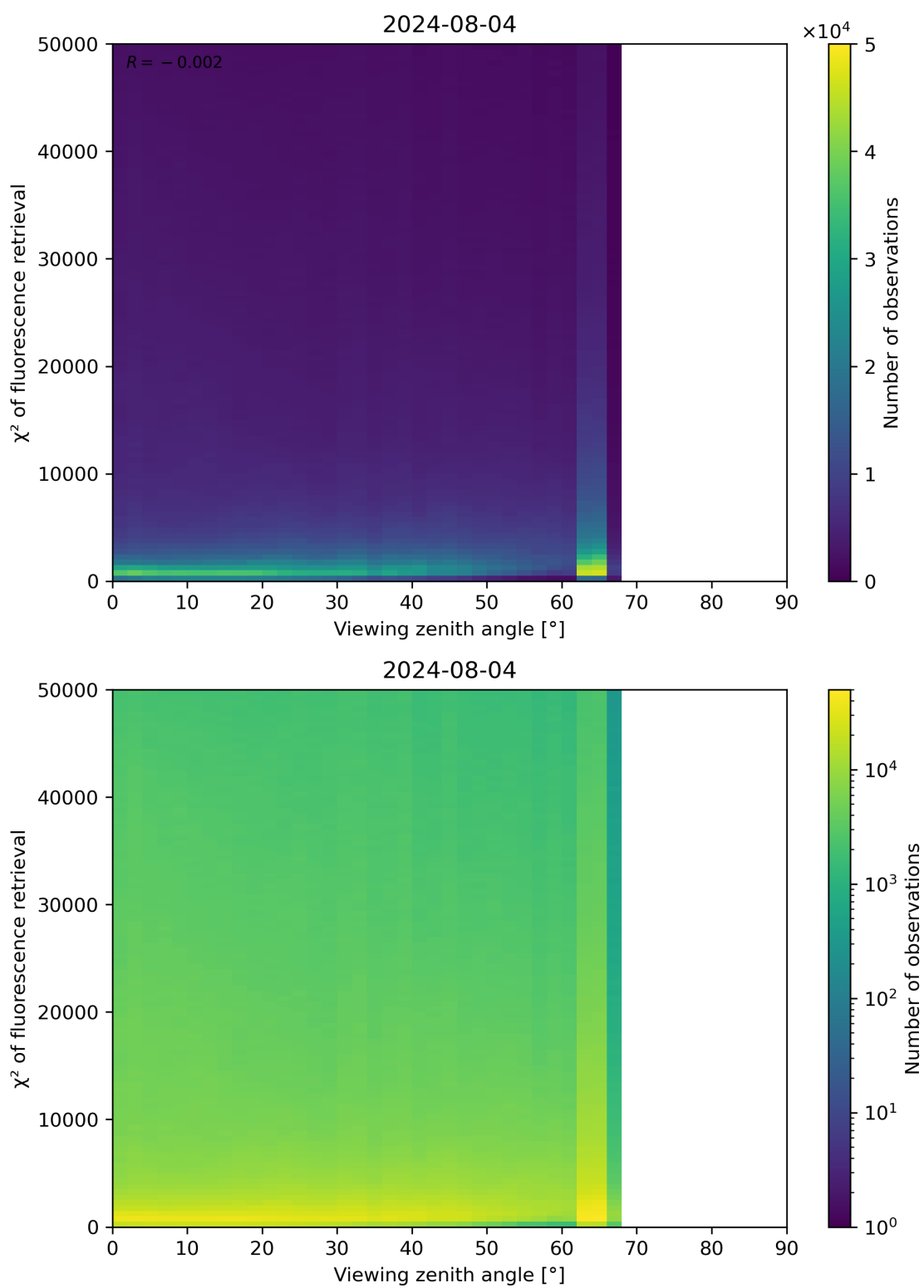
Figure 119: Scatter density plot of “Viewing zenith angle” against “ \chi^2 of fluorescence retrieval” for 2024-08-03 to 2024-08-05.
