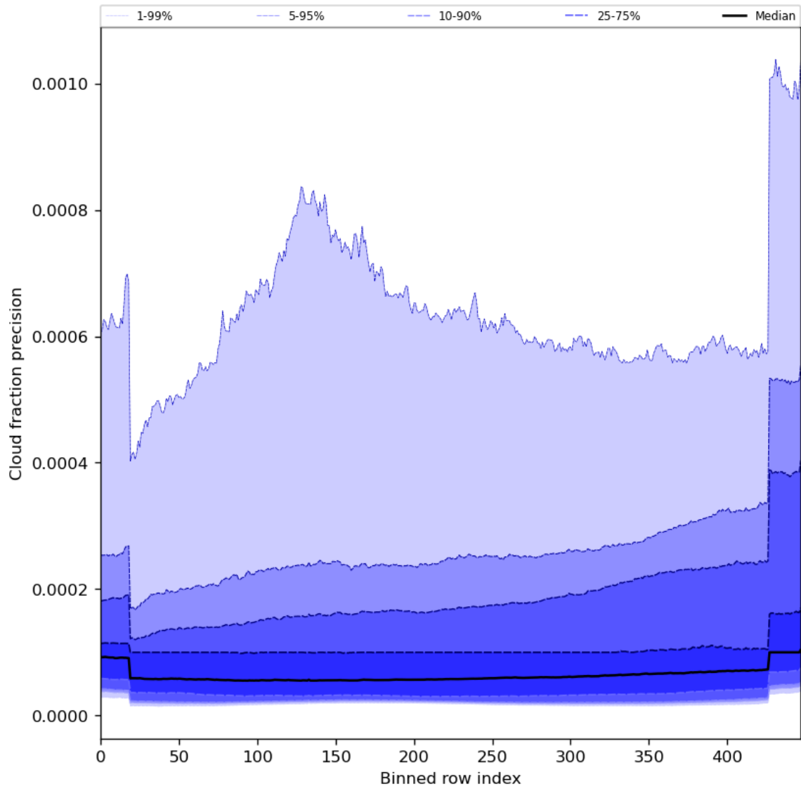
Figure 50: Along track statistics of “Cloud fraction precision” for 2024-08-03 to 2024-08-05
