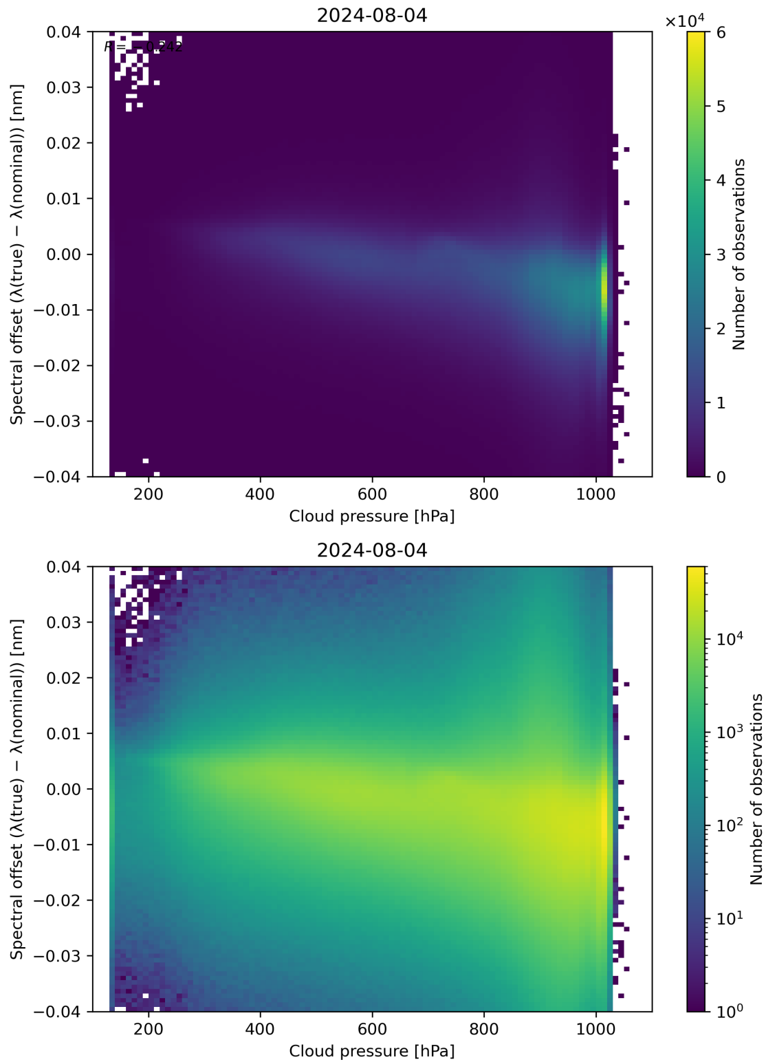
Figure 84: Scatter density plot of “Cloud pressure” against “Spectral offset ( \lambda(\text{true}) - \lambda(\text{nominal}) )” for 2024-08-03 to 2024-08-05.
