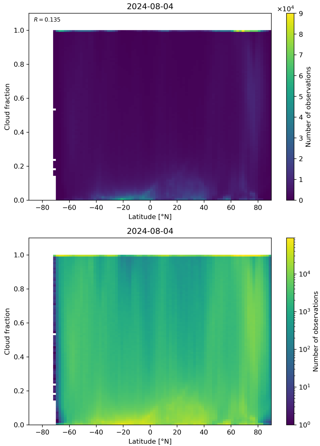
Figure 90: Scatter density plot of “Latitude” against “Cloud fraction” for 2024-08-03 to 2024-08-05.
