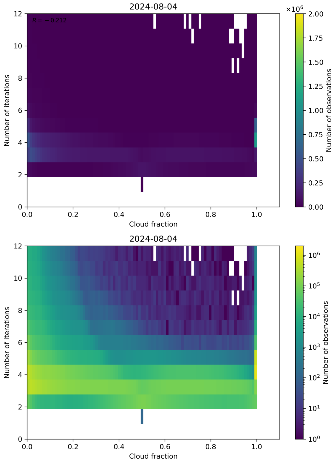
Figure 73: Scatter density plot of “Cloud fraction” against “Number of iterations” for 2024-08-03 to 2024-08-05.
