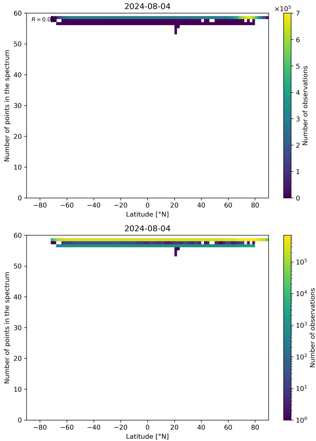
Figure 94: Scatter density plot of “Latitude” against “Number of points in the spectrum” for 2024-08-03 to 2024-08-05.
