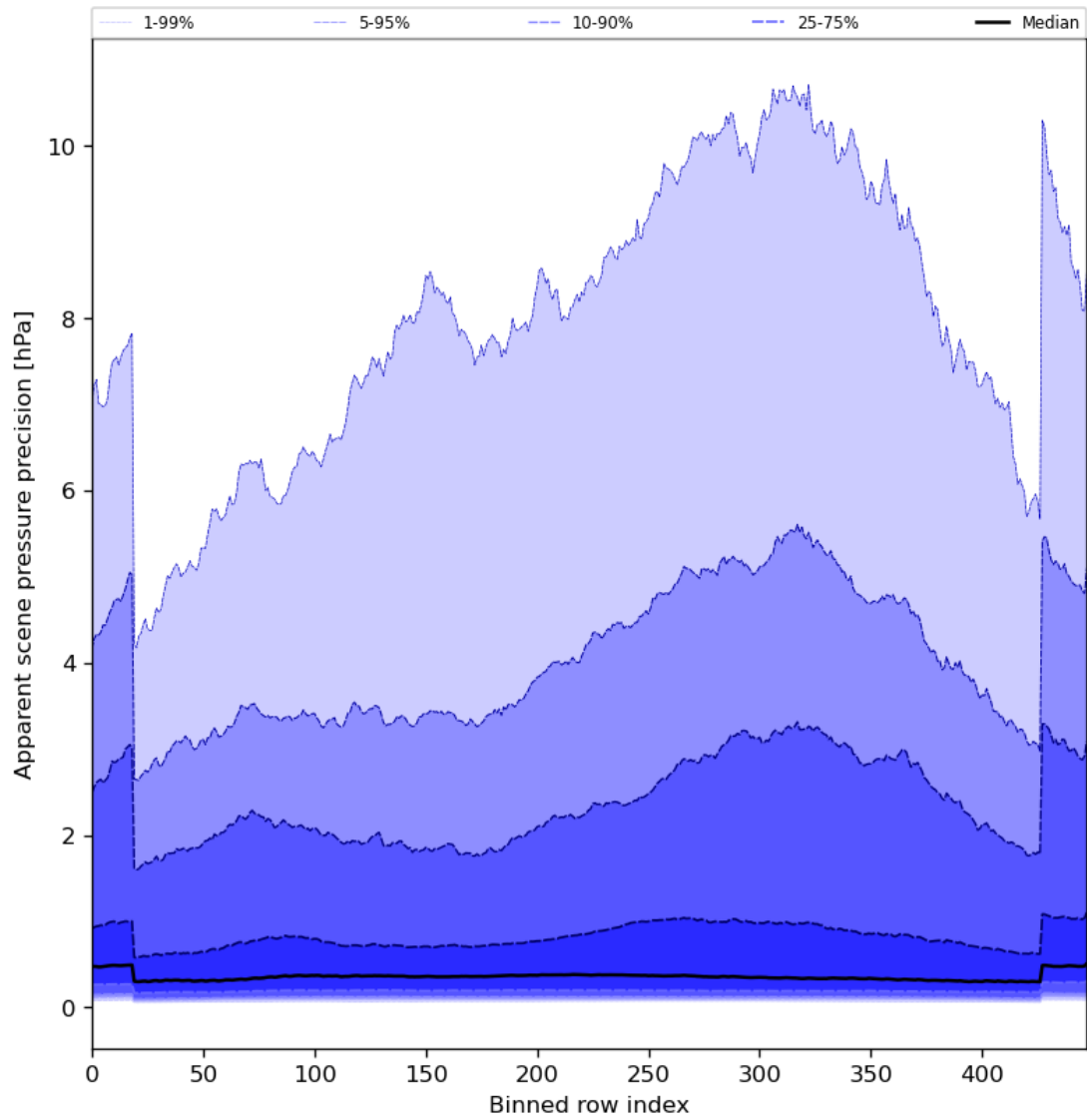
Figure 54: Along track statistics of “Apparent scene pressure precision” for 2024-08-03 to 2024-08-05
