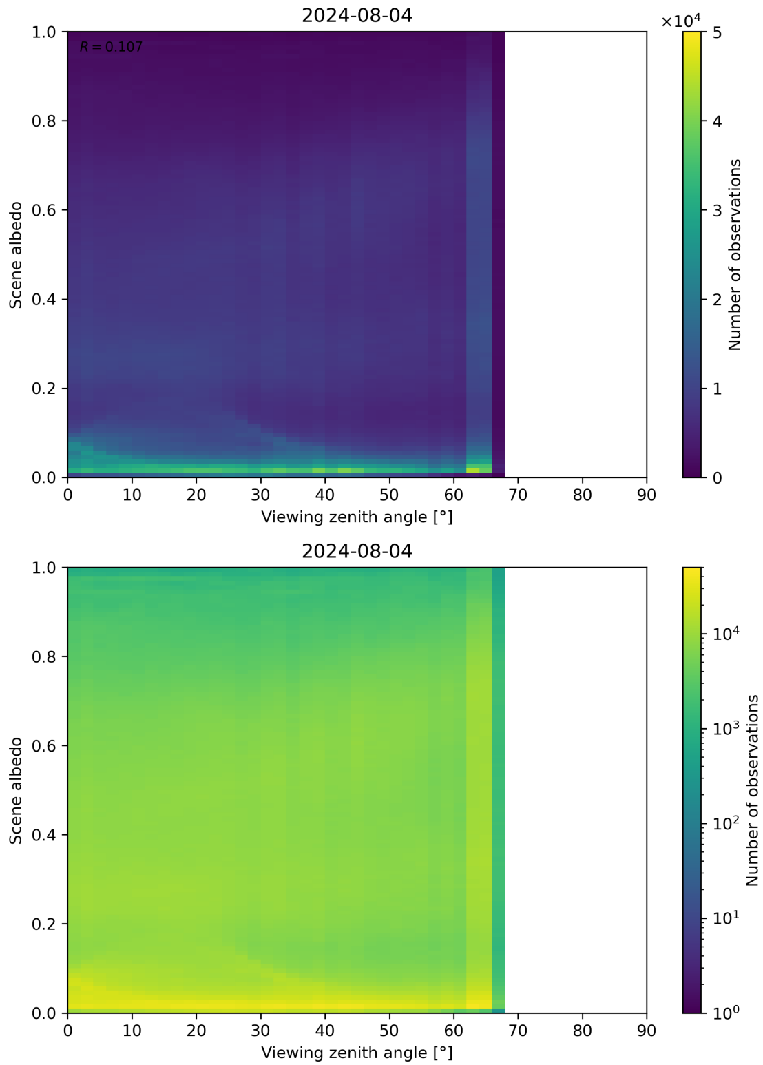
Figure 126: Scatter density plot of “Viewing zenith angle” against “Scene albedo” for 2024-08-03 to 2024-08-05.
