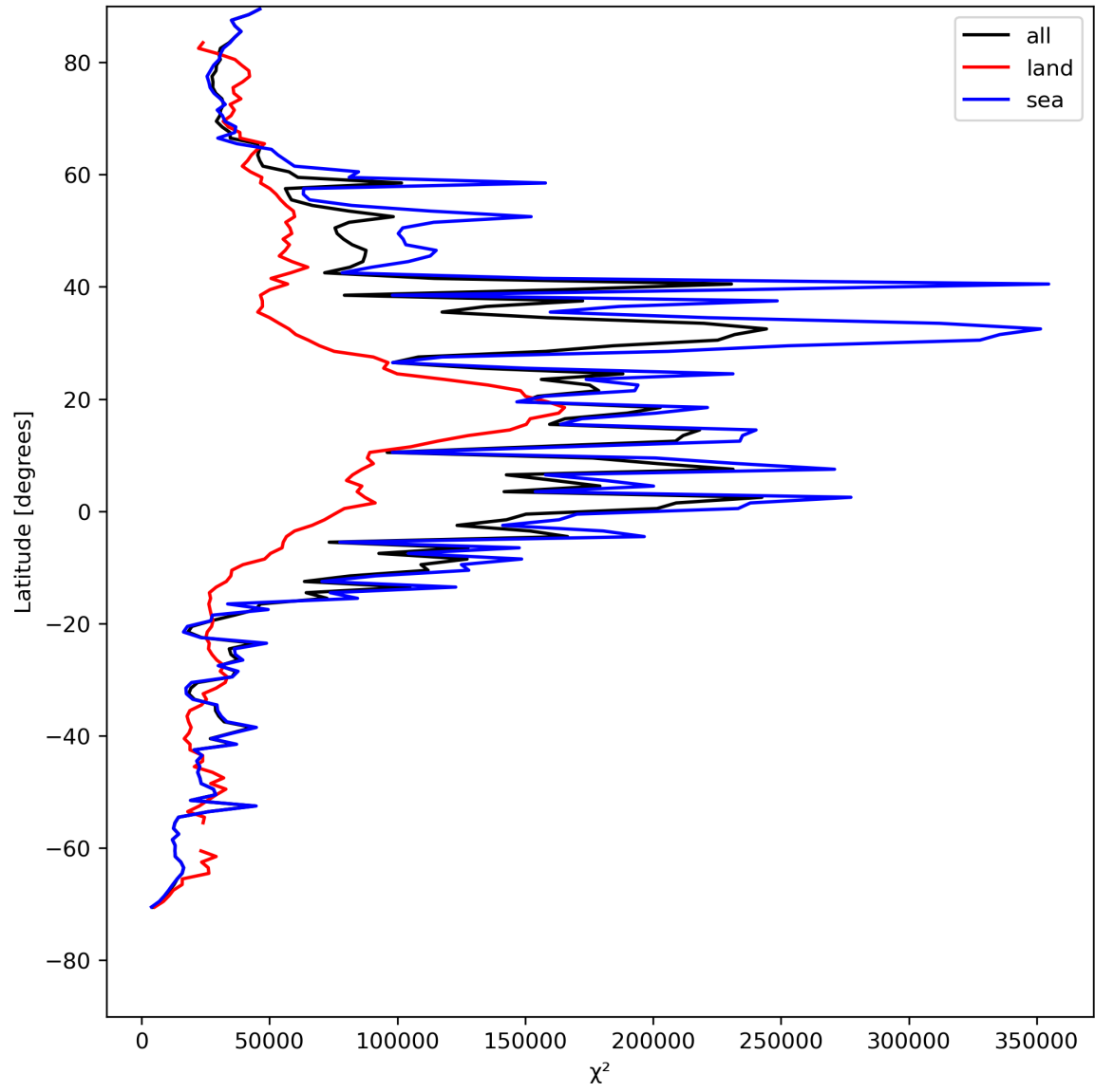
Figure 21: Zonal average of “ \chi^2 ” for 2024-08-03 to 2024-08-05.
