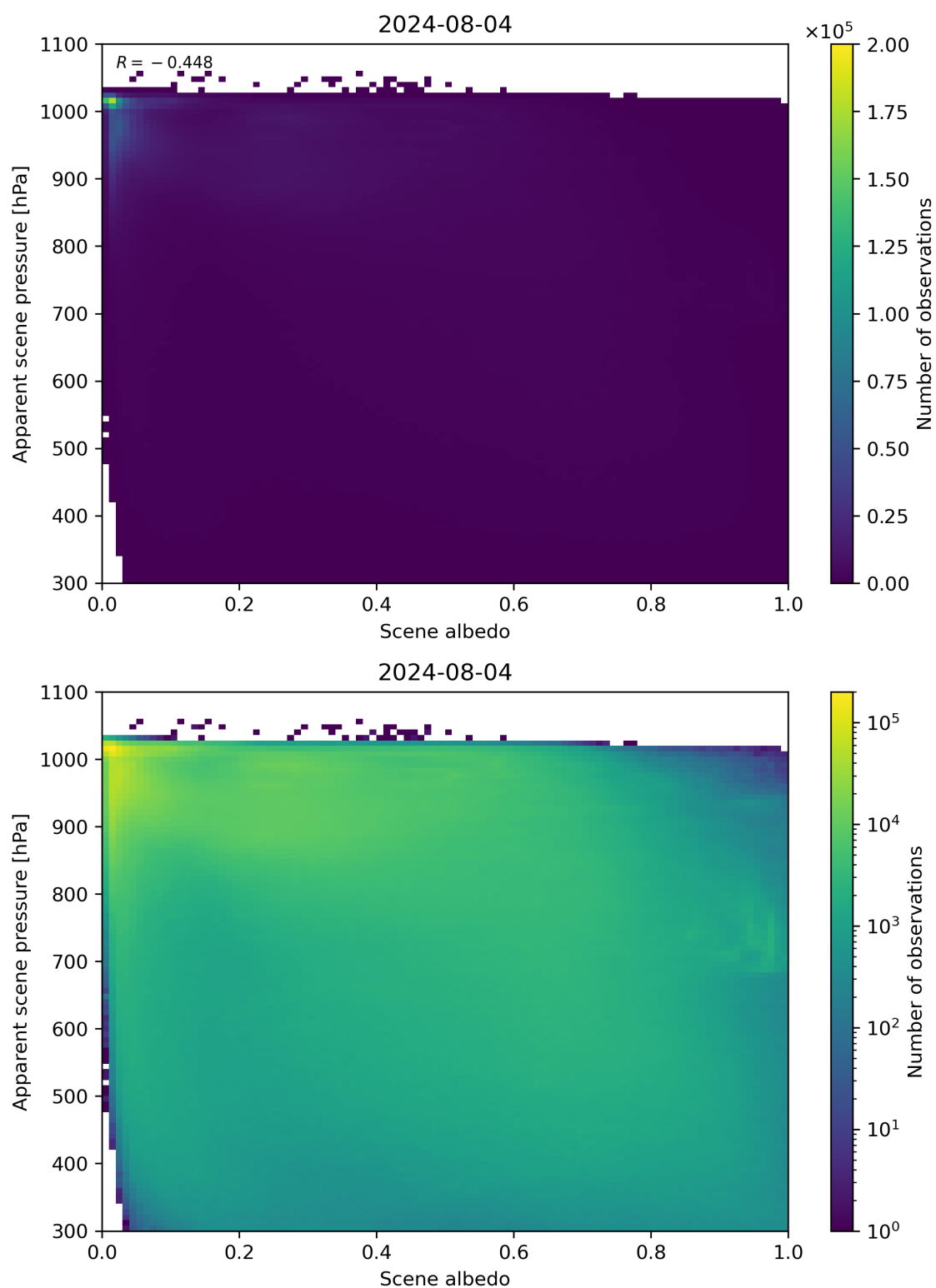
Figure 102: Scatter density plot of “Scene albedo” against “Apparent scene pressure” for 2024-08-03 to 2024-08-05.
