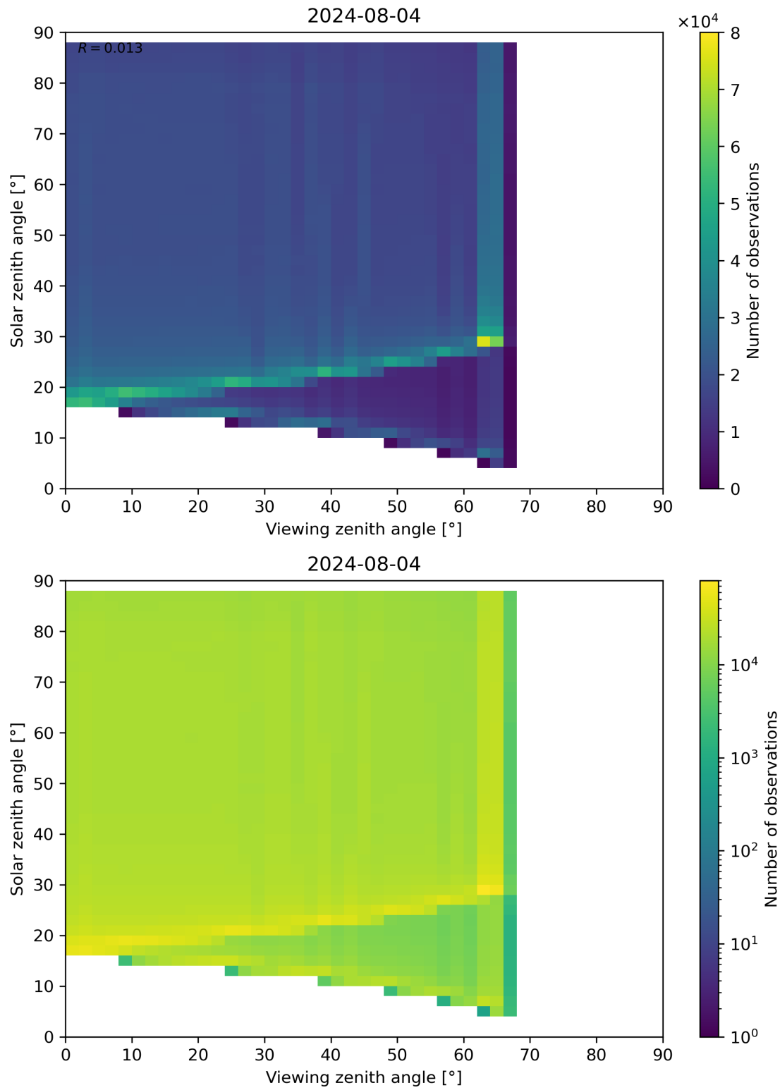
Figure 127: Scatter density plot of “Viewing zenith angle” against “Solar zenith angle” for 2024-08-03 to 2024-08-05.
