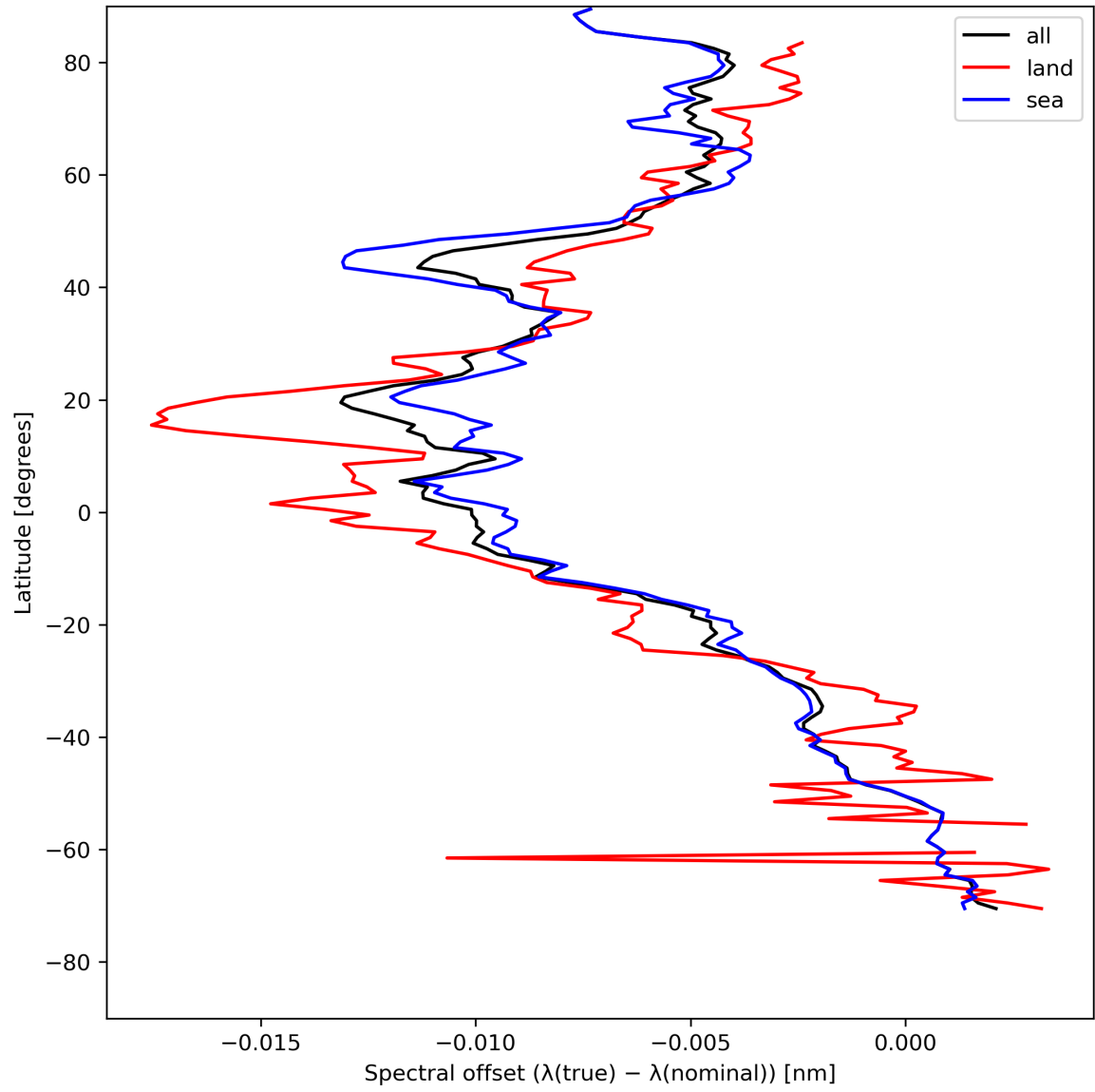
Figure 28: Zonal average of “Spectral offset ( \lambda(\text{true}) - \lambda(\text{nominal}) )” for 2024-08-03 to 2024-08-05.
