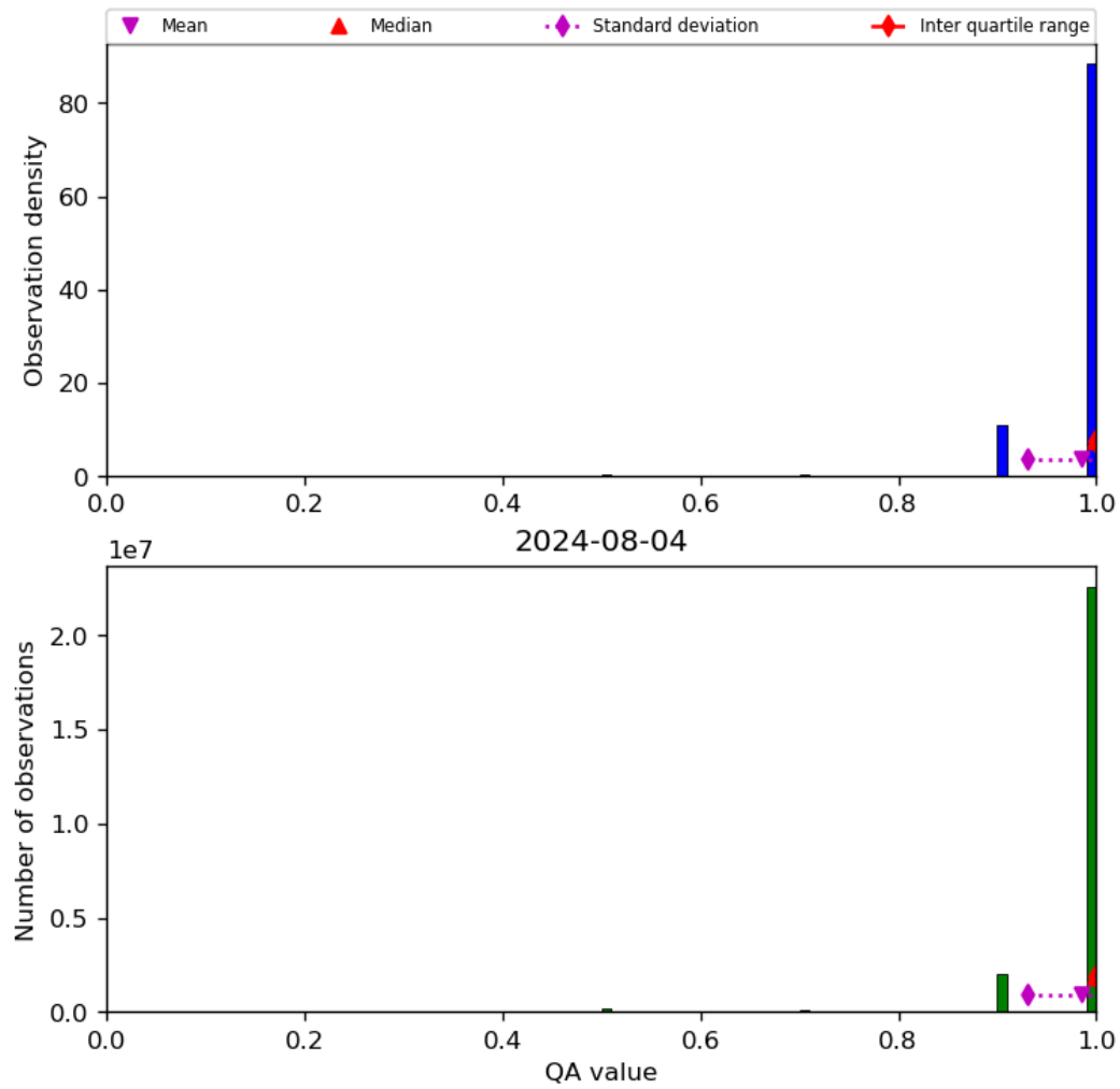
Figure 29: Histogram of “QA value” for 2024-08-03 to 2024-08-05
