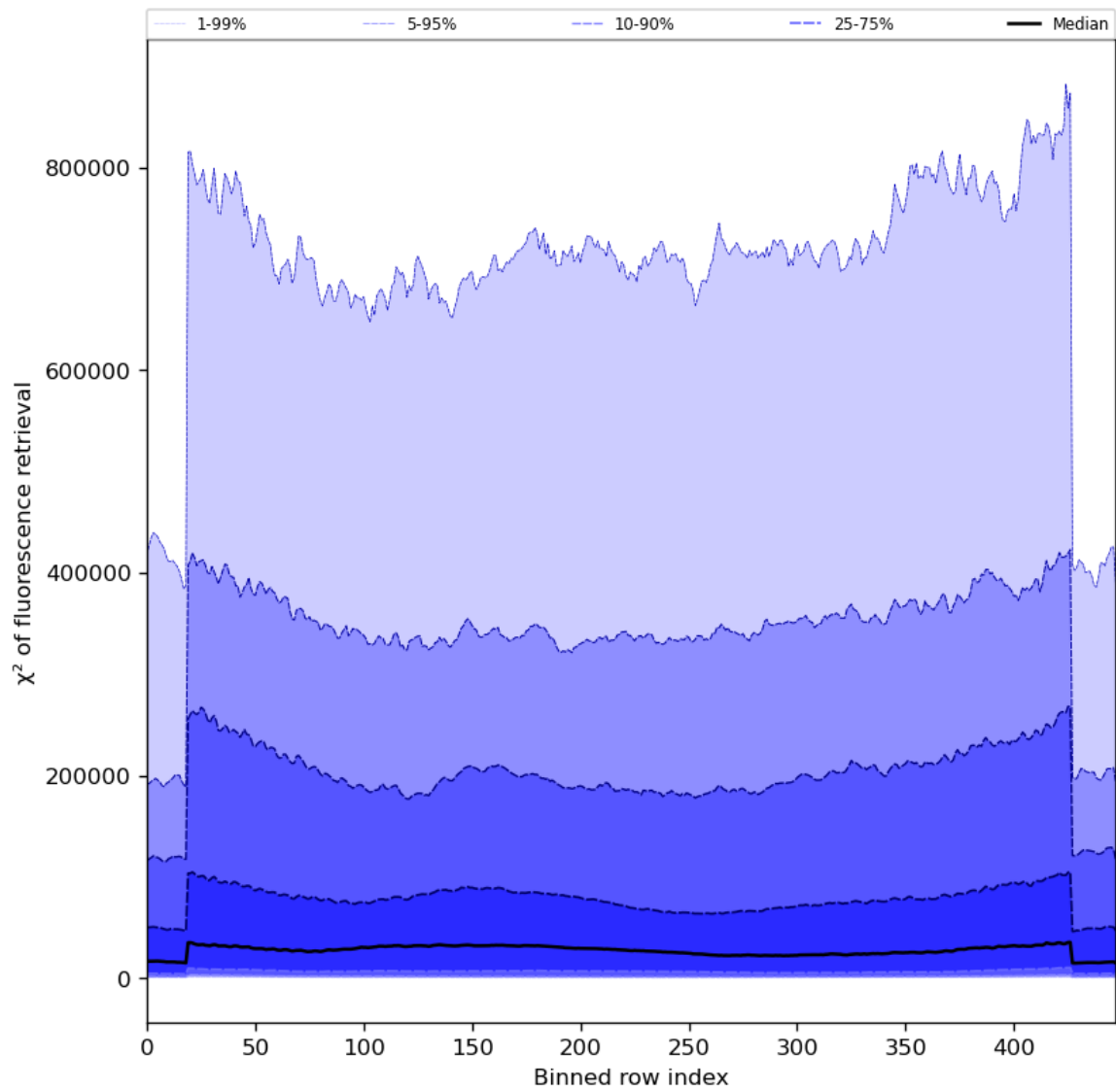
Figure 59: Along track statistics of “ \chi^2 of fluorescence retrieval” for 2024-08-03 to 2024-08-05
