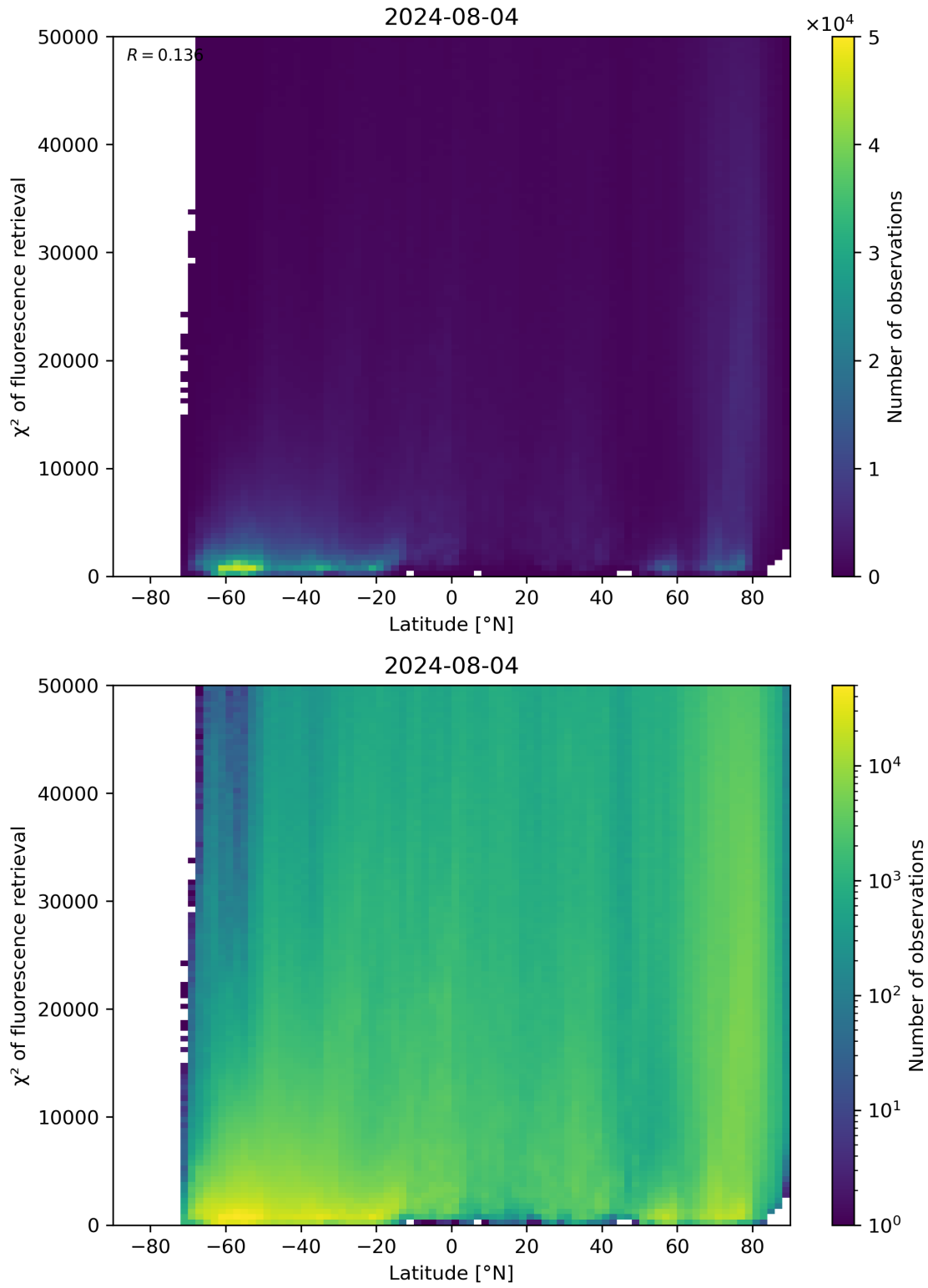
Figure 89: Scatter density plot of “Latitude” against “ \chi^2 of fluorescence retrieval” for 2024-08-03 to 2024-08-05.
