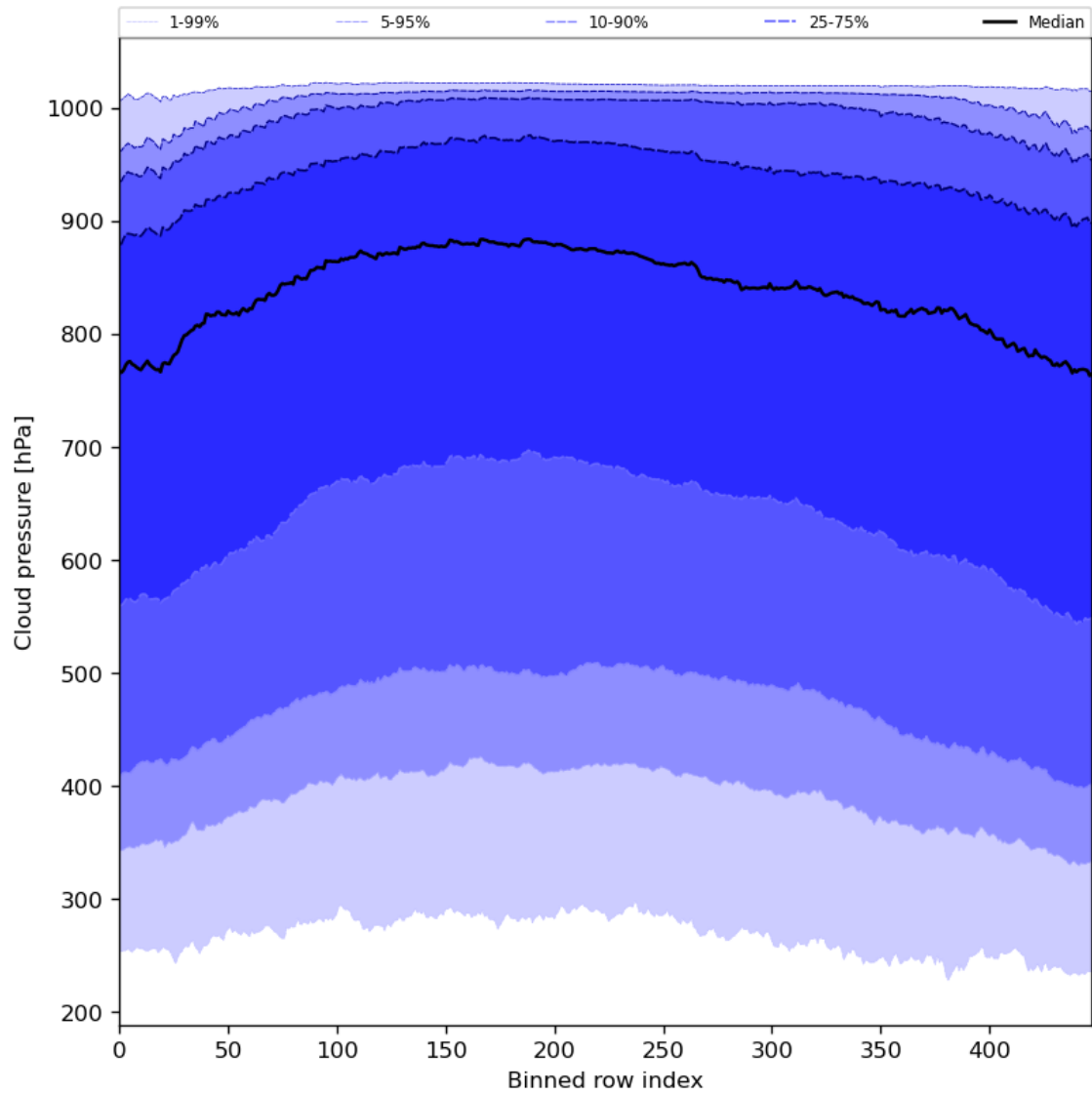
Figure 47: Along track statistics of “Cloud pressure” for 2024-08-03 to 2024-08-05
