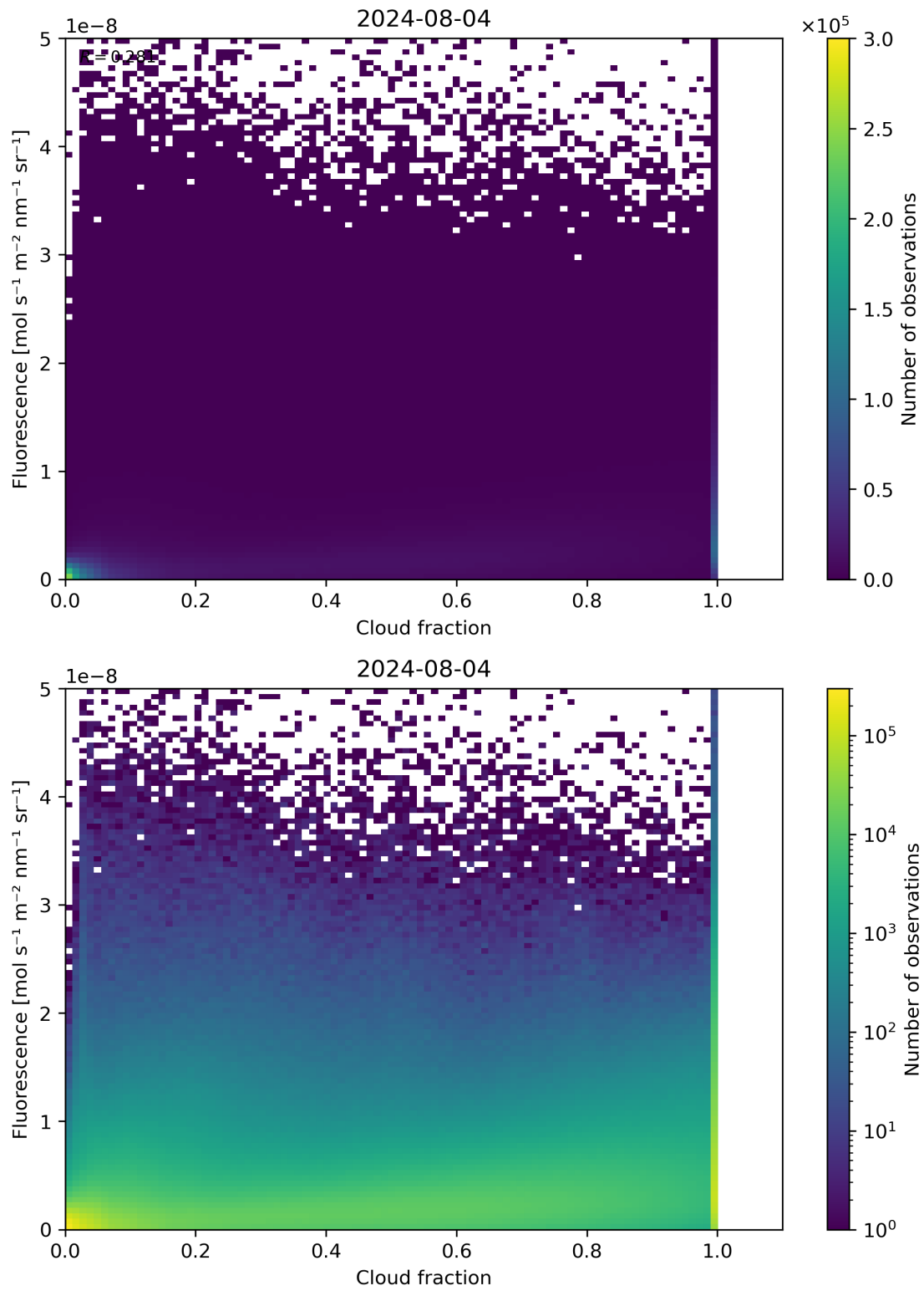
Figure 72: Scatter density plot of “Cloud fraction” against “Fluorescence” for 2024-08-03 to 2024-08-05.
