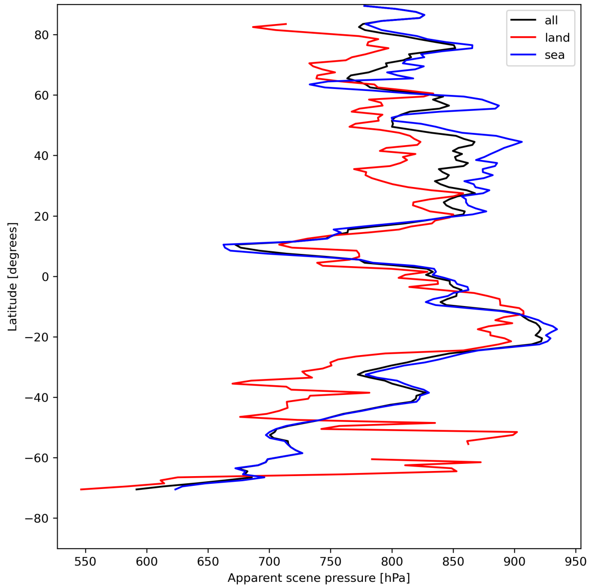
Figure 19: Zonal average of “Apparent scene pressure” for 2024-08-03 to 2024-08-05.
