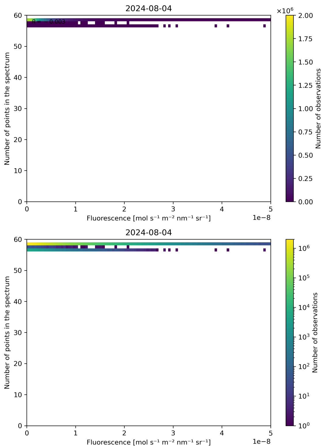
Figure 86: Scatter density plot of “Fluorescence” against “Number of points in the spectrum” for 2024-08-03 to 2024-08-05.
