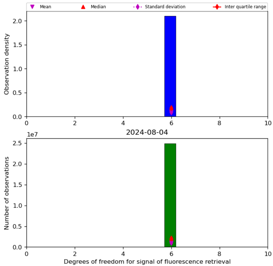
Figure 43: Histogram of “Degrees of freedom for signal of fluorescence retrieval” for 2024-08-03 to 2024-08-05
