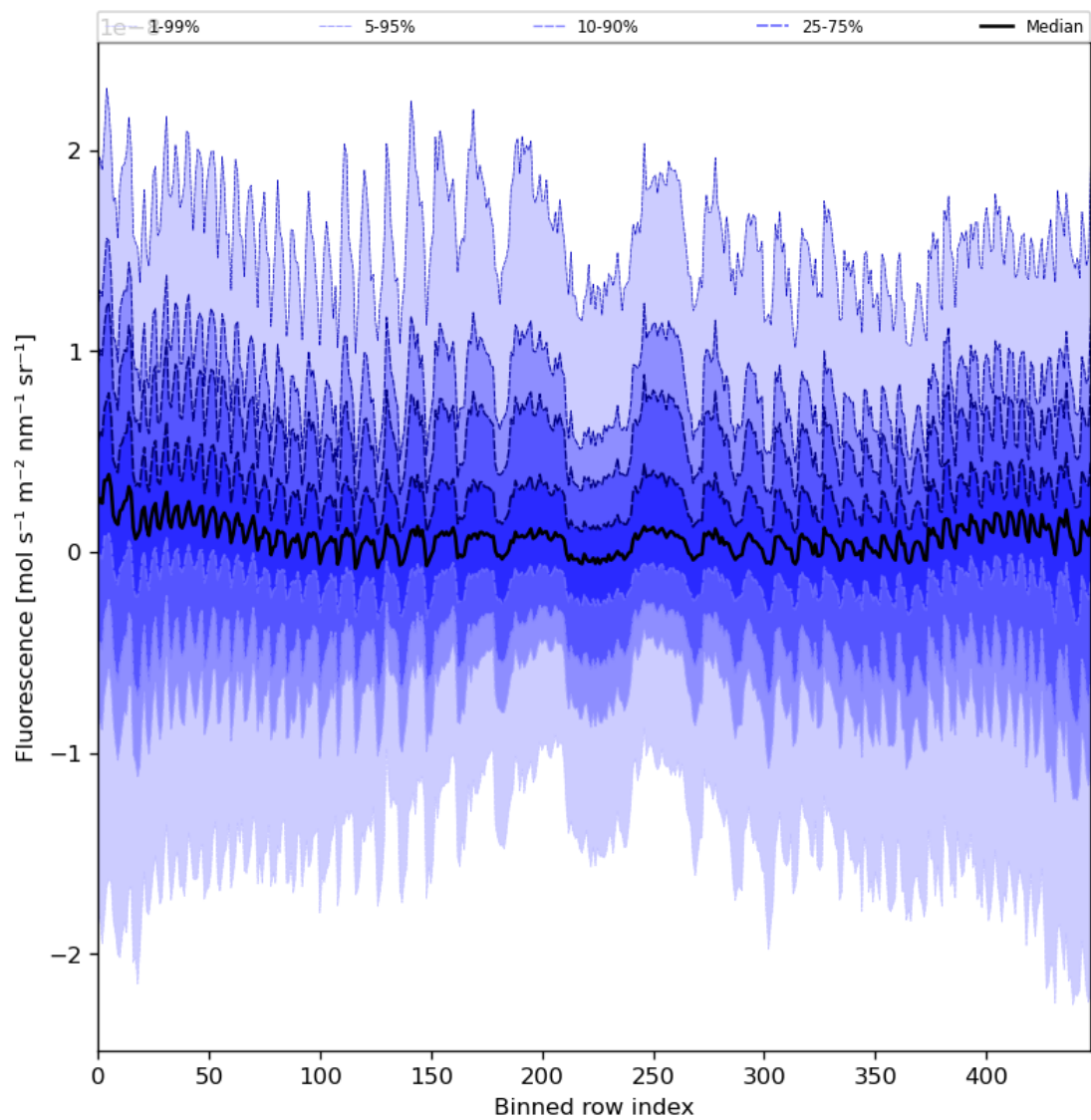
Figure 57: Along track statistics of “Fluorescence” for 2024-08-03 to 2024-08-05
