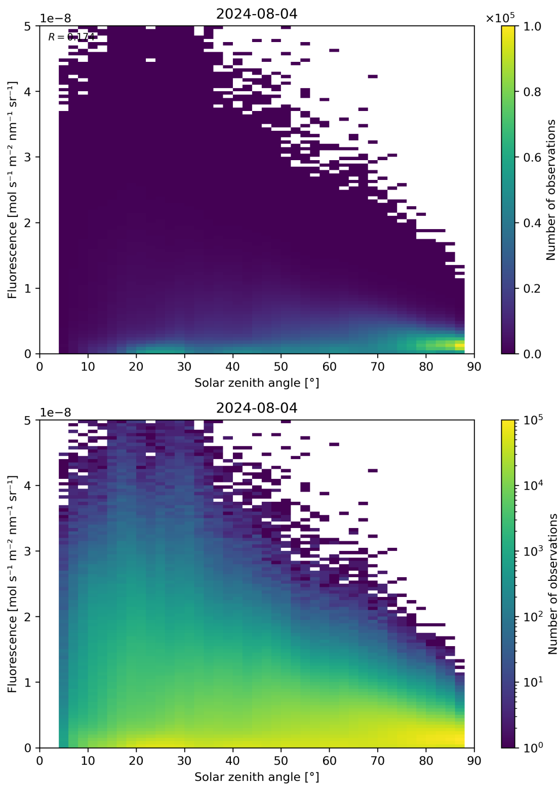
Figure 112: Scatter density plot of “Solar zenith angle” against “Fluorescence” for 2024-08-03 to 2024-08-05.
