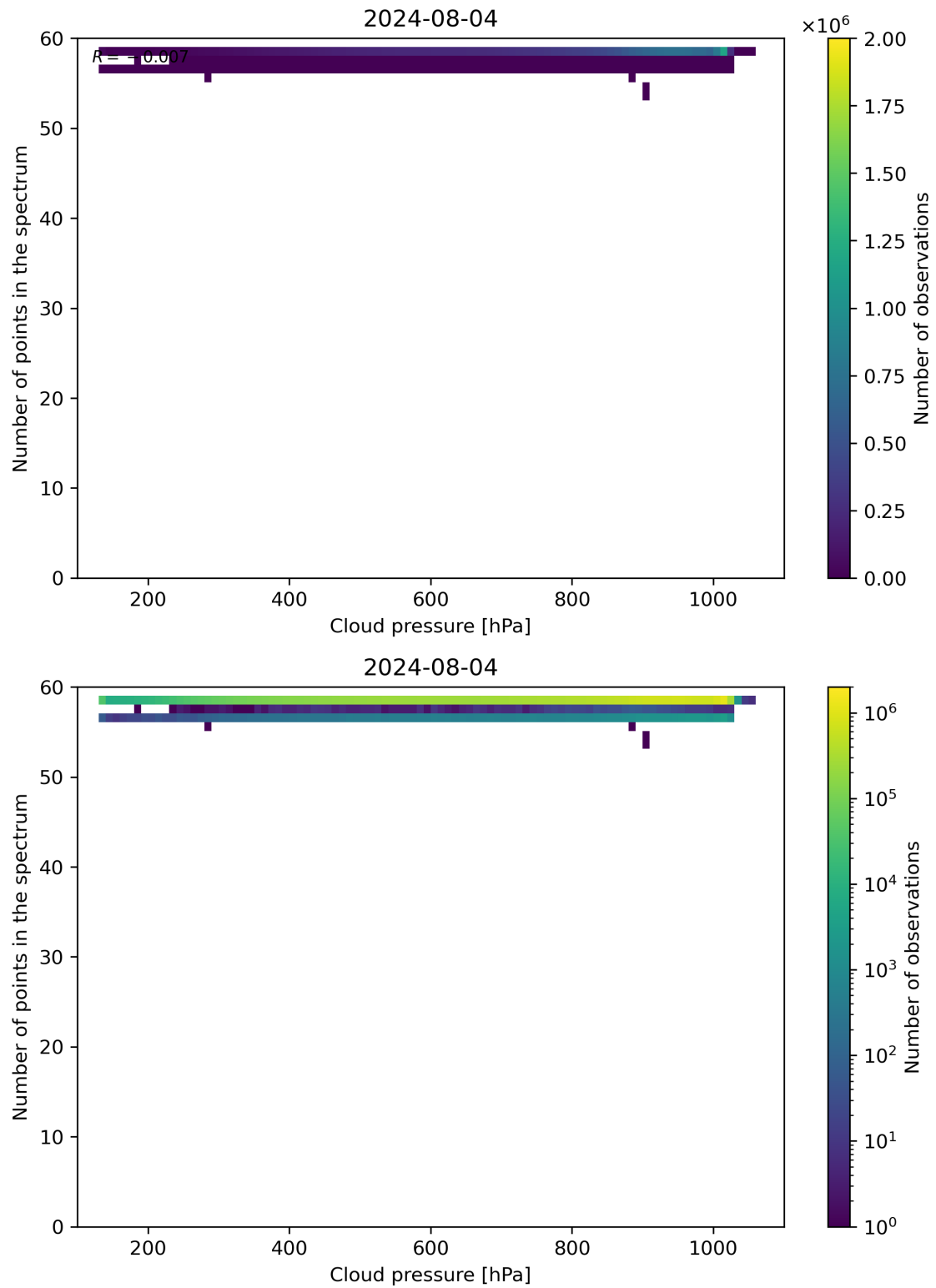
Figure 82: Scatter density plot of “Cloud pressure” against “Number of points in the spectrum” for 2024-08-03 to 2024-08-05.
