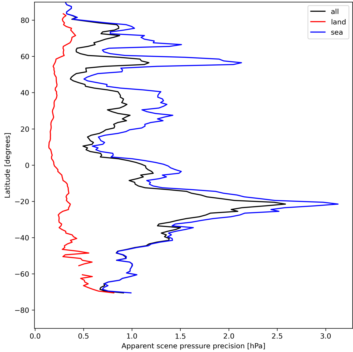
Figure 20: Zonal average of “Apparent scene pressure precision” for 2024-08-03 to 2024-08-05.
