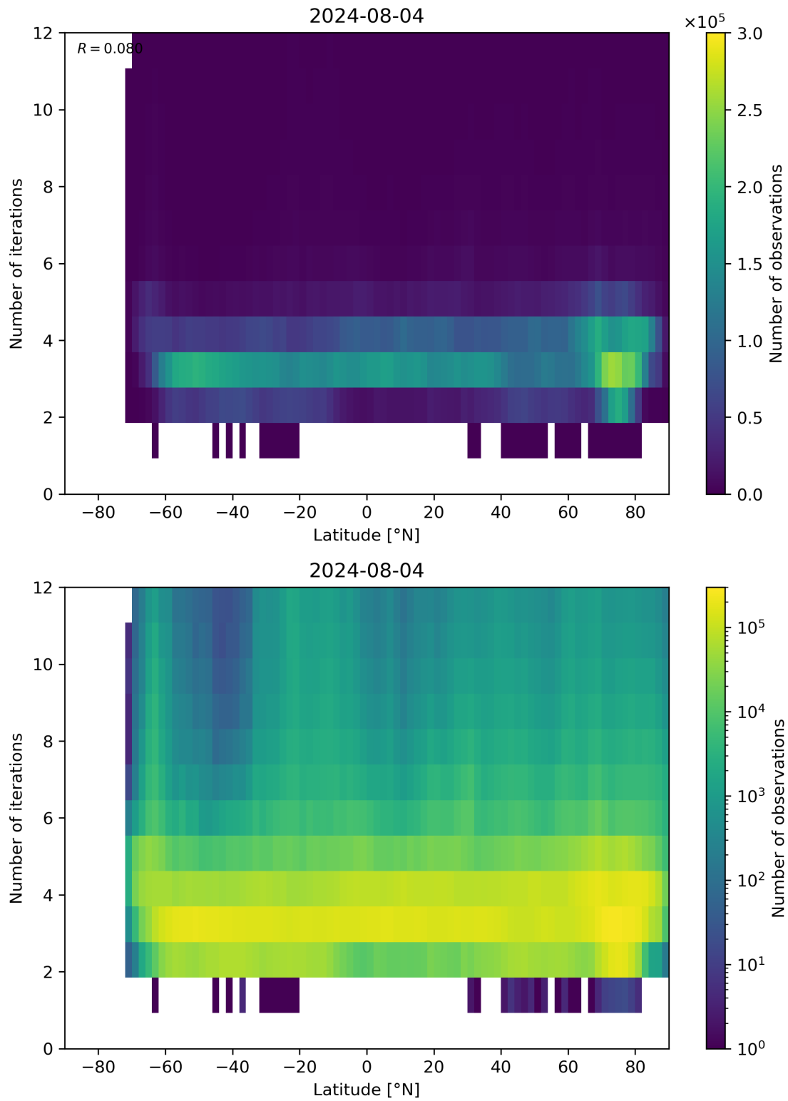
Figure 93: Scatter density plot of “Latitude” against “Number of iterations” for 2024-08-03 to 2024-08-05.
