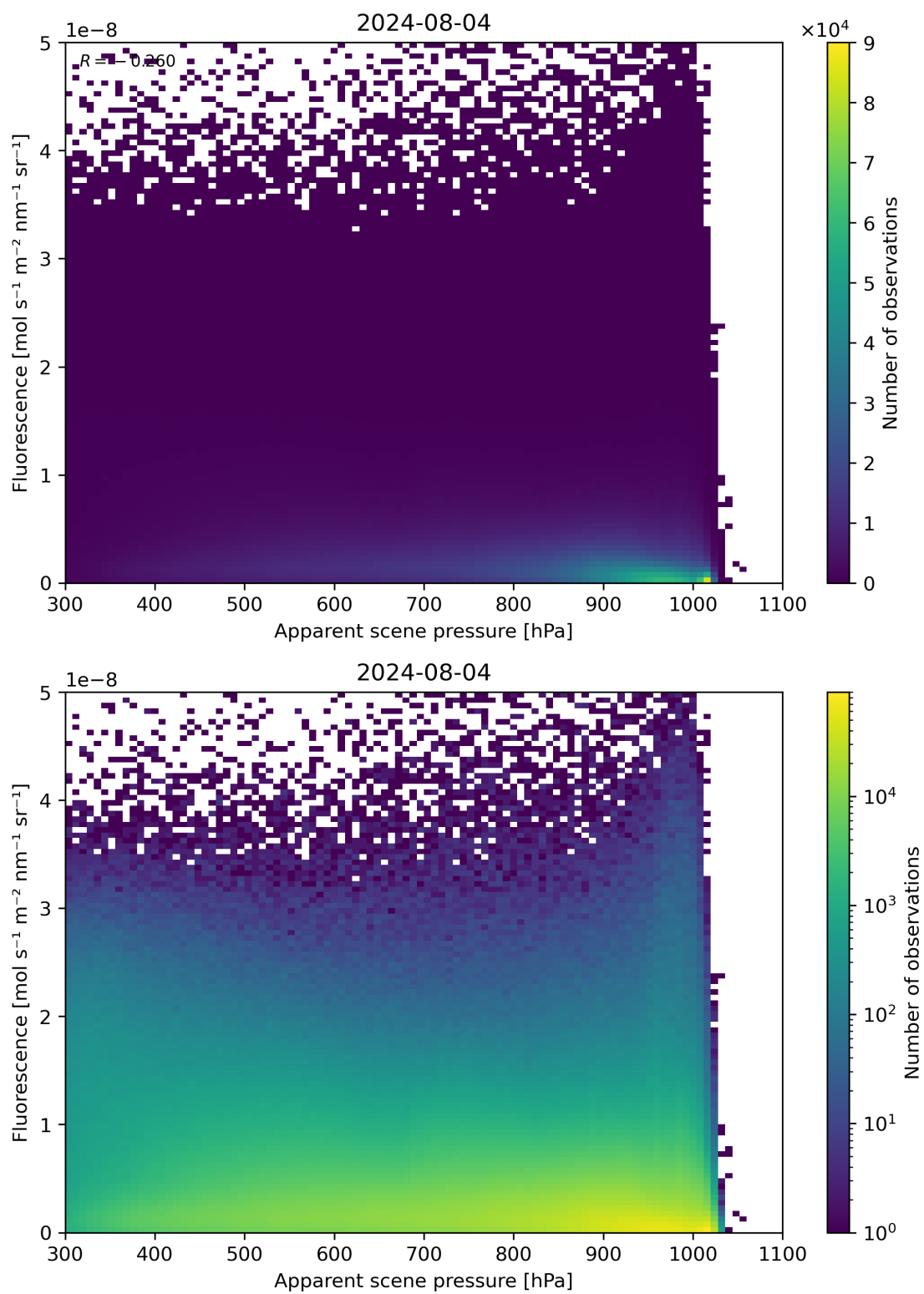
Figure 64: Scatter density plot of “Apparent scene pressure” against “Fluorescence” for 2024-08-03 to 2024-08-05.
