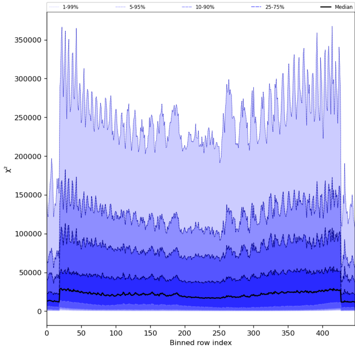
Figure 55: Along track statistics of “ \chi^2 ” for 2024-08-03 to 2024-08-05
