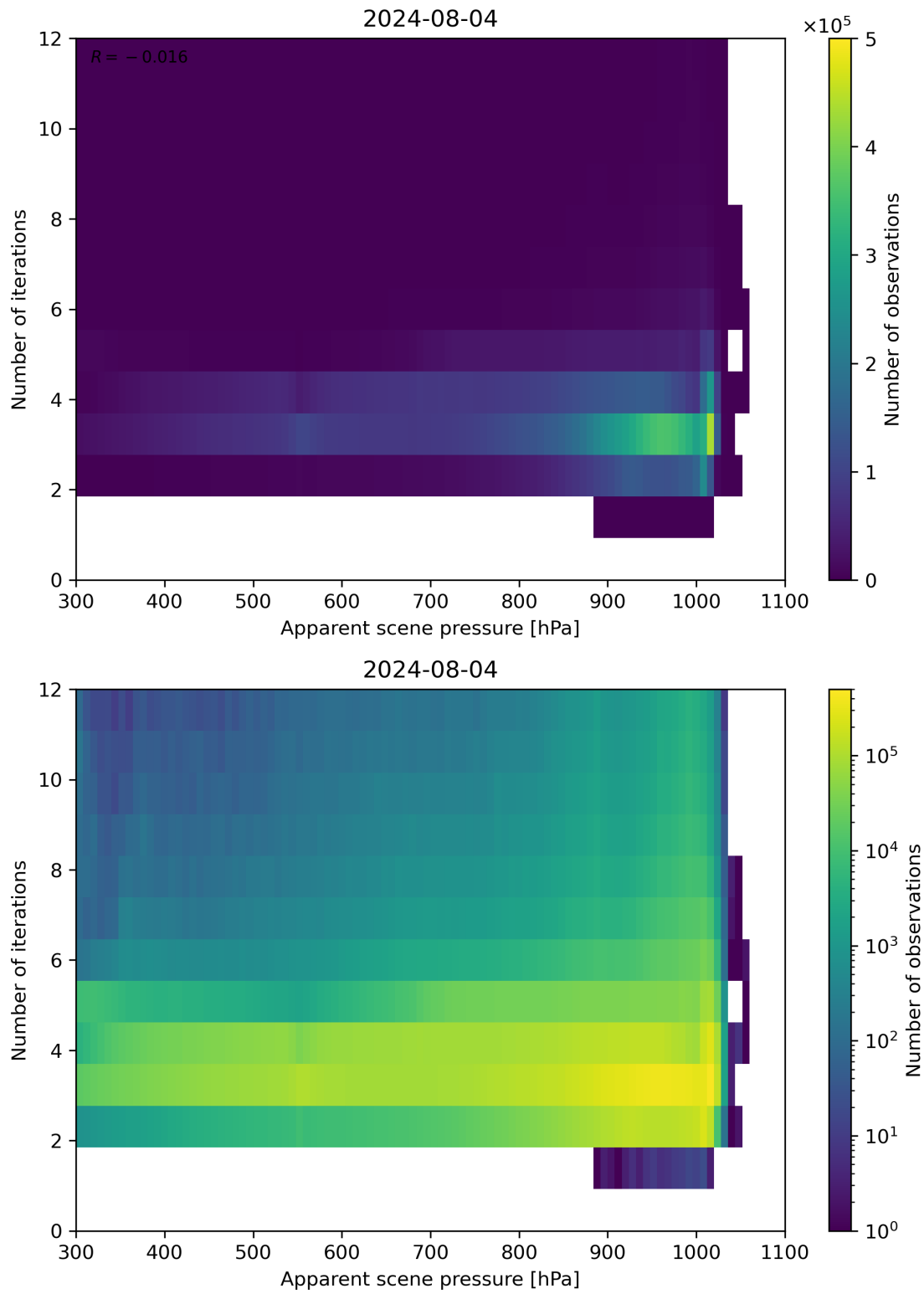
Figure 65: Scatter density plot of “Apparent scene pressure” against “Number of iterations” for 2024-08-03 to 2024-08-05.
