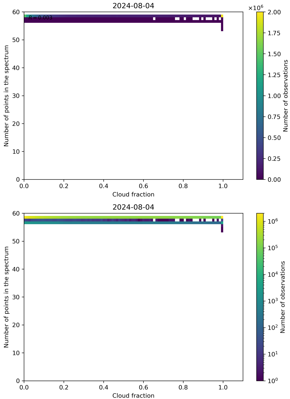
Figure 74: Scatter density plot of “Cloud fraction” against “Number of points in the spectrum” for 2024-08-03 to 2024-08-05.
