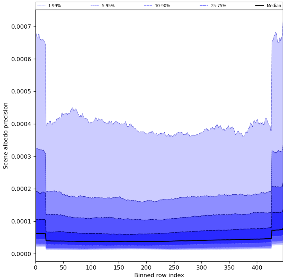
Figure 52: Along track statistics of “Scene albedo precision” for 2024-08-03 to 2024-08-05
