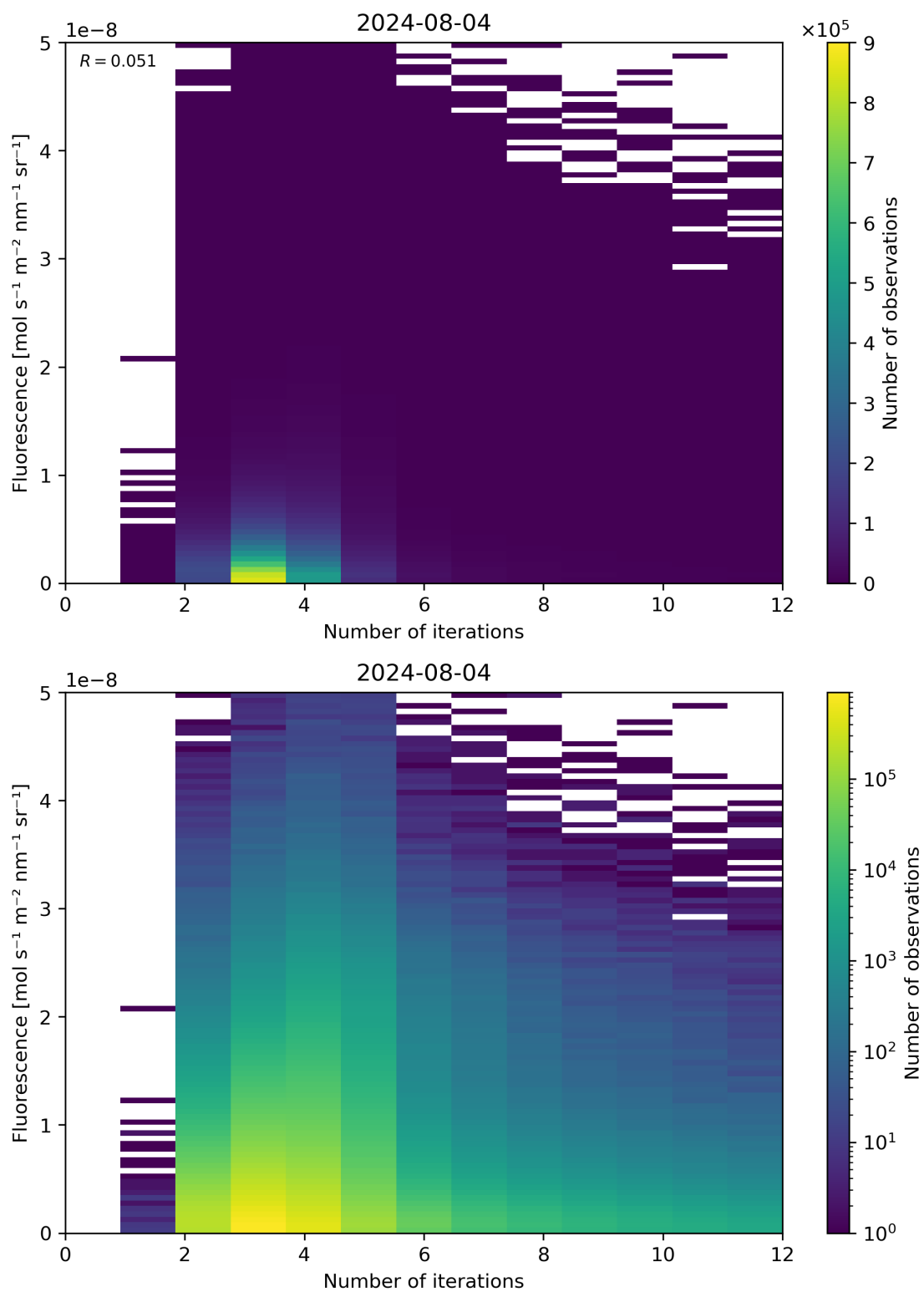
Figure 98: Scatter density plot of “Number of iterations” against “Fluorescence” for 2024-08-03 to 2024-08-05.
