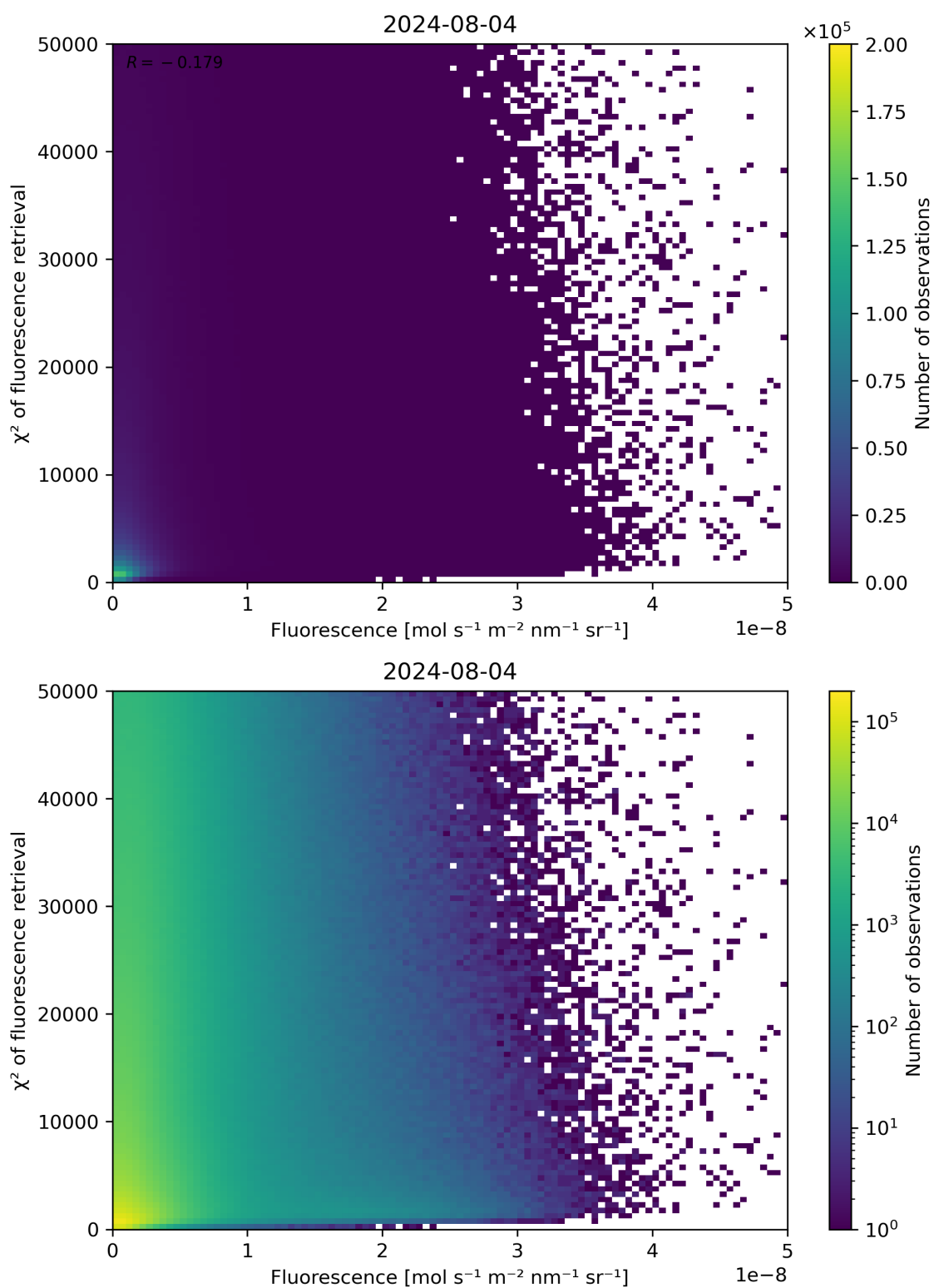
Figure 85: Scatter density plot of “Fluorescence” against “ \chi^2 of fluorescence retrieval” for 2024-08-03 to 2024-08-05.
