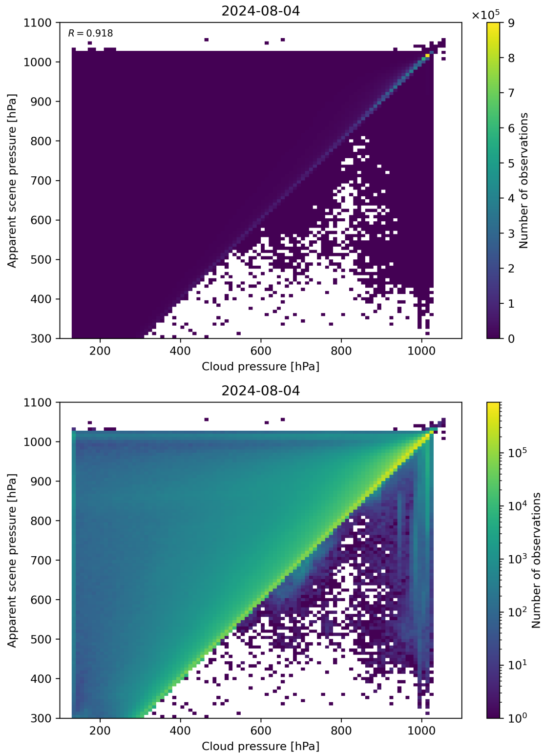
Figure 77: Scatter density plot of “Cloud pressure” against “Apparent scene pressure” for 2024-08-03 to 2024-08-05.
