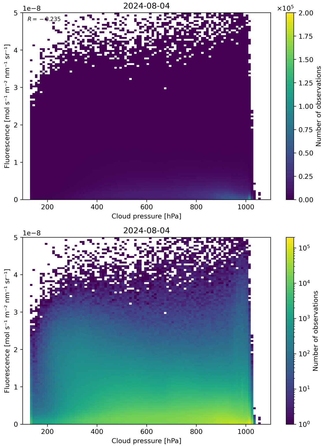
Figure 80: Scatter density plot of “Cloud pressure” against “Fluorescence” for 2024-08-03 to 2024-08-05.
