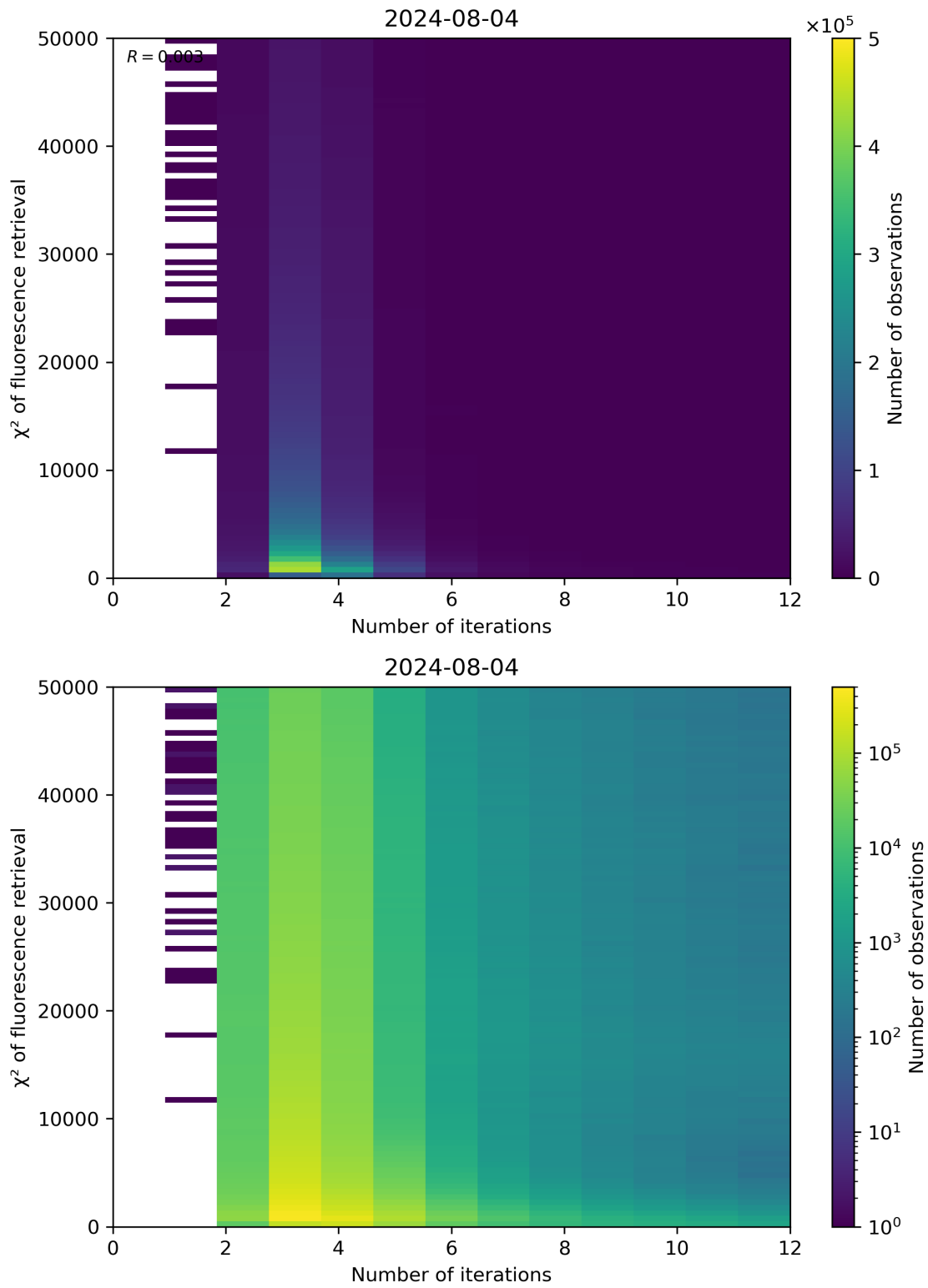
Figure 97: Scatter density plot of “Number of iterations” against “ \chi^2 of fluorescence retrieval” for 2024-08-03 to 2024-08-05.
