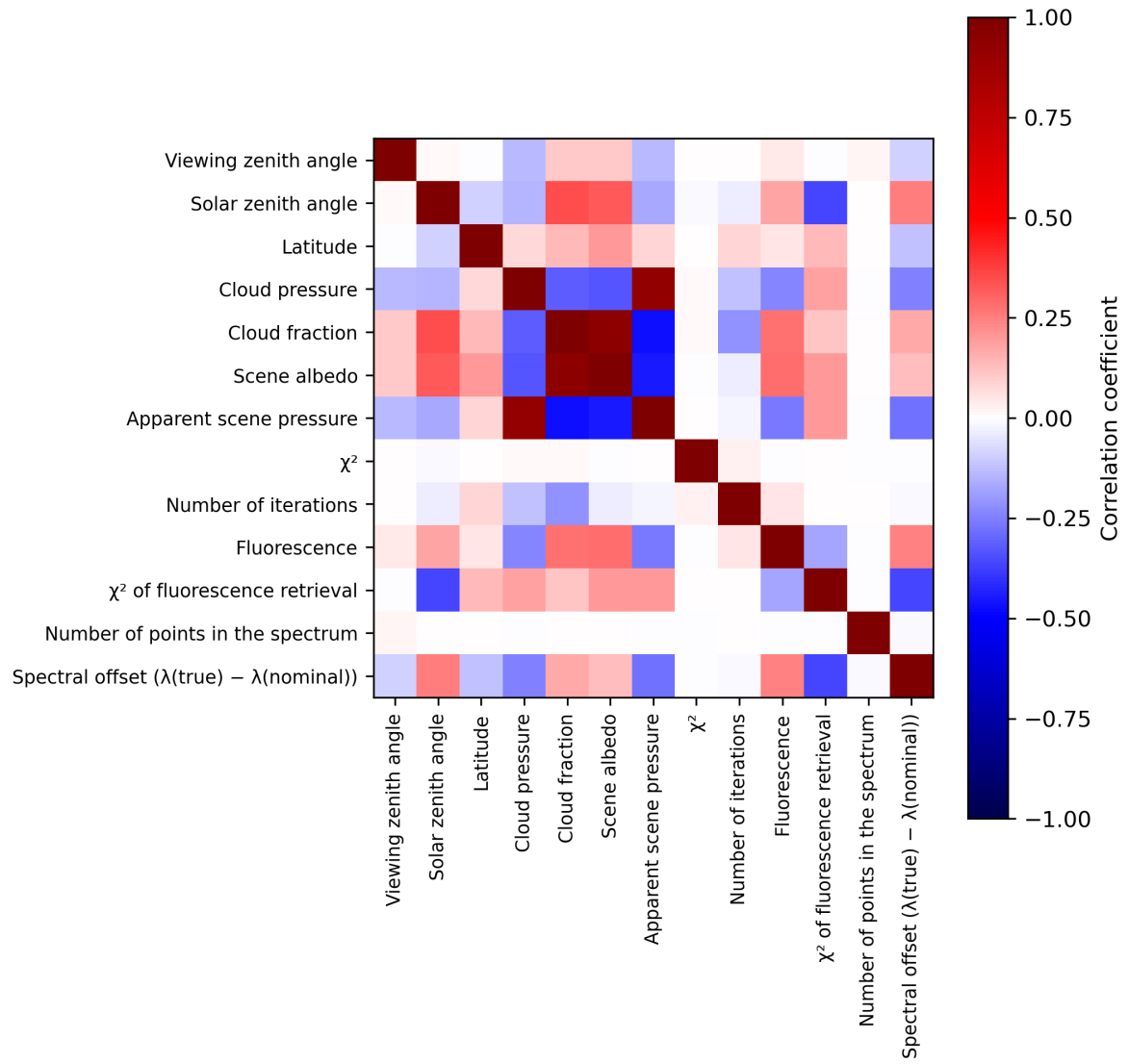
Figure 2: Map of correlation matrix for 2024-08-03 to 2024-08-05.
