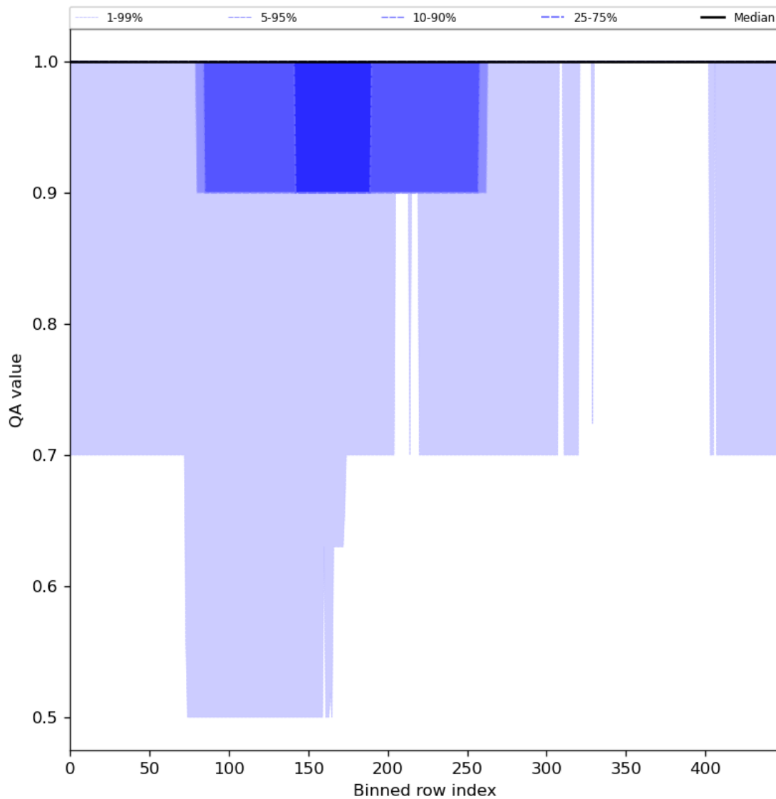
Figure 46: Along track statistics of “QA value” for 2024-08-03 to 2024-08-05
