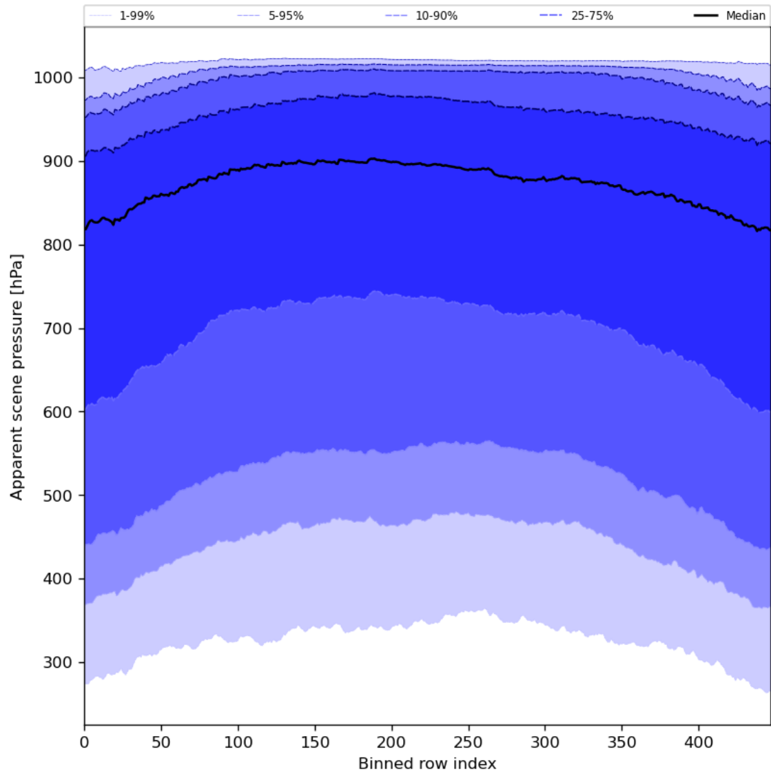
Figure 53: Along track statistics of “Apparent scene pressure” for 2024-08-03 to 2024-08-05
