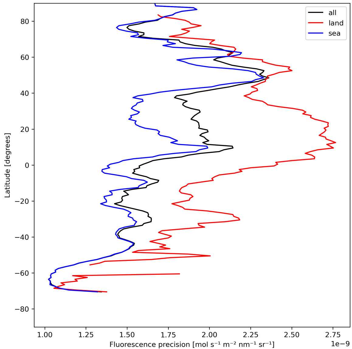
Figure 24: Zonal average of “Fluorescence precision” for 2024-08-03 to 2024-08-05.
