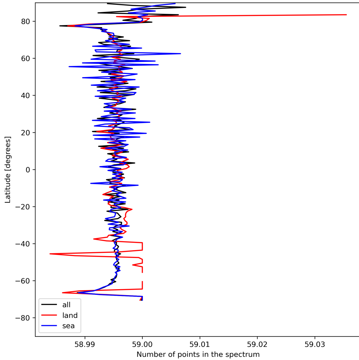
Figure 27: Zonal average of “Number of points in the spectrum” for 2024-08-03 to 2024-08-05.
