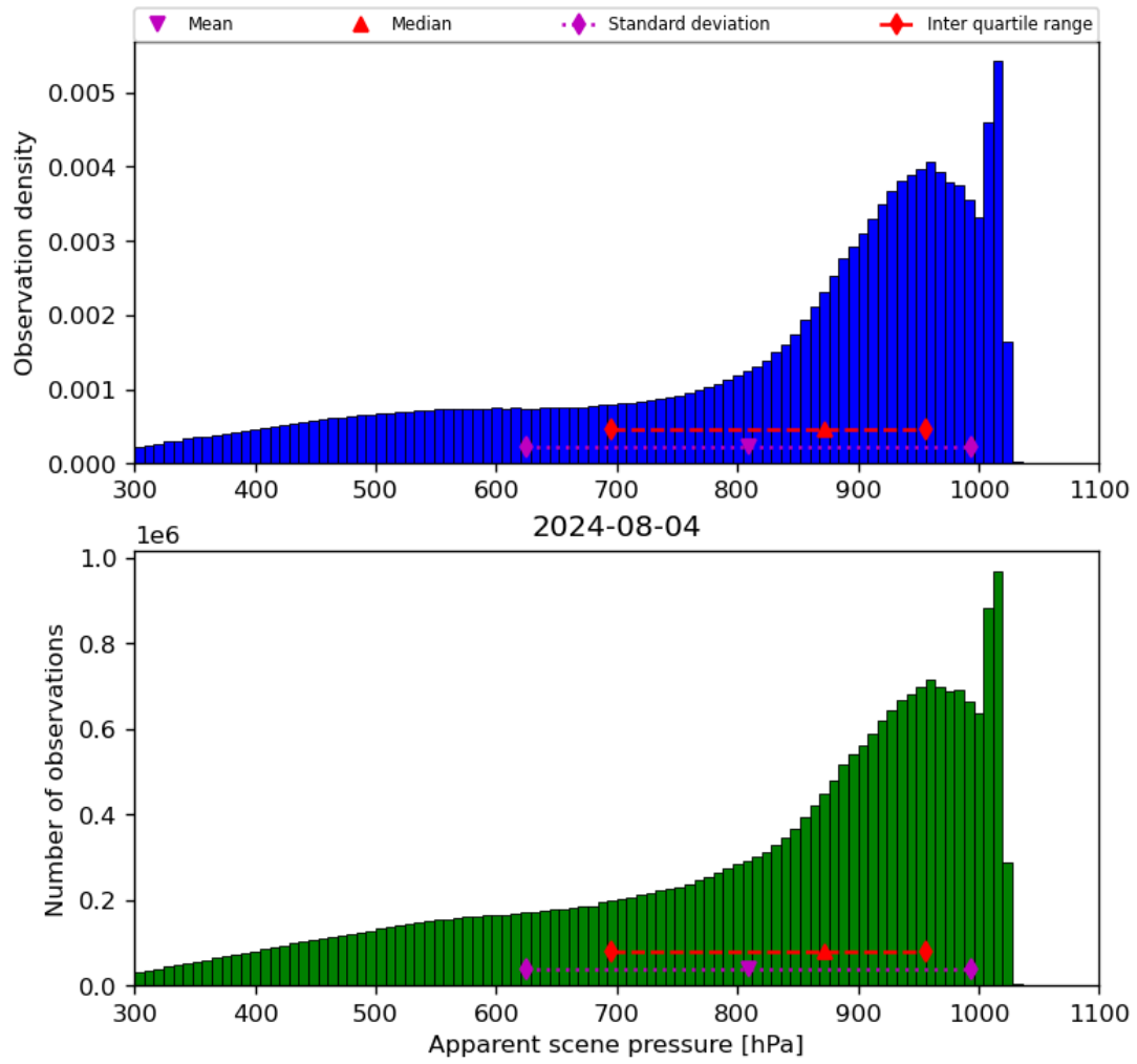
Figure 36: Histogram of “Apparent scene pressure” for 2024-08-03 to 2024-08-05
