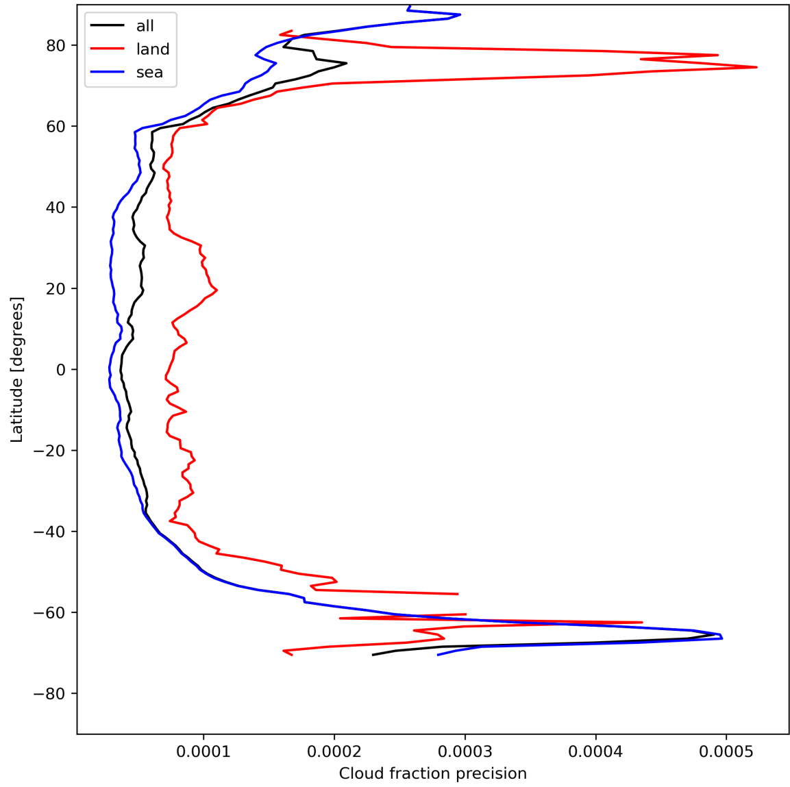
Figure 16: Zonal average of “Cloud fraction precision” for 2024-08-03 to 2024-08-05.
