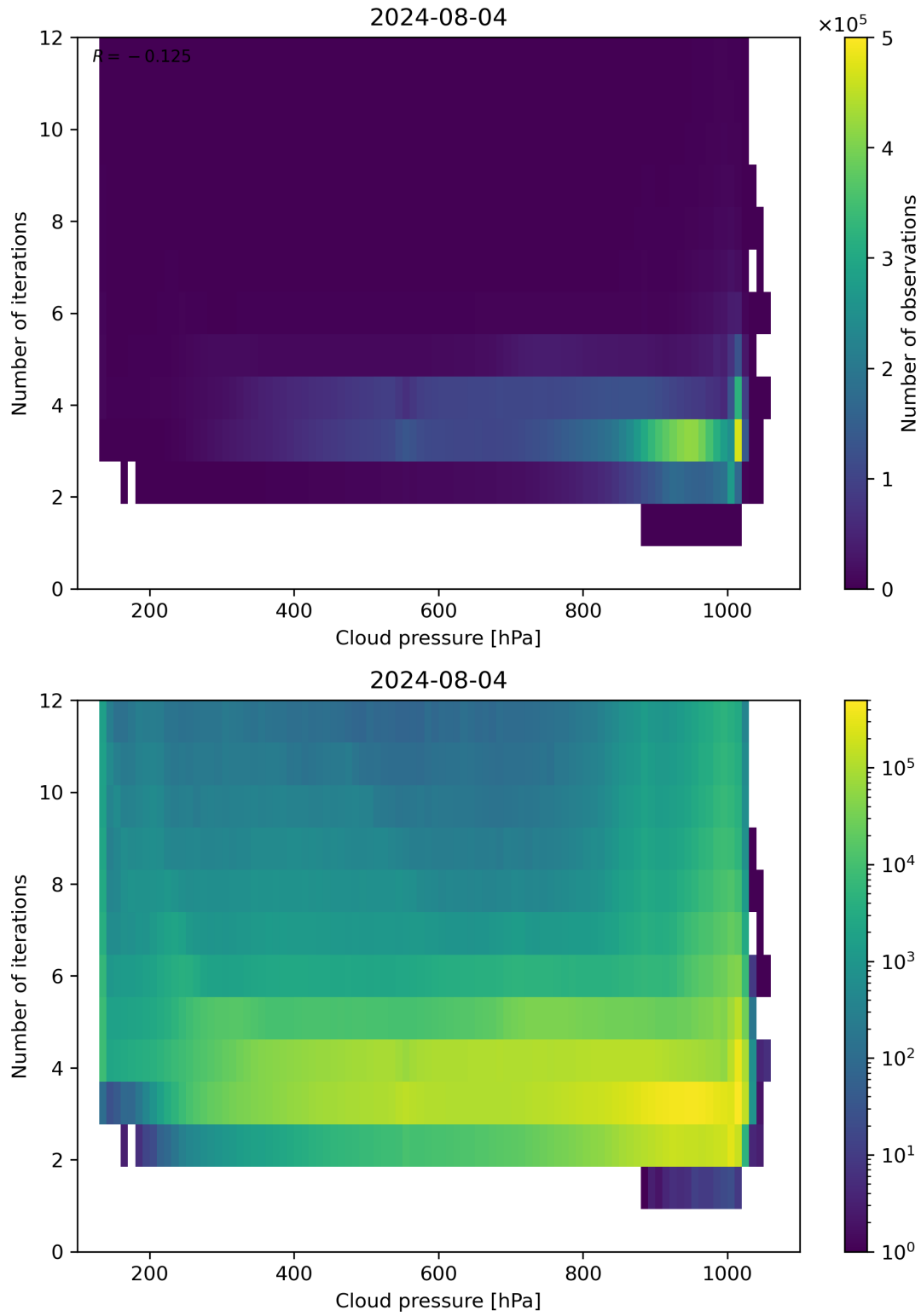
Figure 81: Scatter density plot of “Cloud pressure” against “Number of iterations” for 2024-08-03 to 2024-08-05.
