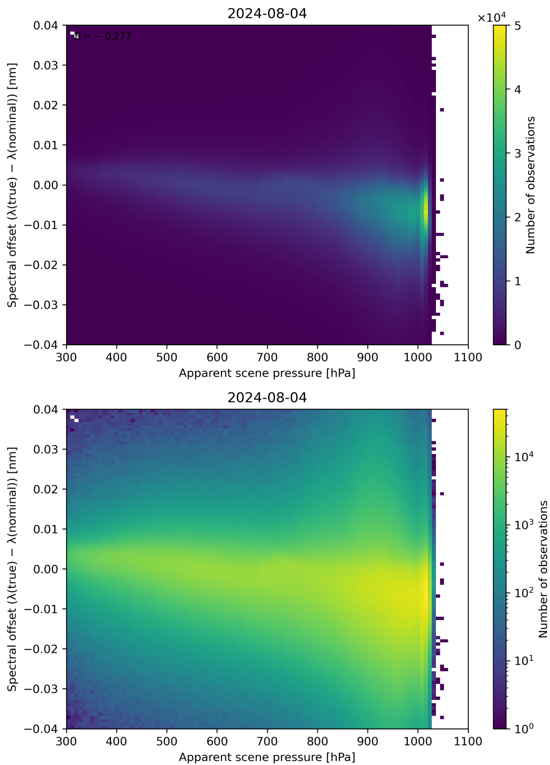
Figure 67: Scatter density plot of “Apparent scene pressure” against “Spectral offset ( \lambda(\text{true}) - \lambda(\text{nominal}) )” for 2024-08-03 to 2024-08-05.
