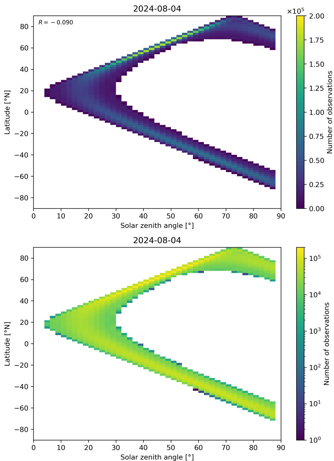
Figure 113: Scatter density plot of “Solar zenith angle” against “Latitude” for 2024-08-03 to 2024-08-05.
