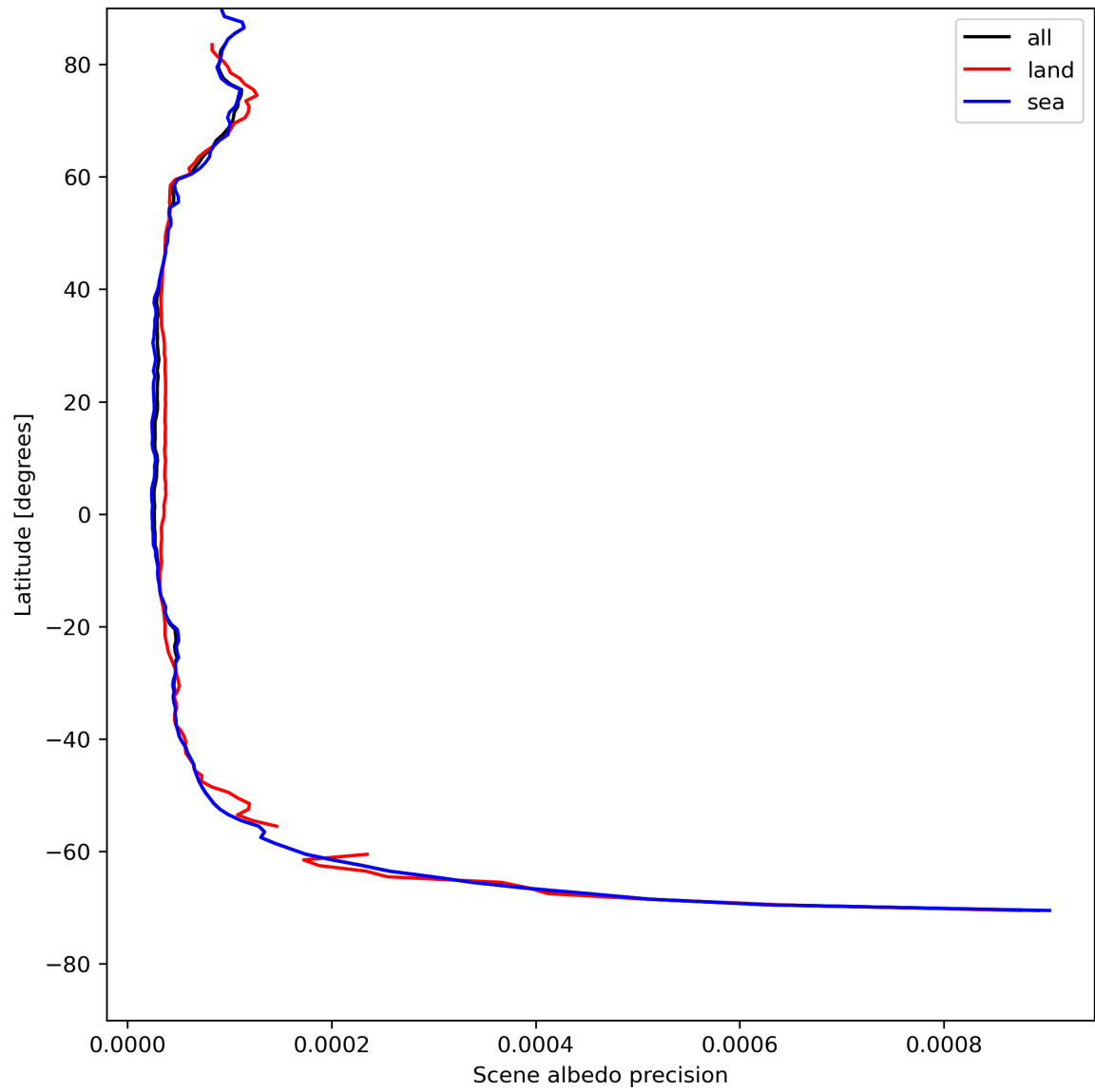
Figure 18: Zonal average of “Scene albedo precision” for 2024-08-03 to 2024-08-05.
