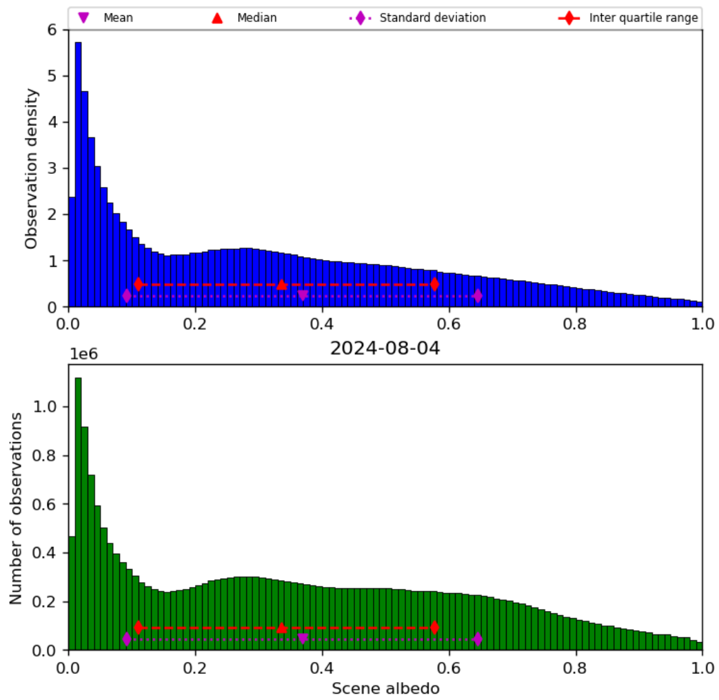
Figure 34: Histogram of “Scene albedo” for 2024-08-03 to 2024-08-05
