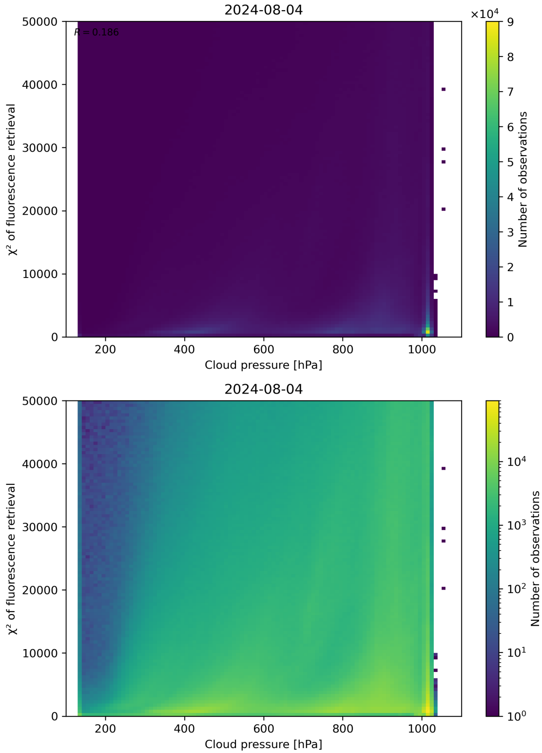
Figure 78: Scatter density plot of “Cloud pressure” against “ \chi^2 of fluorescence retrieval” for 2024-08-03 to 2024-08-05.
