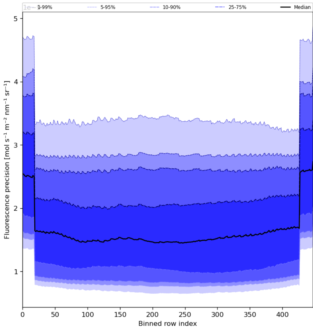
Figure 58: Along track statistics of “Fluorescence precision” for 2024-08-03 to 2024-08-05
