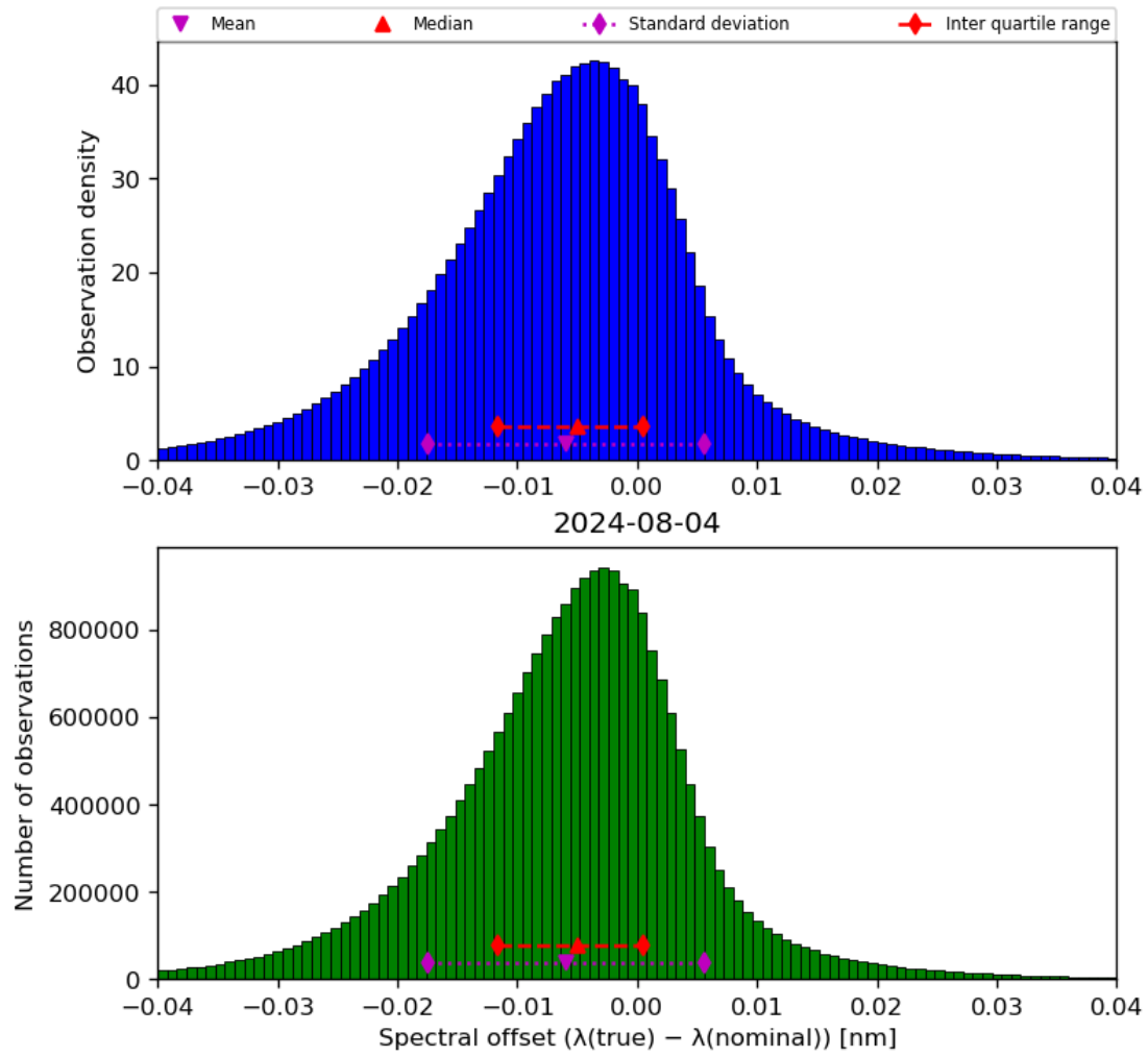
Figure 45: Histogram of “Spectral offset ( \lambda(\text{true}) - \lambda(\text{nominal}) )” for 2024-08-03 to 2024-08-05
