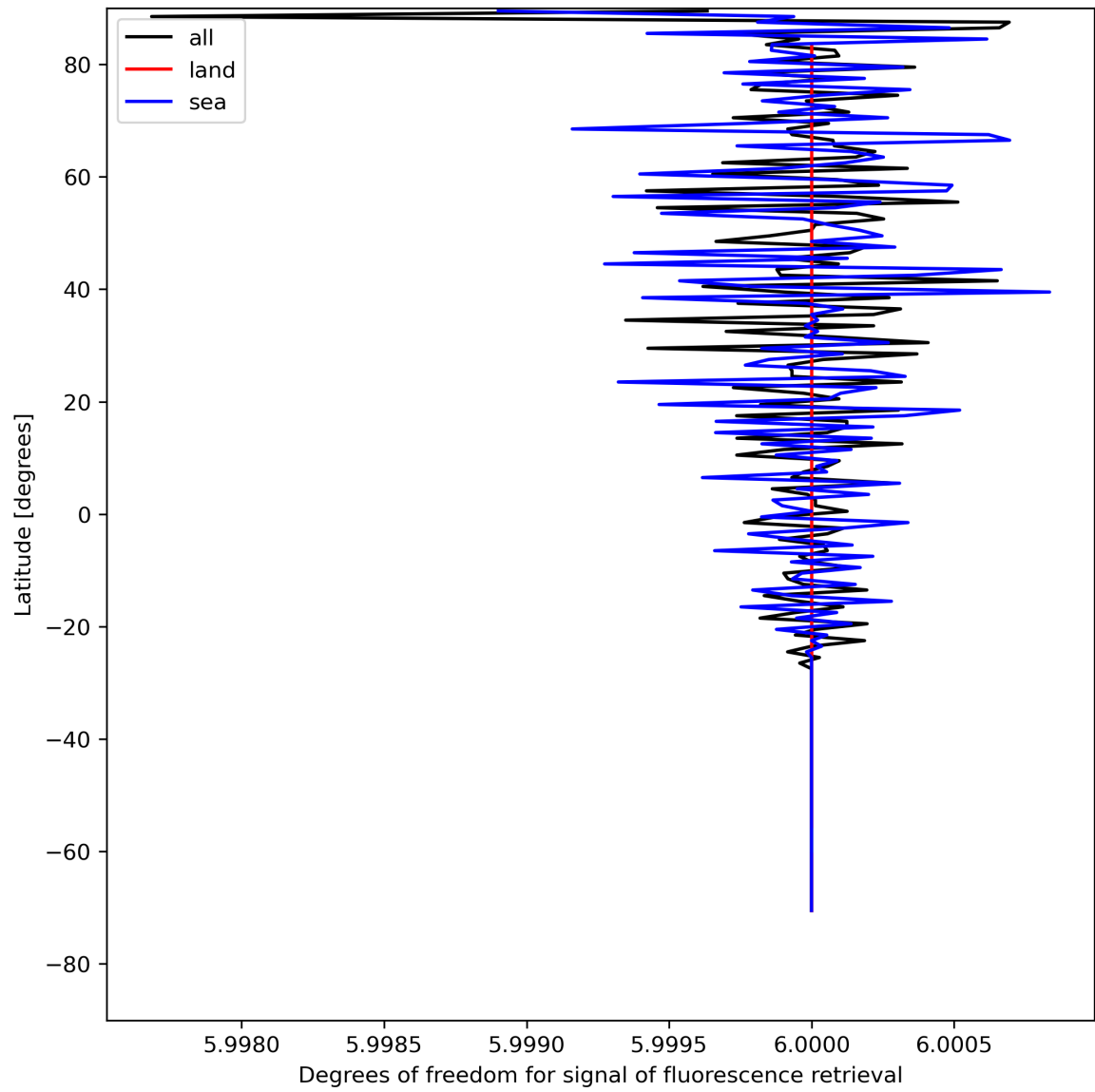
Figure 26: Zonal average of “Degrees of freedom for signal of fluorescence retrieval” for 2024-08-03 to 2024-08-05.
