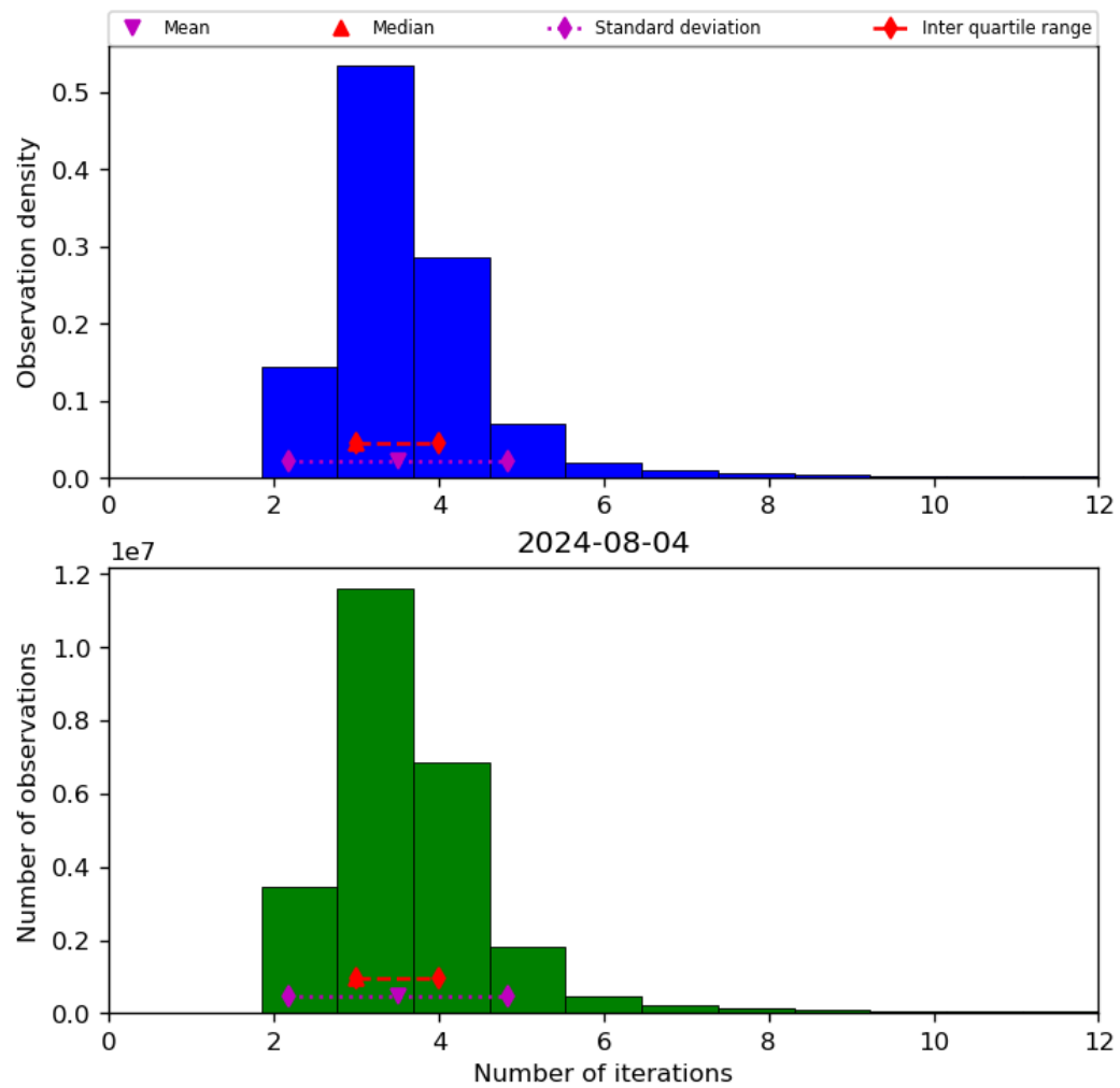
Figure 39: Histogram of “Number of iterations” for 2024-08-03 to 2024-08-05
