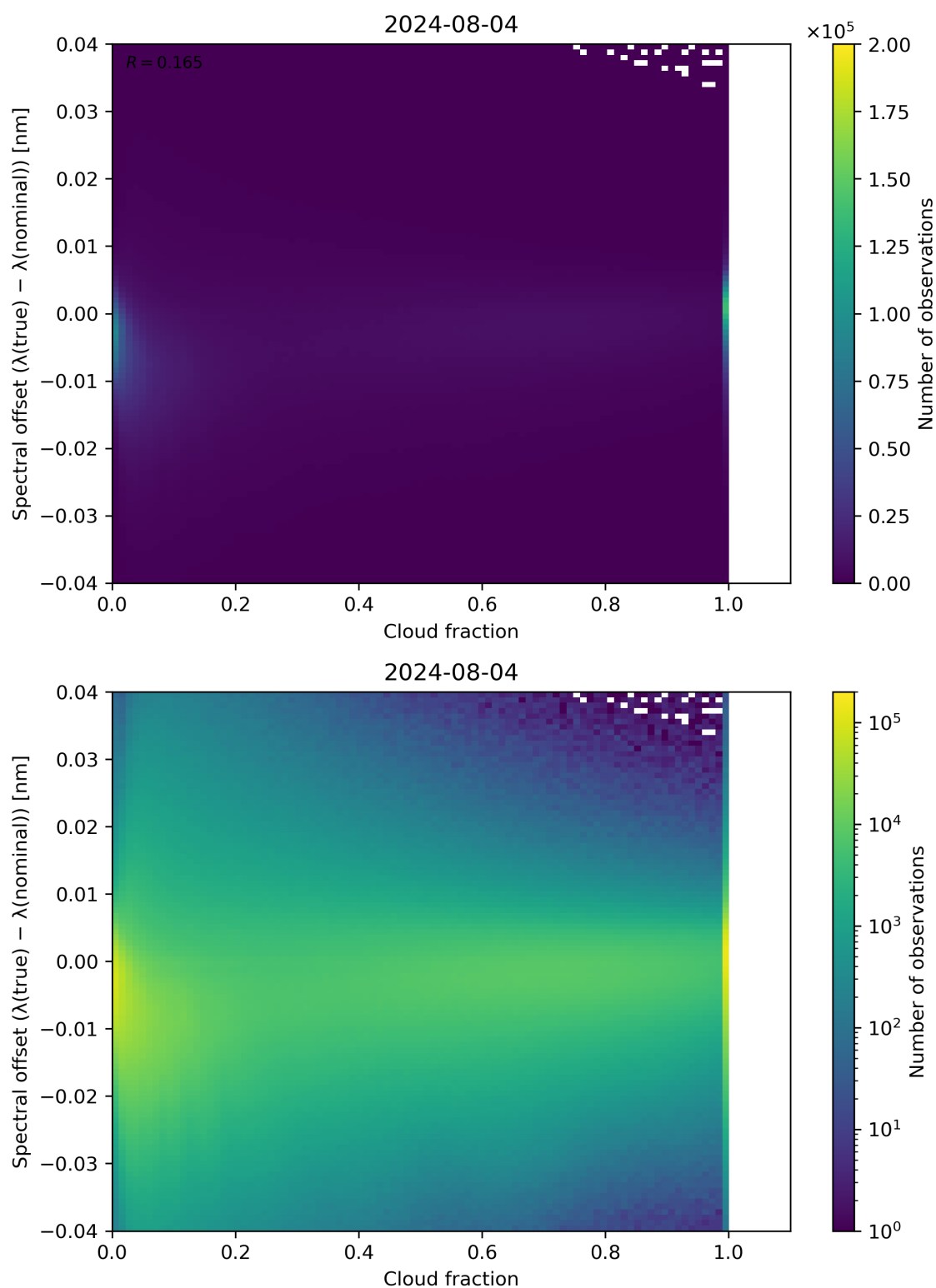
Figure 76: Scatter density plot of “Cloud fraction” against “Spectral offset ( \lambda(\text{true}) - \lambda(\text{nominal}) )” for 2024-08-03 to 2024-08-05.
