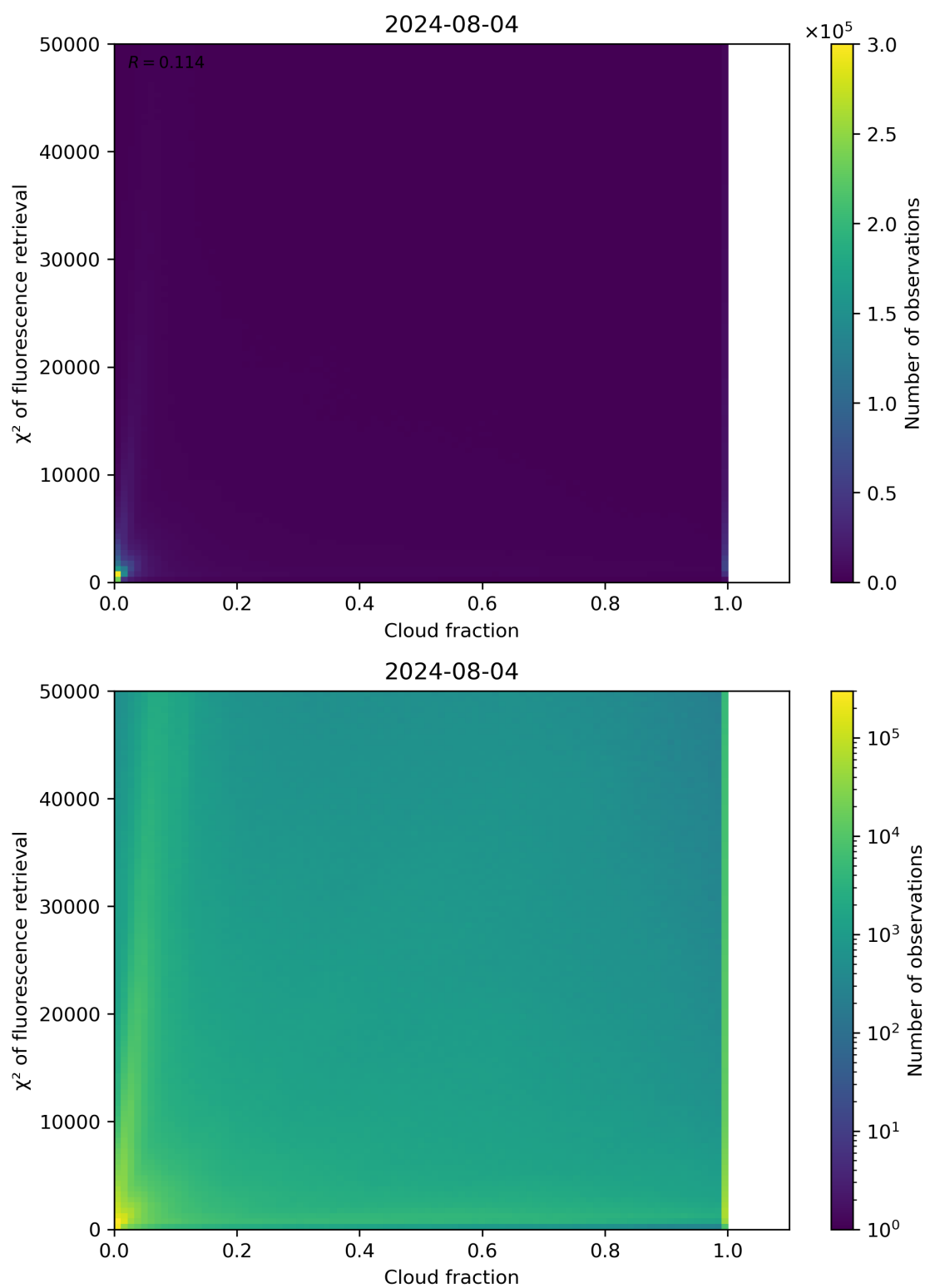
Figure 71: Scatter density plot of “Cloud fraction” against “ \chi^2 of fluorescence retrieval” for 2024-08-03 to 2024-08-05.
