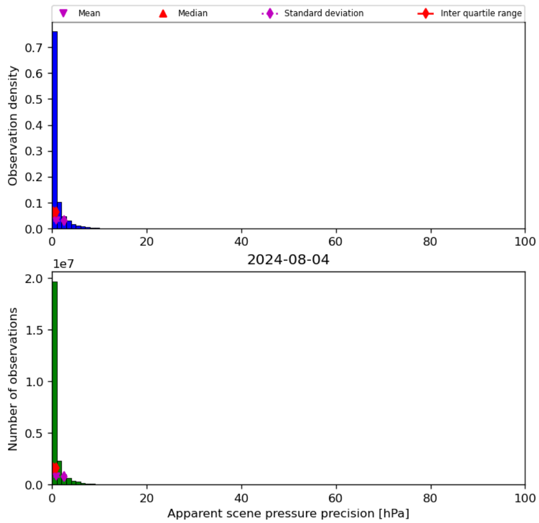
Figure 37: Histogram of “Apparent scene pressure precision” for 2024-08-03 to 2024-08-05
