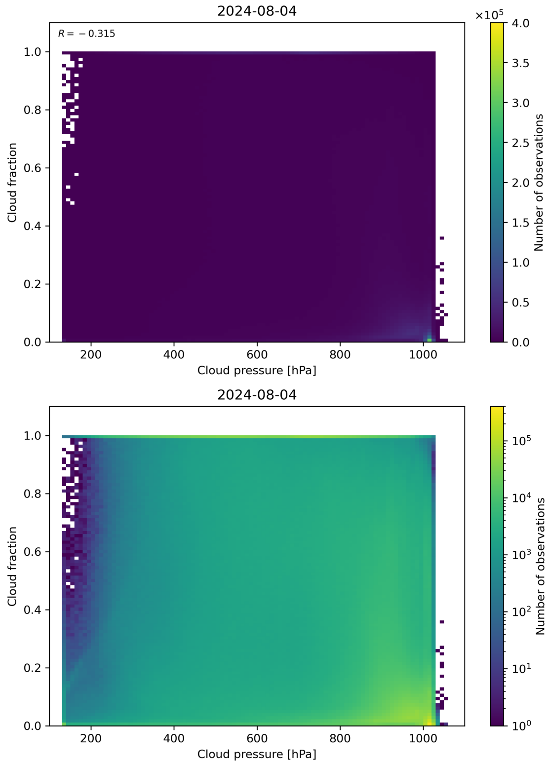
Figure 79: Scatter density plot of “Cloud pressure” against “Cloud fraction” for 2024-08-03 to 2024-08-05.
