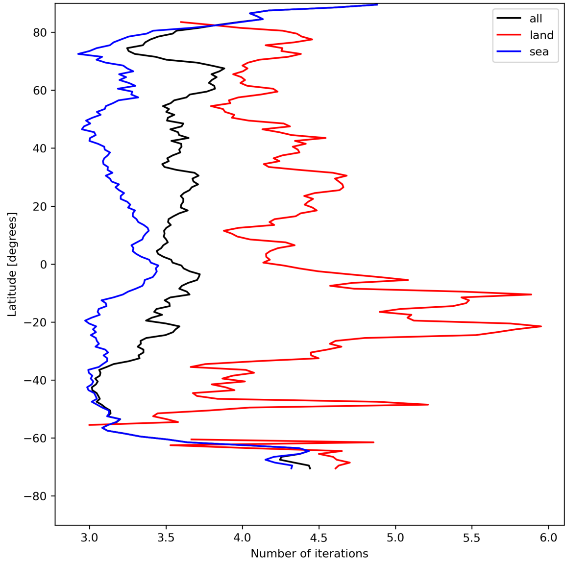
Figure 22: Zonal average of “Number of iterations” for 2024-08-03 to 2024-08-05.
