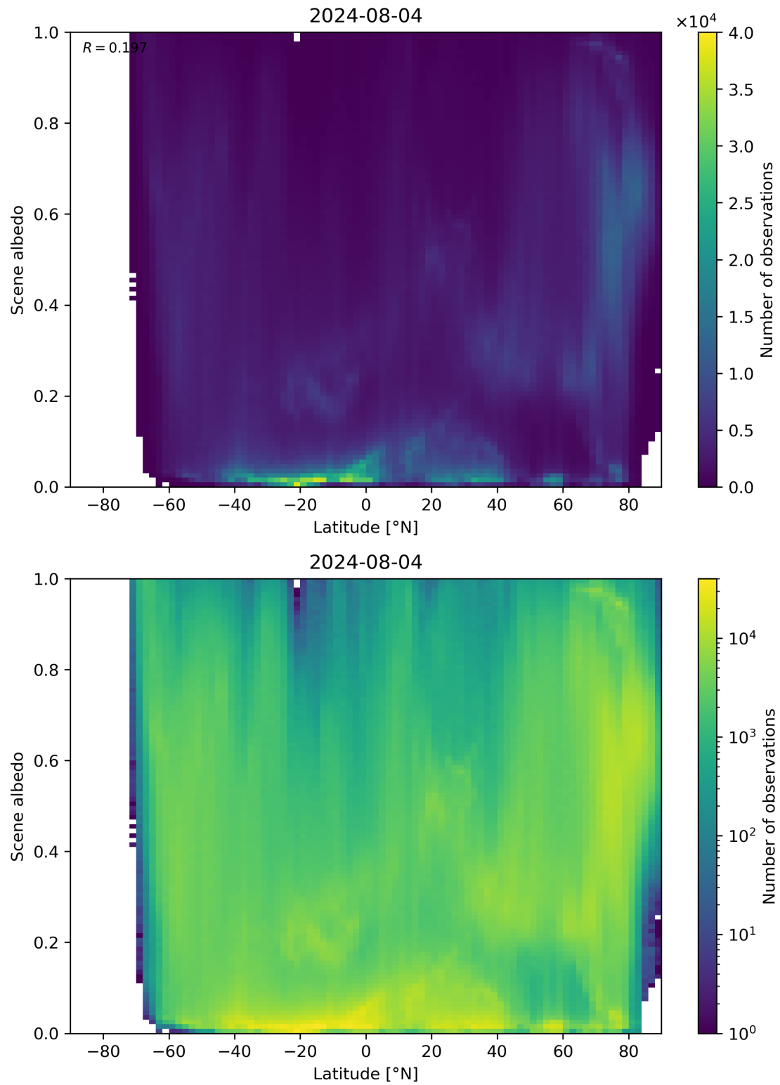
Figure 95: Scatter density plot of “Latitude” against “Scene albedo” for 2024-08-03 to 2024-08-05.
