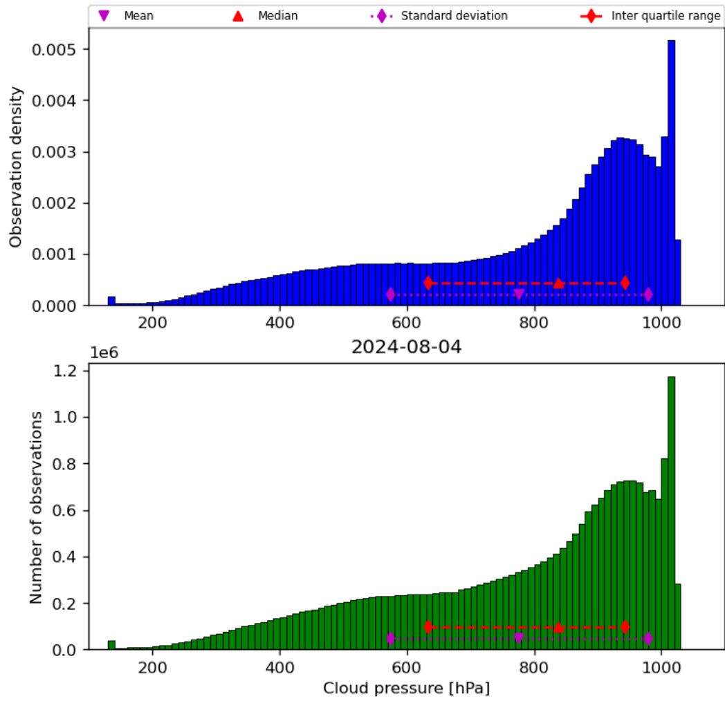
Figure 30: Histogram of “Cloud pressure” for 2024-08-03 to 2024-08-05
