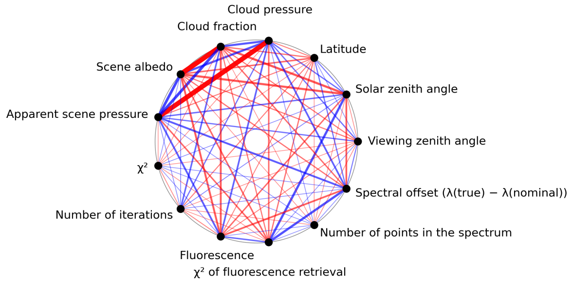
Figure 1: Map of correlation graph for 2024-08-03 to 2024-08-05.
