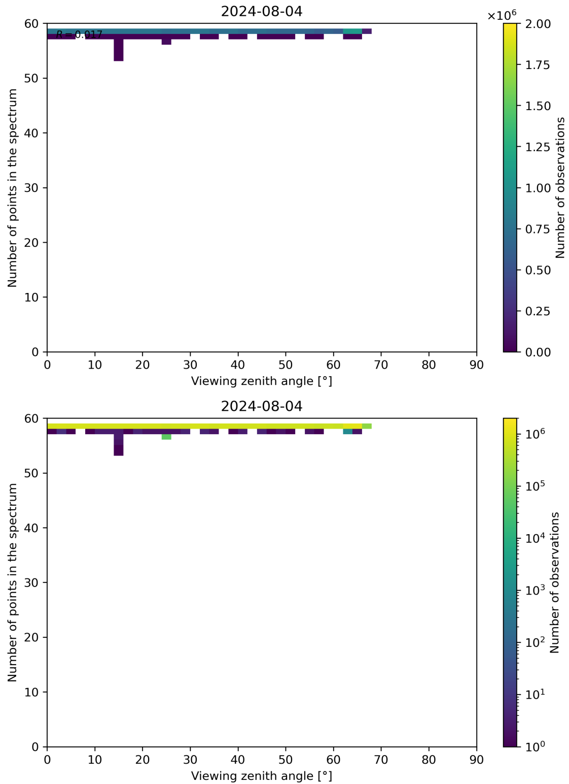
Figure 125: Scatter density plot of “Viewing zenith angle” against “Number of points in the spectrum” for 2024-08-03 to 2024-08-05.
