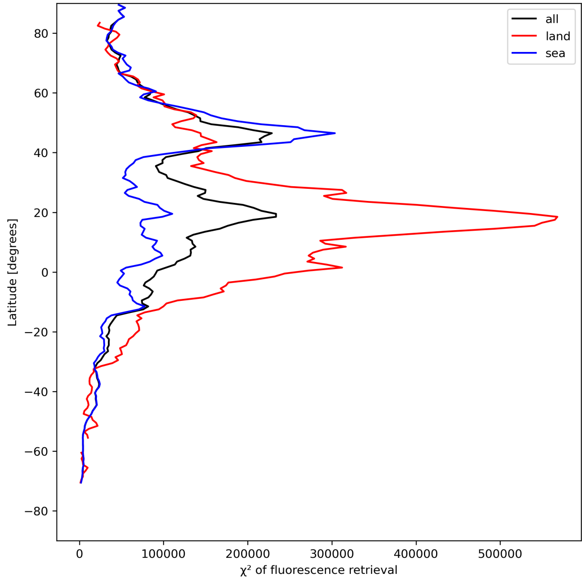
Figure 25: Zonal average of “ \chi^2 of fluorescence retrieval” for 2024-08-03 to 2024-08-05.
