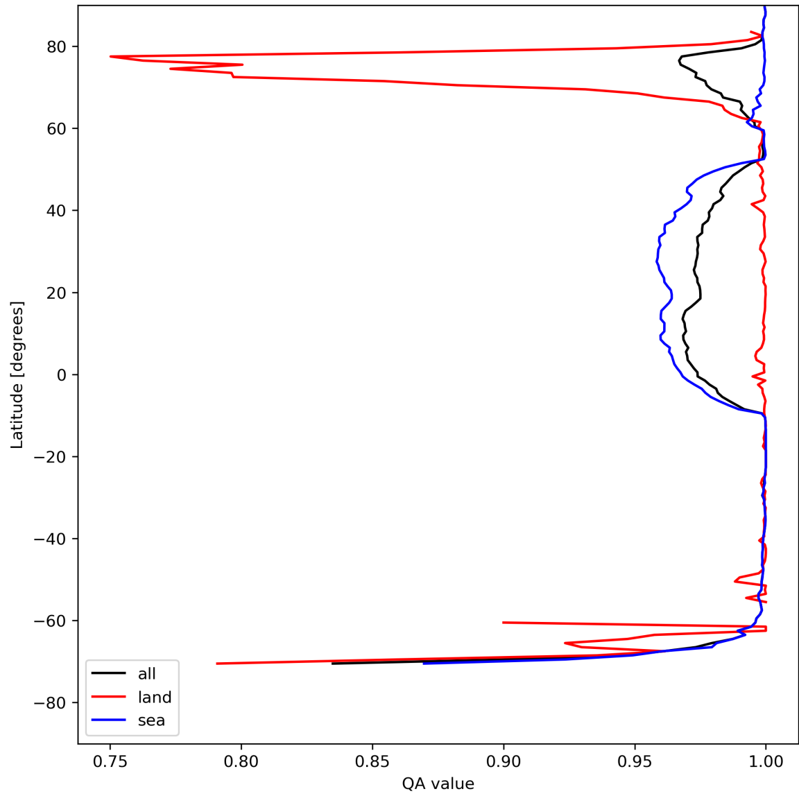
Figure 12: Zonal average of “QA value” for 2024-08-03 to 2024-08-05.
