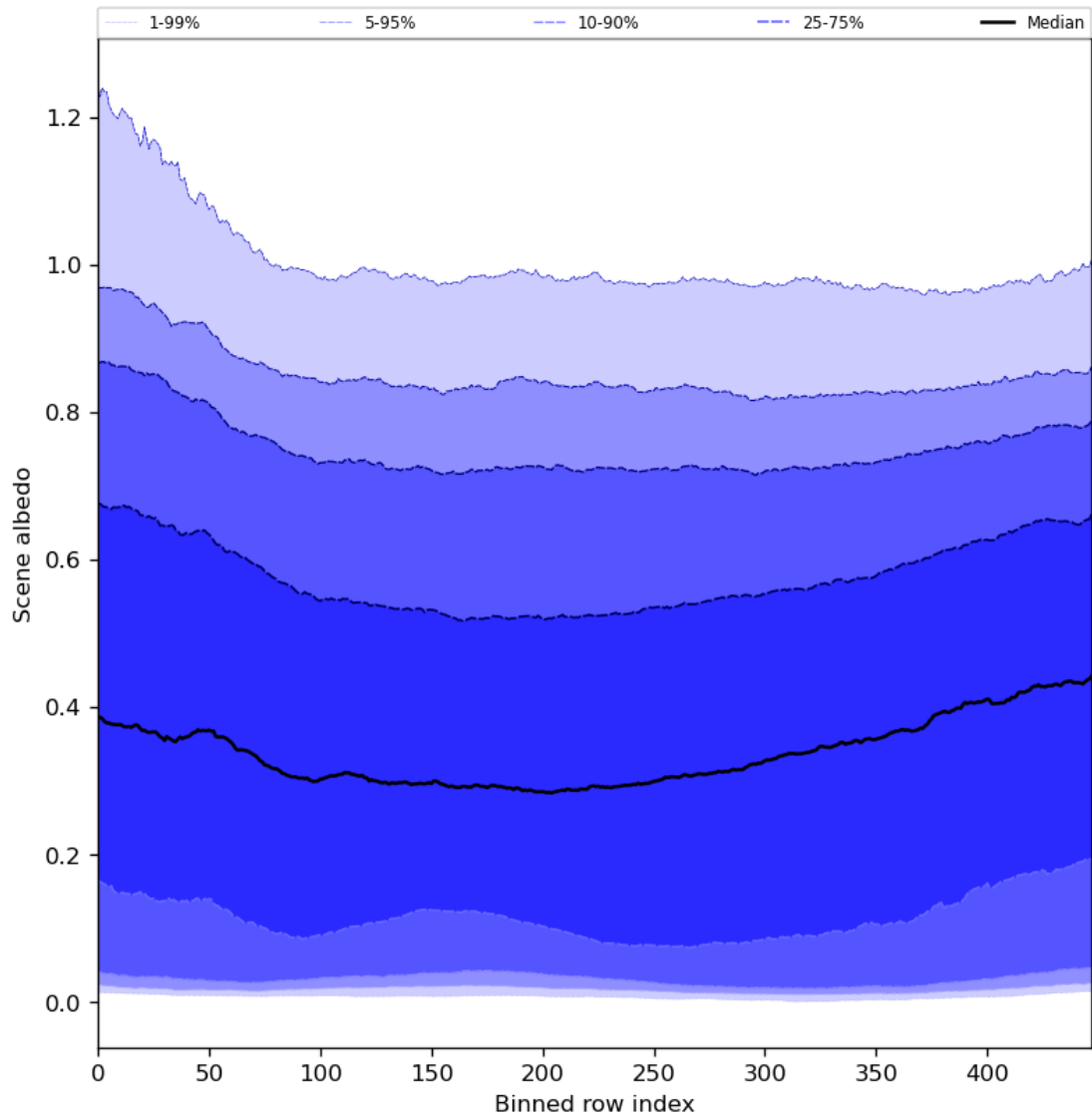
Figure 51: Along track statistics of “Scene albedo” for 2024-08-03 to 2024-08-05
