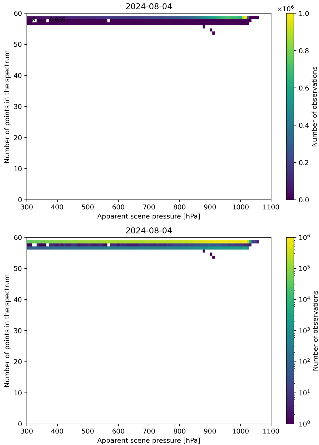
Figure 66: Scatter density plot of “Apparent scene pressure” against “Number of points in the spectrum” for 2024-08-03 to 2024-08-05.
