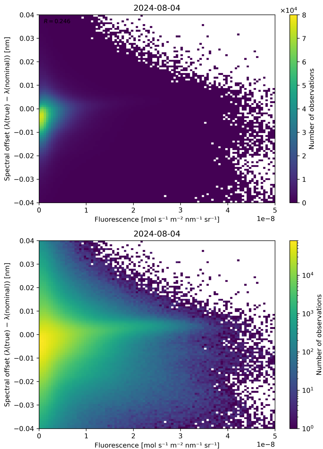
Figure 87: Scatter density plot of “Fluorescence” against “Spectral offset ( \lambda(\text{true}) - \lambda(\text{nominal}) )” for 2024-08-03 to 2024-08-05.
