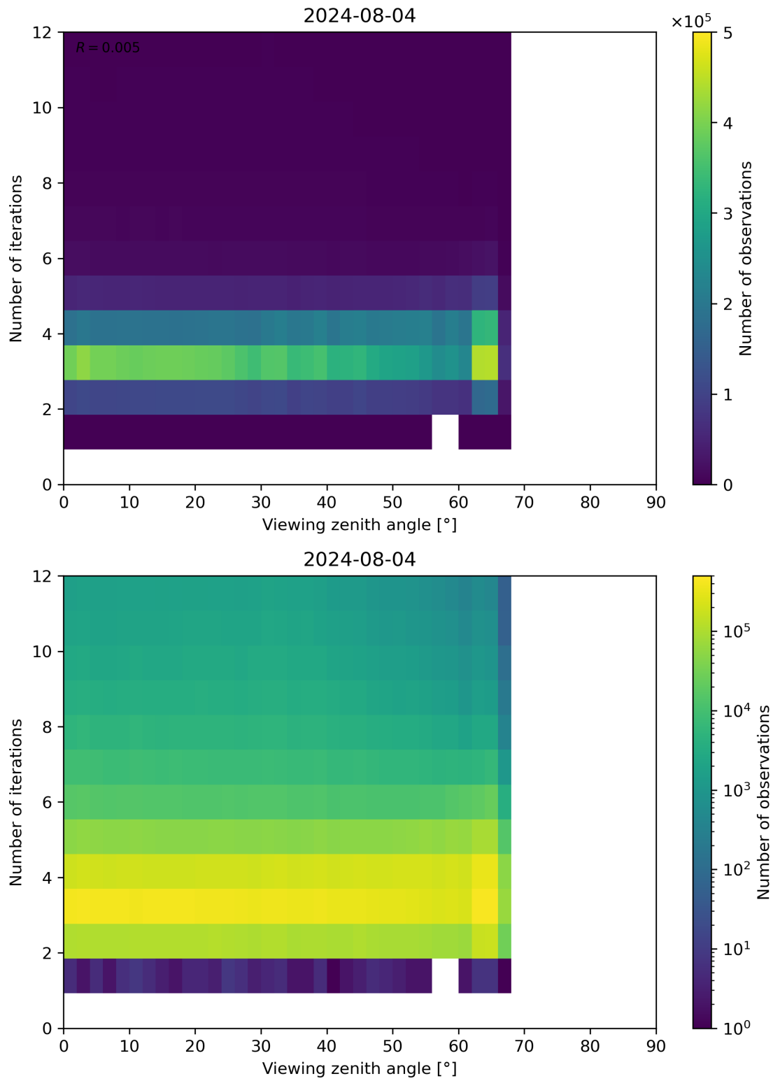
Figure 124: Scatter density plot of “Viewing zenith angle” against “Number of iterations” for 2024-08-03 to 2024-08-05.
