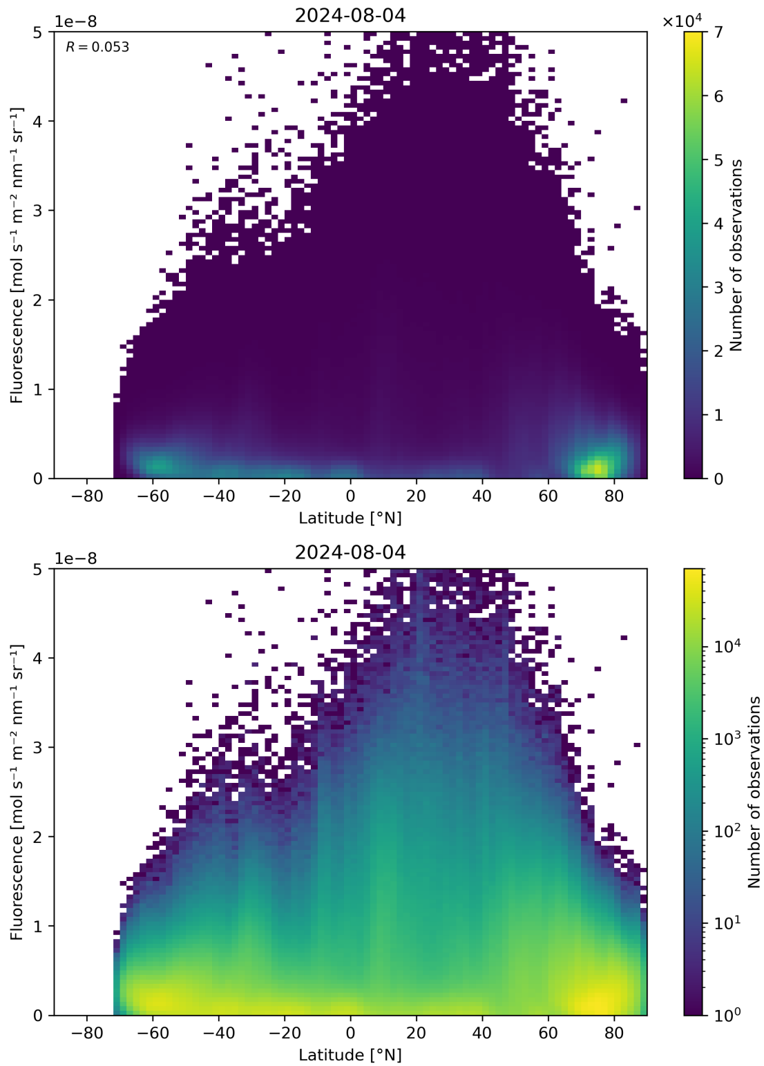
Figure 92: Scatter density plot of “Latitude” against “Fluorescence” for 2024-08-03 to 2024-08-05.
