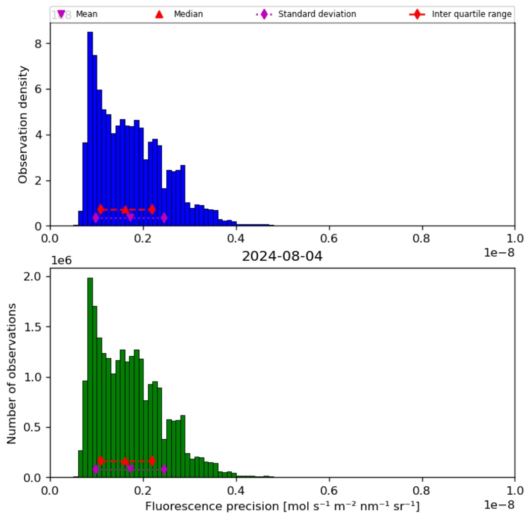
Figure 41: Histogram of “Fluorescence precision” for 2024-08-03 to 2024-08-05
