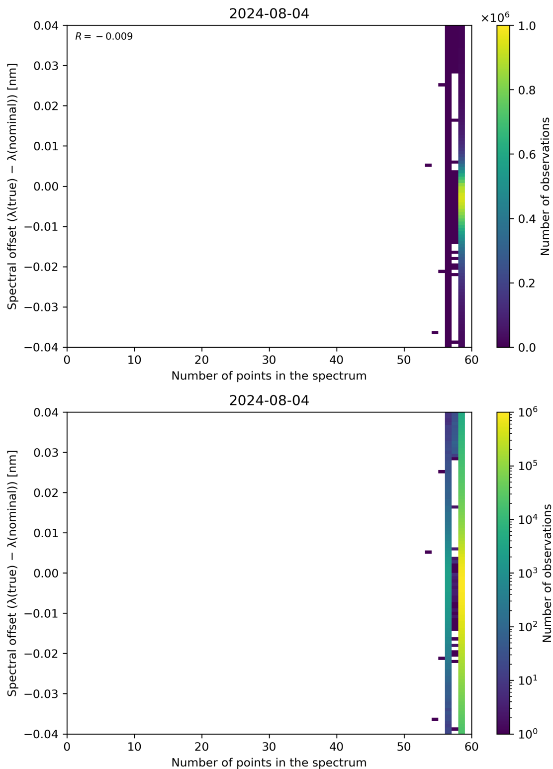
Figure 101: Scatter density plot of “Number of points in the spectrum” against “Spectral offset ( \lambda(\text{true}) - \lambda(\text{nominal}) )” for 2024-08-03 to 2024-08-05.
