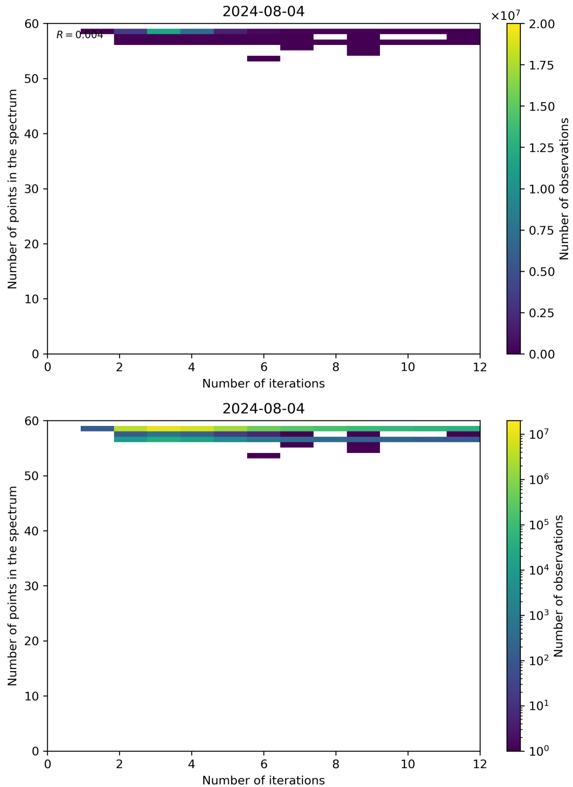
Figure 99: Scatter density plot of “Number of iterations” against “Number of points in the spectrum” for 2024-08-03 to 2024-08-05.
