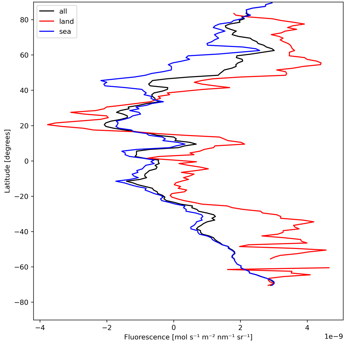
Figure 23: Zonal average of “Fluorescence” for 2024-08-03 to 2024-08-05.
