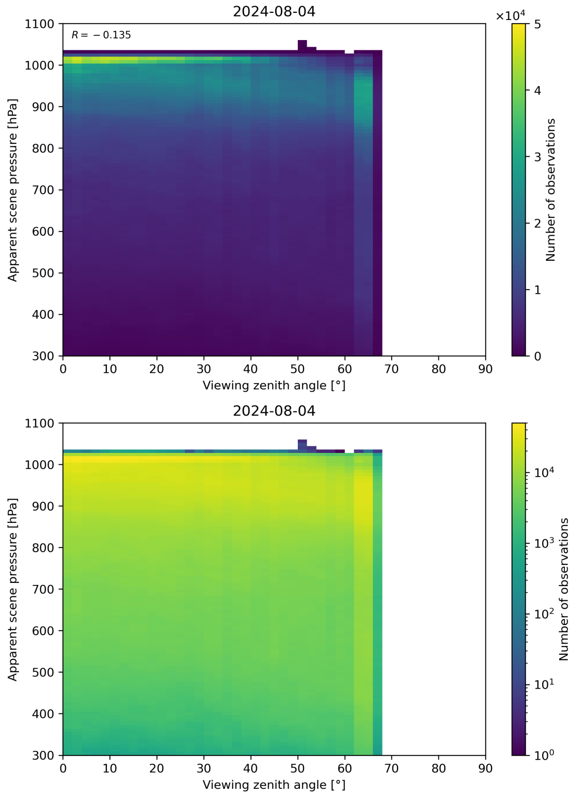
Figure 118: Scatter density plot of “Viewing zenith angle” against “Apparent scene pressure” for 2024-08-03 to 2024-08-05.
