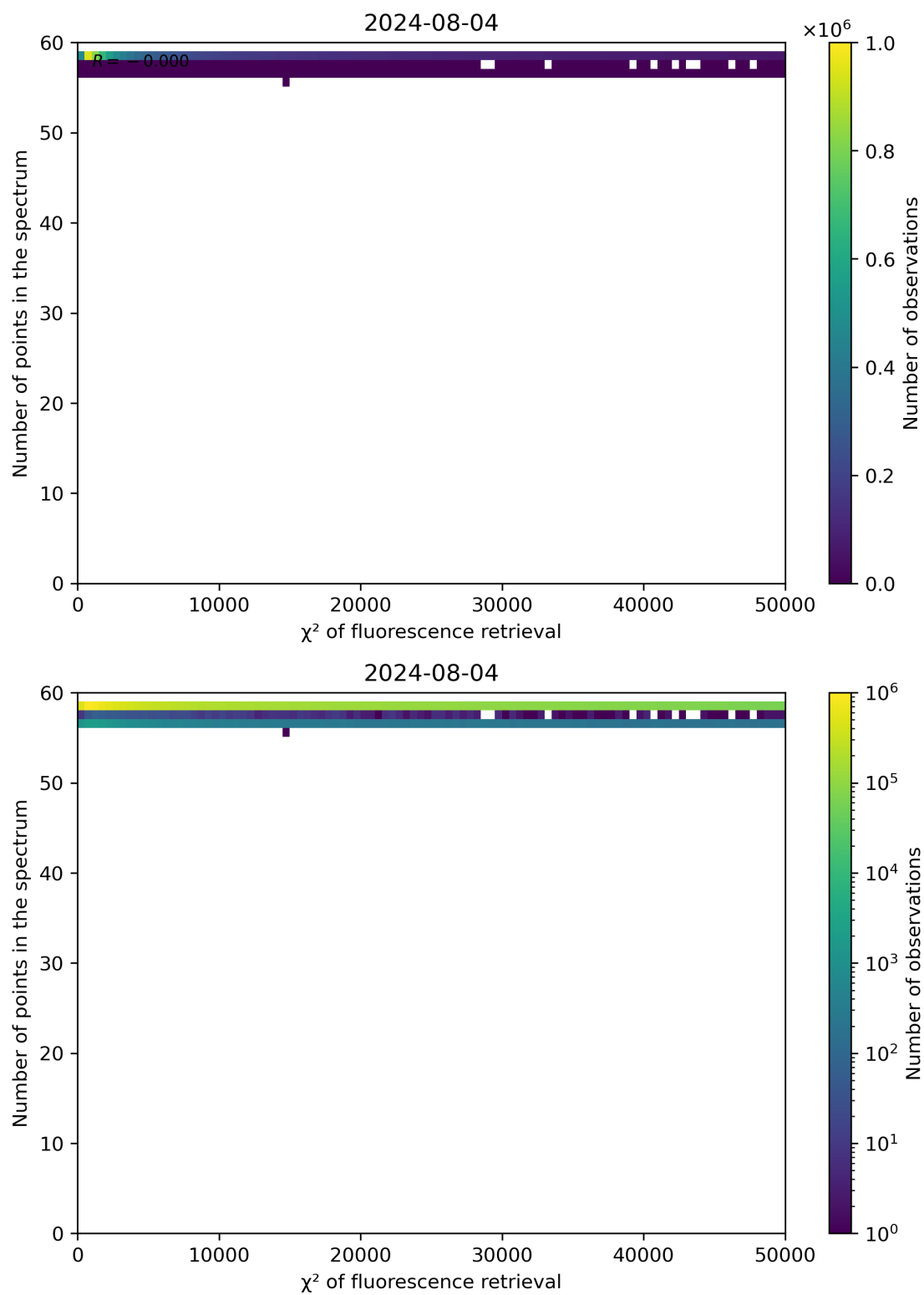
Figure 68: Scatter density plot of " \chi^2 of fluorescence retrieval" against "Number of points in the spectrum" for 2024-08-03 to 2024-08-05.
