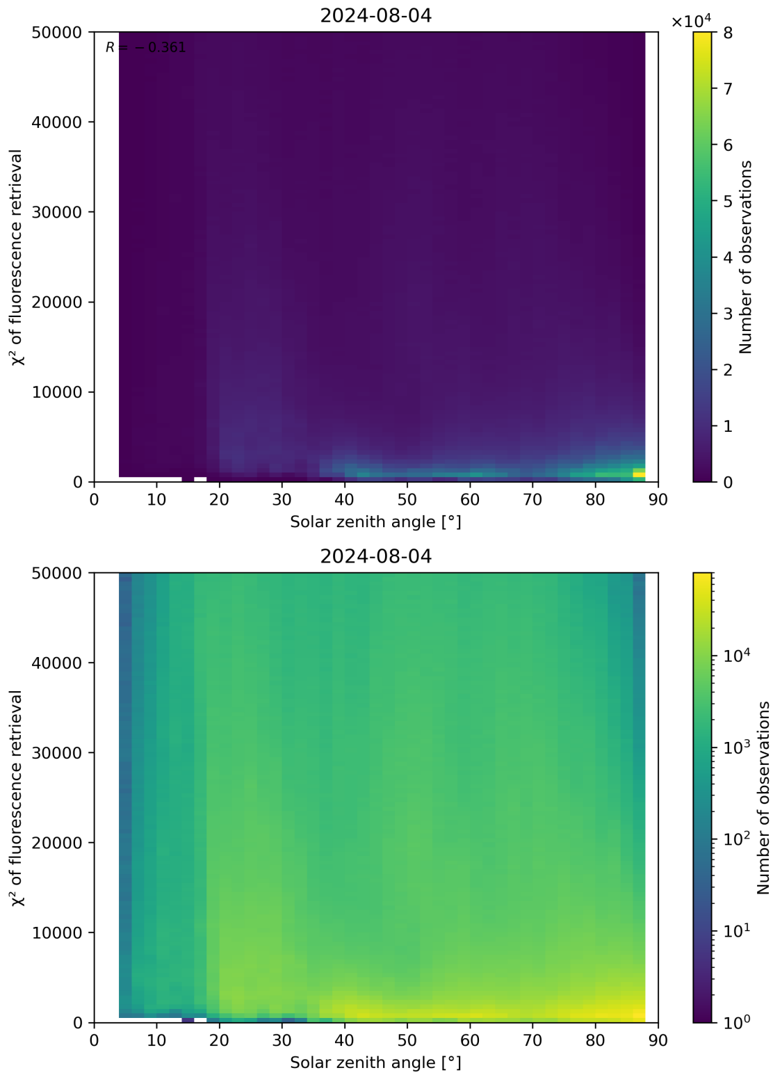
Figure 109: Scatter density plot of “Solar zenith angle” against “ \chi^2 of fluorescence retrieval” for 2024-08-03 to 2024-08-05.
