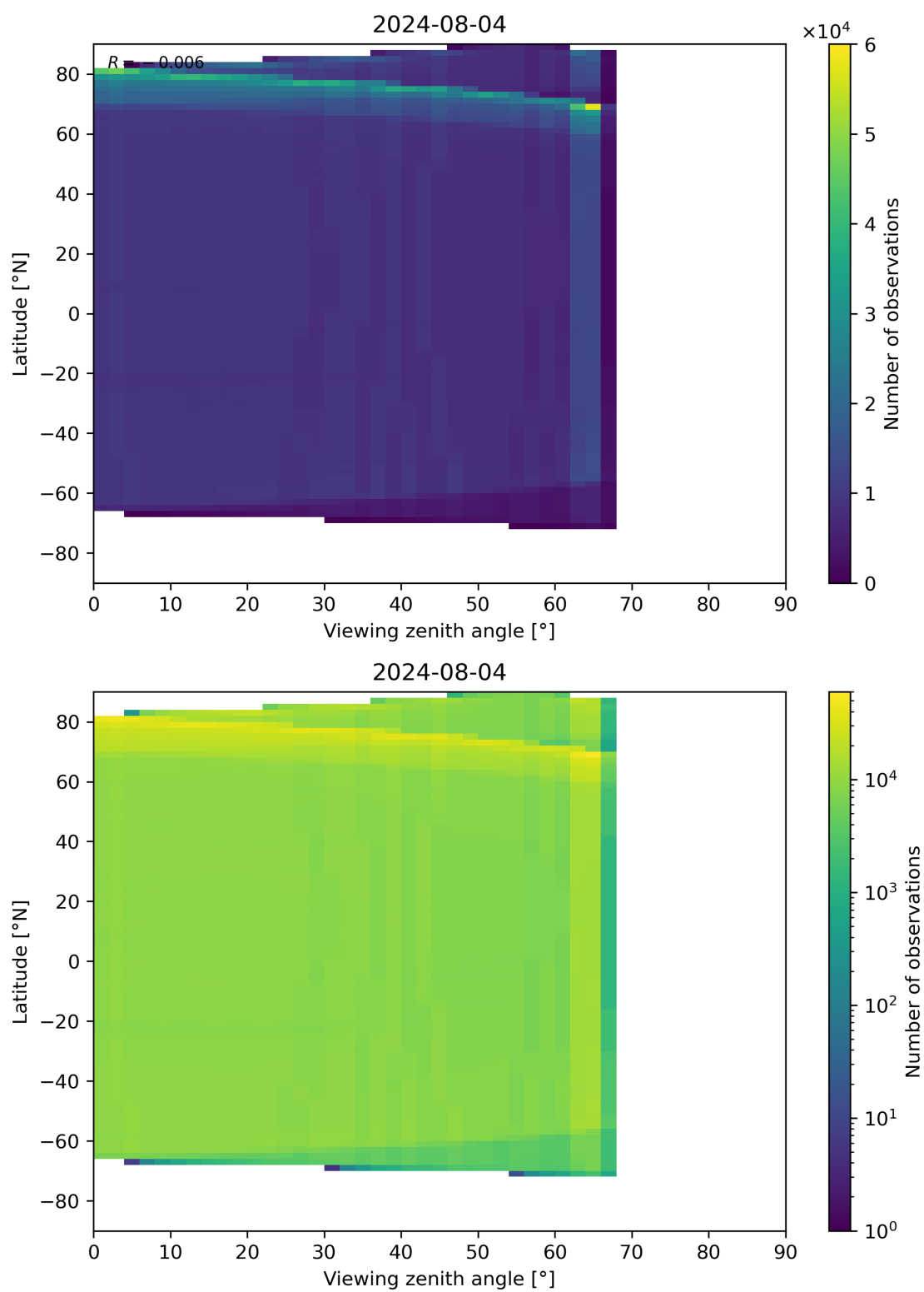
Figure 123: Scatter density plot of “Viewing zenith angle” against “Latitude” for 2024-08-03 to 2024-08-05.
