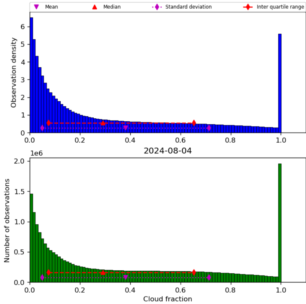
Figure 32: Histogram of “Cloud fraction” for 2024-08-03 to 2024-08-05
