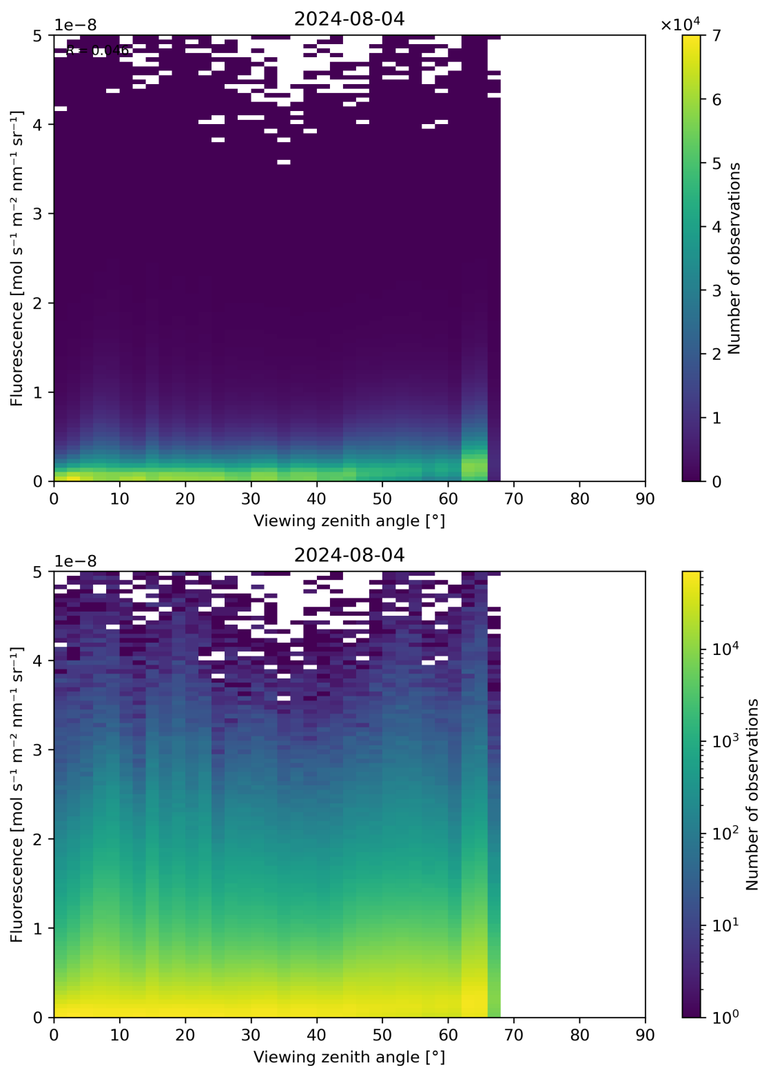
Figure 122: Scatter density plot of “Viewing zenith angle” against “Fluorescence” for 2024-08-03 to 2024-08-05.
