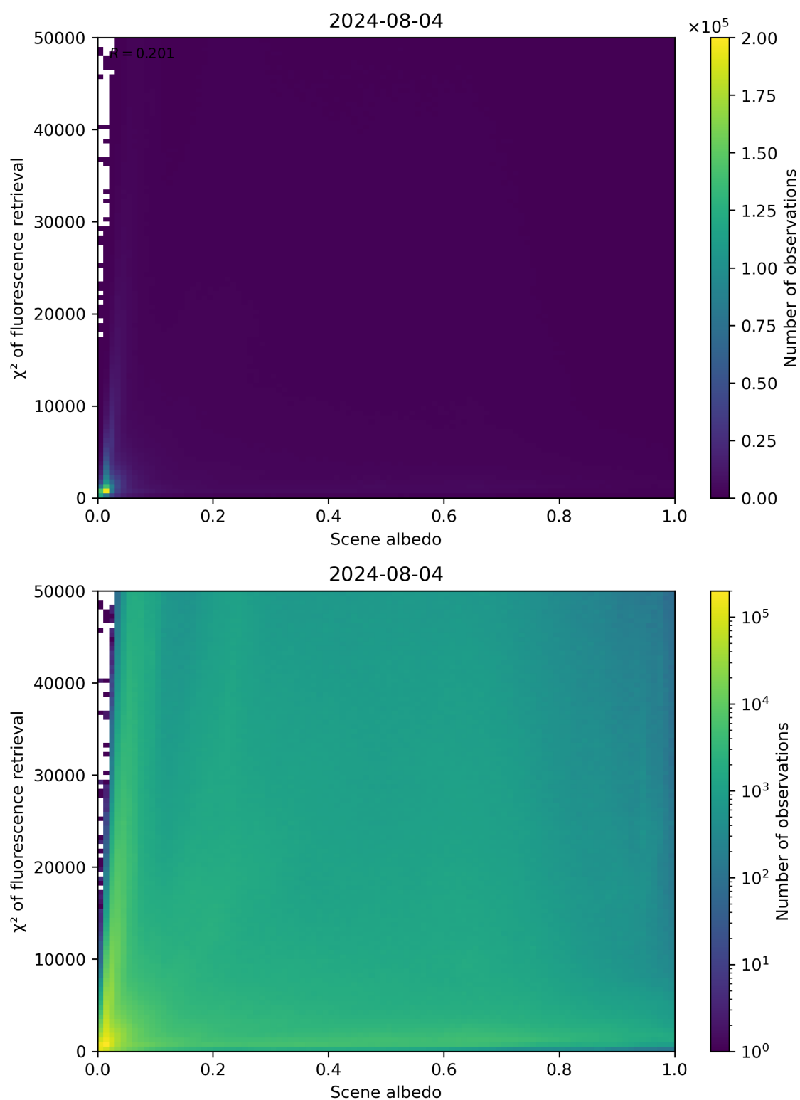
Figure 103: Scatter density plot of “Scene albedo” against “ \chi^2 of fluorescence retrieval” for 2024-08-03 to 2024-08-05.
