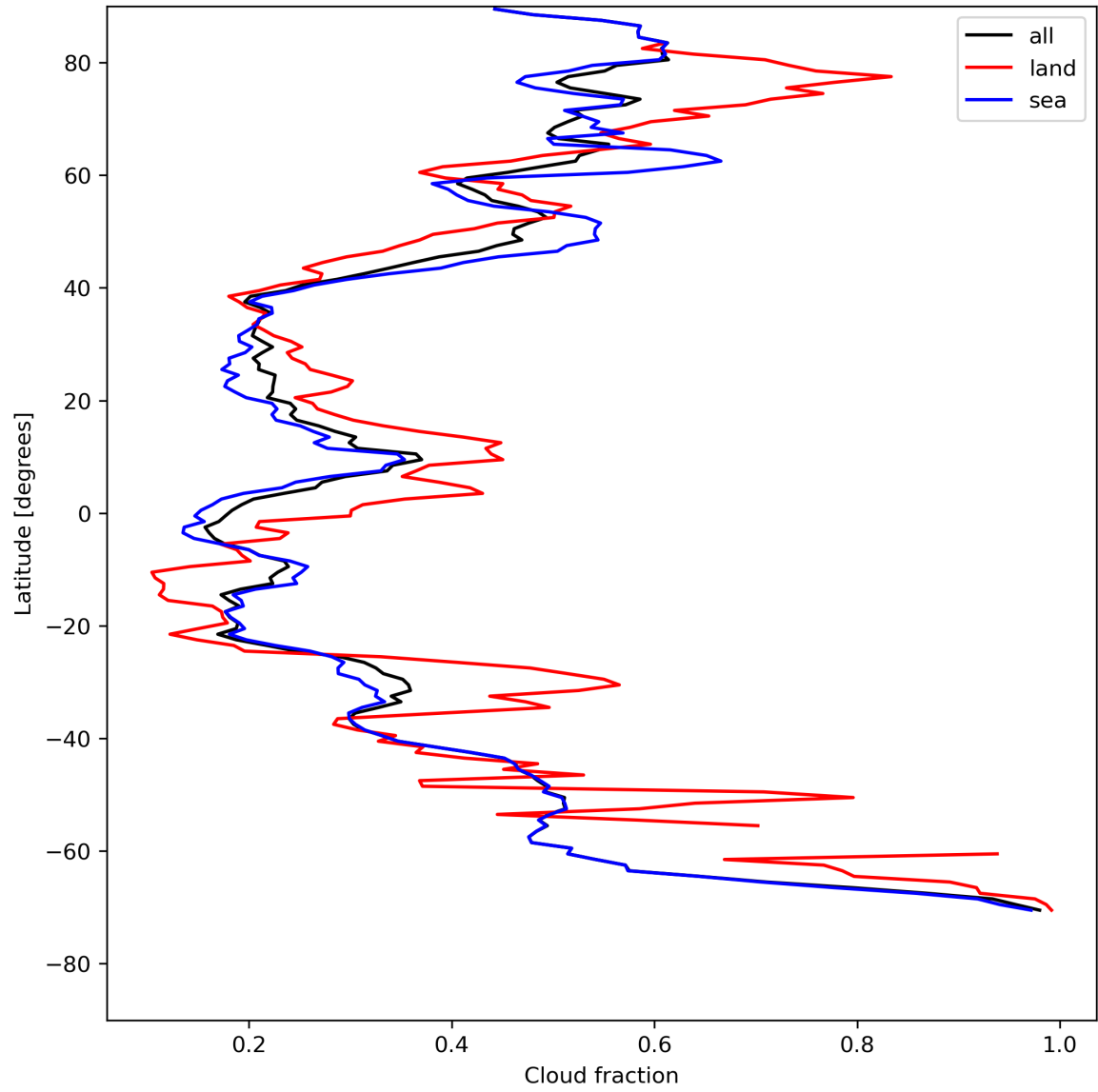
Figure 15: Zonal average of “Cloud fraction” for 2024-08-03 to 2024-08-05.
