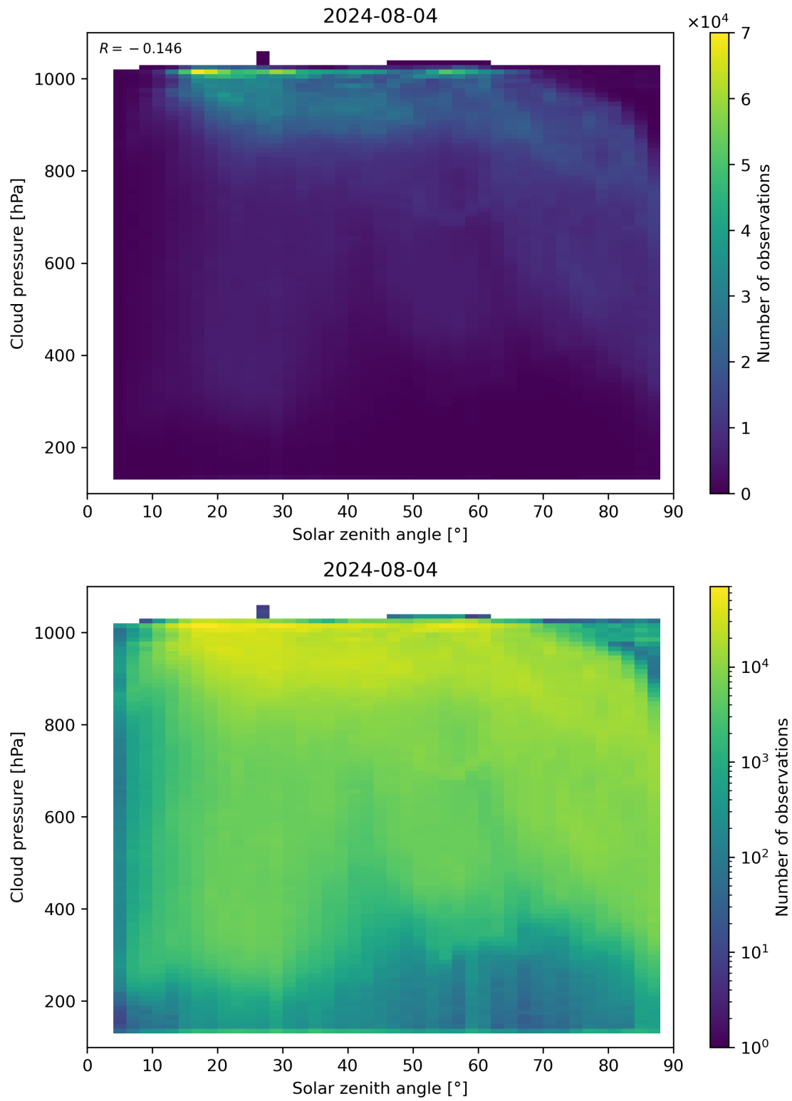
Figure 111: Scatter density plot of “Solar zenith angle” against “Cloud pressure” for 2024-08-03 to 2024-08-05.
