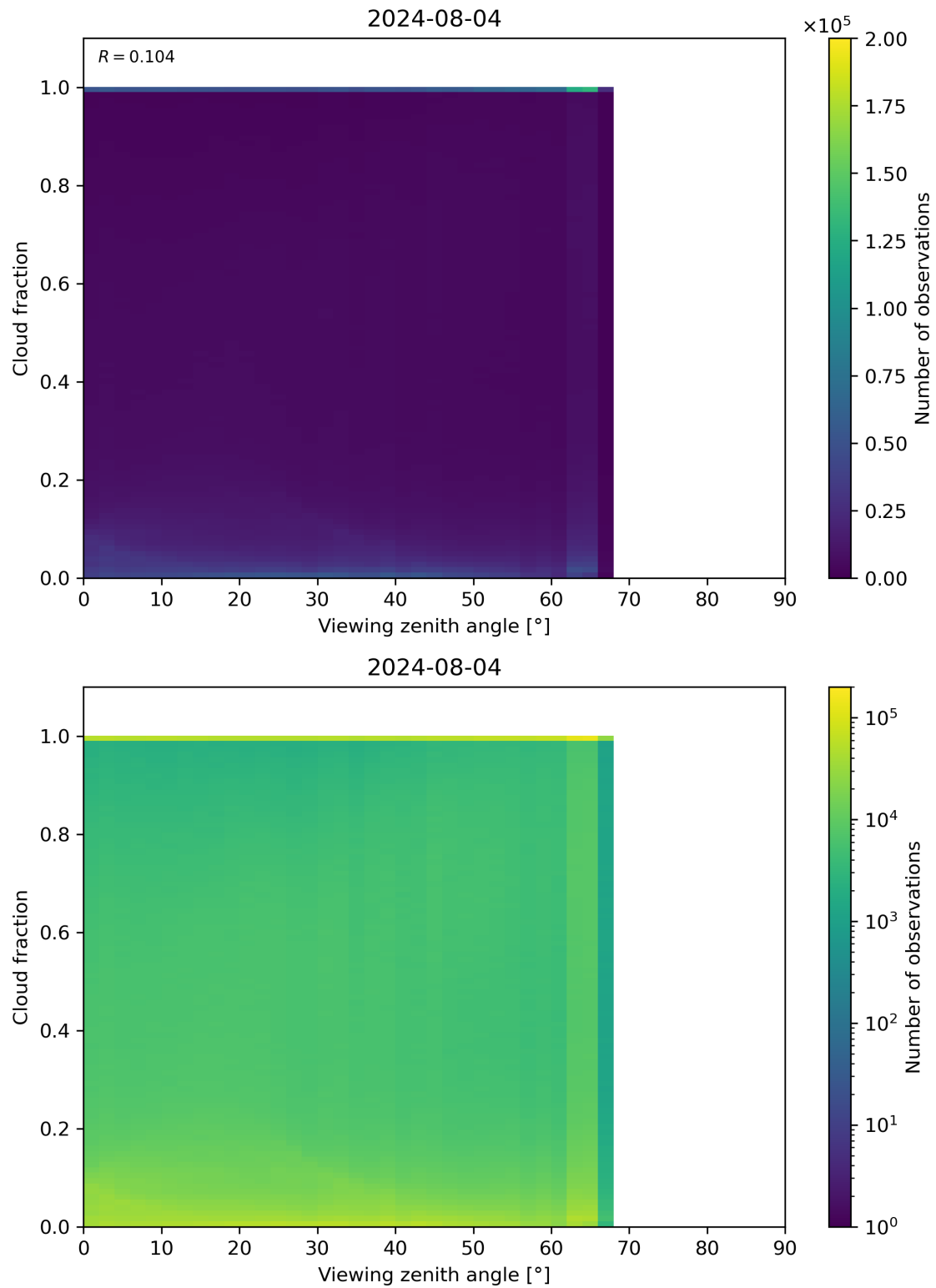
Figure 120: Scatter density plot of “Viewing zenith angle” against “Cloud fraction” for 2024-08-03 to 2024-08-05.
