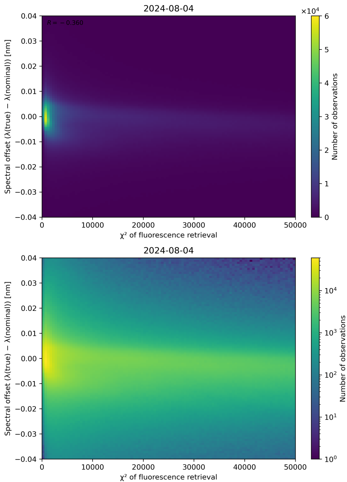
Figure 69: Scatter density plot of “ \chi^2 of fluorescence retrieval” against “Spectral offset ( \lambda(\text{true}) - \lambda(\text{nominal}) )” for 2024-08-03 to 2024-08-05.
