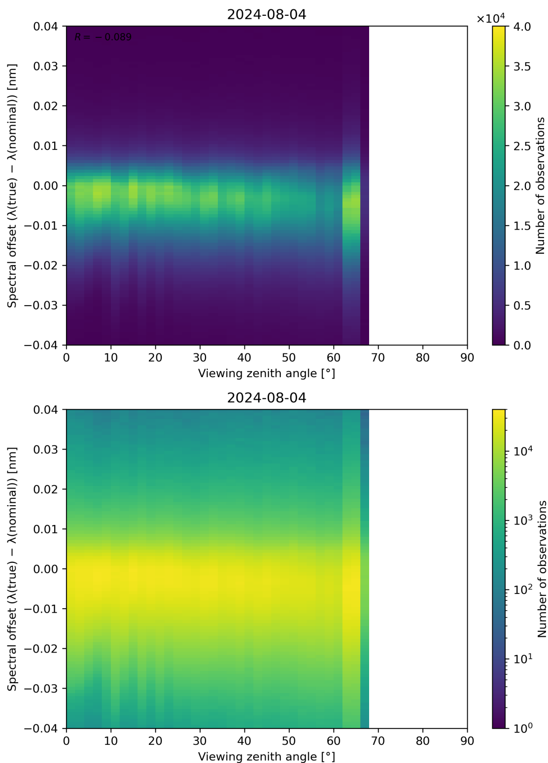
Figure 128: Scatter density plot of “Viewing zenith angle” against “Spectral offset ( \lambda(\text{true}) - \lambda(\text{nominal}) )” for 2024-08-03 to 2024-08-05.
