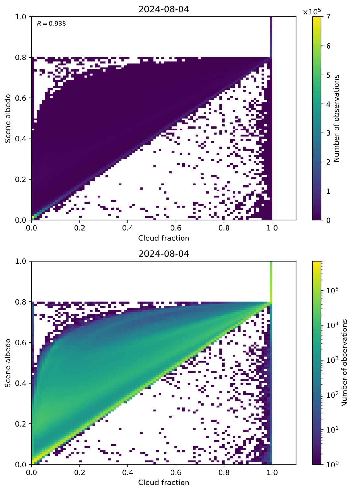
Figure 75: Scatter density plot of “Cloud fraction” against “Scene albedo” for 2024-08-03 to 2024-08-05.
