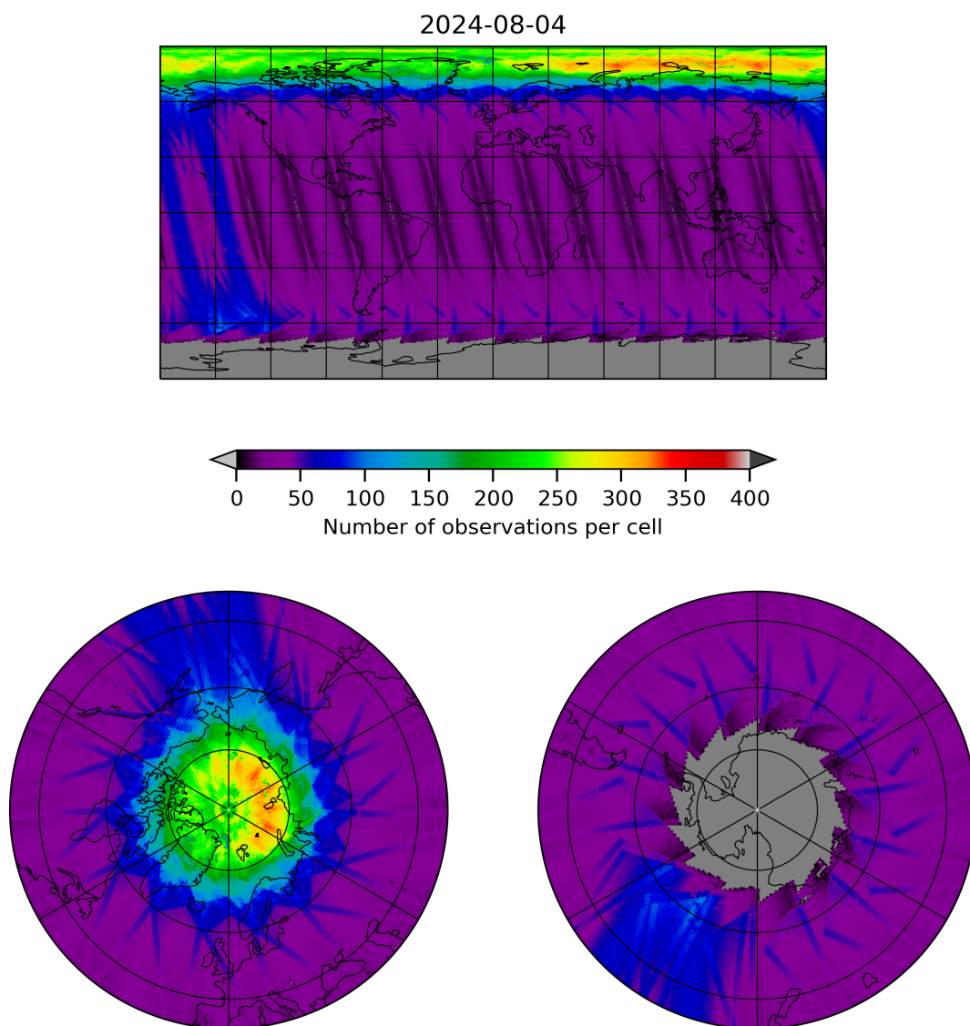
Figure 11: Map of the number of observations for 2024-08-03 to 2024-08-05
