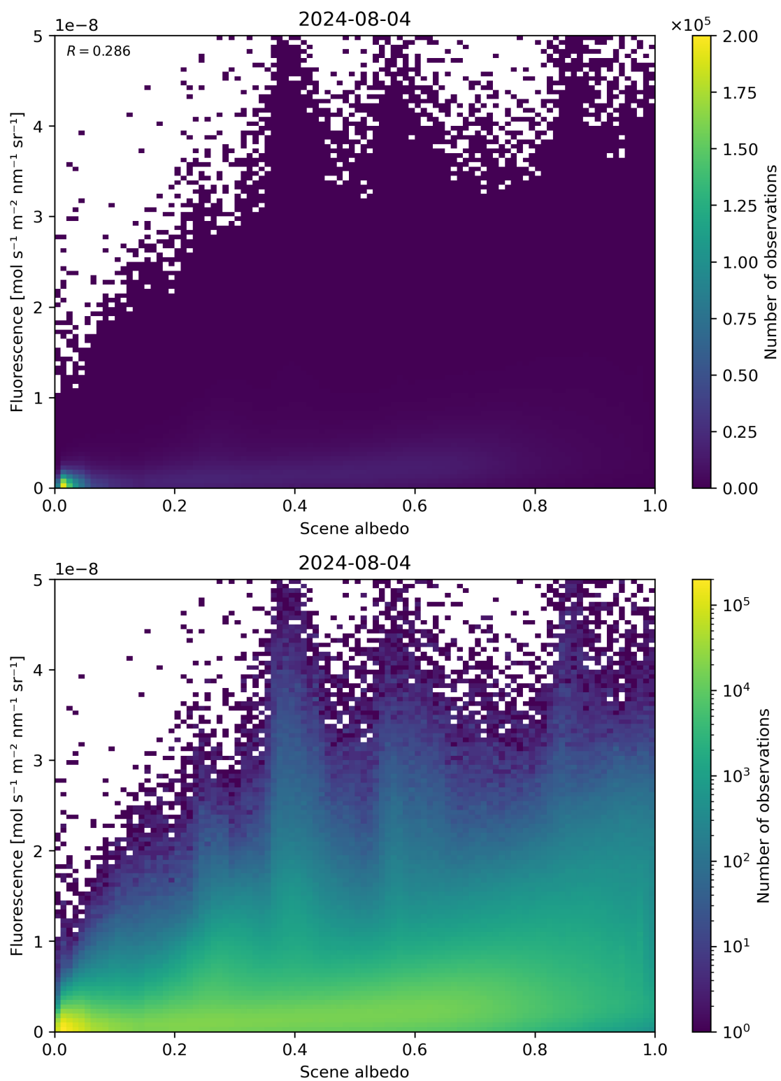
Figure 104: Scatter density plot of “Scene albedo” against “Fluorescence” for 2024-08-03 to 2024-08-05.
