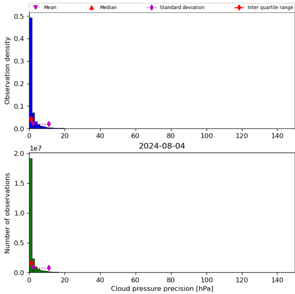
Figure 31: Histogram of “Cloud pressure precision” for 2024-08-03 to 2024-08-05
