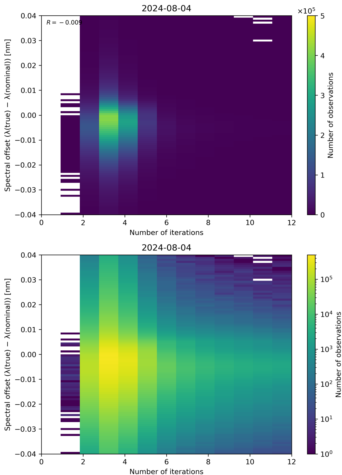
Figure 100: Scatter density plot of “Number of iterations” against “Spectral offset ( \lambda(\text{true}) - \lambda(\text{nominal}) )” for 2024-08-03 to 2024-08-05.
