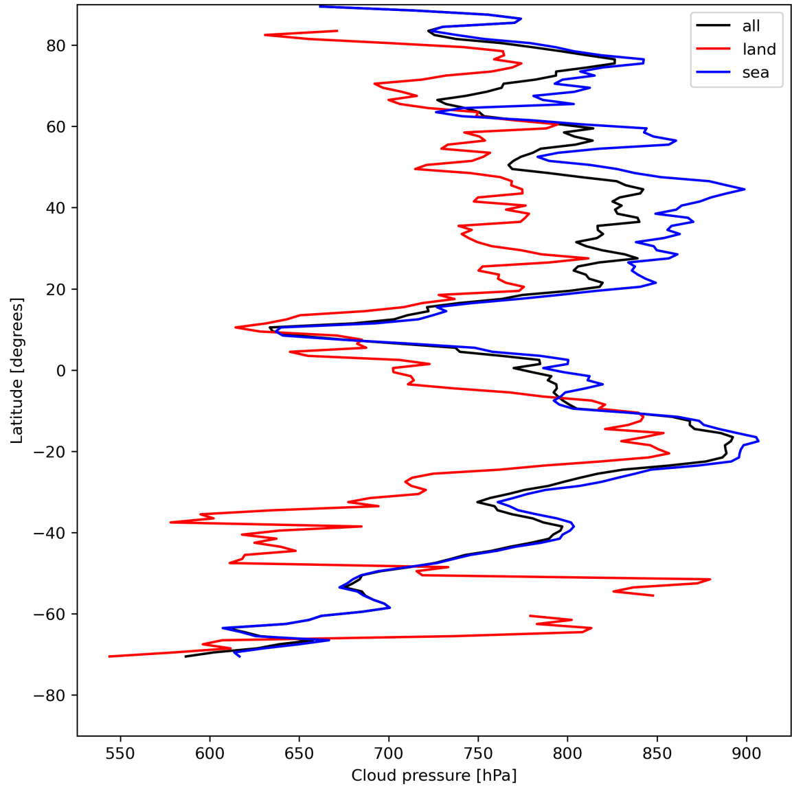
Figure 13: Zonal average of “Cloud pressure” for 2024-08-03 to 2024-08-05.
