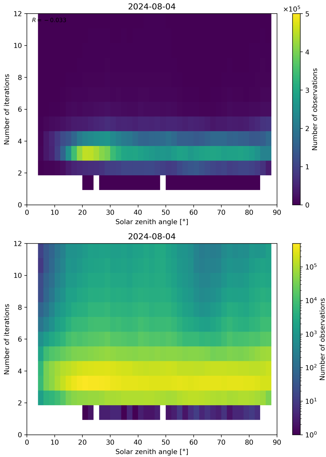
Figure 114: Scatter density plot of “Solar zenith angle” against “Number of iterations” for 2024-08-03 to 2024-08-05.
