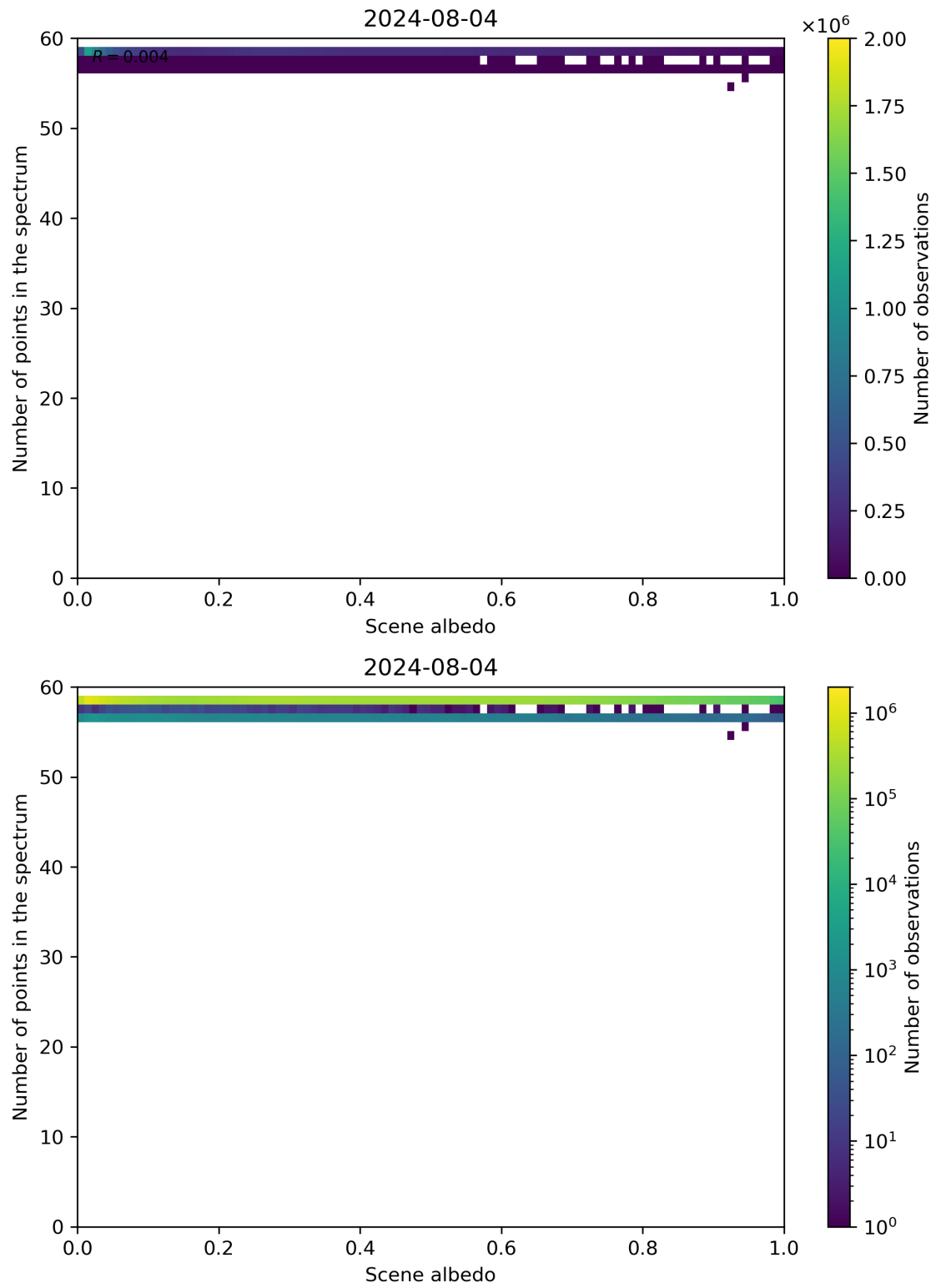
Figure 106: Scatter density plot of “Scene albedo” against “Number of points in the spectrum” for 2024-08-03 to 2024-08-05.
