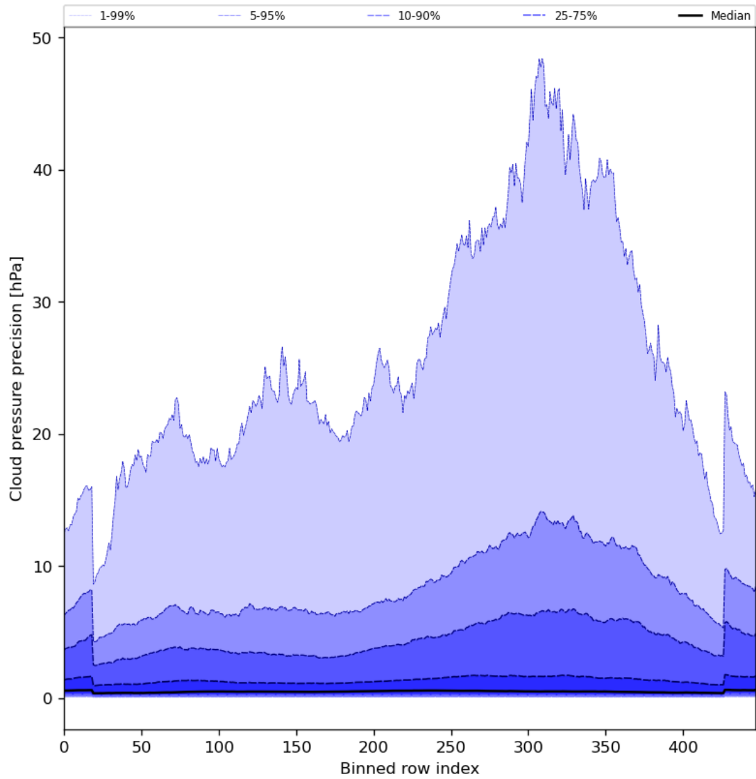
Figure 48: Along track statistics of “Cloud pressure precision” for 2024-08-03 to 2024-08-05
