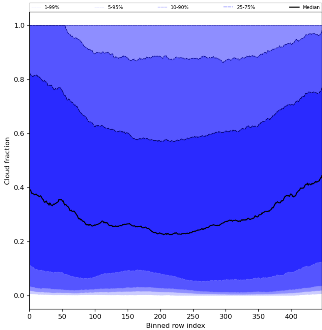
Figure 49: Along track statistics of “Cloud fraction” for 2024-08-03 to 2024-08-05
