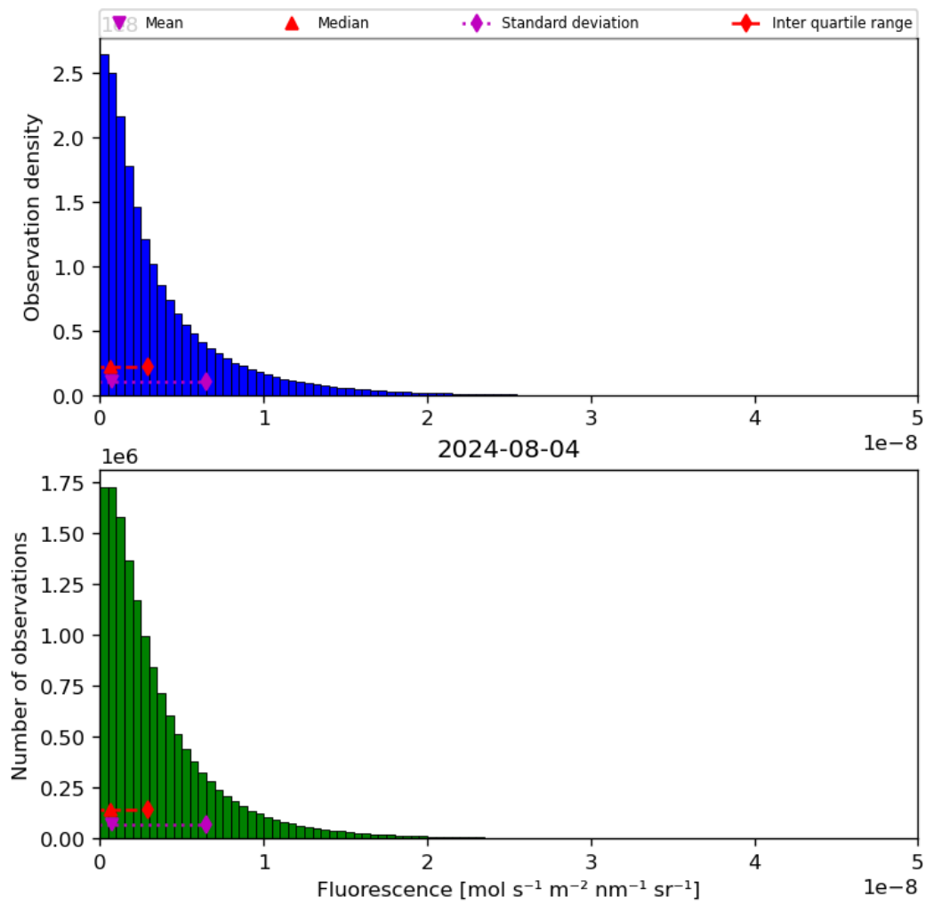
Figure 40: Histogram of “Fluorescence” for 2024-08-03 to 2024-08-05
