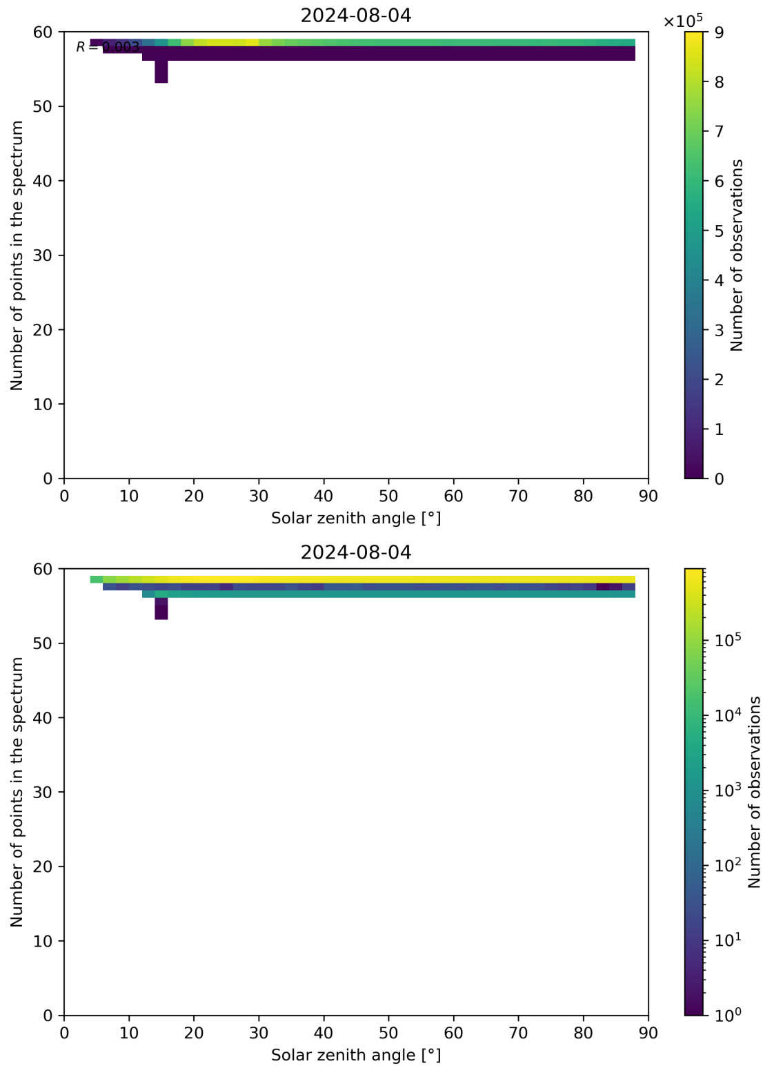
Figure 115: Scatter density plot of “Solar zenith angle” against “Number of points in the spectrum” for 2024-08-03 to 2024-08-05.
