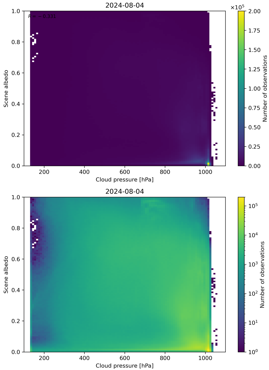
Figure 83: Scatter density plot of “Cloud pressure” against “Scene albedo” for 2024-08-03 to 2024-08-05.
