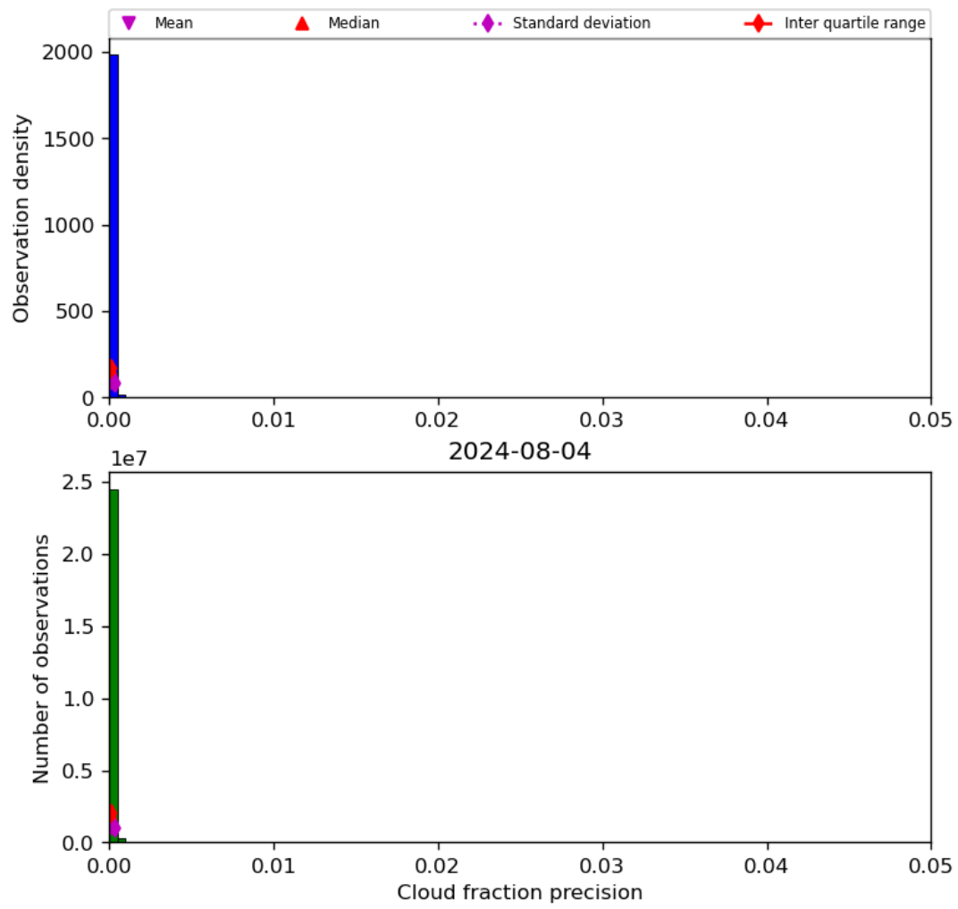
Figure 33: Histogram of “Cloud fraction precision” for 2024-08-03 to 2024-08-05
