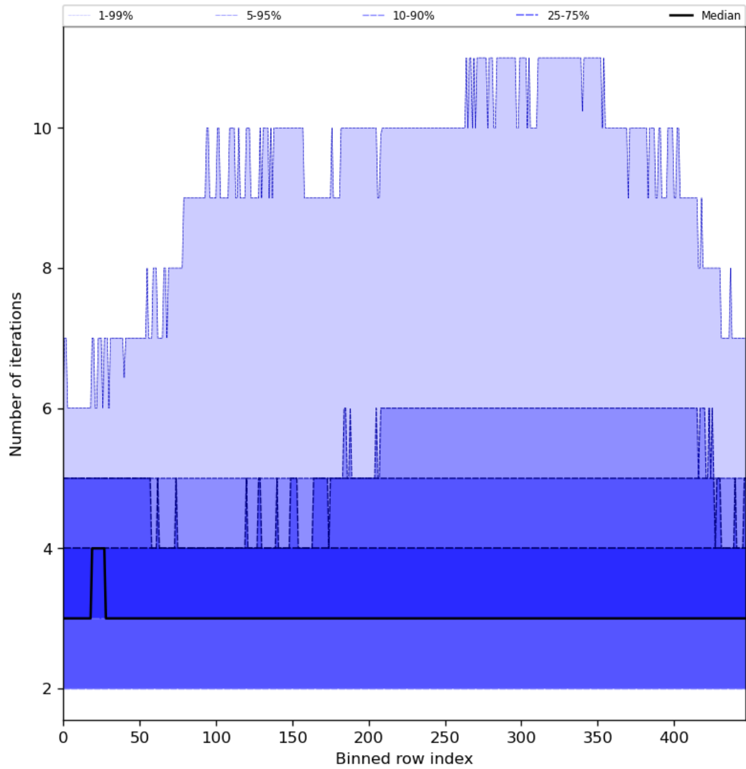
Figure 56: Along track statistics of “Number of iterations” for 2024-08-03 to 2024-08-05
