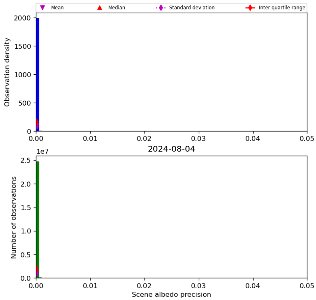
Figure 35: Histogram of “Scene albedo precision” for 2024-08-03 to 2024-08-05
