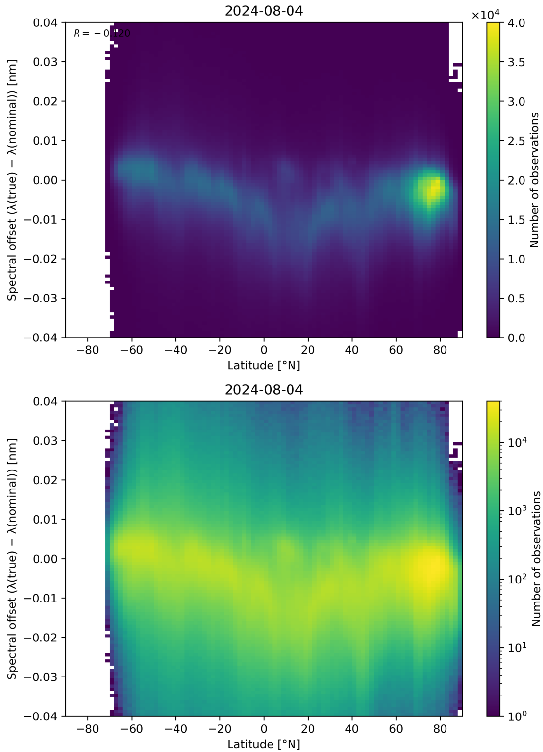
Figure 96: Scatter density plot of “Latitude” against “Spectral offset ( \lambda(\text{true}) - \lambda(\text{nominal}) )” for 2024-08-03 to 2024-08-05.
