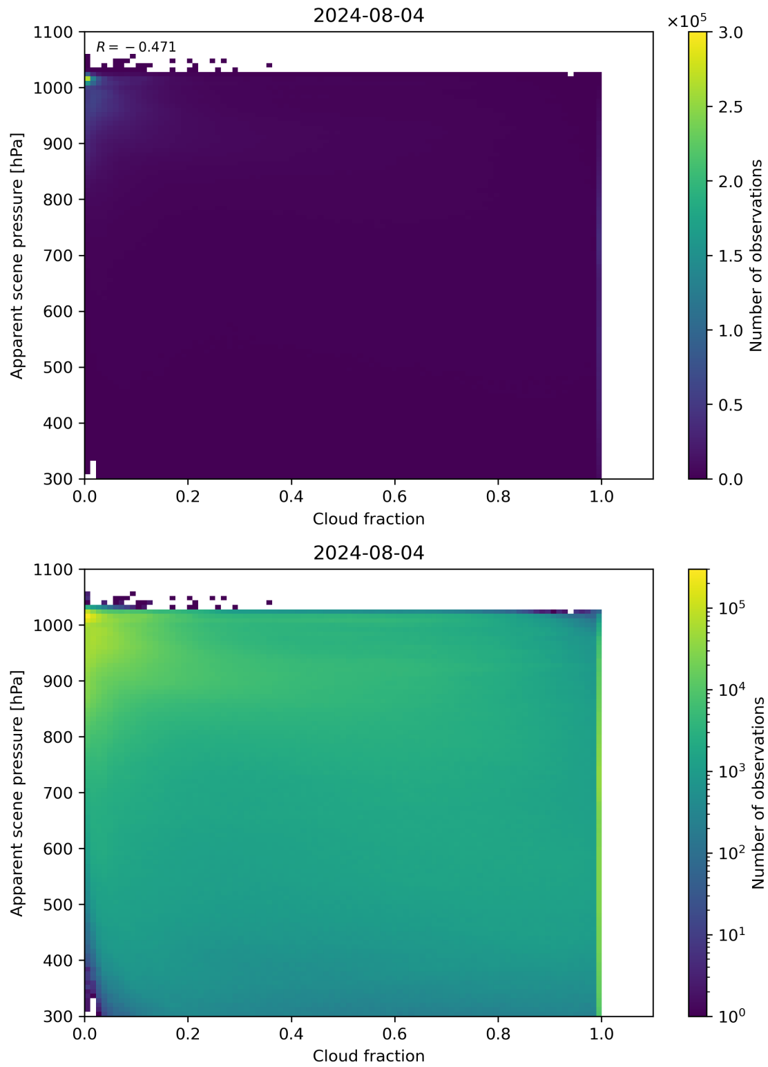
Figure 70: Scatter density plot of “Cloud fraction” against “Apparent scene pressure” for 2024-08-03 to 2024-08-05.
