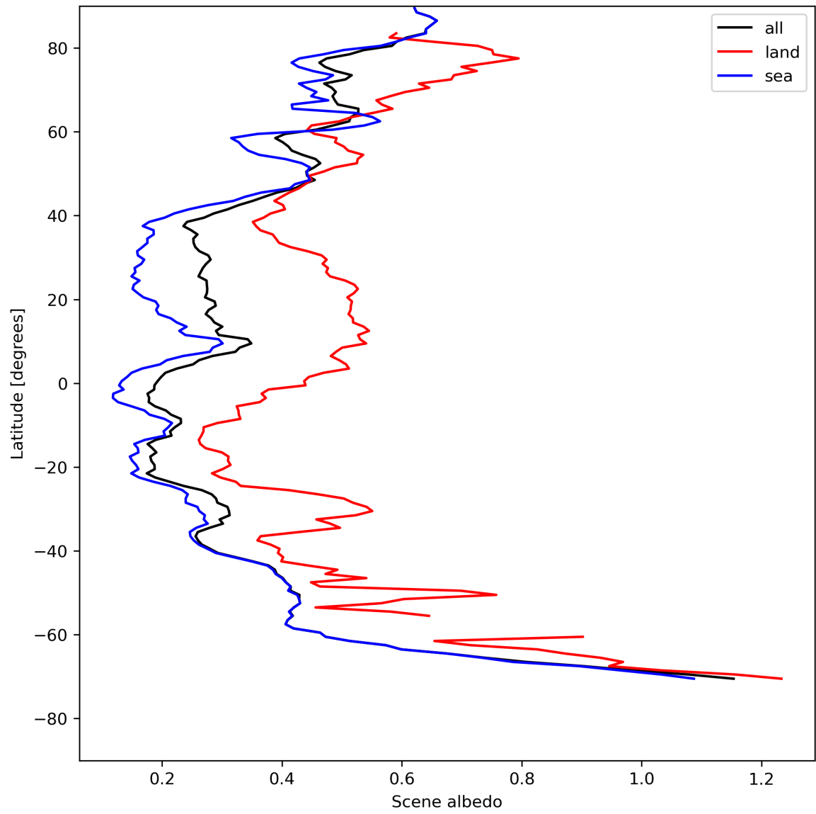
Figure 17: Zonal average of “Scene albedo” for 2024-08-03 to 2024-08-05.
