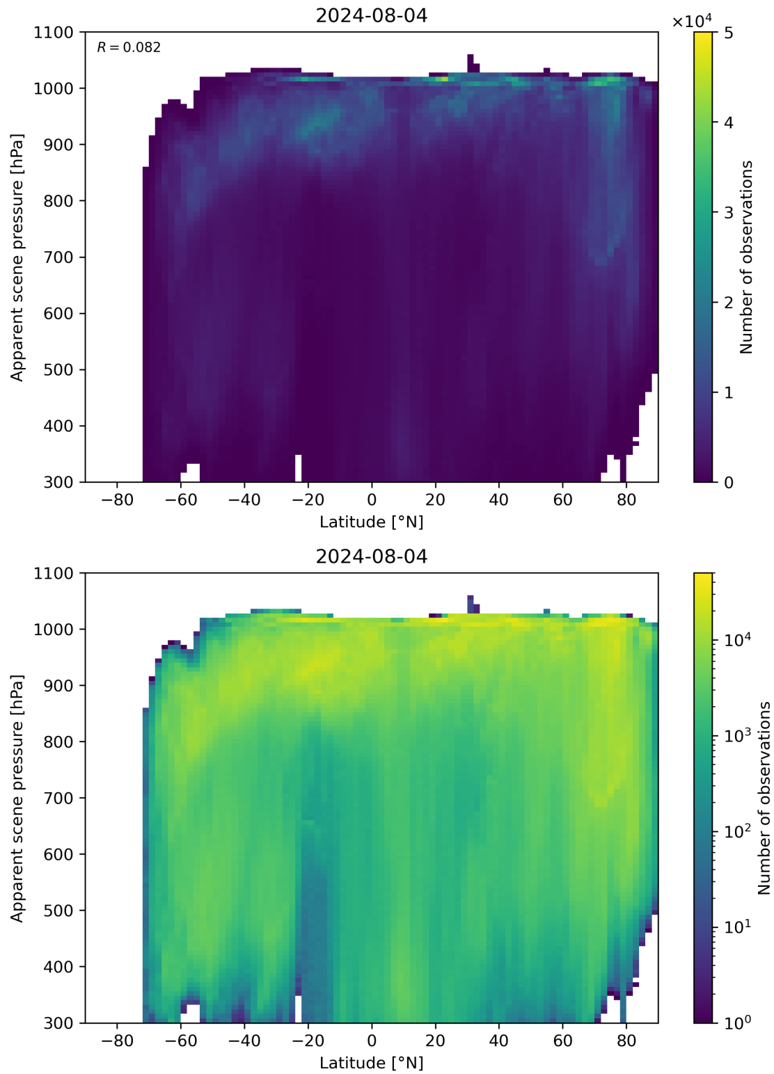
Figure 88: Scatter density plot of “Latitude” against “Apparent scene pressure” for 2024-08-03 to 2024-08-05.
