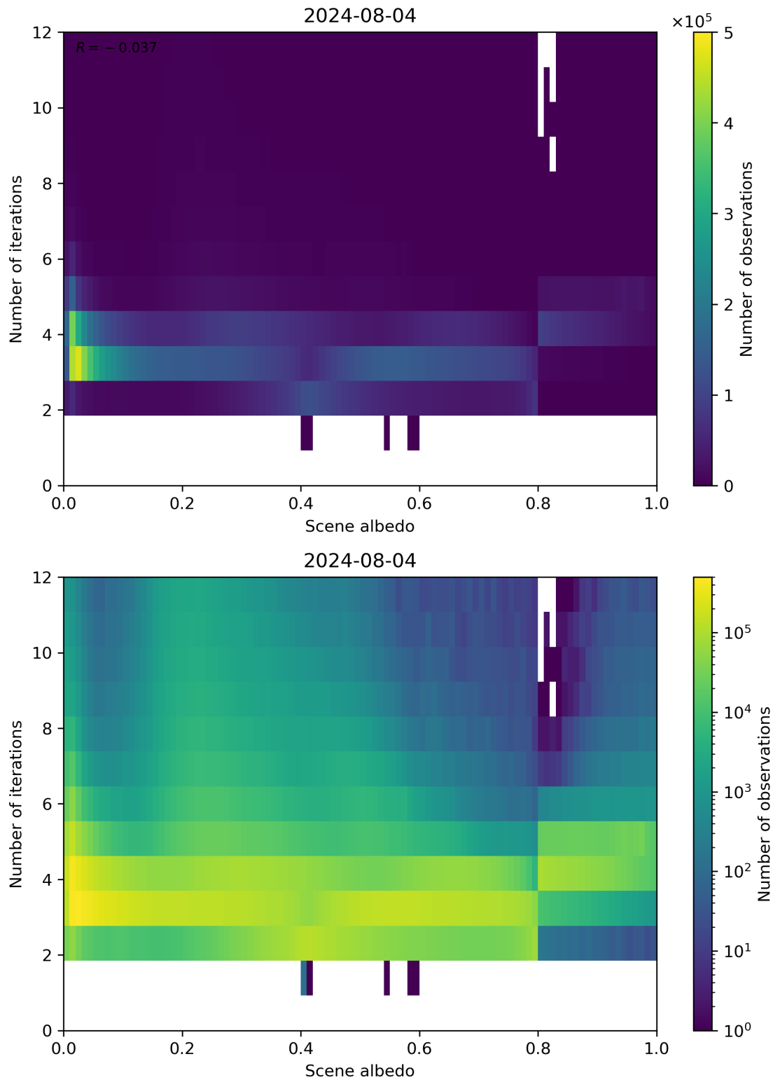
Figure 105: Scatter density plot of “Scene albedo” against “Number of iterations” for 2024-08-03 to 2024-08-05.
