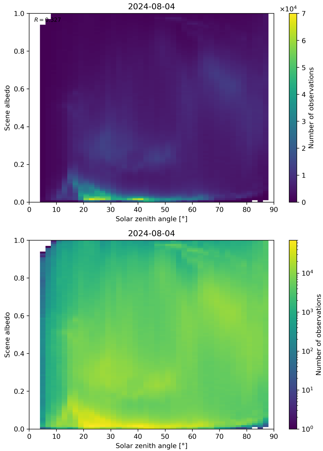
Figure 116: Scatter density plot of “Solar zenith angle” against “Scene albedo” for 2024-08-03 to 2024-08-05.
