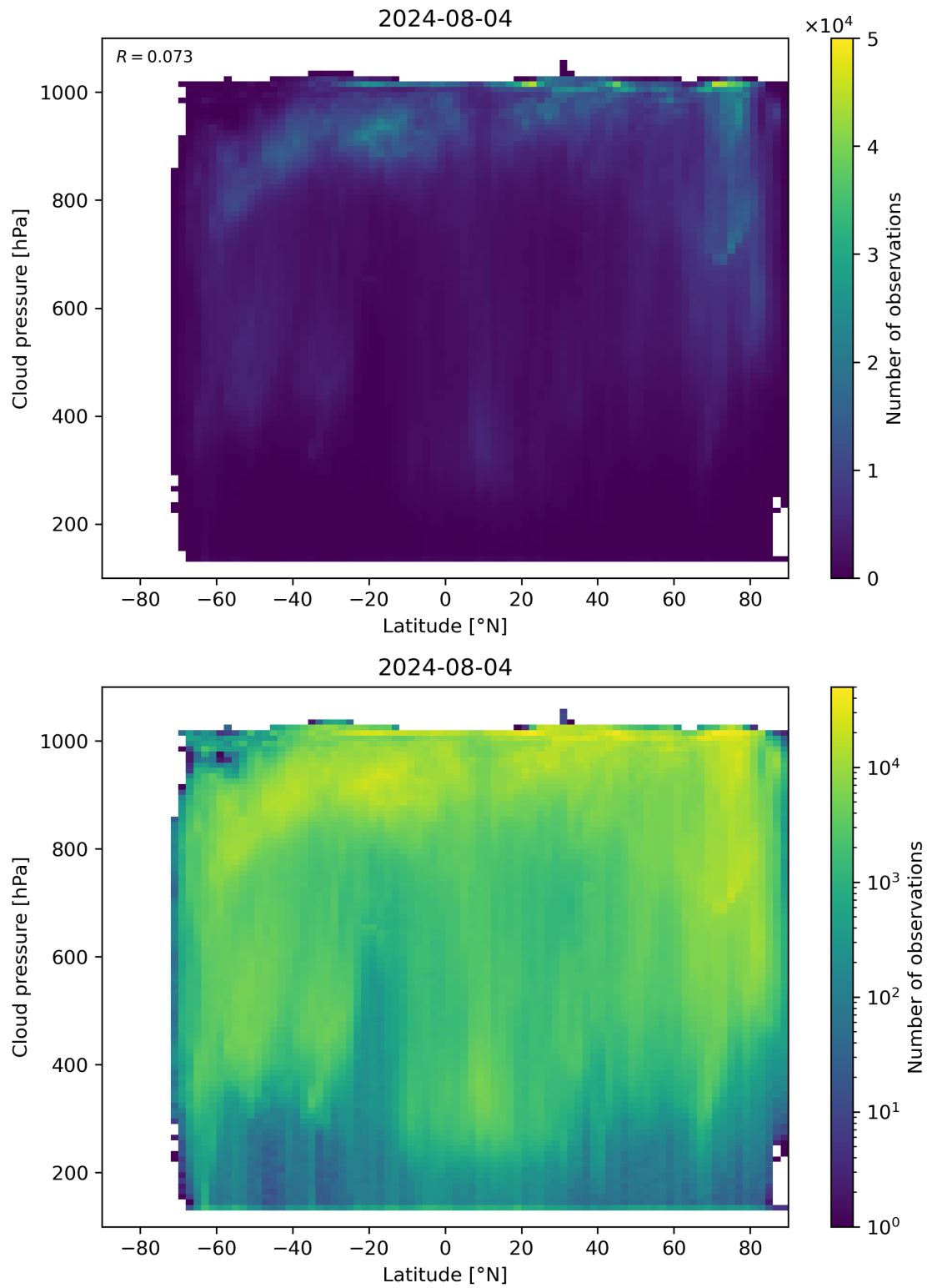
Figure 91: Scatter density plot of “Latitude” against “Cloud pressure” for 2024-08-03 to 2024-08-05.
