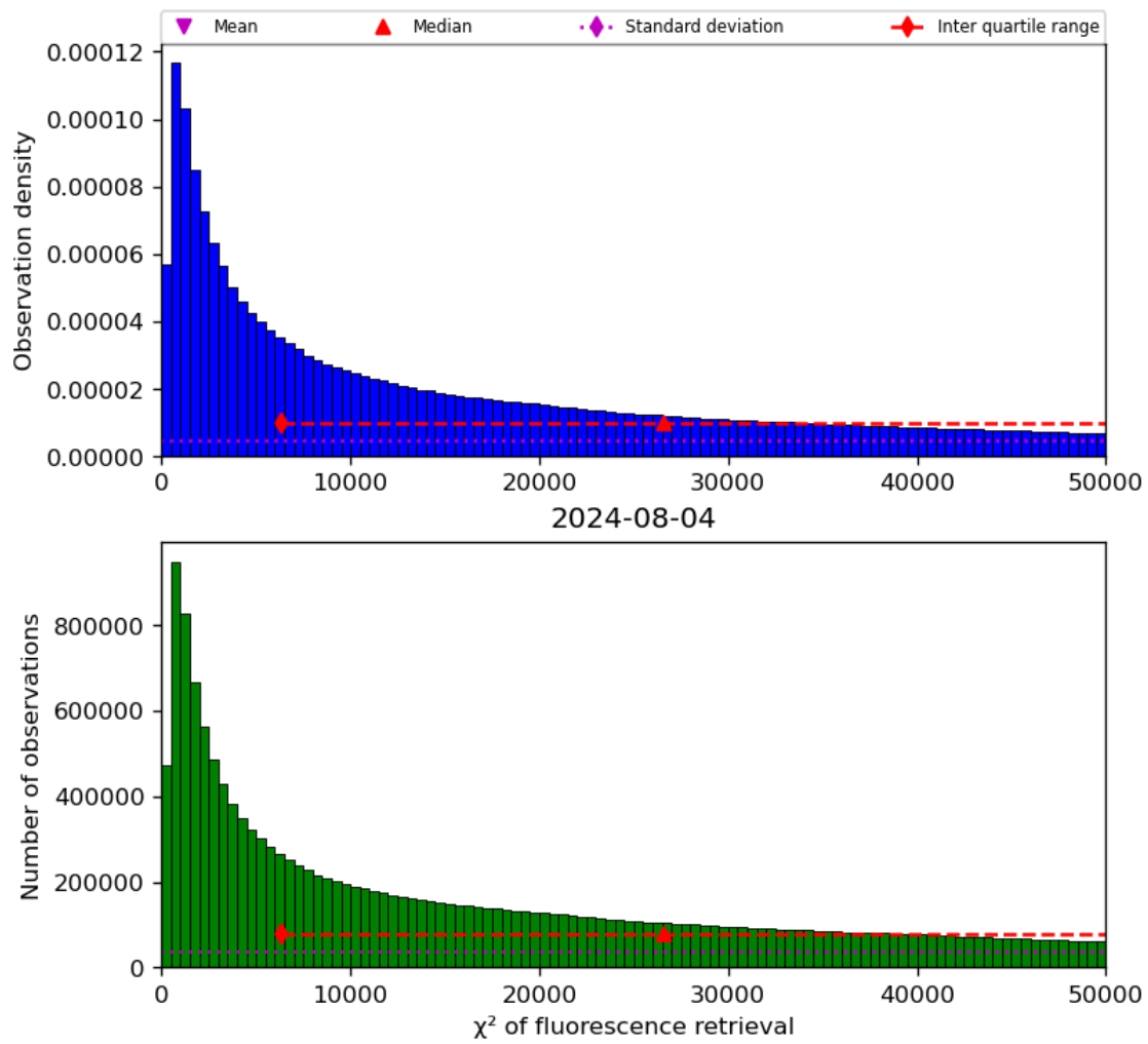
Figure 42: Histogram of “ \chi^2 of fluorescence retrieval” for 2024-08-03 to 2024-08-05
