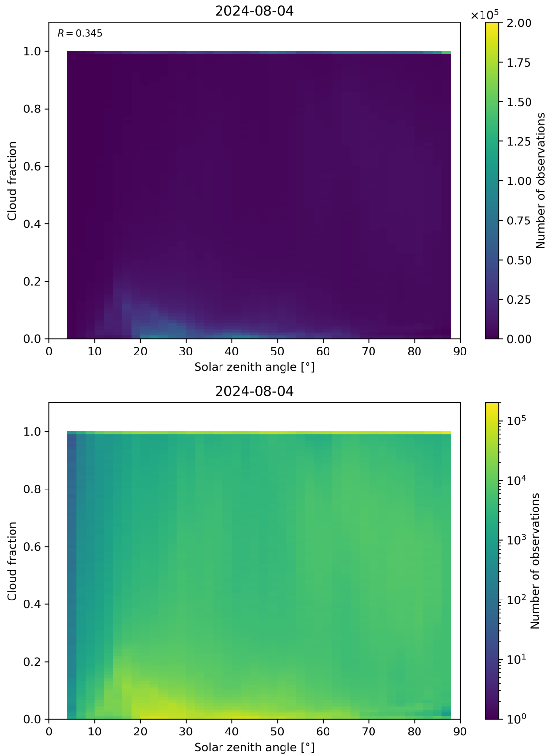
Figure 110: Scatter density plot of “Solar zenith angle” against “Cloud fraction” for 2024-08-03 to 2024-08-05.
