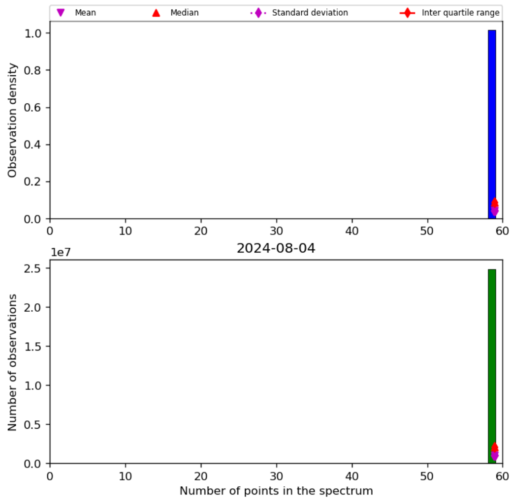
Figure 44: Histogram of "Number of points in the spectrum" for 2024-08-03 to 2024-08-05
