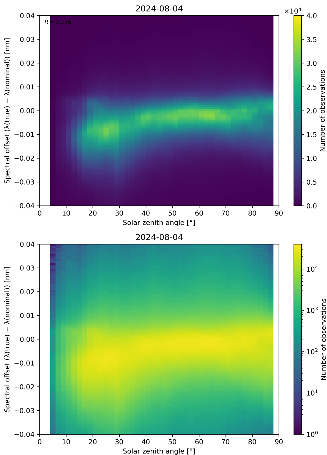
Figure 117: Scatter density plot of “Solar zenith angle” against “Spectral offset ( \lambda(\text{true}) - \lambda(\text{nominal}) )” for 2024-08-03 to 2024-08-05.
