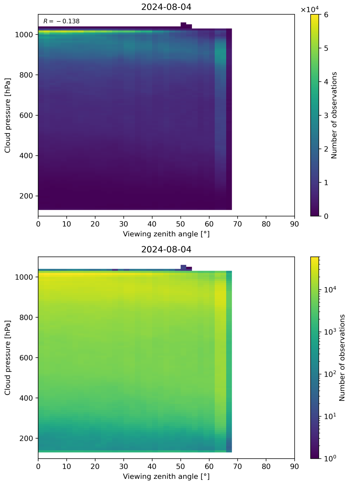
Figure 121: Scatter density plot of “Viewing zenith angle” against “Cloud pressure” for 2024-08-03 to 2024-08-05.
