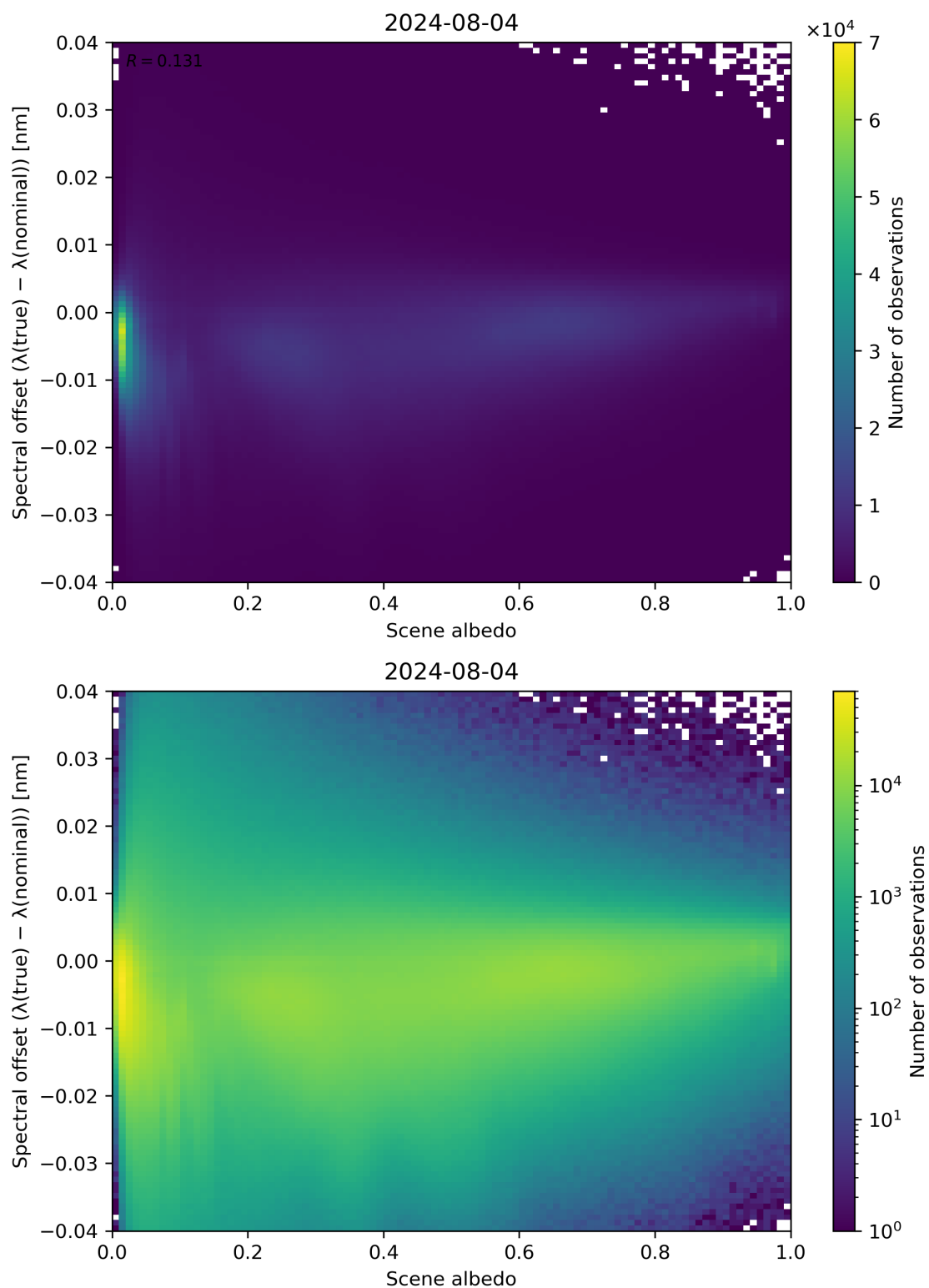
Figure 107: Scatter density plot of “Scene albedo” against “Spectral offset ( \lambda(\text{true}) - \lambda(\text{nominal}) )” for 2024-08-03 to 2024-08-05.
