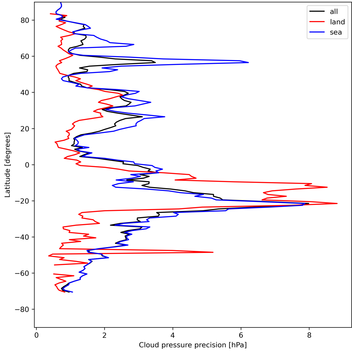
Figure 14: Zonal average of “Cloud pressure precision” for 2024-08-03 to 2024-08-05.
