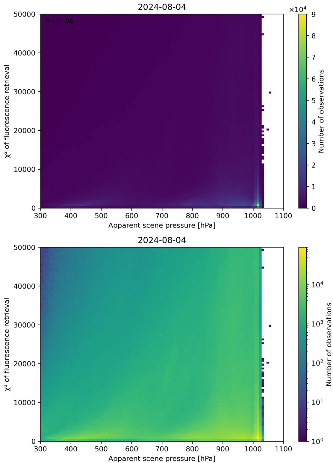
Figure 63: Scatter density plot of “Apparent scene pressure” against “ \chi^2 of fluorescence retrieval” for 2024-08-03 to 2024-08-05.
