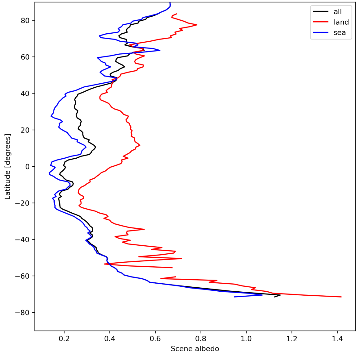
Figure 17: Zonal average of “Scene albedo” for 2024-08-04 to 2024-08-06.
