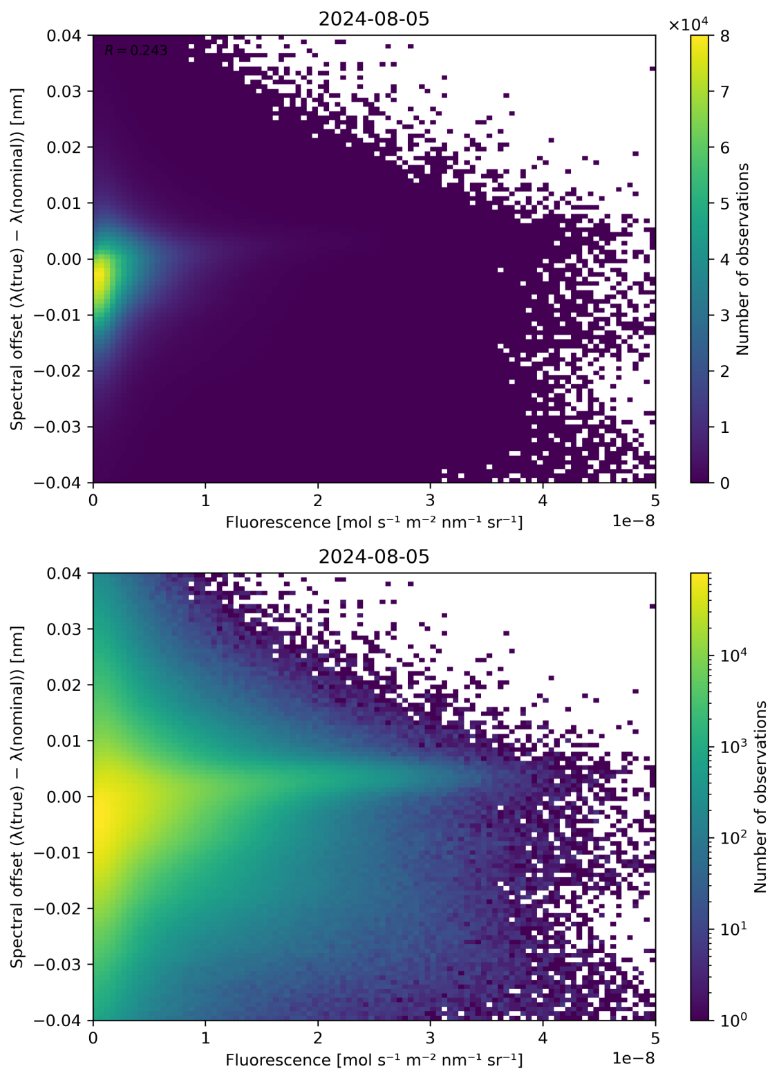
Figure 87: Scatter density plot of “Fluorescence” against “Spectral offset ( \lambda(\text{true}) - \lambda(\text{nominal}) )” for 2024-08-04 to 2024-08-06.
