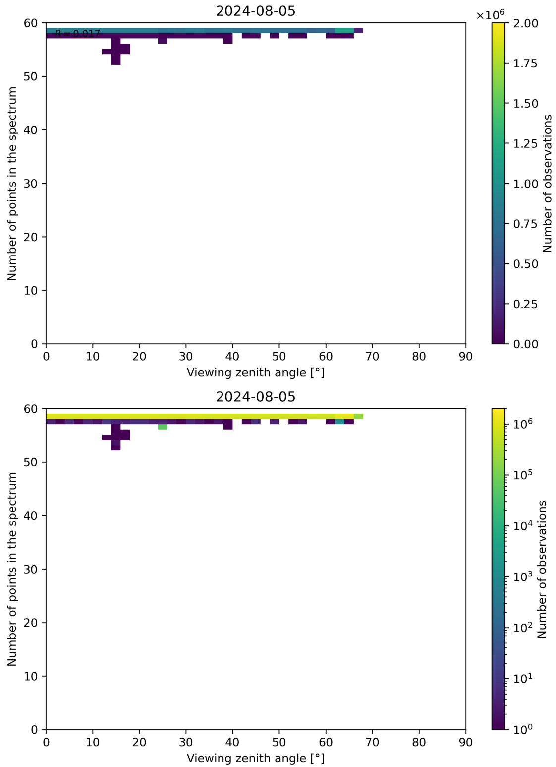
Figure 125: Scatter density plot of “Viewing zenith angle” against “Number of points in the spectrum” for 2024-08-04 to 2024-08-06.
