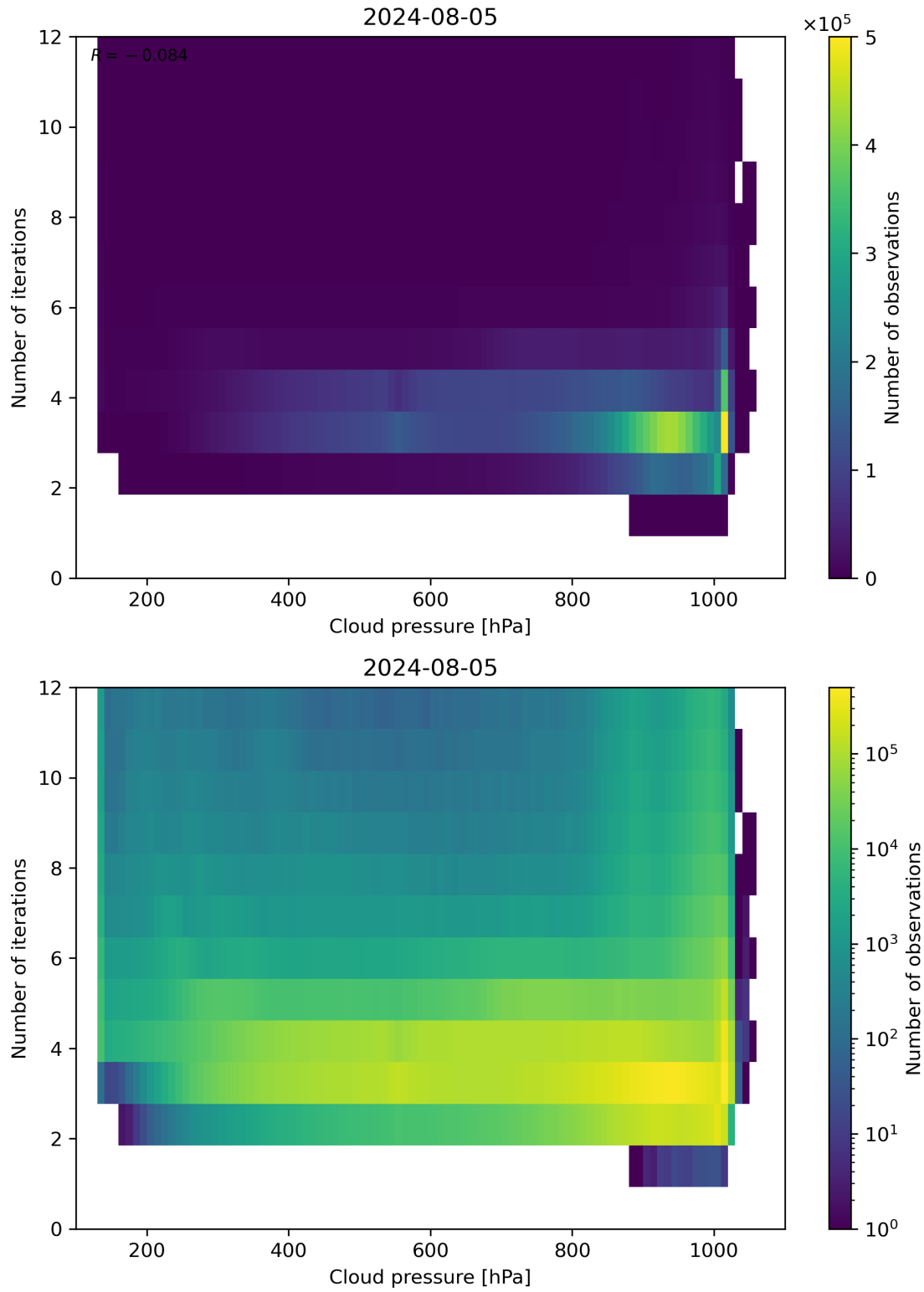
Figure 81: Scatter density plot of “Cloud pressure” against “Number of iterations” for 2024-08-04 to 2024-08-06.
