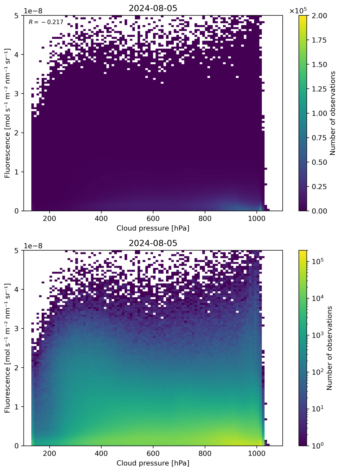
Figure 80: Scatter density plot of “Cloud pressure” against “Fluorescence” for 2024-08-04 to 2024-08-06.
