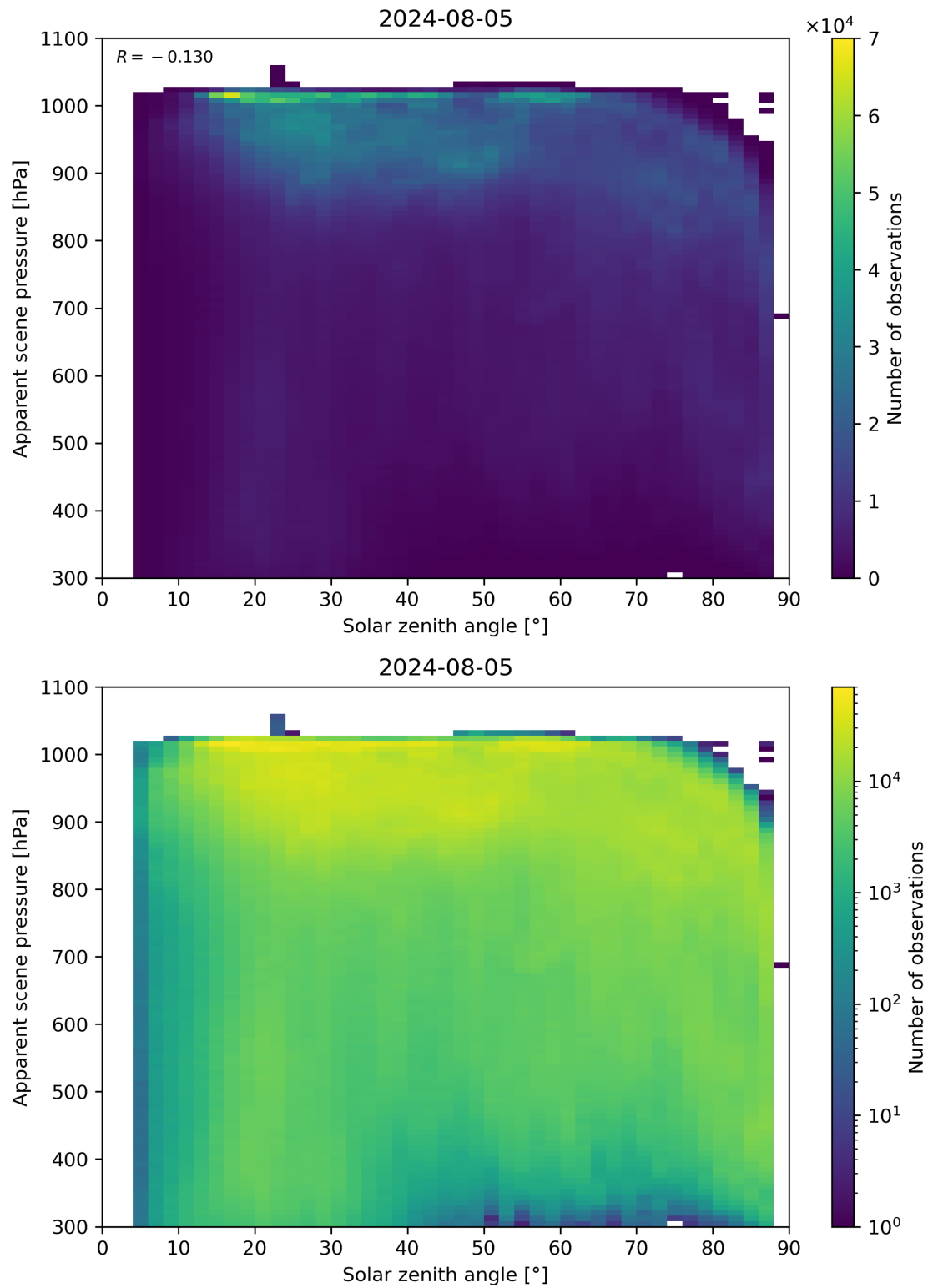
Figure 108: Scatter density plot of “Solar zenith angle” against “Apparent scene pressure” for 2024-08-04 to 2024-08-06.
