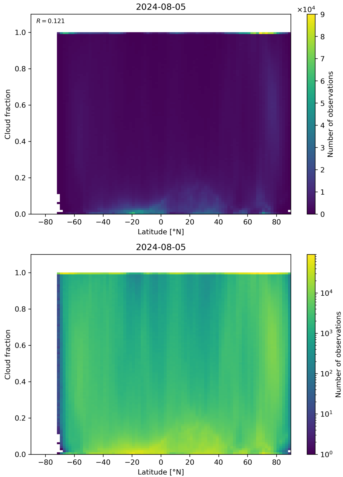
Figure 90: Scatter density plot of “Latitude” against “Cloud fraction” for 2024-08-04 to 2024-08-06.
