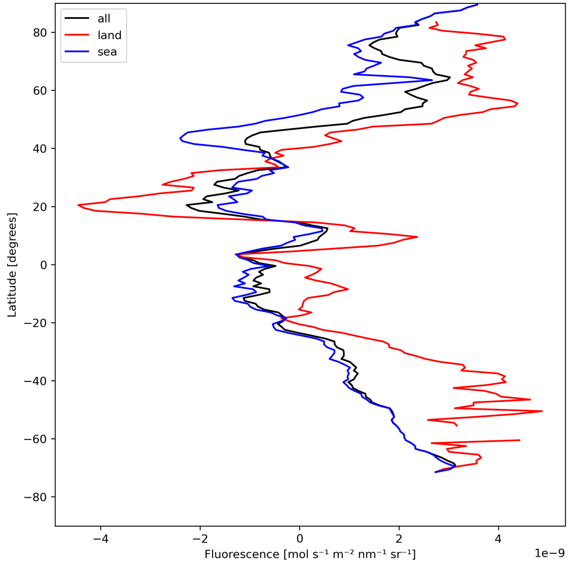
Figure 23: Zonal average of “Fluorescence” for 2024-08-04 to 2024-08-06.
