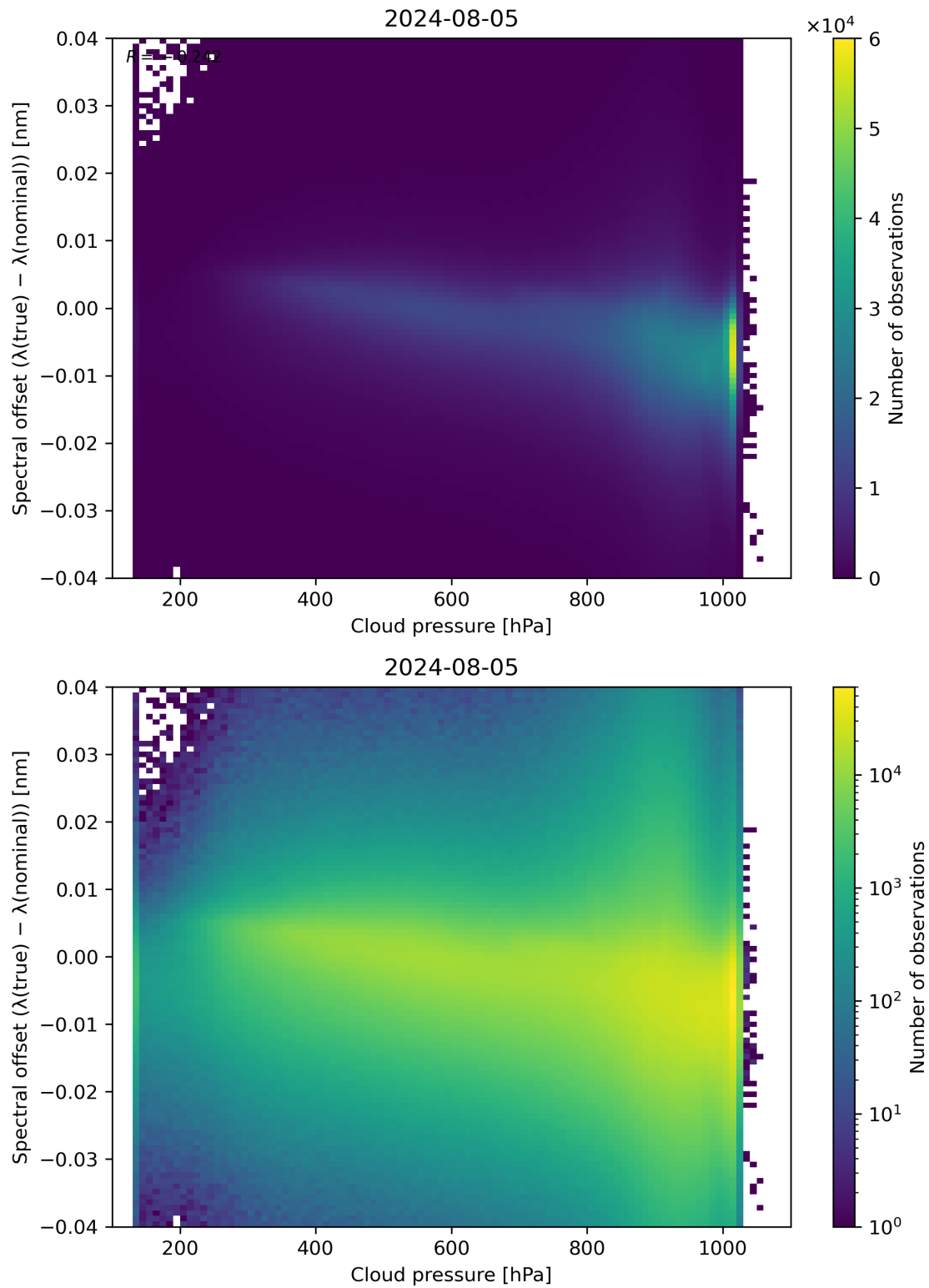
Figure 84: Scatter density plot of “Cloud pressure” against “Spectral offset ( \lambda(\text{true}) - \lambda(\text{nominal}) )” for 2024-08-04 to 2024-08-06.
