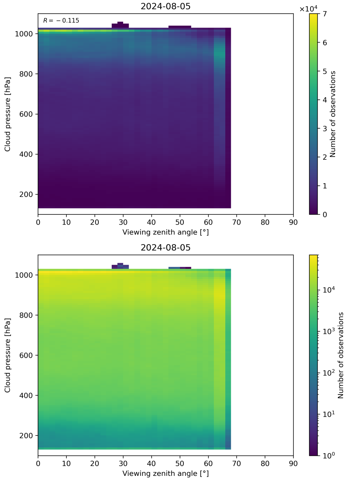
Figure 121: Scatter density plot of “Viewing zenith angle” against “Cloud pressure” for 2024-08-04 to 2024-08-06.
