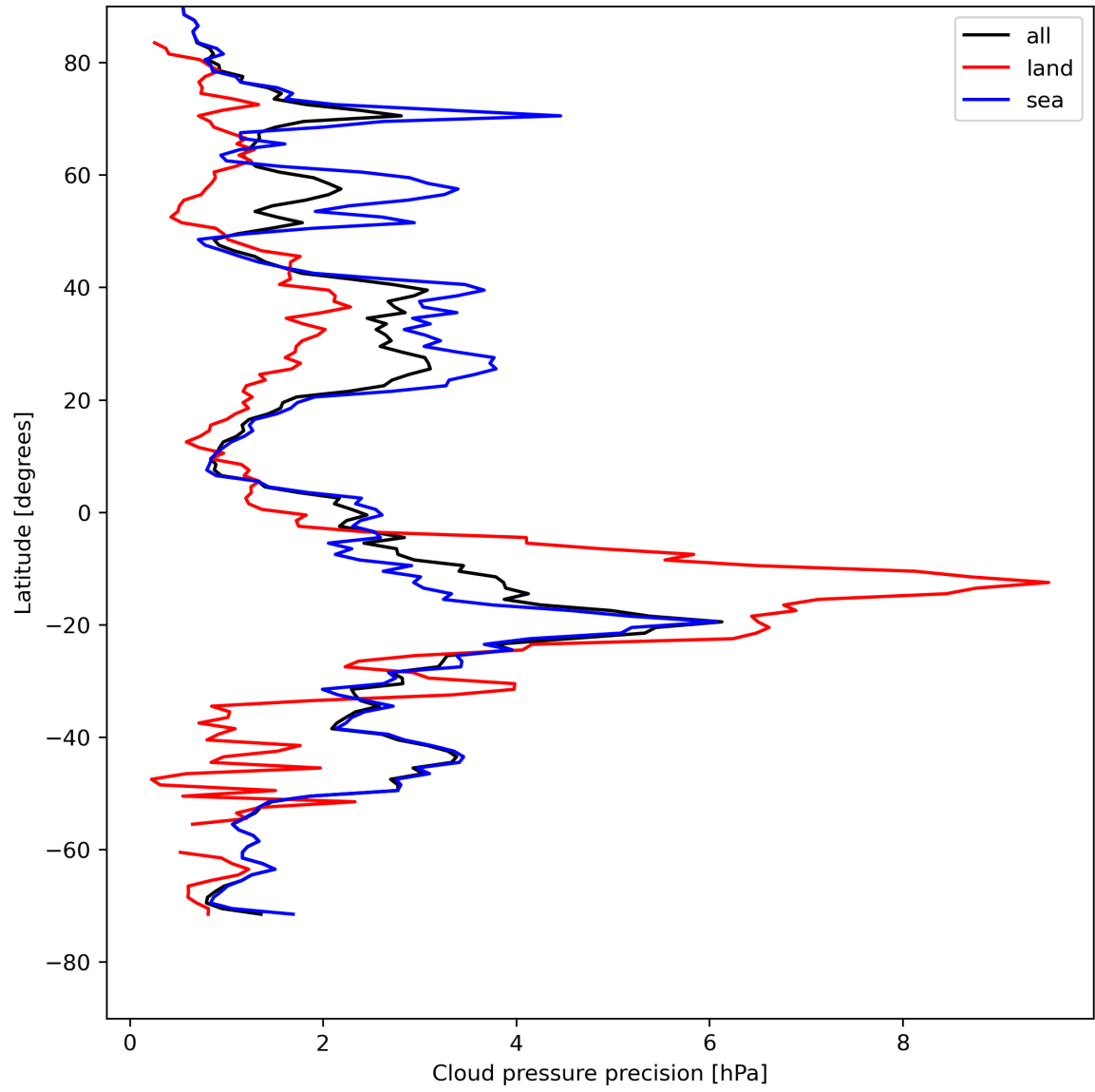
Figure 14: Zonal average of “Cloud pressure precision” for 2024-08-04 to 2024-08-06.
