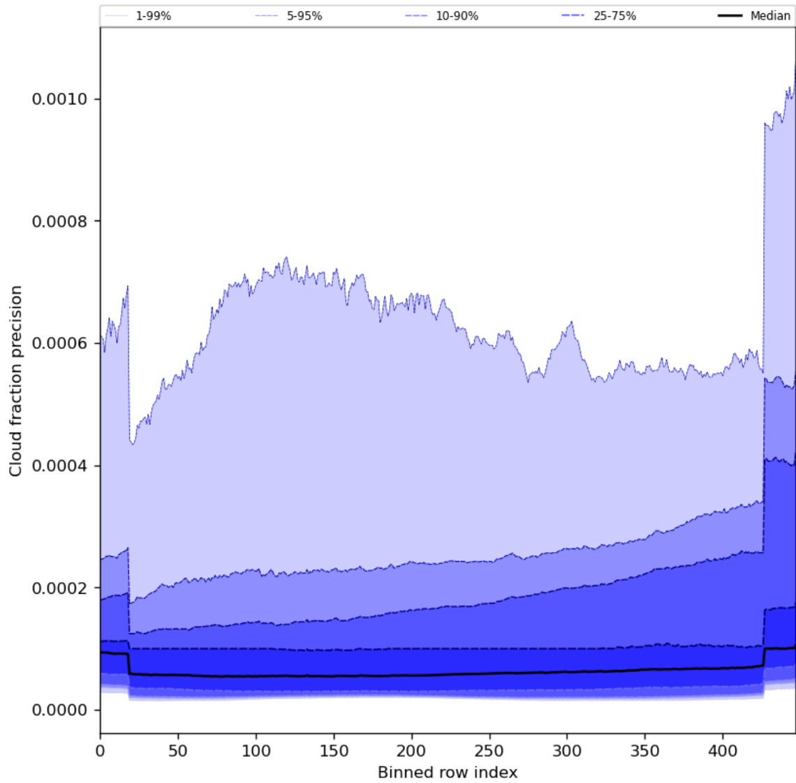
Figure 50: Along track statistics of “Cloud fraction precision” for 2024-08-04 to 2024-08-06
