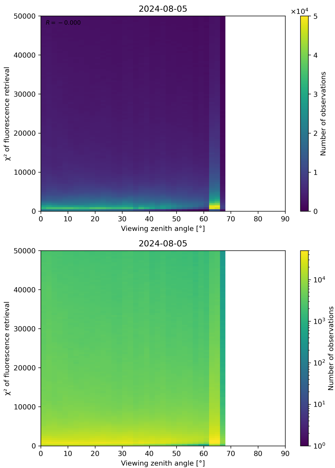
Figure 119: Scatter density plot of “Viewing zenith angle” against “ \chi^2 of fluorescence retrieval” for 2024-08-04 to 2024-08-06.
