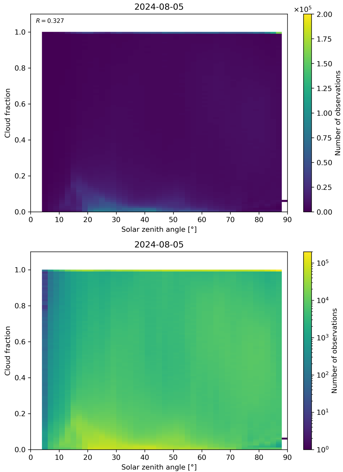
Figure 110: Scatter density plot of “Solar zenith angle” against “Cloud fraction” for 2024-08-04 to 2024-08-06.
