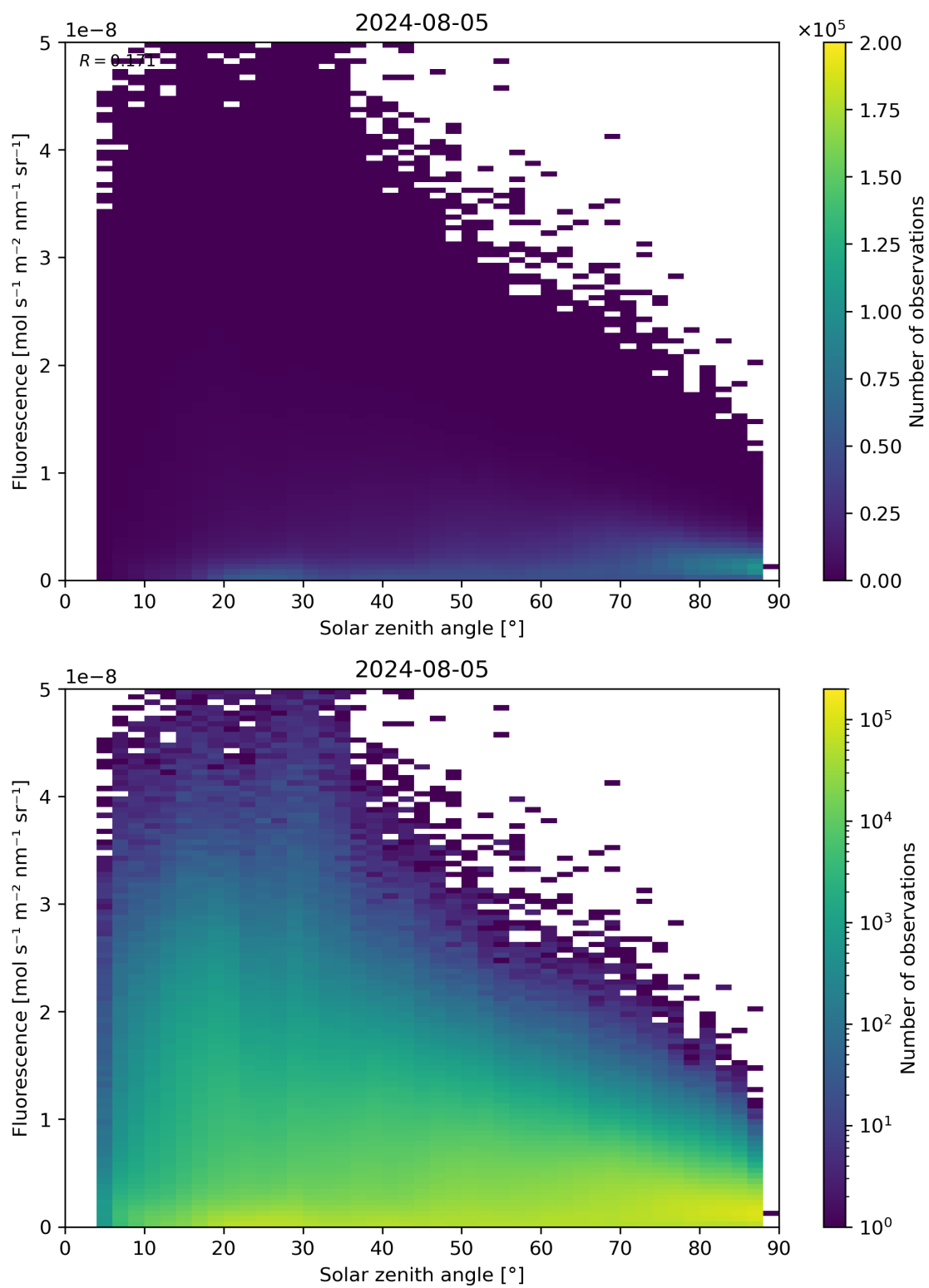
Figure 112: Scatter density plot of “Solar zenith angle” against “Fluorescence” for 2024-08-04 to 2024-08-06.
