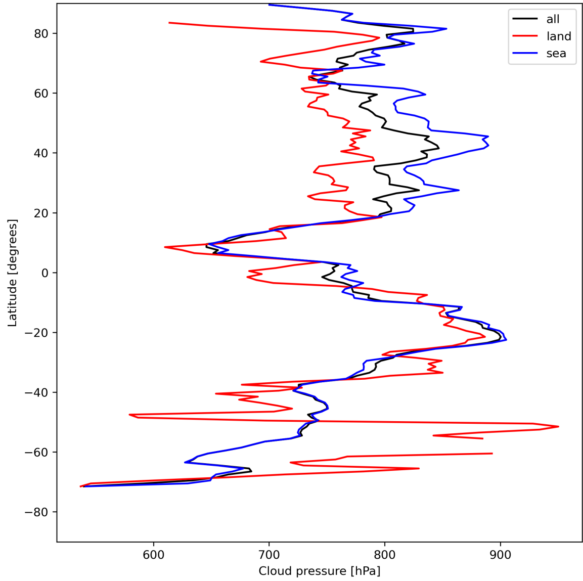
Figure 13: Zonal average of “Cloud pressure” for 2024-08-04 to 2024-08-06.
