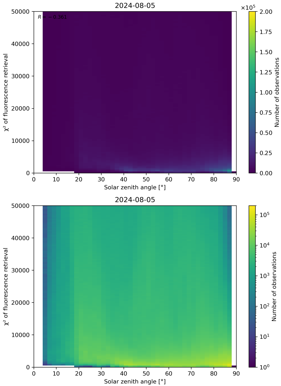
Figure 109: Scatter density plot of “Solar zenith angle” against “ \chi^2 of fluorescence retrieval” for 2024-08-04 to 2024-08-06.
