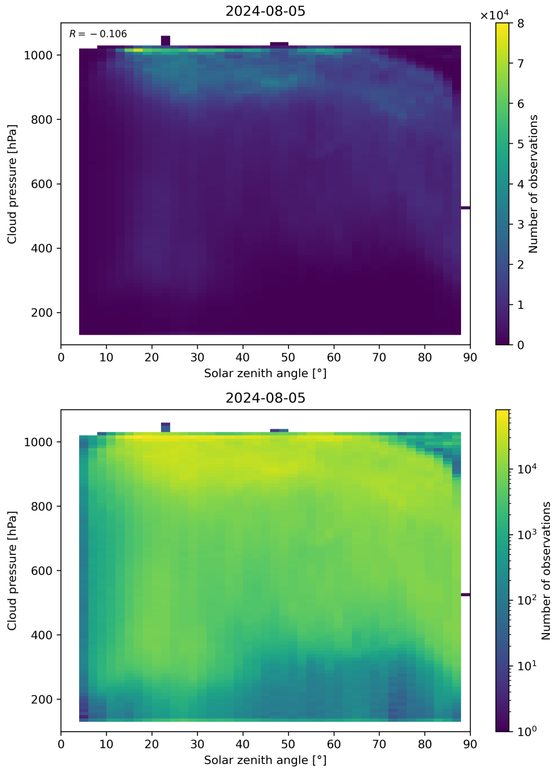
Figure 111: Scatter density plot of “Solar zenith angle” against “Cloud pressure” for 2024-08-04 to 2024-08-06.
