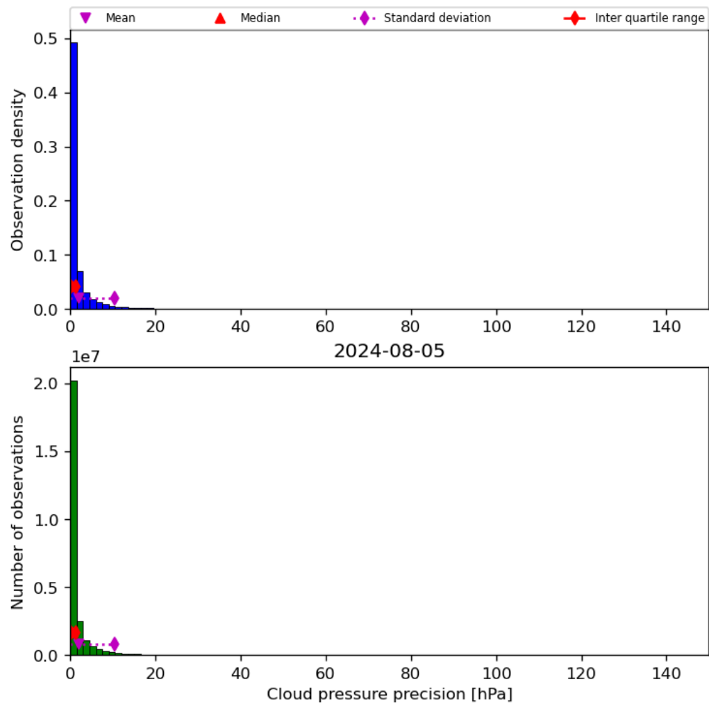
Figure 31: Histogram of “Cloud pressure precision” for 2024-08-04 to 2024-08-06
