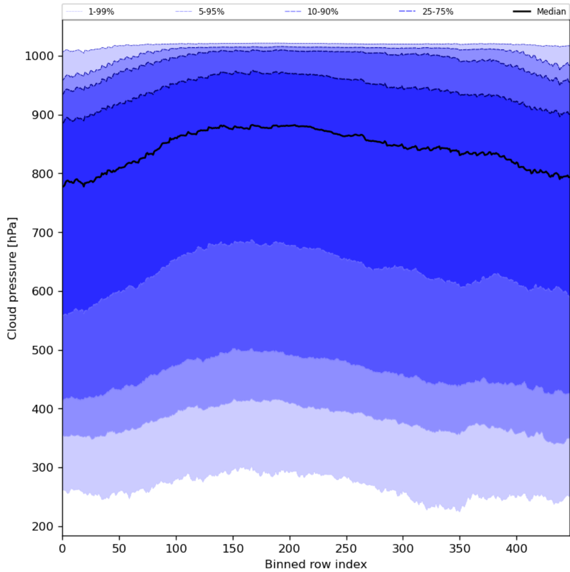
Figure 47: Along track statistics of “Cloud pressure” for 2024-08-04 to 2024-08-06
