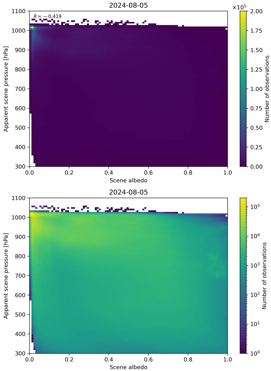
Figure 102: Scatter density plot of “Scene albedo” against “Apparent scene pressure” for 2024-08-04 to 2024-08-06.
