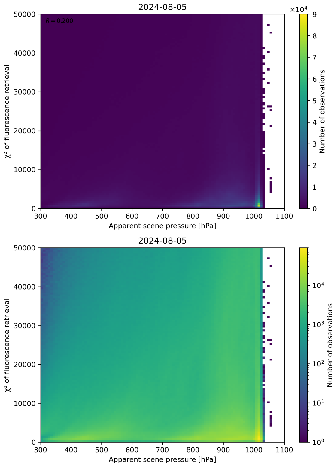
Figure 63: Scatter density plot of “Apparent scene pressure” against “ \chi^2 of fluorescence retrieval” for 2024-08-04 to 2024-08-06.
