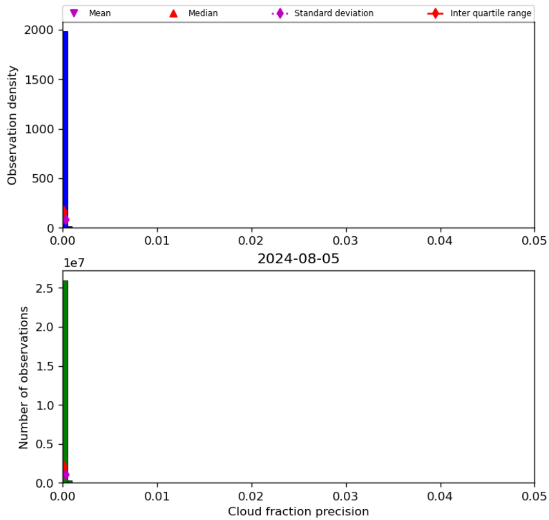
Figure 33: Histogram of “Cloud fraction precision” for 2024-08-04 to 2024-08-06
