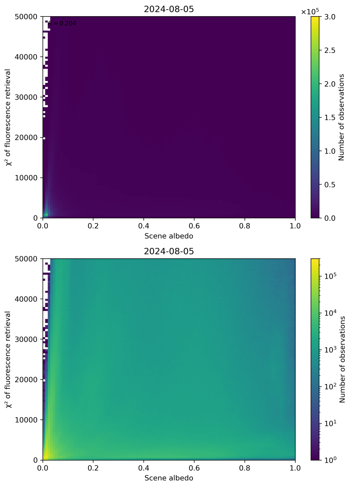
Figure 103: Scatter density plot of “Scene albedo” against “ \chi^2 of fluorescence retrieval” for 2024-08-04 to 2024-08-06.
