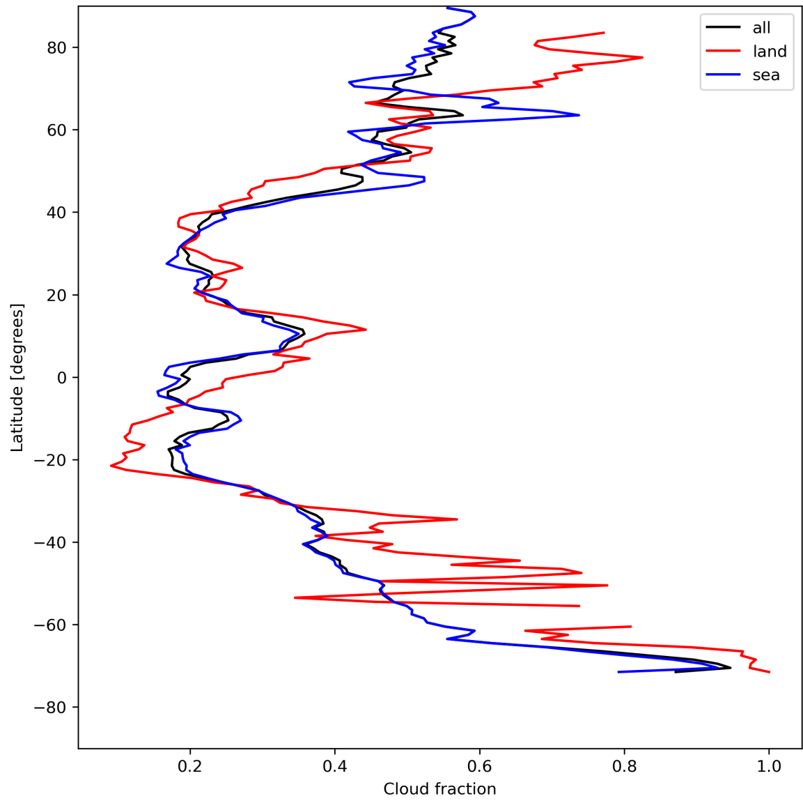
Figure 15: Zonal average of “Cloud fraction” for 2024-08-04 to 2024-08-06.
