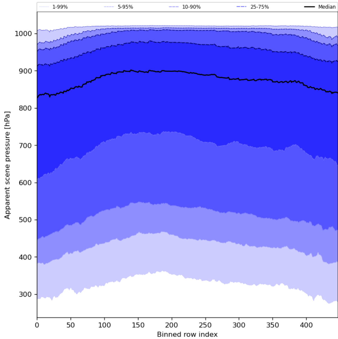
Figure 53: Along track statistics of “Apparent scene pressure” for 2024-08-04 to 2024-08-06
