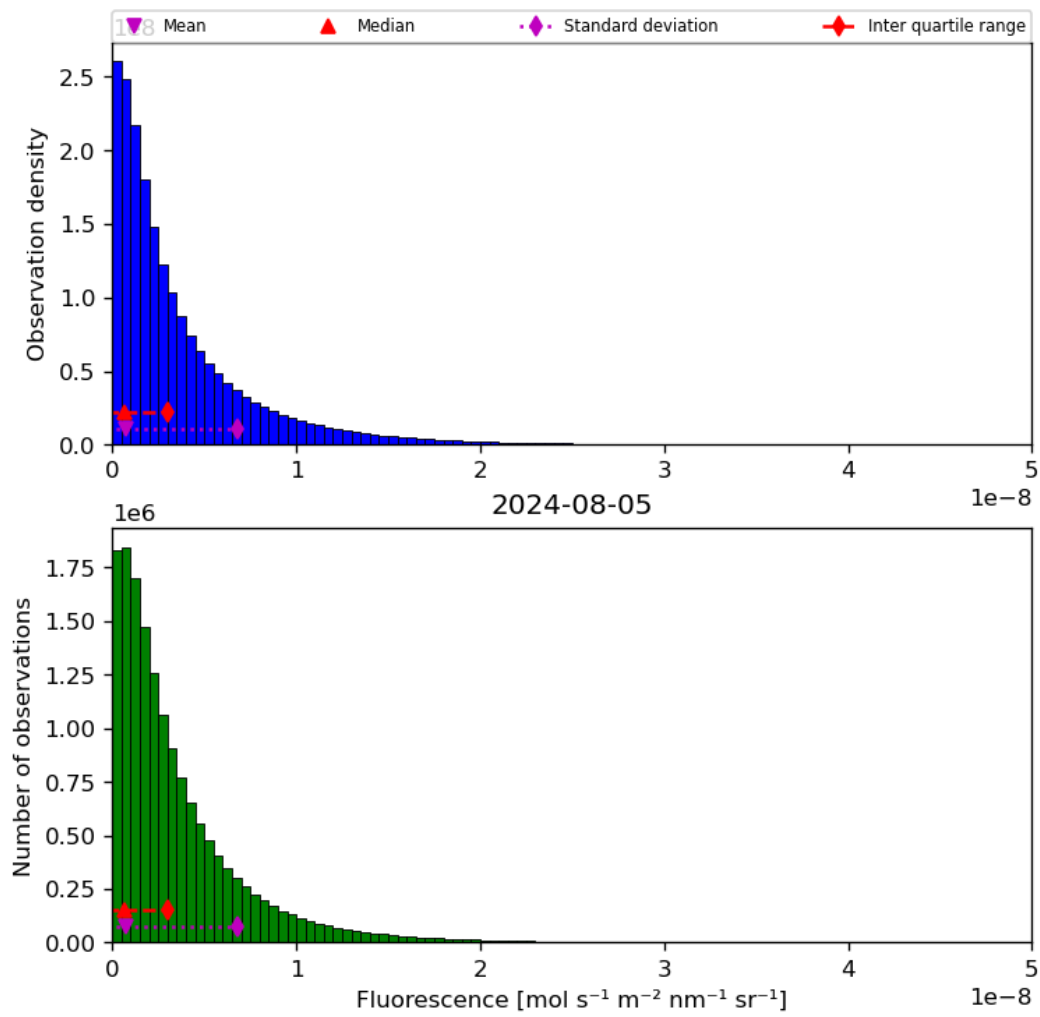
Figure 40: Histogram of “Fluorescence” for 2024-08-04 to 2024-08-06
