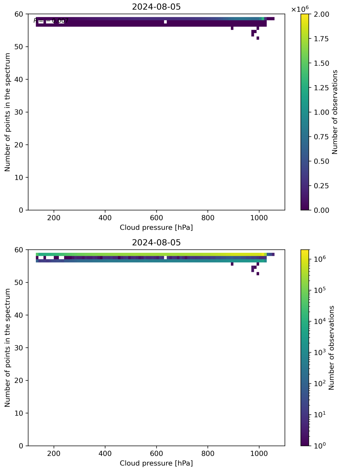
Figure 82: Scatter density plot of “Cloud pressure” against “Number of points in the spectrum” for 2024-08-04 to 2024-08-06.
