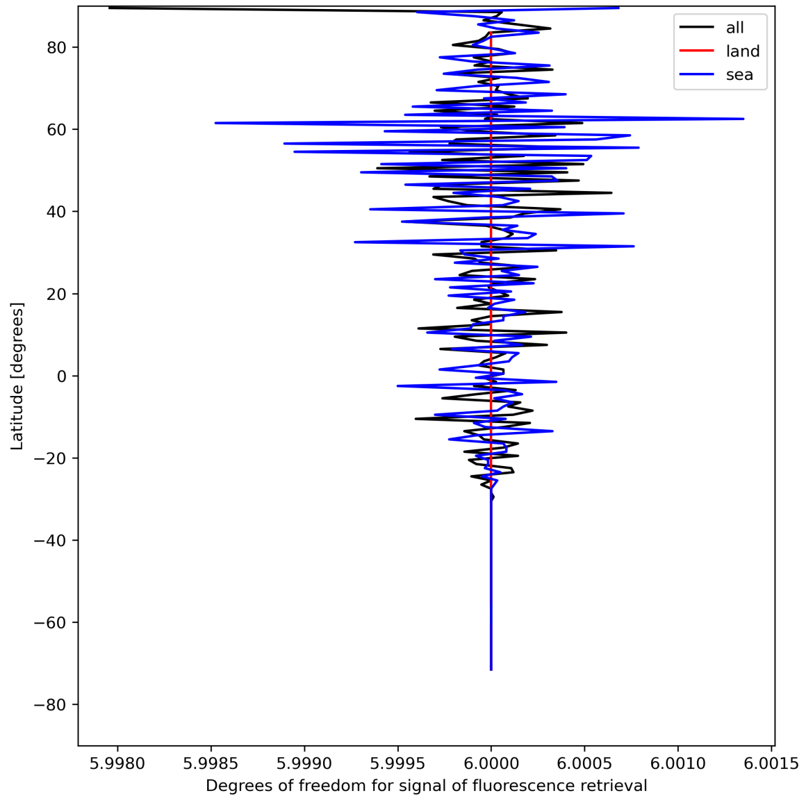
Figure 26: Zonal average of “Degrees of freedom for signal of fluorescence retrieval” for 2024-08-04 to 2024-08-06.
