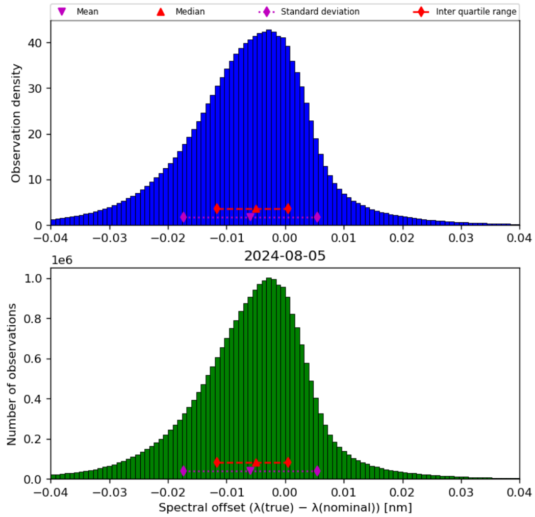
Figure 45: Histogram of “Spectral offset ( \lambda(\text{true}) - \lambda(\text{nominal}) )” for 2024-08-04 to 2024-08-06
