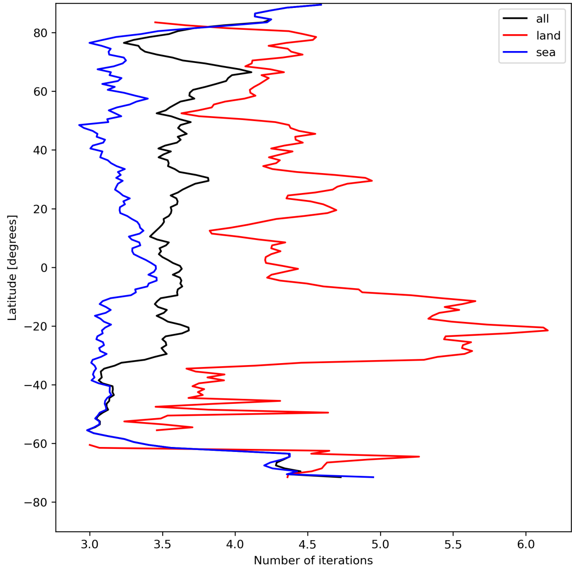
Figure 22: Zonal average of “Number of iterations” for 2024-08-04 to 2024-08-06.
