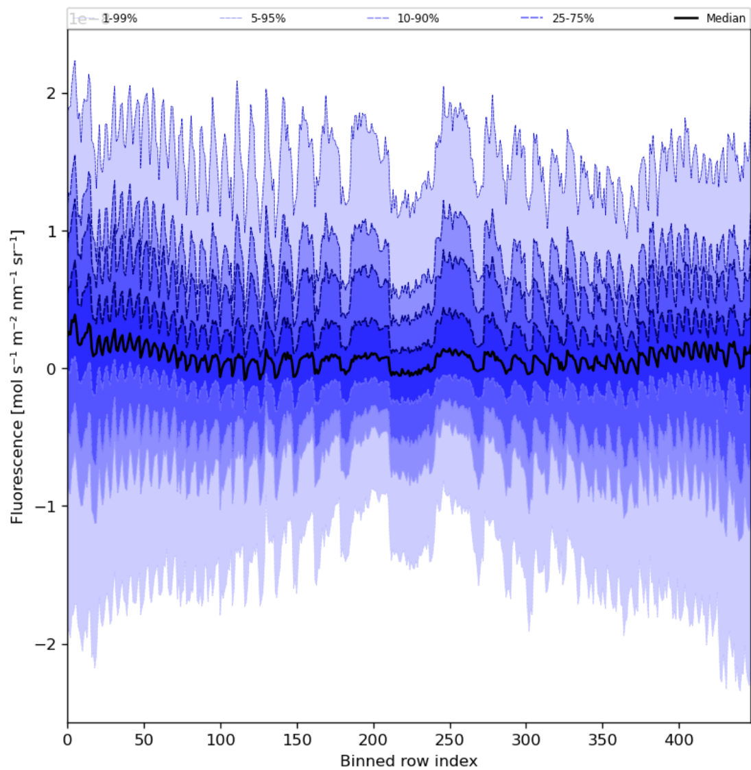
Figure 57: Along track statistics of “Fluorescence” for 2024-08-04 to 2024-08-06
