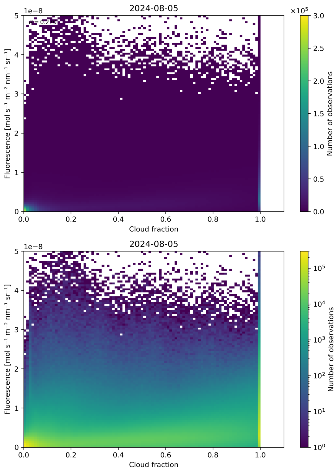
Figure 72: Scatter density plot of “Cloud fraction” against “Fluorescence” for 2024-08-04 to 2024-08-06.
