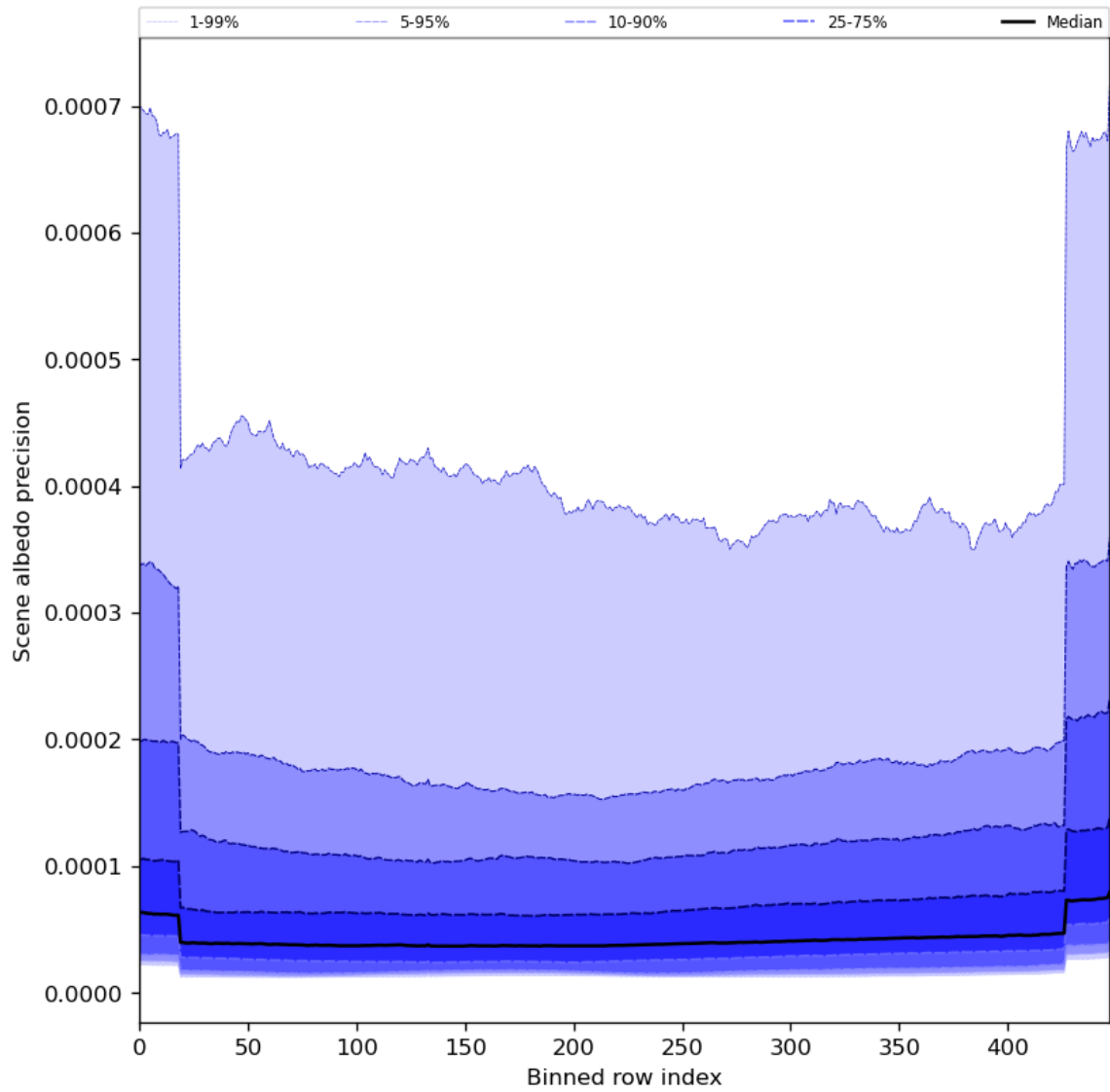
Figure 52: Along track statistics of “Scene albedo precision” for 2024-08-04 to 2024-08-06
