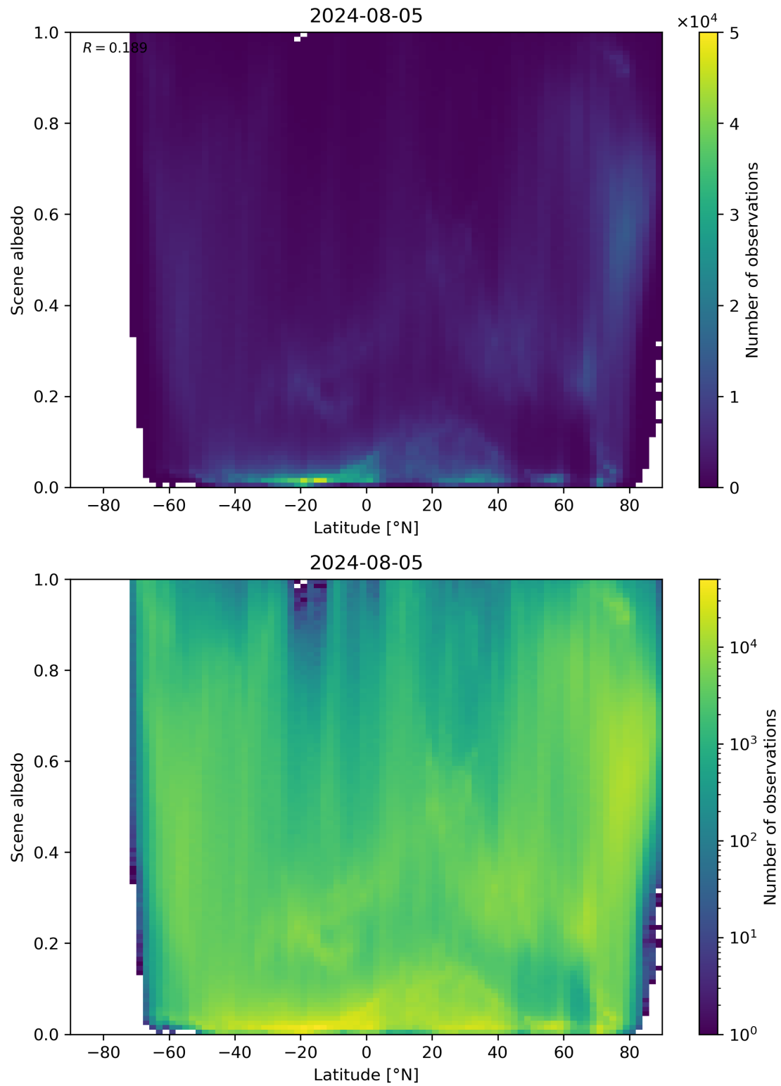
Figure 95: Scatter density plot of “Latitude” against “Scene albedo” for 2024-08-04 to 2024-08-06.
