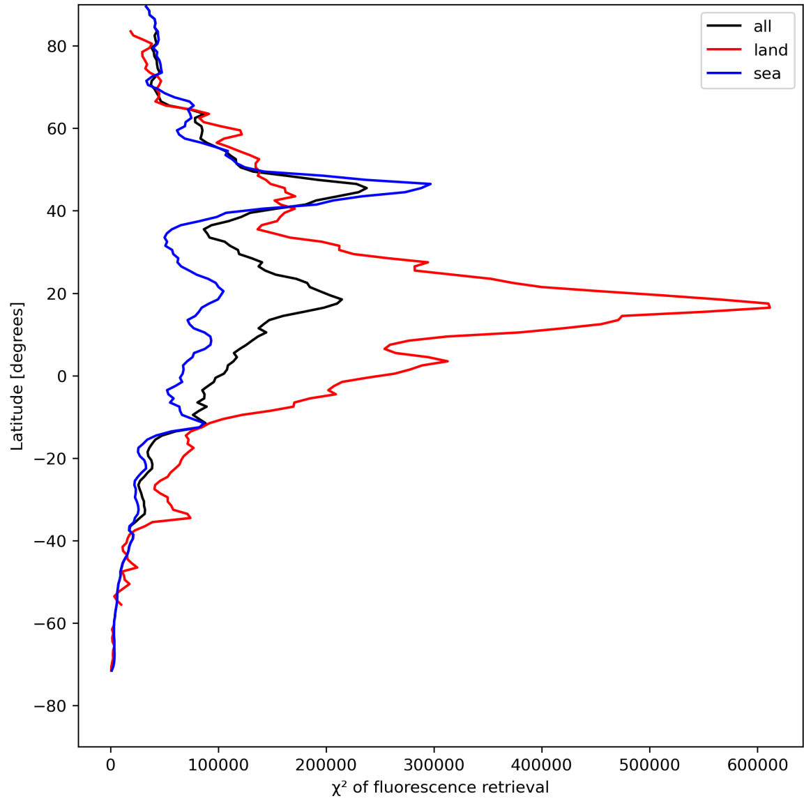
Figure 25: Zonal average of “ \chi^2 of fluorescence retrieval” for 2024-08-04 to 2024-08-06.
