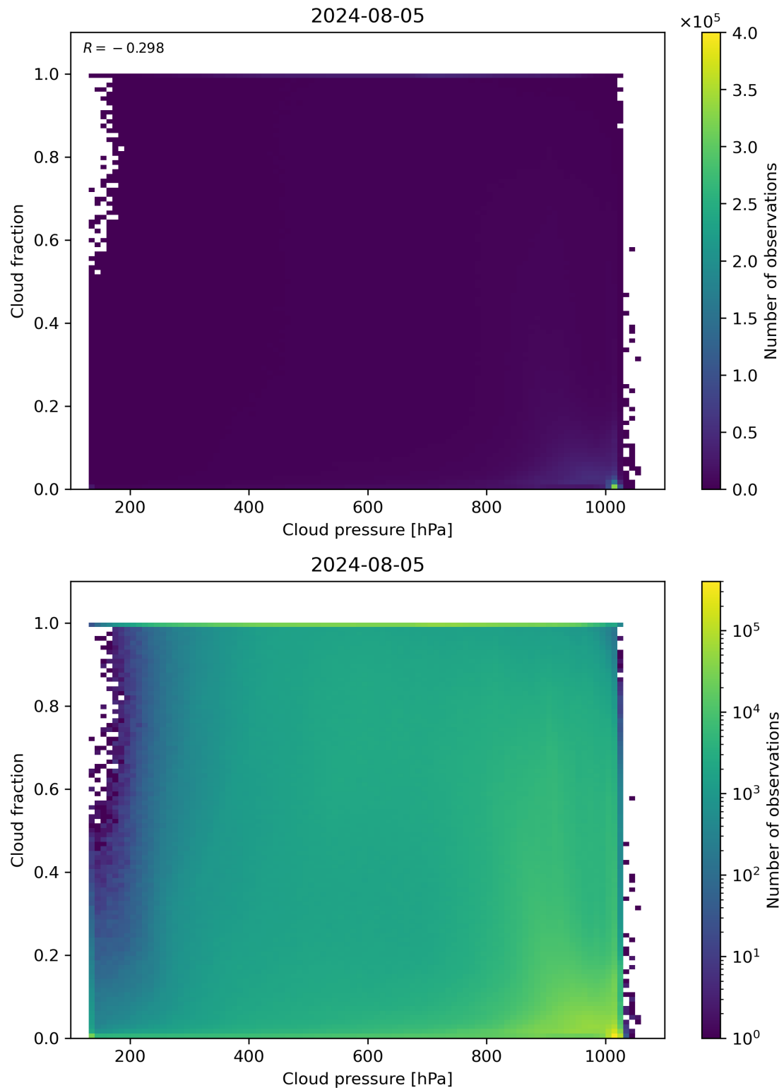
Figure 79: Scatter density plot of “Cloud pressure” against “Cloud fraction” for 2024-08-04 to 2024-08-06.
