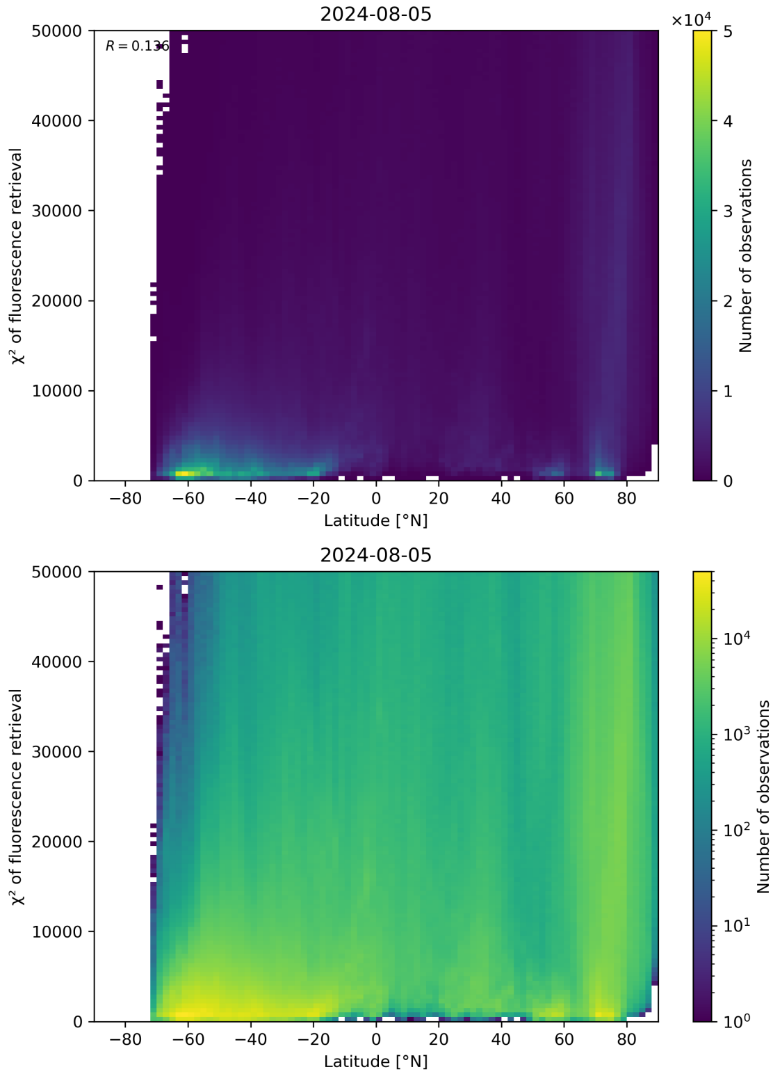
Figure 89: Scatter density plot of “Latitude” against “ \chi^2 of fluorescence retrieval” for 2024-08-04 to 2024-08-06.
