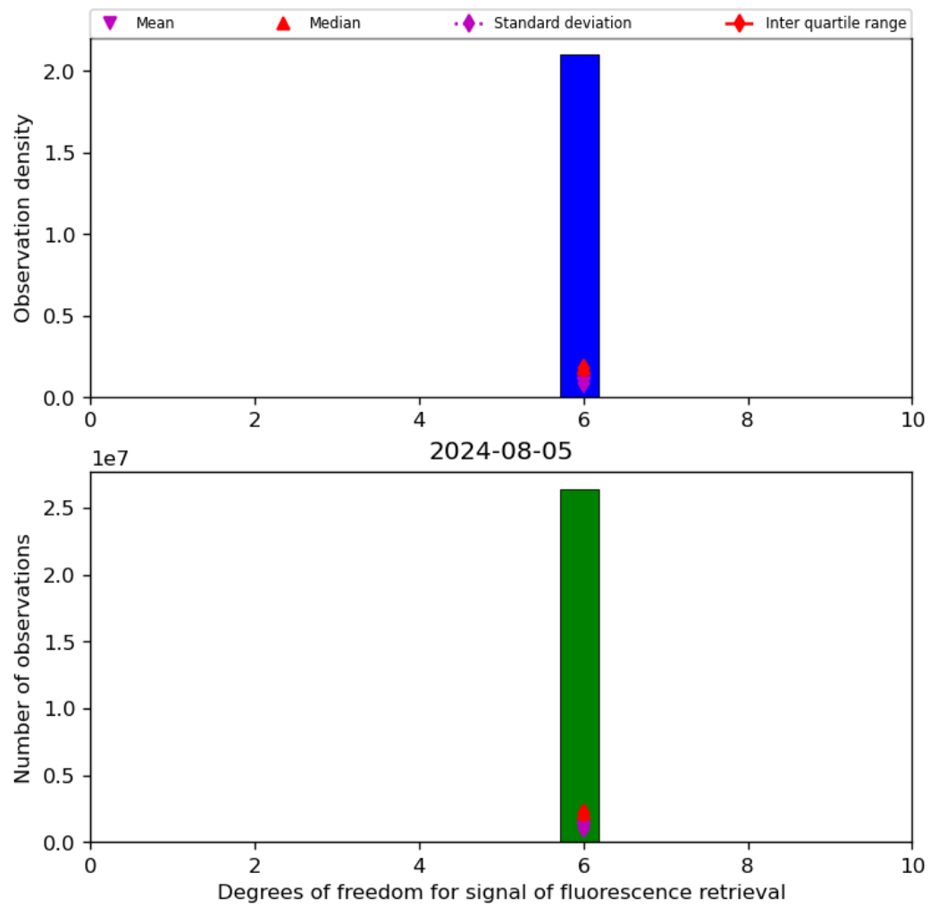
Figure 43: Histogram of “Degrees of freedom for signal of fluorescence retrieval” for 2024-08-04 to 2024-08-06
