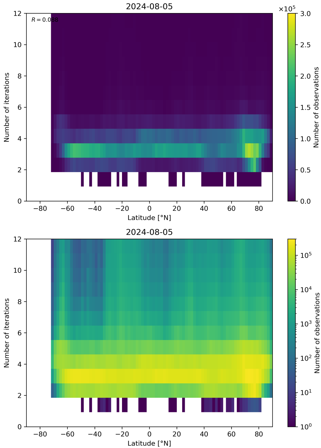
Figure 93: Scatter density plot of “Latitude” against “Number of iterations” for 2024-08-04 to 2024-08-06.
