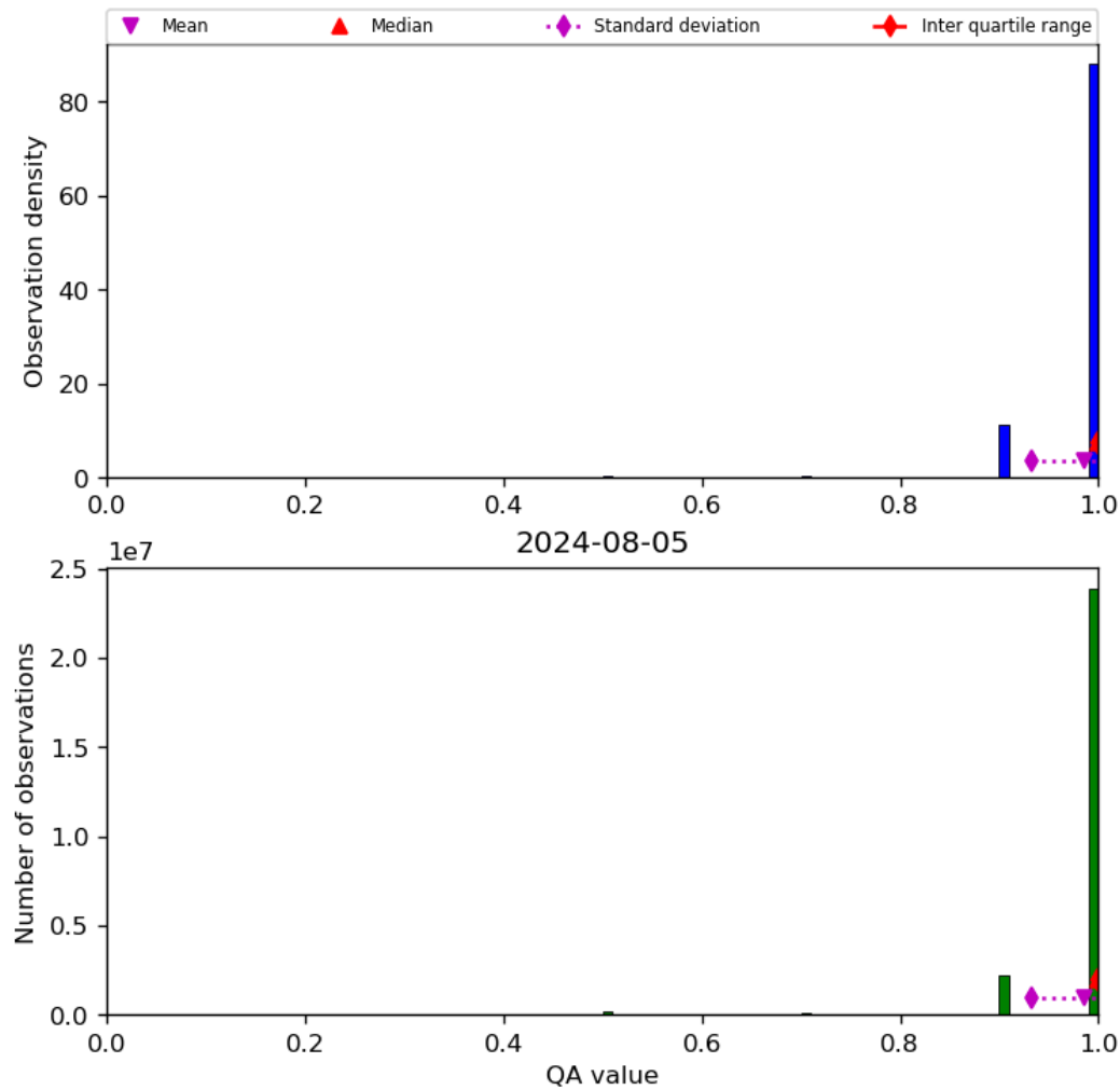
Figure 29: Histogram of “QA value” for 2024-08-04 to 2024-08-06
