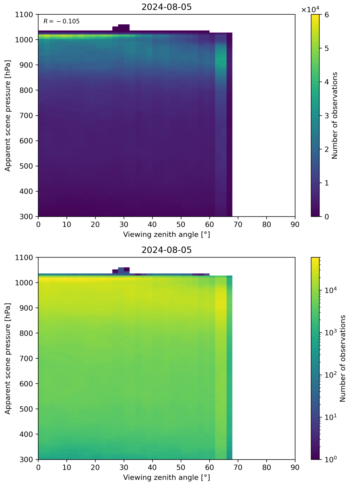
Figure 118: Scatter density plot of “Viewing zenith angle” against “Apparent scene pressure” for 2024-08-04 to 2024-08-06.
