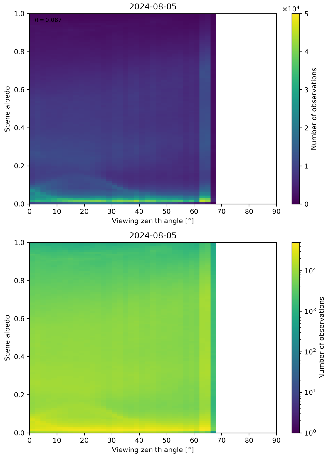
Figure 126: Scatter density plot of “Viewing zenith angle” against “Scene albedo” for 2024-08-04 to 2024-08-06.
