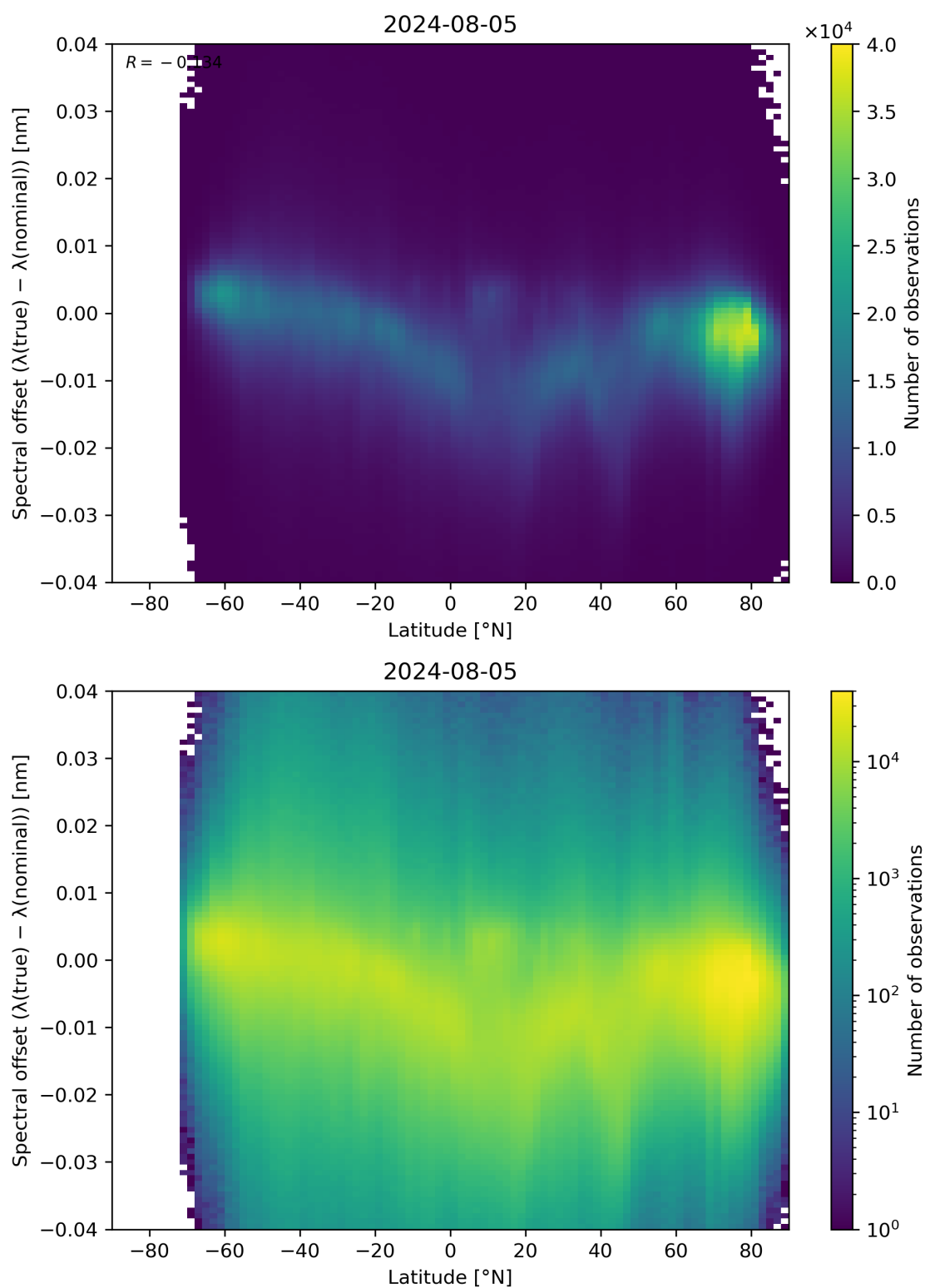
Figure 96: Scatter density plot of “Latitude” against “Spectral offset ( \lambda(\text{true}) - \lambda(\text{nominal}) )” for 2024-08-04 to 2024-08-06.
