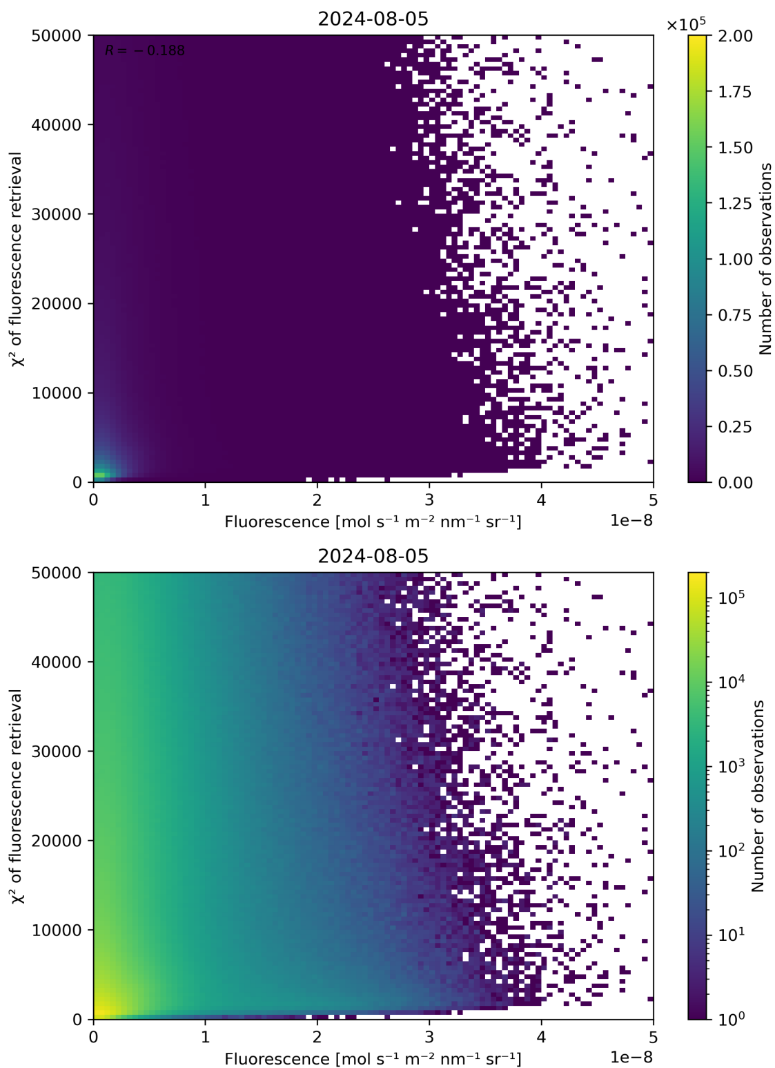
Figure 85: Scatter density plot of “Fluorescence” against “ \chi^2 of fluorescence retrieval” for 2024-08-04 to 2024-08-06.
