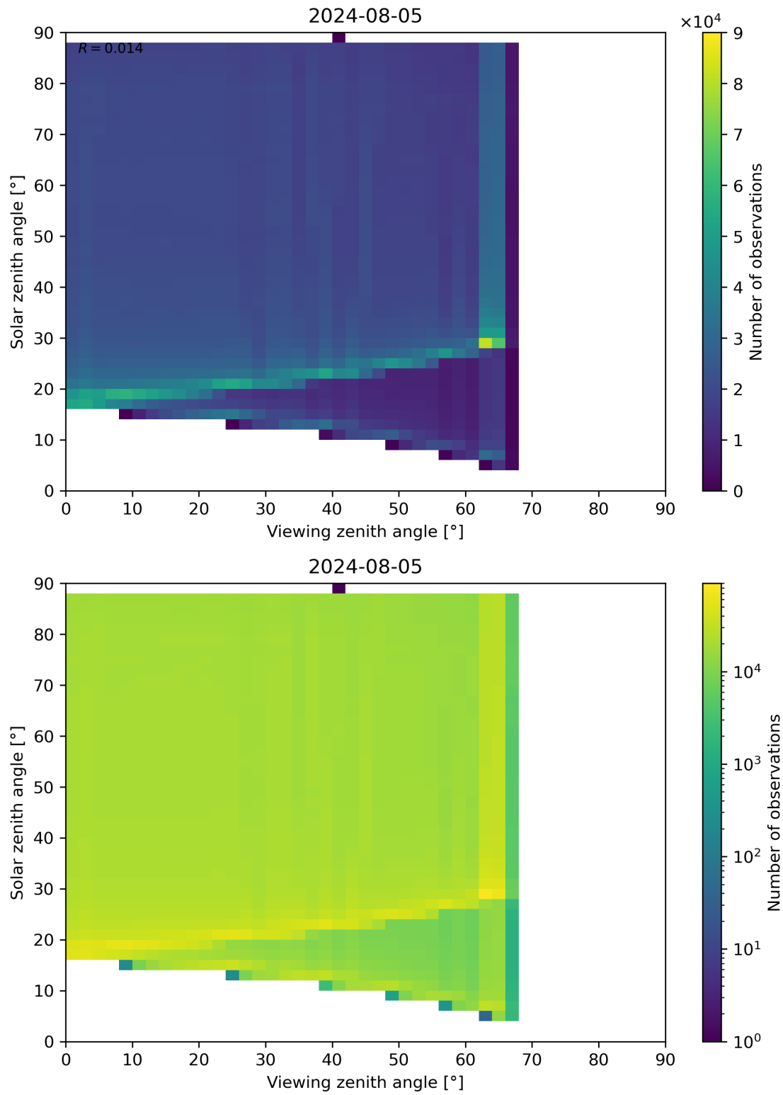
Figure 127: Scatter density plot of “Viewing zenith angle” against “Solar zenith angle” for 2024-08-04 to 2024-08-06.
