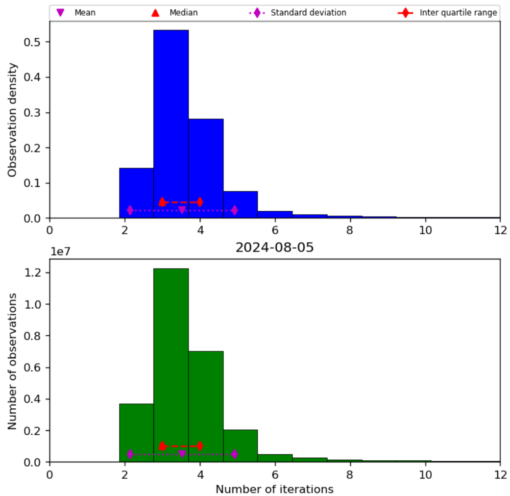
Figure 39: Histogram of “Number of iterations” for 2024-08-04 to 2024-08-06
