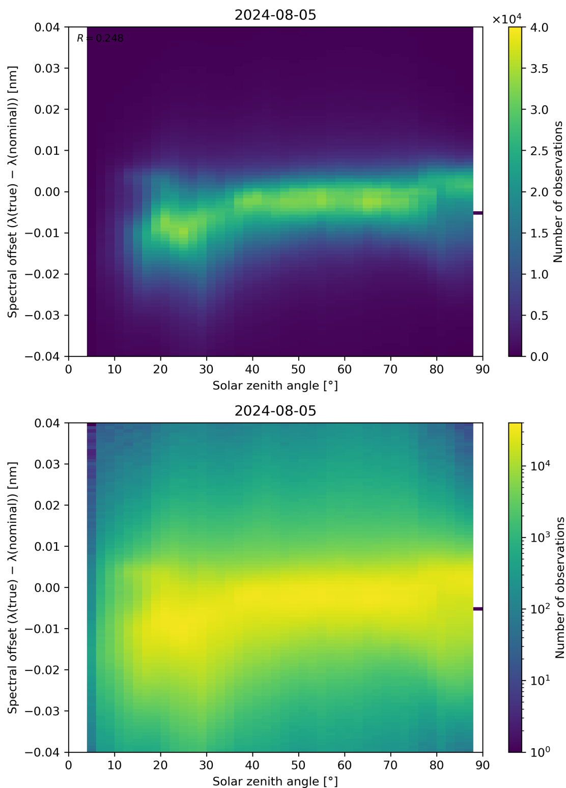
Figure 117: Scatter density plot of “Solar zenith angle” against “Spectral offset ( \lambda(\text{true}) - \lambda(\text{nominal}) )” for 2024-08-04 to 2024-08-06.
