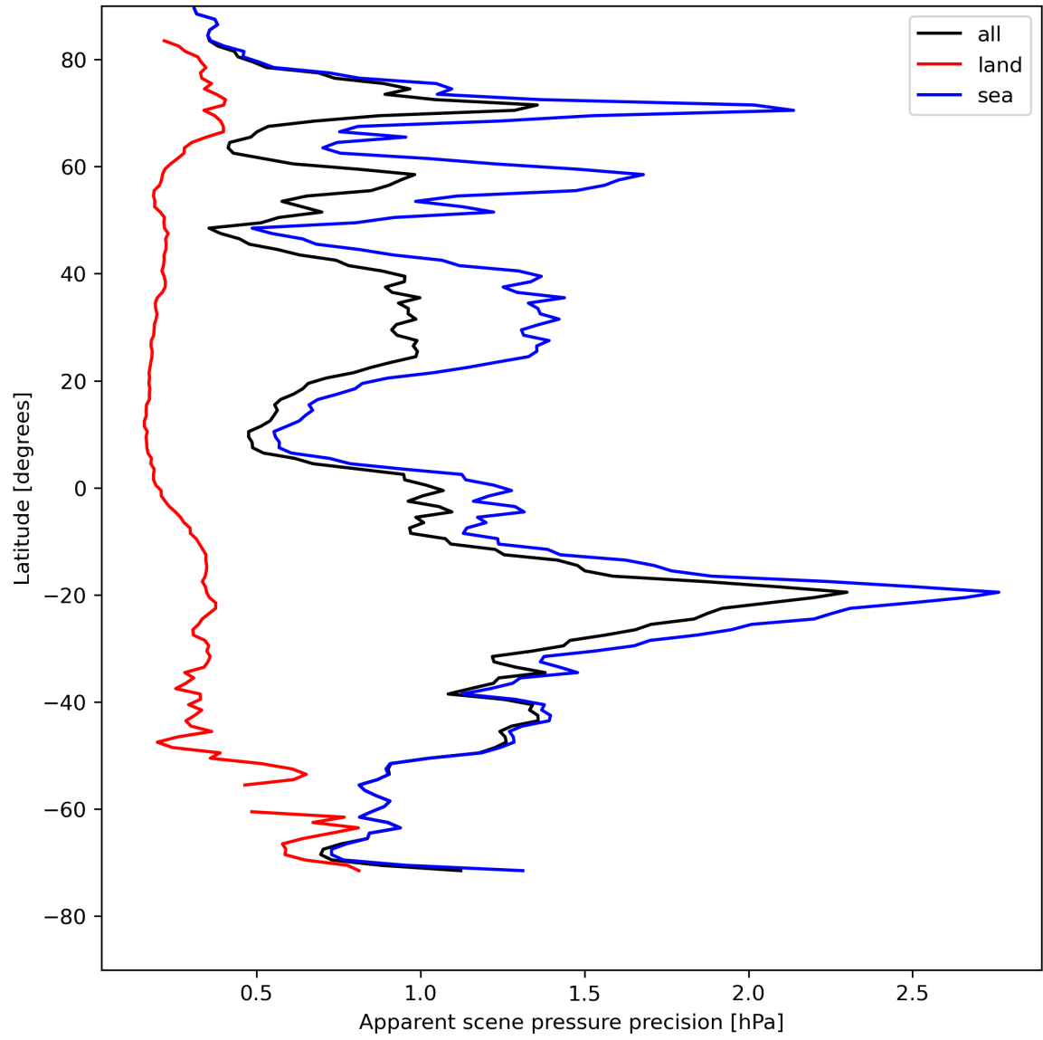
Figure 20: Zonal average of “Apparent scene pressure precision” for 2024-08-04 to 2024-08-06.
