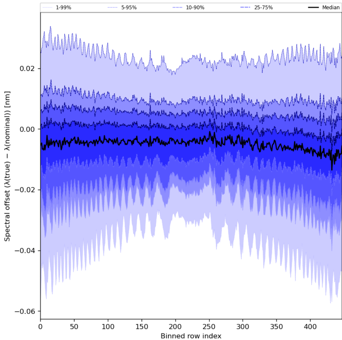
Figure 62: Along track statistics of “Spectral offset ( \lambda(\text{true}) - \lambda(\text{nominal}) )” for 2024-08-04 to 2024-08-06
