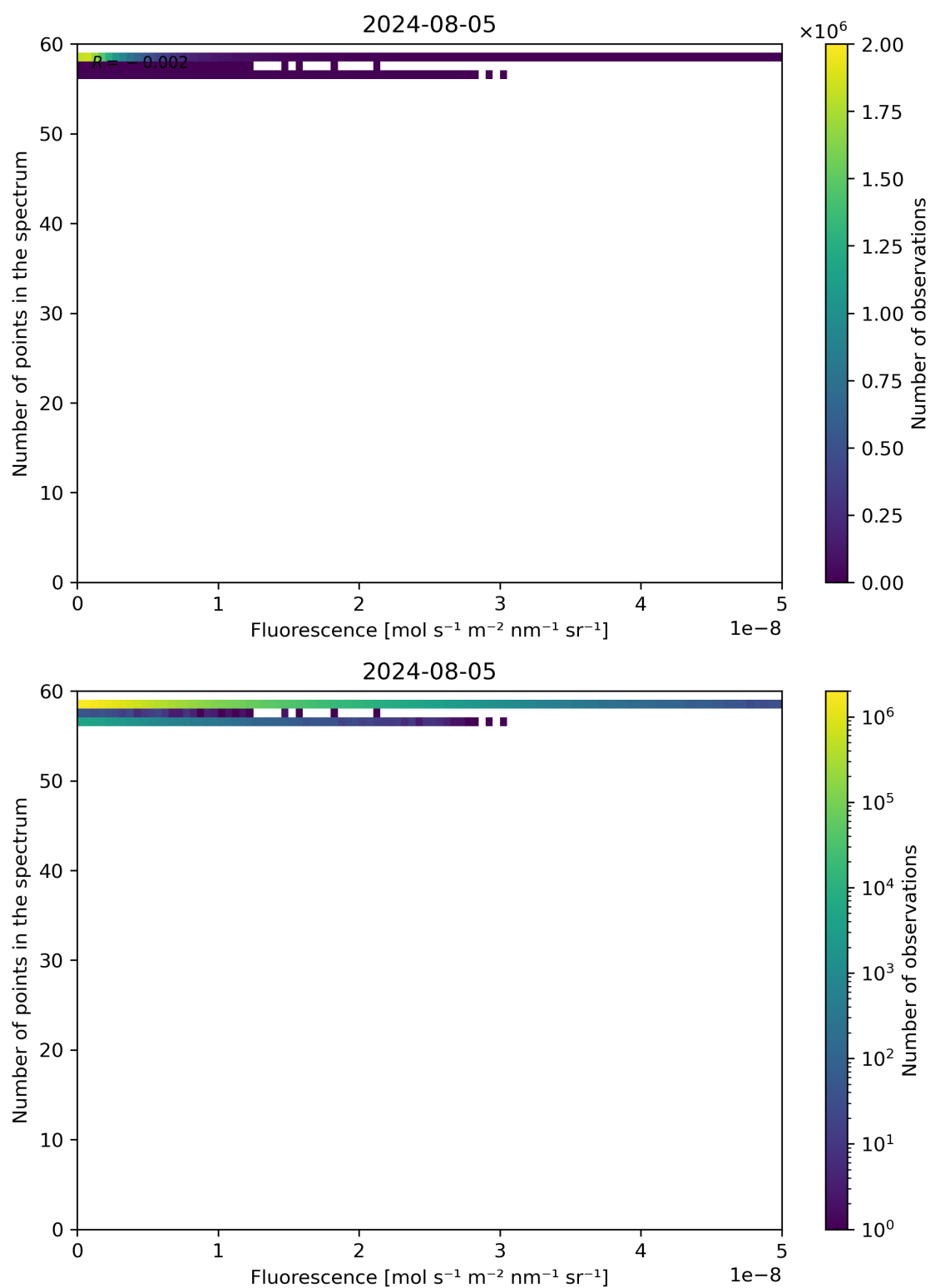
Figure 86: Scatter density plot of “Fluorescence” against “Number of points in the spectrum” for 2024-08-04 to 2024-08-06.
