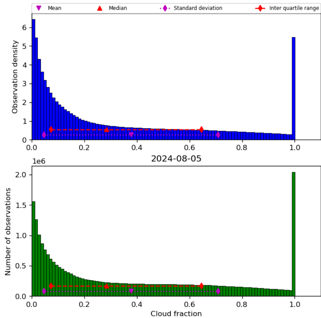
Figure 32: Histogram of “Cloud fraction” for 2024-08-04 to 2024-08-06
