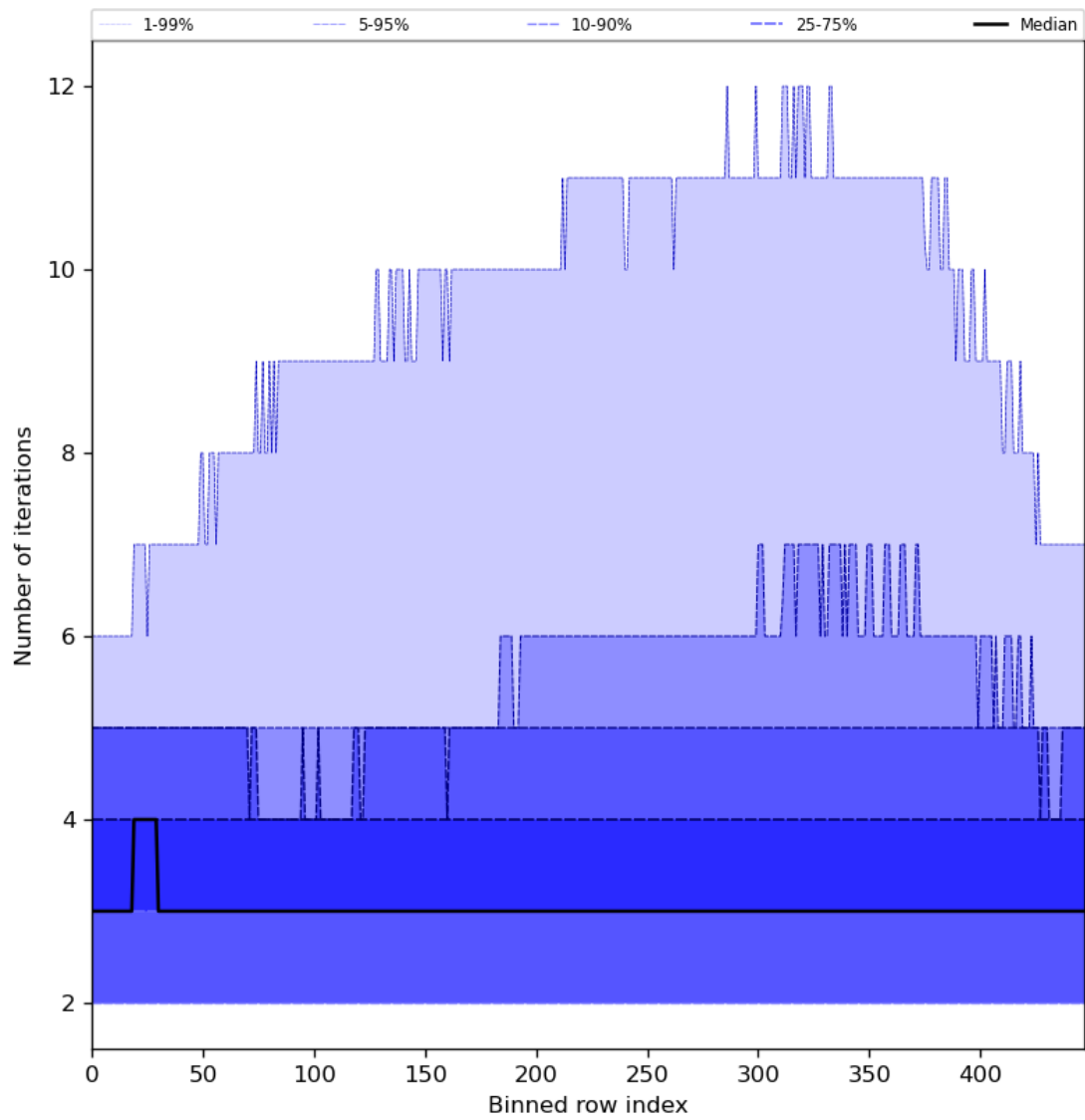
Figure 56: Along track statistics of “Number of iterations” for 2024-08-04 to 2024-08-06
