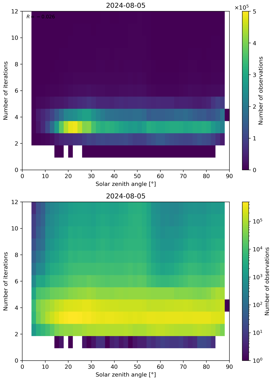
Figure 114: Scatter density plot of “Solar zenith angle” against “Number of iterations” for 2024-08-04 to 2024-08-06.
