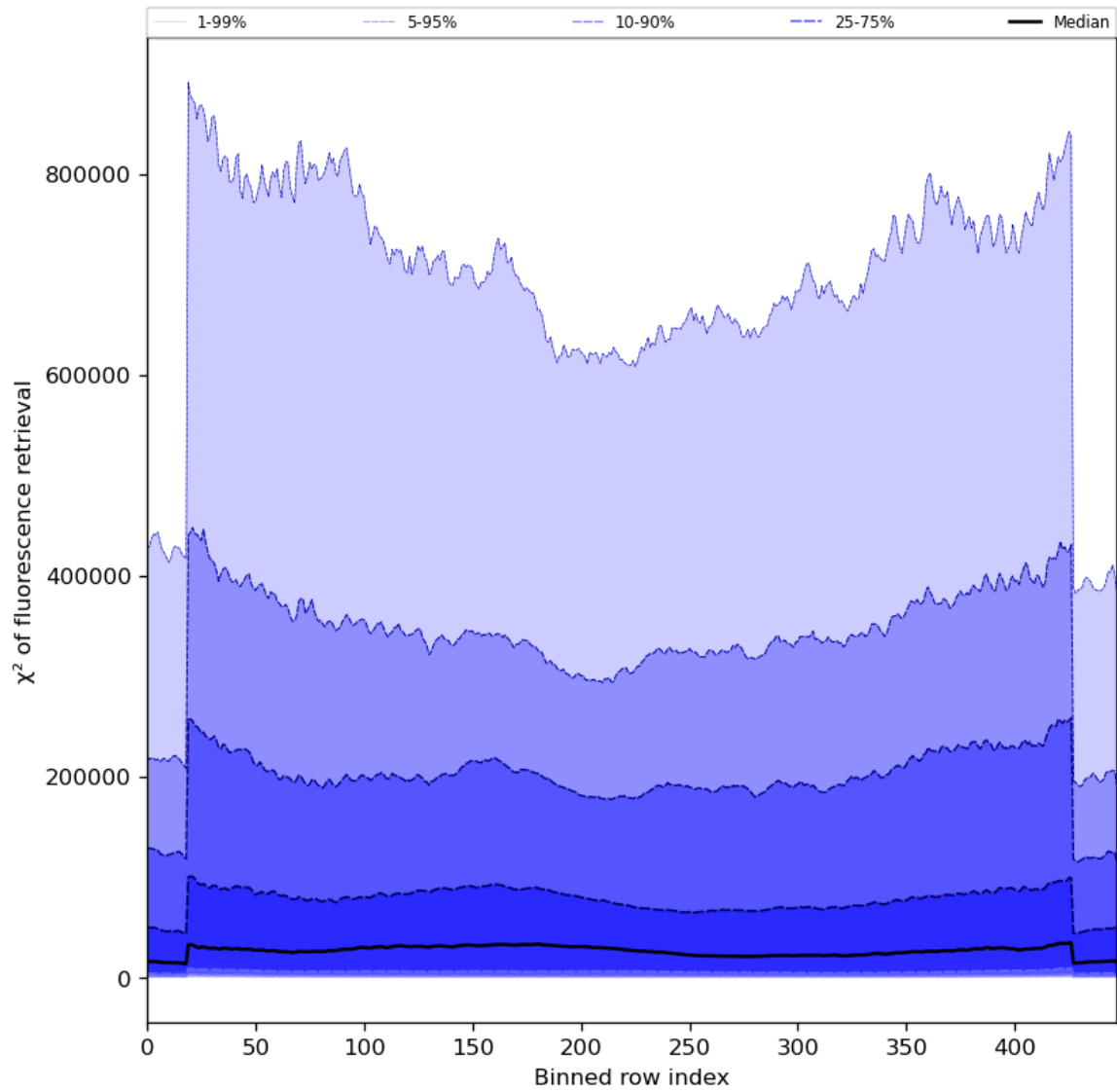
Figure 59: Along track statistics of “ \chi^2 of fluorescence retrieval” for 2024-08-04 to 2024-08-06
