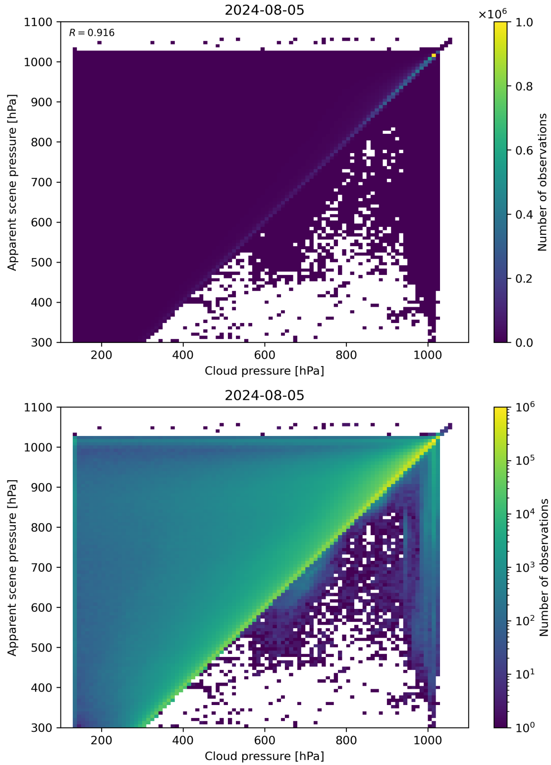
Figure 77: Scatter density plot of “Cloud pressure” against “Apparent scene pressure” for 2024-08-04 to 2024-08-06.
