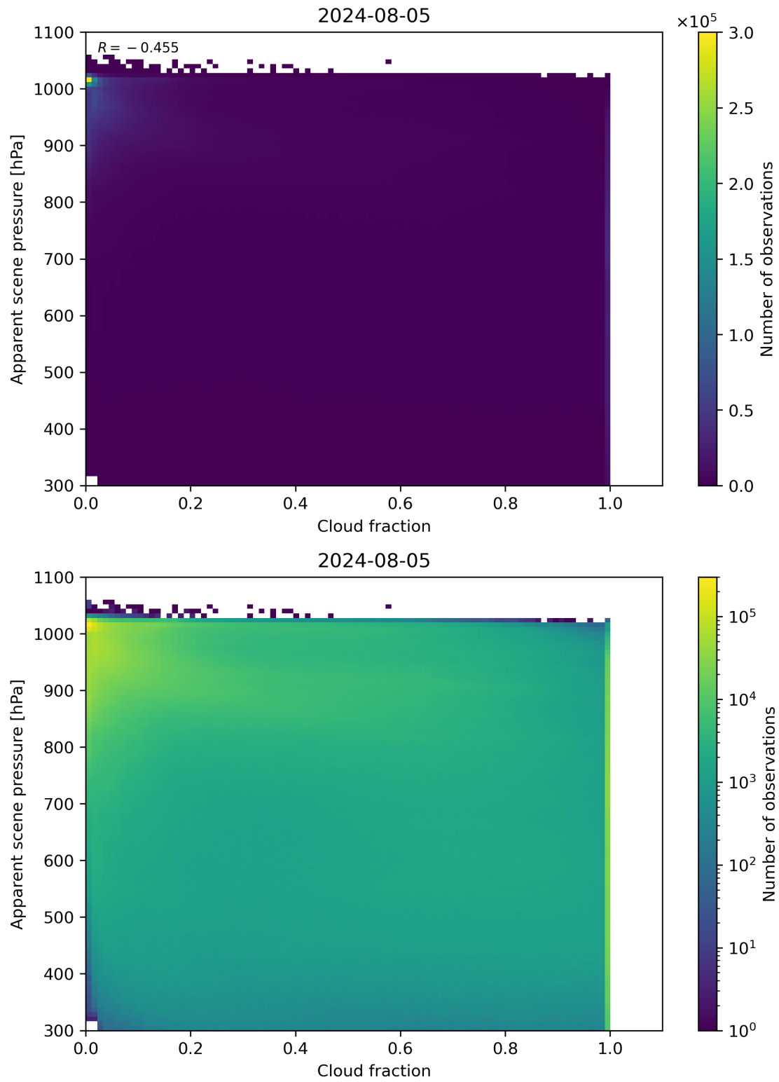
Figure 70: Scatter density plot of “Cloud fraction” against “Apparent scene pressure” for 2024-08-04 to 2024-08-06.
