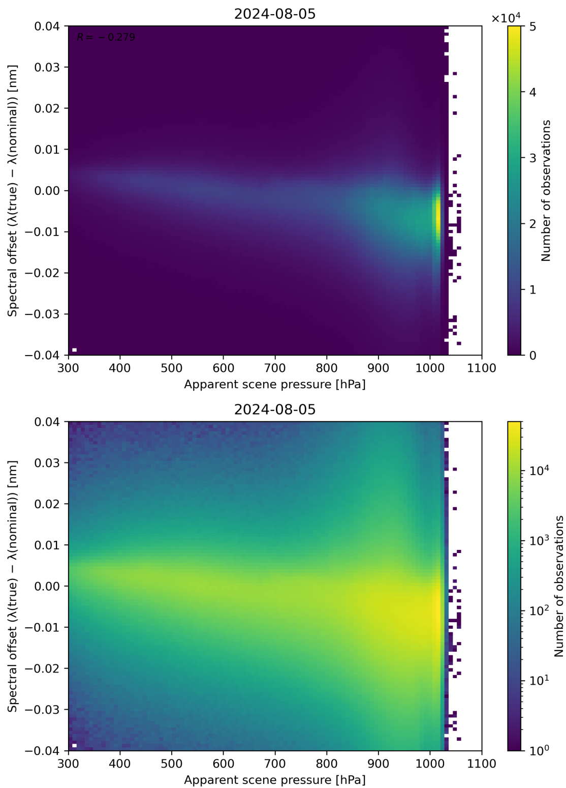
Figure 67: Scatter density plot of “Apparent scene pressure” against “Spectral offset ( \lambda(\text{true}) - \lambda(\text{nominal}) )” for 2024-08-04 to 2024-08-06.
