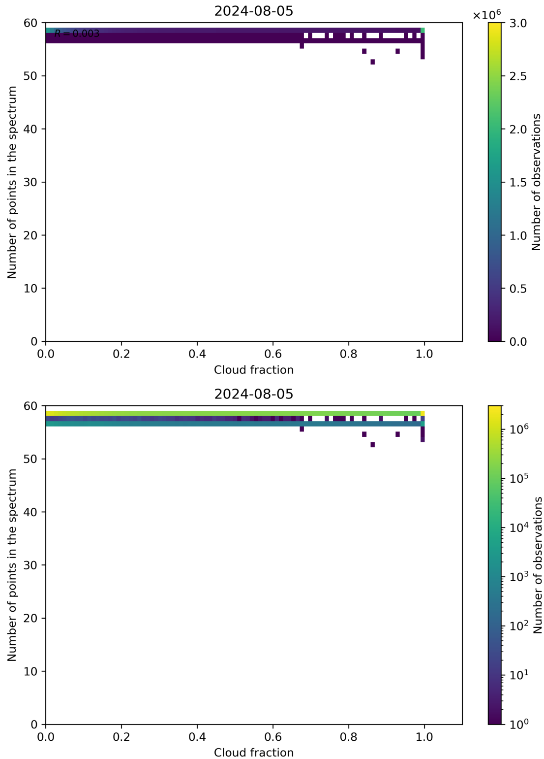
Figure 74: Scatter density plot of “Cloud fraction” against “Number of points in the spectrum” for 2024-08-04 to 2024-08-06.
