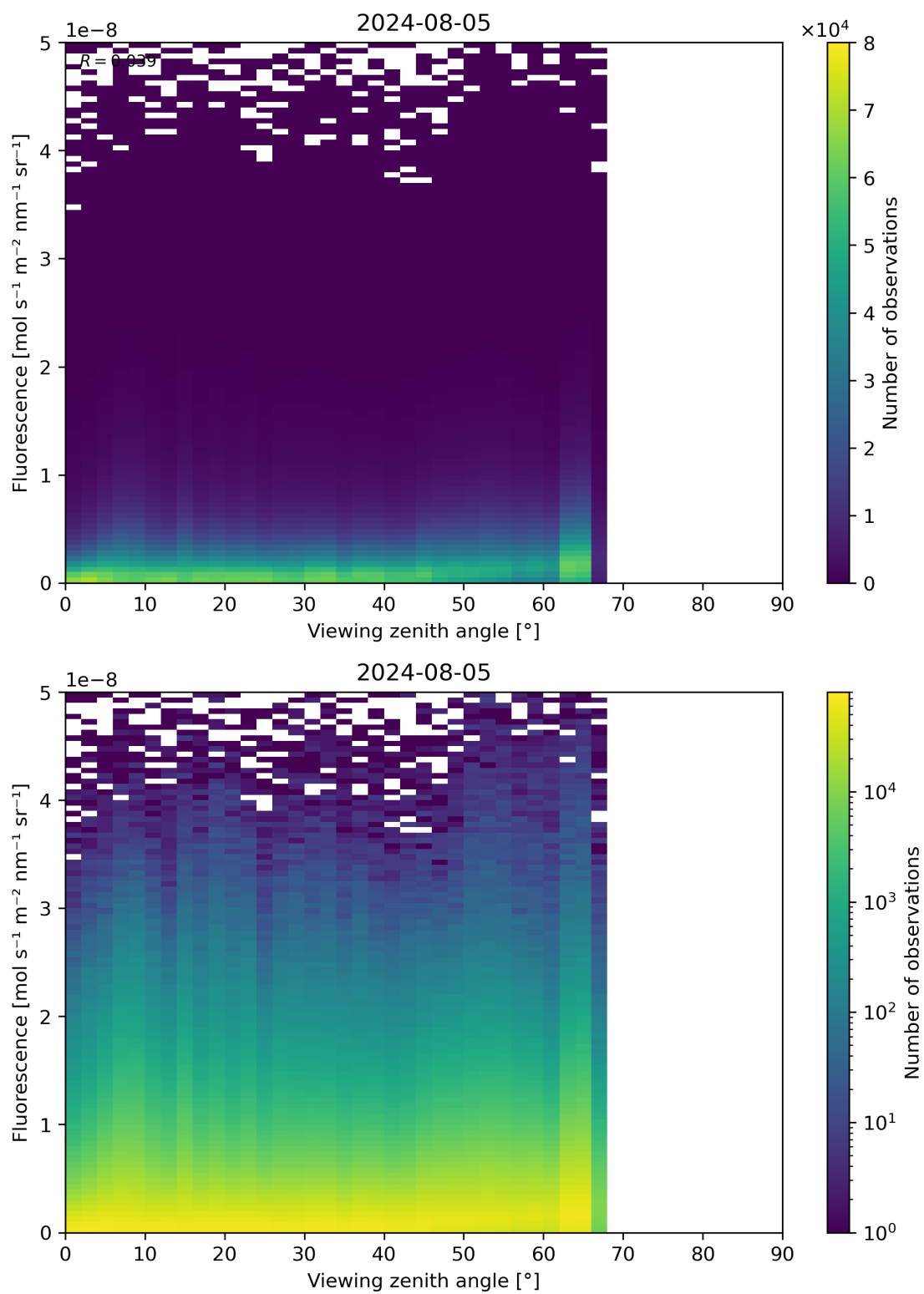
Figure 122: Scatter density plot of “Viewing zenith angle” against “Fluorescence” for 2024-08-04 to 2024-08-06.
