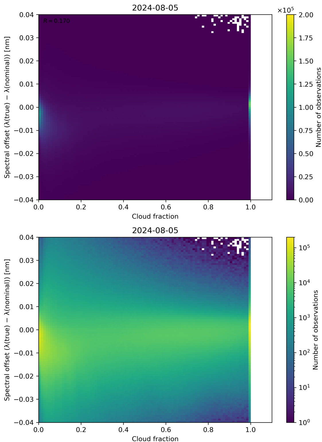
Figure 76: Scatter density plot of “Cloud fraction” against “Spectral offset ( \lambda(\text{true}) - \lambda(\text{nominal}) )” for 2024-08-04 to 2024-08-06.
