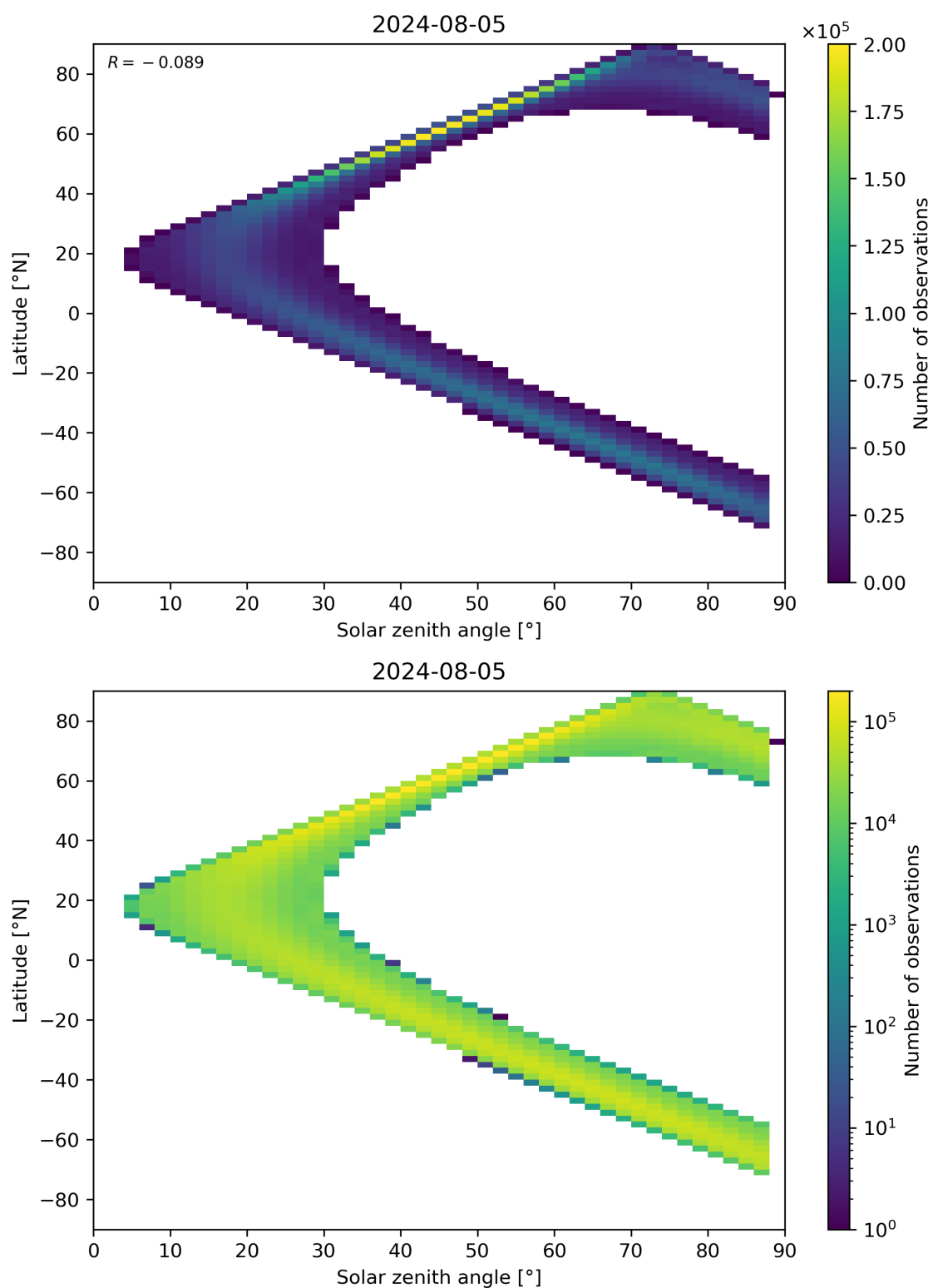
Figure 113: Scatter density plot of “Solar zenith angle” against “Latitude” for 2024-08-04 to 2024-08-06.
