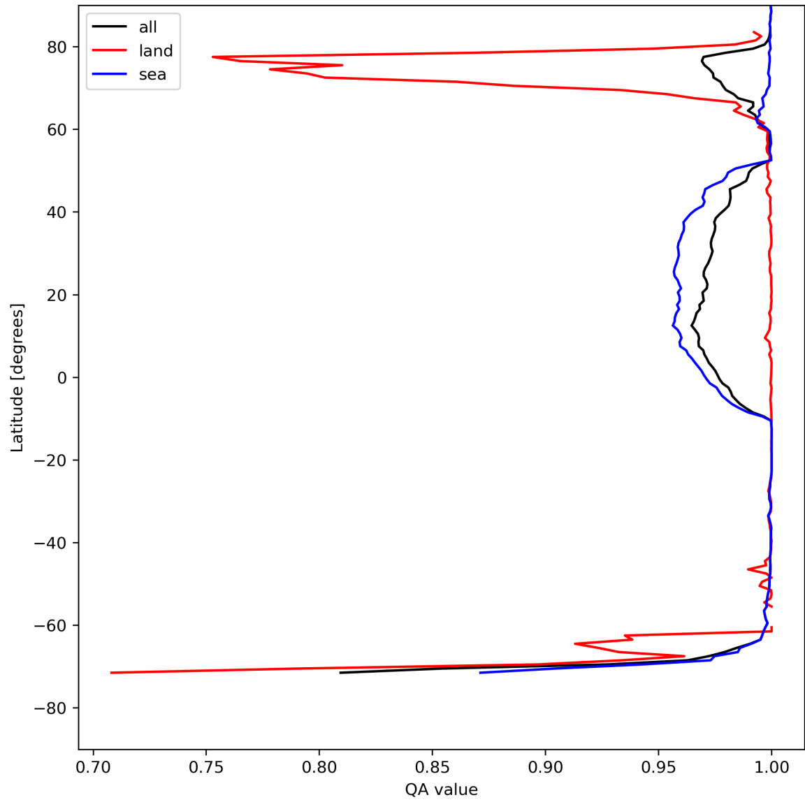
Figure 12: Zonal average of “QA value” for 2024-08-04 to 2024-08-06.
