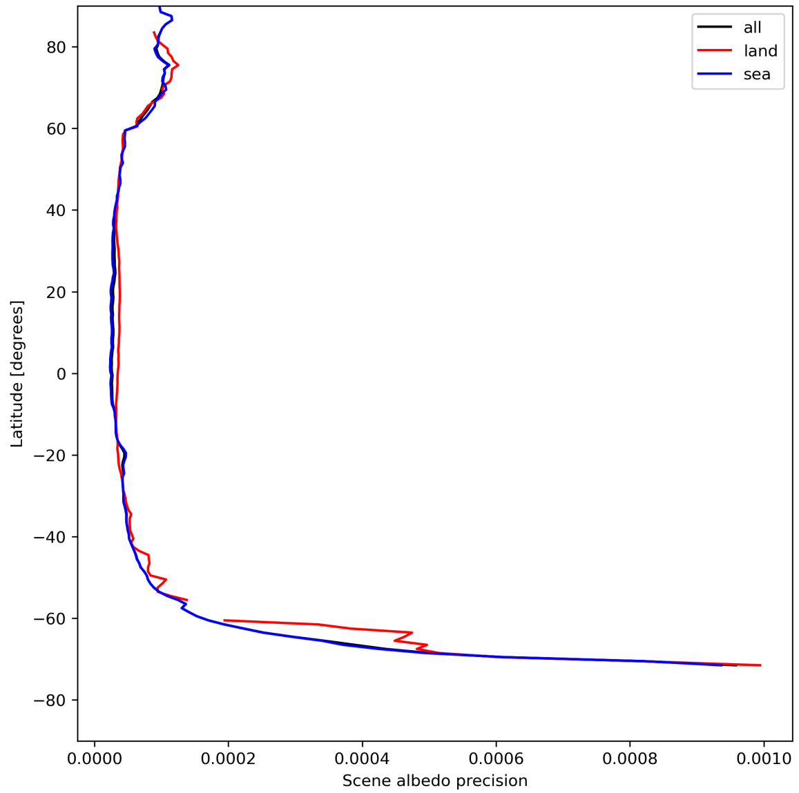
Figure 18: Zonal average of “Scene albedo precision” for 2024-08-04 to 2024-08-06.
