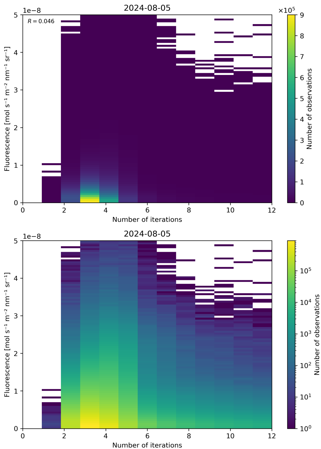
Figure 98: Scatter density plot of “Number of iterations” against “Fluorescence” for 2024-08-04 to 2024-08-06.
