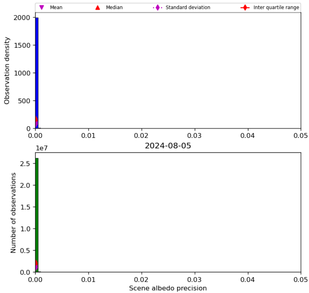
Figure 35: Histogram of “Scene albedo precision” for 2024-08-04 to 2024-08-06
