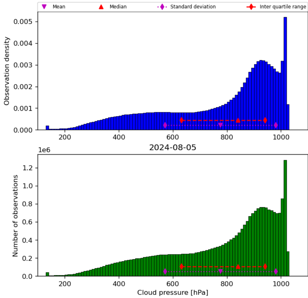
Figure 30: Histogram of “Cloud pressure” for 2024-08-04 to 2024-08-06
