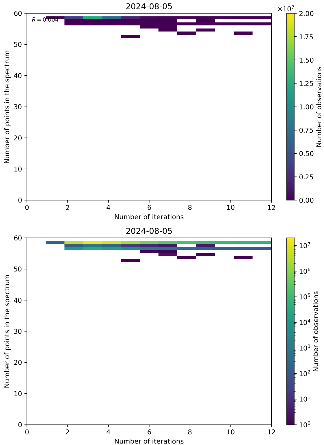
Figure 99: Scatter density plot of “Number of iterations” against “Number of points in the spectrum” for 2024-08-04 to 2024-08-06.
