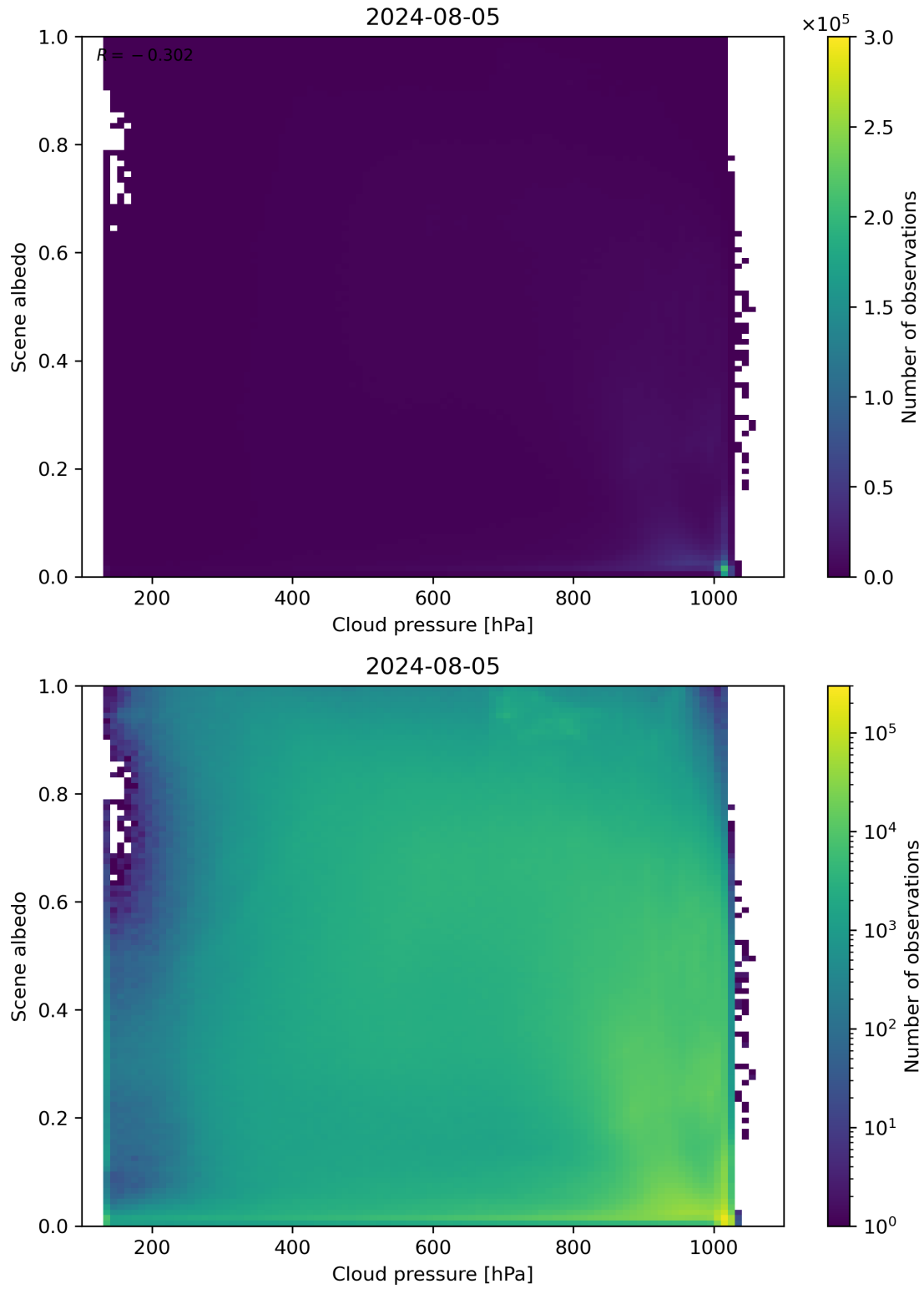
Figure 83: Scatter density plot of “Cloud pressure” against “Scene albedo” for 2024-08-04 to 2024-08-06.
