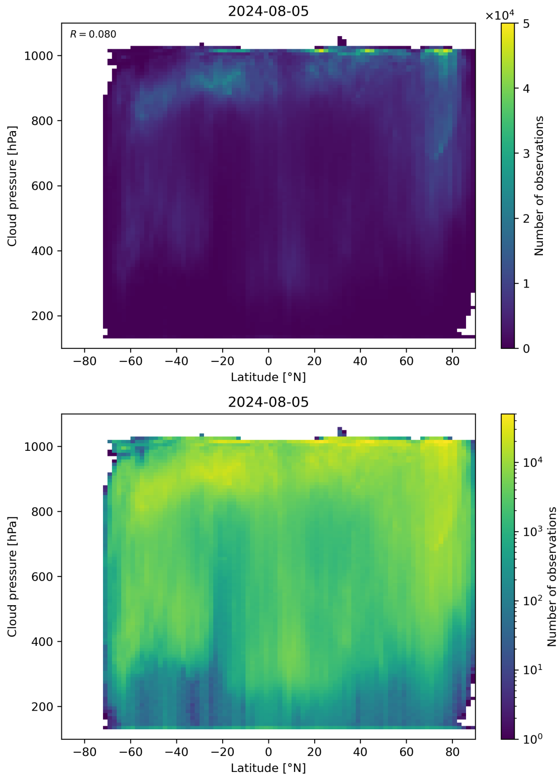
Figure 91: Scatter density plot of “Latitude” against “Cloud pressure” for 2024-08-04 to 2024-08-06.
