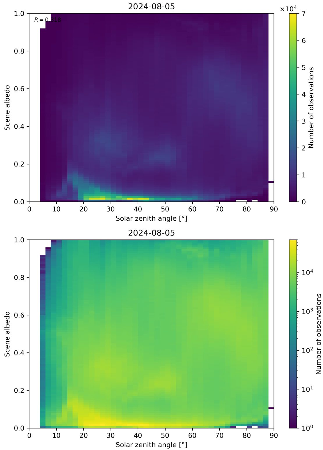
Figure 116: Scatter density plot of “Solar zenith angle” against “Scene albedo” for 2024-08-04 to 2024-08-06.
