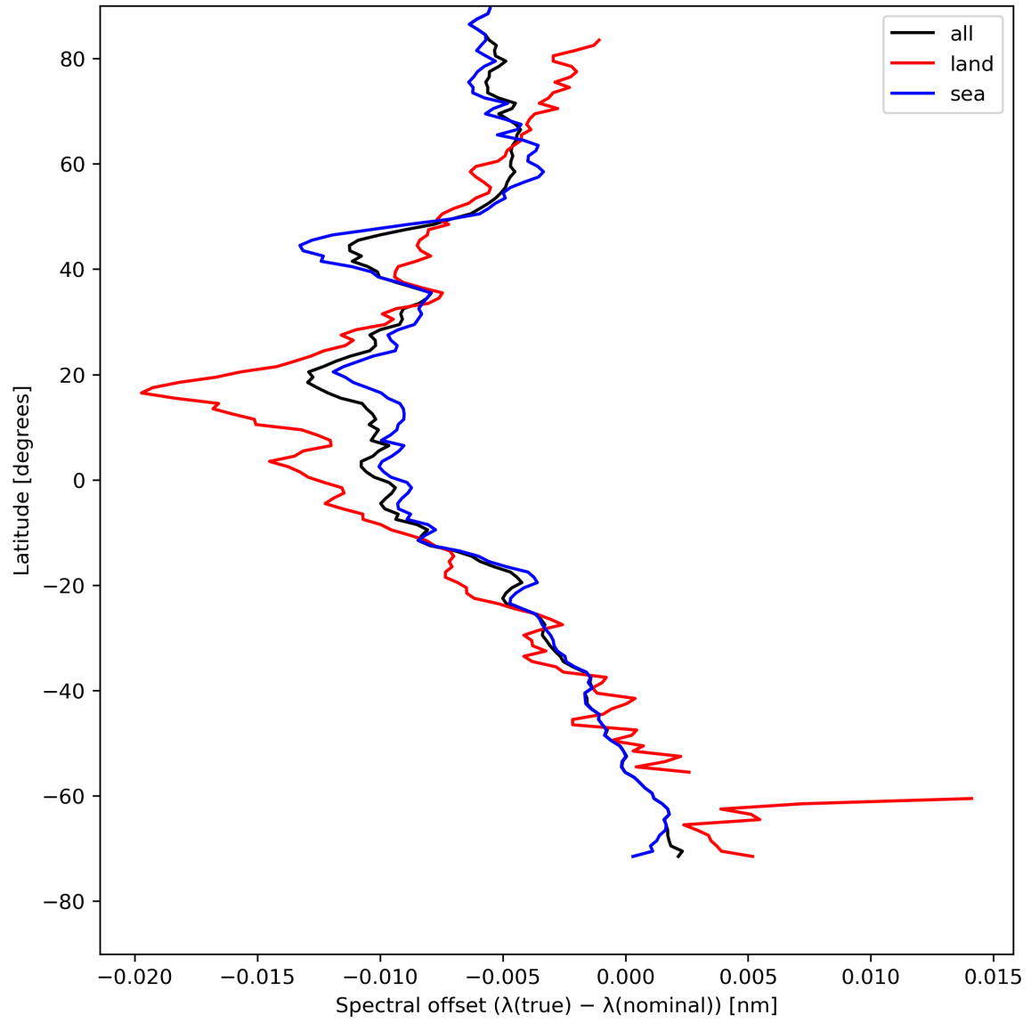
Figure 28: Zonal average of “Spectral offset ( \lambda(\text{true}) - \lambda(\text{nominal}) )” for 2024-08-04 to 2024-08-06.
