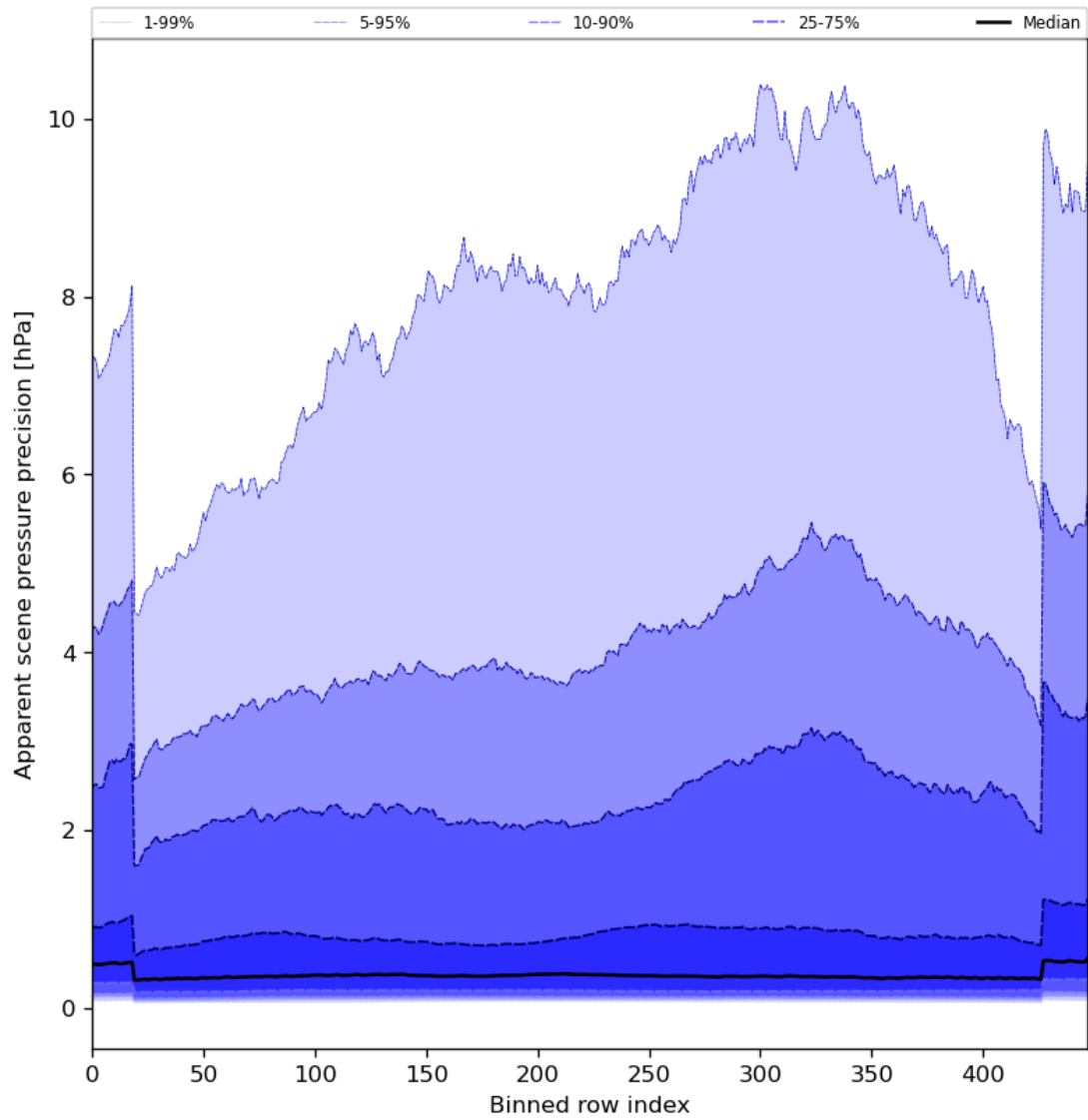
Figure 54: Along track statistics of “Apparent scene pressure precision” for 2024-08-04 to 2024-08-06
