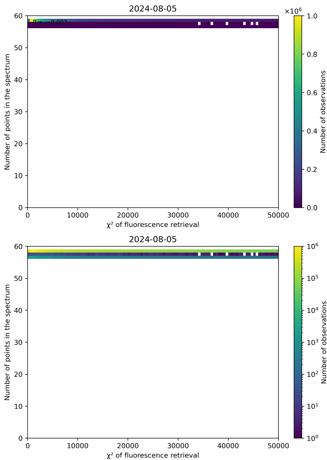
Figure 68: Scatter density plot of " \chi^2 of fluorescence retrieval" against "Number of points in the spectrum" for 2024-08-04 to 2024-08-06.
