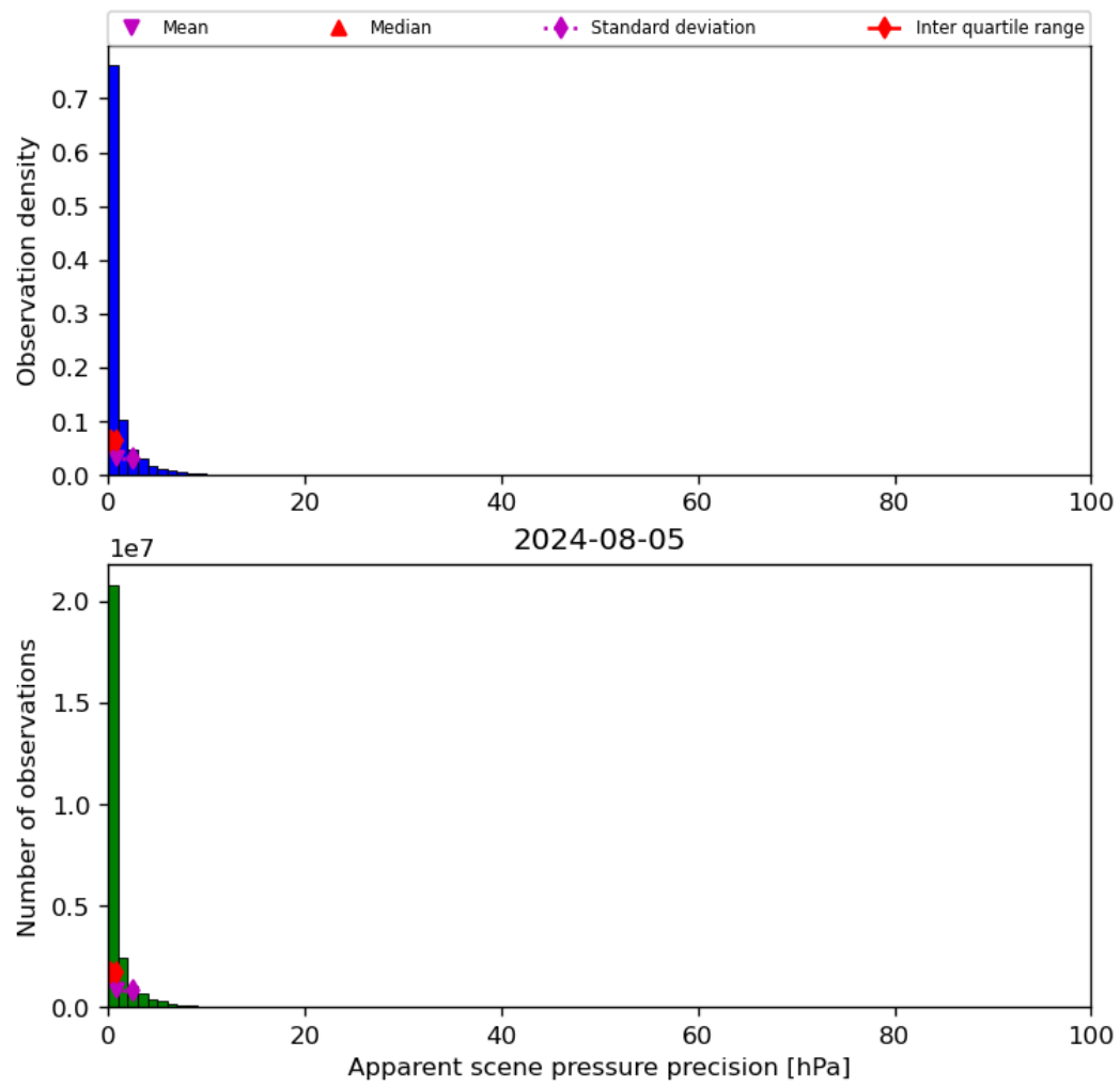
Figure 37: Histogram of “Apparent scene pressure precision” for 2024-08-04 to 2024-08-06
