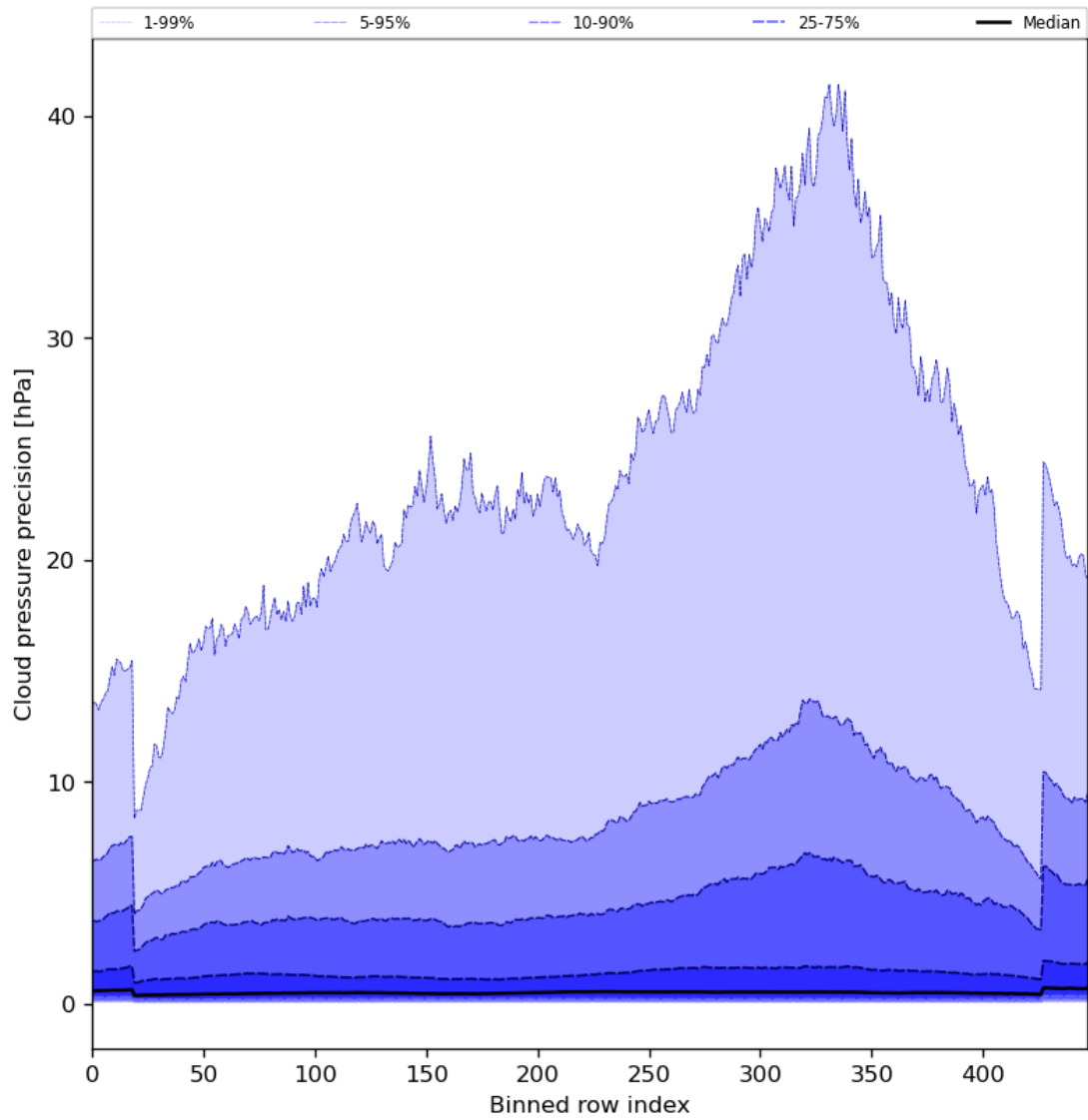
Figure 48: Along track statistics of “Cloud pressure precision” for 2024-08-04 to 2024-08-06
