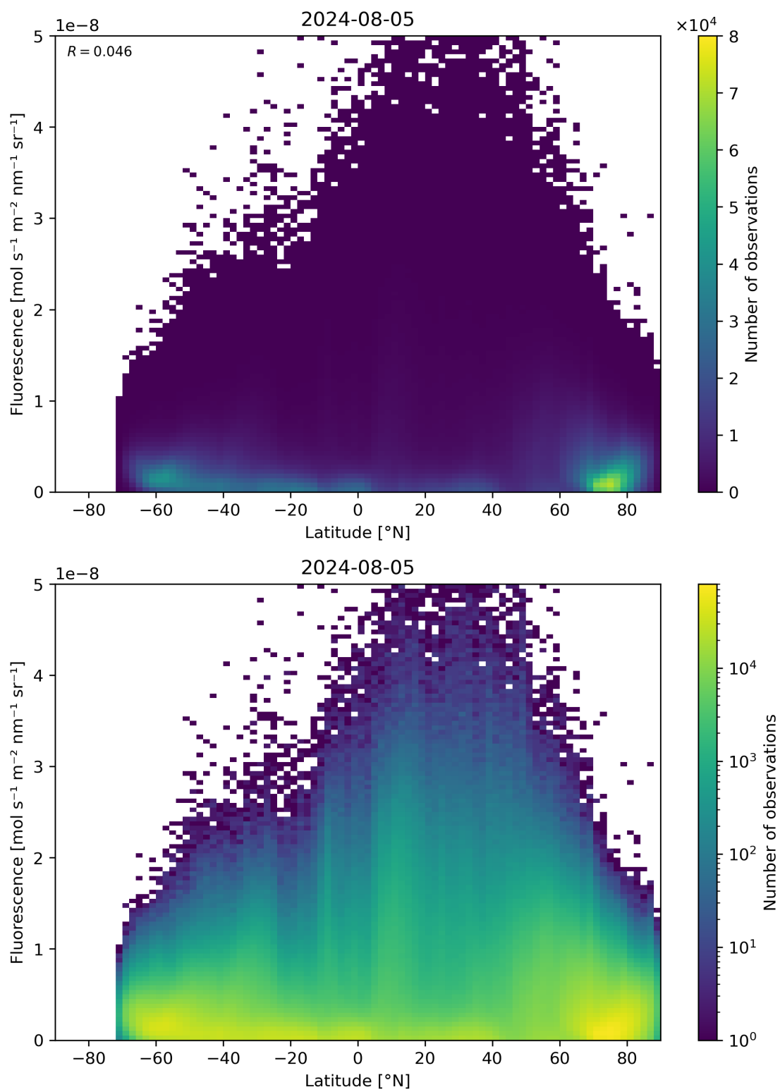
Figure 92: Scatter density plot of “Latitude” against “Fluorescence” for 2024-08-04 to 2024-08-06.
