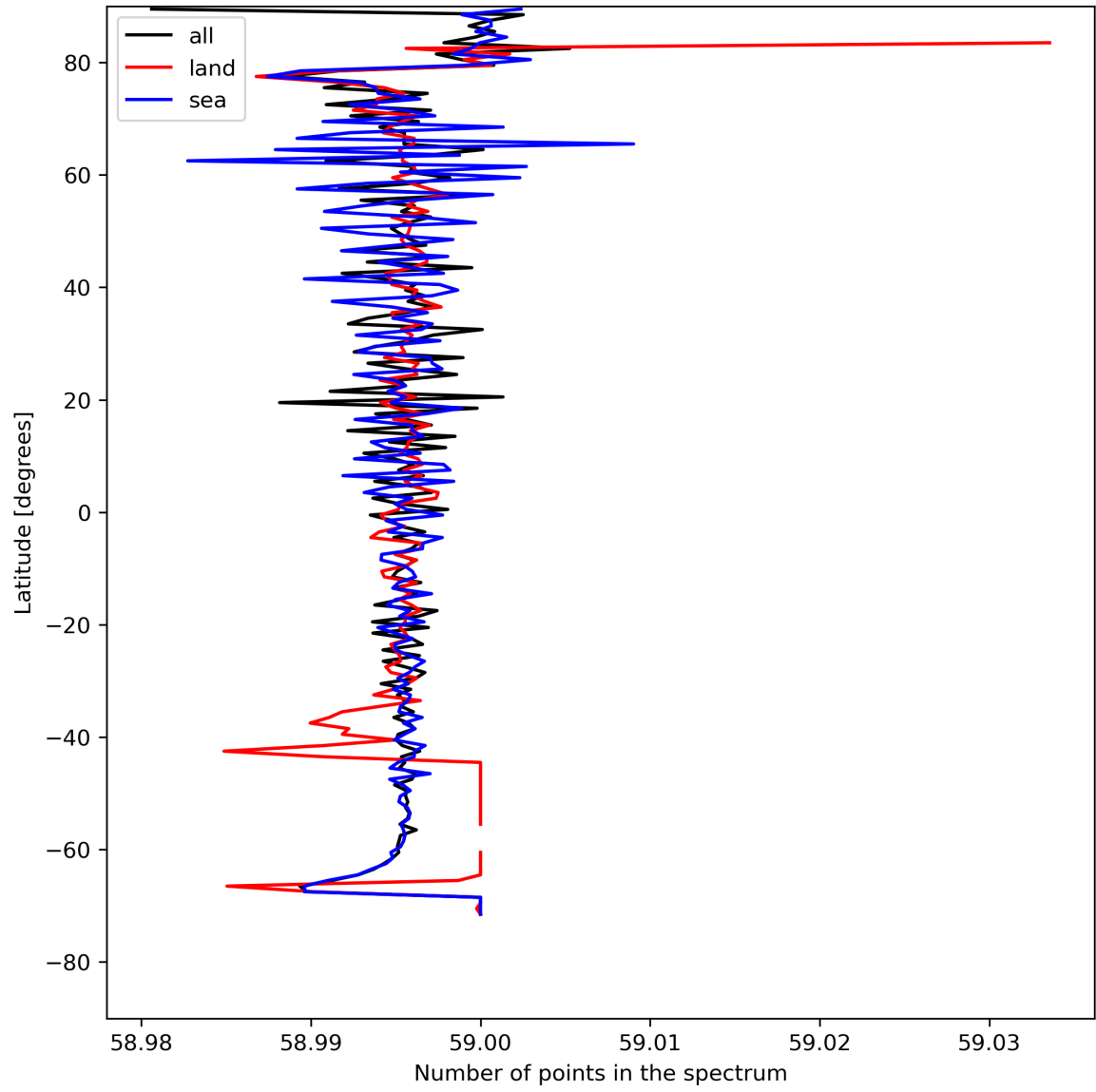
Figure 27: Zonal average of “Number of points in the spectrum” for 2024-08-04 to 2024-08-06.
