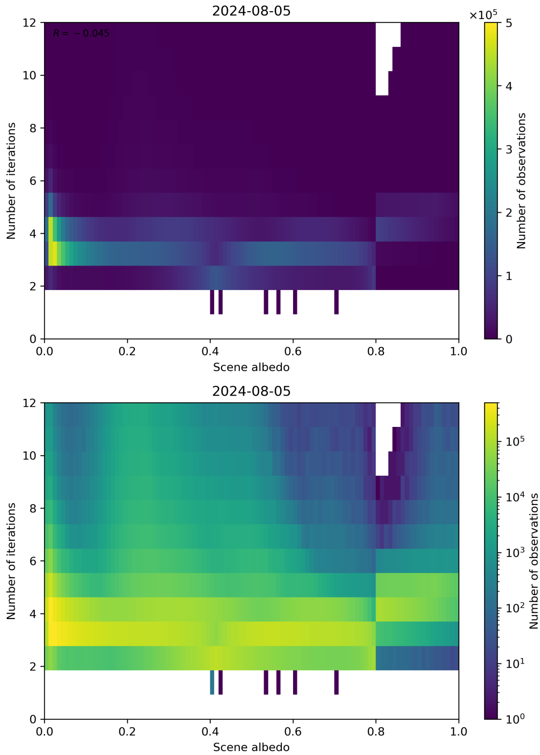
Figure 105: Scatter density plot of “Scene albedo” against “Number of iterations” for 2024-08-04 to 2024-08-06.
