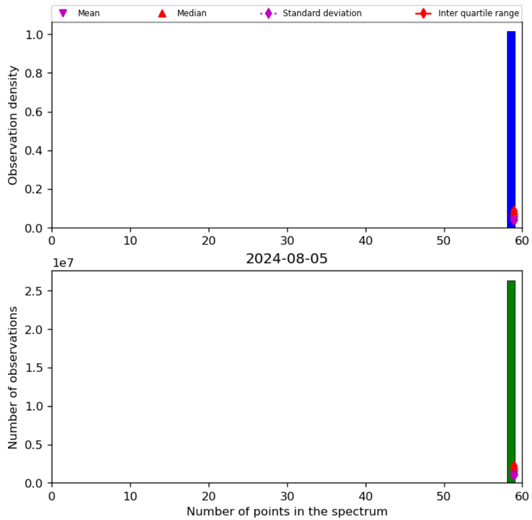
Figure 44: Histogram of "Number of points in the spectrum" for 2024-08-04 to 2024-08-06
