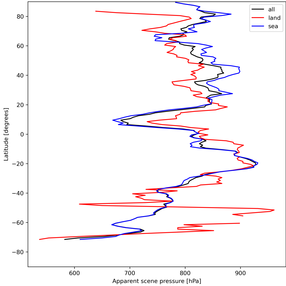
Figure 19: Zonal average of “Apparent scene pressure” for 2024-08-04 to 2024-08-06.
