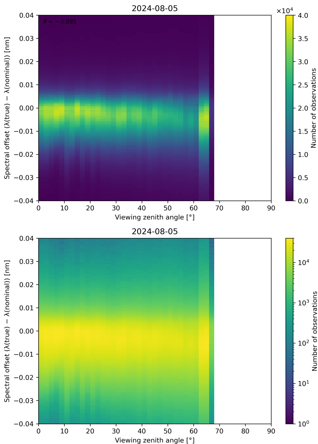
Figure 128: Scatter density plot of “Viewing zenith angle” against “Spectral offset ( \lambda(\text{true}) - \lambda(\text{nominal}) )” for 2024-08-04 to 2024-08-06.
