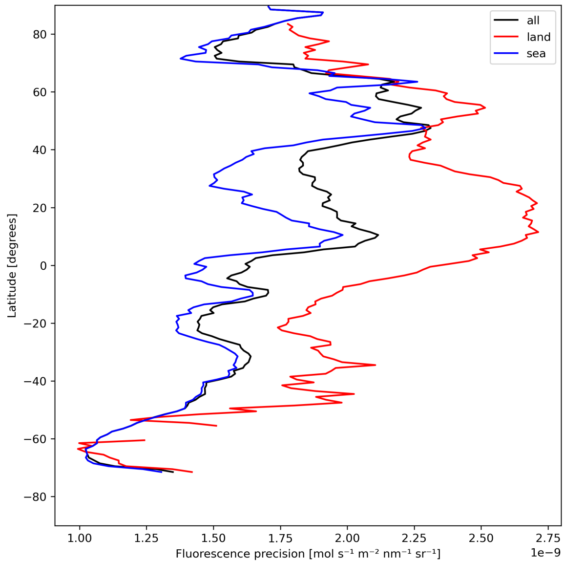
Figure 24: Zonal average of “Fluorescence precision” for 2024-08-04 to 2024-08-06.
