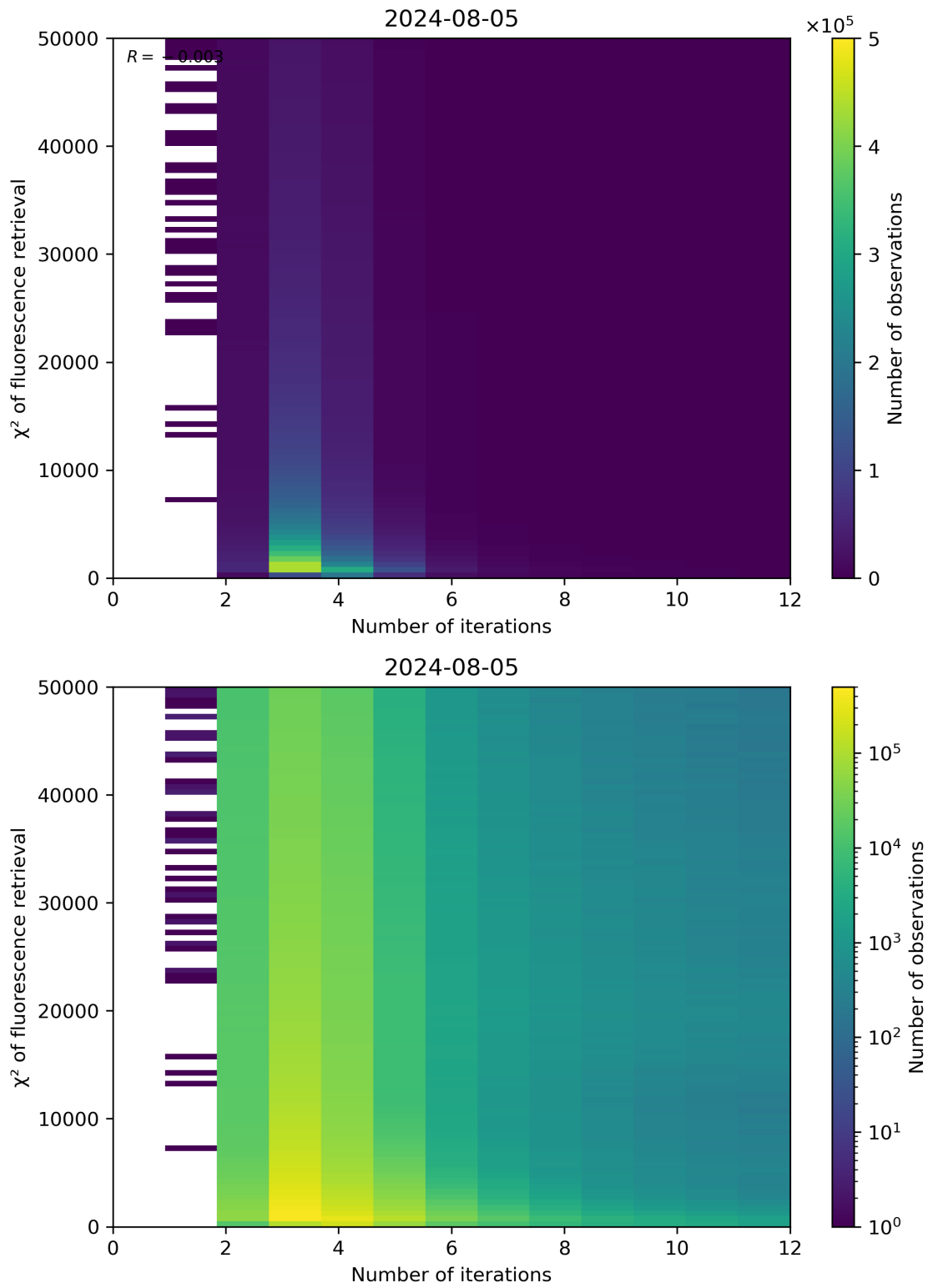
Figure 97: Scatter density plot of “Number of iterations” against “ \chi^2 of fluorescence retrieval” for 2024-08-04 to 2024-08-06.
