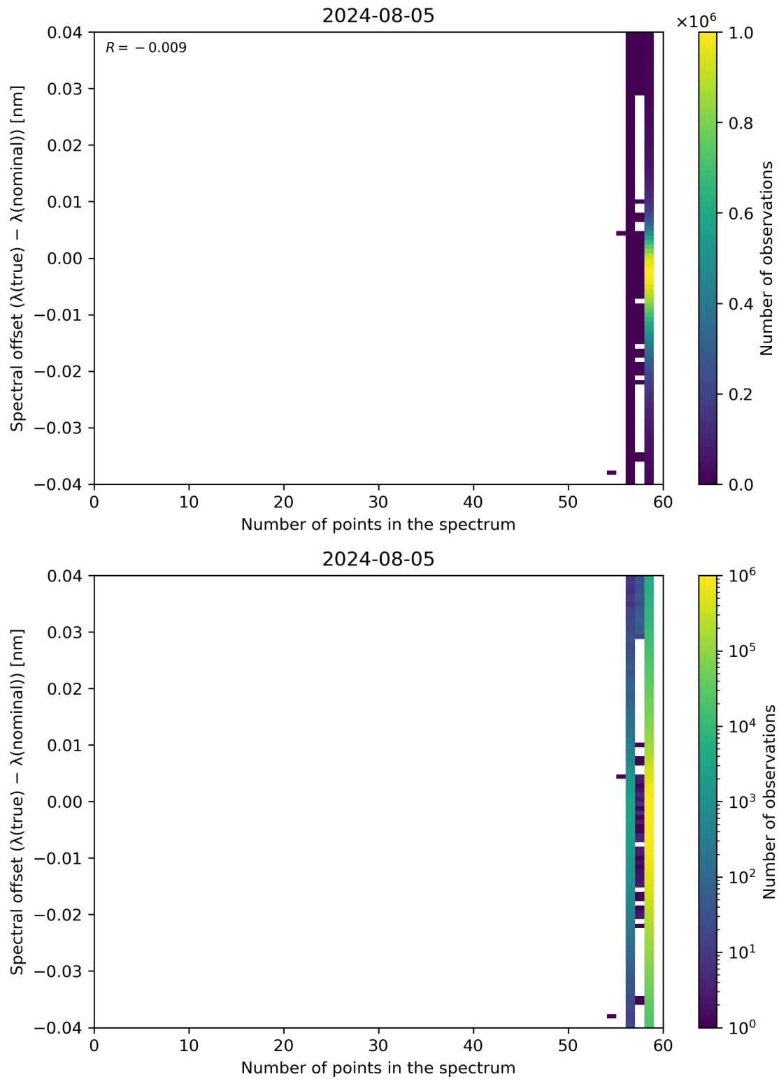
Figure 101: Scatter density plot of “Number of points in the spectrum” against “Spectral offset ( \lambda(\text{true}) - \lambda(\text{nominal}) )” for 2024-08-04 to 2024-08-06.
