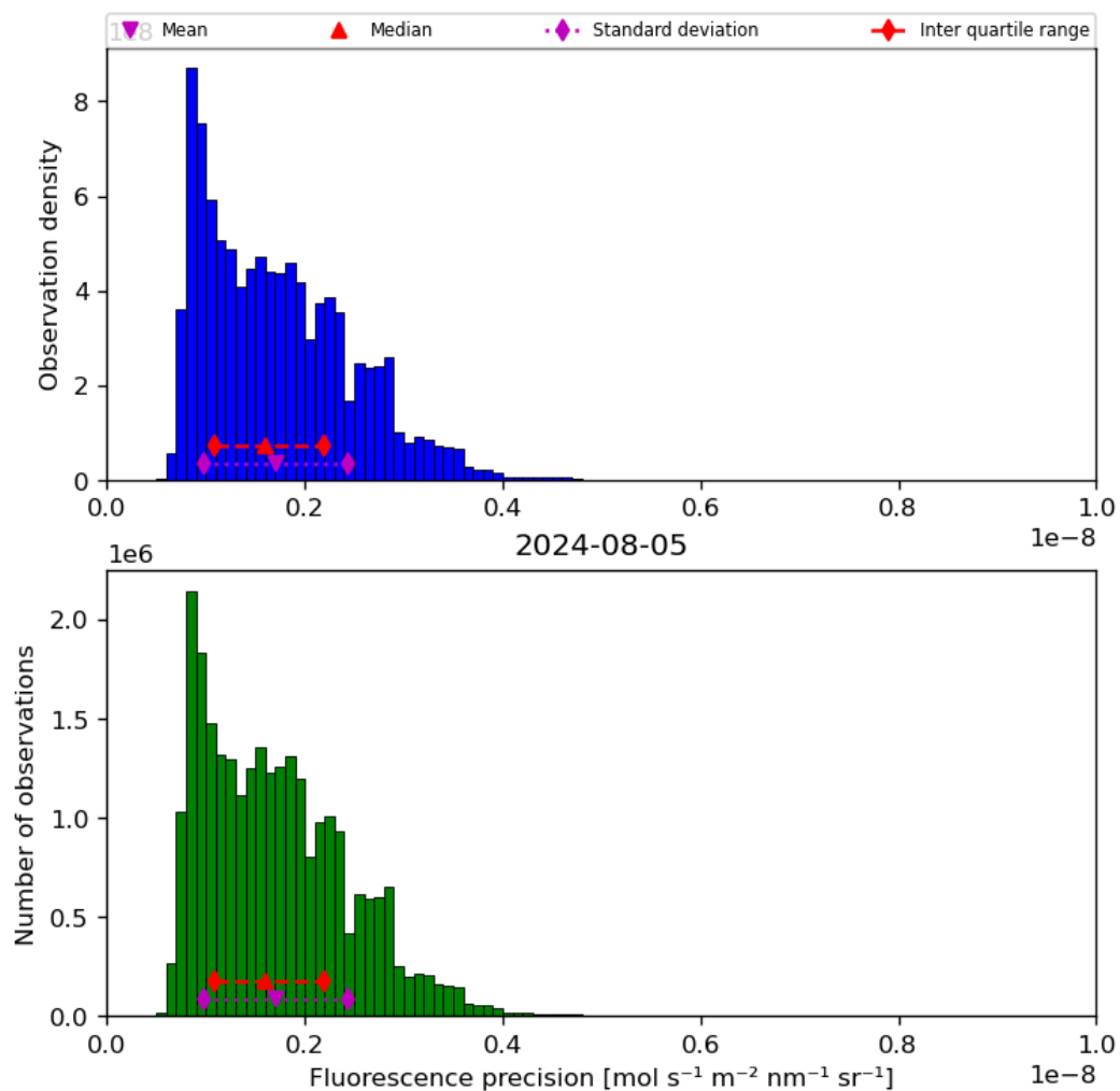
Figure 41: Histogram of “Fluorescence precision” for 2024-08-04 to 2024-08-06
