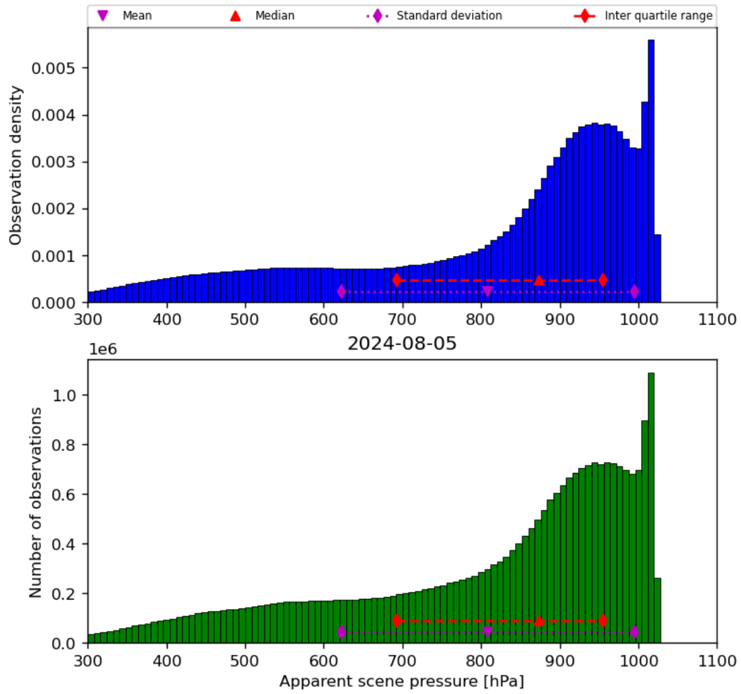
Figure 36: Histogram of “Apparent scene pressure” for 2024-08-04 to 2024-08-06
