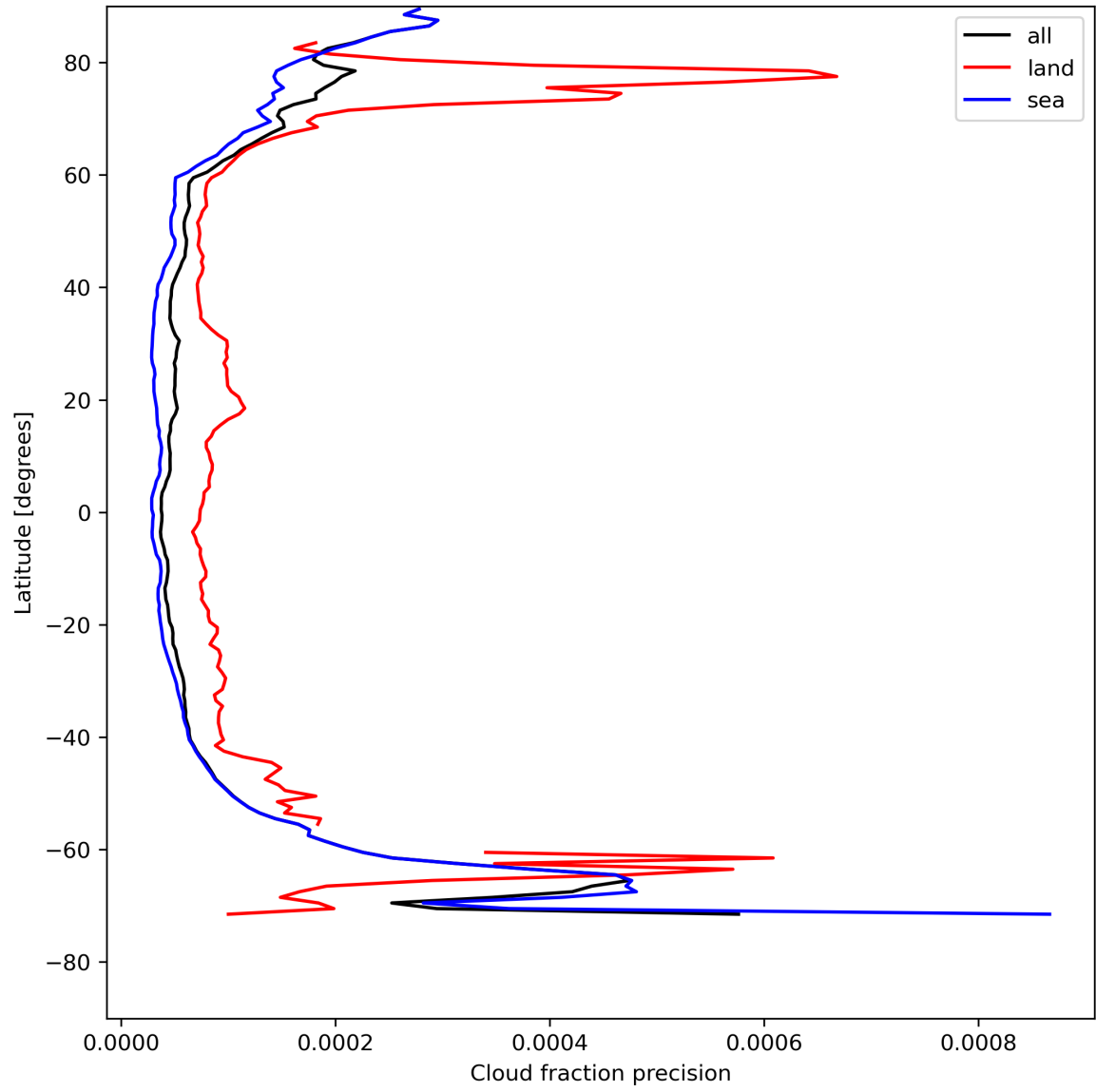
Figure 16: Zonal average of “Cloud fraction precision” for 2024-08-04 to 2024-08-06.
