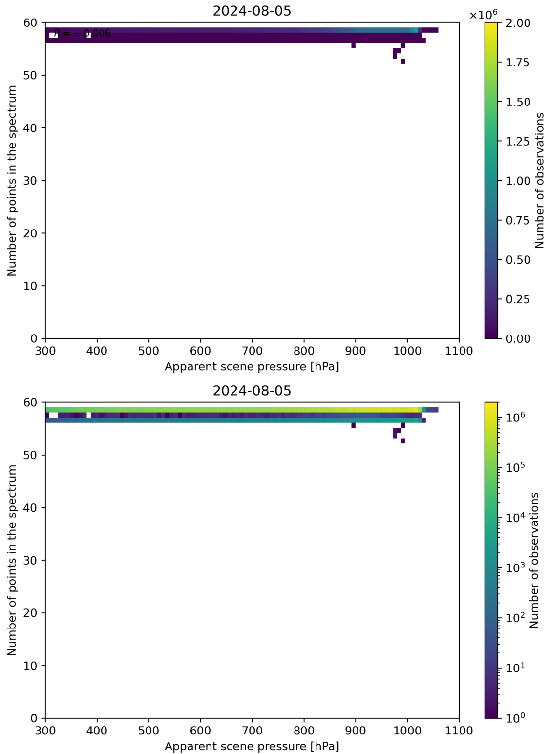
Figure 66: Scatter density plot of “Apparent scene pressure” against “Number of points in the spectrum” for 2024-08-04 to 2024-08-06.
