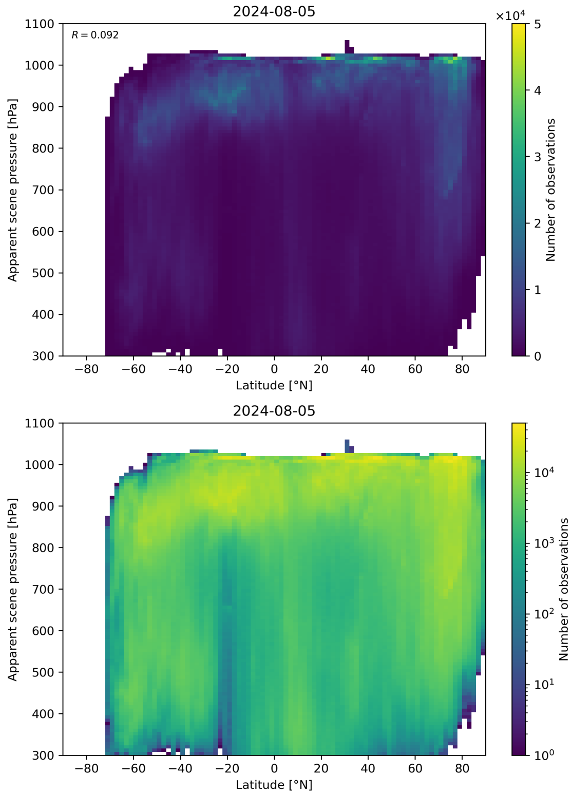
Figure 88: Scatter density plot of “Latitude” against “Apparent scene pressure” for 2024-08-04 to 2024-08-06.
