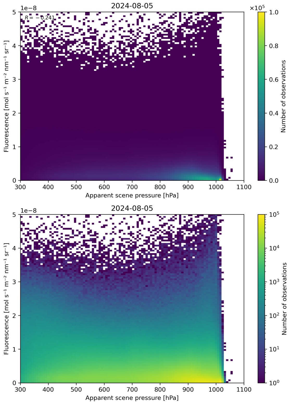
Figure 64: Scatter density plot of “Apparent scene pressure” against “Fluorescence” for 2024-08-04 to 2024-08-06.
