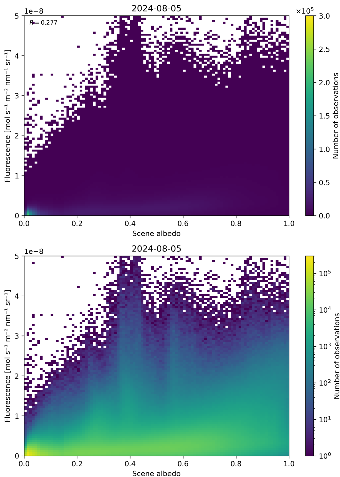
Figure 104: Scatter density plot of “Scene albedo” against “Fluorescence” for 2024-08-04 to 2024-08-06.
