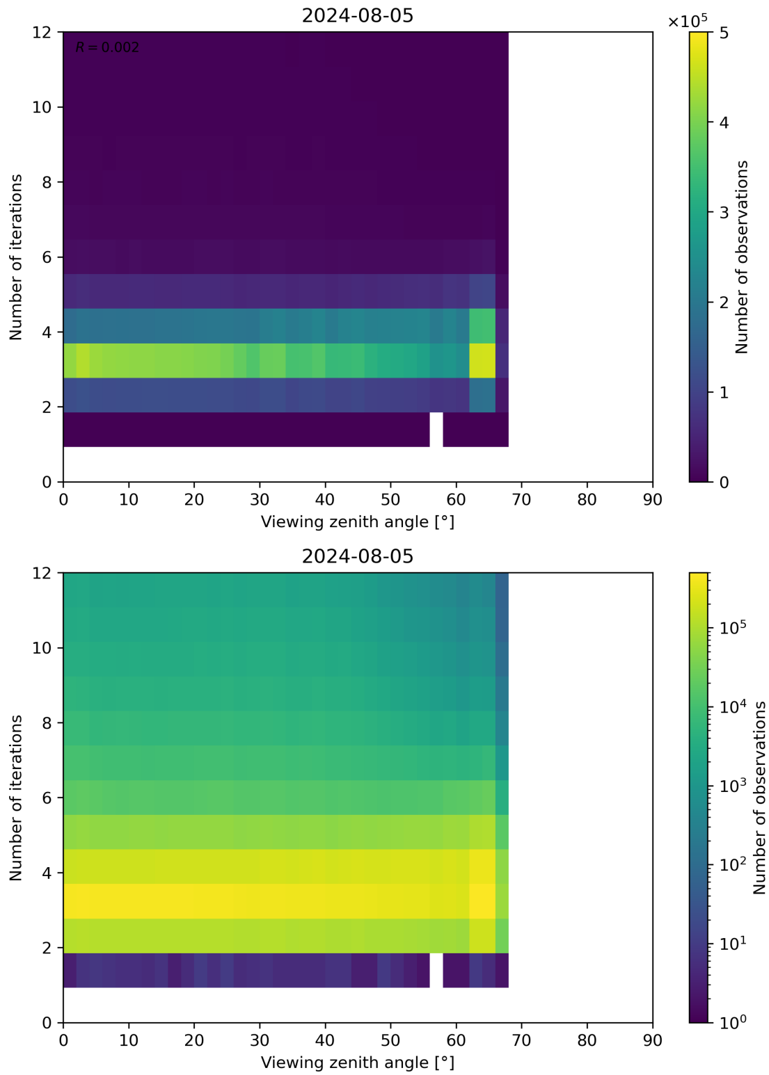
Figure 124: Scatter density plot of “Viewing zenith angle” against “Number of iterations” for 2024-08-04 to 2024-08-06.
