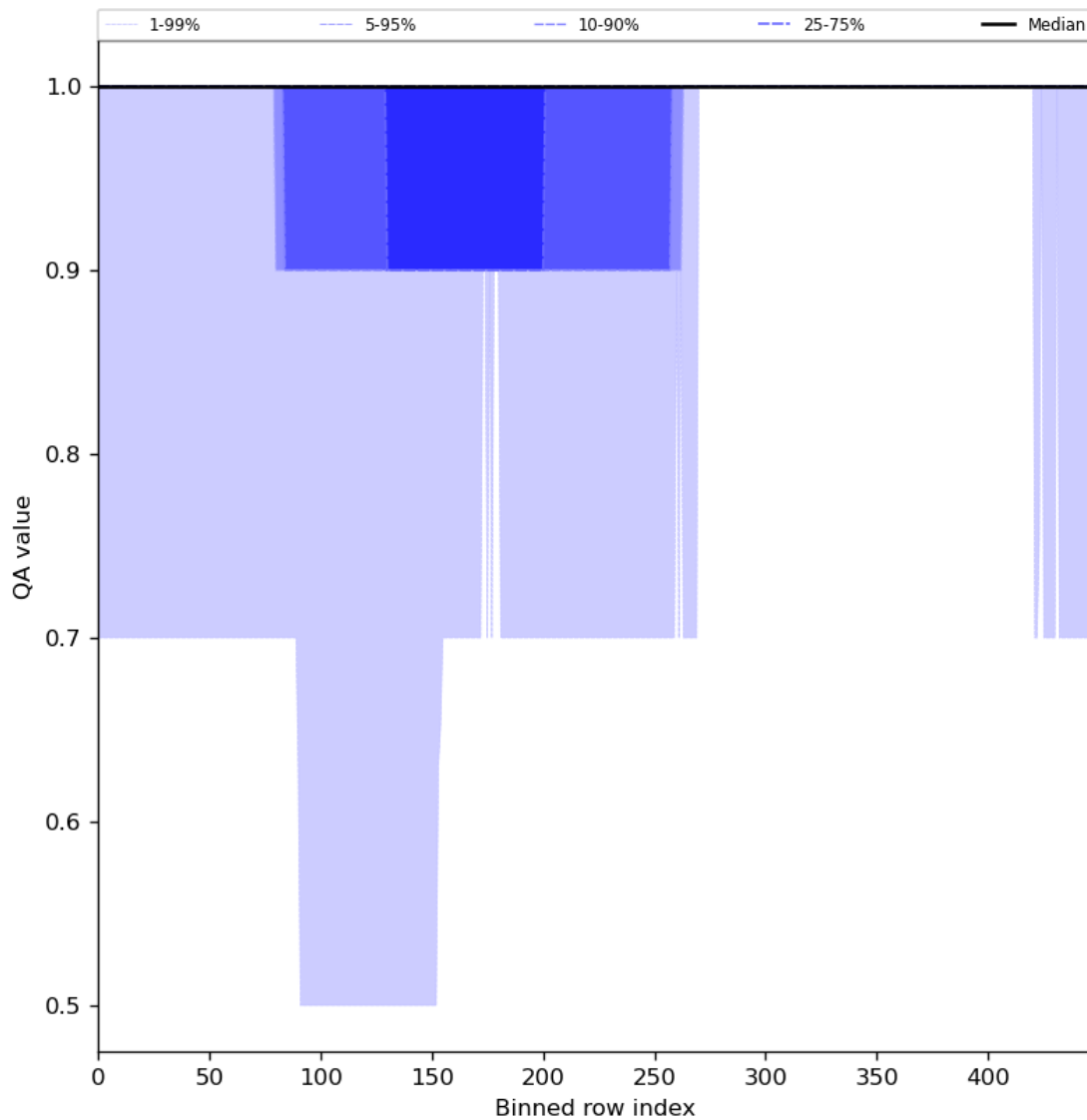
Figure 46: Along track statistics of “QA value” for 2024-08-04 to 2024-08-06
