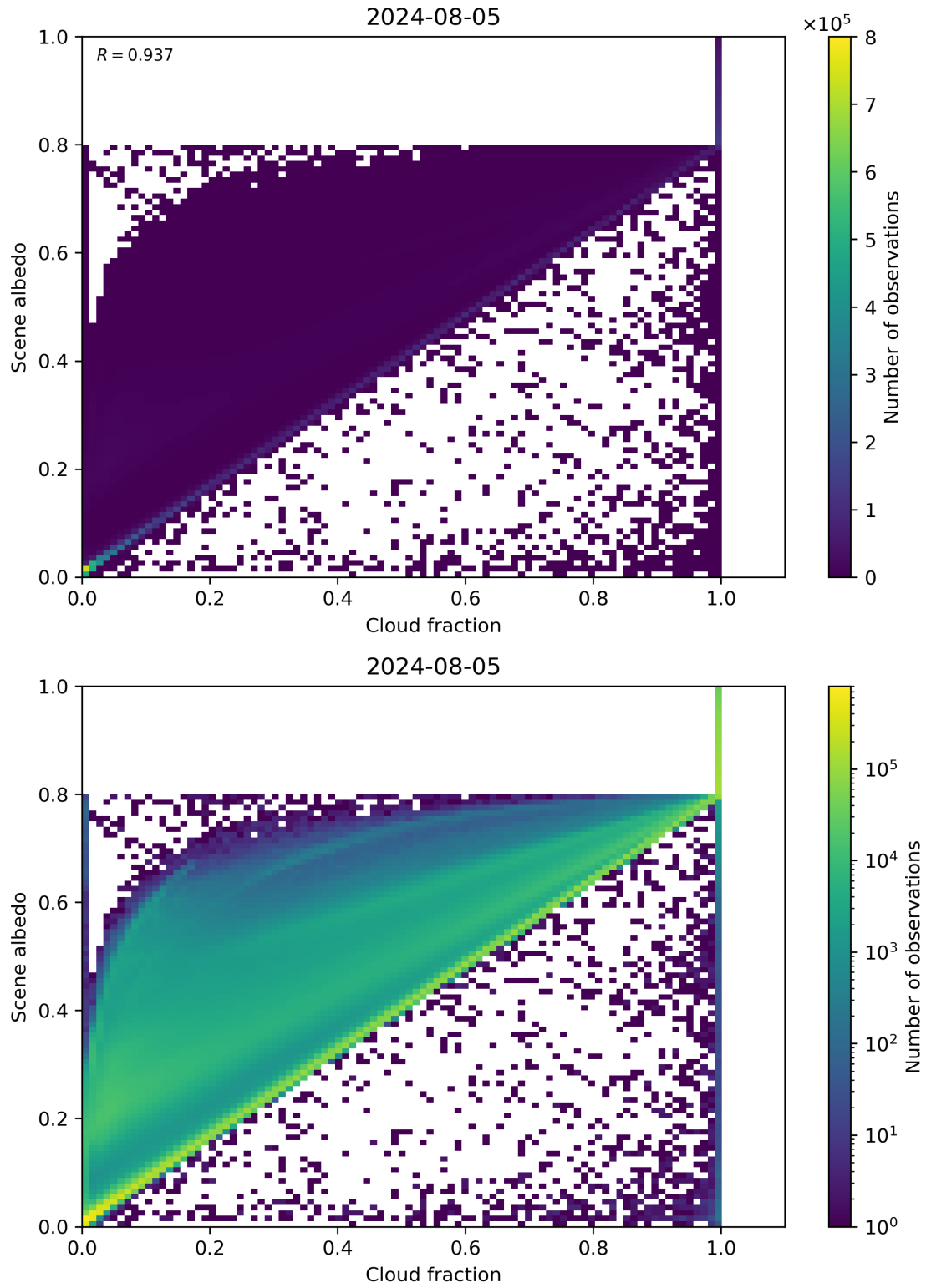
Figure 75: Scatter density plot of “Cloud fraction” against “Scene albedo” for 2024-08-04 to 2024-08-06.
