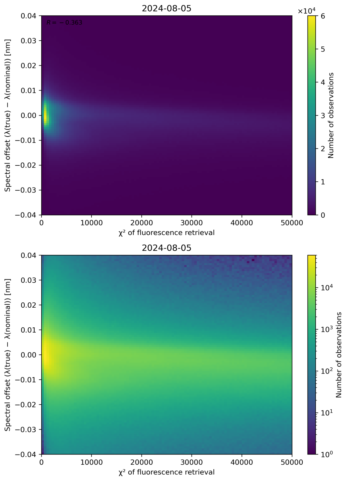
Figure 69: Scatter density plot of " \chi^2 of fluorescence retrieval" against "Spectral offset ( \lambda(\text{true}) - \lambda(\text{nominal}) )" for 2024-08-04 to 2024-08-06.
