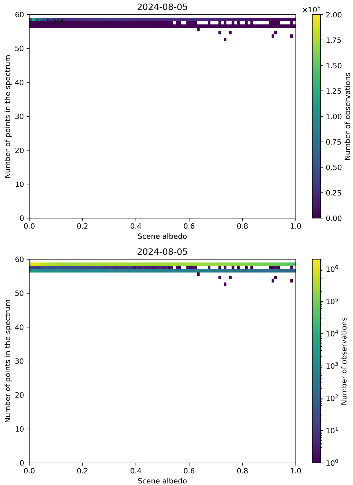
Figure 106: Scatter density plot of “Scene albedo” against “Number of points in the spectrum” for 2024-08-04 to 2024-08-06.
