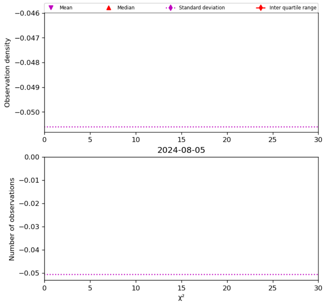
Figure 38: Histogram of “ \chi^2 ” for 2024-08-04 to 2024-08-06
