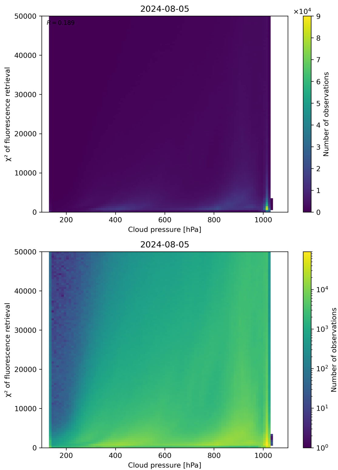
Figure 78: Scatter density plot of “Cloud pressure” against “ \chi^2 of fluorescence retrieval” for 2024-08-04 to 2024-08-06.
