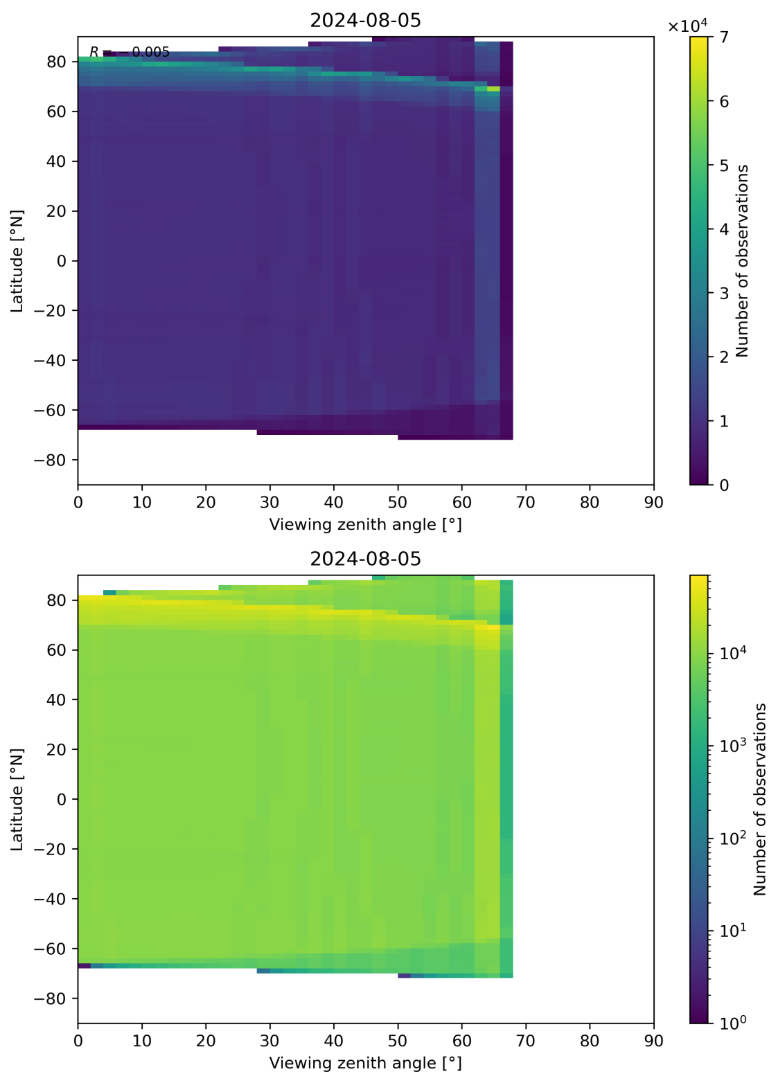
Figure 123: Scatter density plot of “Viewing zenith angle” against “Latitude” for 2024-08-04 to 2024-08-06.
