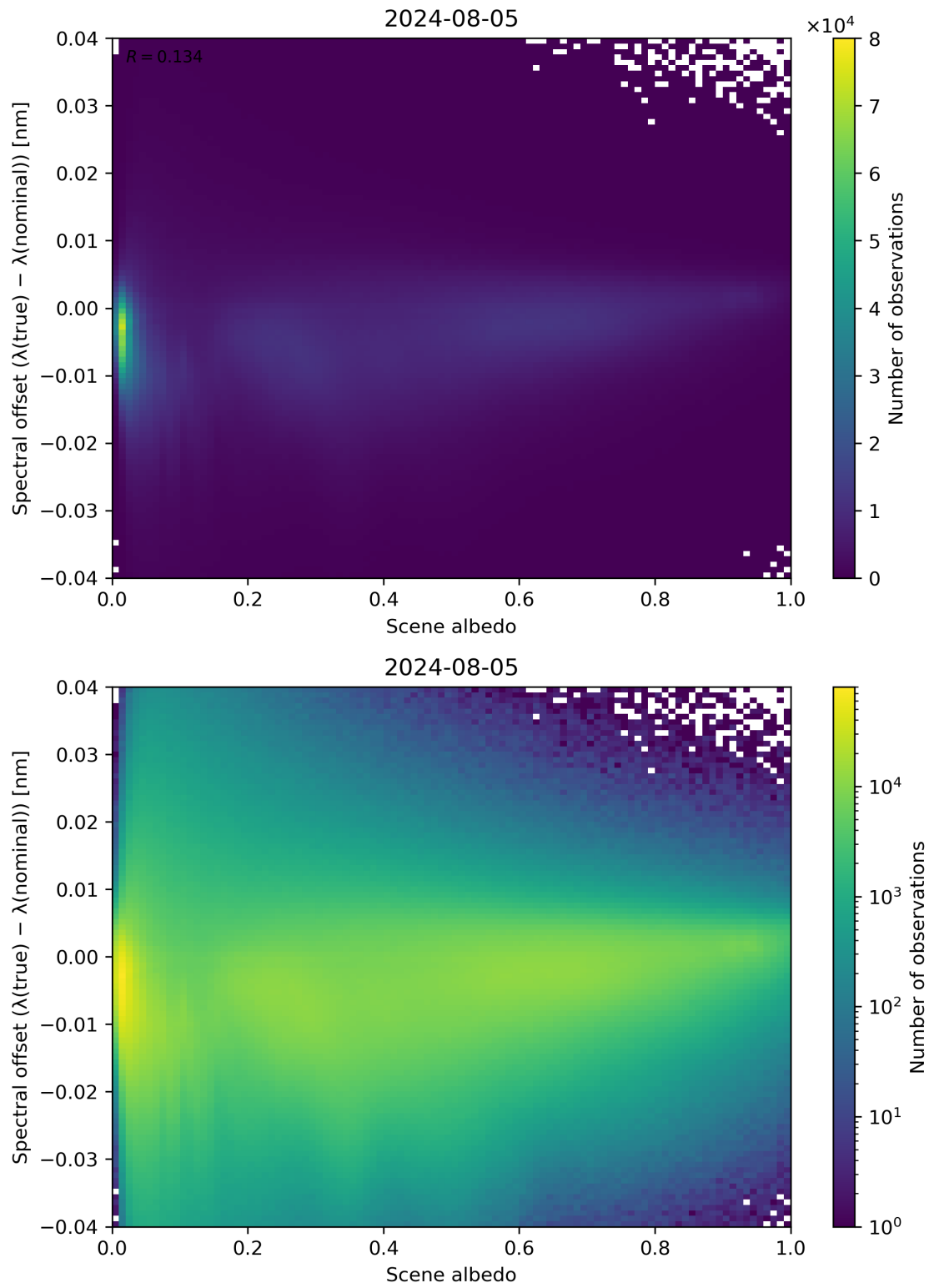
Figure 107: Scatter density plot of “Scene albedo” against “Spectral offset ( \lambda(\text{true}) - \lambda(\text{nominal}) )” for 2024-08-04 to 2024-08-06.
