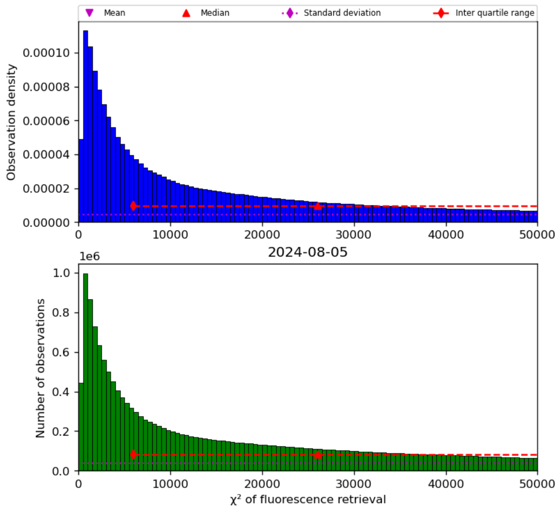
Figure 42: Histogram of “ \chi^2 of fluorescence retrieval” for 2024-08-04 to 2024-08-06
