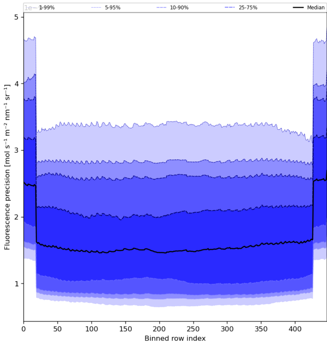
Figure 58: Along track statistics of “Fluorescence precision” for 2024-08-04 to 2024-08-06
