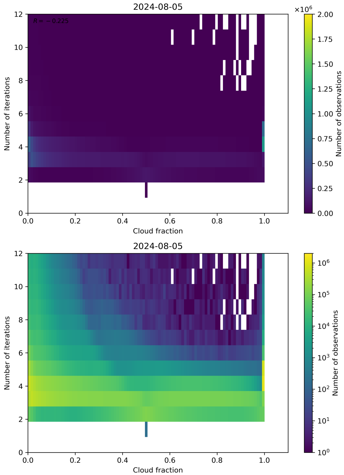
Figure 73: Scatter density plot of “Cloud fraction” against “Number of iterations” for 2024-08-04 to 2024-08-06.
