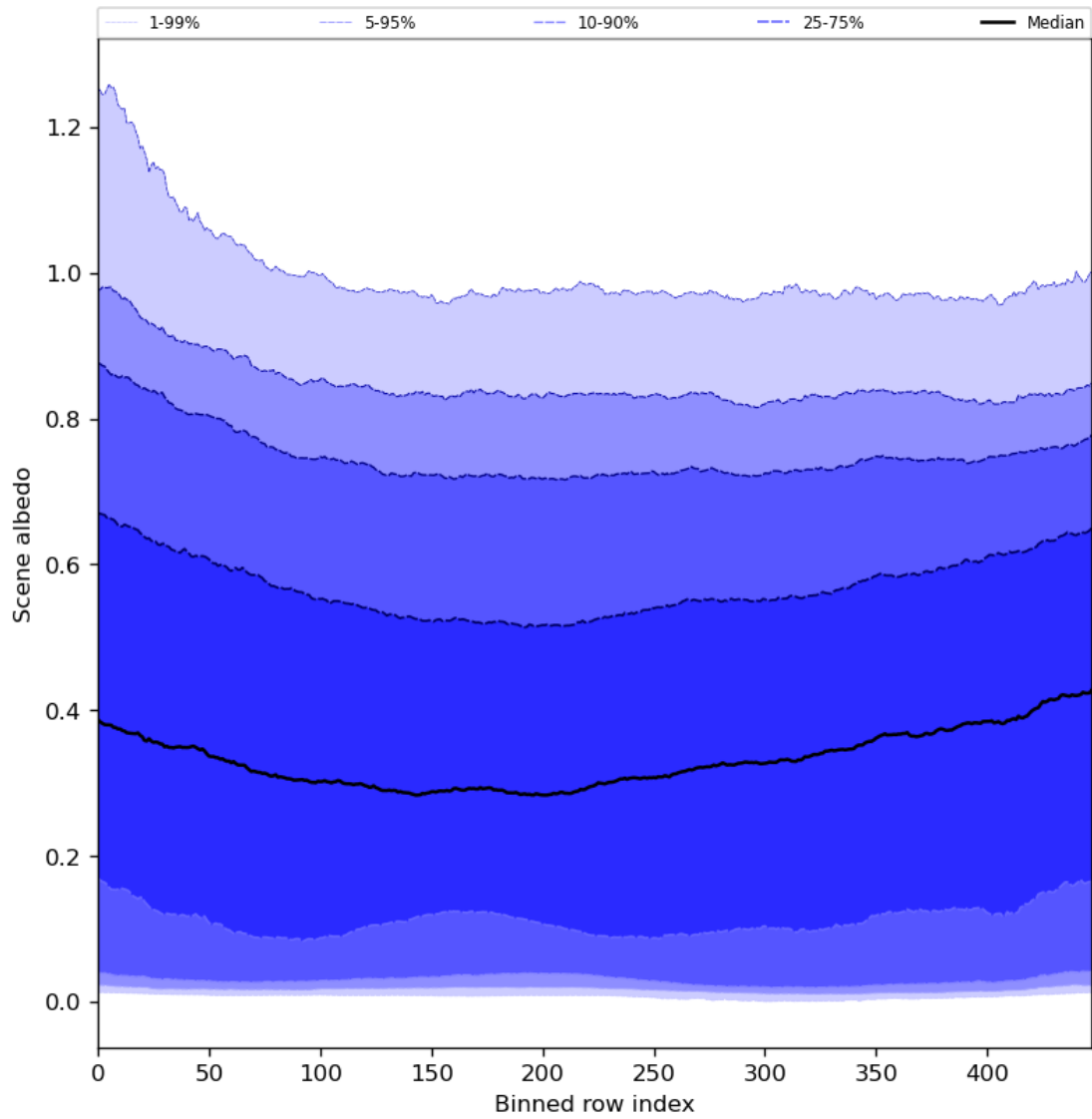
Figure 51: Along track statistics of “Scene albedo” for 2024-08-04 to 2024-08-06
