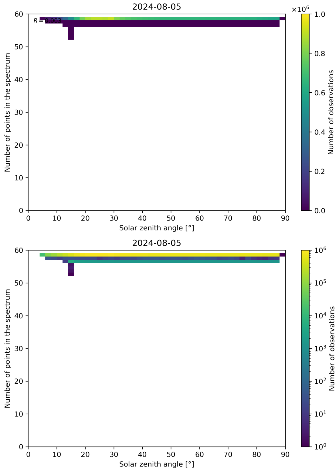
Figure 115: Scatter density plot of “Solar zenith angle” against “Number of points in the spectrum” for 2024-08-04 to 2024-08-06.
