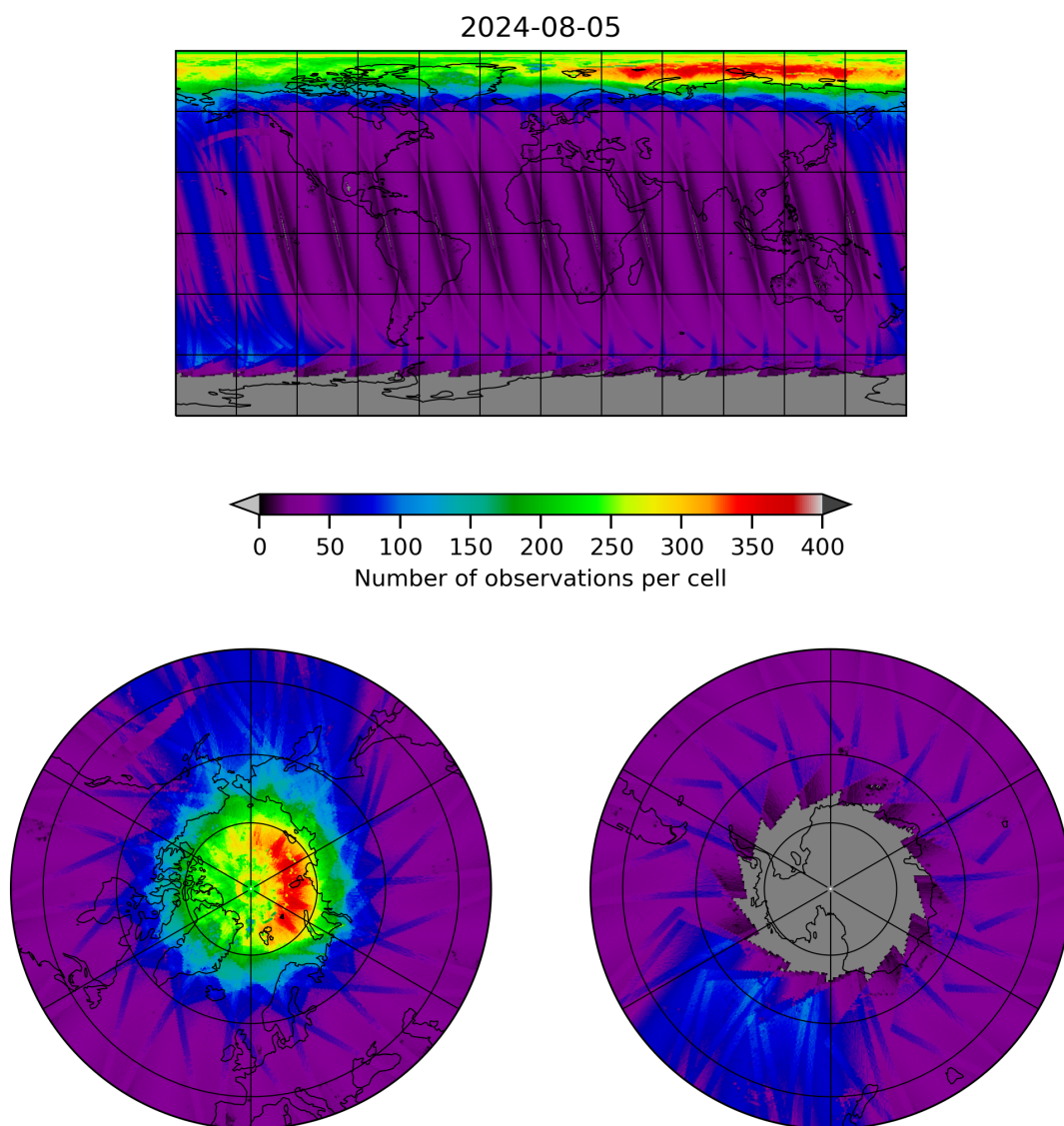
Figure 11: Map of the number of observations for 2024-08-04 to 2024-08-06
