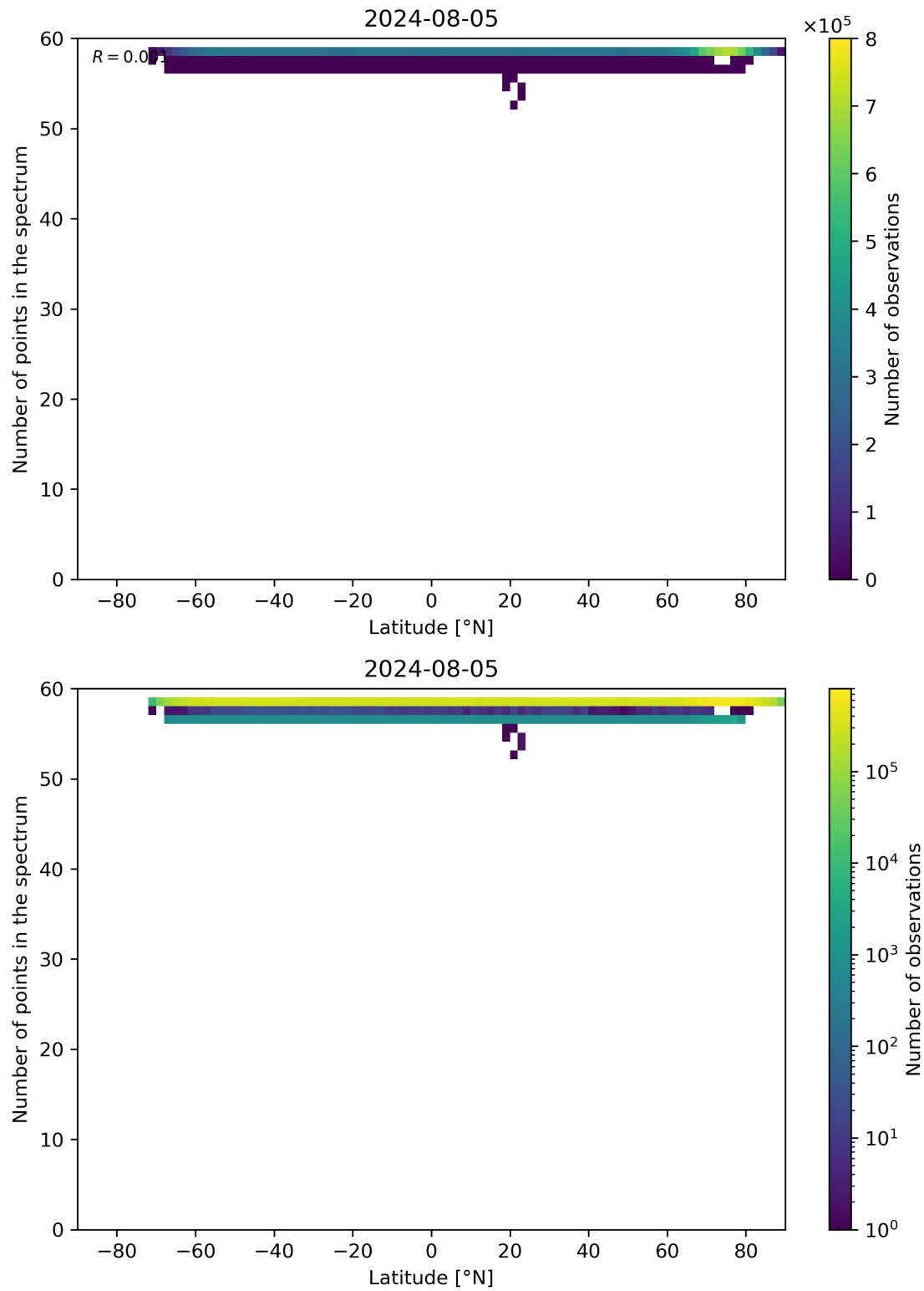
Figure 94: Scatter density plot of “Latitude” against “Number of points in the spectrum” for 2024-08-04 to 2024-08-06.
