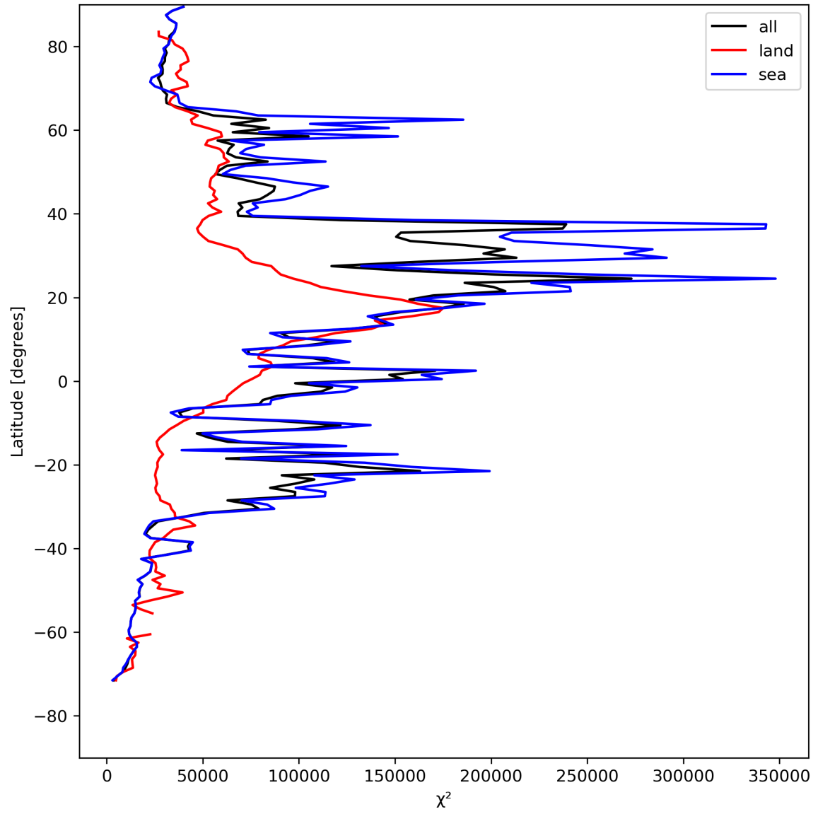
Figure 21: Zonal average of “ \chi^2 ” for 2024-08-04 to 2024-08-06.
