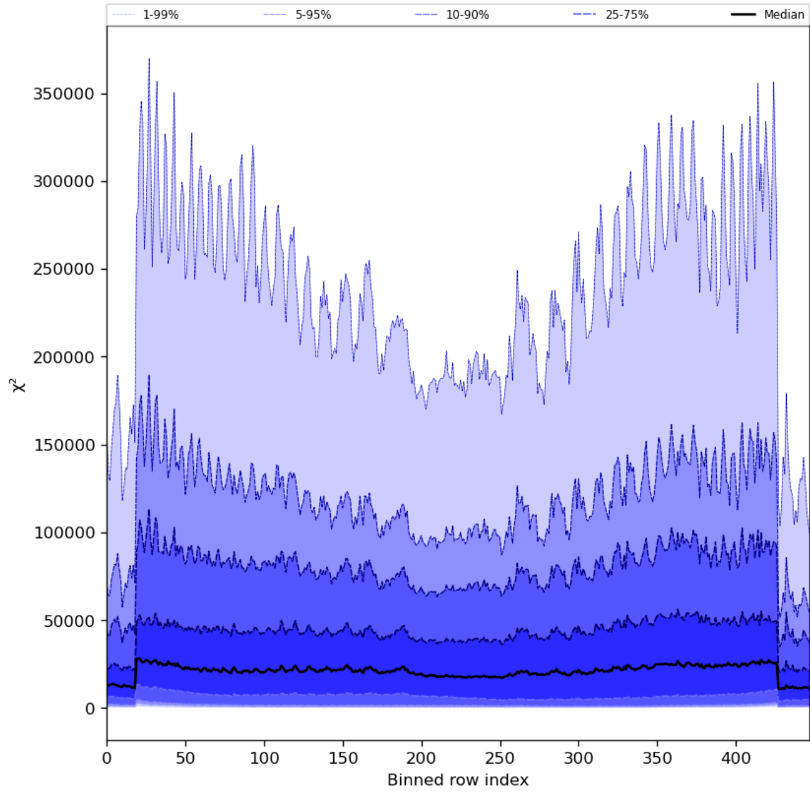
Figure 55: Along track statistics of “ \chi^2 ” for 2024-08-04 to 2024-08-06
