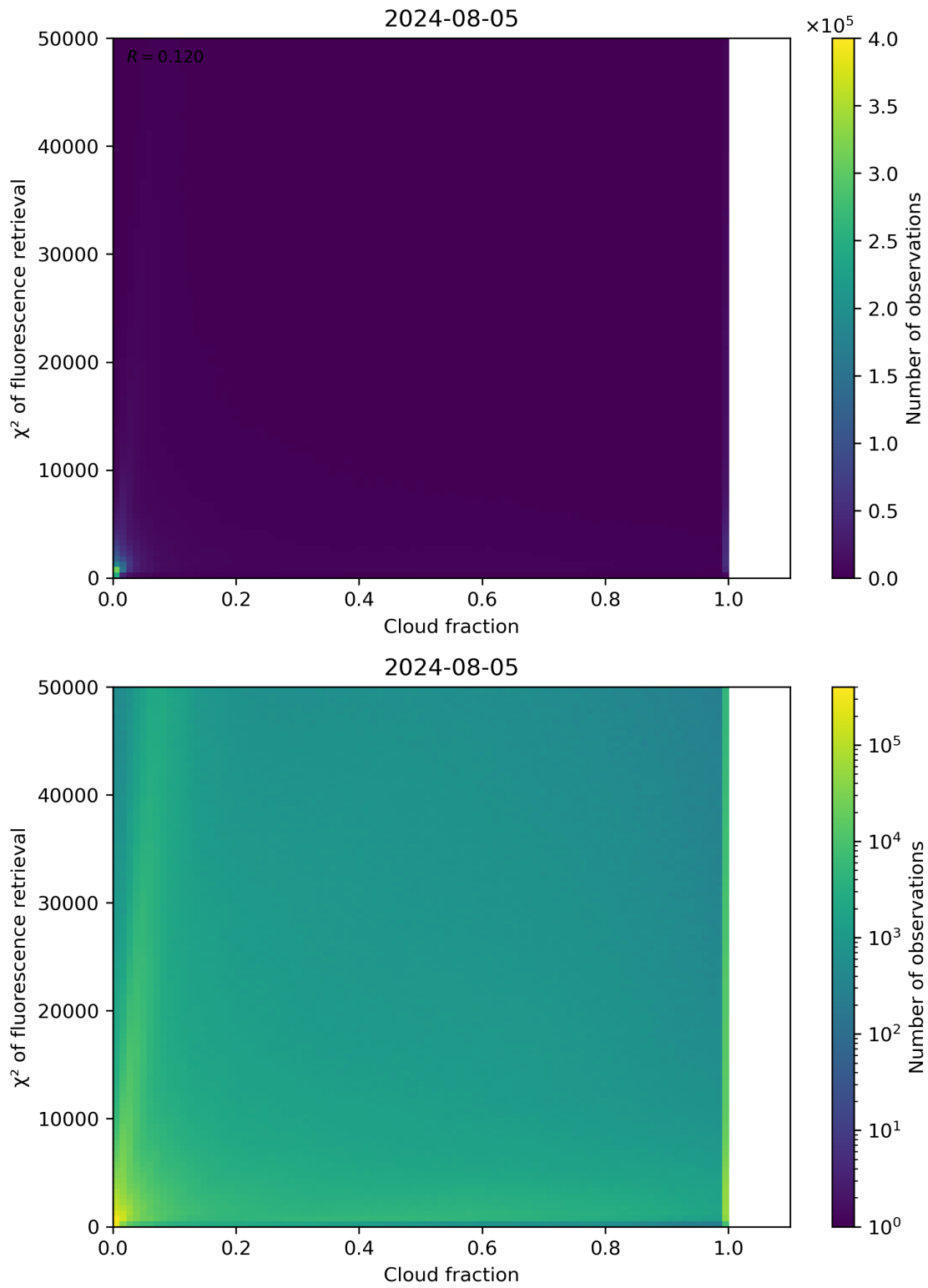
Figure 71: Scatter density plot of “Cloud fraction” against “ \chi^2 of fluorescence retrieval” for 2024-08-04 to 2024-08-06.
