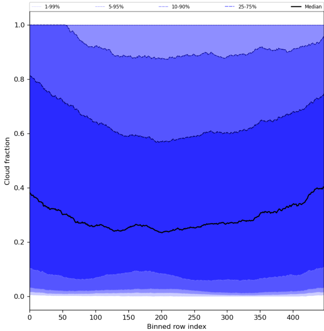
Figure 49: Along track statistics of “Cloud fraction” for 2024-08-04 to 2024-08-06
