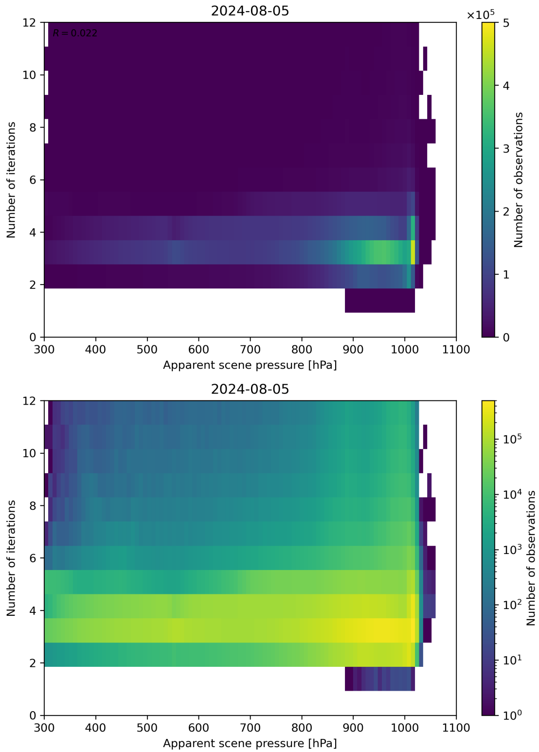
Figure 65: Scatter density plot of “Apparent scene pressure” against “Number of iterations” for 2024-08-04 to 2024-08-06.
