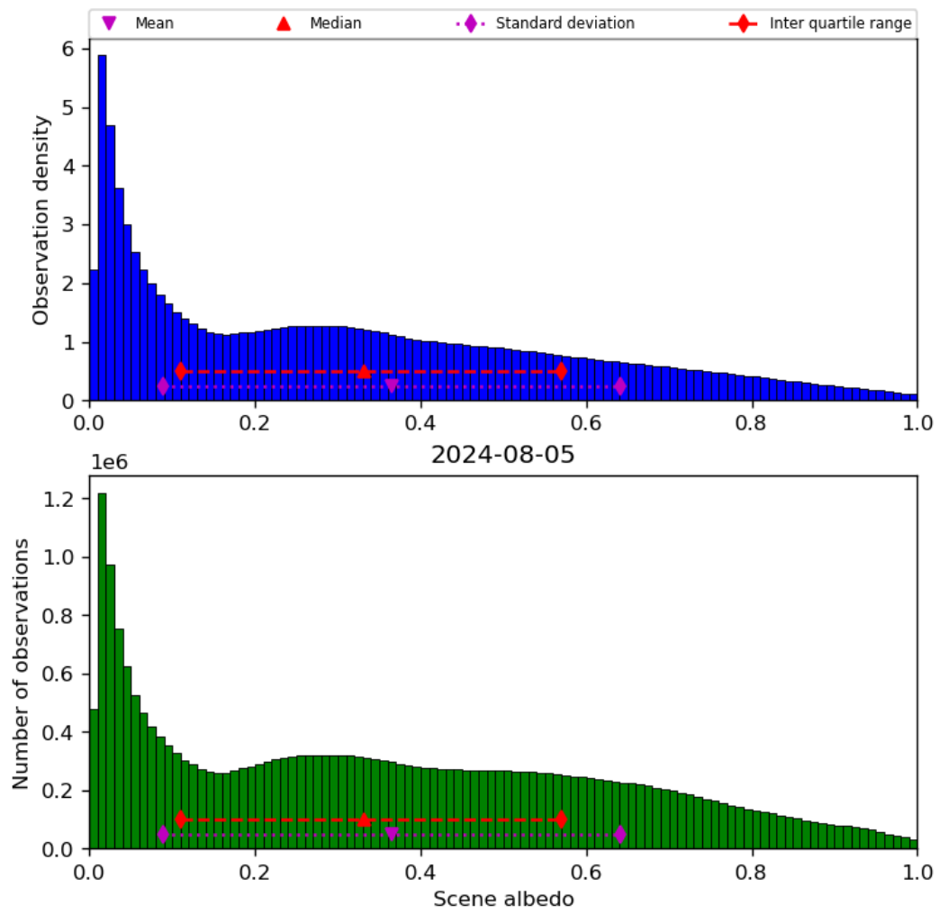
Figure 34: Histogram of “Scene albedo” for 2024-08-04 to 2024-08-06
