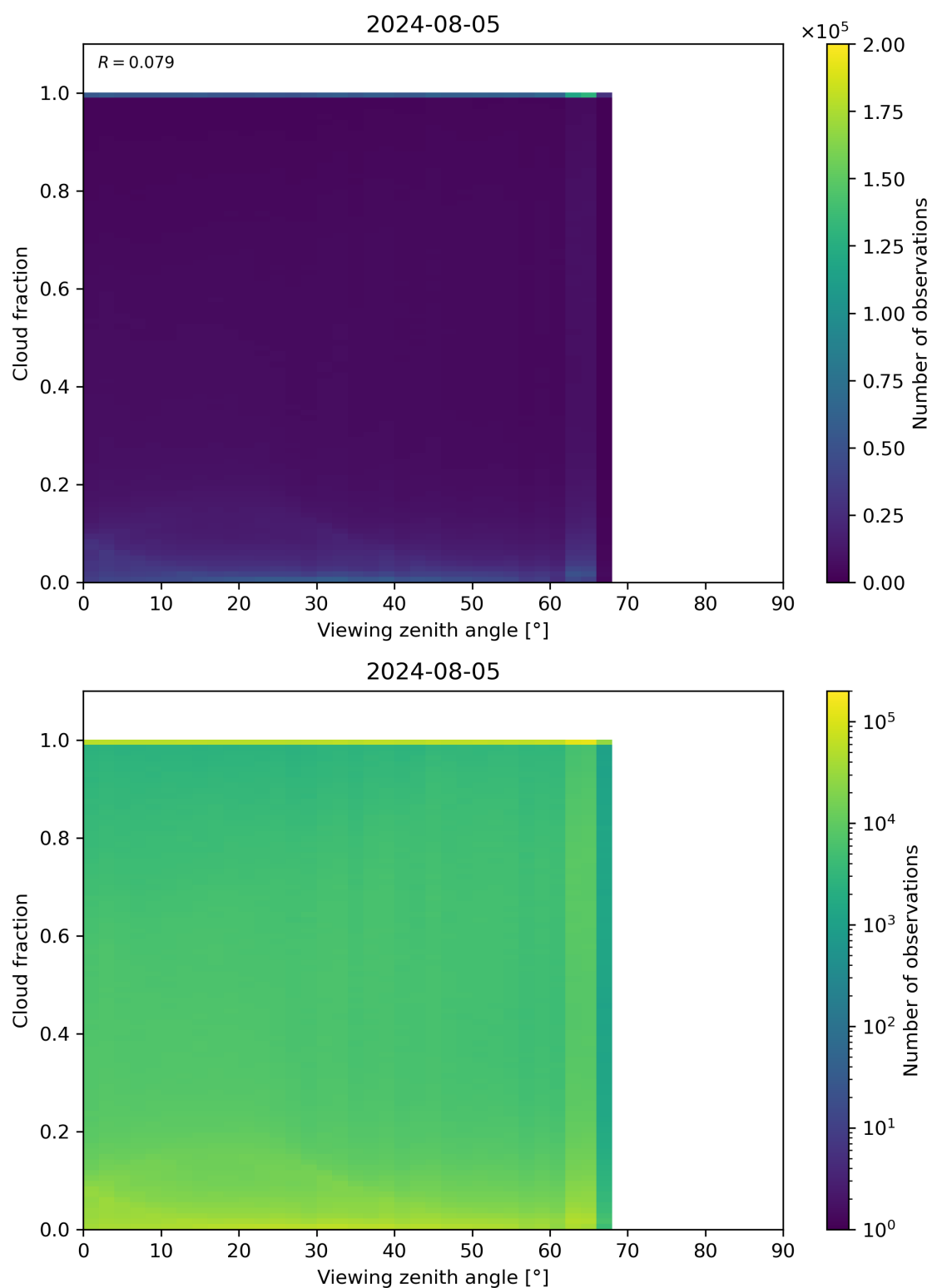
Figure 120: Scatter density plot of “Viewing zenith angle” against “Cloud fraction” for 2024-08-04 to 2024-08-06.
