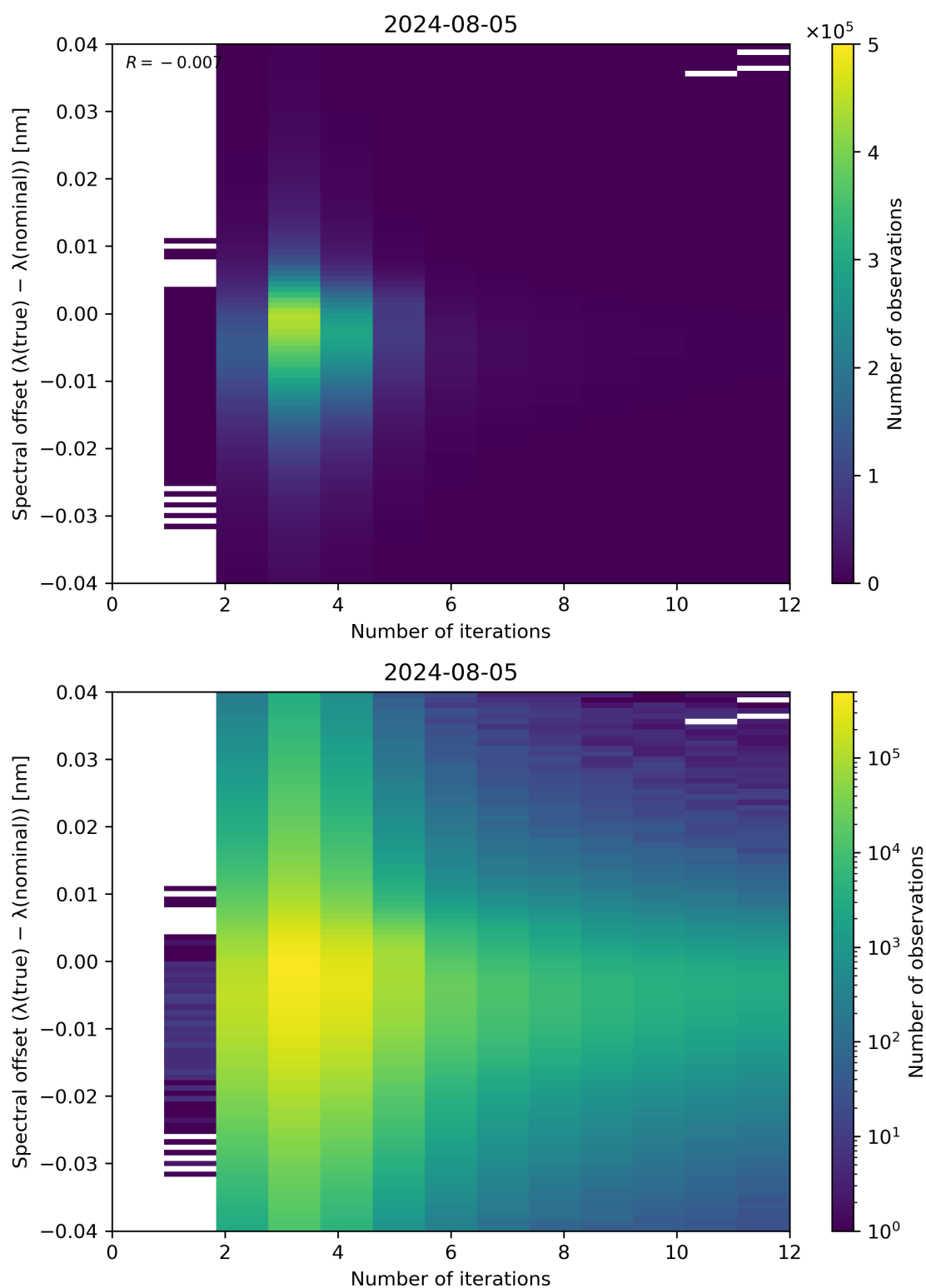
Figure 100: Scatter density plot of “Number of iterations” against “Spectral offset ( \lambda(\text{true}) - \lambda(\text{nominal}) )” for 2024-08-04 to 2024-08-06.
