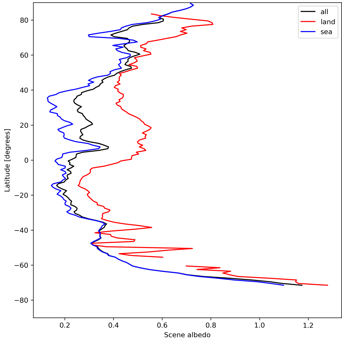
Figure 17: Zonal average of “Scene albedo” for 2024-08-06 to 2024-08-08.
