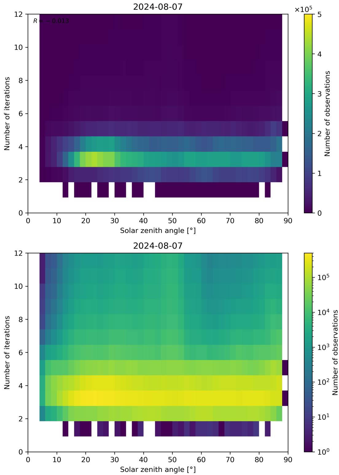
Figure 114: Scatter density plot of “Solar zenith angle” against “Number of iterations” for 2024-08-06 to 2024-08-08.
