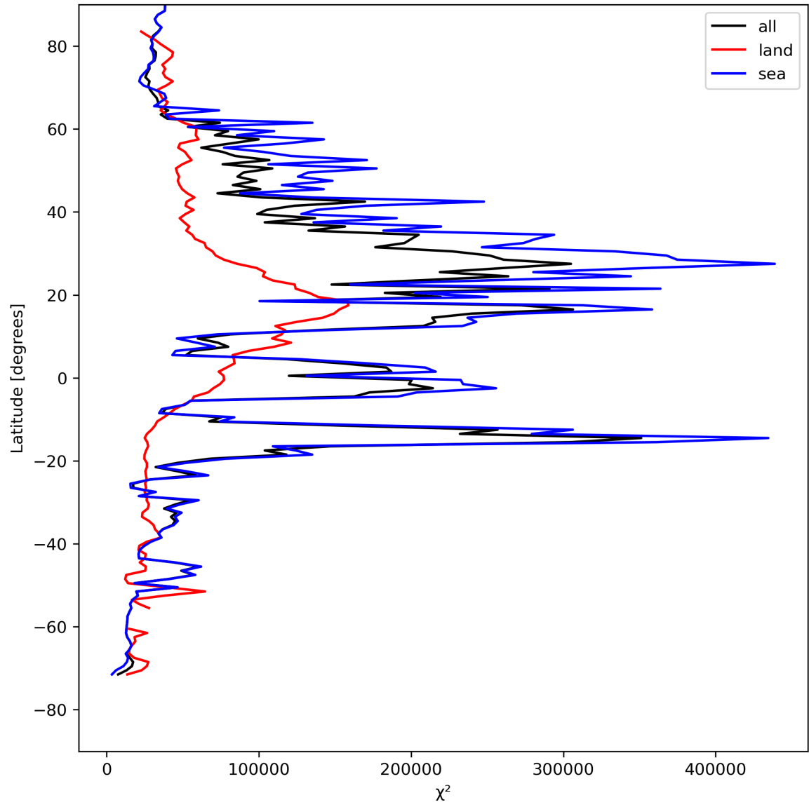
Figure 21: Zonal average of “ \chi^2 ” for 2024-08-06 to 2024-08-08.
