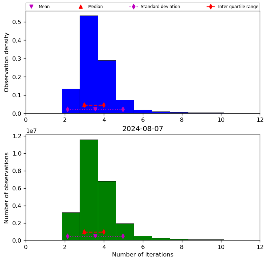
Figure 39: Histogram of “Number of iterations” for 2024-08-06 to 2024-08-08
