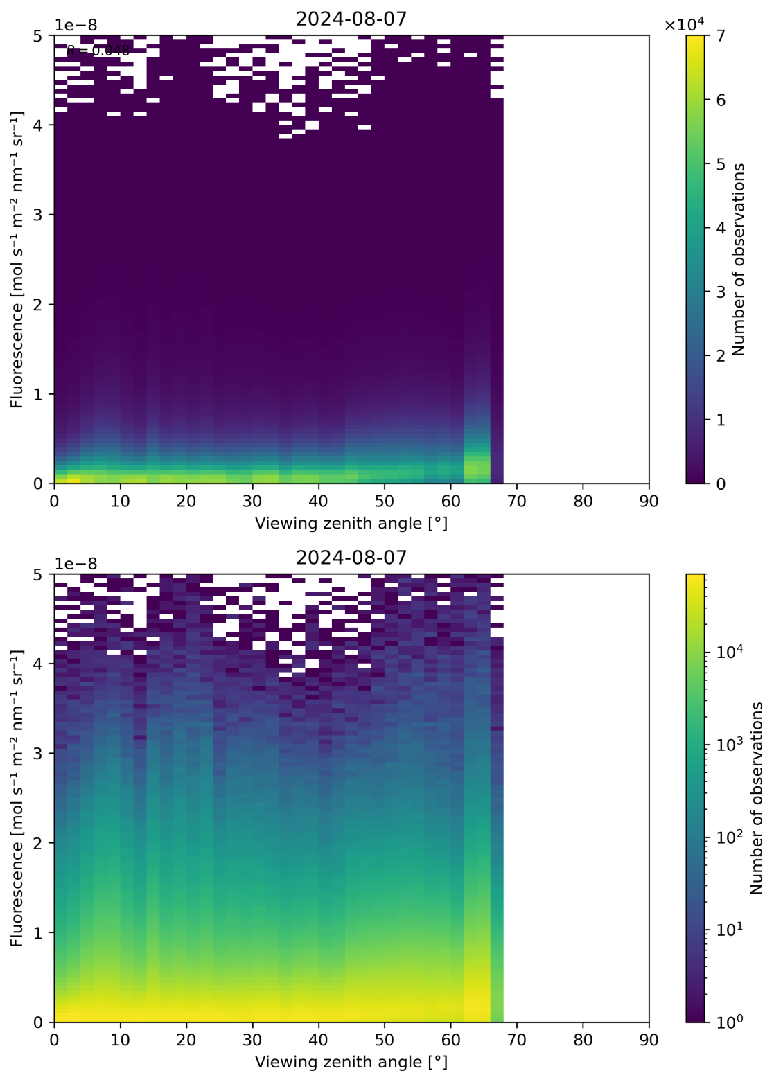
Figure 122: Scatter density plot of “Viewing zenith angle” against “Fluorescence” for 2024-08-06 to 2024-08-08.
