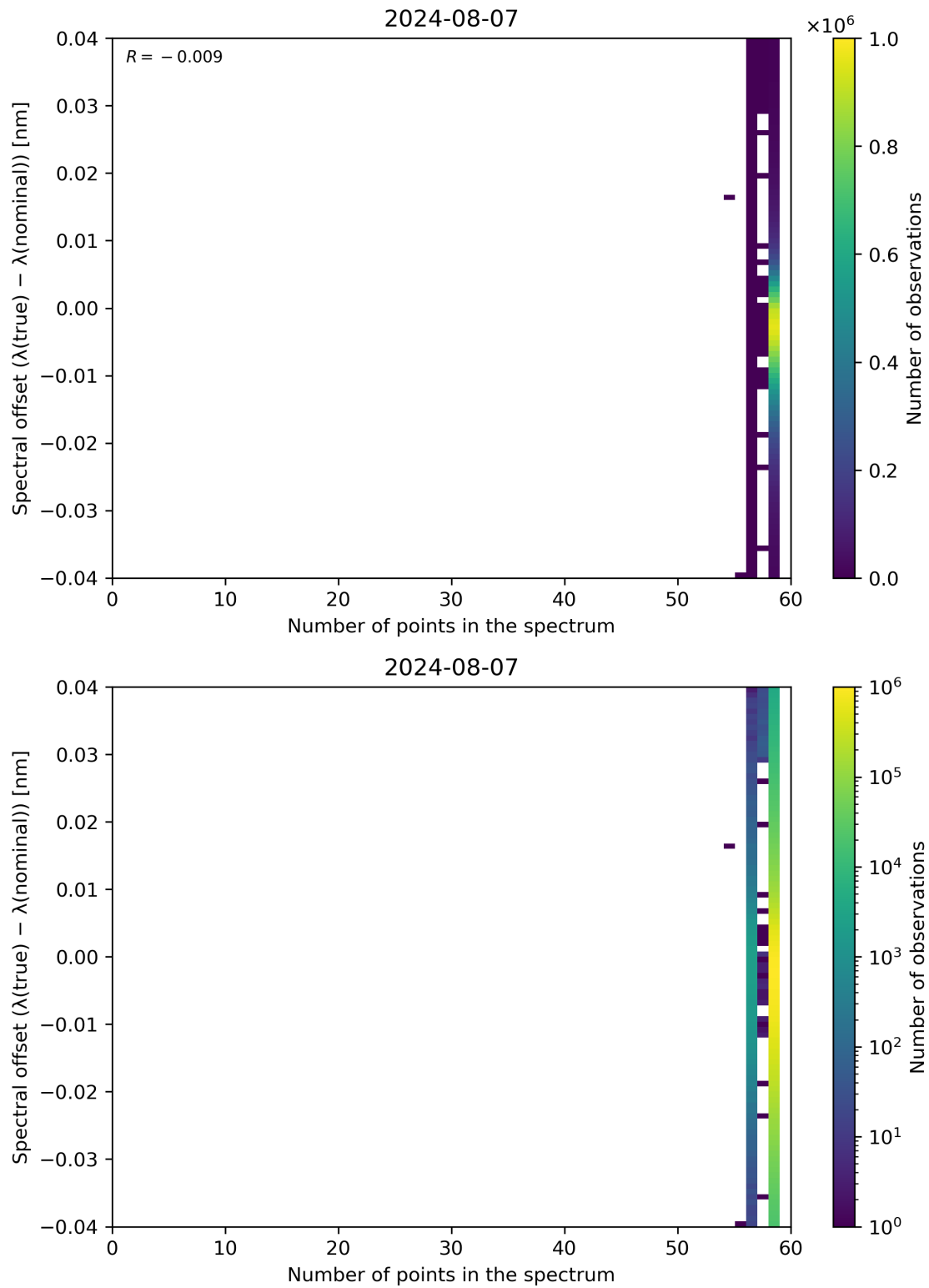
Figure 101: Scatter density plot of “Number of points in the spectrum” against “Spectral offset ( \lambda(\text{true}) - \lambda(\text{nominal}) )” for 2024-08-06 to 2024-08-08.
