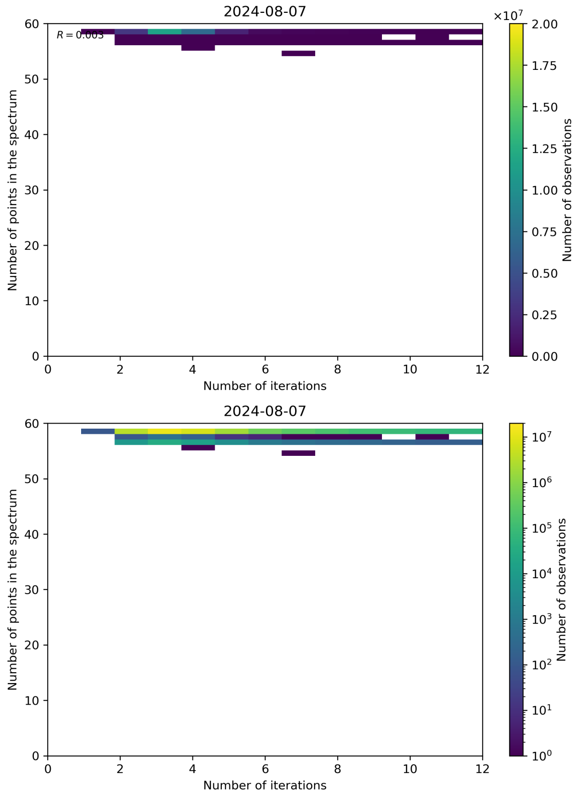
Figure 99: Scatter density plot of “Number of iterations” against “Number of points in the spectrum” for 2024-08-06 to 2024-08-08.
