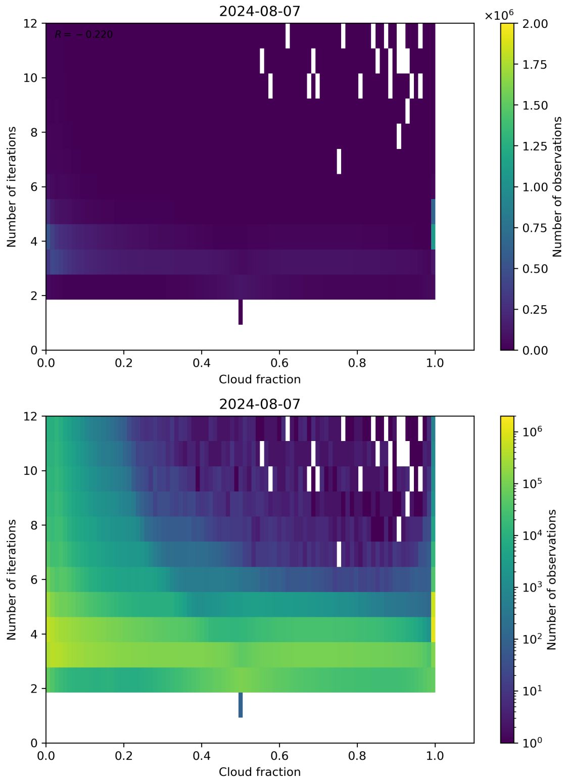
Figure 73: Scatter density plot of “Cloud fraction” against “Number of iterations” for 2024-08-06 to 2024-08-08.
