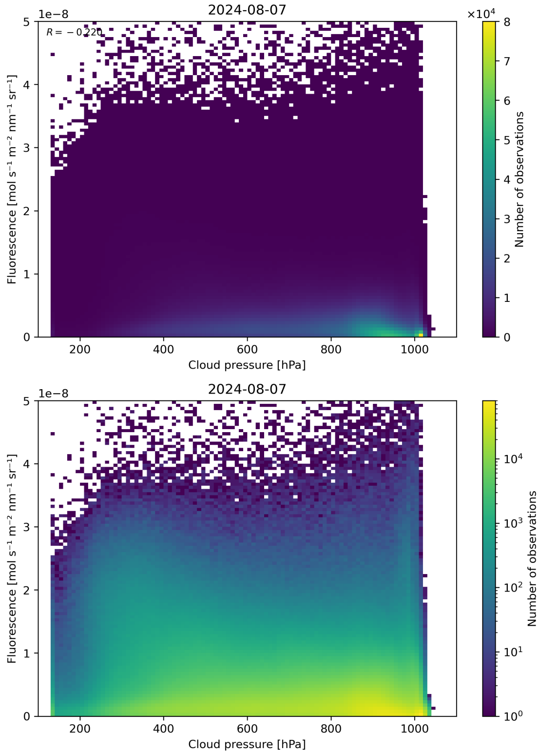
Figure 80: Scatter density plot of “Cloud pressure” against “Fluorescence” for 2024-08-06 to 2024-08-08.
