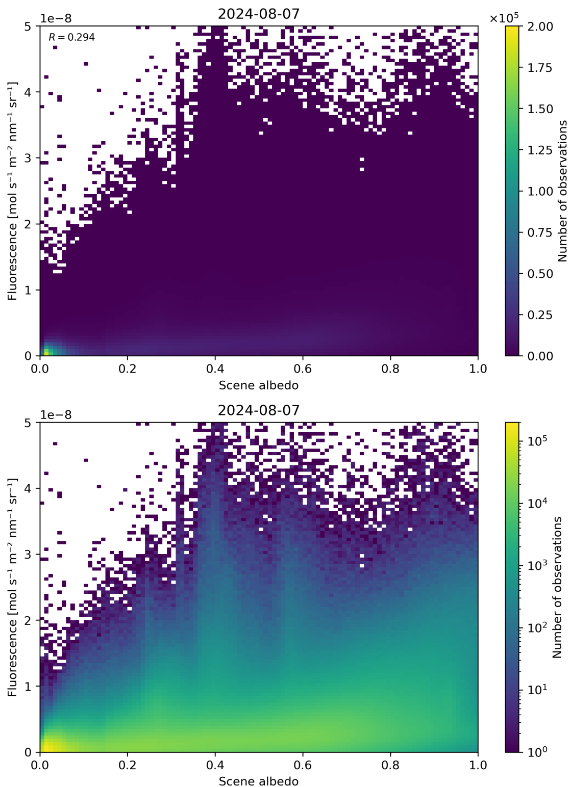
Figure 104: Scatter density plot of “Scene albedo” against “Fluorescence” for 2024-08-06 to 2024-08-08.
