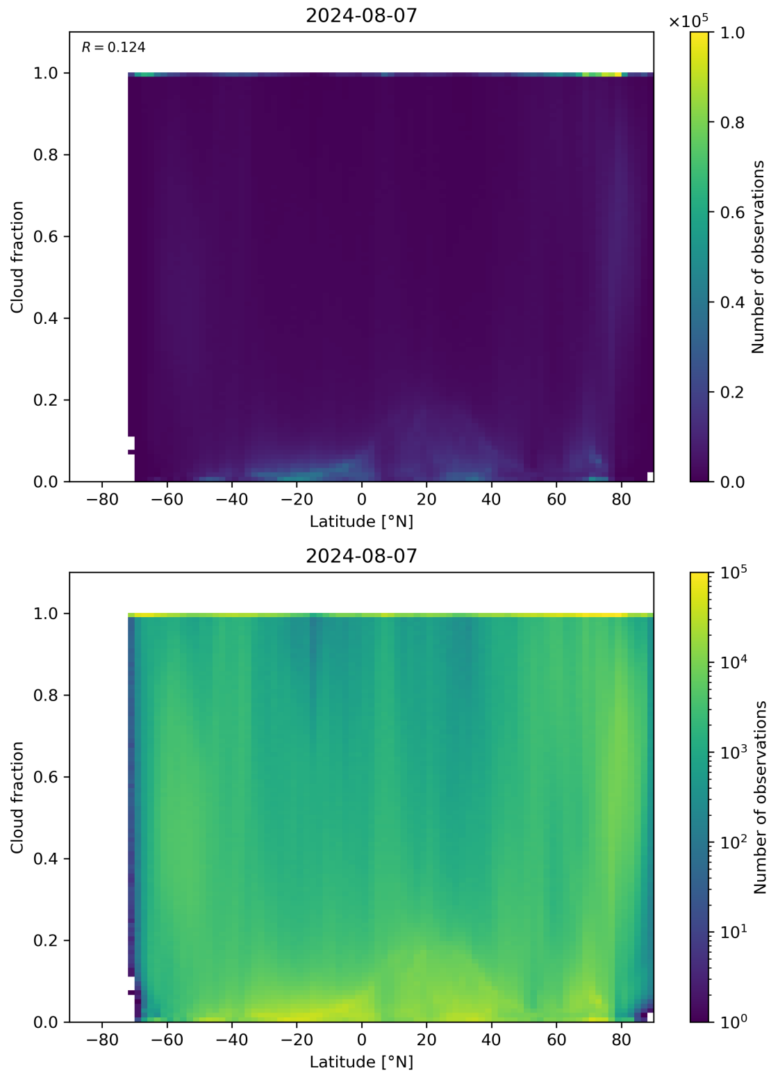
Figure 90: Scatter density plot of “Latitude” against “Cloud fraction” for 2024-08-06 to 2024-08-08.
