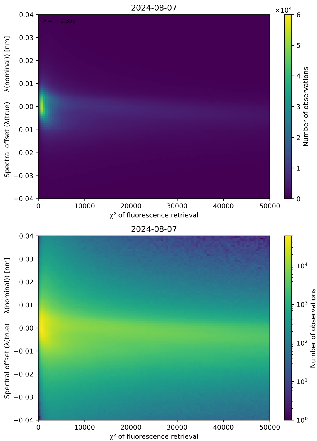
Figure 69: Scatter density plot of " \chi^2 of fluorescence retrieval" against "Spectral offset ( \lambda(\text{true}) - \lambda(\text{nominal}) )" for 2024-08-06 to 2024-08-08.
