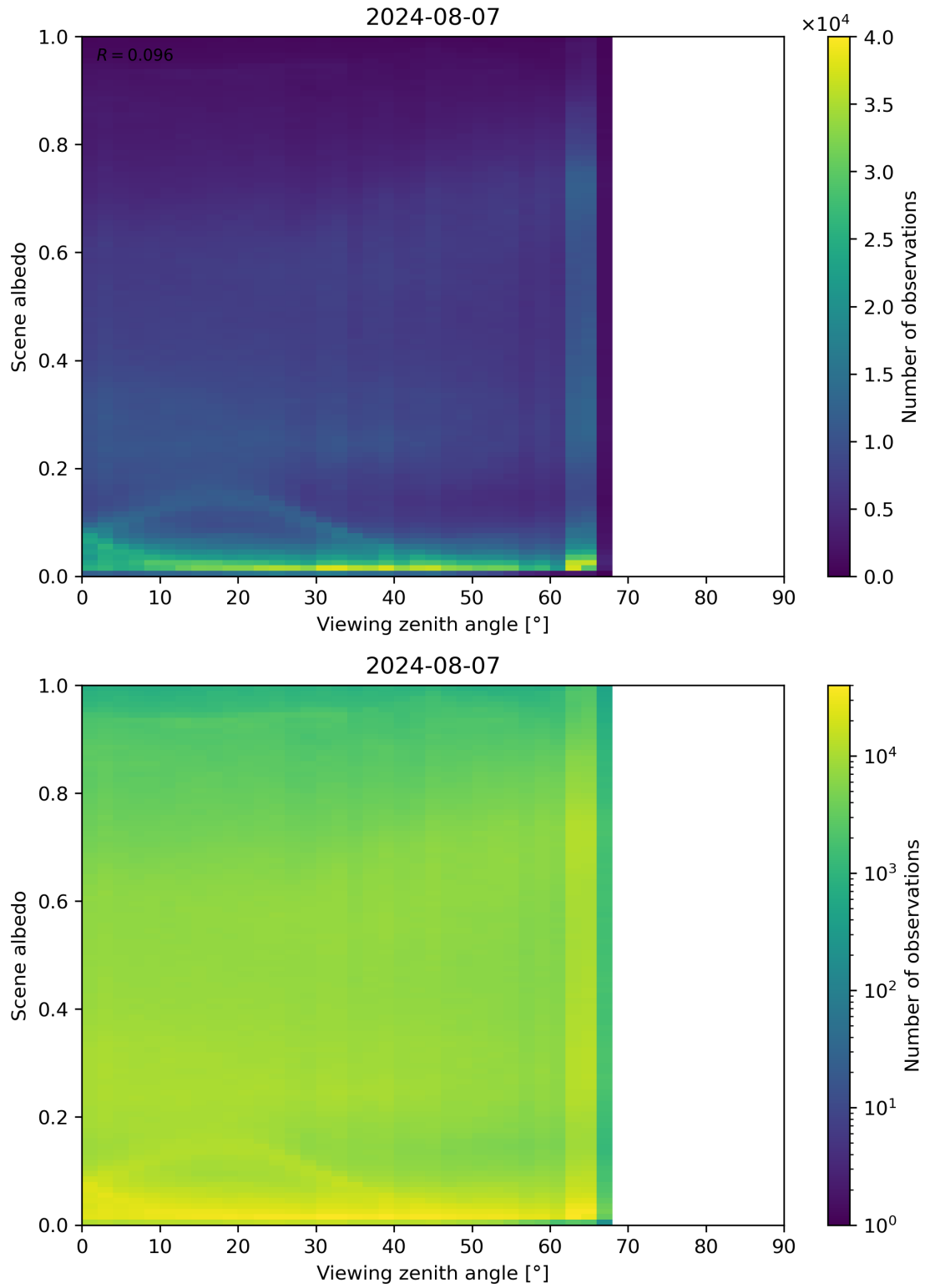
Figure 126: Scatter density plot of “Viewing zenith angle” against “Scene albedo” for 2024-08-06 to 2024-08-08.
