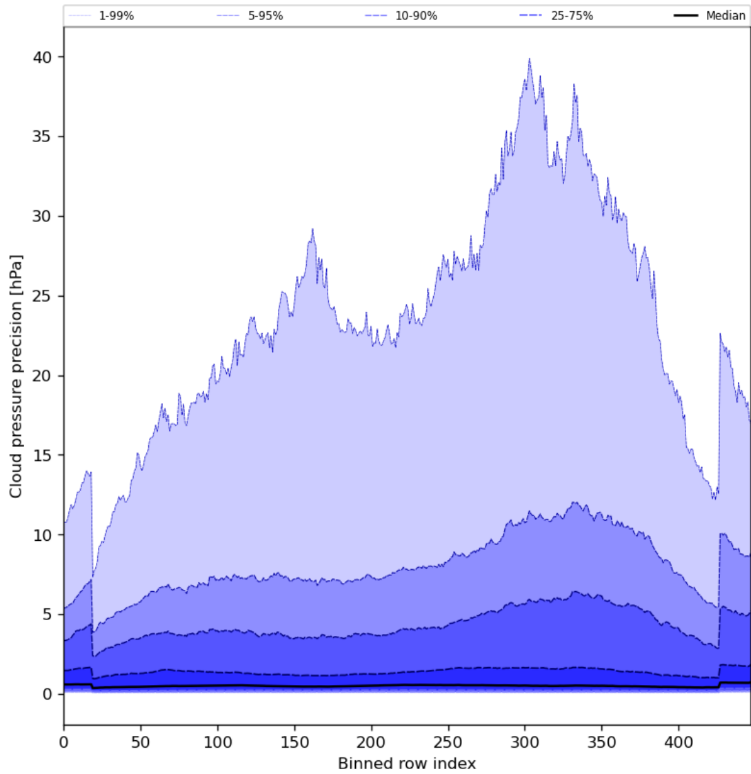
Figure 48: Along track statistics of “Cloud pressure precision” for 2024-08-06 to 2024-08-08
