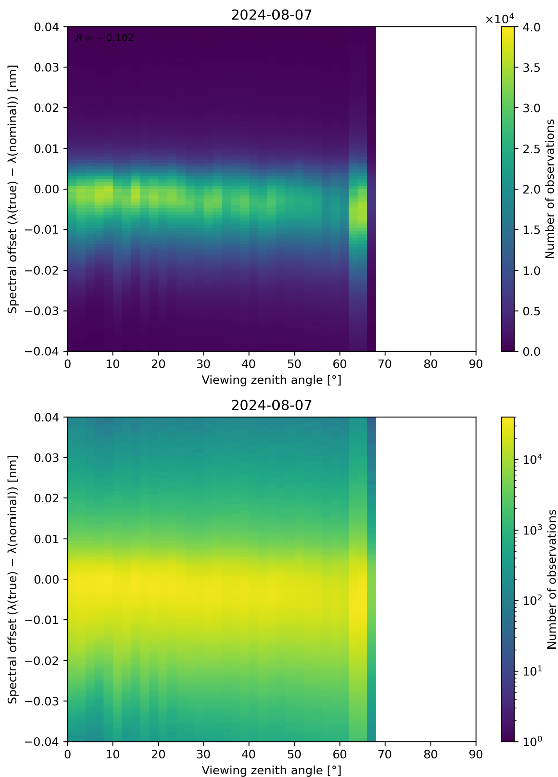
Figure 128: Scatter density plot of “Viewing zenith angle” against “Spectral offset ( \lambda(\text{true}) - \lambda(\text{nominal}) )” for 2024-08-06 to 2024-08-08.
