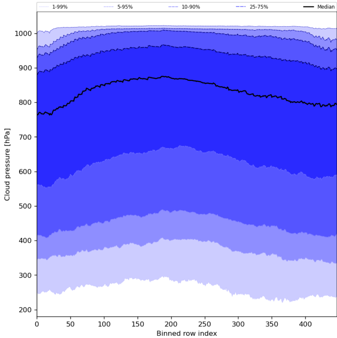
Figure 47: Along track statistics of “Cloud pressure” for 2024-08-06 to 2024-08-08
