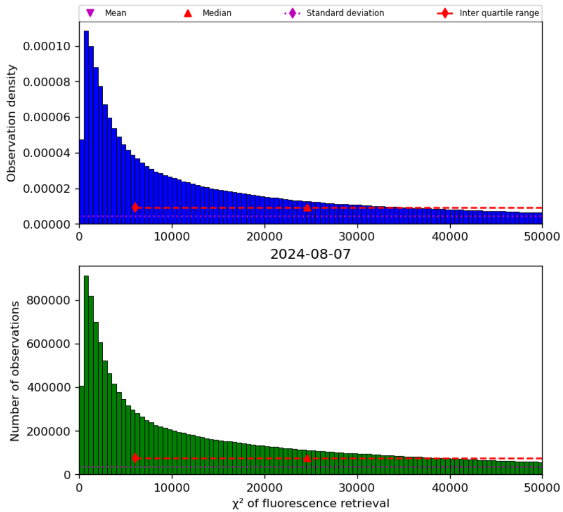
Figure 42: Histogram of “ \chi^2 of fluorescence retrieval” for 2024-08-06 to 2024-08-08
