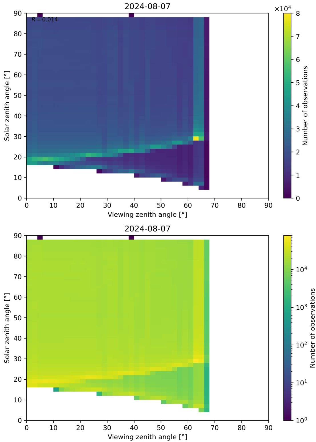
Figure 127: Scatter density plot of “Viewing zenith angle” against “Solar zenith angle” for 2024-08-06 to 2024-08-08.
