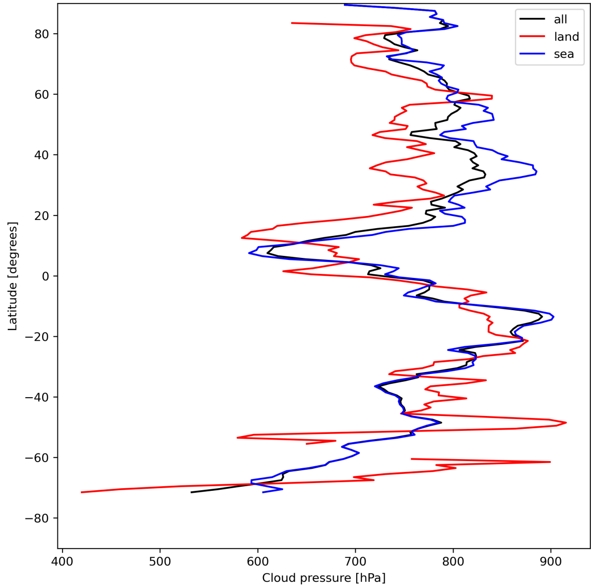
Figure 13: Zonal average of “Cloud pressure” for 2024-08-06 to 2024-08-08.
