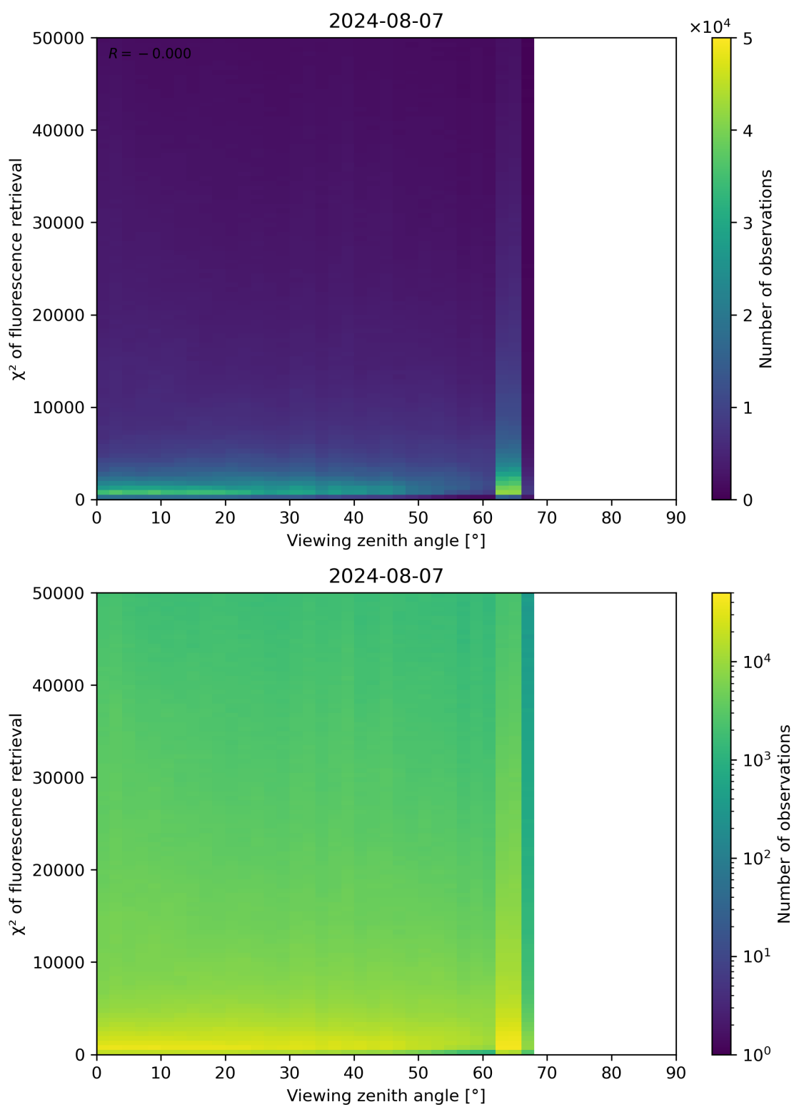
Figure 119: Scatter density plot of “Viewing zenith angle” against “ \chi^2 of fluorescence retrieval” for 2024-08-06 to 2024-08-08.
