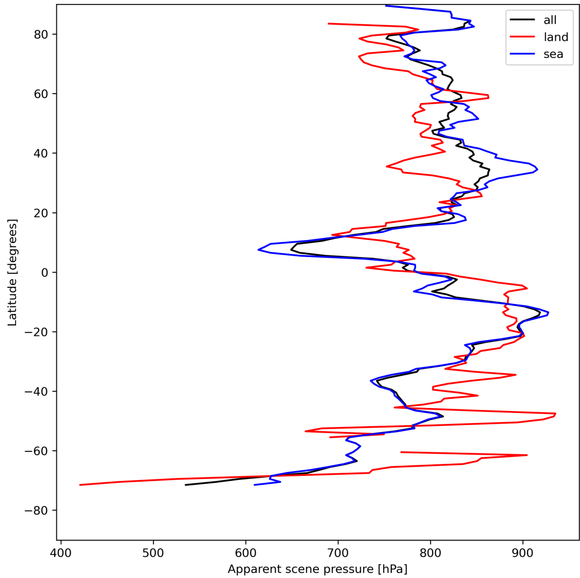
Figure 19: Zonal average of “Apparent scene pressure” for 2024-08-06 to 2024-08-08.
