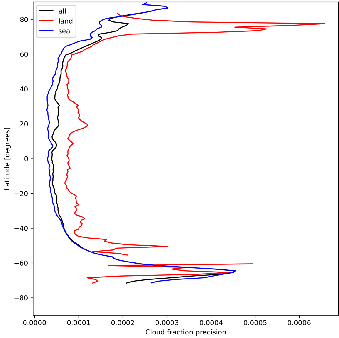
Figure 16: Zonal average of “Cloud fraction precision” for 2024-08-06 to 2024-08-08.
