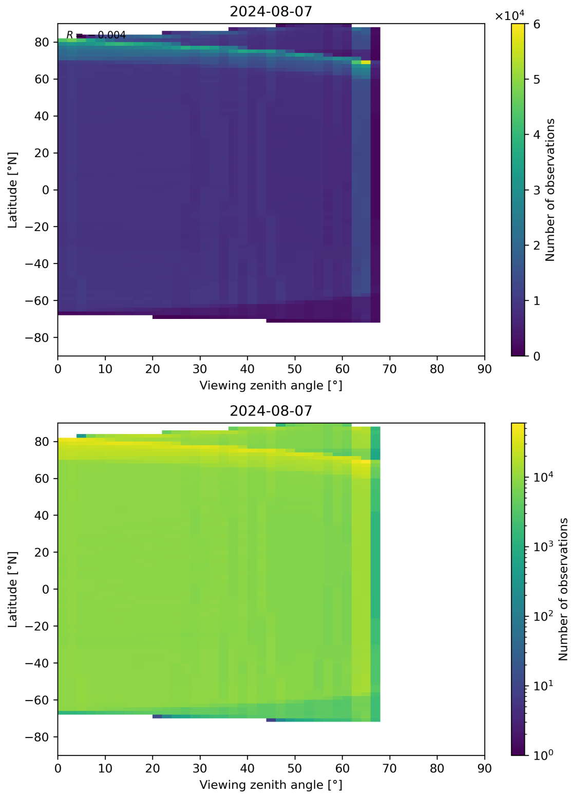
Figure 123: Scatter density plot of “Viewing zenith angle” against “Latitude” for 2024-08-06 to 2024-08-08.
