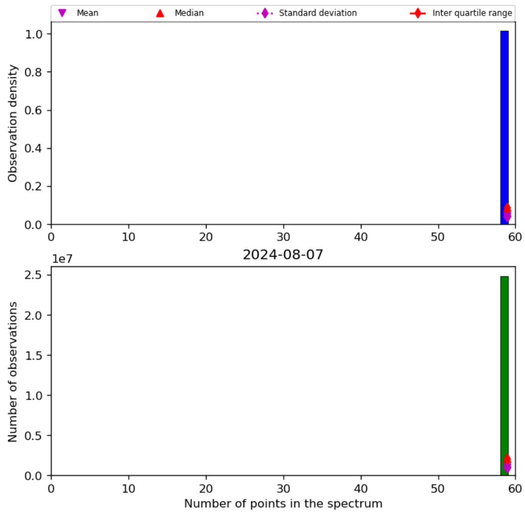
Figure 44: Histogram of “Number of points in the spectrum” for 2024-08-06 to 2024-08-08
