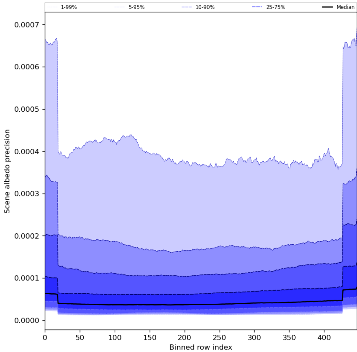
Figure 52: Along track statistics of “Scene albedo precision” for 2024-08-06 to 2024-08-08
