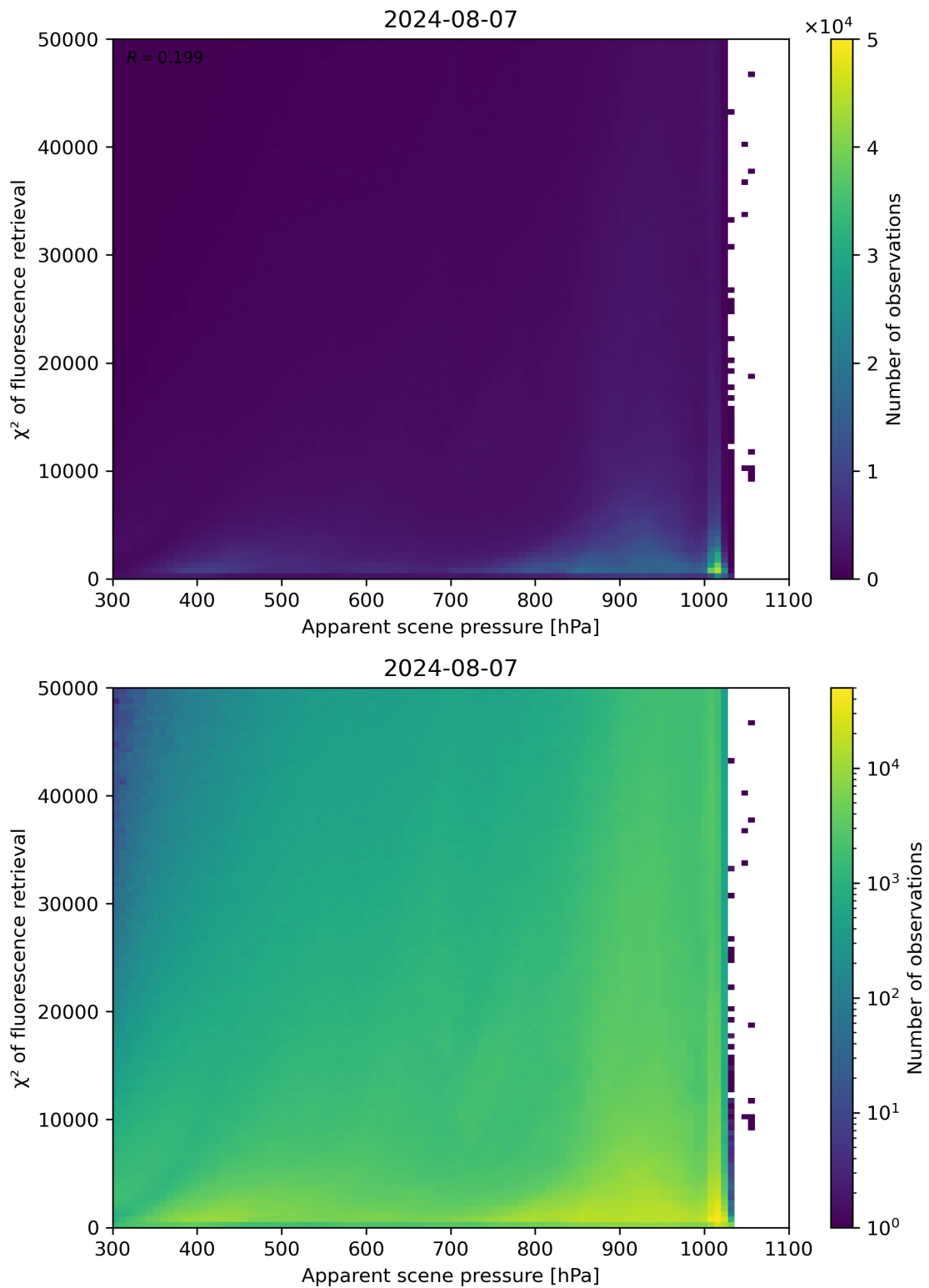
Figure 63: Scatter density plot of “Apparent scene pressure” against “ \chi^2 of fluorescence retrieval” for 2024-08-06 to 2024-08-08.
