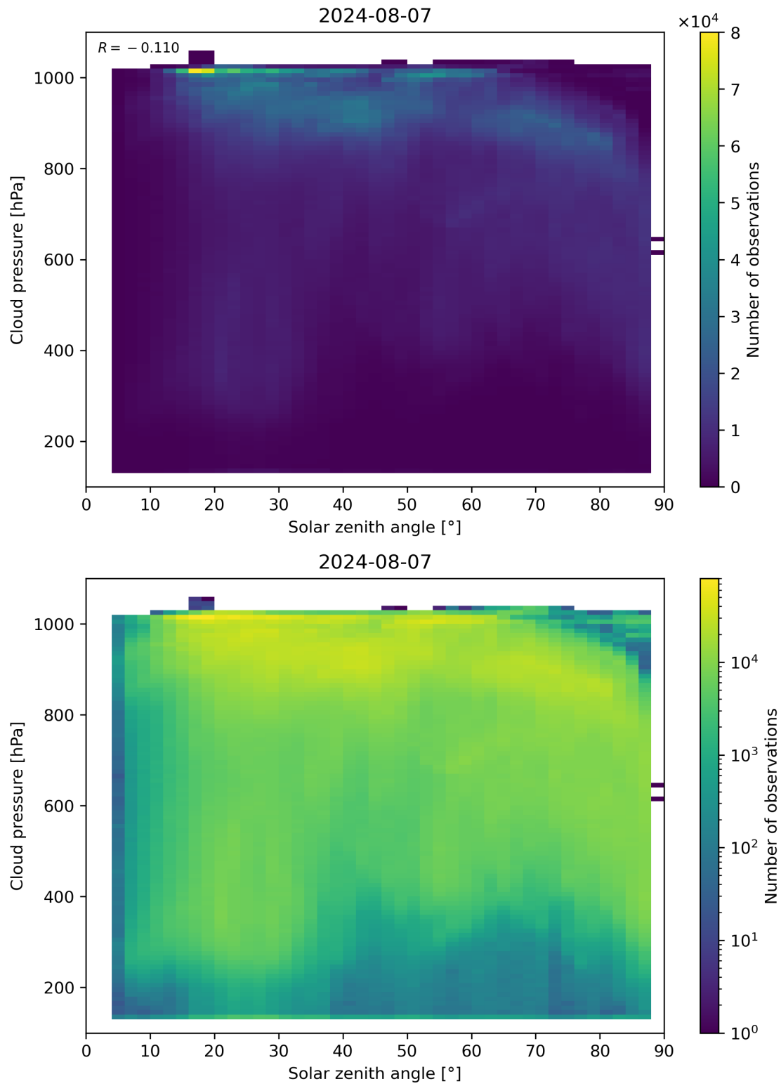
Figure 111: Scatter density plot of “Solar zenith angle” against “Cloud pressure” for 2024-08-06 to 2024-08-08.
