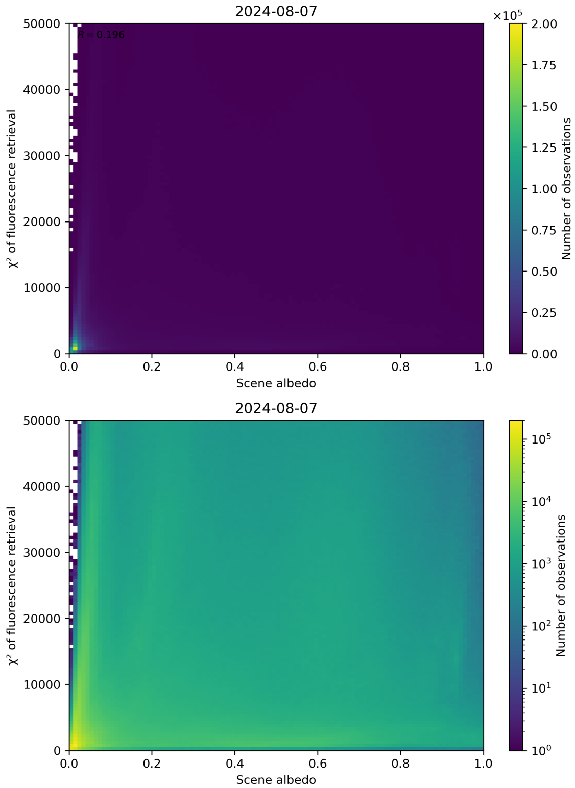
Figure 103: Scatter density plot of “Scene albedo” against “ \chi^2 of fluorescence retrieval” for 2024-08-06 to 2024-08-08.
