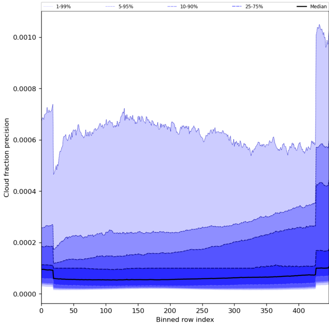
Figure 50: Along track statistics of “Cloud fraction precision” for 2024-08-06 to 2024-08-08
