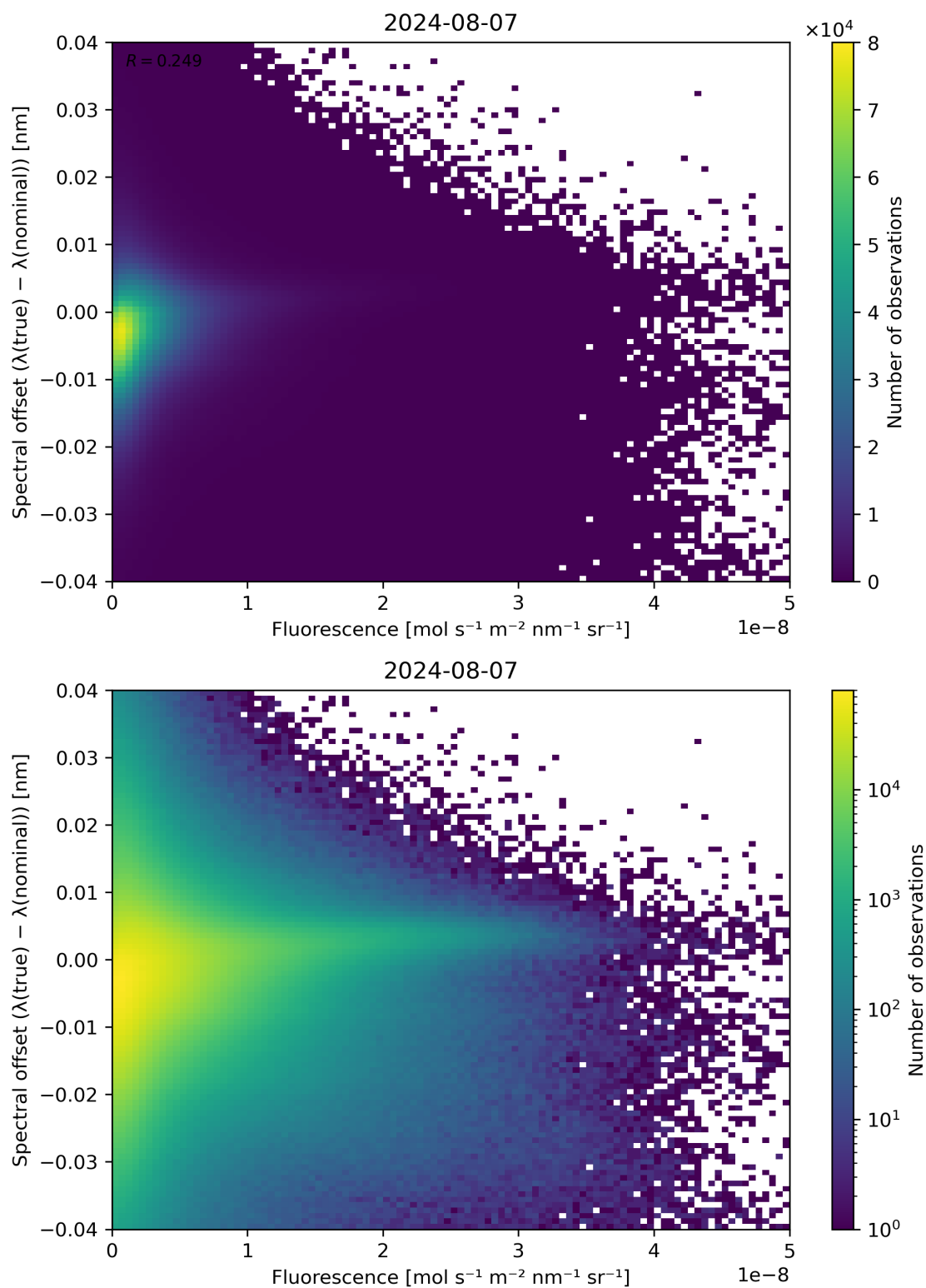
Figure 87: Scatter density plot of “Fluorescence” against “Spectral offset ( \lambda(\text{true}) - \lambda(\text{nominal}) )” for 2024-08-06 to 2024-08-08.
