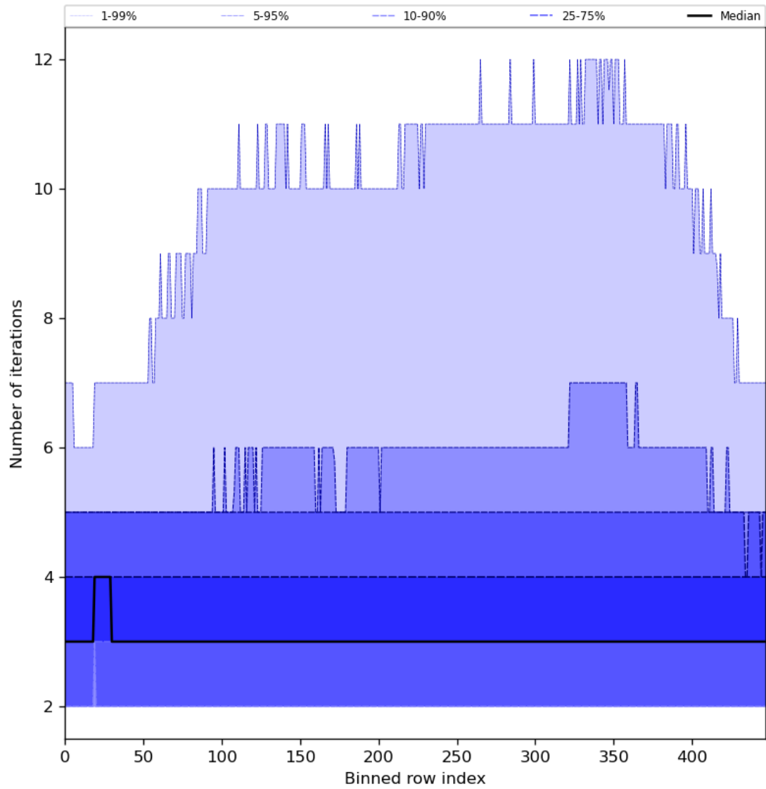
Figure 56: Along track statistics of “Number of iterations” for 2024-08-06 to 2024-08-08
