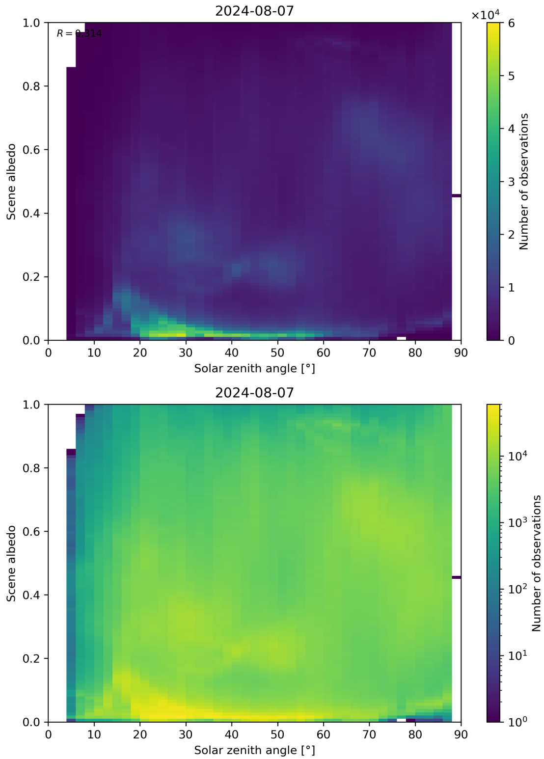
Figure 116: Scatter density plot of “Solar zenith angle” against “Scene albedo” for 2024-08-06 to 2024-08-08.
