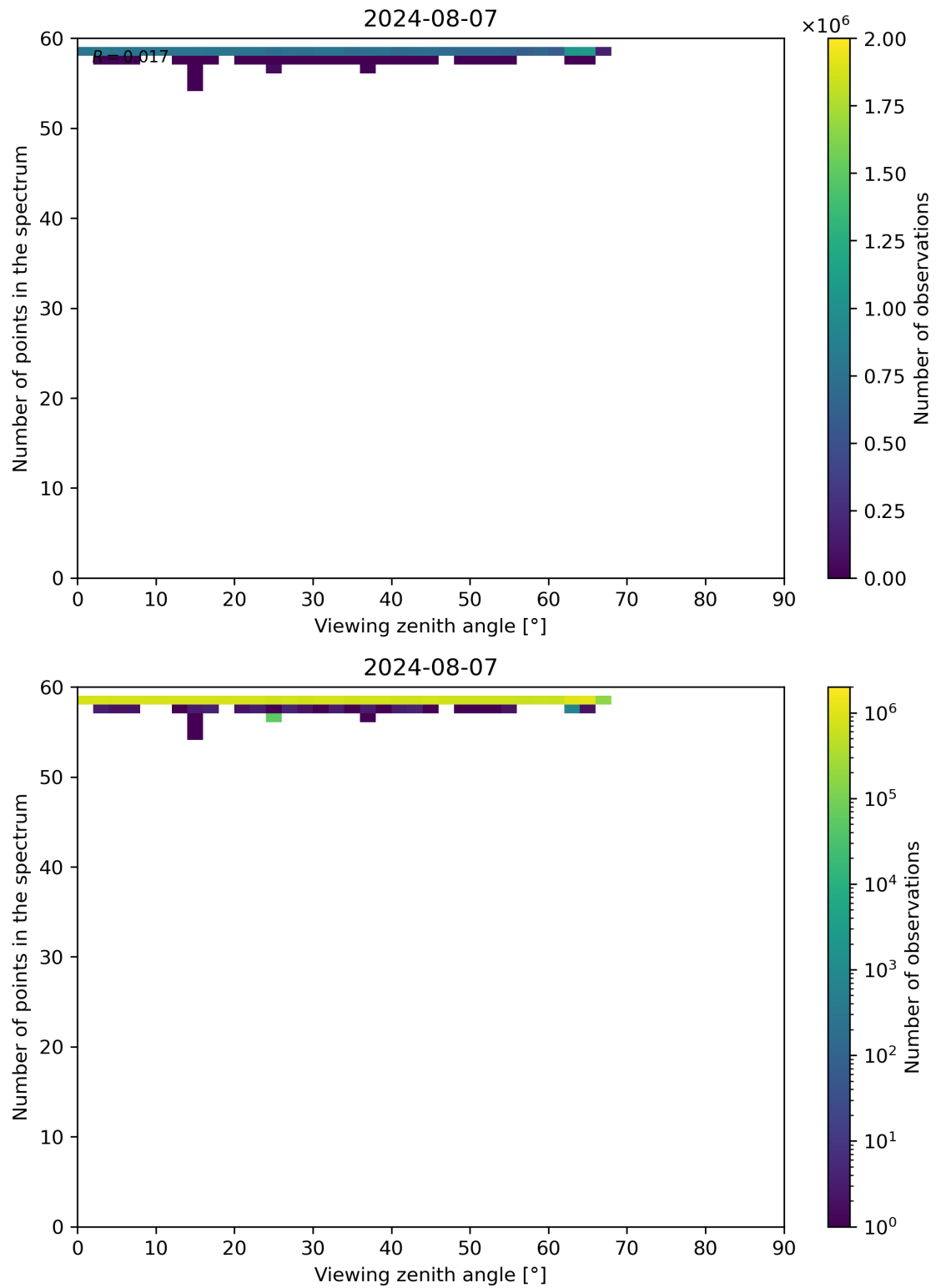
Figure 125: Scatter density plot of “Viewing zenith angle” against “Number of points in the spectrum” for 2024-08-06 to 2024-08-08.
