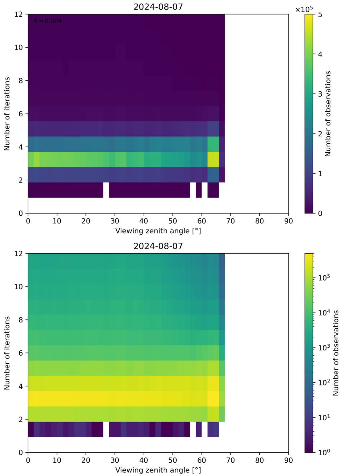
Figure 124: Scatter density plot of “Viewing zenith angle” against “Number of iterations” for 2024-08-06 to 2024-08-08.
