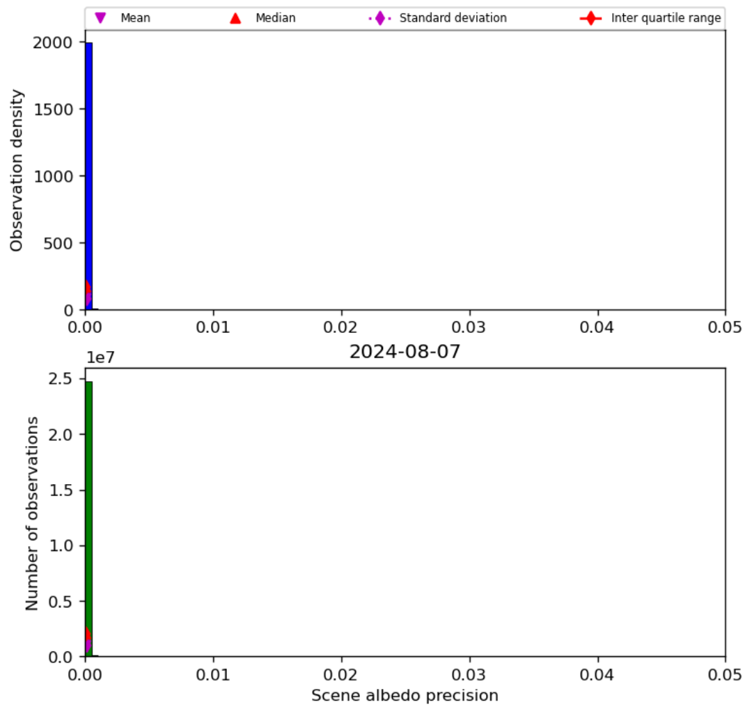
Figure 35: Histogram of “Scene albedo precision” for 2024-08-06 to 2024-08-08
