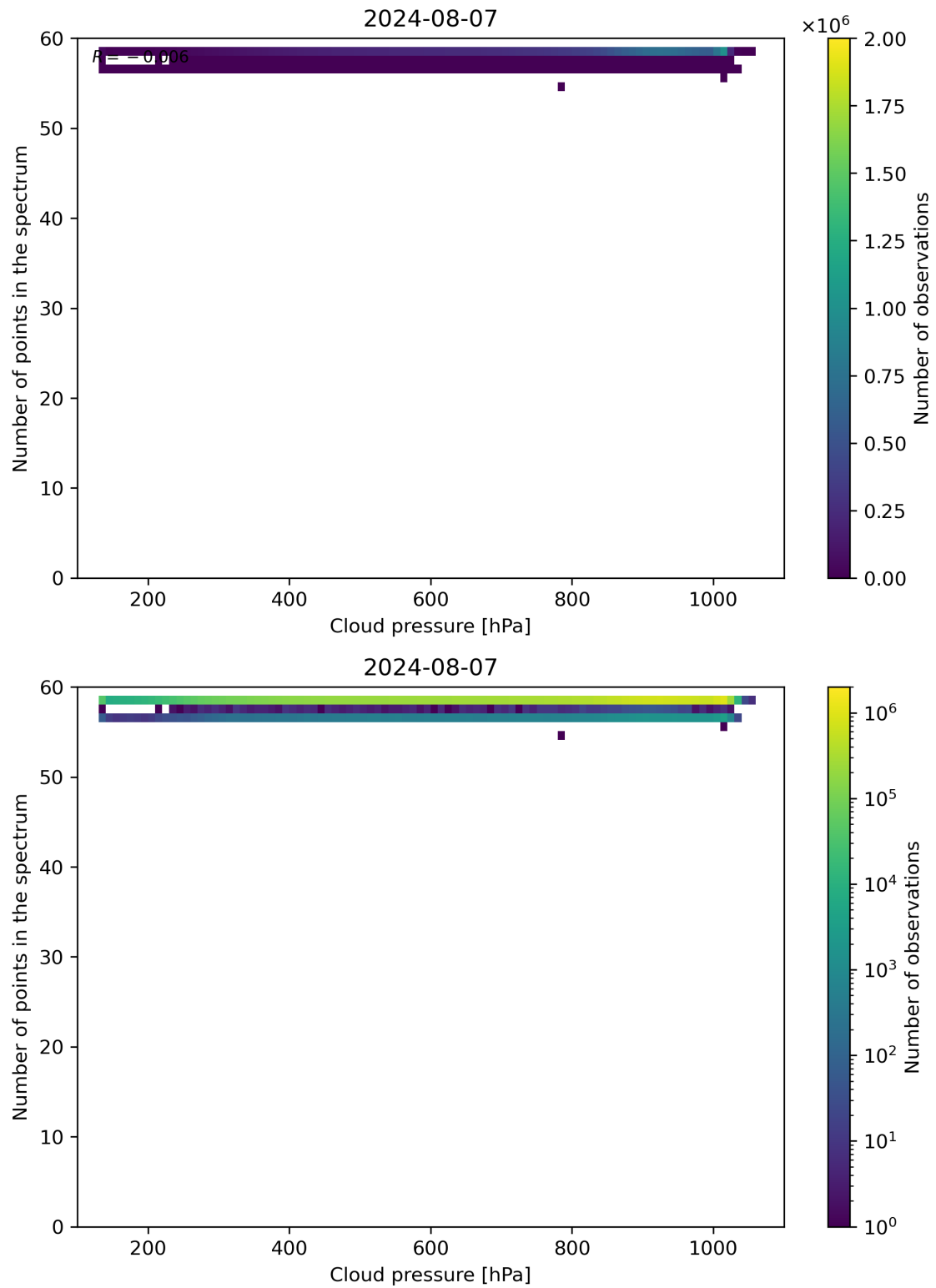
Figure 82: Scatter density plot of “Cloud pressure” against “Number of points in the spectrum” for 2024-08-06 to 2024-08-08.
