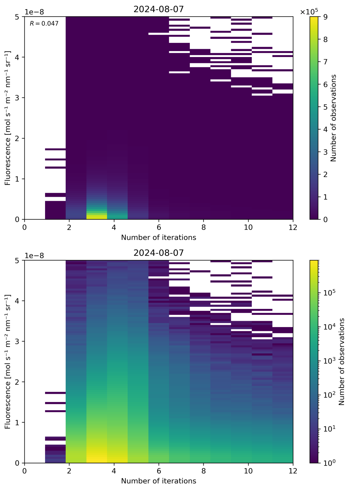
Figure 98: Scatter density plot of “Number of iterations” against “Fluorescence” for 2024-08-06 to 2024-08-08.
