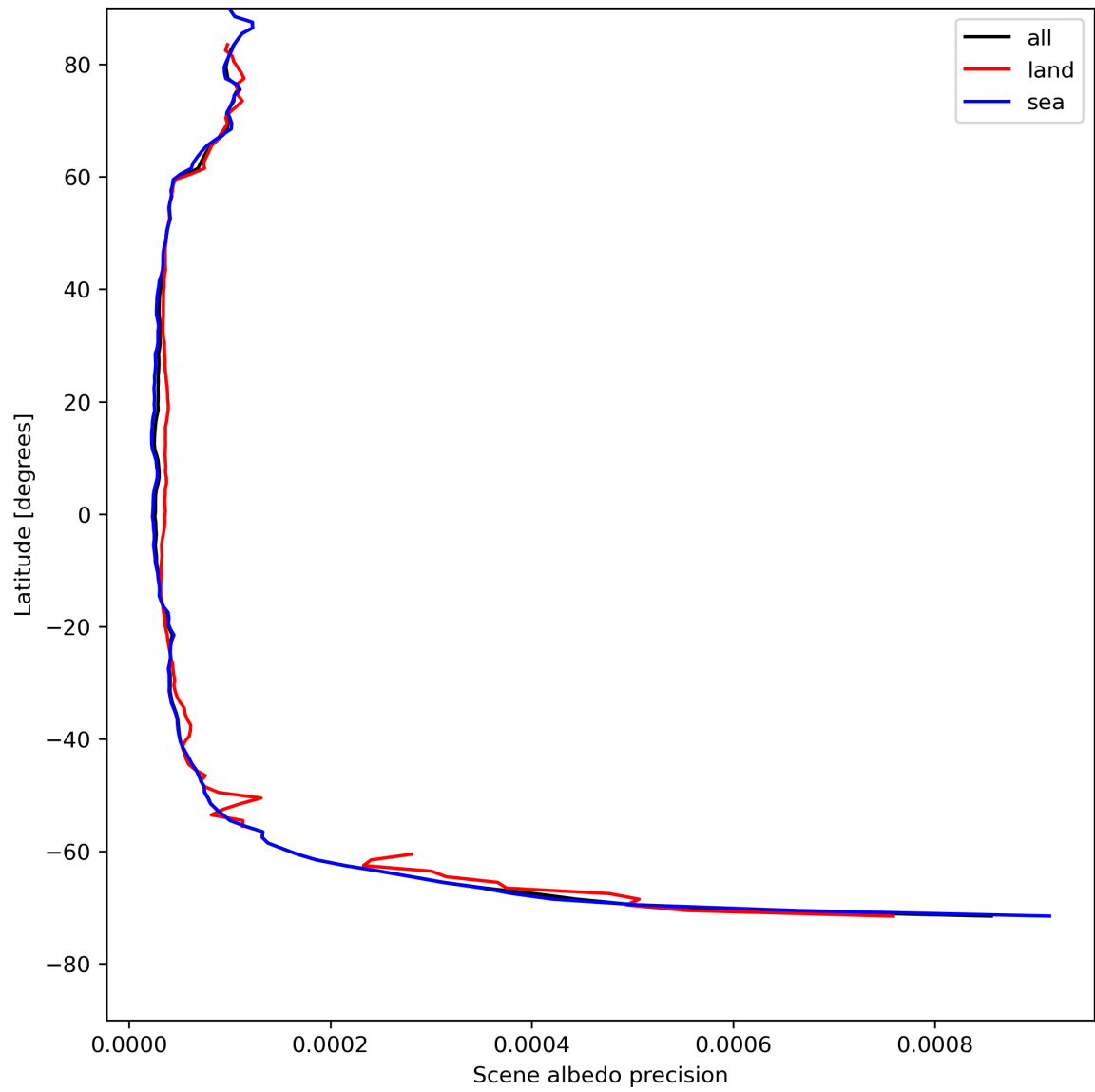
Figure 18: Zonal average of “Scene albedo precision” for 2024-08-06 to 2024-08-08.
