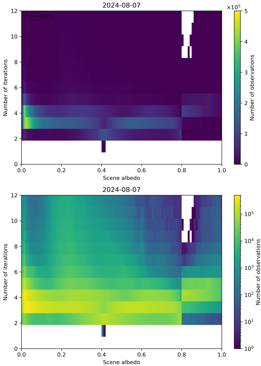
Figure 105: Scatter density plot of “Scene albedo” against “Number of iterations” for 2024-08-06 to 2024-08-08.
