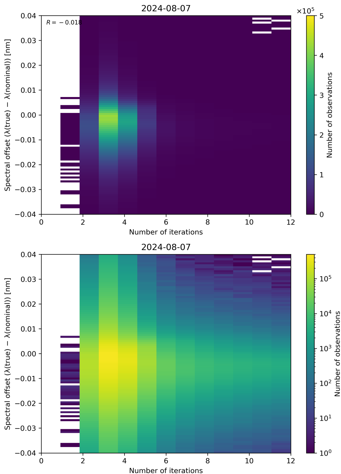
Figure 100: Scatter density plot of “Number of iterations” against “Spectral offset ( \lambda(\text{true}) - \lambda(\text{nominal}) )” for 2024-08-06 to 2024-08-08.
