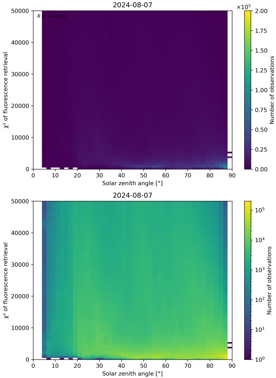
Figure 109: Scatter density plot of “Solar zenith angle” against “ \chi^2 of fluorescence retrieval” for 2024-08-06 to 2024-08-08.
