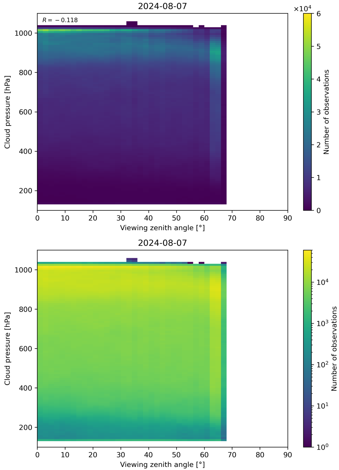
Figure 121: Scatter density plot of “Viewing zenith angle” against “Cloud pressure” for 2024-08-06 to 2024-08-08.
