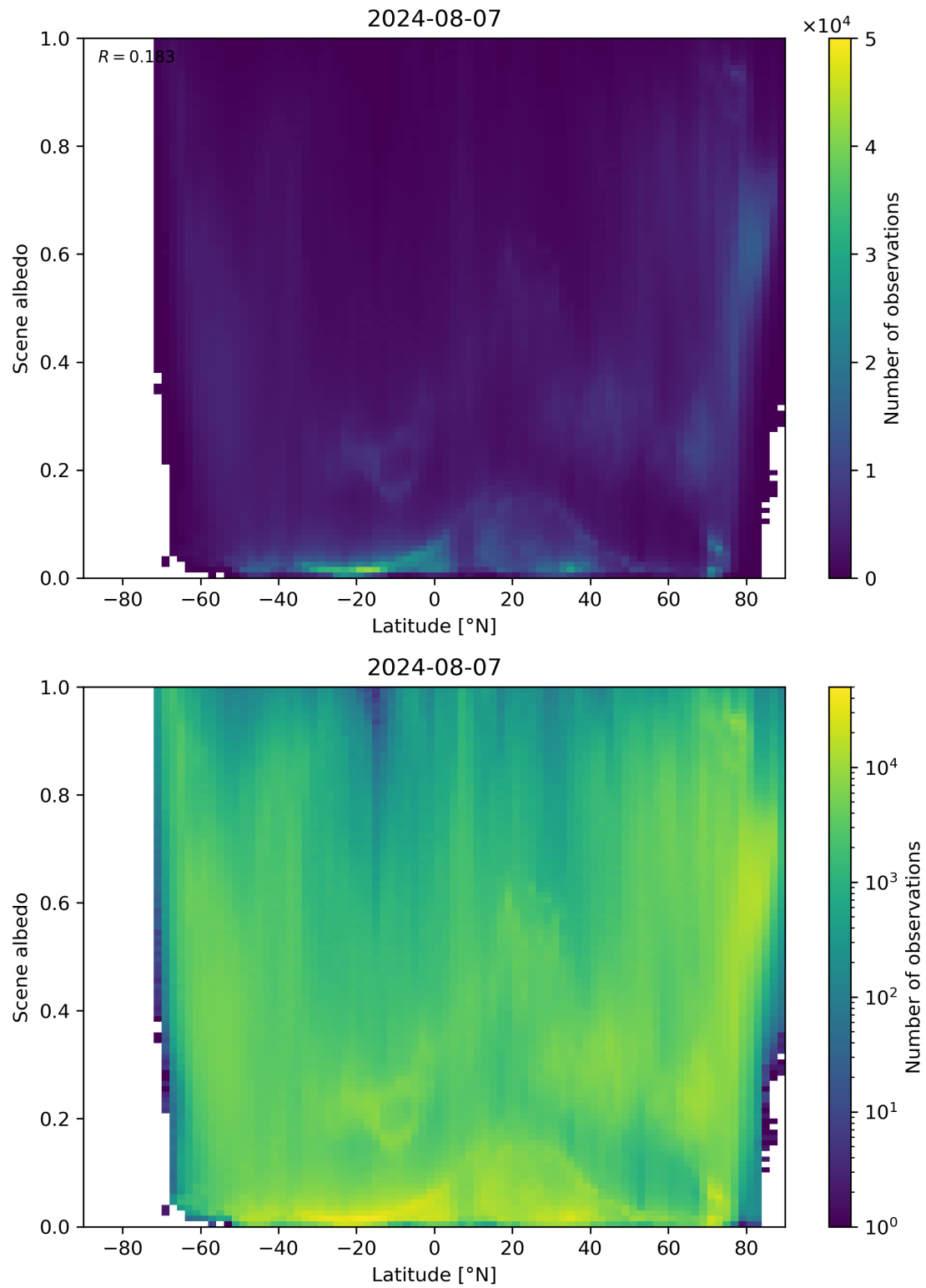
Figure 95: Scatter density plot of “Latitude” against “Scene albedo” for 2024-08-06 to 2024-08-08.
