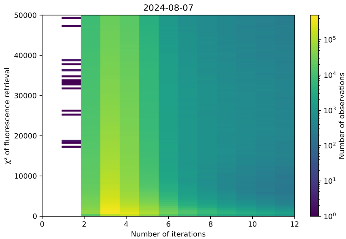
Figure 97: Scatter density plot of “Number of iterations” against “ \chi^2 of fluorescence retrieval” for 2024-08-06 to 2024-08-08.
