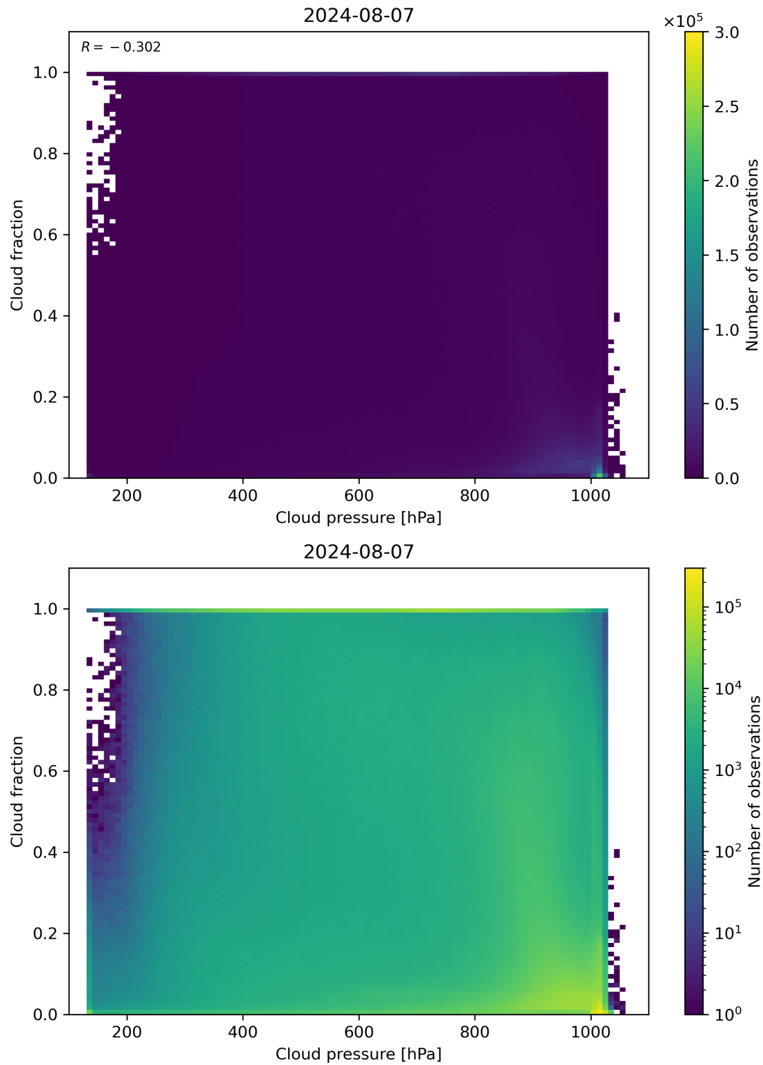
Figure 79: Scatter density plot of “Cloud pressure” against “Cloud fraction” for 2024-08-06 to 2024-08-08.
