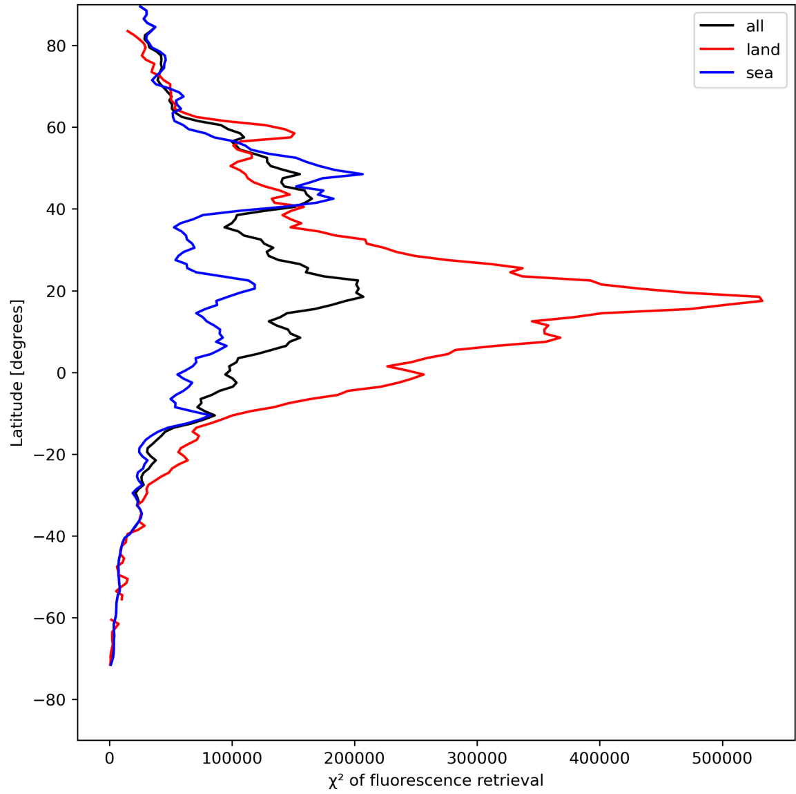
Figure 25: Zonal average of “ \chi^2 of fluorescence retrieval” for 2024-08-06 to 2024-08-08.
