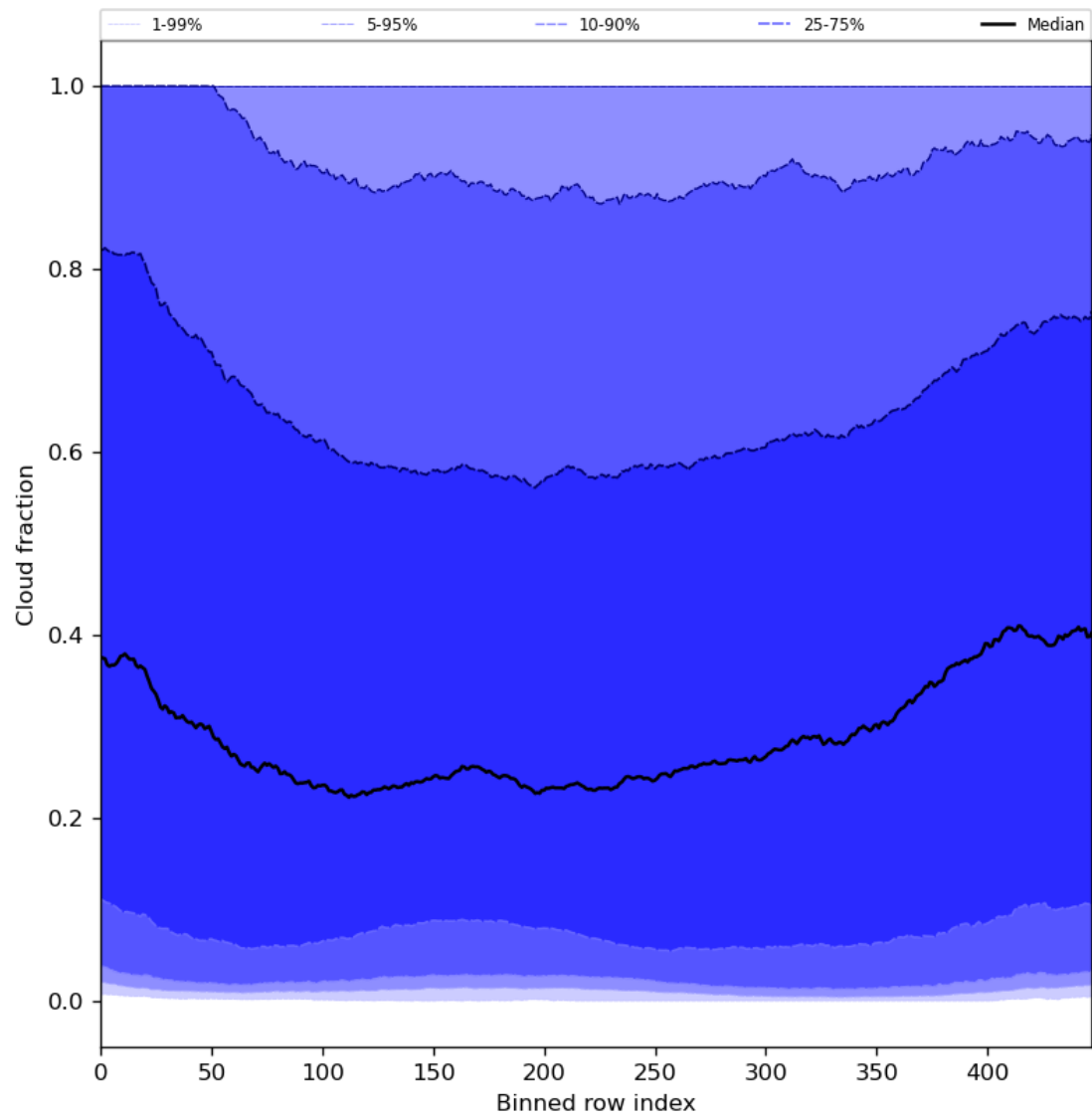
Figure 49: Along track statistics of “Cloud fraction” for 2024-08-06 to 2024-08-08
