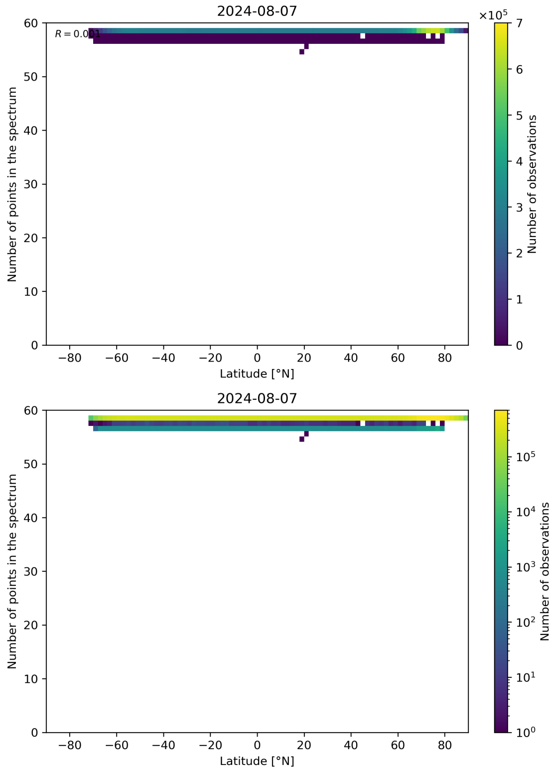
Figure 94: Scatter density plot of “Latitude” against “Number of points in the spectrum” for 2024-08-06 to 2024-08-08.
