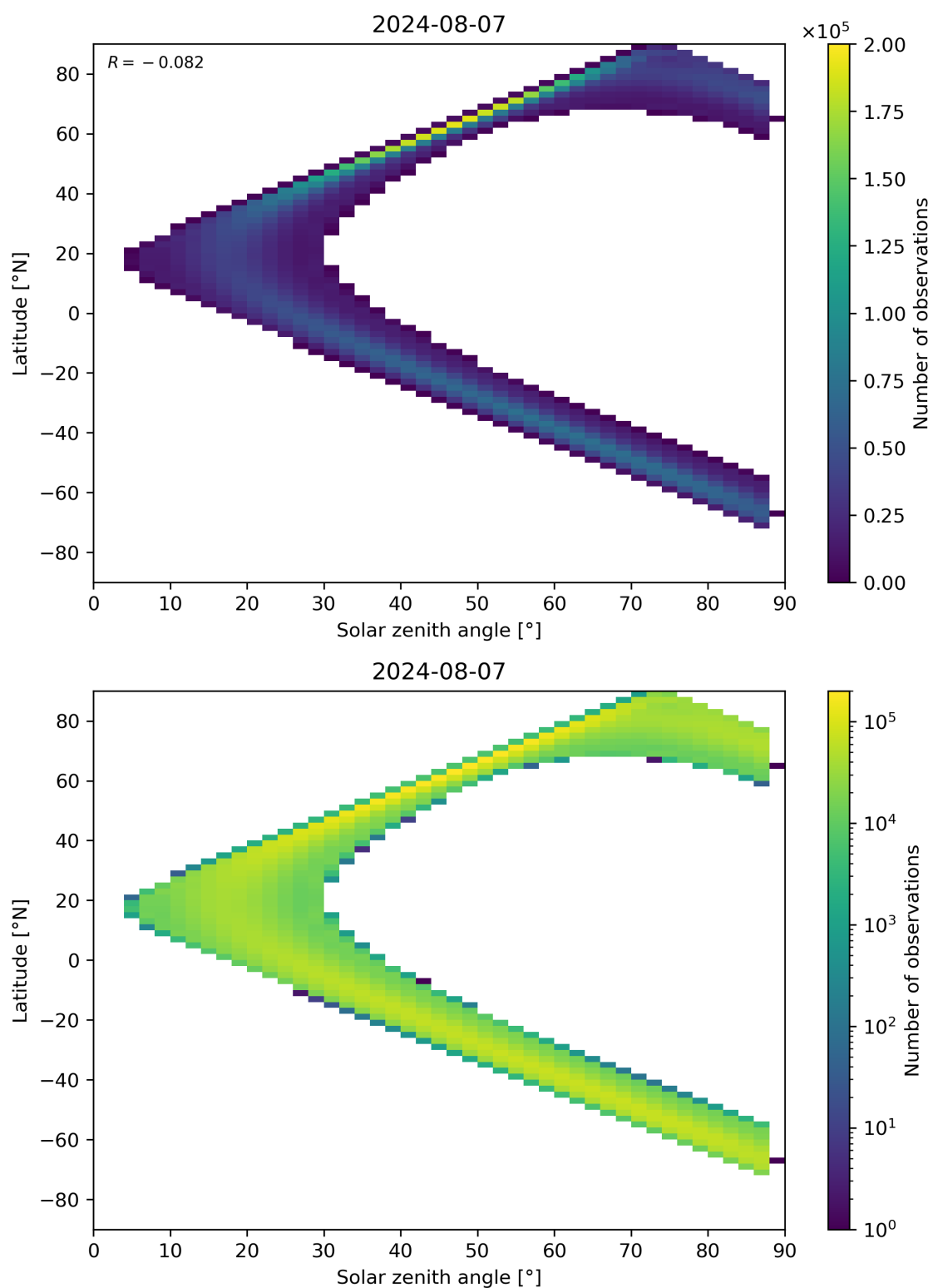
Figure 113: Scatter density plot of “Solar zenith angle” against “Latitude” for 2024-08-06 to 2024-08-08.
