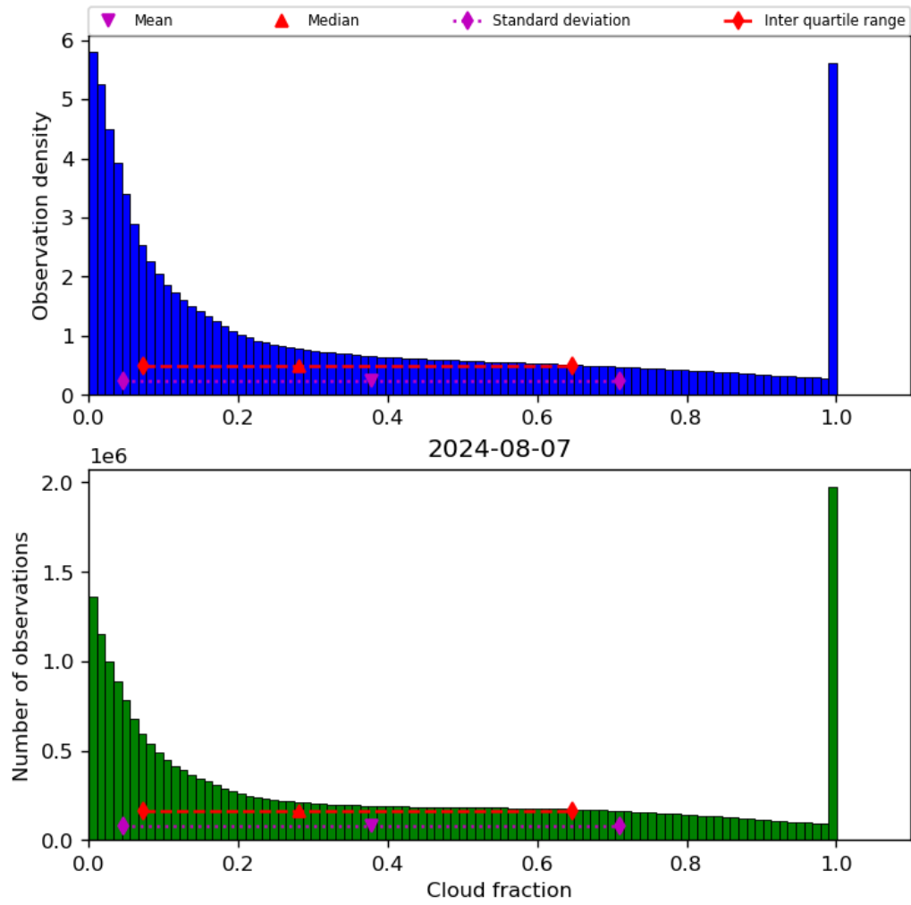
Figure 32: Histogram of “Cloud fraction” for 2024-08-06 to 2024-08-08
