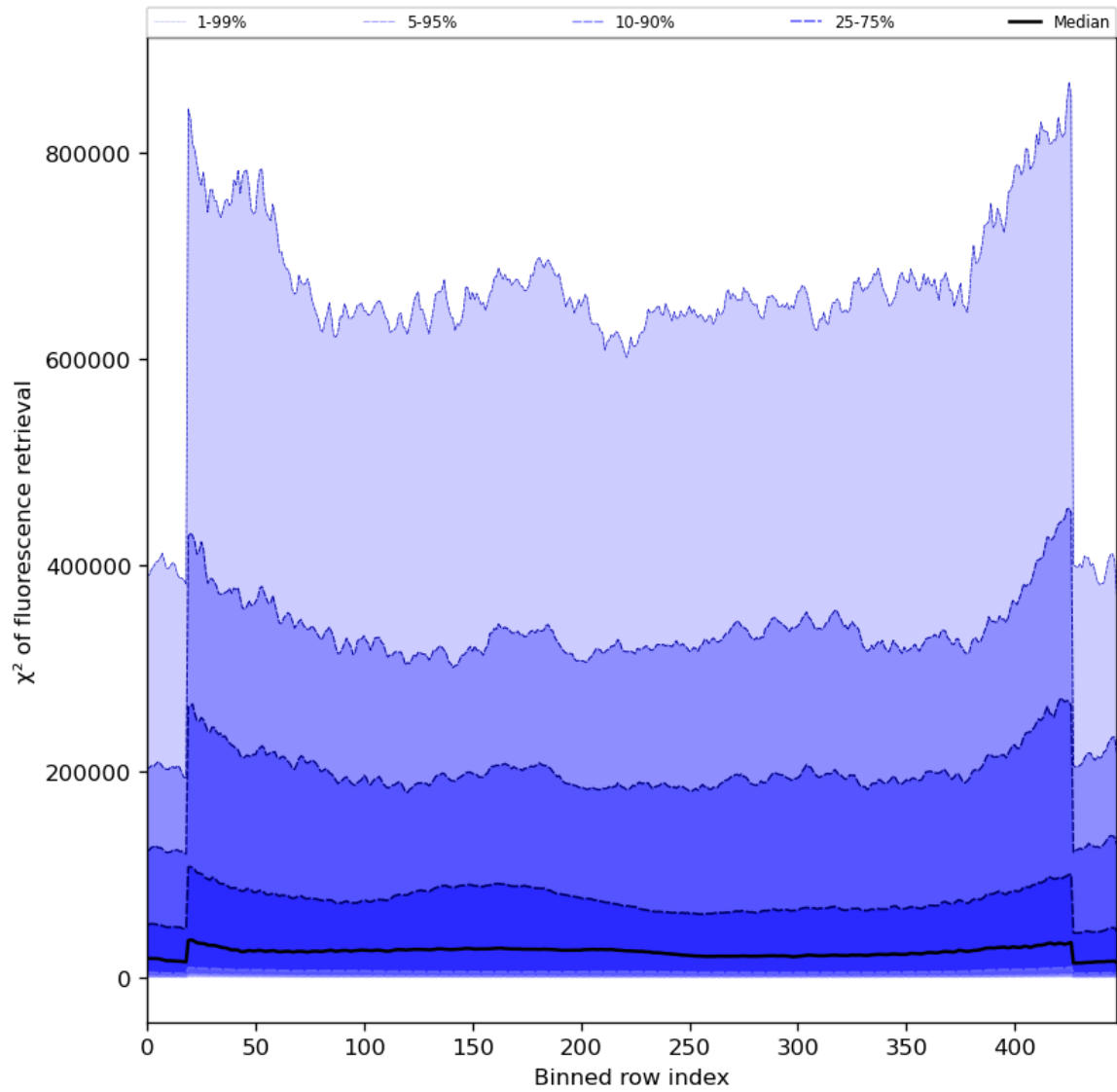
Figure 59: Along track statistics of “ \chi^2 of fluorescence retrieval” for 2024-08-06 to 2024-08-08
