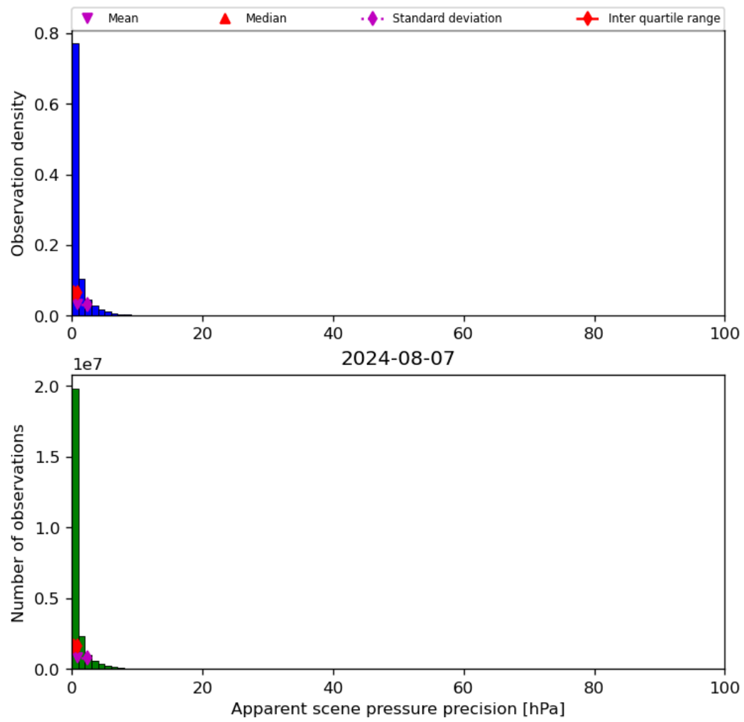
Figure 37: Histogram of “Apparent scene pressure precision” for 2024-08-06 to 2024-08-08
