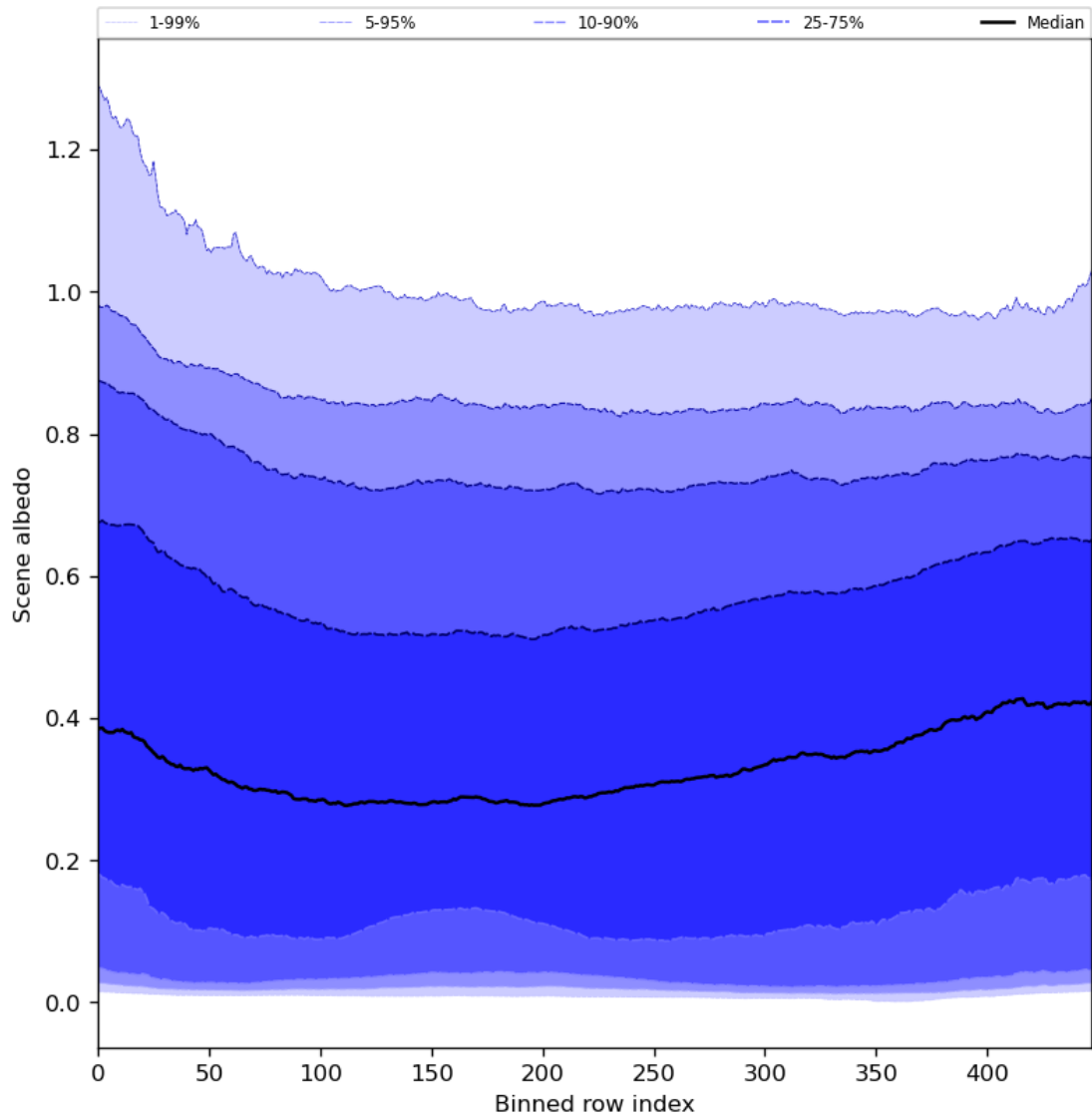
Figure 51: Along track statistics of “Scene albedo” for 2024-08-06 to 2024-08-08
