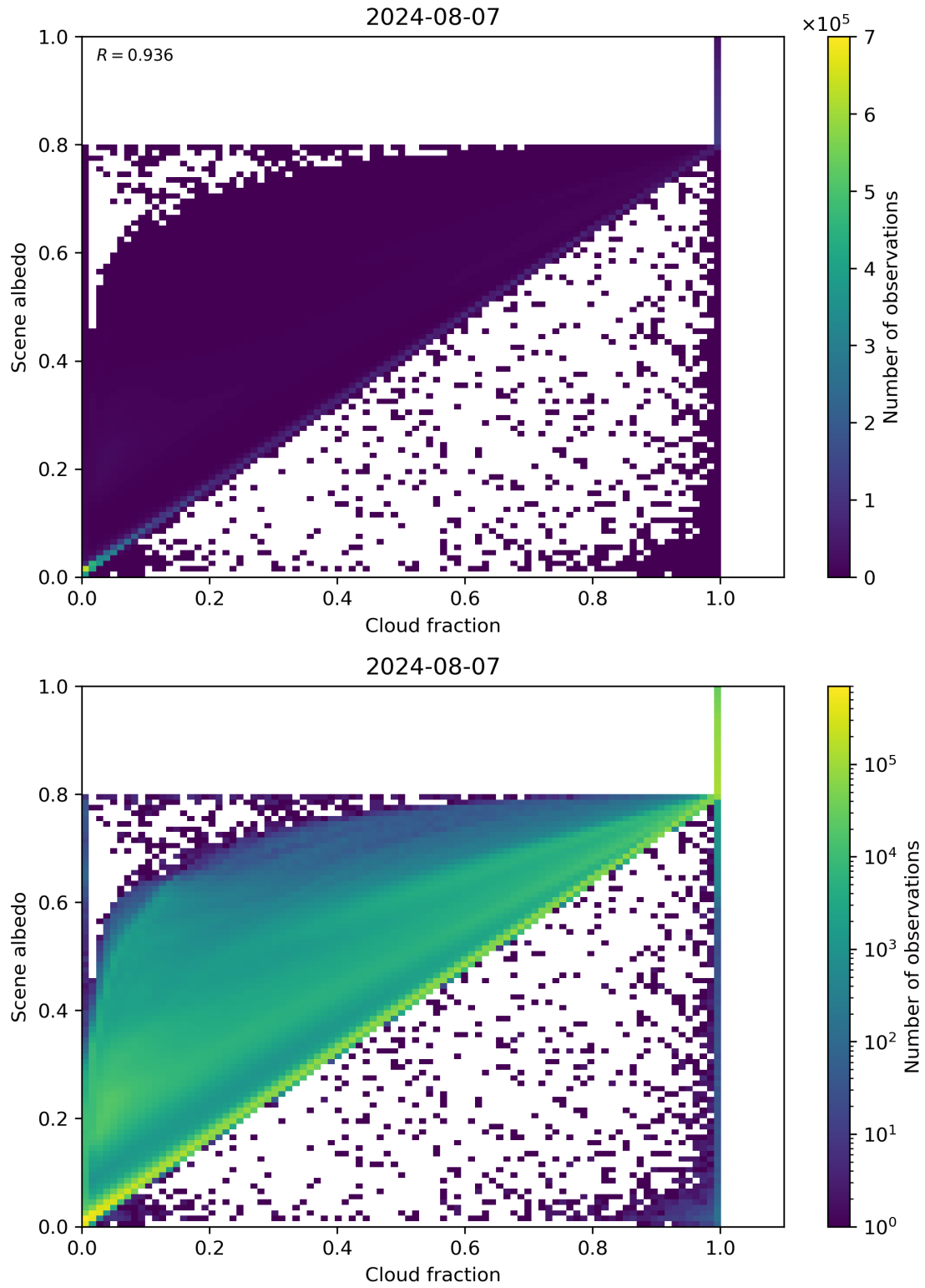
Figure 75: Scatter density plot of “Cloud fraction” against “Scene albedo” for 2024-08-06 to 2024-08-08.
