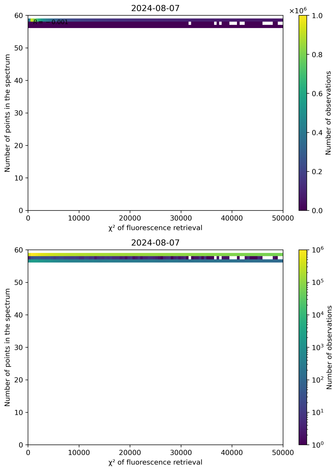
Figure 68: Scatter density plot of " \chi^2 of fluorescence retrieval" against "Number of points in the spectrum" for 2024-08-06 to 2024-08-08.
