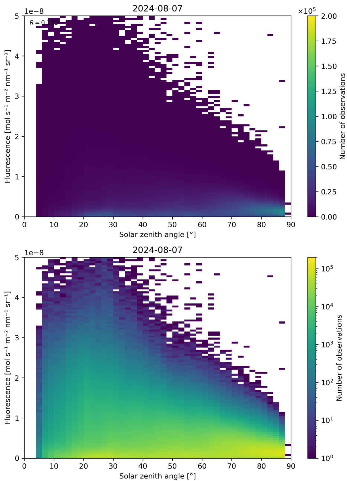
Figure 112: Scatter density plot of “Solar zenith angle” against “Fluorescence” for 2024-08-06 to 2024-08-08.
