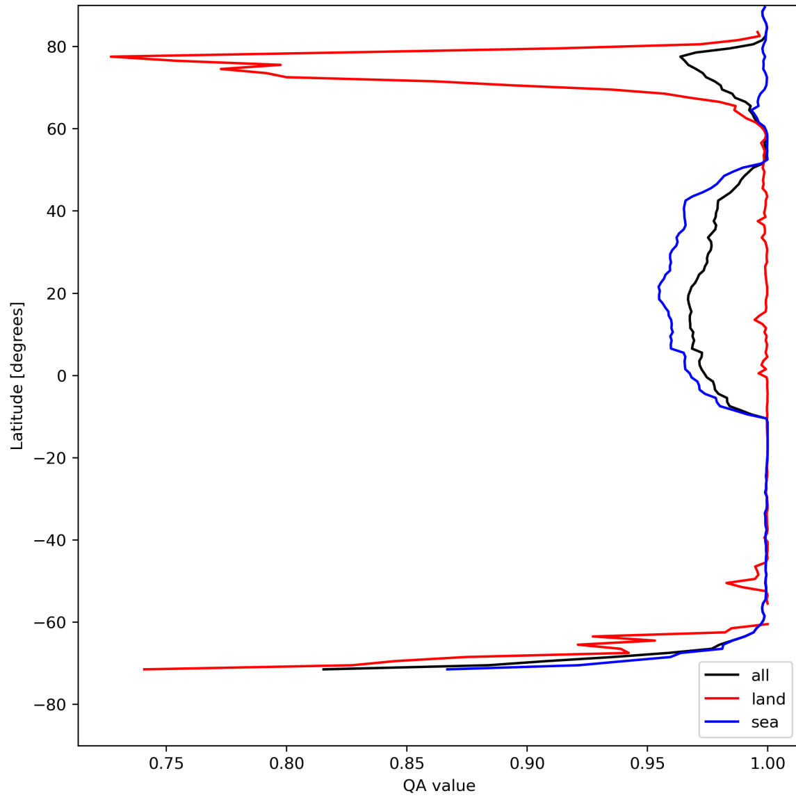
Figure 12: Zonal average of “QA value” for 2024-08-06 to 2024-08-08.
