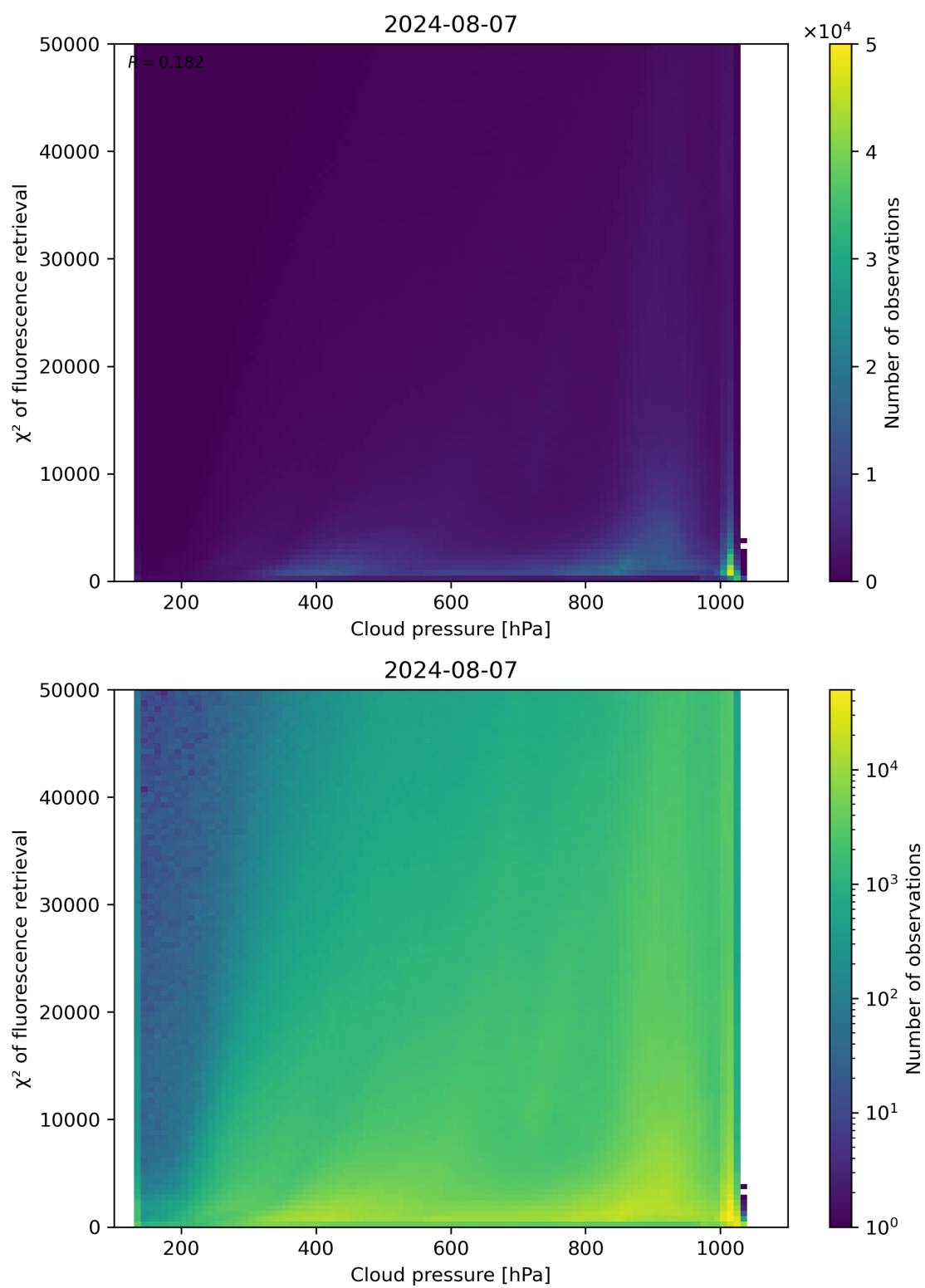
Figure 78: Scatter density plot of “Cloud pressure” against “ \chi^2 of fluorescence retrieval” for 2024-08-06 to 2024-08-08.
