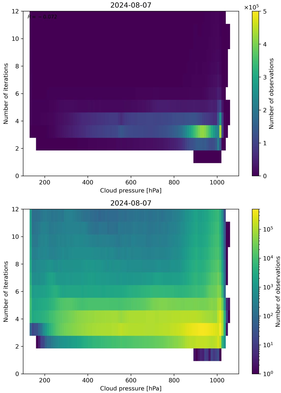
Figure 81: Scatter density plot of “Cloud pressure” against “Number of iterations” for 2024-08-06 to 2024-08-08.
