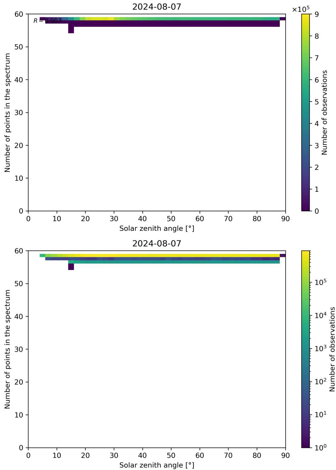
Figure 115: Scatter density plot of “Solar zenith angle” against “Number of points in the spectrum” for 2024-08-06 to 2024-08-08.
