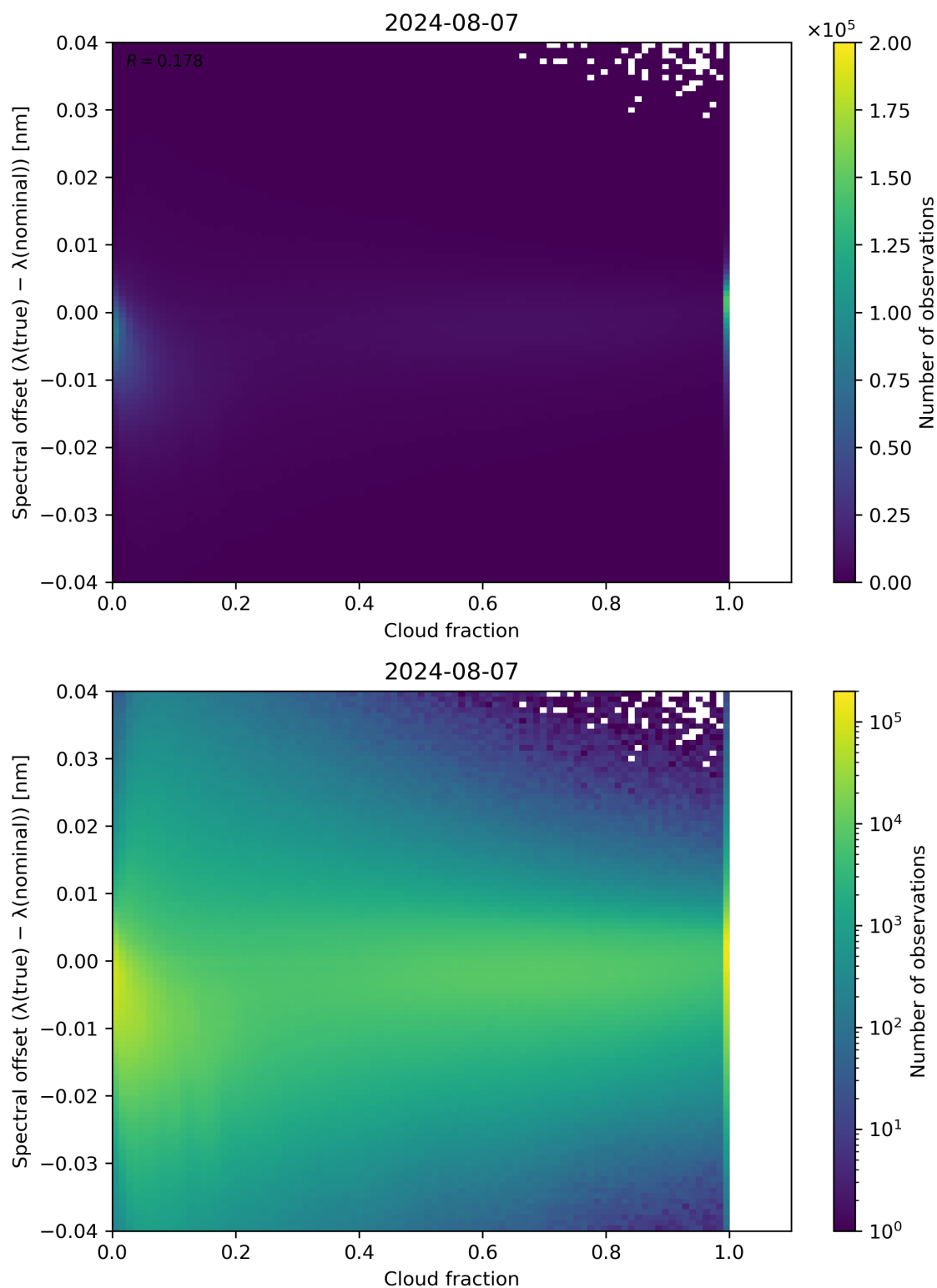
Figure 76: Scatter density plot of “Cloud fraction” against “Spectral offset ( \lambda(\text{true}) - \lambda(\text{nominal}) )” for 2024-08-06 to 2024-08-08.
