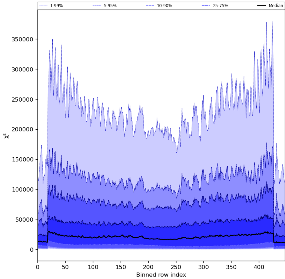
Figure 55: Along track statistics of “ \chi^2 ” for 2024-08-06 to 2024-08-08
