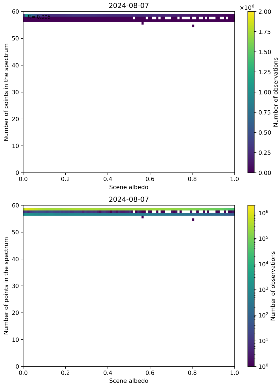
Figure 106: Scatter density plot of “Scene albedo” against “Number of points in the spectrum” for 2024-08-06 to 2024-08-08.
