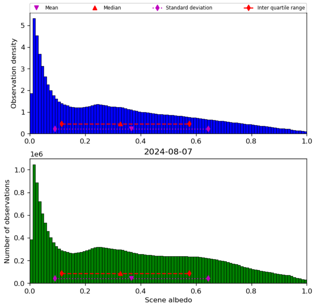
Figure 34: Histogram of “Scene albedo” for 2024-08-06 to 2024-08-08
