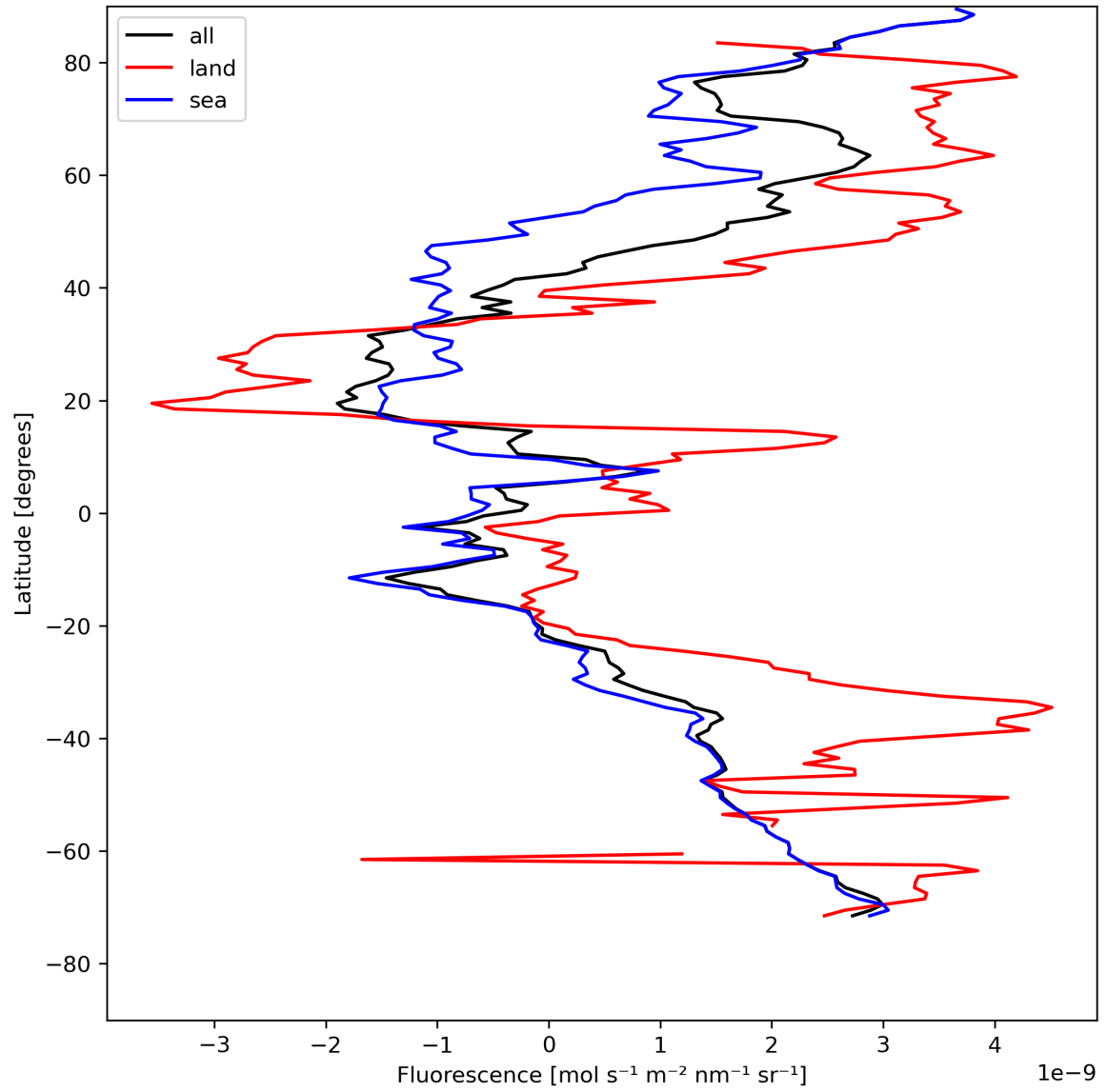
Figure 23: Zonal average of “Fluorescence” for 2024-08-06 to 2024-08-08.
