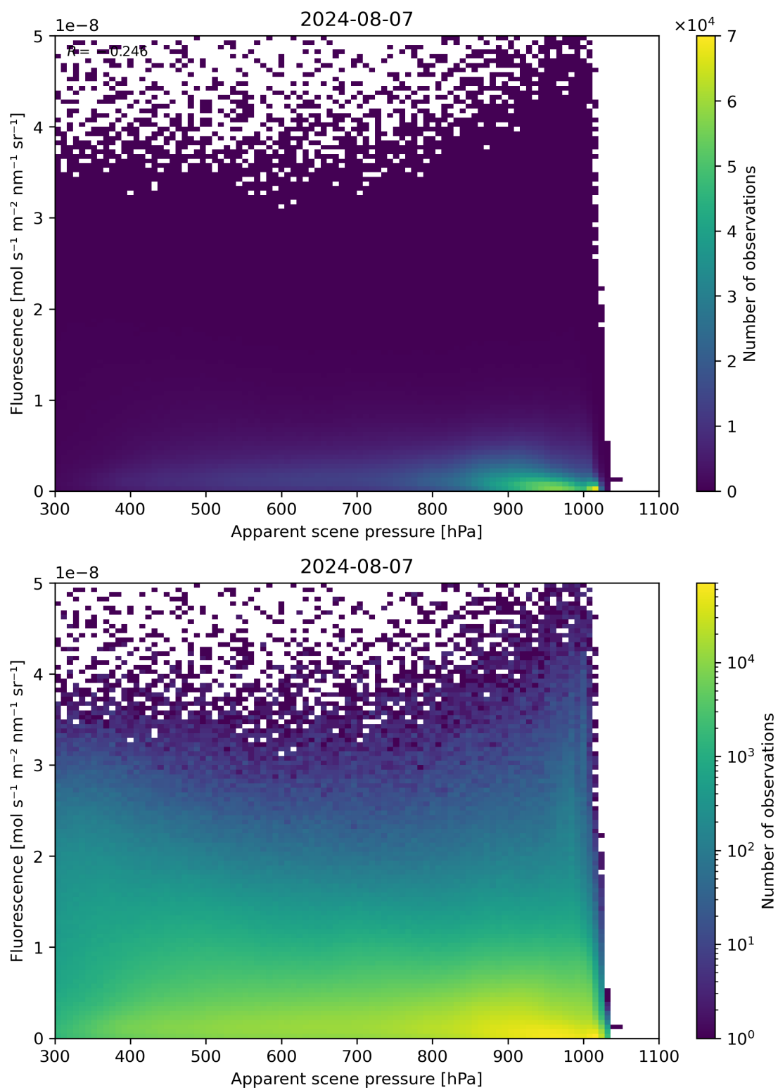
Figure 64: Scatter density plot of “Apparent scene pressure” against “Fluorescence” for 2024-08-06 to 2024-08-08.
