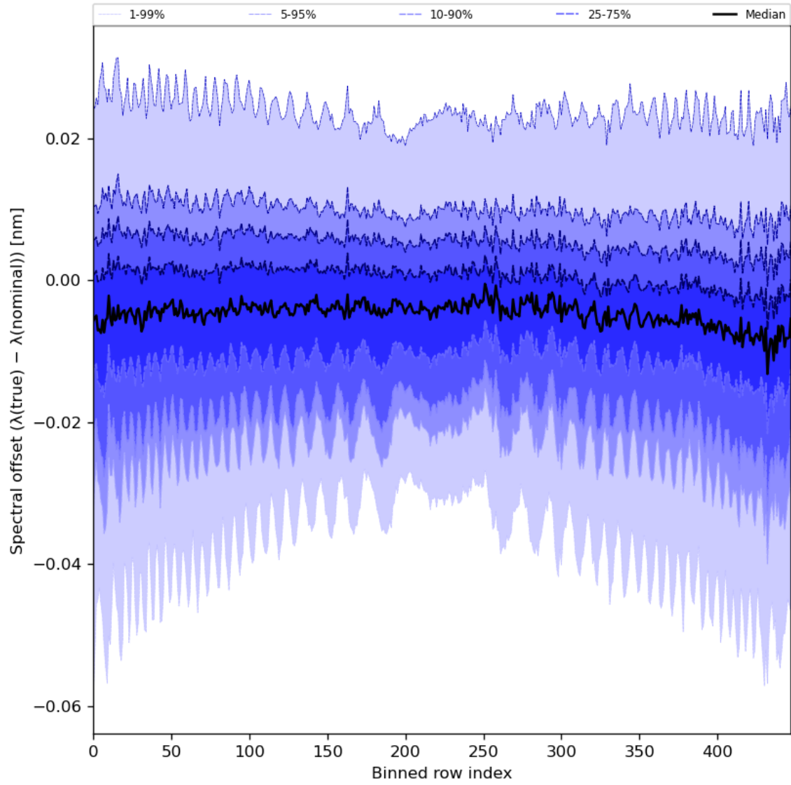
Figure 62: Along track statistics of “Spectral offset ( \lambda(\text{true}) - \lambda(\text{nominal}) )” for 2024-08-06 to 2024-08-08
