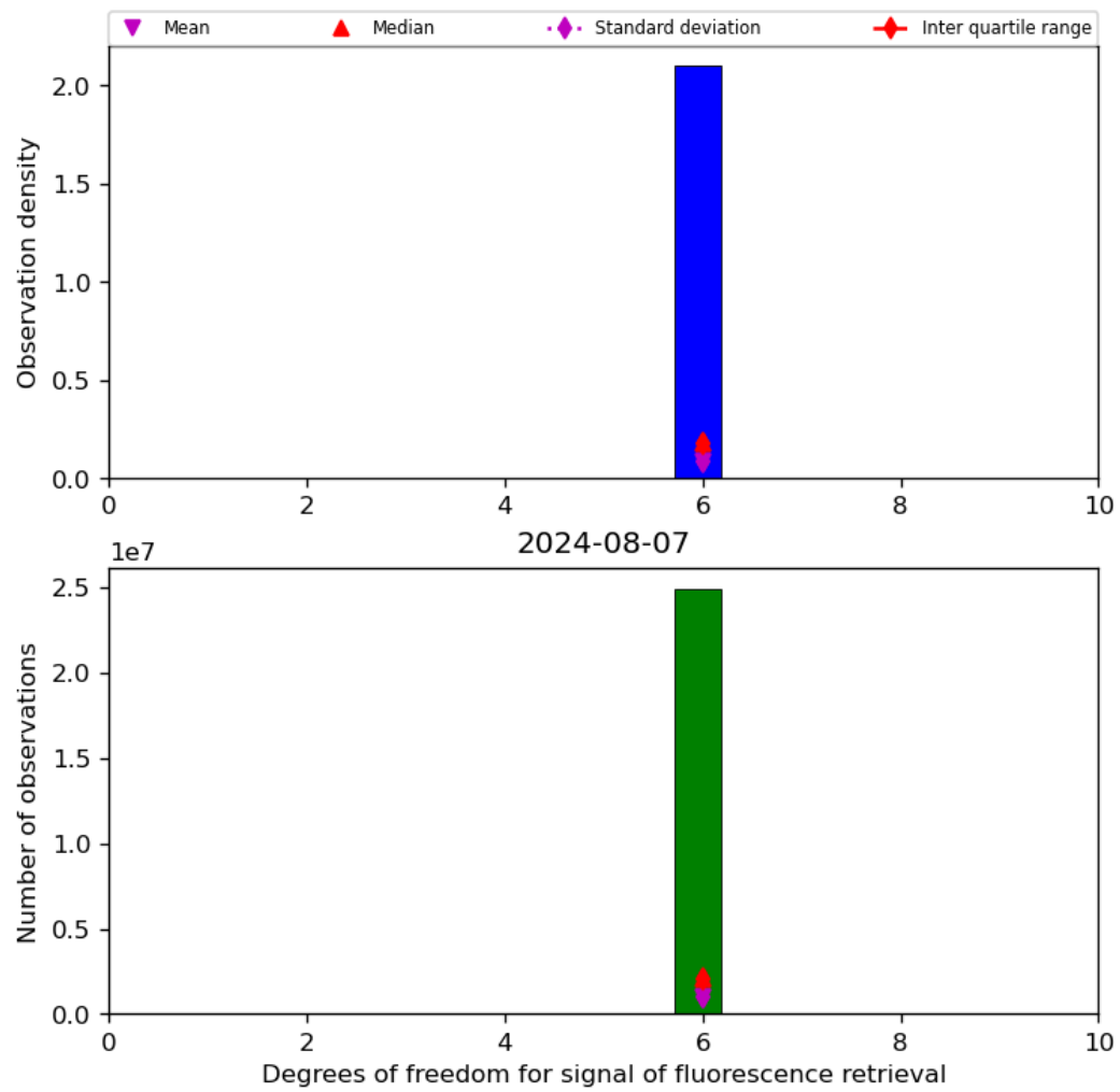
Figure 43: Histogram of “Degrees of freedom for signal of fluorescence retrieval” for 2024-08-06 to 2024-08-08
