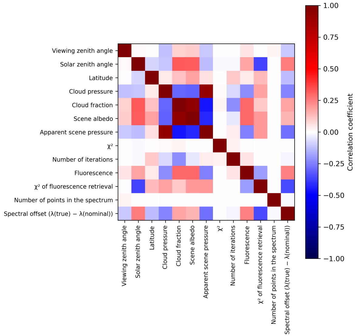
Figure 2: Map of correlation matrix for 2024-08-06 to 2024-08-08.
