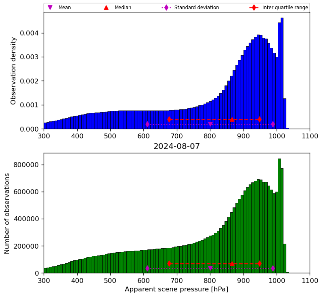
Figure 36: Histogram of “Apparent scene pressure” for 2024-08-06 to 2024-08-08
