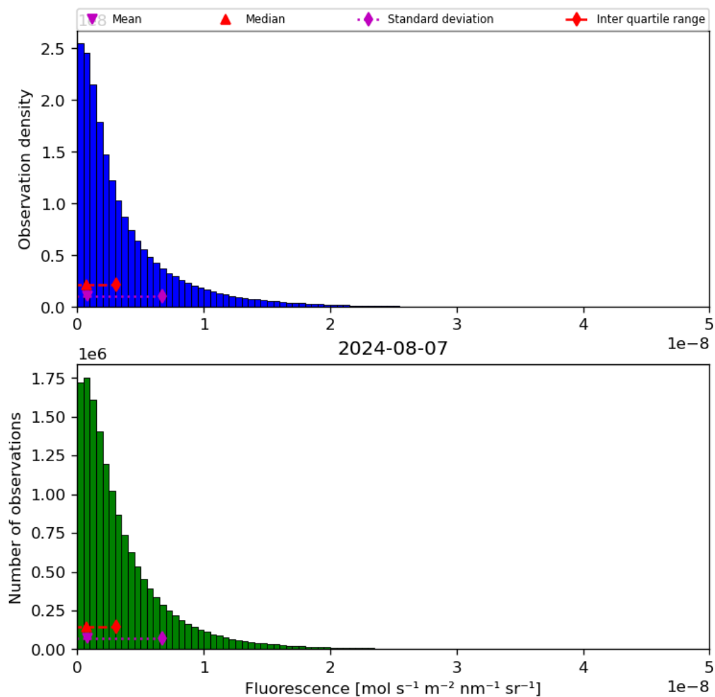
Figure 40: Histogram of “Fluorescence” for 2024-08-06 to 2024-08-08
