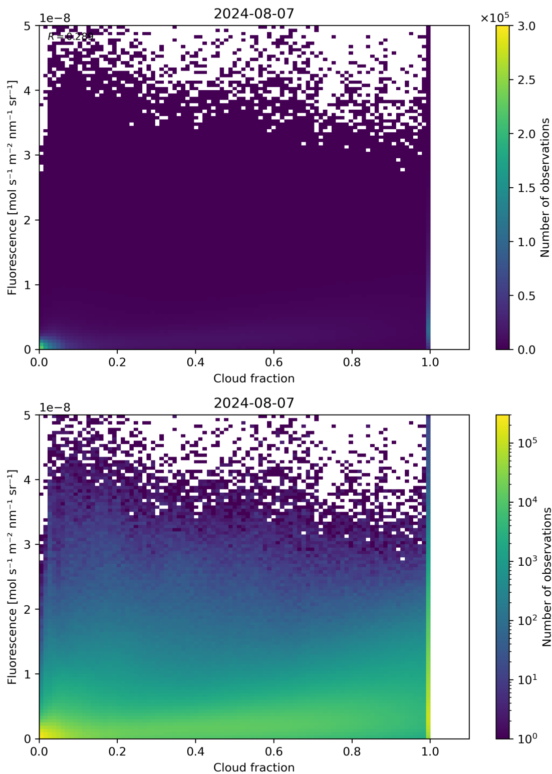
Figure 72: Scatter density plot of “Cloud fraction” against “Fluorescence” for 2024-08-06 to 2024-08-08.
