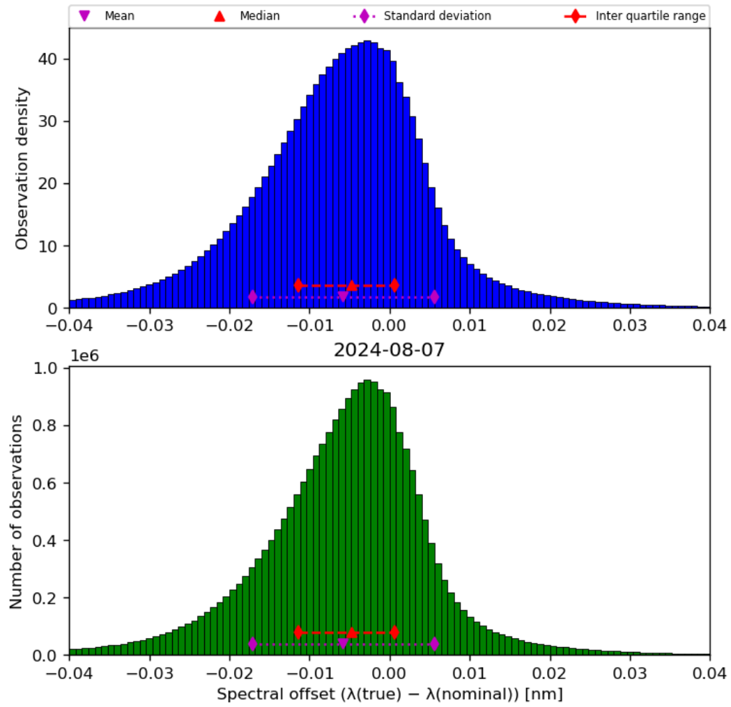
Figure 45: Histogram of “Spectral offset ( \lambda(\text{true}) - \lambda(\text{nominal}) )” for 2024-08-06 to 2024-08-08
