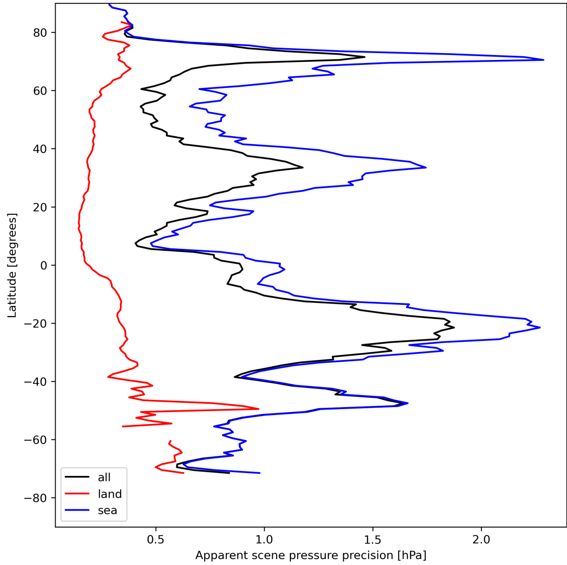
Figure 20: Zonal average of “Apparent scene pressure precision” for 2024-08-06 to 2024-08-08.
