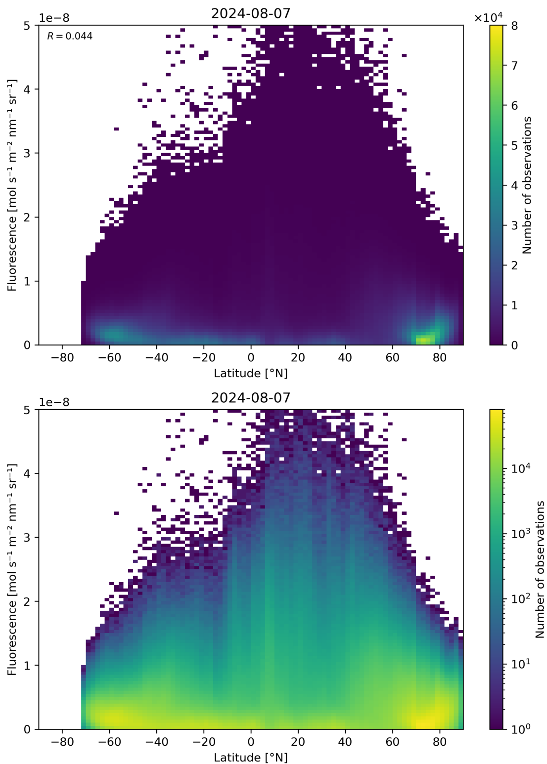
Figure 92: Scatter density plot of “Latitude” against “Fluorescence” for 2024-08-06 to 2024-08-08.
