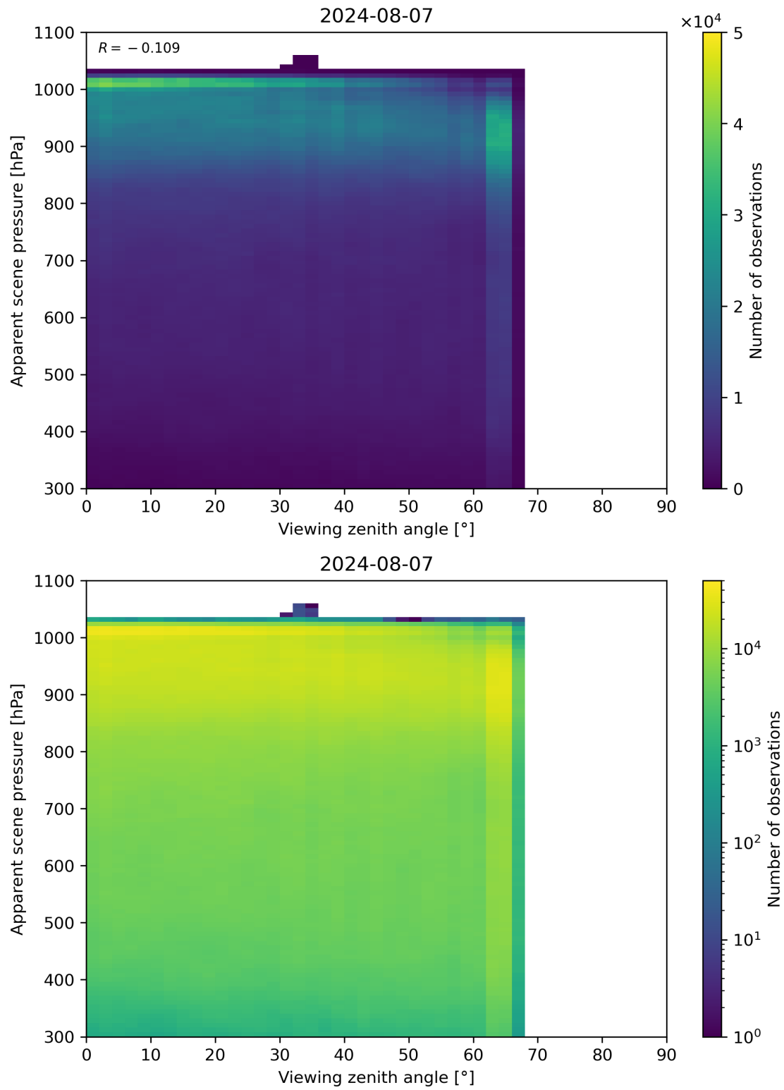
Figure 118: Scatter density plot of “Viewing zenith angle” against “Apparent scene pressure” for 2024-08-06 to 2024-08-08.
