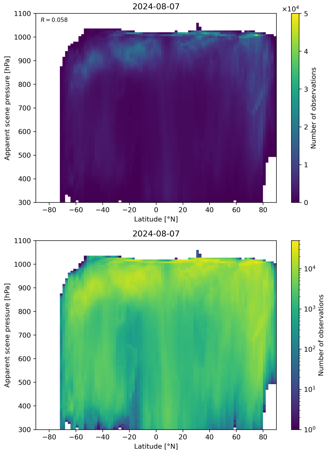
Figure 88: Scatter density plot of “Latitude” against “Apparent scene pressure” for 2024-08-06 to 2024-08-08.
