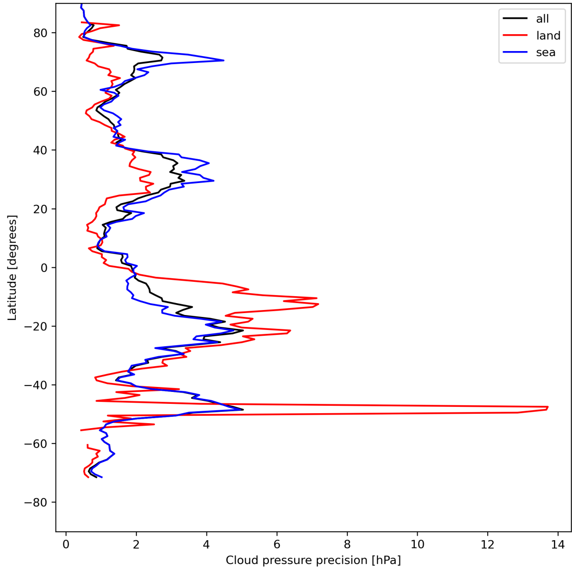
Figure 14: Zonal average of “Cloud pressure precision” for 2024-08-06 to 2024-08-08.
