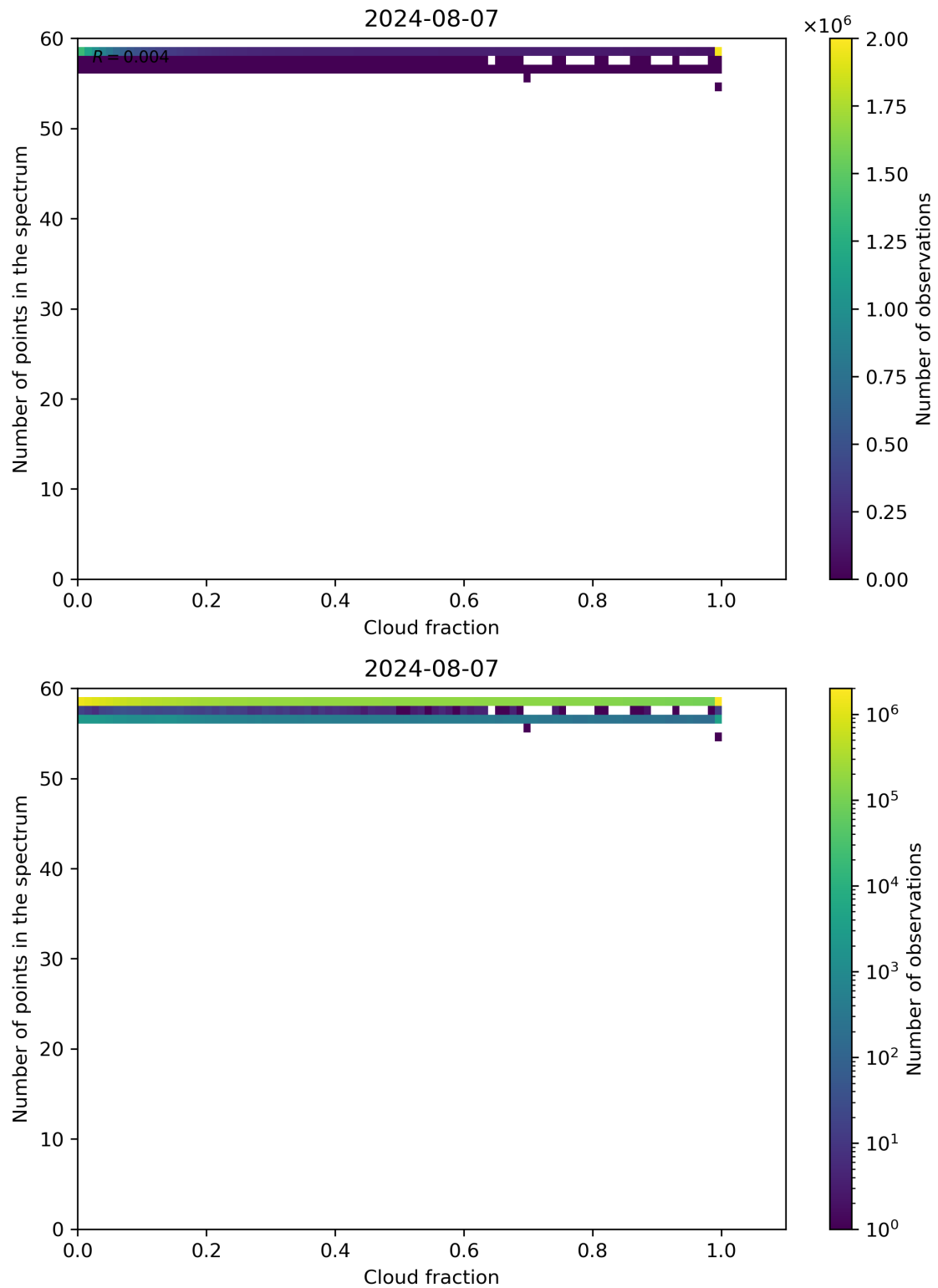
Figure 74: Scatter density plot of “Cloud fraction” against “Number of points in the spectrum” for 2024-08-06 to 2024-08-08.
