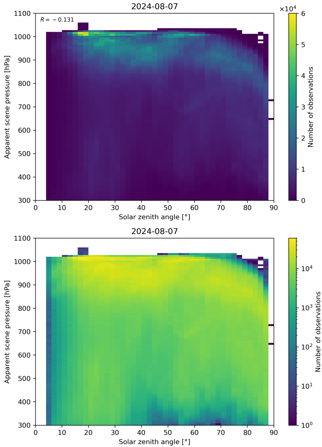
Figure 108: Scatter density plot of “Solar zenith angle” against “Apparent scene pressure” for 2024-08-06 to 2024-08-08.
