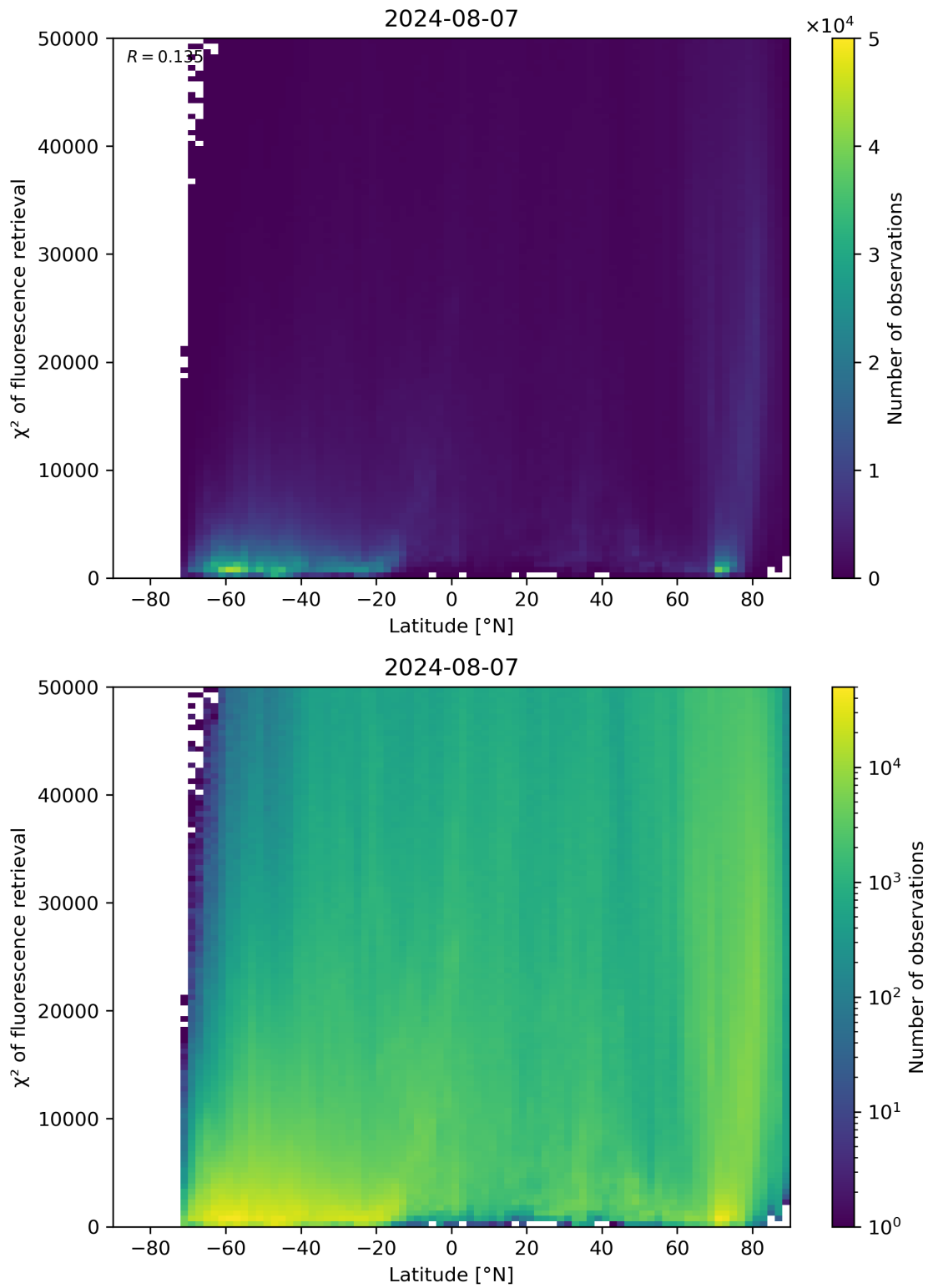
Figure 89: Scatter density plot of “Latitude” against “ \chi^2 of fluorescence retrieval” for 2024-08-06 to 2024-08-08.
