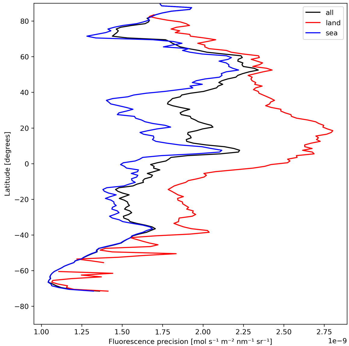
Figure 24: Zonal average of “Fluorescence precision” for 2024-08-06 to 2024-08-08.
