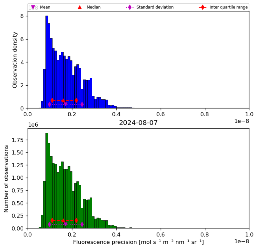
Figure 41: Histogram of “Fluorescence precision” for 2024-08-06 to 2024-08-08
