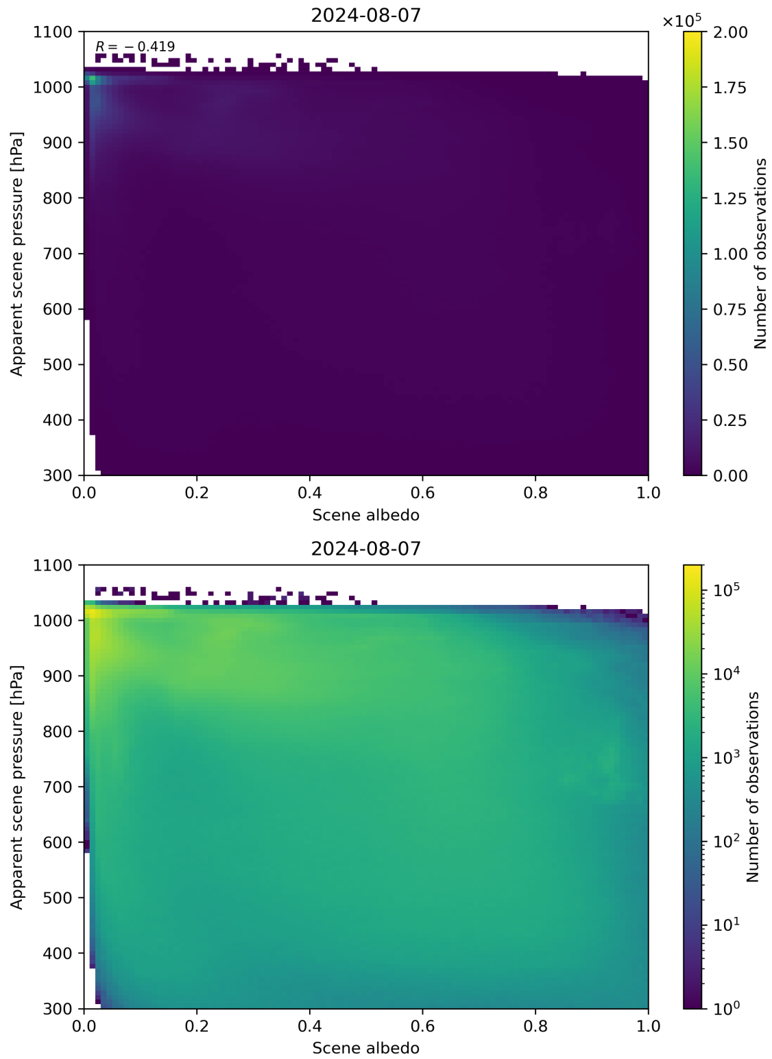
Figure 102: Scatter density plot of “Scene albedo” against “Apparent scene pressure” for 2024-08-06 to 2024-08-08.
