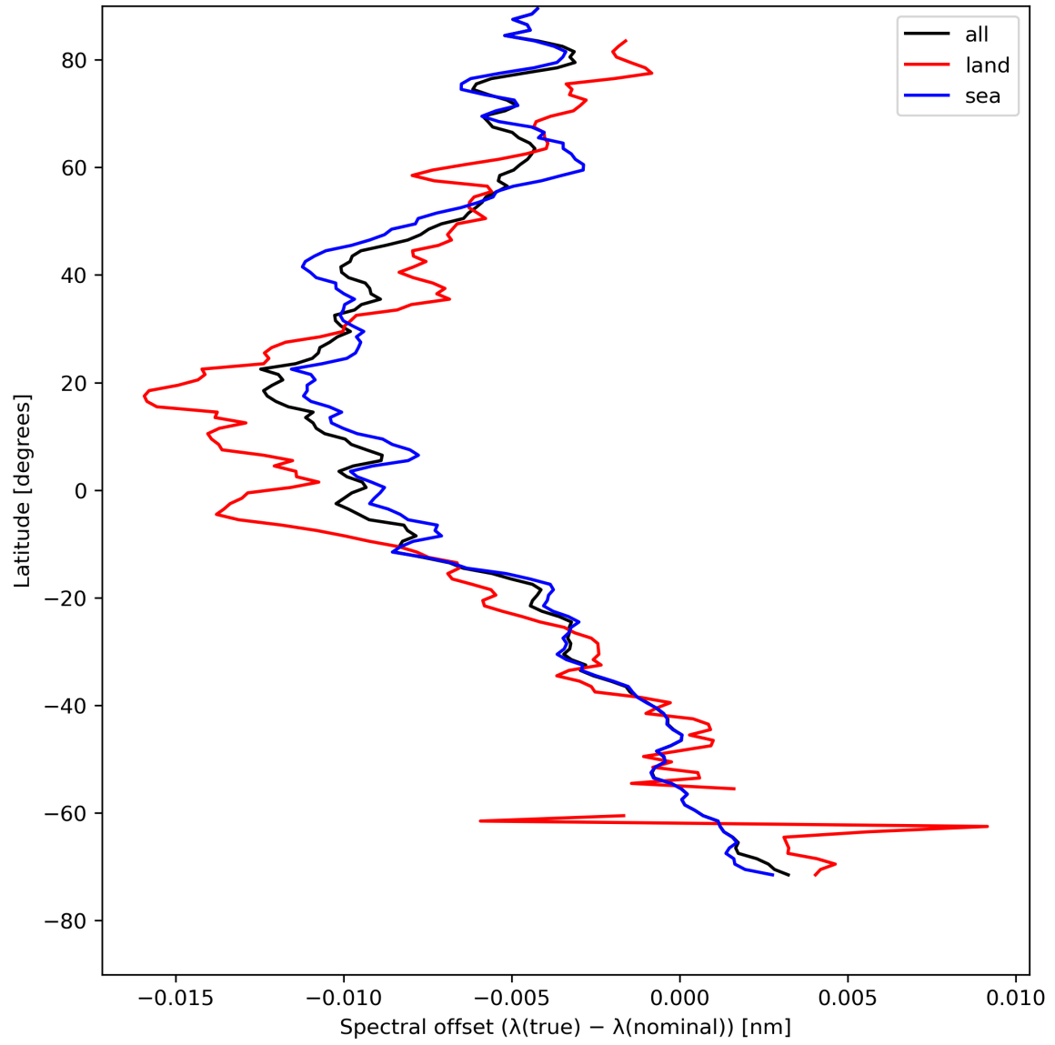
Figure 28: Zonal average of “Spectral offset ( \lambda(\text{true}) - \lambda(\text{nominal}) )” for 2024-08-06 to 2024-08-08.
