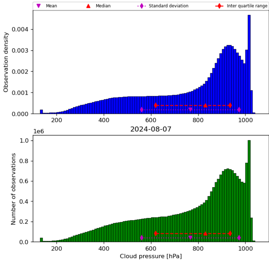
Figure 30: Histogram of “Cloud pressure” for 2024-08-06 to 2024-08-08
