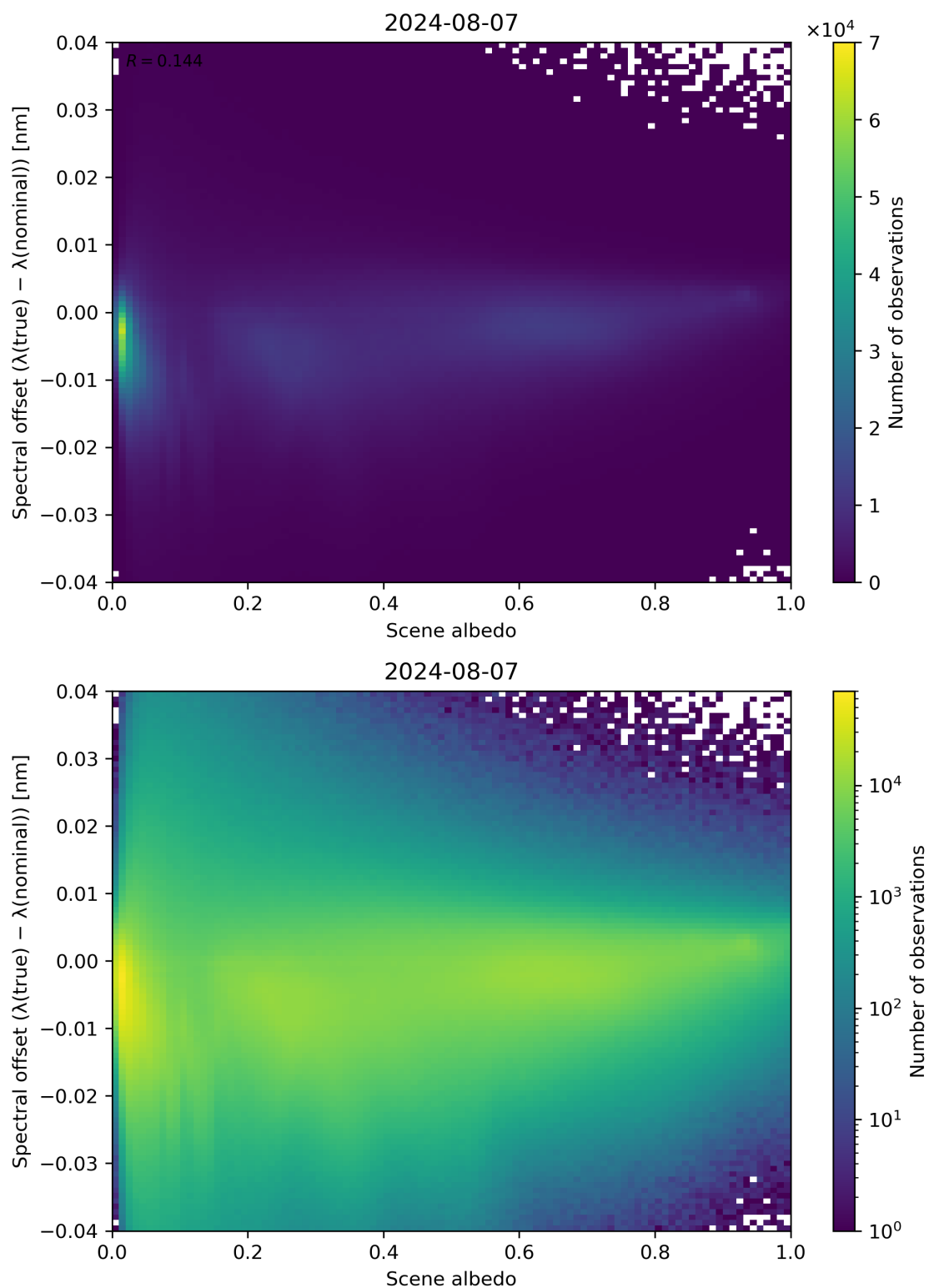
Figure 107: Scatter density plot of “Scene albedo” against “Spectral offset ( \lambda(\text{true}) - \lambda(\text{nominal}) )” for 2024-08-06 to 2024-08-08.
