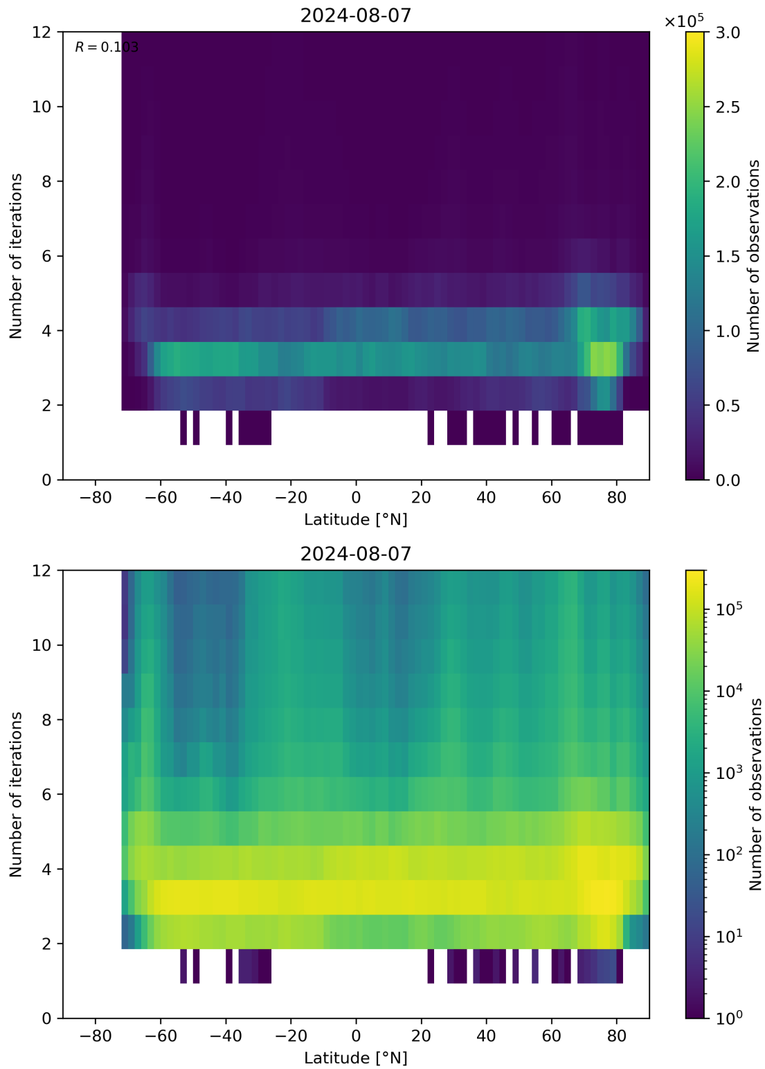
Figure 93: Scatter density plot of “Latitude” against “Number of iterations” for 2024-08-06 to 2024-08-08.
