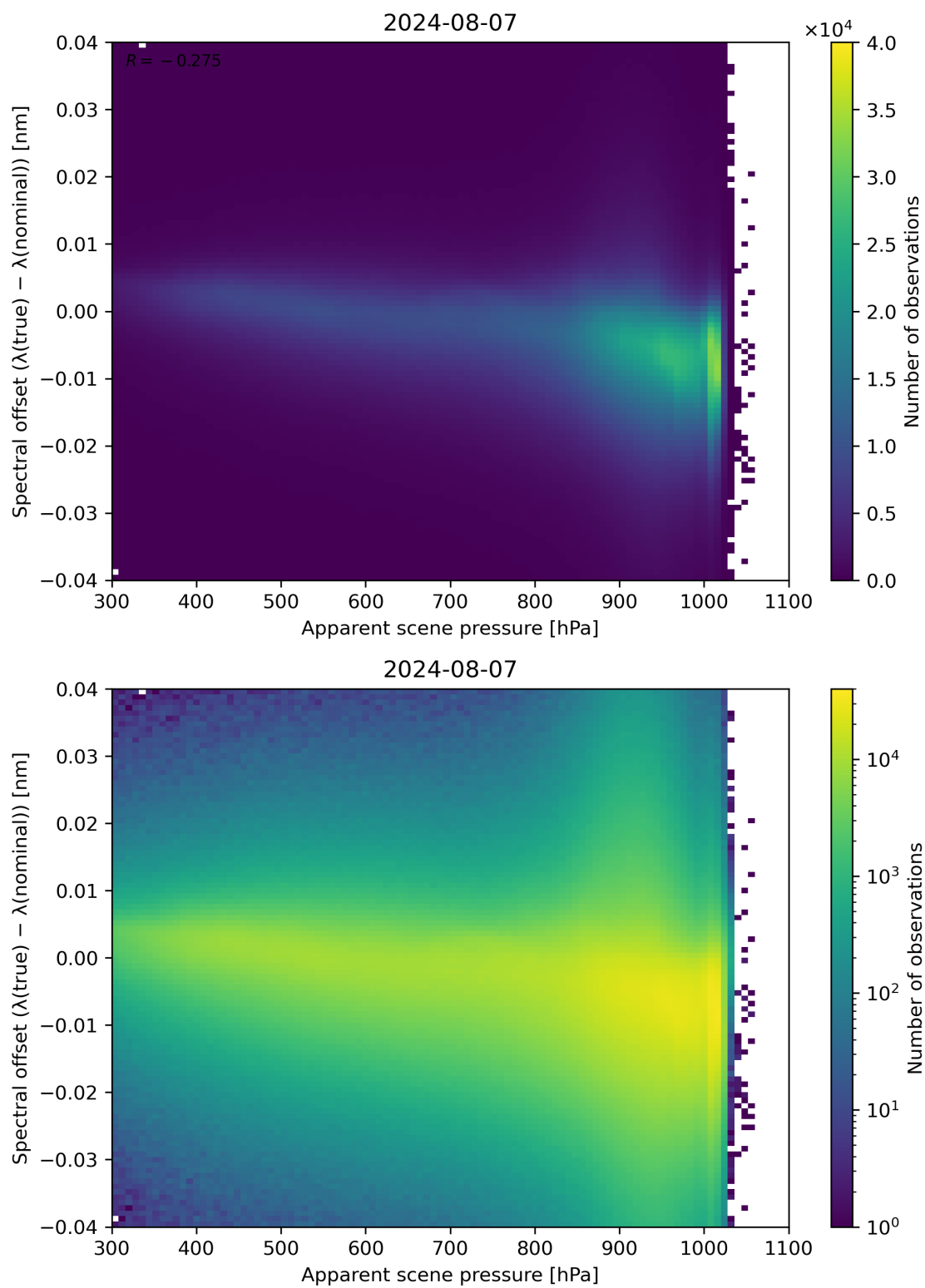
Figure 67: Scatter density plot of “Apparent scene pressure” against “Spectral offset ( \lambda(\text{true}) - \lambda(\text{nominal}) )” for 2024-08-06 to 2024-08-08.
