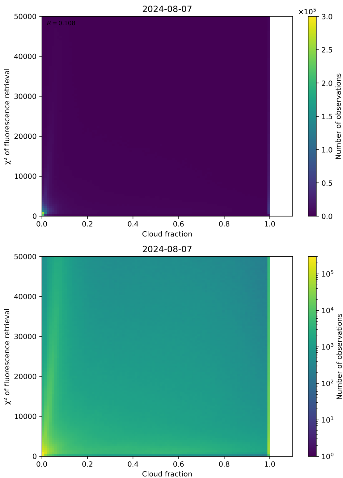
Figure 71: Scatter density plot of “Cloud fraction” against “ \chi^2 of fluorescence retrieval” for 2024-08-06 to 2024-08-08.
