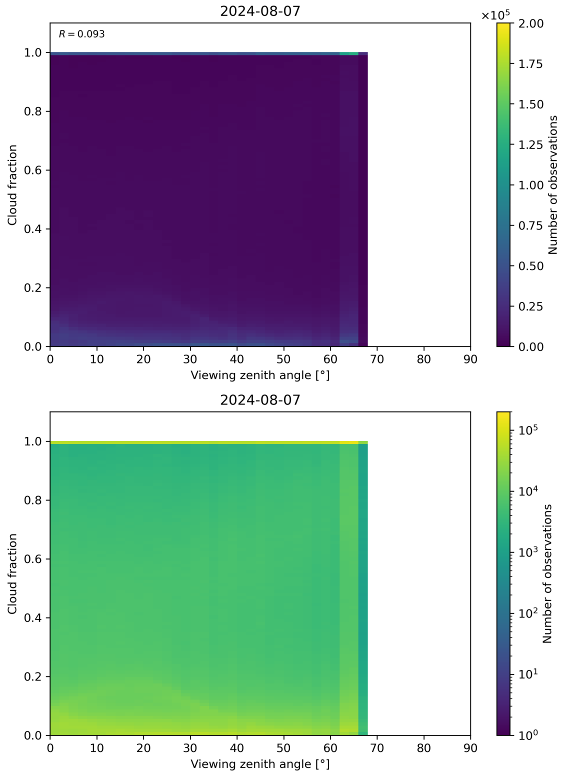
Figure 120: Scatter density plot of “Viewing zenith angle” against “Cloud fraction” for 2024-08-06 to 2024-08-08.
