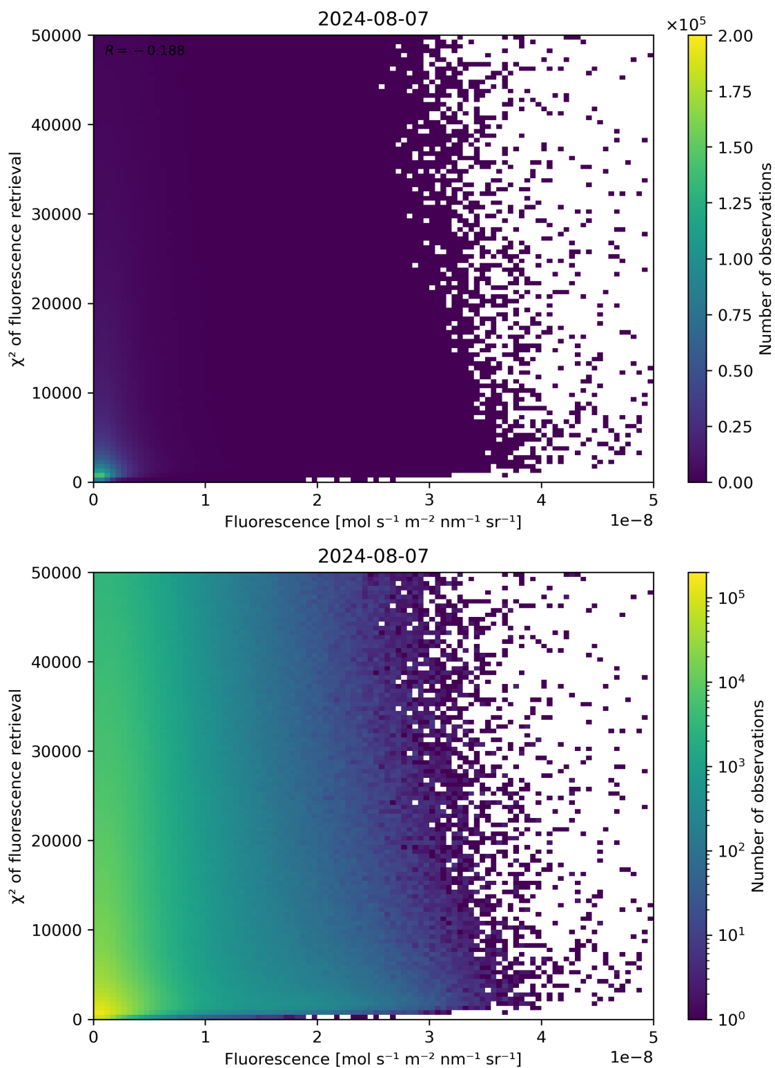
Figure 85: Scatter density plot of “Fluorescence” against “ \chi^2 of fluorescence retrieval” for 2024-08-06 to 2024-08-08.
