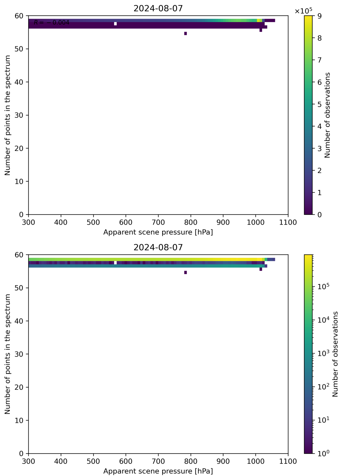
Figure 66: Scatter density plot of “Apparent scene pressure” against “Number of points in the spectrum” for 2024-08-06 to 2024-08-08.
