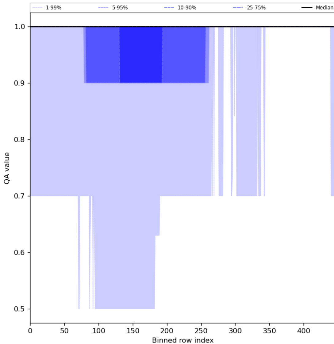
Figure 46: Along track statistics of “QA value” for 2024-08-06 to 2024-08-08
