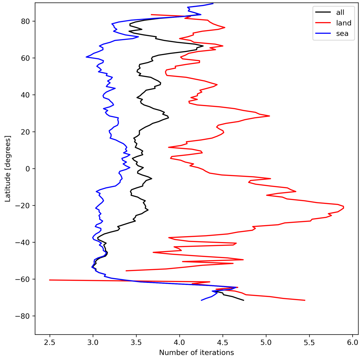
Figure 22: Zonal average of “Number of iterations” for 2024-08-06 to 2024-08-08.
