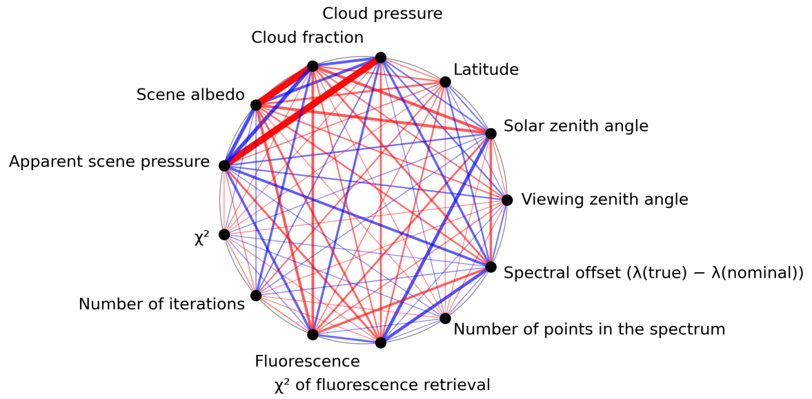
Figure 1: Map of correlation graph for 2024-08-06 to 2024-08-08.
