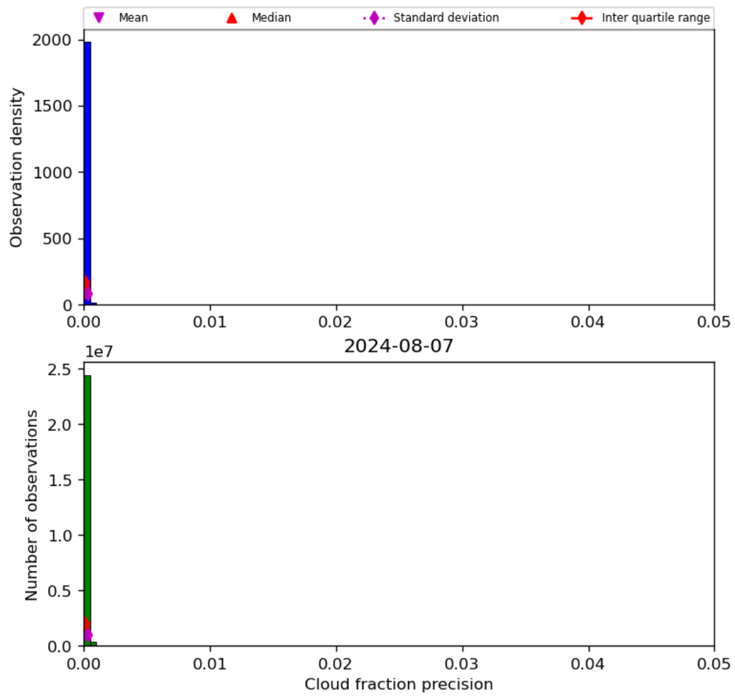
Figure 33: Histogram of “Cloud fraction precision” for 2024-08-06 to 2024-08-08
