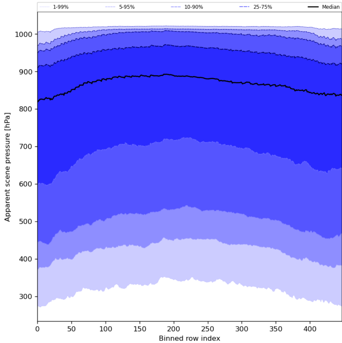
Figure 53: Along track statistics of “Apparent scene pressure” for 2024-08-06 to 2024-08-08
