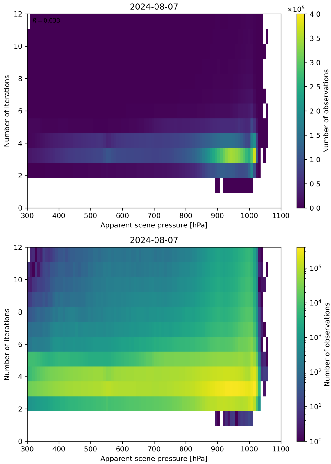
Figure 65: Scatter density plot of “Apparent scene pressure” against “Number of iterations” for 2024-08-06 to 2024-08-08.
