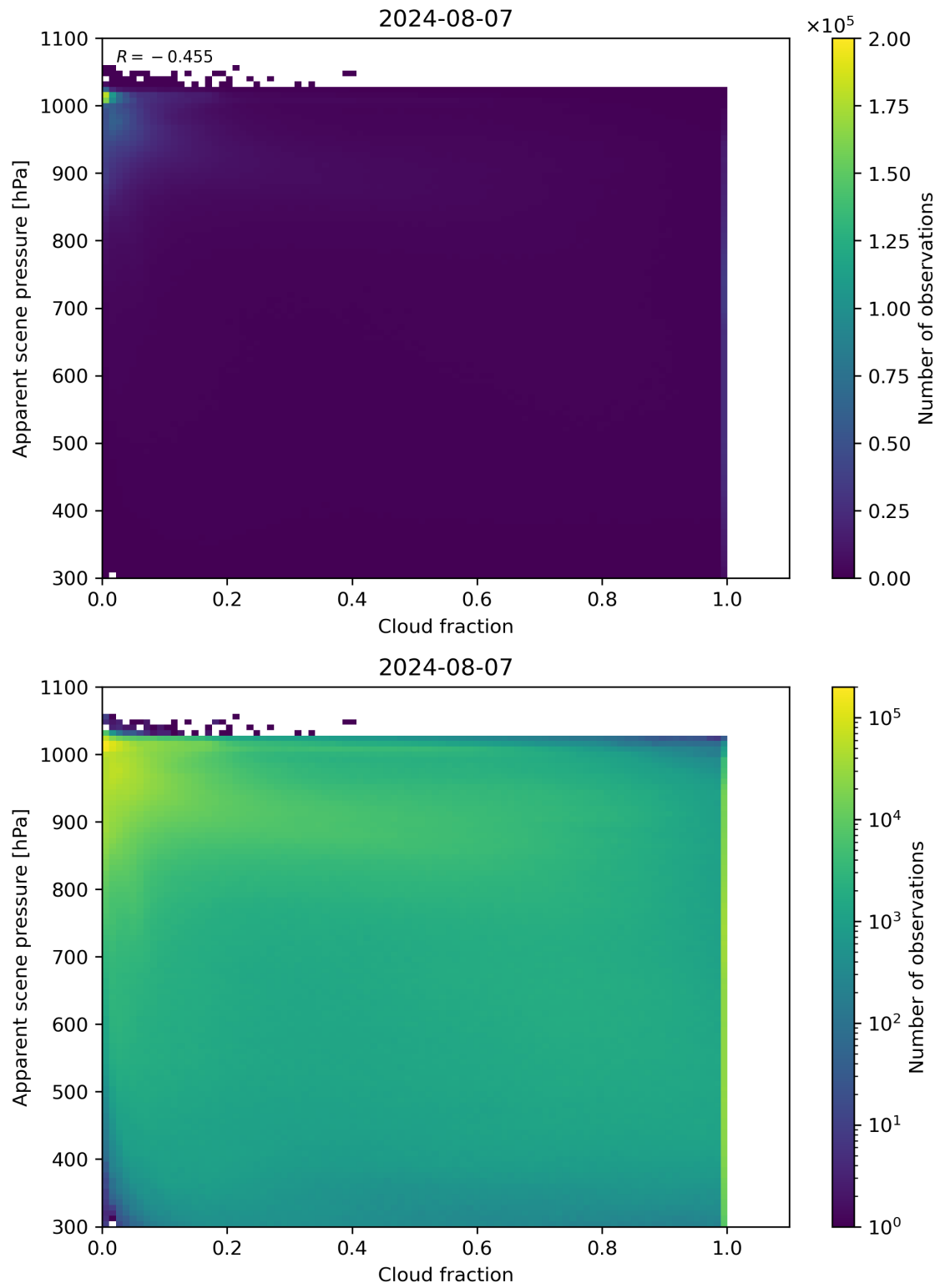
Figure 70: Scatter density plot of “Cloud fraction” against “Apparent scene pressure” for 2024-08-06 to 2024-08-08.
