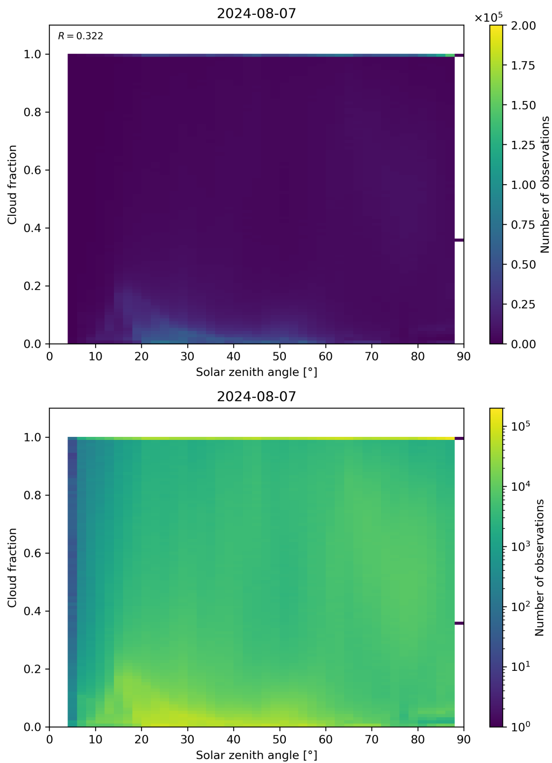
Figure 110: Scatter density plot of “Solar zenith angle” against “Cloud fraction” for 2024-08-06 to 2024-08-08.
