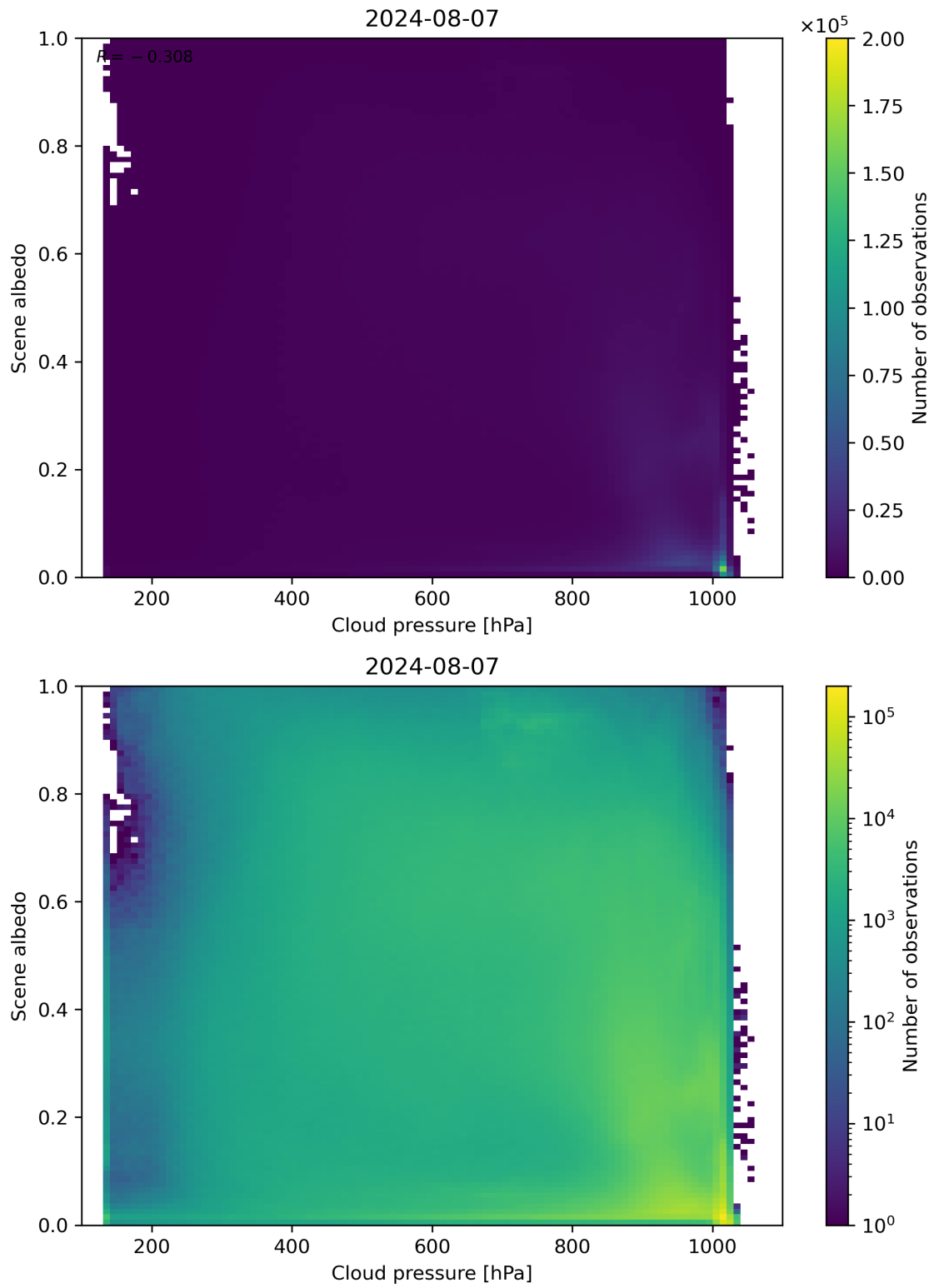
Figure 83: Scatter density plot of “Cloud pressure” against “Scene albedo” for 2024-08-06 to 2024-08-08.
