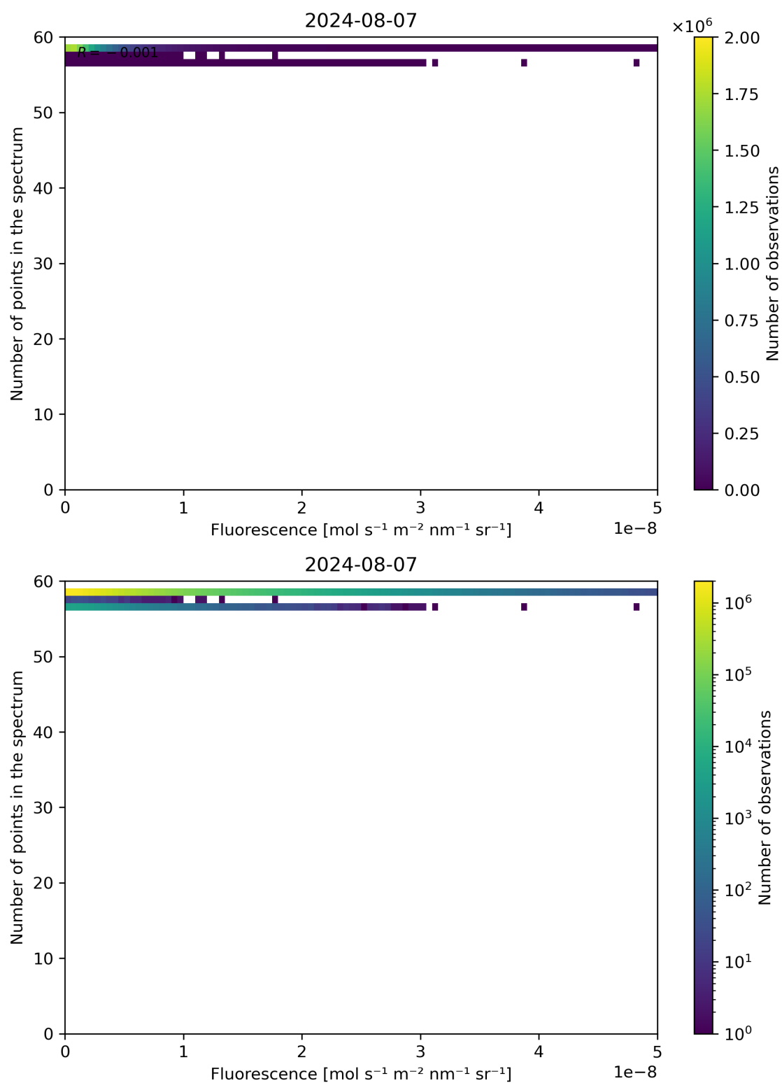
Figure 86: Scatter density plot of “Fluorescence” against “Number of points in the spectrum” for 2024-08-06 to 2024-08-08.
