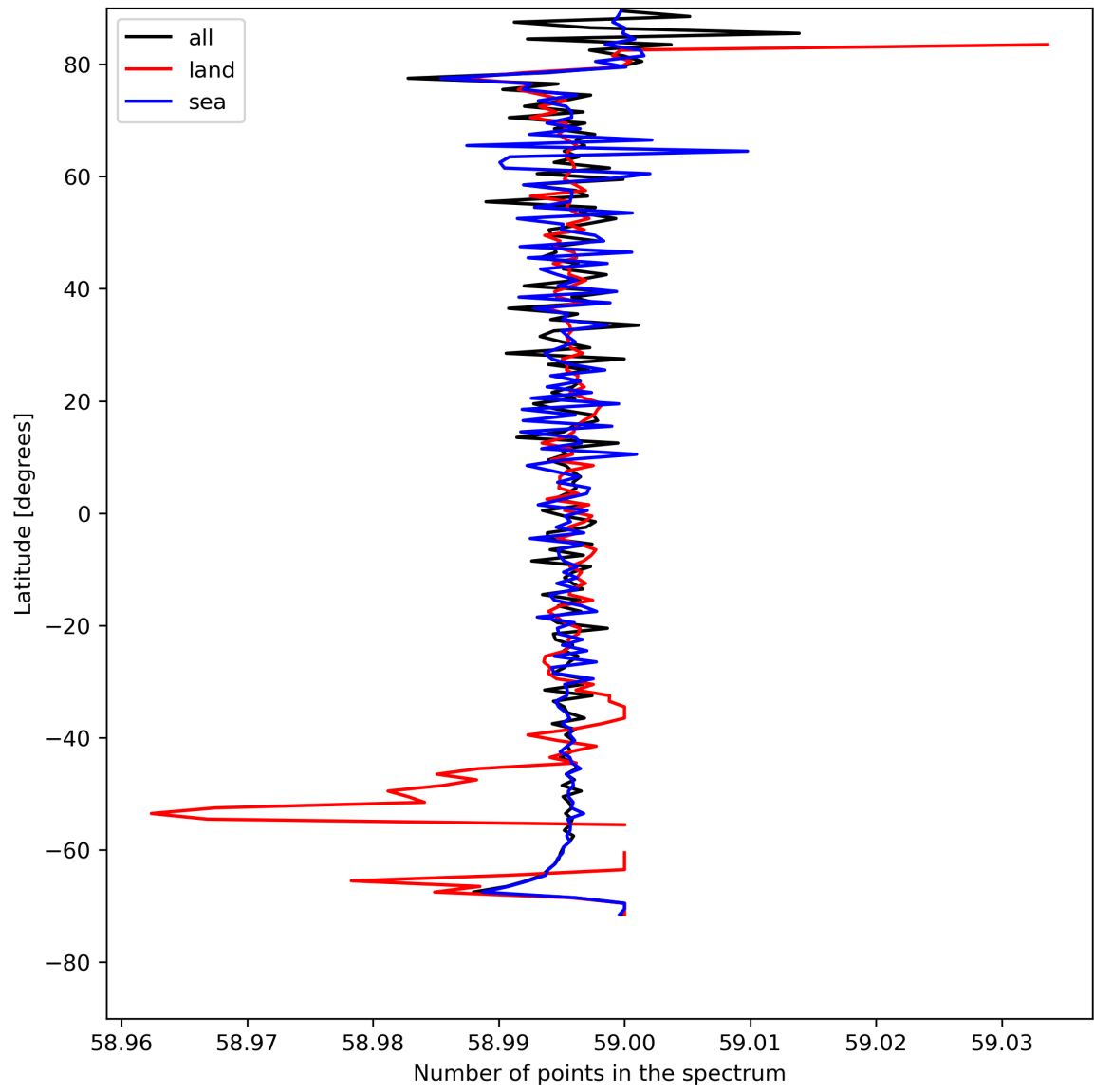
Figure 27: Zonal average of “Number of points in the spectrum” for 2024-08-06 to 2024-08-08.
