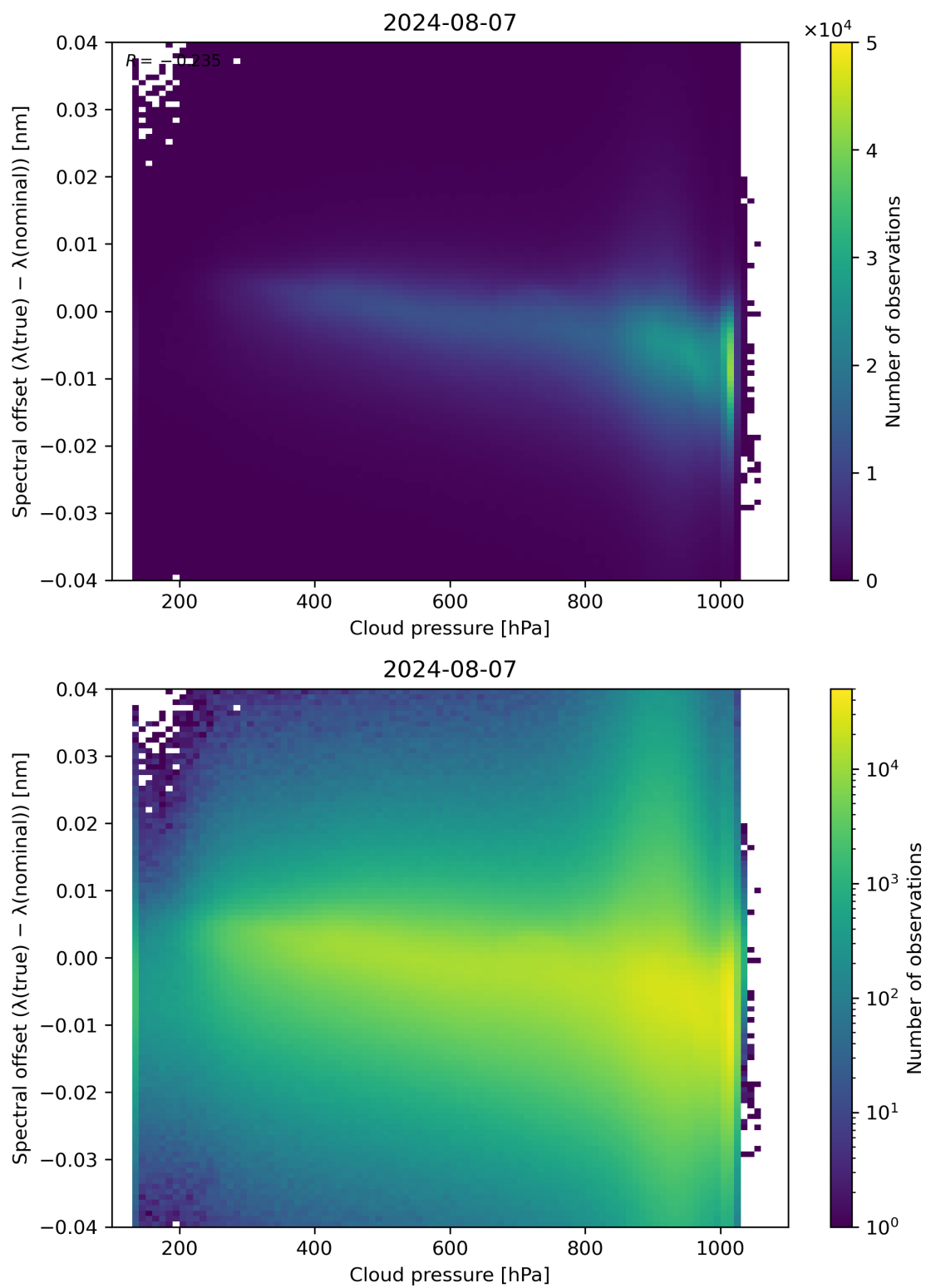
Figure 84: Scatter density plot of “Cloud pressure” against “Spectral offset ( \lambda(\text{true}) - \lambda(\text{nominal}) )” for 2024-08-06 to 2024-08-08.
