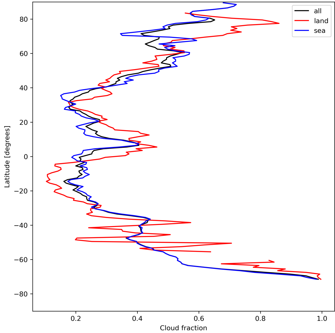
Figure 15: Zonal average of “Cloud fraction” for 2024-08-06 to 2024-08-08.
