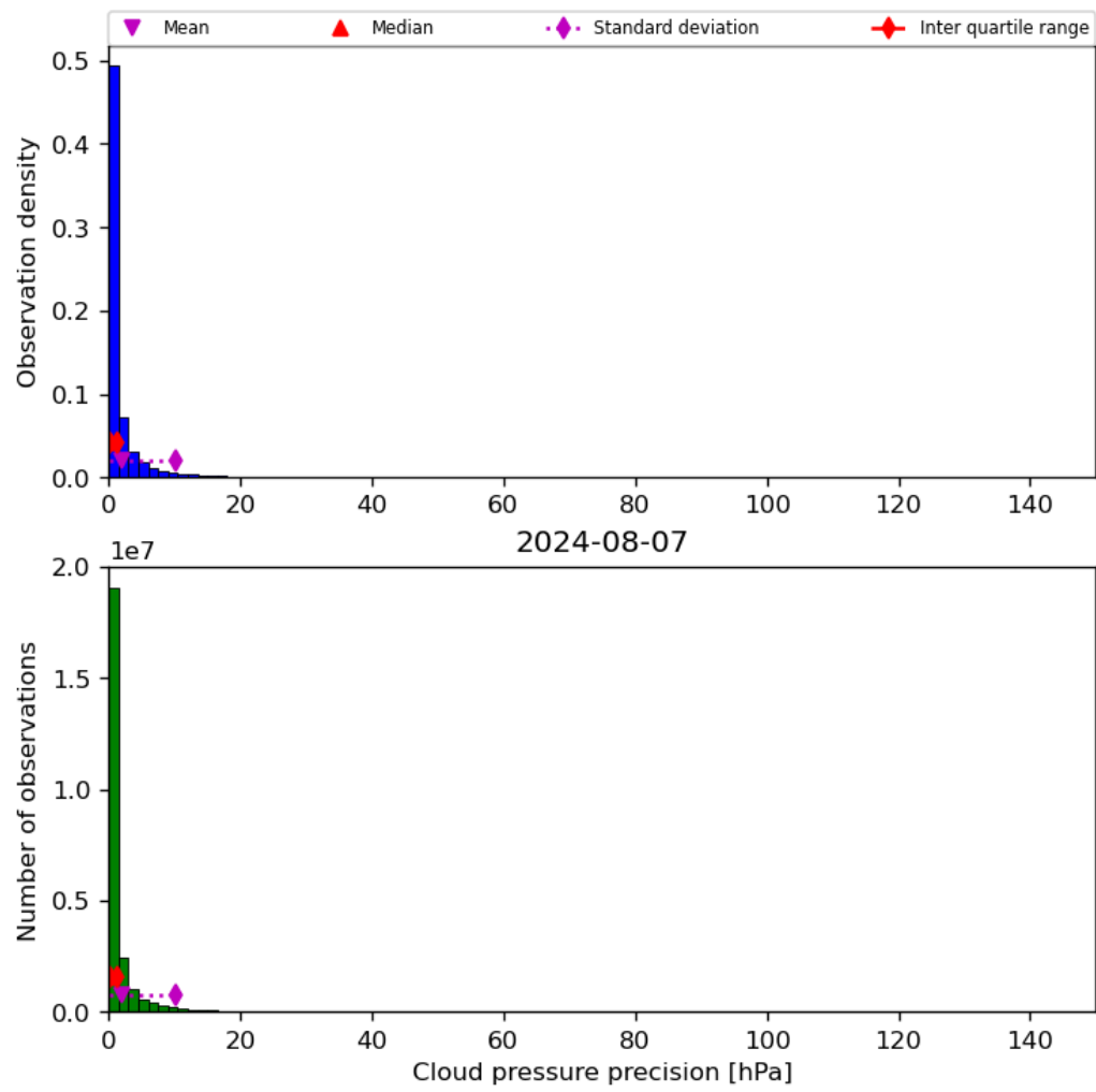
Figure 31: Histogram of “Cloud pressure precision” for 2024-08-06 to 2024-08-08
