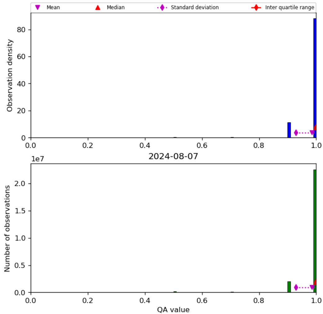
Figure 29: Histogram of “QA value” for 2024-08-06 to 2024-08-08
