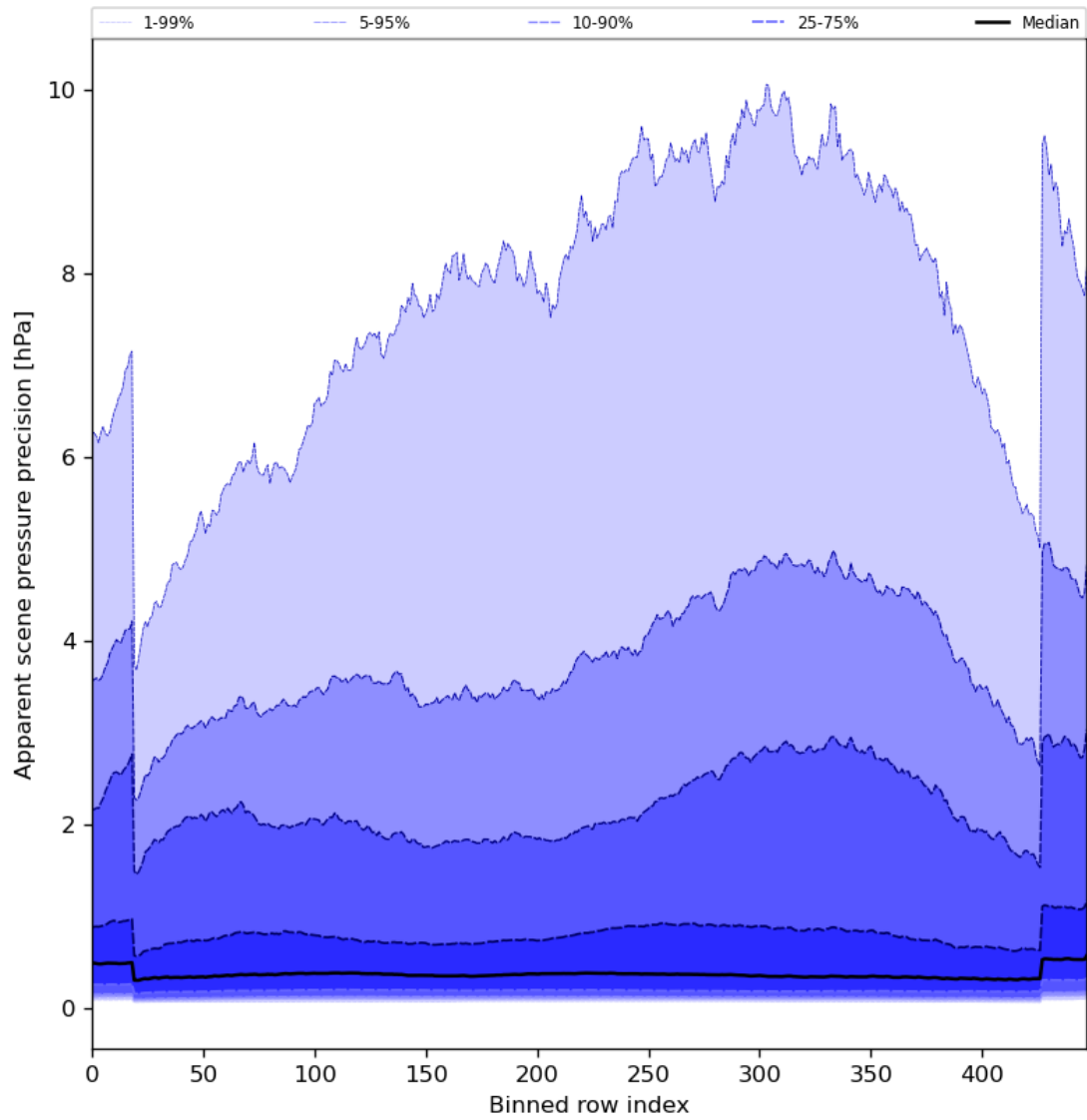
Figure 54: Along track statistics of “Apparent scene pressure precision” for 2024-08-06 to 2024-08-08
