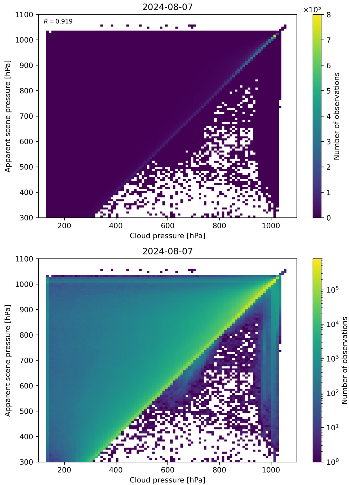
Figure 77: Scatter density plot of “Cloud pressure” against “Apparent scene pressure” for 2024-08-06 to 2024-08-08.
