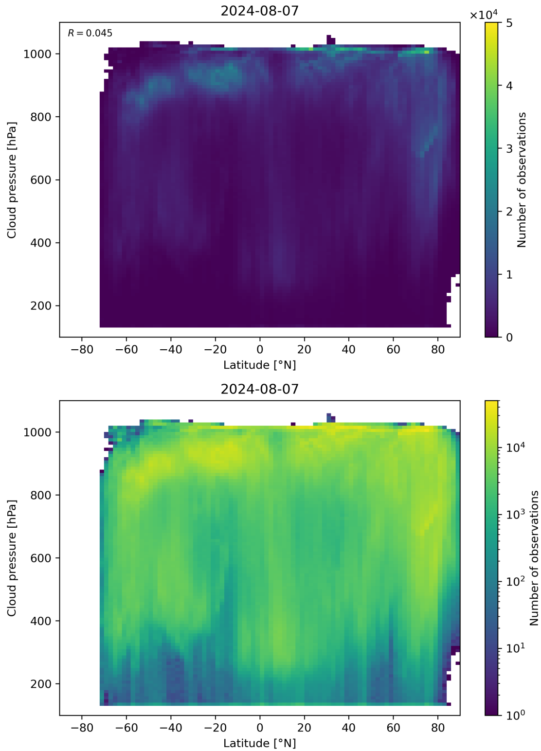
Figure 91: Scatter density plot of “Latitude” against “Cloud pressure” for 2024-08-06 to 2024-08-08.
