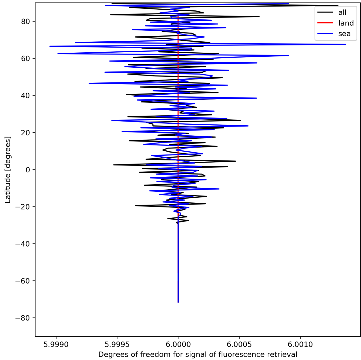
Figure 26: Zonal average of “Degrees of freedom for signal of fluorescence retrieval” for 2024-08-06 to 2024-08-08.
