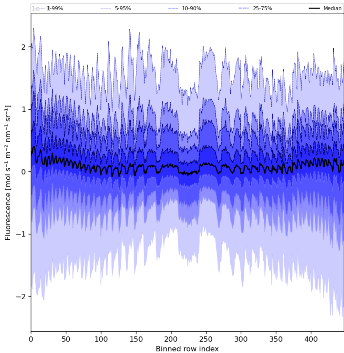
Figure 57: Along track statistics of “Fluorescence” for 2024-08-06 to 2024-08-08
