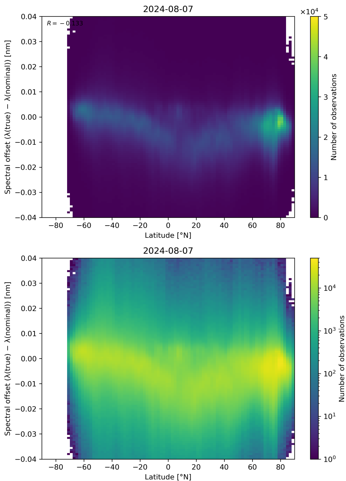
Figure 96: Scatter density plot of “Latitude” against “Spectral offset ( \lambda(\text{true}) - \lambda(\text{nominal}) )” for 2024-08-06 to 2024-08-08.
