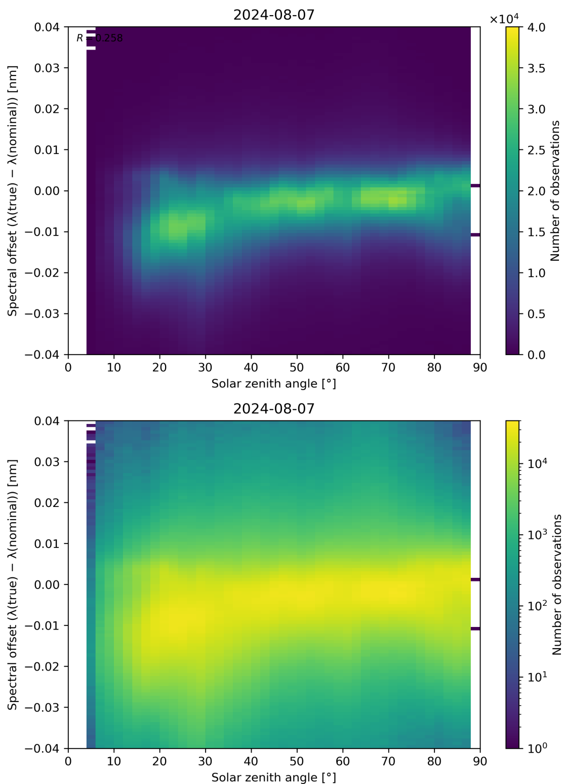
Figure 117: Scatter density plot of “Solar zenith angle” against “Spectral offset ( \lambda(\text{true}) - \lambda(\text{nominal}) )” for 2024-08-06 to 2024-08-08.
