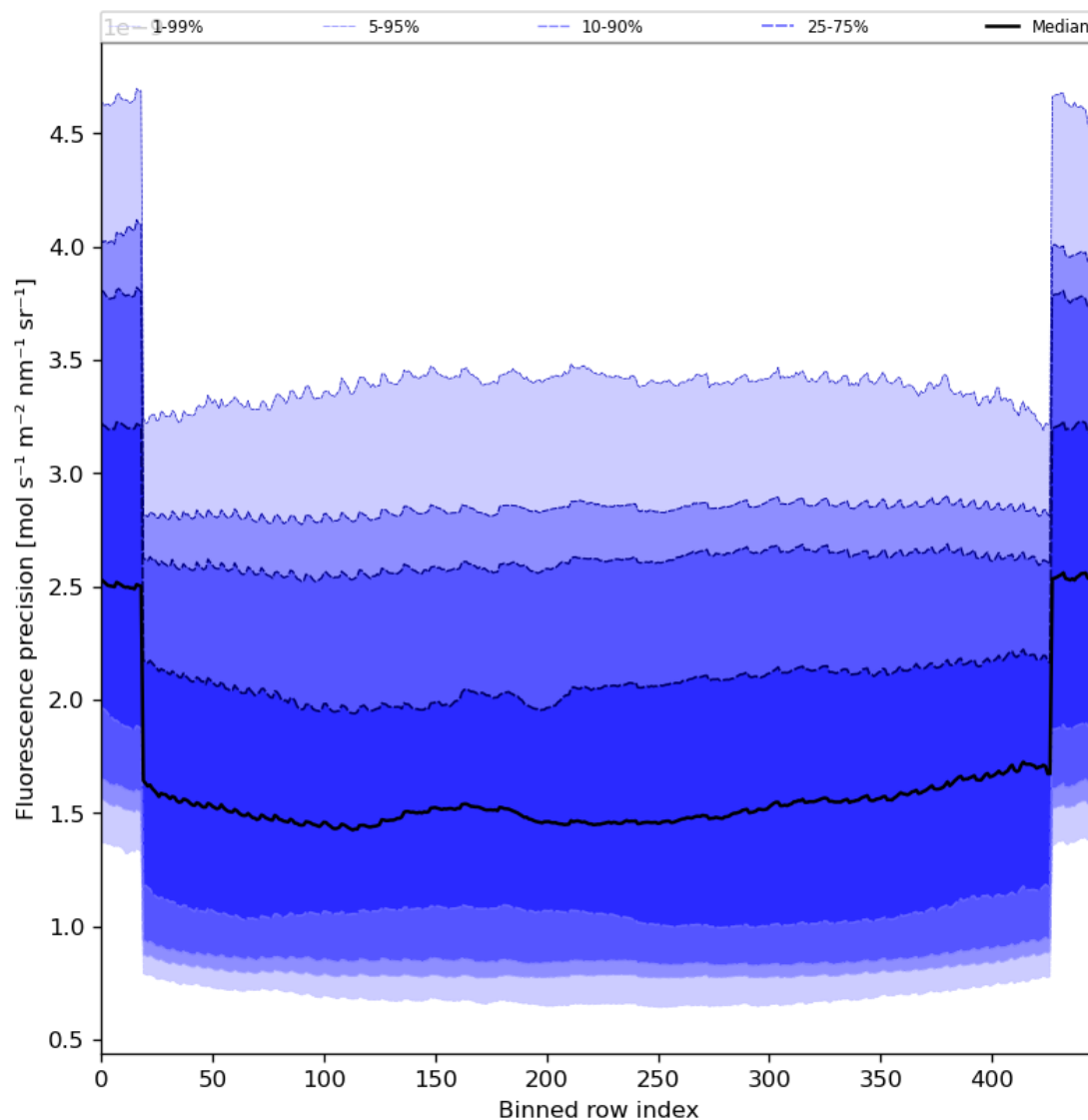
Figure 58: Along track statistics of “Fluorescence precision” for 2024-08-06 to 2024-08-08
