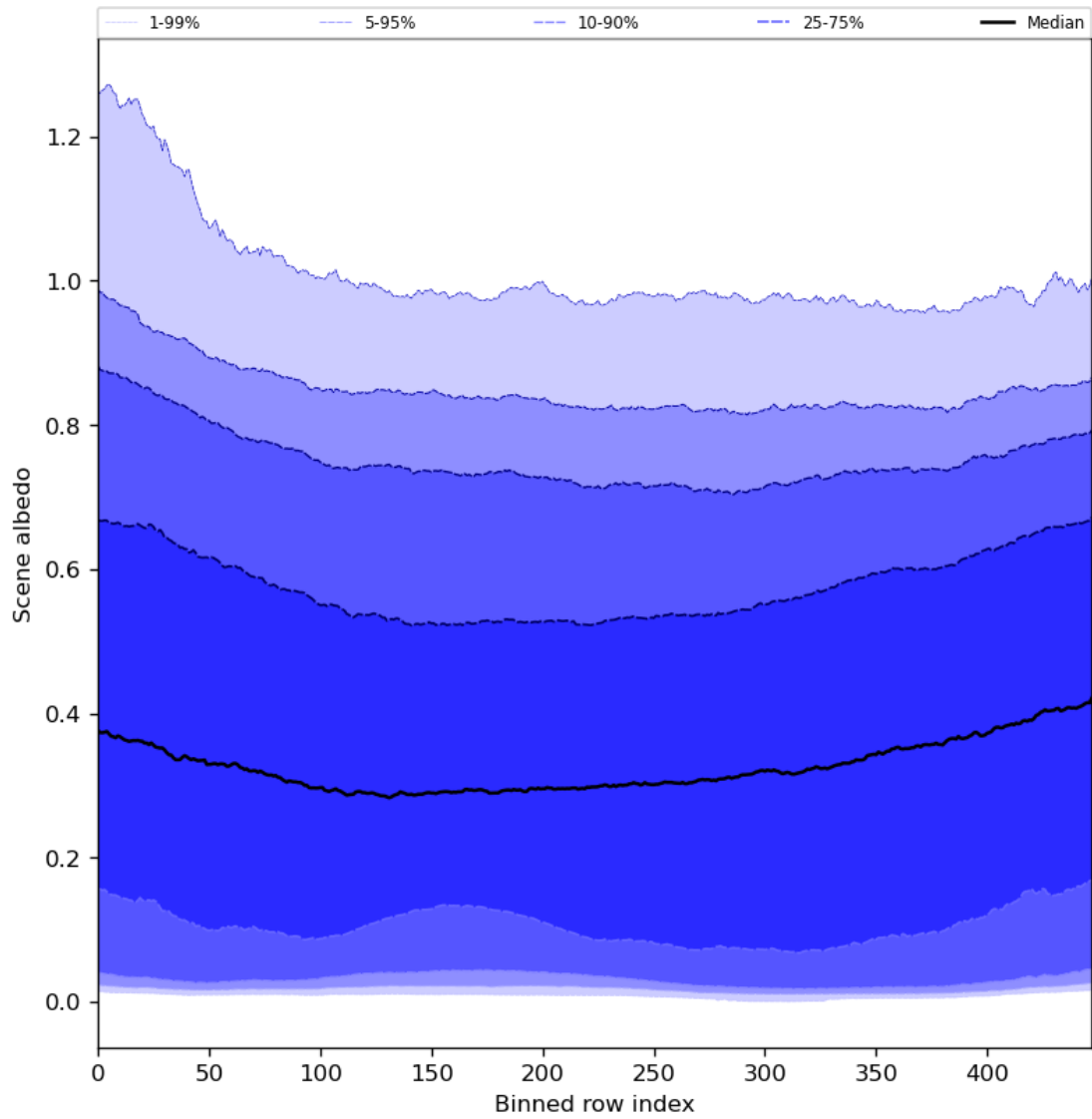
Figure 51: Along track statistics of “Scene albedo” for 2024-08-08 to 2024-08-10
