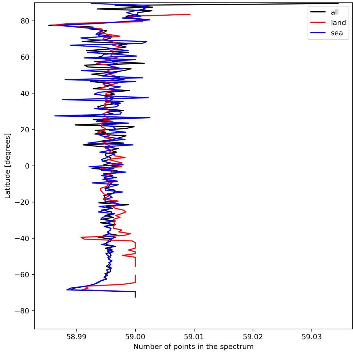
Figure 27: Zonal average of “Number of points in the spectrum” for 2024-08-08 to 2024-08-10.
