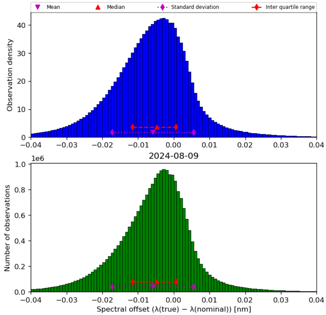
Figure 45: Histogram of “Spectral offset ( \lambda(\text{true}) - \lambda(\text{nominal}) )” for 2024-08-08 to 2024-08-10
