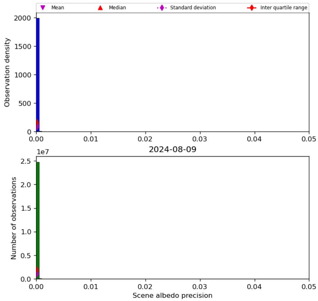
Figure 35: Histogram of “Scene albedo precision” for 2024-08-08 to 2024-08-10
