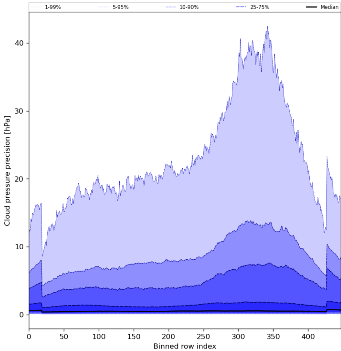
Figure 48: Along track statistics of “Cloud pressure precision” for 2024-08-08 to 2024-08-10
