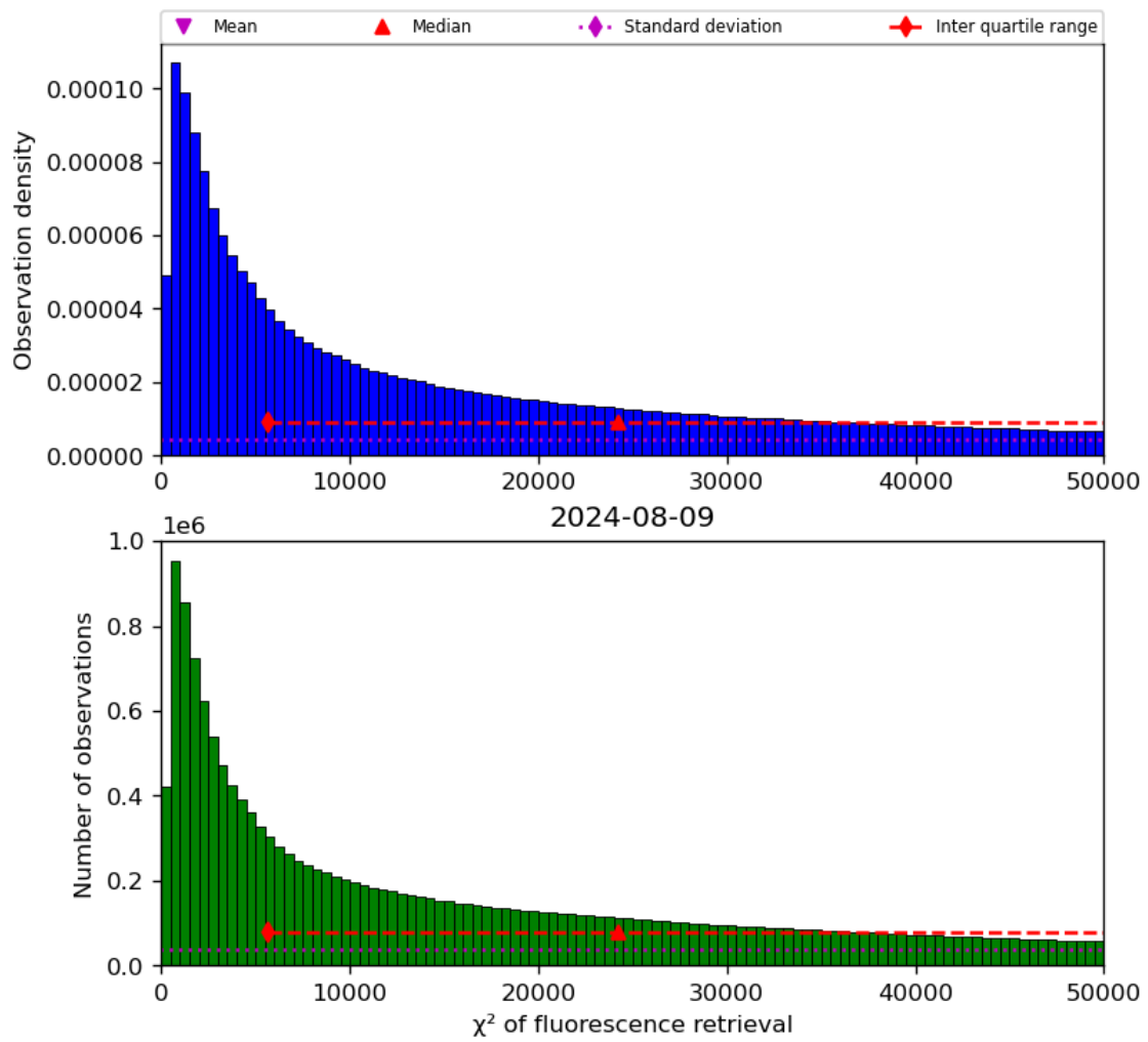
Figure 42: Histogram of “ \chi^2 of fluorescence retrieval” for 2024-08-08 to 2024-08-10
