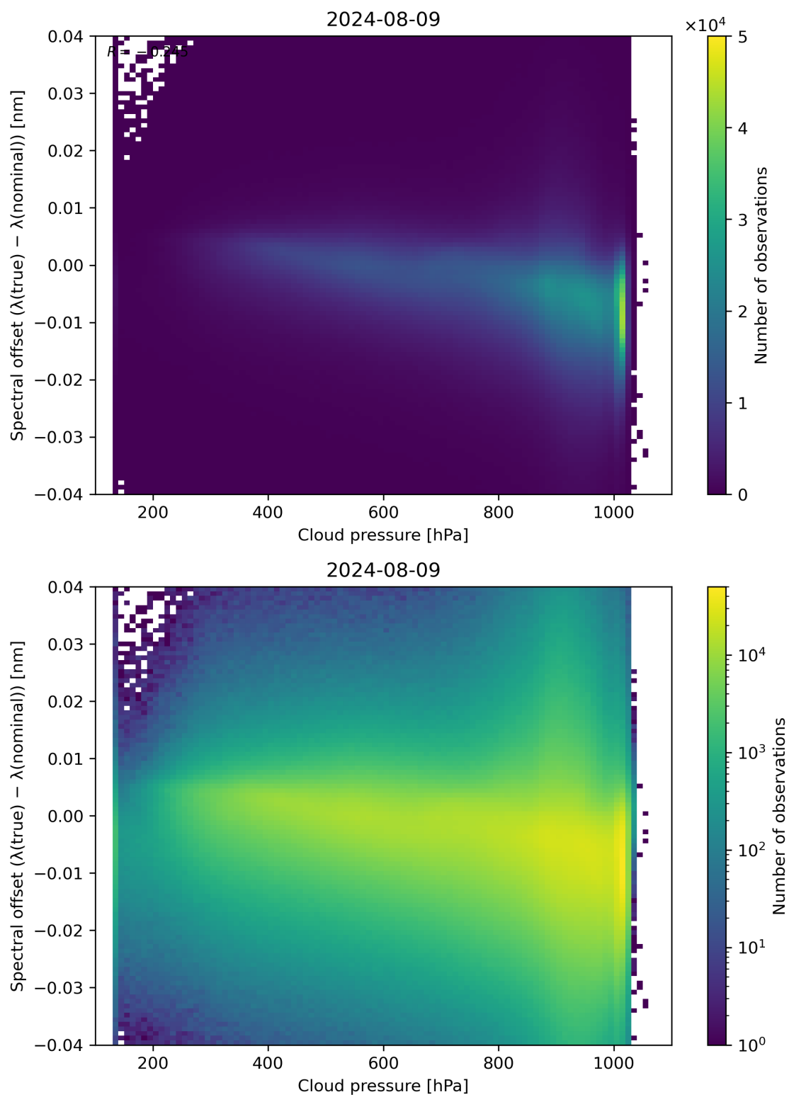
Figure 84: Scatter density plot of “Cloud pressure” against “Spectral offset ( \lambda(\text{true}) - \lambda(\text{nominal}) )” for 2024-08-08 to 2024-08-10.
