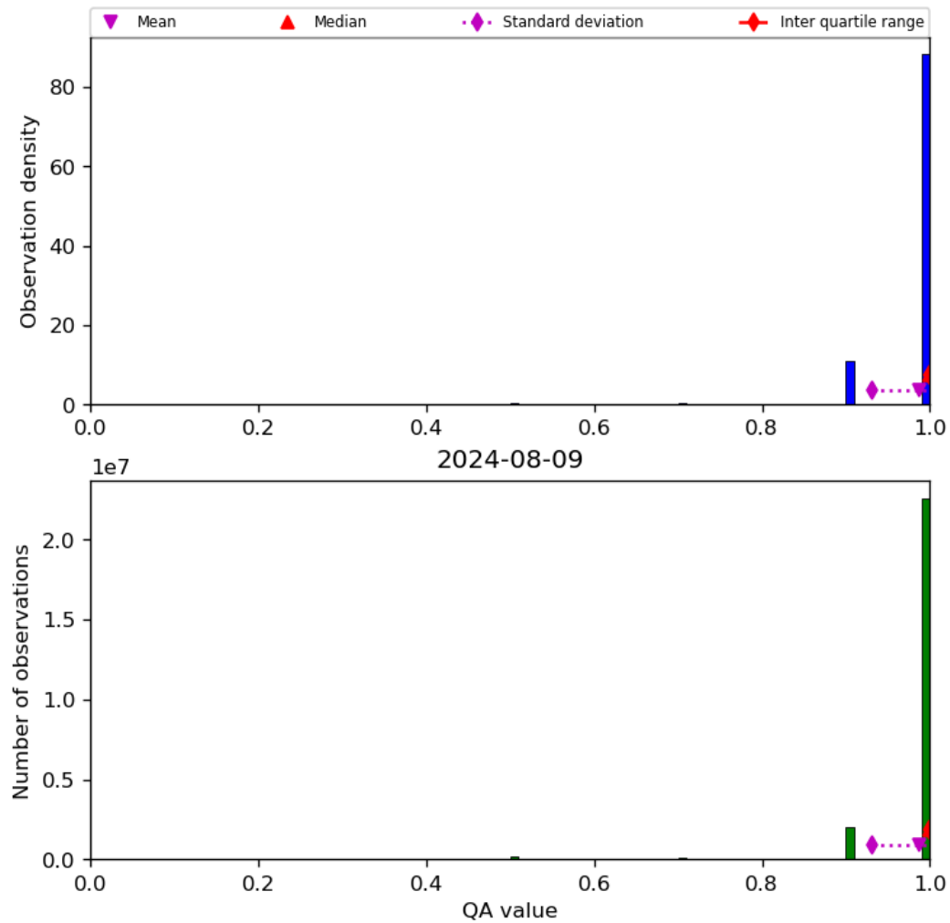
Figure 29: Histogram of “QA value” for 2024-08-08 to 2024-08-10
