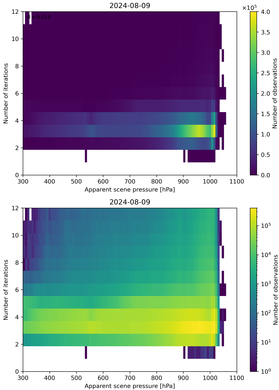
Figure 65: Scatter density plot of “Apparent scene pressure” against “Number of iterations” for 2024-08-08 to 2024-08-10.
