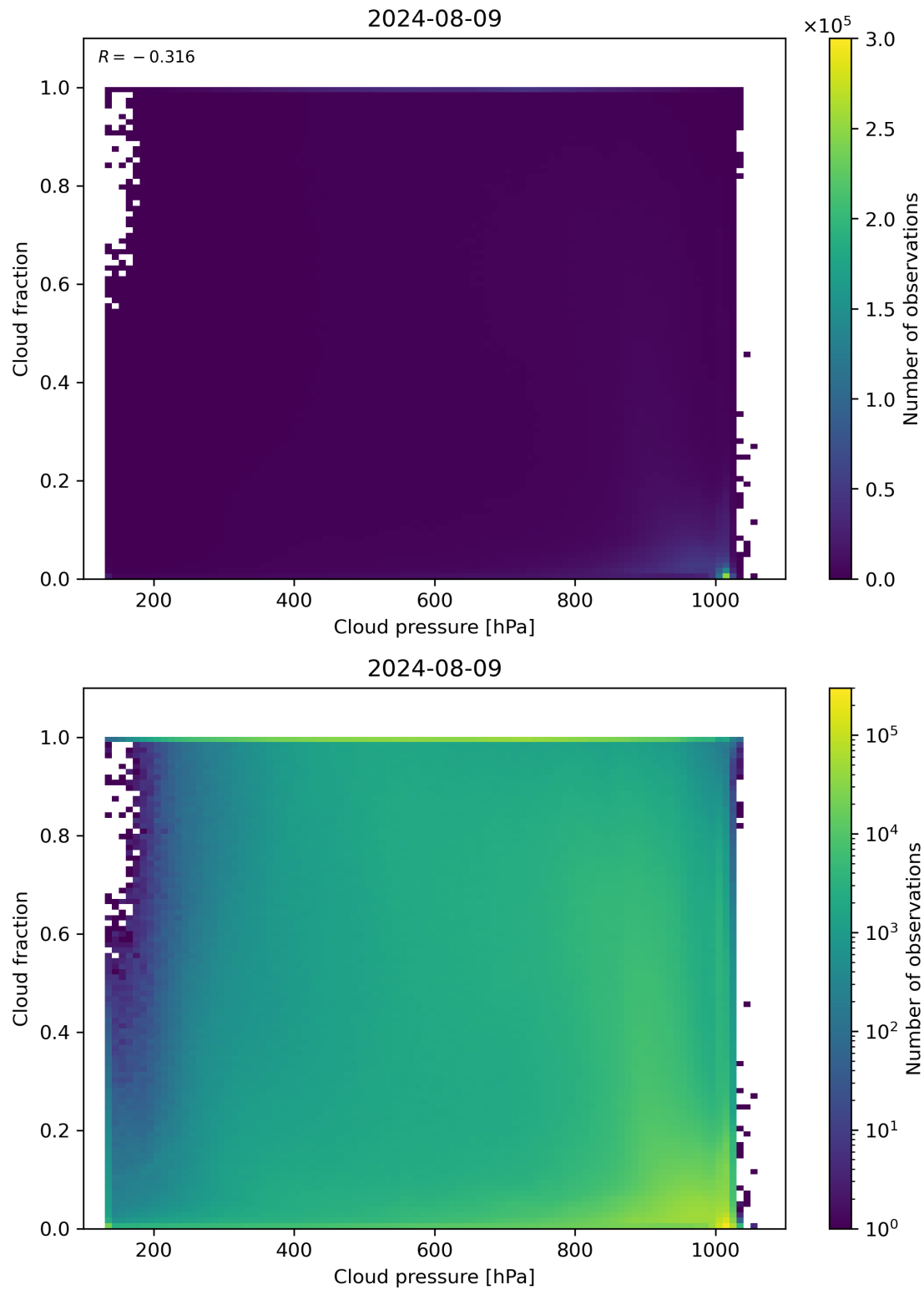
Figure 79: Scatter density plot of “Cloud pressure” against “Cloud fraction” for 2024-08-08 to 2024-08-10.
