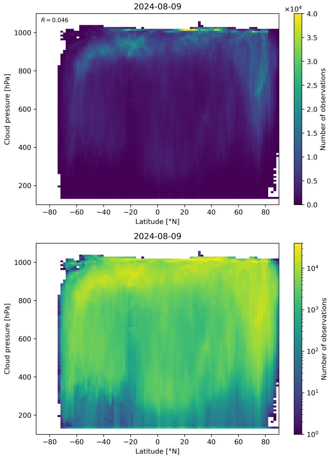
Figure 91: Scatter density plot of “Latitude” against “Cloud pressure” for 2024-08-08 to 2024-08-10.
