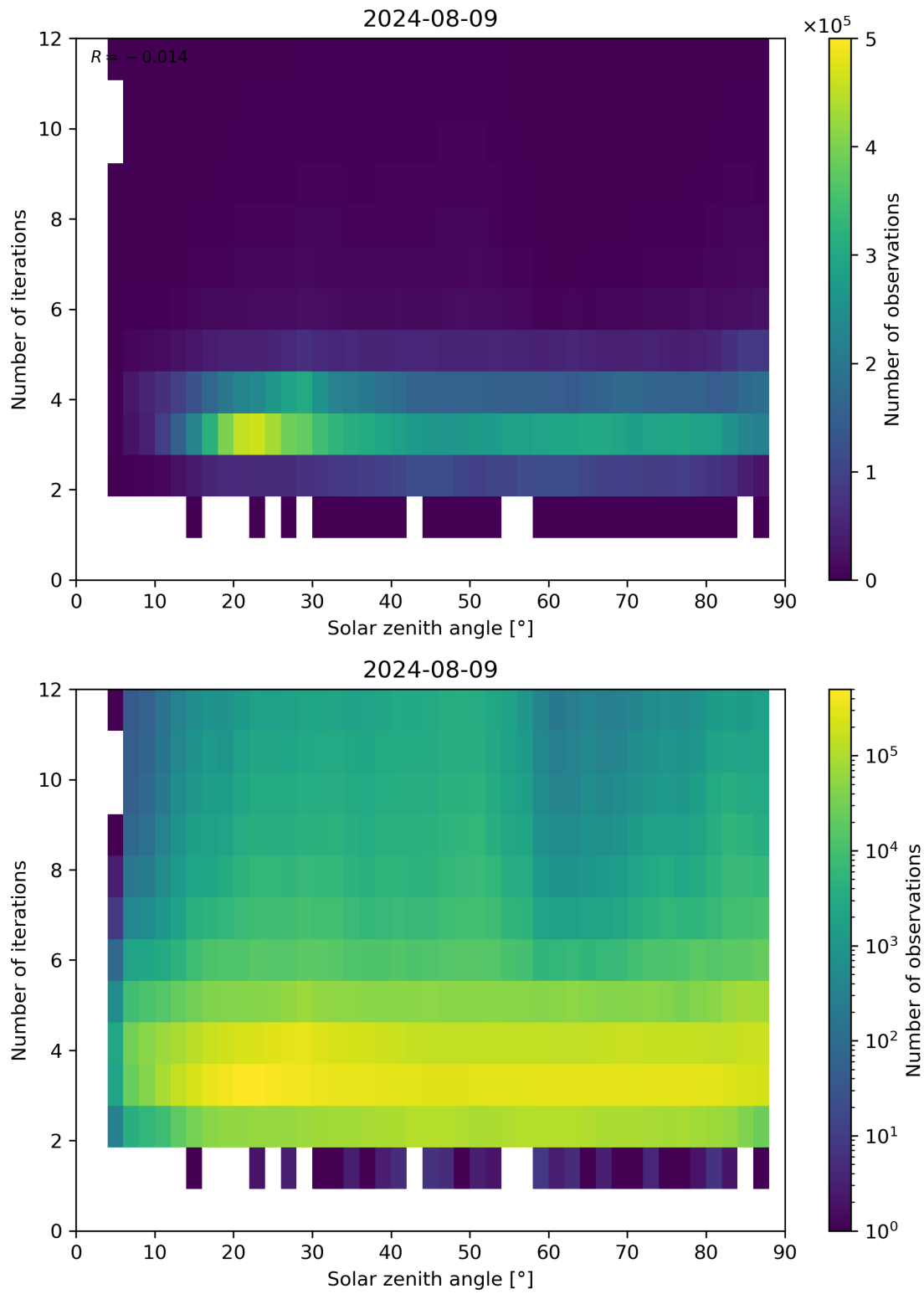
Figure 114: Scatter density plot of “Solar zenith angle” against “Number of iterations” for 2024-08-08 to 2024-08-10.
