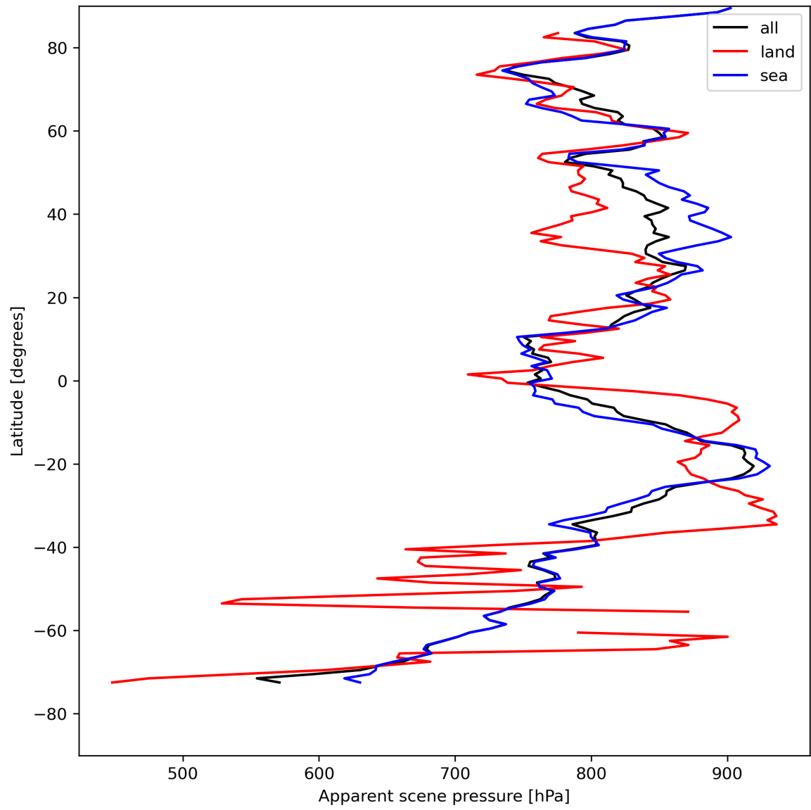
Figure 19: Zonal average of “Apparent scene pressure” for 2024-08-08 to 2024-08-10.
