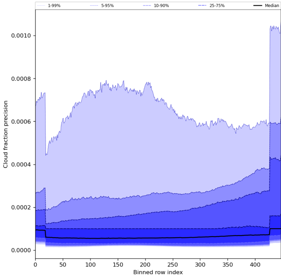
Figure 50: Along track statistics of “Cloud fraction precision” for 2024-08-08 to 2024-08-10
