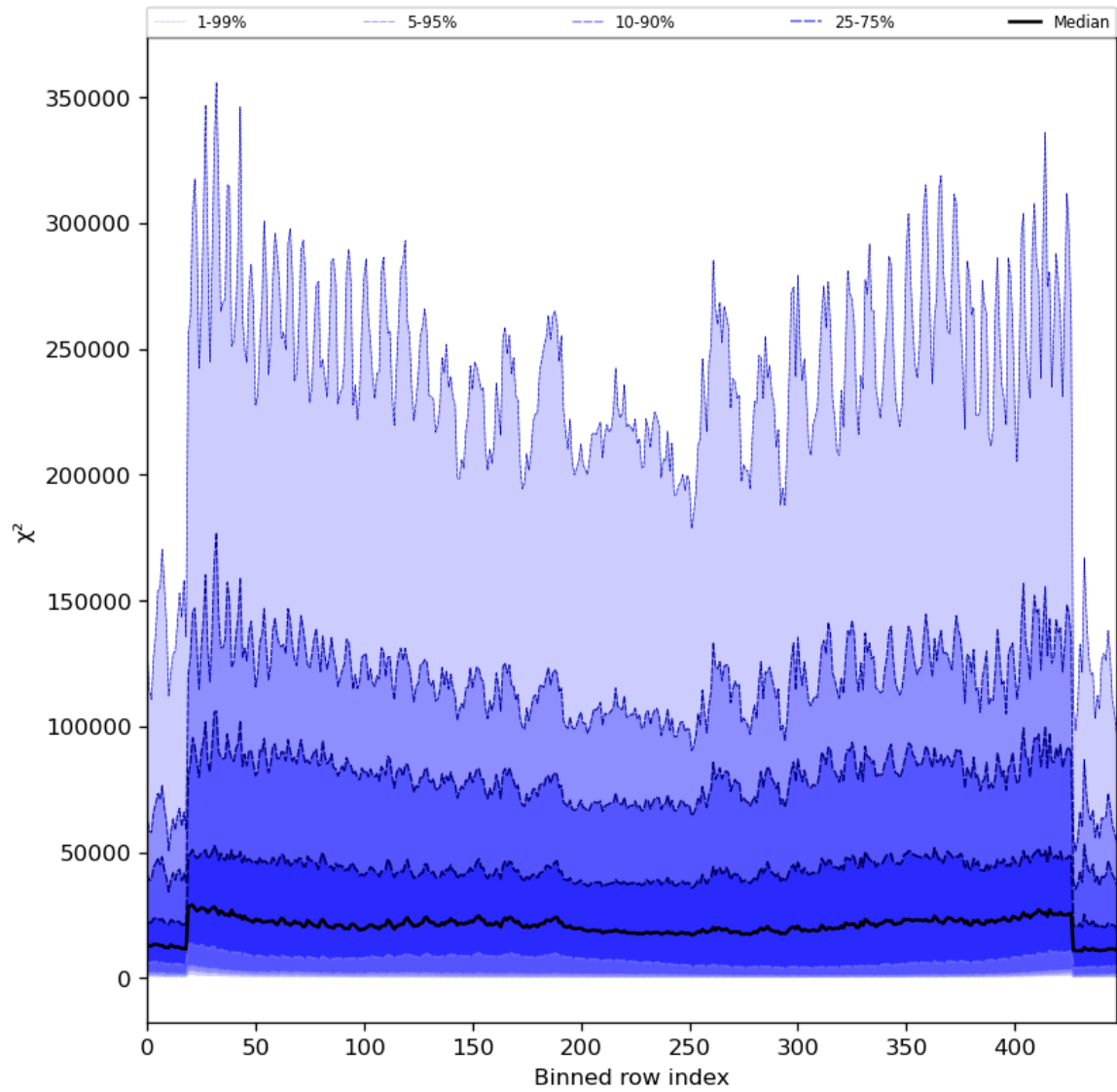
Figure 55: Along track statistics of “ \chi^2 ” for 2024-08-08 to 2024-08-10
