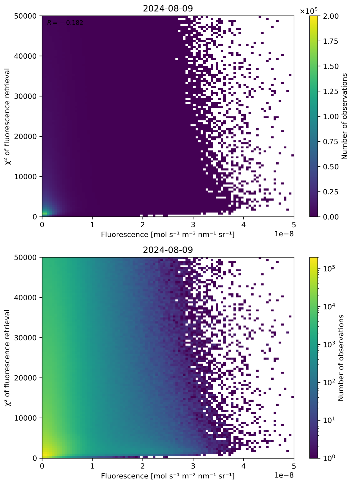
Figure 85: Scatter density plot of “Fluorescence” against “ \chi^2 of fluorescence retrieval” for 2024-08-08 to 2024-08-10.
