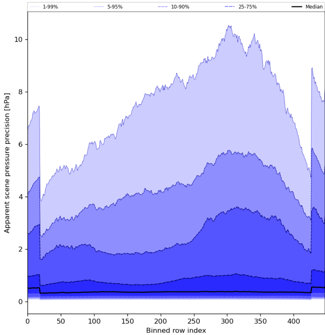
Figure 54: Along track statistics of “Apparent scene pressure precision” for 2024-08-08 to 2024-08-10
