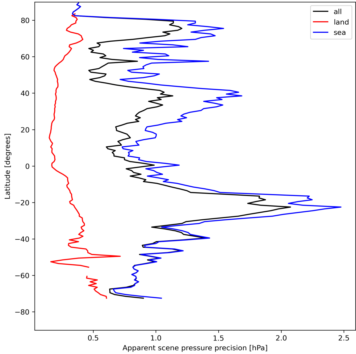
Figure 20: Zonal average of “Apparent scene pressure precision” for 2024-08-08 to 2024-08-10.
