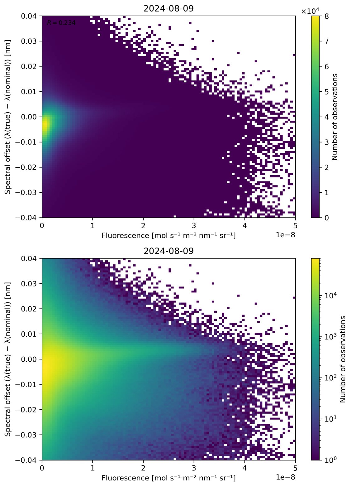
Figure 87: Scatter density plot of “Fluorescence” against “Spectral offset ( \lambda(\text{true}) - \lambda(\text{nominal}) )” for 2024-08-08 to 2024-08-10.
