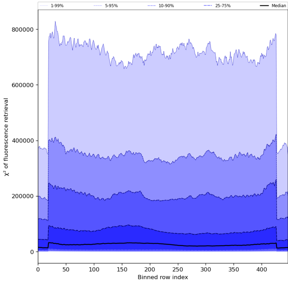
Figure 59: Along track statistics of “ \chi^2 of fluorescence retrieval” for 2024-08-08 to 2024-08-10
