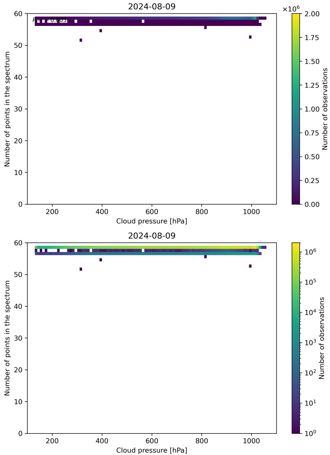
Figure 82: Scatter density plot of “Cloud pressure” against “Number of points in the spectrum” for 2024-08-08 to 2024-08-10.
