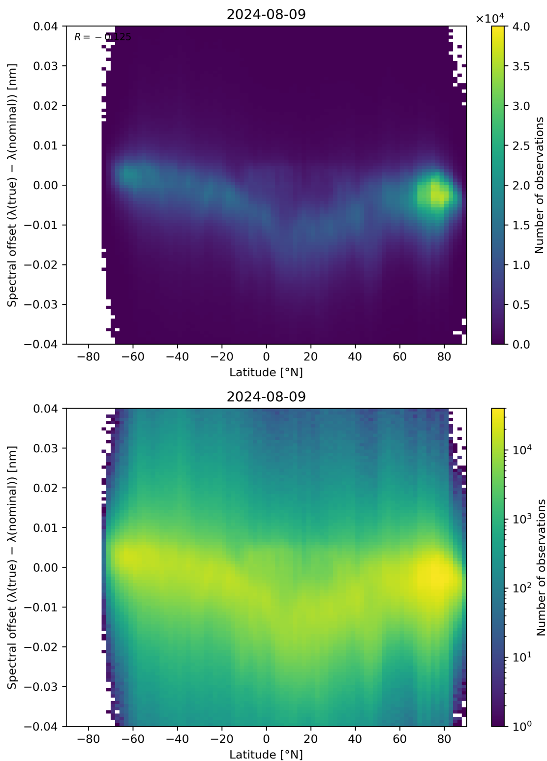
Figure 96: Scatter density plot of “Latitude” against “Spectral offset ( \lambda(\text{true}) - \lambda(\text{nominal}) )” for 2024-08-08 to 2024-08-10.
