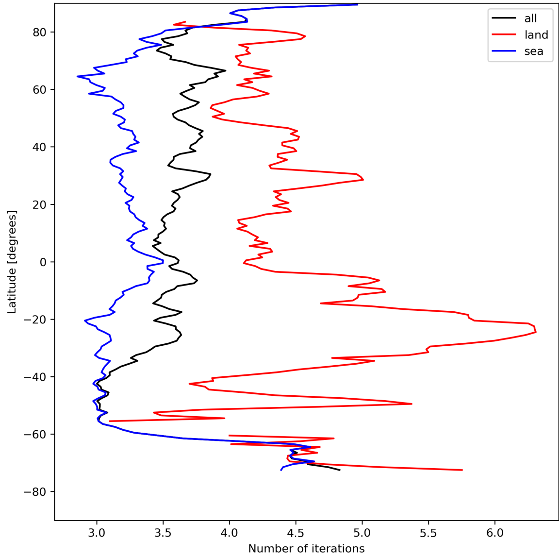
Figure 22: Zonal average of “Number of iterations” for 2024-08-08 to 2024-08-10.
