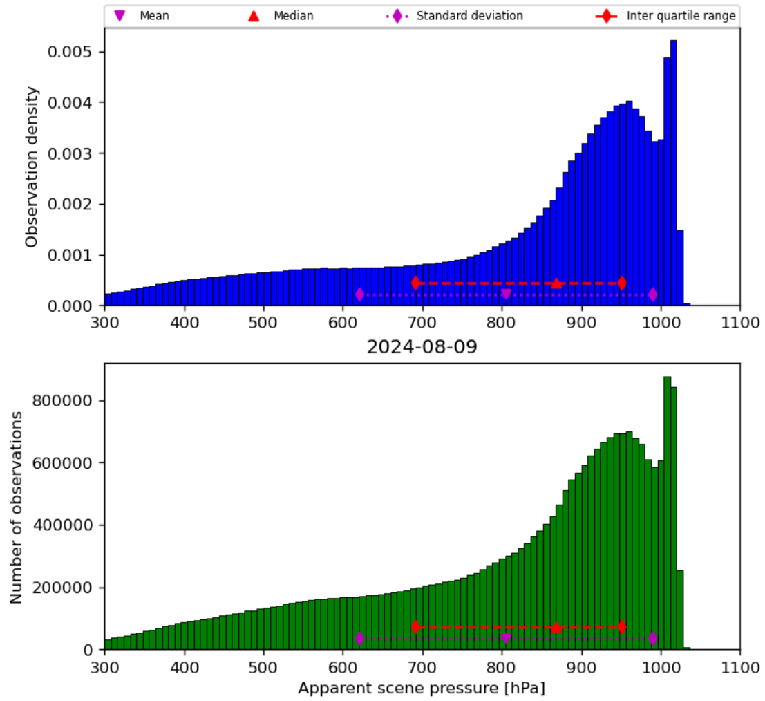
Figure 36: Histogram of “Apparent scene pressure” for 2024-08-08 to 2024-08-10
