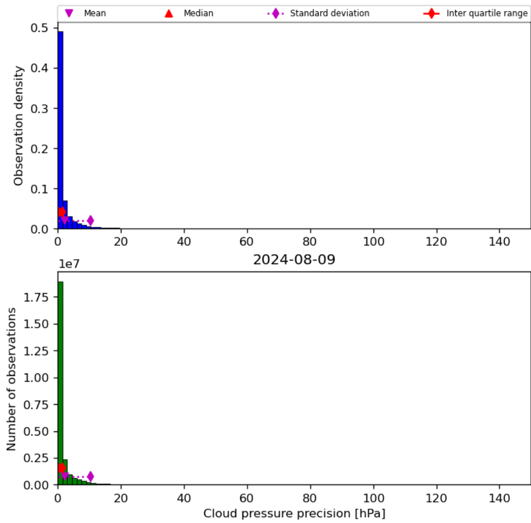
Figure 31: Histogram of “Cloud pressure precision” for 2024-08-08 to 2024-08-10
