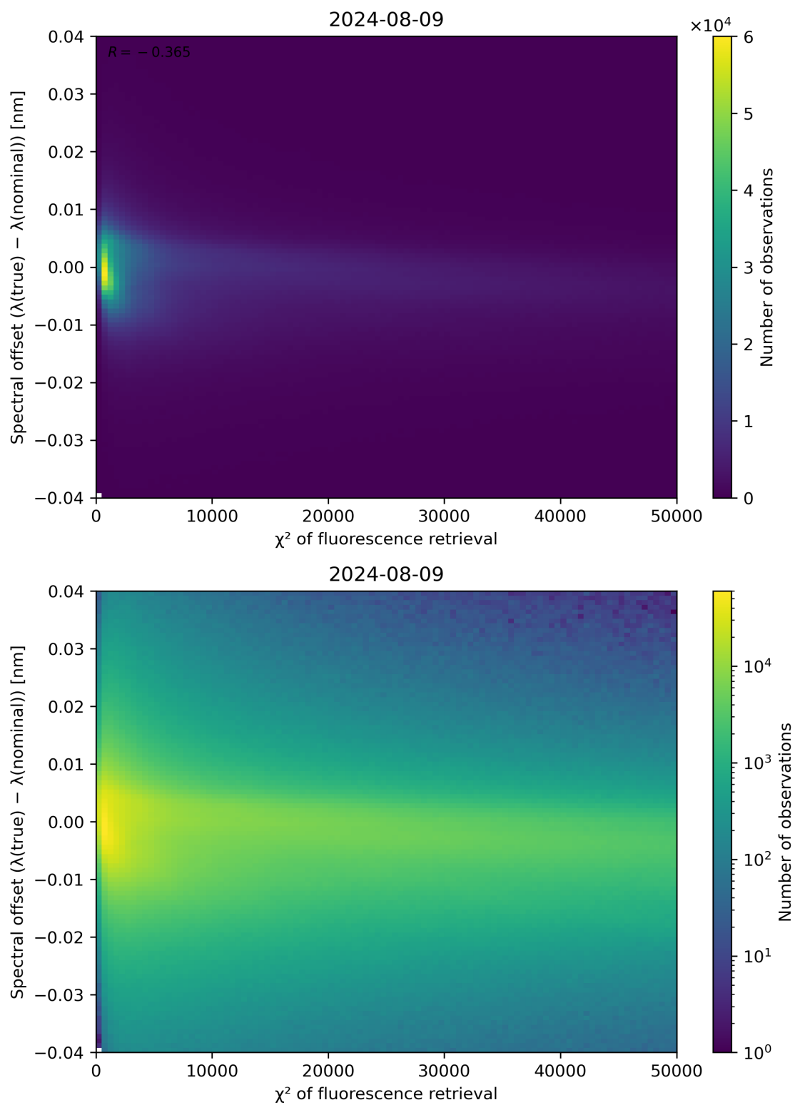
Figure 69: Scatter density plot of " \chi^2 of fluorescence retrieval" against "Spectral offset ( \lambda(\text{true}) - \lambda(\text{nominal}) )" for 2024-08-08 to 2024-08-10.
