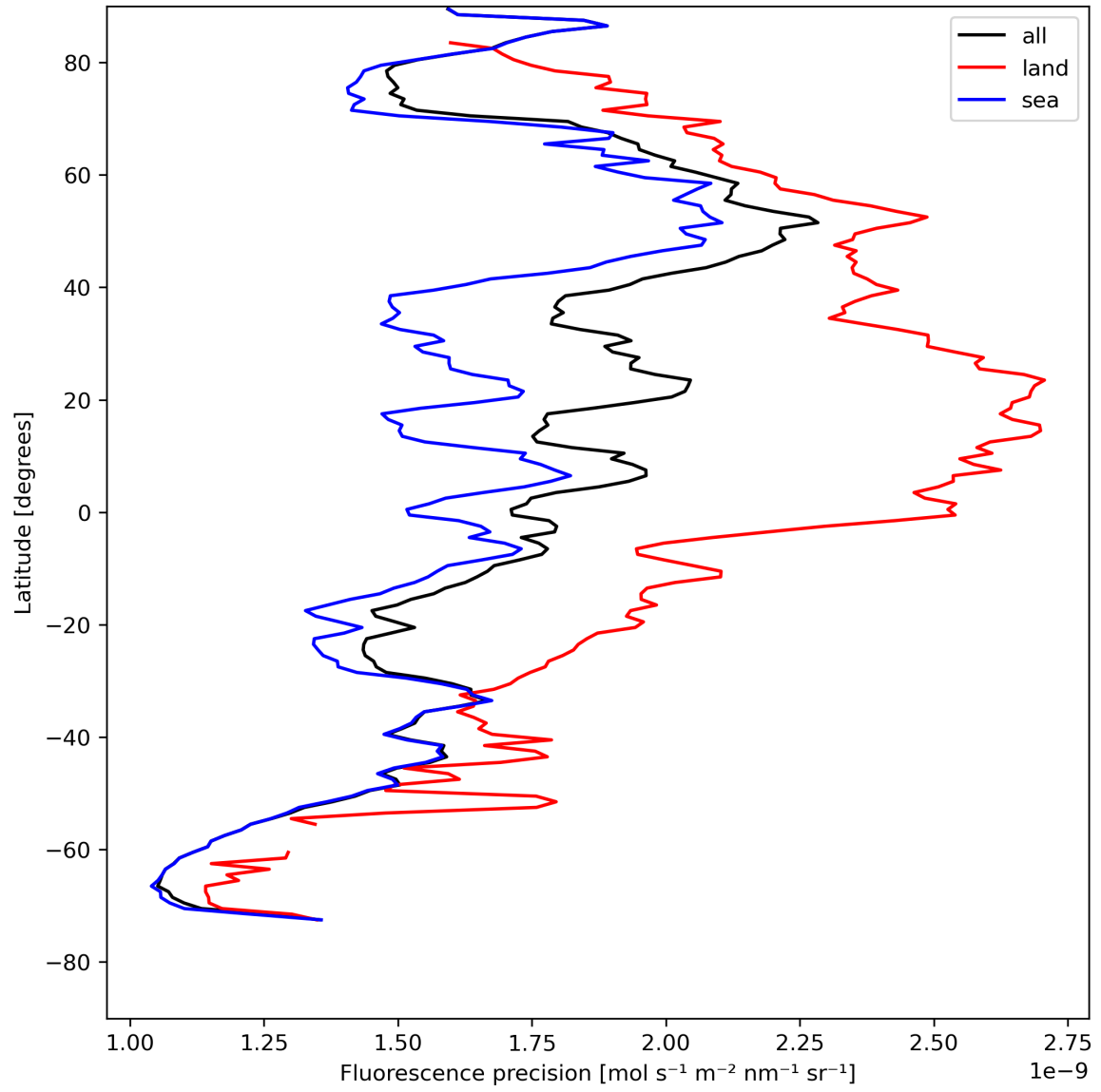
Figure 24: Zonal average of “Fluorescence precision” for 2024-08-08 to 2024-08-10.
