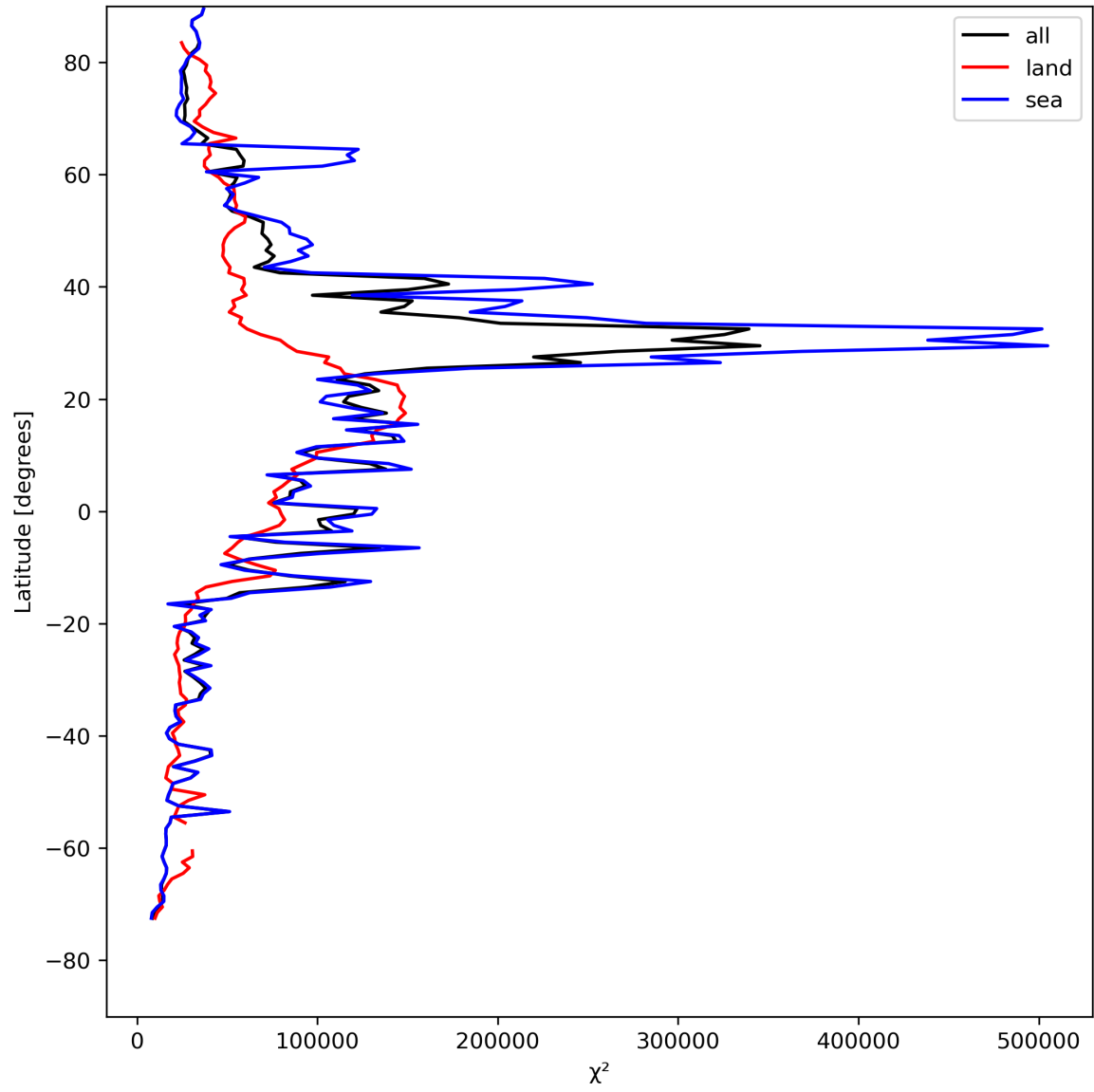
Figure 21: Zonal average of “ \chi^2 ” for 2024-08-08 to 2024-08-10.
