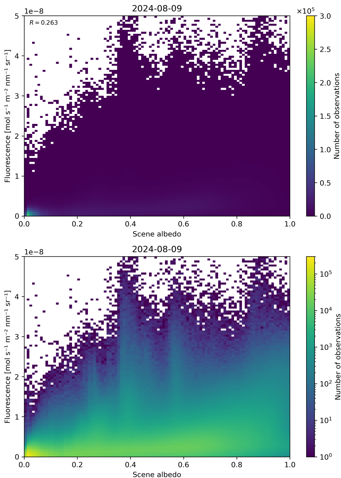
Figure 104: Scatter density plot of “Scene albedo” against “Fluorescence” for 2024-08-08 to 2024-08-10.
