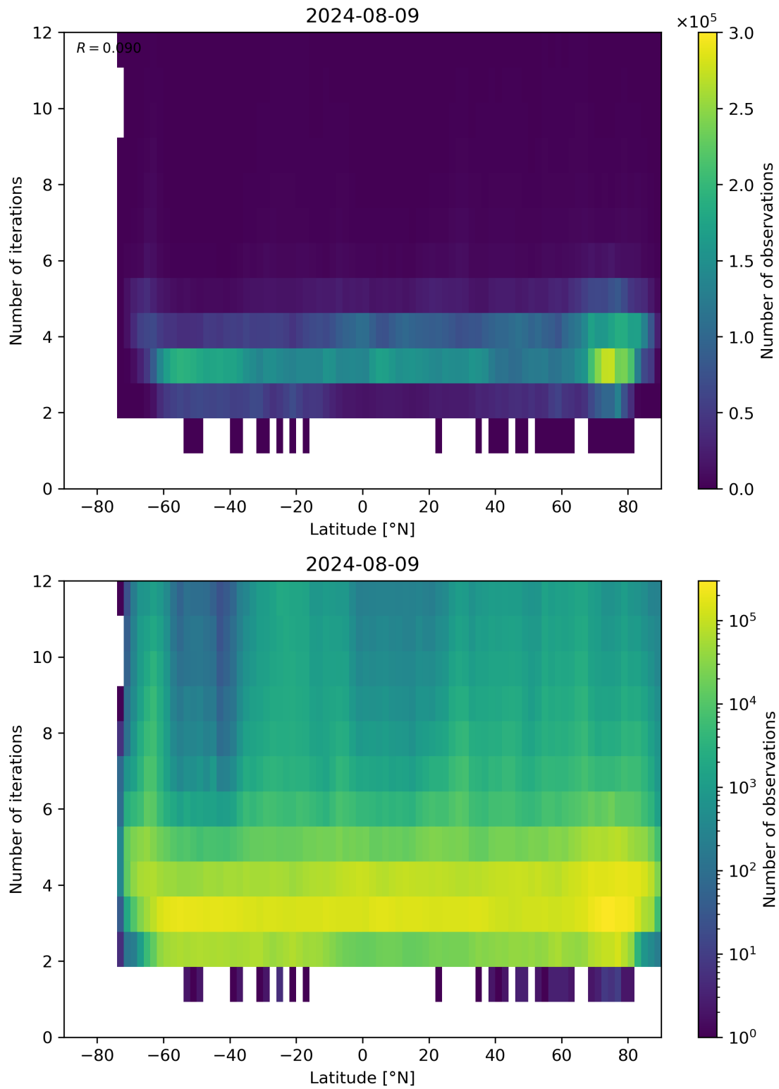
Figure 93: Scatter density plot of “Latitude” against “Number of iterations” for 2024-08-08 to 2024-08-10.
