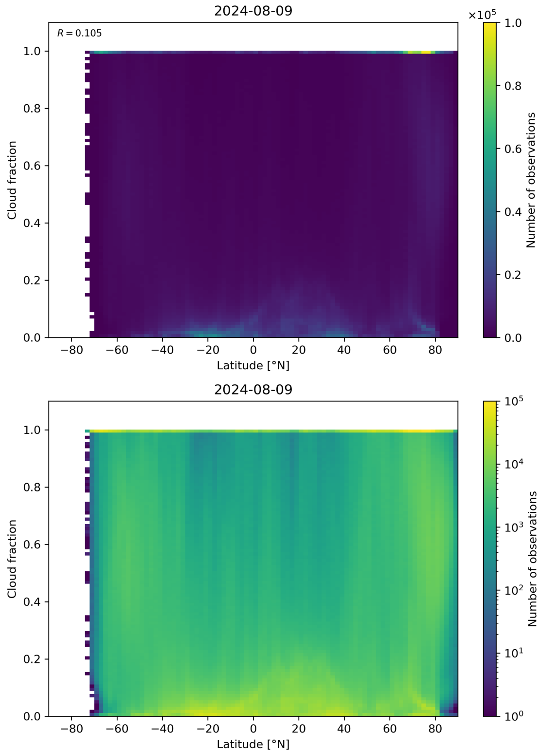
Figure 90: Scatter density plot of “Latitude” against “Cloud fraction” for 2024-08-08 to 2024-08-10.
