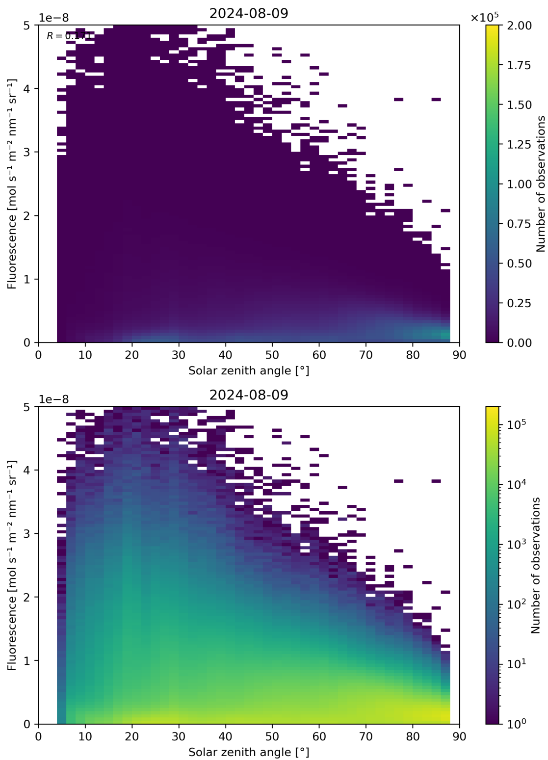
Figure 112: Scatter density plot of “Solar zenith angle” against “Fluorescence” for 2024-08-08 to 2024-08-10.
