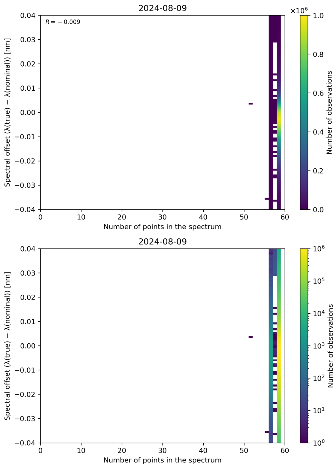
Figure 101: Scatter density plot of “Number of points in the spectrum” against “Spectral offset ( \lambda(\text{true}) - \lambda(\text{nominal}) )” for 2024-08-08 to 2024-08-10.
