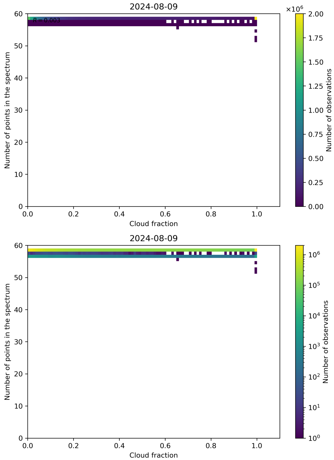
Figure 74: Scatter density plot of “Cloud fraction” against “Number of points in the spectrum” for 2024-08-08 to 2024-08-10.
