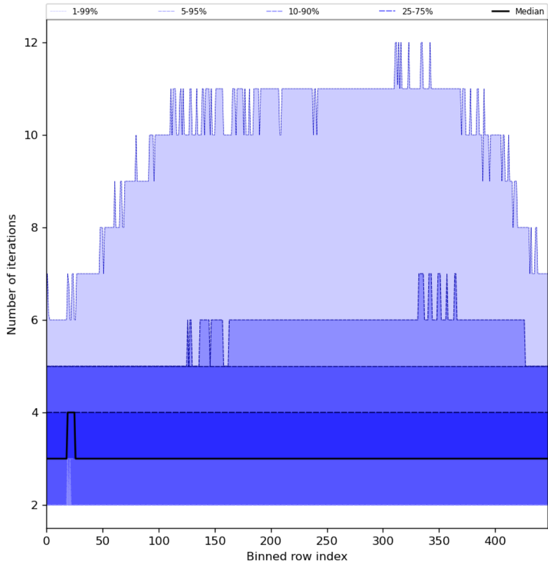
Figure 56: Along track statistics of “Number of iterations” for 2024-08-08 to 2024-08-10
