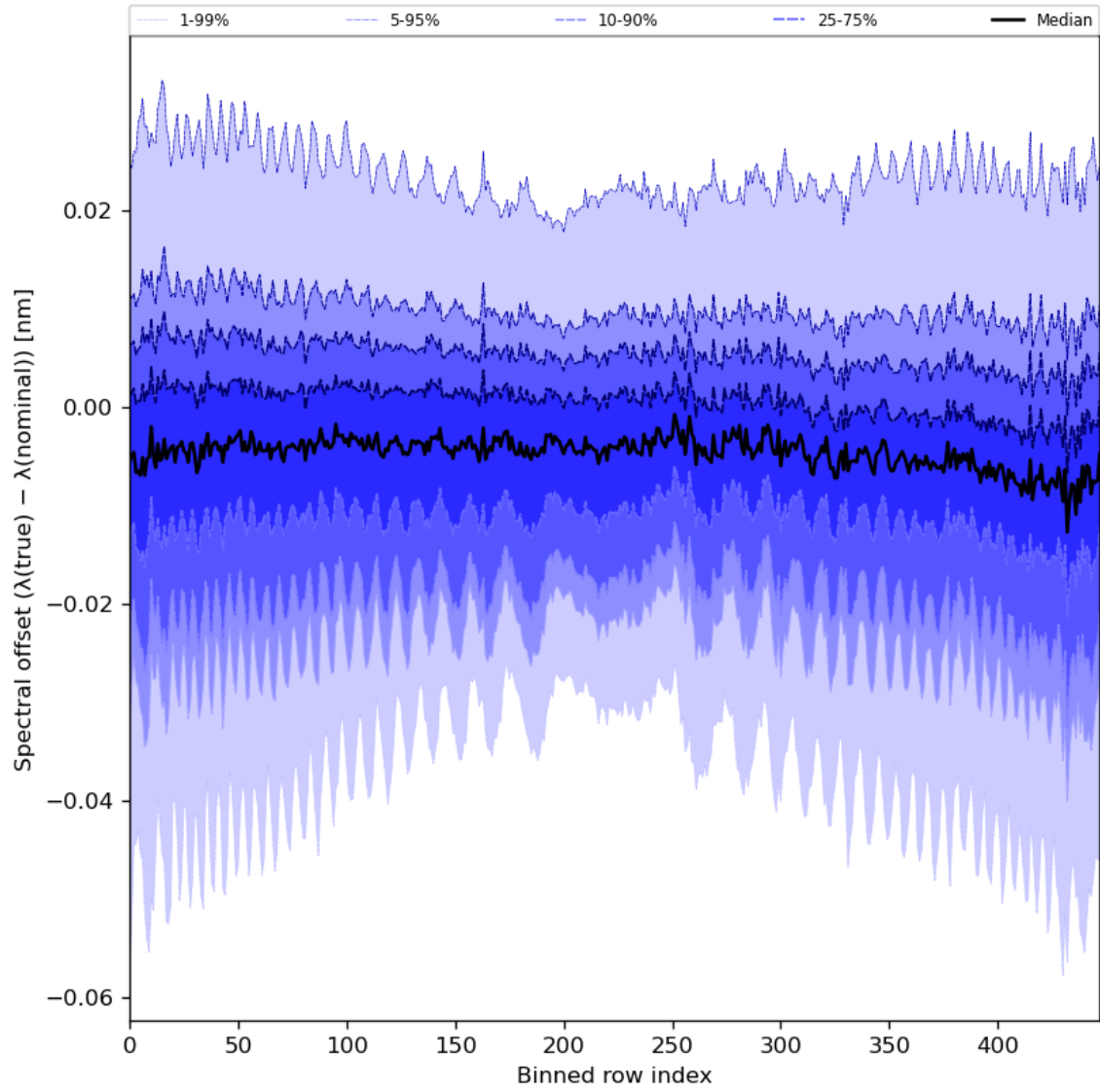
Figure 62: Along track statistics of “Spectral offset ( \lambda(\text{true}) - \lambda(\text{nominal}) )” for 2024-08-08 to 2024-08-10
