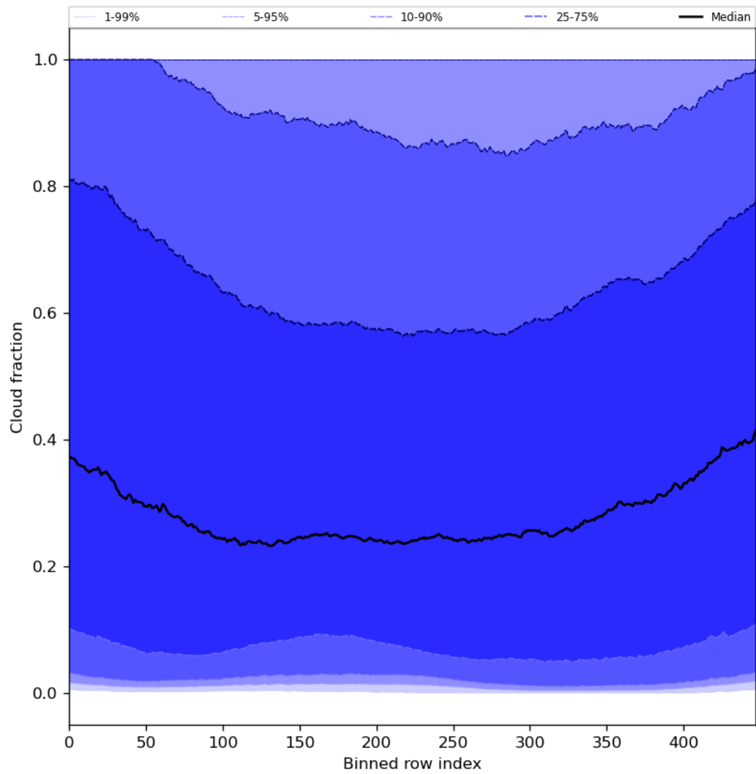
Figure 49: Along track statistics of “Cloud fraction” for 2024-08-08 to 2024-08-10
