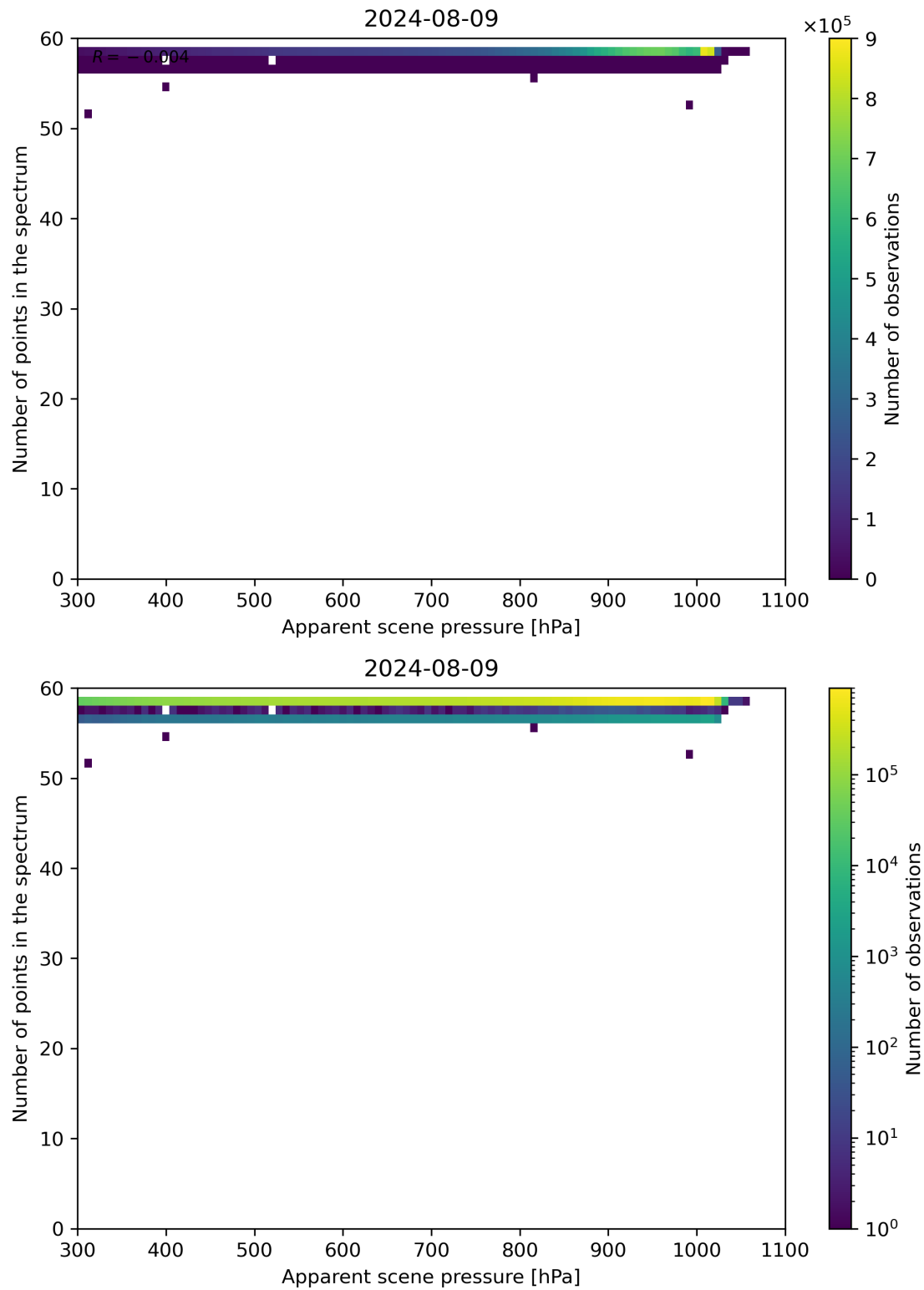
Figure 66: Scatter density plot of “Apparent scene pressure” against “Number of points in the spectrum” for 2024-08-08 to 2024-08-10.
