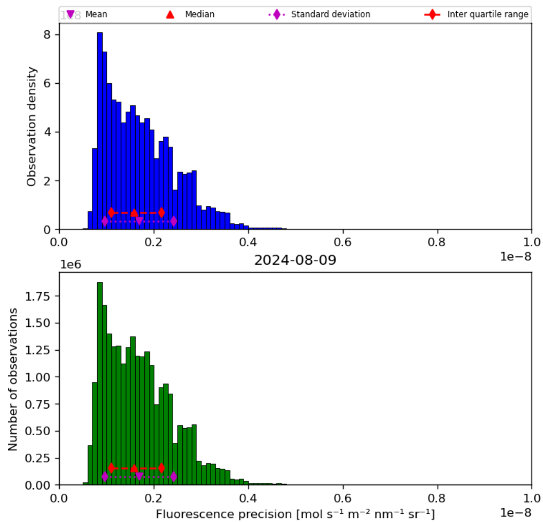
Figure 41: Histogram of “Fluorescence precision” for 2024-08-08 to 2024-08-10
