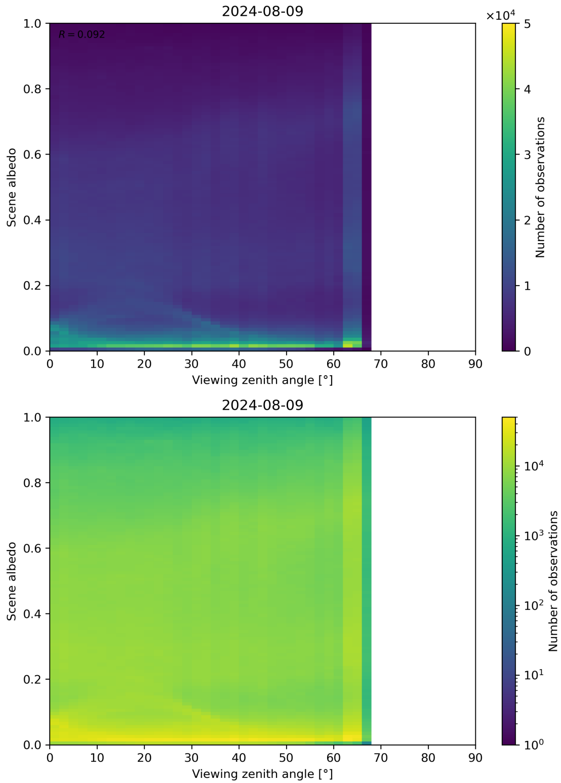
Figure 126: Scatter density plot of “Viewing zenith angle” against “Scene albedo” for 2024-08-08 to 2024-08-10.
