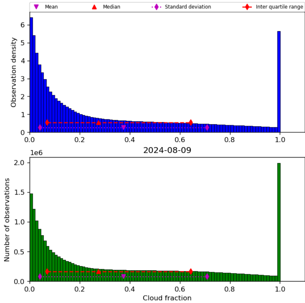
Figure 32: Histogram of “Cloud fraction” for 2024-08-08 to 2024-08-10
