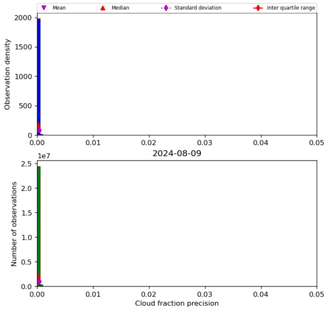
Figure 33: Histogram of “Cloud fraction precision” for 2024-08-08 to 2024-08-10
