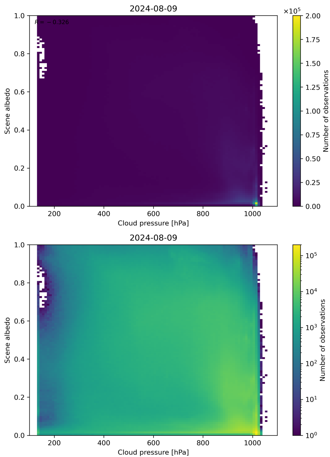
Figure 83: Scatter density plot of “Cloud pressure” against “Scene albedo” for 2024-08-08 to 2024-08-10.
