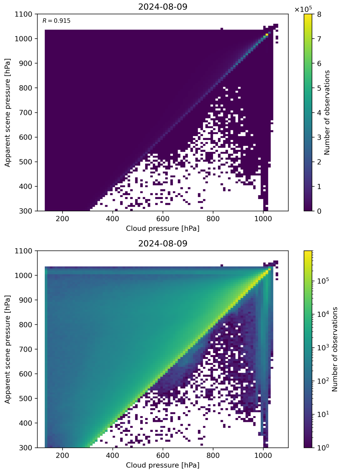
Figure 77: Scatter density plot of “Cloud pressure” against “Apparent scene pressure” for 2024-08-08 to 2024-08-10.
