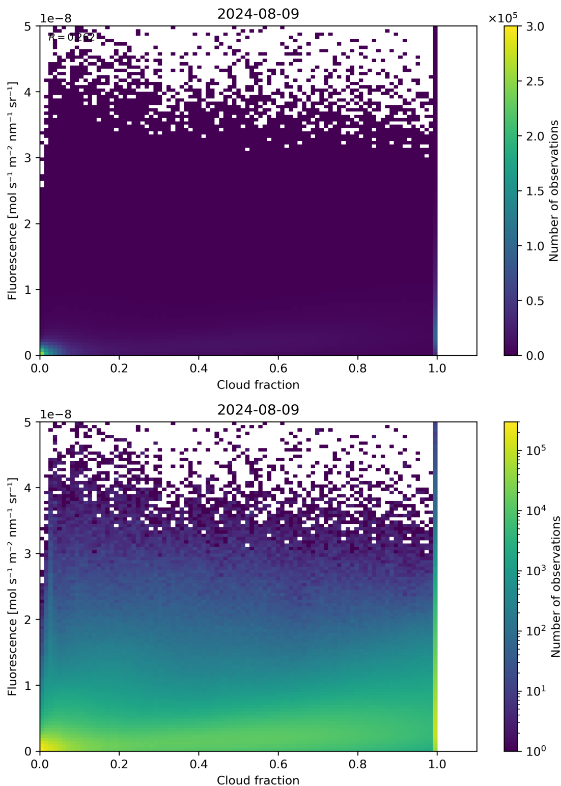
Figure 72: Scatter density plot of “Cloud fraction” against “Fluorescence” for 2024-08-08 to 2024-08-10.
