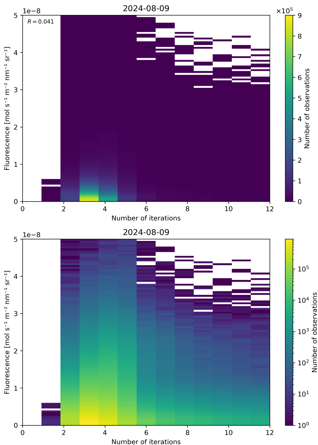
Figure 98: Scatter density plot of “Number of iterations” against “Fluorescence” for 2024-08-08 to 2024-08-10.
