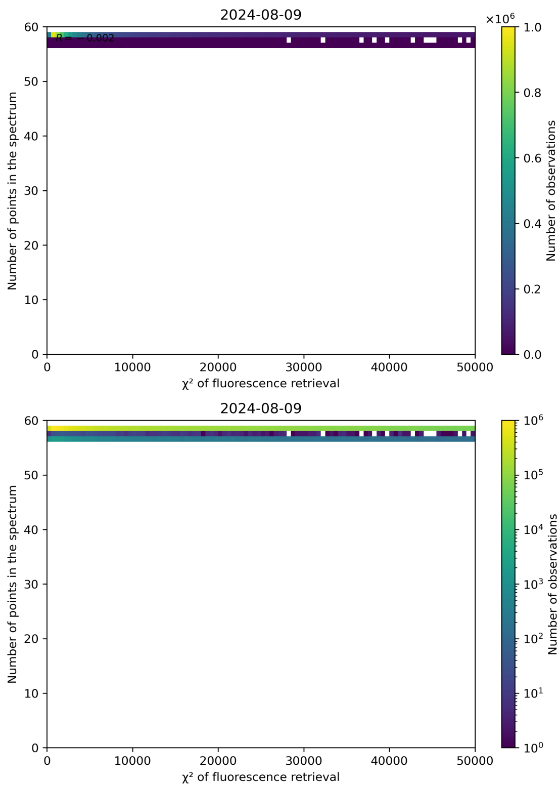
Figure 68: Scatter density plot of “ \chi^2 of fluorescence retrieval” against “Number of points in the spectrum” for 2024-08-08 to 2024-08-10.
