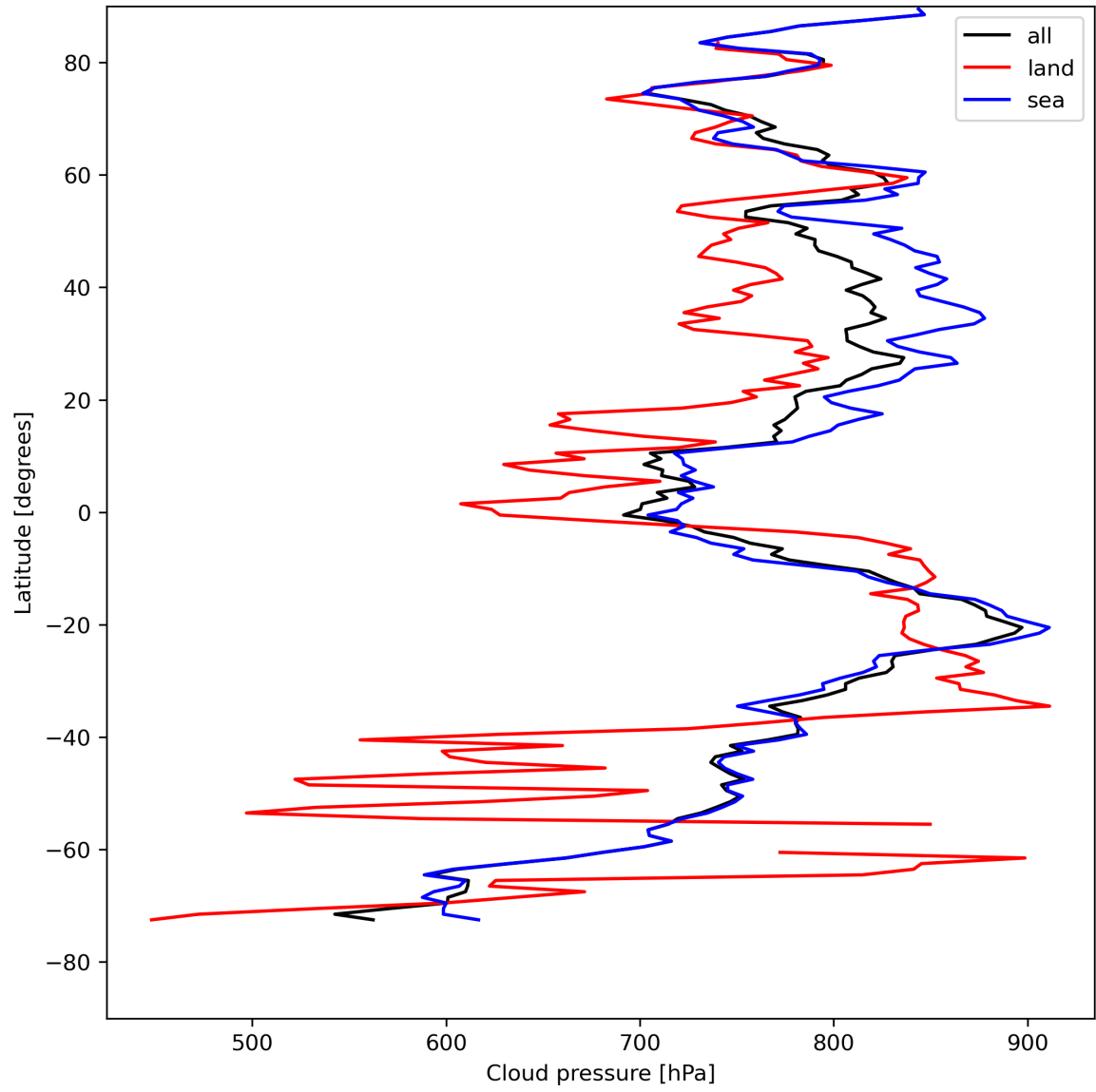
Figure 13: Zonal average of “Cloud pressure” for 2024-08-08 to 2024-08-10.
