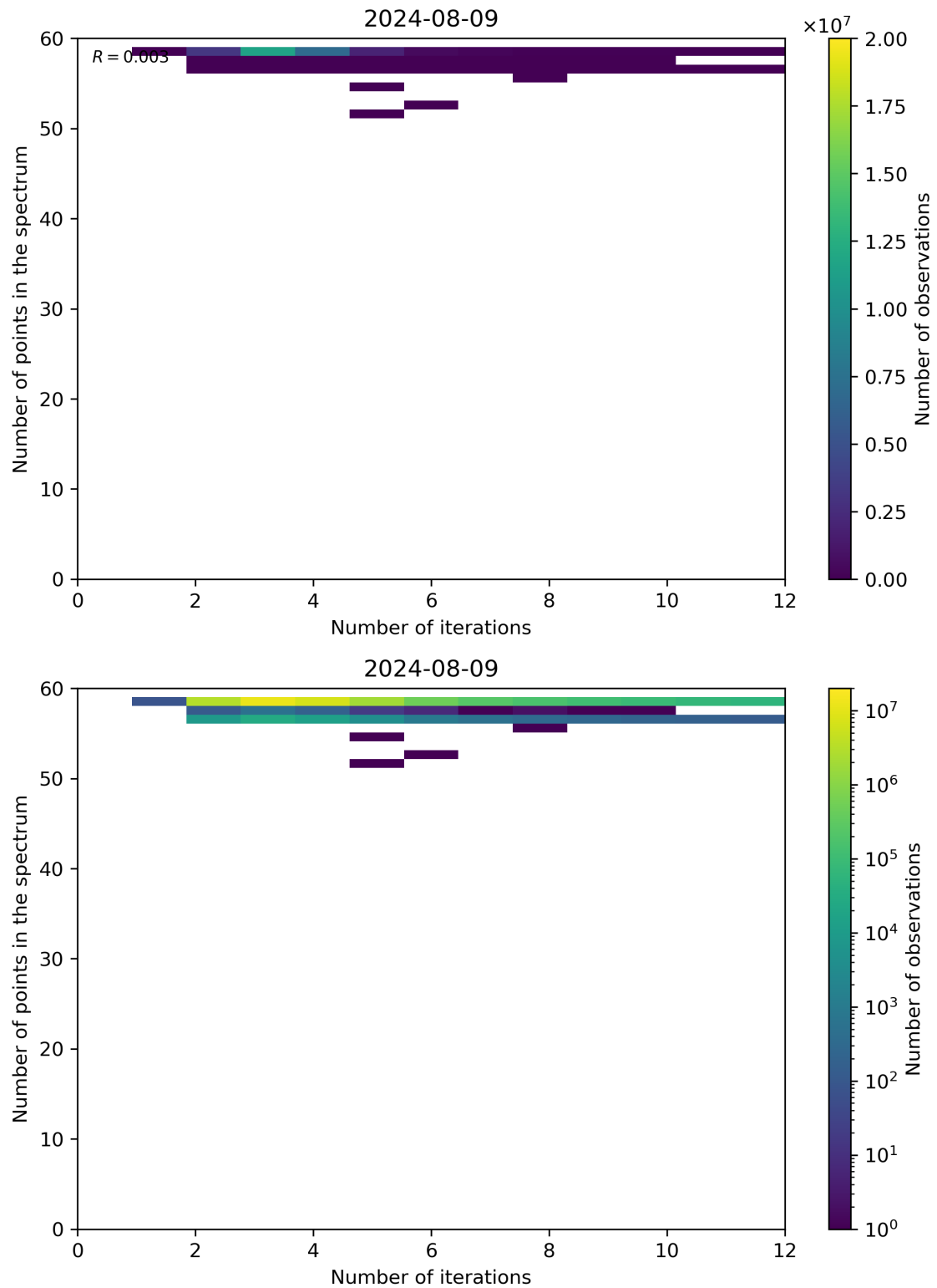
Figure 99: Scatter density plot of “Number of iterations” against “Number of points in the spectrum” for 2024-08-08 to 2024-08-10.
