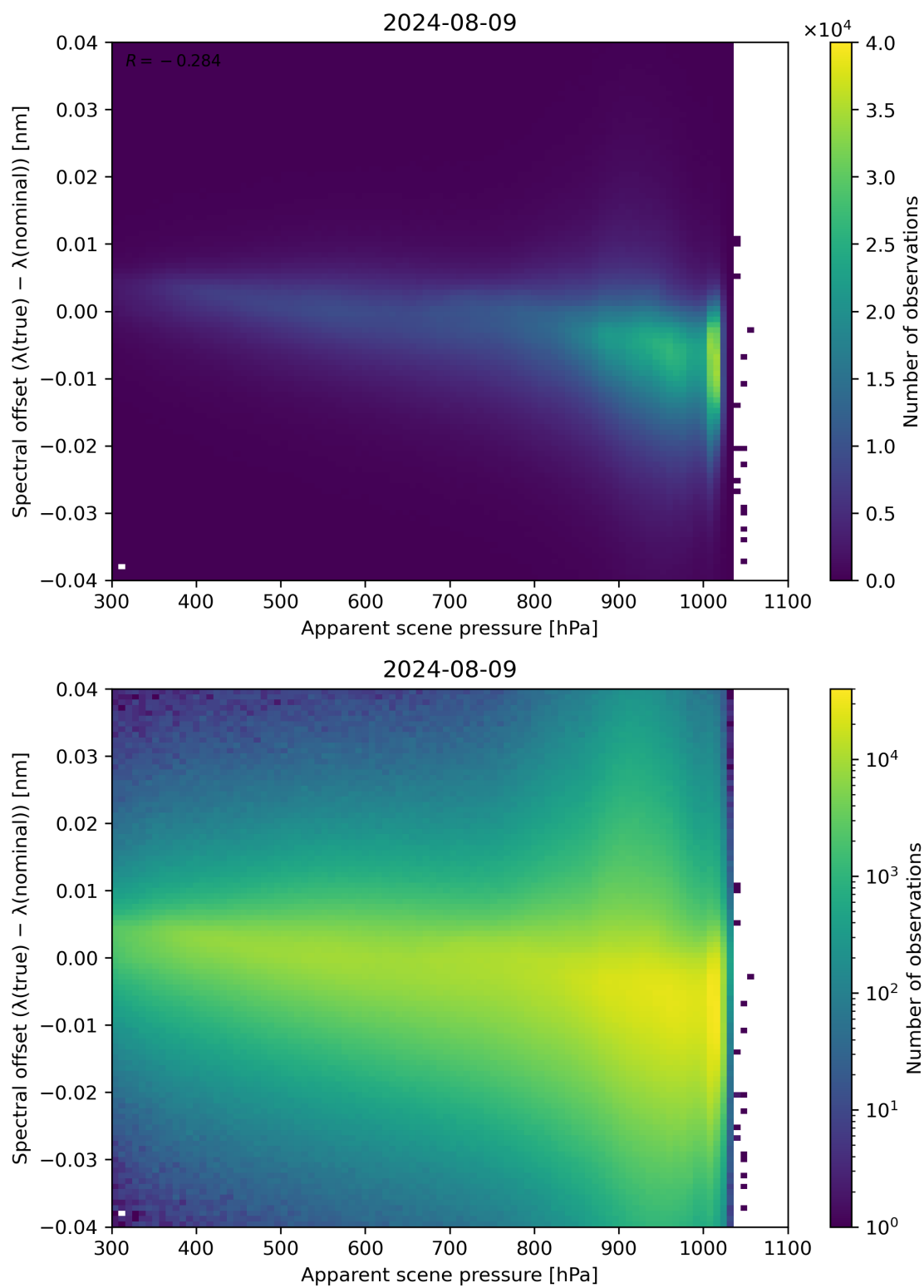
Figure 67: Scatter density plot of “Apparent scene pressure” against “Spectral offset ( \lambda(\text{true}) - \lambda(\text{nominal}) )” for 2024-08-08 to 2024-08-10.
