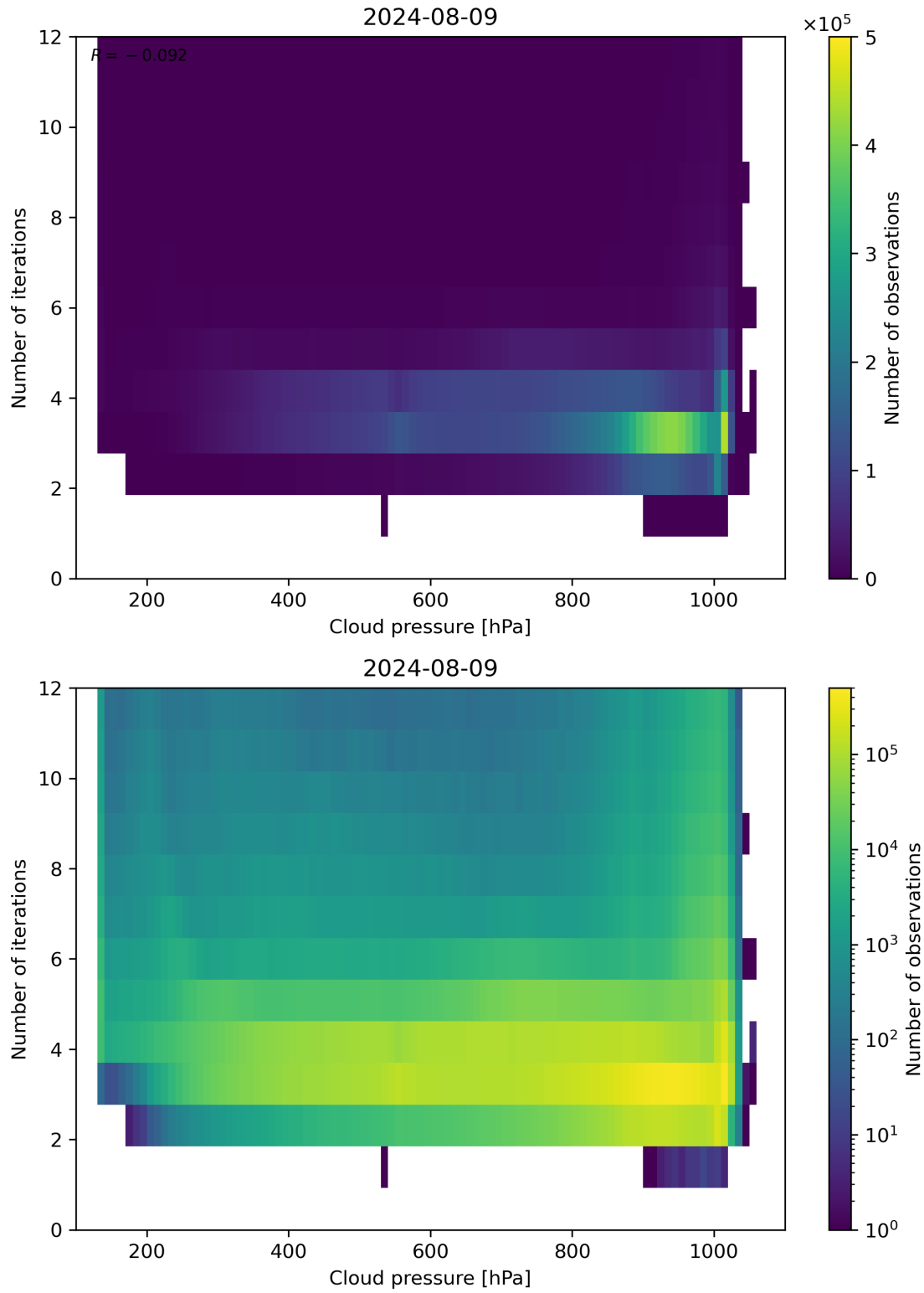
Figure 81: Scatter density plot of “Cloud pressure” against “Number of iterations” for 2024-08-08 to 2024-08-10.
