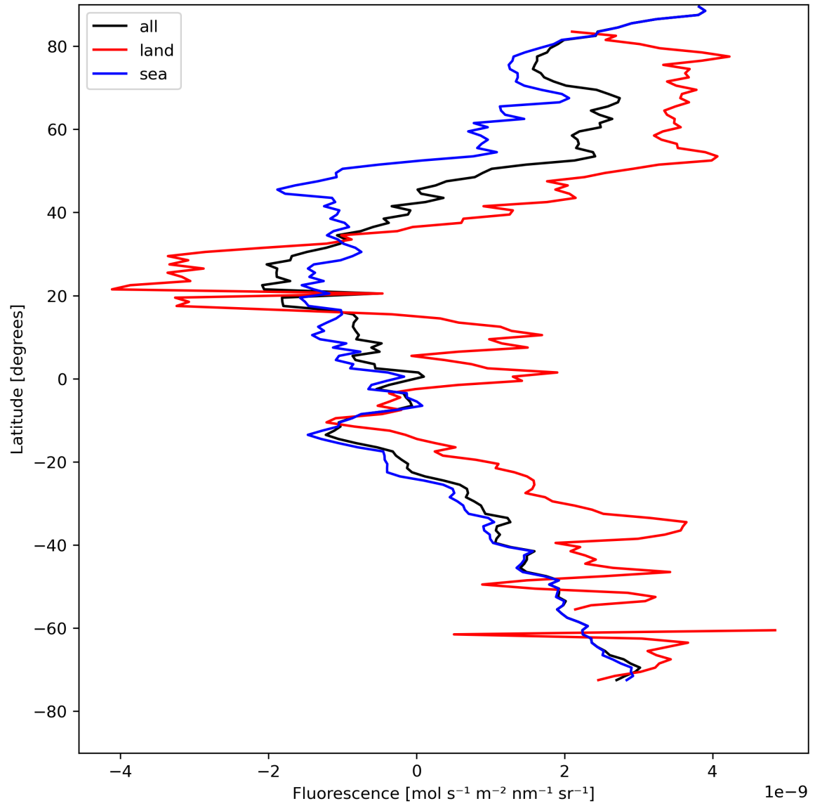
Figure 23: Zonal average of “Fluorescence” for 2024-08-08 to 2024-08-10.
