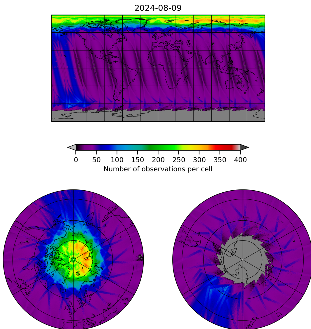
Figure 11: Map of the number of observations for 2024-08-08 to 2024-08-10
