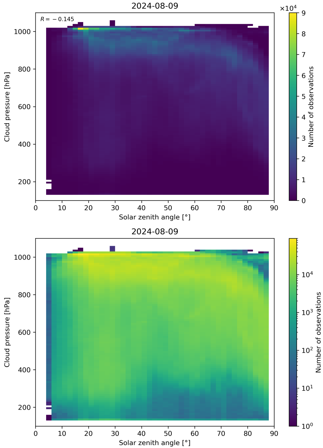
Figure 111: Scatter density plot of “Solar zenith angle” against “Cloud pressure” for 2024-08-08 to 2024-08-10.
