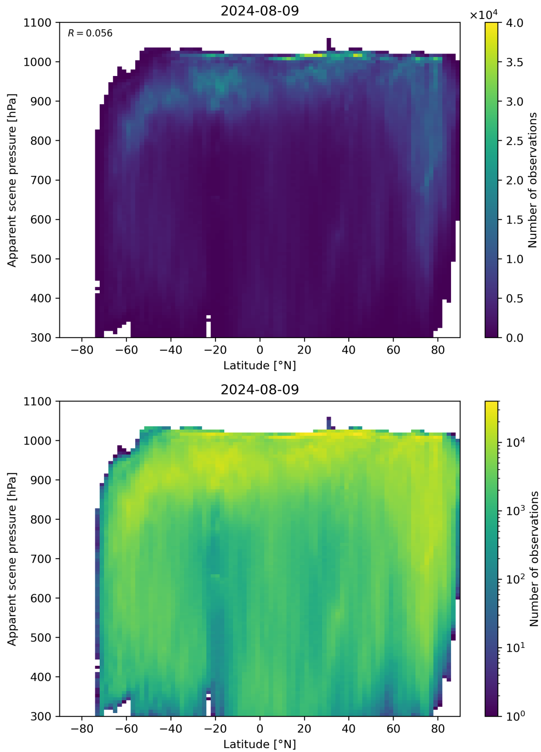
Figure 88: Scatter density plot of “Latitude” against “Apparent scene pressure” for 2024-08-08 to 2024-08-10.
