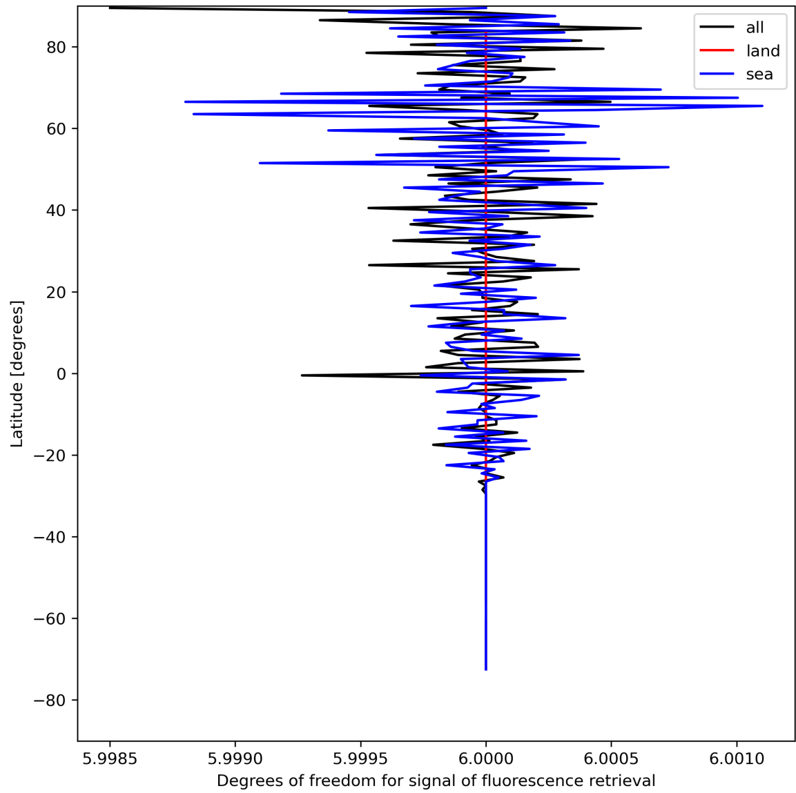
Figure 26: Zonal average of “Degrees of freedom for signal of fluorescence retrieval” for 2024-08-08 to 2024-08-10.
