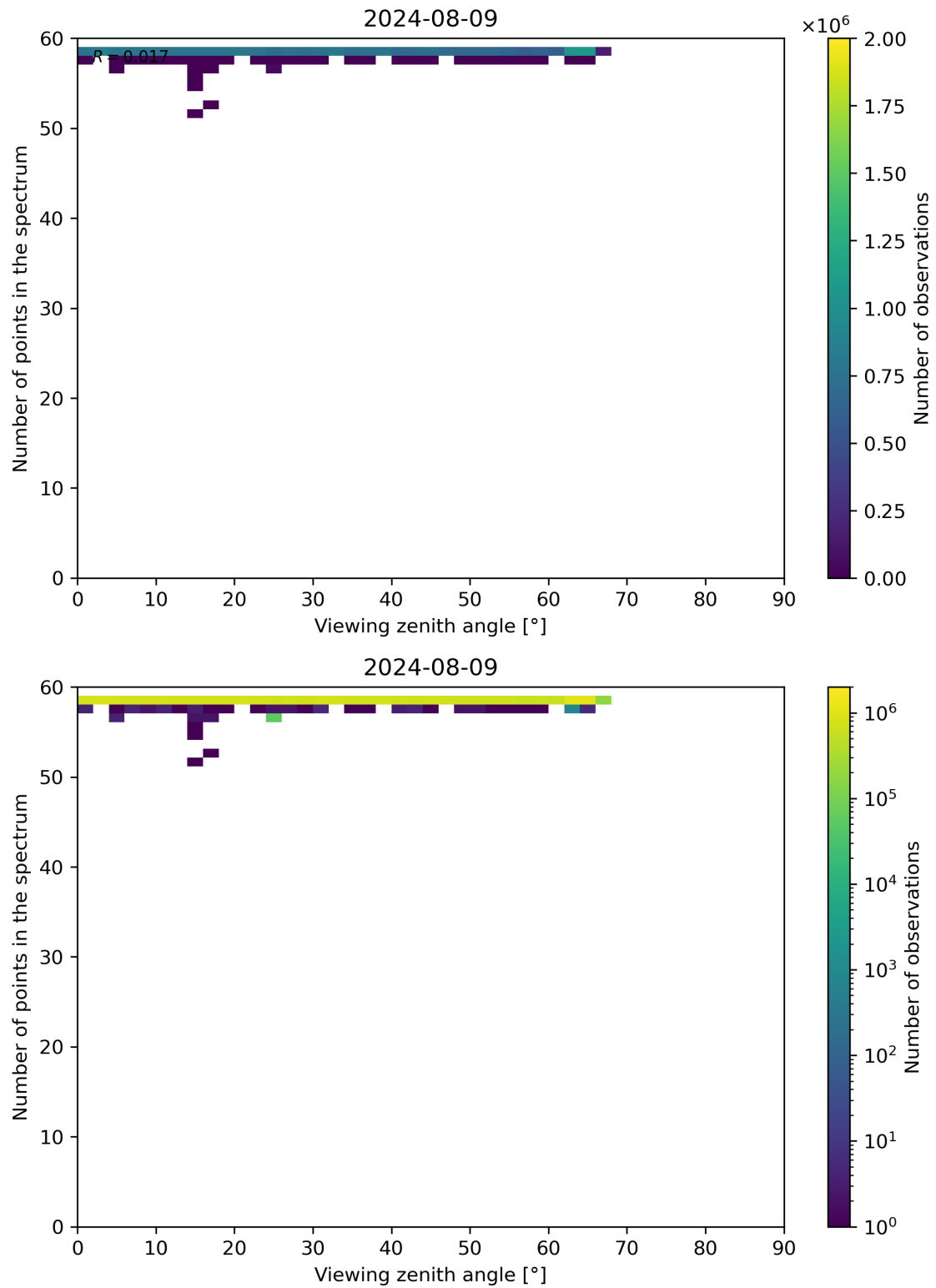
Figure 125: Scatter density plot of “Viewing zenith angle” against “Number of points in the spectrum” for 2024-08-08 to 2024-08-10.
