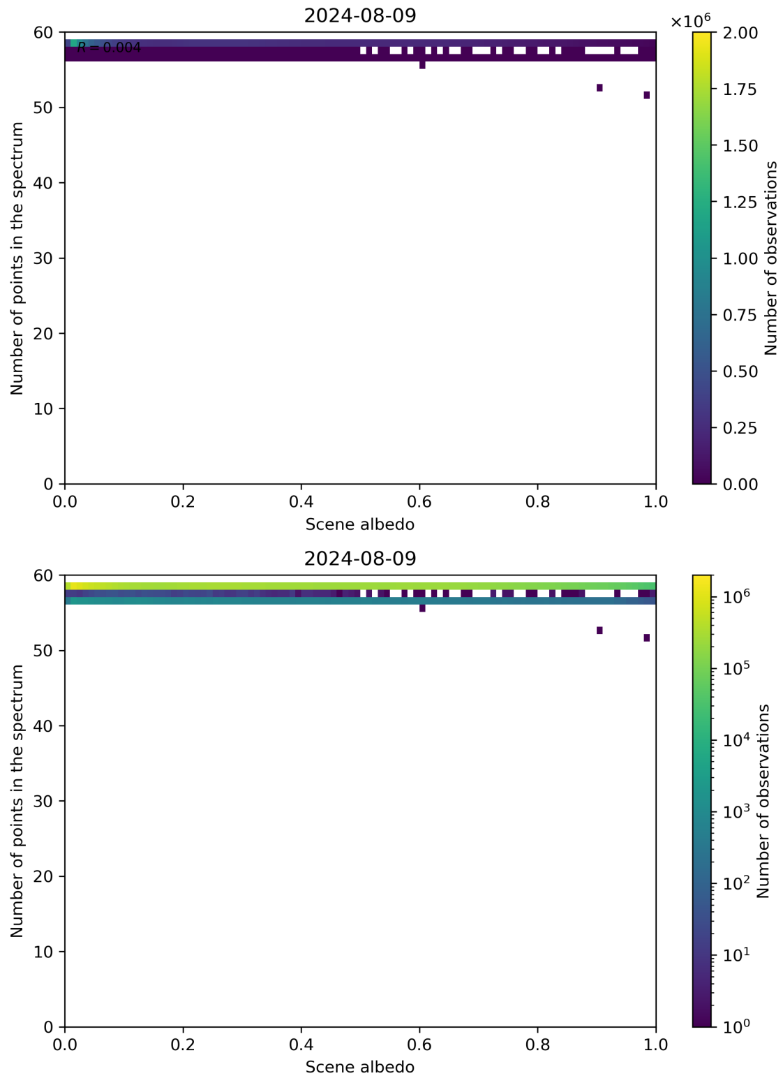
Figure 106: Scatter density plot of “Scene albedo” against “Number of points in the spectrum” for 2024-08-08 to 2024-08-10.
