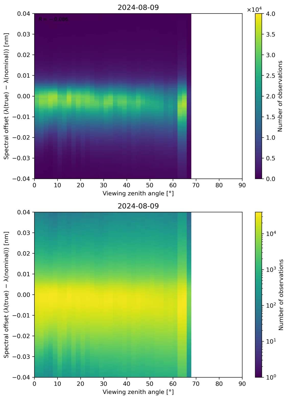
Figure 128: Scatter density plot of “Viewing zenith angle” against “Spectral offset ( \lambda(\text{true}) - \lambda(\text{nominal}) )” for 2024-08-08 to 2024-08-10.
