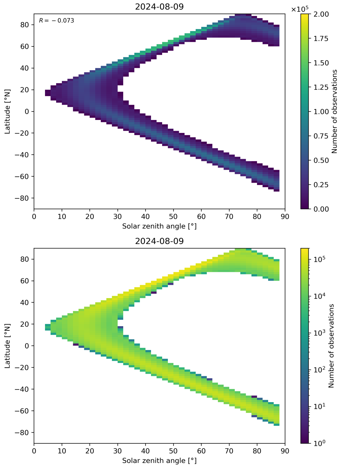
Figure 113: Scatter density plot of “Solar zenith angle” against “Latitude” for 2024-08-08 to 2024-08-10.
