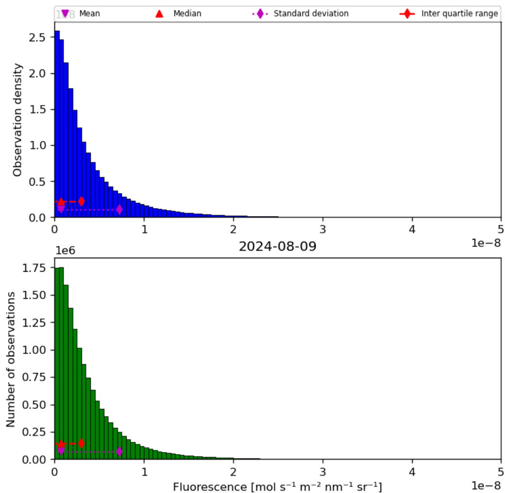
Figure 40: Histogram of “Fluorescence” for 2024-08-08 to 2024-08-10
