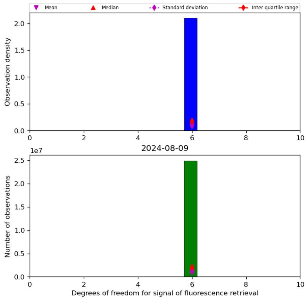
Figure 43: Histogram of “Degrees of freedom for signal of fluorescence retrieval” for 2024-08-08 to 2024-08-10
