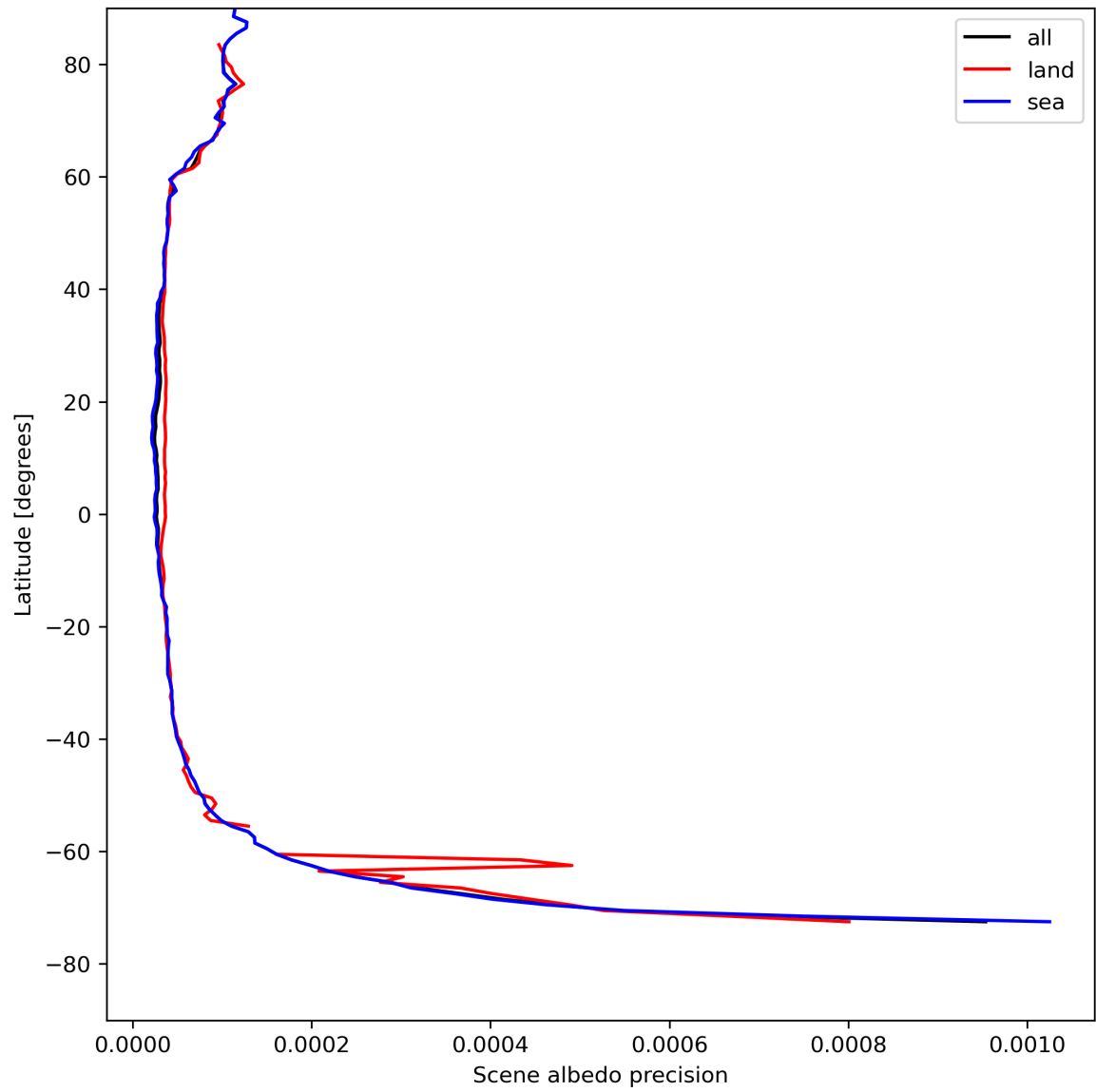
Figure 18: Zonal average of “Scene albedo precision” for 2024-08-08 to 2024-08-10.
