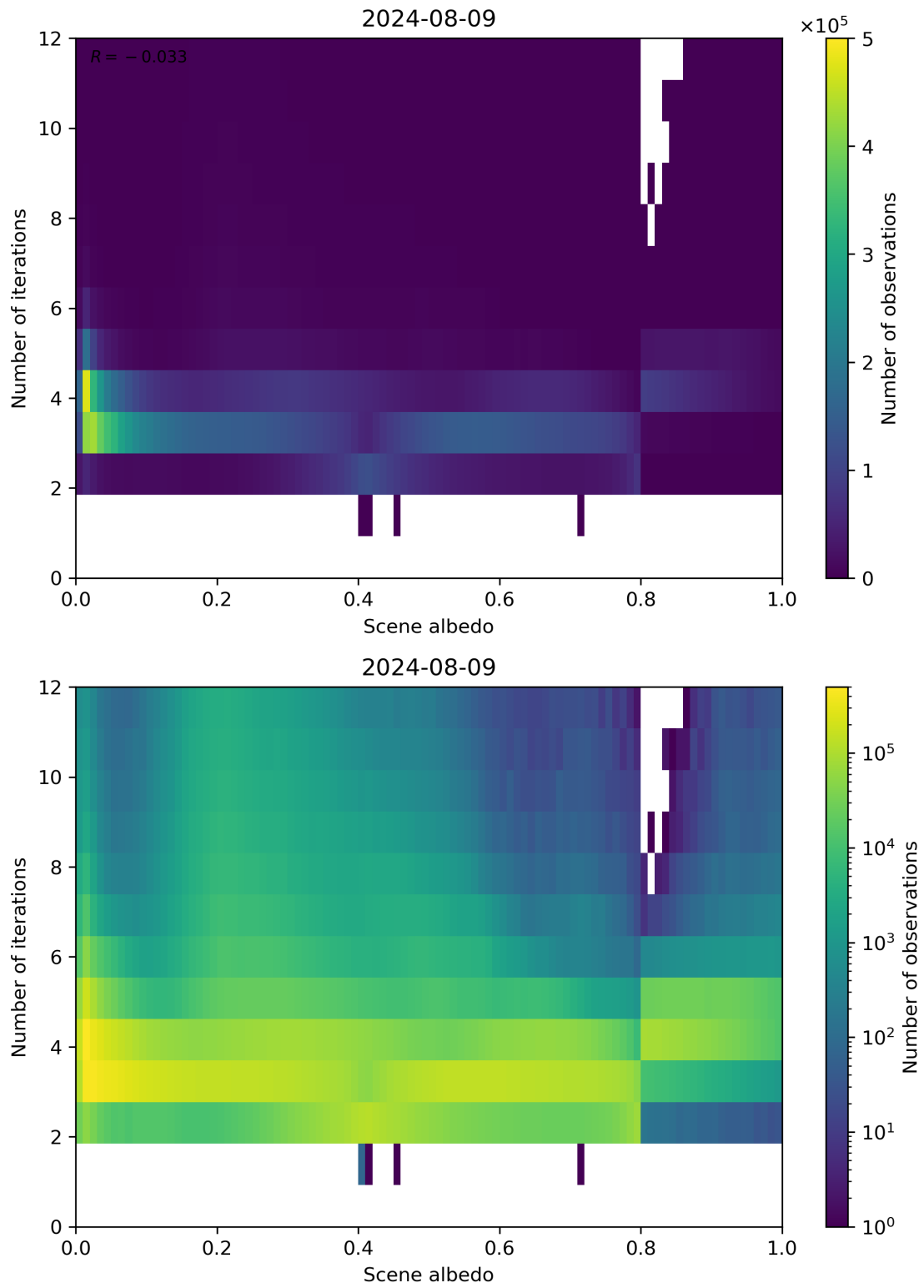
Figure 105: Scatter density plot of “Scene albedo” against “Number of iterations” for 2024-08-08 to 2024-08-10.
