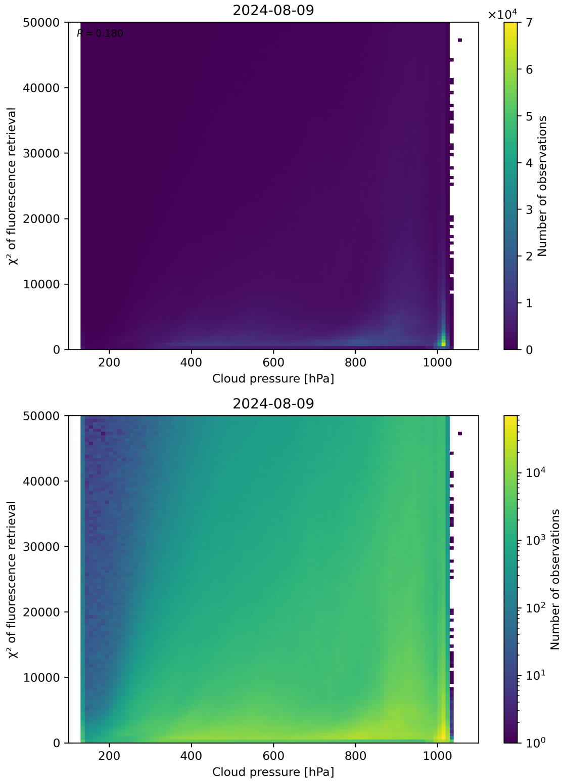
Figure 78: Scatter density plot of “Cloud pressure” against “ \chi^2 of fluorescence retrieval” for 2024-08-08 to 2024-08-10.
