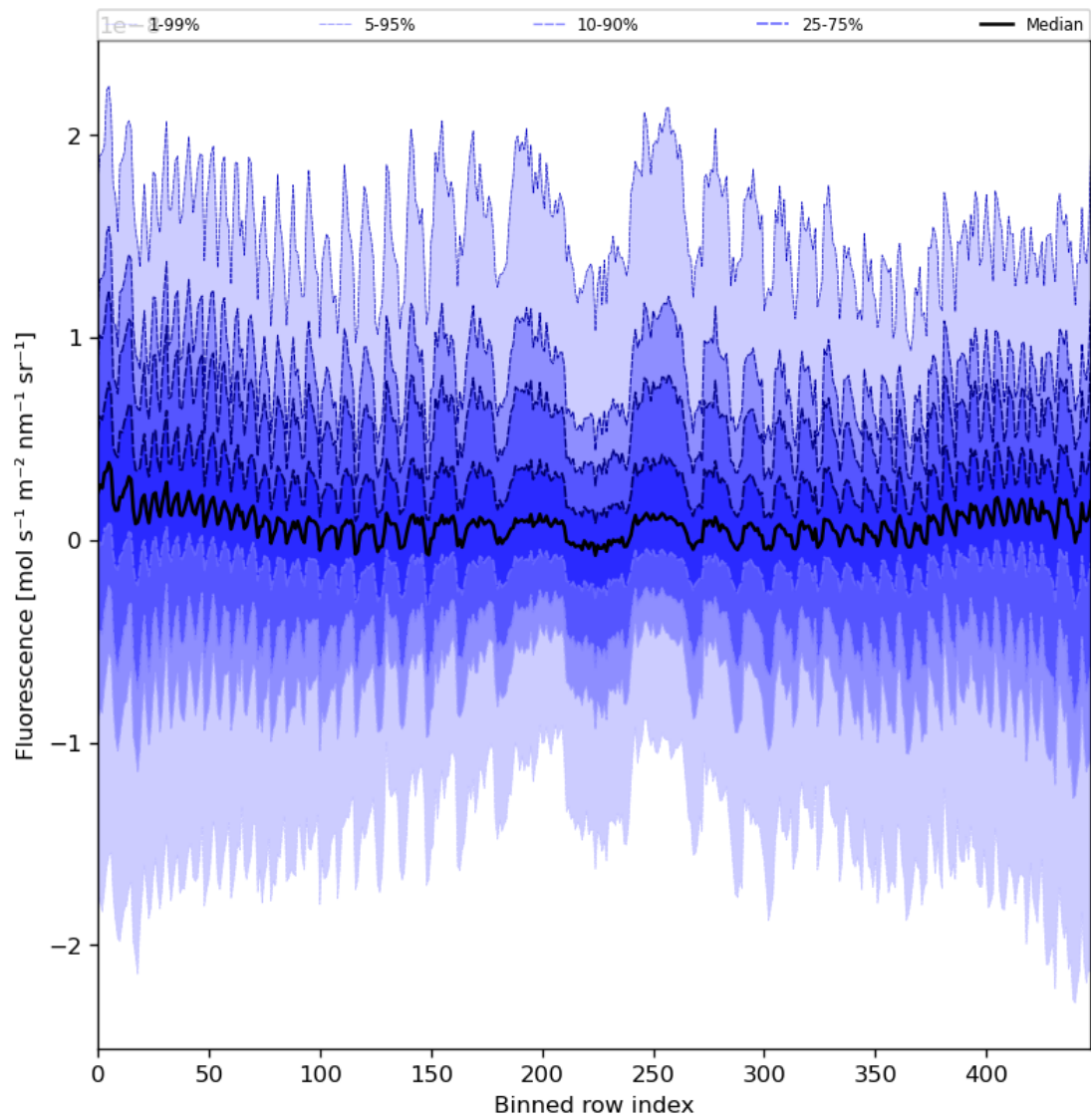
Figure 57: Along track statistics of “Fluorescence” for 2024-08-08 to 2024-08-10
