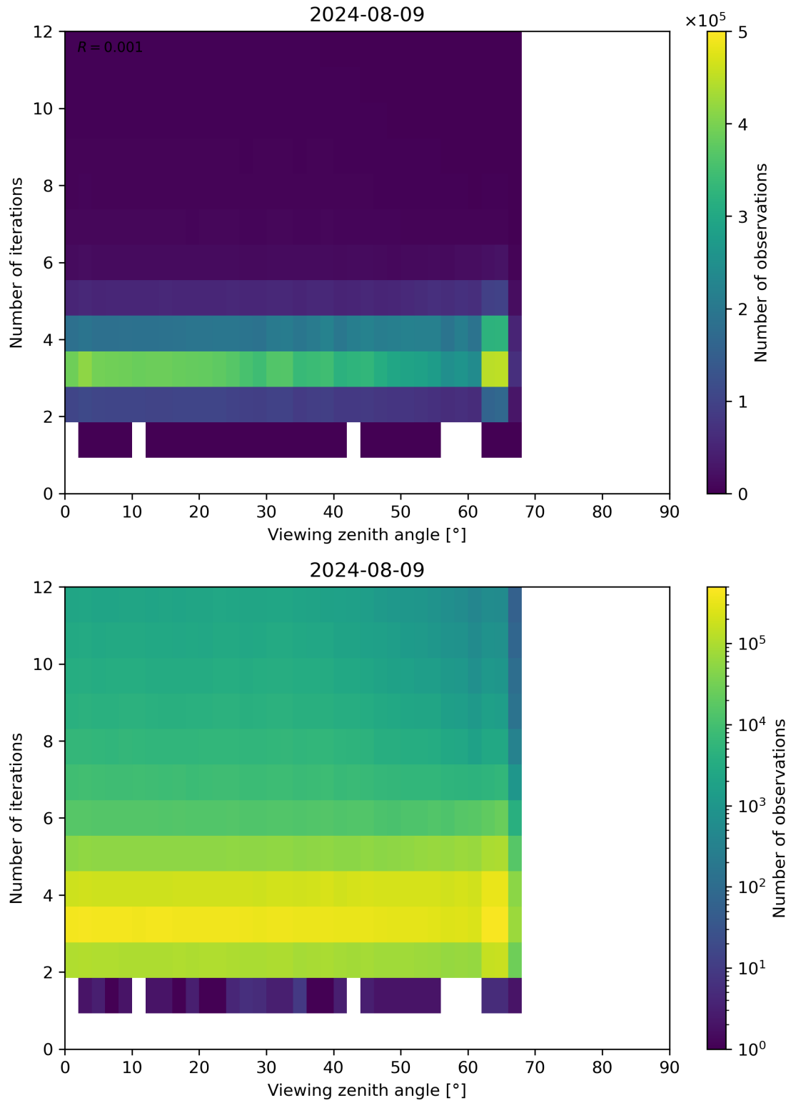
Figure 124: Scatter density plot of “Viewing zenith angle” against “Number of iterations” for 2024-08-08 to 2024-08-10.
