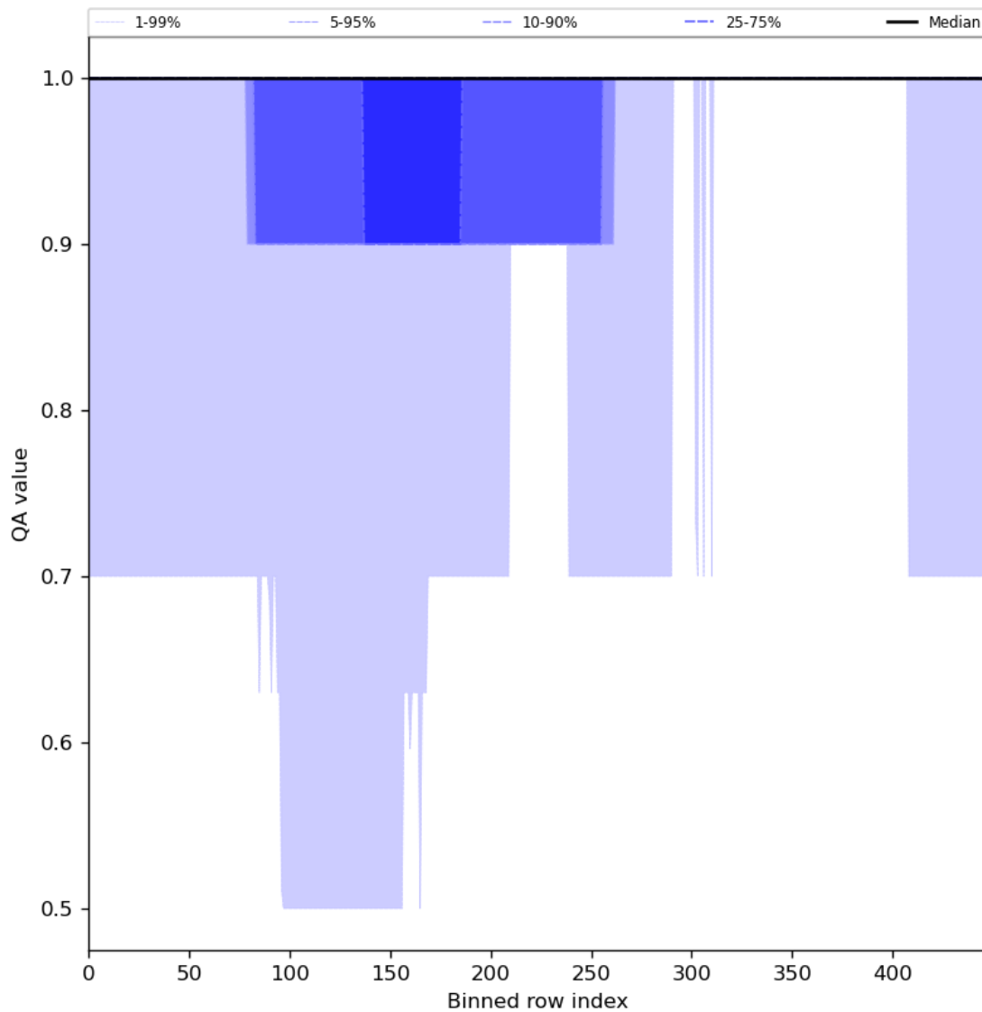
Figure 46: Along track statistics of “QA value” for 2024-08-08 to 2024-08-10
