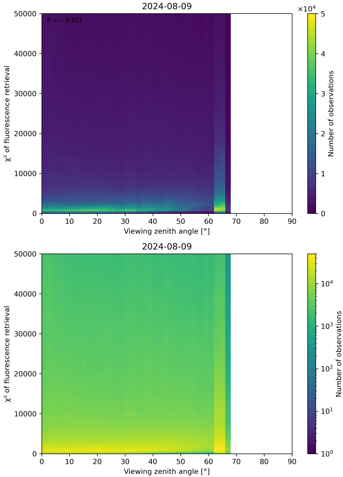
Figure 119: Scatter density plot of “Viewing zenith angle” against “ \chi^2 of fluorescence retrieval” for 2024-08-08 to 2024-08-10.
