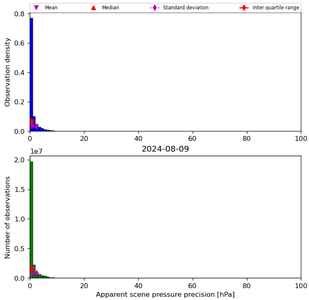
Figure 37: Histogram of “Apparent scene pressure precision” for 2024-08-08 to 2024-08-10
