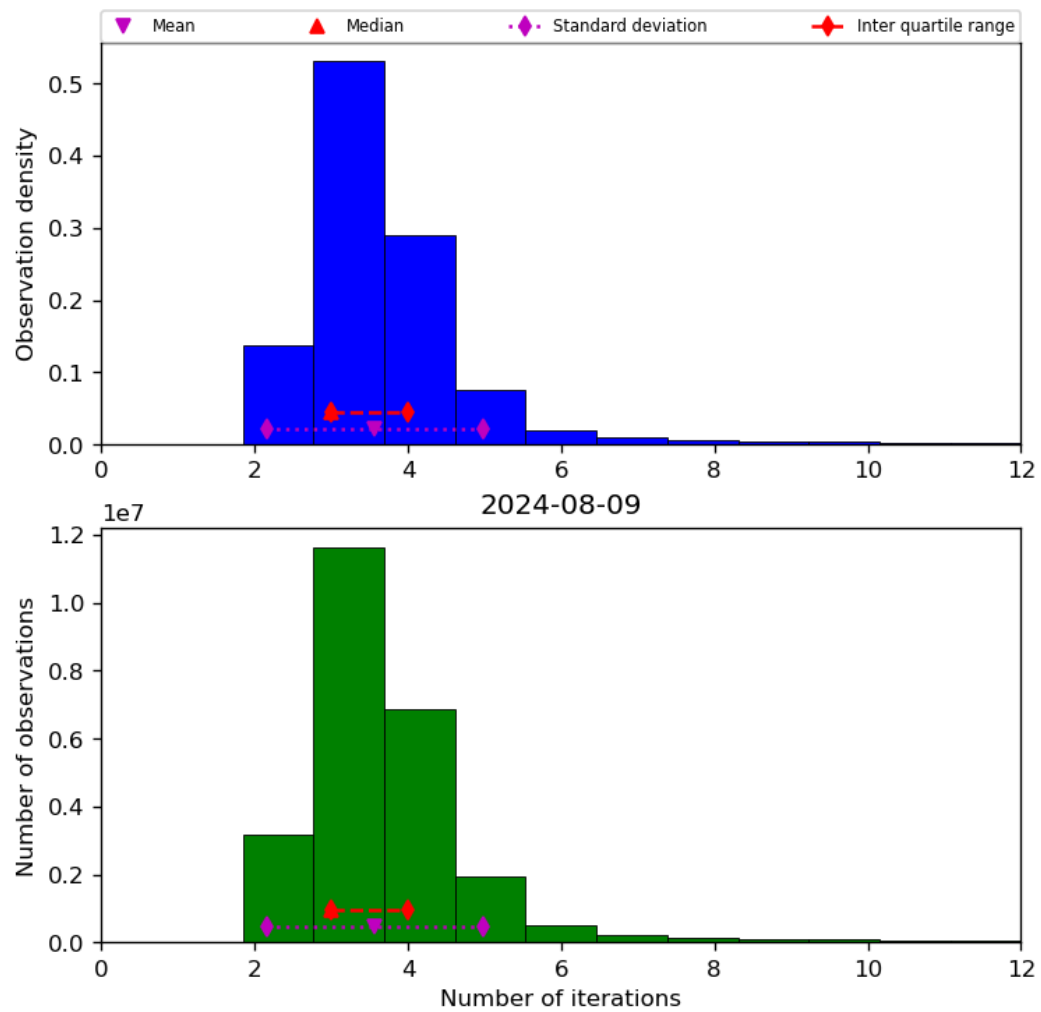
Figure 39: Histogram of “Number of iterations” for 2024-08-08 to 2024-08-10
