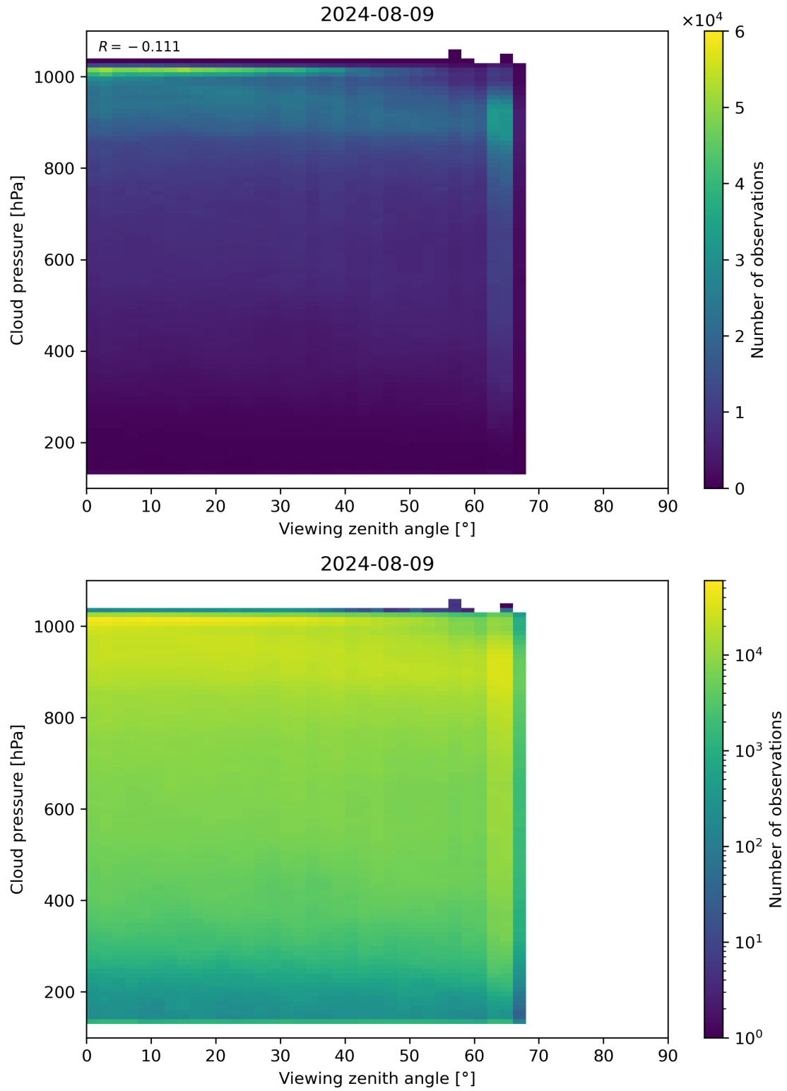
Figure 121: Scatter density plot of “Viewing zenith angle” against “Cloud pressure” for 2024-08-08 to 2024-08-10.
