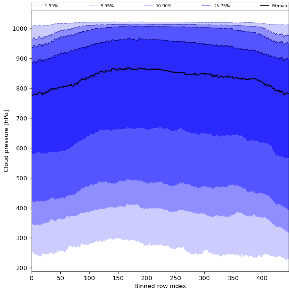
Figure 47: Along track statistics of “Cloud pressure” for 2024-08-08 to 2024-08-10
