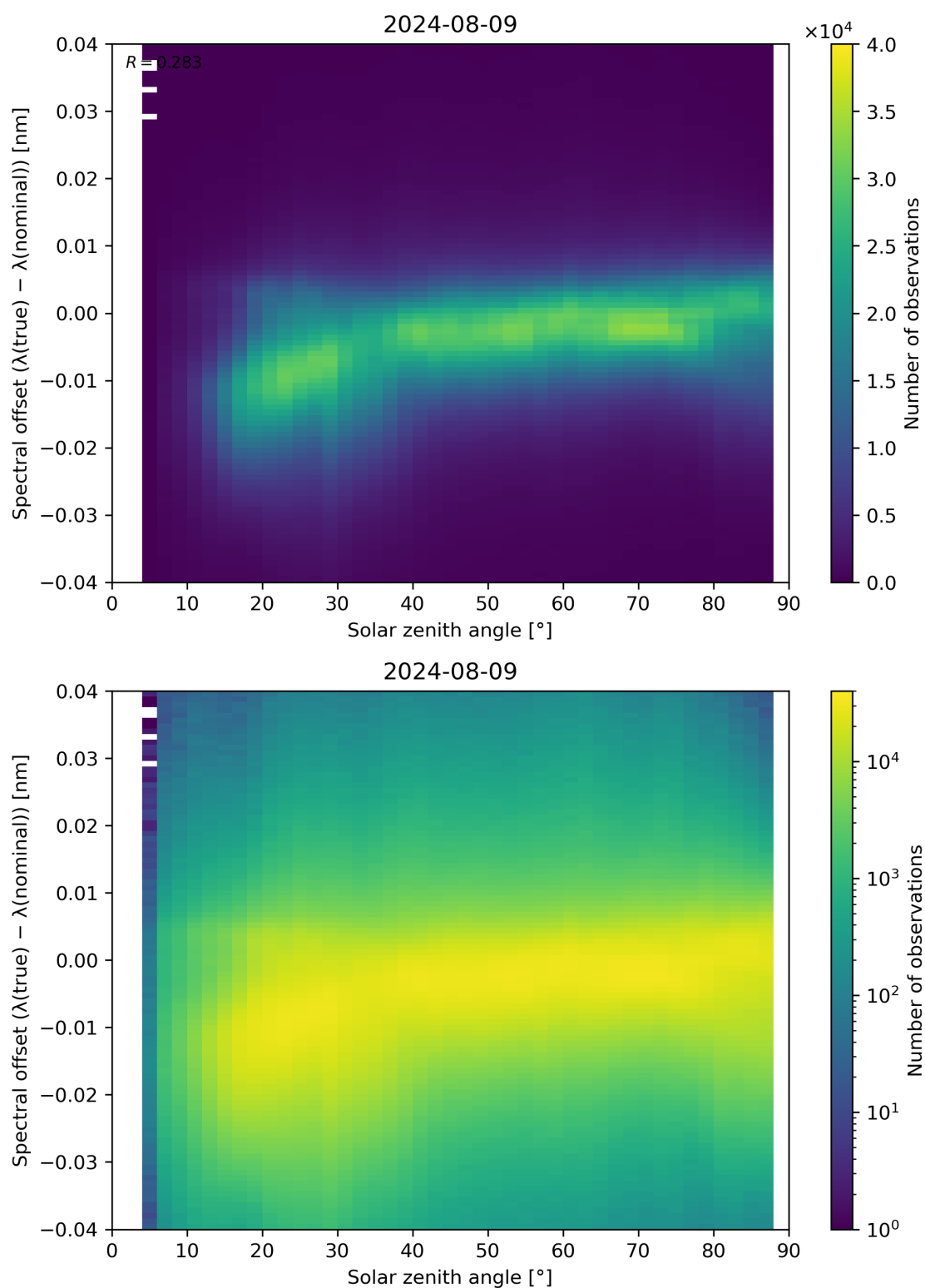
Figure 117: Scatter density plot of “Solar zenith angle” against “Spectral offset ( \lambda(\text{true}) - \lambda(\text{nominal}) )” for 2024-08-08 to 2024-08-10.
