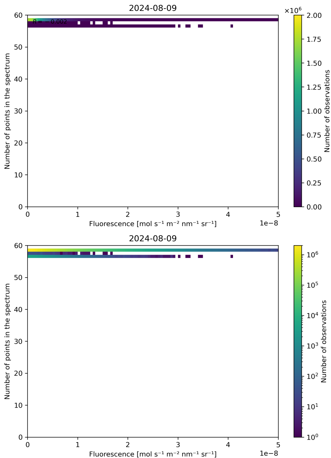
Figure 86: Scatter density plot of “Fluorescence” against “Number of points in the spectrum” for 2024-08-08 to 2024-08-10.
