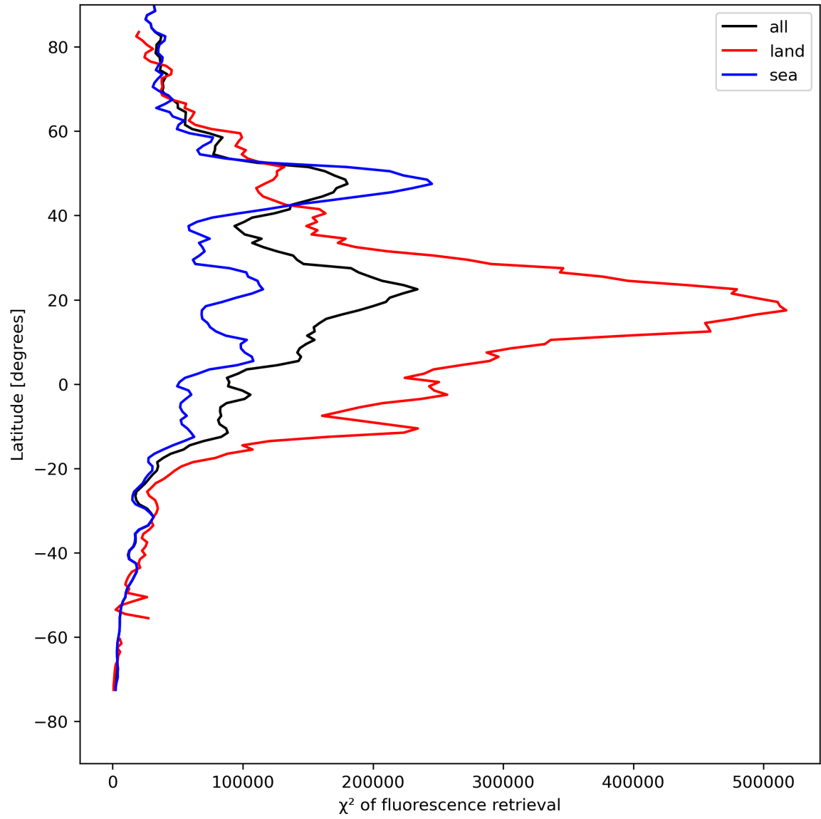
Figure 25: Zonal average of “ \chi^2 of fluorescence retrieval” for 2024-08-08 to 2024-08-10.
