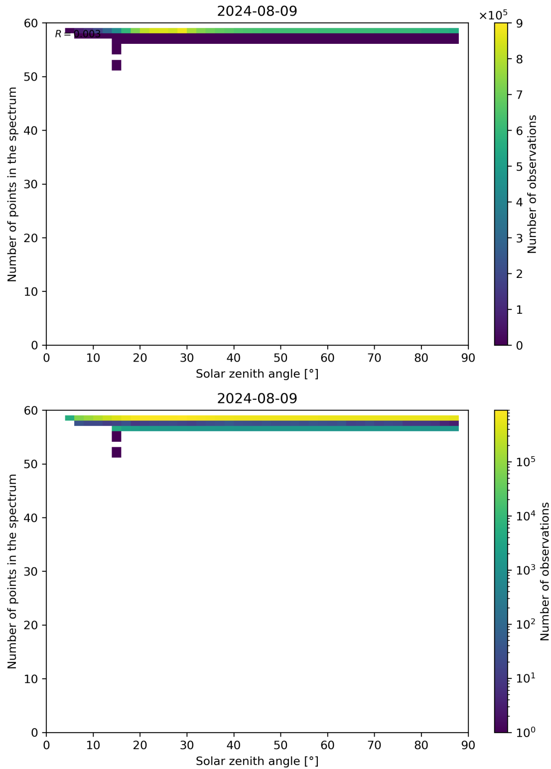
Figure 115: Scatter density plot of “Solar zenith angle” against “Number of points in the spectrum” for 2024-08-08 to 2024-08-10.
