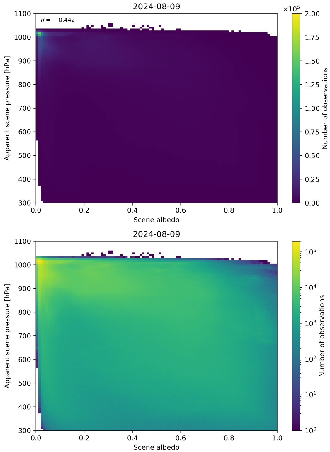
Figure 102: Scatter density plot of “Scene albedo” against “Apparent scene pressure” for 2024-08-08 to 2024-08-10.
