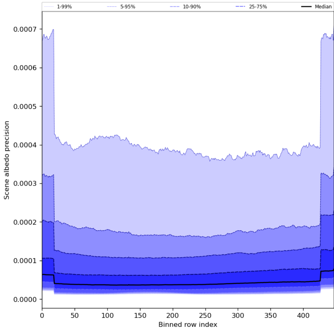
Figure 52: Along track statistics of “Scene albedo precision” for 2024-08-08 to 2024-08-10
