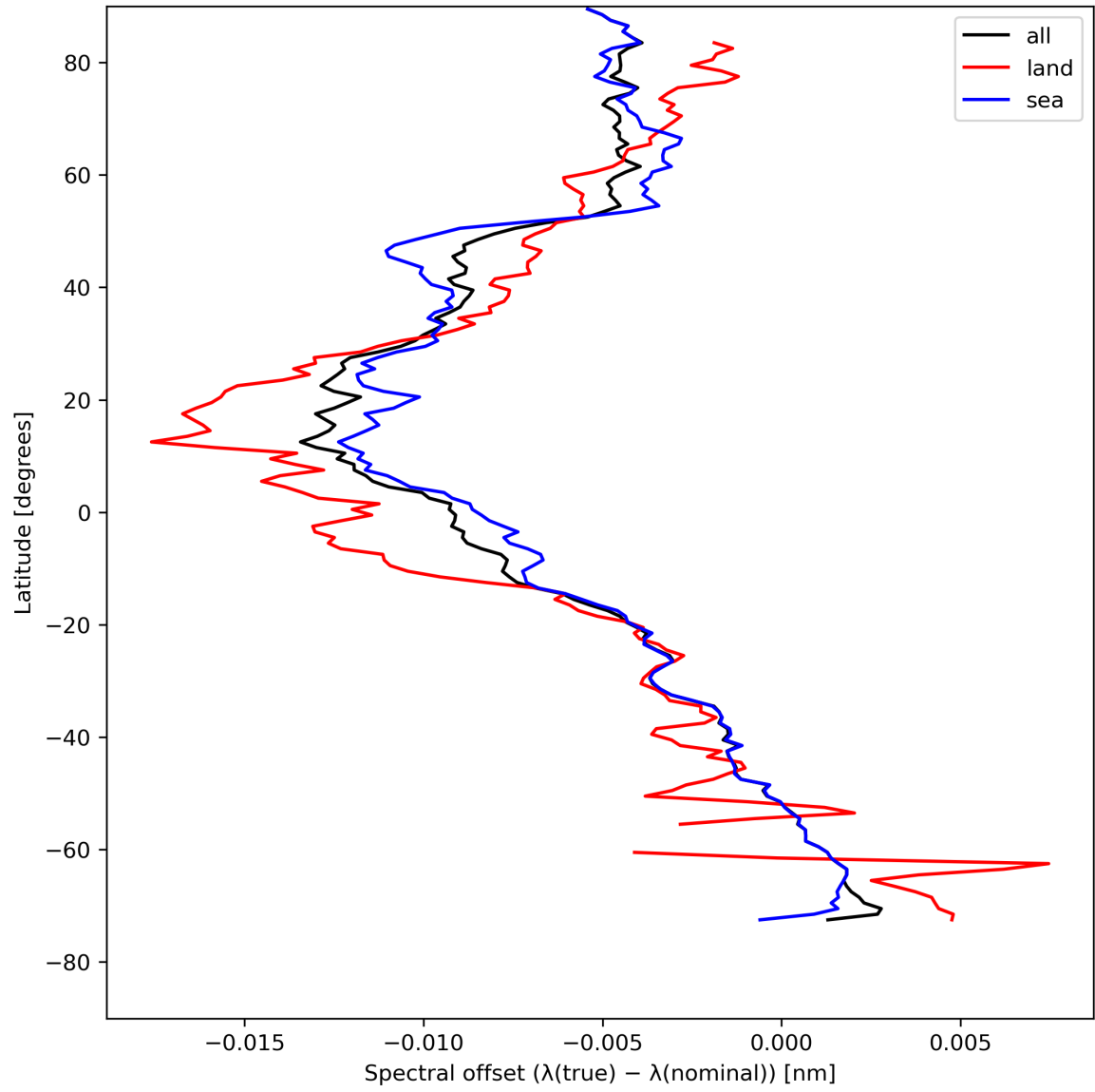
Figure 28: Zonal average of “Spectral offset ( \lambda(\text{true}) - \lambda(\text{nominal}) )” for 2024-08-08 to 2024-08-10.
