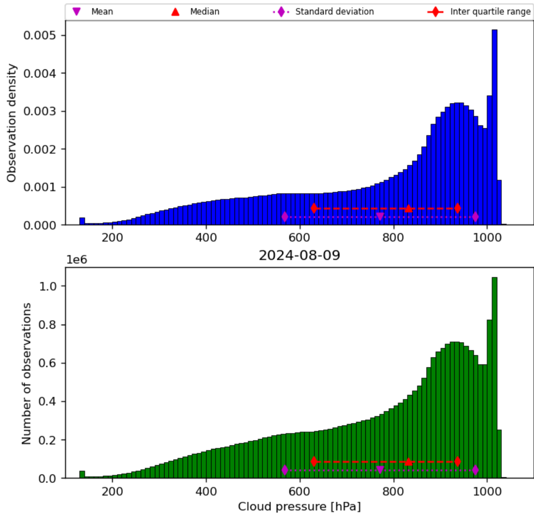
Figure 30: Histogram of “Cloud pressure” for 2024-08-08 to 2024-08-10
