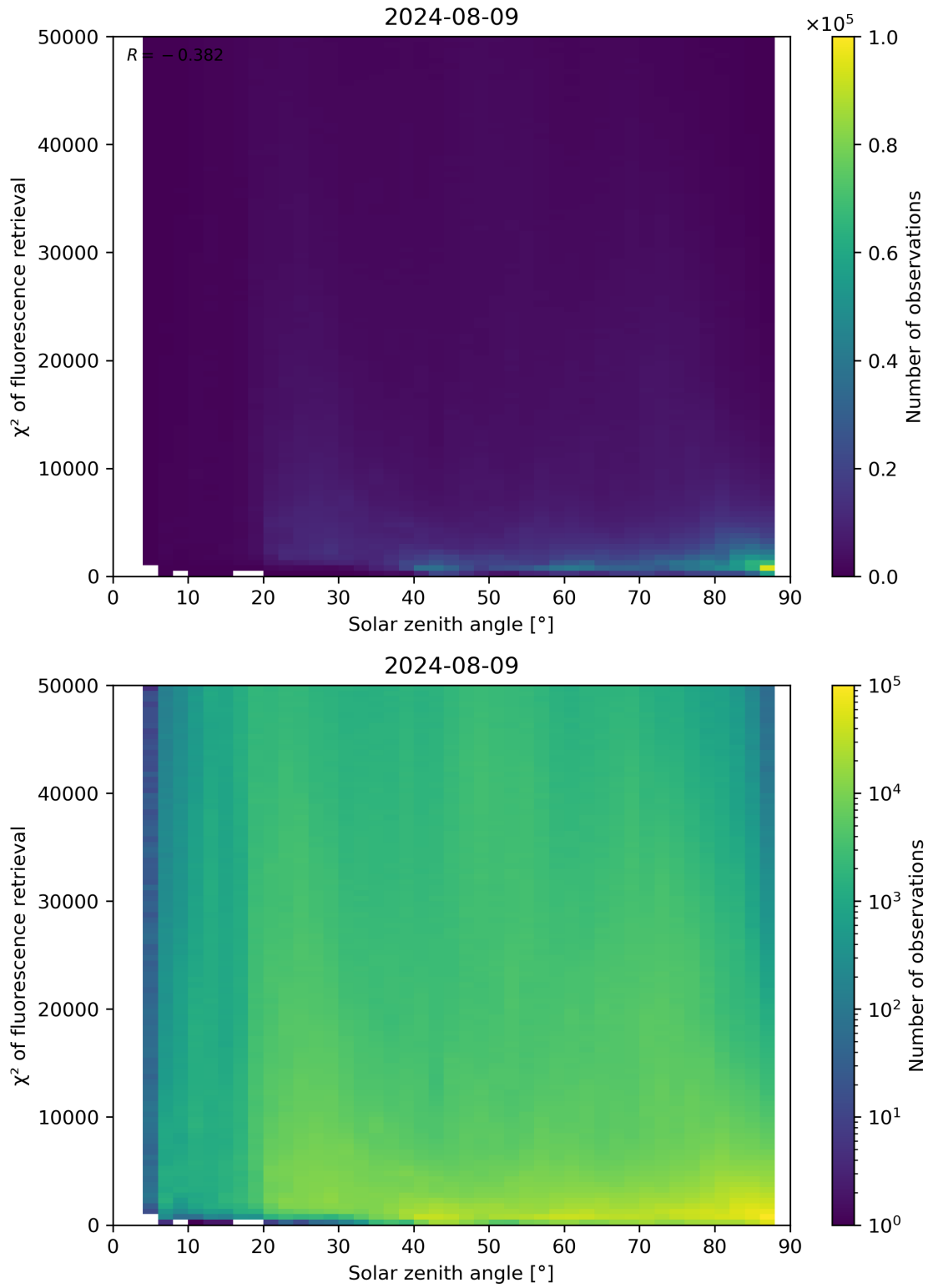
Figure 109: Scatter density plot of “Solar zenith angle” against “ \chi^2 of fluorescence retrieval” for 2024-08-08 to 2024-08-10.
