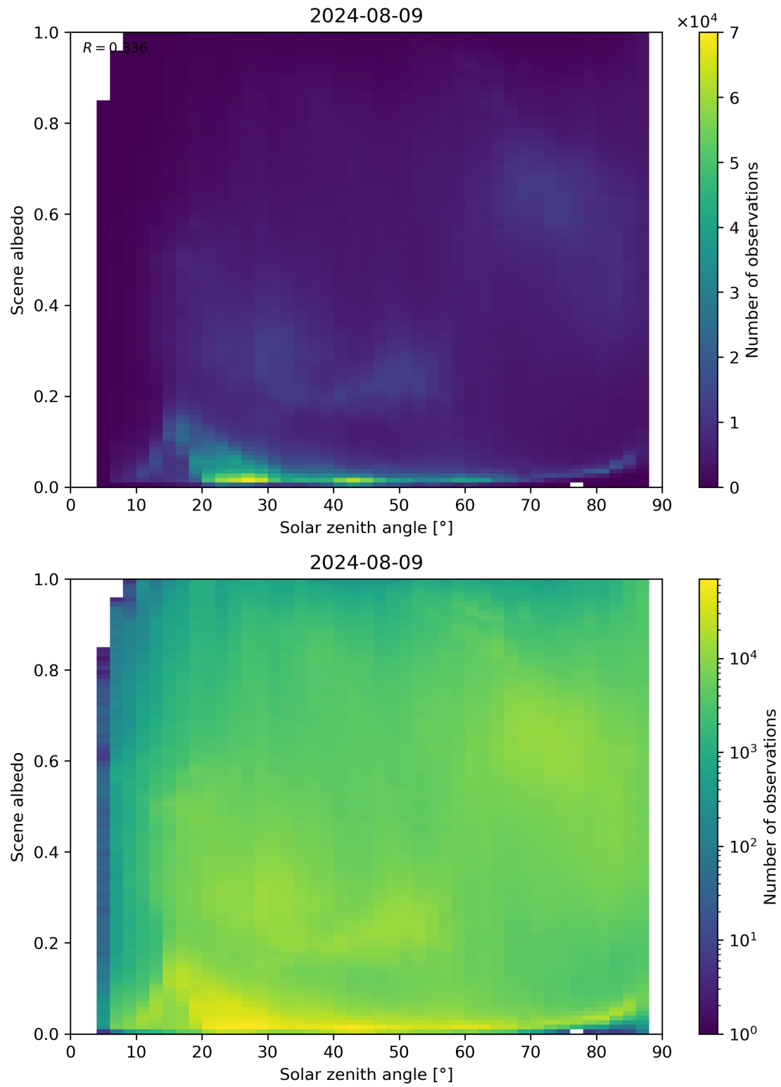
Figure 116: Scatter density plot of “Solar zenith angle” against “Scene albedo” for 2024-08-08 to 2024-08-10.
