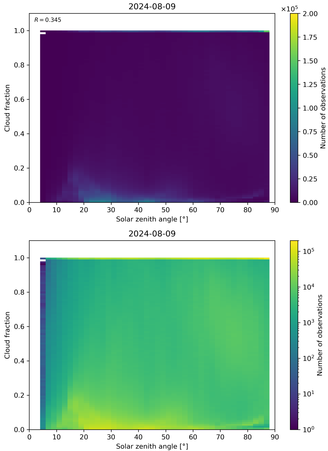
Figure 110: Scatter density plot of “Solar zenith angle” against “Cloud fraction” for 2024-08-08 to 2024-08-10.
