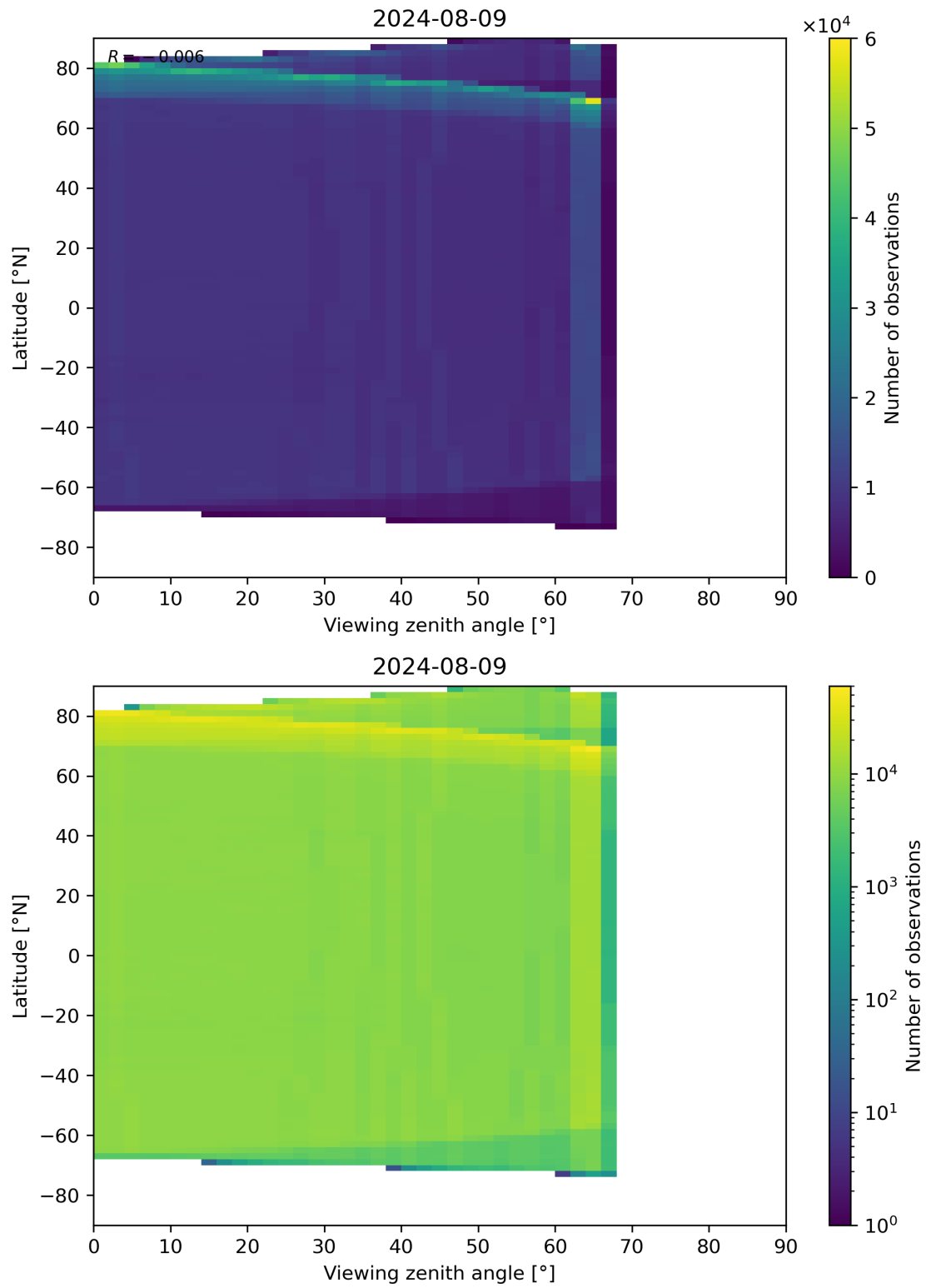
Figure 123: Scatter density plot of “Viewing zenith angle” against “Latitude” for 2024-08-08 to 2024-08-10.
