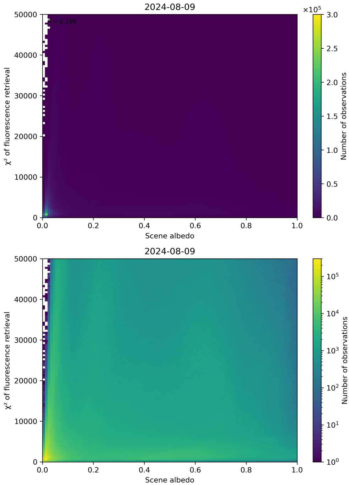
Figure 103: Scatter density plot of “Scene albedo” against “ \chi^2 of fluorescence retrieval” for 2024-08-08 to 2024-08-10.
