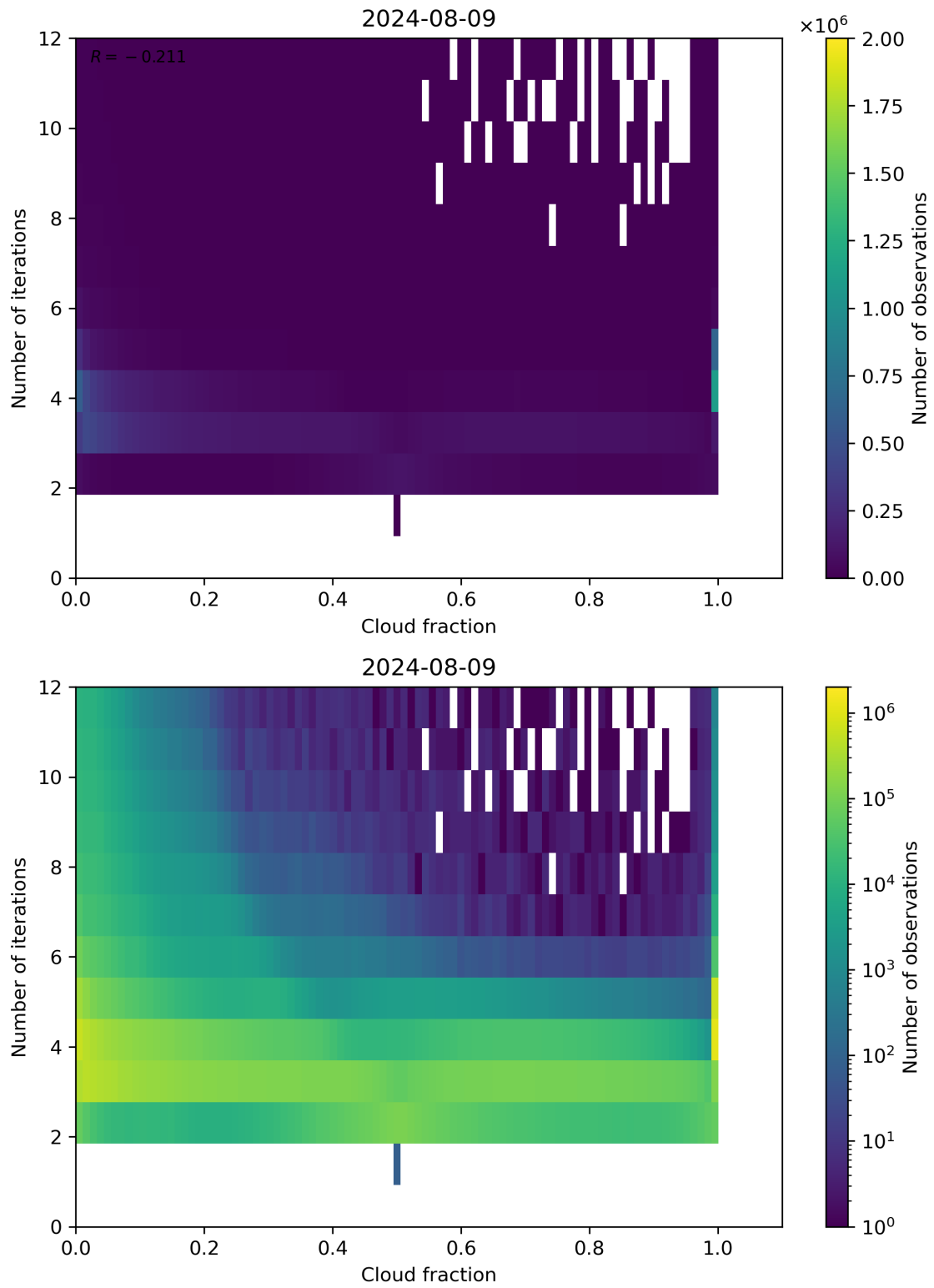
Figure 73: Scatter density plot of “Cloud fraction” against “Number of iterations” for 2024-08-08 to 2024-08-10.
