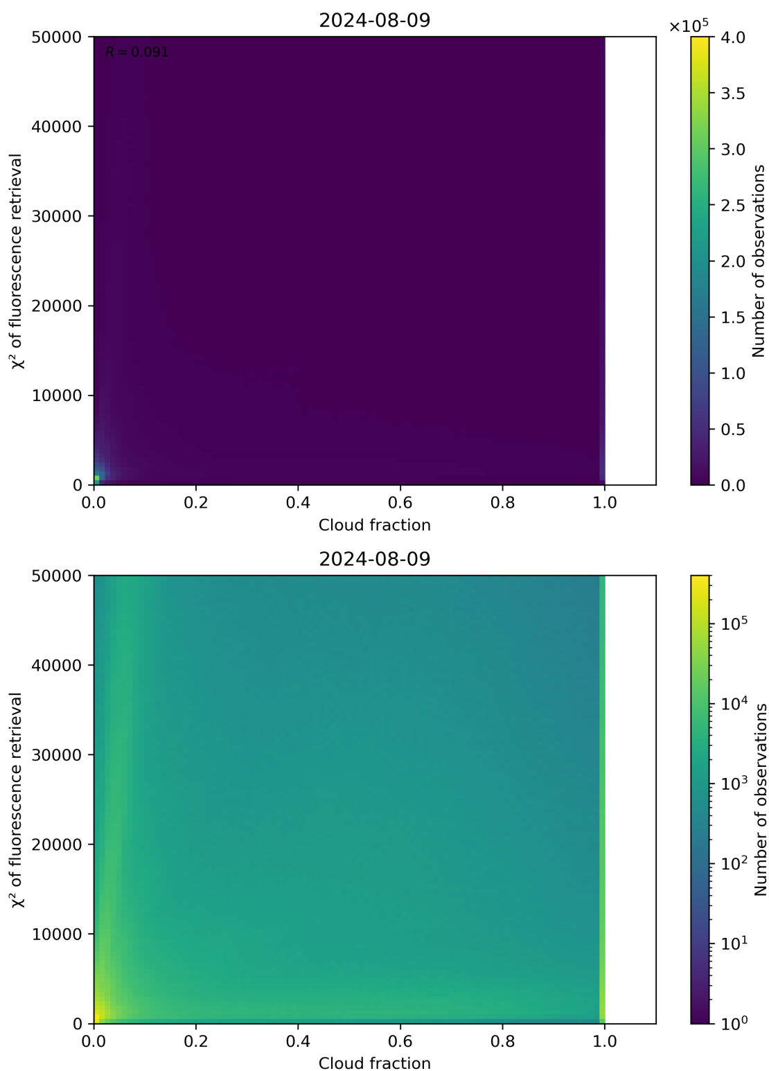
Figure 71: Scatter density plot of “Cloud fraction” against “ \chi^2 of fluorescence retrieval” for 2024-08-08 to 2024-08-10.
