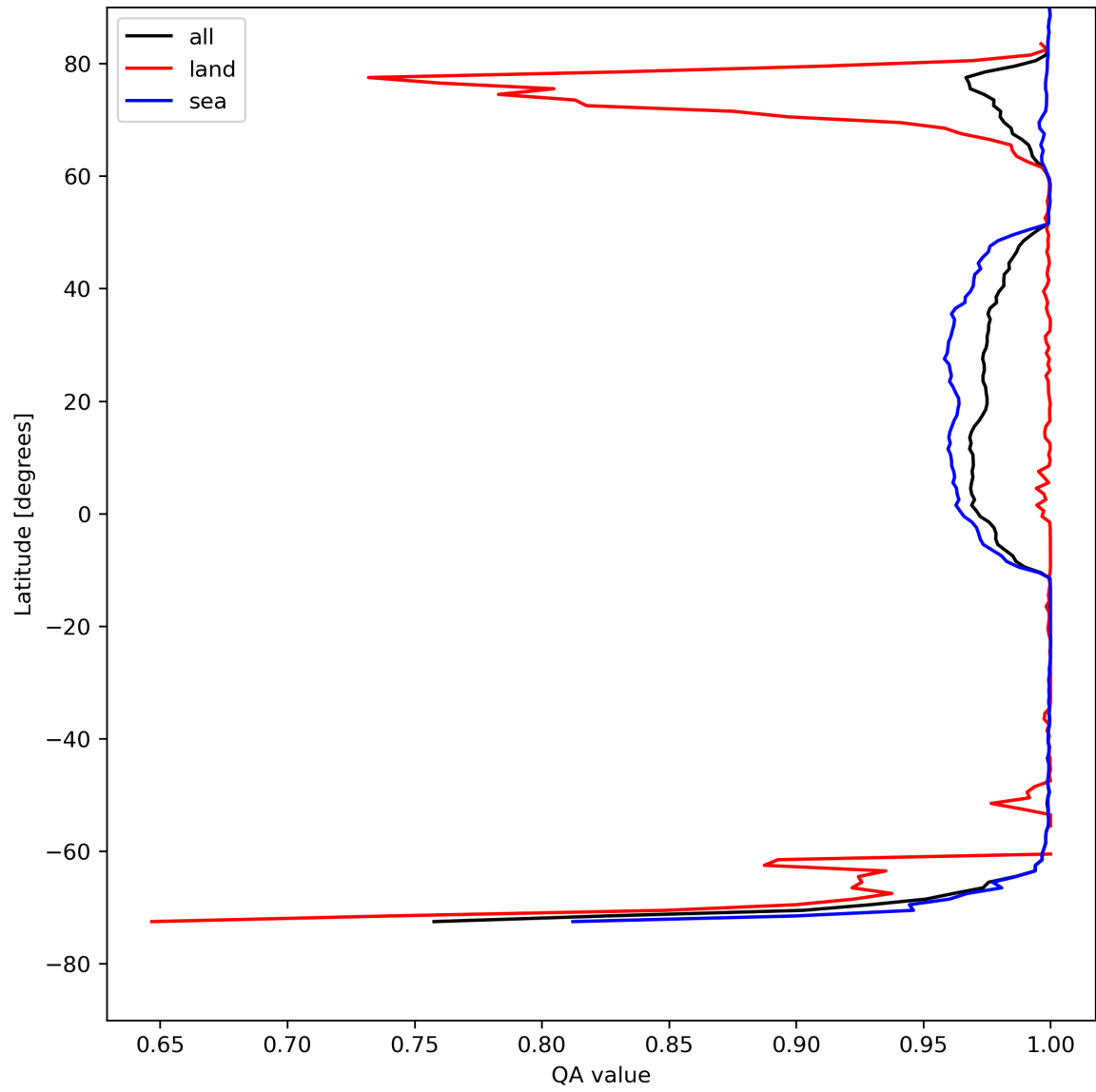
Figure 12: Zonal average of “QA value” for 2024-08-08 to 2024-08-10.
