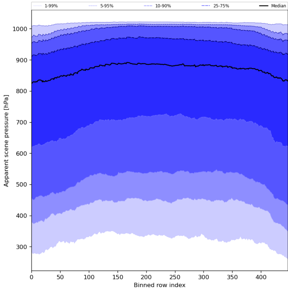
Figure 53: Along track statistics of “Apparent scene pressure” for 2024-08-08 to 2024-08-10
