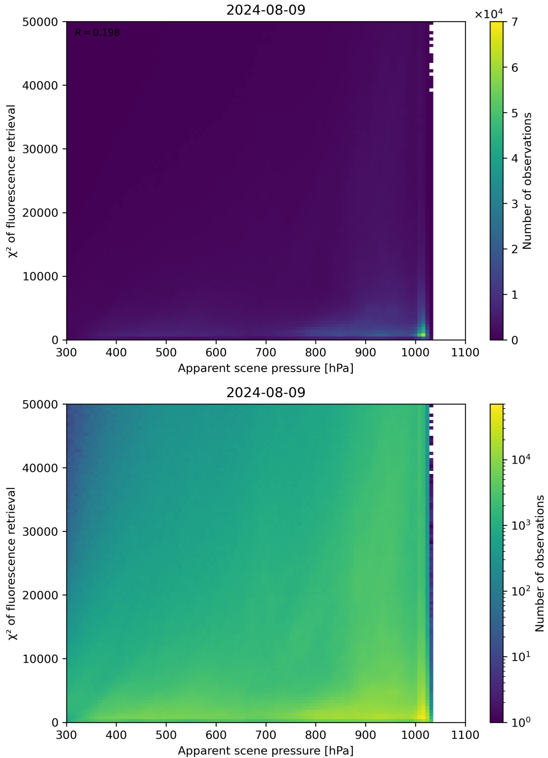
Figure 63: Scatter density plot of “Apparent scene pressure” against “ \chi^2 of fluorescence retrieval” for 2024-08-08 to 2024-08-10.
