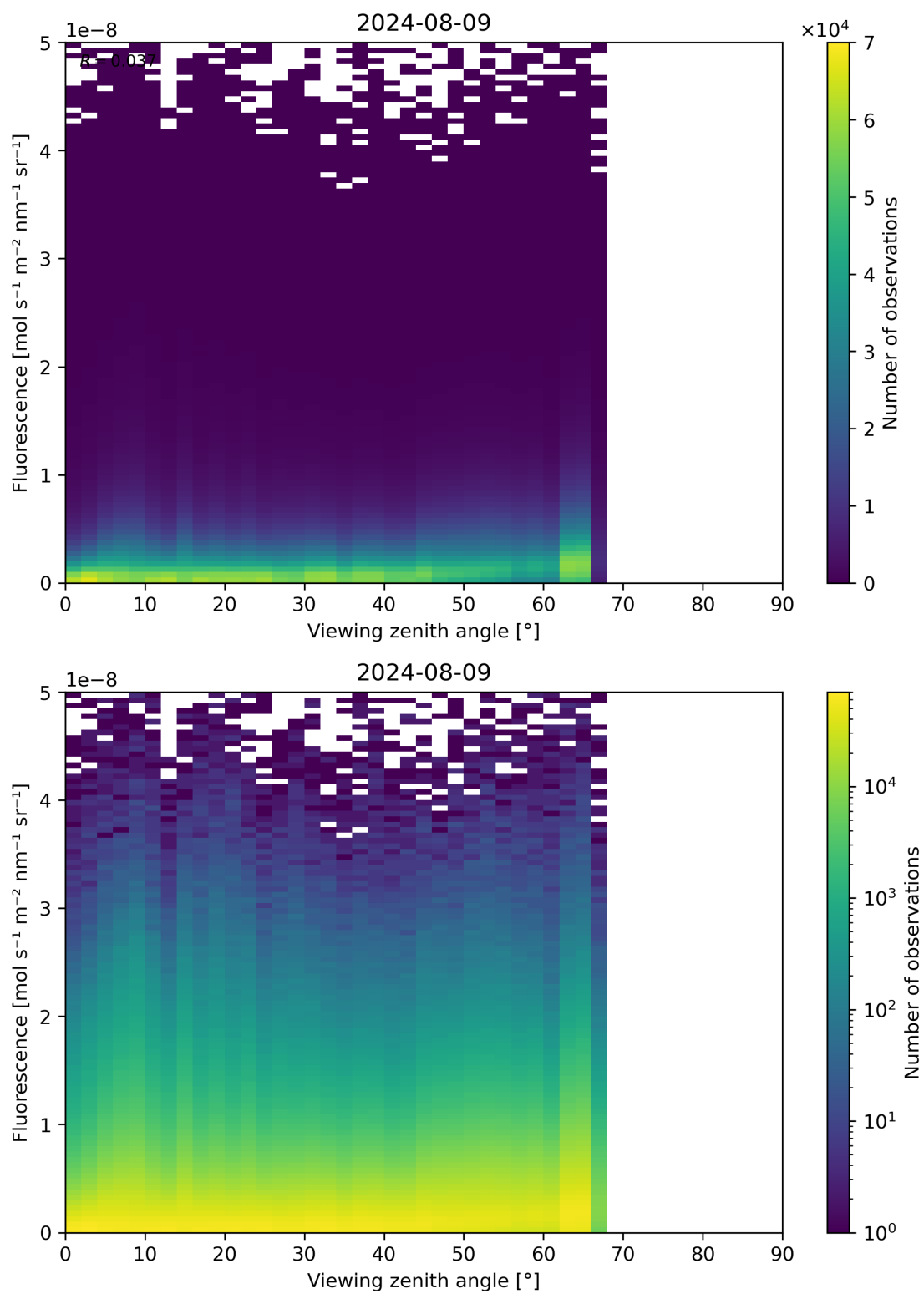
Figure 122: Scatter density plot of “Viewing zenith angle” against “Fluorescence” for 2024-08-08 to 2024-08-10.
