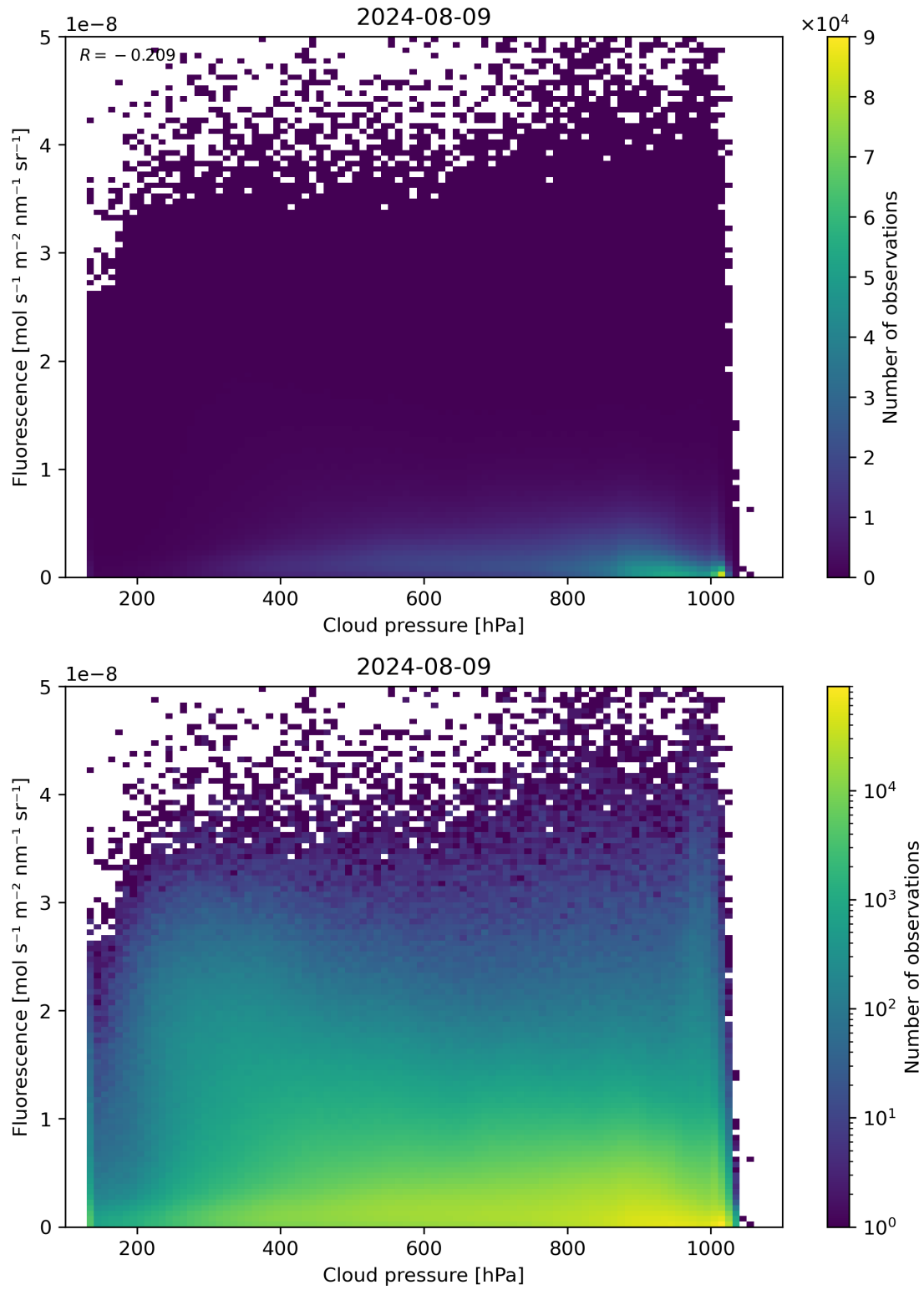
Figure 80: Scatter density plot of “Cloud pressure” against “Fluorescence” for 2024-08-08 to 2024-08-10.
