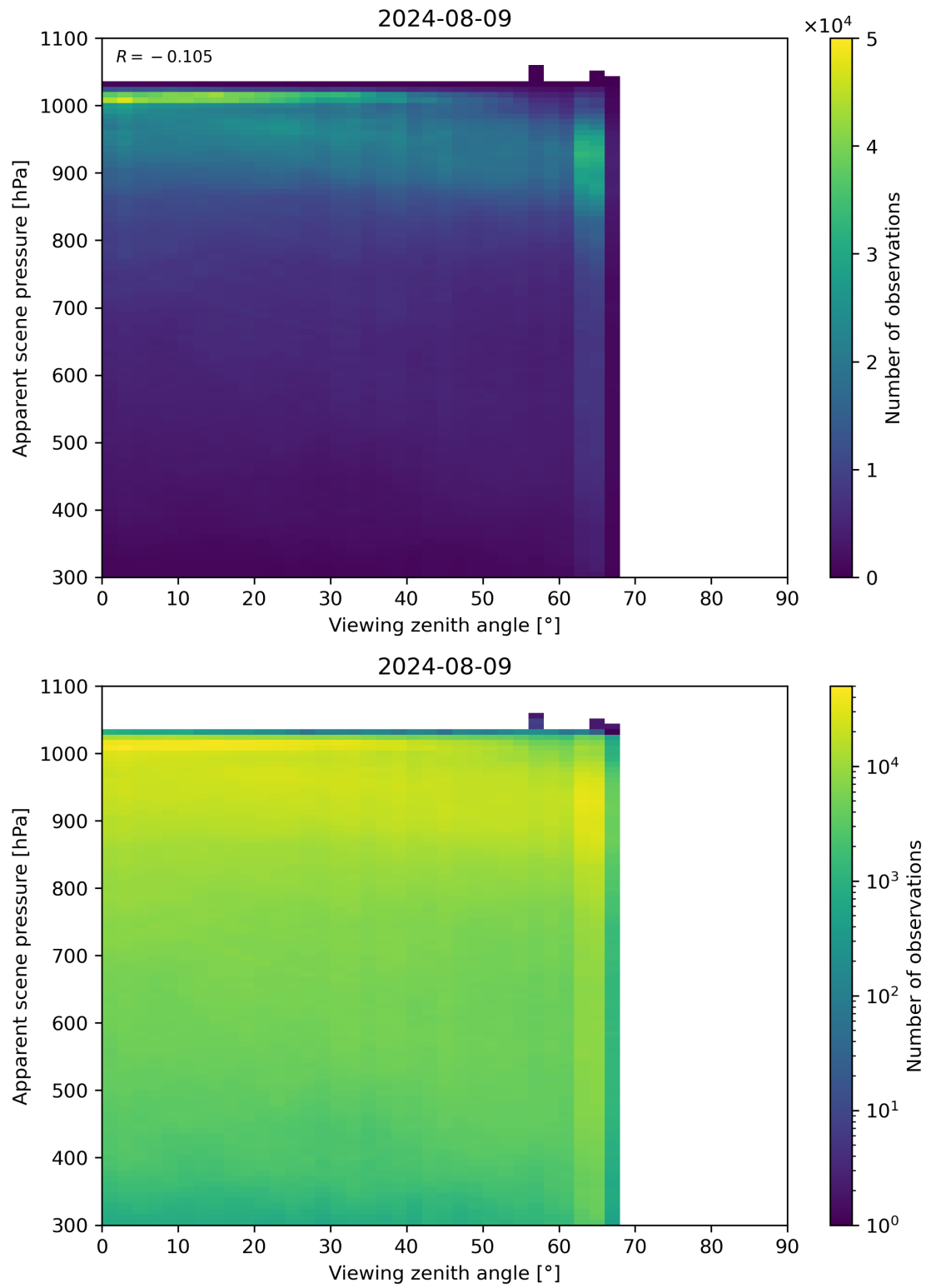
Figure 118: Scatter density plot of “Viewing zenith angle” against “Apparent scene pressure” for 2024-08-08 to 2024-08-10.
