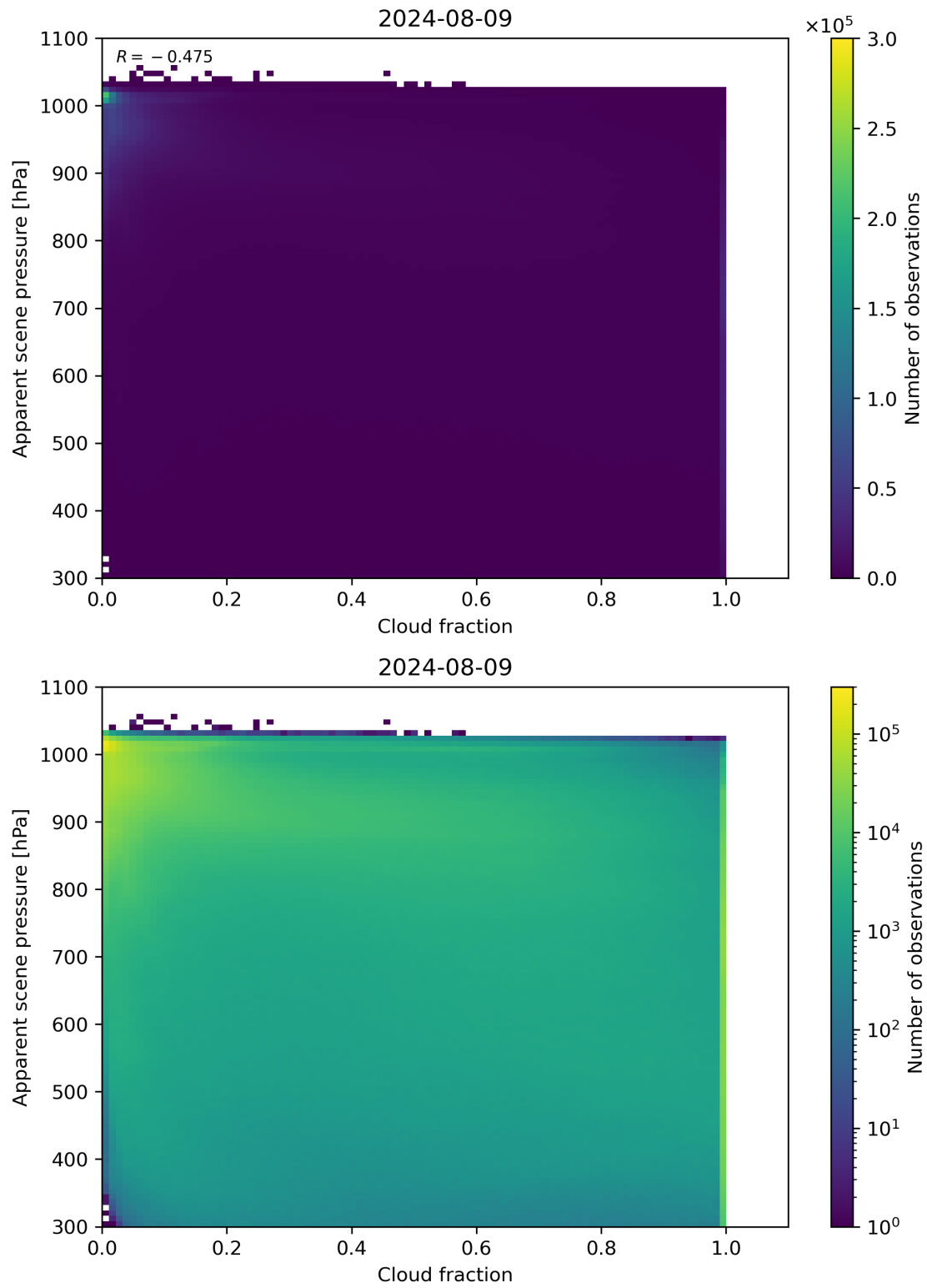
Figure 70: Scatter density plot of “Cloud fraction” against “Apparent scene pressure” for 2024-08-08 to 2024-08-10.
