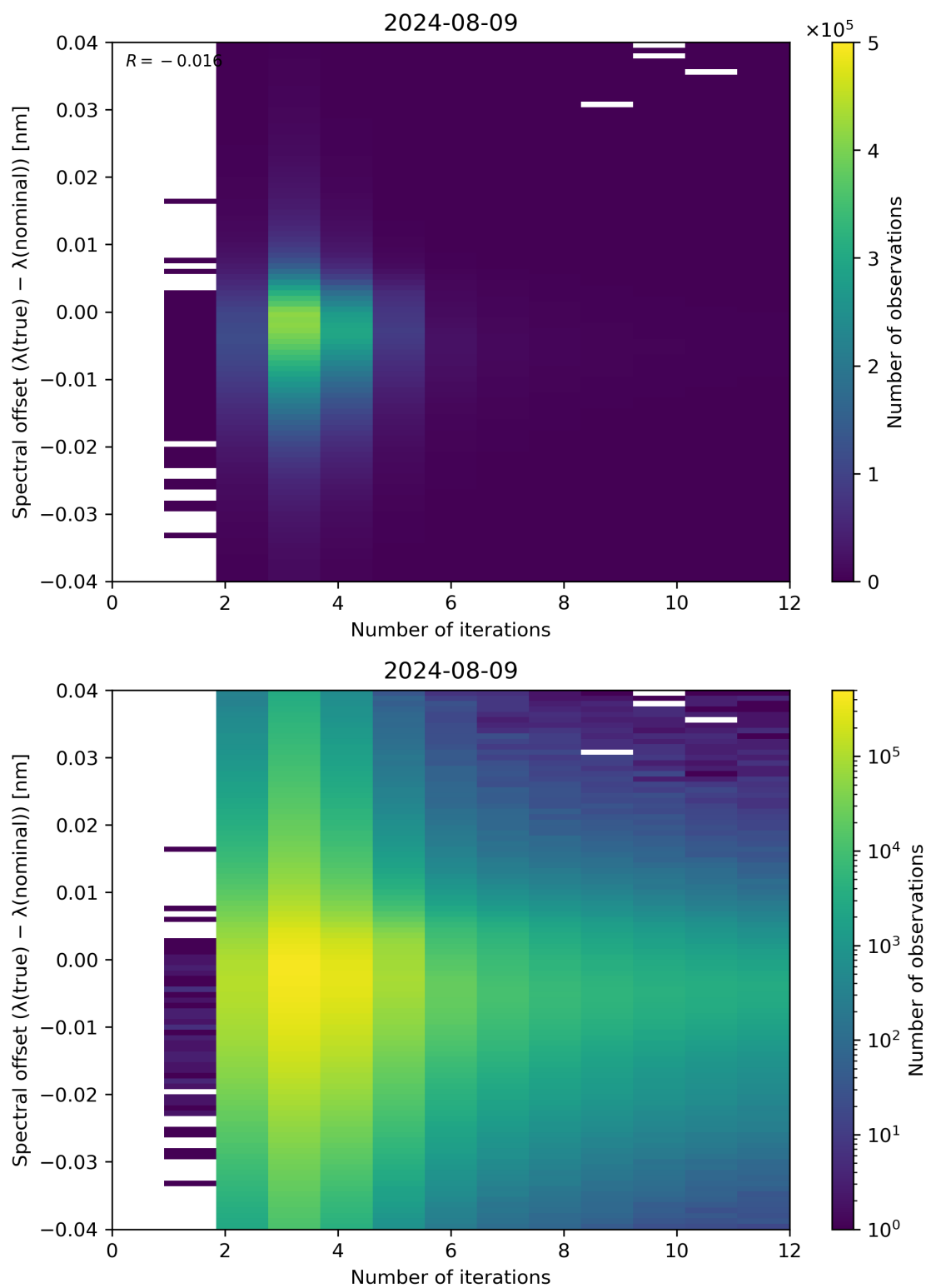
Figure 100: Scatter density plot of “Number of iterations” against “Spectral offset ( \lambda(\text{true}) - \lambda(\text{nominal}) )” for 2024-08-08 to 2024-08-10.
