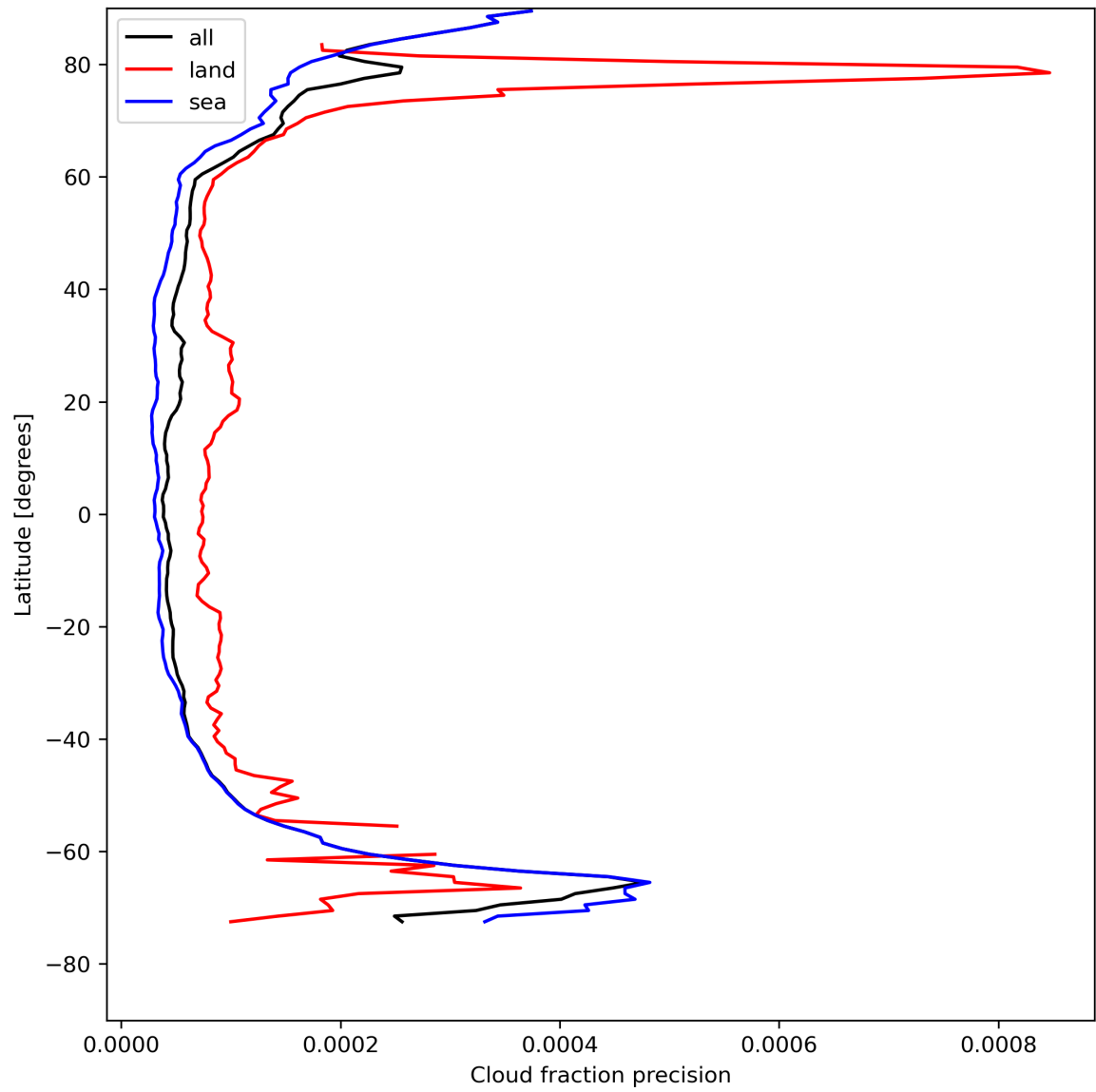
Figure 16: Zonal average of “Cloud fraction precision” for 2024-08-08 to 2024-08-10.
