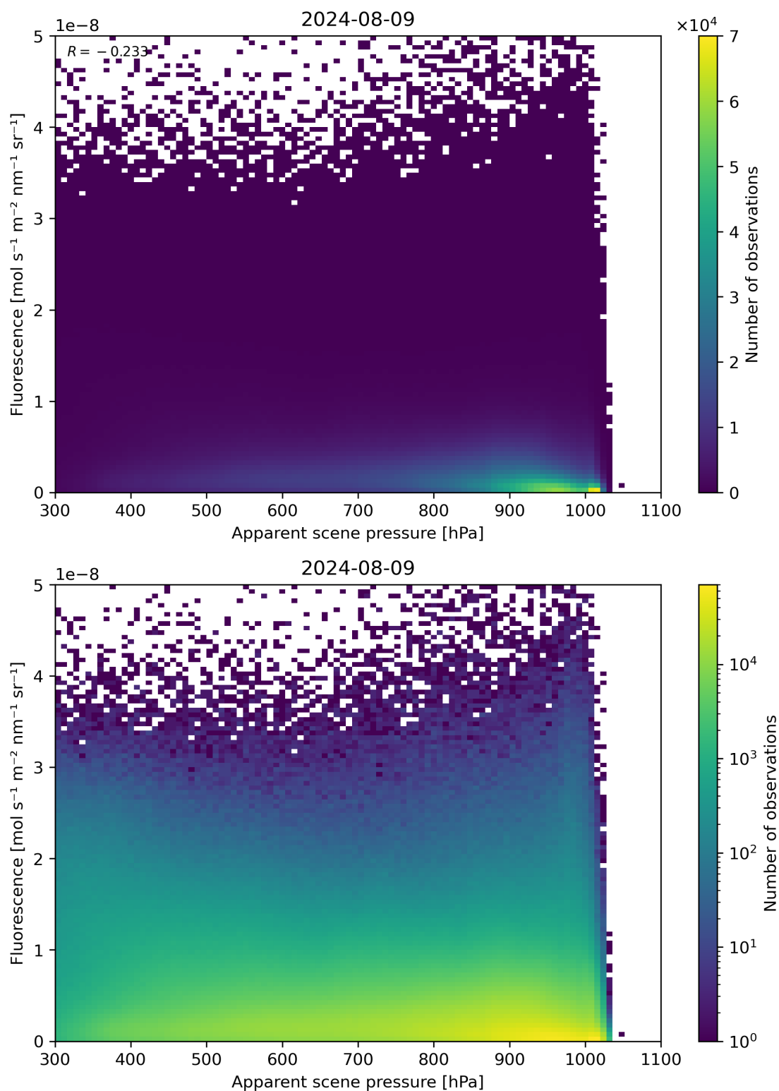
Figure 64: Scatter density plot of “Apparent scene pressure” against “Fluorescence” for 2024-08-08 to 2024-08-10.
