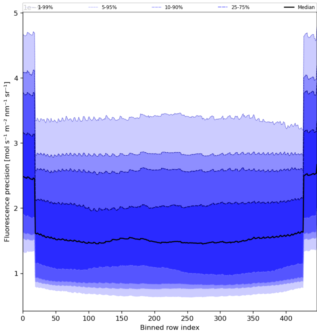
Figure 58: Along track statistics of “Fluorescence precision” for 2024-08-08 to 2024-08-10
