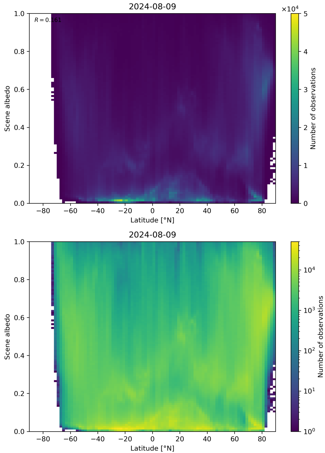
Figure 95: Scatter density plot of “Latitude” against “Scene albedo” for 2024-08-08 to 2024-08-10.
