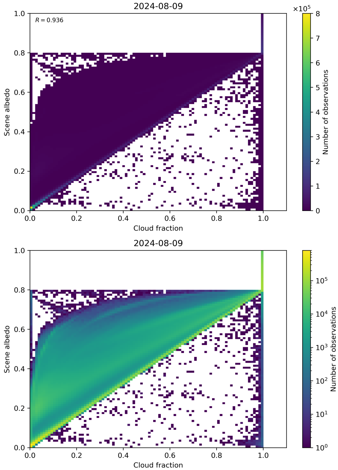
Figure 75: Scatter density plot of “Cloud fraction” against “Scene albedo” for 2024-08-08 to 2024-08-10.
