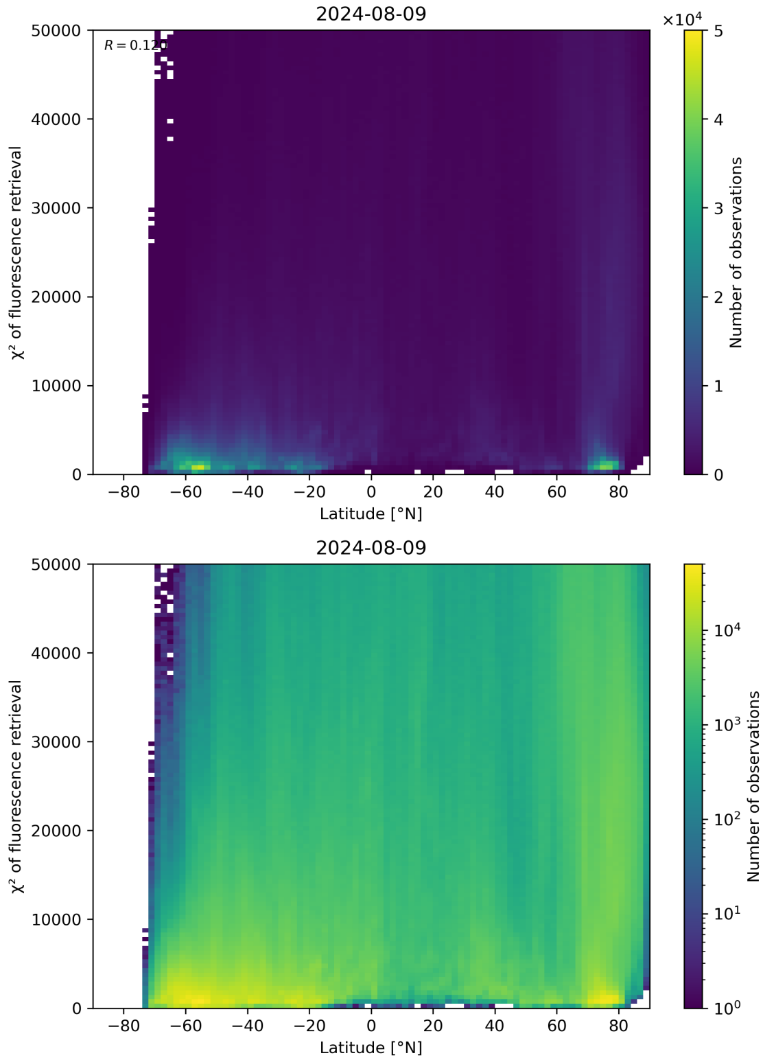
Figure 89: Scatter density plot of “Latitude” against “ \chi^2 of fluorescence retrieval” for 2024-08-08 to 2024-08-10.
