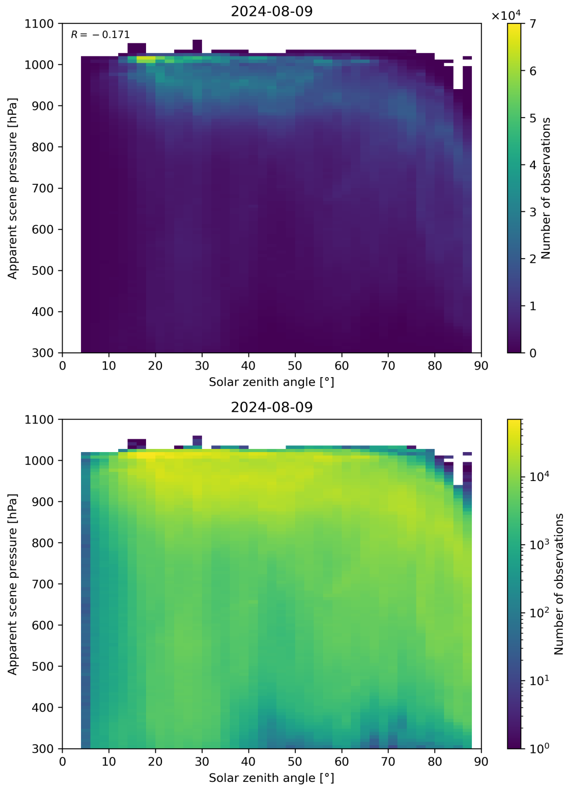
Figure 108: Scatter density plot of “Solar zenith angle” against “Apparent scene pressure” for 2024-08-08 to 2024-08-10.
