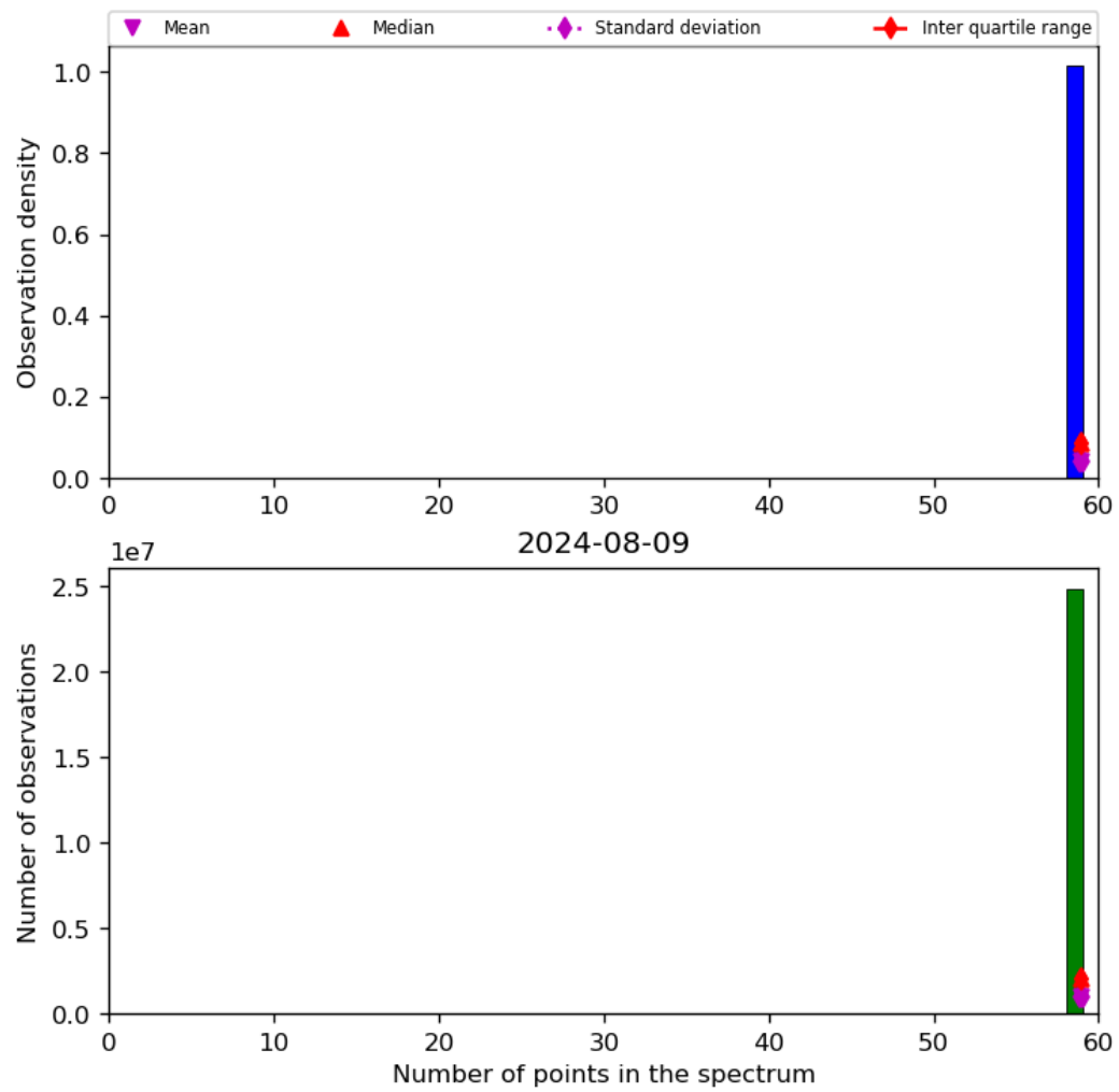
Figure 44: Histogram of “Number of points in the spectrum” for 2024-08-08 to 2024-08-10
