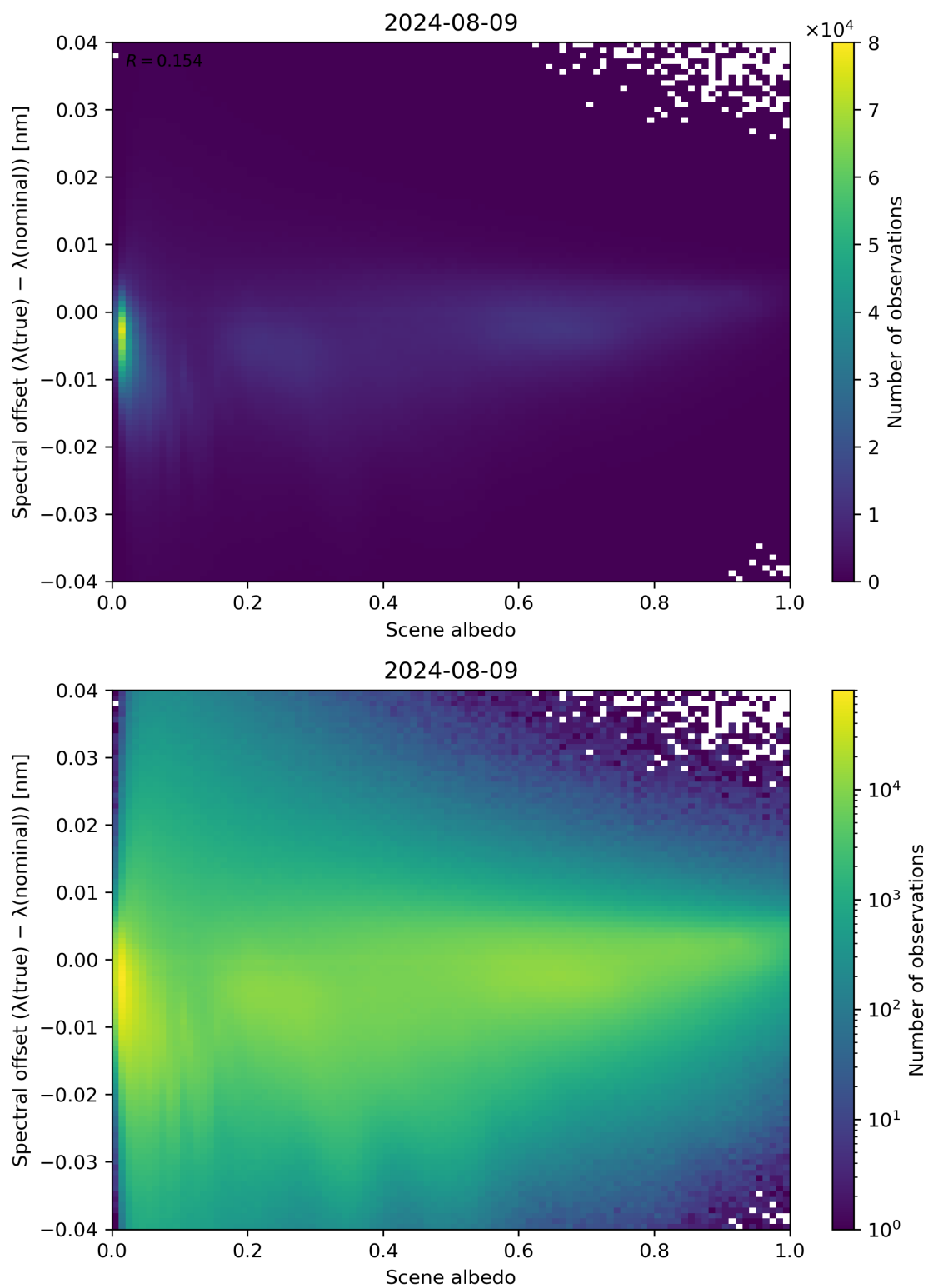
Figure 107: Scatter density plot of “Scene albedo” against “Spectral offset ( \lambda(\text{true}) - \lambda(\text{nominal}) )” for 2024-08-08 to 2024-08-10.
