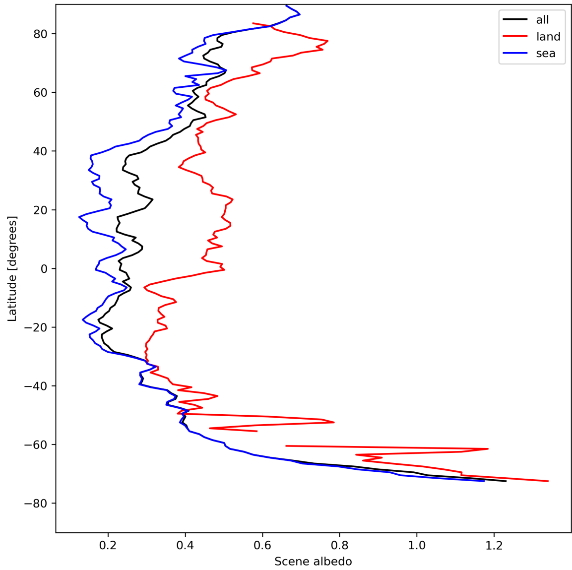
Figure 17: Zonal average of “Scene albedo” for 2024-08-08 to 2024-08-10.
