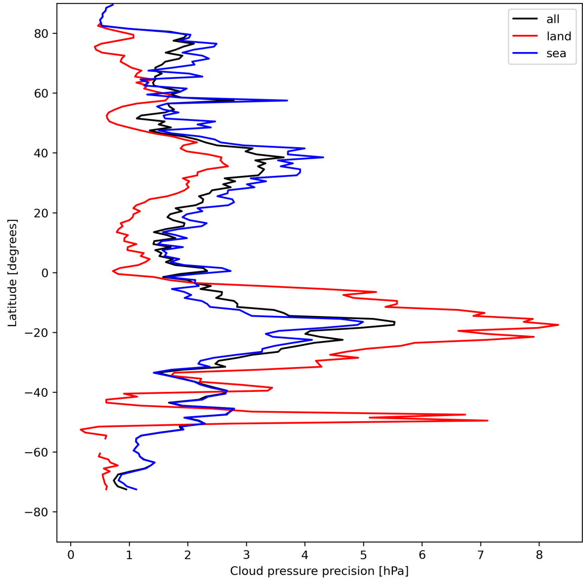
Figure 14: Zonal average of “Cloud pressure precision” for 2024-08-08 to 2024-08-10.
