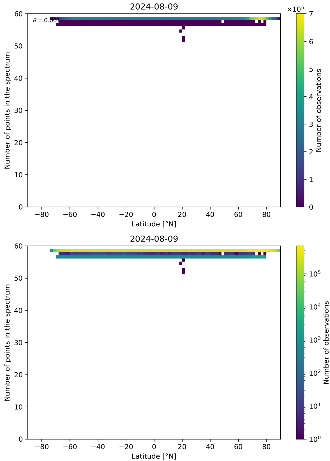
Figure 94: Scatter density plot of “Latitude” against “Number of points in the spectrum” for 2024-08-08 to 2024-08-10.
