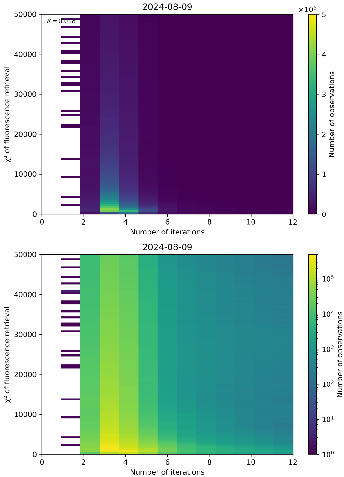
Figure 97: Scatter density plot of “Number of iterations” against “ \chi^2 of fluorescence retrieval” for 2024-08-08 to 2024-08-10.
