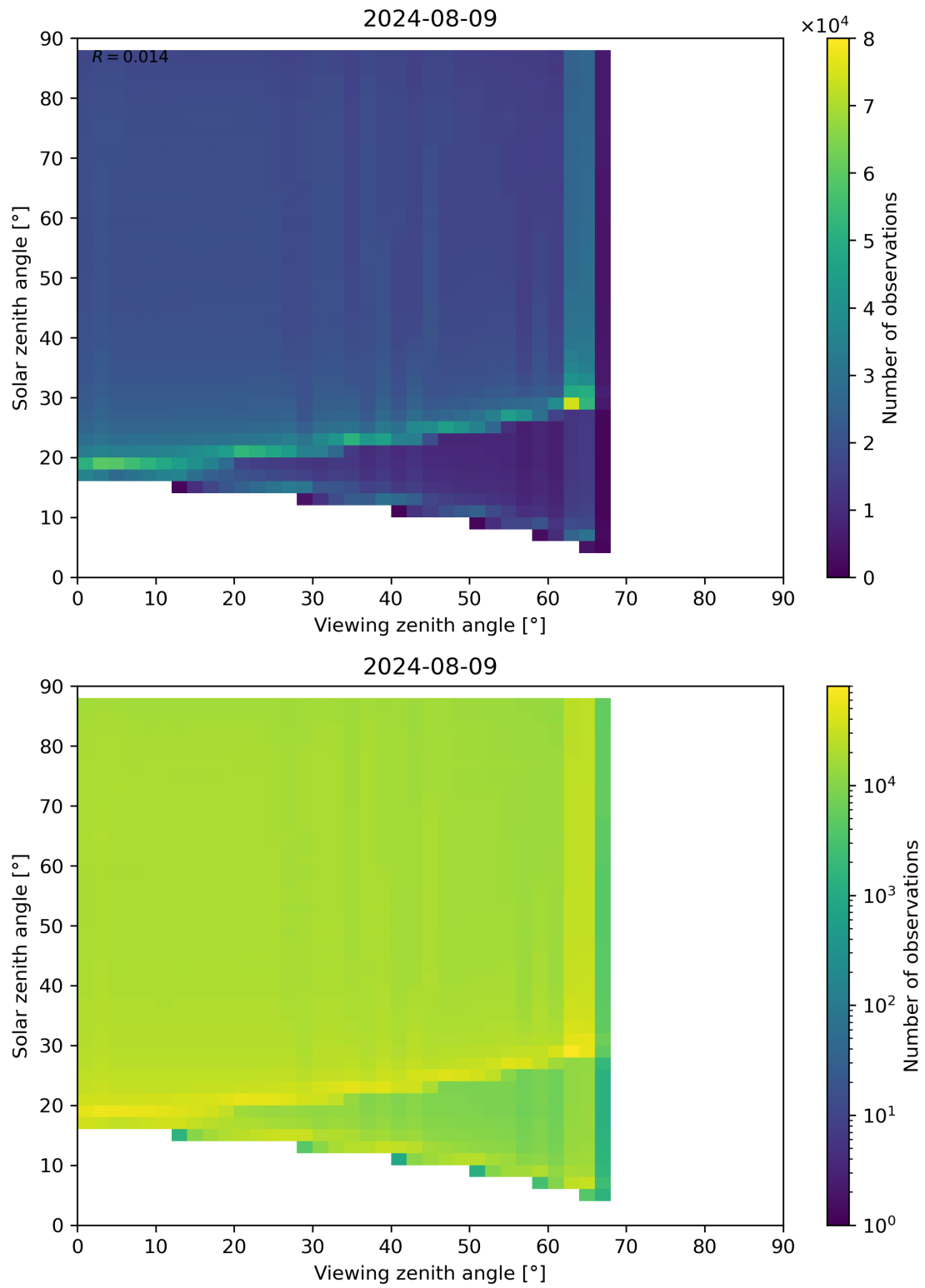
Figure 127: Scatter density plot of “Viewing zenith angle” against “Solar zenith angle” for 2024-08-08 to 2024-08-10.
