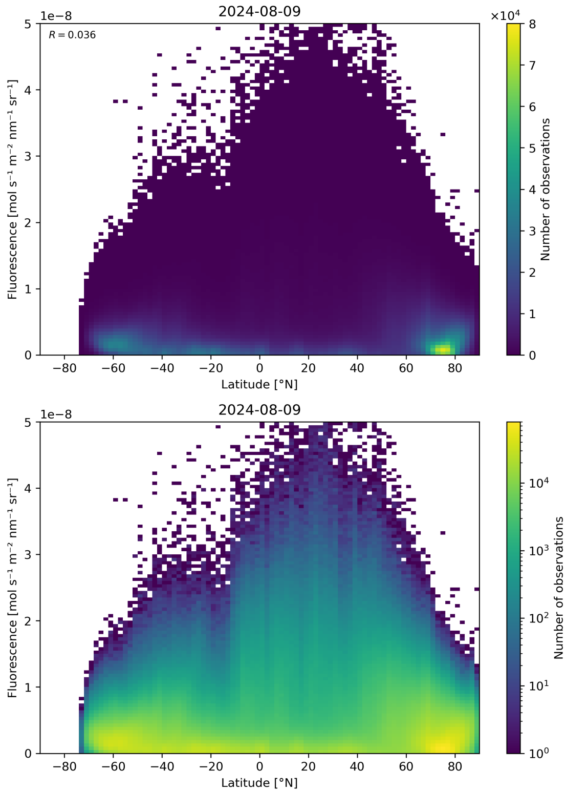
Figure 92: Scatter density plot of “Latitude” against “Fluorescence” for 2024-08-08 to 2024-08-10.
