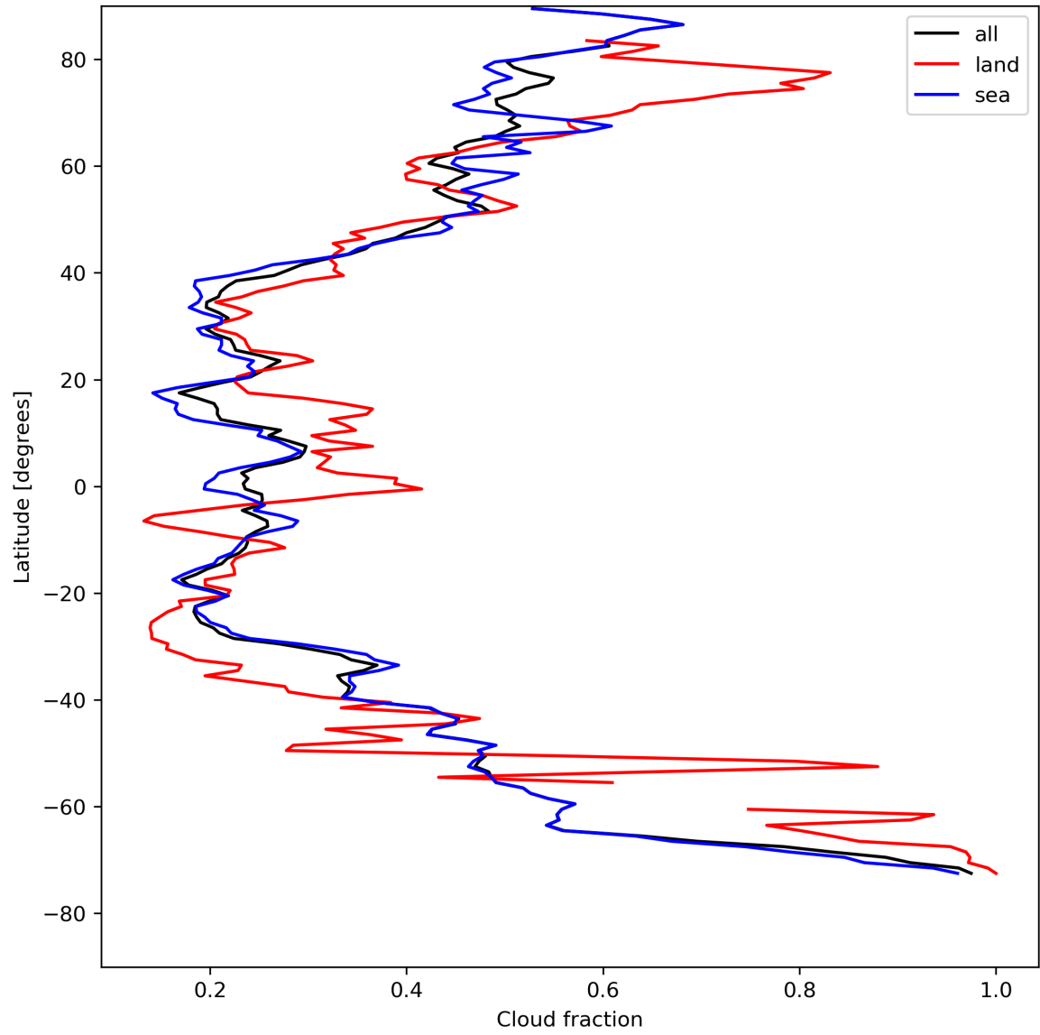
Figure 15: Zonal average of “Cloud fraction” for 2024-08-08 to 2024-08-10.
