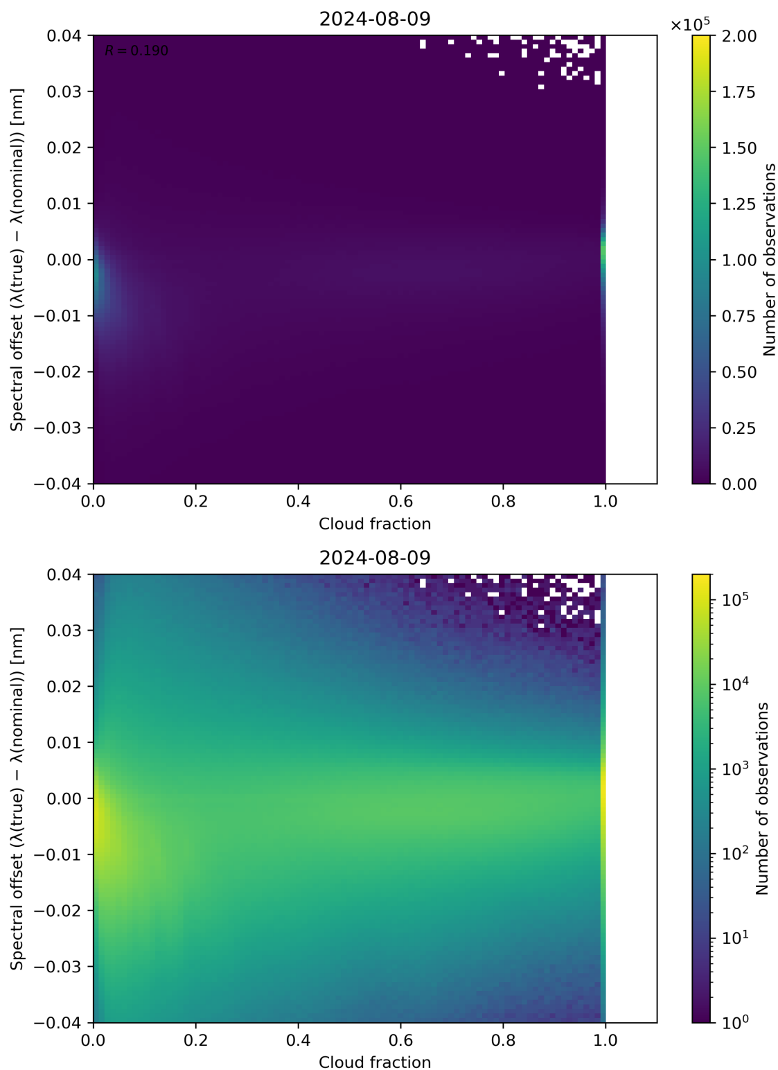
Figure 76: Scatter density plot of “Cloud fraction” against “Spectral offset ( \lambda(\text{true}) - \lambda(\text{nominal}) )” for 2024-08-08 to 2024-08-10.
