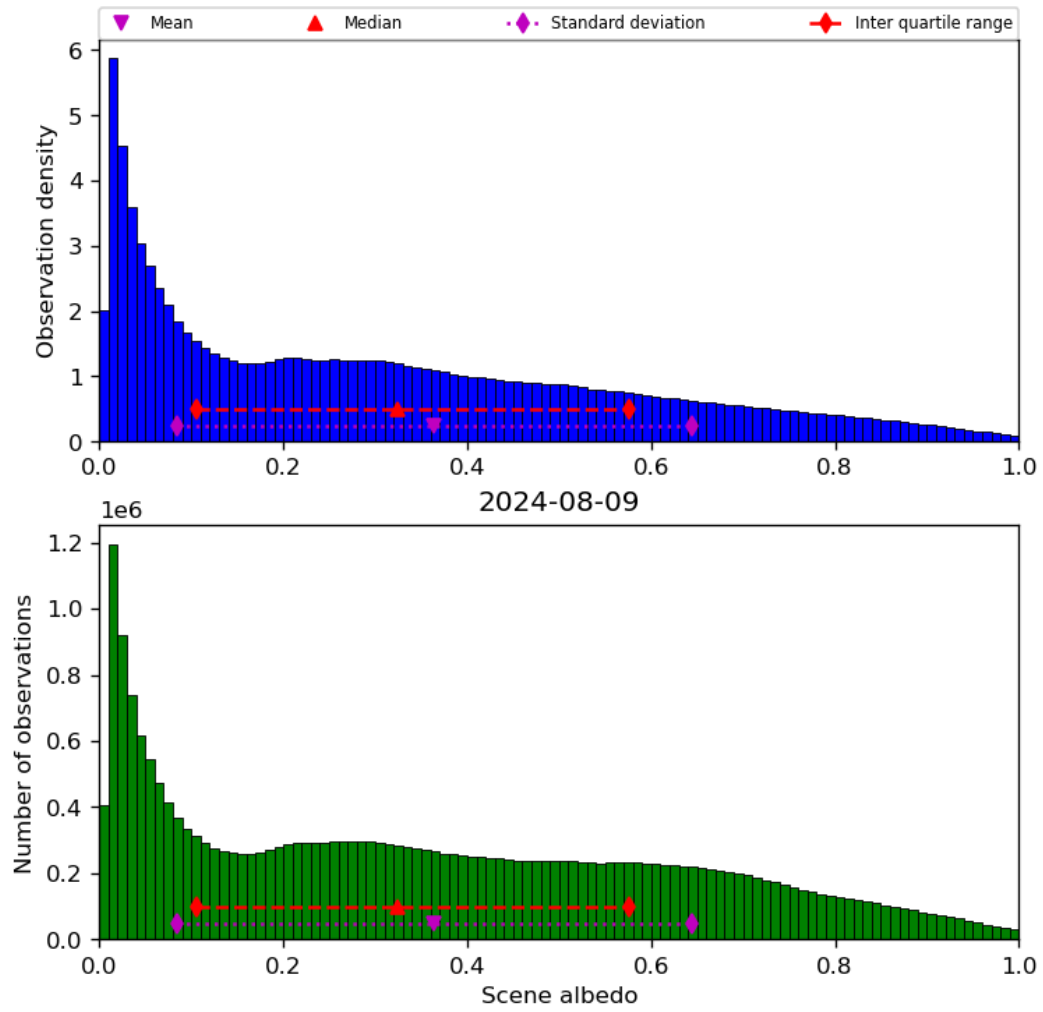
Figure 34: Histogram of “Scene albedo” for 2024-08-08 to 2024-08-10
