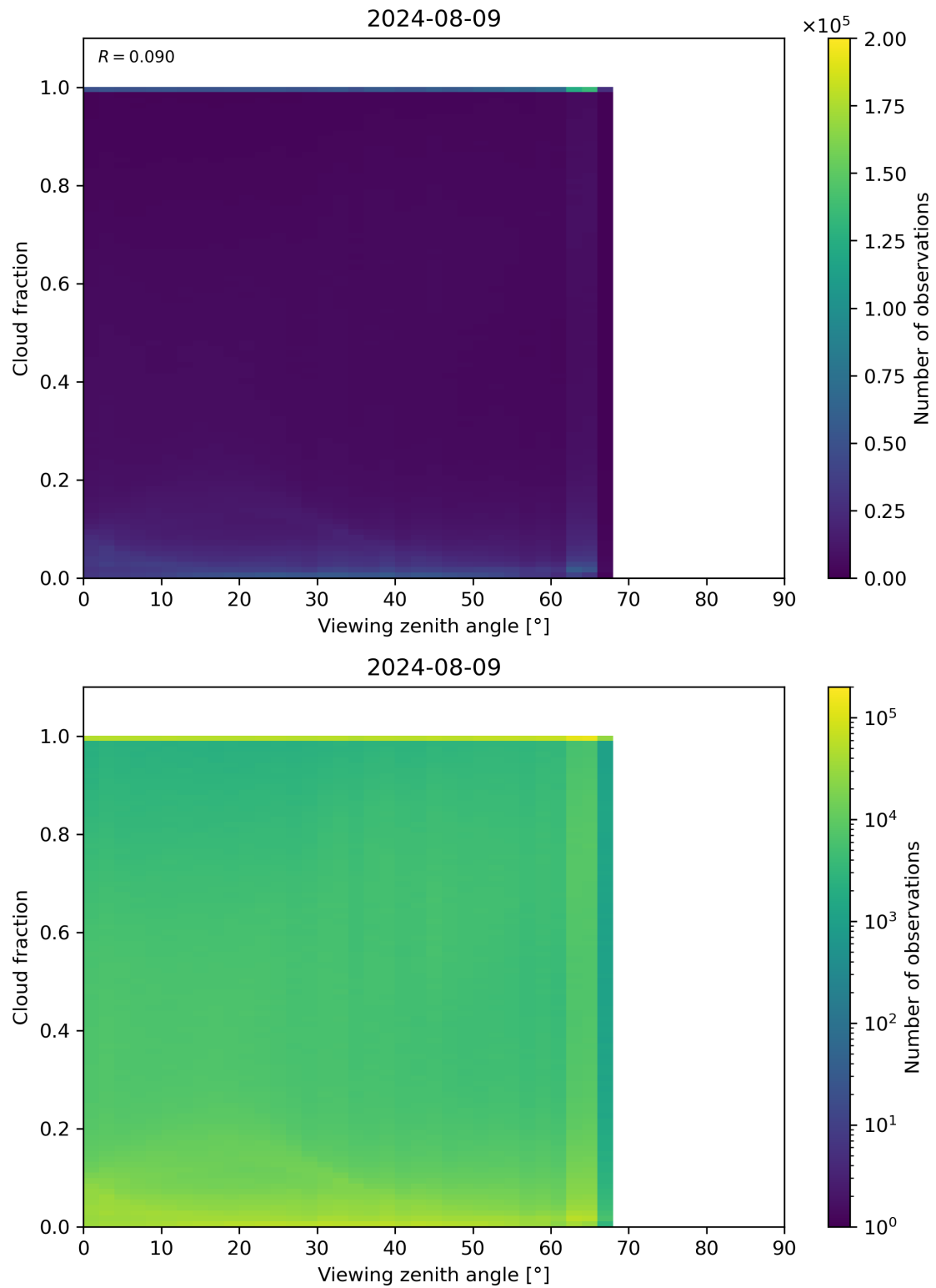
Figure 120: Scatter density plot of “Viewing zenith angle” against “Cloud fraction” for 2024-08-08 to 2024-08-10.
