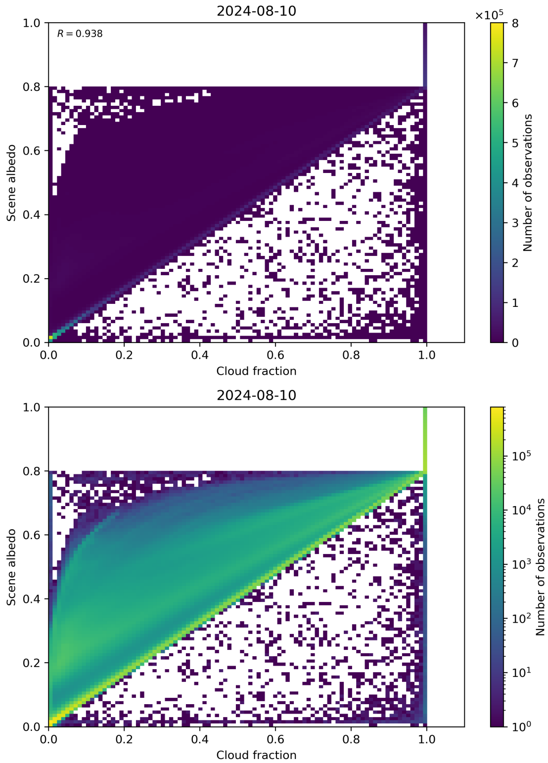
Figure 75: Scatter density plot of “Cloud fraction” against “Scene albedo” for 2024-08-09 to 2024-08-11.
