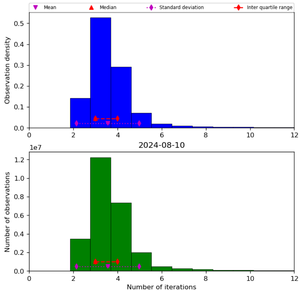
Figure 39: Histogram of “Number of iterations” for 2024-08-09 to 2024-08-11
