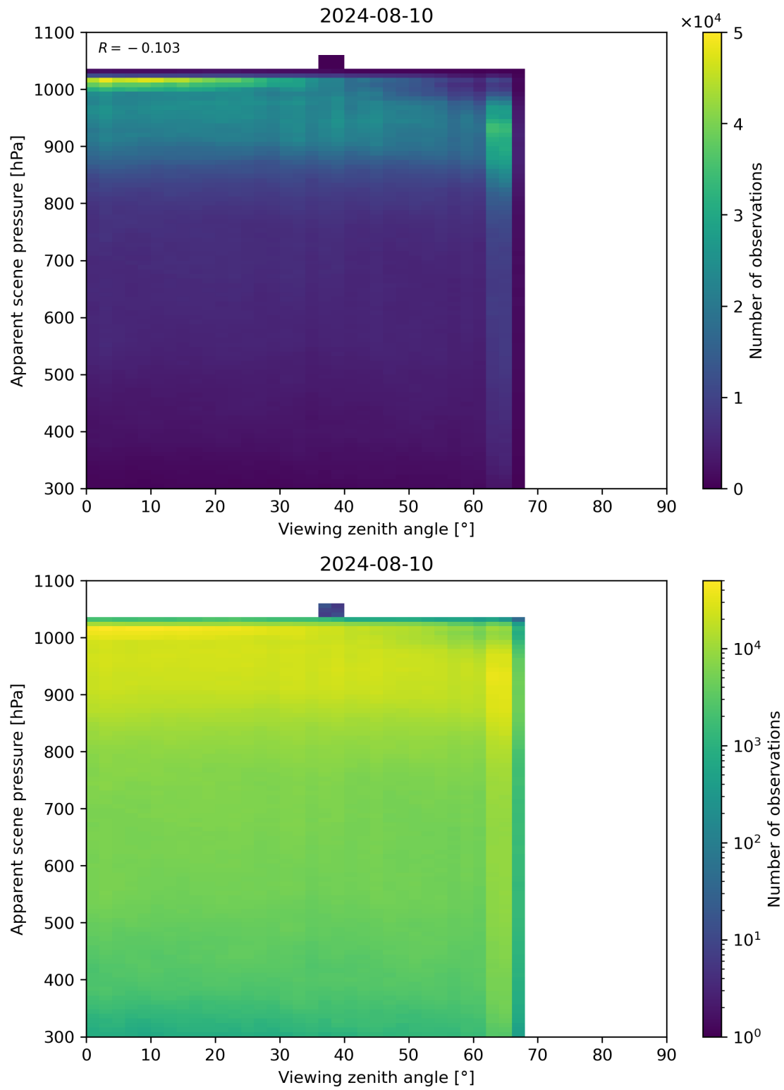
Figure 118: Scatter density plot of “Viewing zenith angle” against “Apparent scene pressure” for 2024-08-09 to 2024-08-11.
