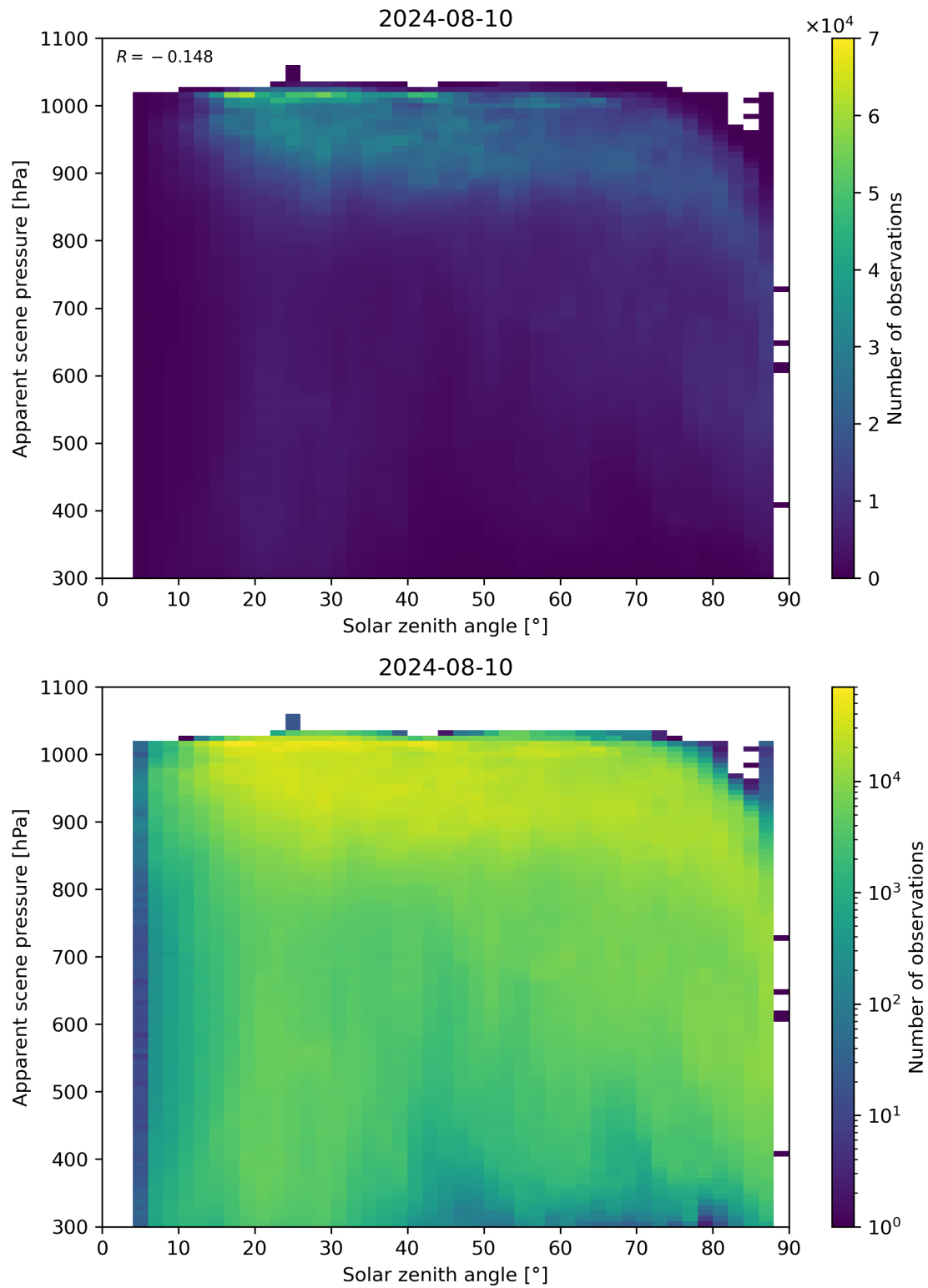
Figure 108: Scatter density plot of “Solar zenith angle” against “Apparent scene pressure” for 2024-08-09 to 2024-08-11.
