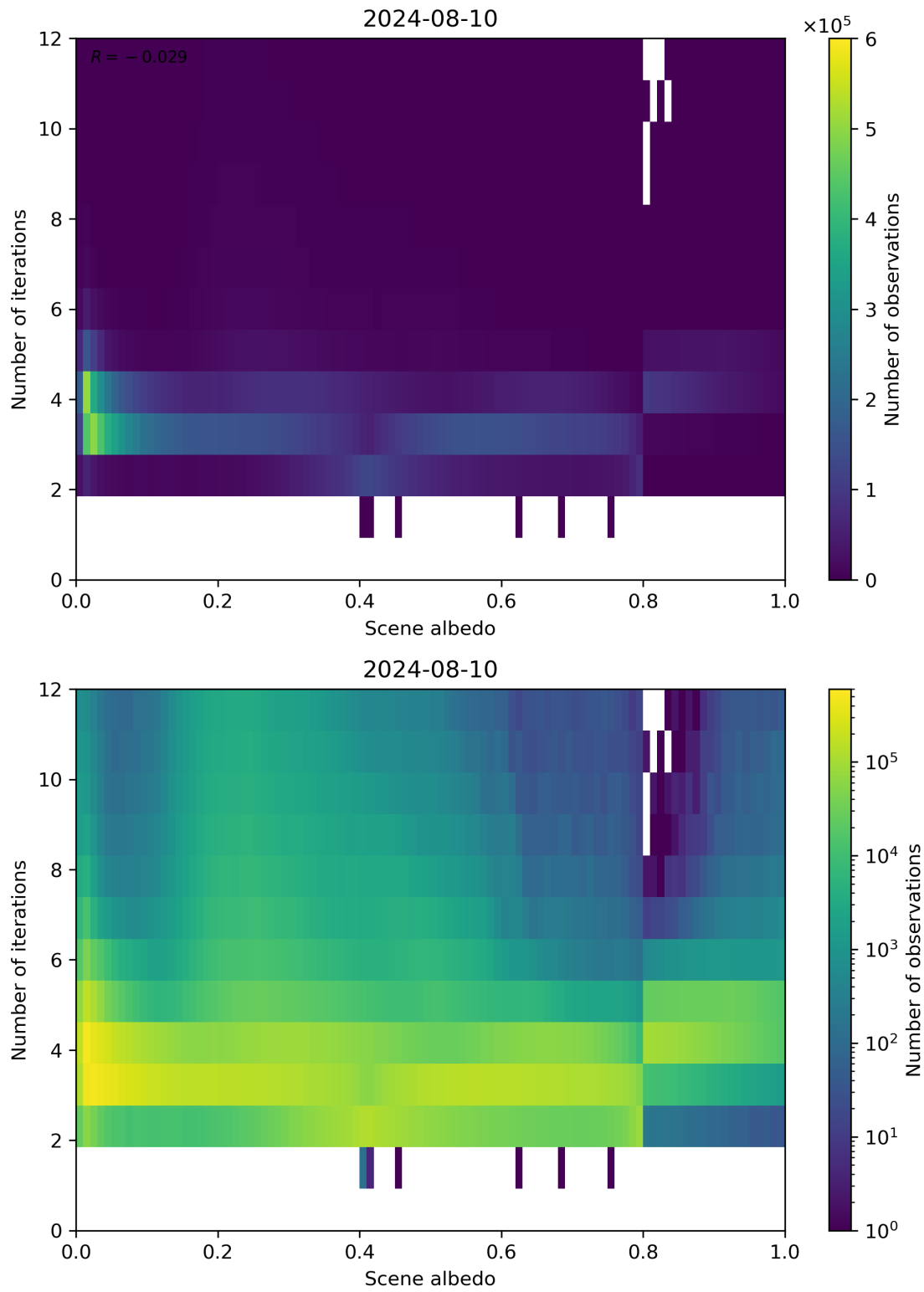
Figure 105: Scatter density plot of “Scene albedo” against “Number of iterations” for 2024-08-09 to 2024-08-11.
