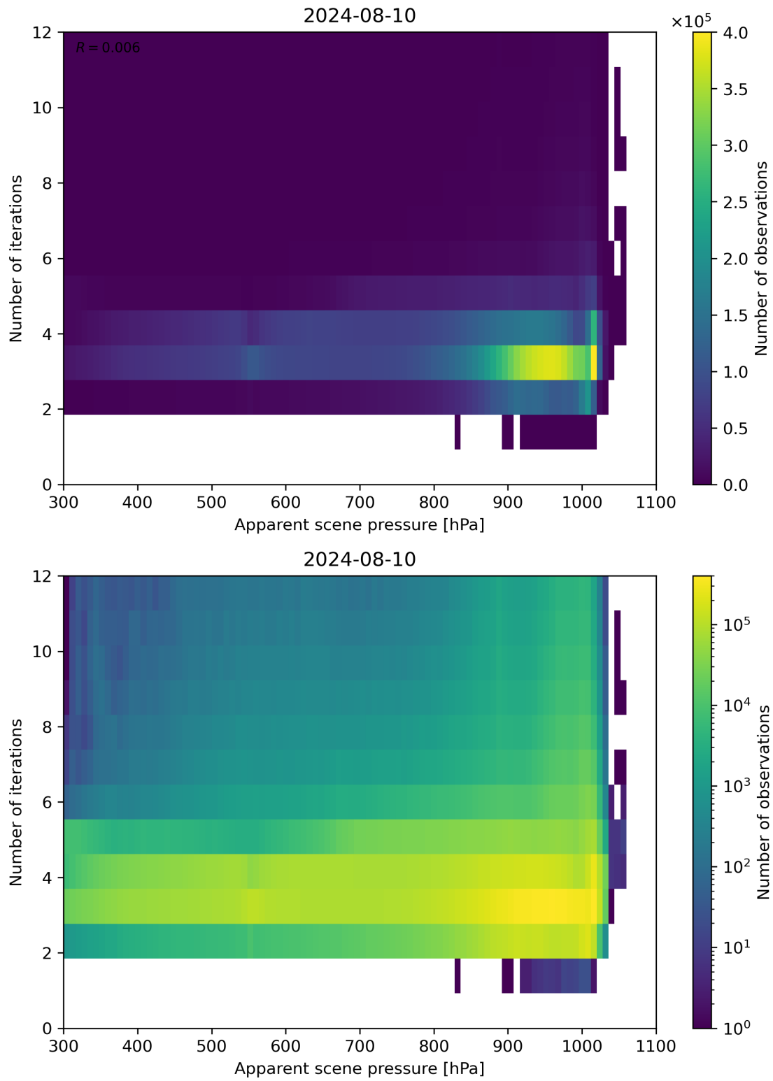
Figure 65: Scatter density plot of “Apparent scene pressure” against “Number of iterations” for 2024-08-09 to 2024-08-11.
