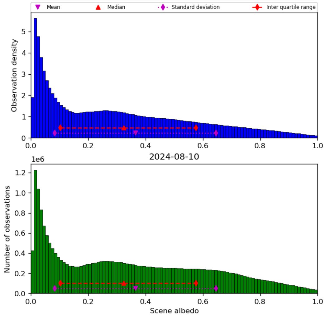
Figure 34: Histogram of “Scene albedo” for 2024-08-09 to 2024-08-11
