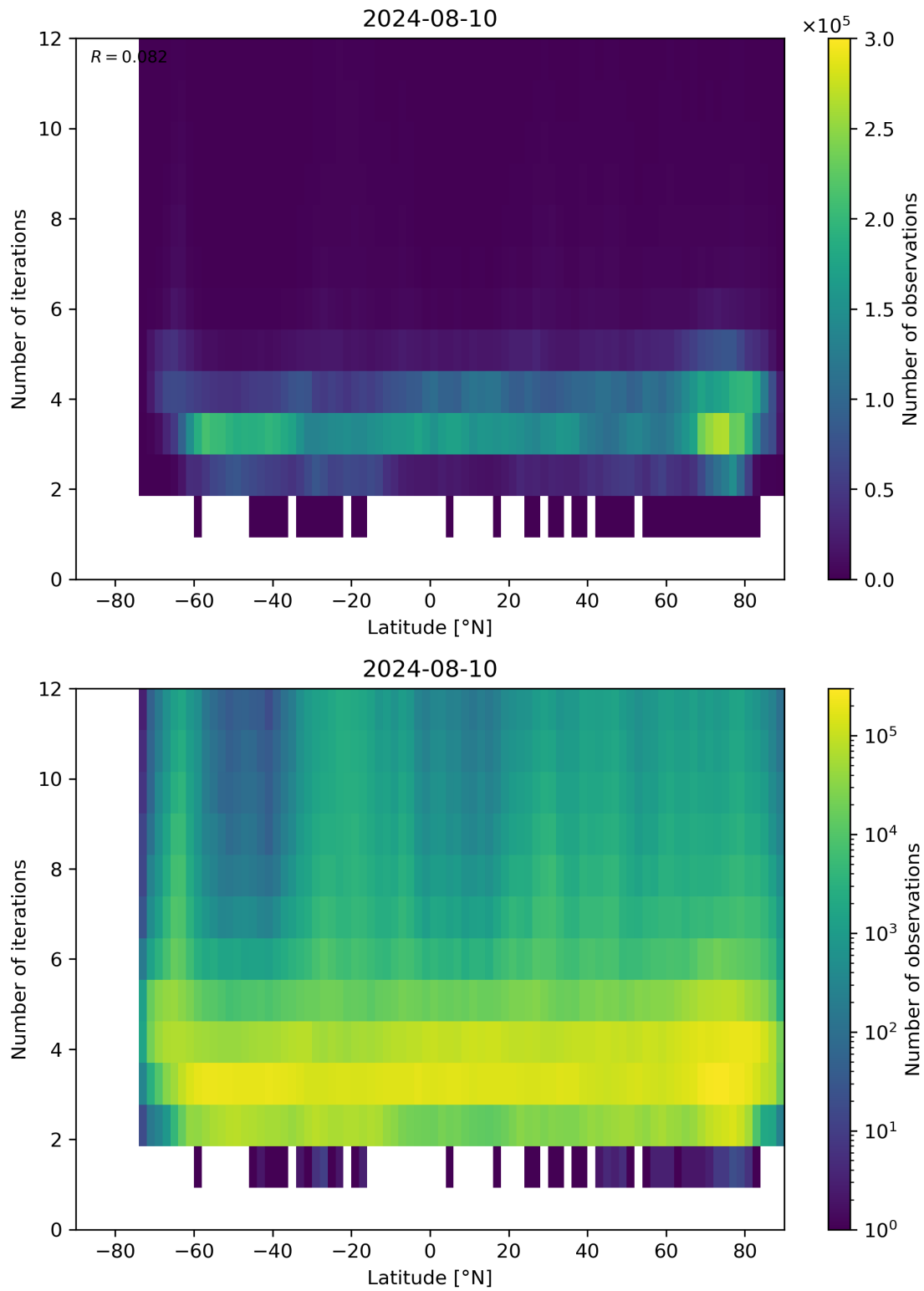
Figure 93: Scatter density plot of “Latitude” against “Number of iterations” for 2024-08-09 to 2024-08-11.
