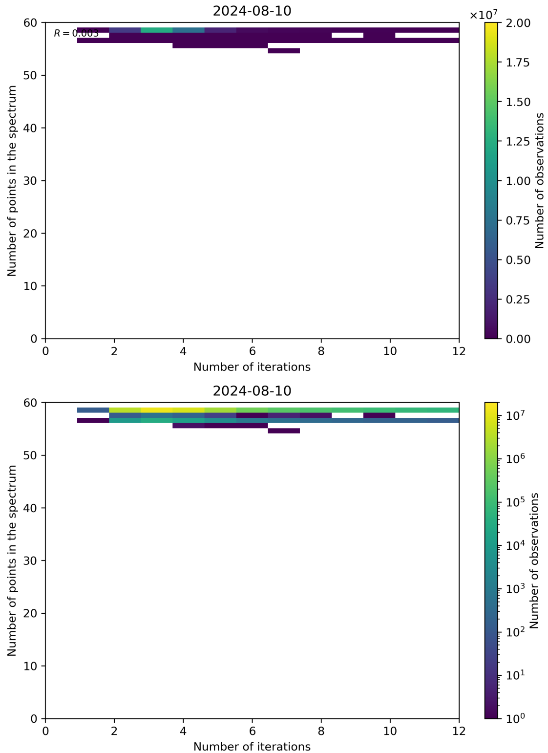
Figure 99: Scatter density plot of “Number of iterations” against “Number of points in the spectrum” for 2024-08-09 to 2024-08-11.
