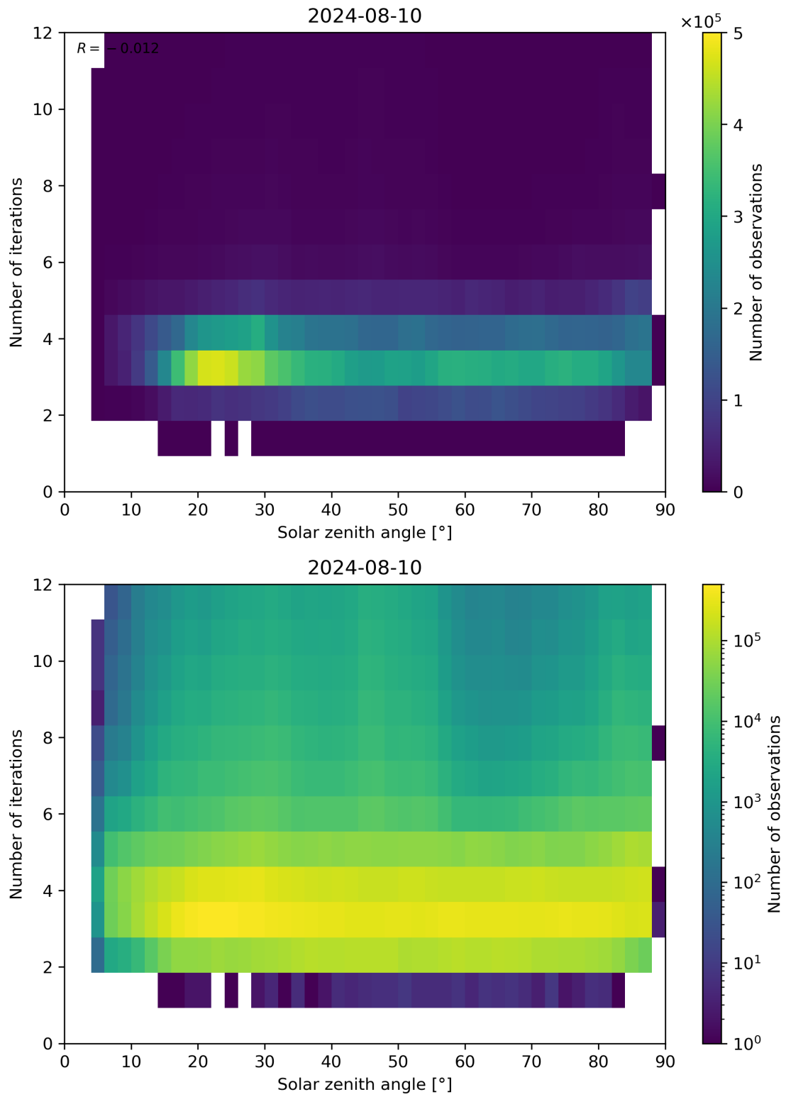
Figure 114: Scatter density plot of “Solar zenith angle” against “Number of iterations” for 2024-08-09 to 2024-08-11.
