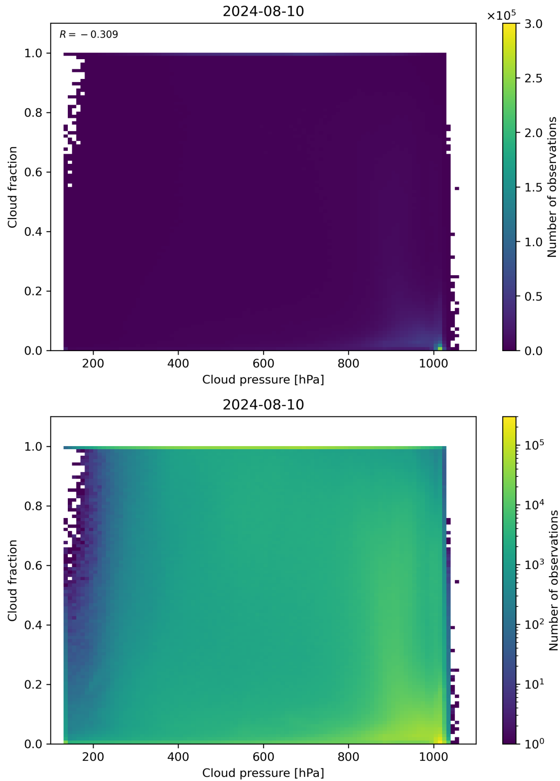
Figure 79: Scatter density plot of “Cloud pressure” against “Cloud fraction” for 2024-08-09 to 2024-08-11.
