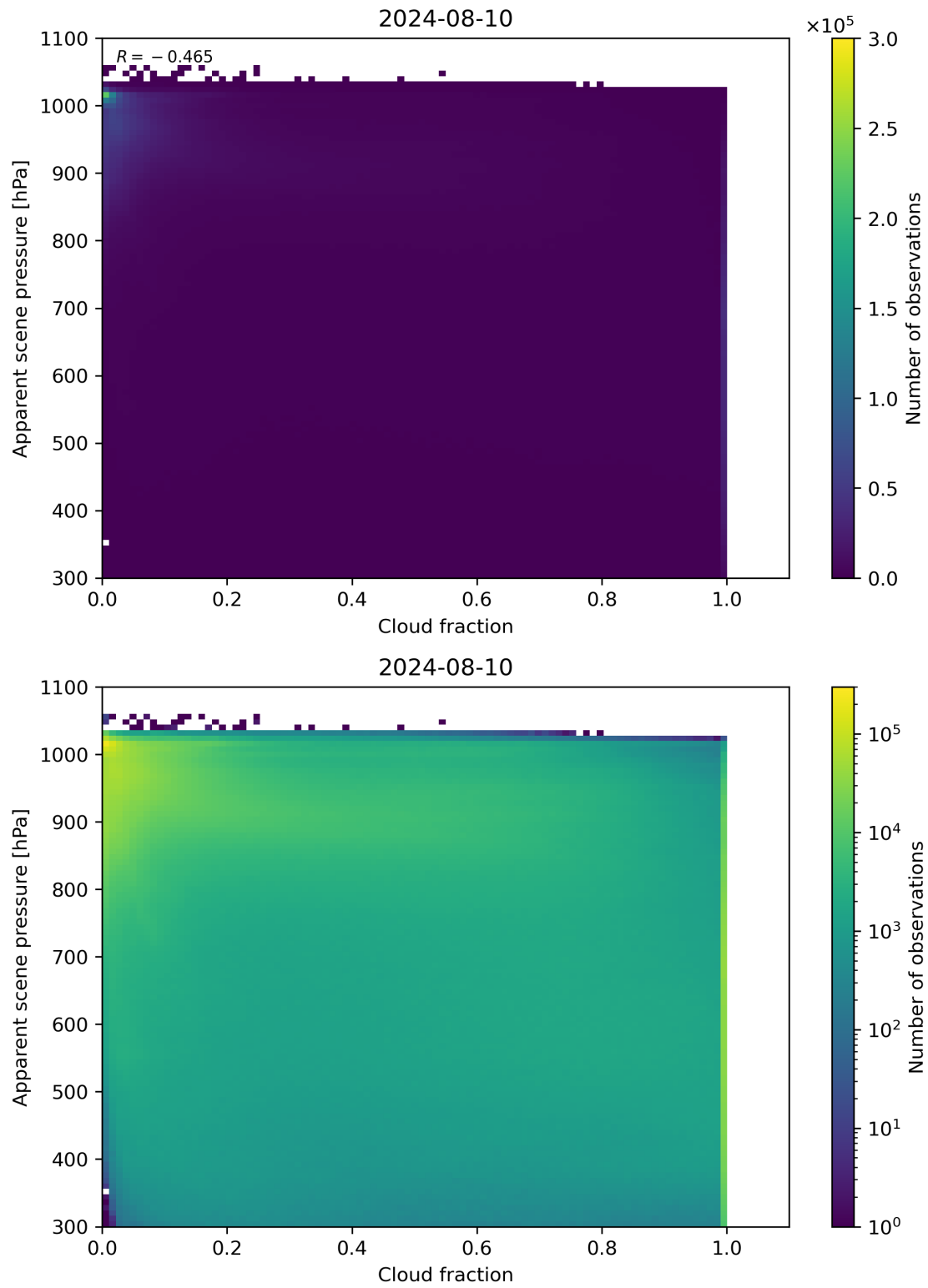
Figure 70: Scatter density plot of “Cloud fraction” against “Apparent scene pressure” for 2024-08-09 to 2024-08-11.
