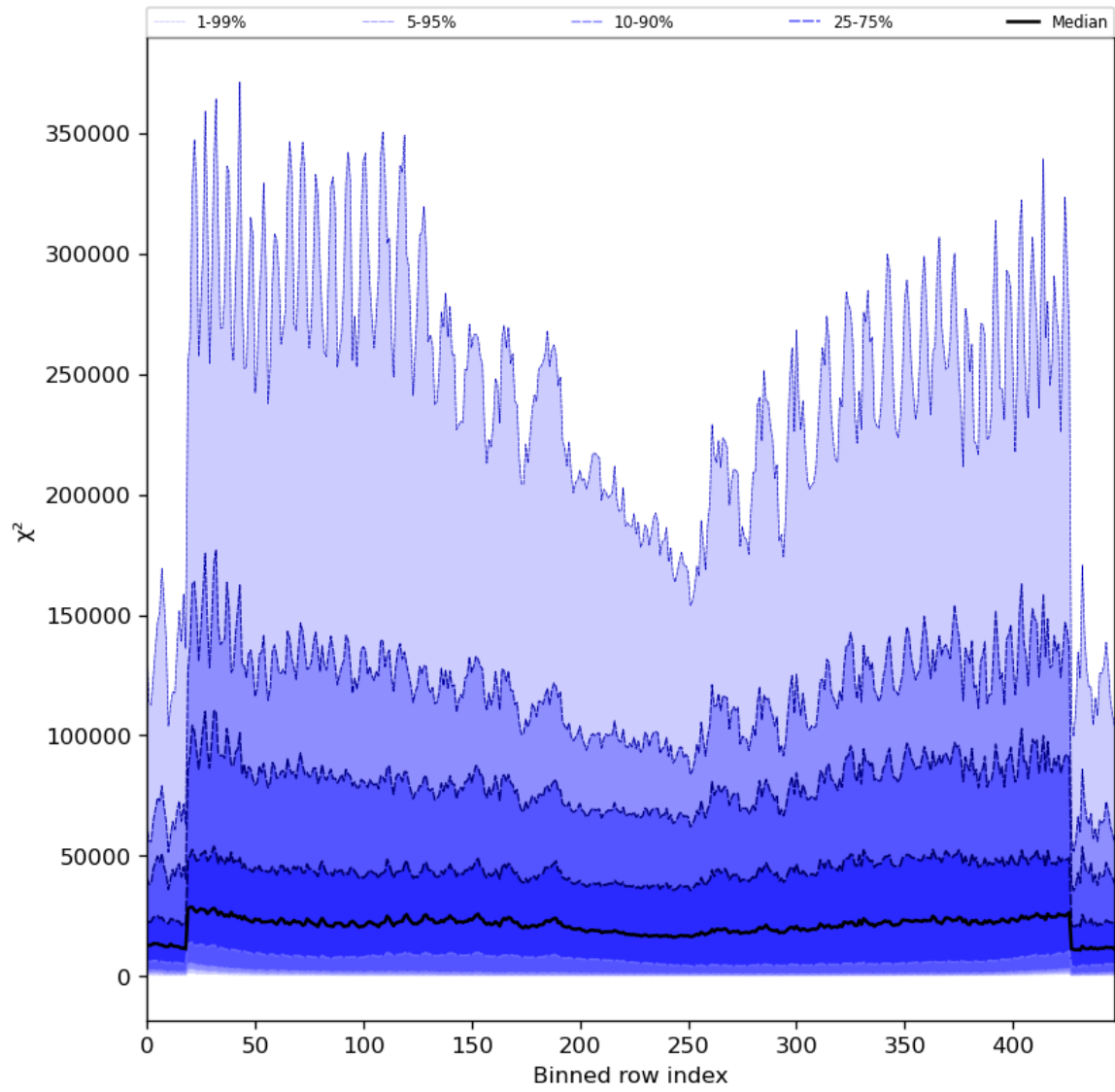
Figure 55: Along track statistics of “ \chi^2 ” for 2024-08-09 to 2024-08-11
