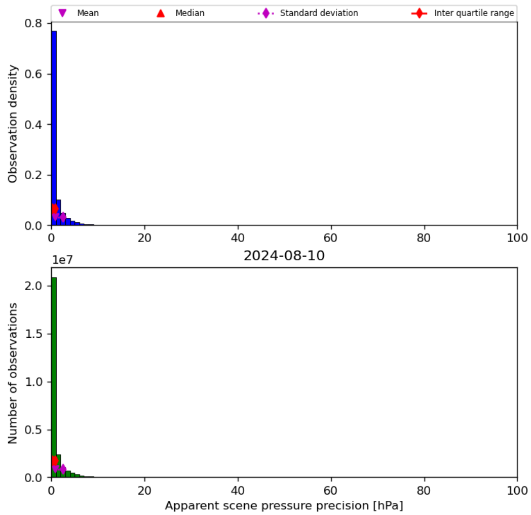
Figure 37: Histogram of “Apparent scene pressure precision” for 2024-08-09 to 2024-08-11
