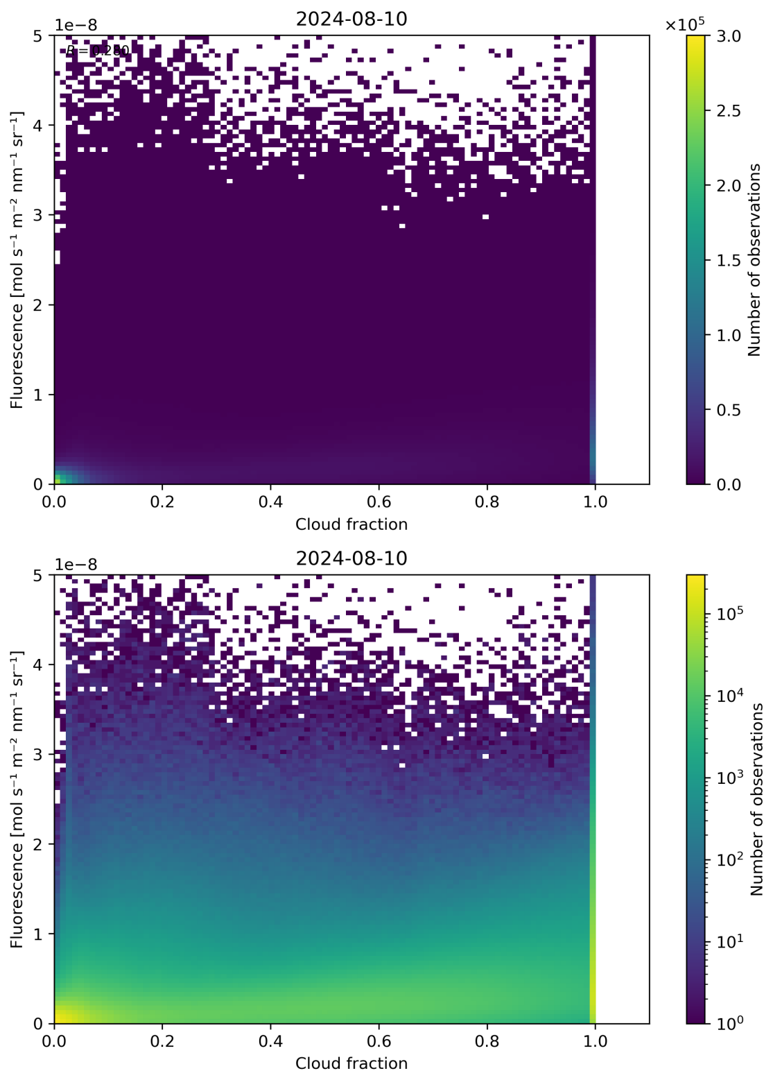
Figure 72: Scatter density plot of “Cloud fraction” against “Fluorescence” for 2024-08-09 to 2024-08-11.
