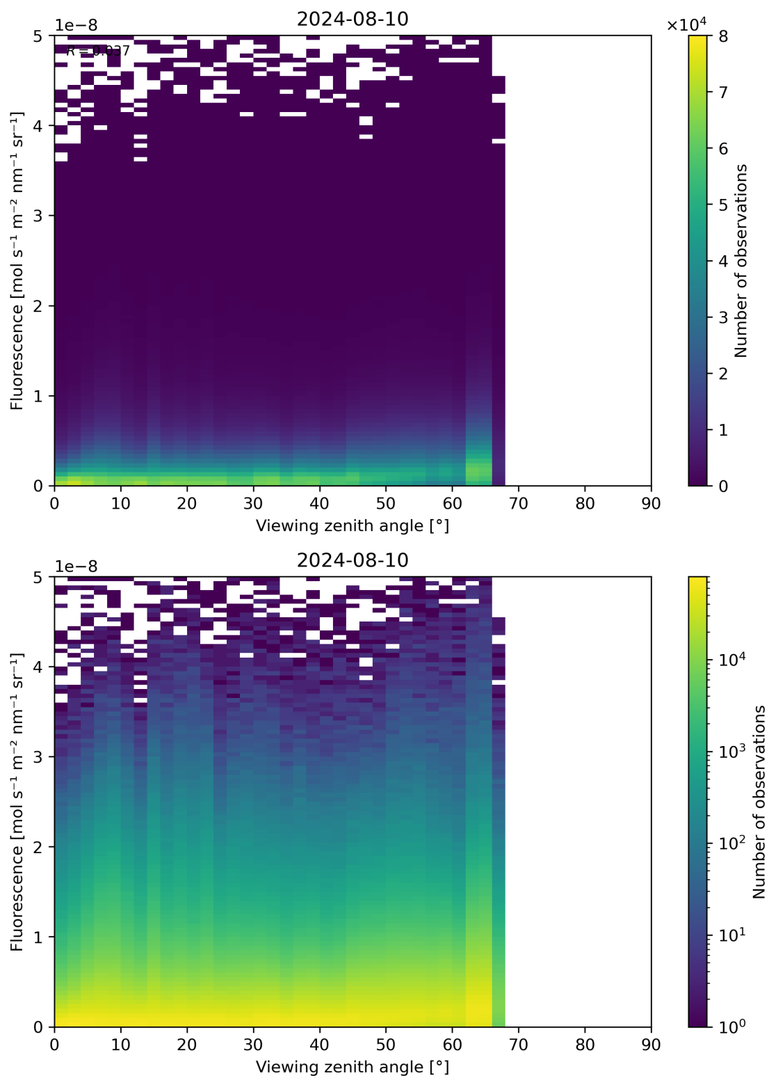
Figure 122: Scatter density plot of “Viewing zenith angle” against “Fluorescence” for 2024-08-09 to 2024-08-11.
