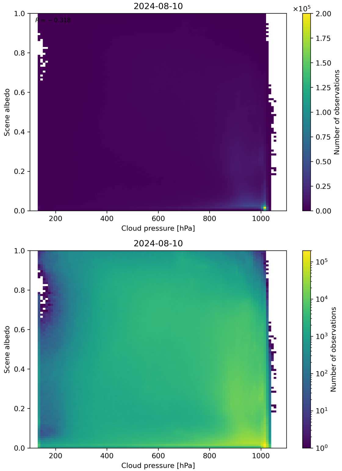
Figure 83: Scatter density plot of “Cloud pressure” against “Scene albedo” for 2024-08-09 to 2024-08-11.
