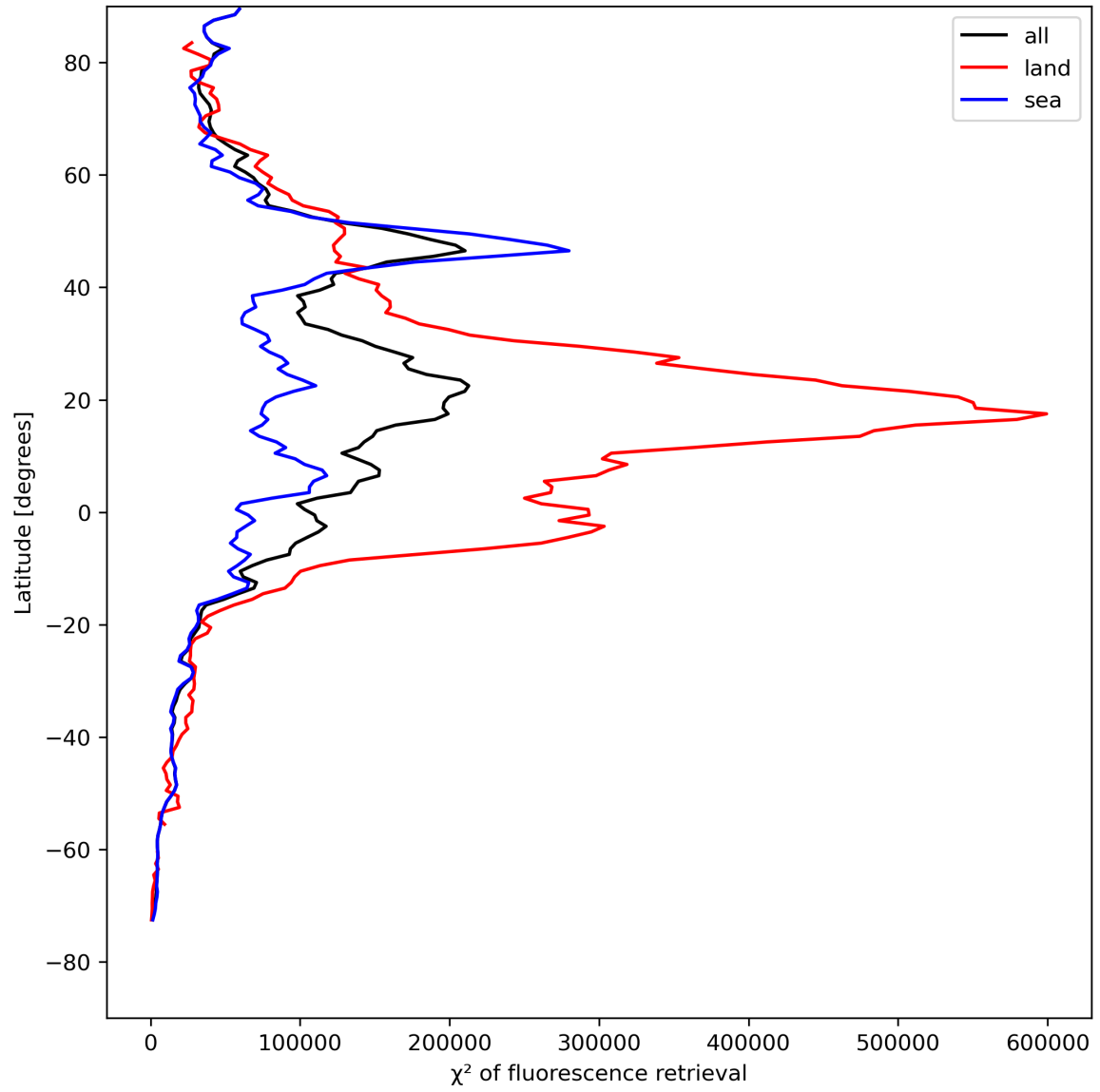
Figure 25: Zonal average of “ \chi^2 of fluorescence retrieval” for 2024-08-09 to 2024-08-11.
