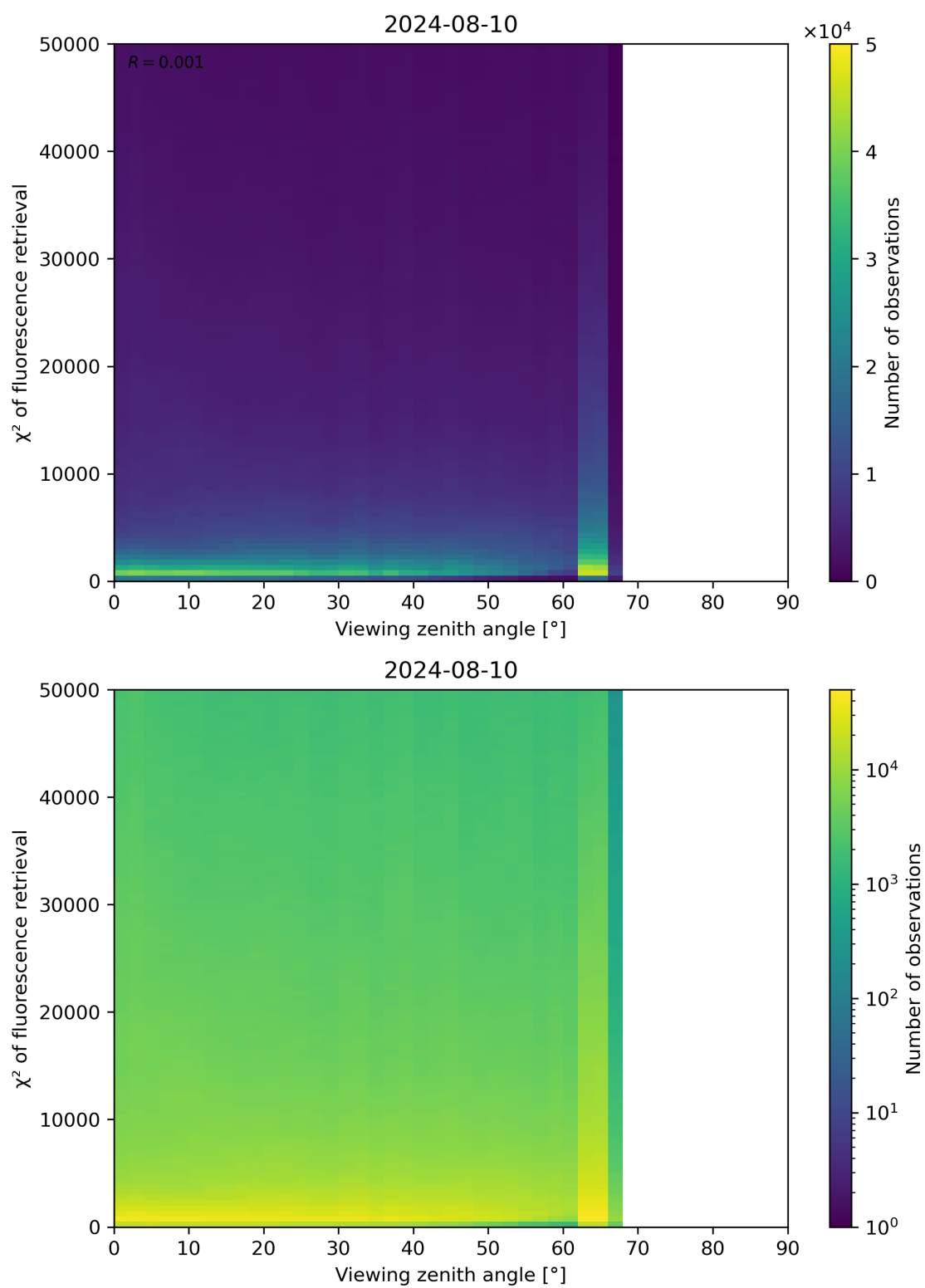
Figure 119: Scatter density plot of “Viewing zenith angle” against “ \chi^2 of fluorescence retrieval” for 2024-08-09 to 2024-08-11.
