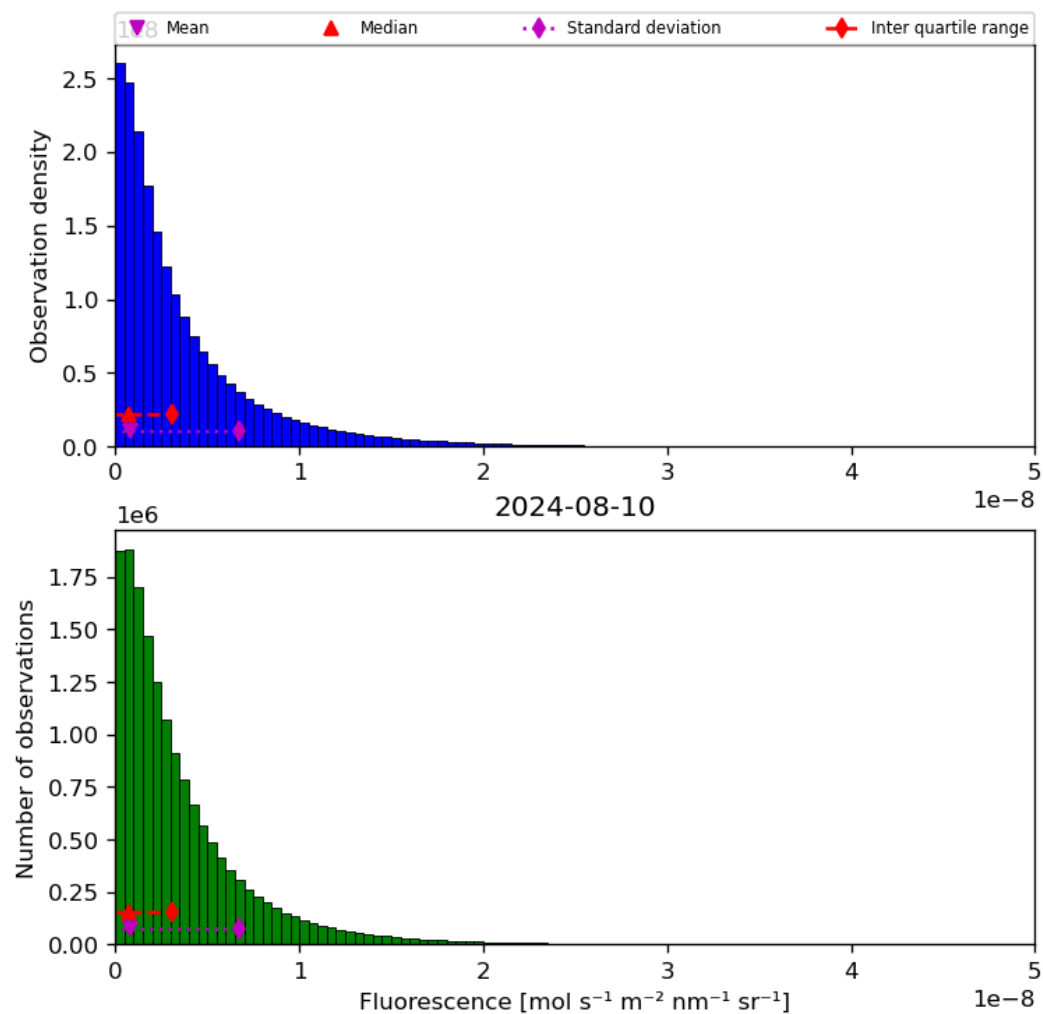
Figure 40: Histogram of “Fluorescence” for 2024-08-09 to 2024-08-11
