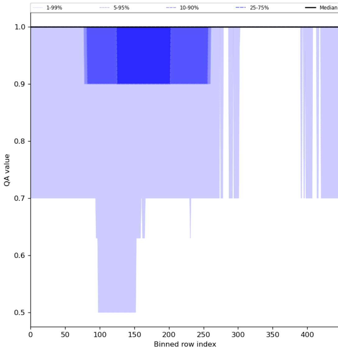
Figure 46: Along track statistics of “QA value” for 2024-08-09 to 2024-08-11
