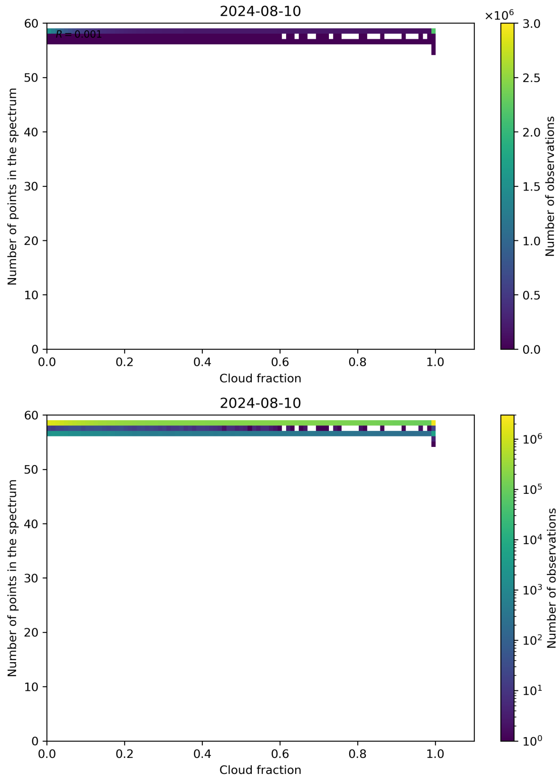
Figure 74: Scatter density plot of “Cloud fraction” against “Number of points in the spectrum” for 2024-08-09 to 2024-08-11.
