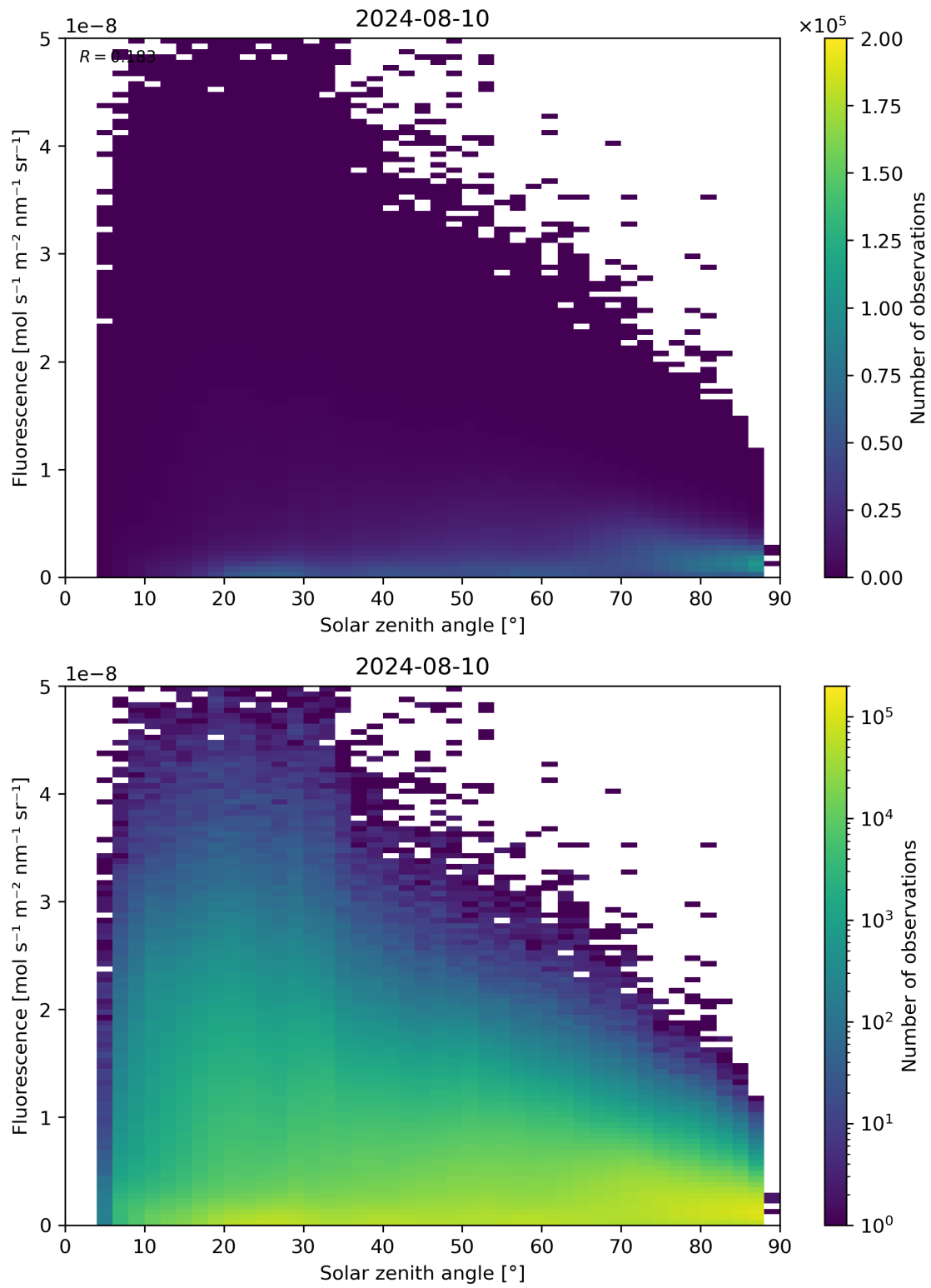
Figure 112: Scatter density plot of “Solar zenith angle” against “Fluorescence” for 2024-08-09 to 2024-08-11.
