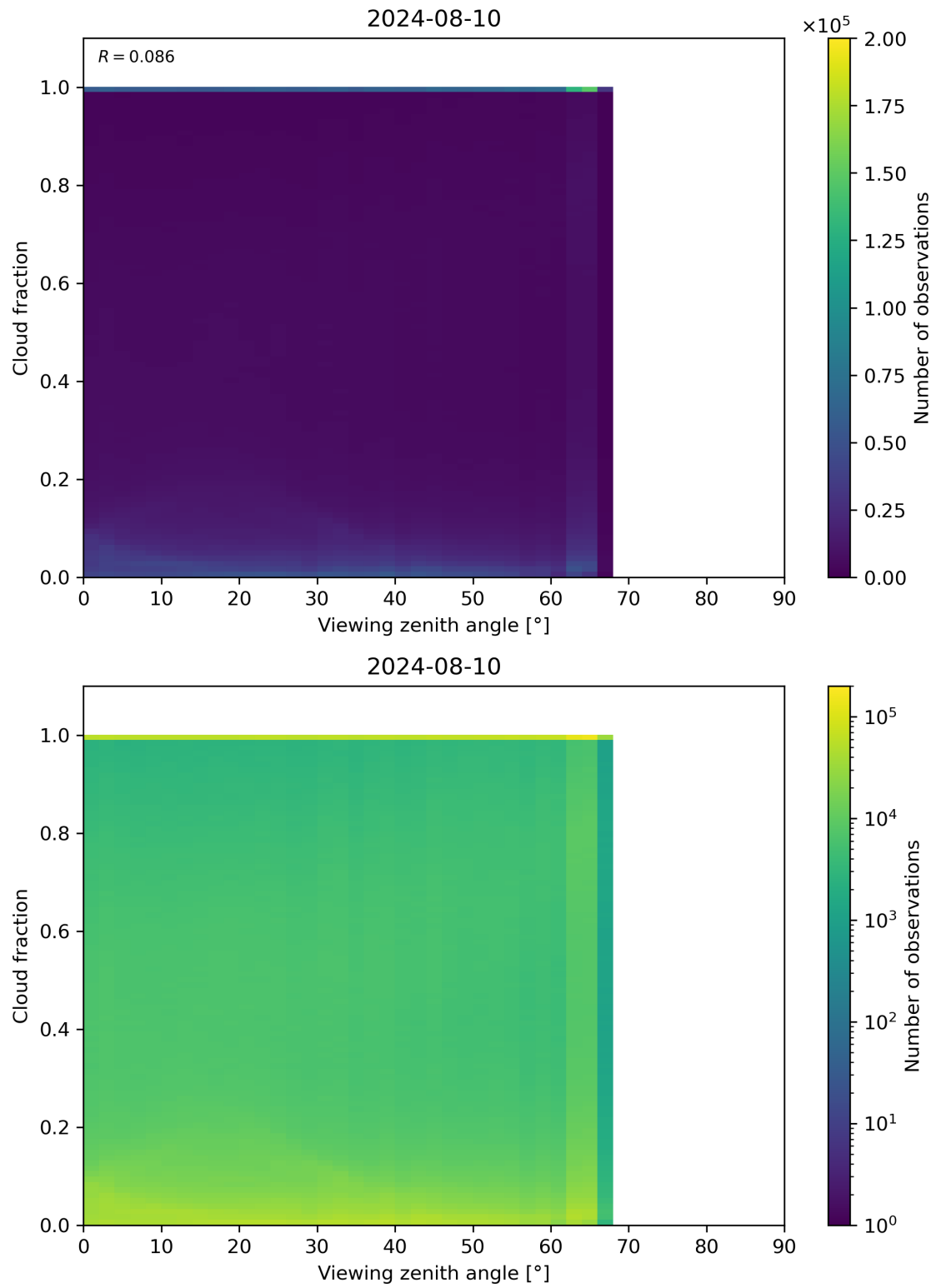
Figure 120: Scatter density plot of “Viewing zenith angle” against “Cloud fraction” for 2024-08-09 to 2024-08-11.
