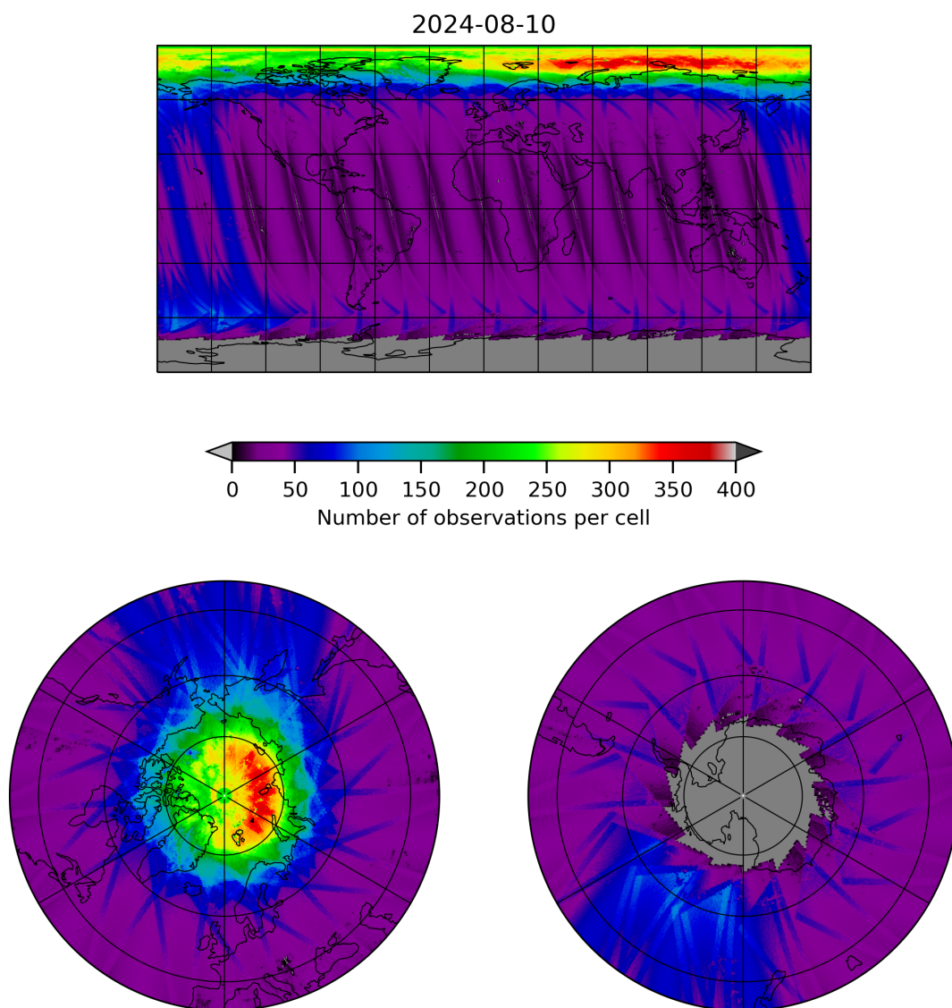
Figure 11: Map of the number of observations for 2024-08-09 to 2024-08-11
