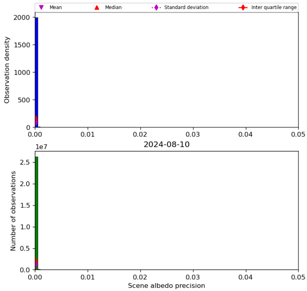
Figure 35: Histogram of “Scene albedo precision” for 2024-08-09 to 2024-08-11
