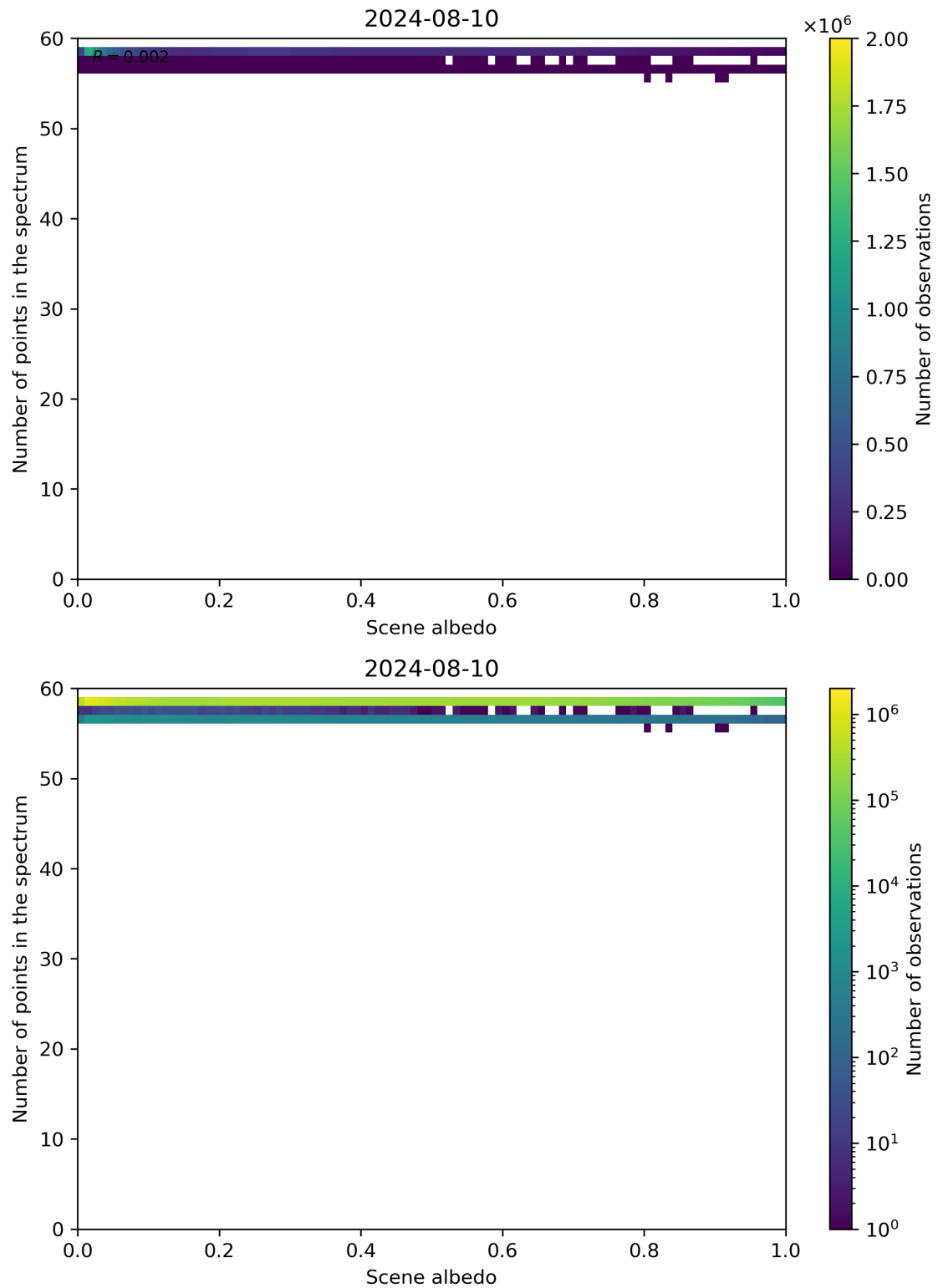
Figure 106: Scatter density plot of “Scene albedo” against “Number of points in the spectrum” for 2024-08-09 to 2024-08-11.
