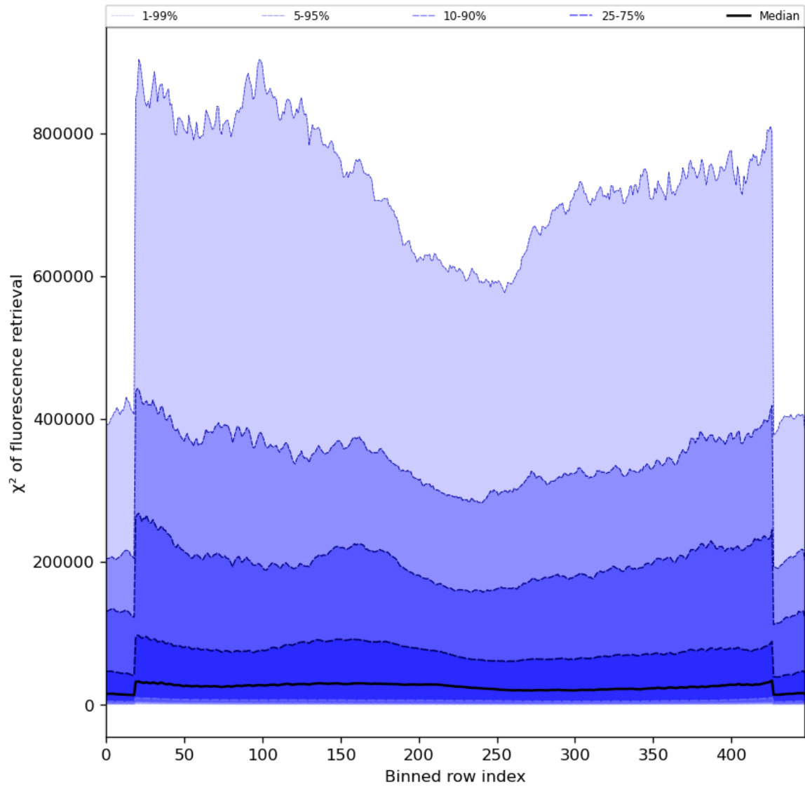
Figure 59: Along track statistics of “ \chi^2 of fluorescence retrieval” for 2024-08-09 to 2024-08-11
