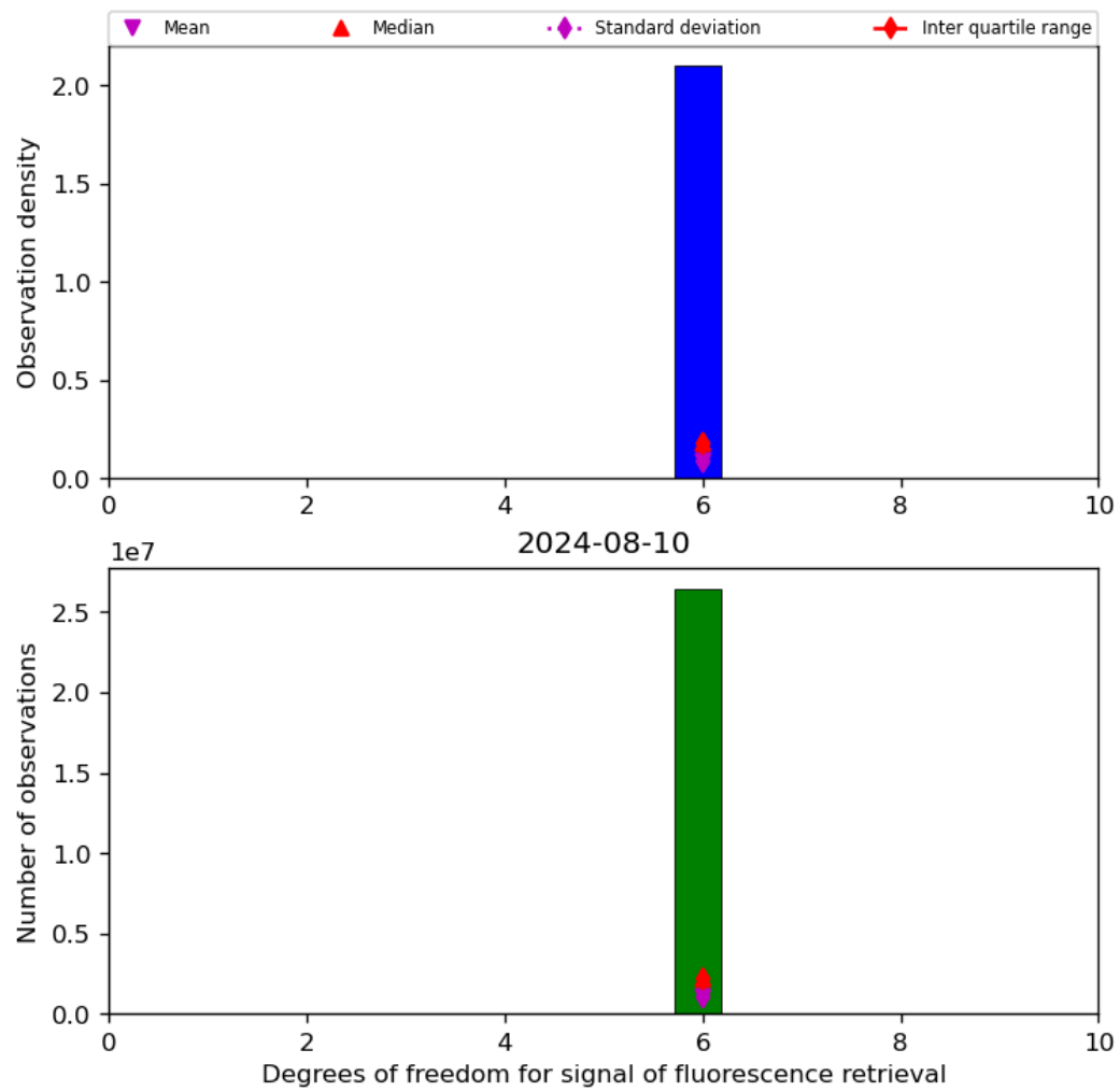
Figure 43: Histogram of “Degrees of freedom for signal of fluorescence retrieval” for 2024-08-09 to 2024-08-11
