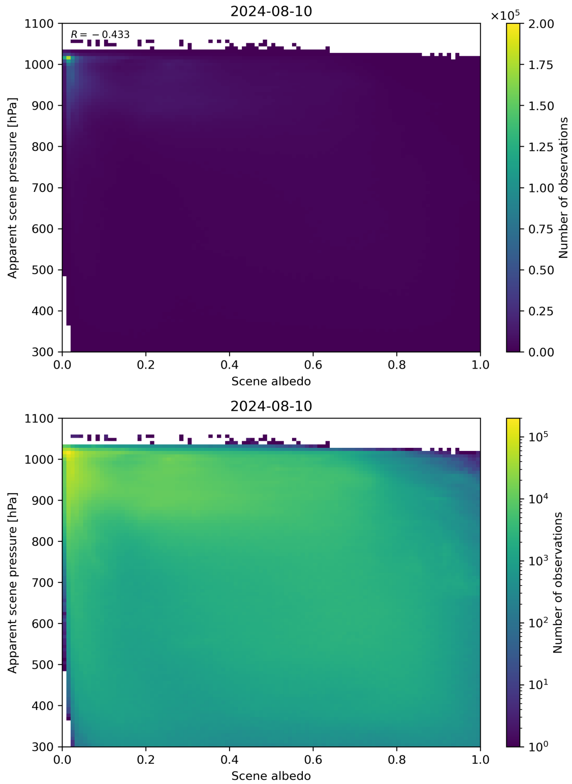
Figure 102: Scatter density plot of “Scene albedo” against “Apparent scene pressure” for 2024-08-09 to 2024-08-11.
