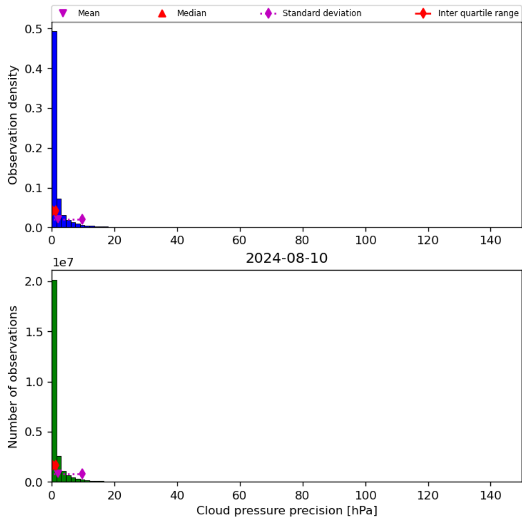
Figure 31: Histogram of “Cloud pressure precision” for 2024-08-09 to 2024-08-11
