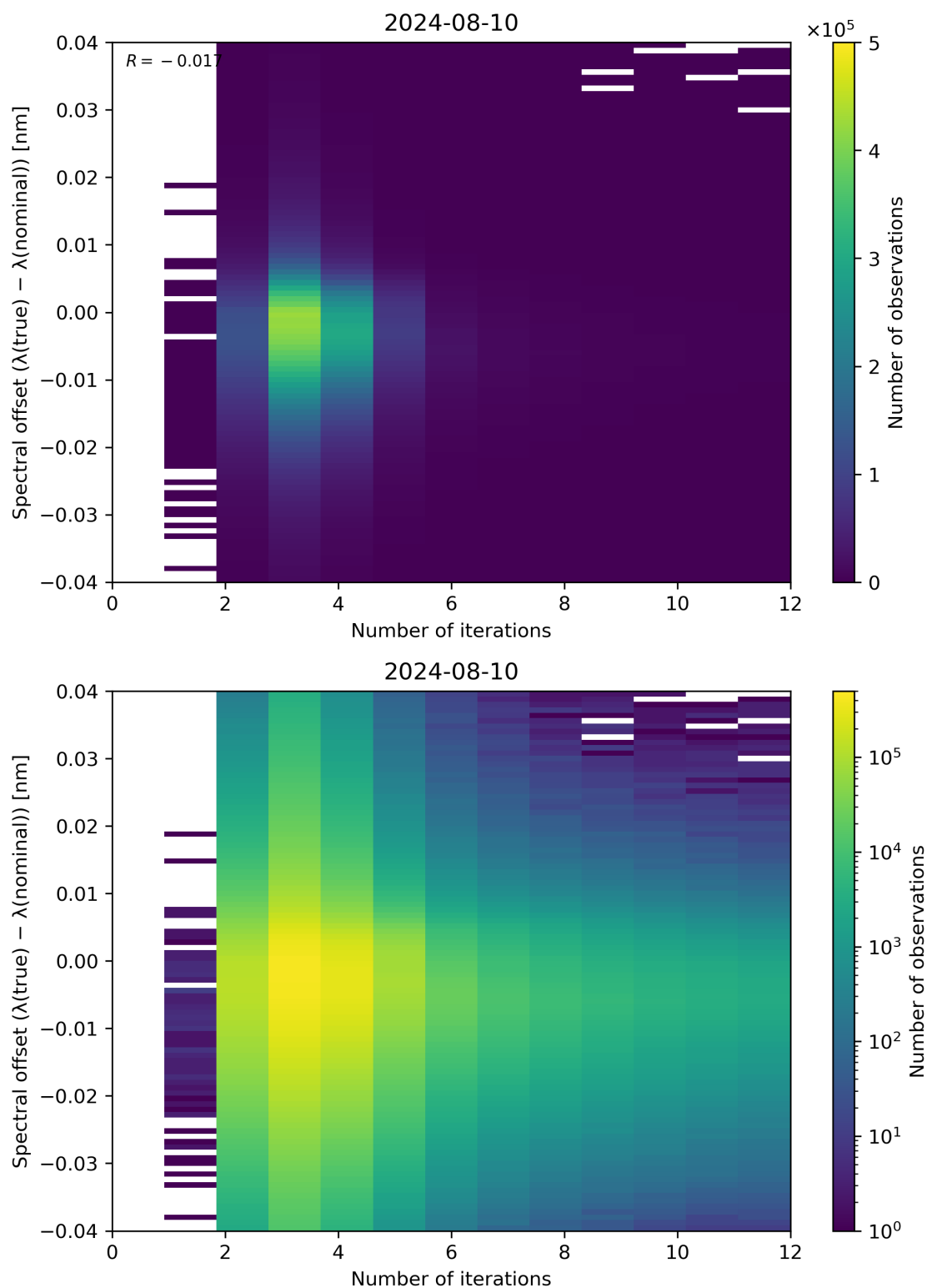
Figure 100: Scatter density plot of “Number of iterations” against “Spectral offset ( \lambda(\text{true}) - \lambda(\text{nominal}) )” for 2024-08-09 to 2024-08-11.
