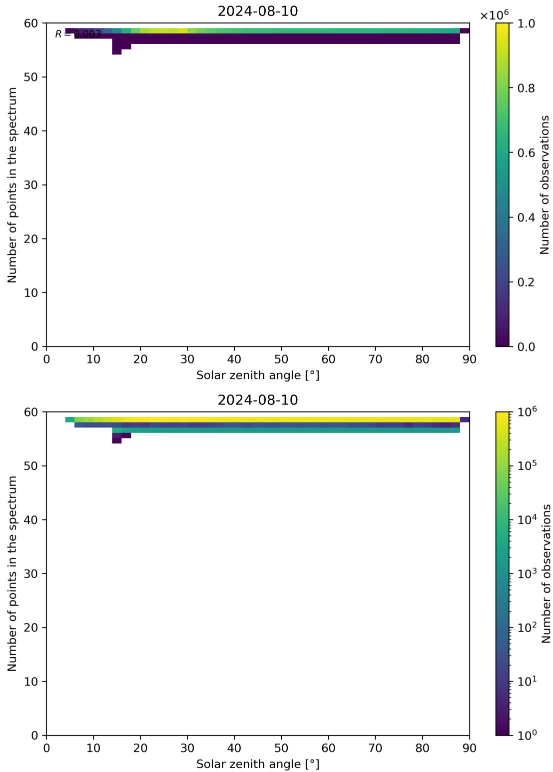
Figure 115: Scatter density plot of “Solar zenith angle” against “Number of points in the spectrum” for 2024-08-09 to 2024-08-11.
