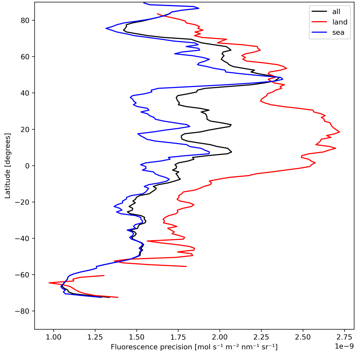
Figure 24: Zonal average of “Fluorescence precision” for 2024-08-09 to 2024-08-11.
