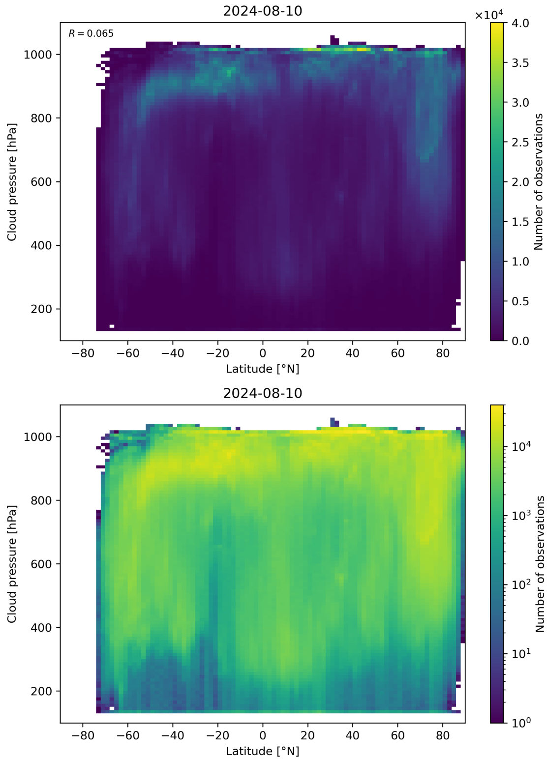
Figure 91: Scatter density plot of “Latitude” against “Cloud pressure” for 2024-08-09 to 2024-08-11.
