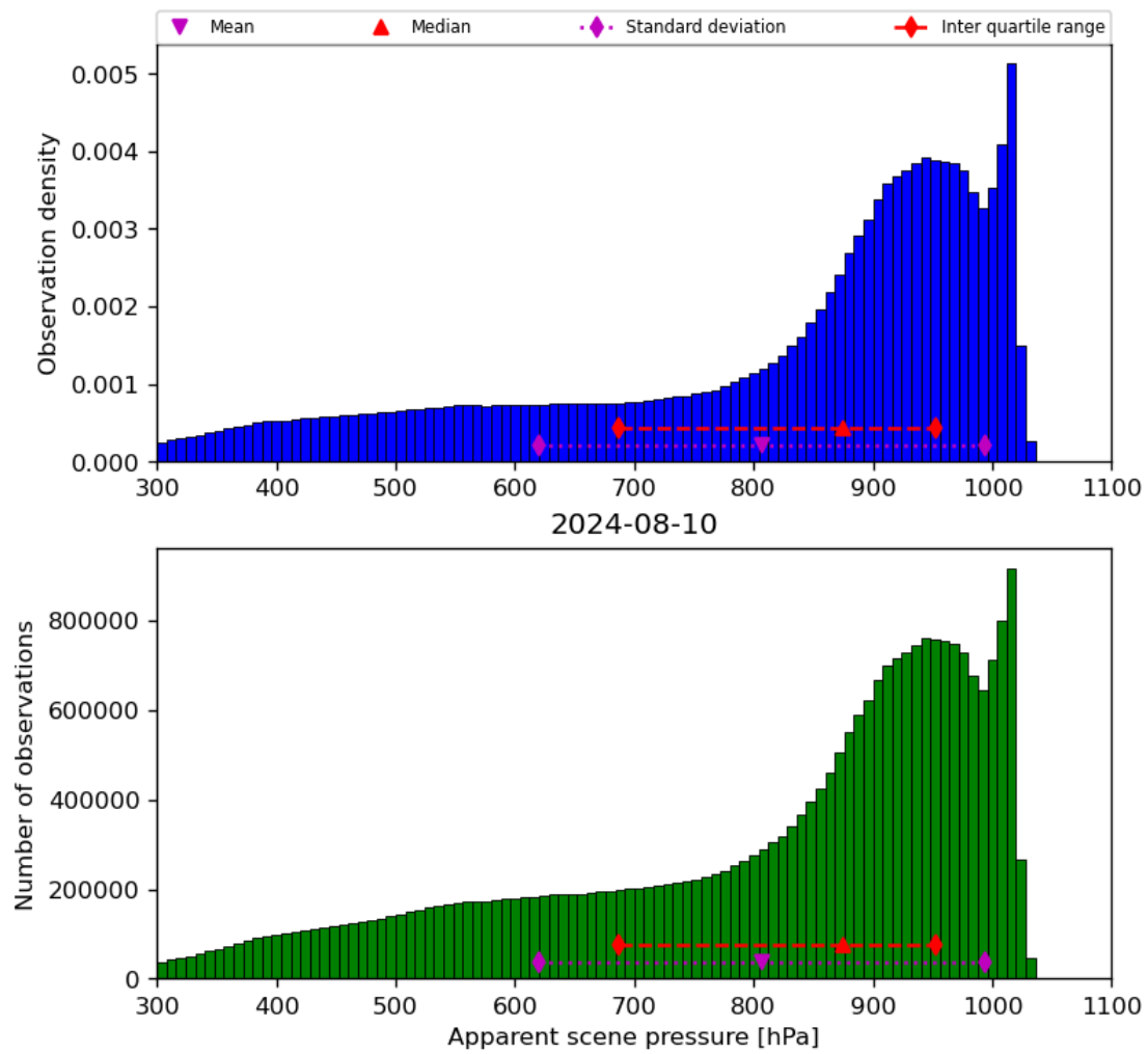
Figure 36: Histogram of “Apparent scene pressure” for 2024-08-09 to 2024-08-11
