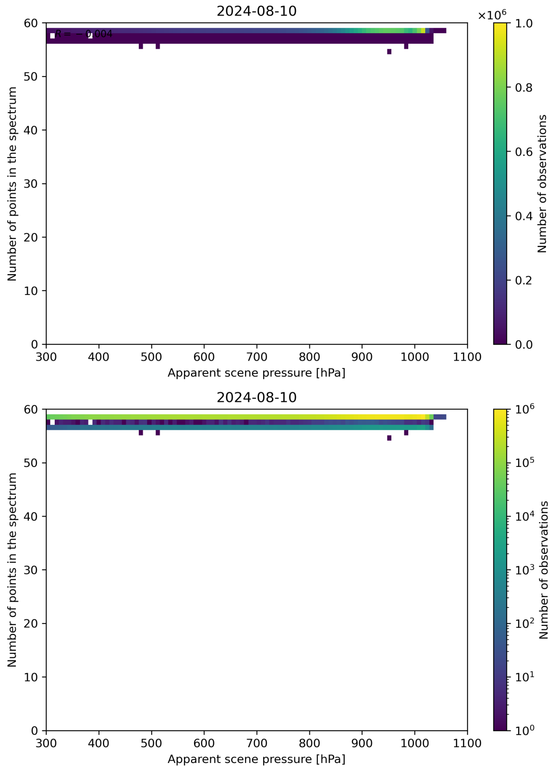
Figure 66: Scatter density plot of “Apparent scene pressure” against “Number of points in the spectrum” for 2024-08-09 to 2024-08-11.
