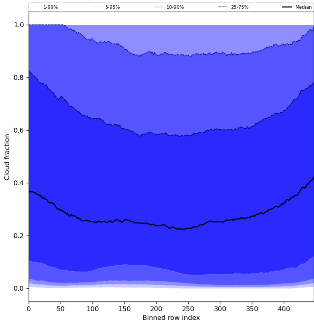
Figure 49: Along track statistics of “Cloud fraction” for 2024-08-09 to 2024-08-11
