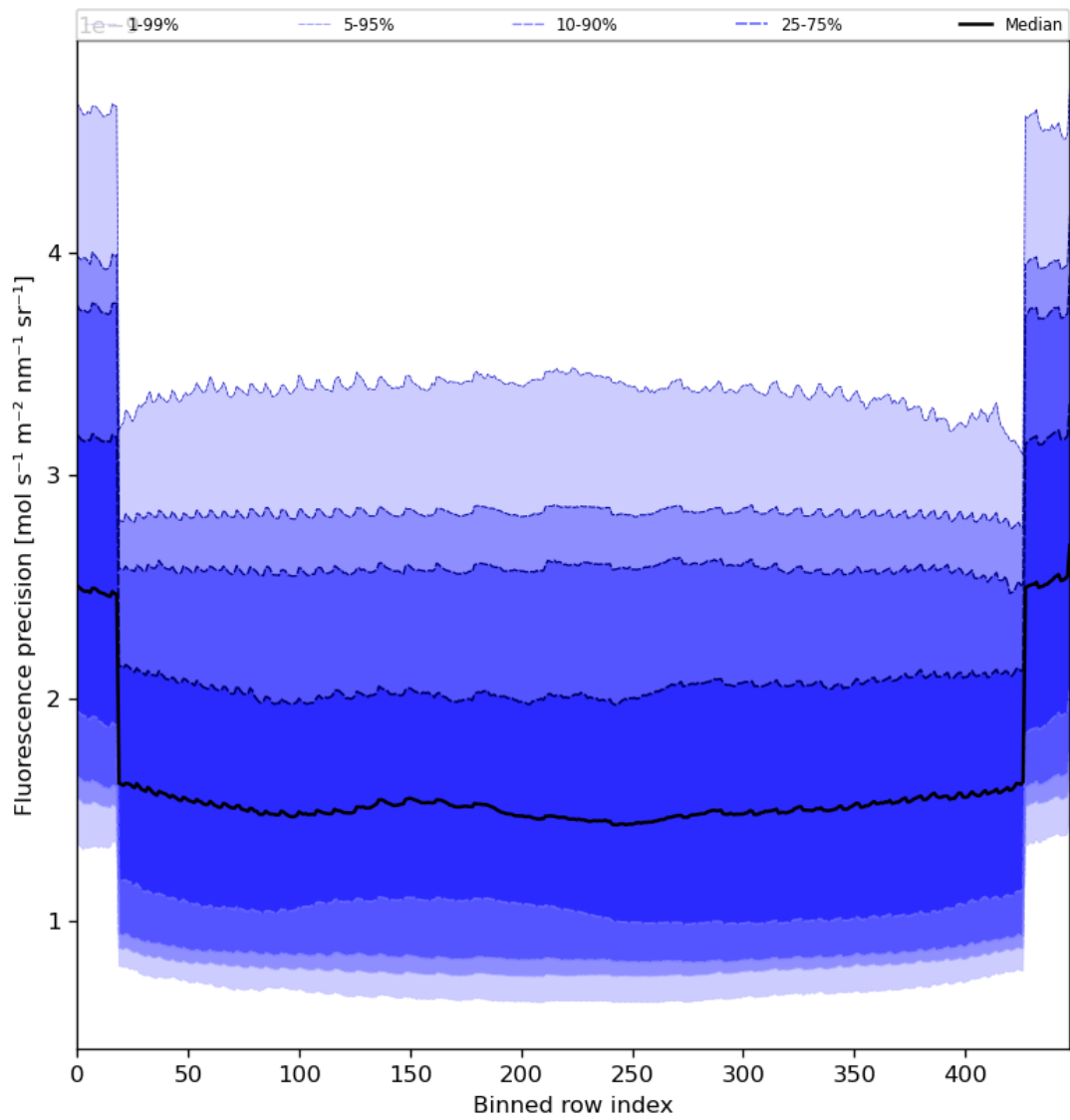
Figure 58: Along track statistics of “Fluorescence precision” for 2024-08-09 to 2024-08-11
