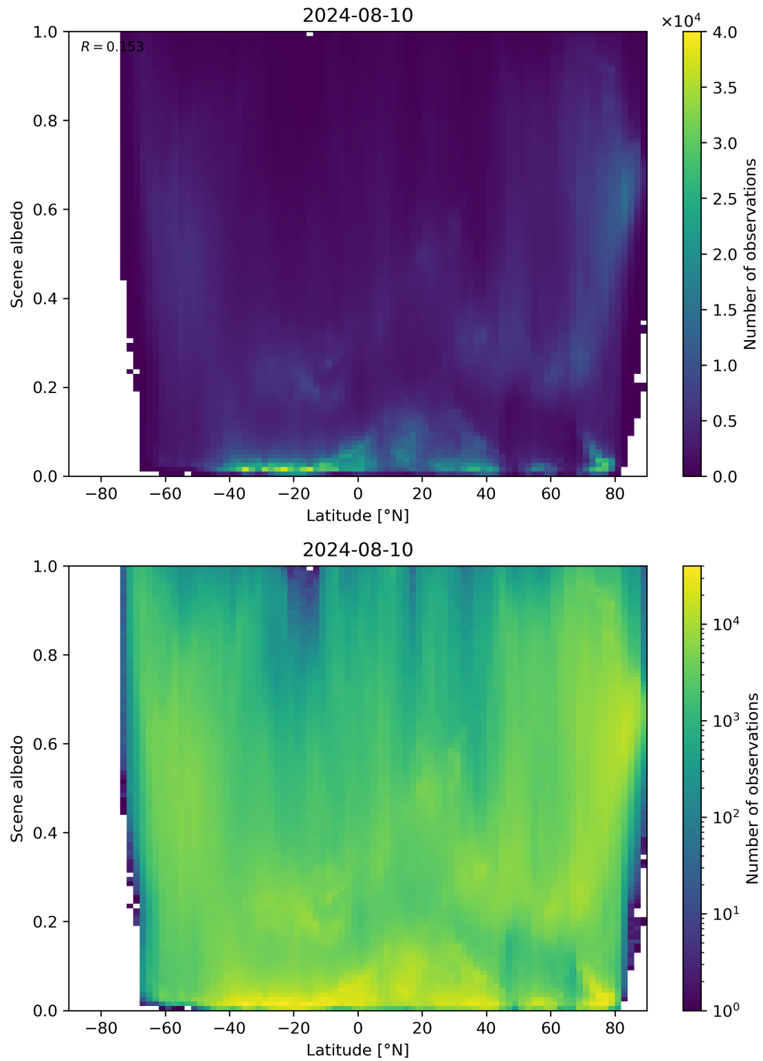
Figure 95: Scatter density plot of “Latitude” against “Scene albedo” for 2024-08-09 to 2024-08-11.
