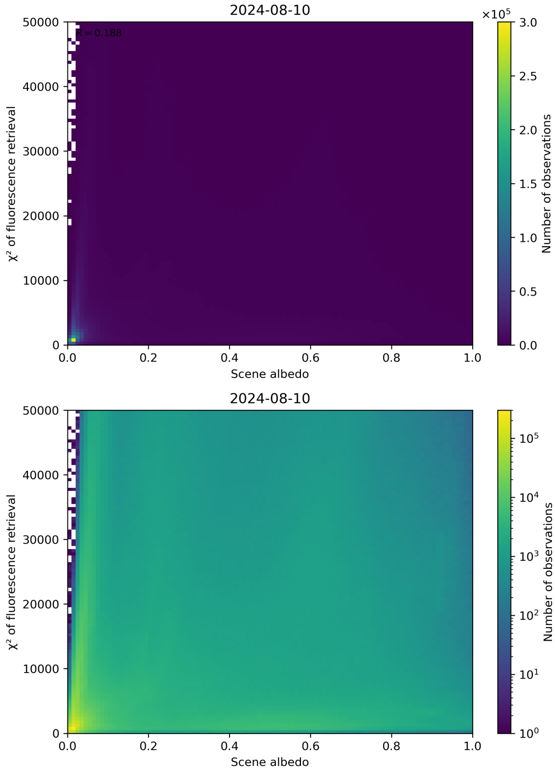
Figure 103: Scatter density plot of “Scene albedo” against “ \chi^2 of fluorescence retrieval” for 2024-08-09 to 2024-08-11.
