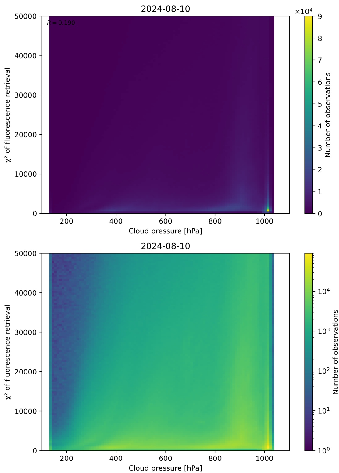
Figure 78: Scatter density plot of “Cloud pressure” against “ \chi^2 of fluorescence retrieval” for 2024-08-09 to 2024-08-11.
