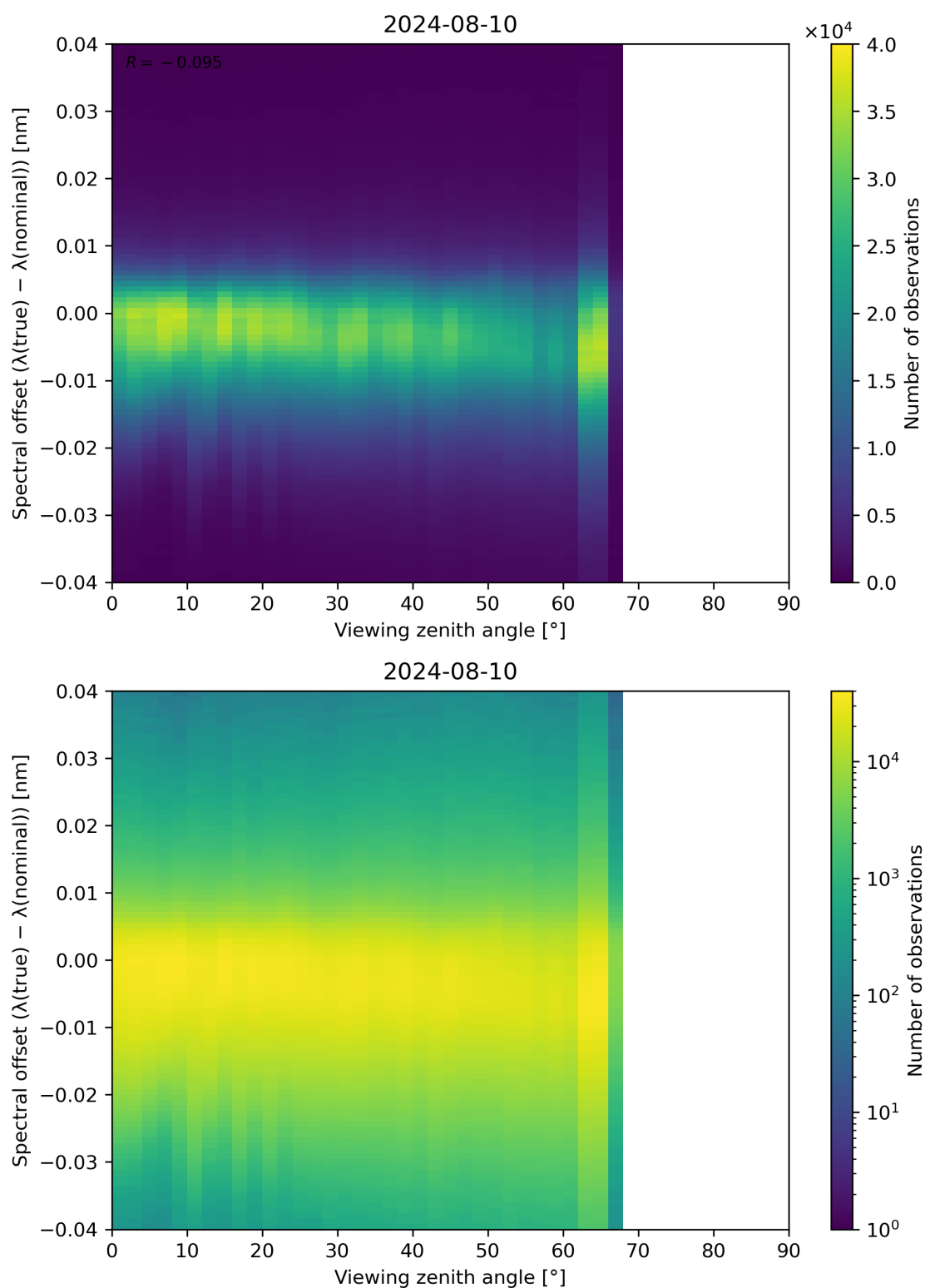
Figure 128: Scatter density plot of “Viewing zenith angle” against “Spectral offset ( \lambda(\text{true}) - \lambda(\text{nominal}) )” for 2024-08-09 to 2024-08-11.
