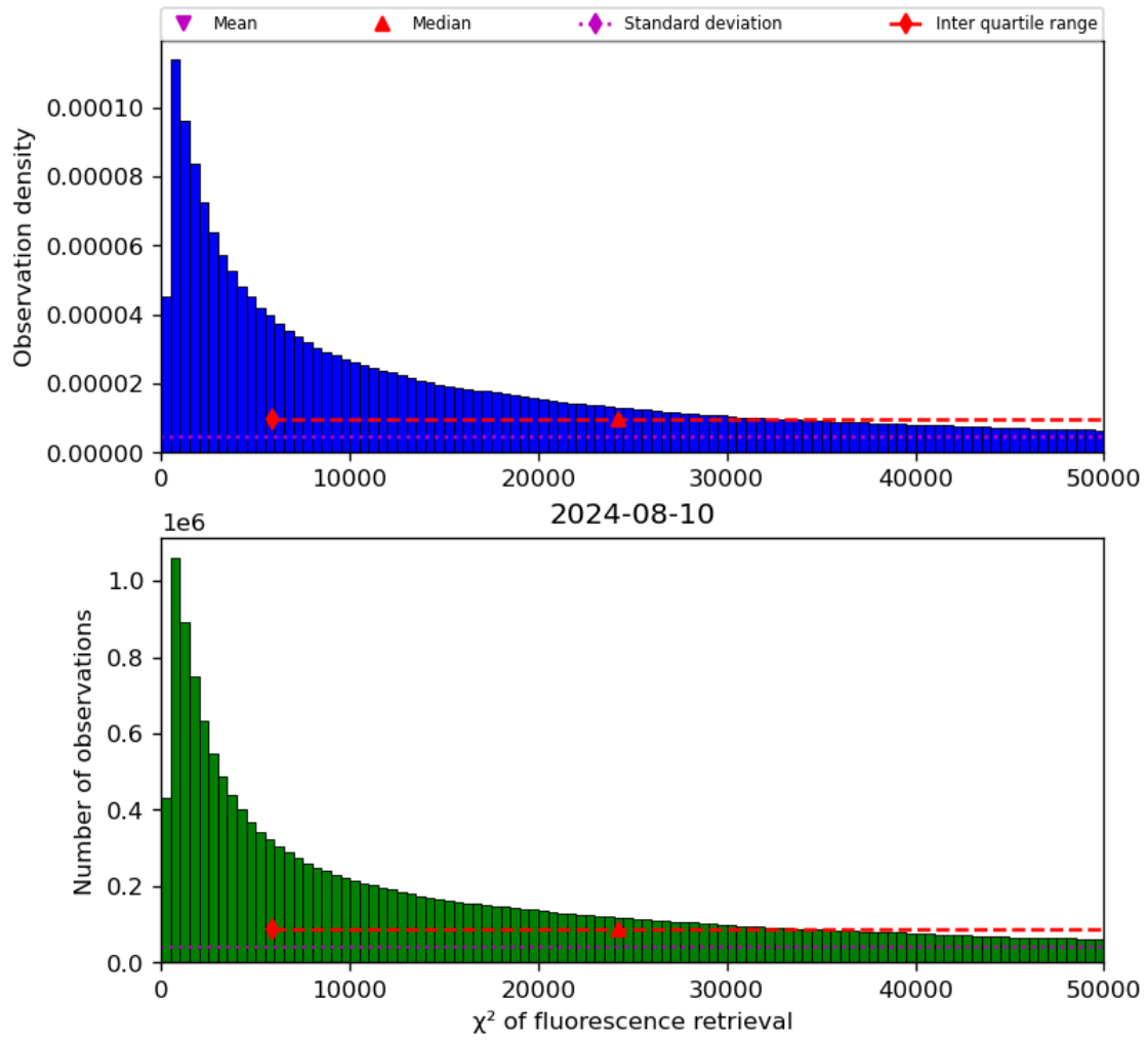
Figure 42: Histogram of “ \chi^2 of fluorescence retrieval” for 2024-08-09 to 2024-08-11
