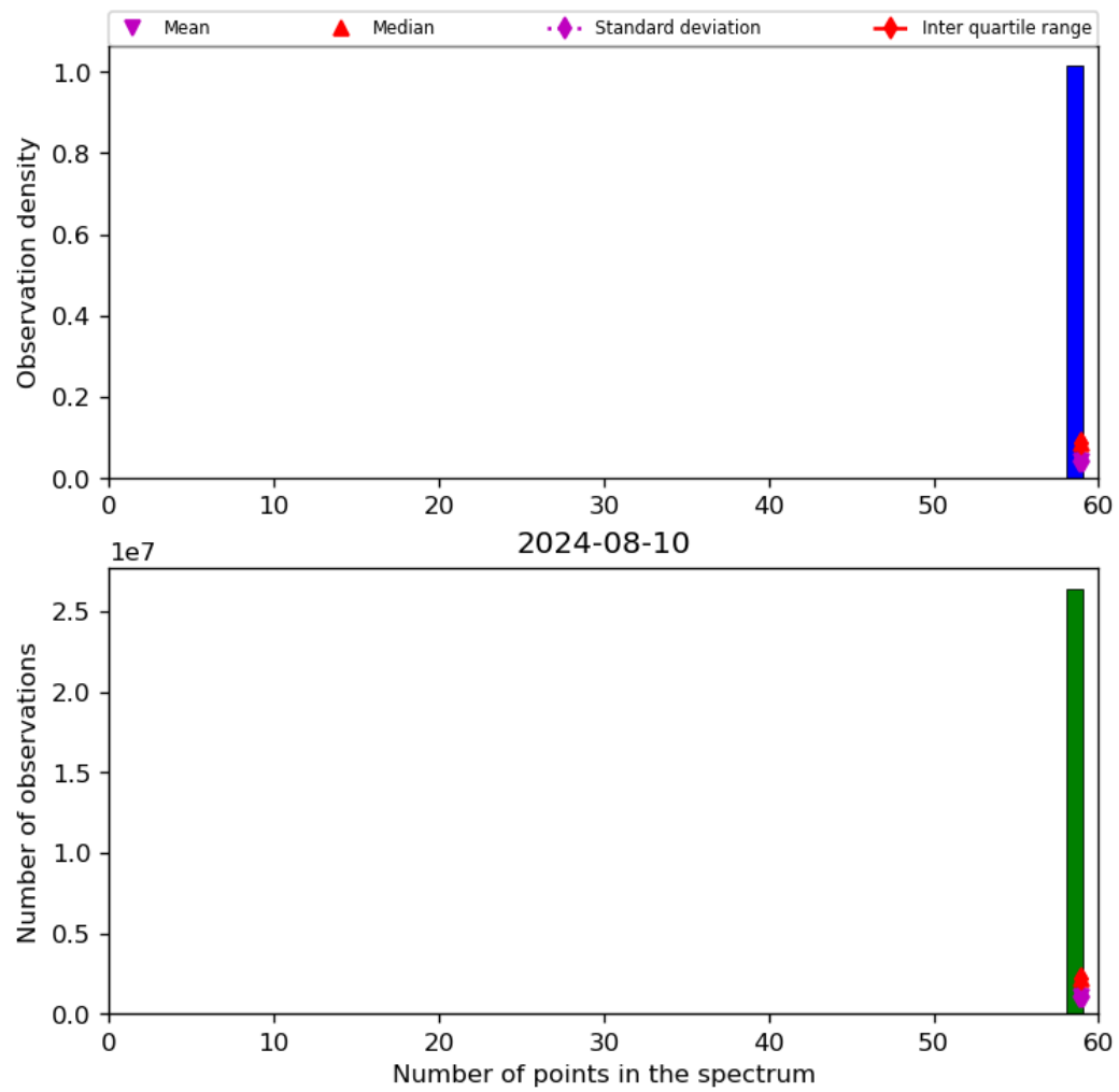
Figure 44: Histogram of “Number of points in the spectrum” for 2024-08-09 to 2024-08-11
