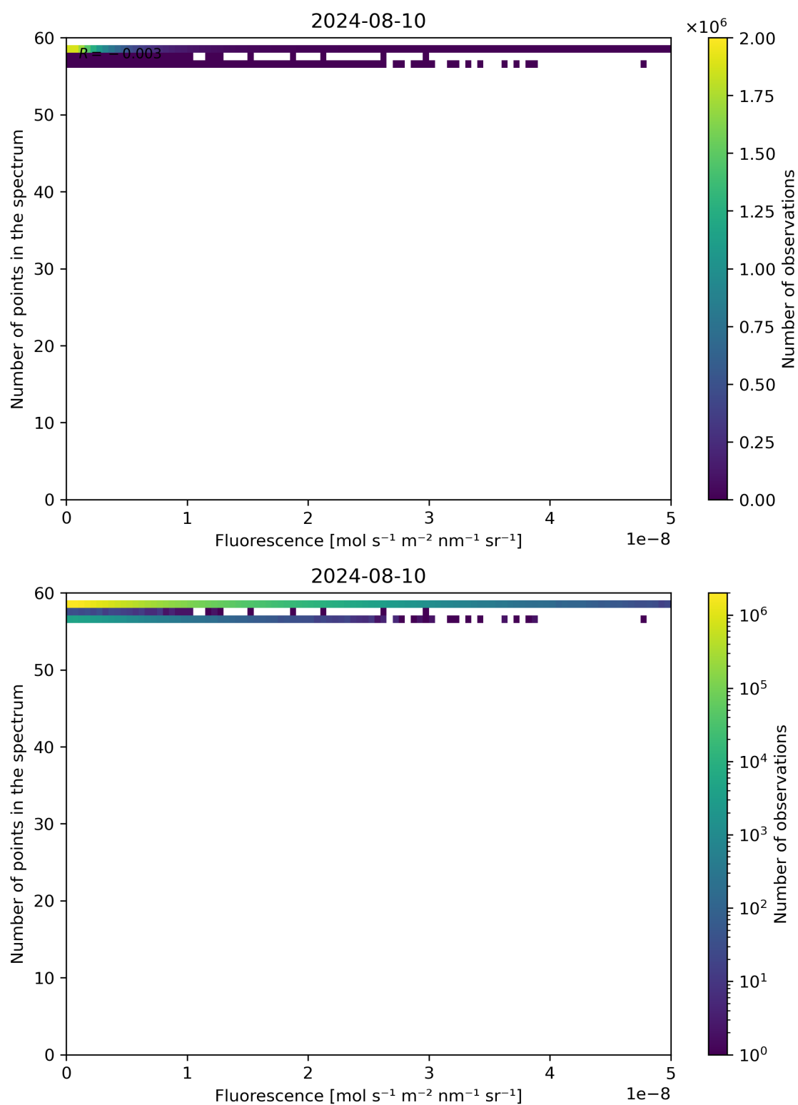
Figure 86: Scatter density plot of “Fluorescence” against “Number of points in the spectrum” for 2024-08-09 to 2024-08-11.
