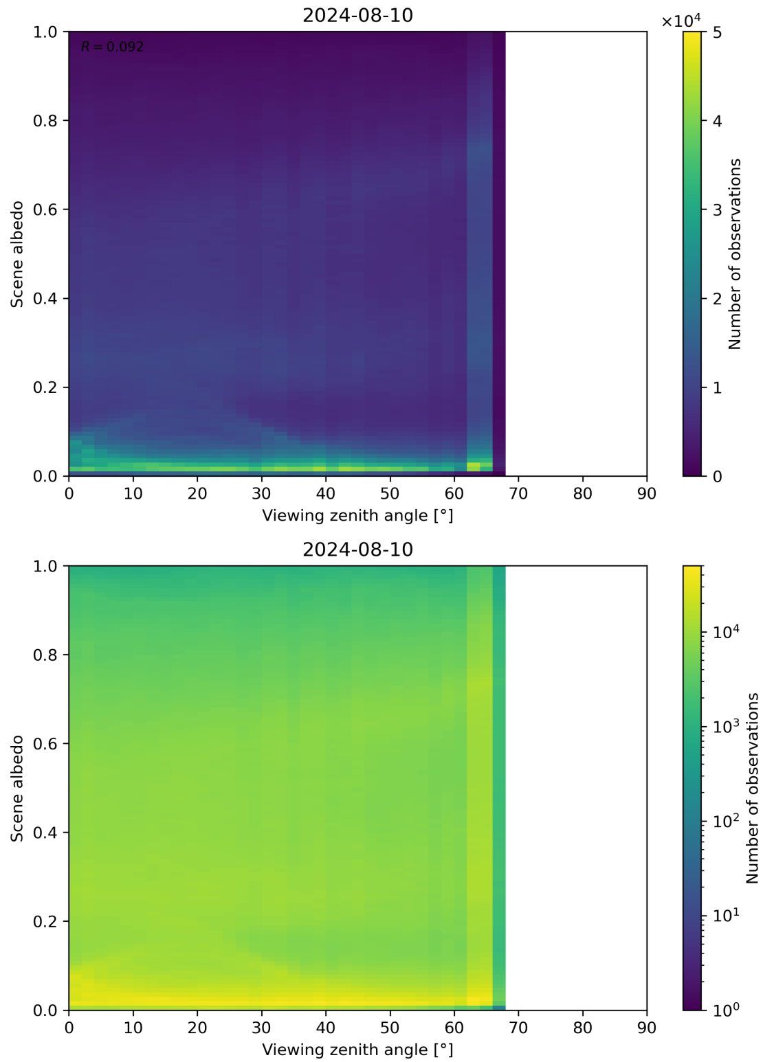
Figure 126: Scatter density plot of “Viewing zenith angle” against “Scene albedo” for 2024-08-09 to 2024-08-11.
