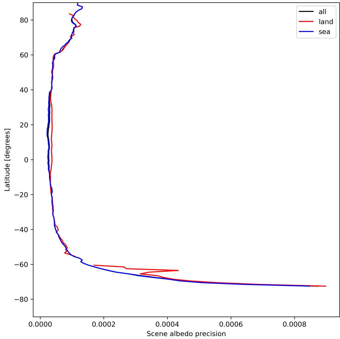
Figure 18: Zonal average of “Scene albedo precision” for 2024-08-09 to 2024-08-11.
