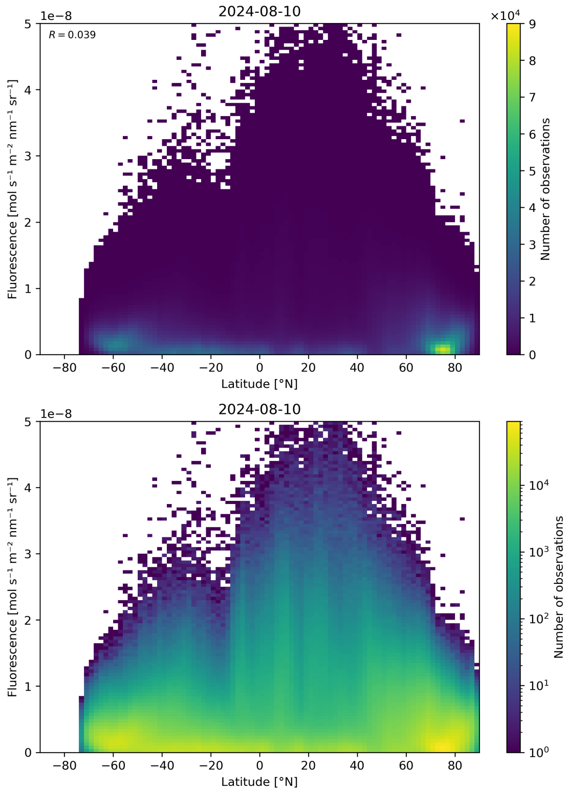
Figure 92: Scatter density plot of “Latitude” against “Fluorescence” for 2024-08-09 to 2024-08-11.
