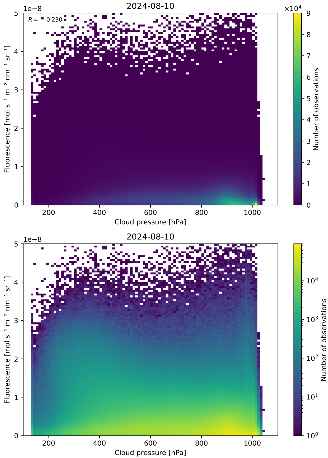
Figure 80: Scatter density plot of “Cloud pressure” against “Fluorescence” for 2024-08-09 to 2024-08-11.
