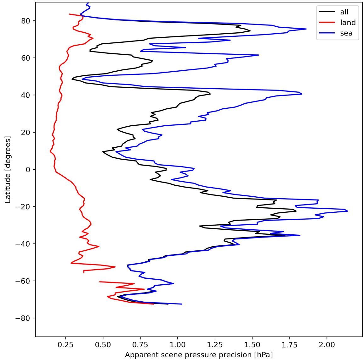
Figure 20: Zonal average of “Apparent scene pressure precision” for 2024-08-09 to 2024-08-11.
