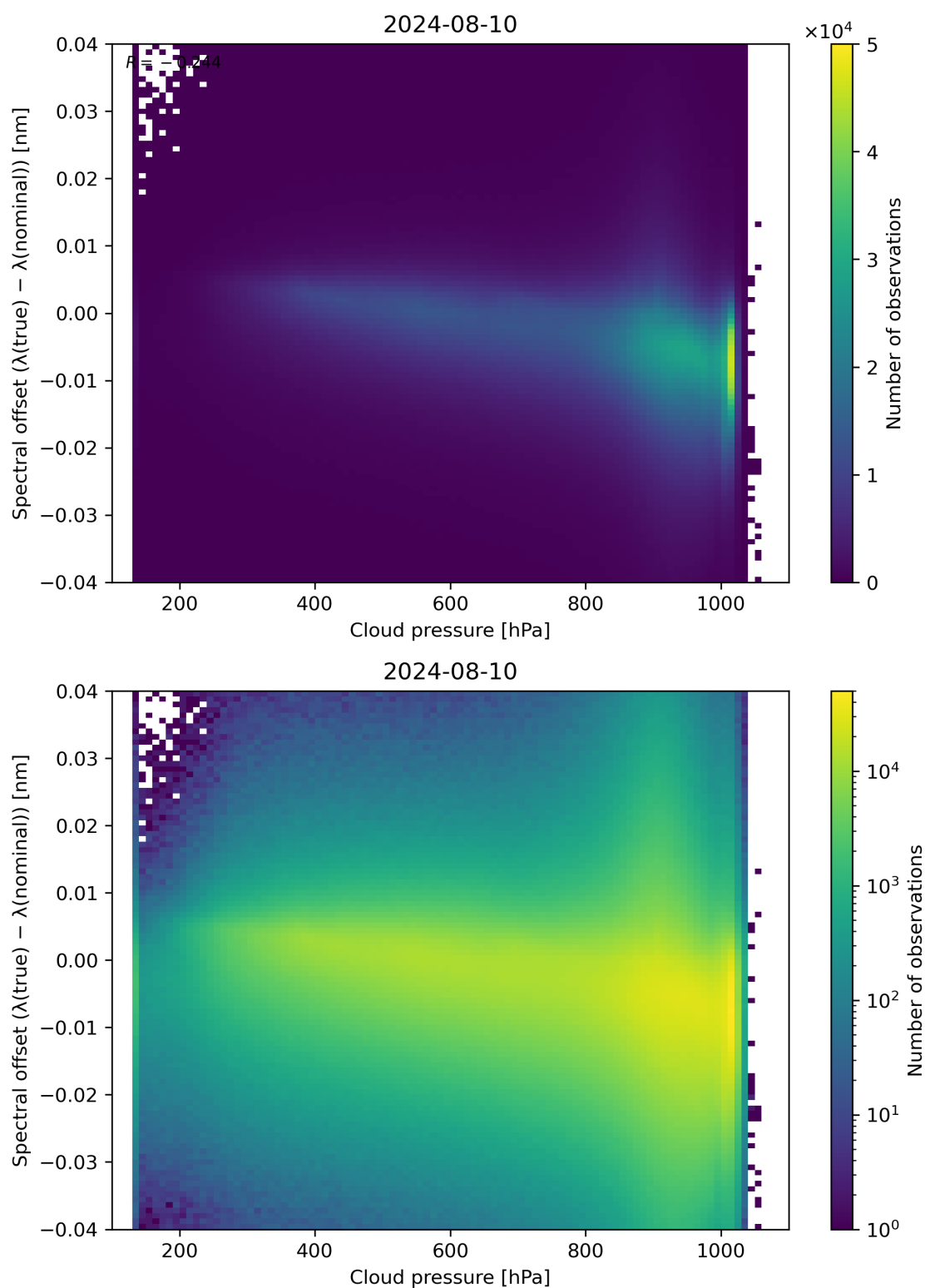
Figure 84: Scatter density plot of “Cloud pressure” against “Spectral offset ( \lambda(\text{true}) - \lambda(\text{nominal}) )” for 2024-08-09 to 2024-08-11.
