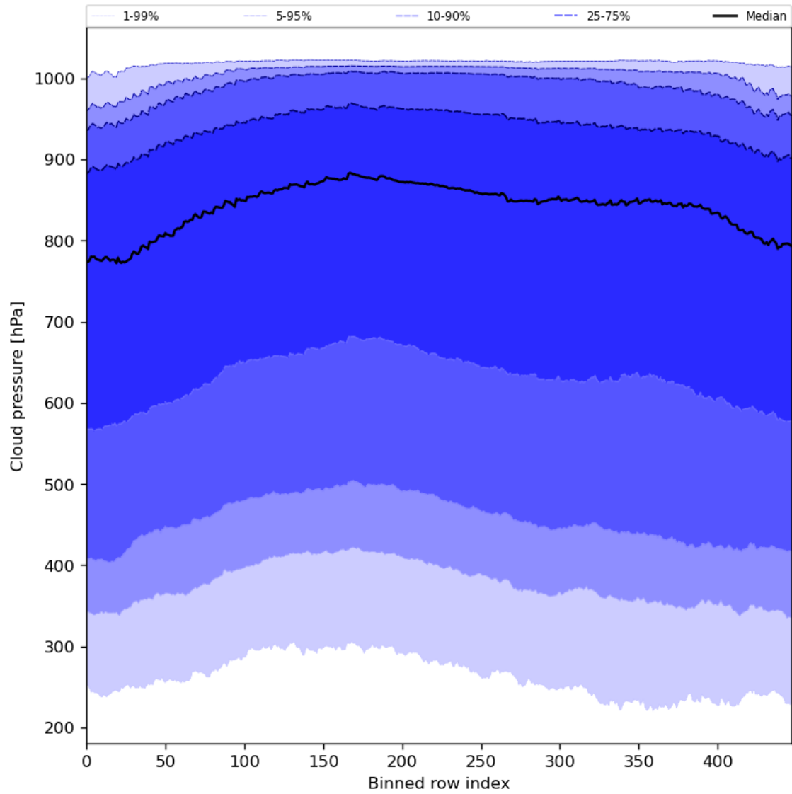
Figure 47: Along track statistics of “Cloud pressure” for 2024-08-09 to 2024-08-11
