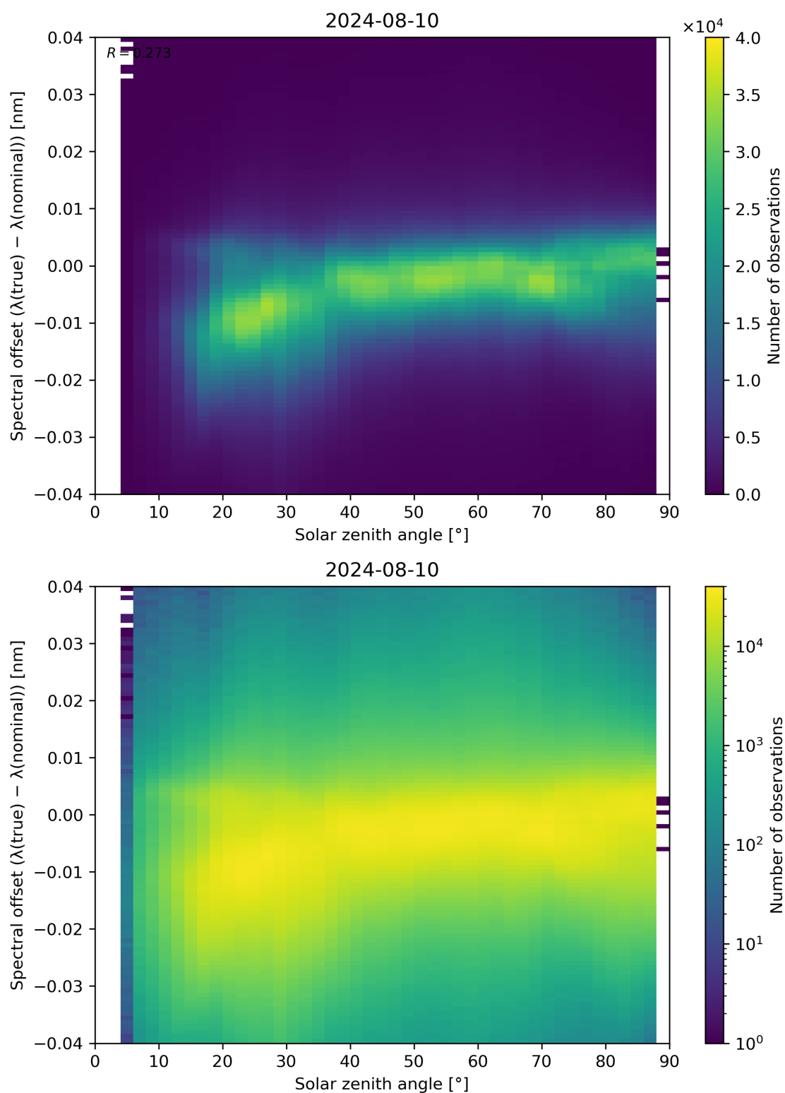
Figure 117: Scatter density plot of “Solar zenith angle” against “Spectral offset ( \lambda(\text{true}) - \lambda(\text{nominal}) )” for 2024-08-09 to 2024-08-11.
