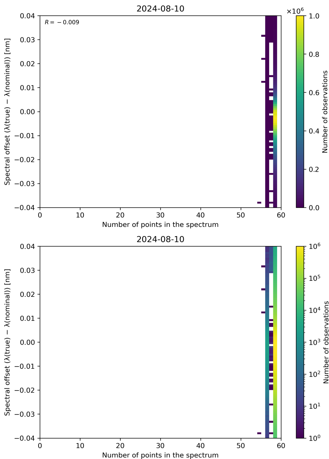
Figure 101: Scatter density plot of “Number of points in the spectrum” against “Spectral offset ( \lambda(\text{true}) - \lambda(\text{nominal}) )” for 2024-08-09 to 2024-08-11.
