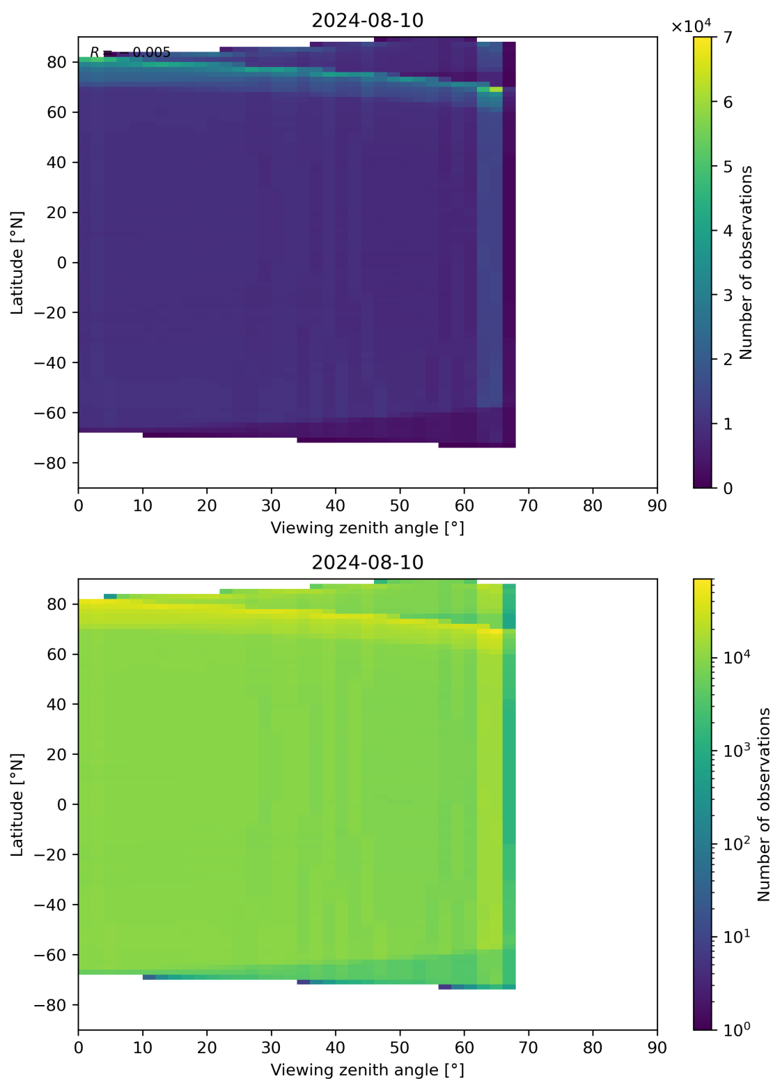
Figure 123: Scatter density plot of “Viewing zenith angle” against “Latitude” for 2024-08-09 to 2024-08-11.
