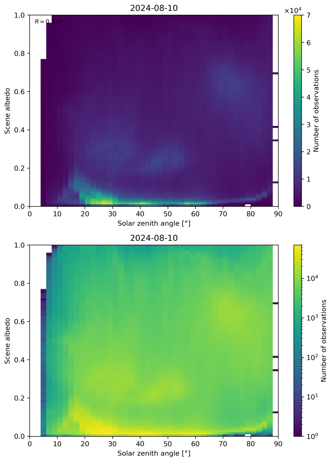
Figure 116: Scatter density plot of “Solar zenith angle” against “Scene albedo” for 2024-08-09 to 2024-08-11.
