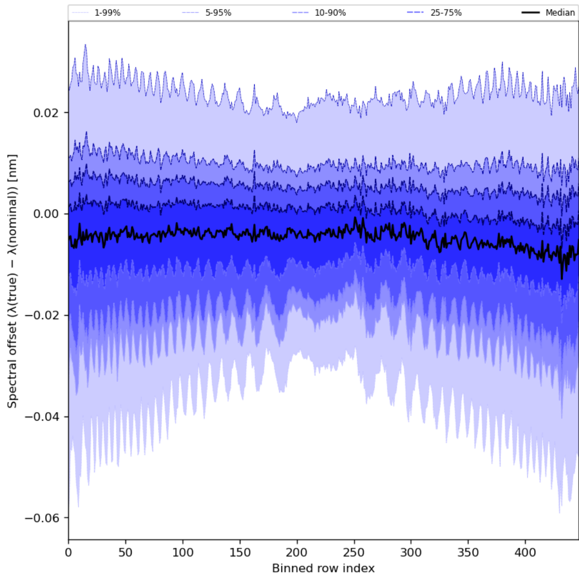
Figure 62: Along track statistics of “Spectral offset ( \lambda(\text{true}) - \lambda(\text{nominal}) )” for 2024-08-09 to 2024-08-11
