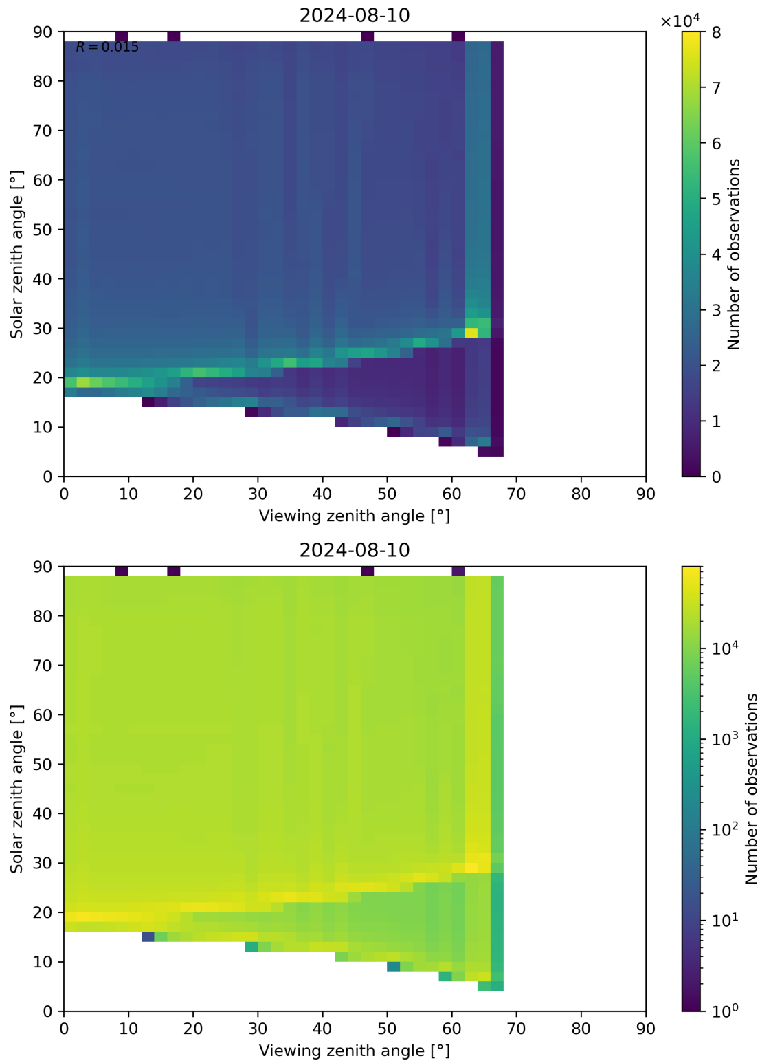
Figure 127: Scatter density plot of “Viewing zenith angle” against “Solar zenith angle” for 2024-08-09 to 2024-08-11.
