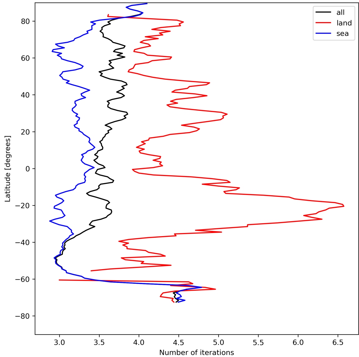
Figure 22: Zonal average of “Number of iterations” for 2024-08-09 to 2024-08-11.
