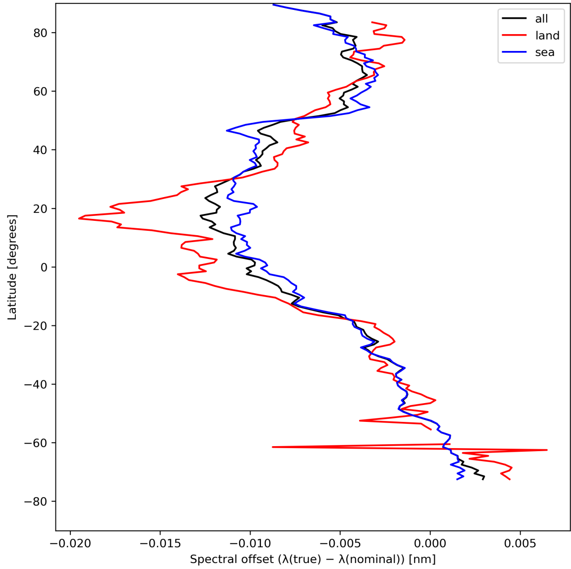
Figure 28: Zonal average of “Spectral offset ( \lambda(\text{true}) - \lambda(\text{nominal}) )” for 2024-08-09 to 2024-08-11.
