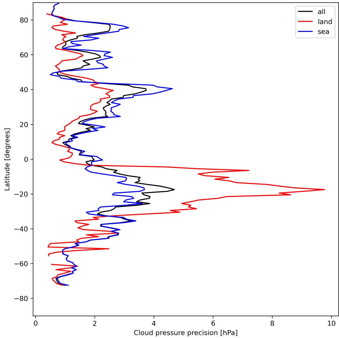
Figure 14: Zonal average of “Cloud pressure precision” for 2024-08-09 to 2024-08-11.
