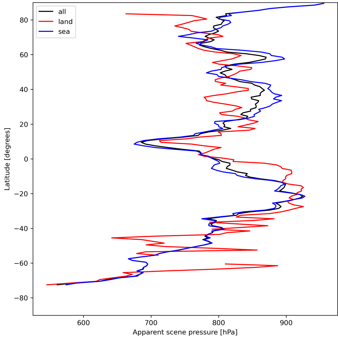
Figure 19: Zonal average of “Apparent scene pressure” for 2024-08-09 to 2024-08-11.
