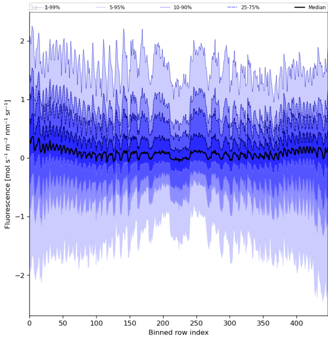
Figure 57: Along track statistics of “Fluorescence” for 2024-08-09 to 2024-08-11
