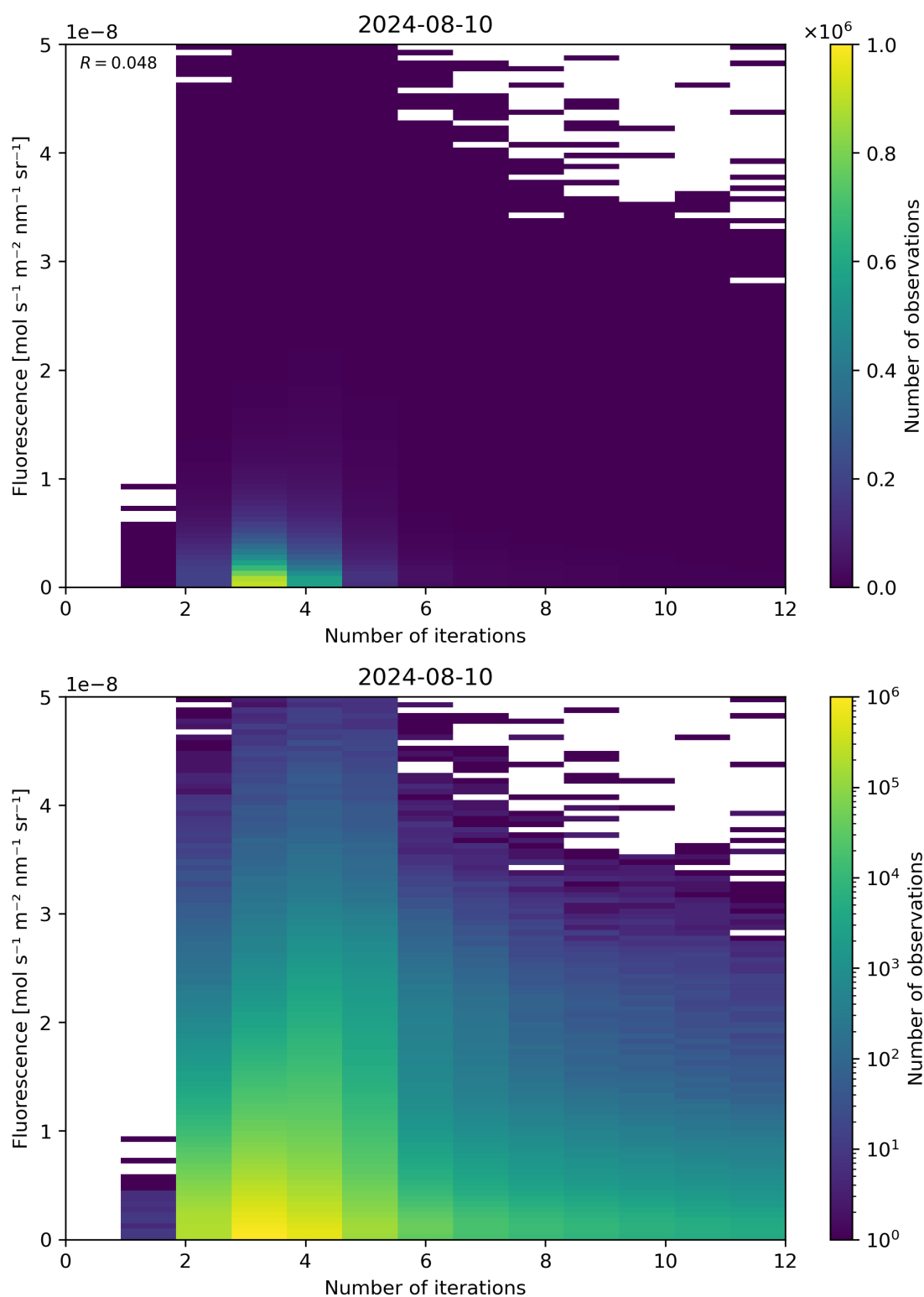
Figure 98: Scatter density plot of “Number of iterations” against “Fluorescence” for 2024-08-09 to 2024-08-11.
