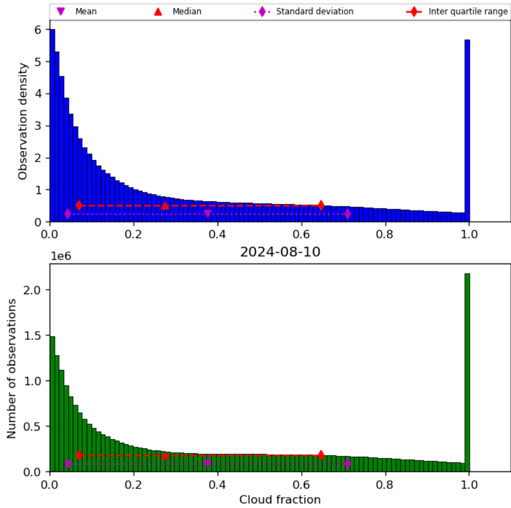
Figure 32: Histogram of “Cloud fraction” for 2024-08-09 to 2024-08-11
