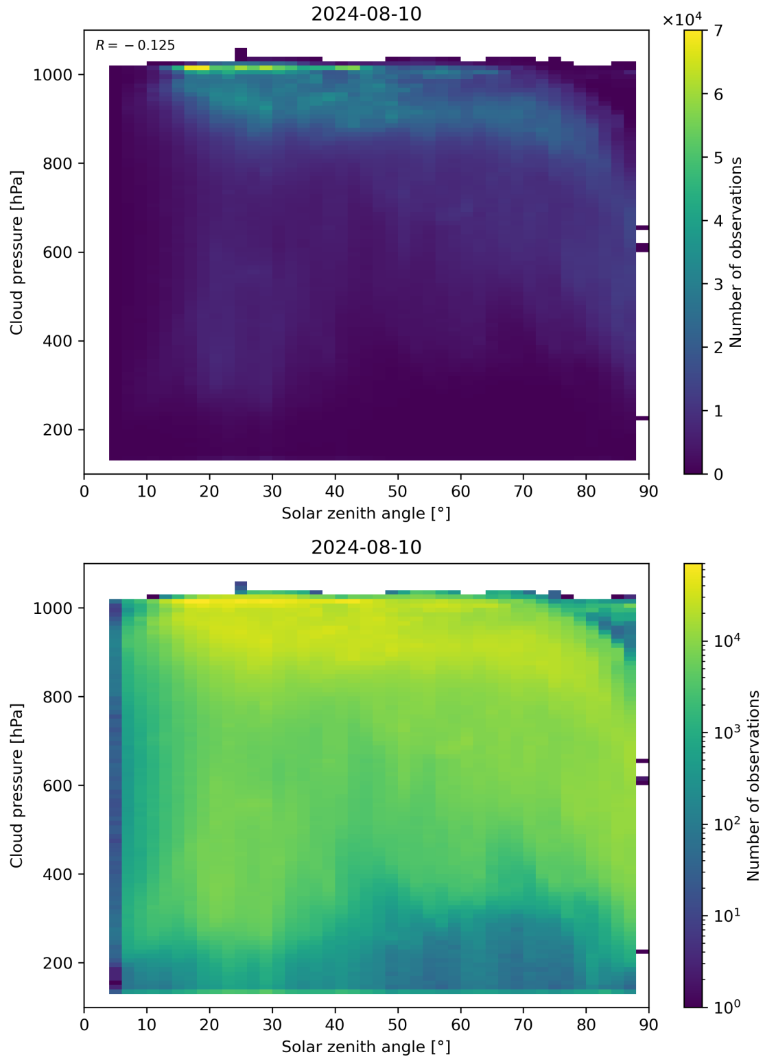
Figure 111: Scatter density plot of “Solar zenith angle” against “Cloud pressure” for 2024-08-09 to 2024-08-11.
