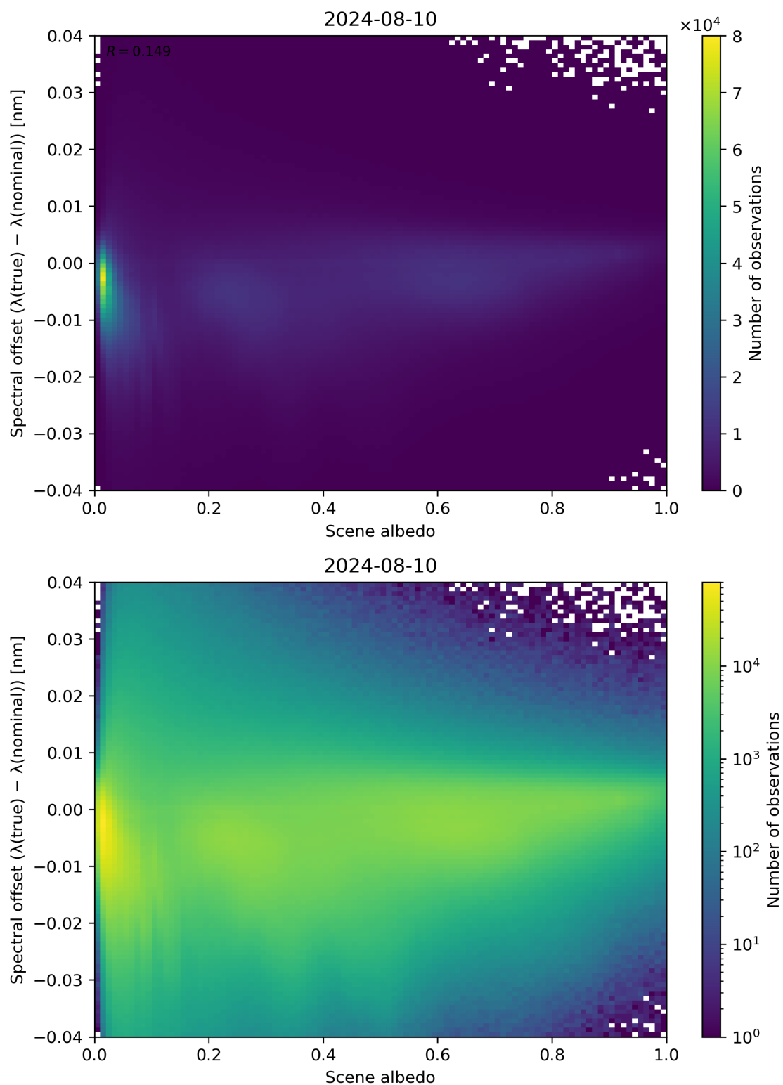
Figure 107: Scatter density plot of “Scene albedo” against “Spectral offset ( \lambda(\text{true}) - \lambda(\text{nominal}) )” for 2024-08-09 to 2024-08-11.
