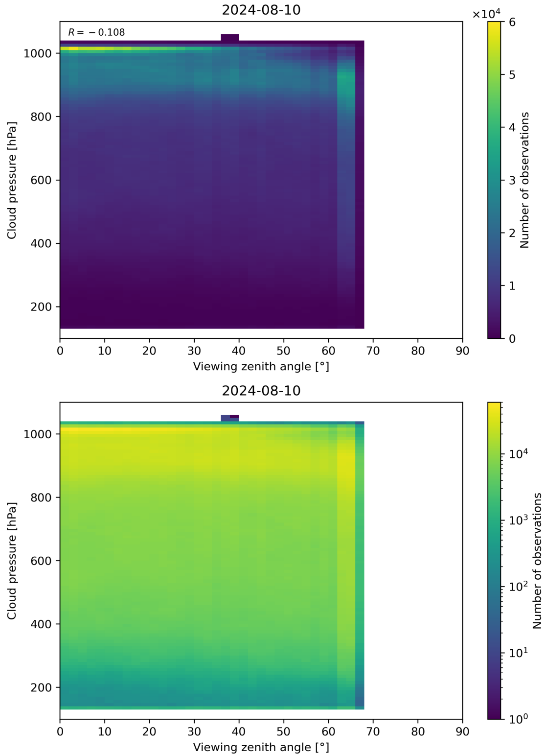
Figure 121: Scatter density plot of “Viewing zenith angle” against “Cloud pressure” for 2024-08-09 to 2024-08-11.
