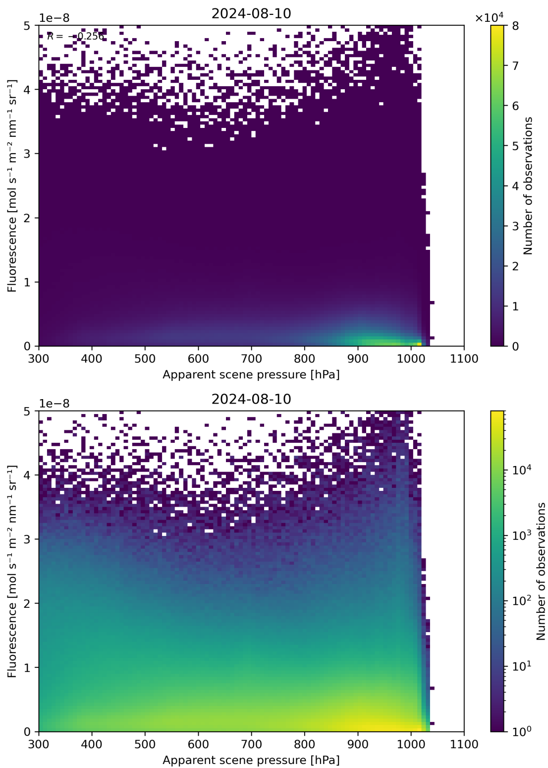
Figure 64: Scatter density plot of “Apparent scene pressure” against “Fluorescence” for 2024-08-09 to 2024-08-11.
