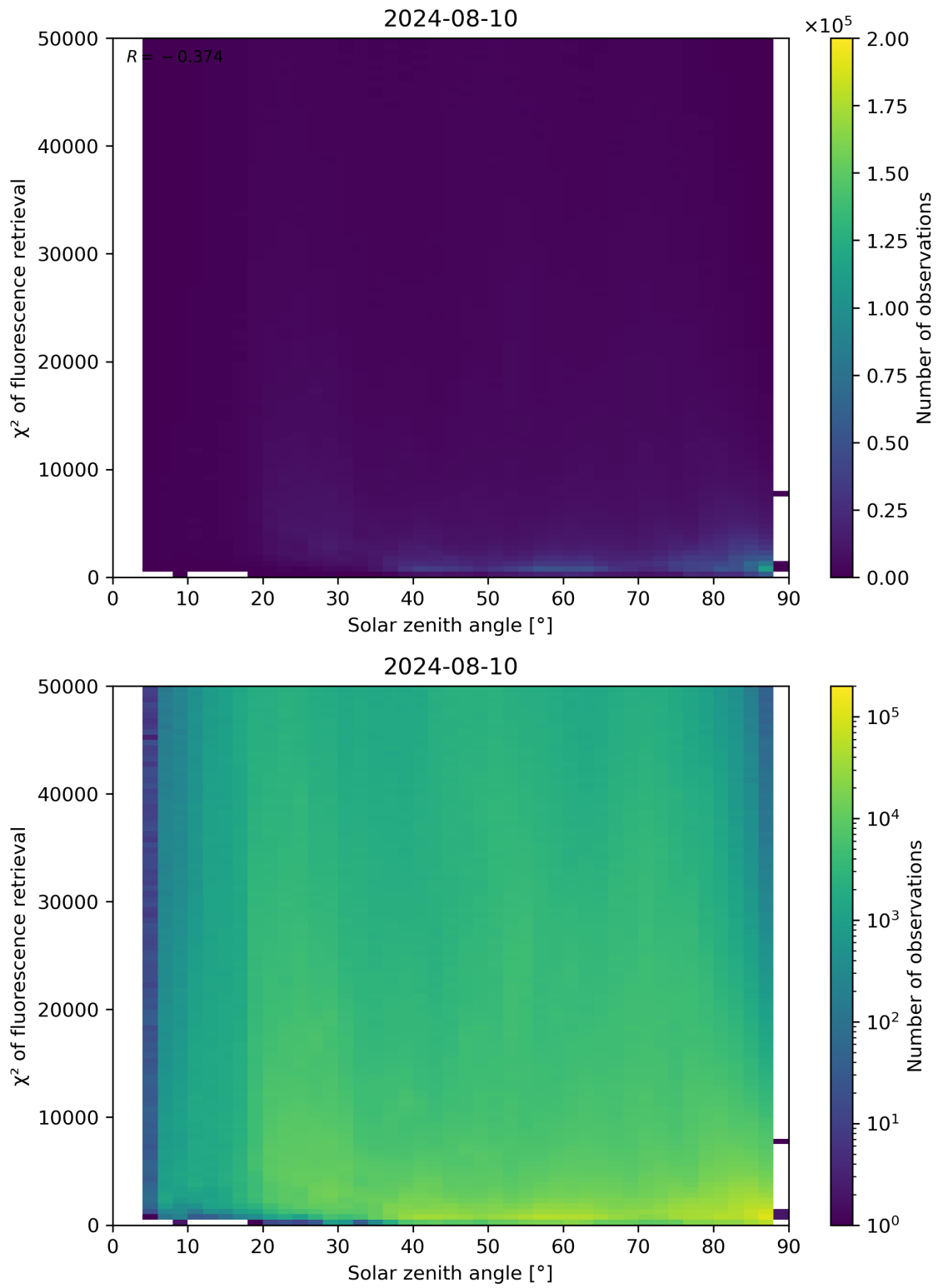
Figure 109: Scatter density plot of “Solar zenith angle” against “ \chi^2 of fluorescence retrieval” for 2024-08-09 to 2024-08-11.
