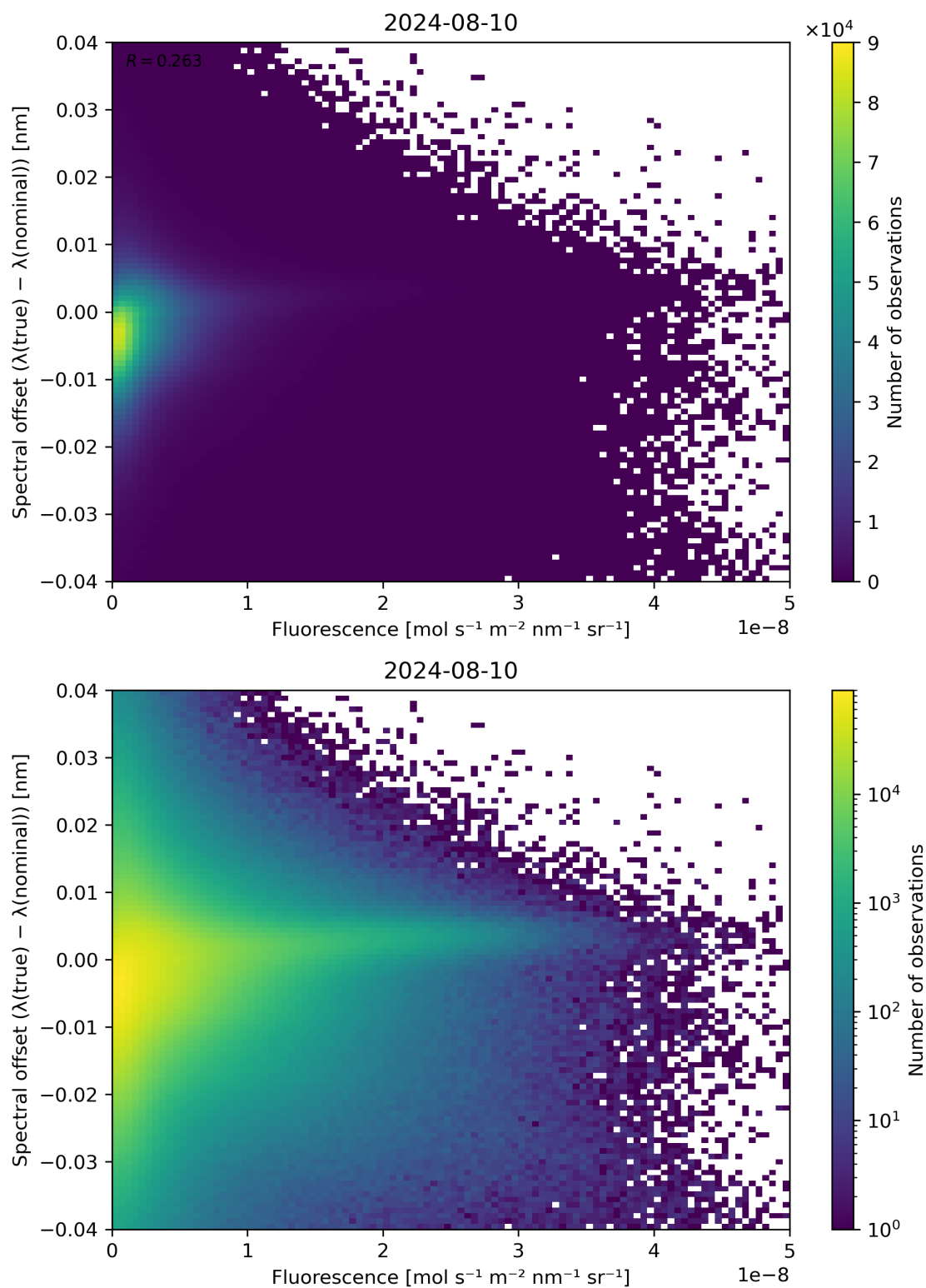
Figure 87: Scatter density plot of “Fluorescence” against “Spectral offset ( \lambda(\text{true}) - \lambda(\text{nominal}) )” for 2024-08-09 to 2024-08-11.
