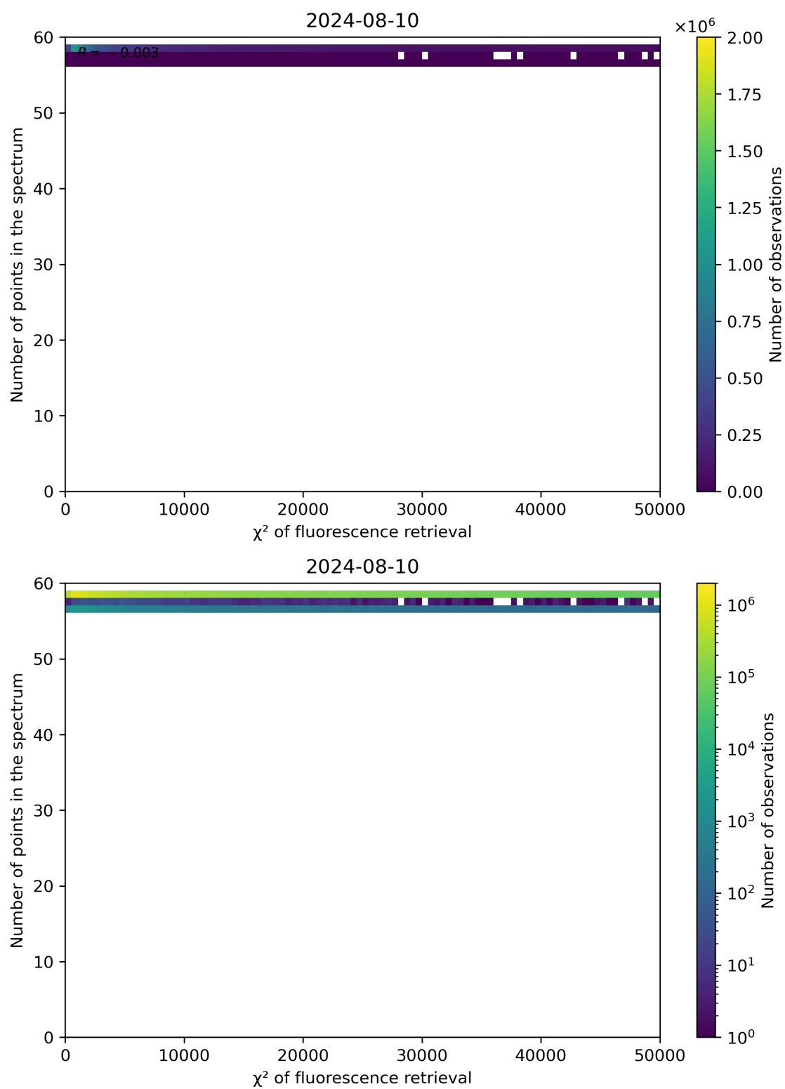
Figure 68: Scatter density plot of " \chi^2 of fluorescence retrieval" against "Number of points in the spectrum" for 2024-08-09 to 2024-08-11.
