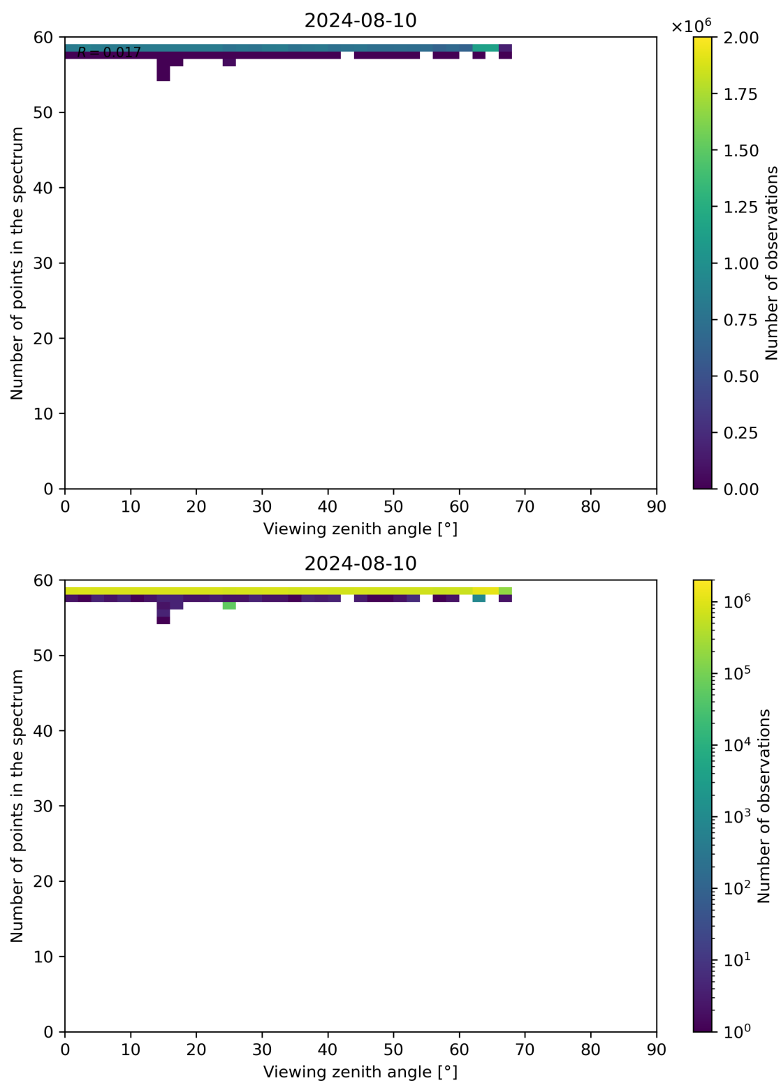
Figure 125: Scatter density plot of “Viewing zenith angle” against “Number of points in the spectrum” for 2024-08-09 to 2024-08-11.
