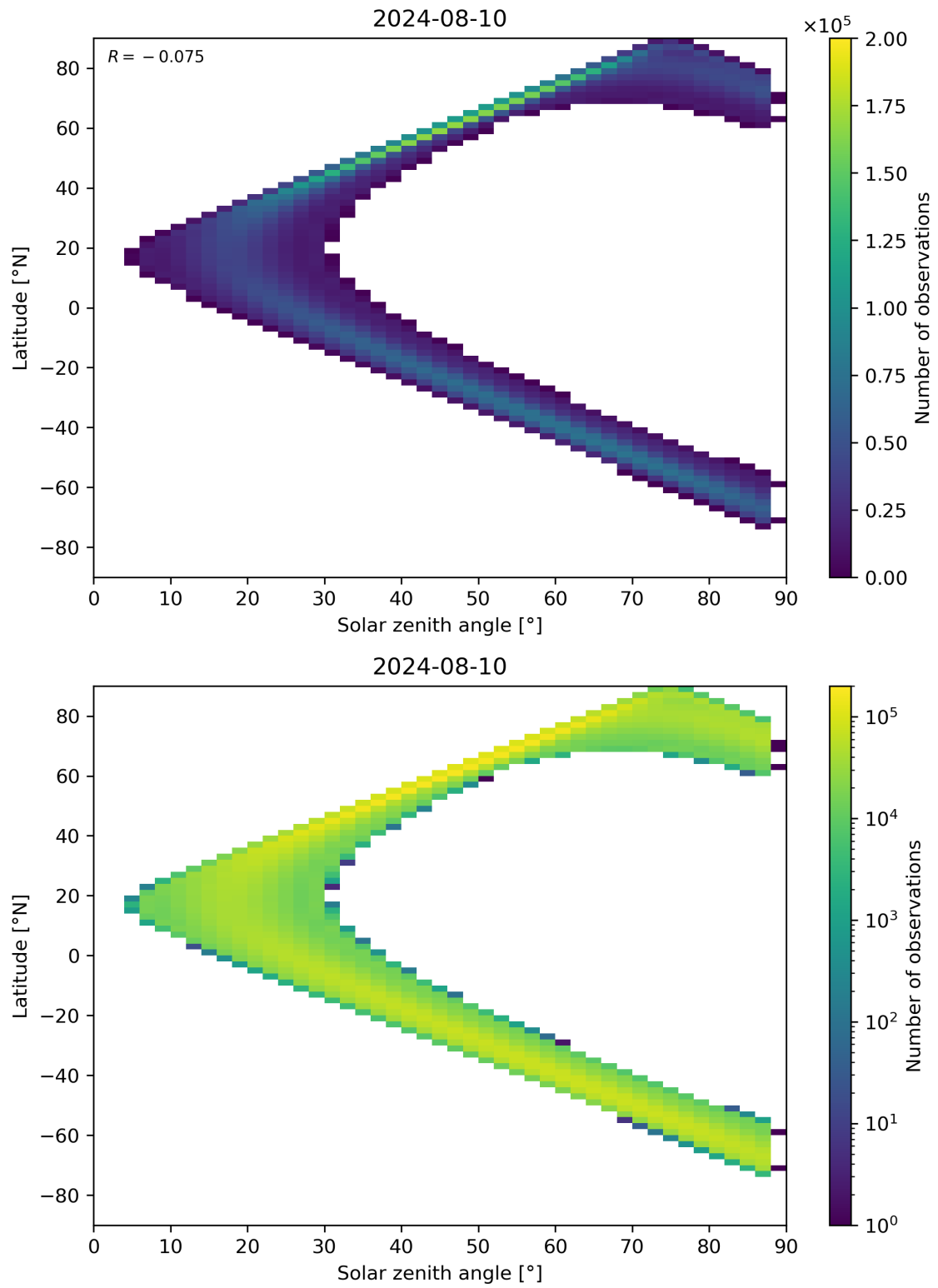
Figure 113: Scatter density plot of “Solar zenith angle” against “Latitude” for 2024-08-09 to 2024-08-11.
