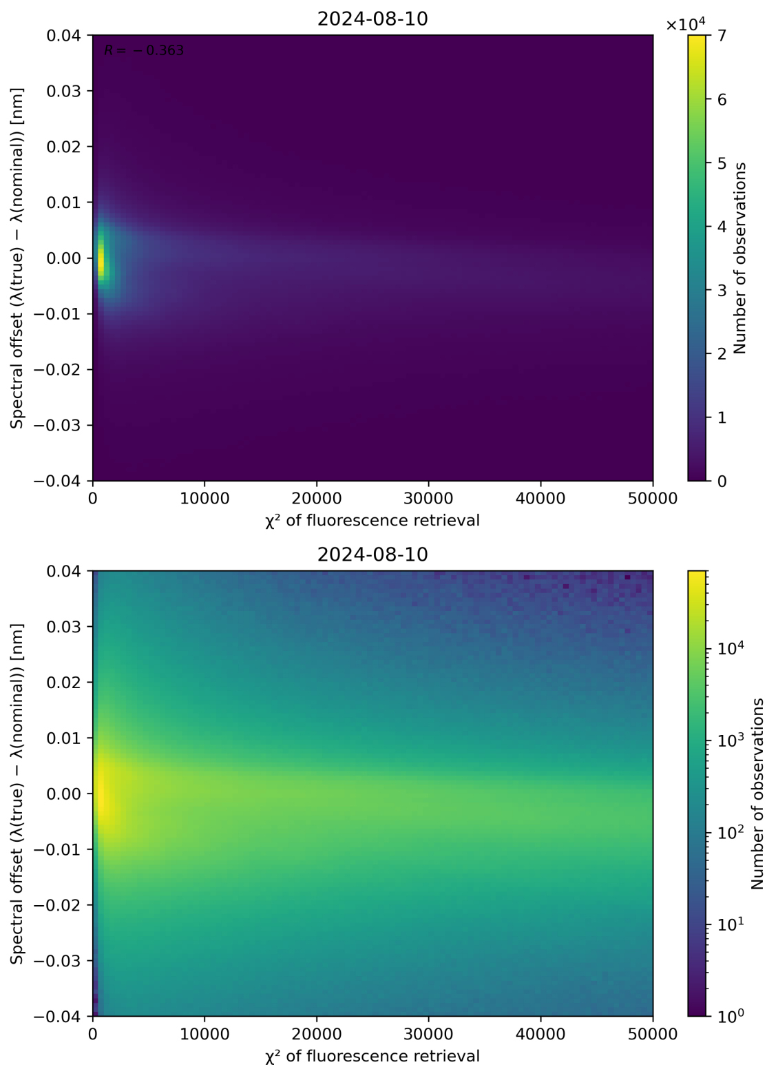
Figure 69: Scatter density plot of “ \chi^2 of fluorescence retrieval” against “Spectral offset ( \lambda(\text{true}) - \lambda(\text{nominal}) )” for 2024-08-09 to 2024-08-11.
