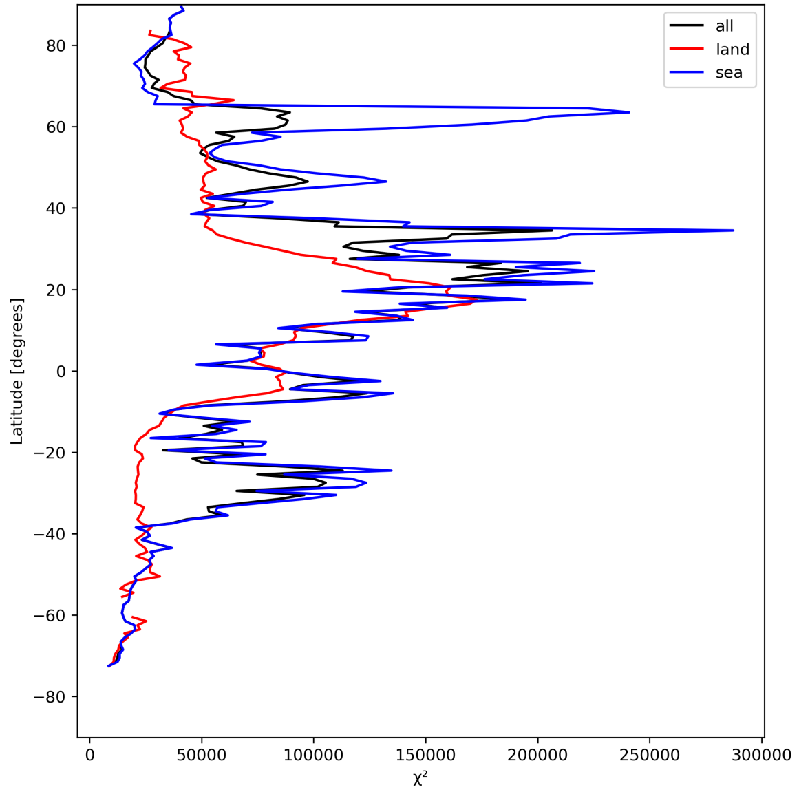
Figure 21: Zonal average of “ \chi^2 ” for 2024-08-09 to 2024-08-11.
