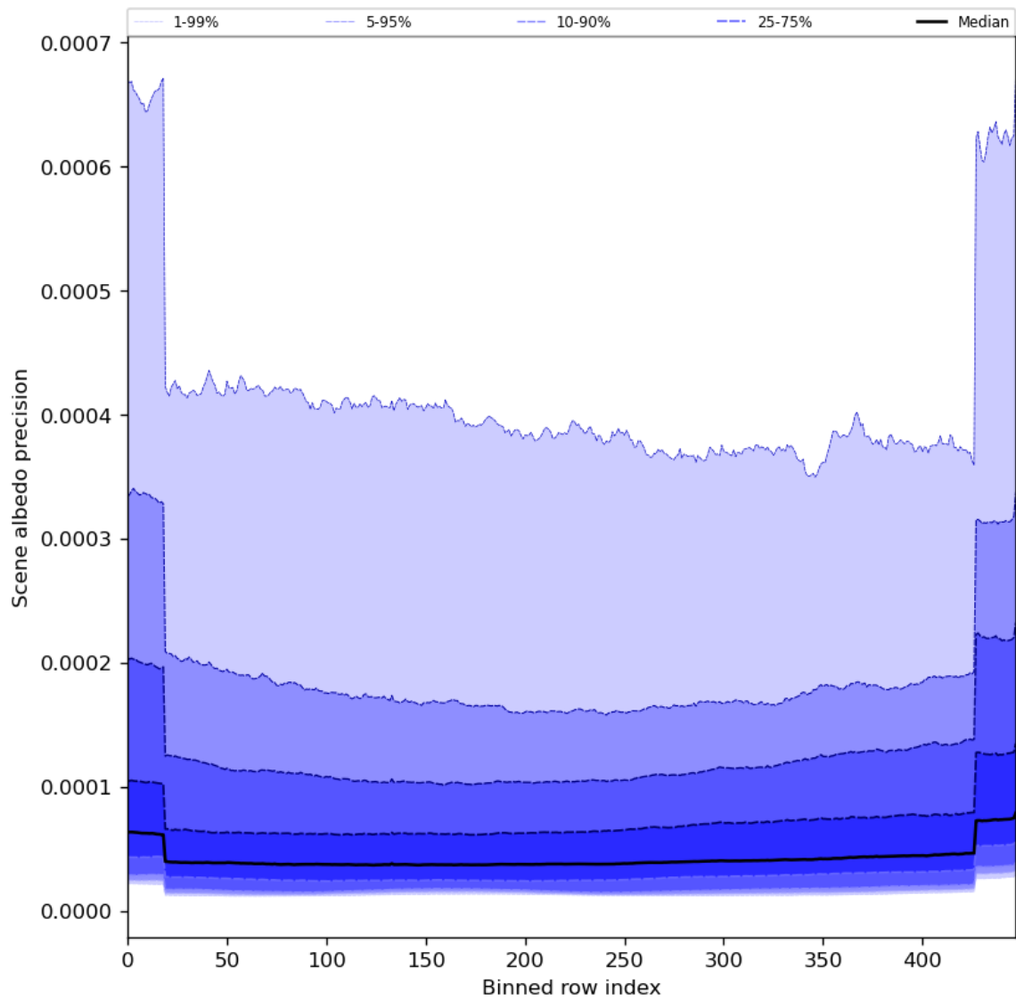
Figure 52: Along track statistics of “Scene albedo precision” for 2024-08-09 to 2024-08-11
