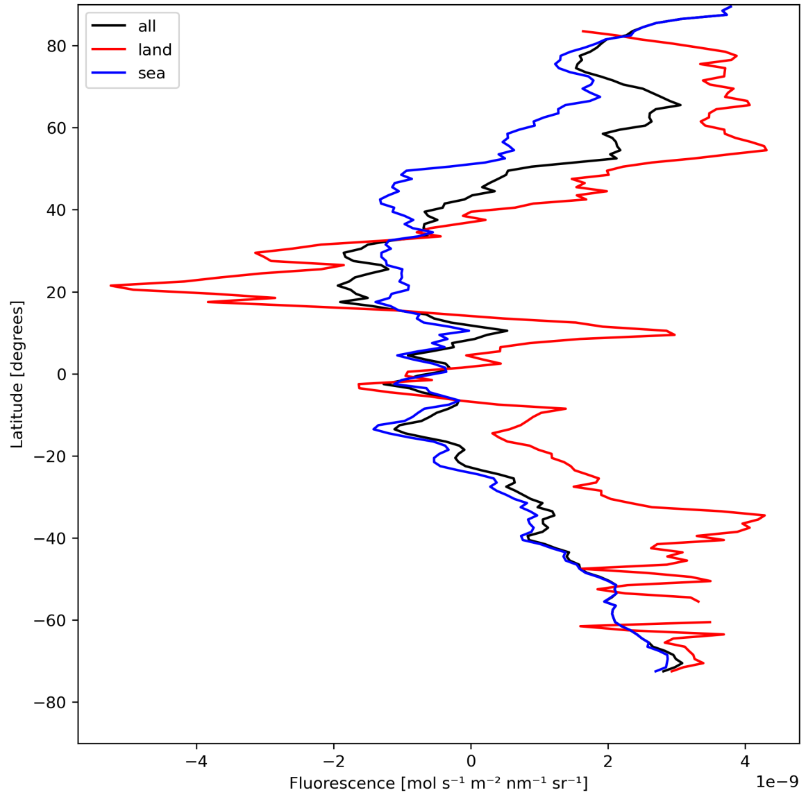
Figure 23: Zonal average of “Fluorescence” for 2024-08-09 to 2024-08-11.
