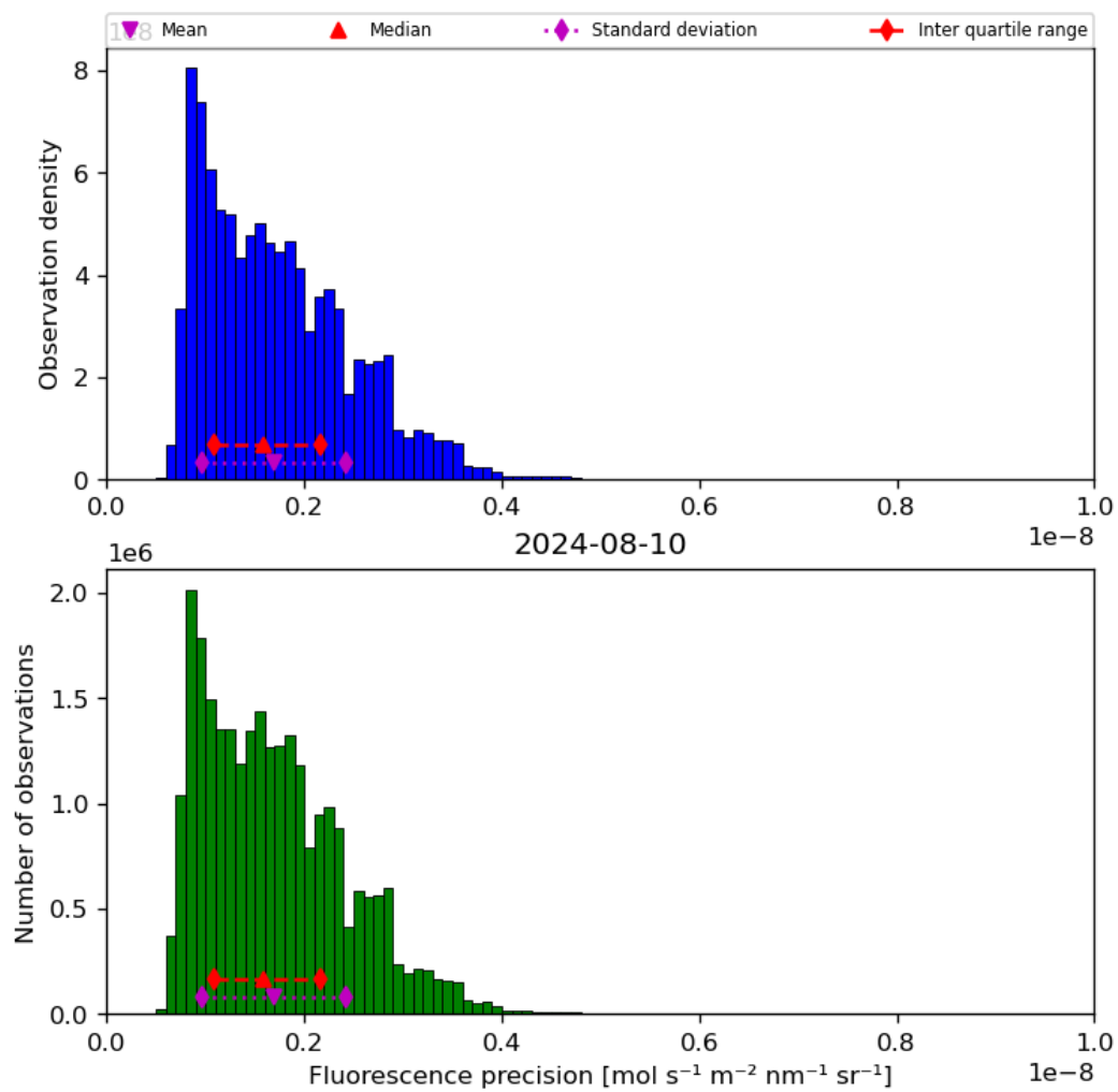
Figure 41: Histogram of “Fluorescence precision” for 2024-08-09 to 2024-08-11
