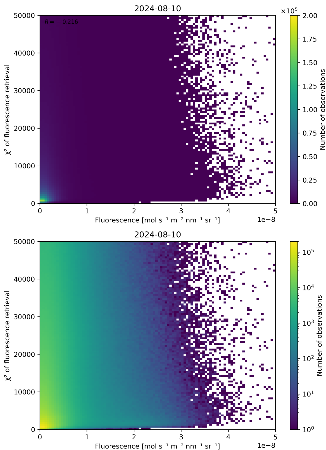
Figure 85: Scatter density plot of “Fluorescence” against “ \chi^2 of fluorescence retrieval” for 2024-08-09 to 2024-08-11.
