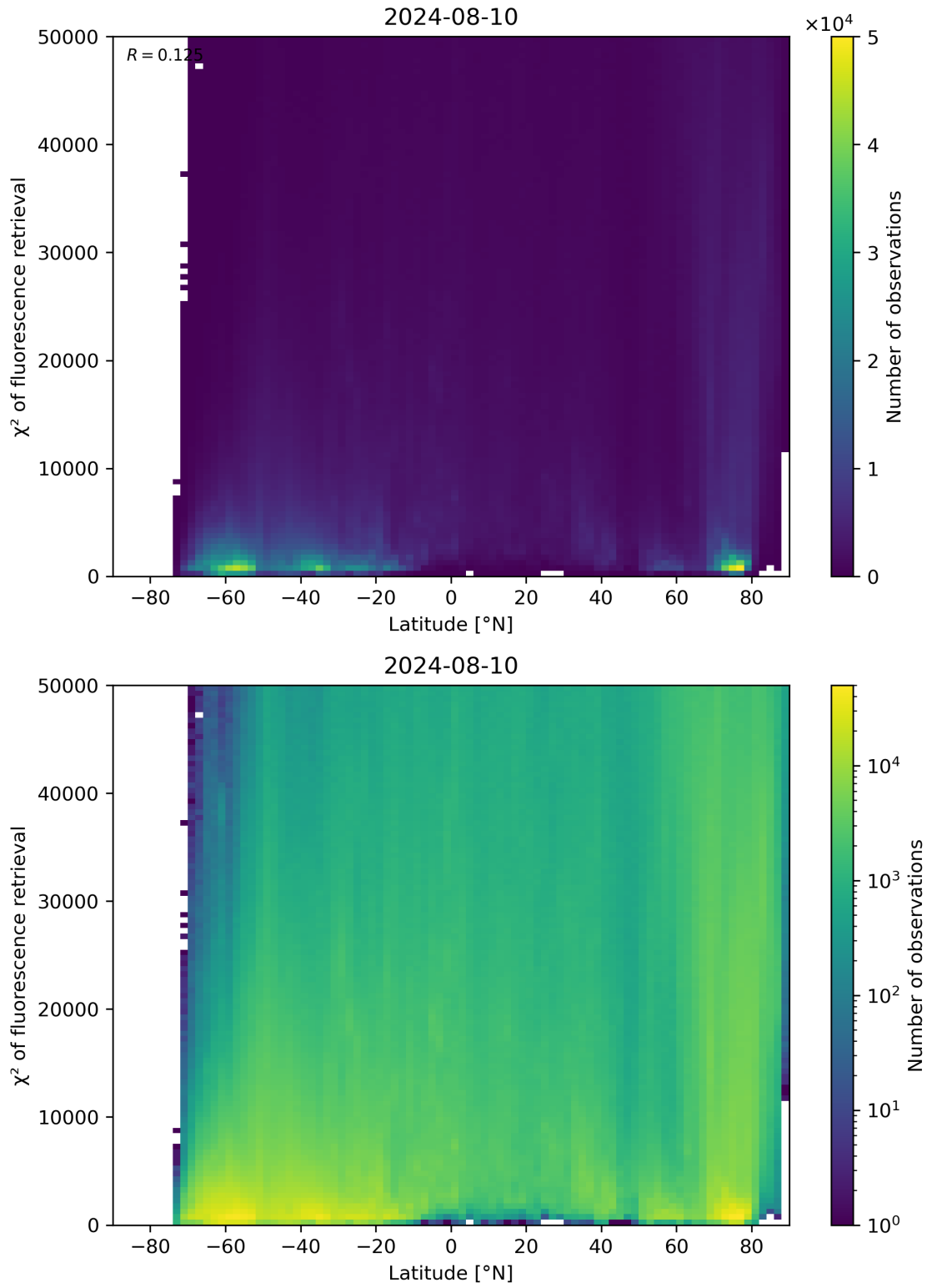
Figure 89: Scatter density plot of “Latitude” against “ \chi^2 of fluorescence retrieval” for 2024-08-09 to 2024-08-11.
