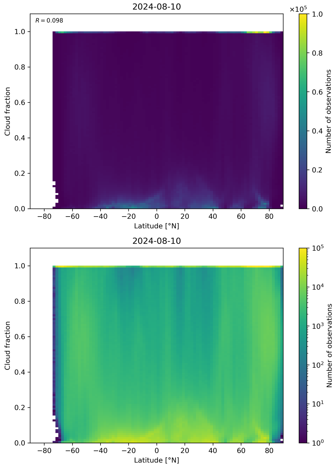
Figure 90: Scatter density plot of “Latitude” against “Cloud fraction” for 2024-08-09 to 2024-08-11.
