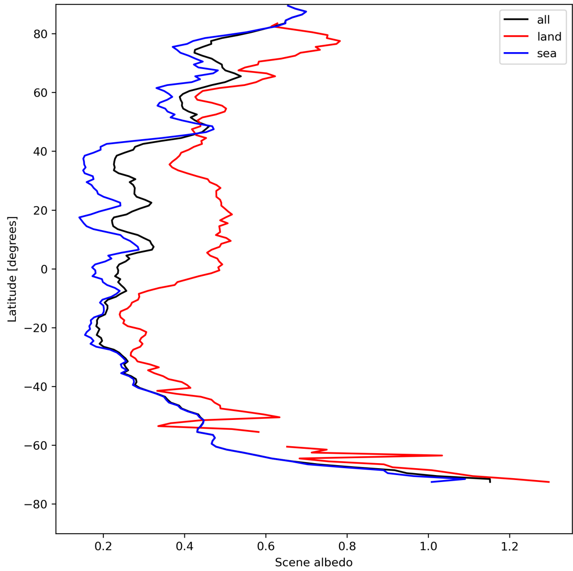
Figure 17: Zonal average of “Scene albedo” for 2024-08-09 to 2024-08-11.
