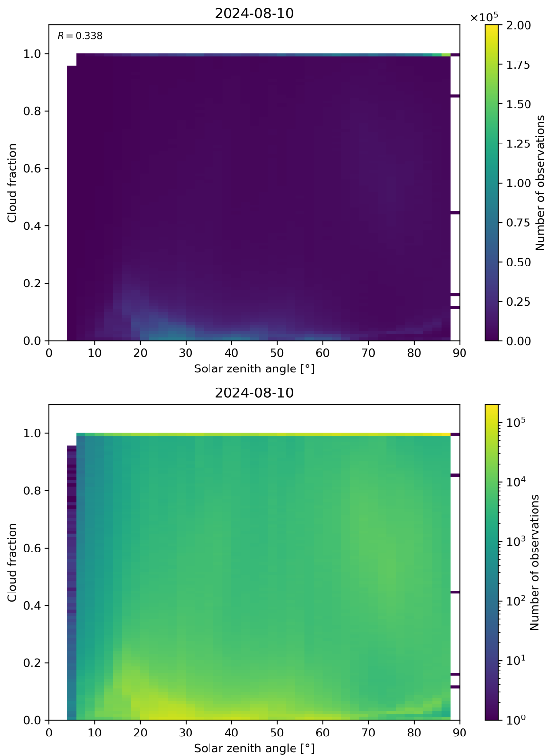
Figure 110: Scatter density plot of “Solar zenith angle” against “Cloud fraction” for 2024-08-09 to 2024-08-11.
