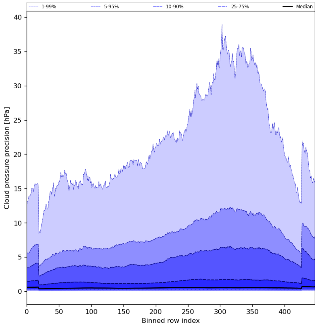
Figure 48: Along track statistics of “Cloud pressure precision” for 2024-08-09 to 2024-08-11
