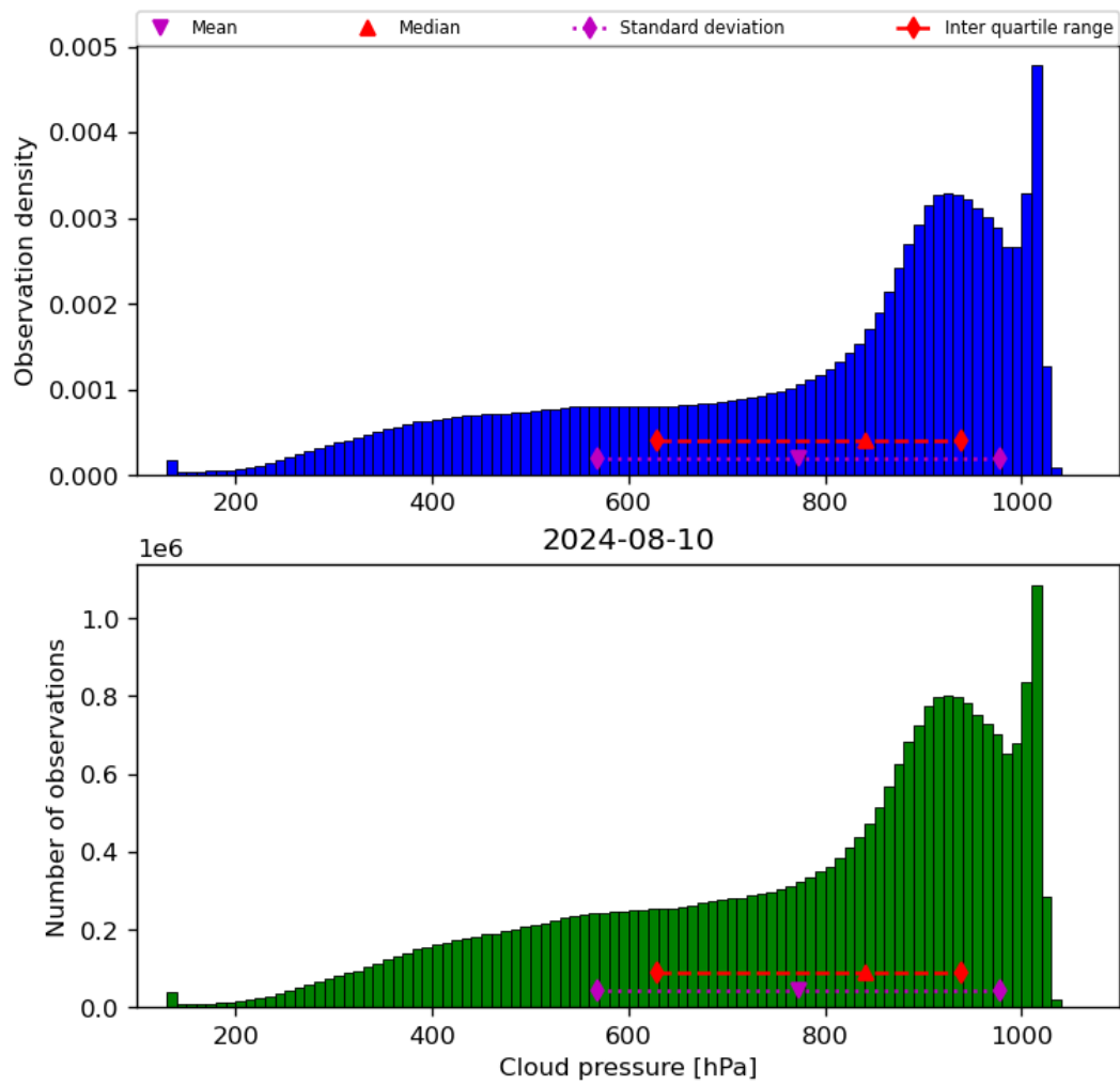
Figure 30: Histogram of “Cloud pressure” for 2024-08-09 to 2024-08-11
