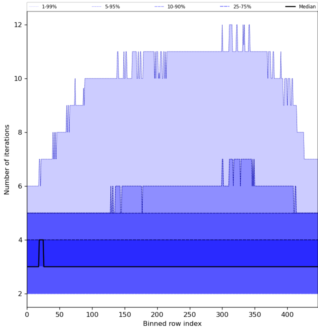
Figure 56: Along track statistics of “Number of iterations” for 2024-08-09 to 2024-08-11
