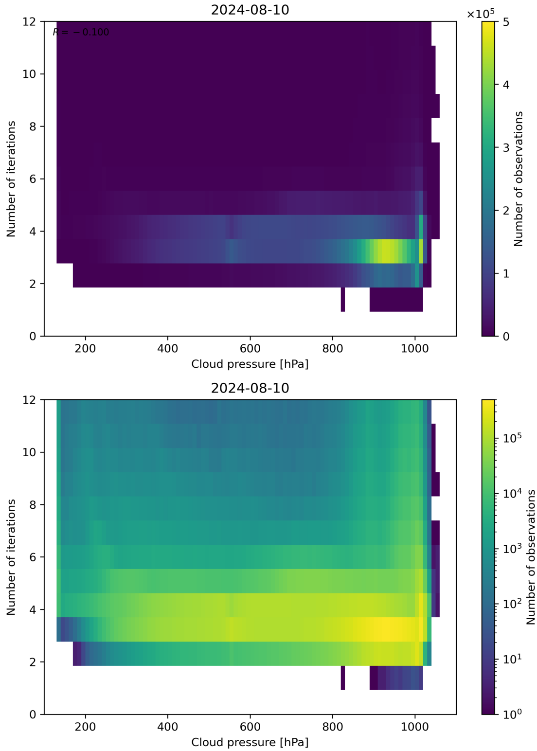
Figure 81: Scatter density plot of “Cloud pressure” against “Number of iterations” for 2024-08-09 to 2024-08-11.
