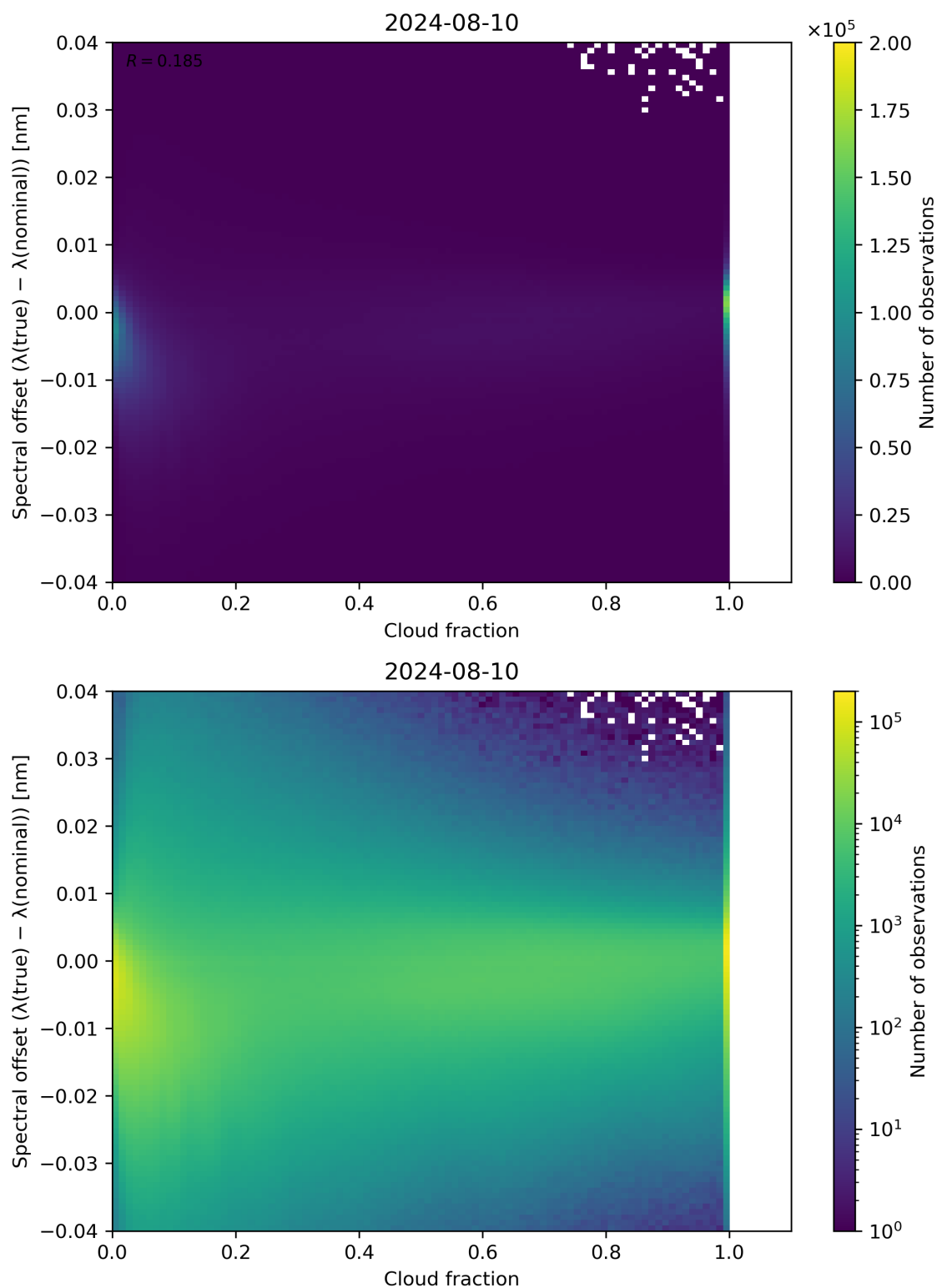
Figure 76: Scatter density plot of “Cloud fraction” against “Spectral offset ( \lambda(\text{true}) - \lambda(\text{nominal}) )” for 2024-08-09 to 2024-08-11.
