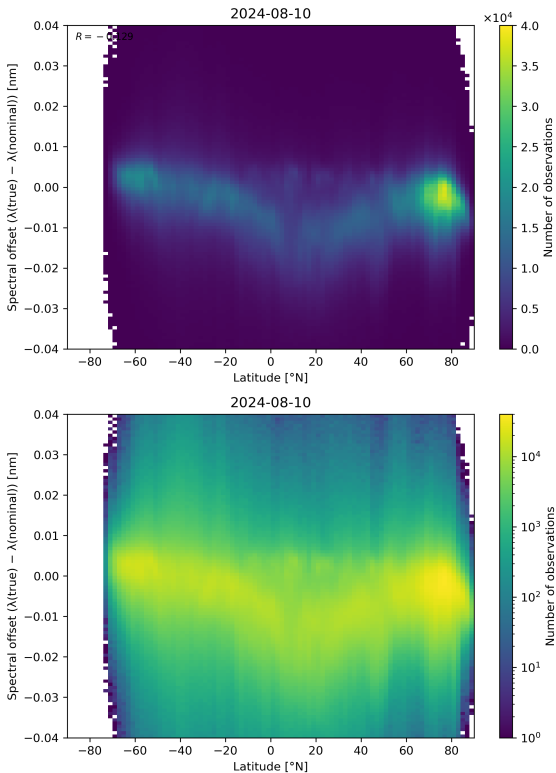
Figure 96: Scatter density plot of “Latitude” against “Spectral offset ( \lambda(\text{true}) - \lambda(\text{nominal}) )” for 2024-08-09 to 2024-08-11.
