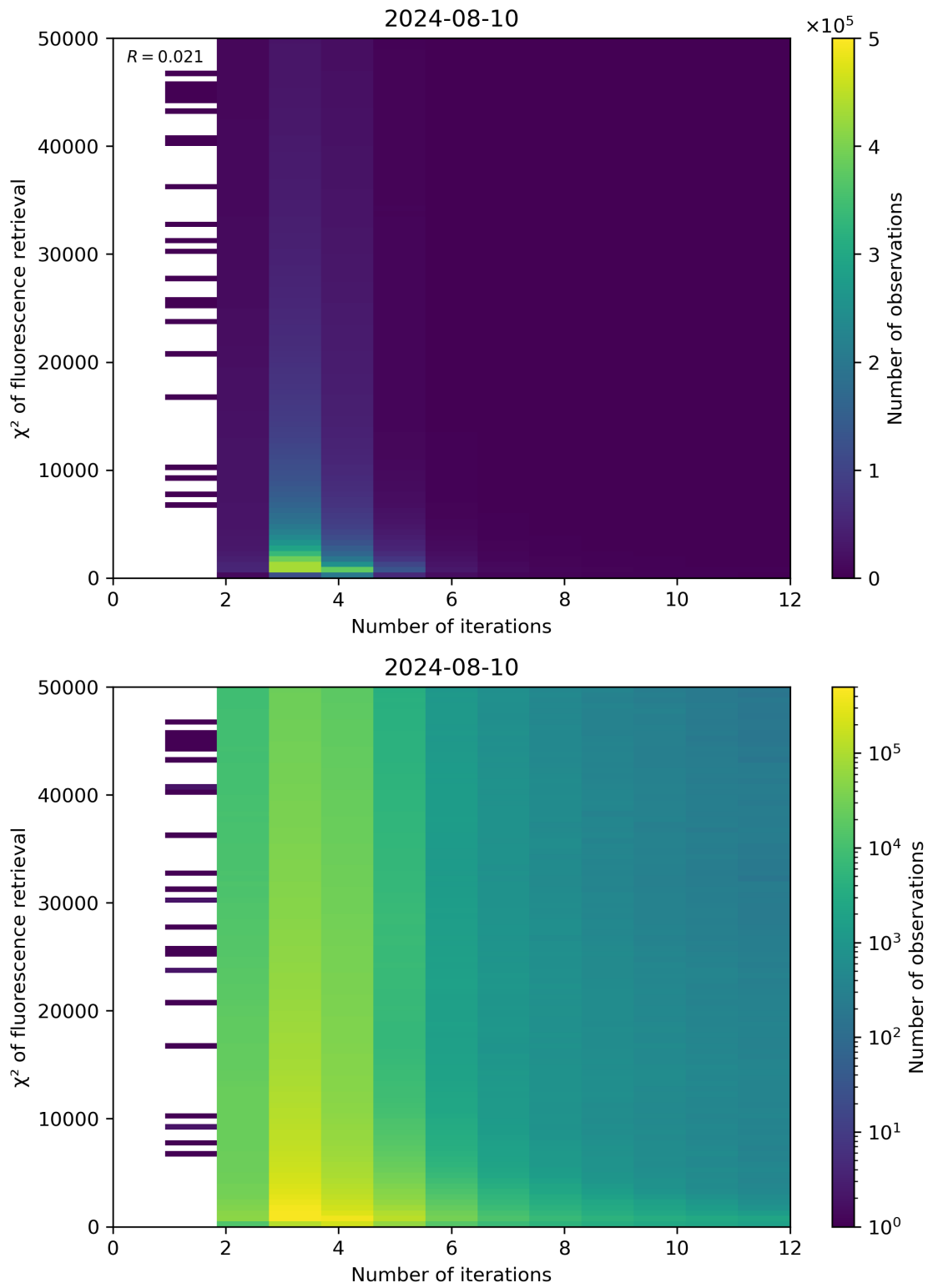
Figure 97: Scatter density plot of “Number of iterations” against “ \chi^2 of fluorescence retrieval” for 2024-08-09 to 2024-08-11.
