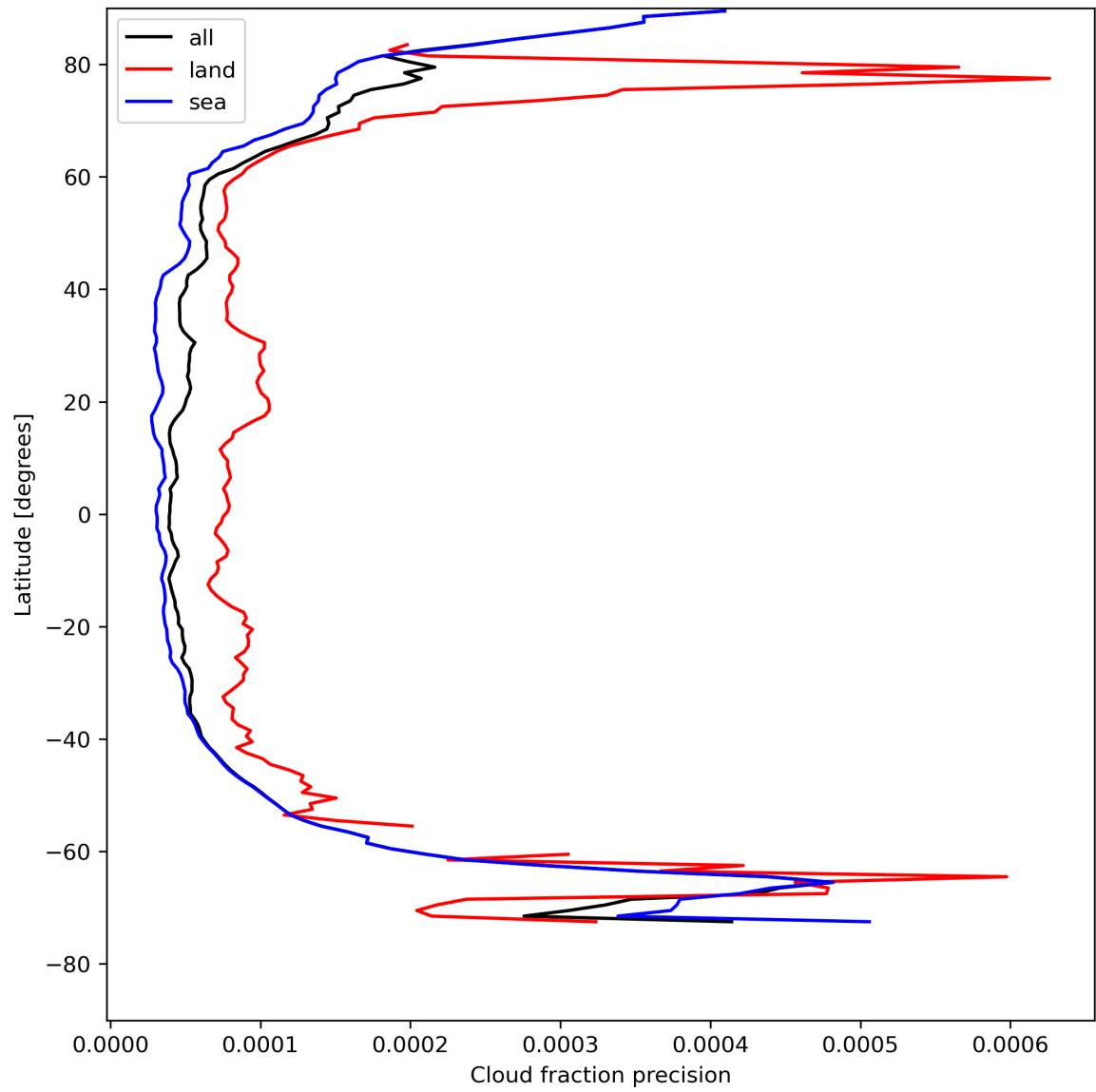
Figure 16: Zonal average of “Cloud fraction precision” for 2024-08-09 to 2024-08-11.
