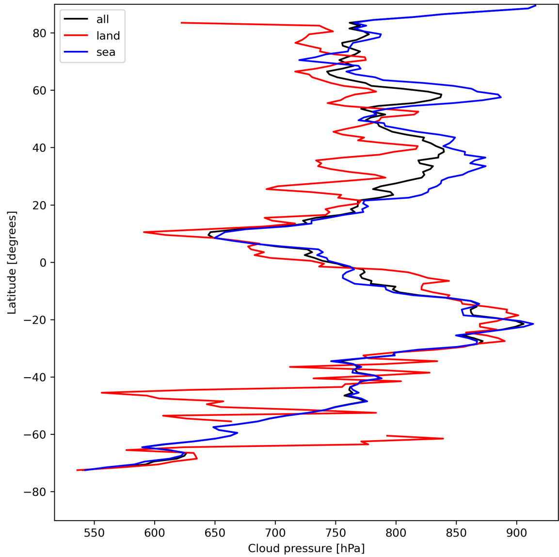
Figure 13: Zonal average of “Cloud pressure” for 2024-08-09 to 2024-08-11.
