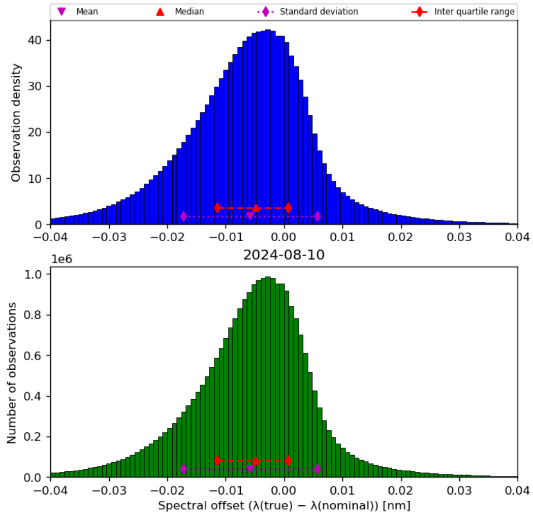
Figure 45: Histogram of “Spectral offset ( \lambda(\text{true}) - \lambda(\text{nominal}) )” for 2024-08-09 to 2024-08-11
