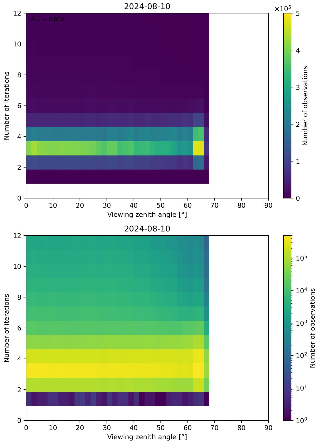
Figure 124: Scatter density plot of “Viewing zenith angle” against “Number of iterations” for 2024-08-09 to 2024-08-11.
