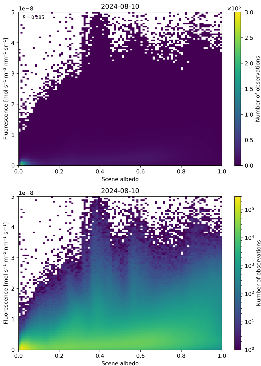
Figure 104: Scatter density plot of “Scene albedo” against “Fluorescence” for 2024-08-09 to 2024-08-11.
