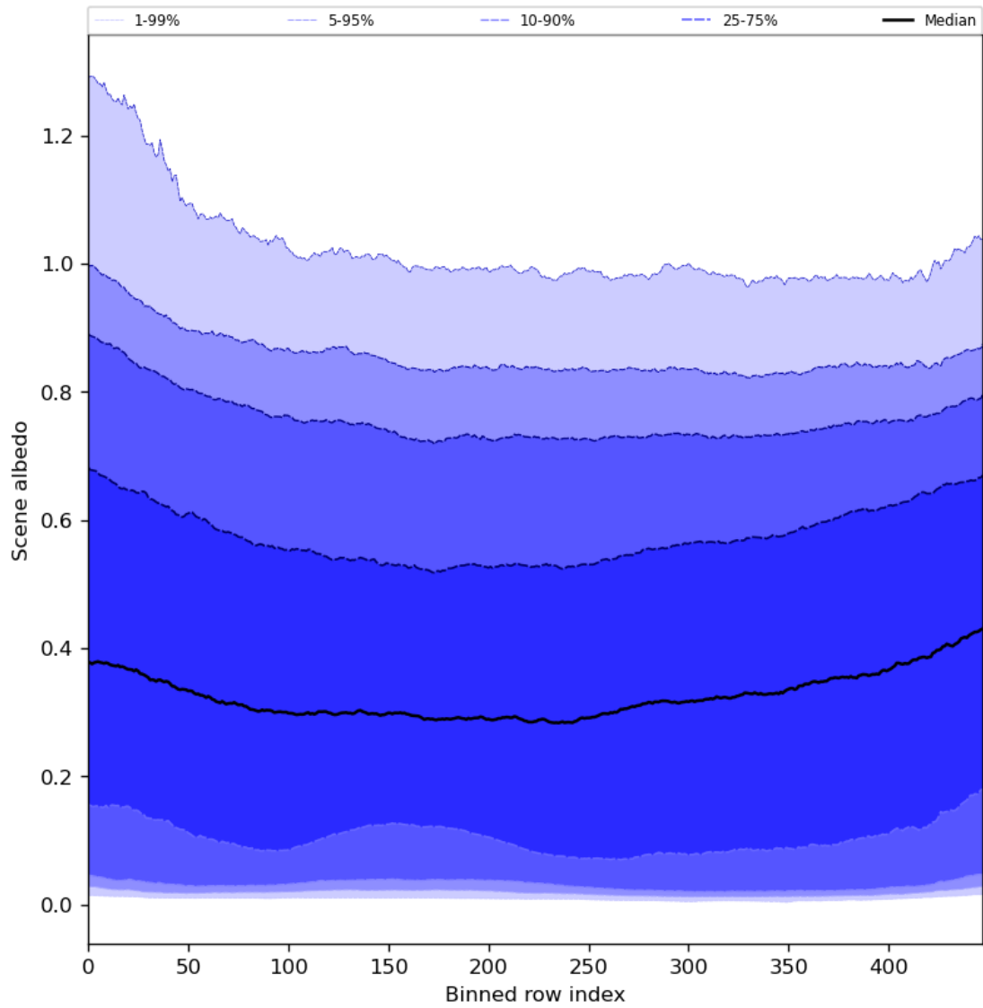
Figure 51: Along track statistics of “Scene albedo” for 2024-08-09 to 2024-08-11
