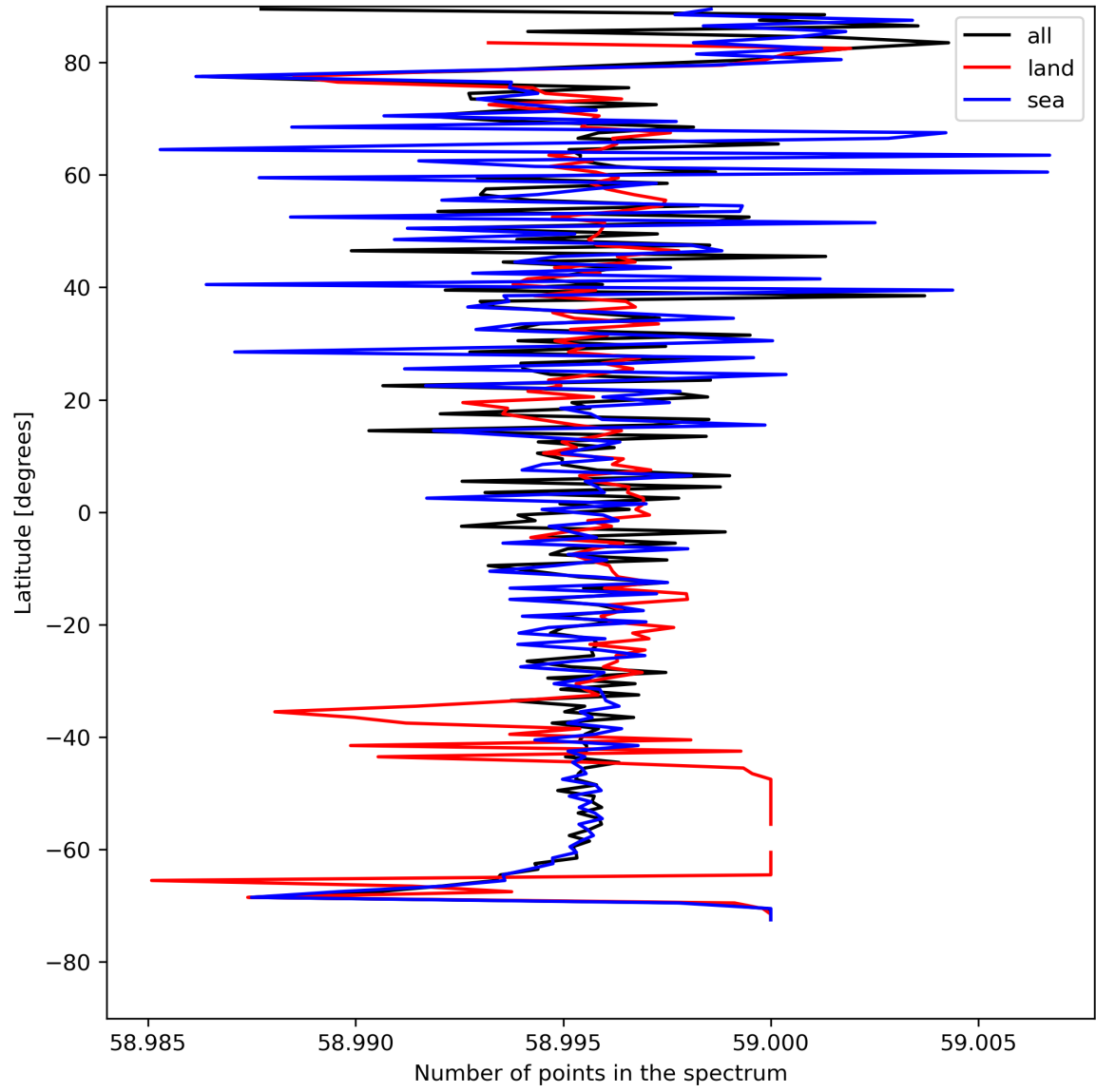
Figure 27: Zonal average of “Number of points in the spectrum” for 2024-08-09 to 2024-08-11.
