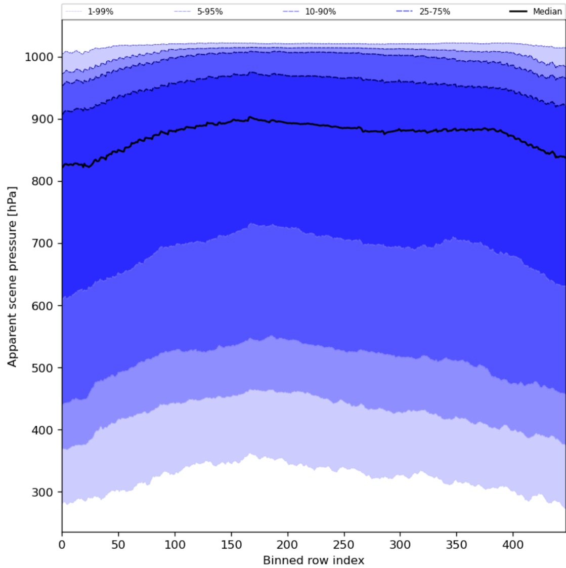
Figure 53: Along track statistics of “Apparent scene pressure” for 2024-08-09 to 2024-08-11
