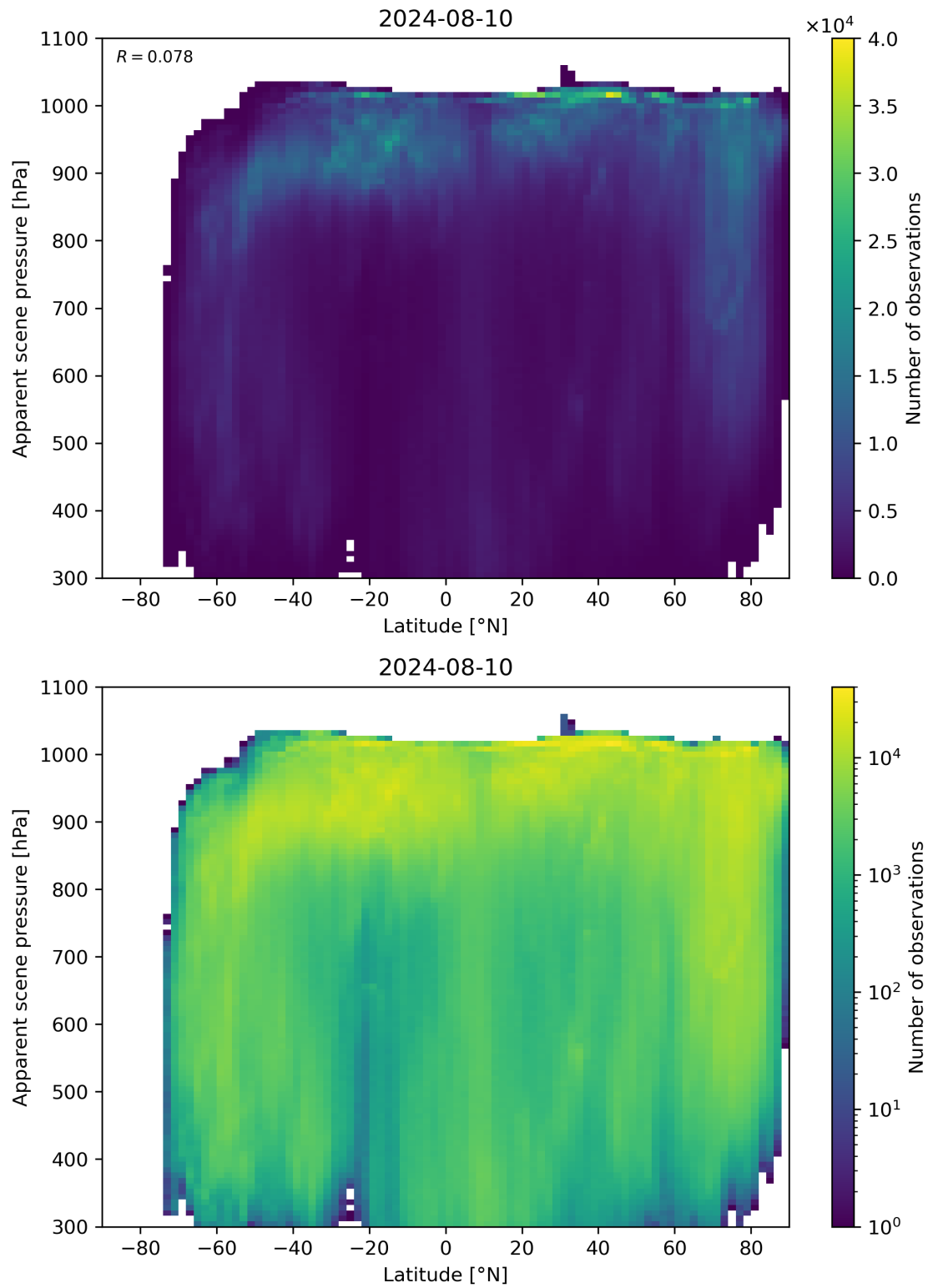
Figure 88: Scatter density plot of “Latitude” against “Apparent scene pressure” for 2024-08-09 to 2024-08-11.
