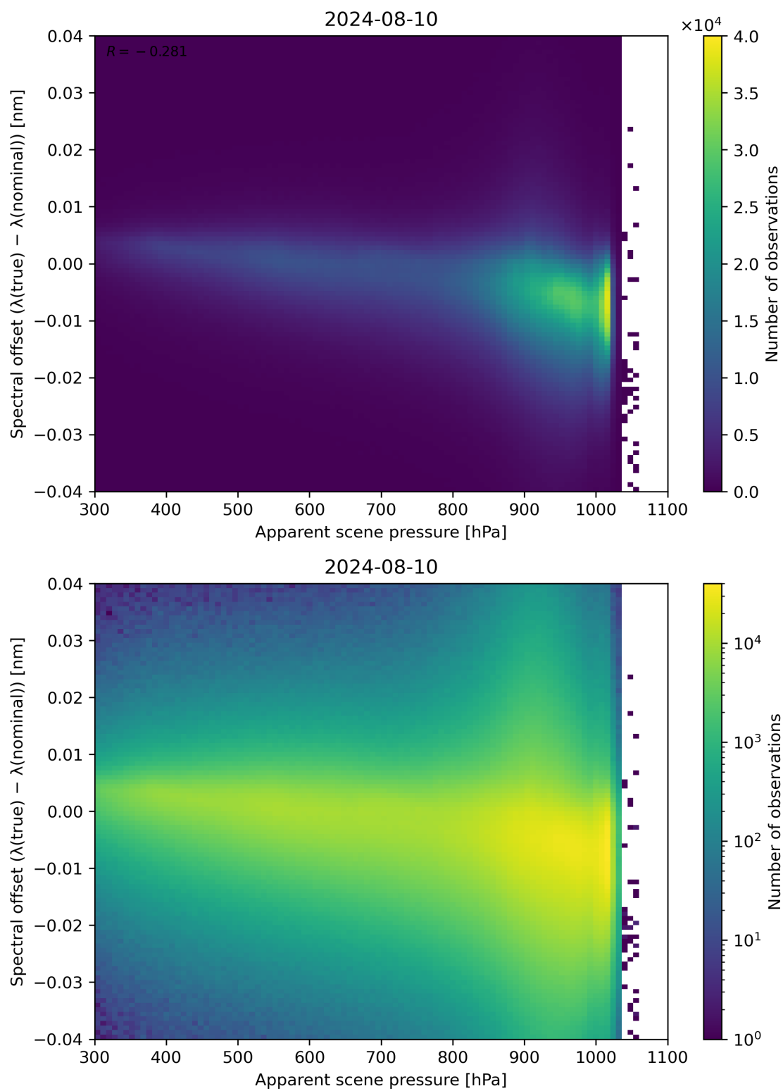
Figure 67: Scatter density plot of “Apparent scene pressure” against “Spectral offset ( \lambda(\text{true}) - \lambda(\text{nominal}) )” for 2024-08-09 to 2024-08-11.
