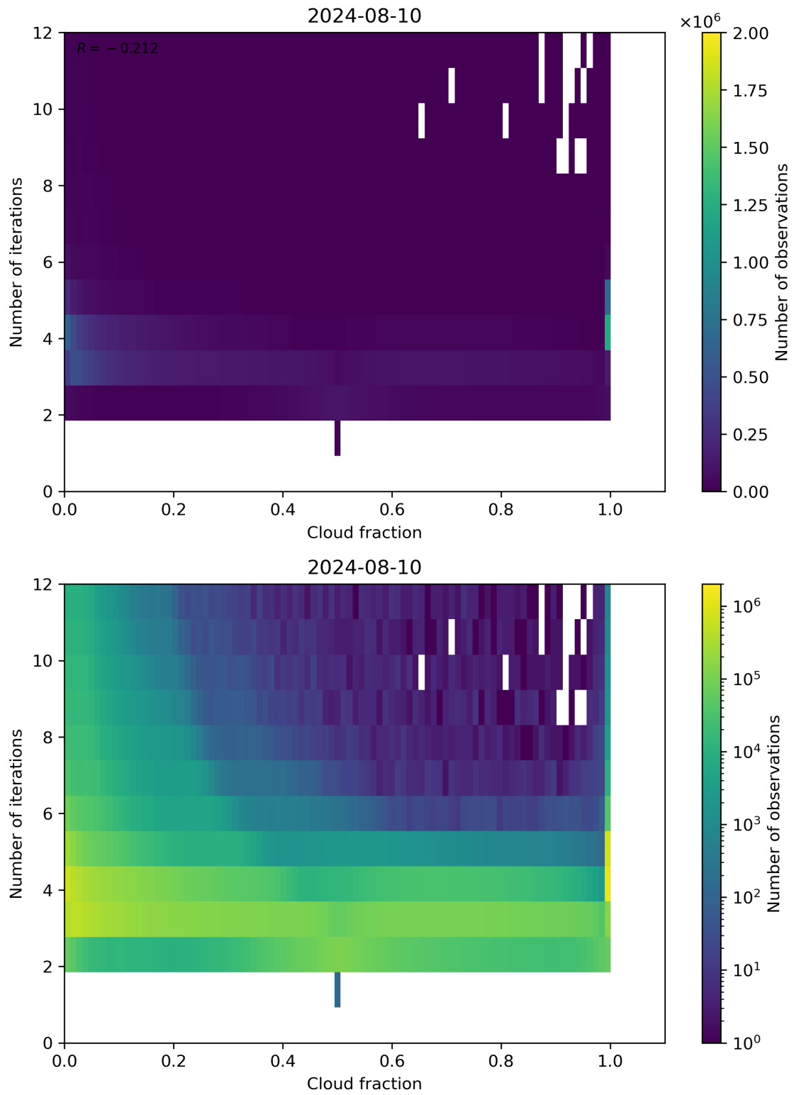
Figure 73: Scatter density plot of “Cloud fraction” against “Number of iterations” for 2024-08-09 to 2024-08-11.
