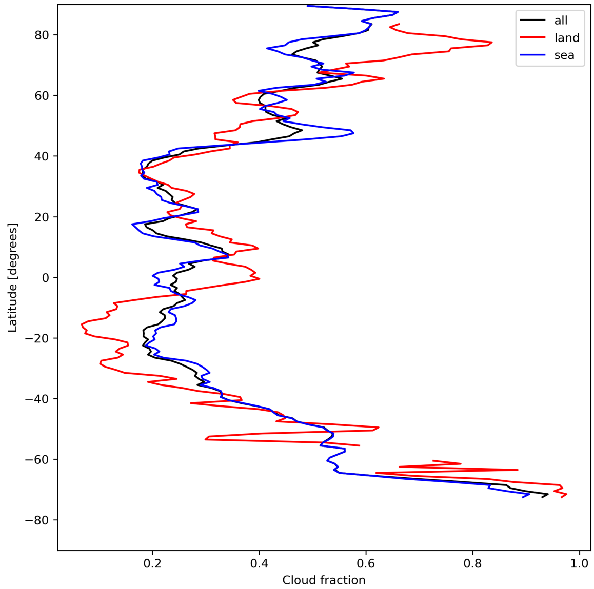
Figure 15: Zonal average of “Cloud fraction” for 2024-08-09 to 2024-08-11.
