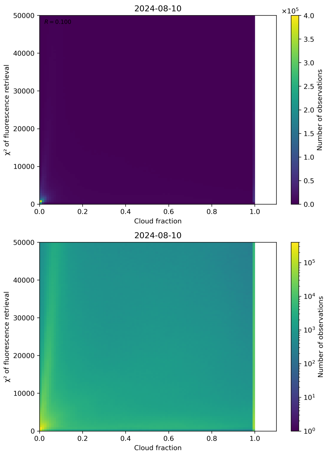
Figure 71: Scatter density plot of “Cloud fraction” against “ \chi^2 of fluorescence retrieval” for 2024-08-09 to 2024-08-11.
