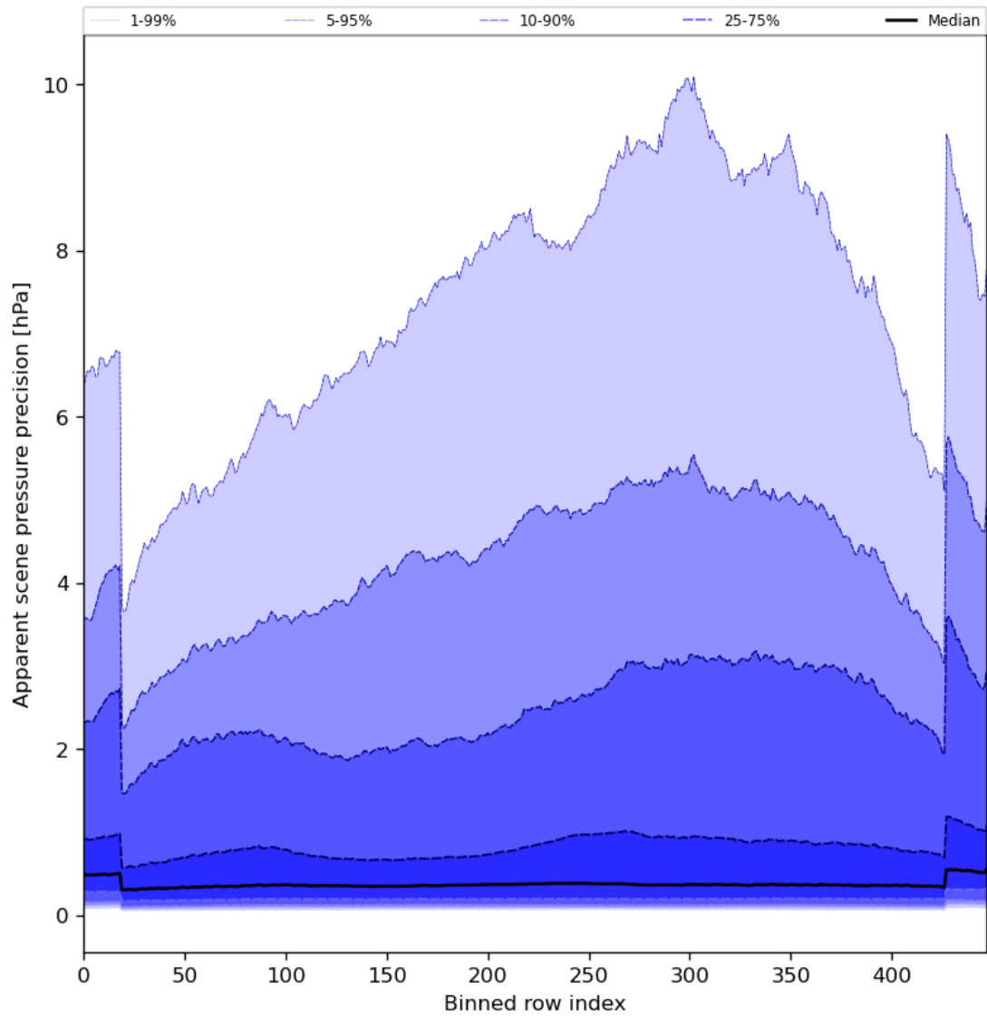
Figure 54: Along track statistics of “Apparent scene pressure precision” for 2024-08-09 to 2024-08-11
