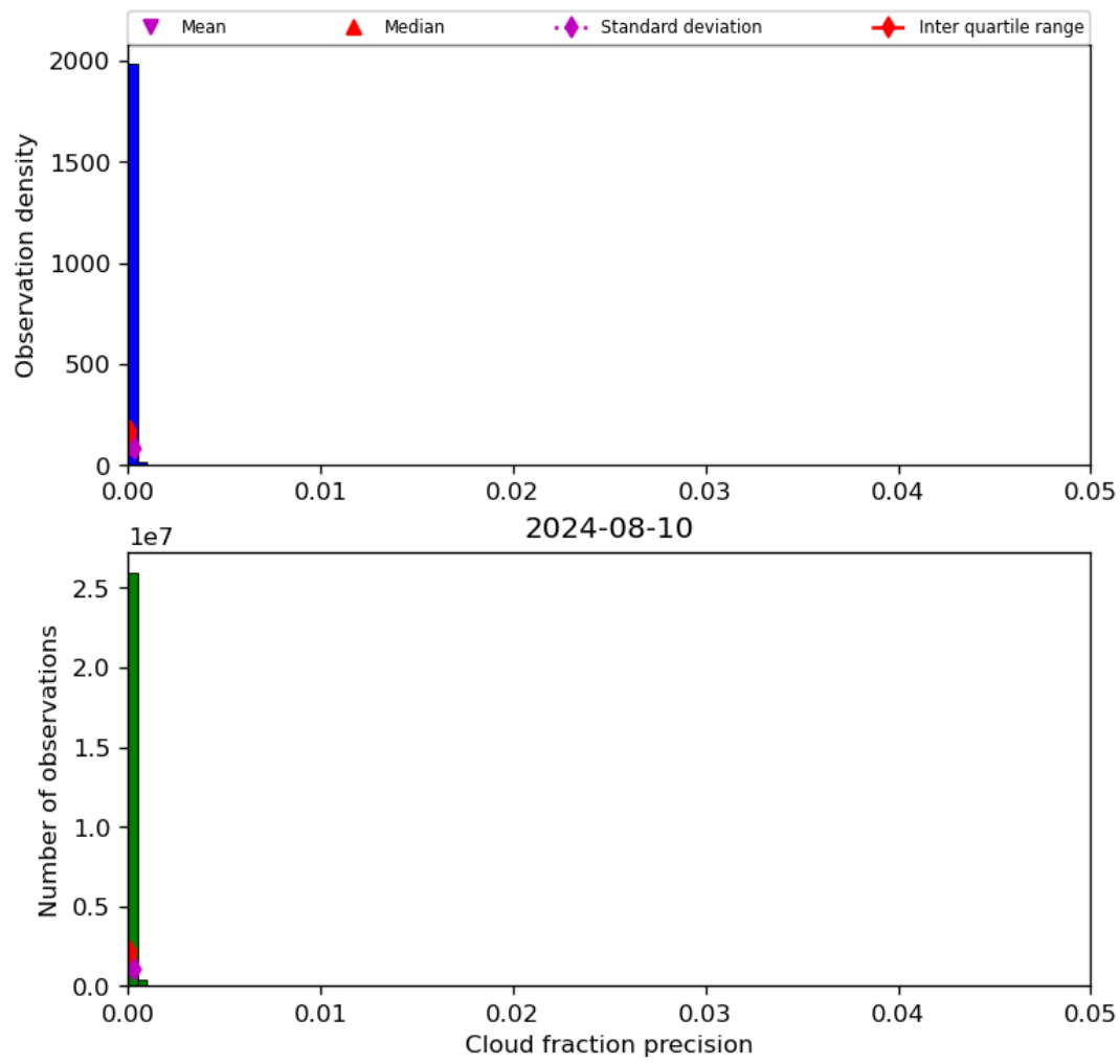
Figure 33: Histogram of “Cloud fraction precision” for 2024-08-09 to 2024-08-11
