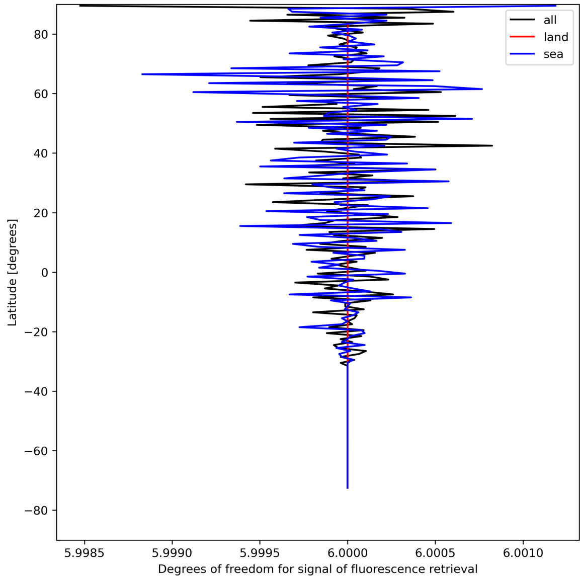
Figure 26: Zonal average of “Degrees of freedom for signal of fluorescence retrieval” for 2024-08-09 to 2024-08-11.
