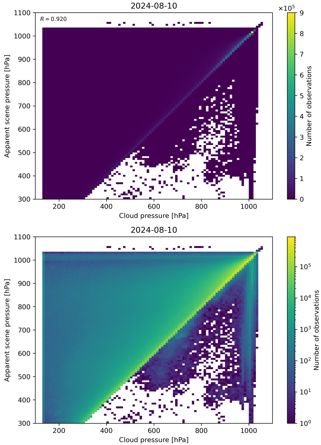
Figure 77: Scatter density plot of “Cloud pressure” against “Apparent scene pressure” for 2024-08-09 to 2024-08-11.
