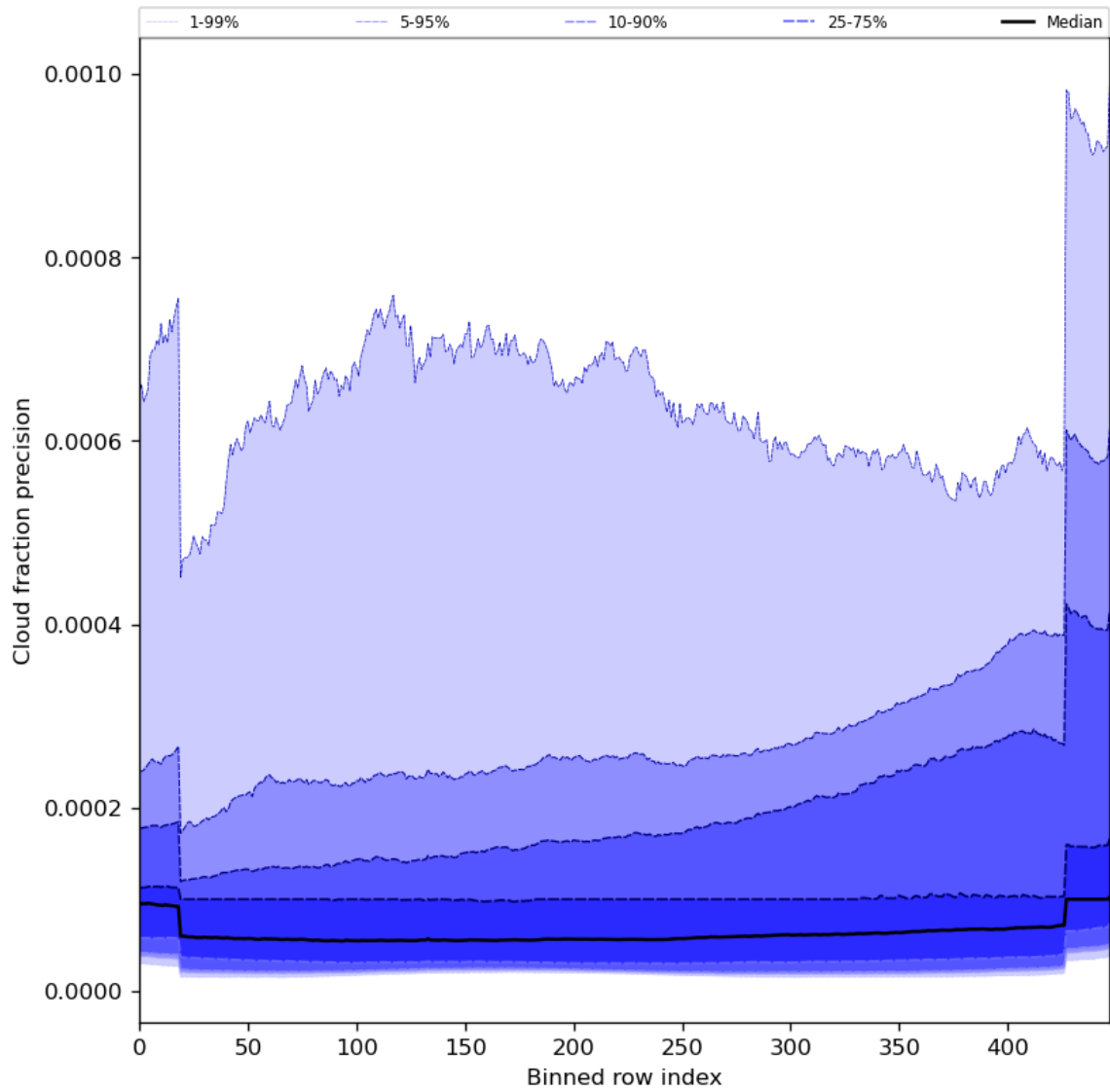
Figure 50: Along track statistics of “Cloud fraction precision” for 2024-08-09 to 2024-08-11
