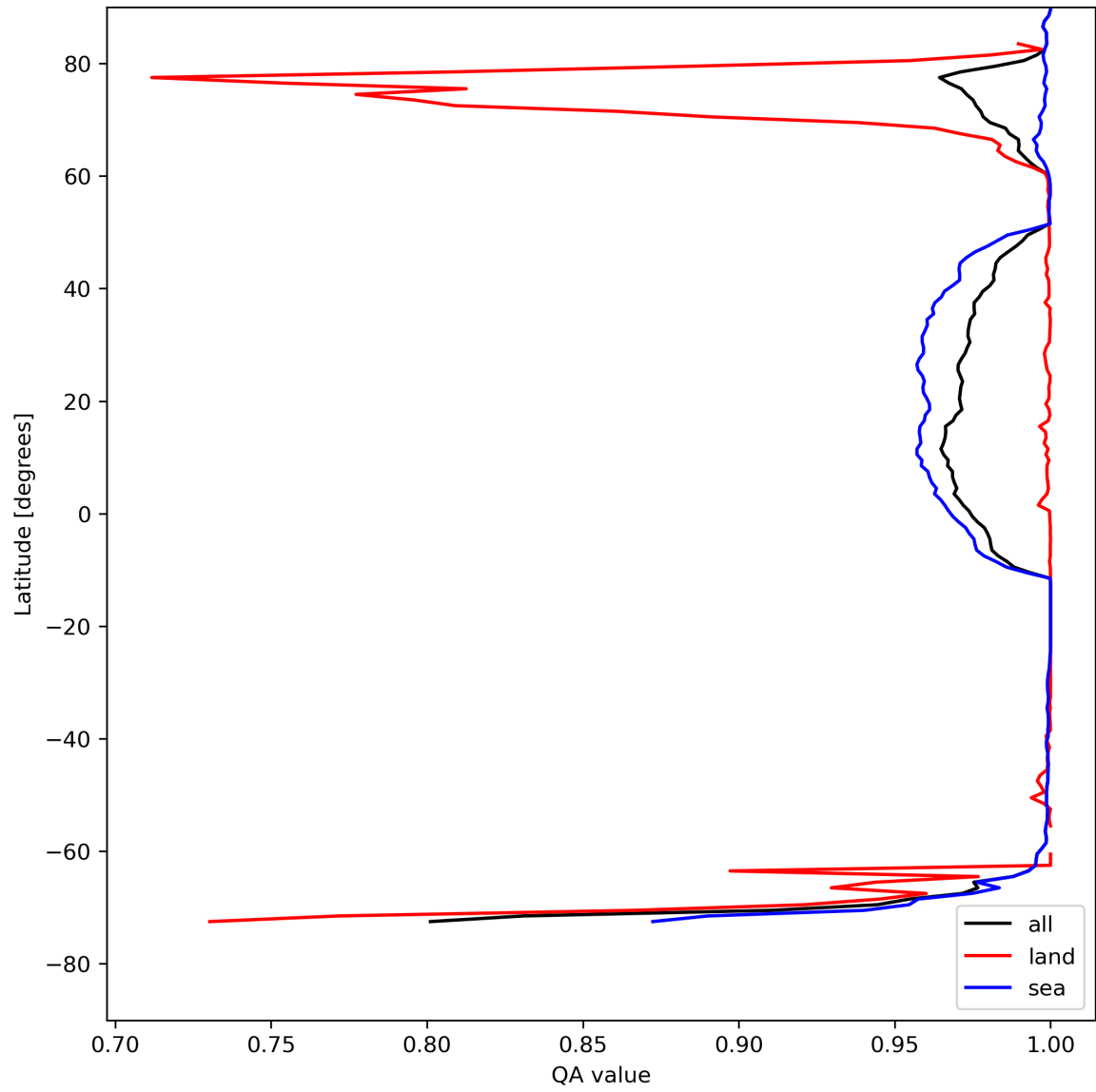
Figure 12: Zonal average of "QA value" for 2024-08-09 to 2024-08-11.
