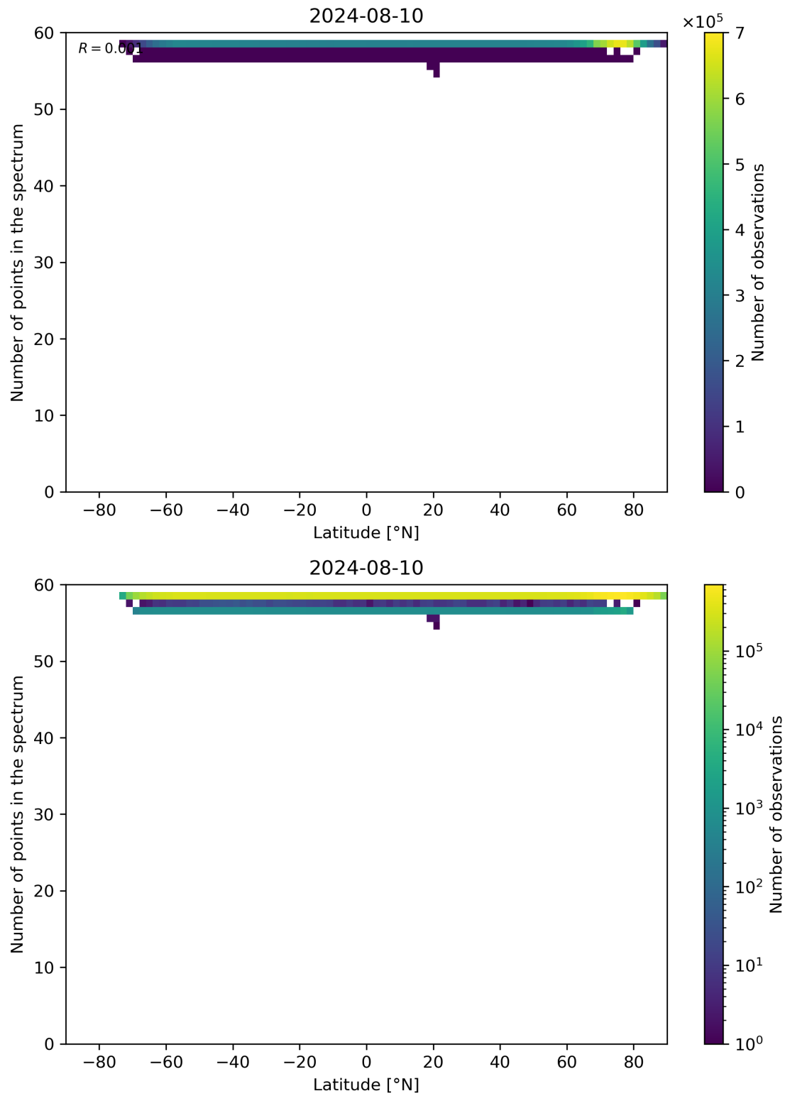
Figure 94: Scatter density plot of “Latitude” against “Number of points in the spectrum” for 2024-08-09 to 2024-08-11.
