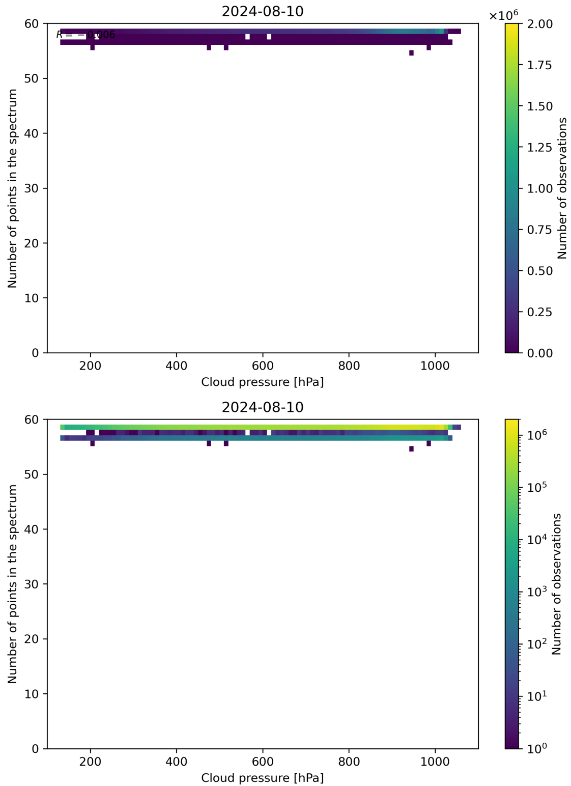
Figure 82: Scatter density plot of “Cloud pressure” against “Number of points in the spectrum” for 2024-08-09 to 2024-08-11.
