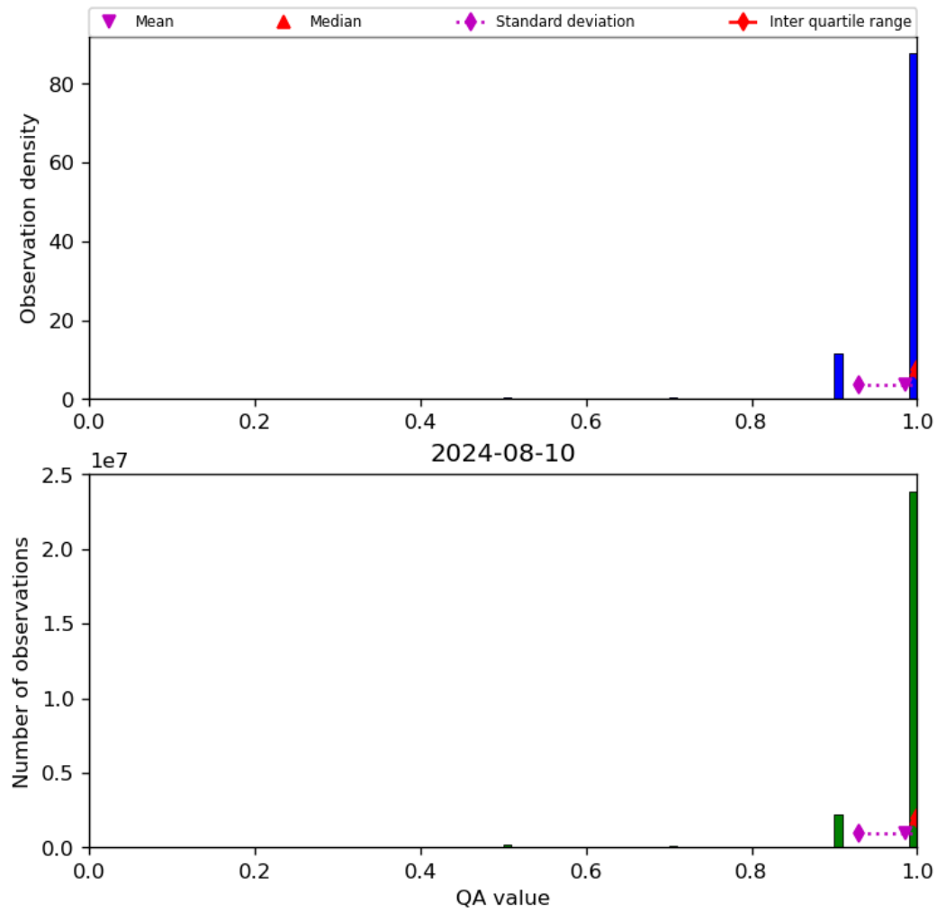
Figure 29: Histogram of “QA value” for 2024-08-09 to 2024-08-11
