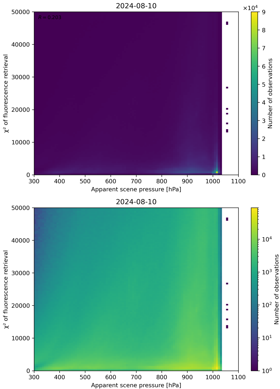
Figure 63: Scatter density plot of “Apparent scene pressure” against “ \chi^2 of fluorescence retrieval” for 2024-08-09 to 2024-08-11.
