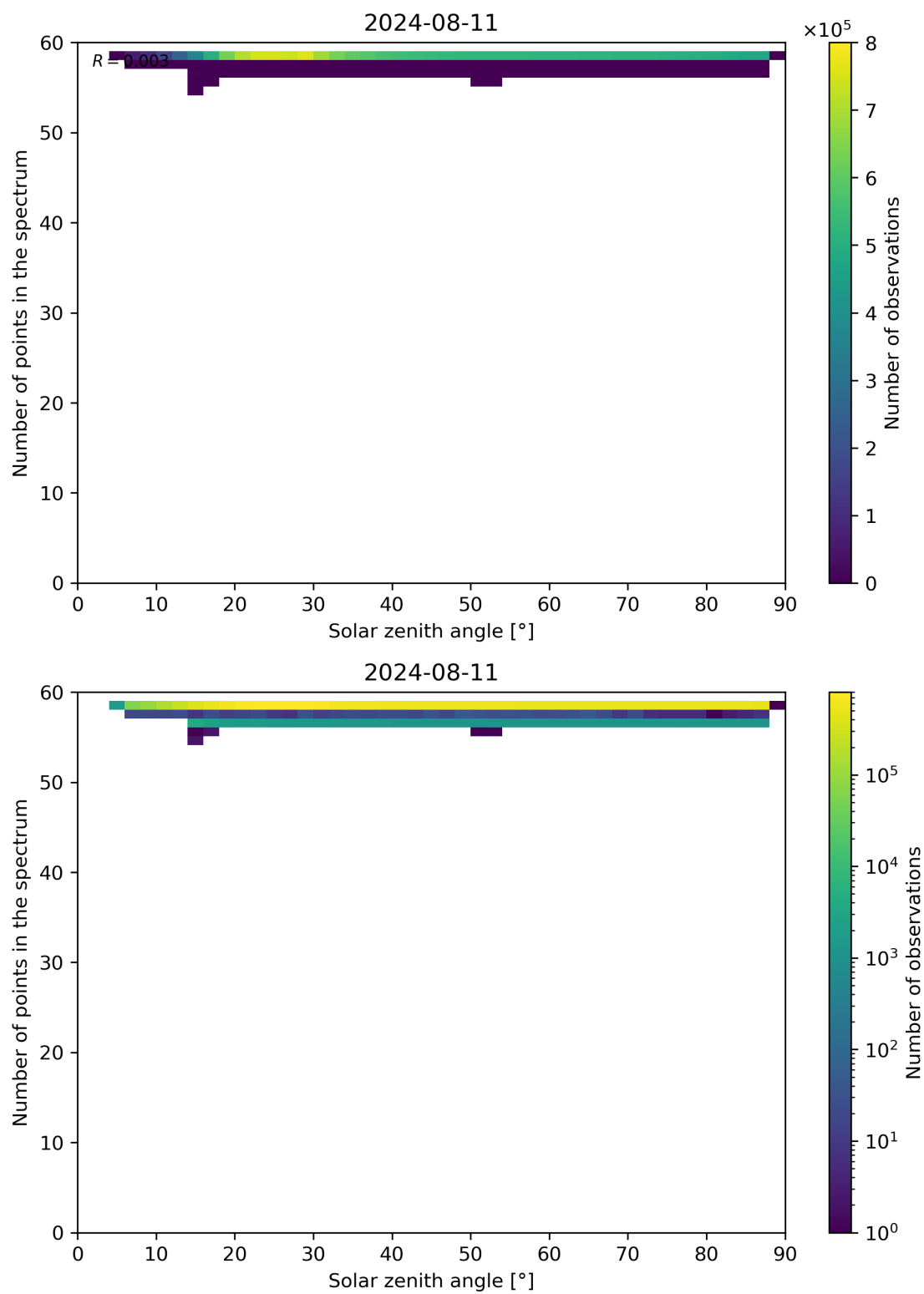
Figure 115: Scatter density plot of “Solar zenith angle” against “Number of points in the spectrum” for 2024-08-11 to 2024-08-11.
