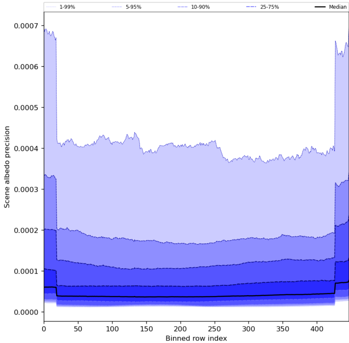
Figure 52: Along track statistics of “Scene albedo precision” for 2024-08-11 to 2024-08-11
