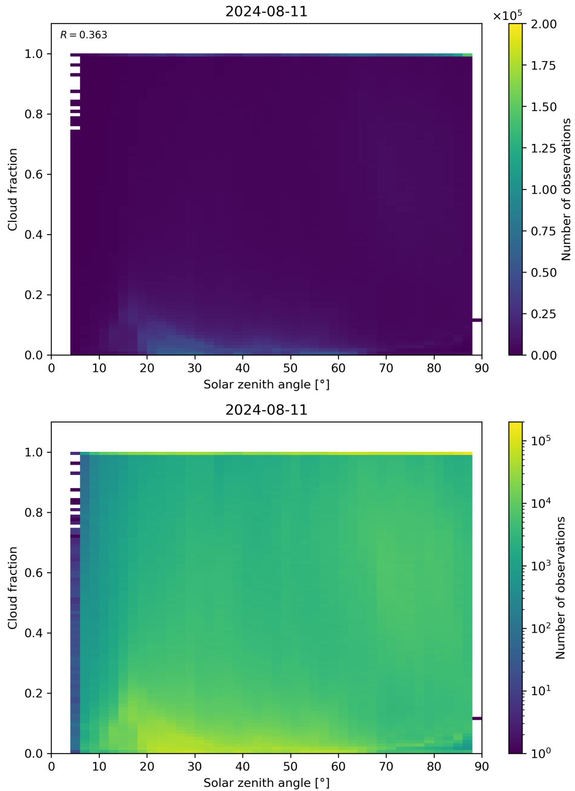
Figure 110: Scatter density plot of “Solar zenith angle” against “Cloud fraction” for 2024-08-11 to 2024-08-11.
