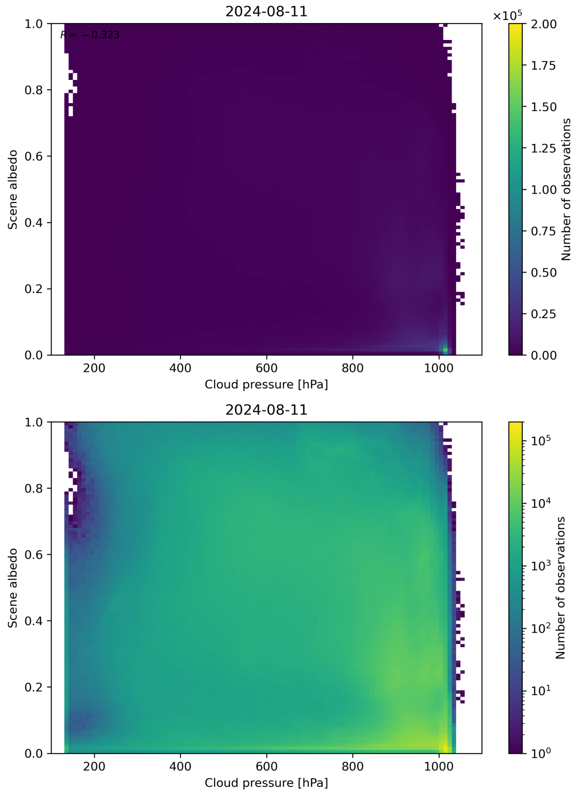
Figure 83: Scatter density plot of “Cloud pressure” against “Scene albedo” for 2024-08-11 to 2024-08-11.
