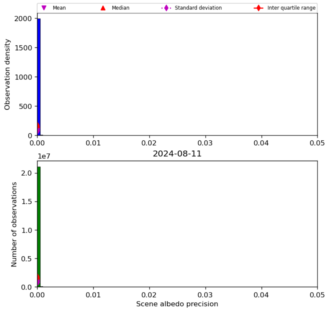
Figure 35: Histogram of “Scene albedo precision” for 2024-08-11 to 2024-08-11
