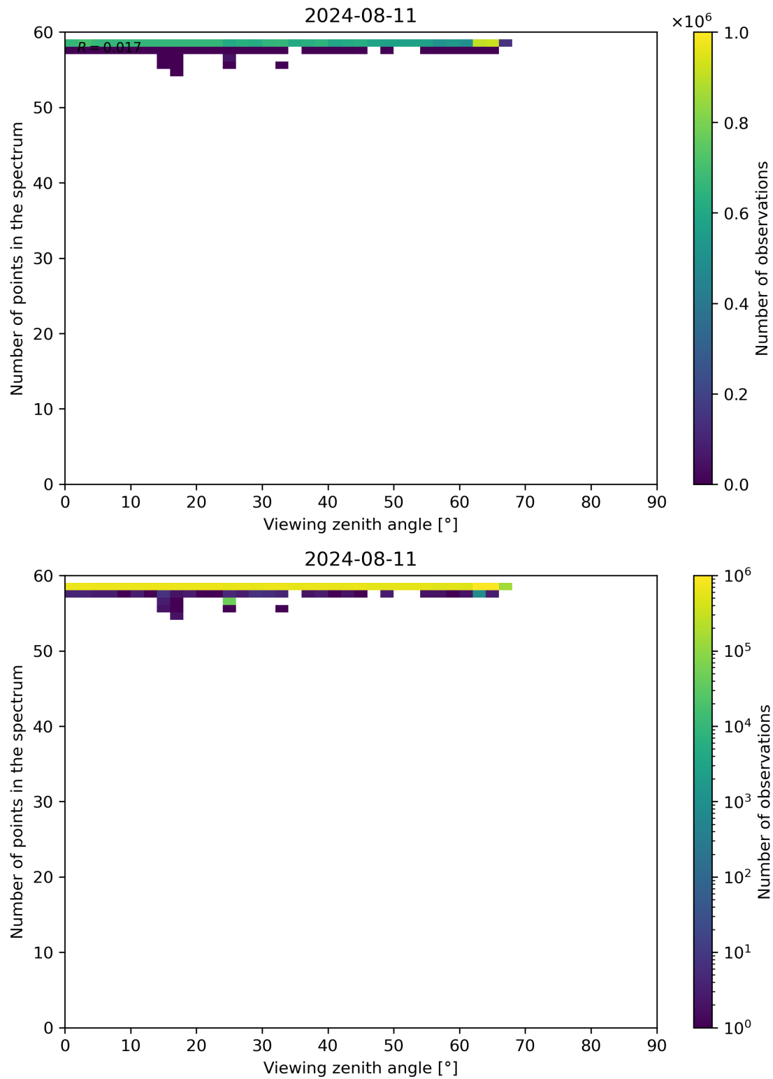
Figure 125: Scatter density plot of “Viewing zenith angle” against “Number of points in the spectrum” for 2024-08-11 to 2024-08-11.
