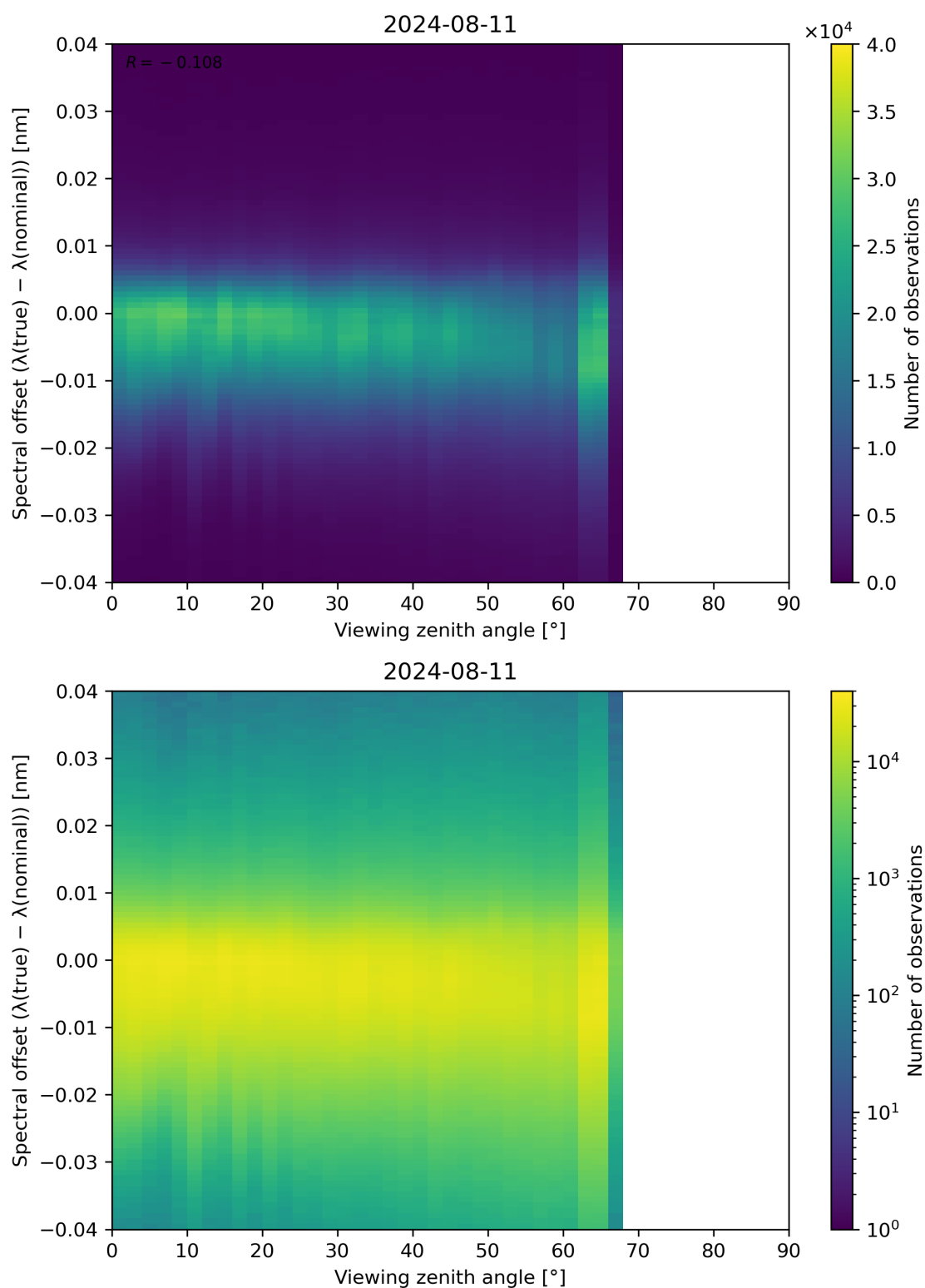
Figure 128: Scatter density plot of “Viewing zenith angle” against “Spectral offset ( \lambda(\text{true}) - \lambda(\text{nominal}) )” for 2024-08-11 to 2024-08-11.
