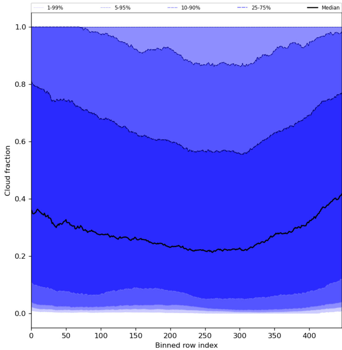
Figure 49: Along track statistics of “Cloud fraction” for 2024-08-11 to 2024-08-11
