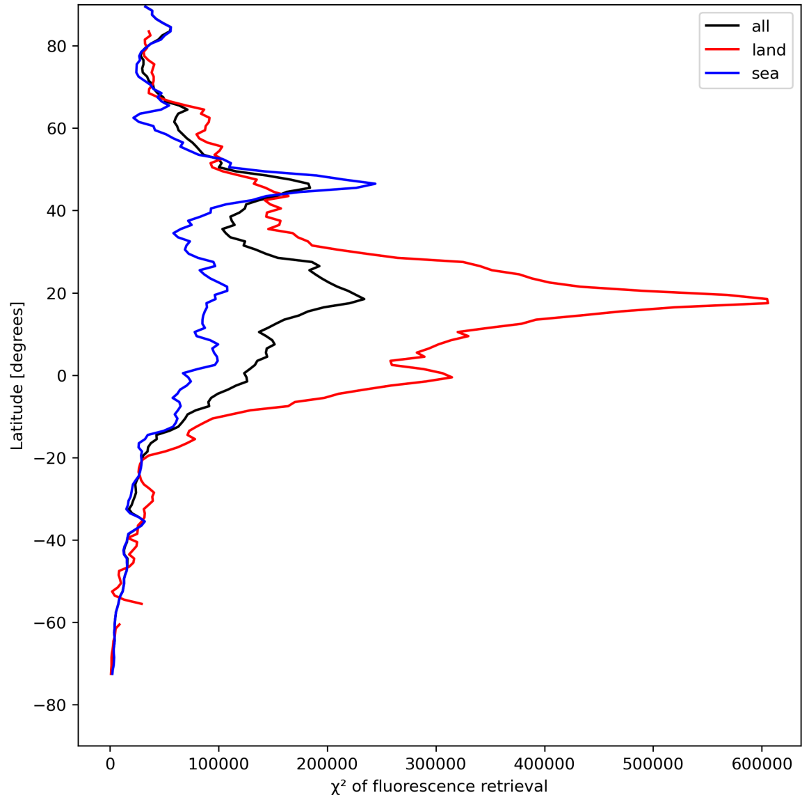
Figure 25: Zonal average of “ \chi^2 of fluorescence retrieval” for 2024-08-11 to 2024-08-11.
