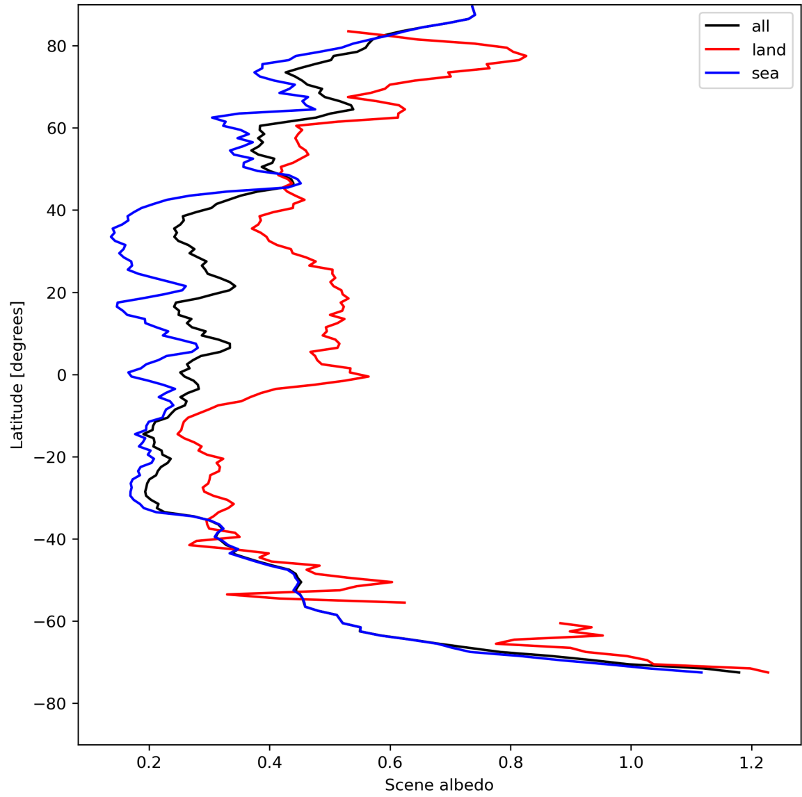
Figure 17: Zonal average of “Scene albedo” for 2024-08-11 to 2024-08-11.
