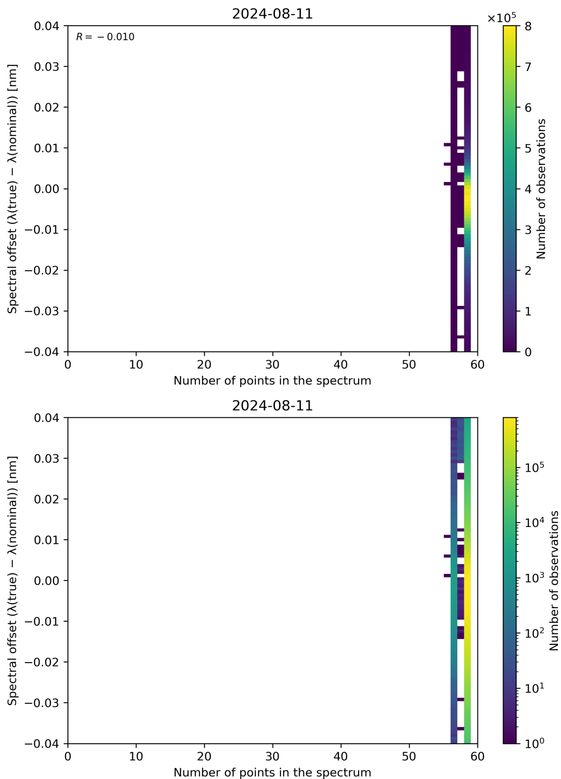
Figure 101: Scatter density plot of “Number of points in the spectrum” against “Spectral offset ( \lambda(\text{true}) - \lambda(\text{nominal}) )” for 2024-08-11 to 2024-08-11.
