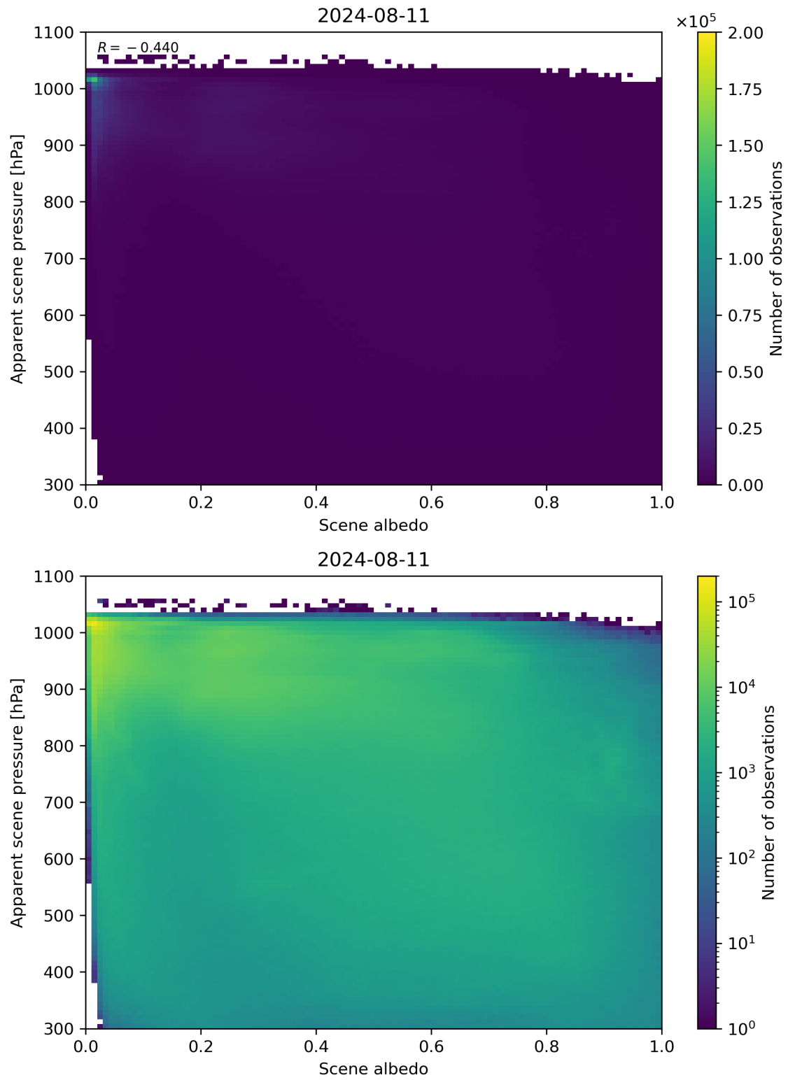
Figure 102: Scatter density plot of “Scene albedo” against “Apparent scene pressure” for 2024-08-11 to 2024-08-11.
