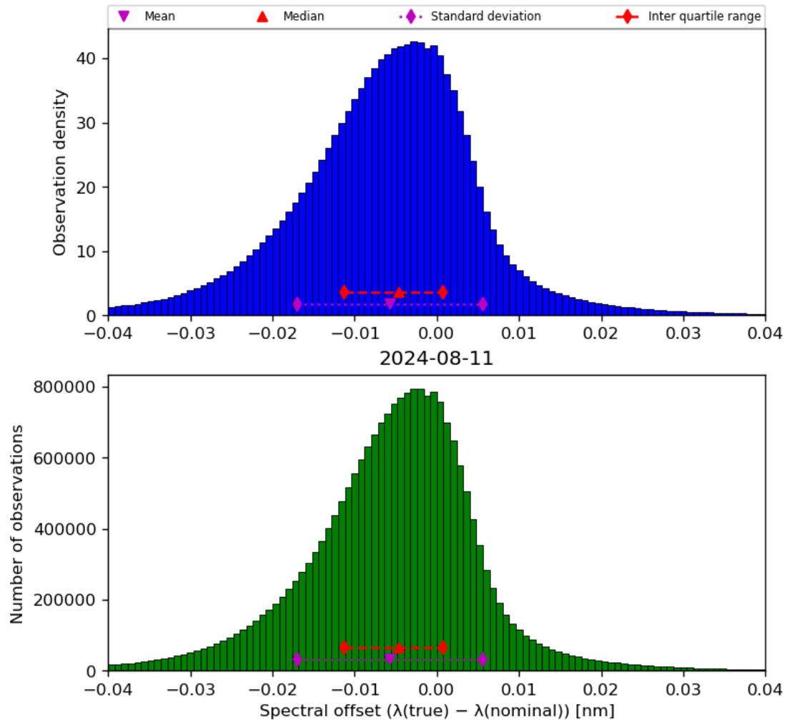
Figure 45: Histogram of “Spectral offset ( \lambda(\text{true}) - \lambda(\text{nominal}) )” for 2024-08-11 to 2024-08-11
