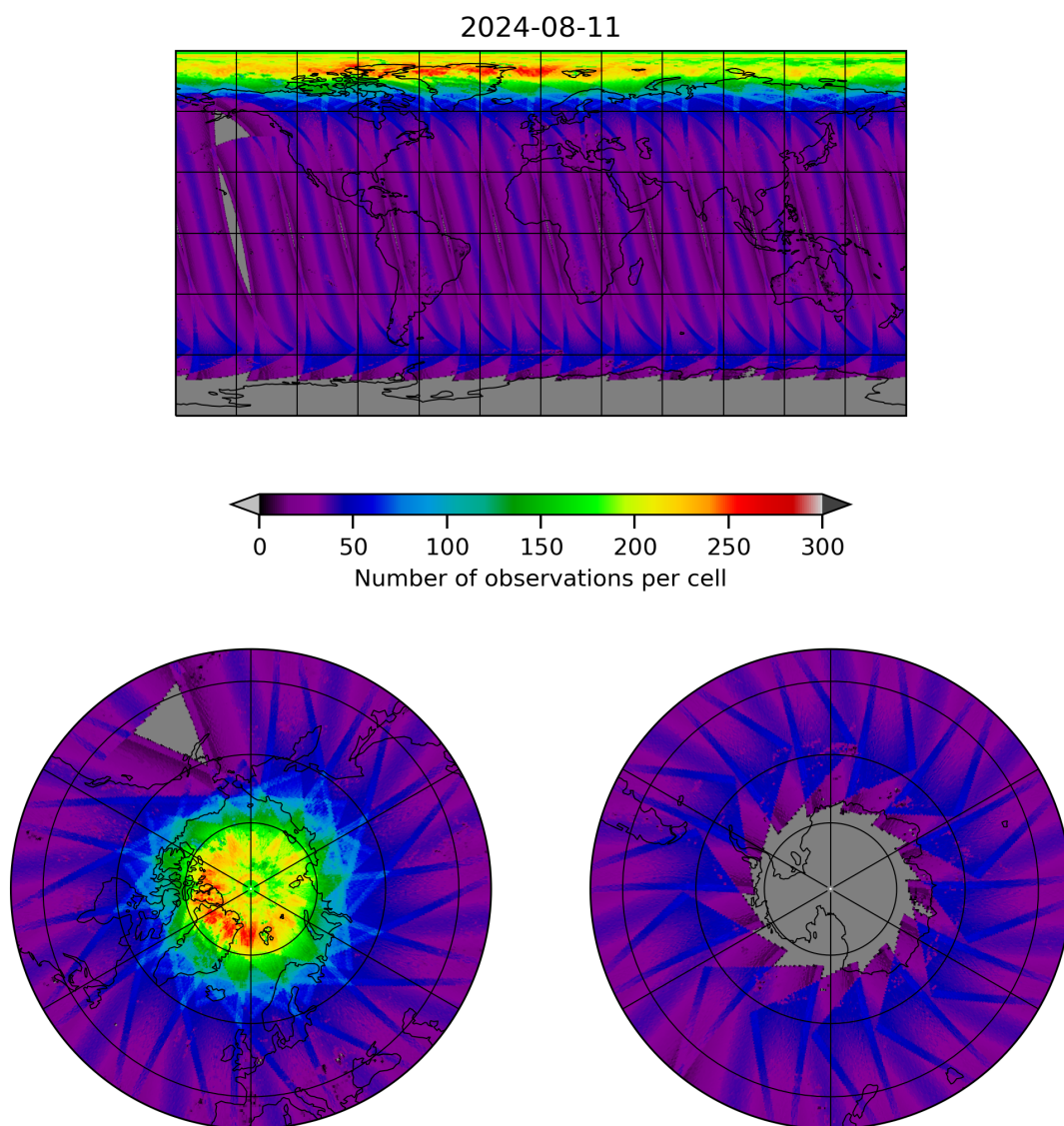
Figure 11: Map of the number of observations for 2024-08-11 to 2024-08-11
