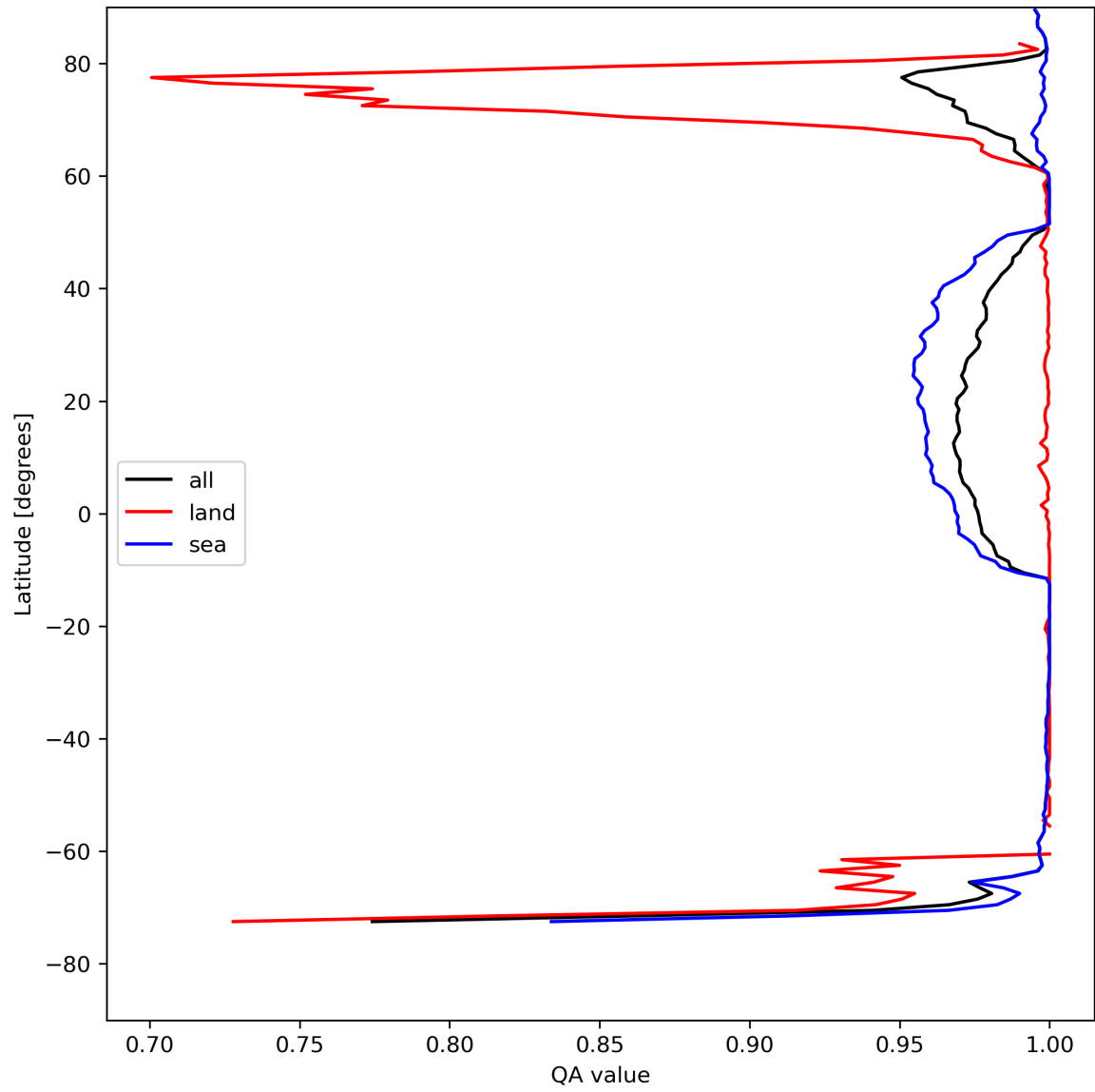
Figure 12: Zonal average of “QA value” for 2024-08-11 to 2024-08-11.
