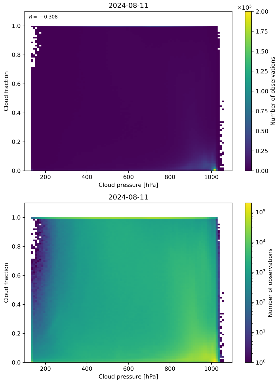
Figure 79: Scatter density plot of “Cloud pressure” against “Cloud fraction” for 2024-08-11 to 2024-08-11.
