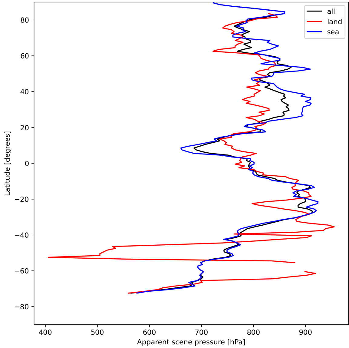
Figure 19: Zonal average of “Apparent scene pressure” for 2024-08-11 to 2024-08-11.
