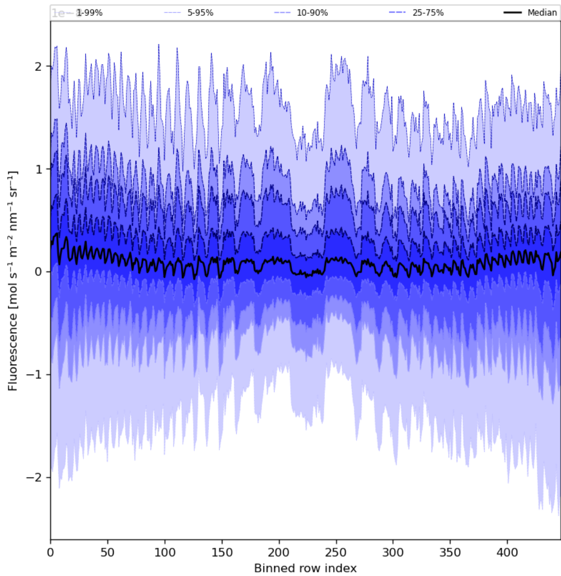
Figure 57: Along track statistics of “Fluorescence” for 2024-08-11 to 2024-08-11
