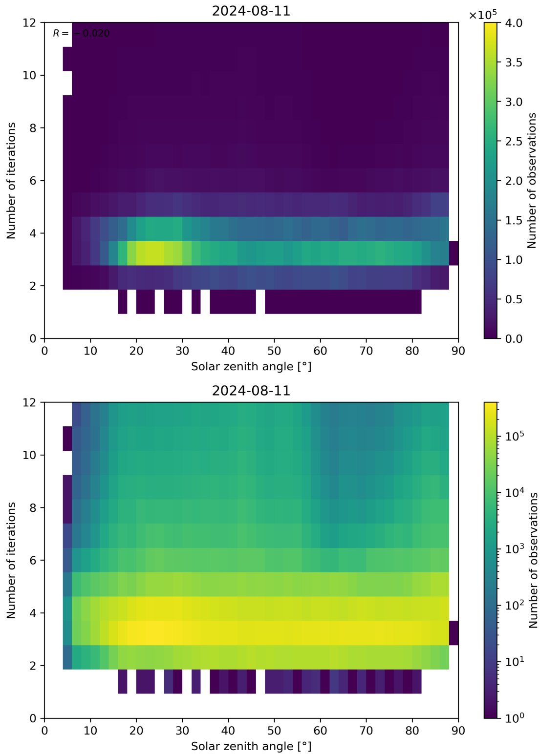
Figure 114: Scatter density plot of “Solar zenith angle” against “Number of iterations” for 2024-08-11 to 2024-08-11.
