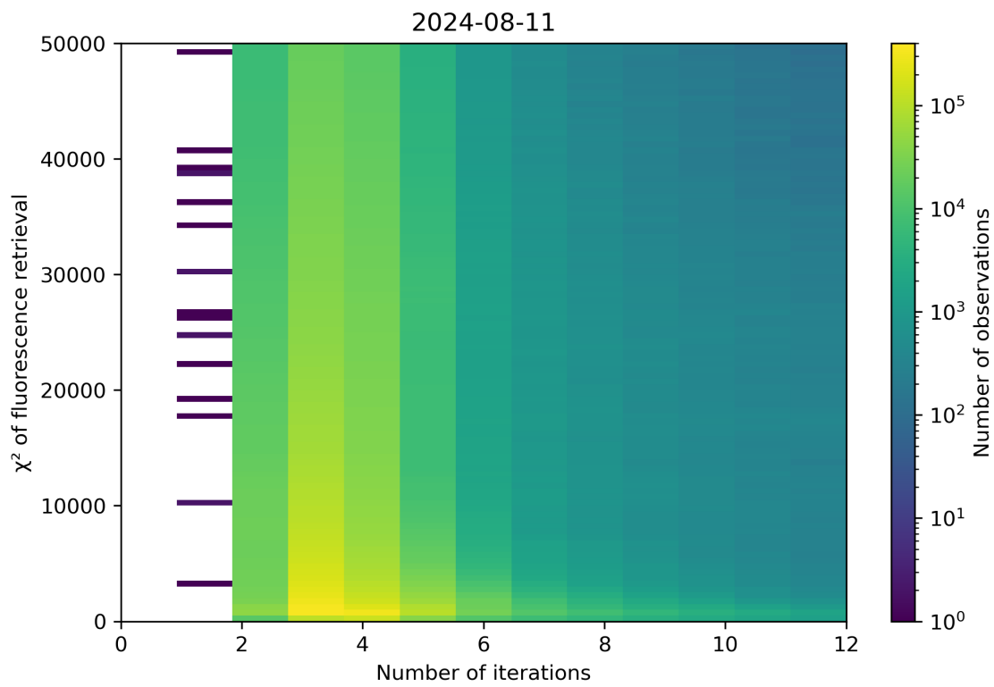
Figure 97: Scatter density plot of “Number of iterations” against “ \chi^2 of fluorescence retrieval” for 2024-08-11 to 2024-08-11.
