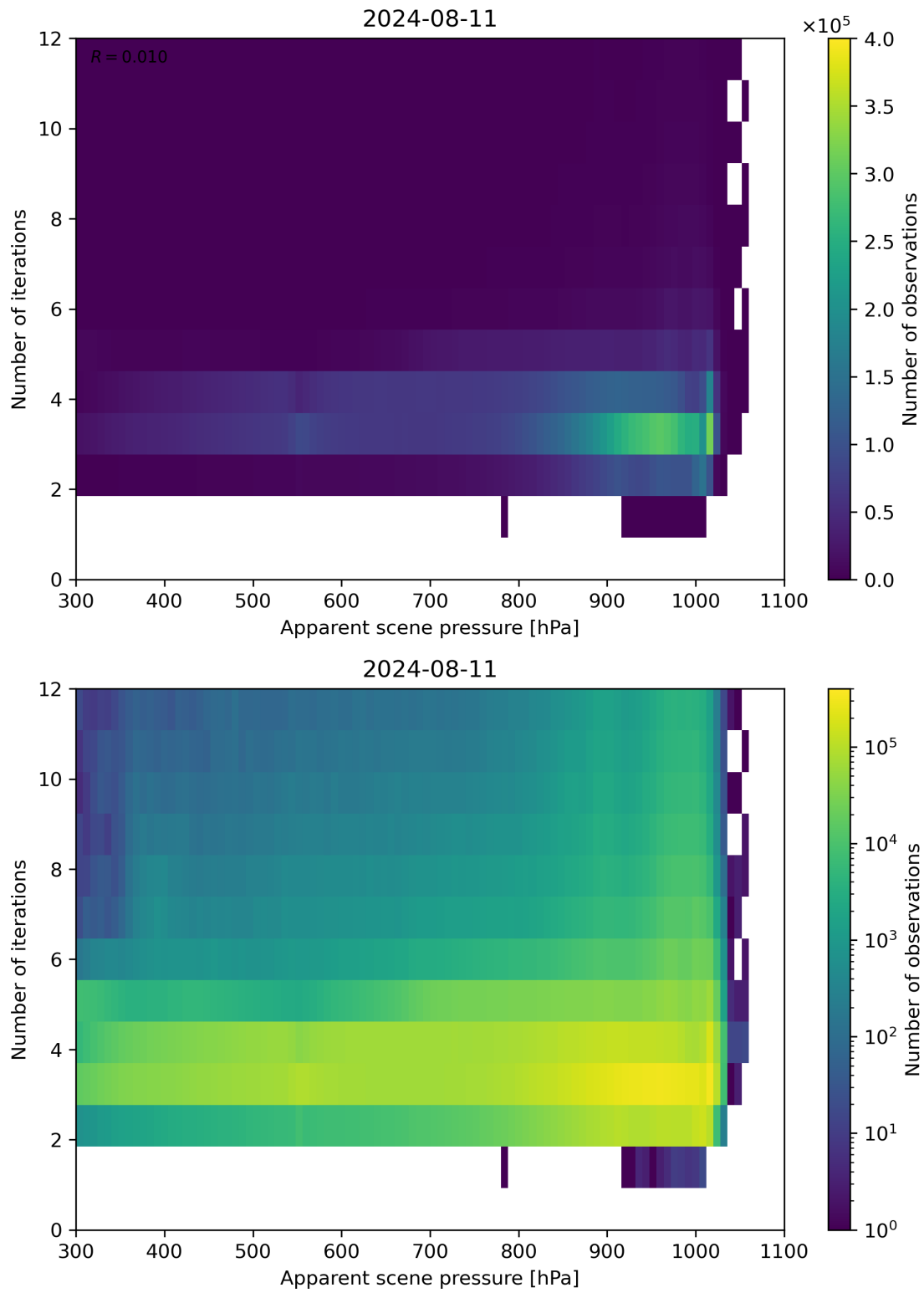
Figure 65: Scatter density plot of “Apparent scene pressure” against “Number of iterations” for 2024-08-11 to 2024-08-11.
