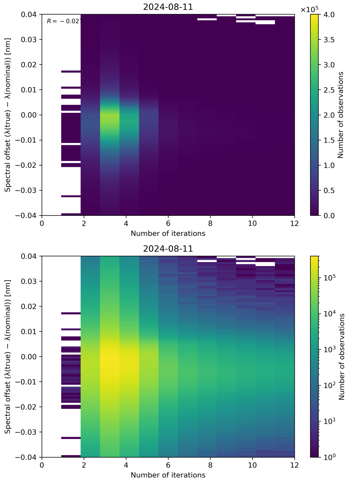
Figure 100: Scatter density plot of “Number of iterations” against “Spectral offset ( \lambda(\text{true}) - \lambda(\text{nominal}) )” for 2024-08-11 to 2024-08-11.
