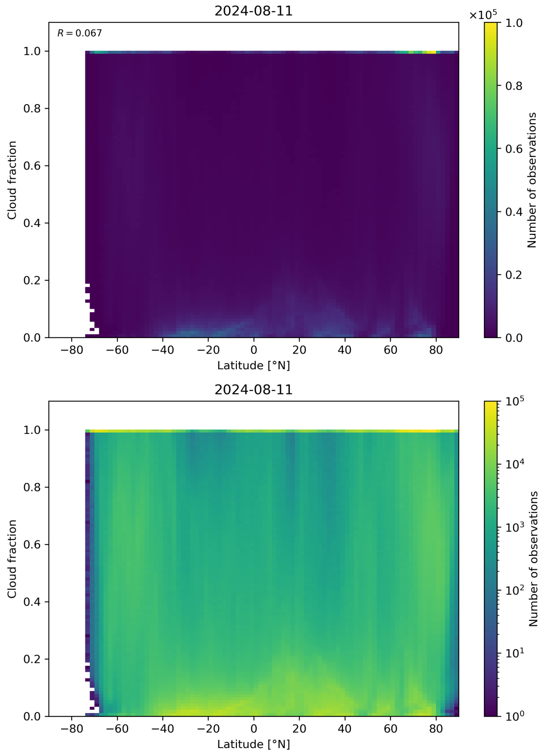
Figure 90: Scatter density plot of “Latitude” against “Cloud fraction” for 2024-08-11 to 2024-08-11.
