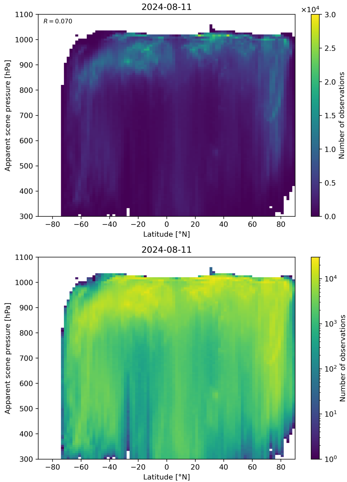
Figure 88: Scatter density plot of “Latitude” against “Apparent scene pressure” for 2024-08-11 to 2024-08-11.
