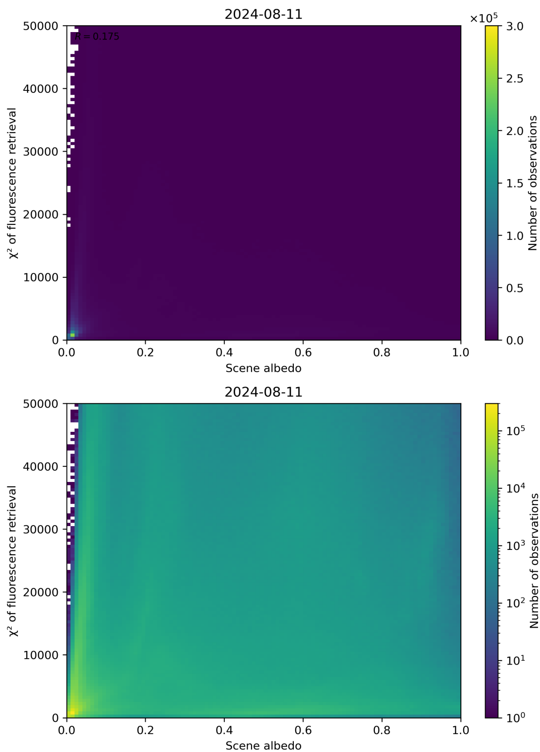
Figure 103: Scatter density plot of “Scene albedo” against “ \chi^2 of fluorescence retrieval” for 2024-08-11 to 2024-08-11.
