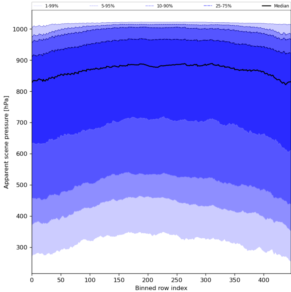
Figure 53: Along track statistics of “Apparent scene pressure” for 2024-08-11 to 2024-08-11
