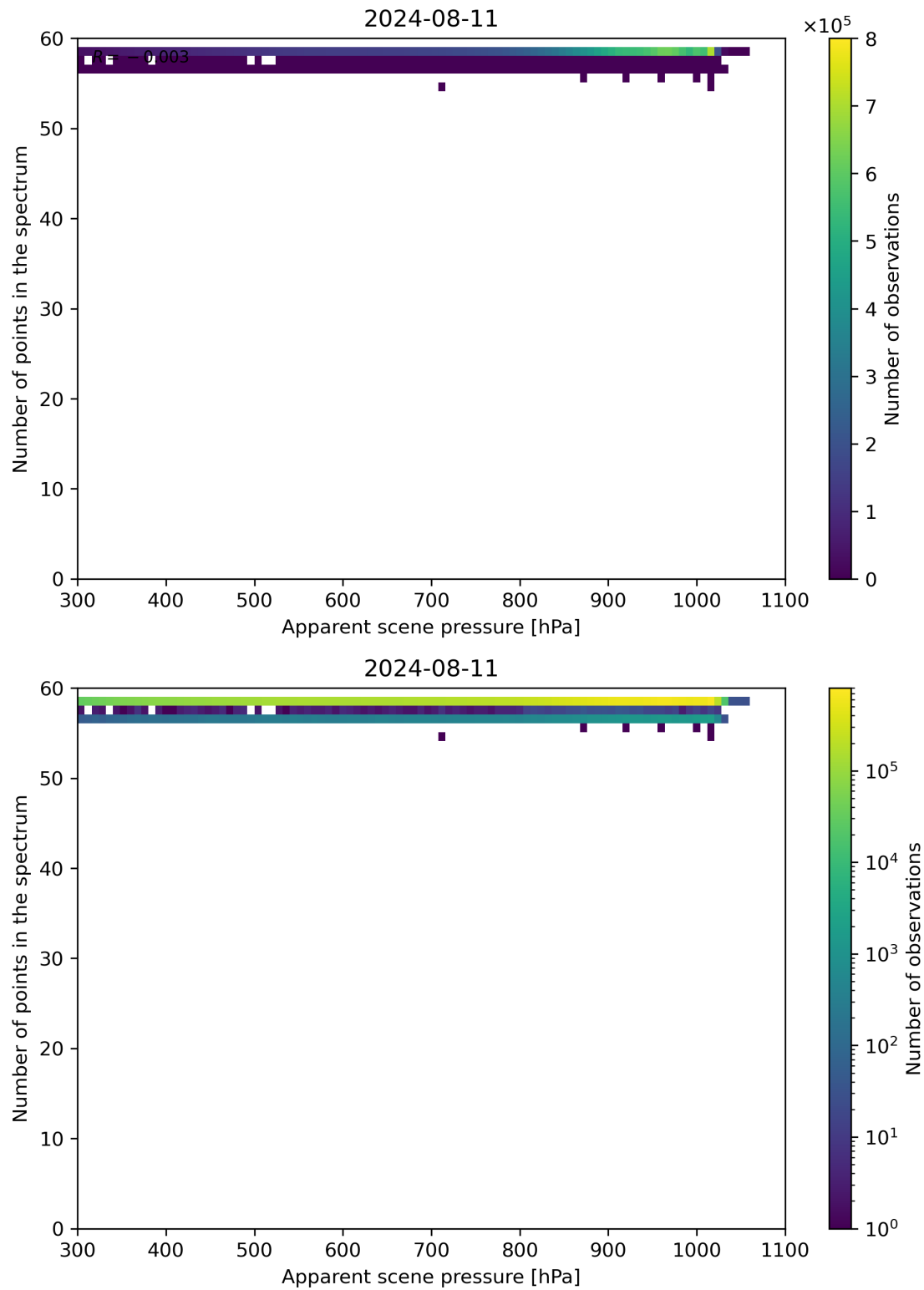
Figure 66: Scatter density plot of “Apparent scene pressure” against “Number of points in the spectrum” for 2024-08-11 to 2024-08-11.
