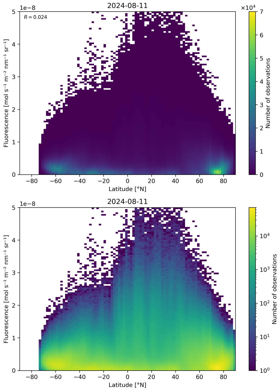
Figure 92: Scatter density plot of “Latitude” against “Fluorescence” for 2024-08-11 to 2024-08-11.
