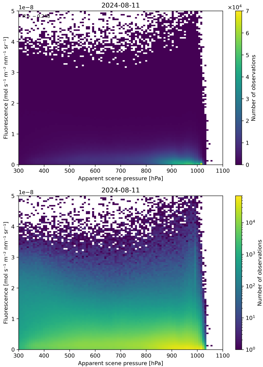
Figure 64: Scatter density plot of “Apparent scene pressure” against “Fluorescence” for 2024-08-11 to 2024-08-11.
