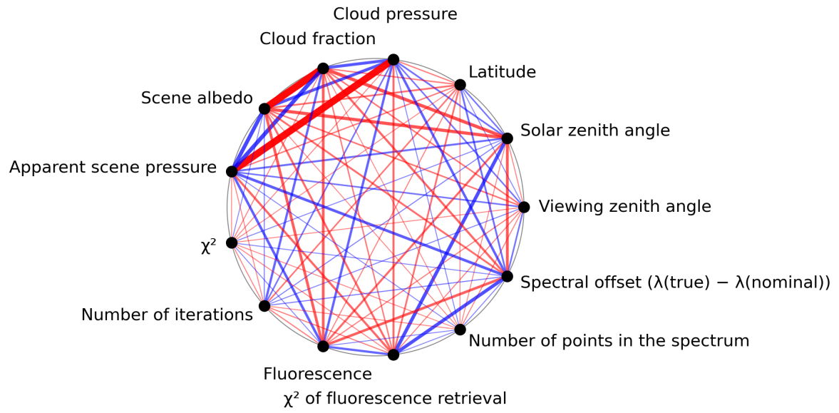
Figure 1: Map of correlation graph for 2024-08-11 to 2024-08-11.
