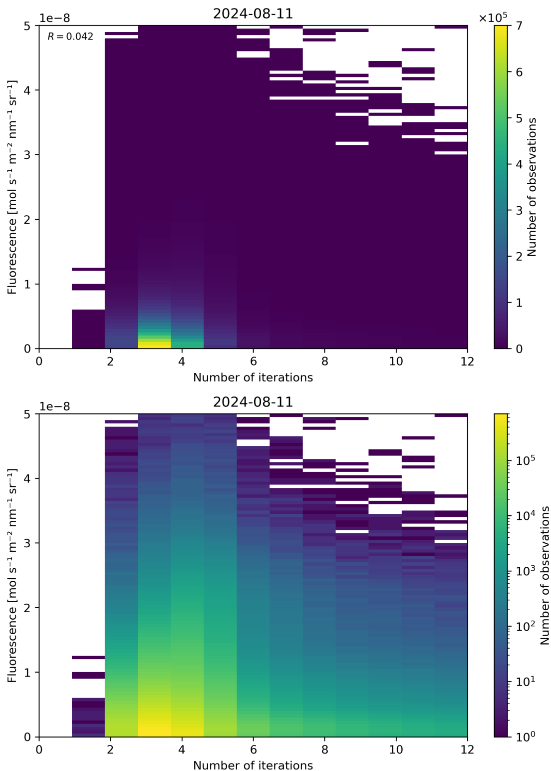
Figure 98: Scatter density plot of “Number of iterations” against “Fluorescence” for 2024-08-11 to 2024-08-11.
