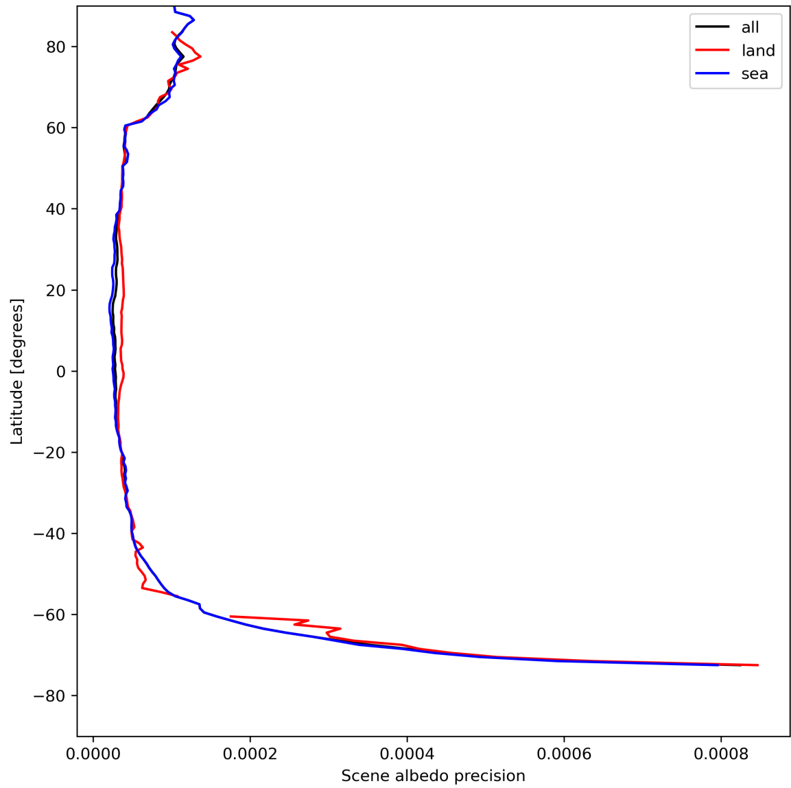
Figure 18: Zonal average of "Scene albedo precision" for 2024-08-11 to 2024-08-11.
