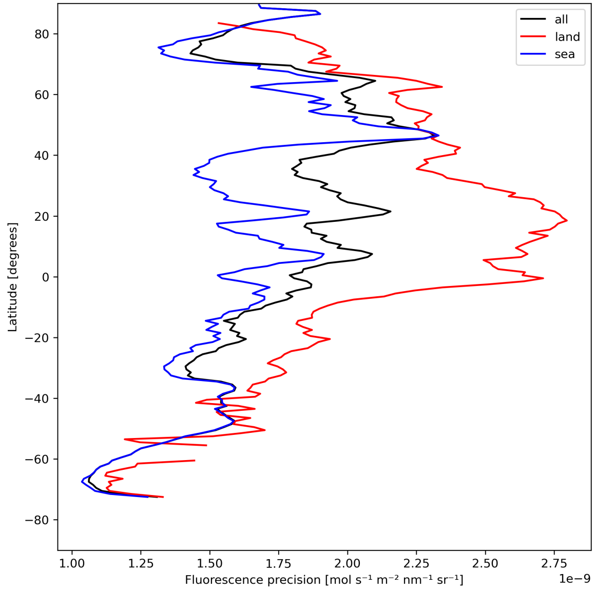
Figure 24: Zonal average of “Fluorescence precision” for 2024-08-11 to 2024-08-11.
