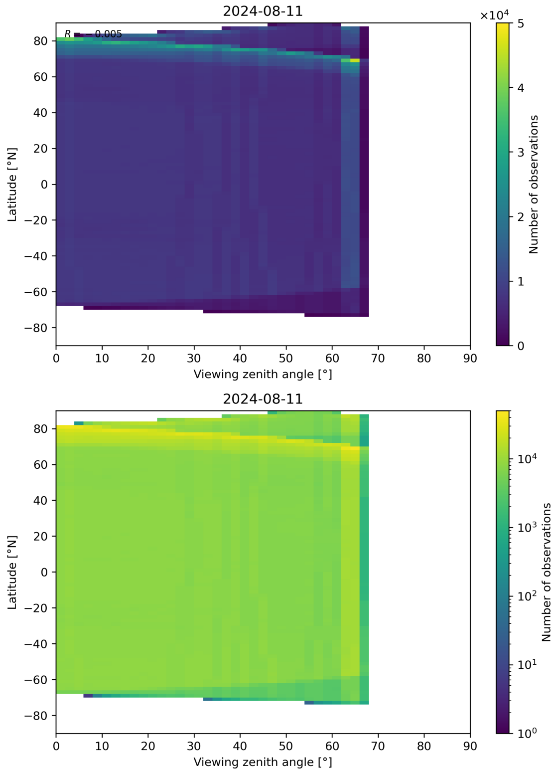
Figure 123: Scatter density plot of “Viewing zenith angle” against “Latitude” for 2024-08-11 to 2024-08-11.
