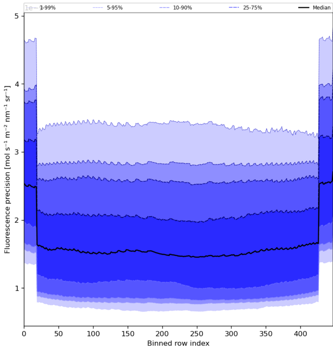
Figure 58: Along track statistics of “Fluorescence precision” for 2024-08-11 to 2024-08-11
