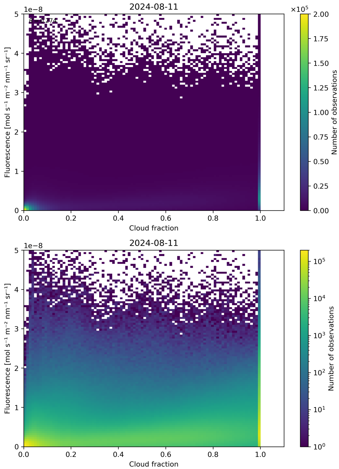
Figure 72: Scatter density plot of “Cloud fraction” against “Fluorescence” for 2024-08-11 to 2024-08-11.
