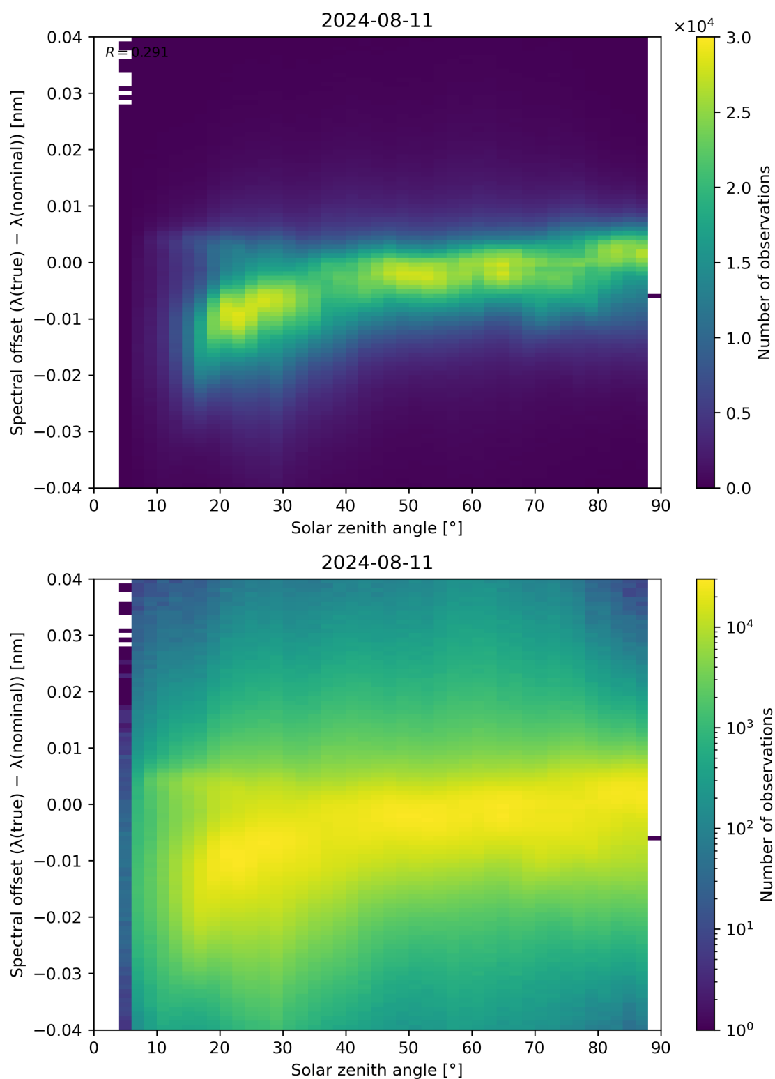
Figure 117: Scatter density plot of “Solar zenith angle” against “Spectral offset ( \lambda(\text{true}) - \lambda(\text{nominal}) )” for 2024-08-11 to 2024-08-11.
