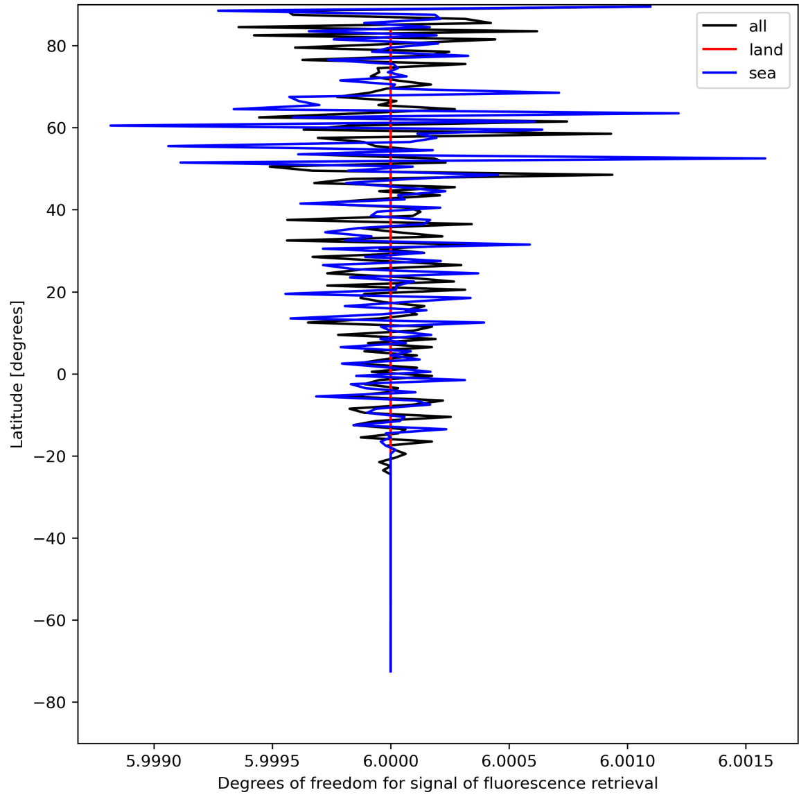
Figure 26: Zonal average of “Degrees of freedom for signal of fluorescence retrieval” for 2024-08-11 to 2024-08-11.
