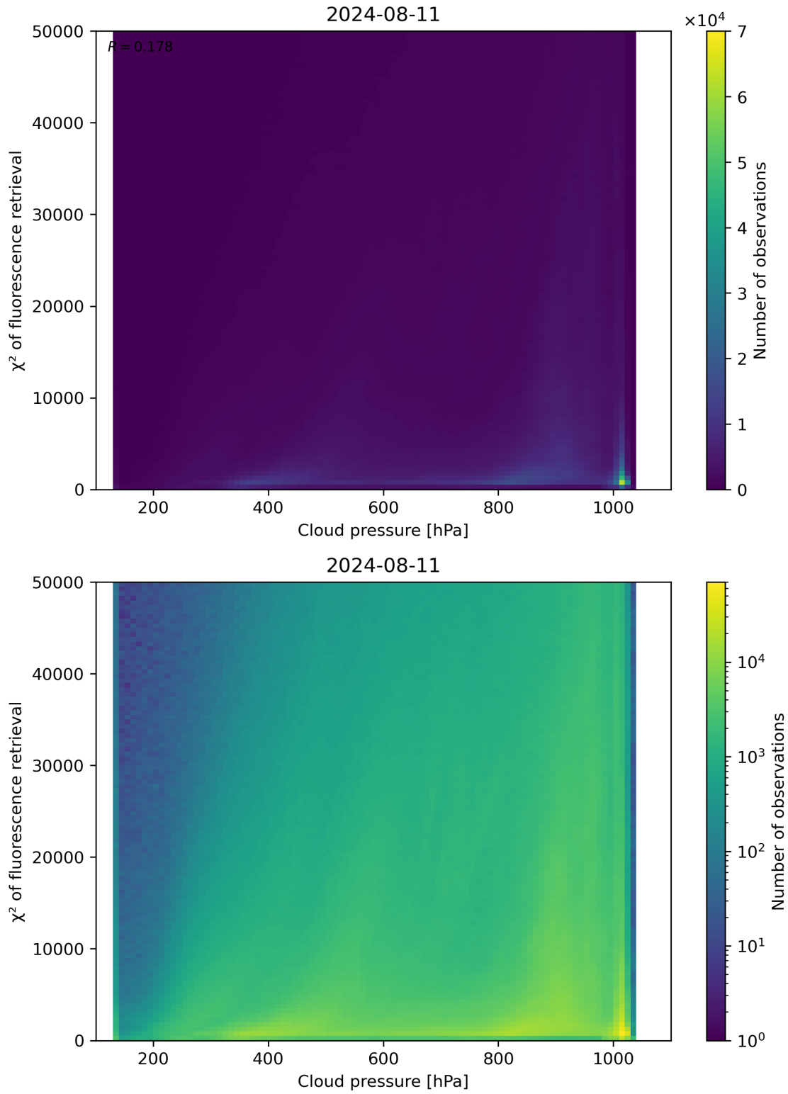
Figure 78: Scatter density plot of “Cloud pressure” against “ \chi^2 of fluorescence retrieval” for 2024-08-11 to 2024-08-11.
