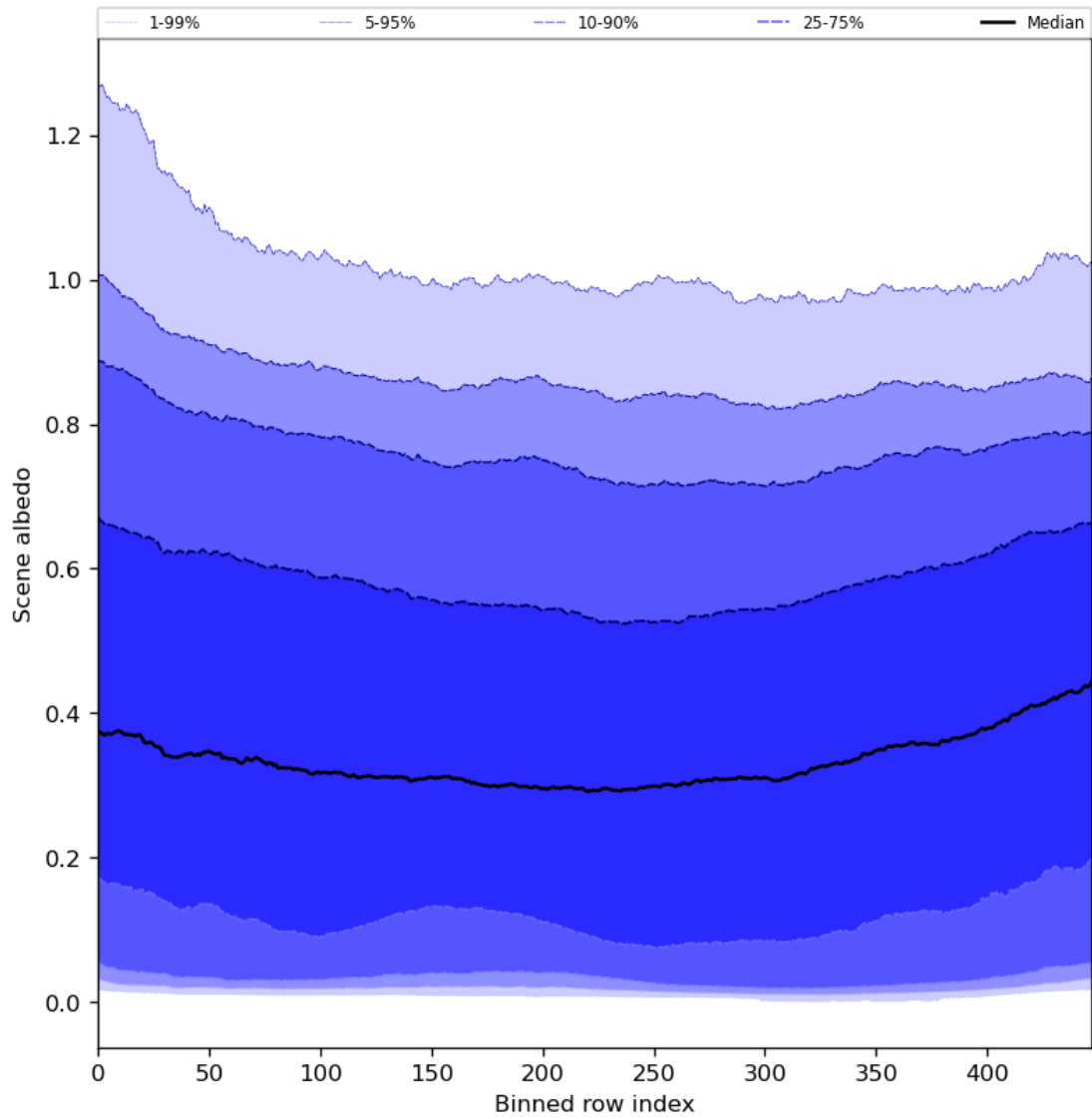
Figure 51: Along track statistics of “Scene albedo” for 2024-08-11 to 2024-08-11
