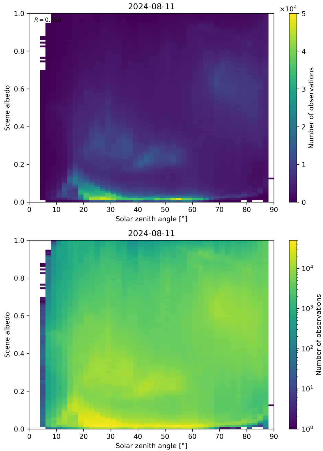
Figure 116: Scatter density plot of “Solar zenith angle” against “Scene albedo” for 2024-08-11 to 2024-08-11.
