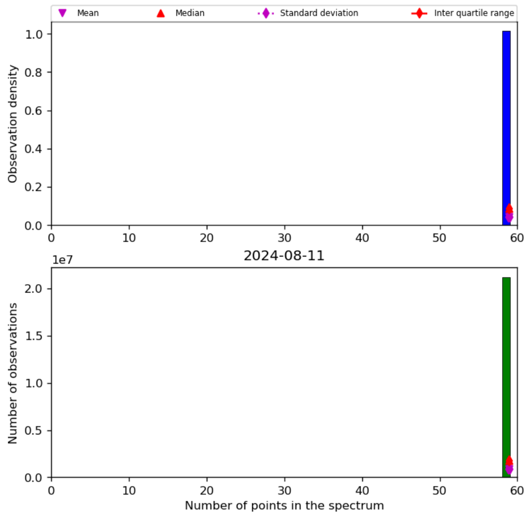
Figure 44: Histogram of “Number of points in the spectrum” for 2024-08-11 to 2024-08-11
