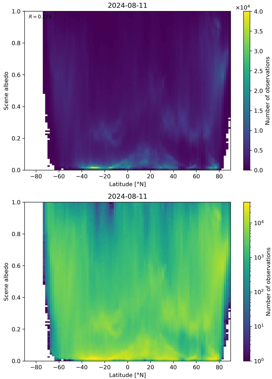
Figure 95: Scatter density plot of “Latitude” against “Scene albedo” for 2024-08-11 to 2024-08-11.
