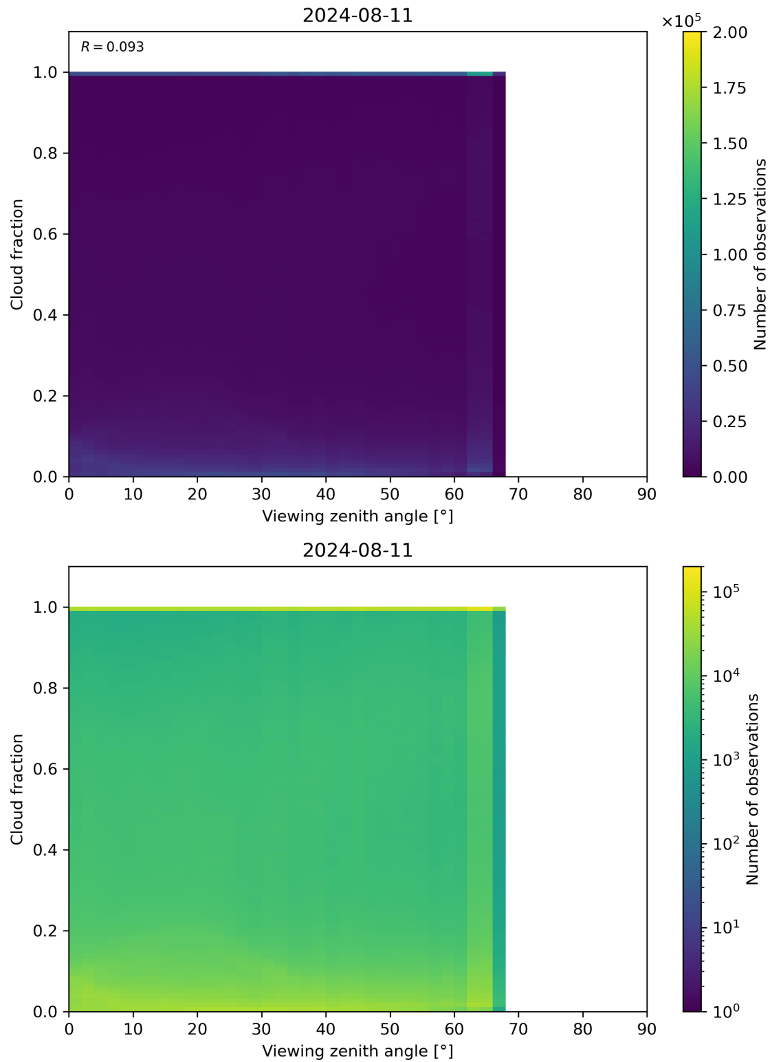
Figure 120: Scatter density plot of “Viewing zenith angle” against “Cloud fraction” for 2024-08-11 to 2024-08-11.
