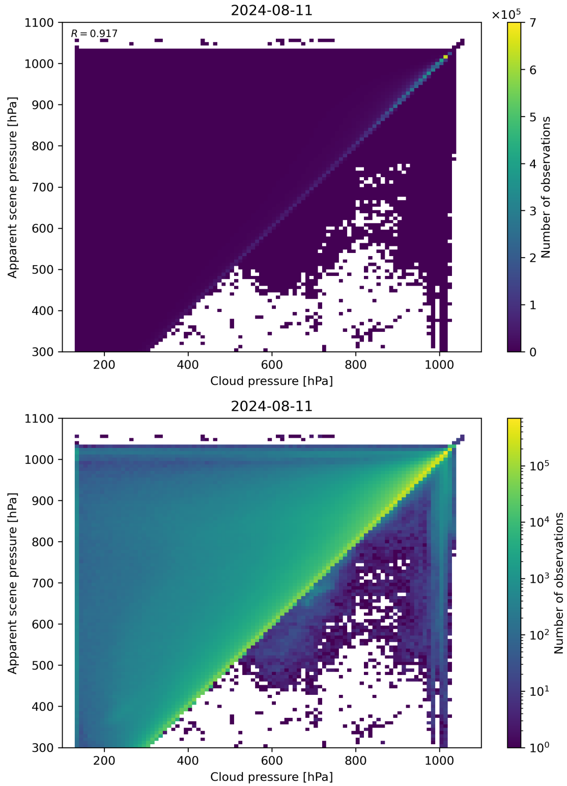
Figure 77: Scatter density plot of “Cloud pressure” against “Apparent scene pressure” for 2024-08-11 to 2024-08-11.
