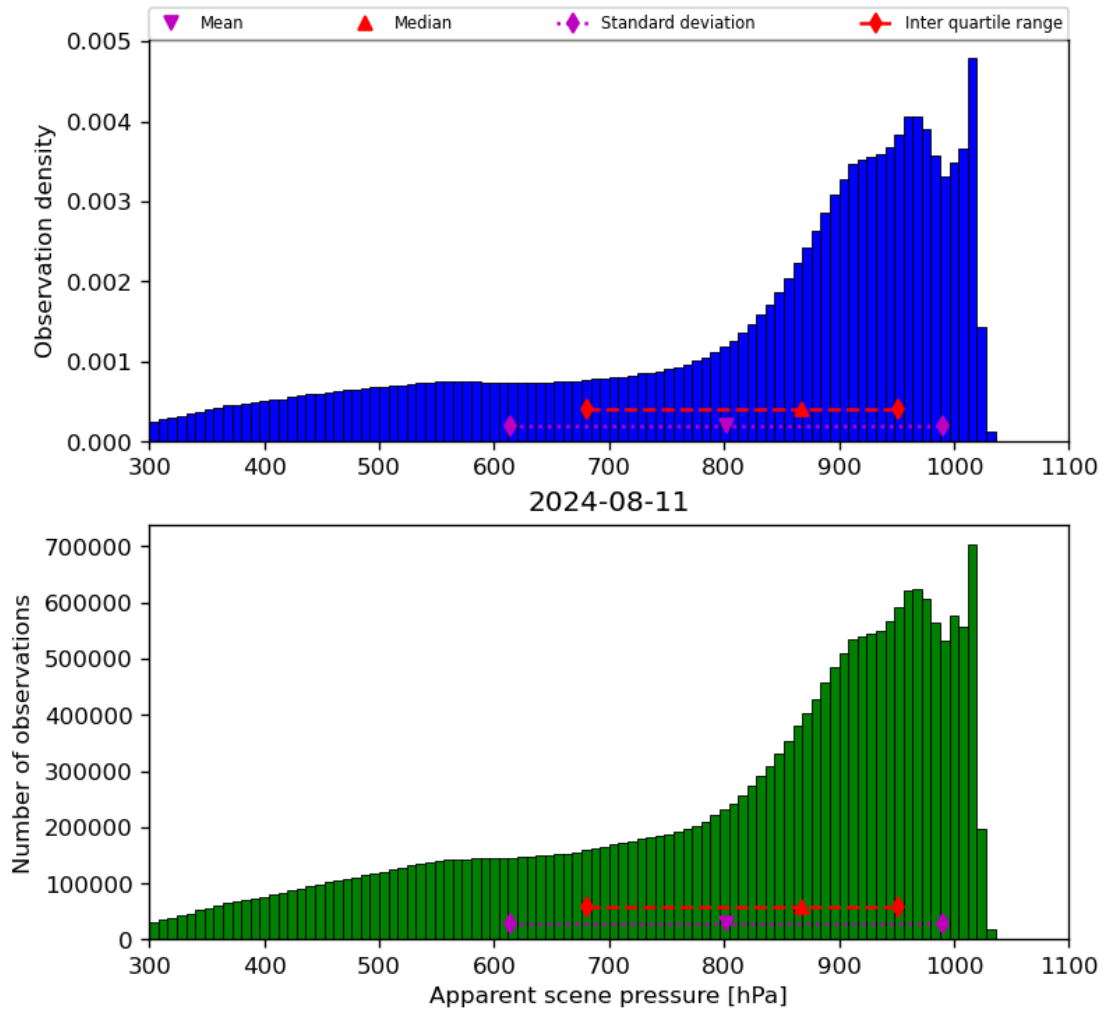
Figure 36: Histogram of “Apparent scene pressure” for 2024-08-11 to 2024-08-11
