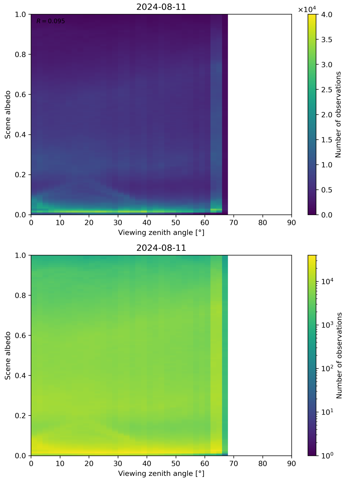
Figure 126: Scatter density plot of “Viewing zenith angle” against “Scene albedo” for 2024-08-11 to 2024-08-11.
