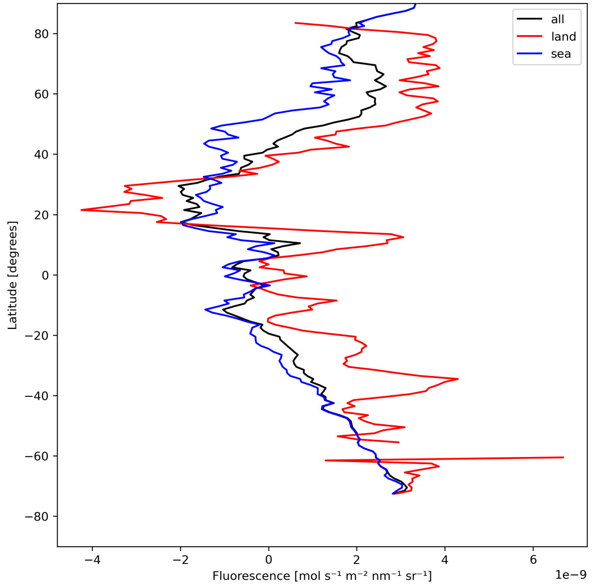
Figure 23: Zonal average of “Fluorescence” for 2024-08-11 to 2024-08-11.
