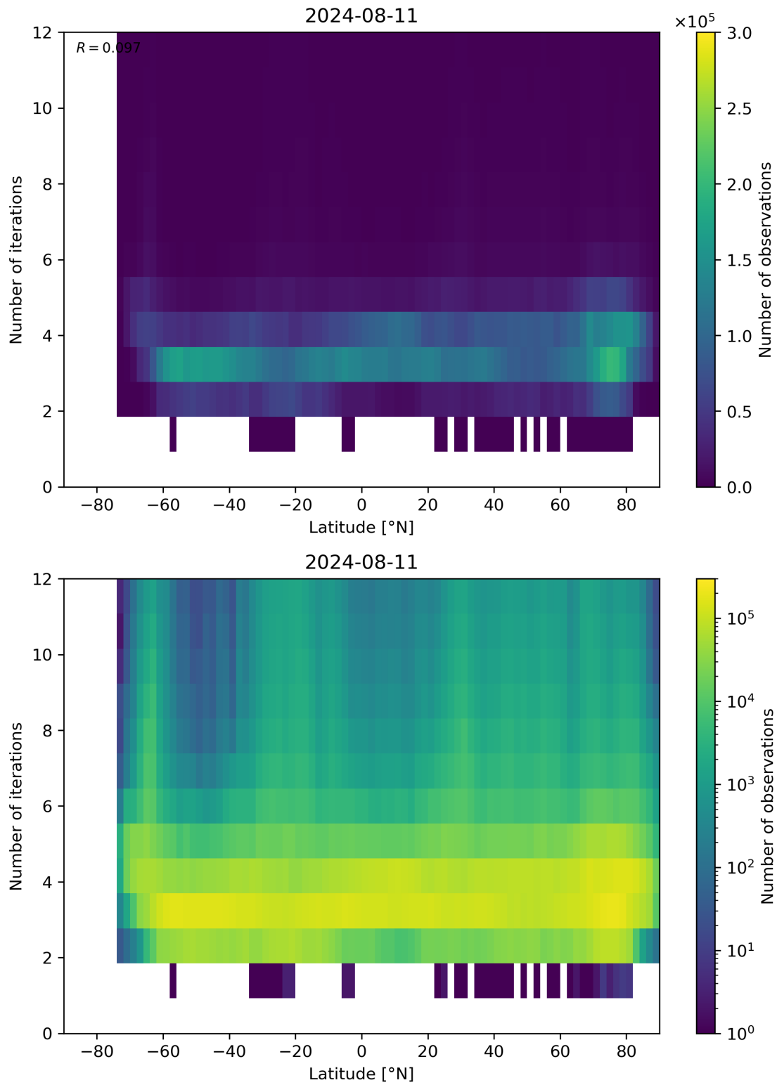
Figure 93: Scatter density plot of “Latitude” against “Number of iterations” for 2024-08-11 to 2024-08-11.
