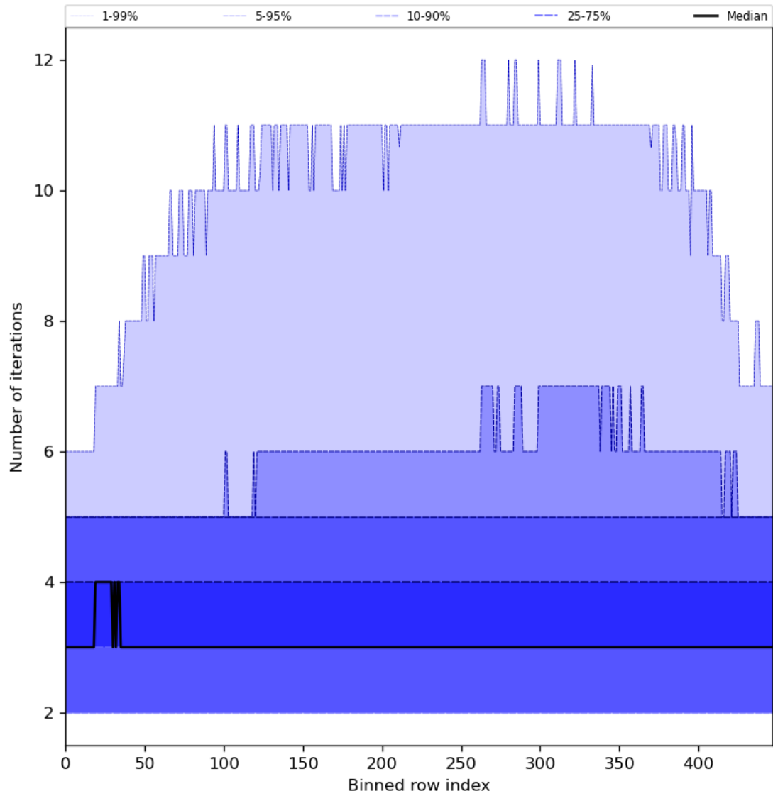
Figure 56: Along track statistics of “Number of iterations” for 2024-08-11 to 2024-08-11
