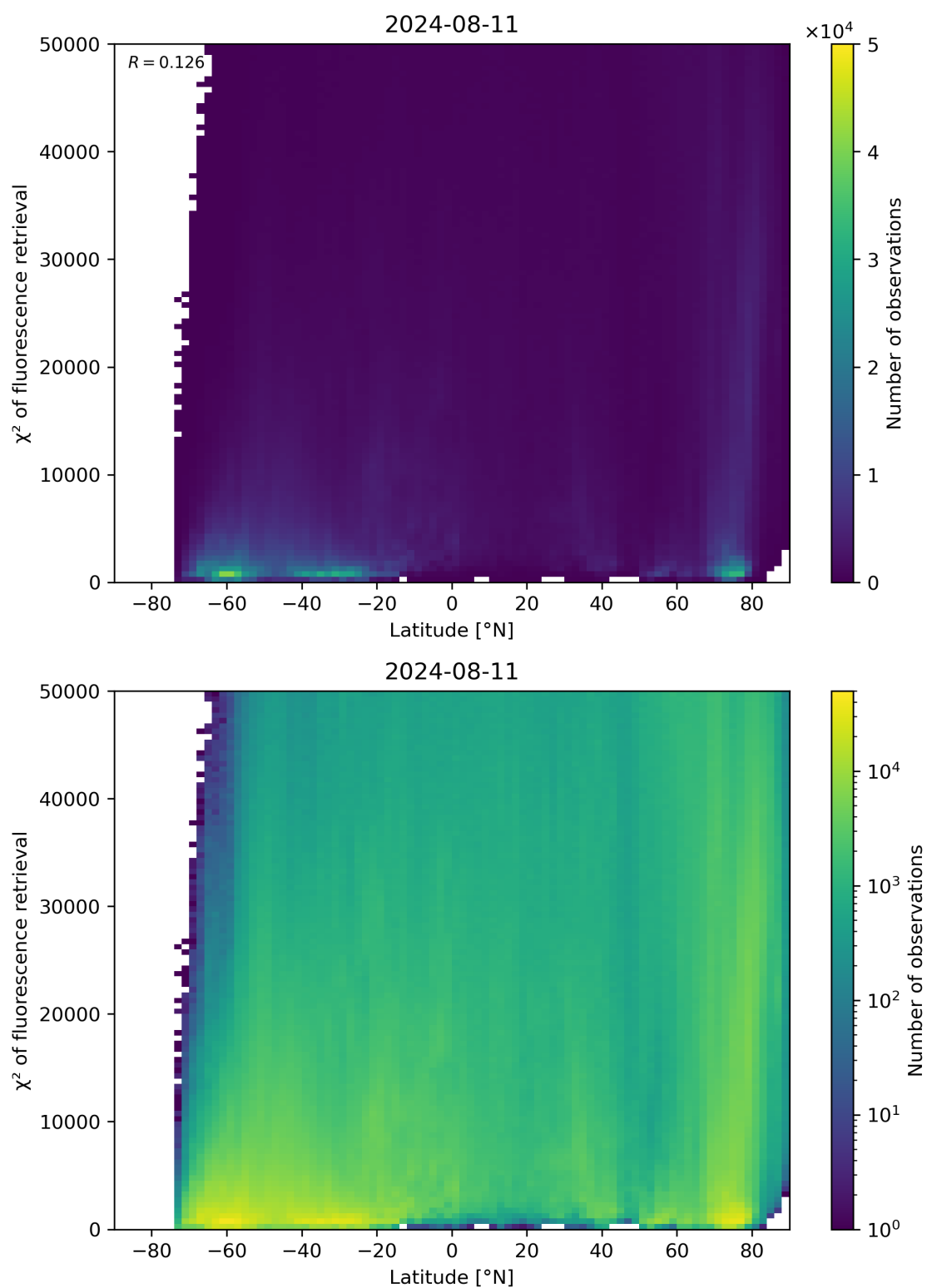
Figure 89: Scatter density plot of “Latitude” against “ \chi^2 of fluorescence retrieval” for 2024-08-11 to 2024-08-11.
