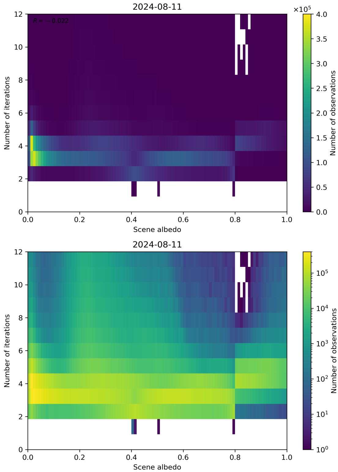
Figure 105: Scatter density plot of “Scene albedo” against “Number of iterations” for 2024-08-11 to 2024-08-11.
