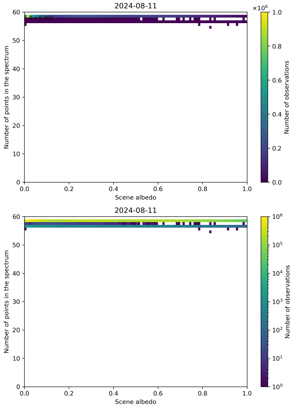
Figure 106: Scatter density plot of “Scene albedo” against “Number of points in the spectrum” for 2024-08-11 to 2024-08-11.
