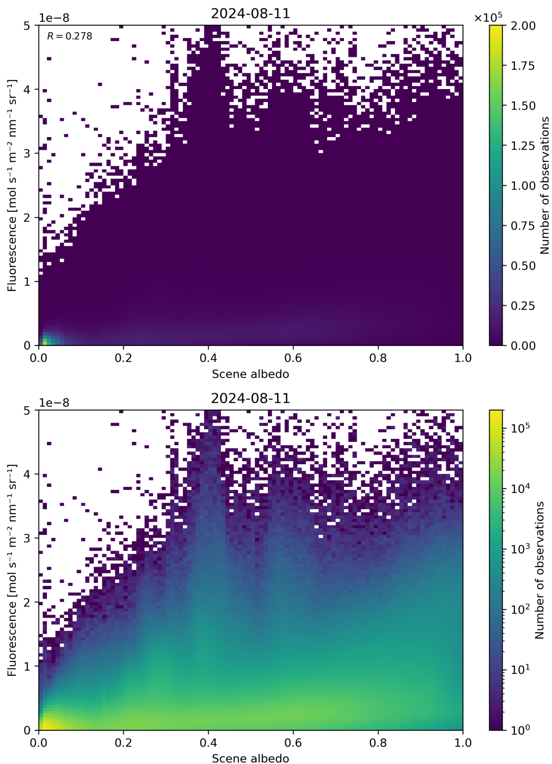
Figure 104: Scatter density plot of “Scene albedo” against “Fluorescence” for 2024-08-11 to 2024-08-11.
