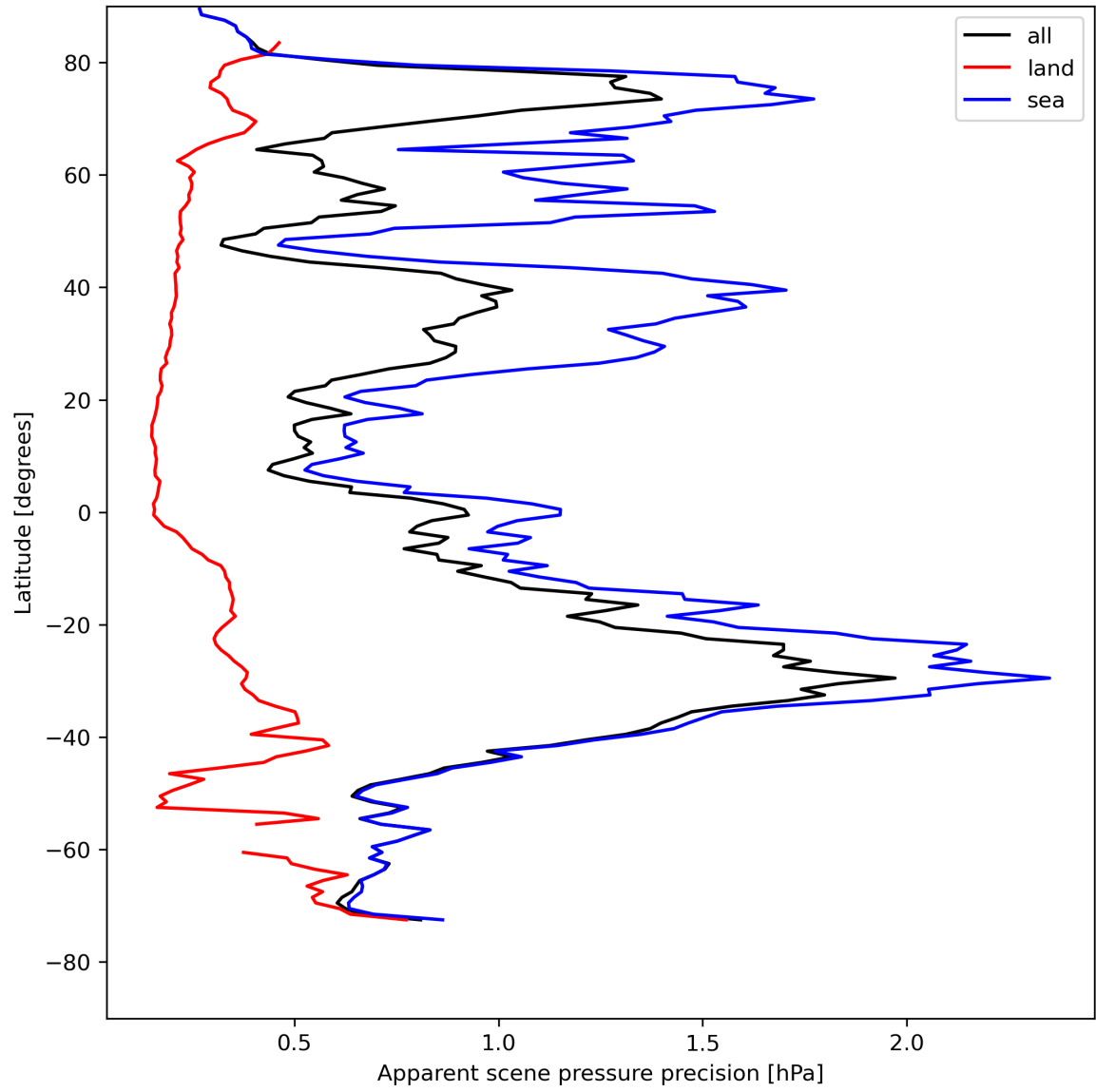
Figure 20: Zonal average of “Apparent scene pressure precision” for 2024-08-11 to 2024-08-11.
