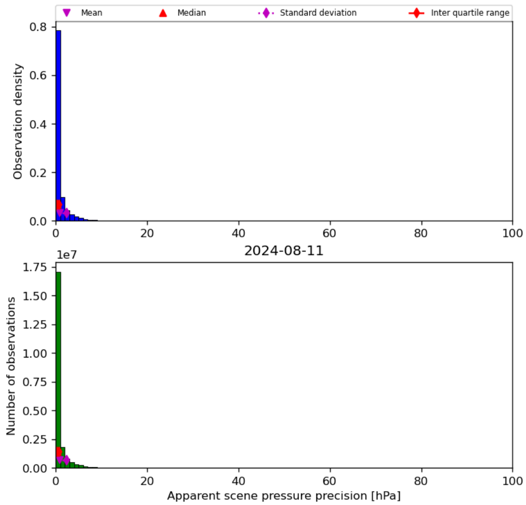
Figure 37: Histogram of “Apparent scene pressure precision” for 2024-08-11 to 2024-08-11
