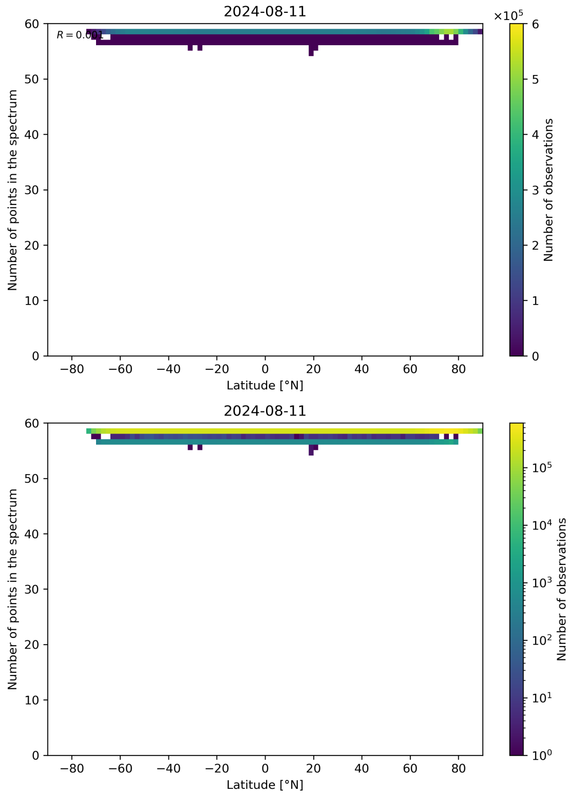
Figure 94: Scatter density plot of “Latitude” against “Number of points in the spectrum” for 2024-08-11 to 2024-08-11.
