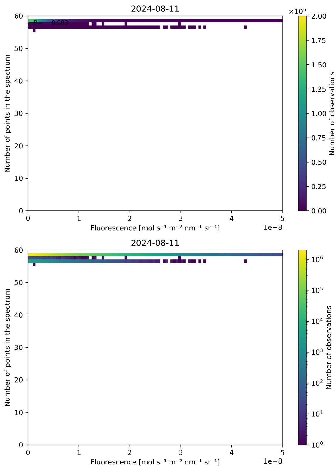
Figure 86: Scatter density plot of “Fluorescence” against “Number of points in the spectrum” for 2024-08-11 to 2024-08-11.
