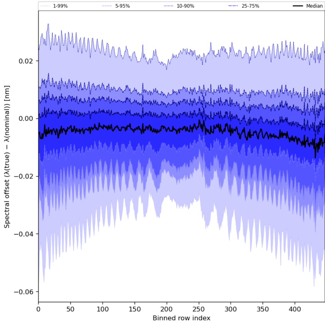
Figure 62: Along track statistics of “Spectral offset ( \lambda(\text{true}) - \lambda(\text{nominal}) )” for 2024-08-11 to 2024-08-11
