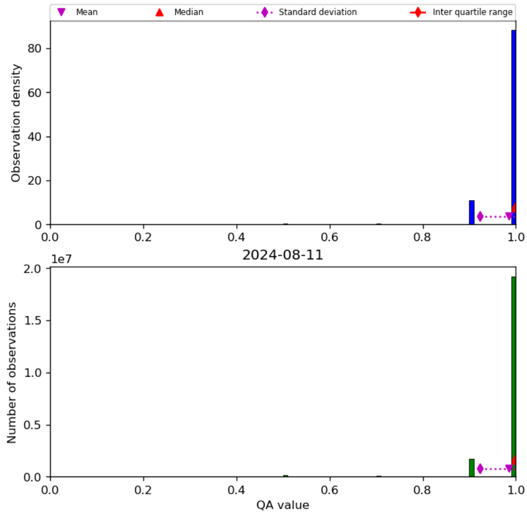
Figure 29: Histogram of “QA value” for 2024-08-11 to 2024-08-11
