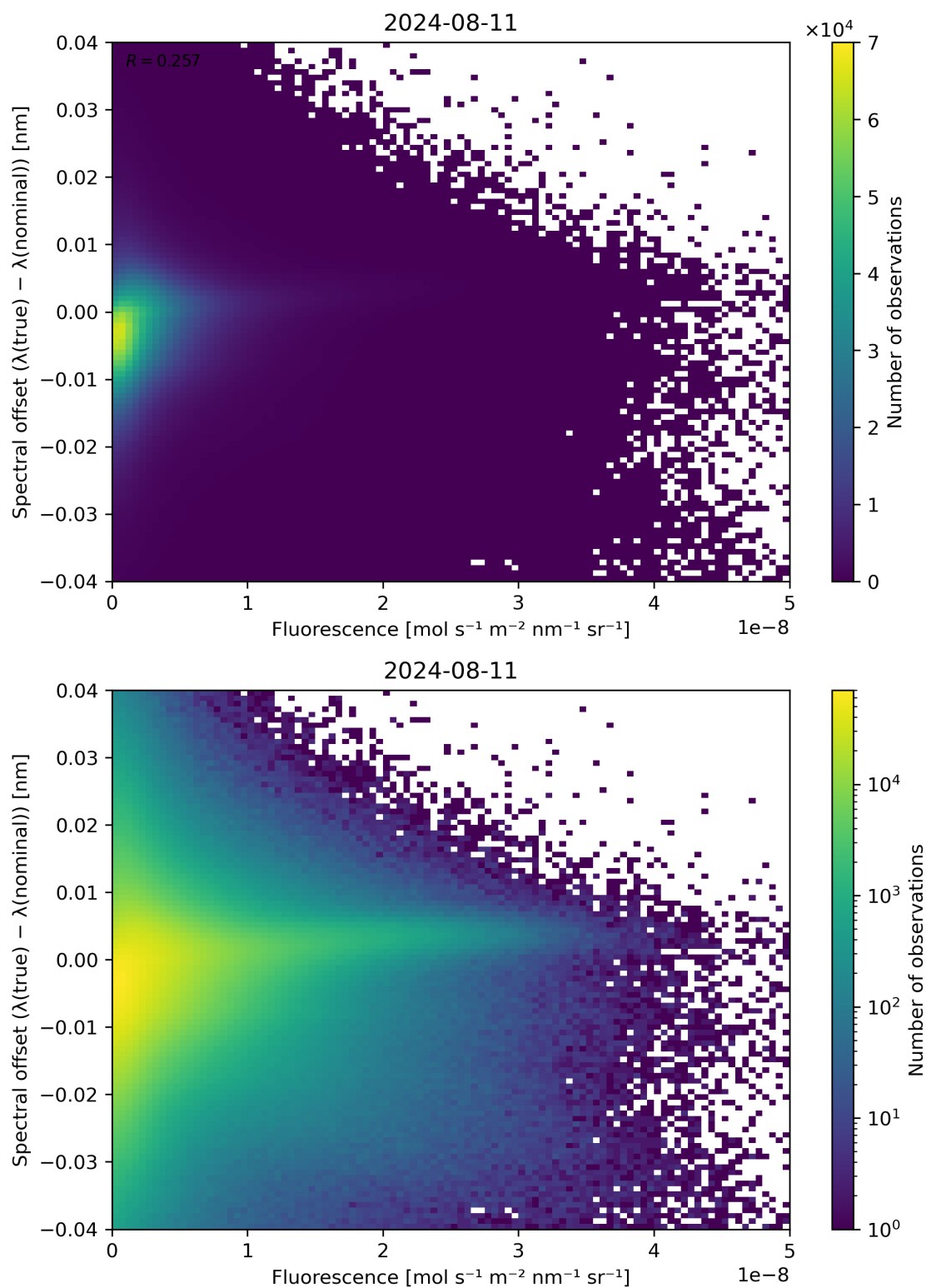
Figure 87: Scatter density plot of “Fluorescence” against “Spectral offset ( \lambda(\text{true}) - \lambda(\text{nominal}) )” for 2024-08-11 to 2024-08-11.
