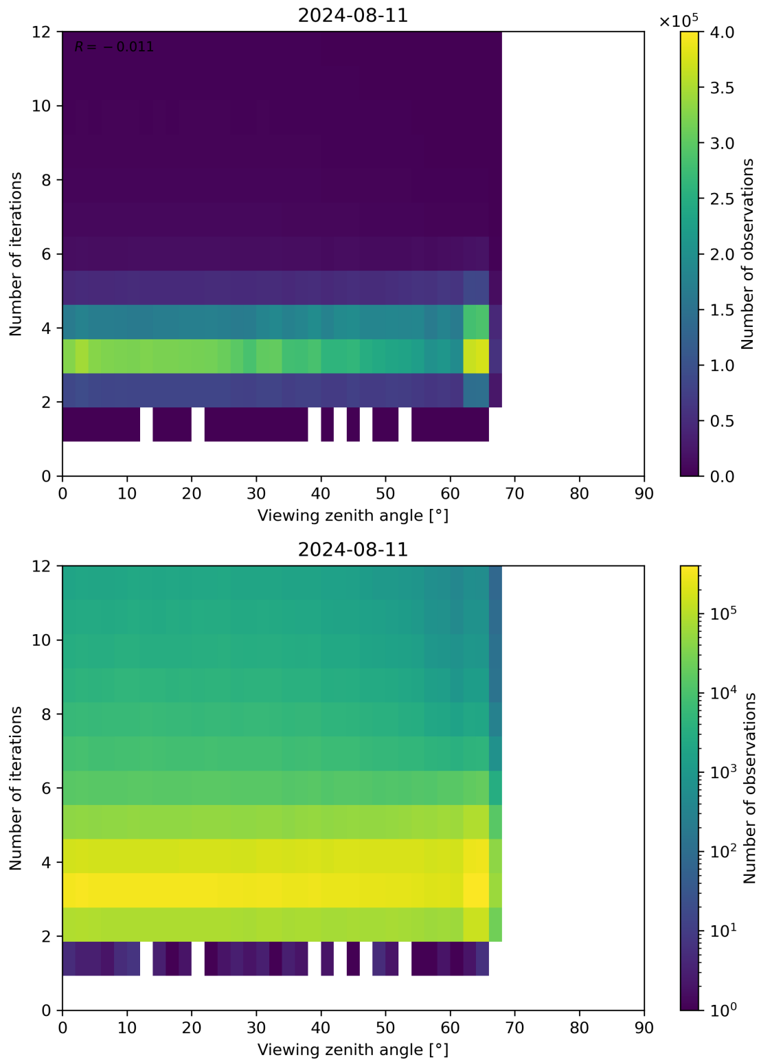
Figure 124: Scatter density plot of “Viewing zenith angle” against “Number of iterations” for 2024-08-11 to 2024-08-11.
