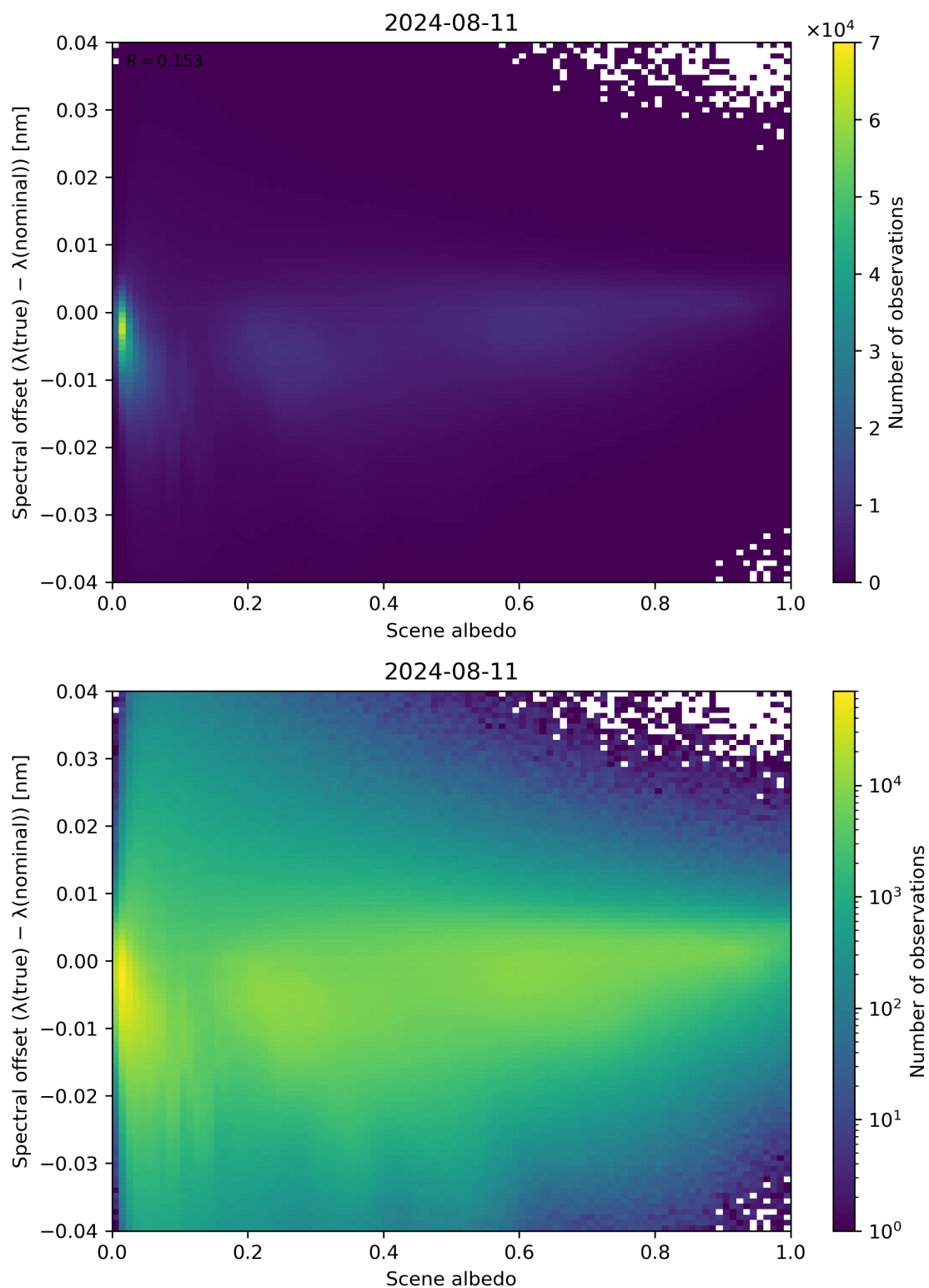
Figure 107: Scatter density plot of “Scene albedo” against “Spectral offset ( \lambda(\text{true}) - \lambda(\text{nominal}) )” for 2024-08-11 to 2024-08-11.
