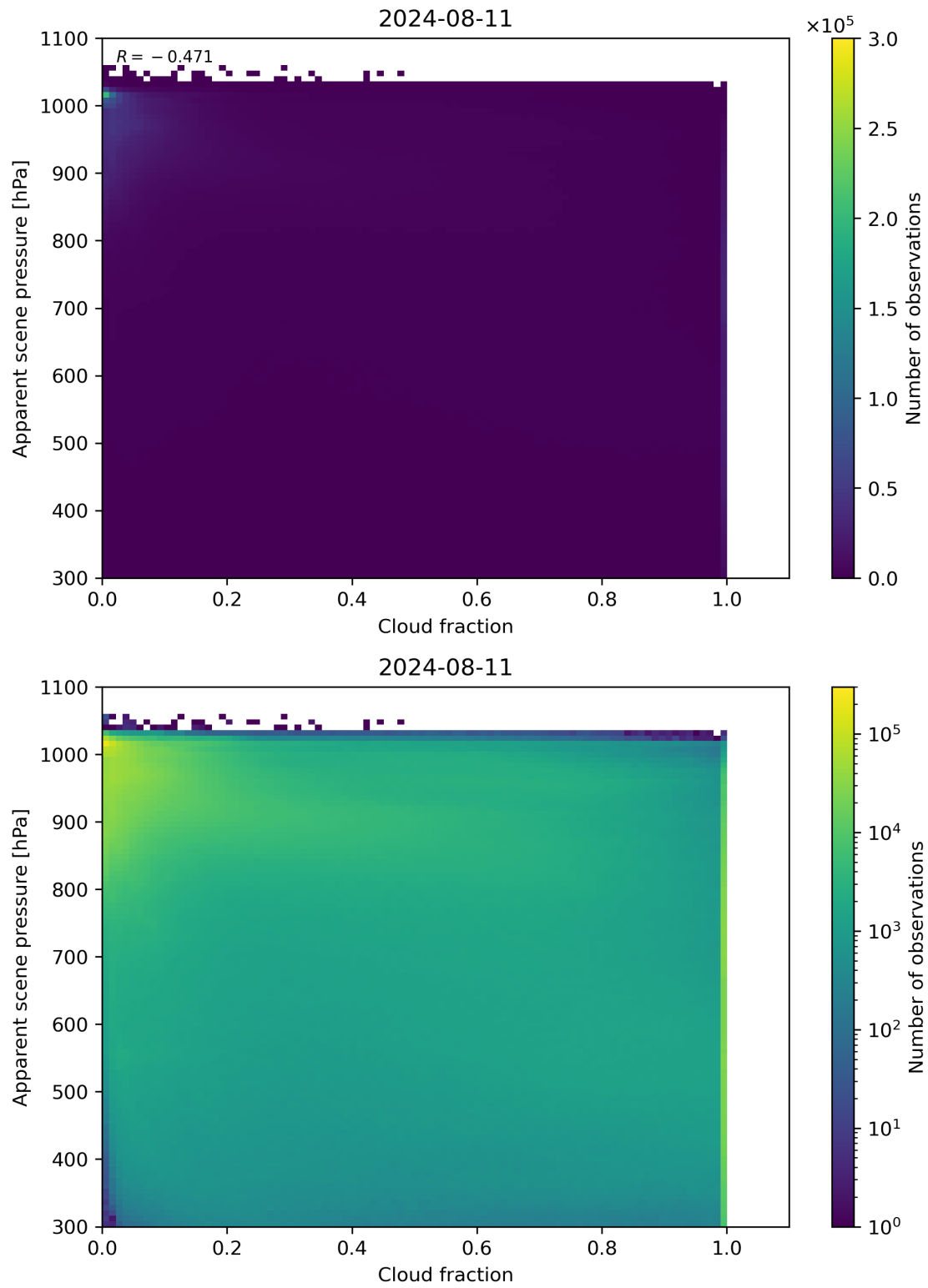
Figure 70: Scatter density plot of “Cloud fraction” against “Apparent scene pressure” for 2024-08-11 to 2024-08-11.
