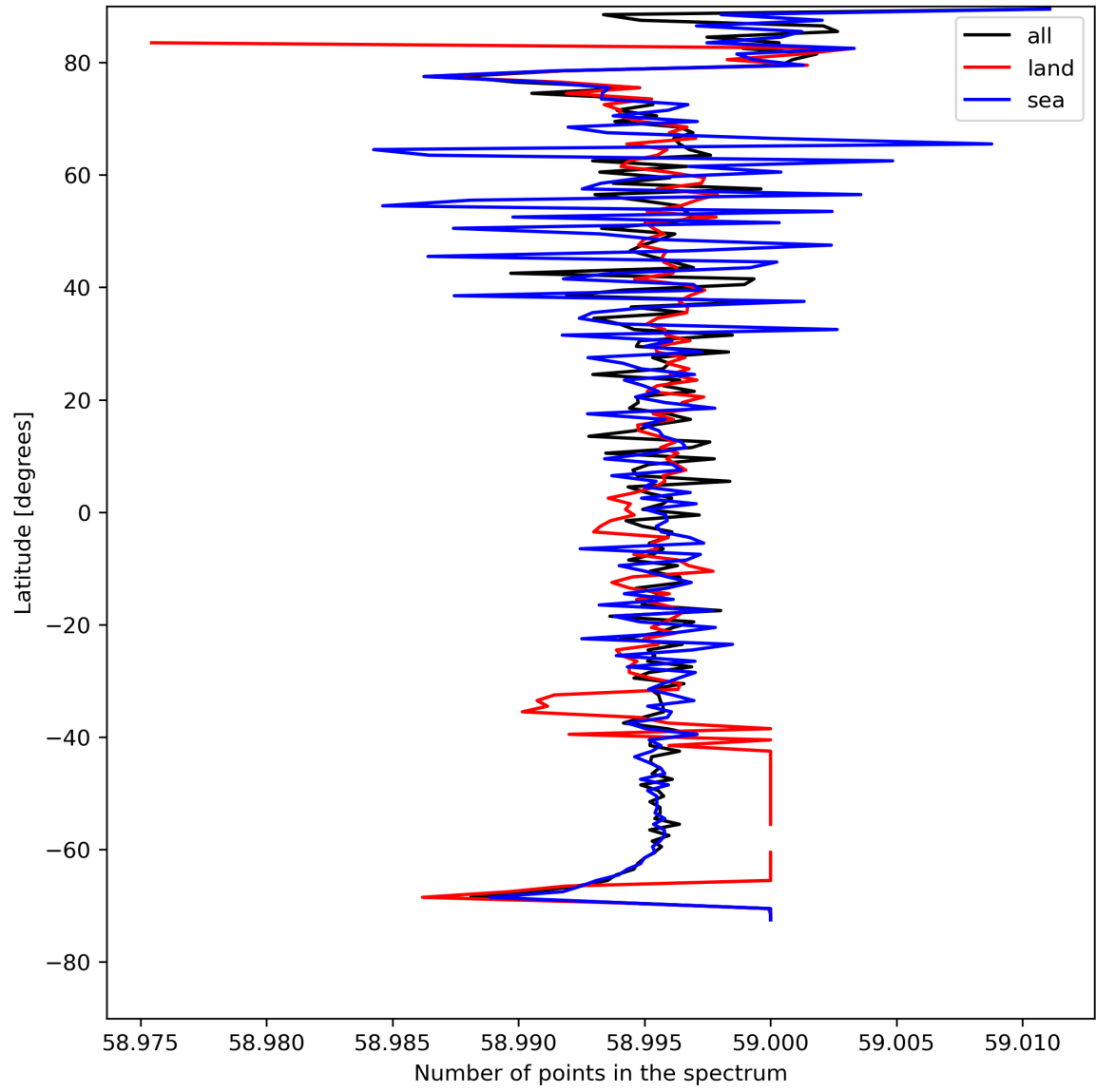
Figure 27: Zonal average of “Number of points in the spectrum” for 2024-08-11 to 2024-08-11.
