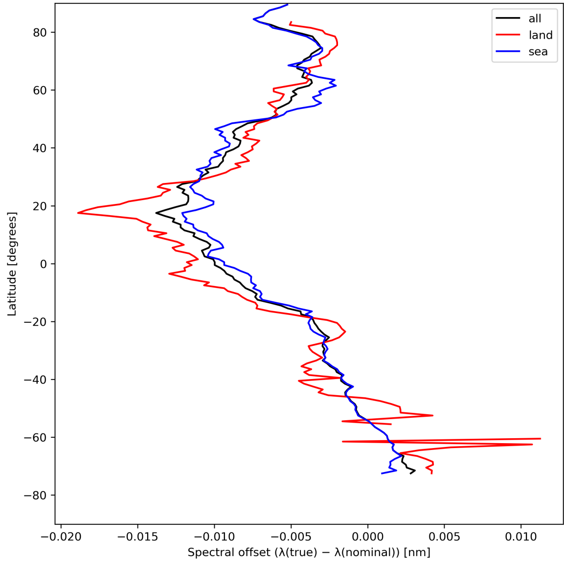
Figure 28: Zonal average of “Spectral offset ( \lambda(\text{true}) - \lambda(\text{nominal}) )” for 2024-08-11 to 2024-08-11.
