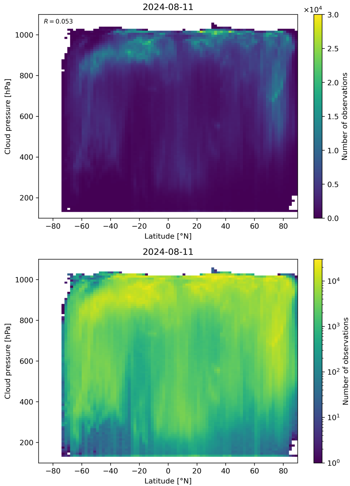
Figure 91: Scatter density plot of “Latitude” against “Cloud pressure” for 2024-08-11 to 2024-08-11.
