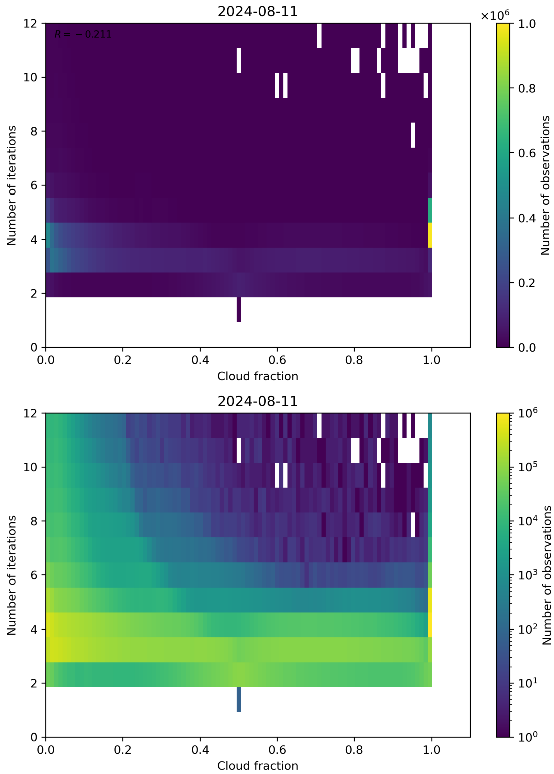
Figure 73: Scatter density plot of “Cloud fraction” against “Number of iterations” for 2024-08-11 to 2024-08-11.
