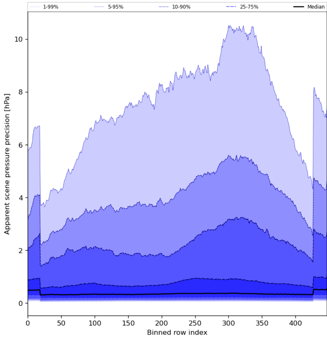
Figure 54: Along track statistics of “Apparent scene pressure precision” for 2024-08-11 to 2024-08-11
