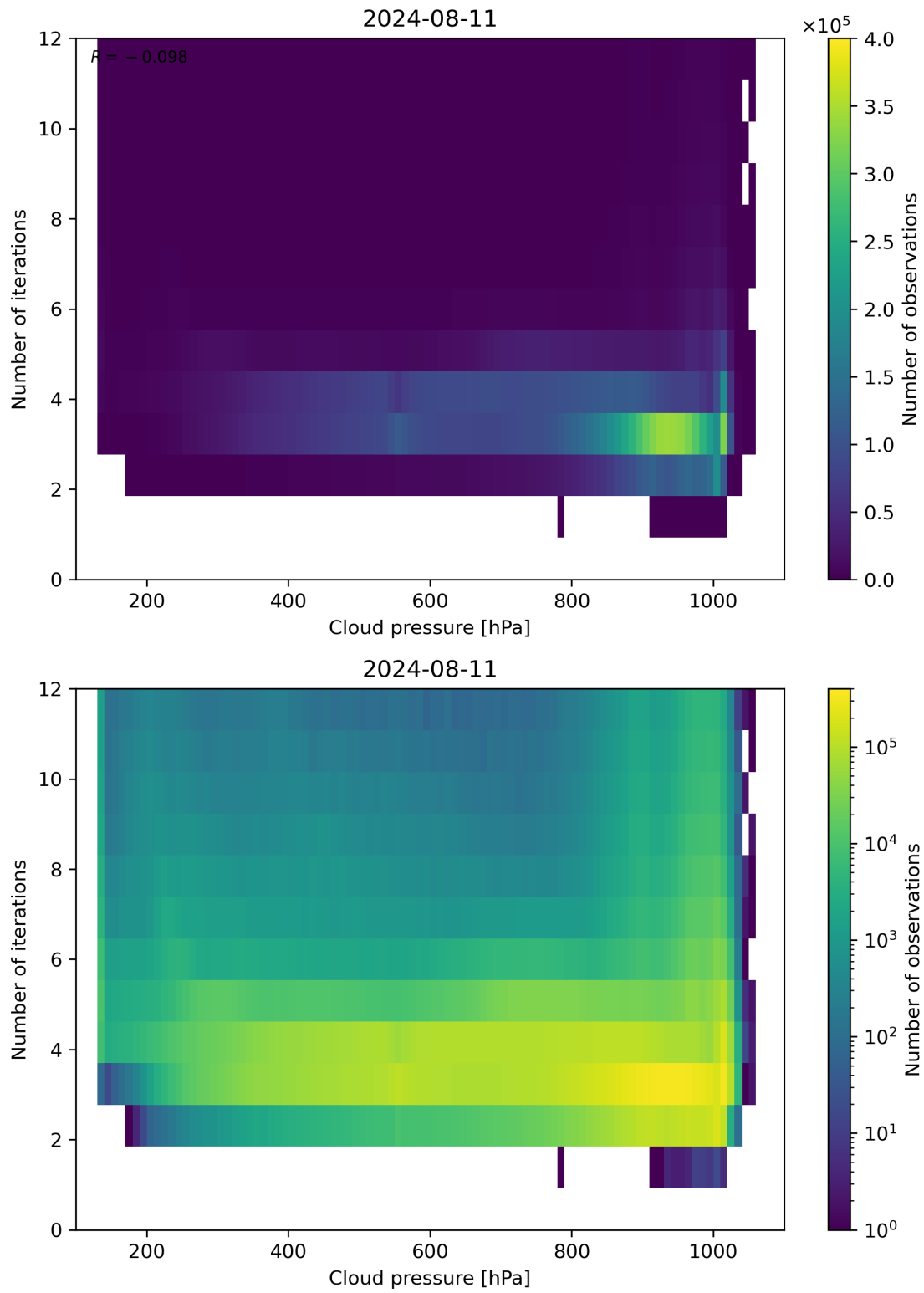
Figure 81: Scatter density plot of “Cloud pressure” against “Number of iterations” for 2024-08-11 to 2024-08-11.
