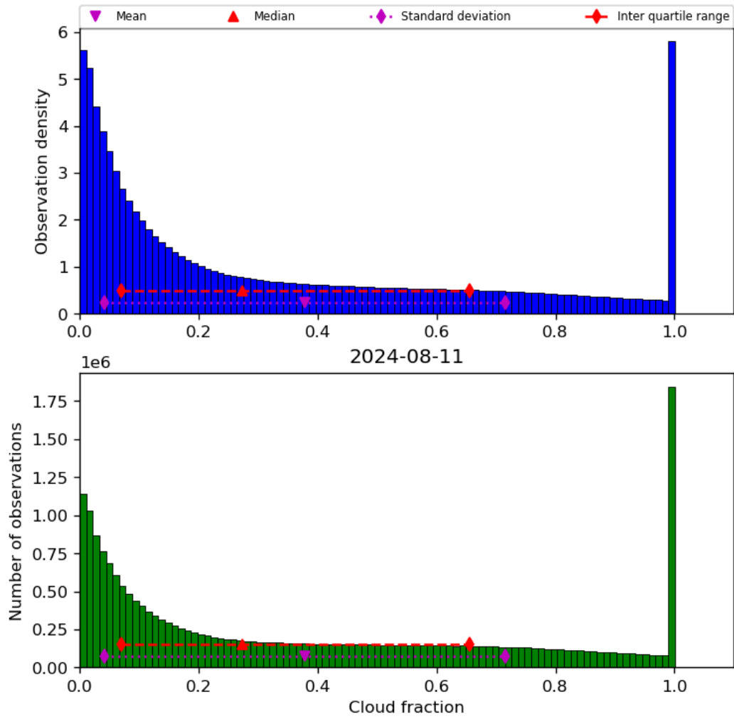
Figure 32: Histogram of “Cloud fraction” for 2024-08-11 to 2024-08-11
