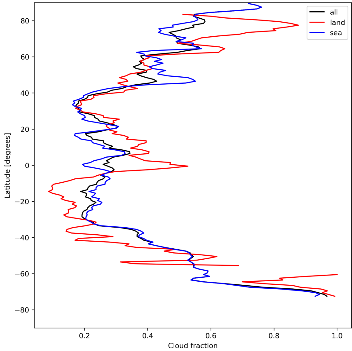
Figure 15: Zonal average of “Cloud fraction” for 2024-08-11 to 2024-08-11.
