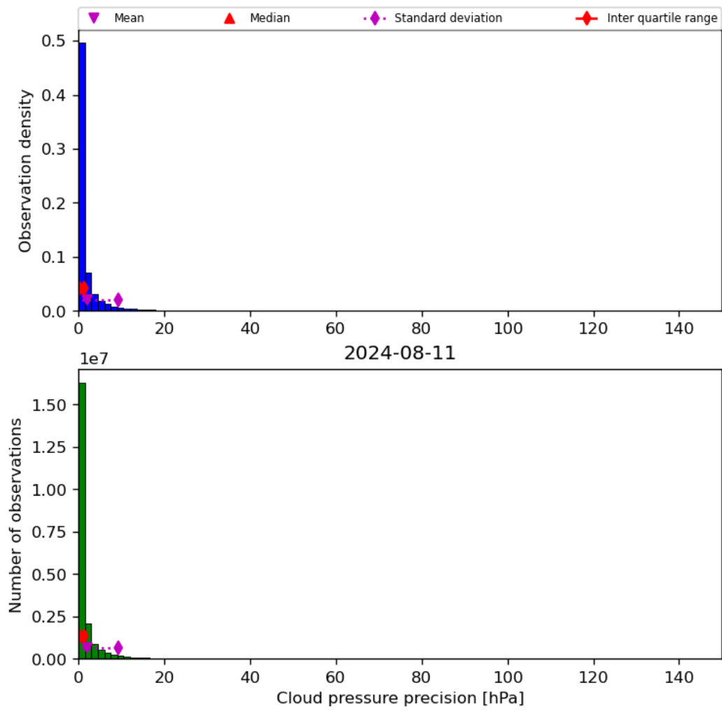
Figure 31: Histogram of “Cloud pressure precision” for 2024-08-11 to 2024-08-11
