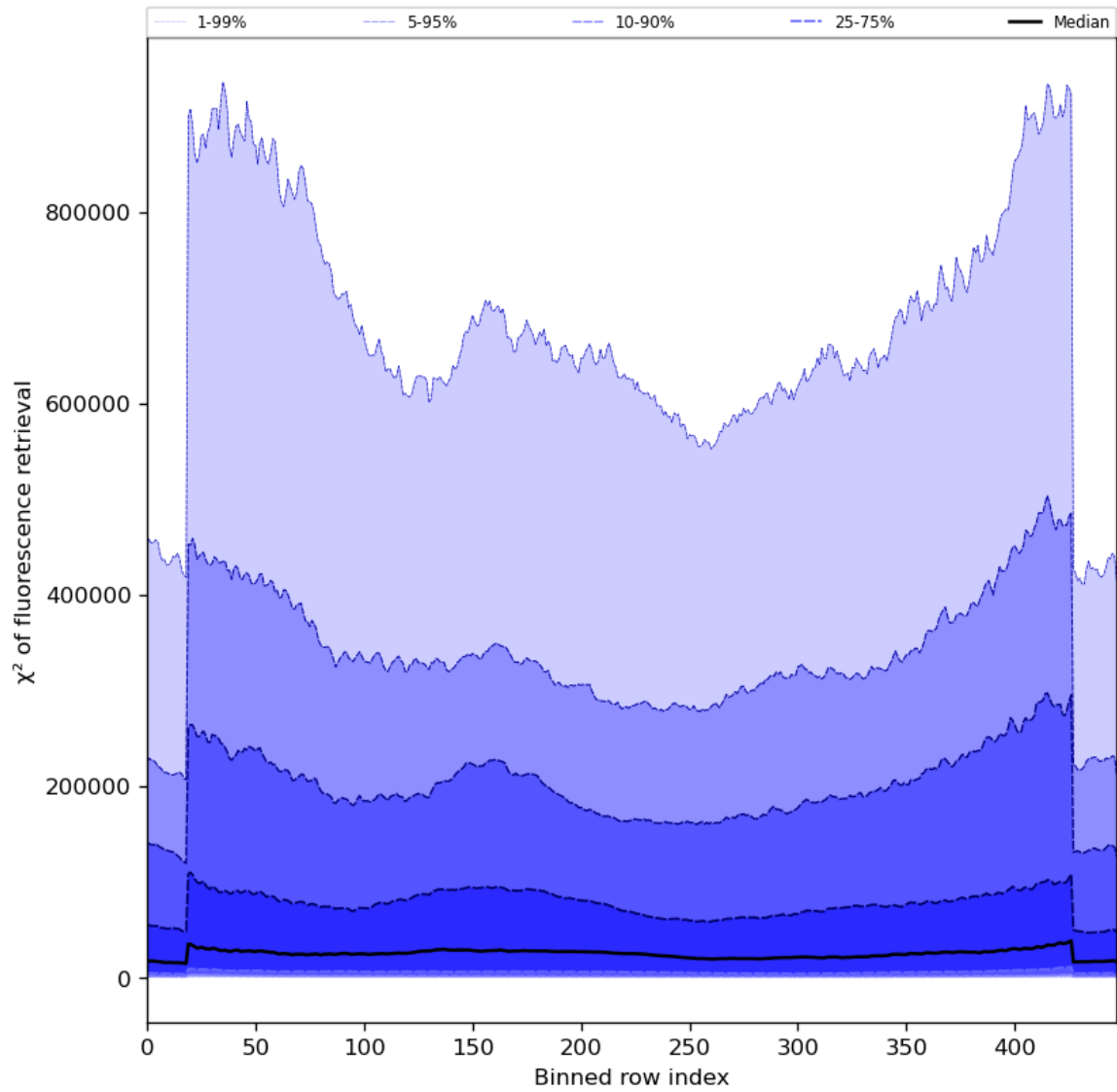
Figure 59: Along track statistics of “ \chi^2 of fluorescence retrieval” for 2024-08-11 to 2024-08-11
