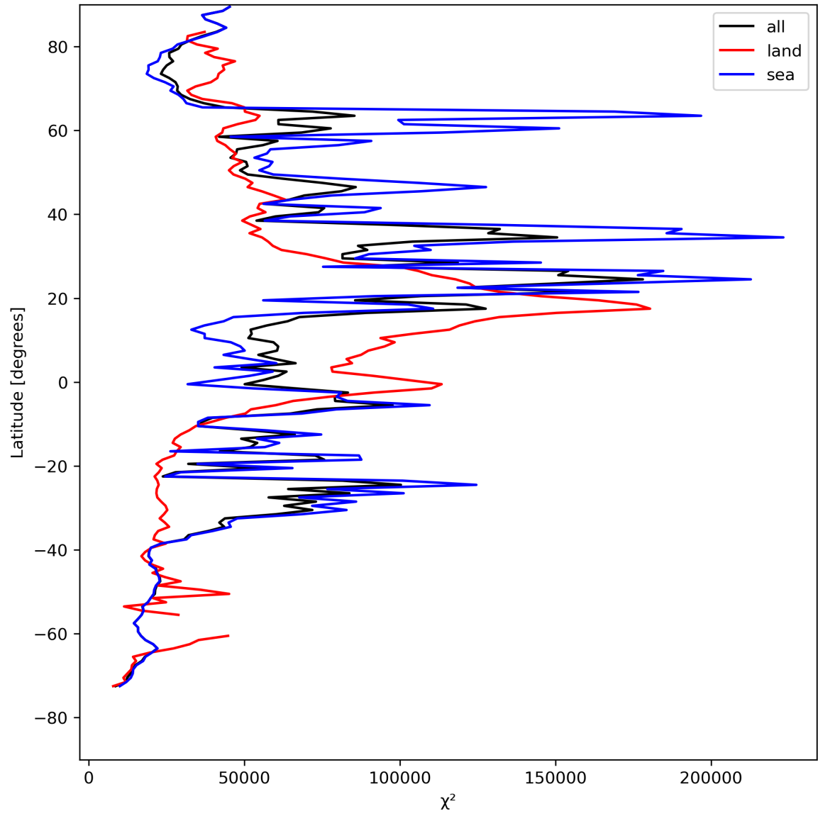
Figure 21: Zonal average of “ \chi^2 ” for 2024-08-11 to 2024-08-11.
