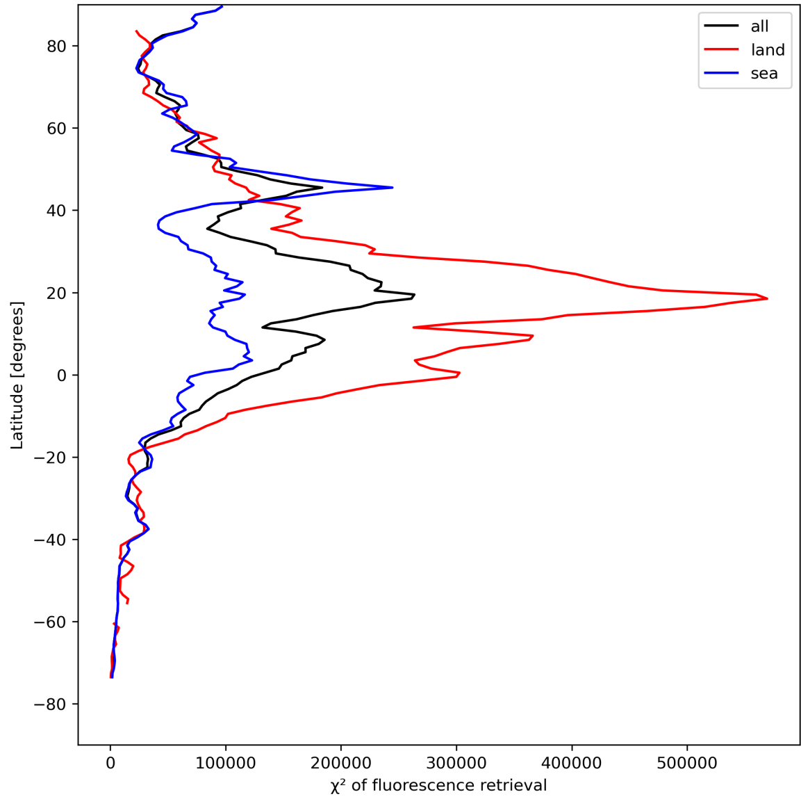
Figure 25: Zonal average of “ \chi^2 of fluorescence retrieval” for 2024-08-12 to 2024-08-13.
