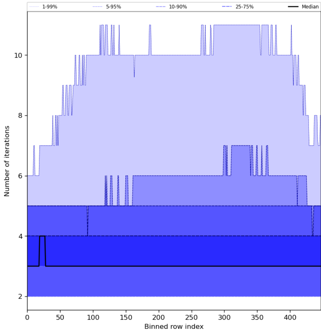
Figure 56: Along track statistics of “Number of iterations” for 2024-08-12 to 2024-08-13
