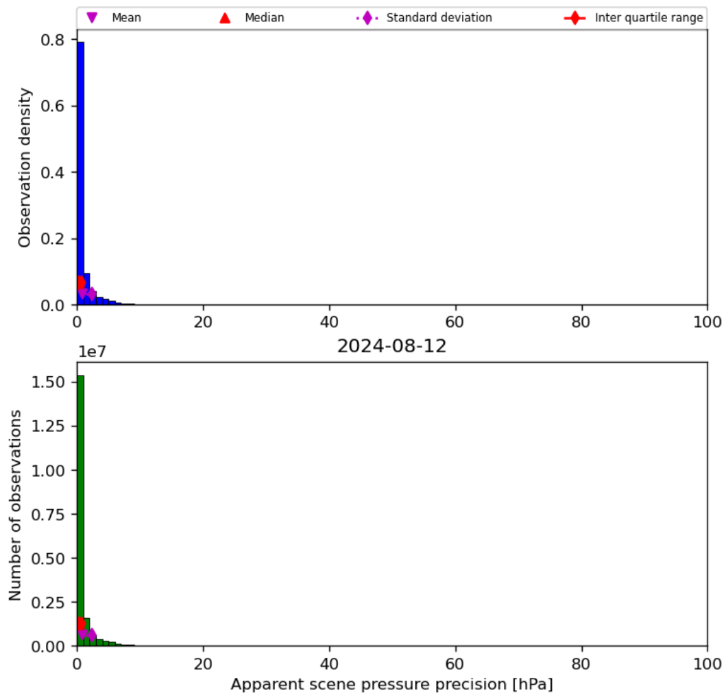
Figure 37: Histogram of “Apparent scene pressure precision” for 2024-08-12 to 2024-08-13
