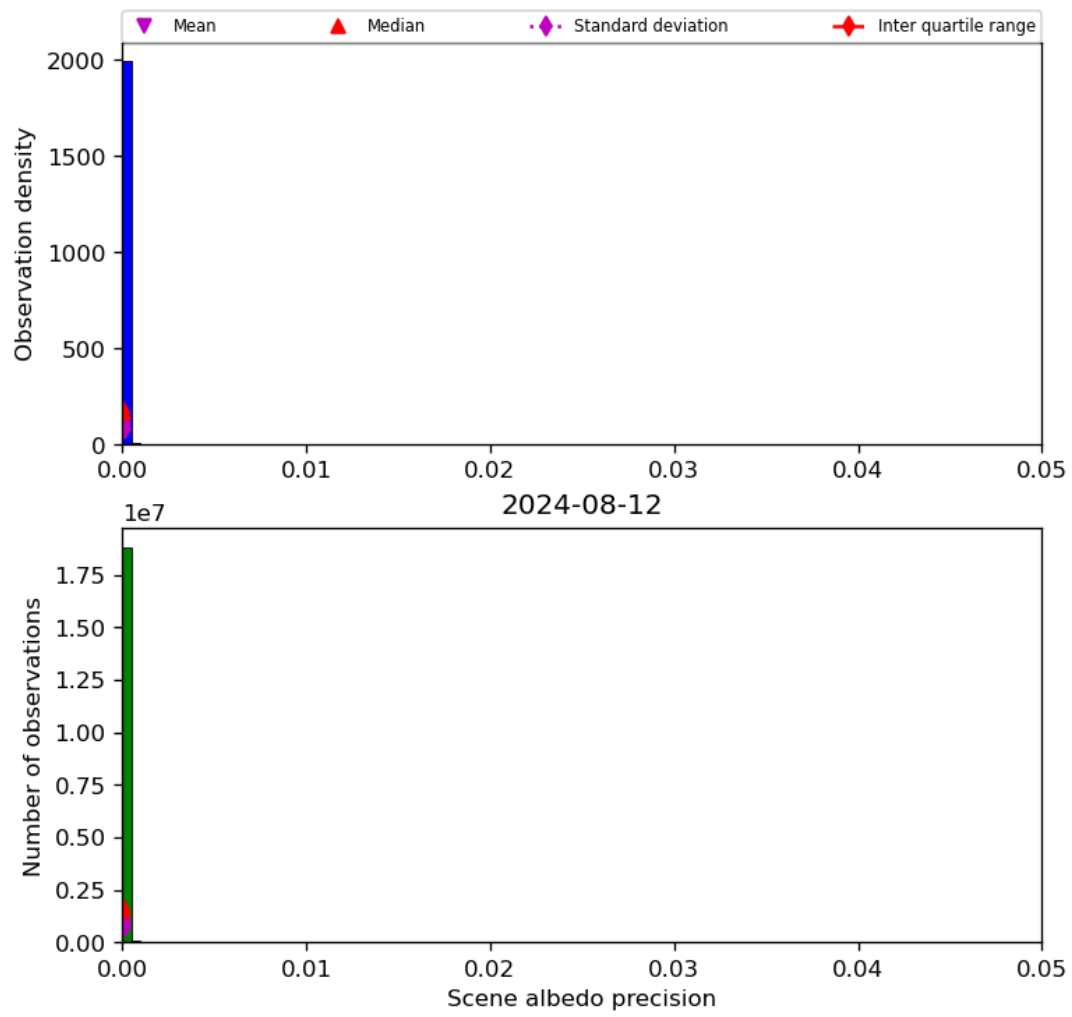
Figure 35: Histogram of “Scene albedo precision” for 2024-08-12 to 2024-08-13
