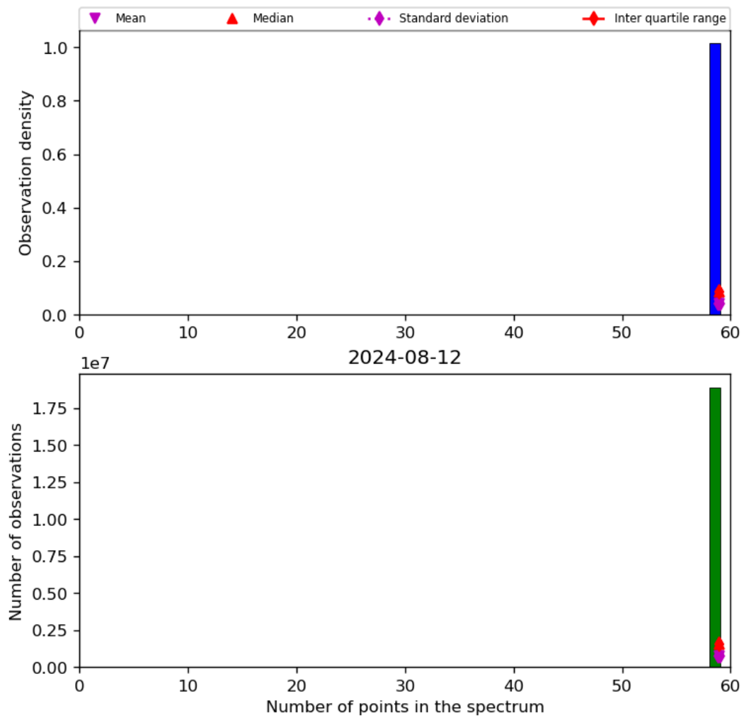
Figure 44: Histogram of “Number of points in the spectrum” for 2024-08-12 to 2024-08-13
