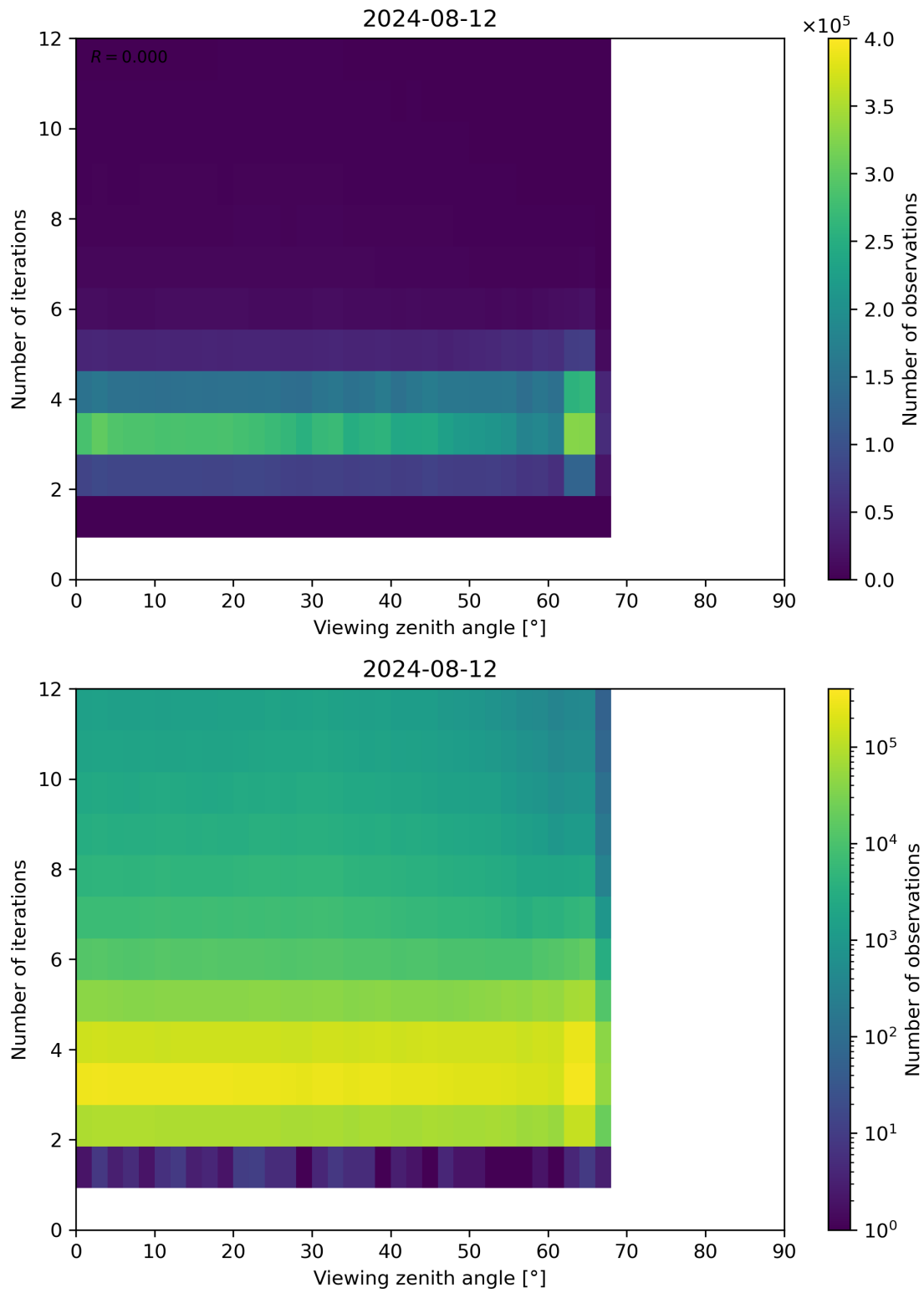
Figure 124: Scatter density plot of “Viewing zenith angle” against “Number of iterations” for 2024-08-12 to 2024-08-13.
