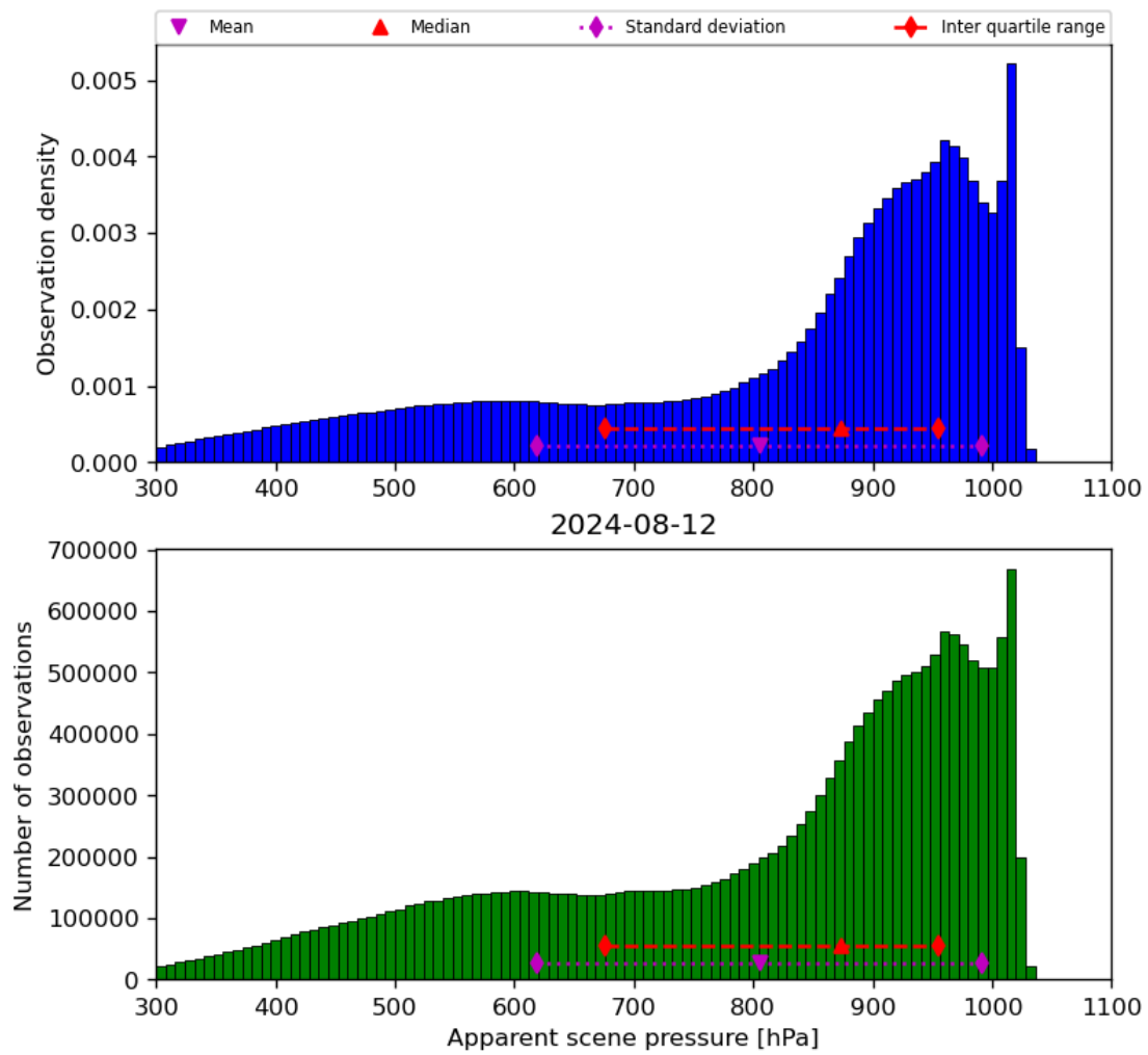
Figure 36: Histogram of “Apparent scene pressure” for 2024-08-12 to 2024-08-13
