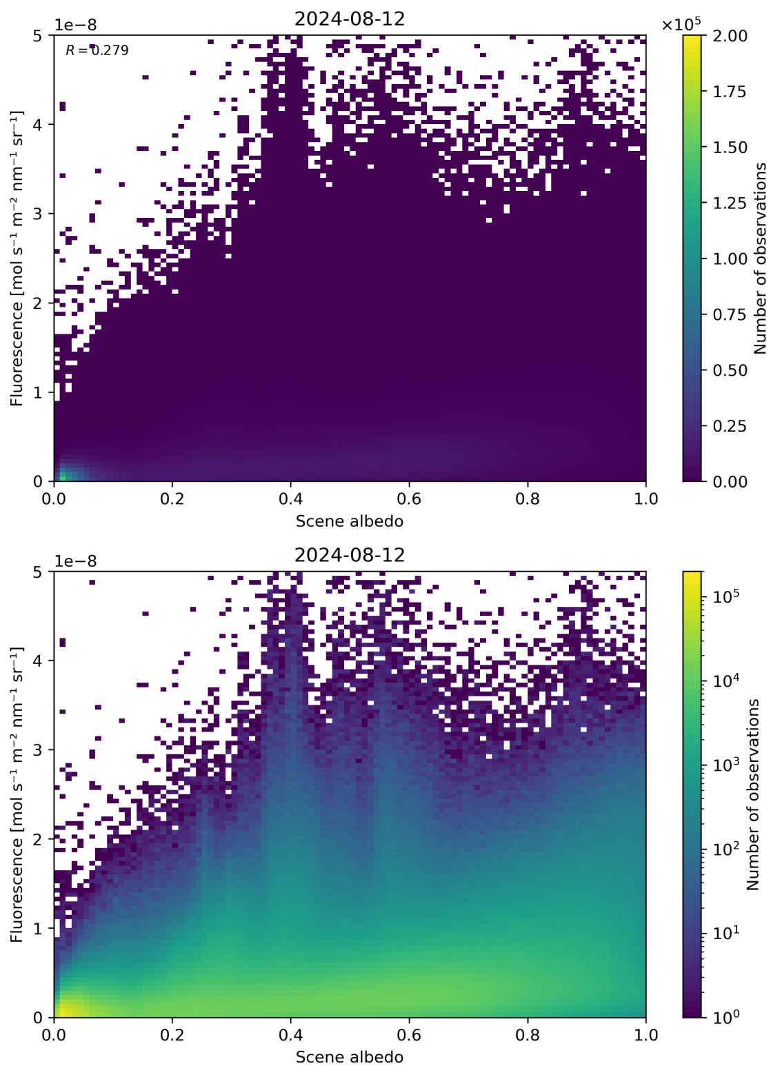
Figure 104: Scatter density plot of “Scene albedo” against “Fluorescence” for 2024-08-12 to 2024-08-13.
