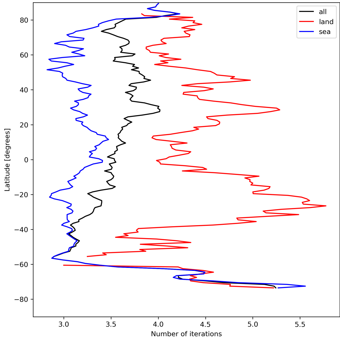
Figure 22: Zonal average of “Number of iterations” for 2024-08-12 to 2024-08-13.
