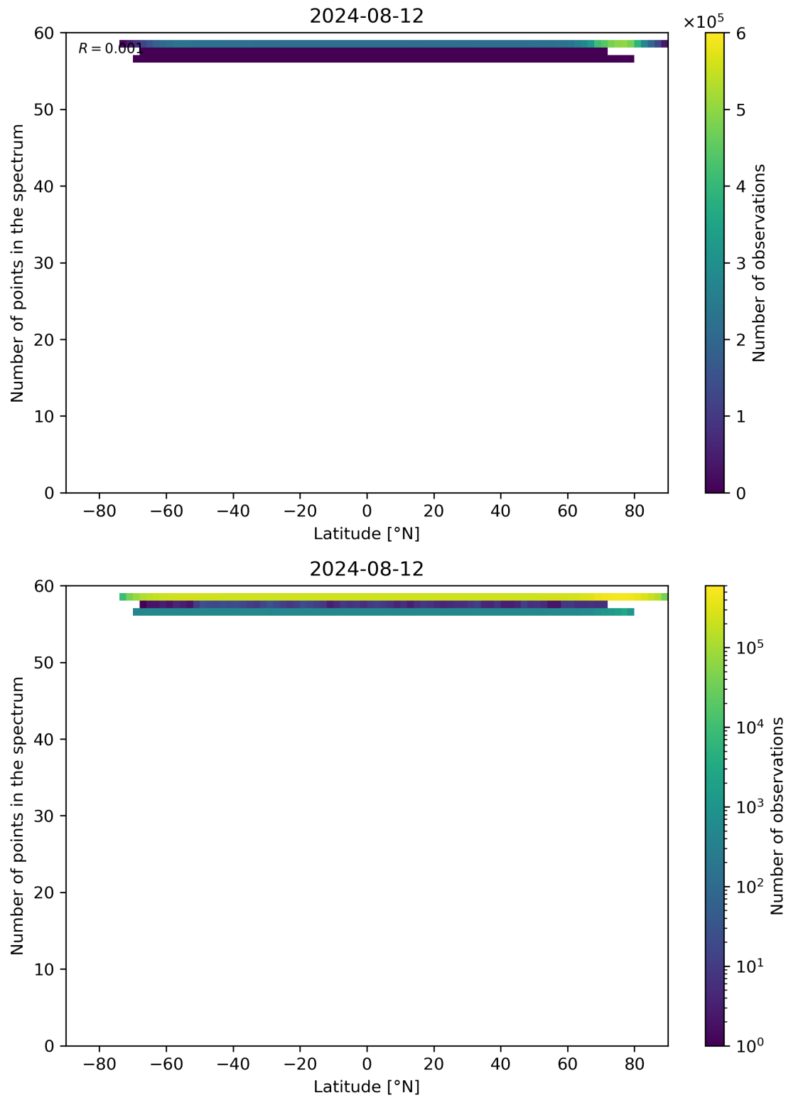
Figure 94: Scatter density plot of “Latitude” against “Number of points in the spectrum” for 2024-08-12 to 2024-08-13.
