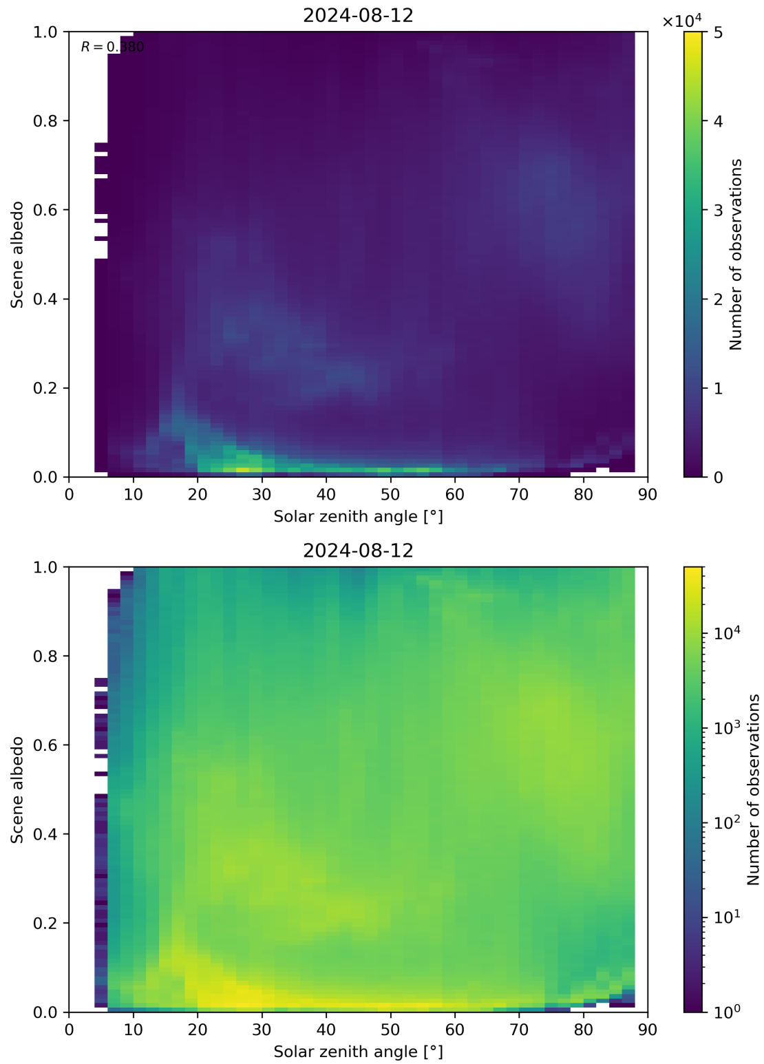
Figure 116: Scatter density plot of “Solar zenith angle” against “Scene albedo” for 2024-08-12 to 2024-08-13.
