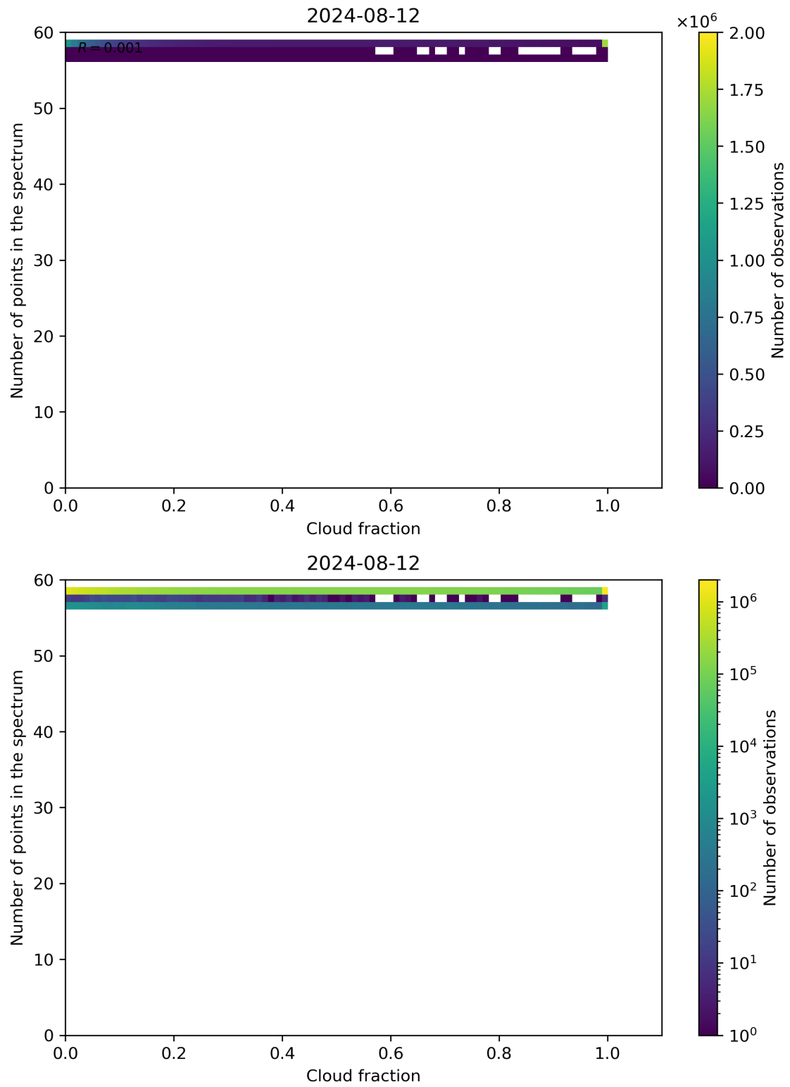
Figure 74: Scatter density plot of “Cloud fraction” against “Number of points in the spectrum” for 2024-08-12 to 2024-08-13.
