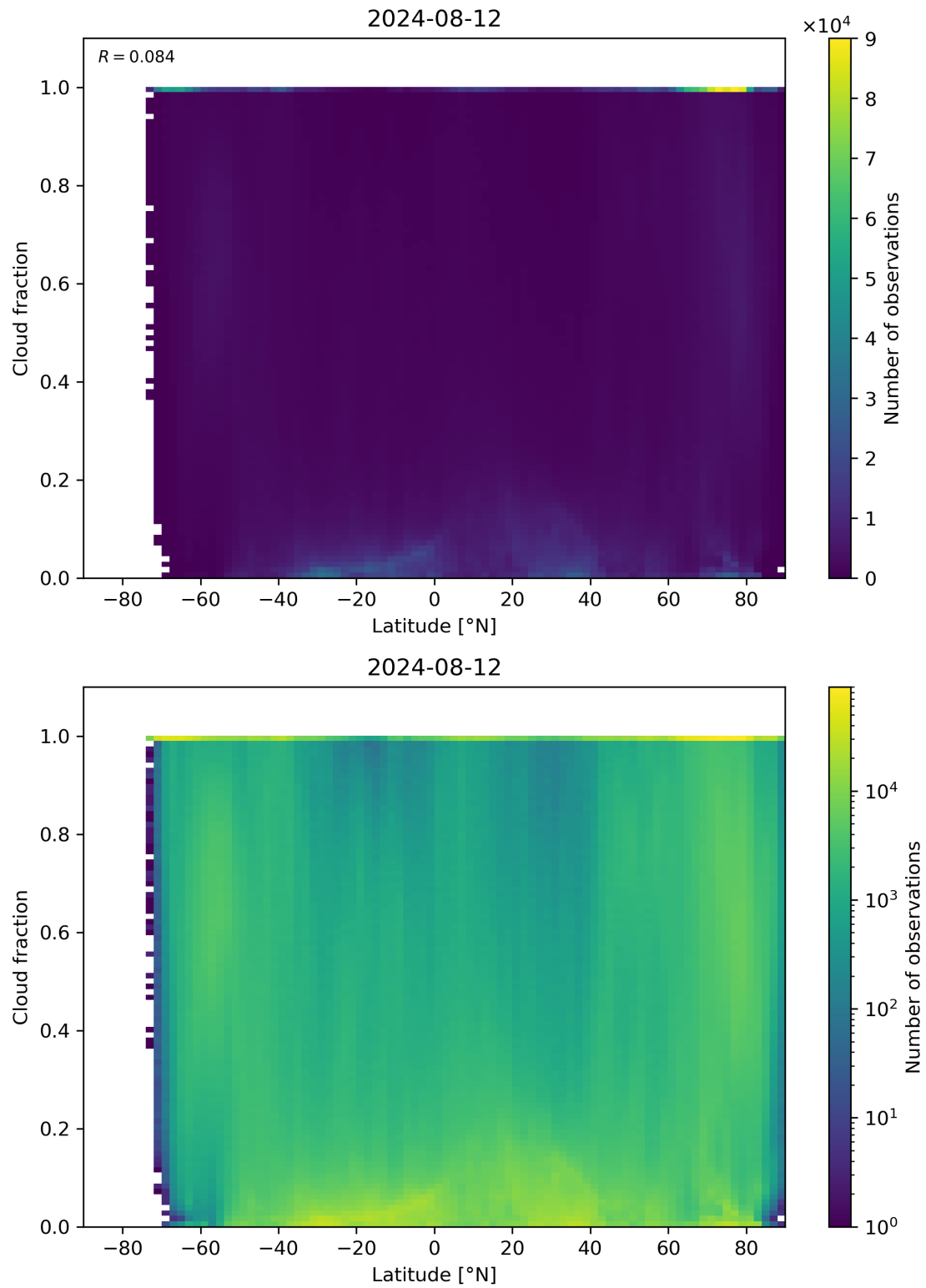
Figure 90: Scatter density plot of “Latitude” against “Cloud fraction” for 2024-08-12 to 2024-08-13.
