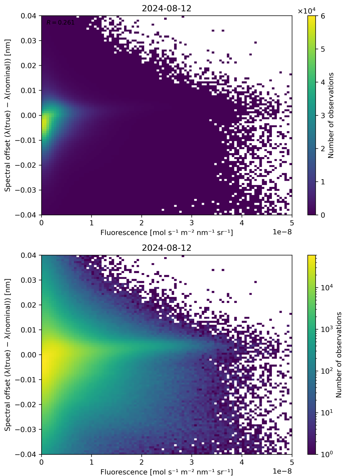
Figure 87: Scatter density plot of “Fluorescence” against “Spectral offset ( \lambda(\text{true}) - \lambda(\text{nominal}) )” for 2024-08-12 to 2024-08-13.
