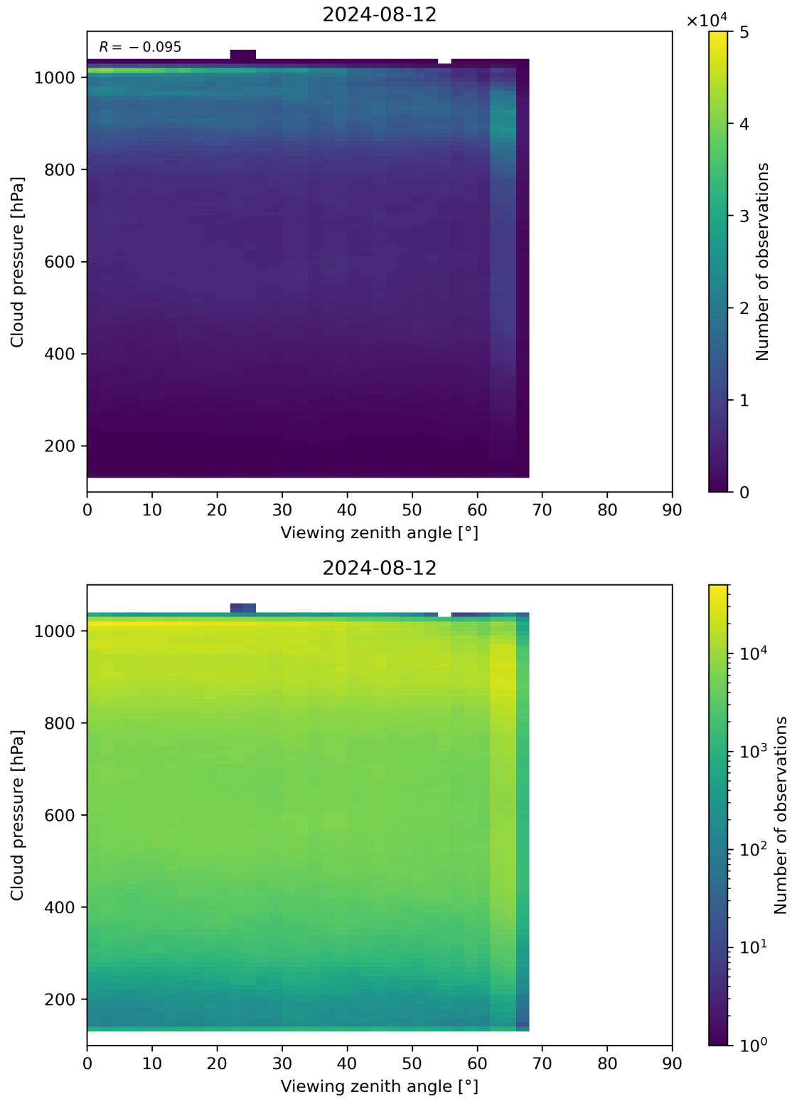
Figure 121: Scatter density plot of “Viewing zenith angle” against “Cloud pressure” for 2024-08-12 to 2024-08-13.
