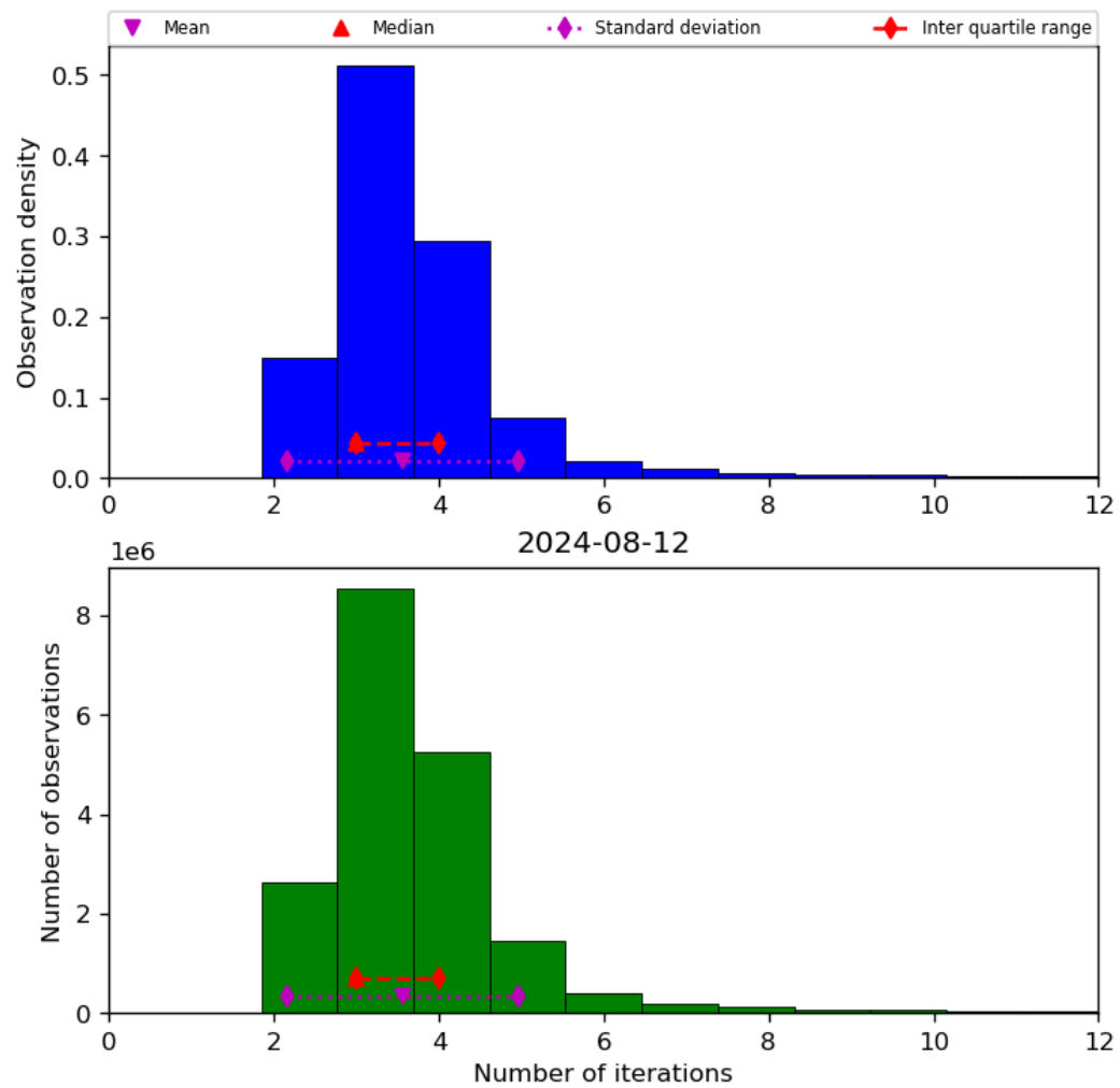
Figure 39: Histogram of “Number of iterations” for 2024-08-12 to 2024-08-13
