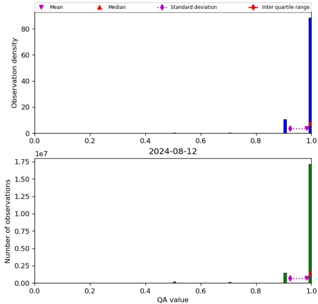
Figure 29: Histogram of “QA value” for 2024-08-12 to 2024-08-13
