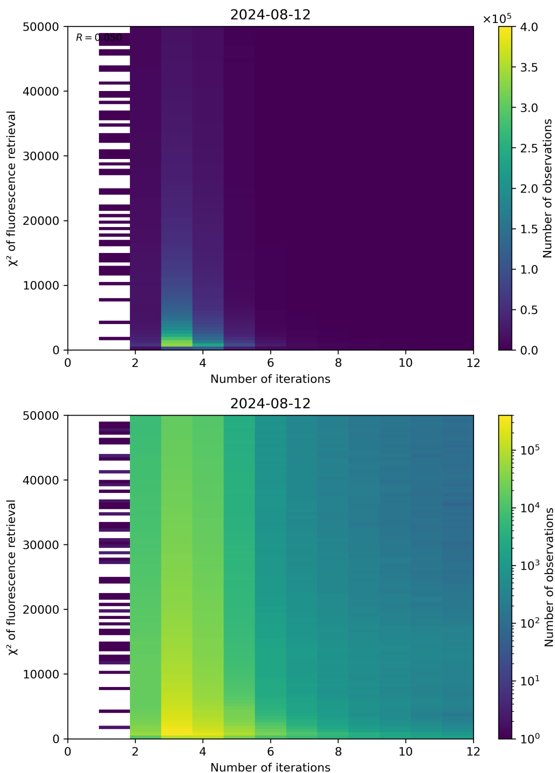
Figure 97: Scatter density plot of “Number of iterations” against “ \chi^2 of fluorescence retrieval” for 2024-08-12 to 2024-08-13.
