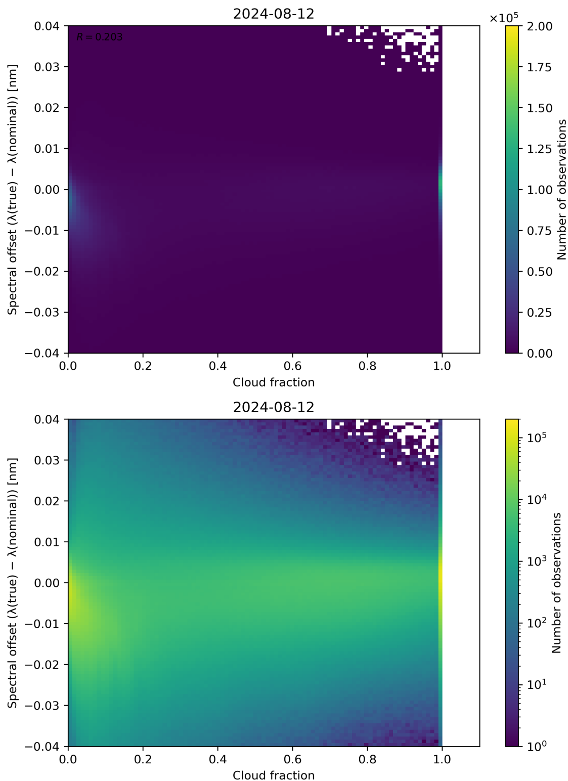
Figure 76: Scatter density plot of “Cloud fraction” against “Spectral offset ( \lambda(\text{true}) - \lambda(\text{nominal}) )” for 2024-08-12 to 2024-08-13.
