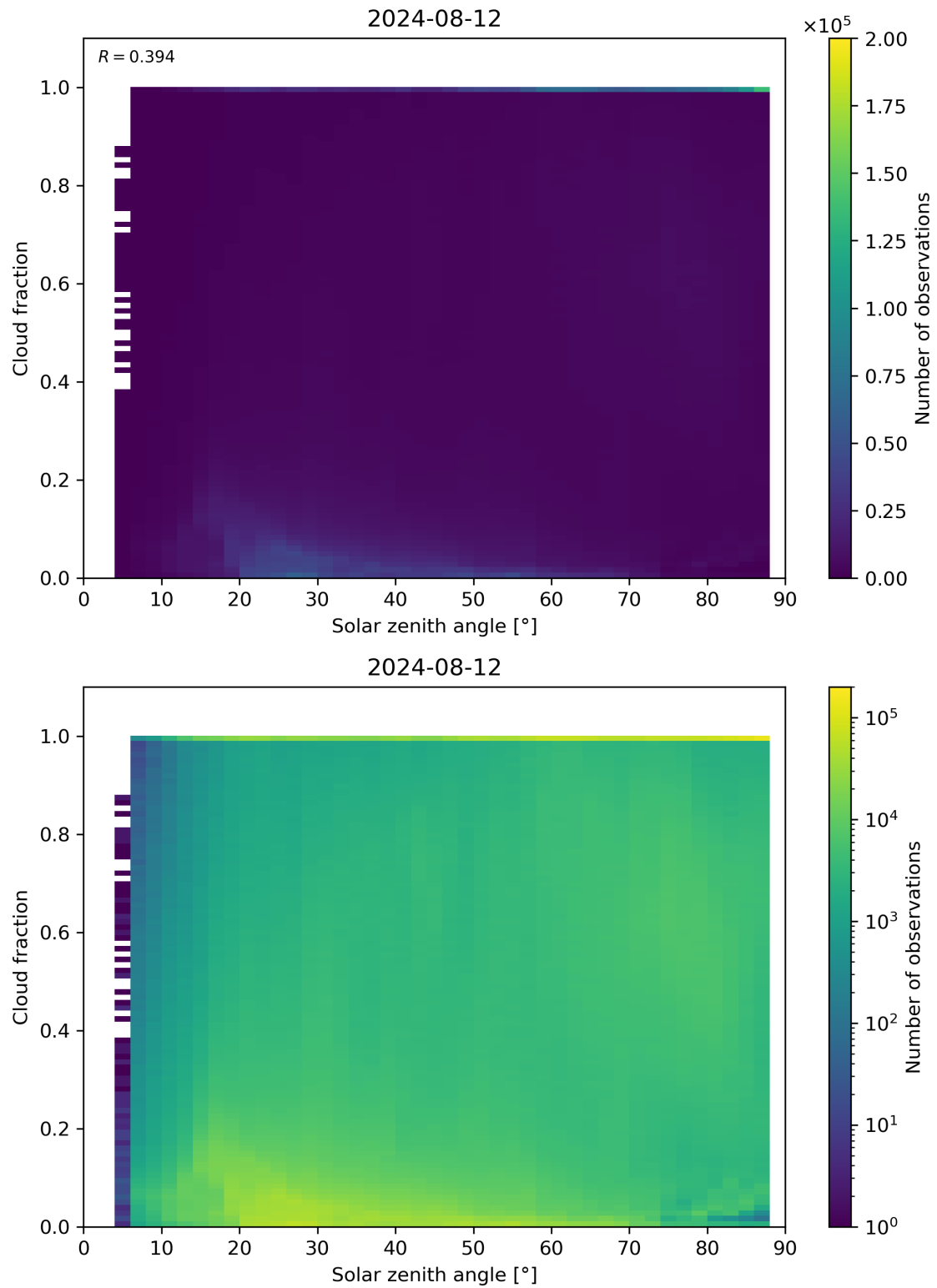
Figure 110: Scatter density plot of “Solar zenith angle” against “Cloud fraction” for 2024-08-12 to 2024-08-13.
