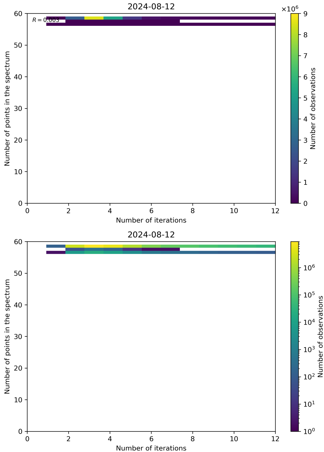
Figure 99: Scatter density plot of “Number of iterations” against “Number of points in the spectrum” for 2024-08-12 to 2024-08-13.
