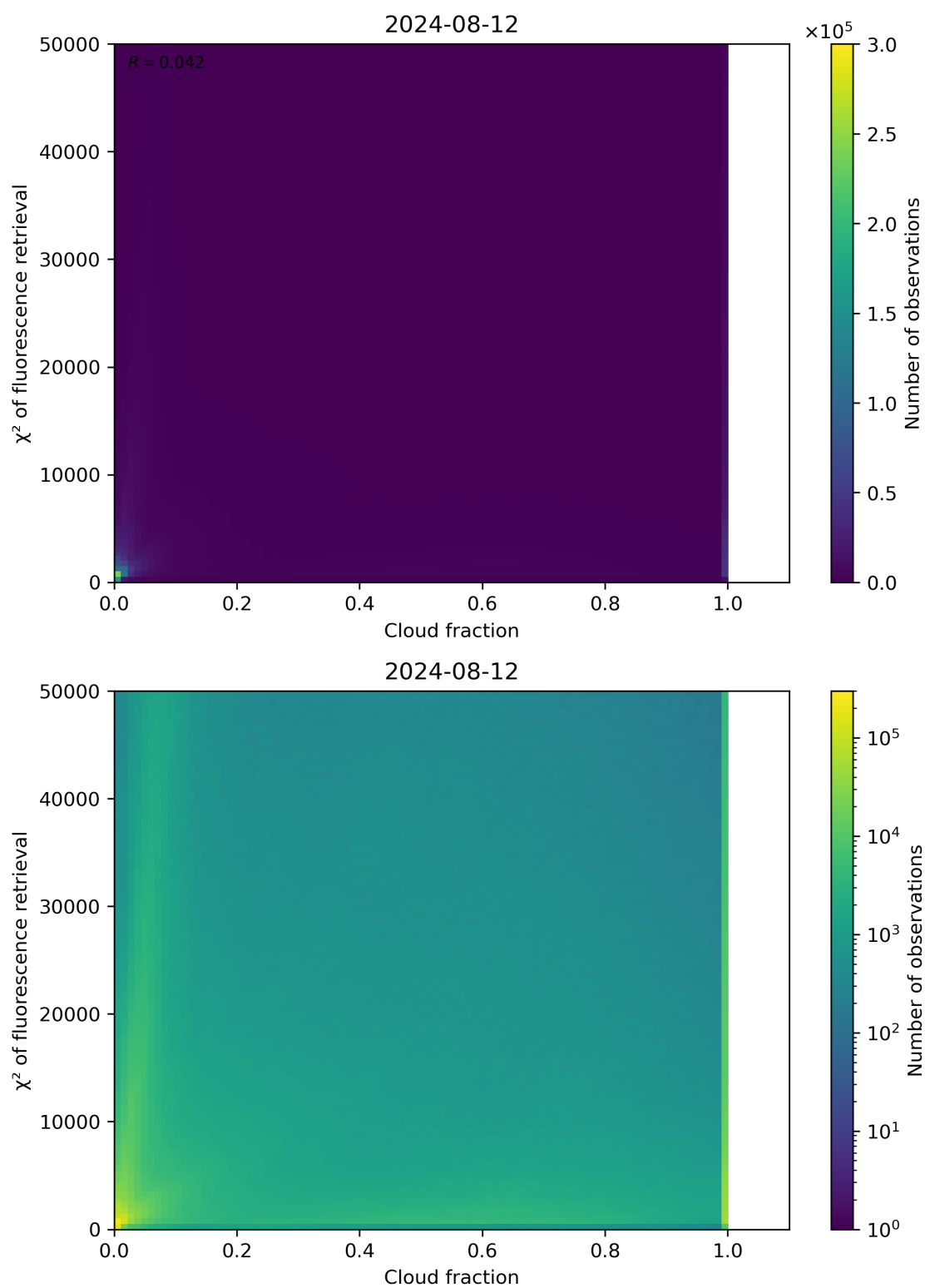
Figure 71: Scatter density plot of “Cloud fraction” against “ \chi^2 of fluorescence retrieval” for 2024-08-12 to 2024-08-13.
