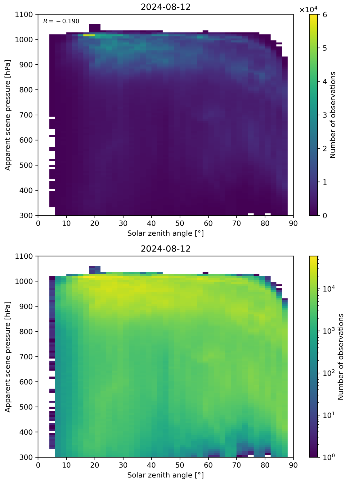
Figure 108: Scatter density plot of “Solar zenith angle” against “Apparent scene pressure” for 2024-08-12 to 2024-08-13.
