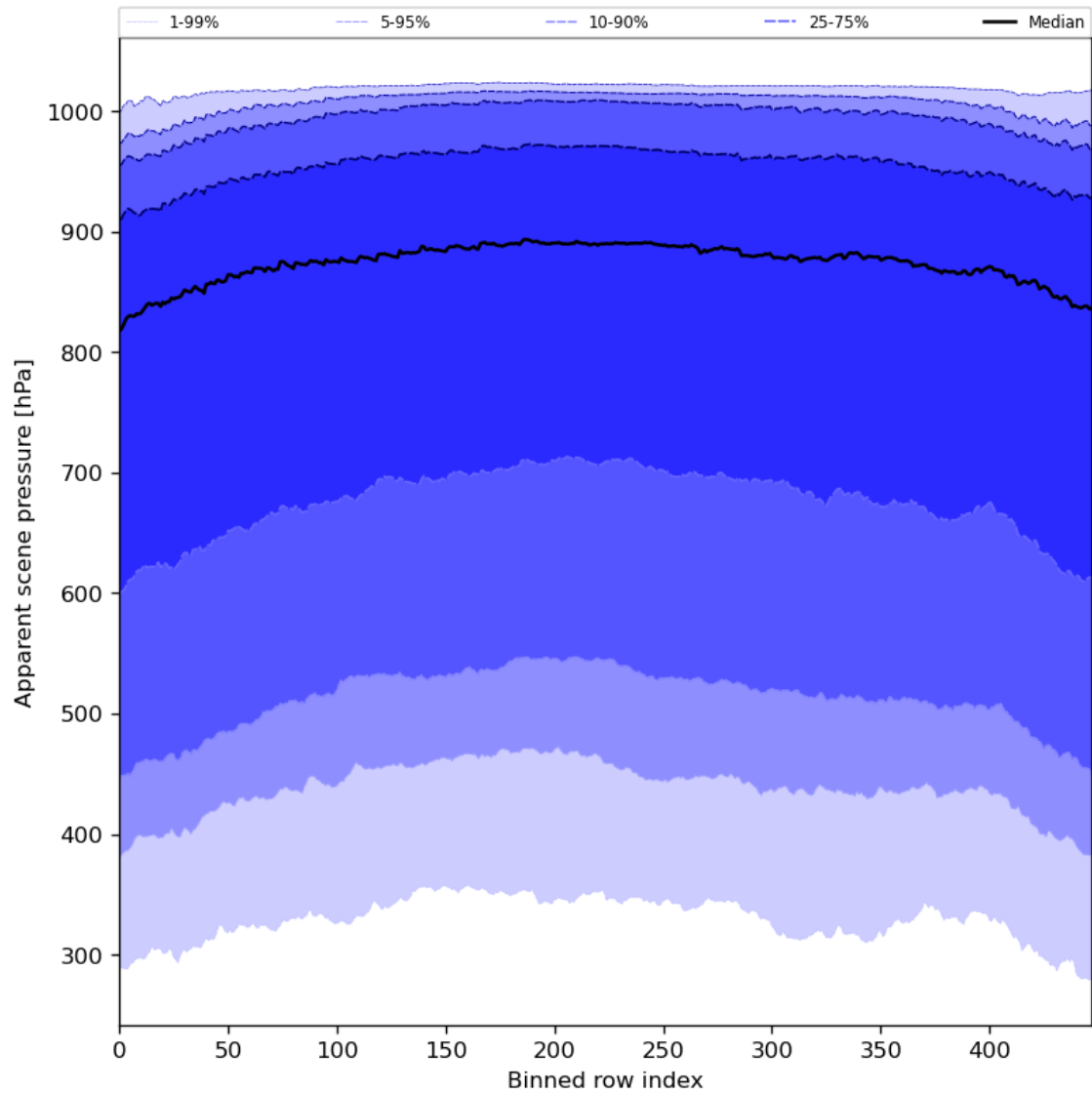
Figure 53: Along track statistics of “Apparent scene pressure” for 2024-08-12 to 2024-08-13
