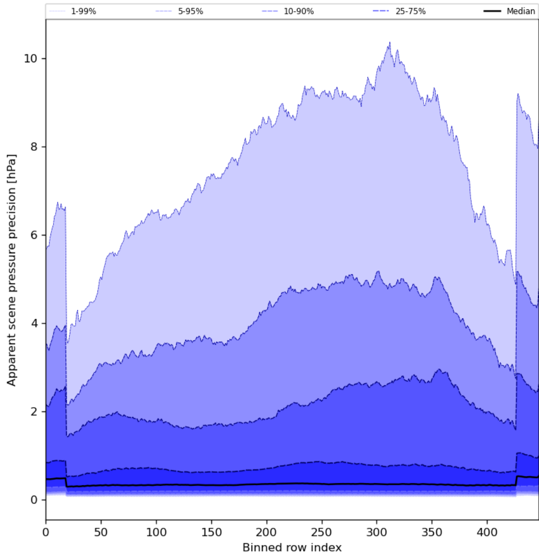
Figure 54: Along track statistics of “Apparent scene pressure precision” for 2024-08-12 to 2024-08-13
