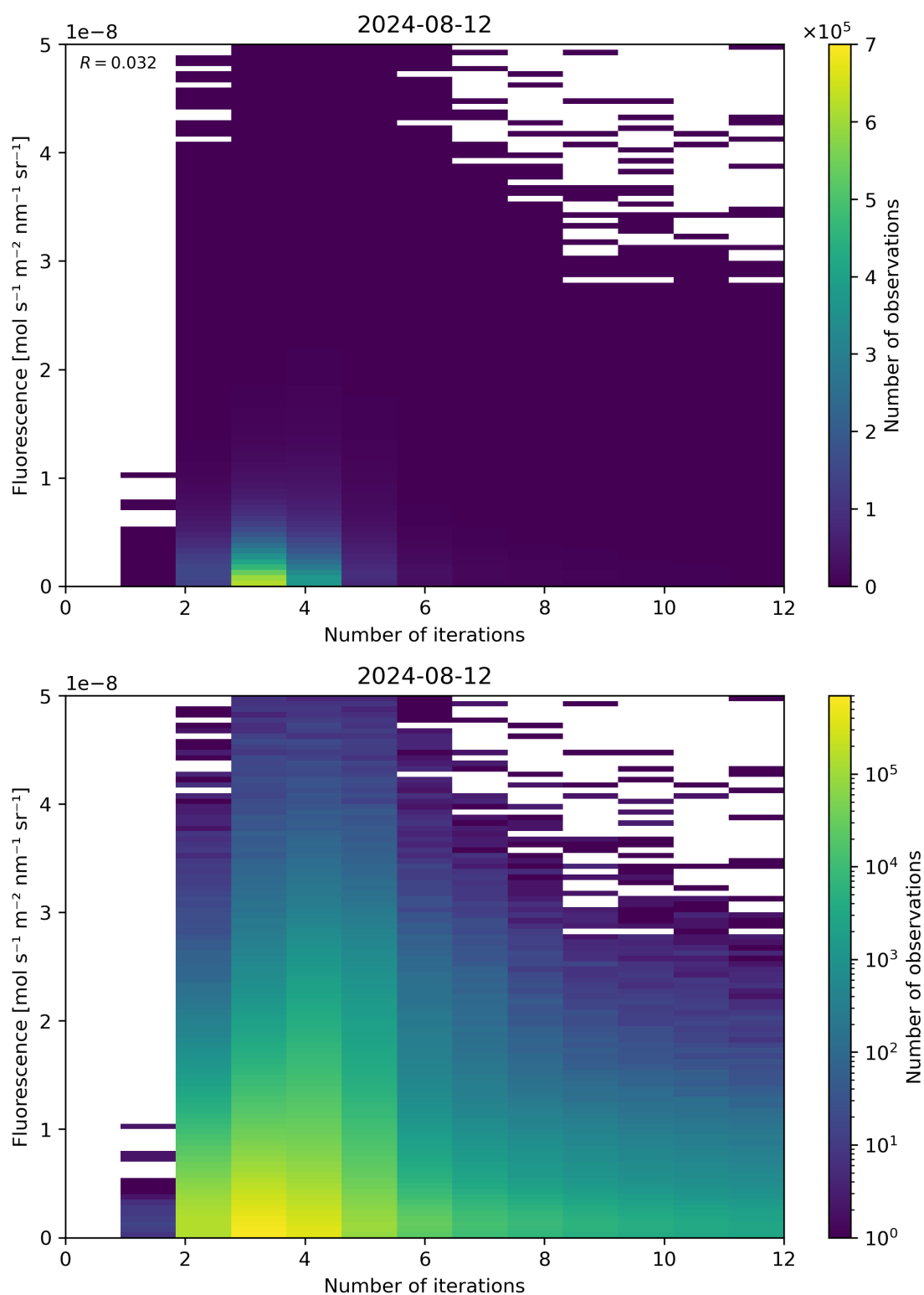
Figure 98: Scatter density plot of “Number of iterations” against “Fluorescence” for 2024-08-12 to 2024-08-13.
