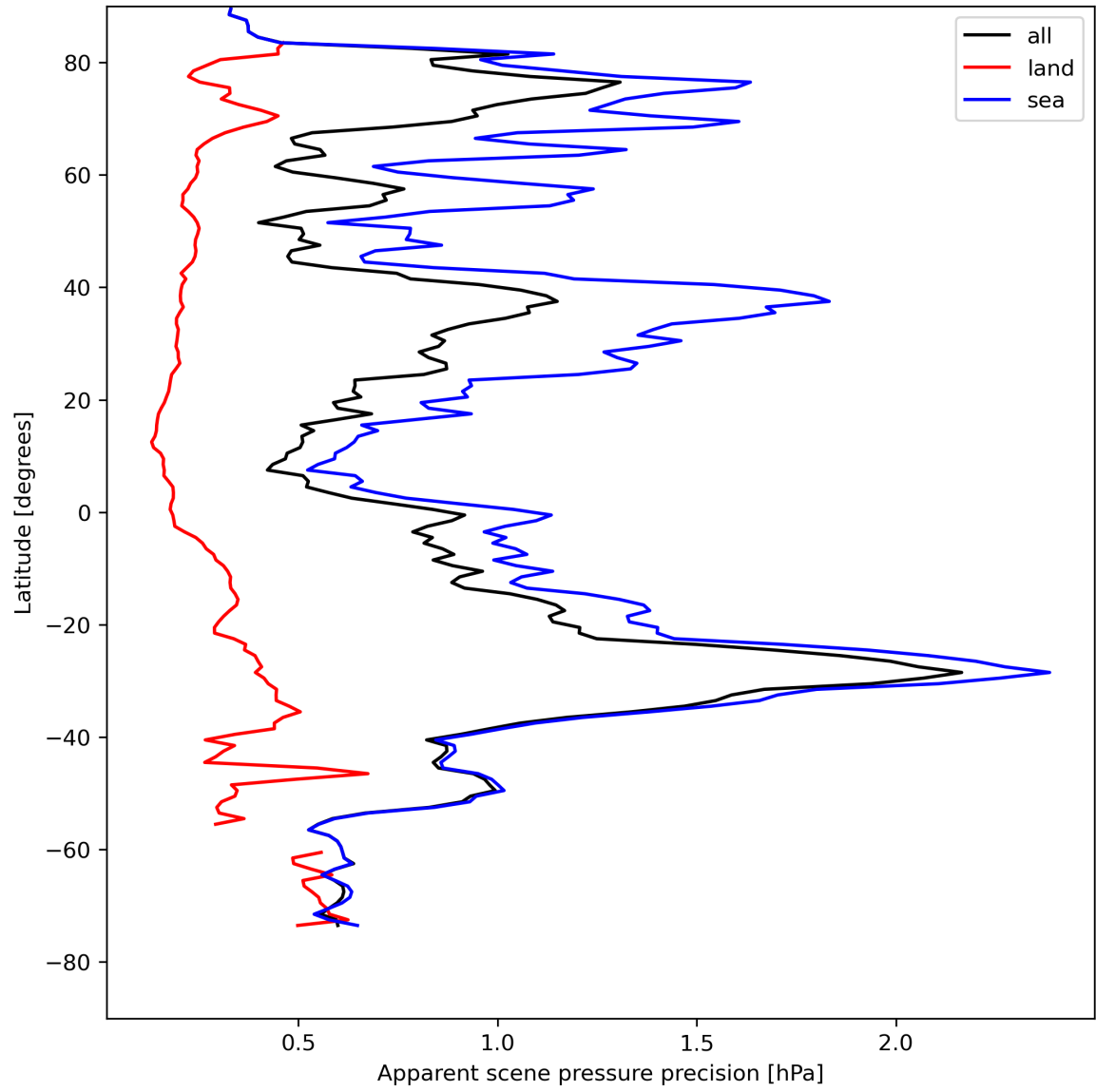
Figure 20: Zonal average of “Apparent scene pressure precision” for 2024-08-12 to 2024-08-13.
