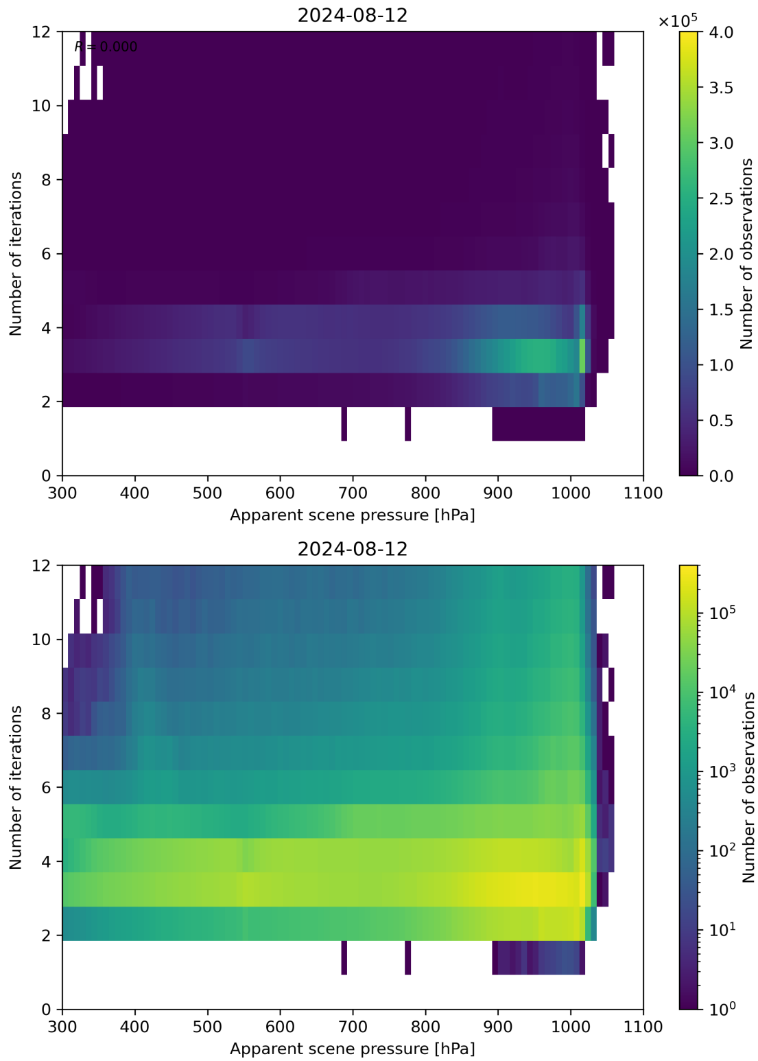
Figure 65: Scatter density plot of “Apparent scene pressure” against “Number of iterations” for 2024-08-12 to 2024-08-13.
