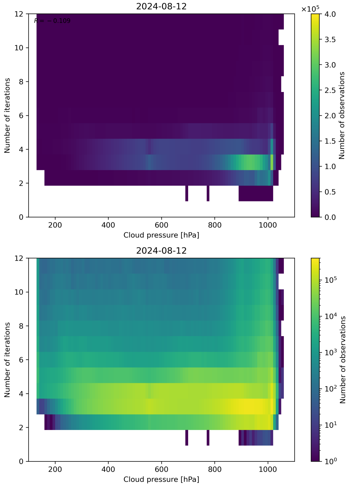
Figure 81: Scatter density plot of “Cloud pressure” against “Number of iterations” for 2024-08-12 to 2024-08-13.
