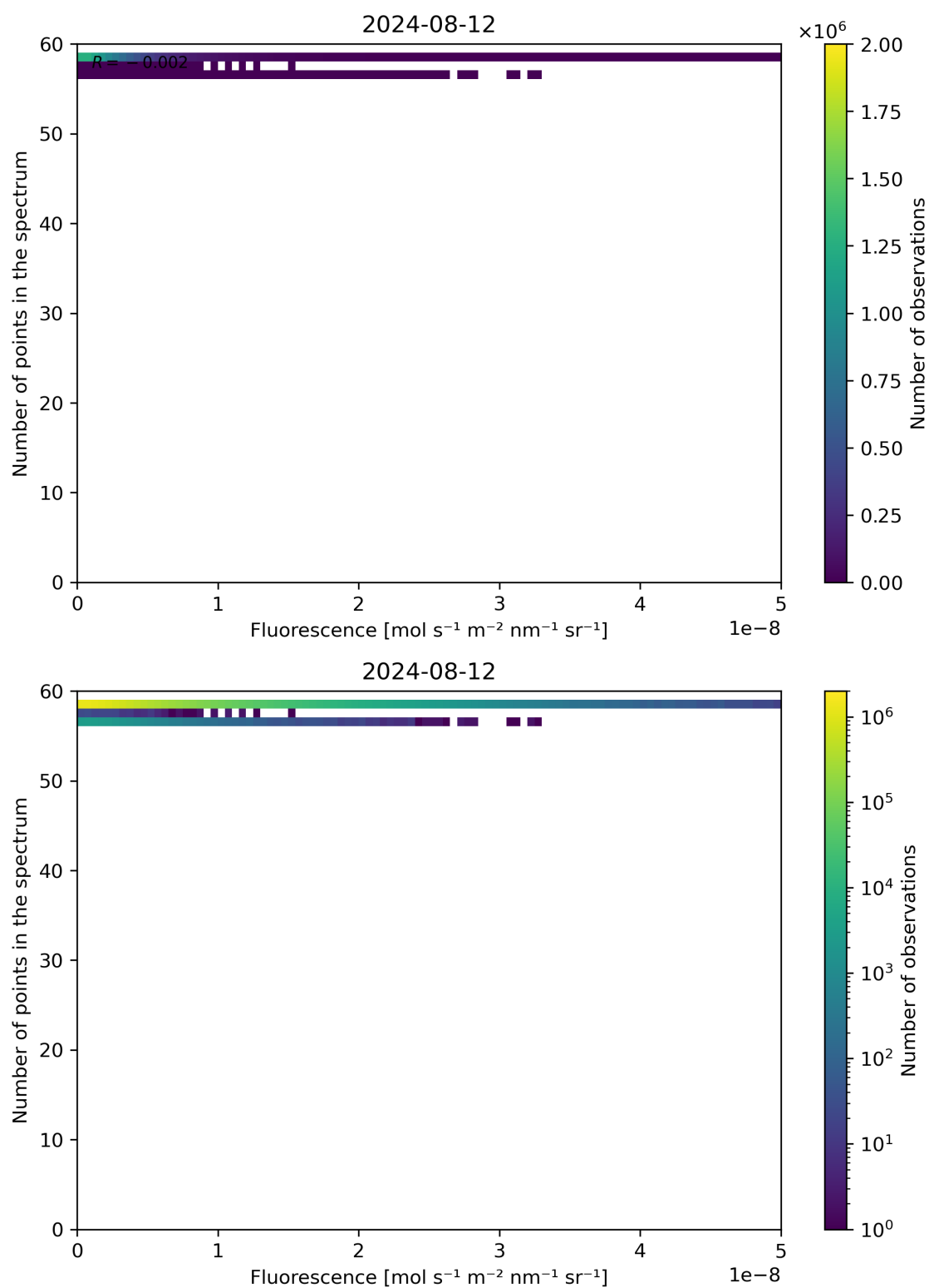
Figure 86: Scatter density plot of “Fluorescence” against “Number of points in the spectrum” for 2024-08-12 to 2024-08-13.
