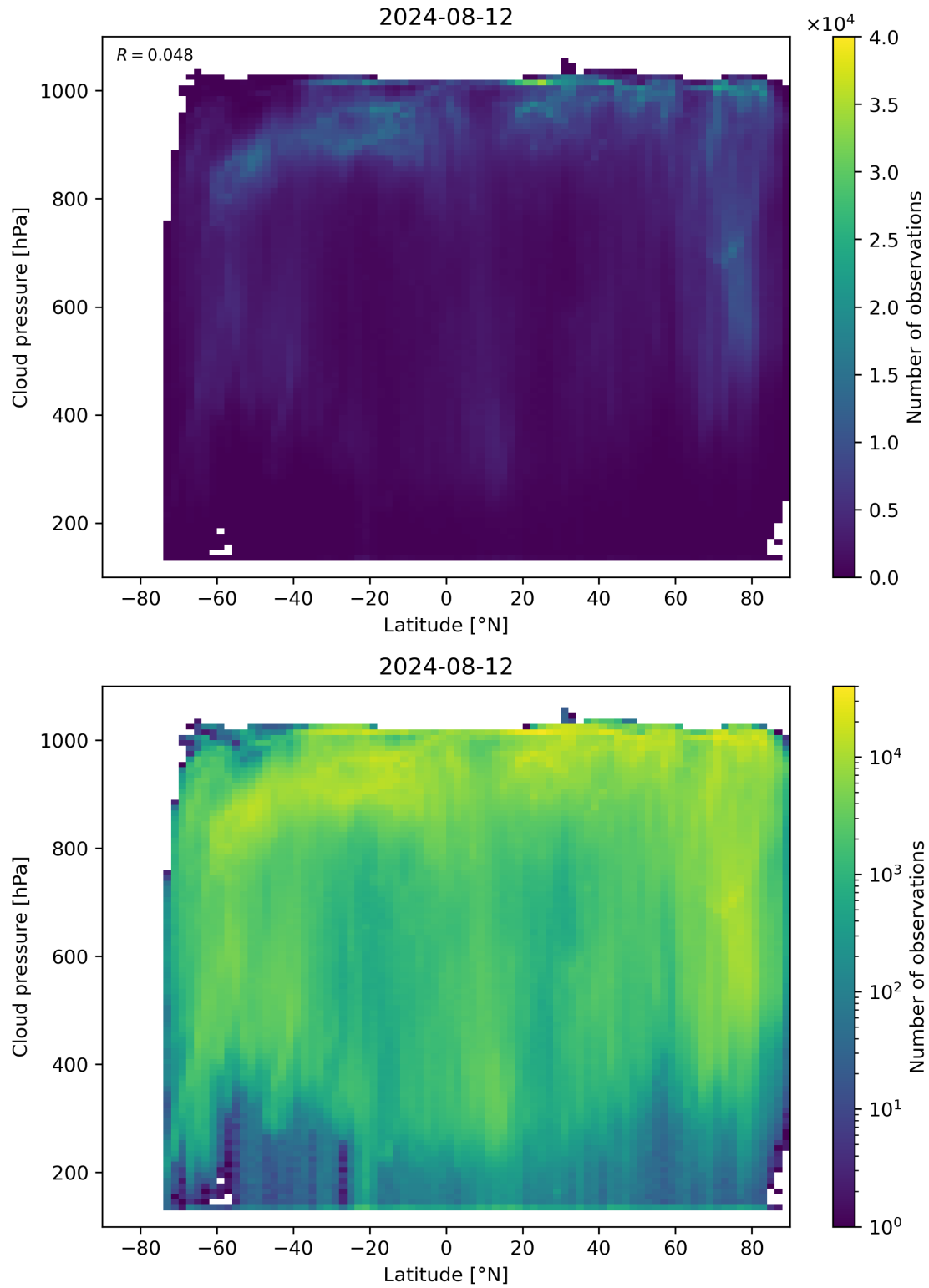
Figure 91: Scatter density plot of “Latitude” against “Cloud pressure” for 2024-08-12 to 2024-08-13.
