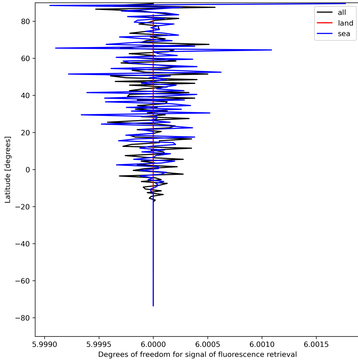
Figure 26: Zonal average of “Degrees of freedom for signal of fluorescence retrieval” for 2024-08-12 to 2024-08-13.
