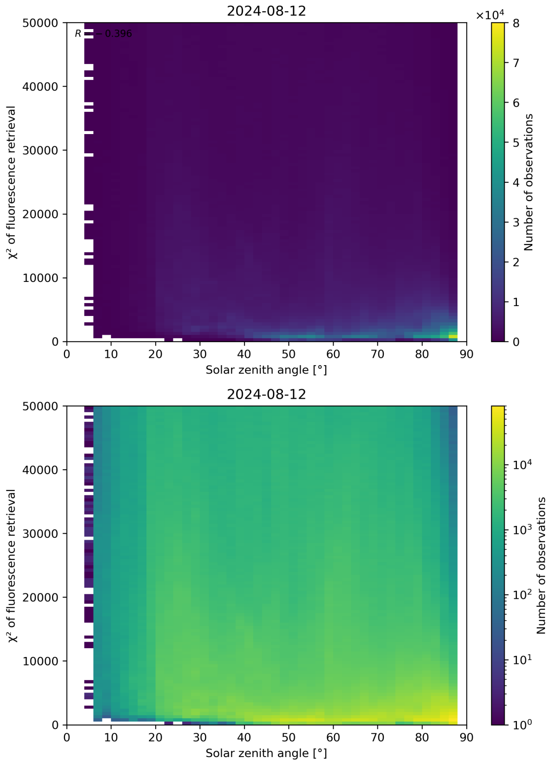
Figure 109: Scatter density plot of “Solar zenith angle” against “ \chi^2 of fluorescence retrieval” for 2024-08-12 to 2024-08-13.
