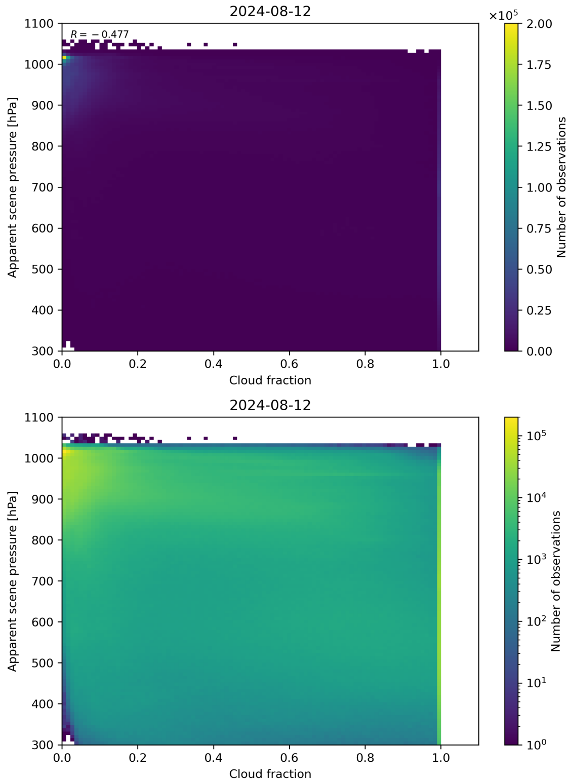
Figure 70: Scatter density plot of “Cloud fraction” against “Apparent scene pressure” for 2024-08-12 to 2024-08-13.
