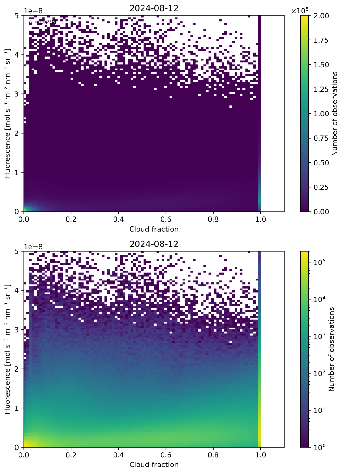
Figure 72: Scatter density plot of “Cloud fraction” against “Fluorescence” for 2024-08-12 to 2024-08-13.
