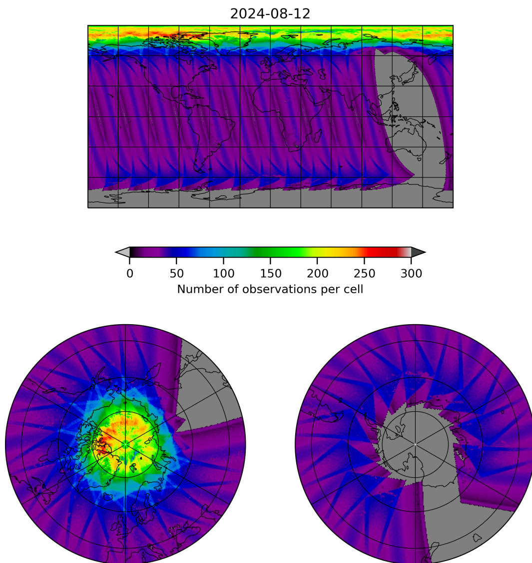
Figure 11: Map of the number of observations for 2024-08-12 to 2024-08-13
