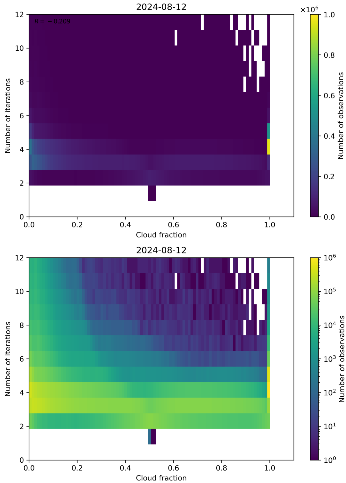
Figure 73: Scatter density plot of “Cloud fraction” against “Number of iterations” for 2024-08-12 to 2024-08-13.
