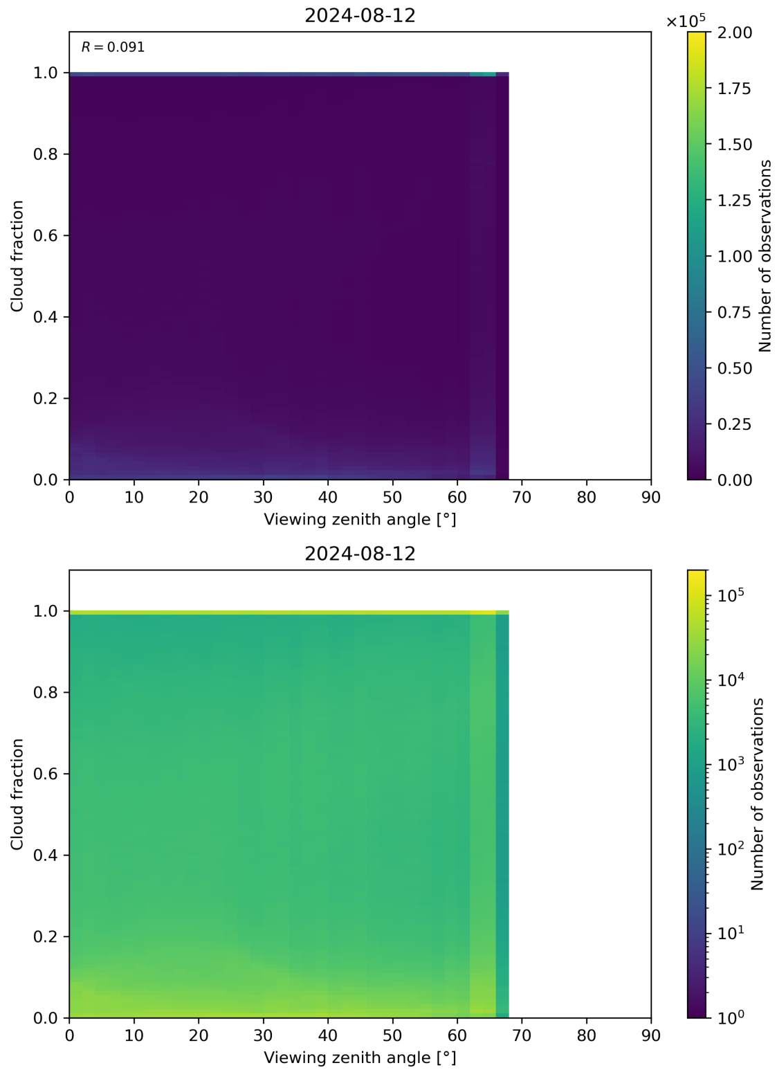
Figure 120: Scatter density plot of “Viewing zenith angle” against “Cloud fraction” for 2024-08-12 to 2024-08-13.
