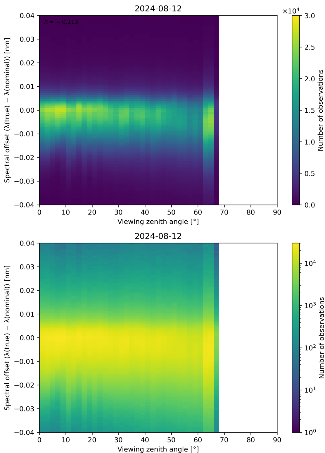
Figure 128: Scatter density plot of “Viewing zenith angle” against “Spectral offset ( \lambda(\text{true}) - \lambda(\text{nominal}) )” for 2024-08-12 to 2024-08-13.
