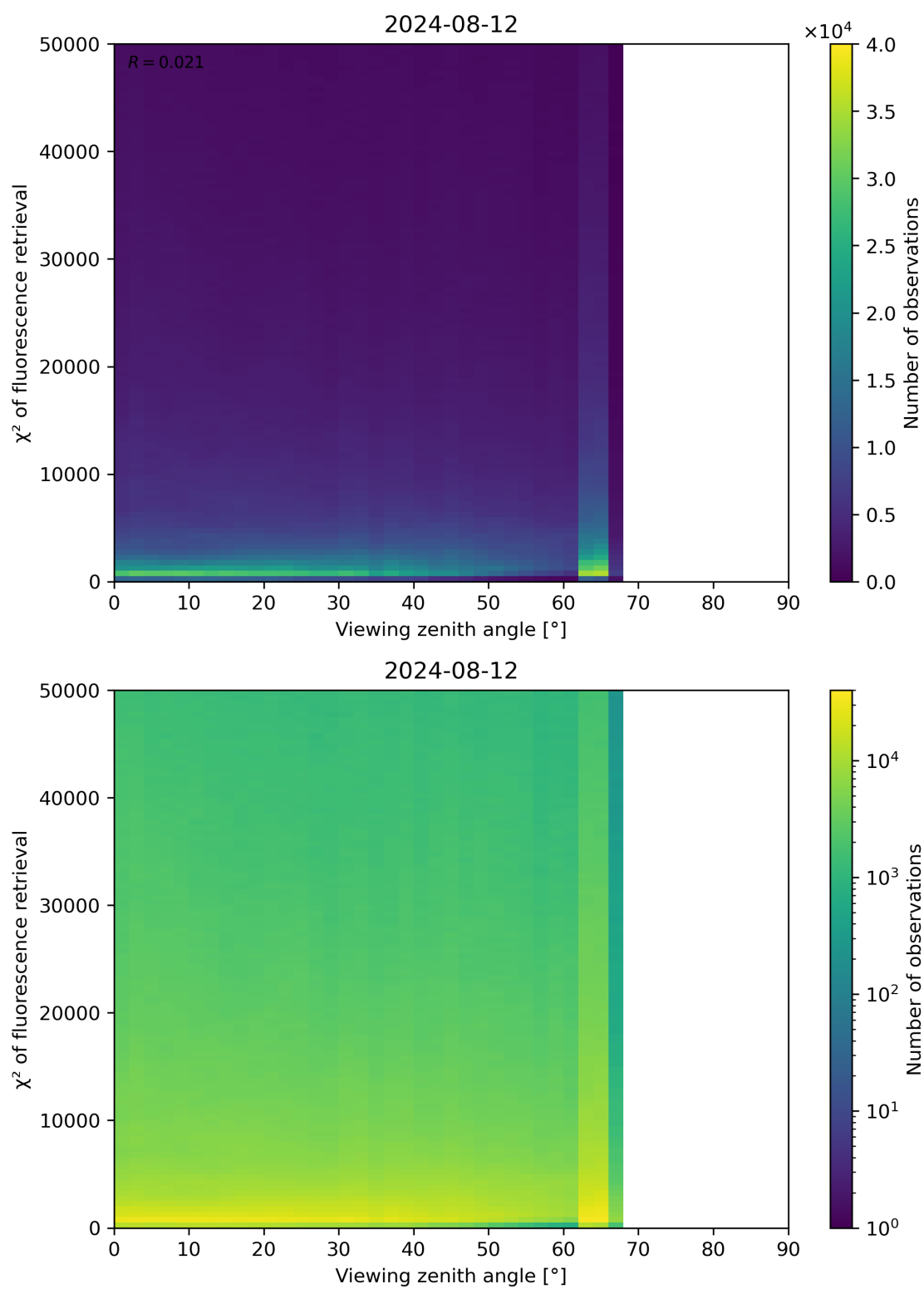
Figure 119: Scatter density plot of “Viewing zenith angle” against “ \chi^2 of fluorescence retrieval” for 2024-08-12 to 2024-08-13.
