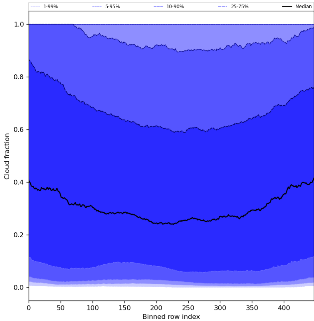
Figure 49: Along track statistics of “Cloud fraction” for 2024-08-12 to 2024-08-13
