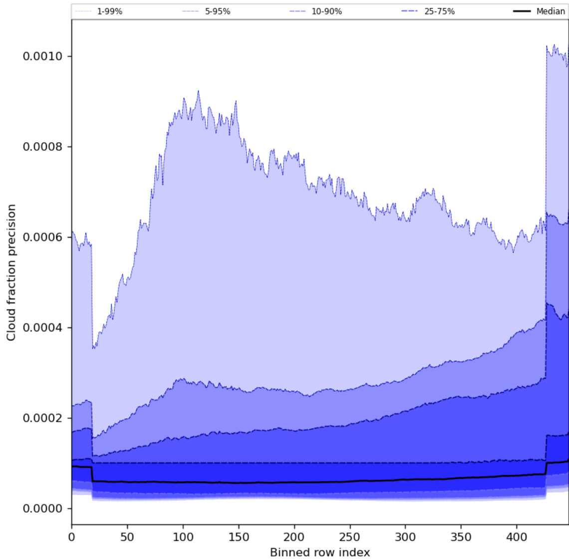
Figure 50: Along track statistics of “Cloud fraction precision” for 2024-08-12 to 2024-08-13
