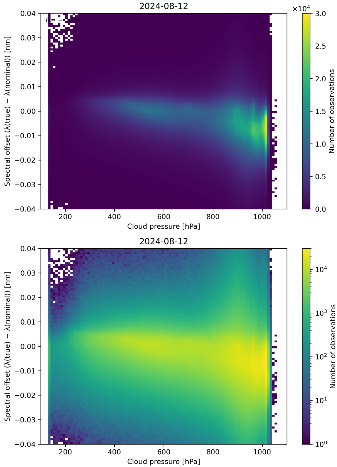
Figure 84: Scatter density plot of “Cloud pressure” against “Spectral offset ( \lambda(\text{true}) - \lambda(\text{nominal}) )” for 2024-08-12 to 2024-08-13.
