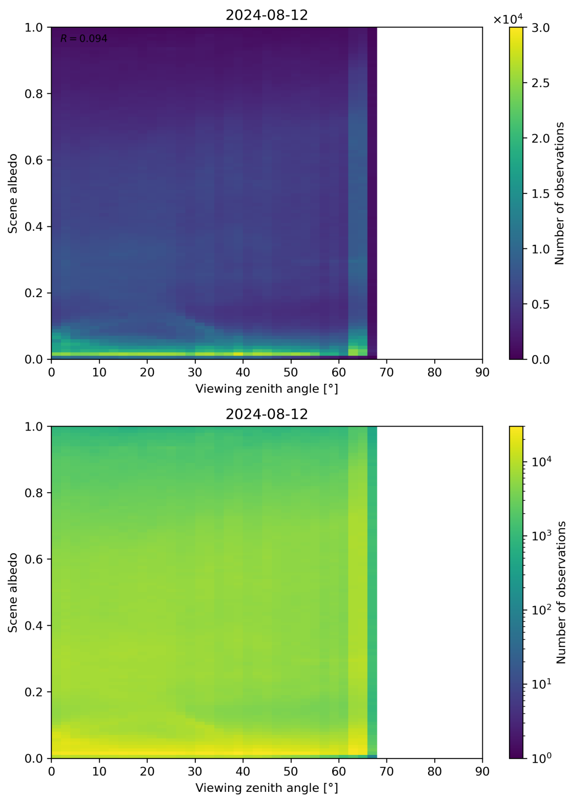
Figure 126: Scatter density plot of “Viewing zenith angle” against “Scene albedo” for 2024-08-12 to 2024-08-13.
