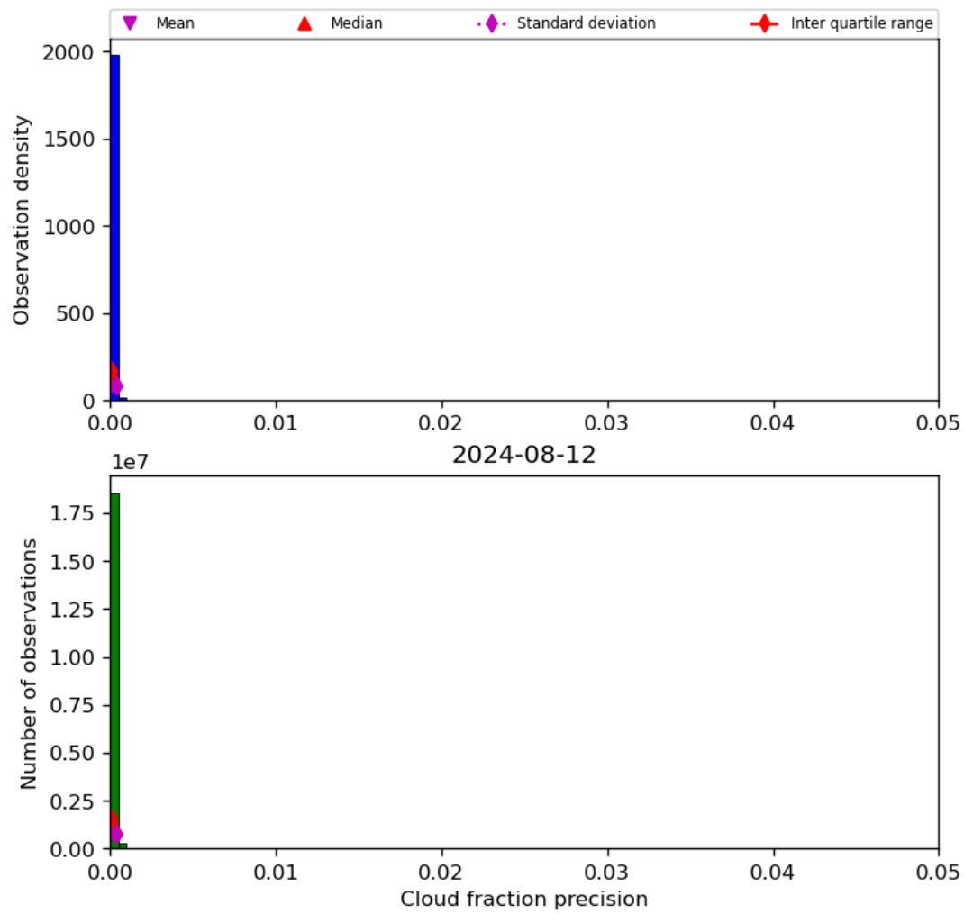
Figure 33: Histogram of “Cloud fraction precision” for 2024-08-12 to 2024-08-13
