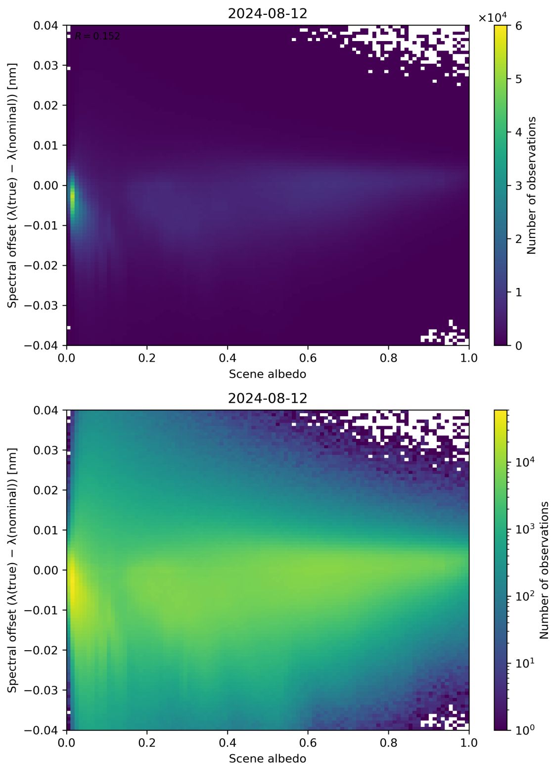
Figure 107: Scatter density plot of “Scene albedo” against “Spectral offset ( \lambda(\text{true}) - \lambda(\text{nominal}) )” for 2024-08-12 to 2024-08-13.
