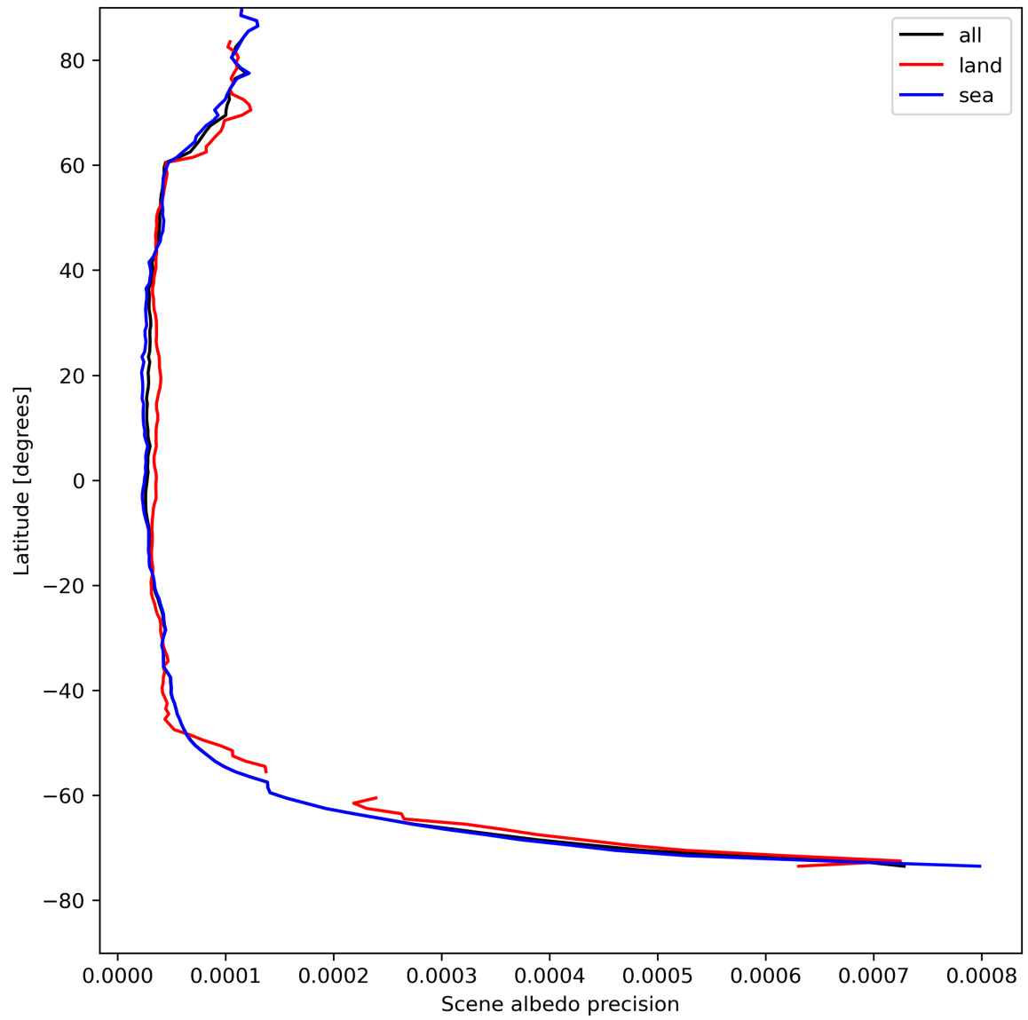
Figure 18: Zonal average of “Scene albedo precision” for 2024-08-12 to 2024-08-13.
