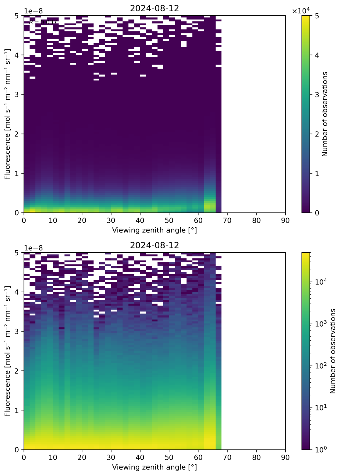
Figure 122: Scatter density plot of “Viewing zenith angle” against “Fluorescence” for 2024-08-12 to 2024-08-13.
