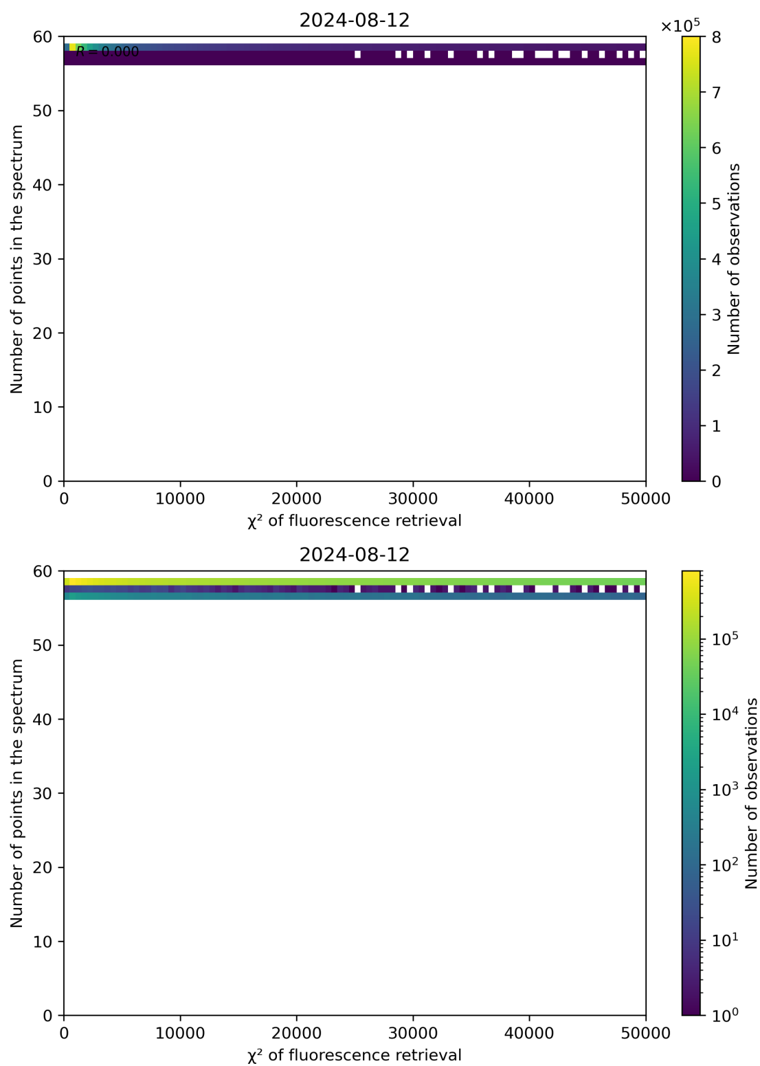
Figure 68: Scatter density plot of " \chi^2 of fluorescence retrieval" against "Number of points in the spectrum" for 2024-08-12 to 2024-08-13.
