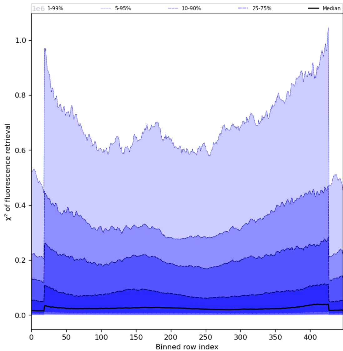
Figure 59: Along track statistics of “ \chi^2 of fluorescence retrieval” for 2024-08-12 to 2024-08-13
