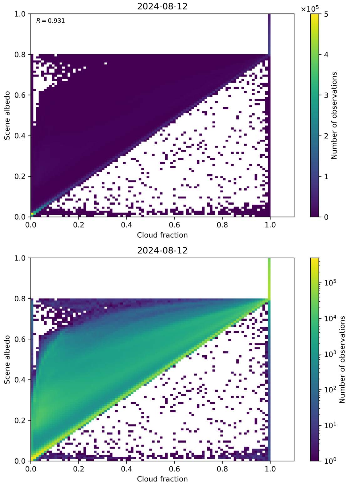
Figure 75: Scatter density plot of “Cloud fraction” against “Scene albedo” for 2024-08-12 to 2024-08-13.
