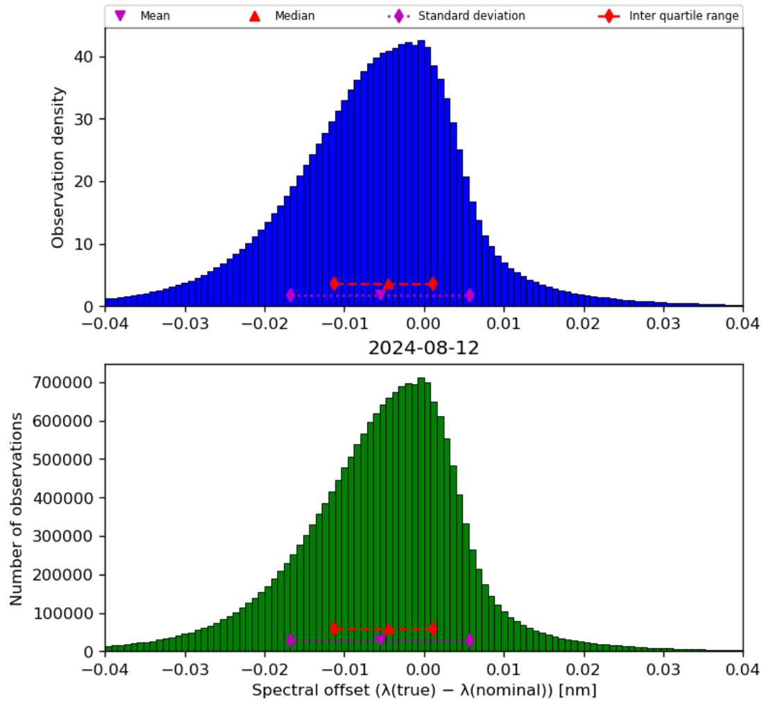
Figure 45: Histogram of “Spectral offset ( \lambda(\text{true}) - \lambda(\text{nominal}) )” for 2024-08-12 to 2024-08-13
