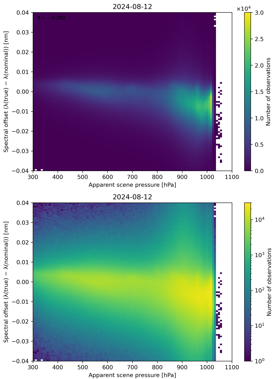
Figure 67: Scatter density plot of “Apparent scene pressure” against “Spectral offset ( \lambda(\text{true}) - \lambda(\text{nominal}) )” for 2024-08-12 to 2024-08-13.
