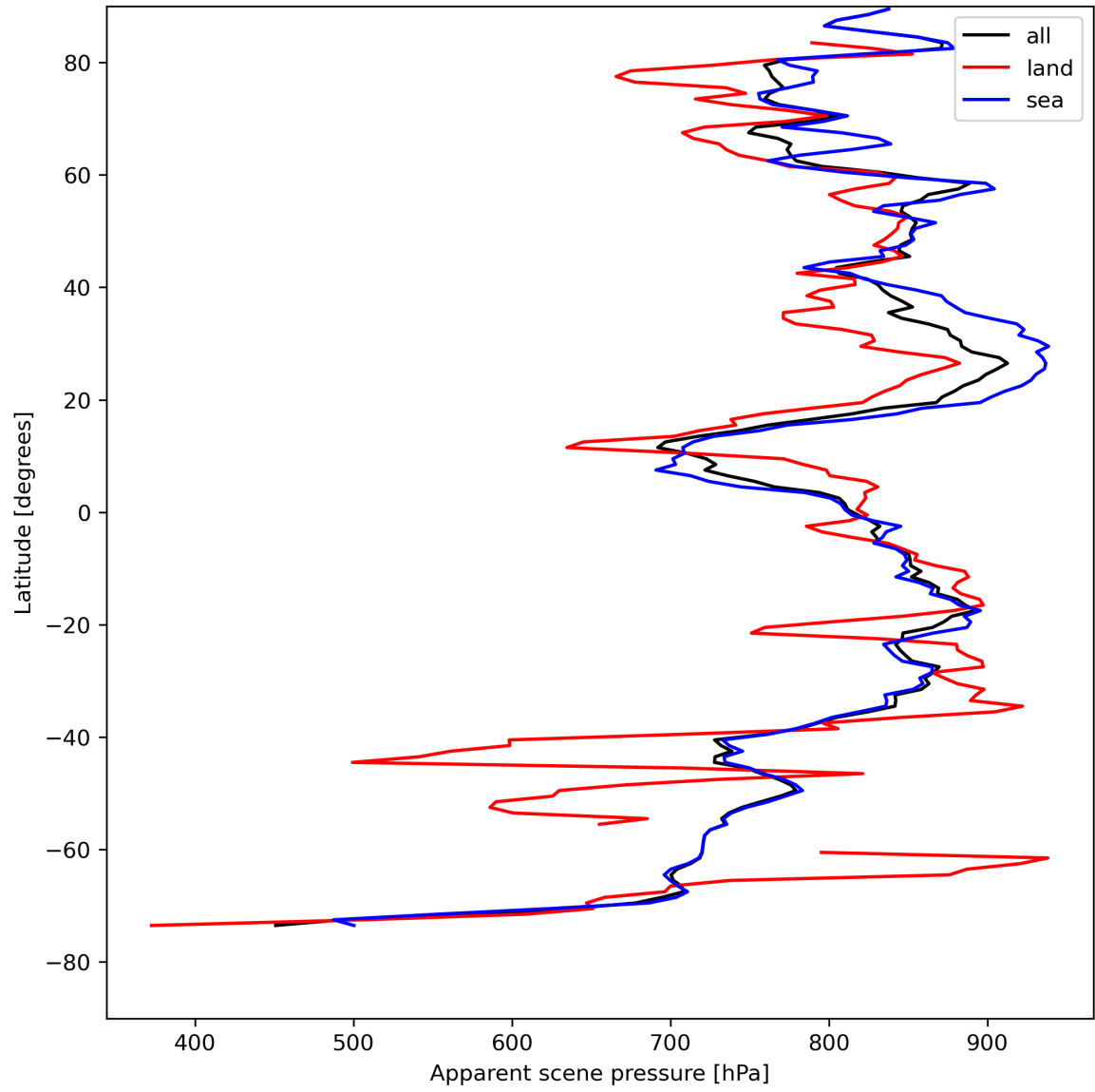
Figure 19: Zonal average of “Apparent scene pressure” for 2024-08-12 to 2024-08-13.
