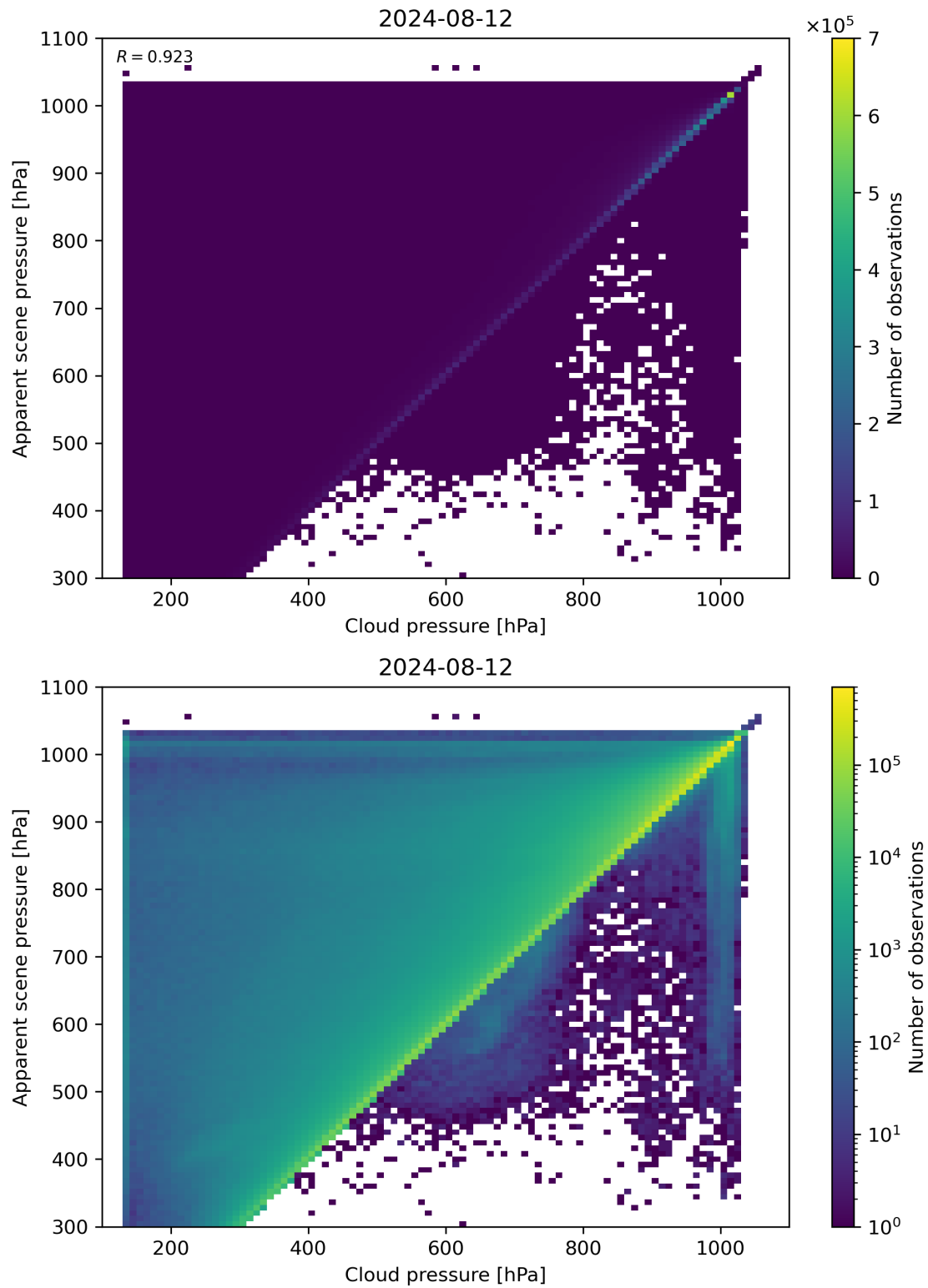
Figure 77: Scatter density plot of “Cloud pressure” against “Apparent scene pressure” for 2024-08-12 to 2024-08-13.
