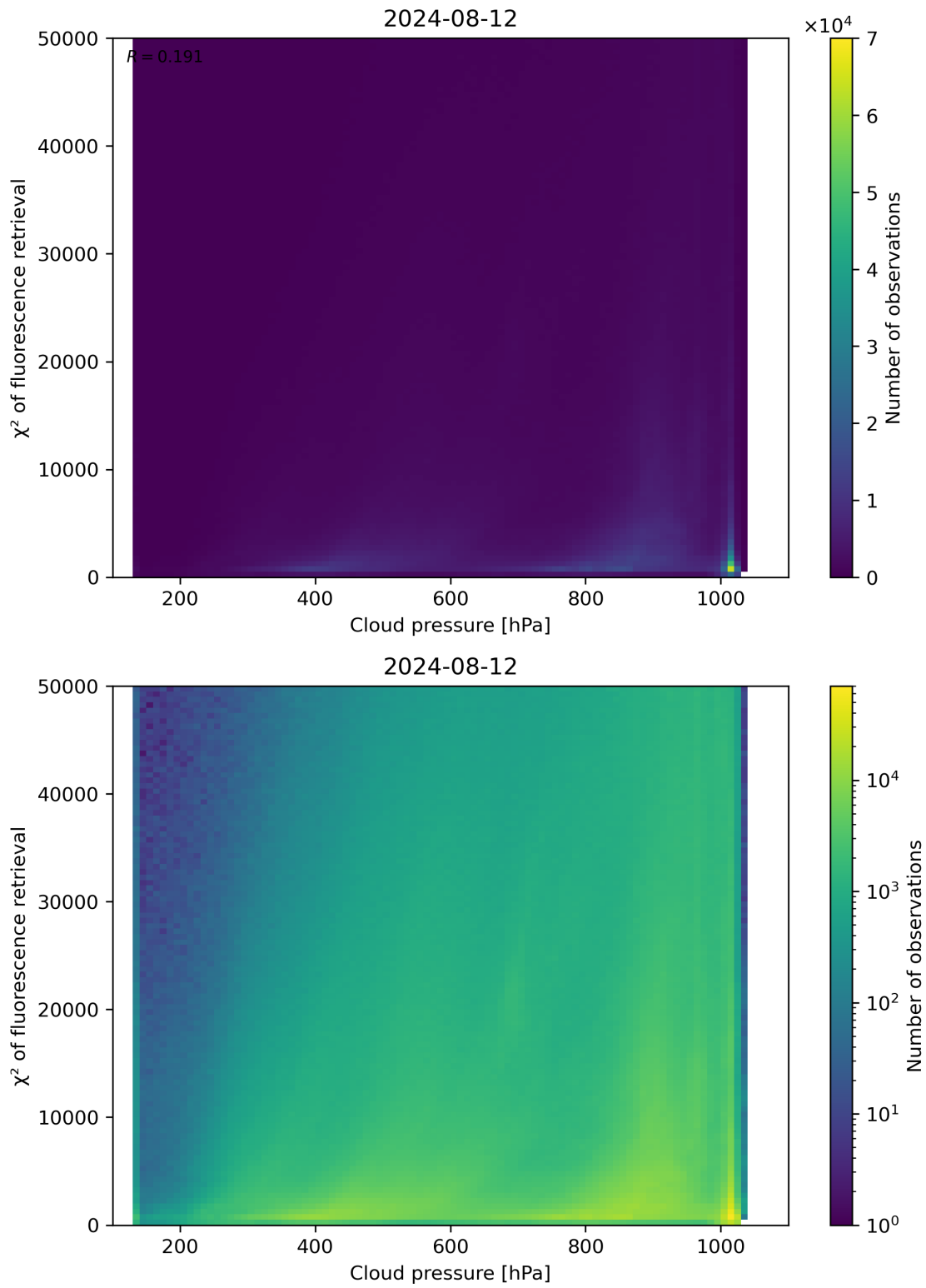
Figure 78: Scatter density plot of “Cloud pressure” against “ \chi^2 of fluorescence retrieval” for 2024-08-12 to 2024-08-13.
