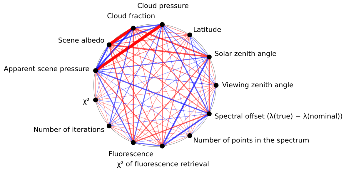
Figure 1: Map of correlation graph for 2024-08-12 to 2024-08-13.
