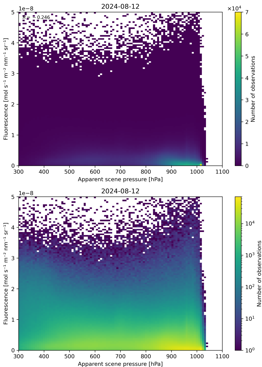
Figure 64: Scatter density plot of “Apparent scene pressure” against “Fluorescence” for 2024-08-12 to 2024-08-13.
