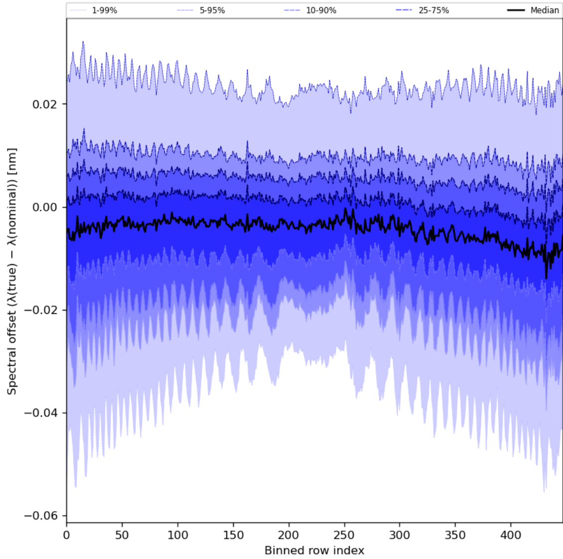
Figure 62: Along track statistics of “Spectral offset ( \lambda(\text{true}) - \lambda(\text{nominal}) )” for 2024-08-12 to 2024-08-13
