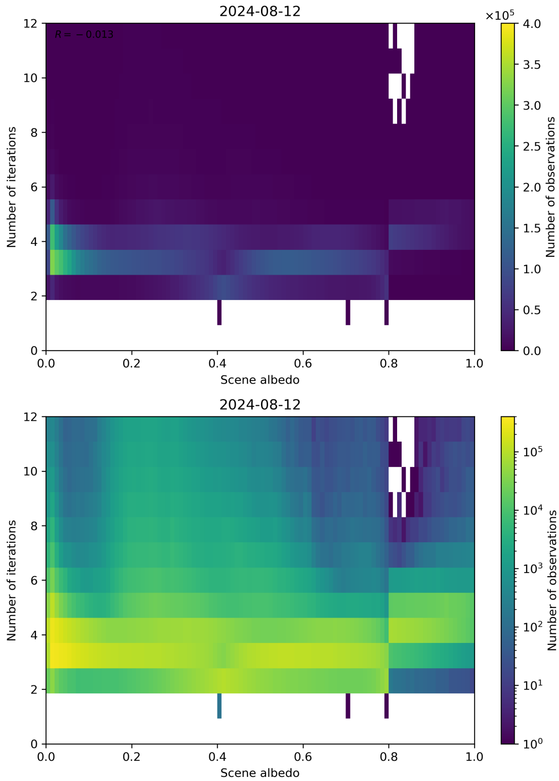
Figure 105: Scatter density plot of “Scene albedo” against “Number of iterations” for 2024-08-12 to 2024-08-13.
