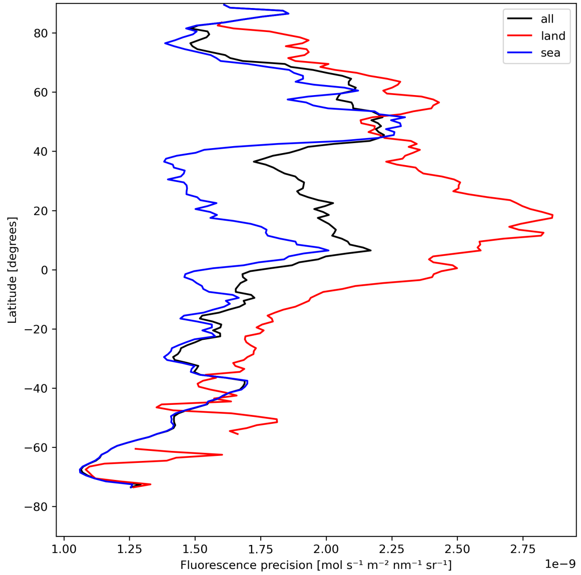
Figure 24: Zonal average of “Fluorescence precision” for 2024-08-12 to 2024-08-13.
