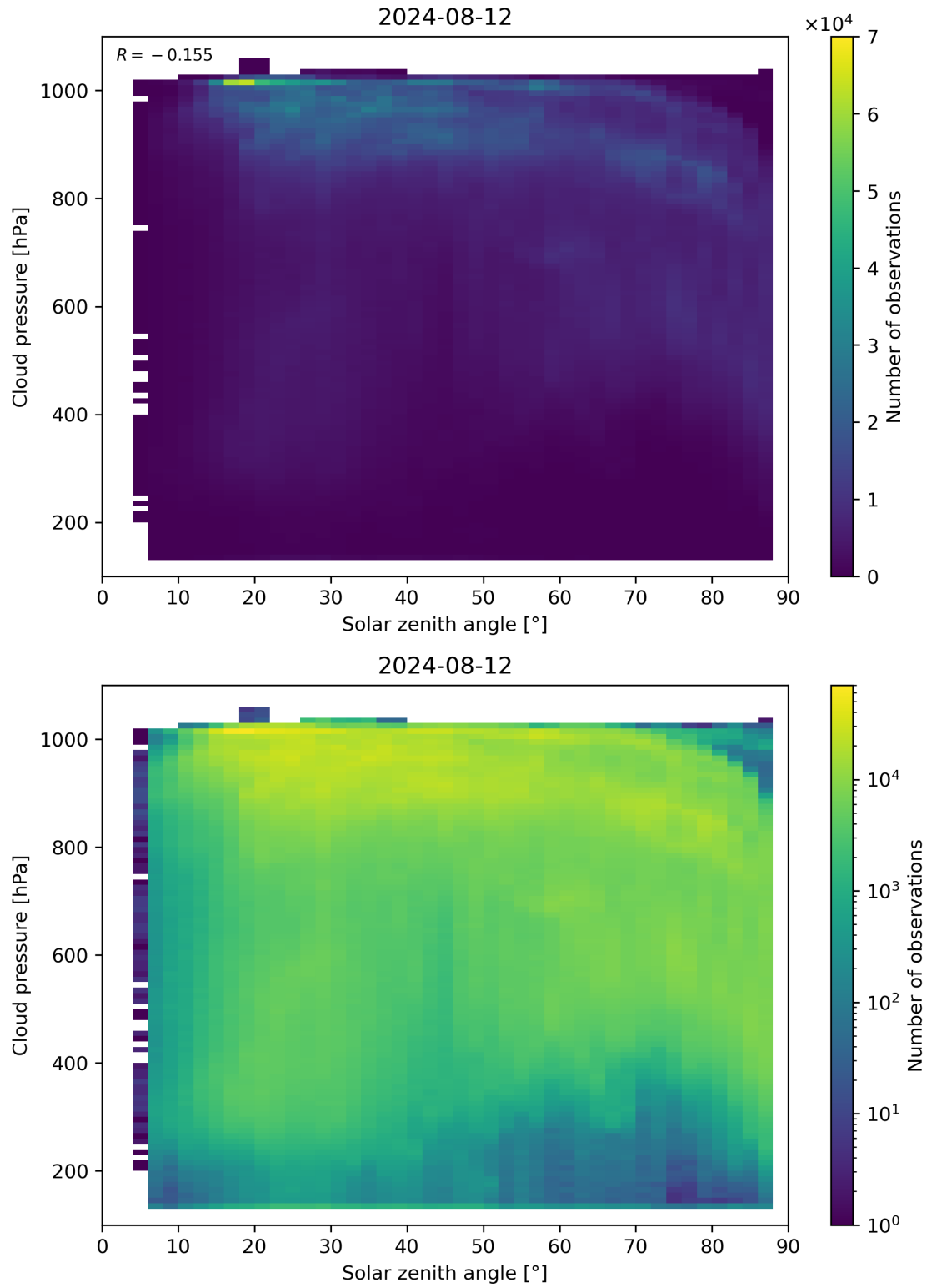
Figure 111: Scatter density plot of “Solar zenith angle” against “Cloud pressure” for 2024-08-12 to 2024-08-13.
