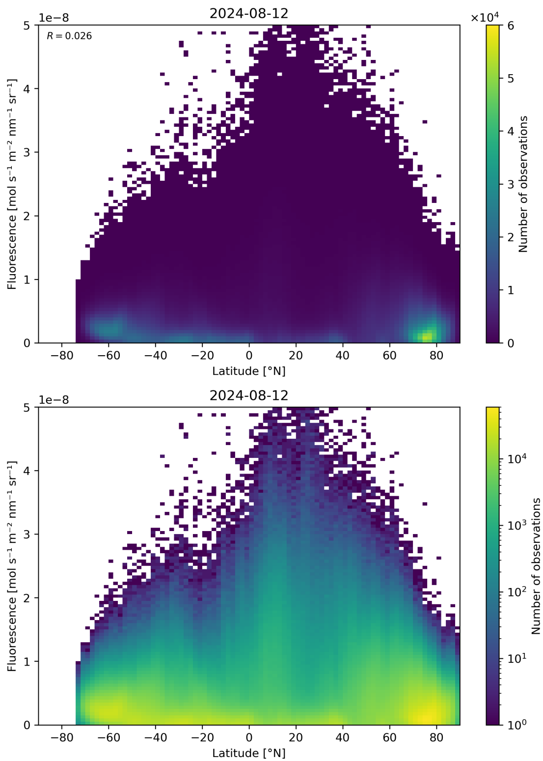
Figure 92: Scatter density plot of “Latitude” against “Fluorescence” for 2024-08-12 to 2024-08-13.
