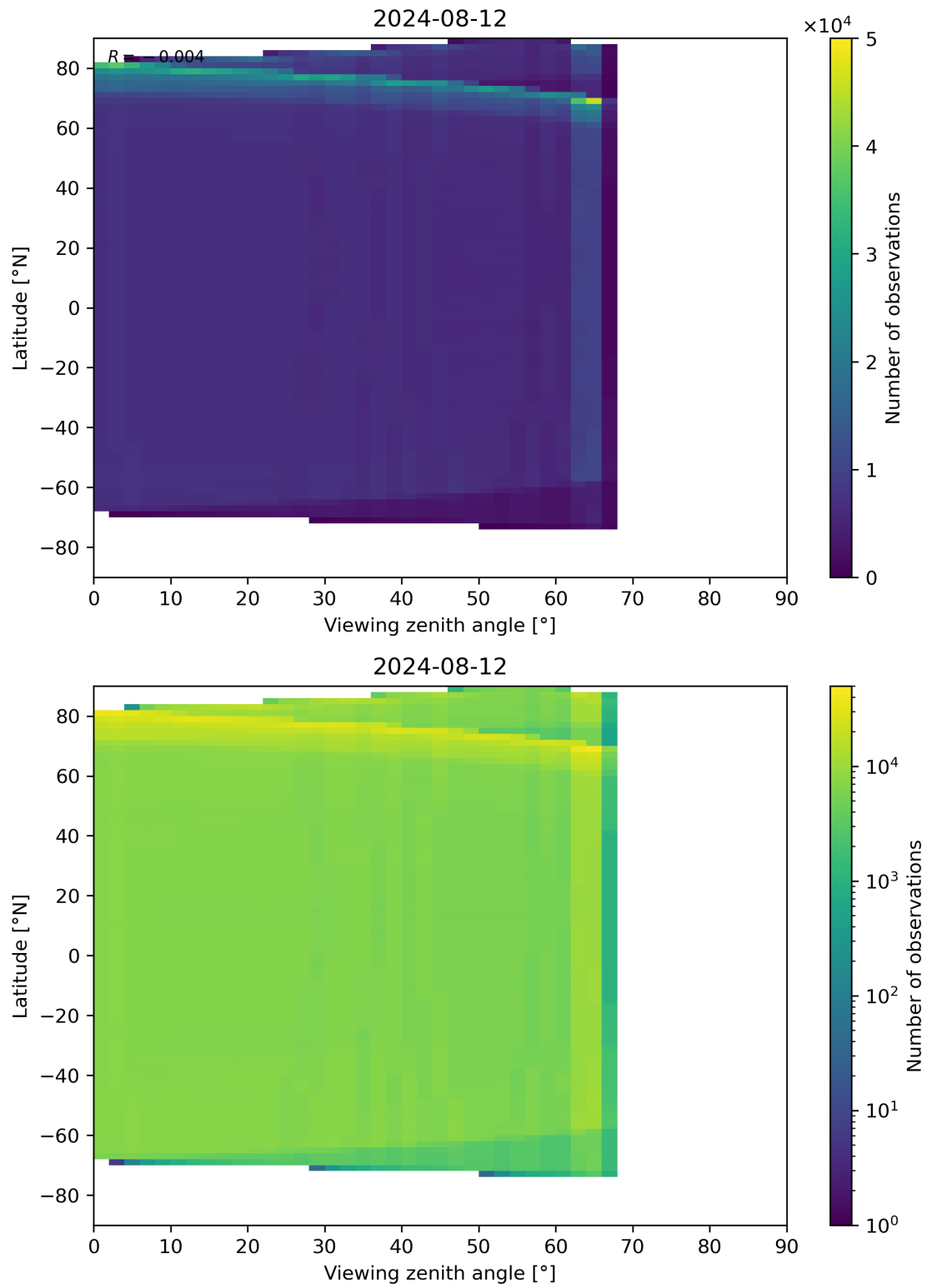
Figure 123: Scatter density plot of “Viewing zenith angle” against “Latitude” for 2024-08-12 to 2024-08-13.
