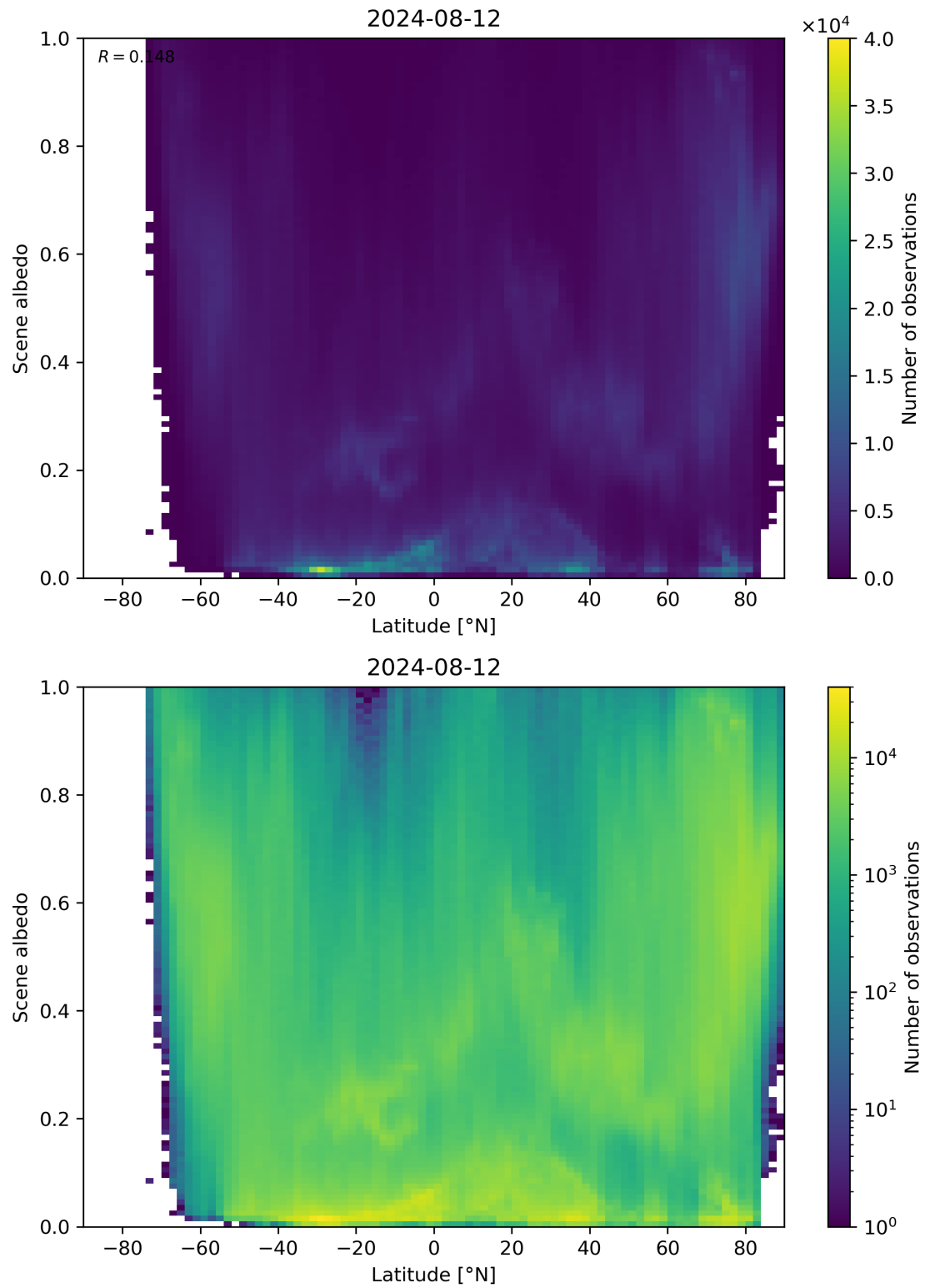
Figure 95: Scatter density plot of “Latitude” against “Scene albedo” for 2024-08-12 to 2024-08-13.
