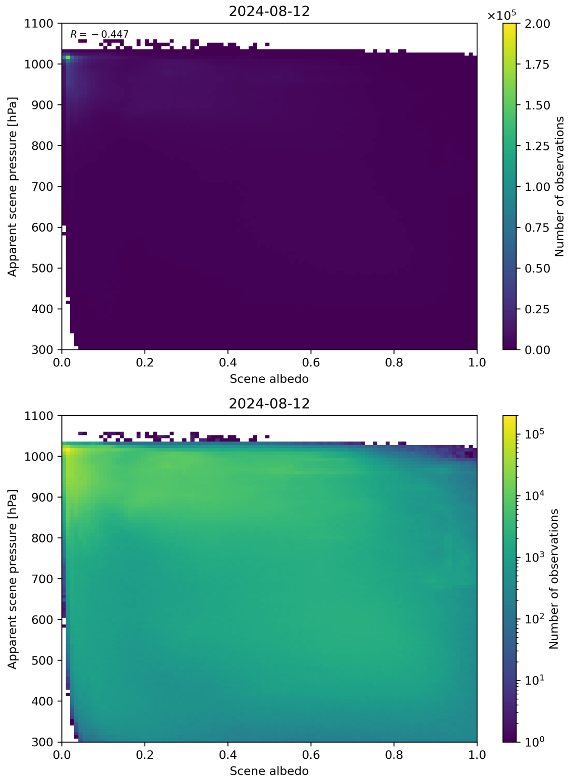
Figure 102: Scatter density plot of “Scene albedo” against “Apparent scene pressure” for 2024-08-12 to 2024-08-13.
