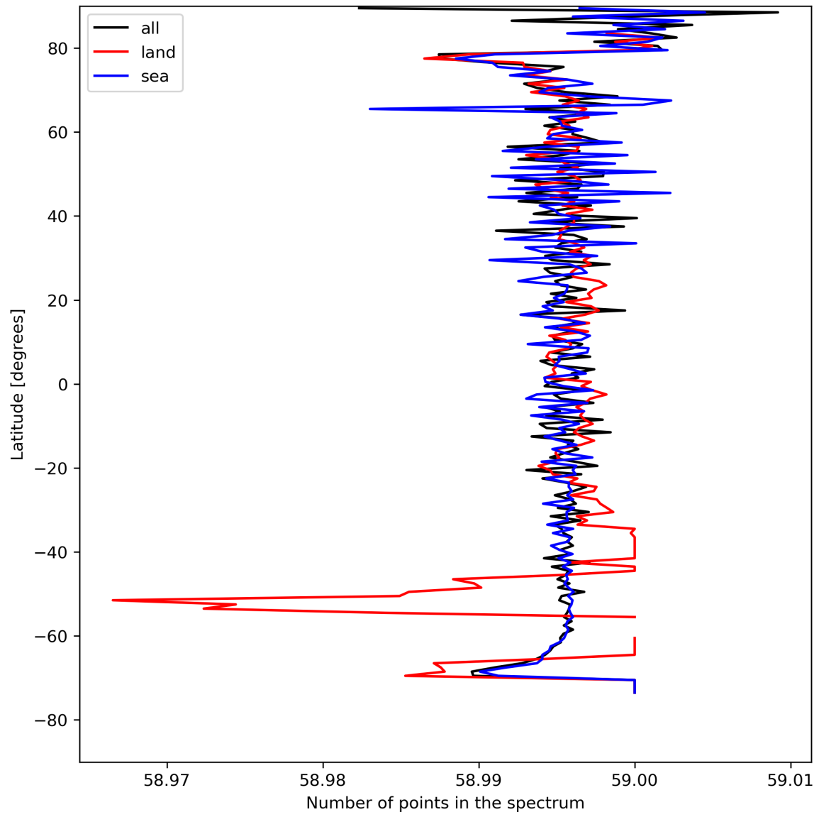
Figure 27: Zonal average of “Number of points in the spectrum” for 2024-08-12 to 2024-08-13.
