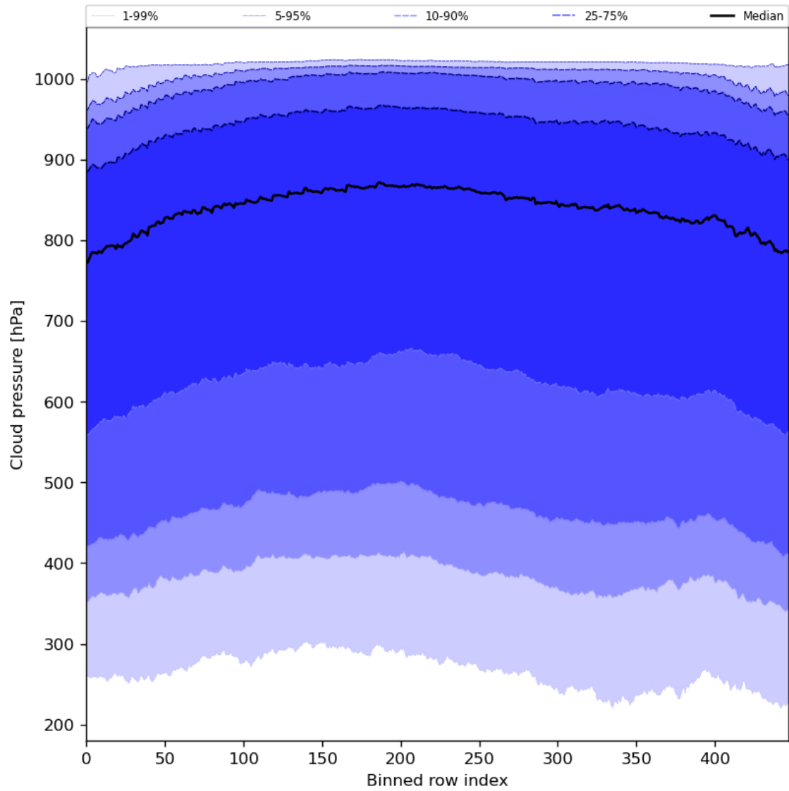
Figure 47: Along track statistics of “Cloud pressure” for 2024-08-12 to 2024-08-13
