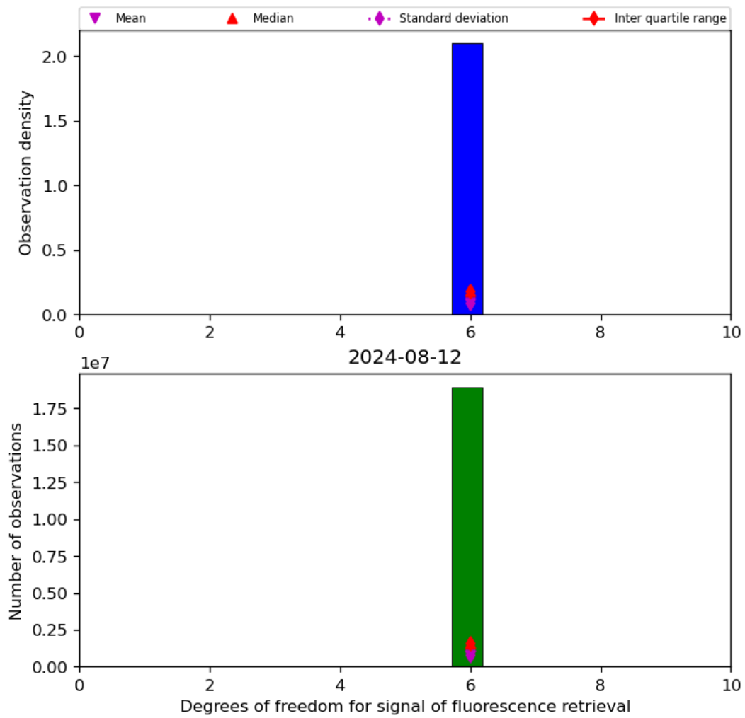
Figure 43: Histogram of “Degrees of freedom for signal of fluorescence retrieval” for 2024-08-12 to 2024-08-13
