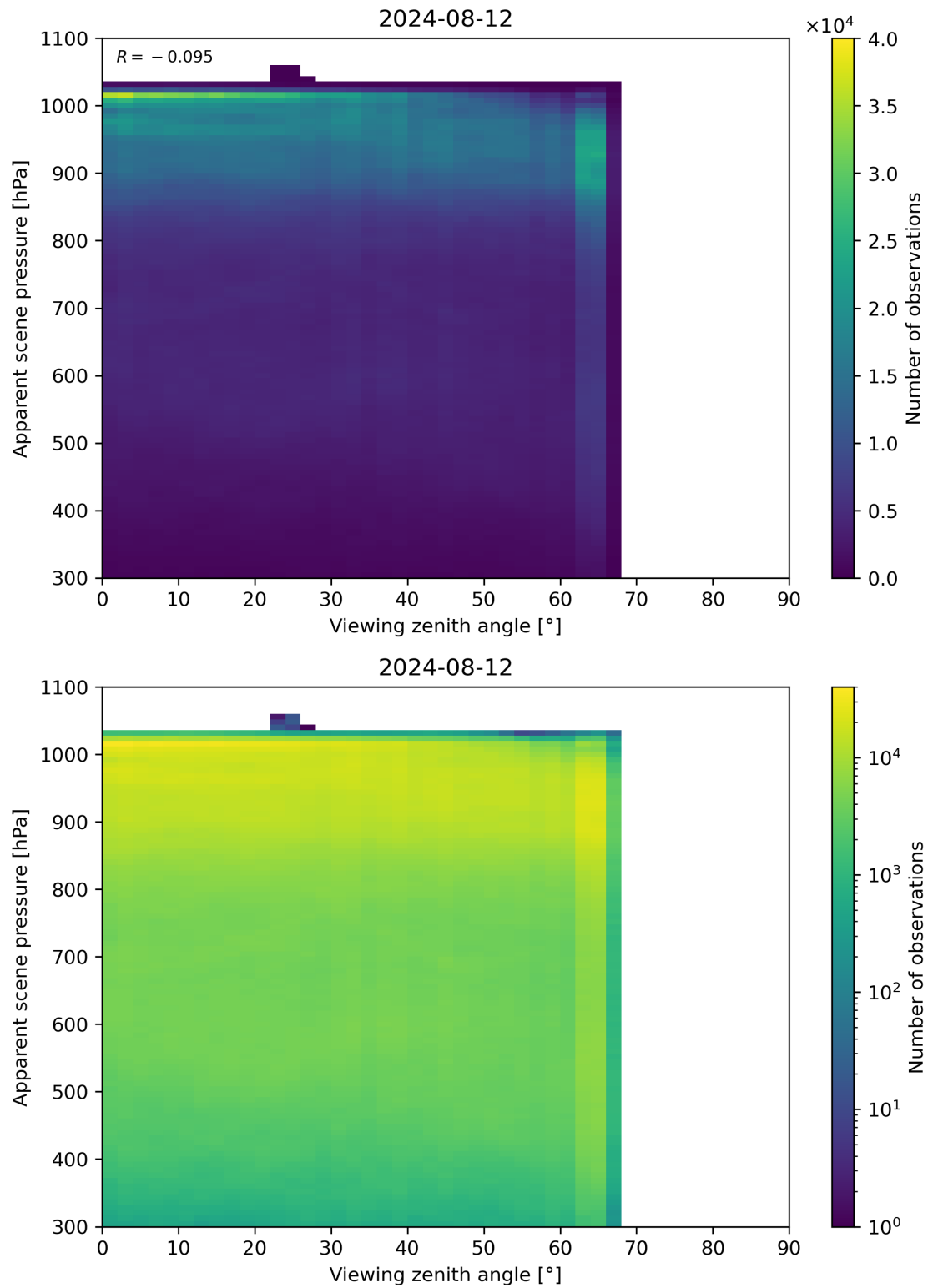
Figure 118: Scatter density plot of “Viewing zenith angle” against “Apparent scene pressure” for 2024-08-12 to 2024-08-13.
