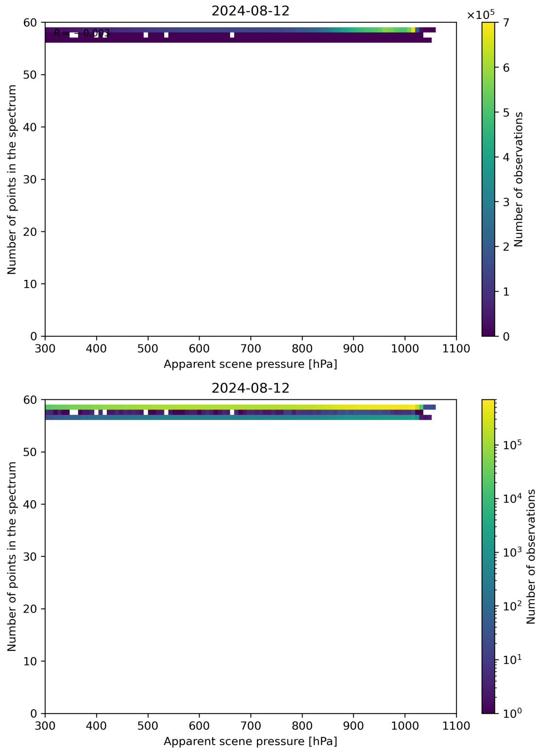
Figure 66: Scatter density plot of “Apparent scene pressure” against “Number of points in the spectrum” for 2024-08-12 to 2024-08-13.
