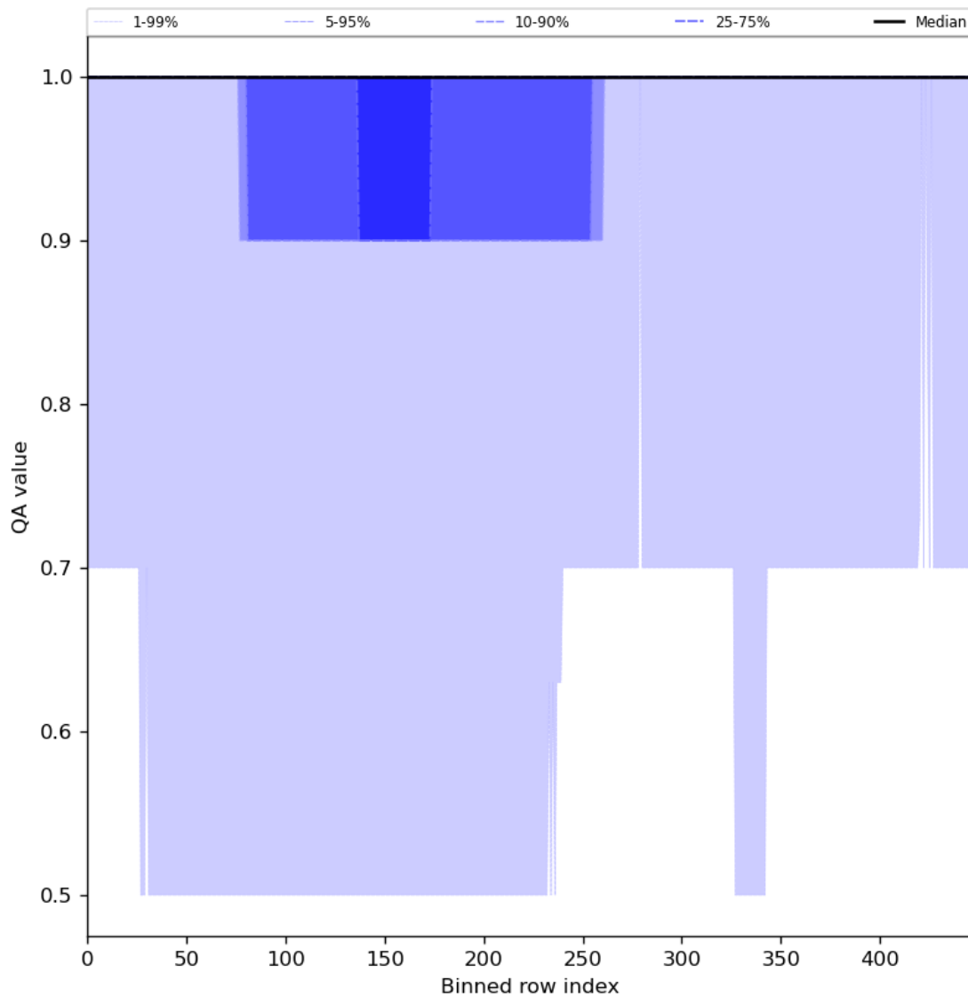
Figure 46: Along track statistics of “QA value” for 2024-08-12 to 2024-08-13
