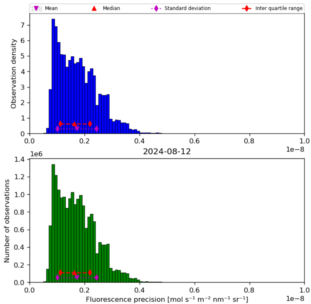
Figure 41: Histogram of “Fluorescence precision” for 2024-08-12 to 2024-08-13
