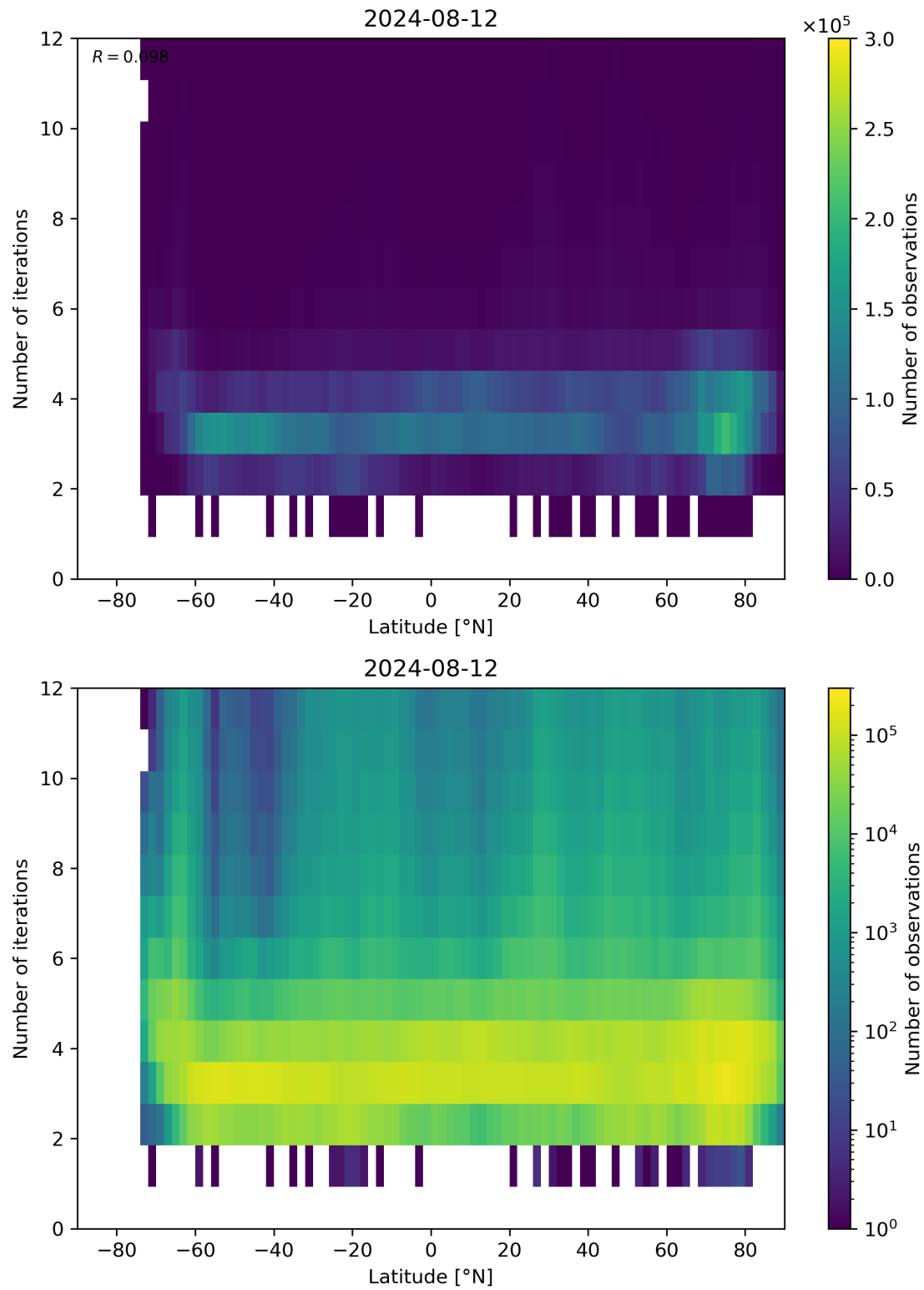
Figure 93: Scatter density plot of “Latitude” against “Number of iterations” for 2024-08-12 to 2024-08-13.
