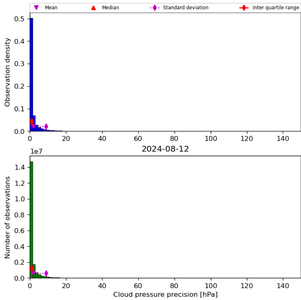
Figure 31: Histogram of “Cloud pressure precision” for 2024-08-12 to 2024-08-13
