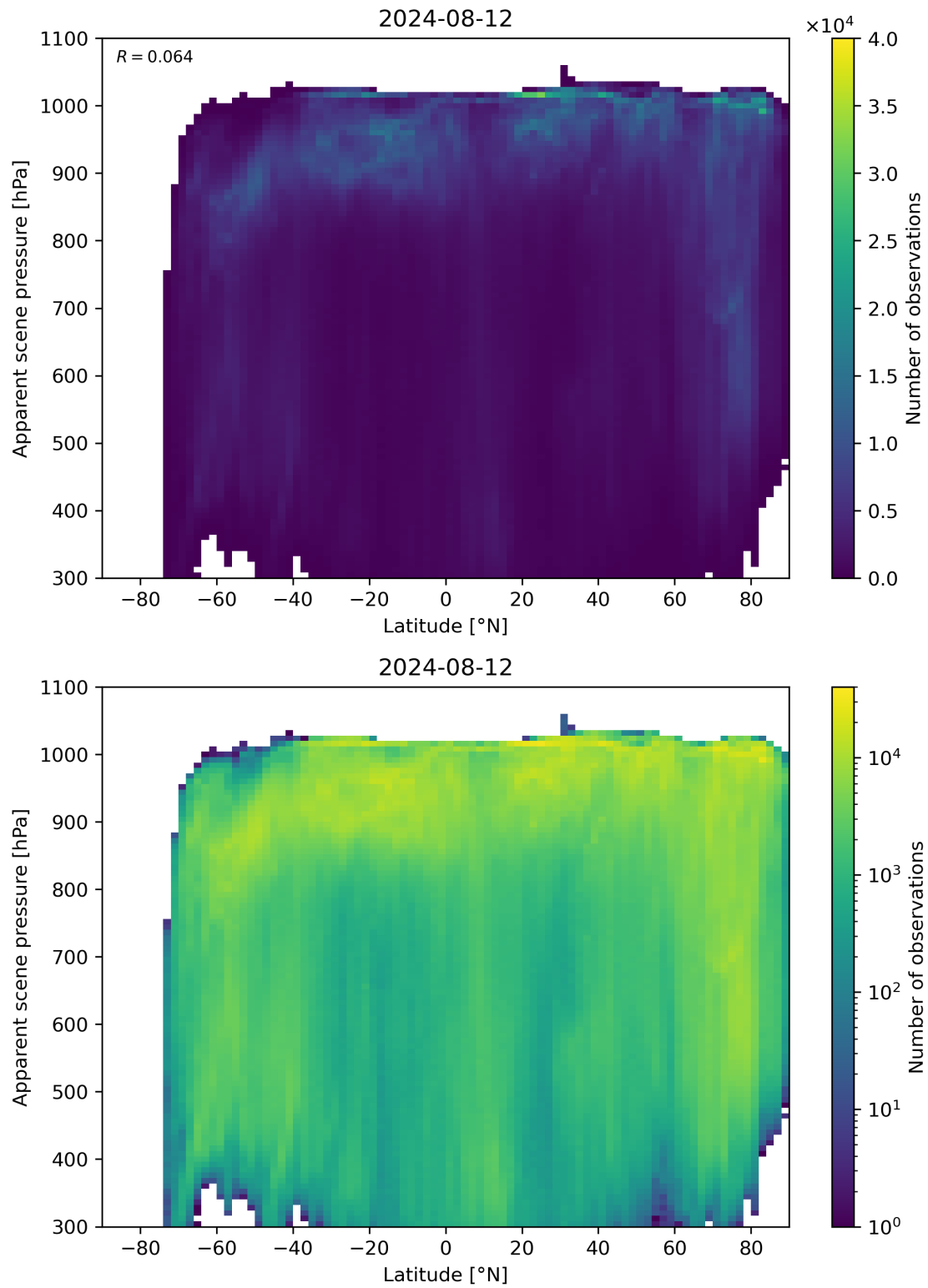
Figure 88: Scatter density plot of “Latitude” against “Apparent scene pressure” for 2024-08-12 to 2024-08-13.
