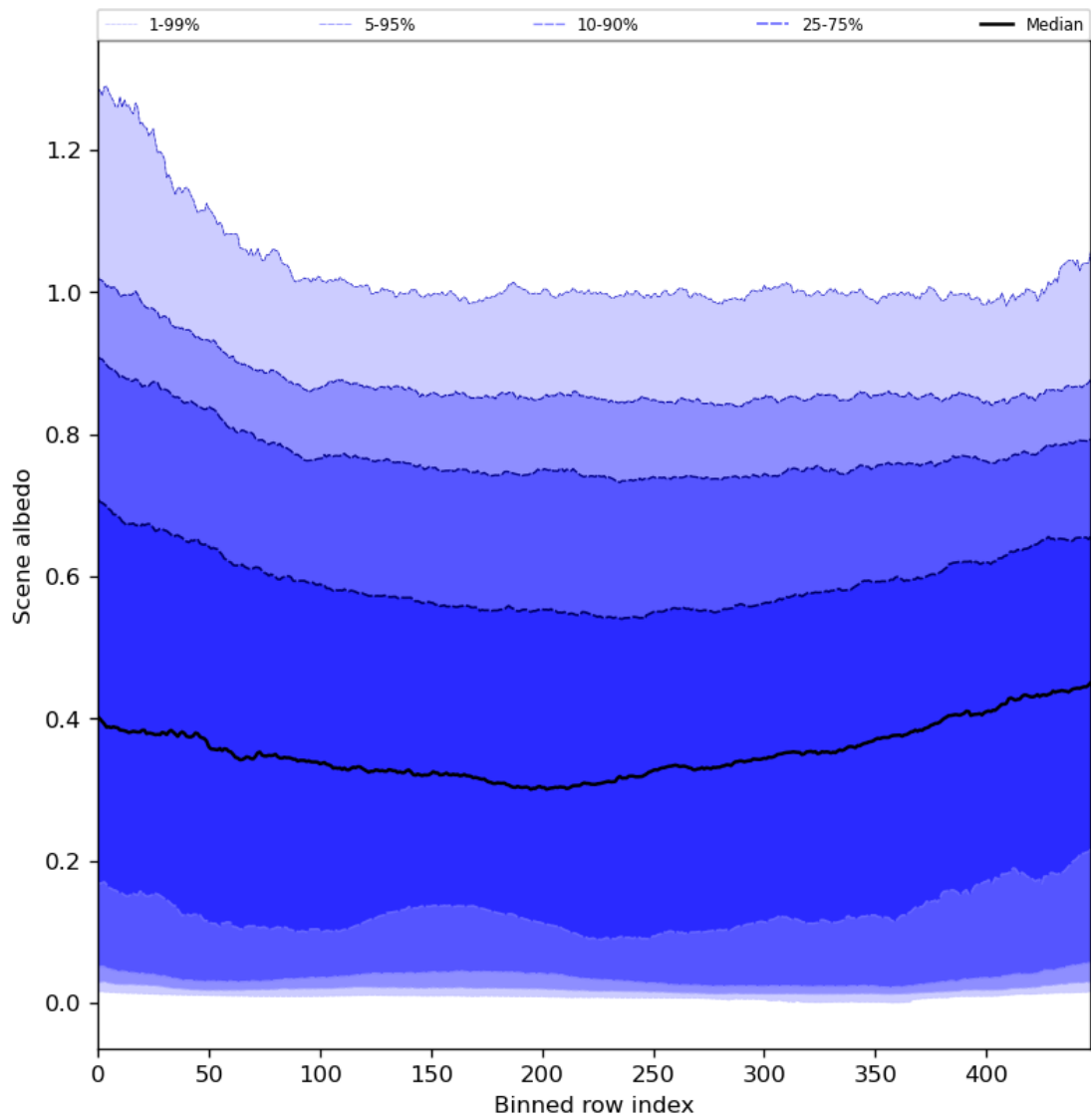
Figure 51: Along track statistics of “Scene albedo” for 2024-08-12 to 2024-08-13
