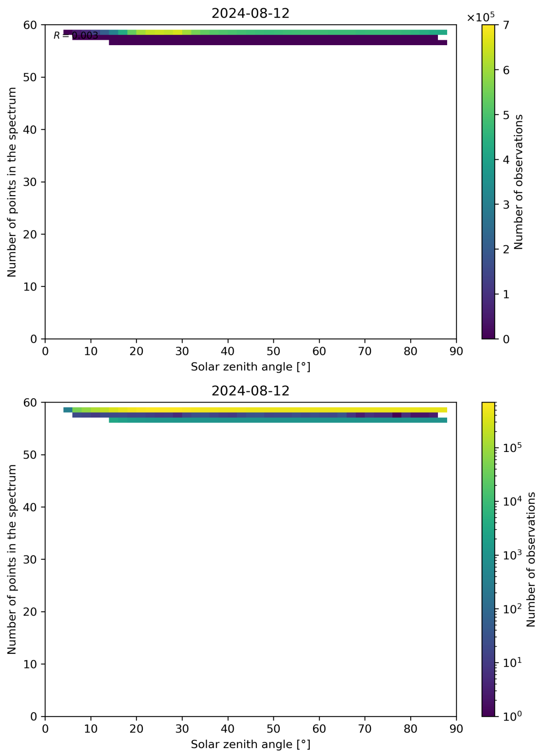
Figure 115: Scatter density plot of “Solar zenith angle” against “Number of points in the spectrum” for 2024-08-12 to 2024-08-13.
