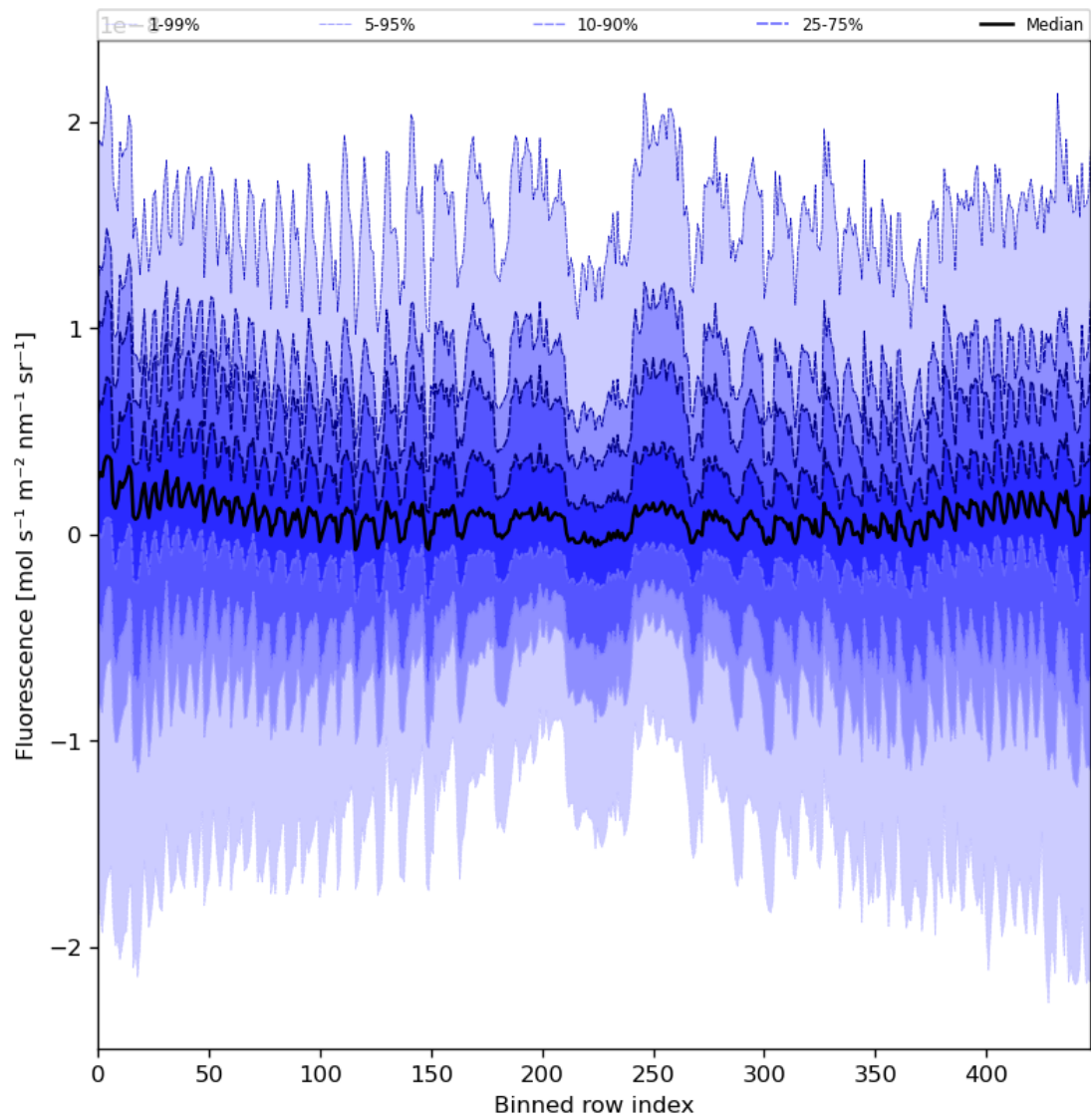
Figure 57: Along track statistics of “Fluorescence” for 2024-08-12 to 2024-08-13
