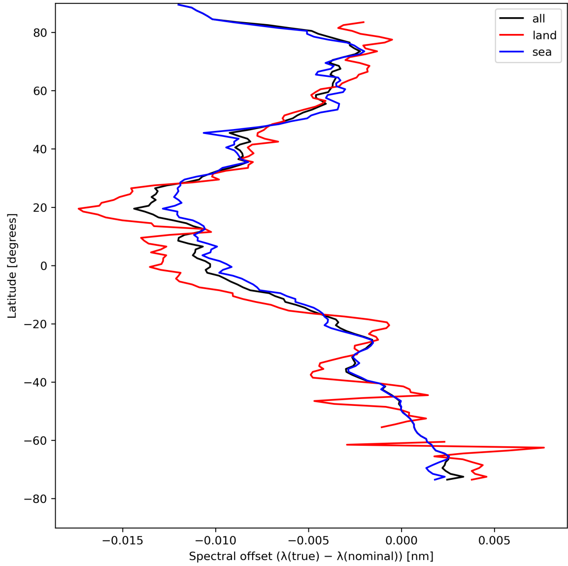
Figure 28: Zonal average of “Spectral offset ( \lambda(\text{true}) - \lambda(\text{nominal}) )” for 2024-08-12 to 2024-08-13.
