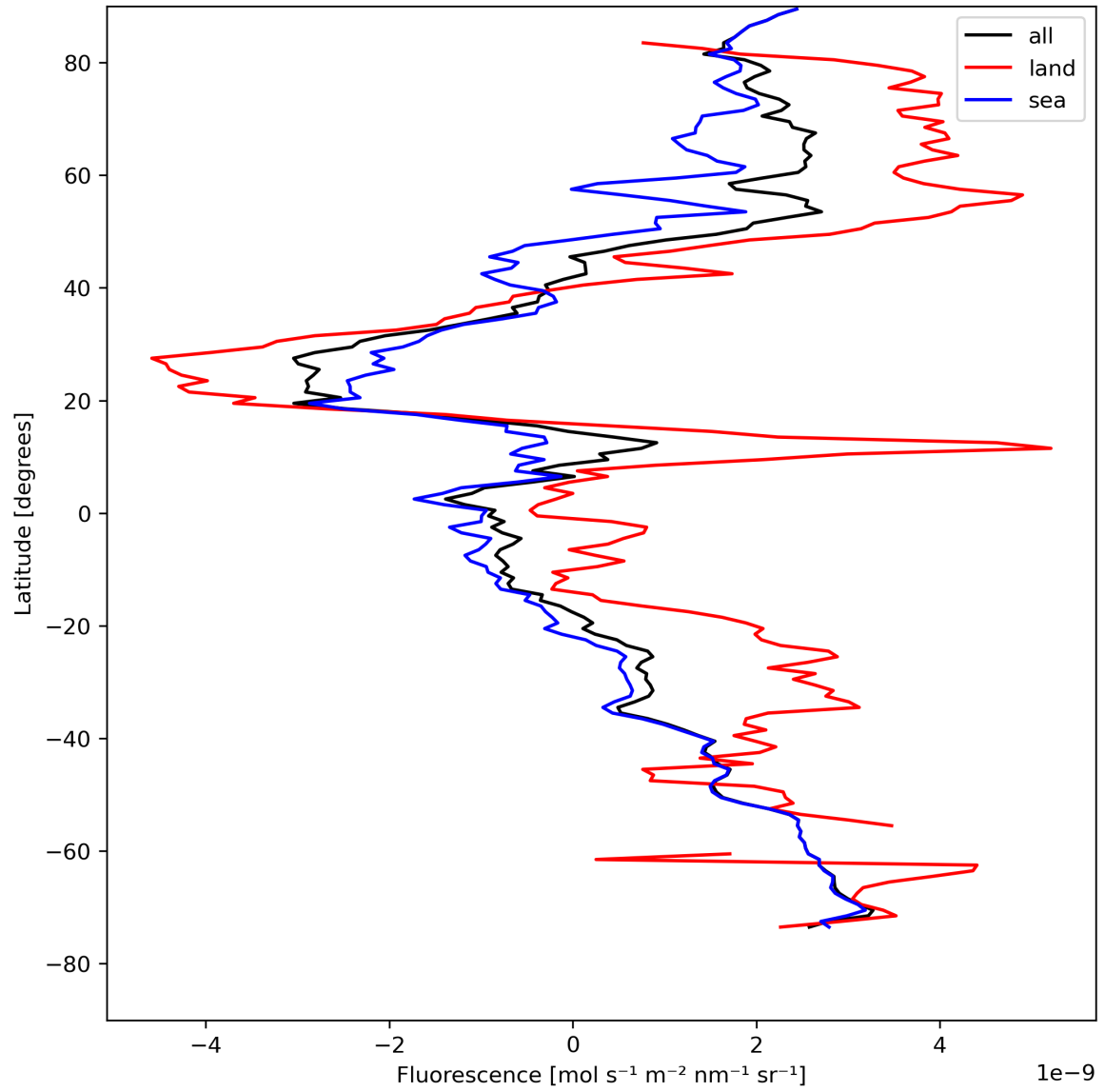
Figure 23: Zonal average of “Fluorescence” for 2024-08-12 to 2024-08-13.
