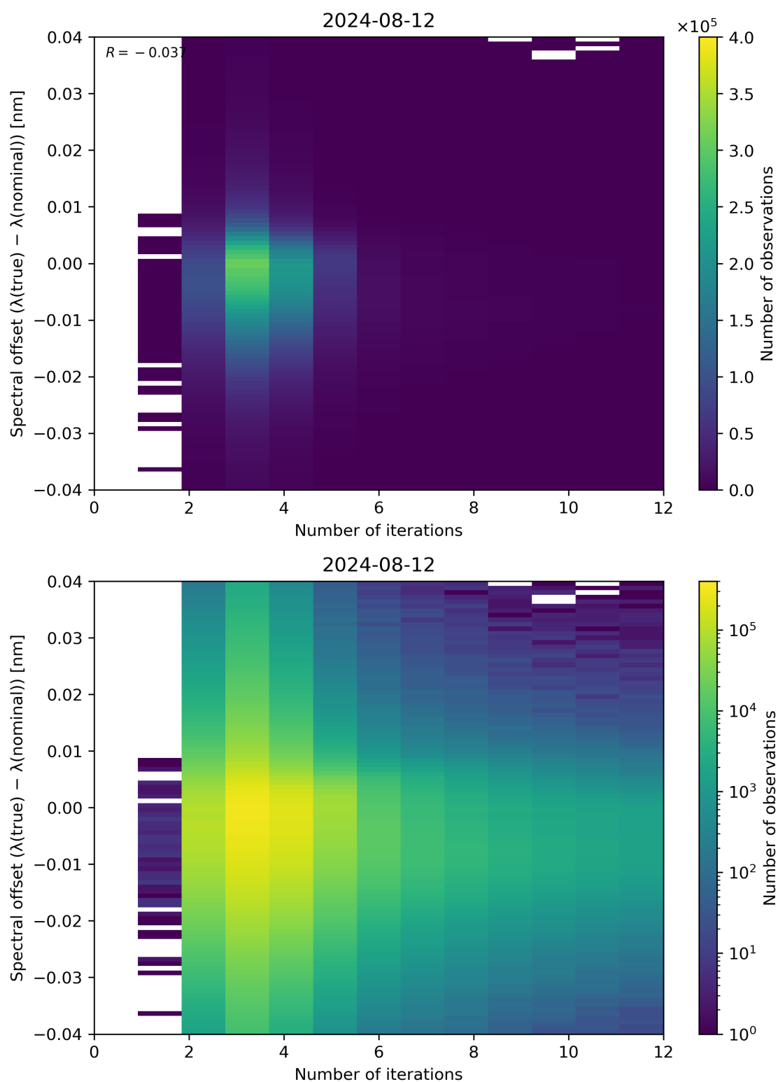
Figure 100: Scatter density plot of “Number of iterations” against “Spectral offset ( \lambda(\text{true}) - \lambda(\text{nominal}) )” for 2024-08-12 to 2024-08-13.
