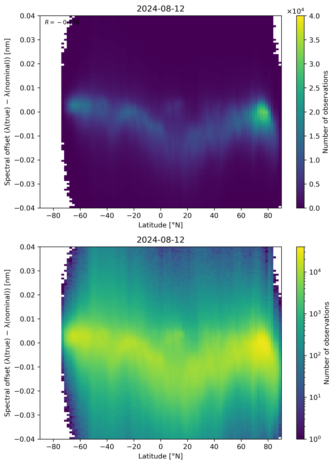
Figure 96: Scatter density plot of “Latitude” against “Spectral offset ( \lambda(\text{true}) - \lambda(\text{nominal}) )” for 2024-08-12 to 2024-08-13.
