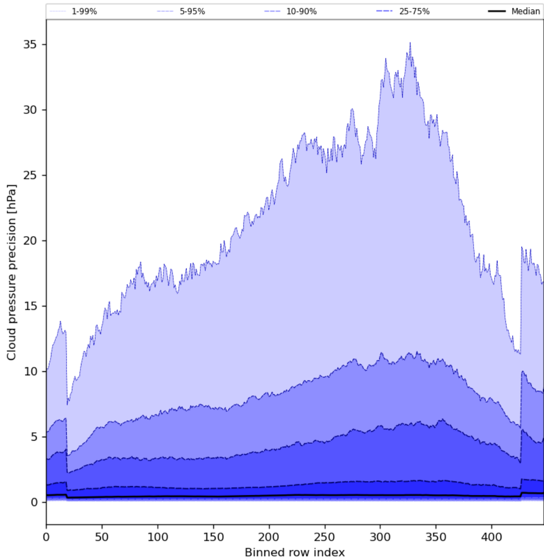
Figure 48: Along track statistics of “Cloud pressure precision” for 2024-08-12 to 2024-08-13
