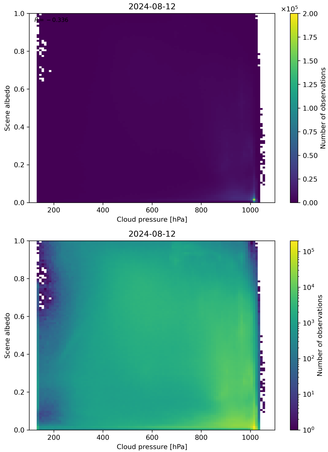
Figure 83: Scatter density plot of “Cloud pressure” against “Scene albedo” for 2024-08-12 to 2024-08-13.
