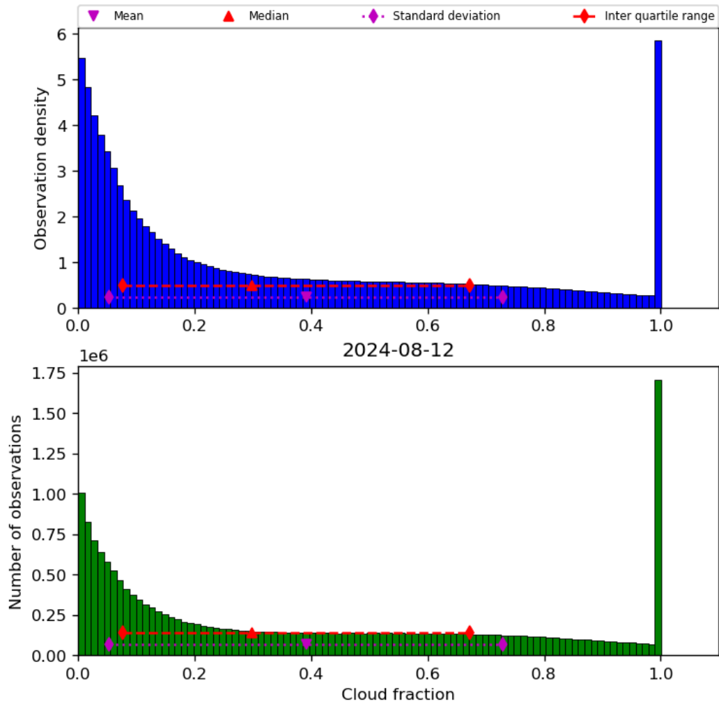
Figure 32: Histogram of “Cloud fraction” for 2024-08-12 to 2024-08-13
