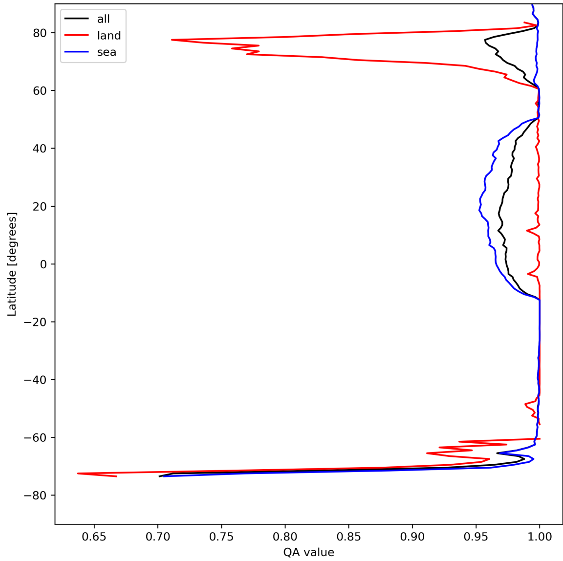
Figure 12: Zonal average of “QA value” for 2024-08-12 to 2024-08-13.
