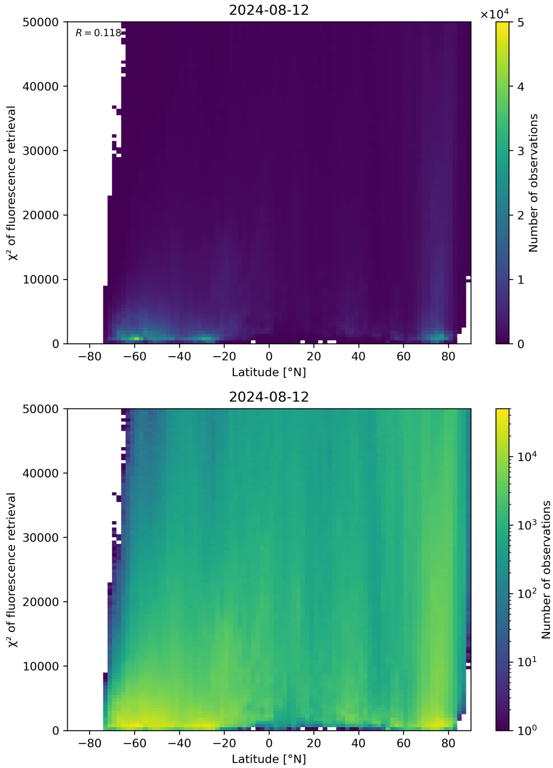
Figure 89: Scatter density plot of “Latitude” against “ \chi^2 of fluorescence retrieval” for 2024-08-12 to 2024-08-13.
