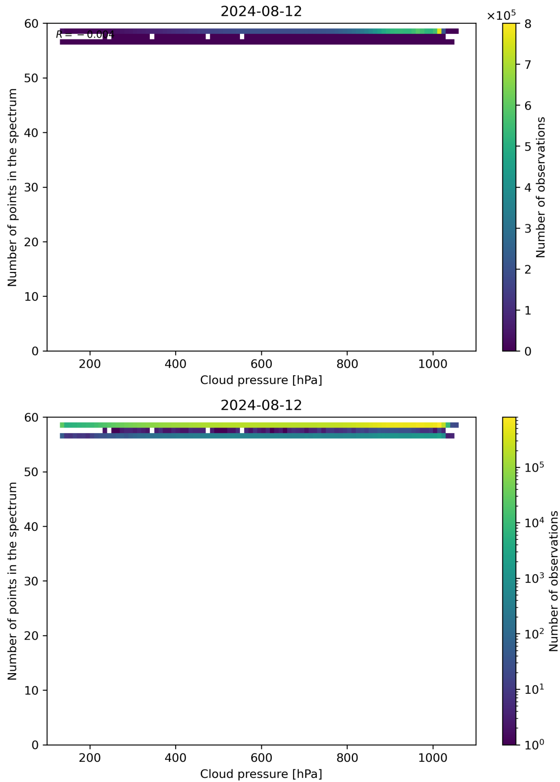
Figure 82: Scatter density plot of “Cloud pressure” against “Number of points in the spectrum” for 2024-08-12 to 2024-08-13.
