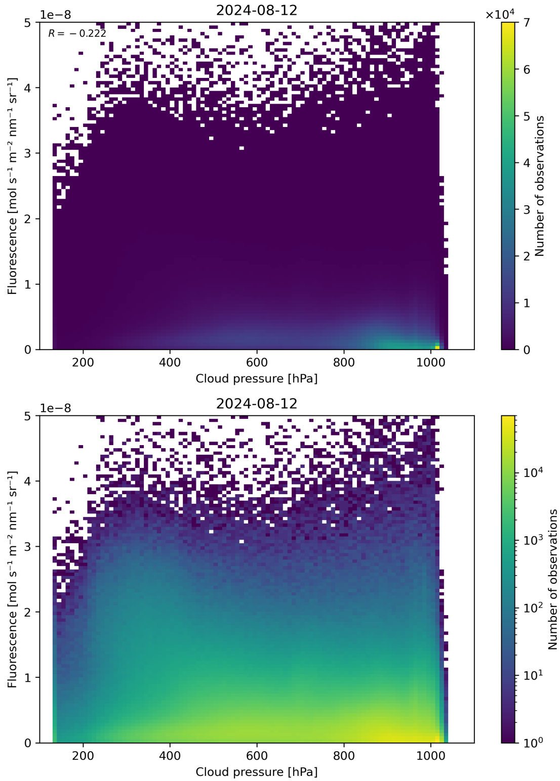
Figure 80: Scatter density plot of “Cloud pressure” against “Fluorescence” for 2024-08-12 to 2024-08-13.
