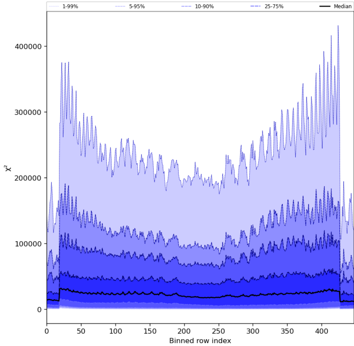
Figure 55: Along track statistics of “ \chi^2 ” for 2024-08-12 to 2024-08-13
