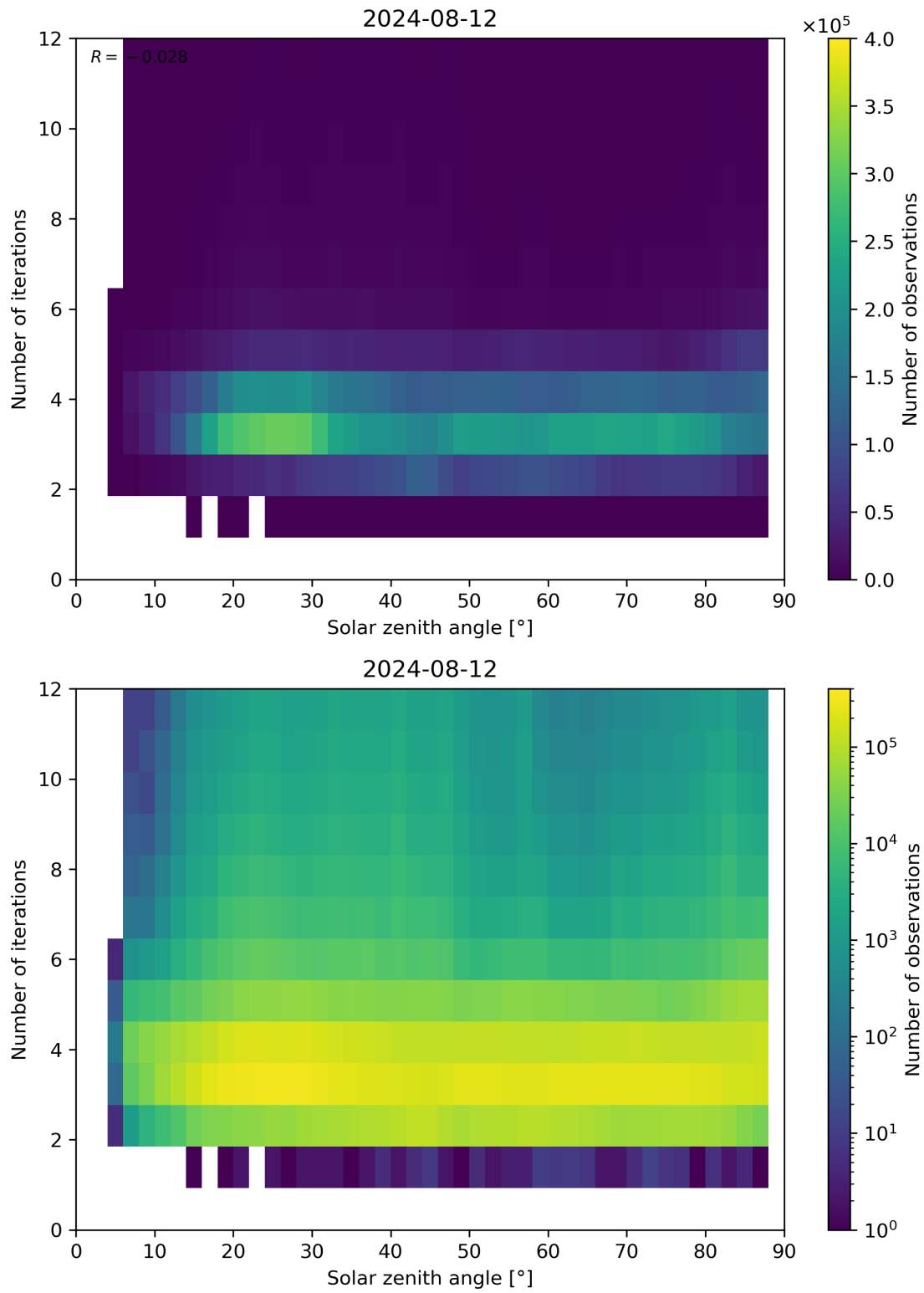
Figure 114: Scatter density plot of “Solar zenith angle” against “Number of iterations” for 2024-08-12 to 2024-08-13.
