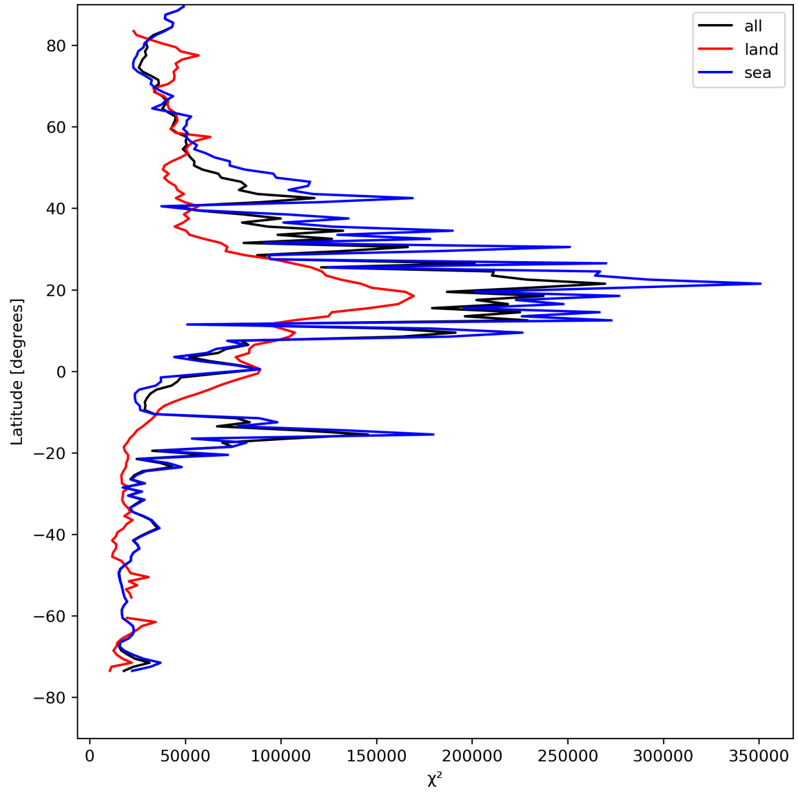
Figure 21: Zonal average of “ \chi^2 ” for 2024-08-12 to 2024-08-13.
