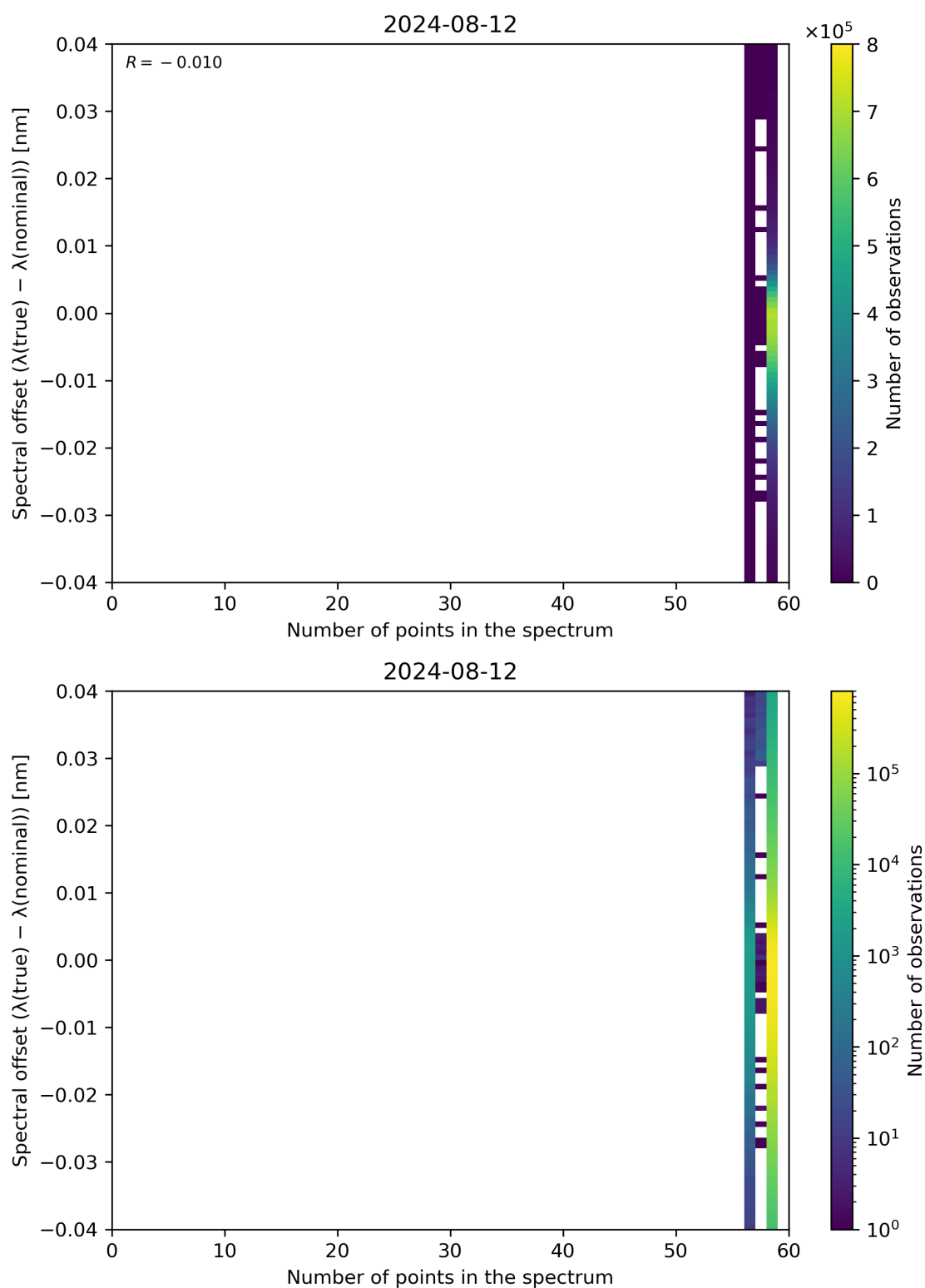
Figure 101: Scatter density plot of “Number of points in the spectrum” against “Spectral offset ( \lambda(\text{true}) - \lambda(\text{nominal}) )” for 2024-08-12 to 2024-08-13.
