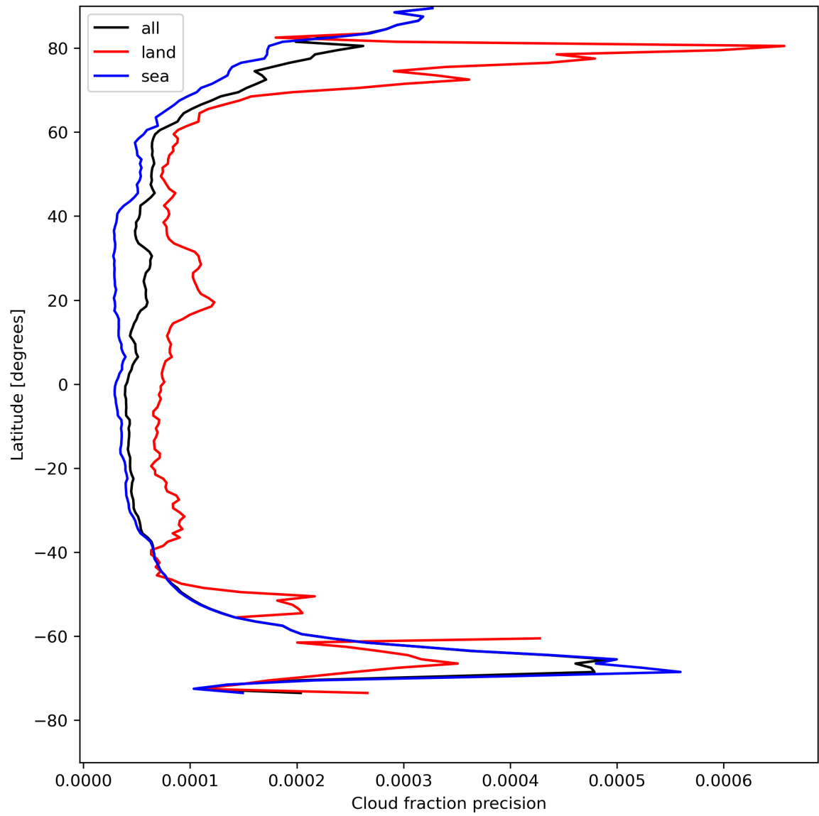
Figure 16: Zonal average of “Cloud fraction precision” for 2024-08-12 to 2024-08-13.
