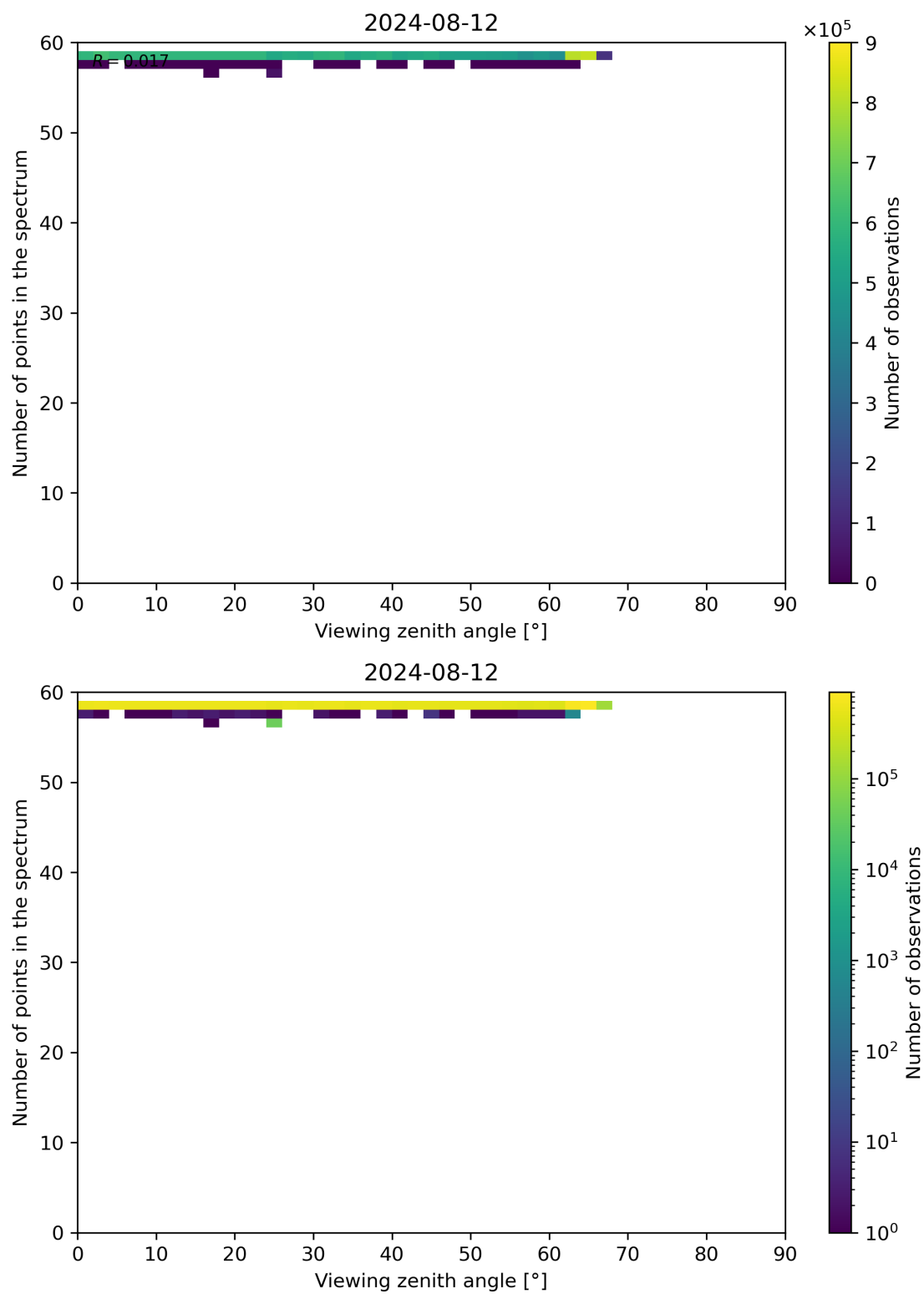
Figure 125: Scatter density plot of “Viewing zenith angle” against “Number of points in the spectrum” for 2024-08-12 to 2024-08-13.
