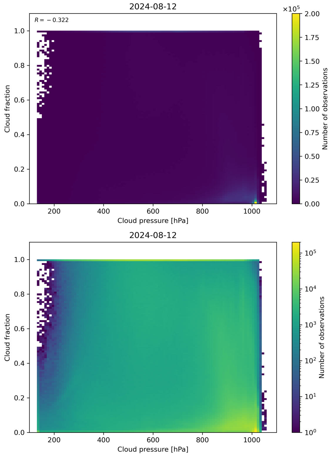
Figure 79: Scatter density plot of “Cloud pressure” against “Cloud fraction” for 2024-08-12 to 2024-08-13.
