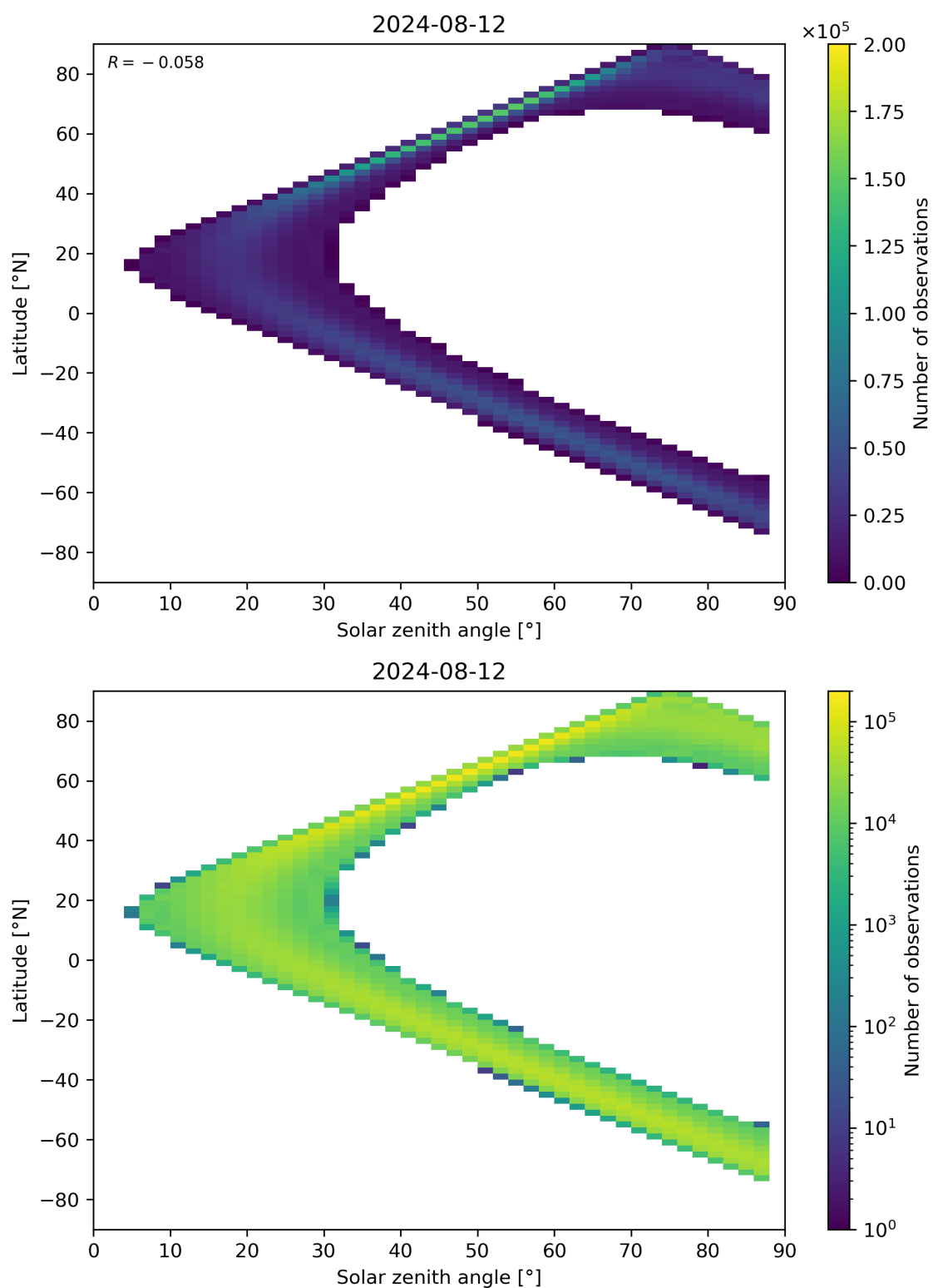
Figure 113: Scatter density plot of “Solar zenith angle” against “Latitude” for 2024-08-12 to 2024-08-13.
