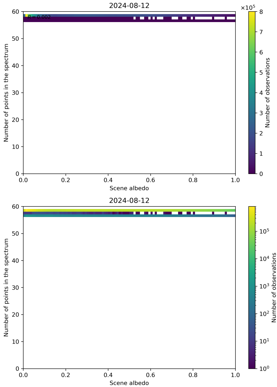
Figure 106: Scatter density plot of “Scene albedo” against “Number of points in the spectrum” for 2024-08-12 to 2024-08-13.
