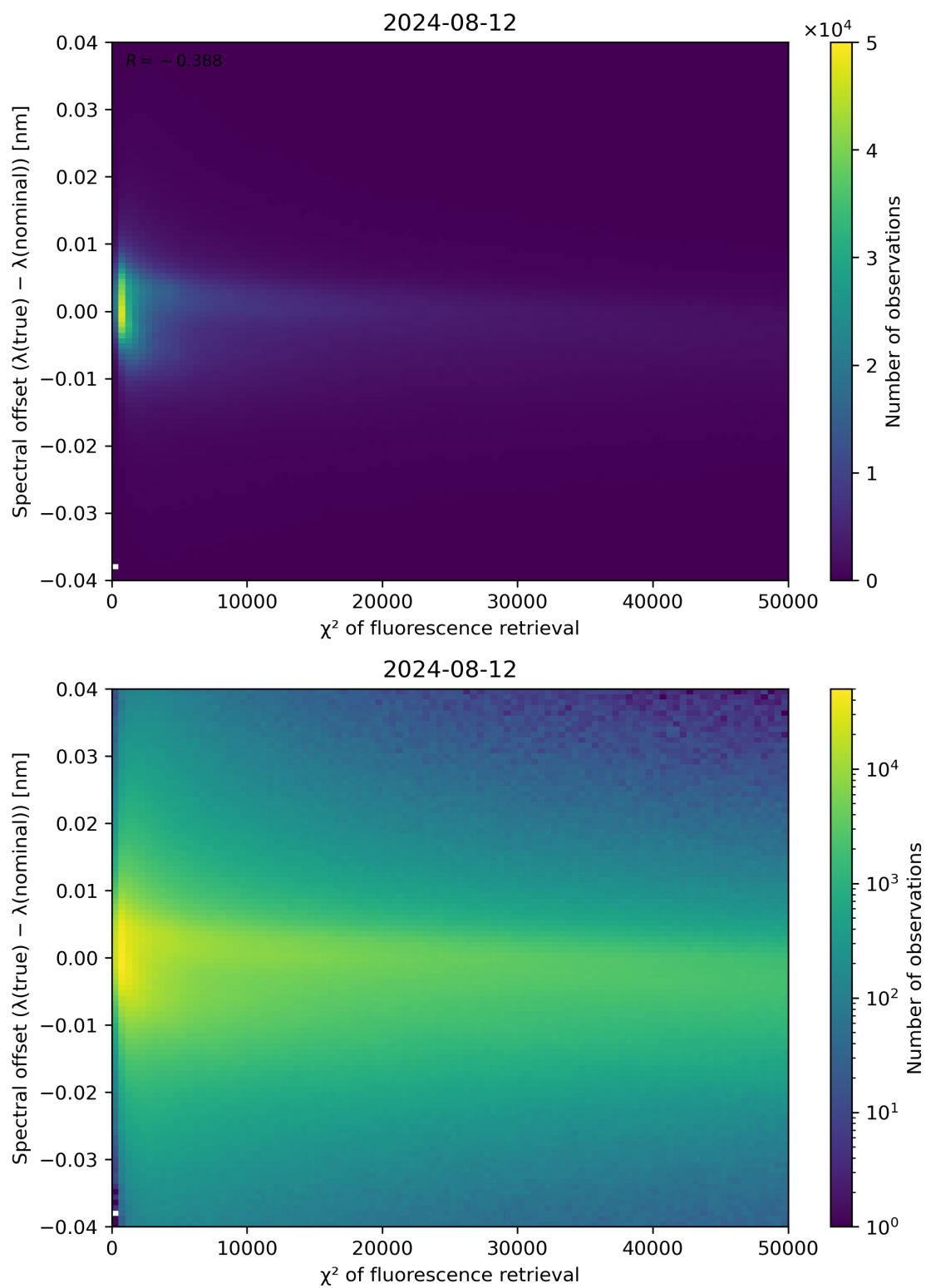
Figure 69: Scatter density plot of " \chi^2 of fluorescence retrieval" against "Spectral offset ( \lambda(\text{true}) - \lambda(\text{nominal}) )" for 2024-08-12 to 2024-08-13.
