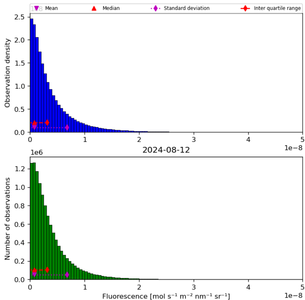
Figure 40: Histogram of “Fluorescence” for 2024-08-12 to 2024-08-13
