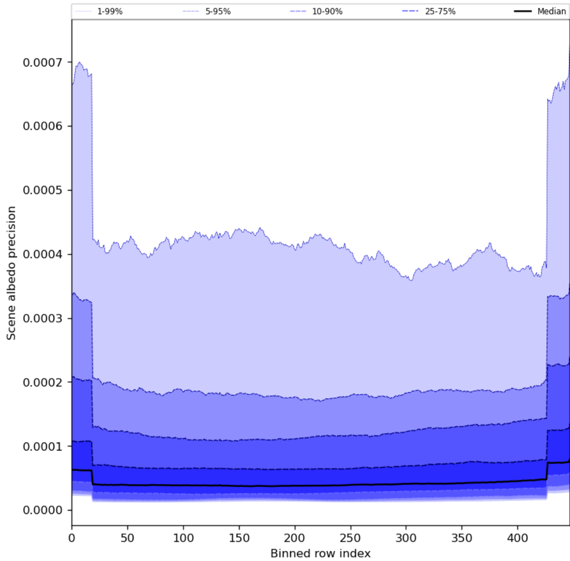
Figure 52: Along track statistics of “Scene albedo precision” for 2024-08-12 to 2024-08-13
