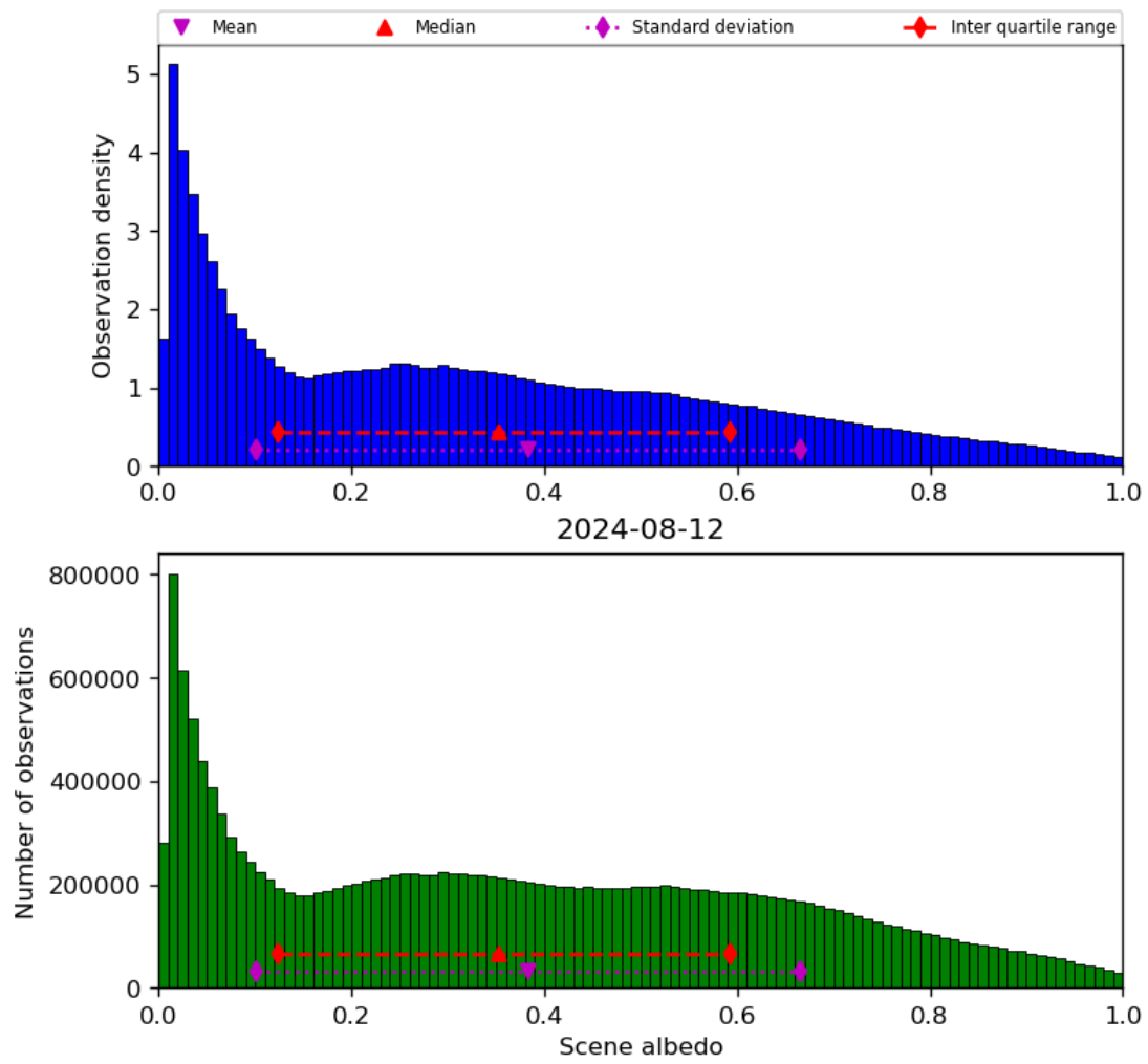
Figure 34: Histogram of “Scene albedo” for 2024-08-12 to 2024-08-13
