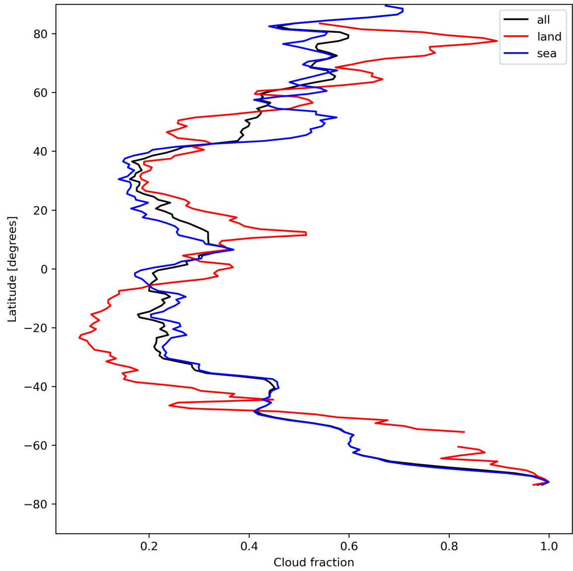
Figure 15: Zonal average of “Cloud fraction” for 2024-08-12 to 2024-08-13.
