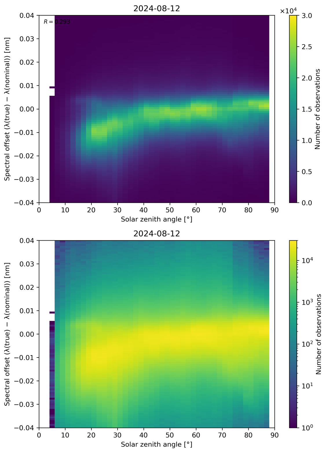
Figure 117: Scatter density plot of “Solar zenith angle” against “Spectral offset ( \lambda(\text{true}) - \lambda(\text{nominal}) )” for 2024-08-12 to 2024-08-13.
