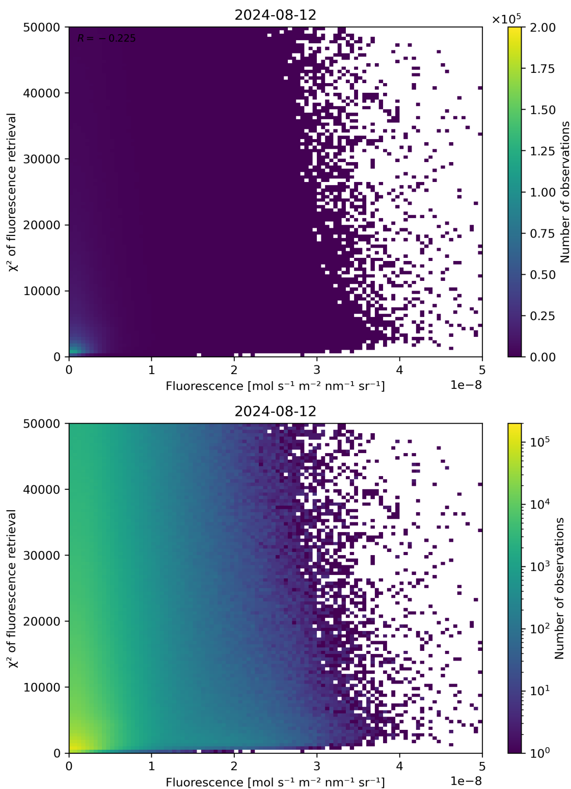
Figure 85: Scatter density plot of “Fluorescence” against “ \chi^2 of fluorescence retrieval” for 2024-08-12 to 2024-08-13.
