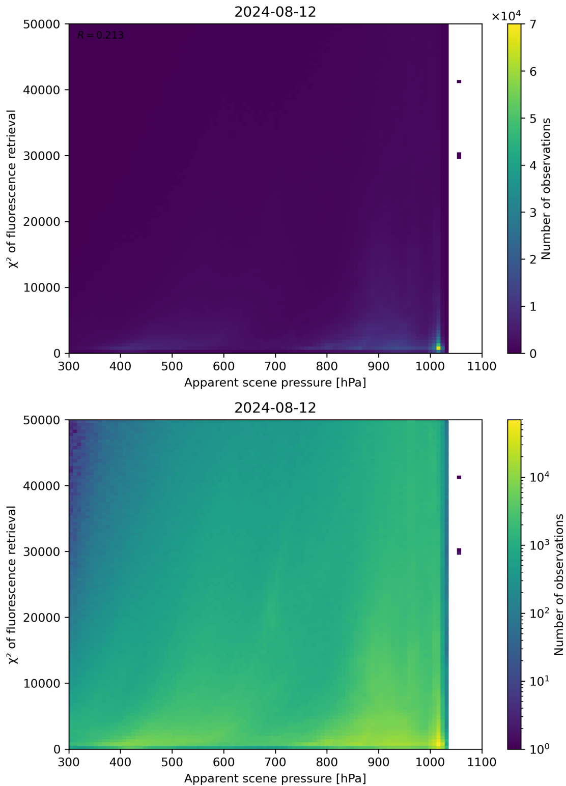
Figure 63: Scatter density plot of “Apparent scene pressure” against “ \chi^2 of fluorescence retrieval” for 2024-08-12 to 2024-08-13.
