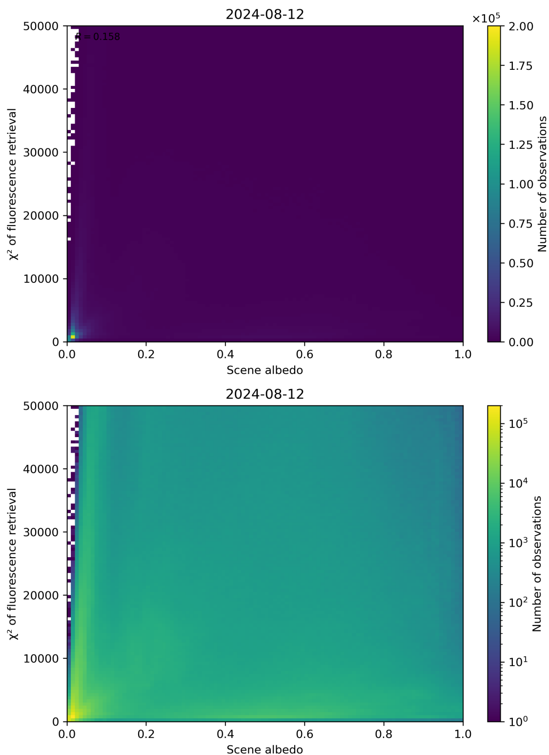
Figure 103: Scatter density plot of “Scene albedo” against “ \chi^2 of fluorescence retrieval” for 2024-08-12 to 2024-08-13.
