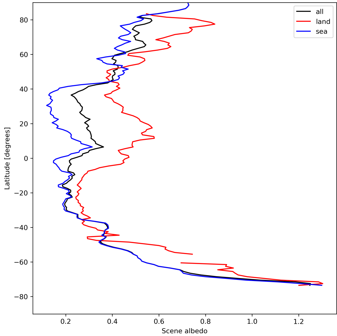
Figure 17: Zonal average of “Scene albedo” for 2024-08-12 to 2024-08-13.
