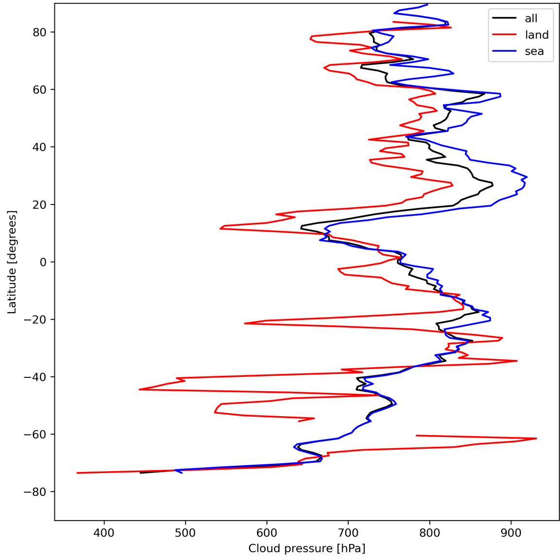
Figure 13: Zonal average of “Cloud pressure” for 2024-08-12 to 2024-08-13.
