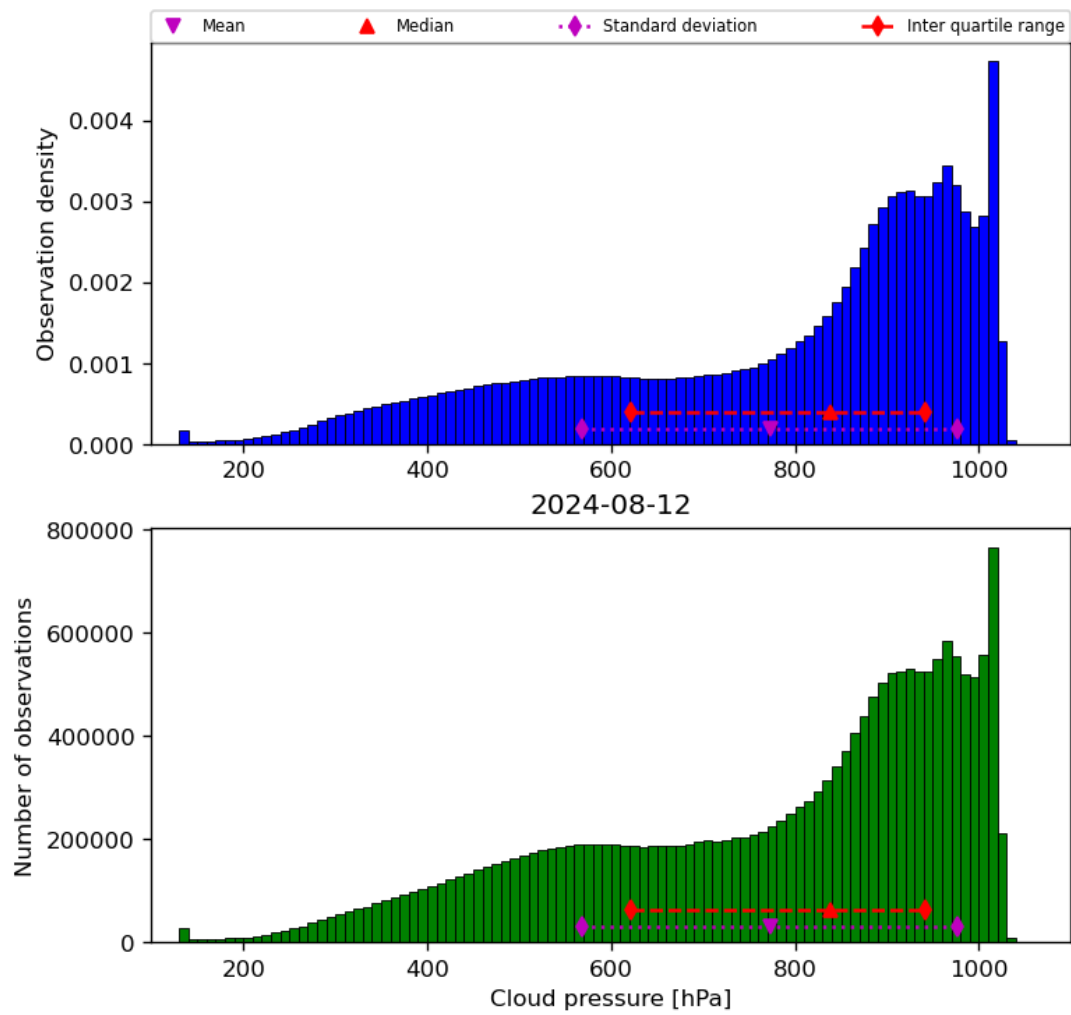
Figure 30: Histogram of “Cloud pressure” for 2024-08-12 to 2024-08-13
