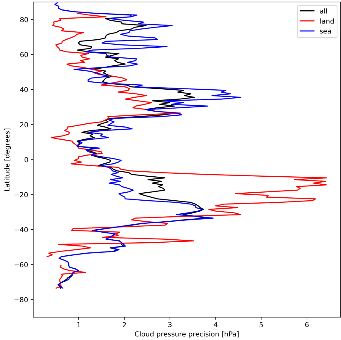
Figure 14: Zonal average of “Cloud pressure precision” for 2024-08-12 to 2024-08-13.
