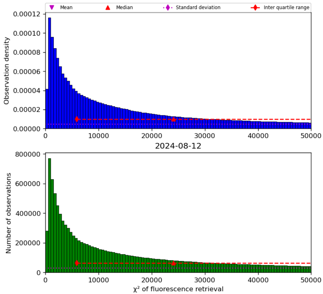
Figure 42: Histogram of “ \chi^2 of fluorescence retrieval” for 2024-08-12 to 2024-08-13
