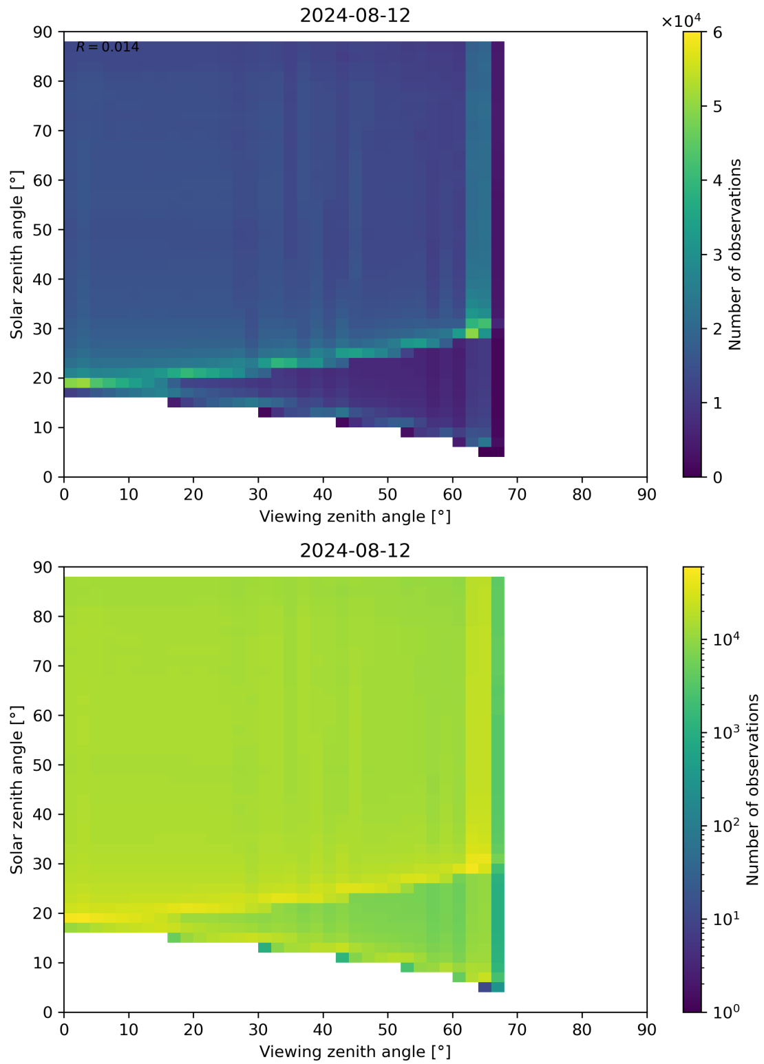
Figure 127: Scatter density plot of “Viewing zenith angle” against “Solar zenith angle” for 2024-08-12 to 2024-08-13.
