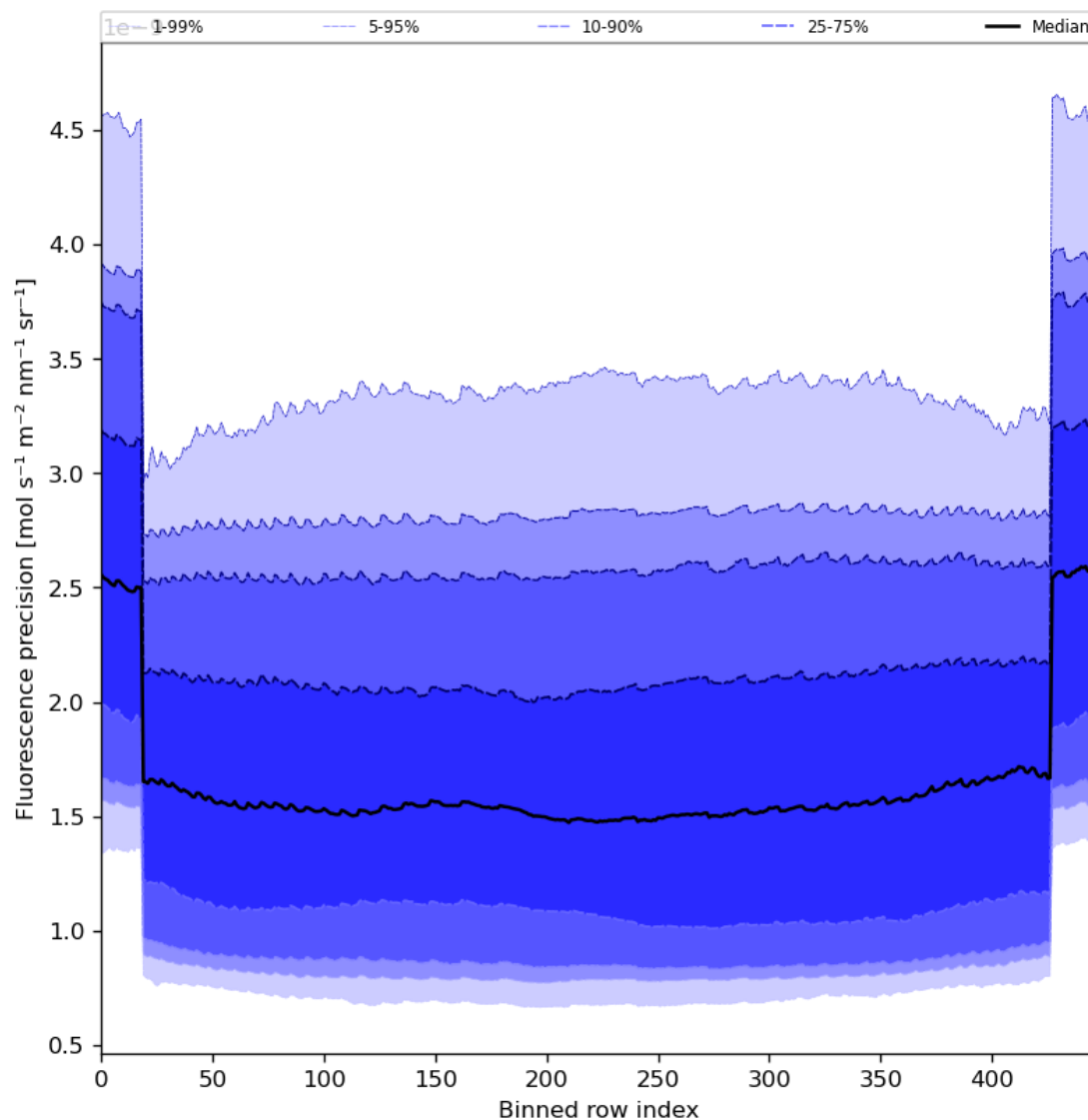
Figure 58: Along track statistics of “Fluorescence precision” for 2024-08-12 to 2024-08-13
