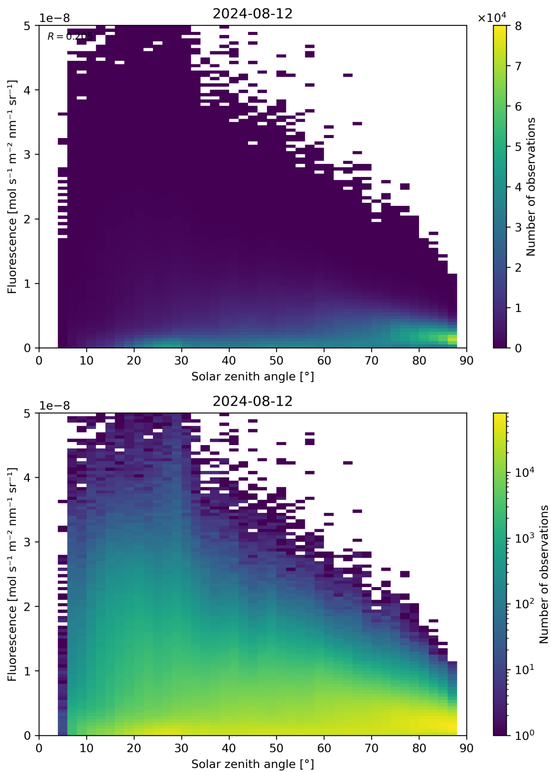
Figure 112: Scatter density plot of “Solar zenith angle” against “Fluorescence” for 2024-08-12 to 2024-08-13.
