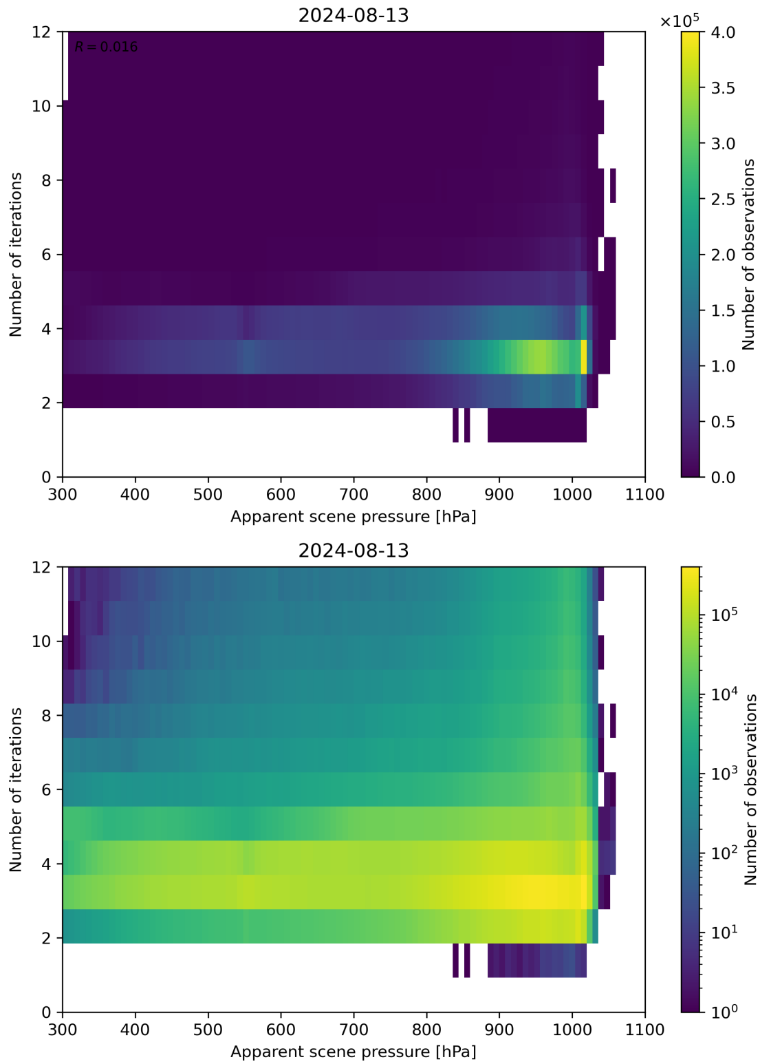
Figure 65: Scatter density plot of “Apparent scene pressure” against “Number of iterations” for 2024-08-12 to 2024-08-14.
