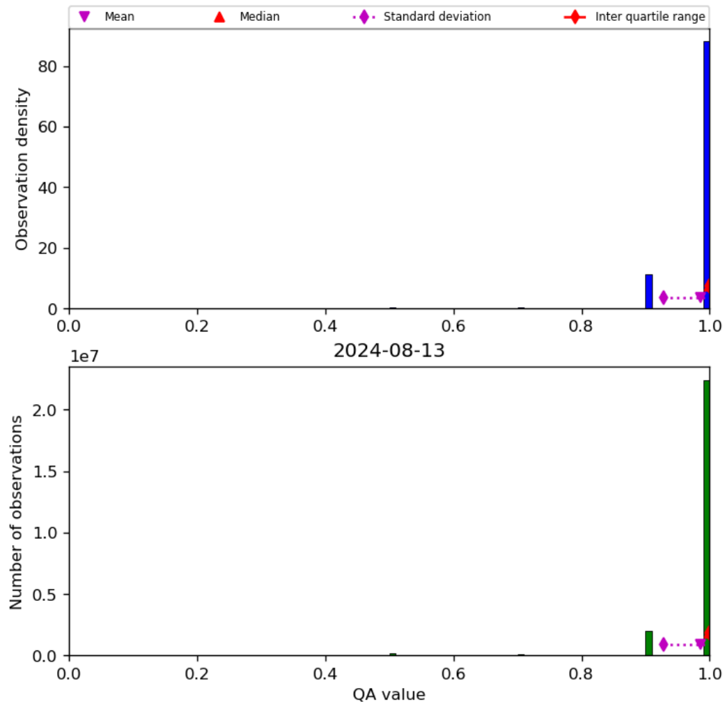
Figure 29: Histogram of “QA value” for 2024-08-12 to 2024-08-14
