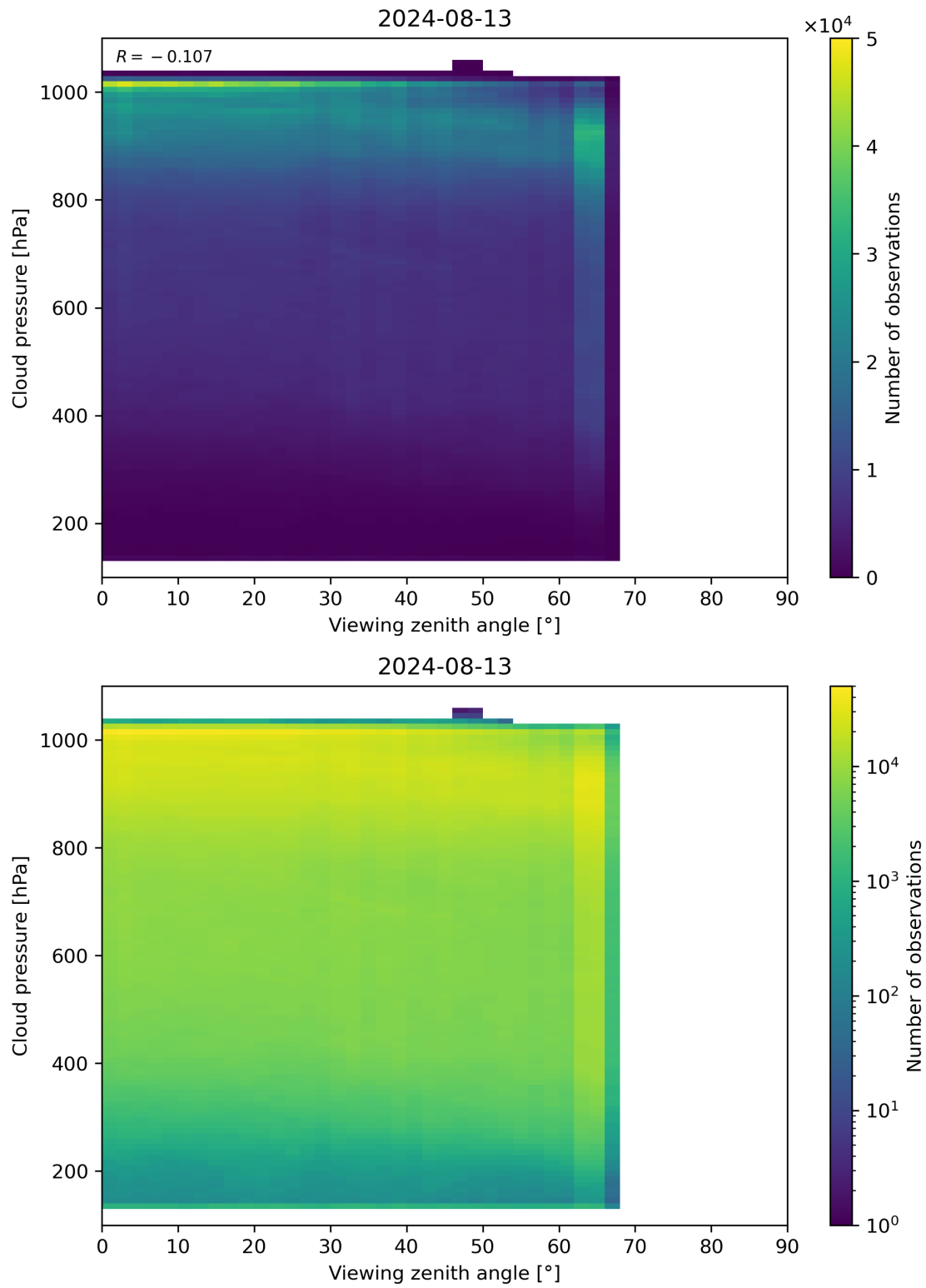
Figure 121: Scatter density plot of “Viewing zenith angle” against “Cloud pressure” for 2024-08-12 to 2024-08-14.
