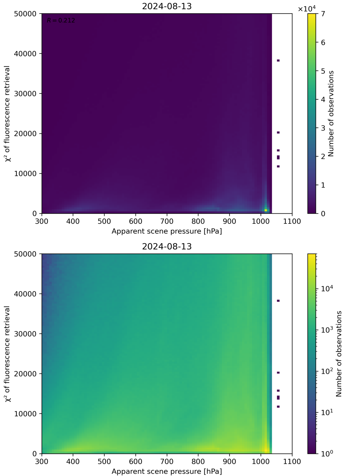
Figure 63: Scatter density plot of “Apparent scene pressure” against “ \chi^2 of fluorescence retrieval” for 2024-08-12 to 2024-08-14.
