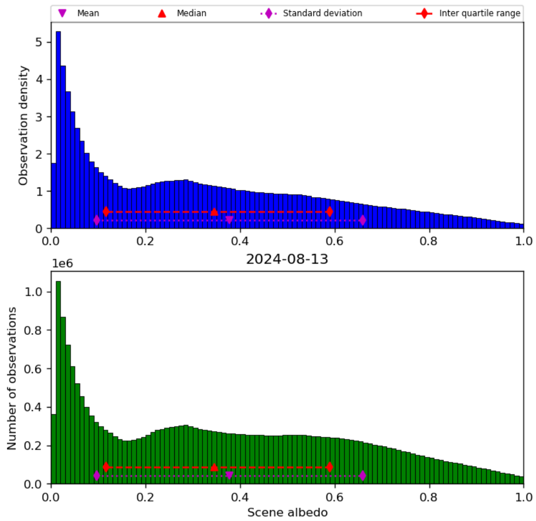
Figure 34: Histogram of “Scene albedo” for 2024-08-12 to 2024-08-14
