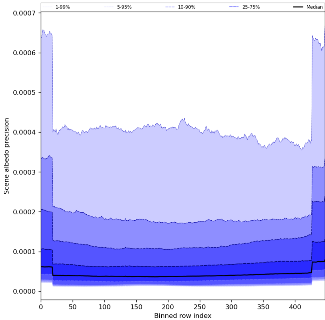
Figure 52: Along track statistics of “Scene albedo precision” for 2024-08-12 to 2024-08-14
