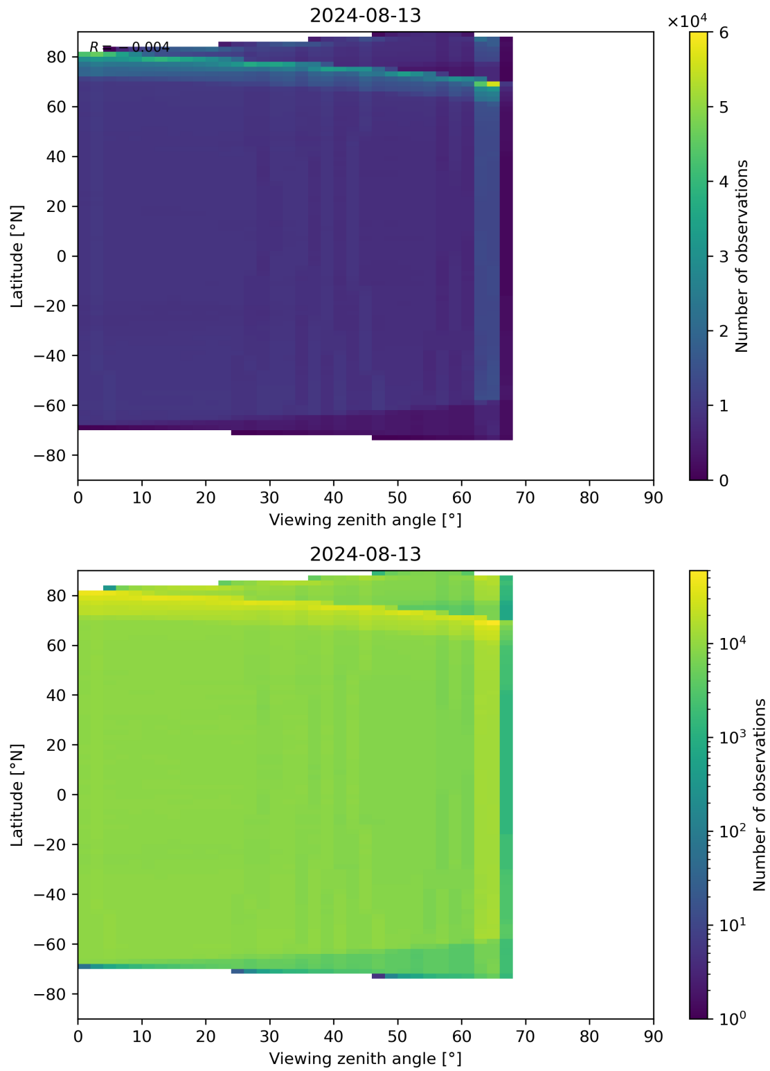
Figure 123: Scatter density plot of “Viewing zenith angle” against “Latitude” for 2024-08-12 to 2024-08-14.
