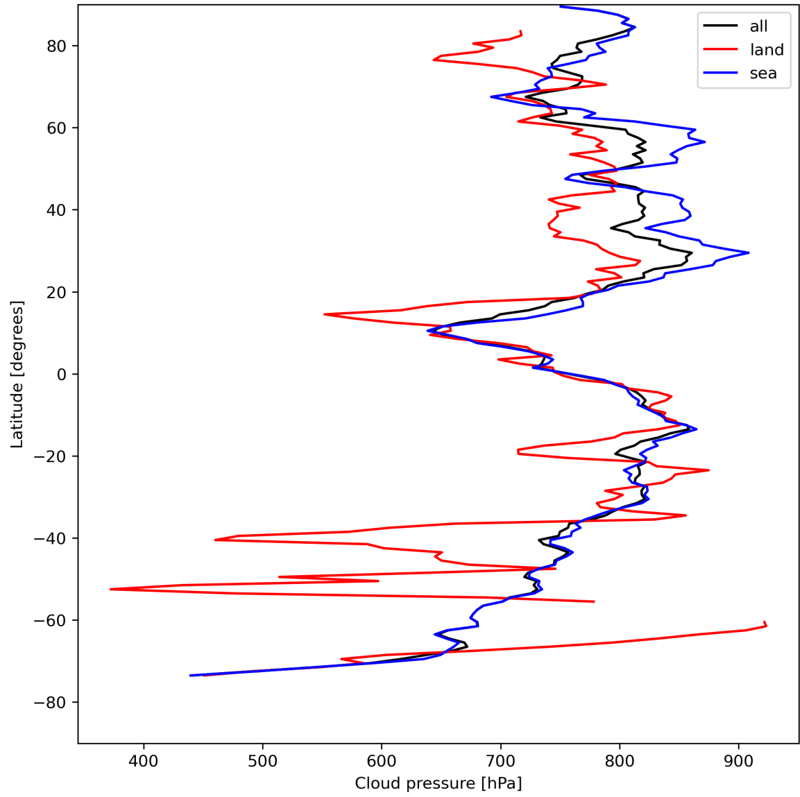
Figure 13: Zonal average of “Cloud pressure” for 2024-08-12 to 2024-08-14.
