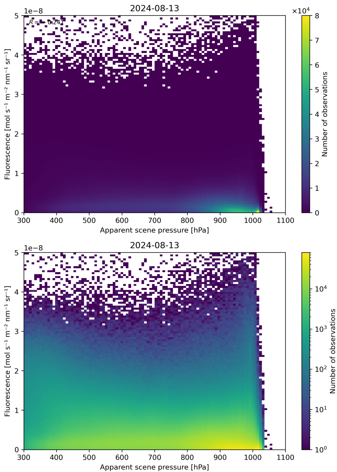
Figure 64: Scatter density plot of “Apparent scene pressure” against “Fluorescence” for 2024-08-12 to 2024-08-14.
