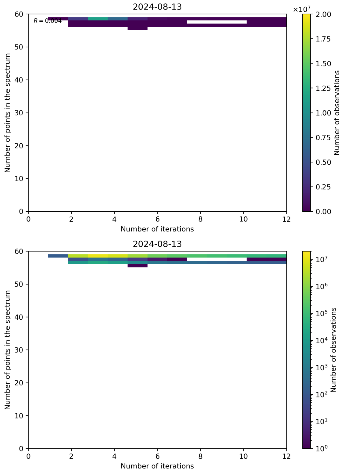
Figure 99: Scatter density plot of “Number of iterations” against “Number of points in the spectrum” for 2024-08-12 to 2024-08-14.
