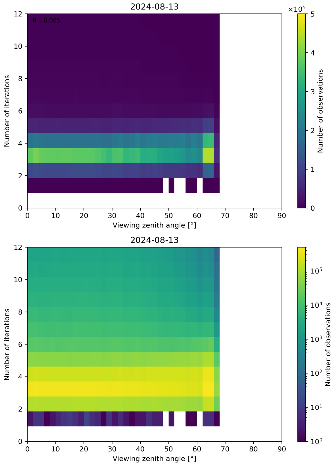
Figure 124: Scatter density plot of “Viewing zenith angle” against “Number of iterations” for 2024-08-12 to 2024-08-14.
