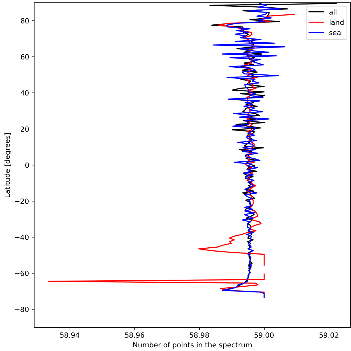
Figure 27: Zonal average of “Number of points in the spectrum” for 2024-08-12 to 2024-08-14.
