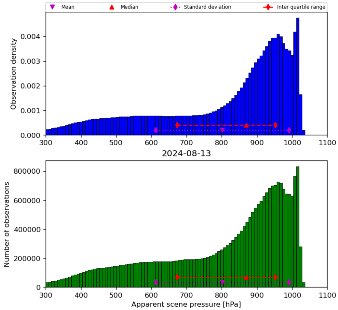
Figure 36: Histogram of "Apparent scene pressure" for 2024-08-12 to 2024-08-14
