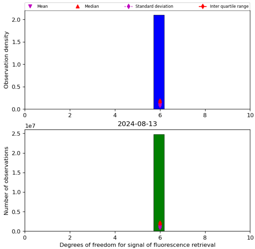
Figure 43: Histogram of “Degrees of freedom for signal of fluorescence retrieval” for 2024-08-12 to 2024-08-14
