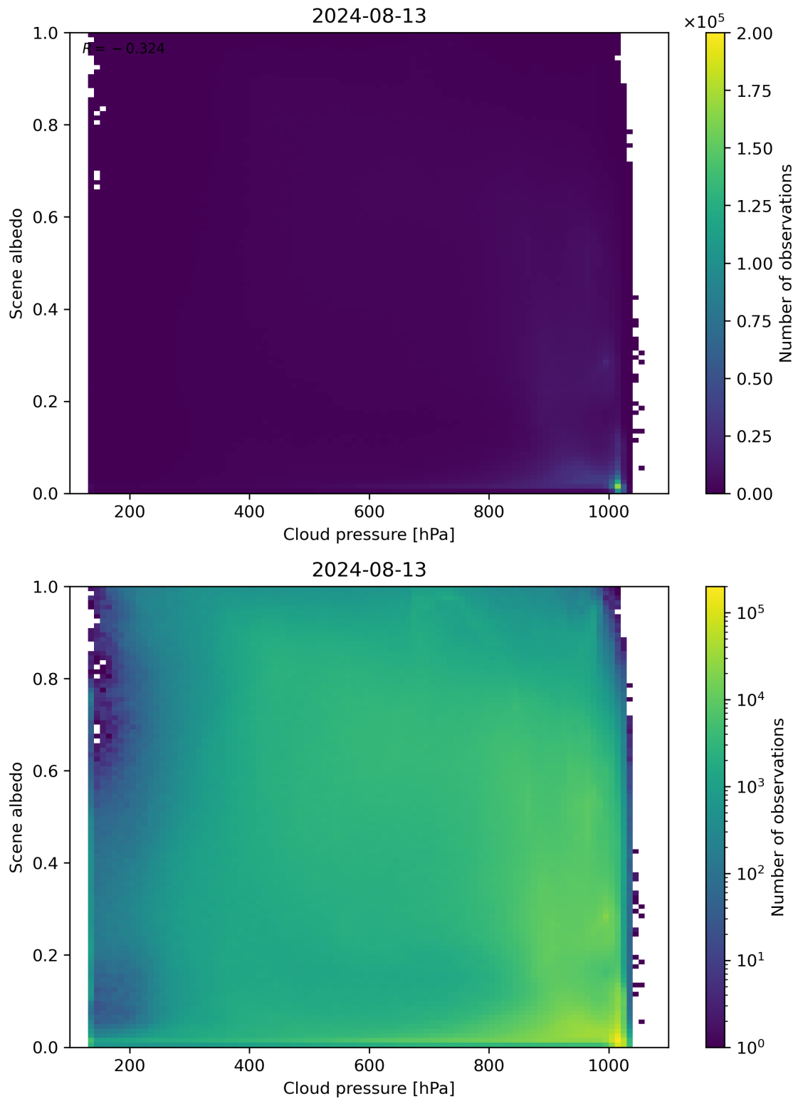
Figure 83: Scatter density plot of “Cloud pressure” against “Scene albedo” for 2024-08-12 to 2024-08-14.
