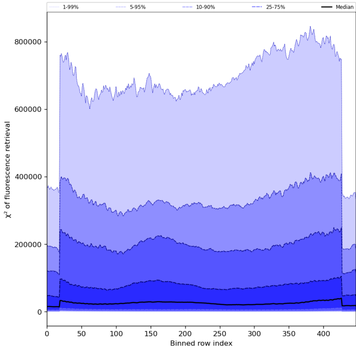
Figure 59: Along track statistics of “ \chi^2 of fluorescence retrieval” for 2024-08-12 to 2024-08-14
