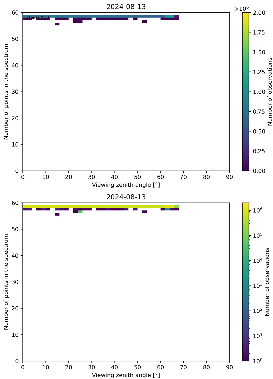
Figure 125: Scatter density plot of “Viewing zenith angle” against “Number of points in the spectrum” for 2024-08-12 to 2024-08-14.
