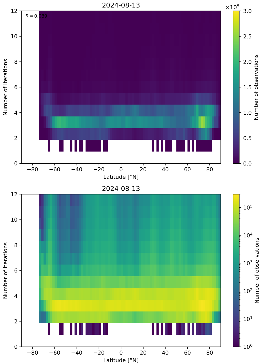
Figure 93: Scatter density plot of “Latitude” against “Number of iterations” for 2024-08-12 to 2024-08-14.
