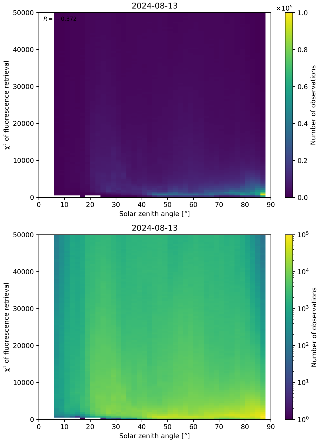
Figure 109: Scatter density plot of “Solar zenith angle” against “ \chi^2 of fluorescence retrieval” for 2024-08-12 to 2024-08-14.
