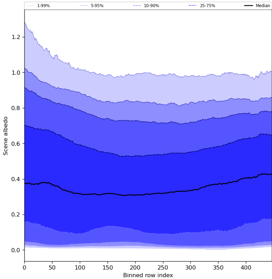
Figure 51: Along track statistics of “Scene albedo” for 2024-08-12 to 2024-08-14
