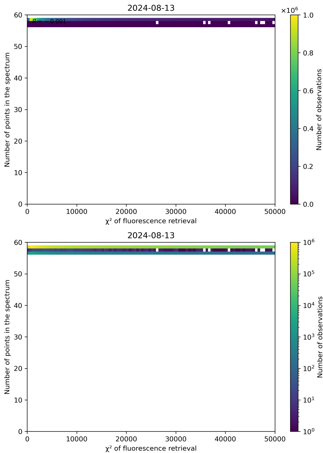
Figure 68: Scatter density plot of " \chi^2 of fluorescence retrieval" against "Number of points in the spectrum" for 2024-08-12 to 2024-08-14.
