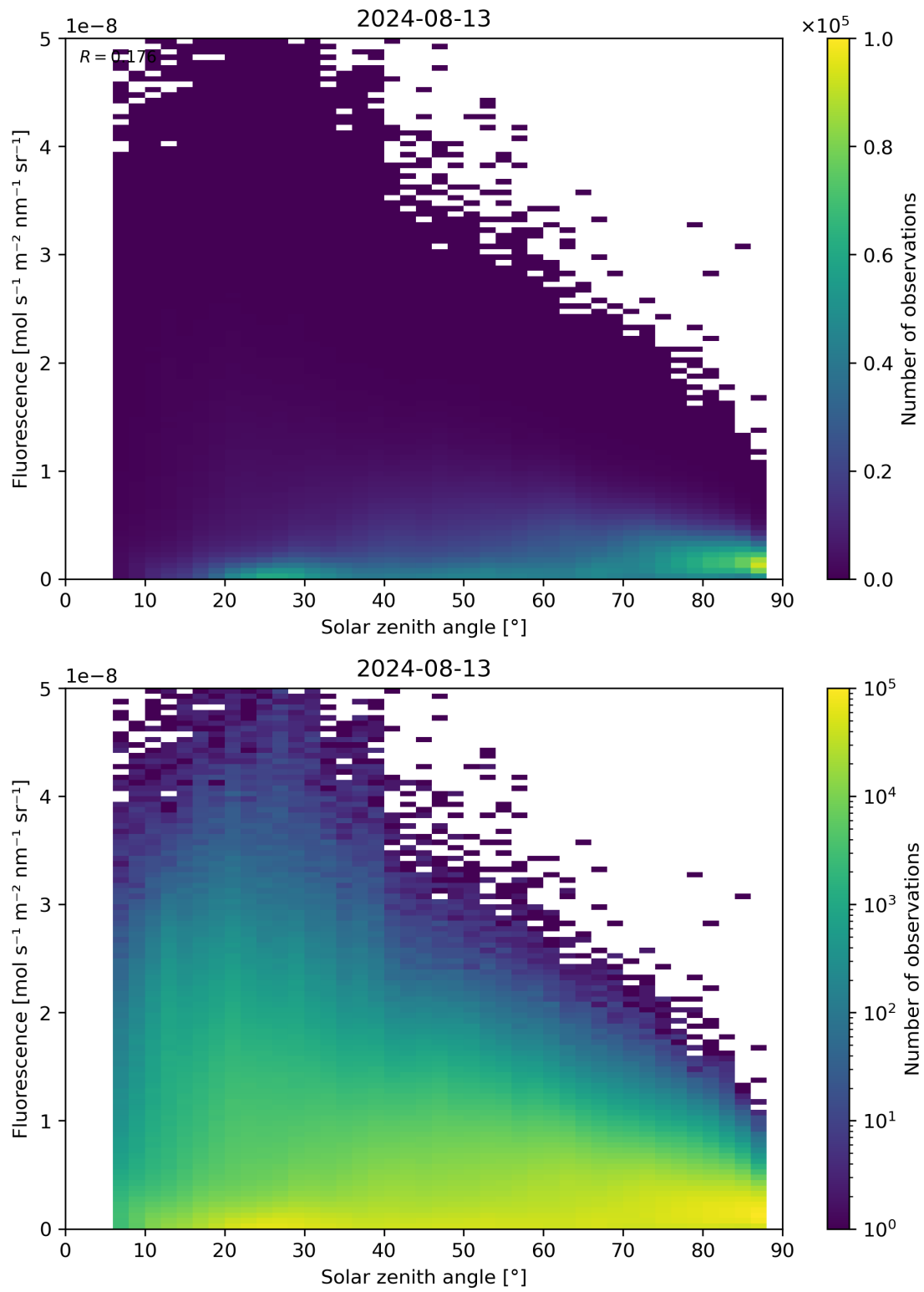
Figure 112: Scatter density plot of “Solar zenith angle” against “Fluorescence” for 2024-08-12 to 2024-08-14.
