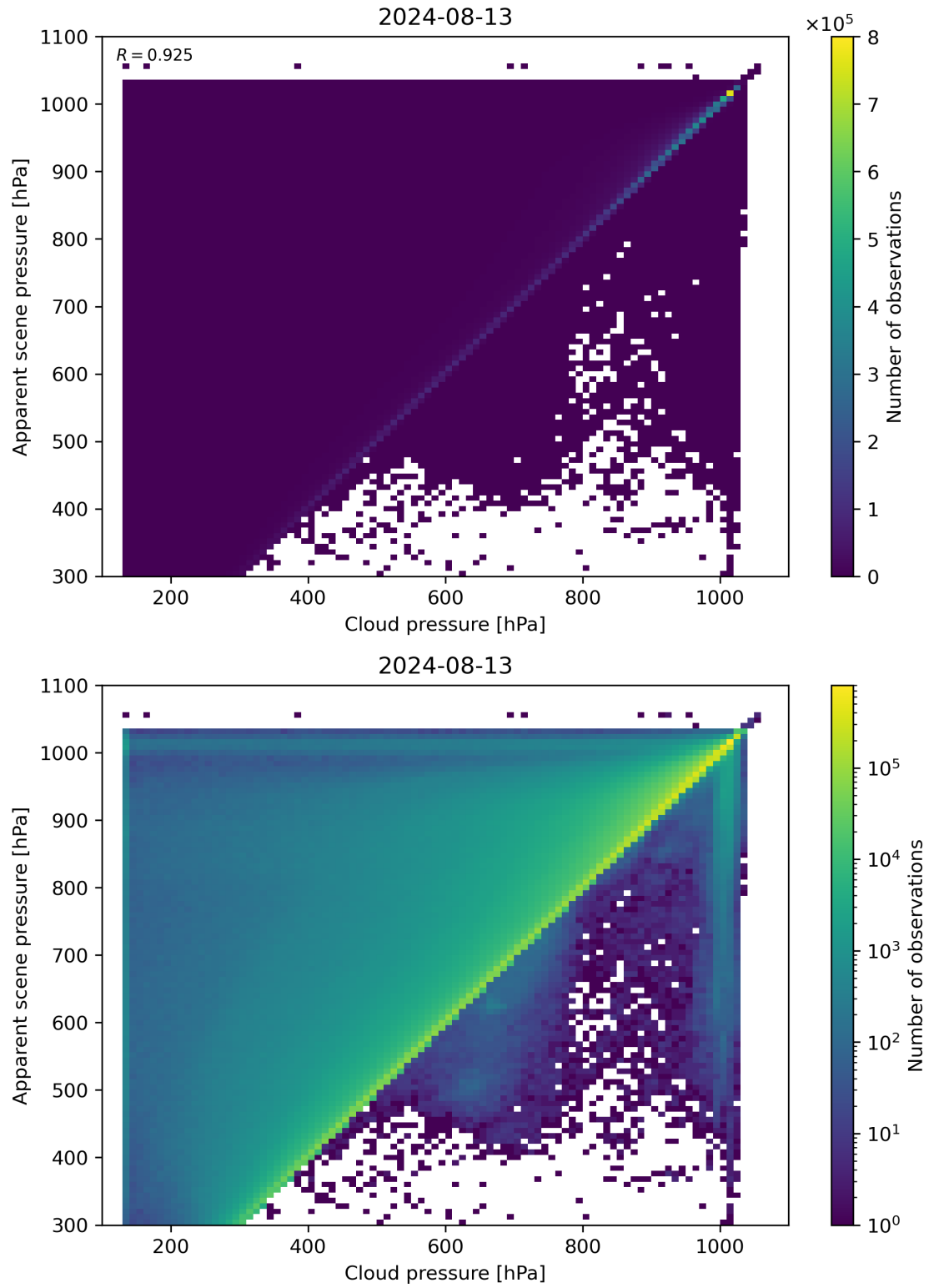
Figure 77: Scatter density plot of “Cloud pressure” against “Apparent scene pressure” for 2024-08-12 to 2024-08-14.
