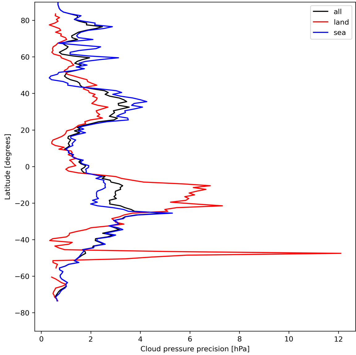
Figure 14: Zonal average of “Cloud pressure precision” for 2024-08-12 to 2024-08-14.
