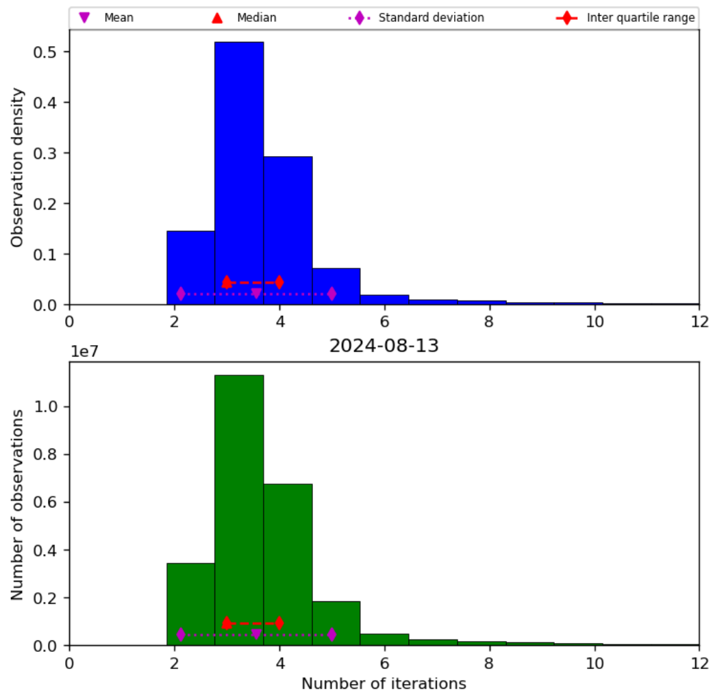
Figure 39: Histogram of “Number of iterations” for 2024-08-12 to 2024-08-14
