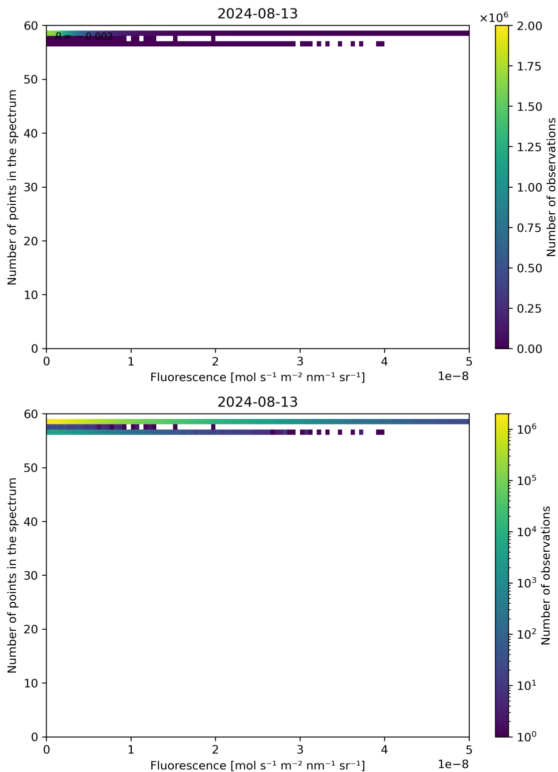
Figure 86: Scatter density plot of “Fluorescence” against “Number of points in the spectrum” for 2024-08-12 to 2024-08-14.
