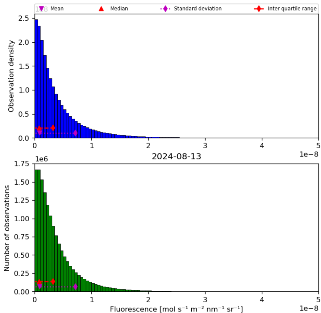
Figure 40: Histogram of “Fluorescence” for 2024-08-12 to 2024-08-14
