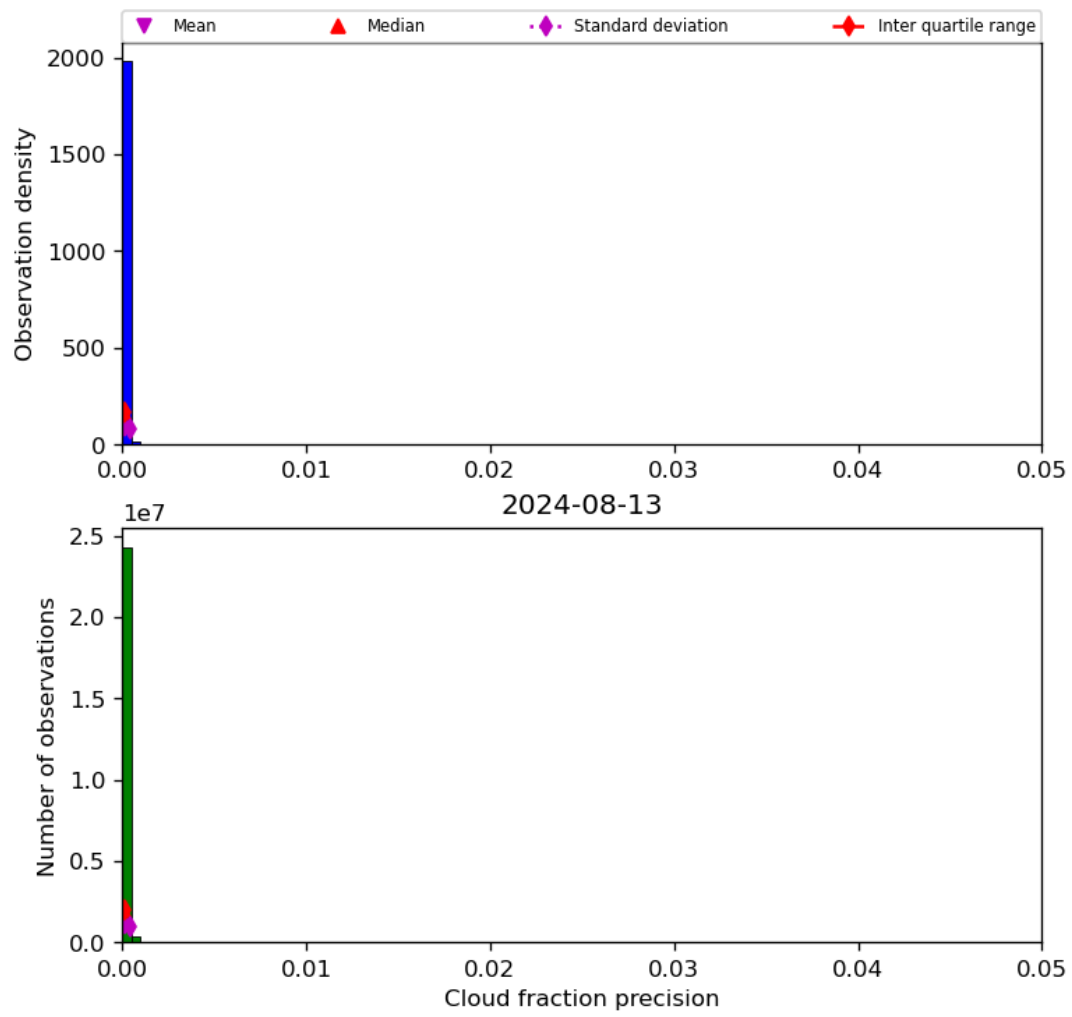
Figure 33: Histogram of “Cloud fraction precision” for 2024-08-12 to 2024-08-14
