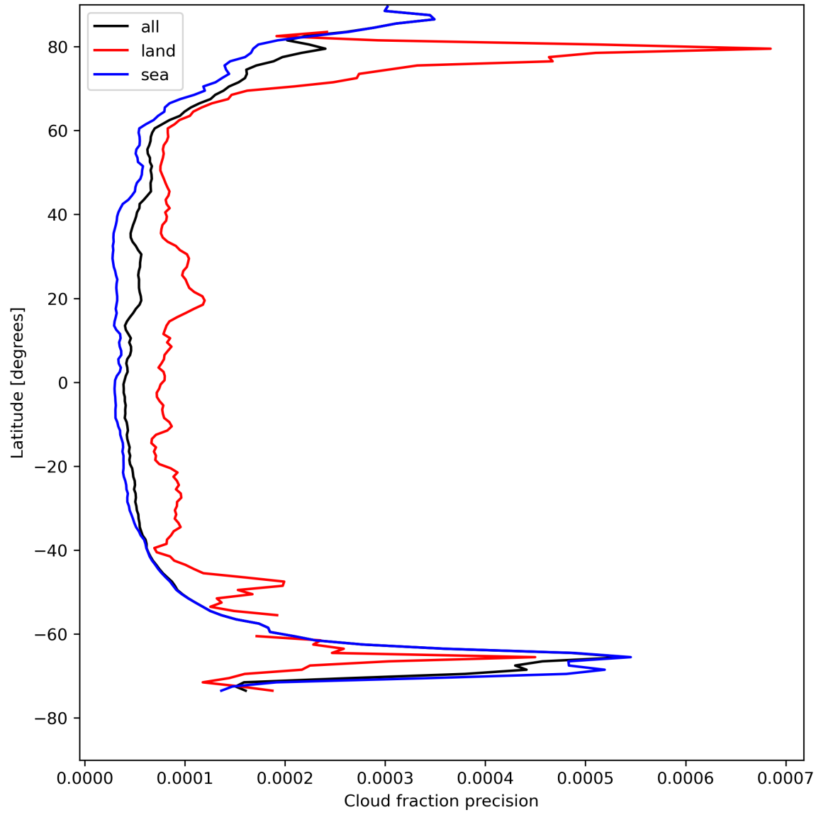
Figure 16: Zonal average of “Cloud fraction precision” for 2024-08-12 to 2024-08-14.
