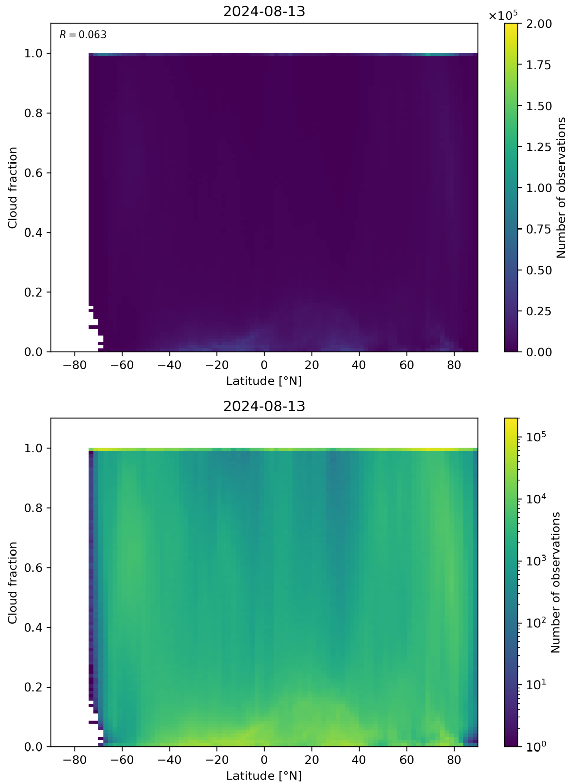
Figure 90: Scatter density plot of “Latitude” against “Cloud fraction” for 2024-08-12 to 2024-08-14.
