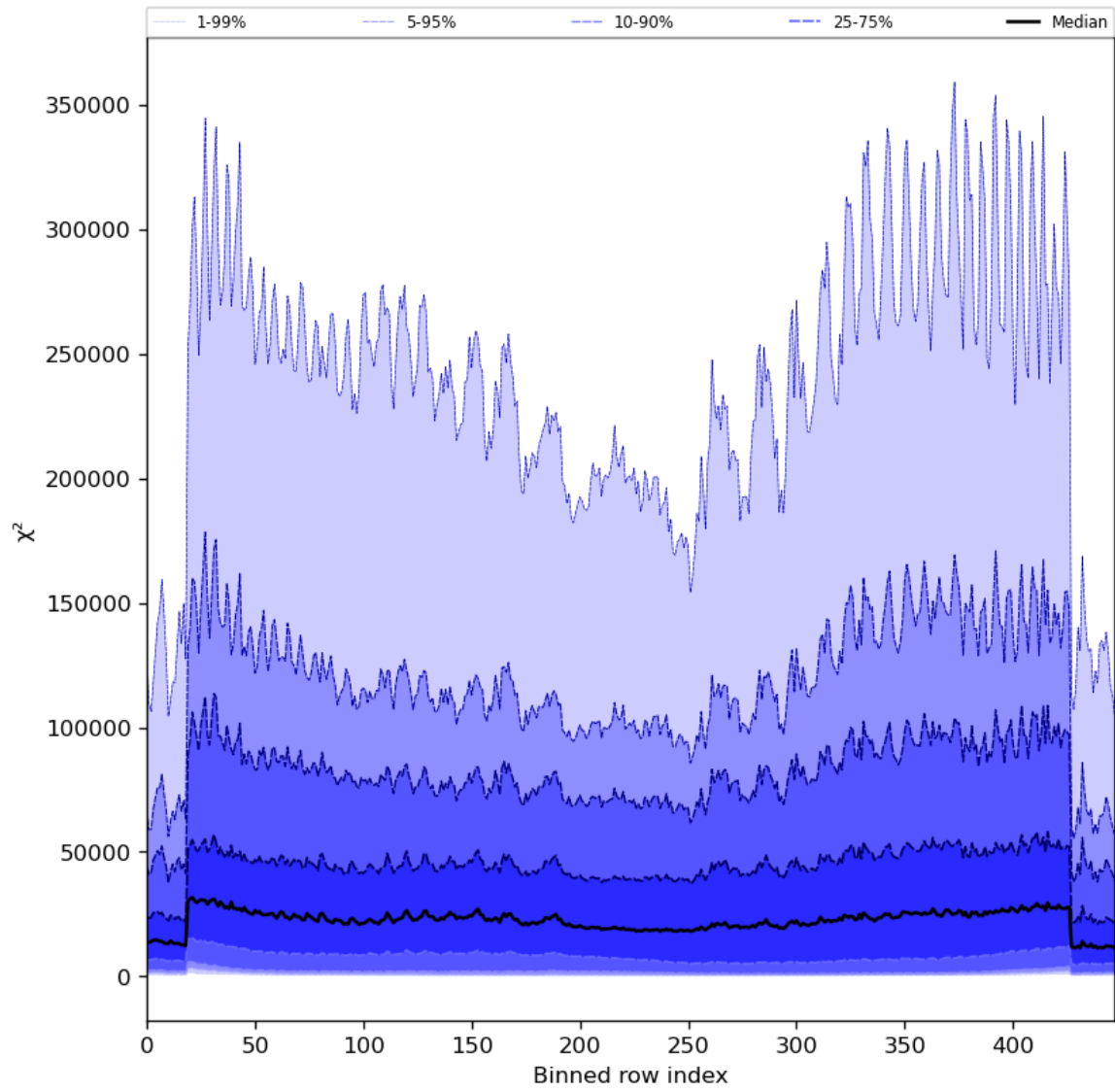
Figure 55: Along track statistics of “ \chi^2 ” for 2024-08-12 to 2024-08-14
