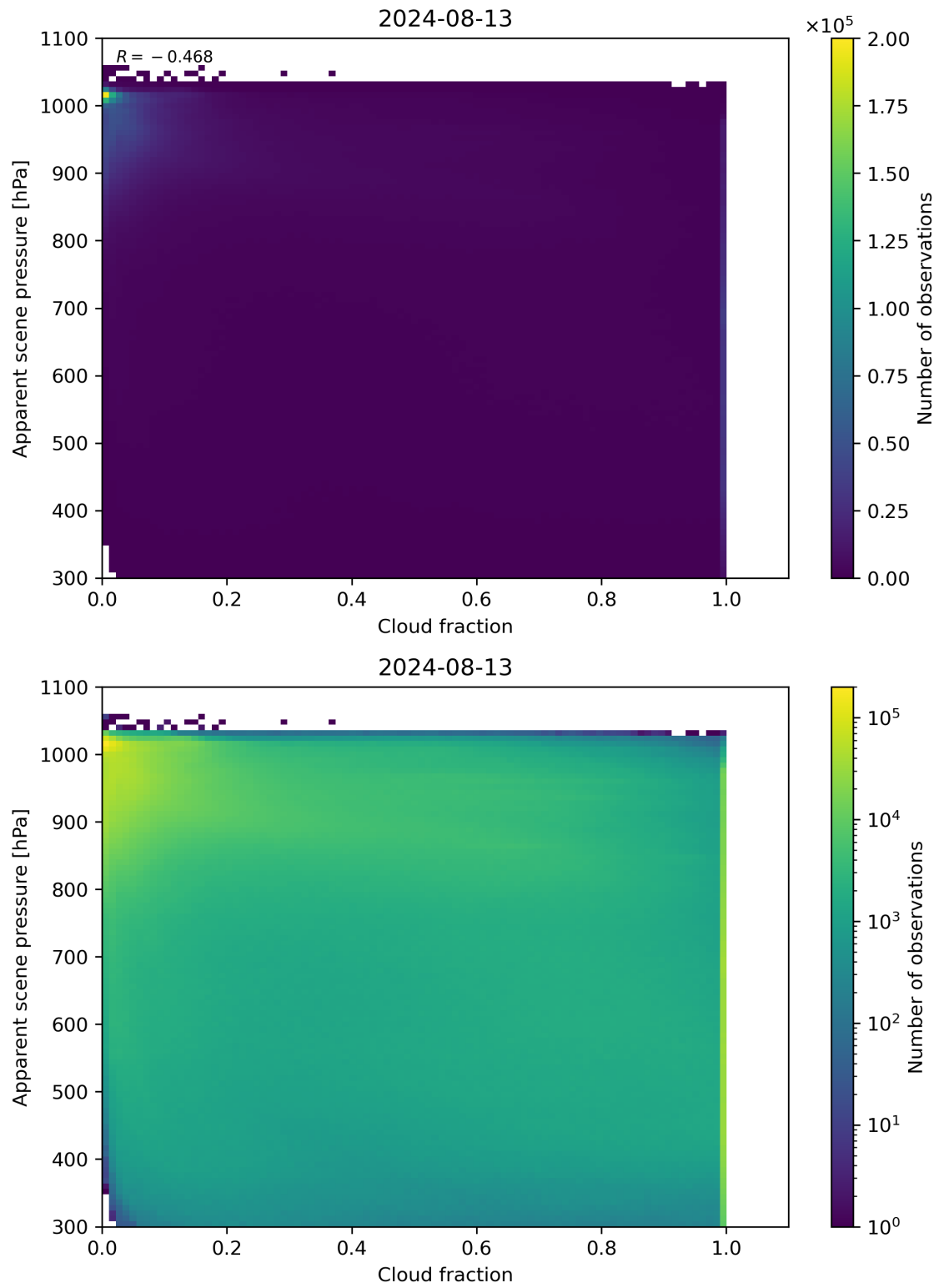
Figure 70: Scatter density plot of “Cloud fraction” against “Apparent scene pressure” for 2024-08-12 to 2024-08-14.
