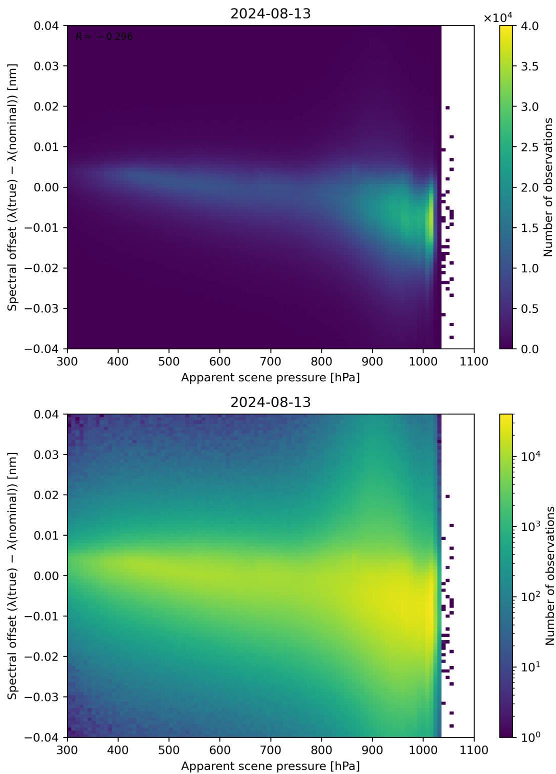
Figure 67: Scatter density plot of “Apparent scene pressure” against “Spectral offset ( \lambda(\text{true}) - \lambda(\text{nominal}) )” for 2024-08-12 to 2024-08-14.
