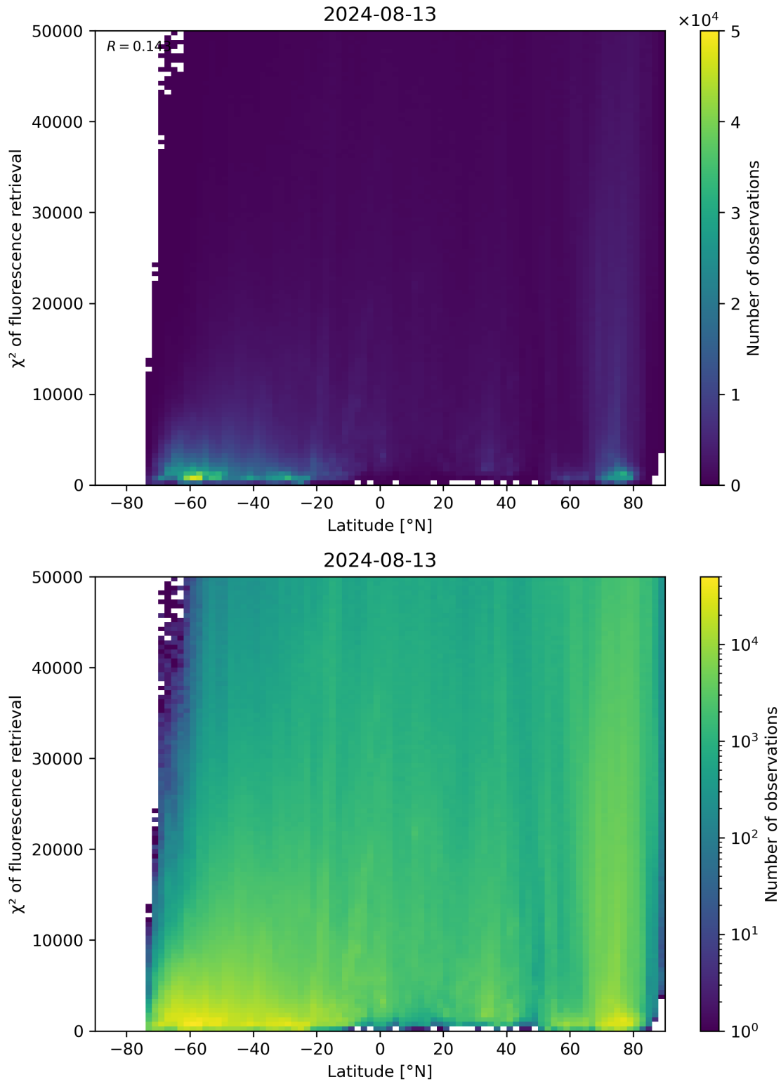
Figure 89: Scatter density plot of “Latitude” against “ \chi^2 of fluorescence retrieval” for 2024-08-12 to 2024-08-14.
