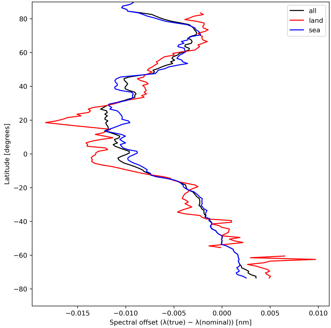
Figure 28: Zonal average of “Spectral offset ( \lambda(\text{true}) - \lambda(\text{nominal}) )” for 2024-08-12 to 2024-08-14.
