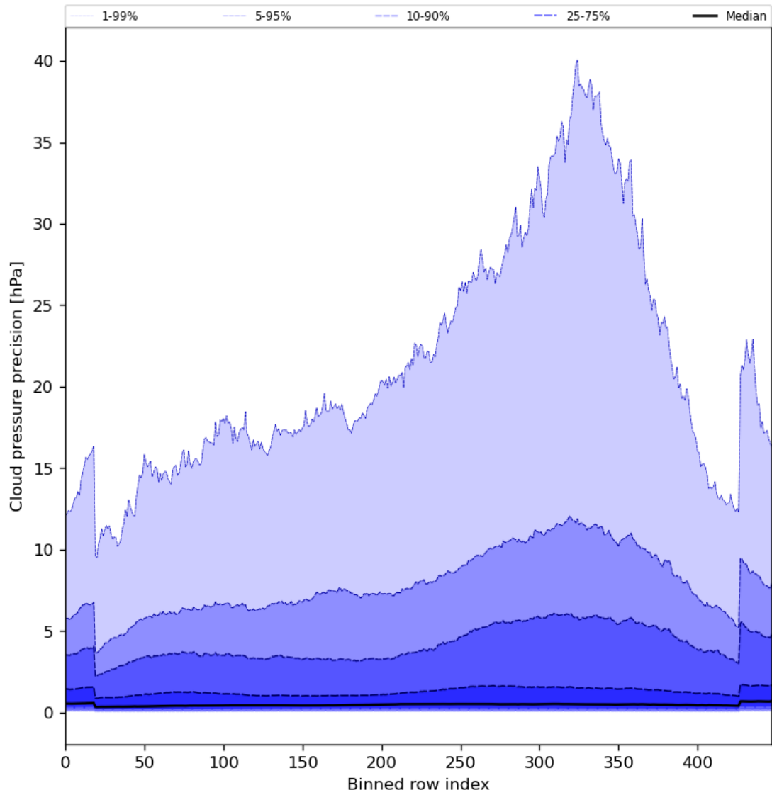
Figure 48: Along track statistics of “Cloud pressure precision” for 2024-08-12 to 2024-08-14
