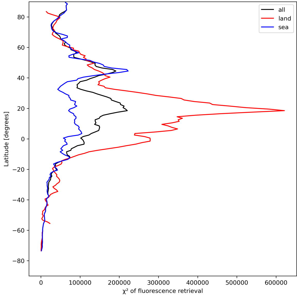
Figure 25: Zonal average of “ \chi^2 of fluorescence retrieval” for 2024-08-12 to 2024-08-14.
