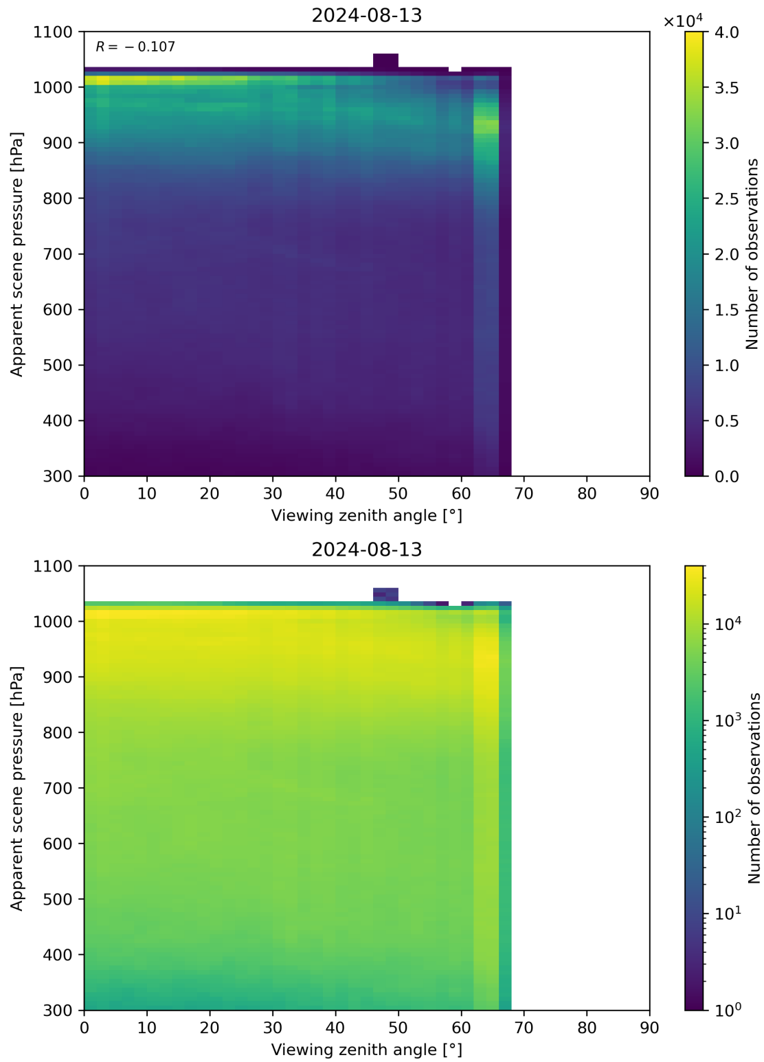
Figure 118: Scatter density plot of “Viewing zenith angle” against “Apparent scene pressure” for 2024-08-12 to 2024-08-14.
