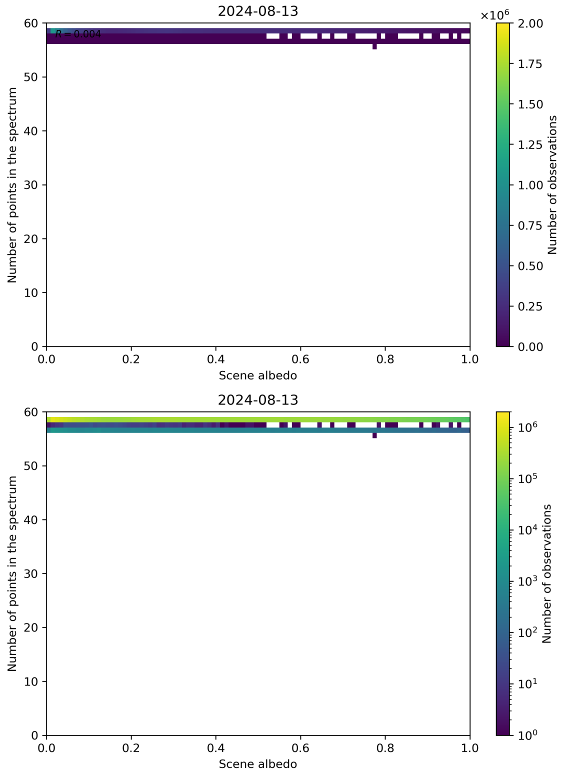
Figure 106: Scatter density plot of “Scene albedo” against “Number of points in the spectrum” for 2024-08-12 to 2024-08-14.
