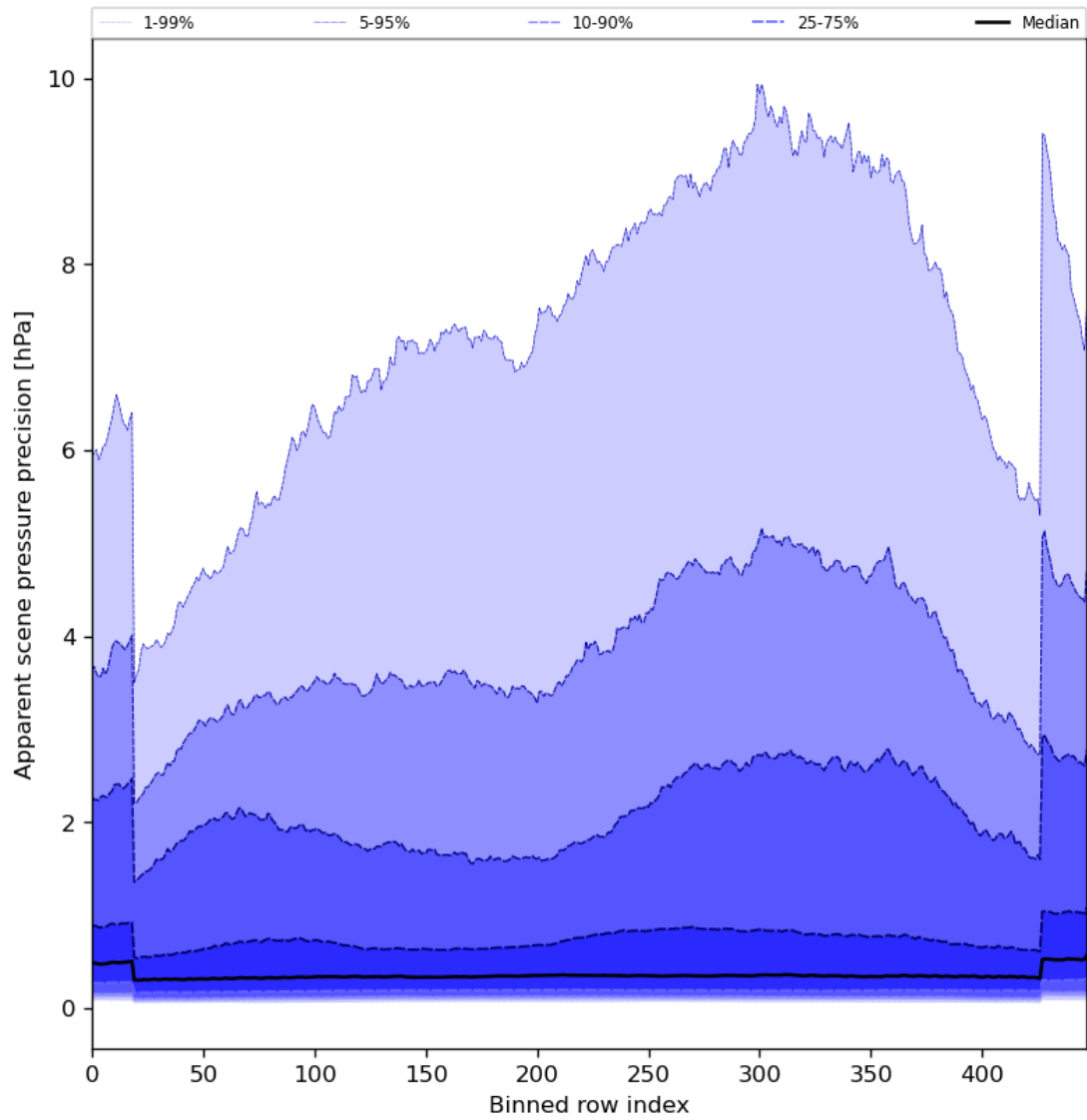
Figure 54: Along track statistics of “Apparent scene pressure precision” for 2024-08-12 to 2024-08-14
