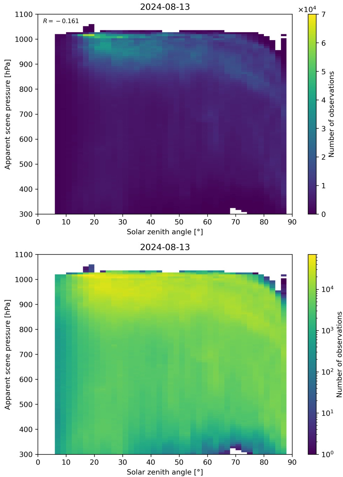
Figure 108: Scatter density plot of “Solar zenith angle” against “Apparent scene pressure” for 2024-08-12 to 2024-08-14.
