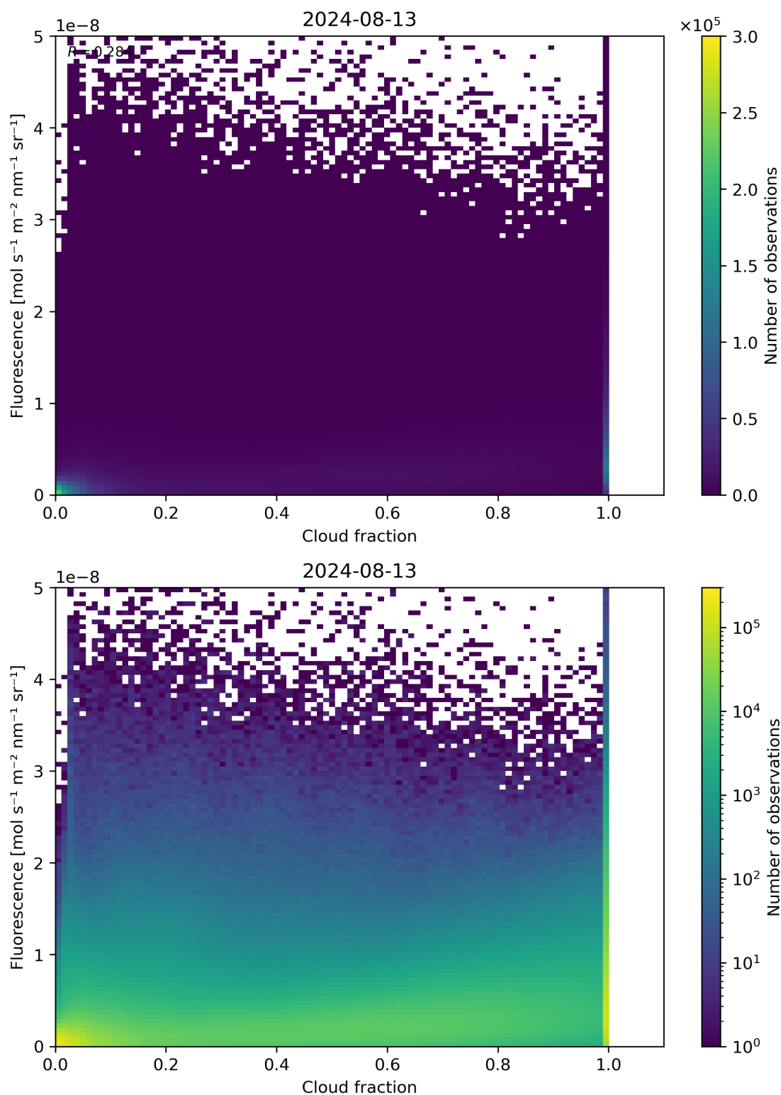
Figure 72: Scatter density plot of “Cloud fraction” against “Fluorescence” for 2024-08-12 to 2024-08-14.
