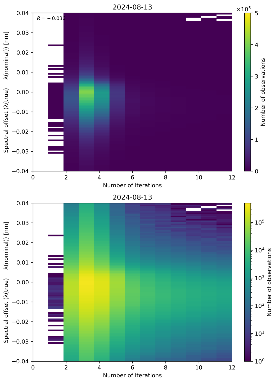
Figure 100: Scatter density plot of “Number of iterations” against “Spectral offset ( \lambda(\text{true}) - \lambda(\text{nominal}) )” for 2024-08-12 to 2024-08-14.
