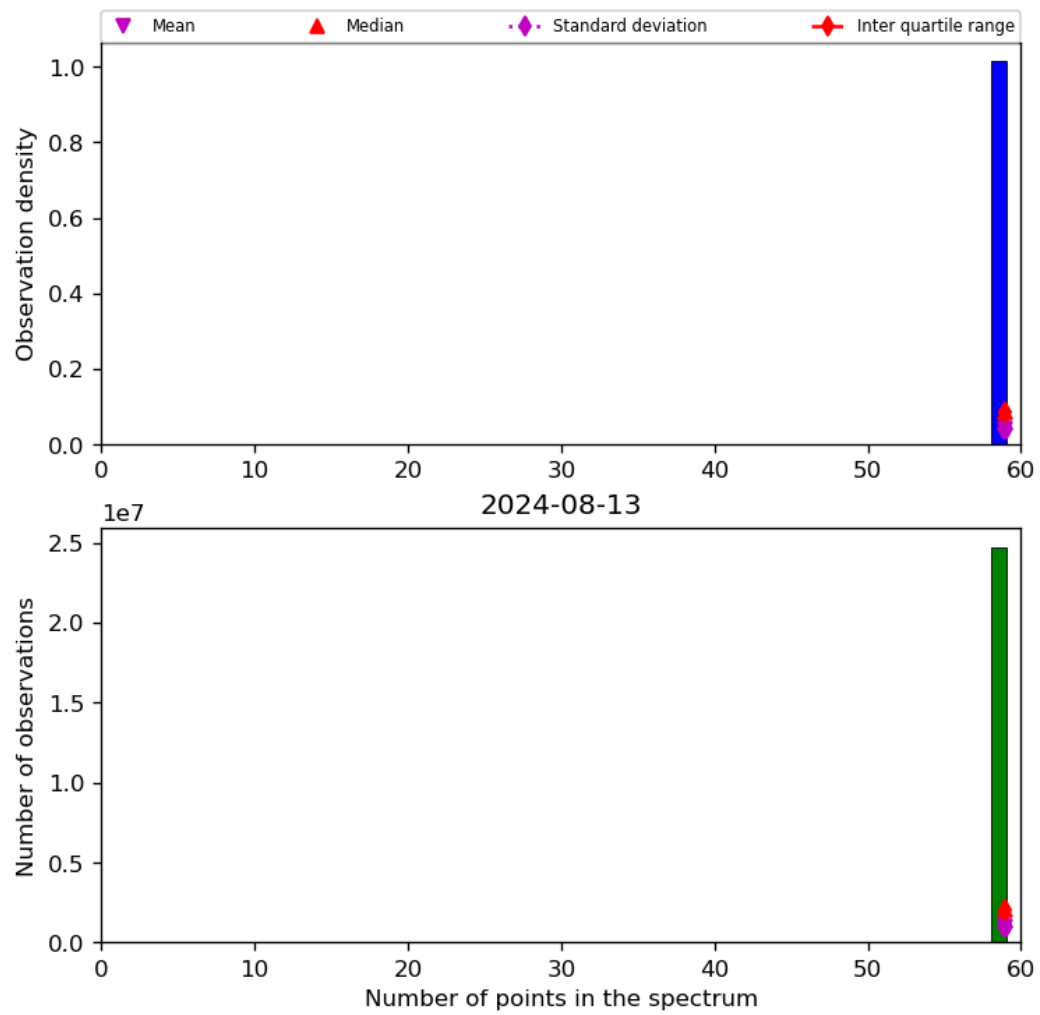
Figure 44: Histogram of “Number of points in the spectrum” for 2024-08-12 to 2024-08-14
