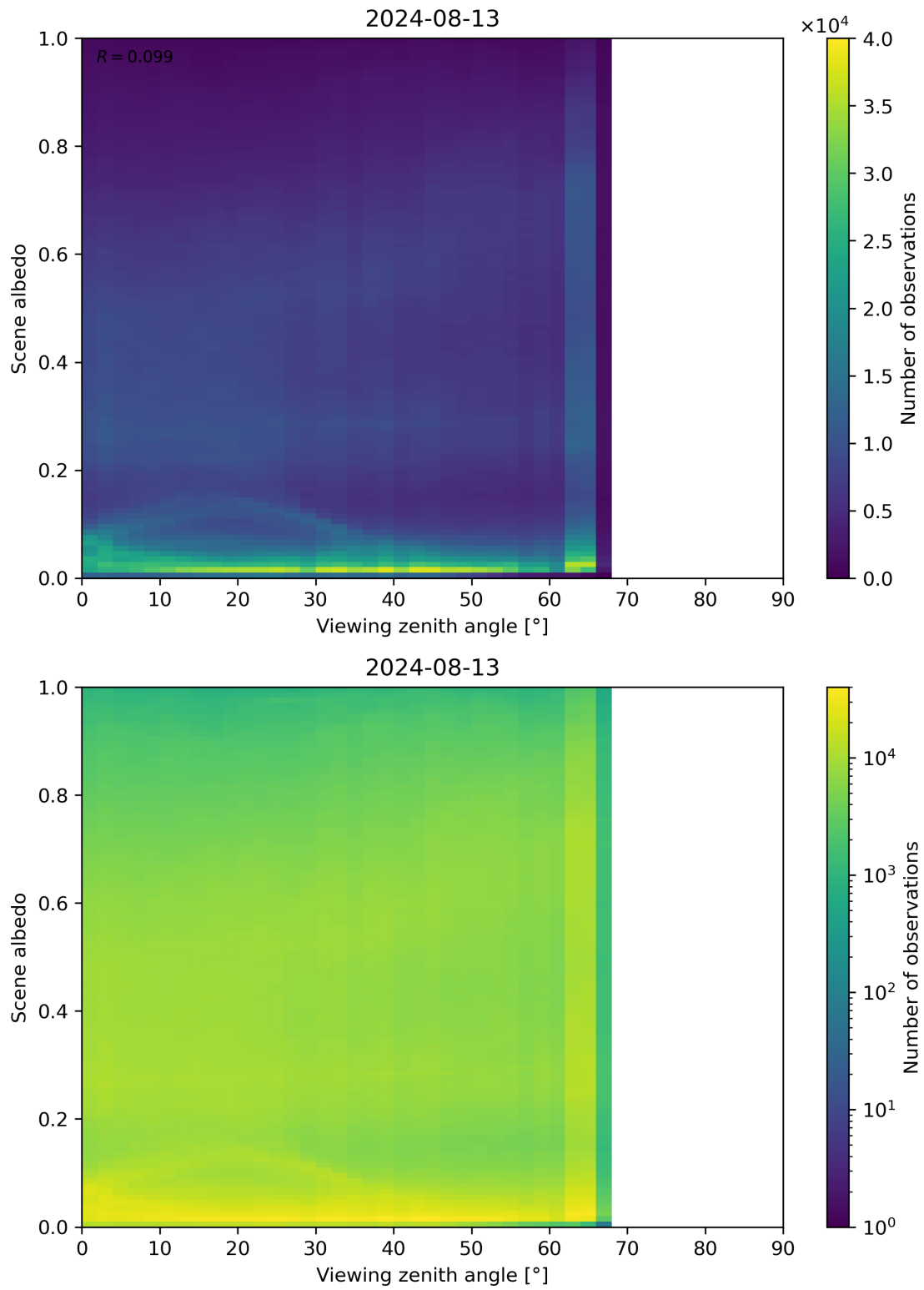
Figure 126: Scatter density plot of “Viewing zenith angle” against “Scene albedo” for 2024-08-12 to 2024-08-14.
