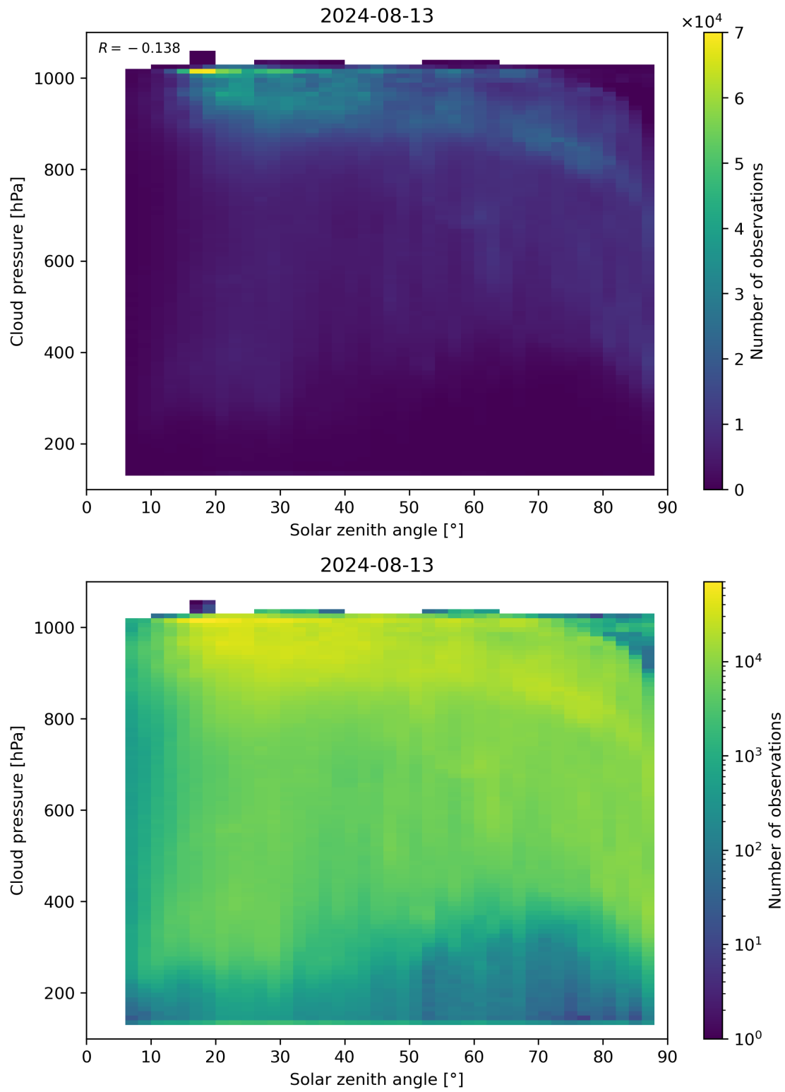
Figure 111: Scatter density plot of “Solar zenith angle” against “Cloud pressure” for 2024-08-12 to 2024-08-14.
