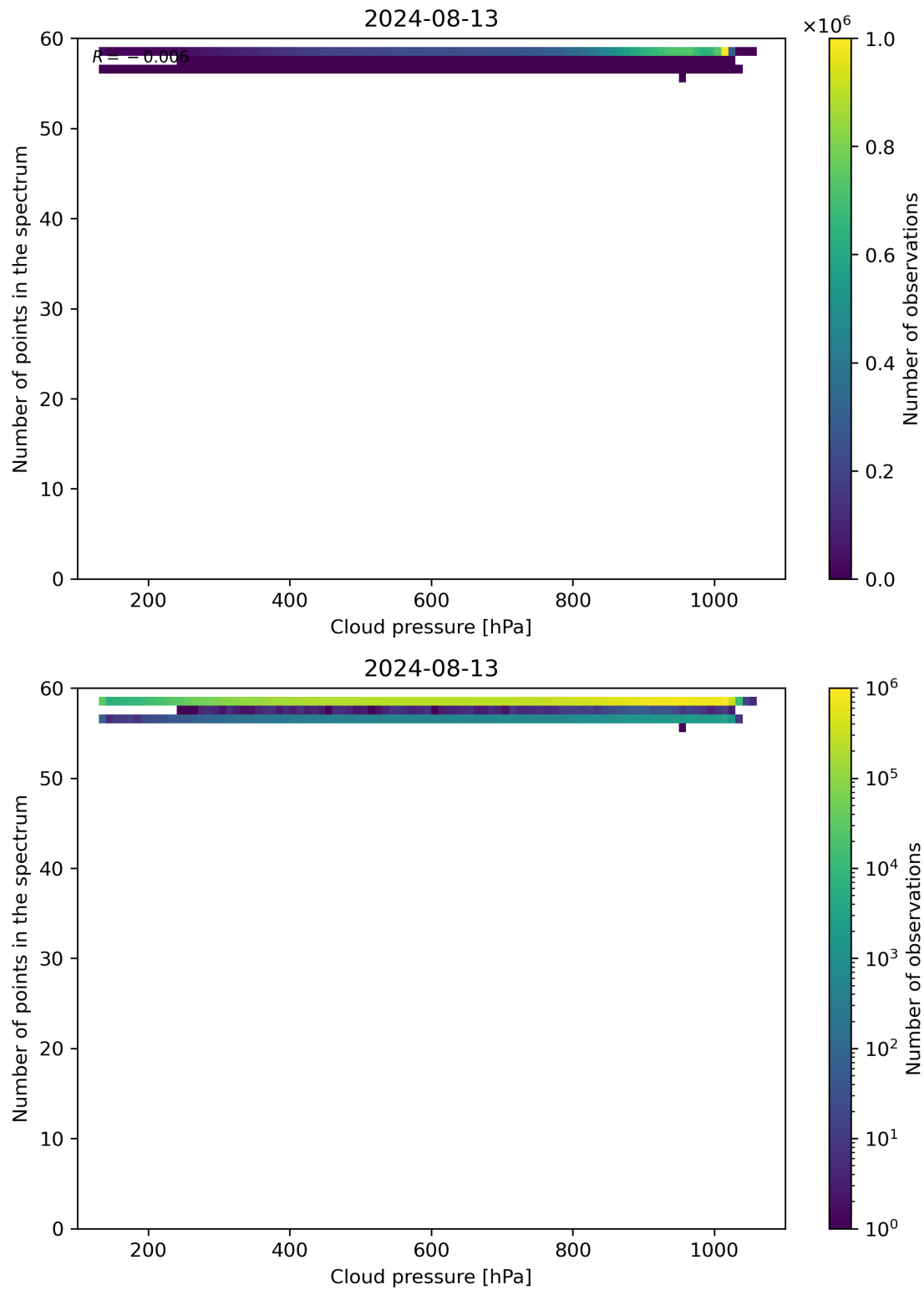
Figure 82: Scatter density plot of “Cloud pressure” against “Number of points in the spectrum” for 2024-08-12 to 2024-08-14.
