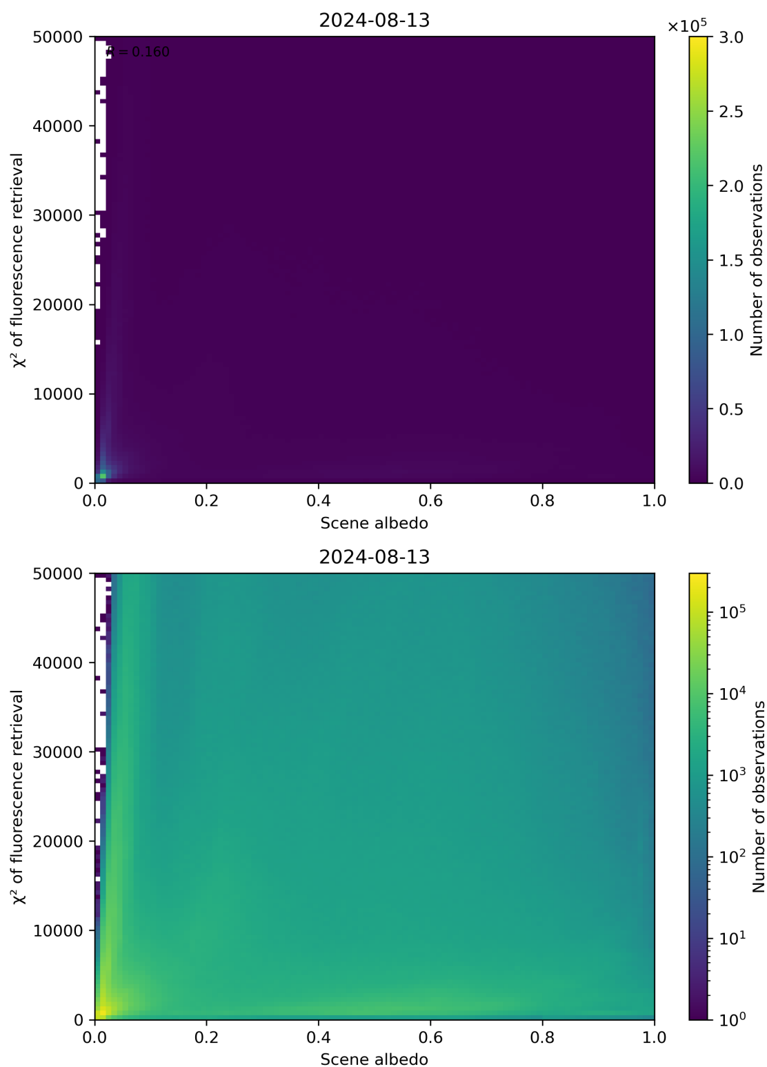
Figure 103: Scatter density plot of “Scene albedo” against “ \chi^2 of fluorescence retrieval” for 2024-08-12 to 2024-08-14.
