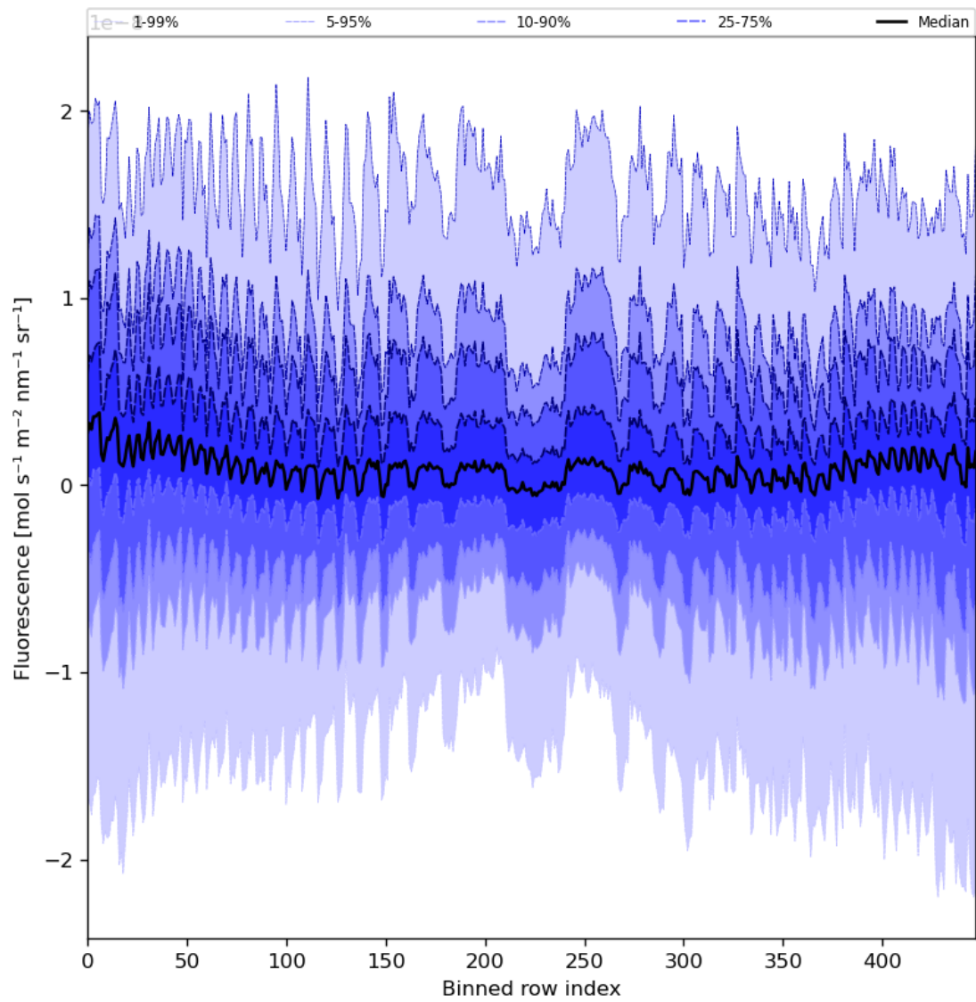
Figure 57: Along track statistics of “Fluorescence” for 2024-08-12 to 2024-08-14
