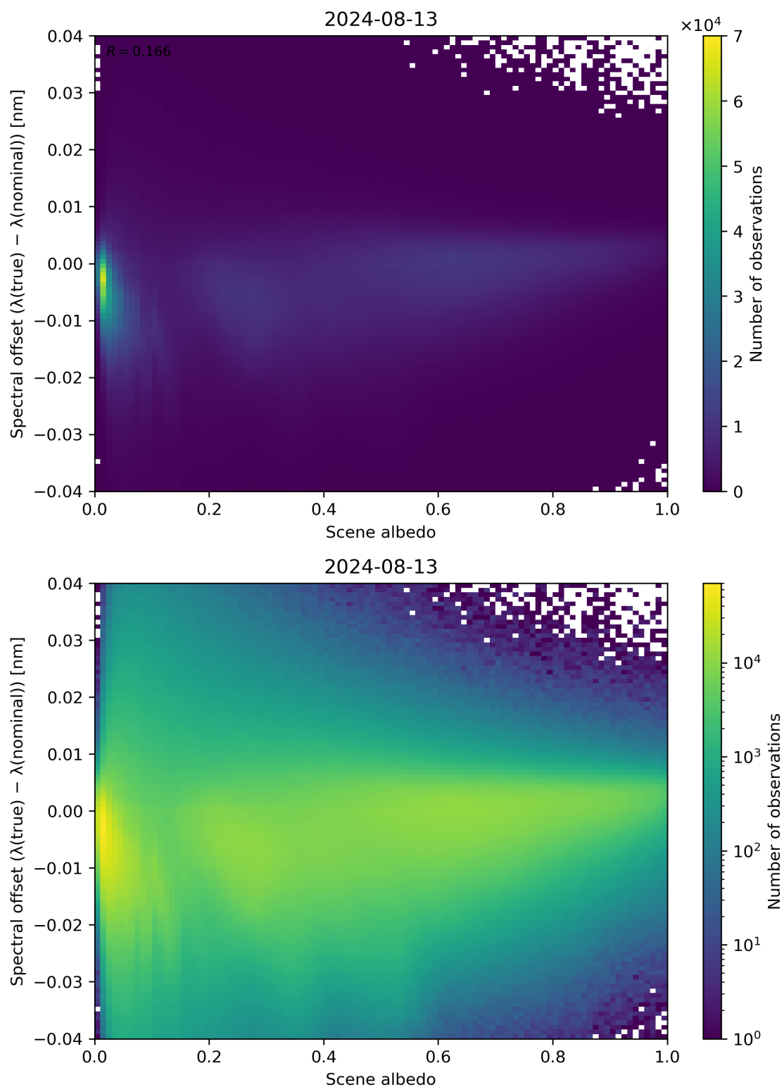
Figure 107: Scatter density plot of “Scene albedo” against “Spectral offset ( \lambda(\text{true}) - \lambda(\text{nominal}) )” for 2024-08-12 to 2024-08-14.
