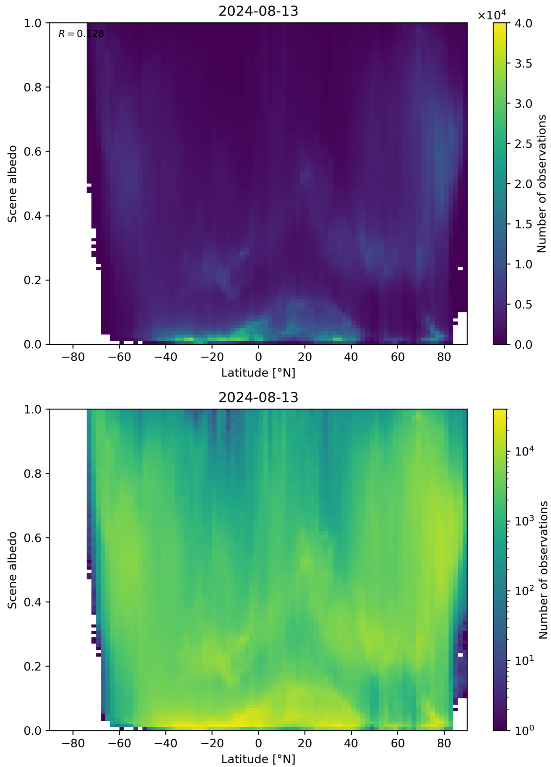
Figure 95: Scatter density plot of “Latitude” against “Scene albedo” for 2024-08-12 to 2024-08-14.
