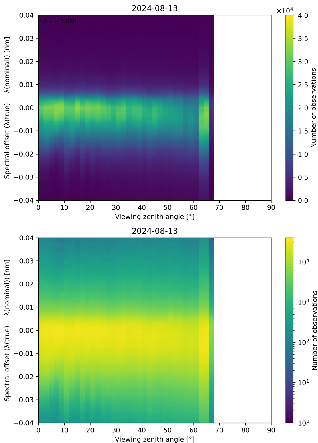
Figure 128: Scatter density plot of “Viewing zenith angle” against “Spectral offset ( \lambda(\text{true}) - \lambda(\text{nominal}) )” for 2024-08-12 to 2024-08-14.
