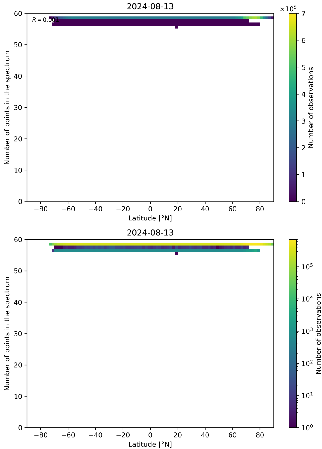
Figure 94: Scatter density plot of “Latitude” against “Number of points in the spectrum” for 2024-08-12 to 2024-08-14.
