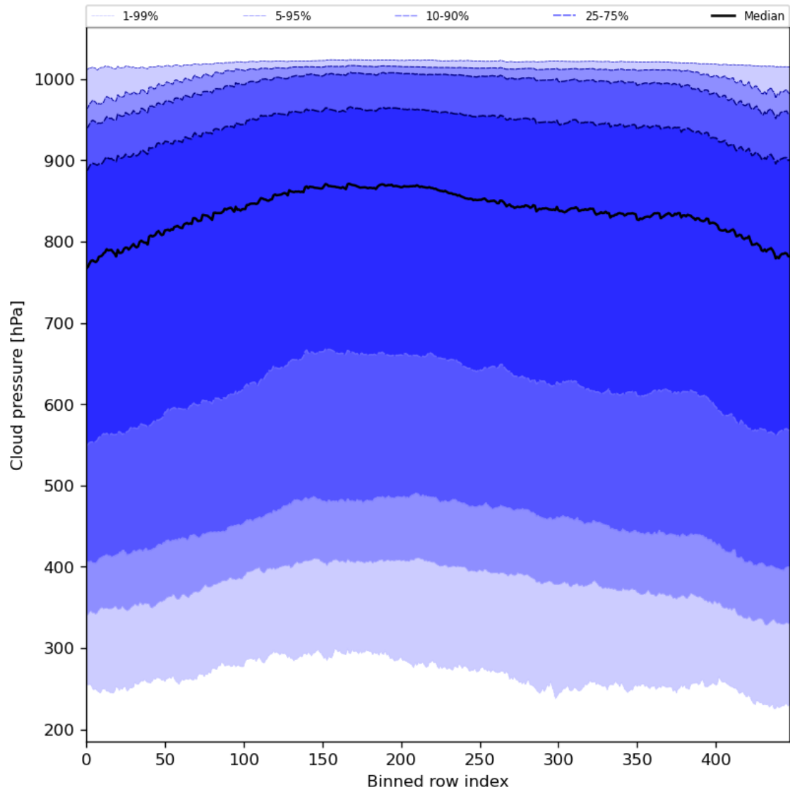
Figure 47: Along track statistics of “Cloud pressure” for 2024-08-12 to 2024-08-14
