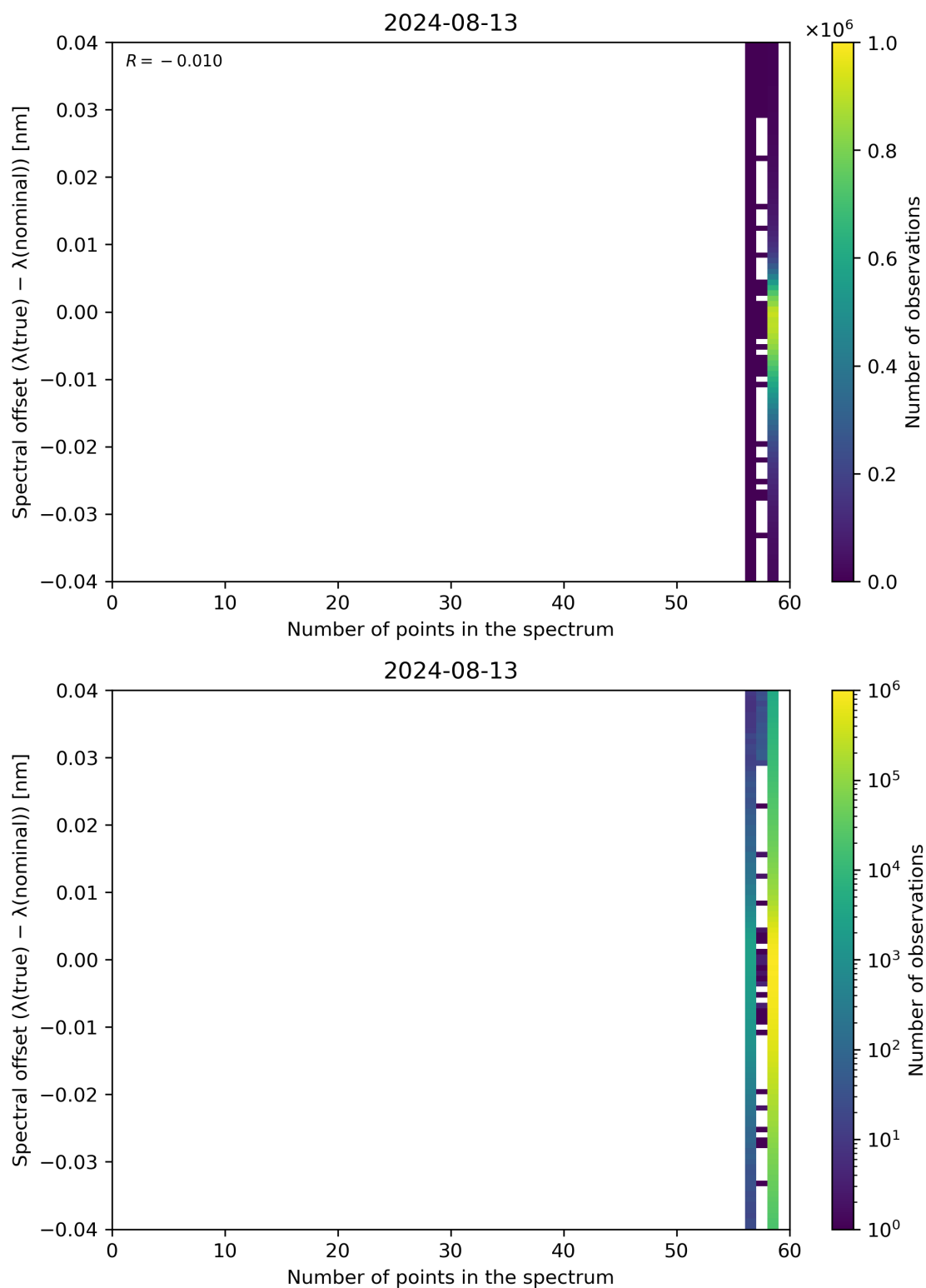
Figure 101: Scatter density plot of “Number of points in the spectrum” against “Spectral offset ( \lambda(\text{true}) - \lambda(\text{nominal}) )” for 2024-08-12 to 2024-08-14.
