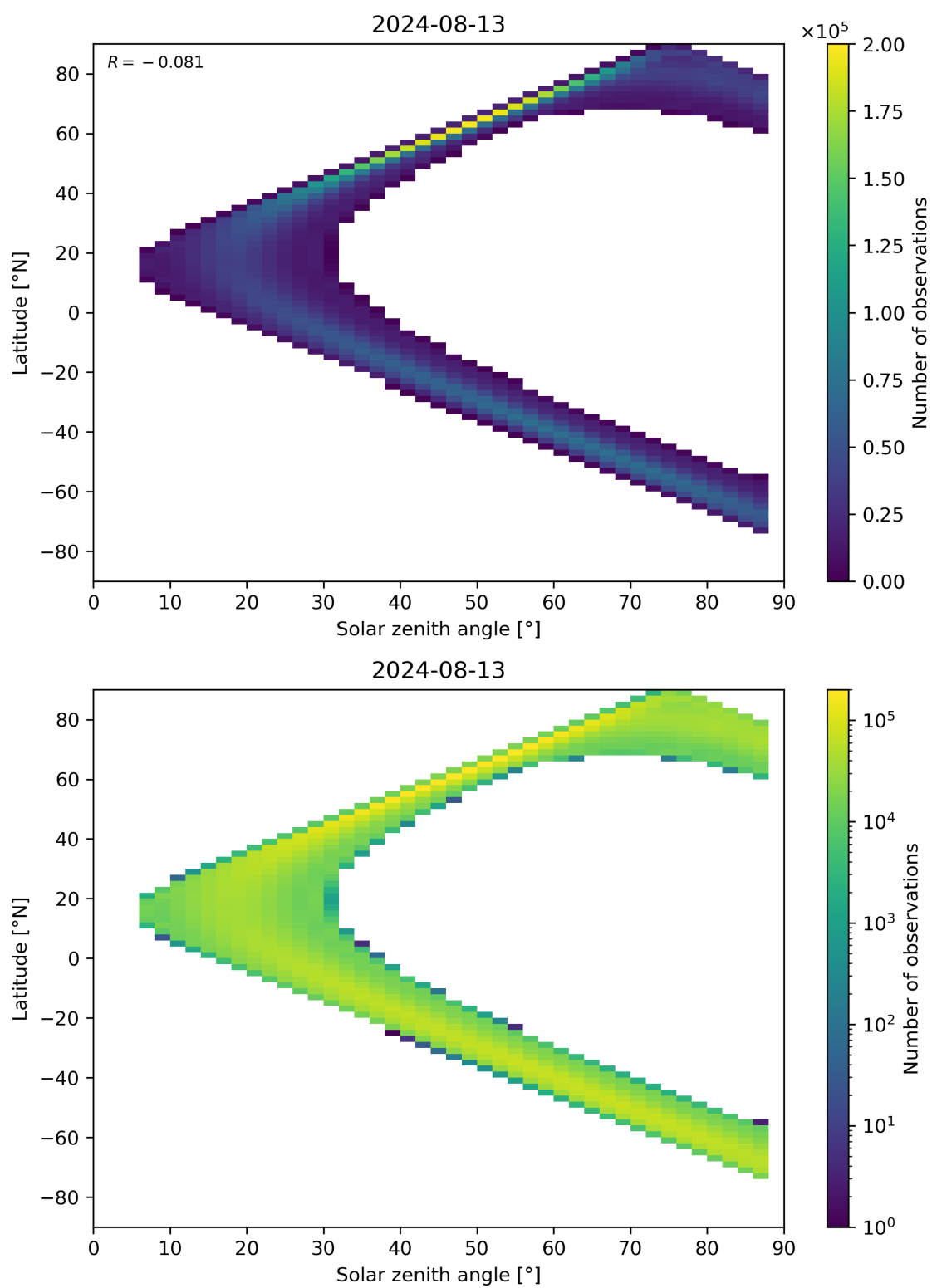
Figure 113: Scatter density plot of “Solar zenith angle” against “Latitude” for 2024-08-12 to 2024-08-14.
