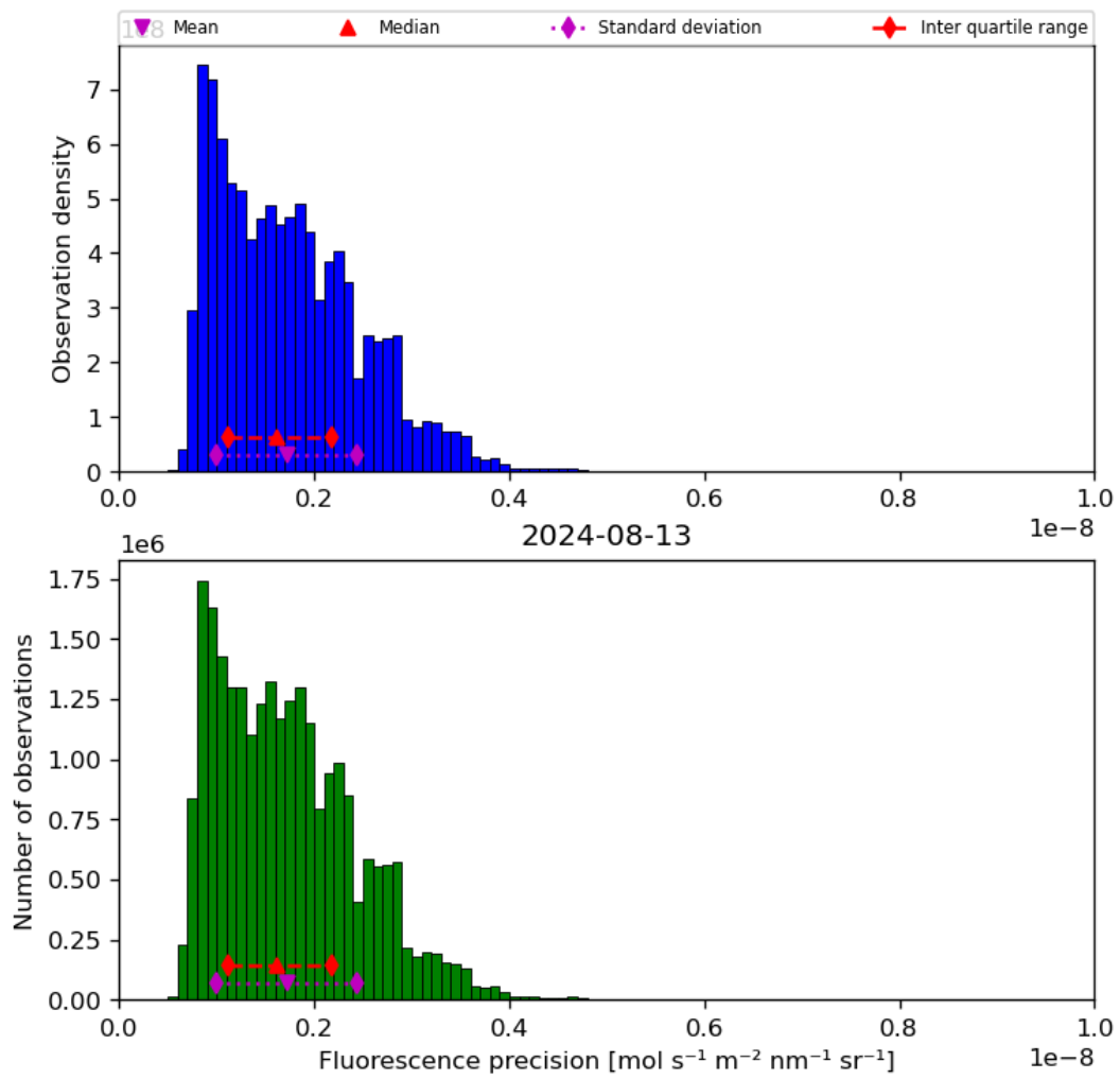
Figure 41: Histogram of “Fluorescence precision” for 2024-08-12 to 2024-08-14
