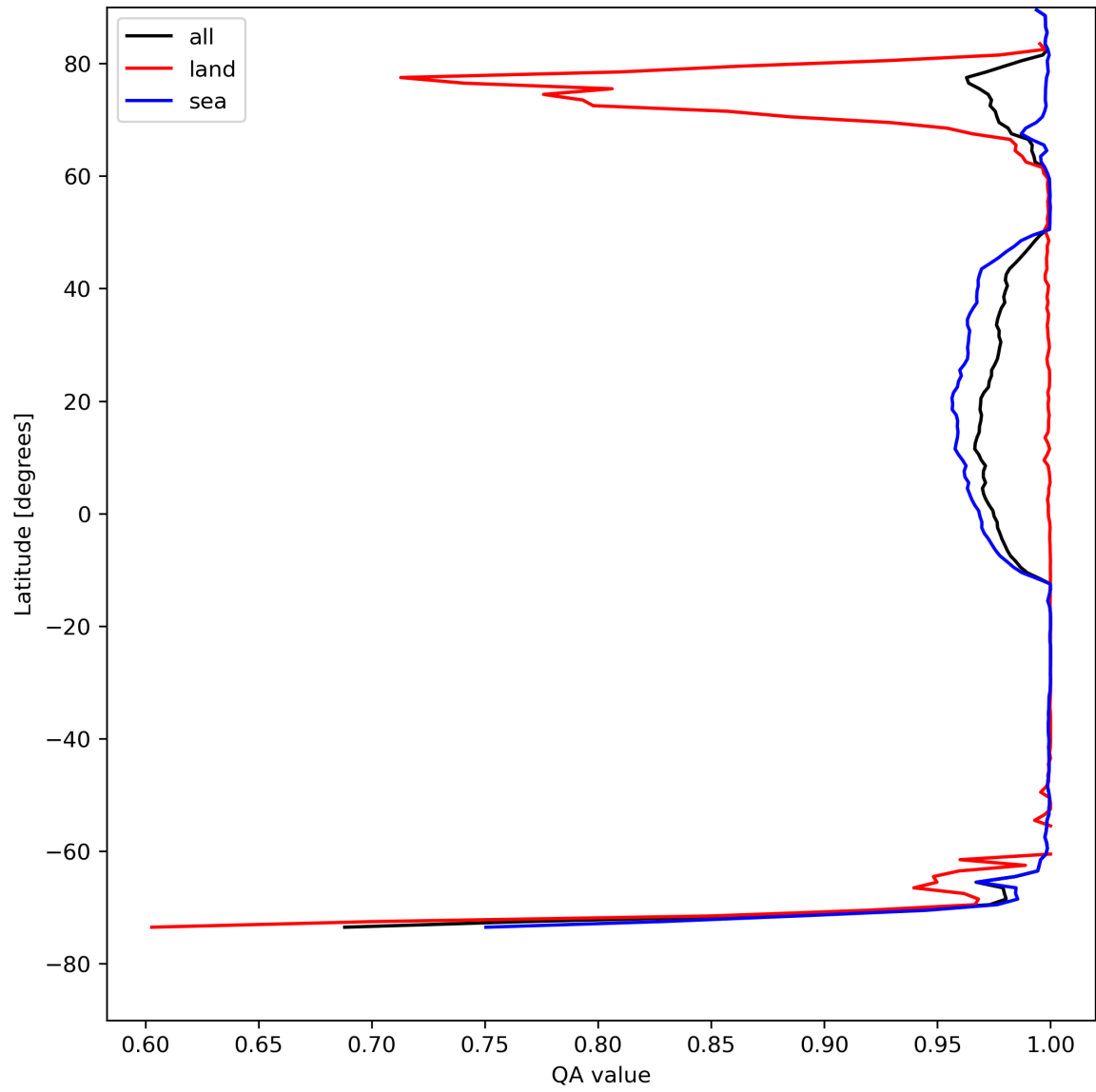
Figure 12: Zonal average of “QA value” for 2024-08-12 to 2024-08-14.
