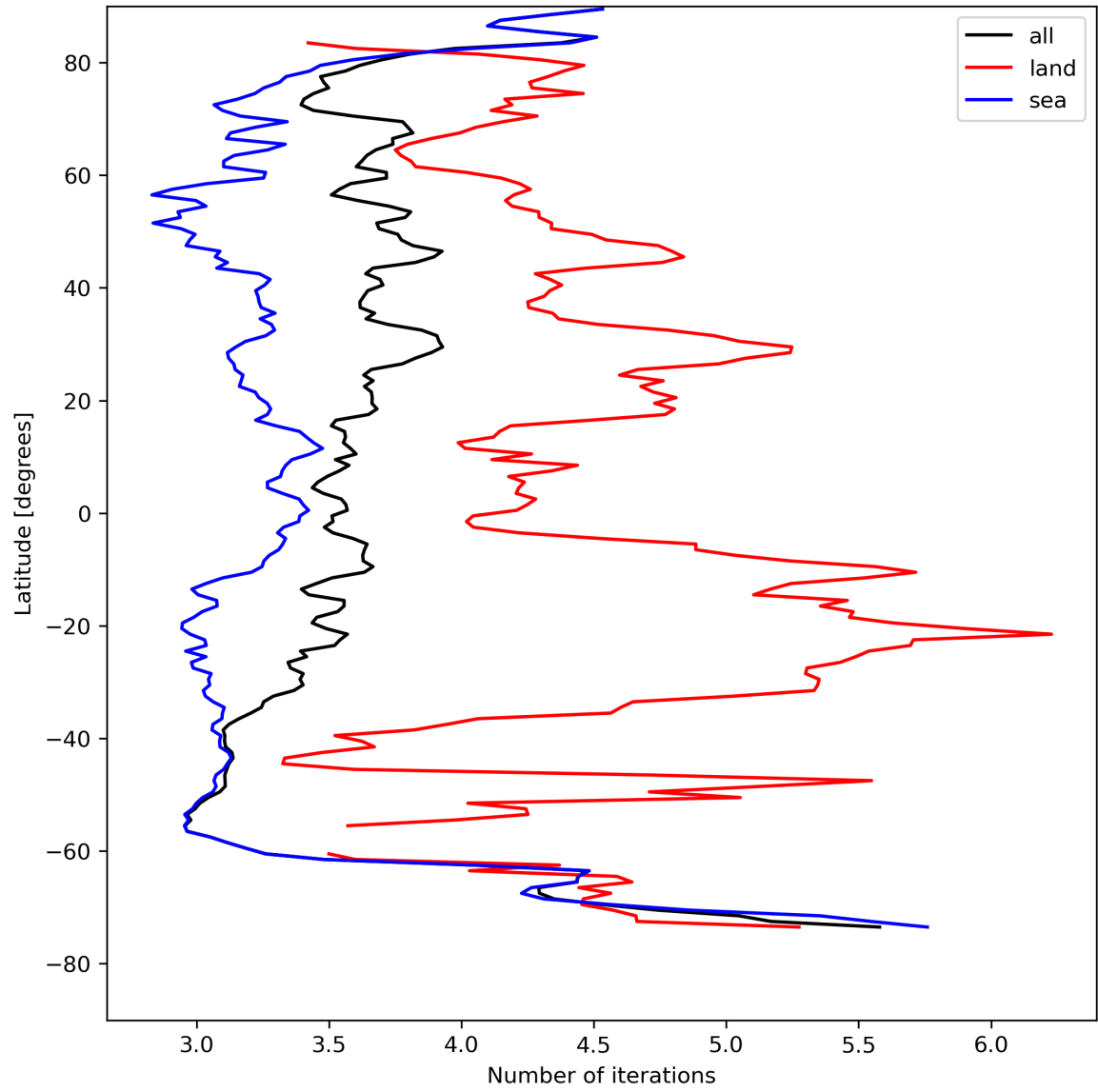
Figure 22: Zonal average of “Number of iterations” for 2024-08-12 to 2024-08-14.
