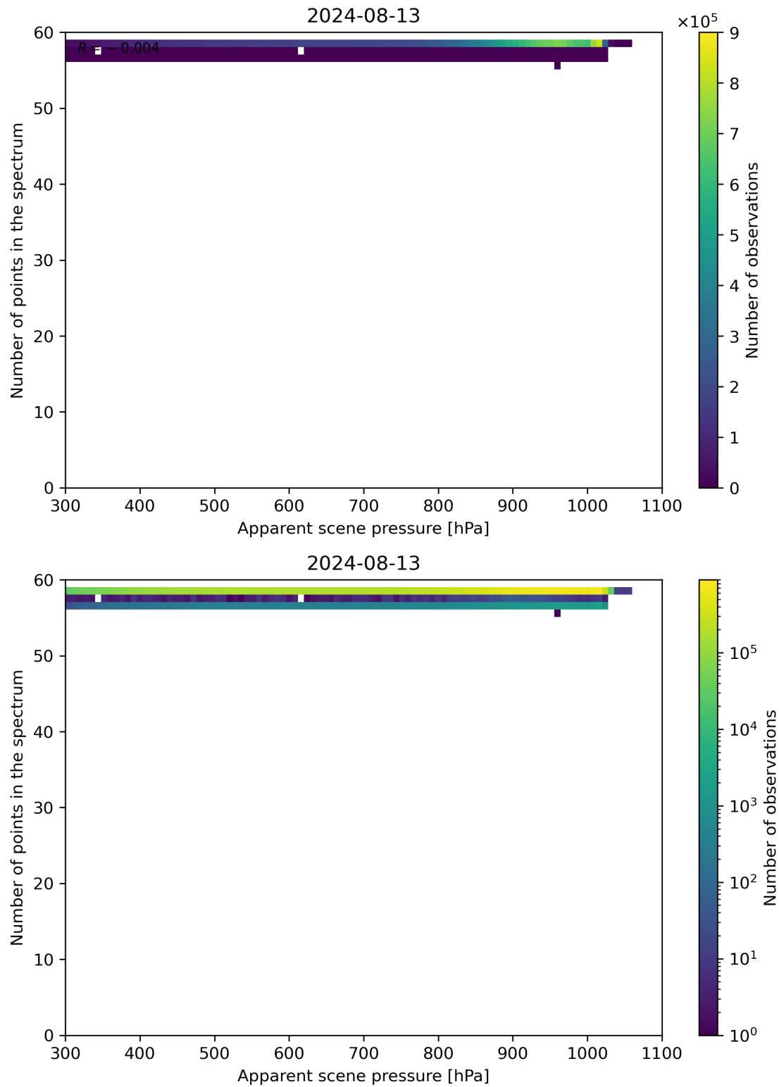
Figure 66: Scatter density plot of “Apparent scene pressure” against “Number of points in the spectrum” for 2024-08-12 to 2024-08-14.
