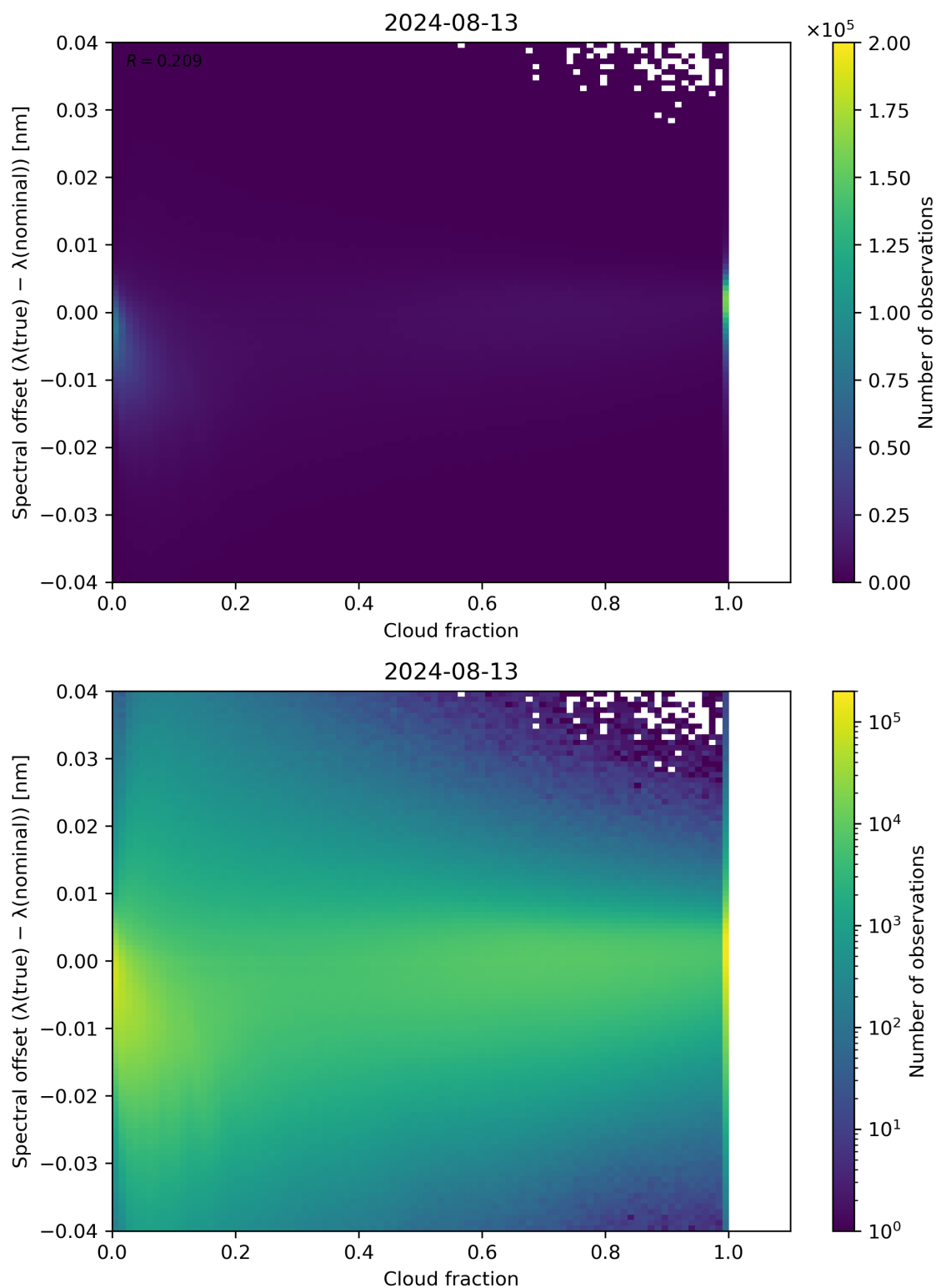
Figure 76: Scatter density plot of “Cloud fraction” against “Spectral offset ( \lambda(\text{true}) - \lambda(\text{nominal}) )” for 2024-08-12 to 2024-08-14.
