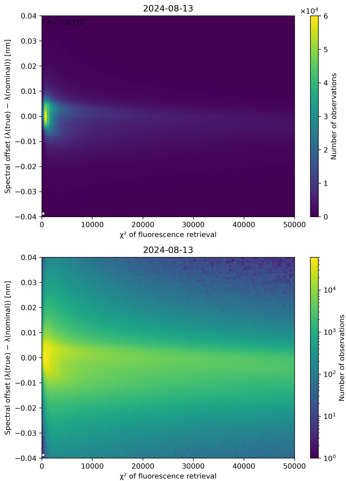
Figure 69: Scatter density plot of " \chi^2 of fluorescence retrieval" against "Spectral offset ( \lambda(\text{true}) - \lambda(\text{nominal}) )" for 2024-08-12 to 2024-08-14.
