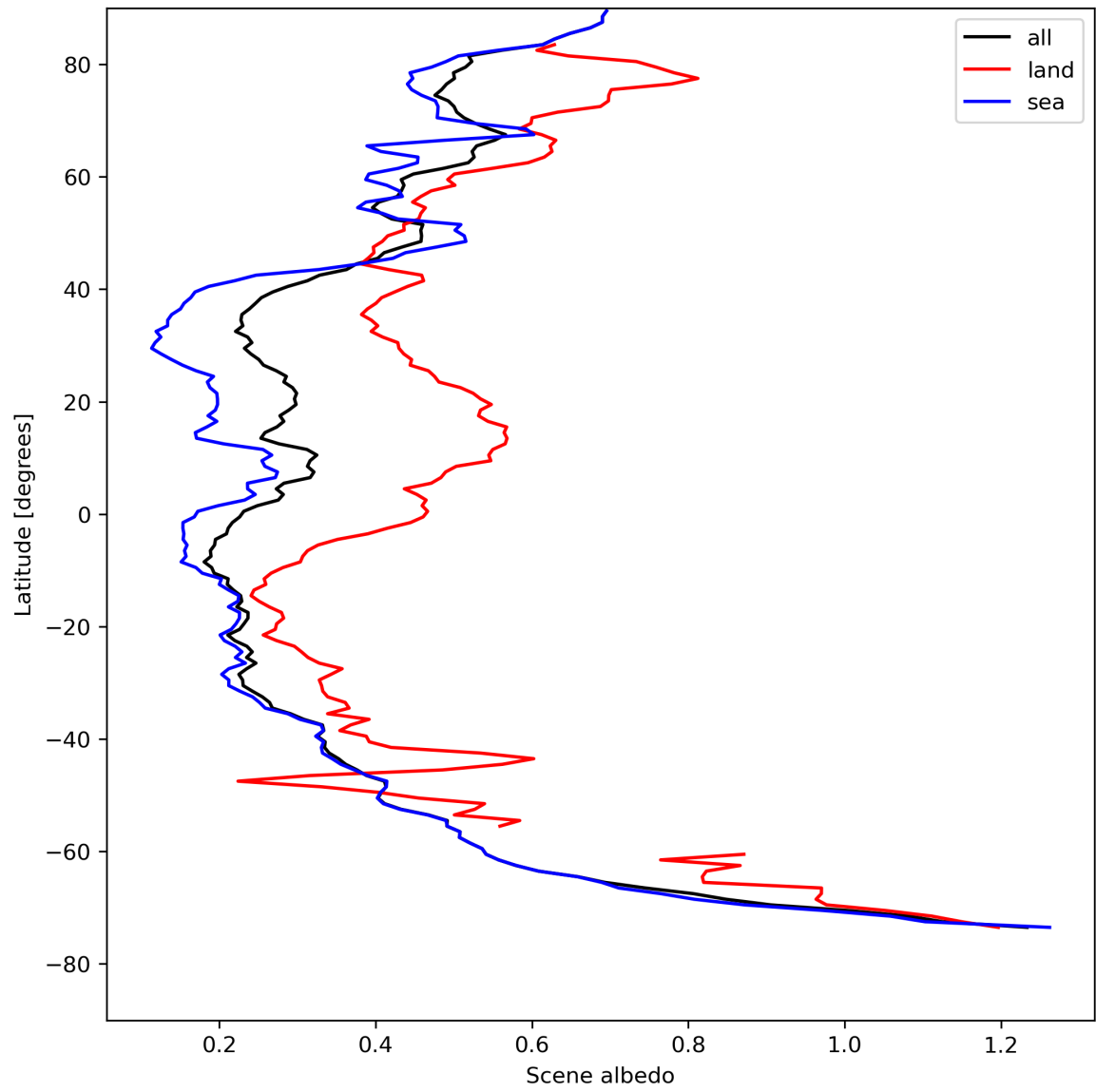
Figure 17: Zonal average of “Scene albedo” for 2024-08-12 to 2024-08-14.
