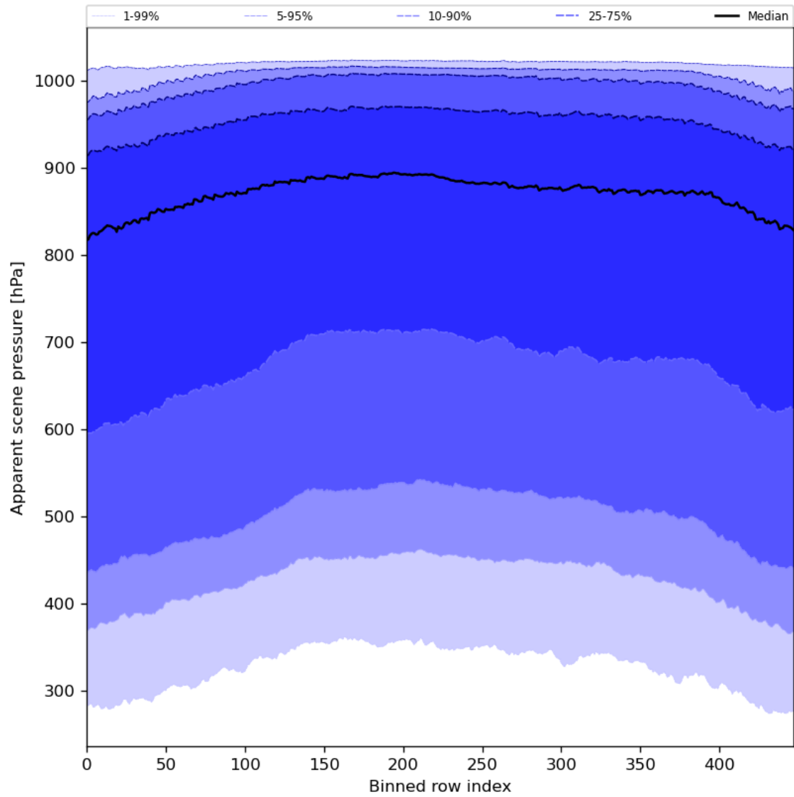
Figure 53: Along track statistics of “Apparent scene pressure” for 2024-08-12 to 2024-08-14
