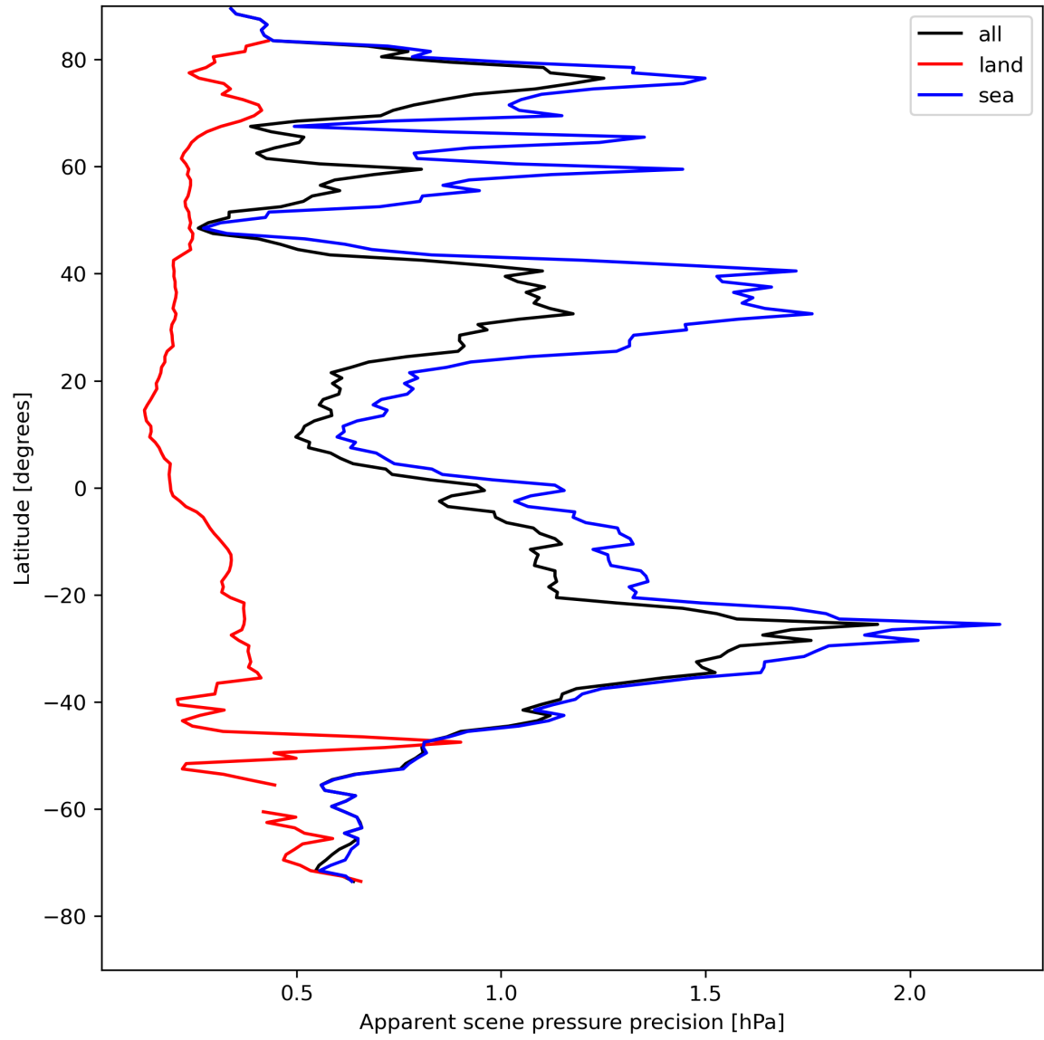
Figure 20: Zonal average of “Apparent scene pressure precision” for 2024-08-12 to 2024-08-14.
