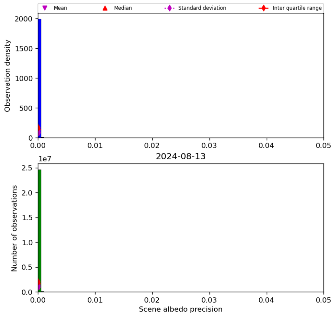
Figure 35: Histogram of “Scene albedo precision” for 2024-08-12 to 2024-08-14
