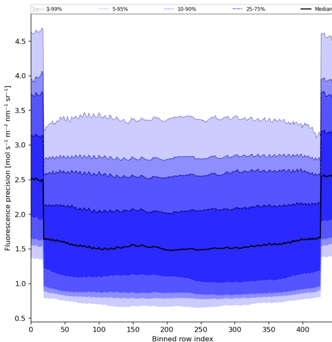
Figure 58: Along track statistics of “Fluorescence precision” for 2024-08-12 to 2024-08-14
