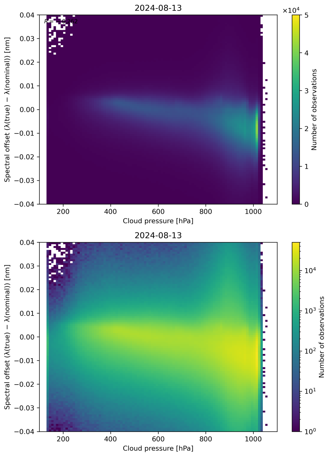
Figure 84: Scatter density plot of “Cloud pressure” against “Spectral offset ( \lambda(\text{true}) - \lambda(\text{nominal}) )” for 2024-08-12 to 2024-08-14.
