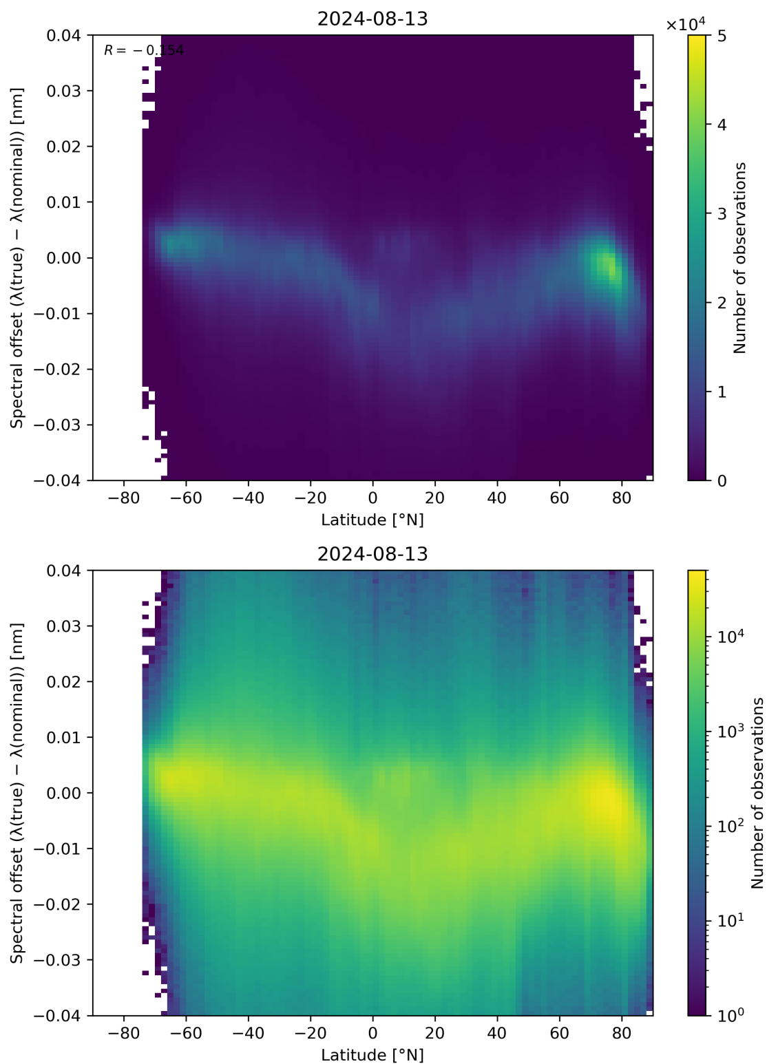
Figure 96: Scatter density plot of “Latitude” against “Spectral offset ( \lambda(\text{true}) - \lambda(\text{nominal}) )” for 2024-08-12 to 2024-08-14.
