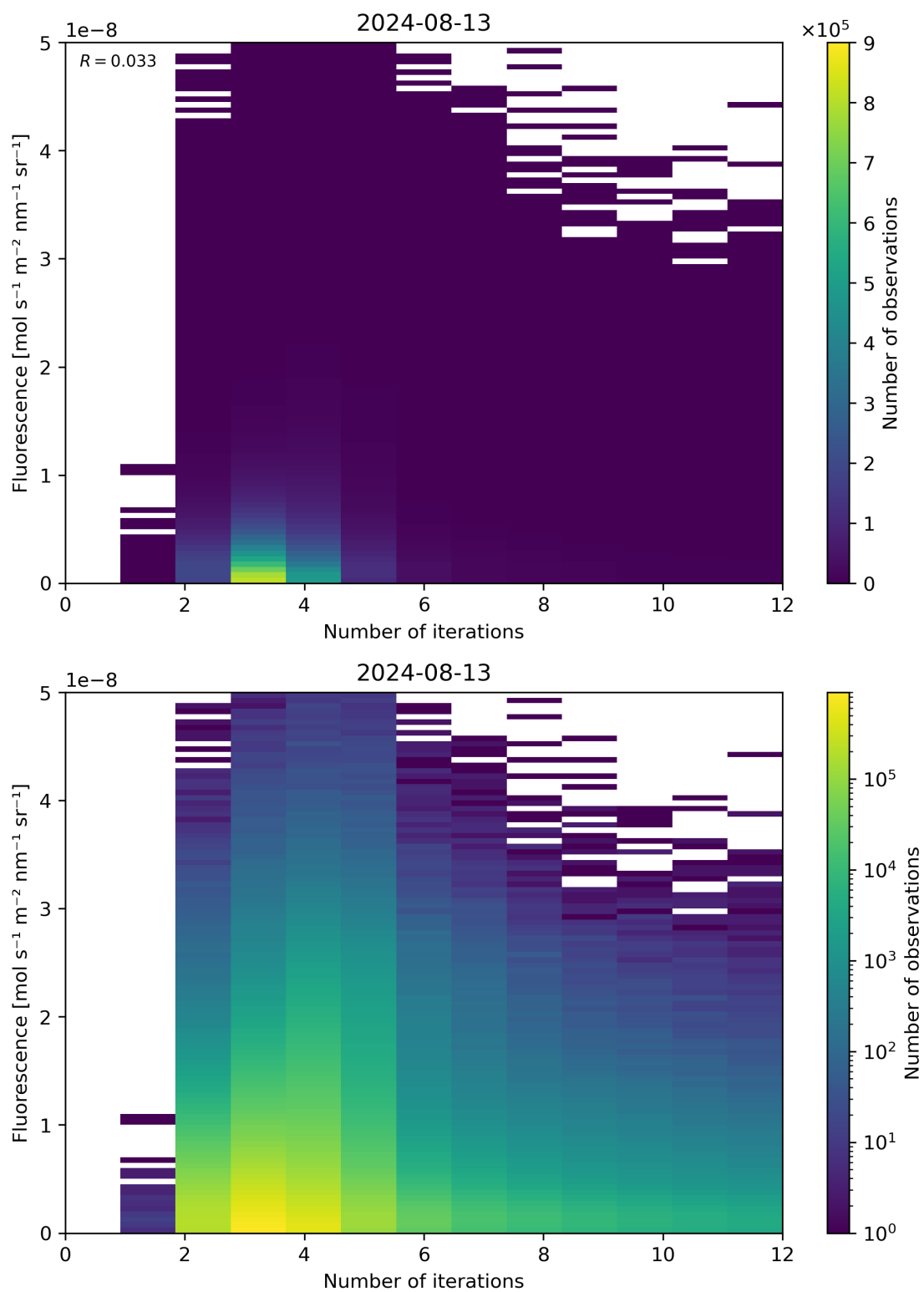
Figure 98: Scatter density plot of “Number of iterations” against “Fluorescence” for 2024-08-12 to 2024-08-14.
