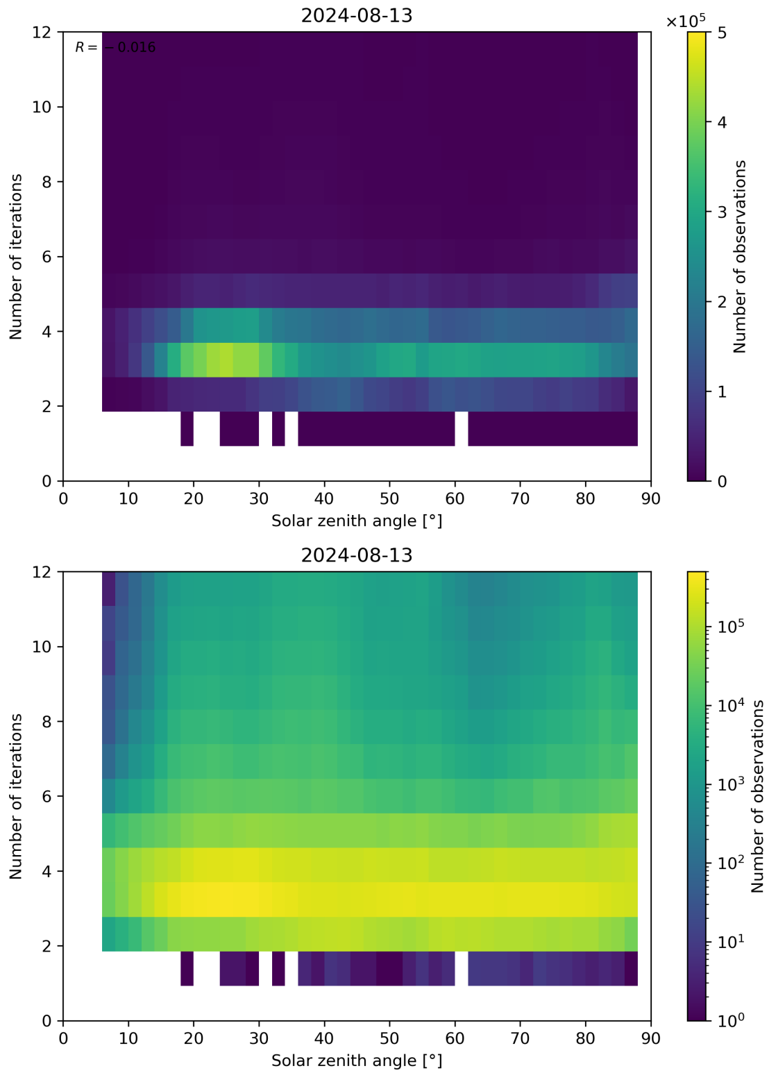
Figure 114: Scatter density plot of “Solar zenith angle” against “Number of iterations” for 2024-08-12 to 2024-08-14.
