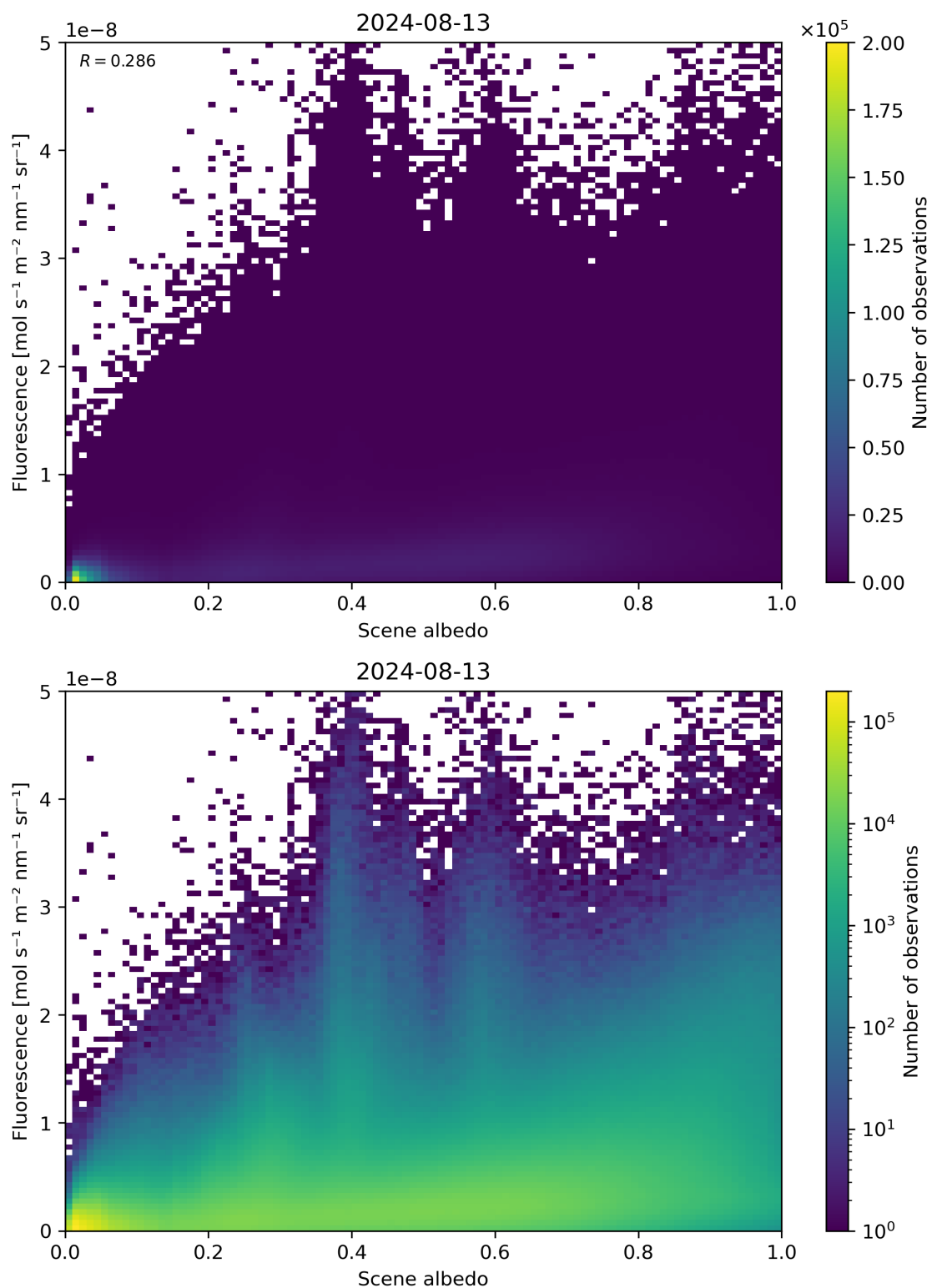
Figure 104: Scatter density plot of “Scene albedo” against “Fluorescence” for 2024-08-12 to 2024-08-14.
