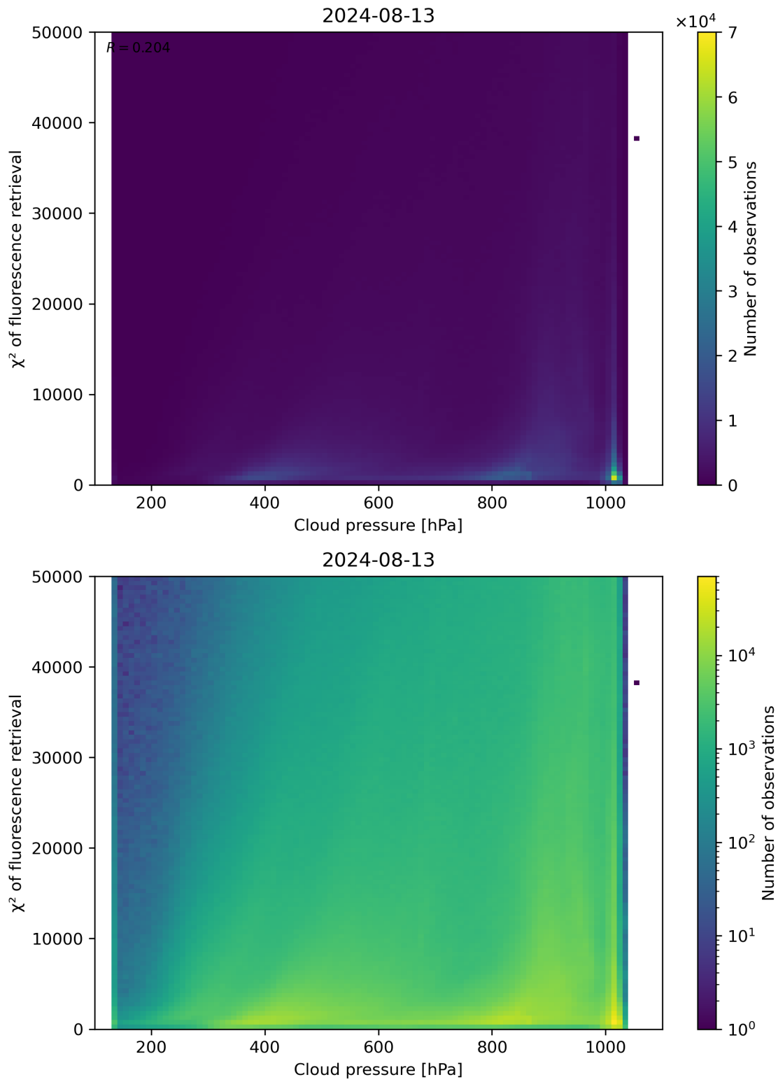
Figure 78: Scatter density plot of “Cloud pressure” against “ \chi^2 of fluorescence retrieval” for 2024-08-12 to 2024-08-14.
