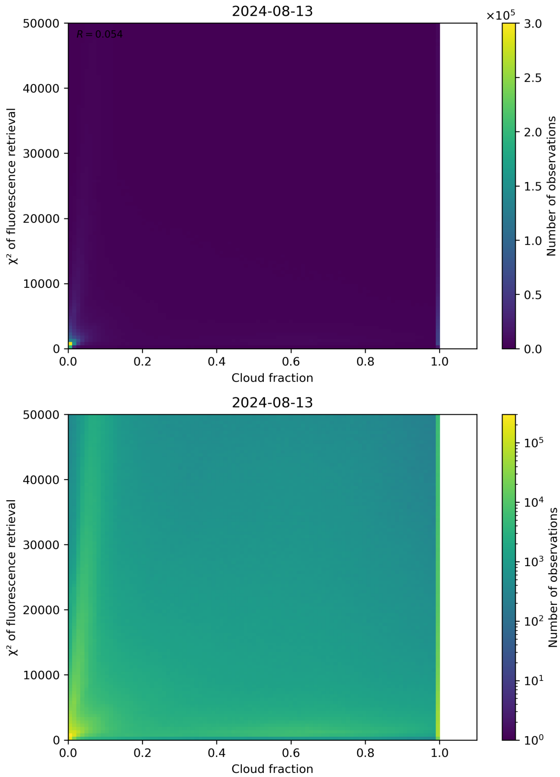
Figure 71: Scatter density plot of “Cloud fraction” against “ \chi^2 of fluorescence retrieval” for 2024-08-12 to 2024-08-14.
