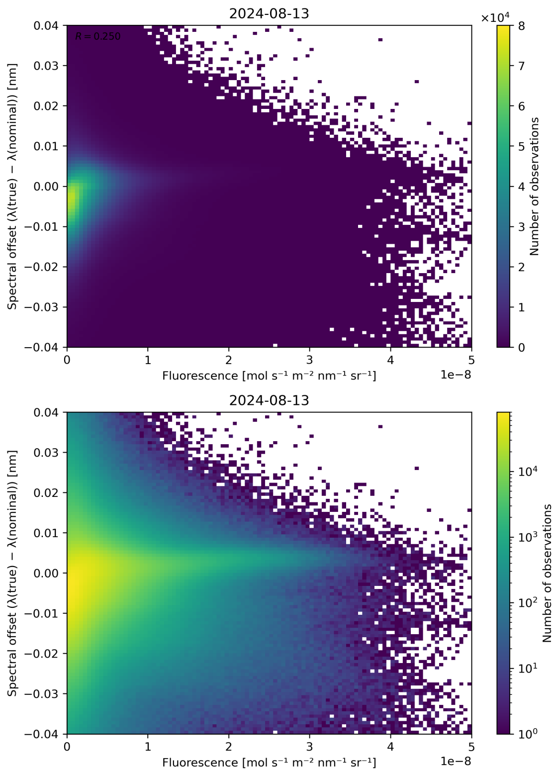
Figure 87: Scatter density plot of “Fluorescence” against “Spectral offset ( \lambda(\text{true}) - \lambda(\text{nominal}) )” for 2024-08-12 to 2024-08-14.
