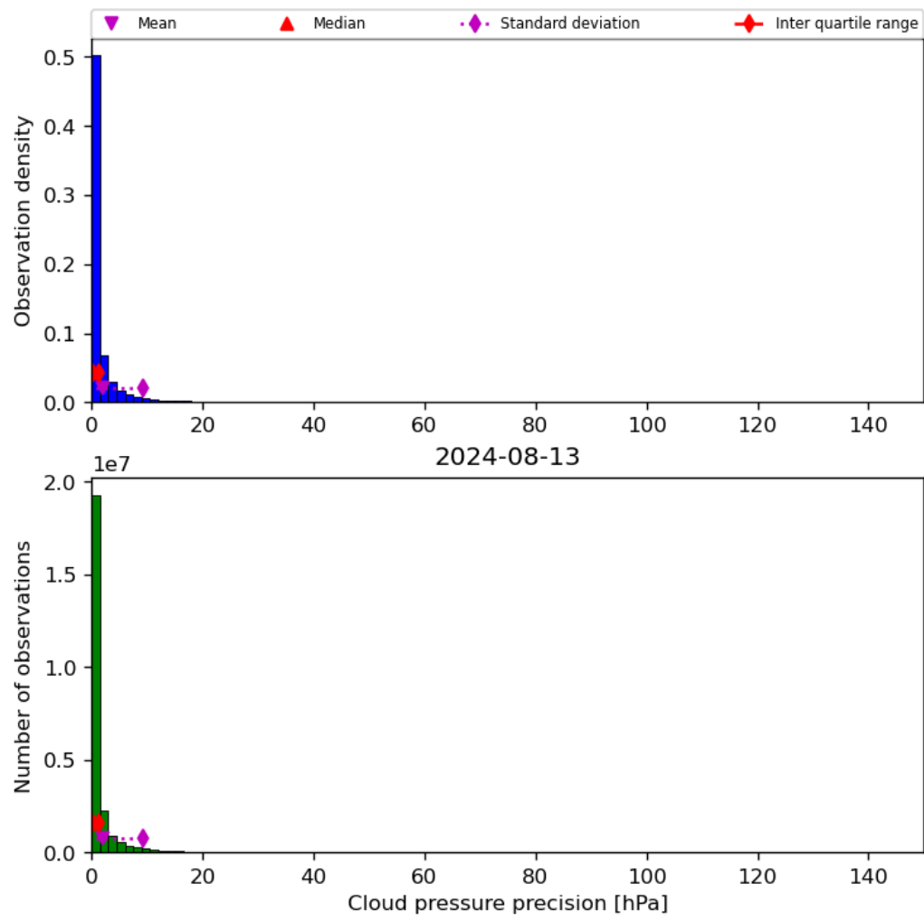
Figure 31: Histogram of “Cloud pressure precision” for 2024-08-12 to 2024-08-14
