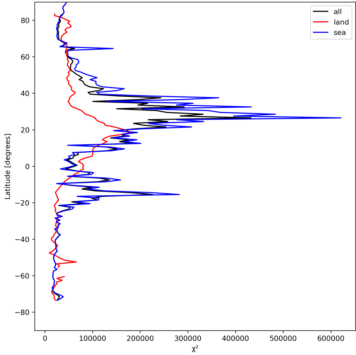
Figure 21: Zonal average of “ \chi^2 ” for 2024-08-12 to 2024-08-14.
