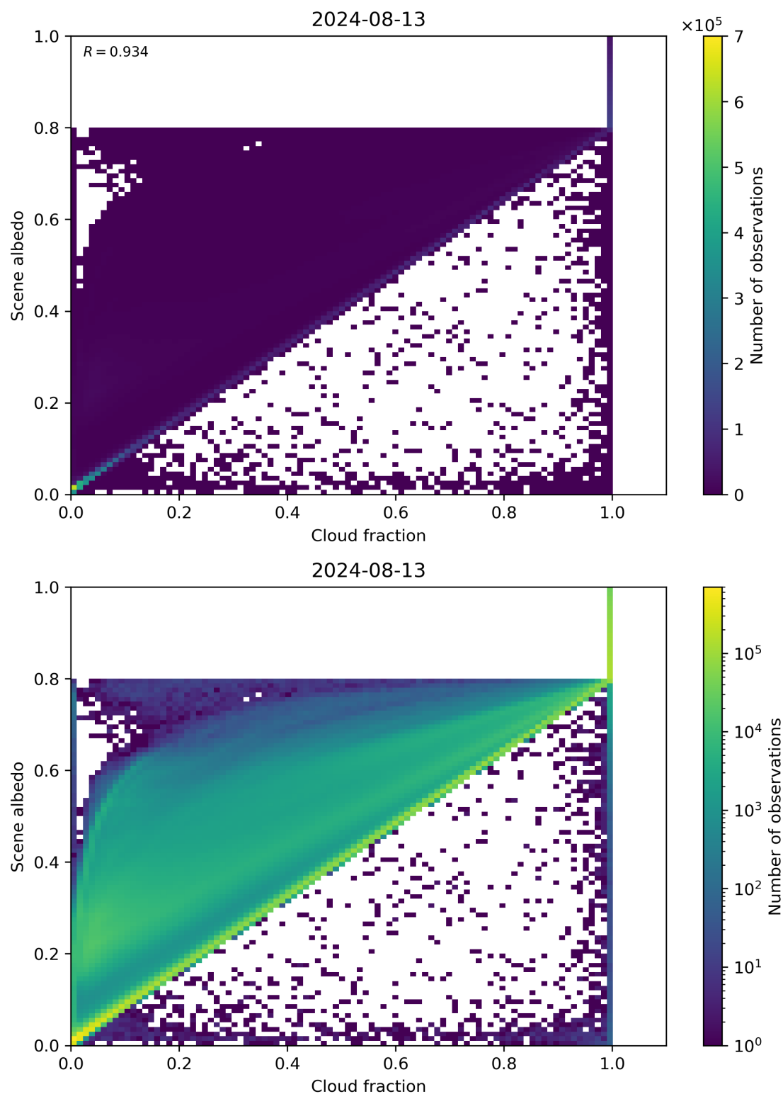
Figure 75: Scatter density plot of “Cloud fraction” against “Scene albedo” for 2024-08-12 to 2024-08-14.
