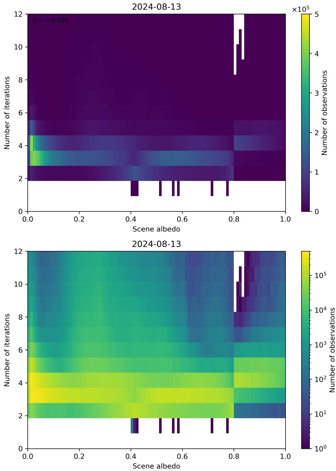
Figure 105: Scatter density plot of “Scene albedo” against “Number of iterations” for 2024-08-12 to 2024-08-14.
