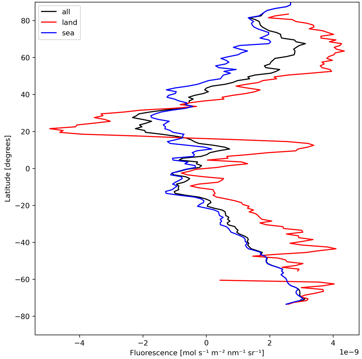
Figure 23: Zonal average of “Fluorescence” for 2024-08-12 to 2024-08-14.
