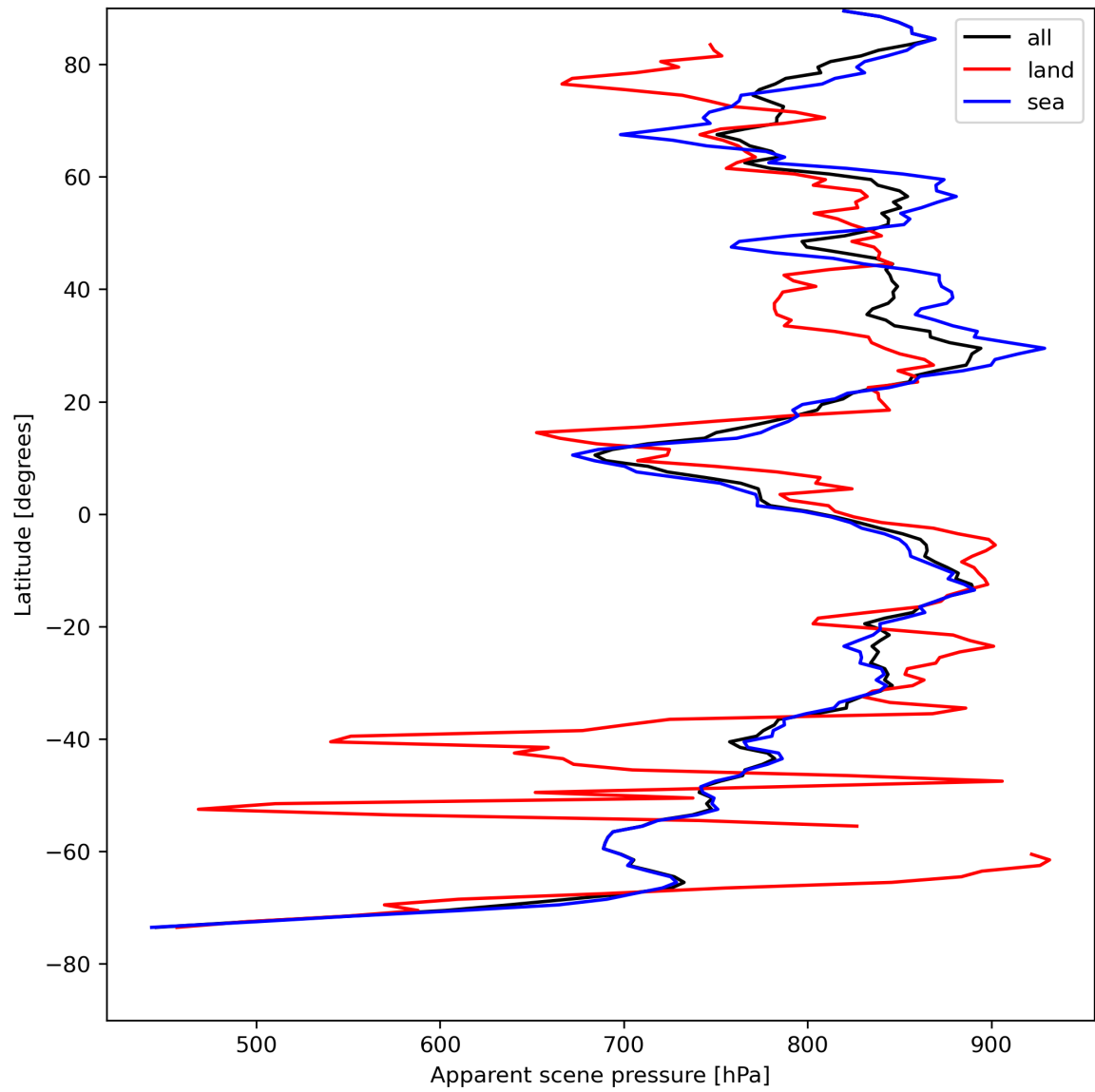
Figure 19: Zonal average of “Apparent scene pressure” for 2024-08-12 to 2024-08-14.
