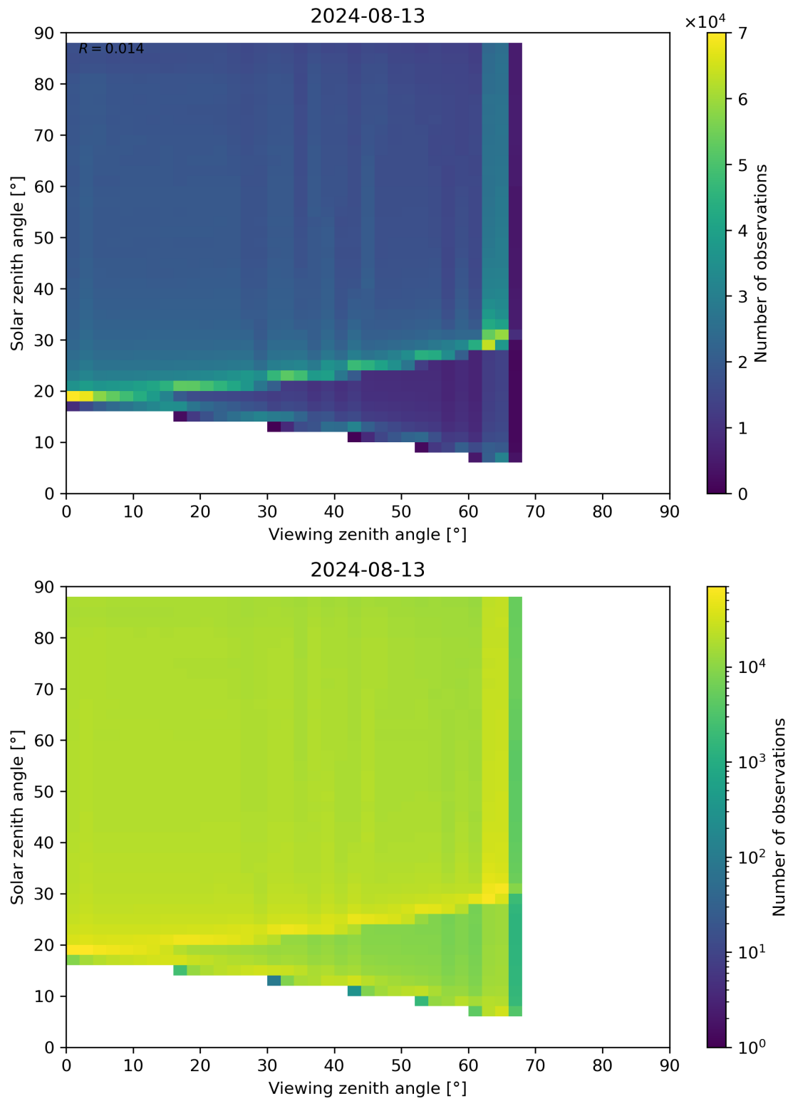
Figure 127: Scatter density plot of “Viewing zenith angle” against “Solar zenith angle” for 2024-08-12 to 2024-08-14.
