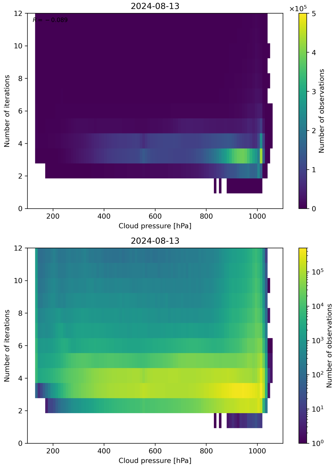
Figure 81: Scatter density plot of “Cloud pressure” against “Number of iterations” for 2024-08-12 to 2024-08-14.
