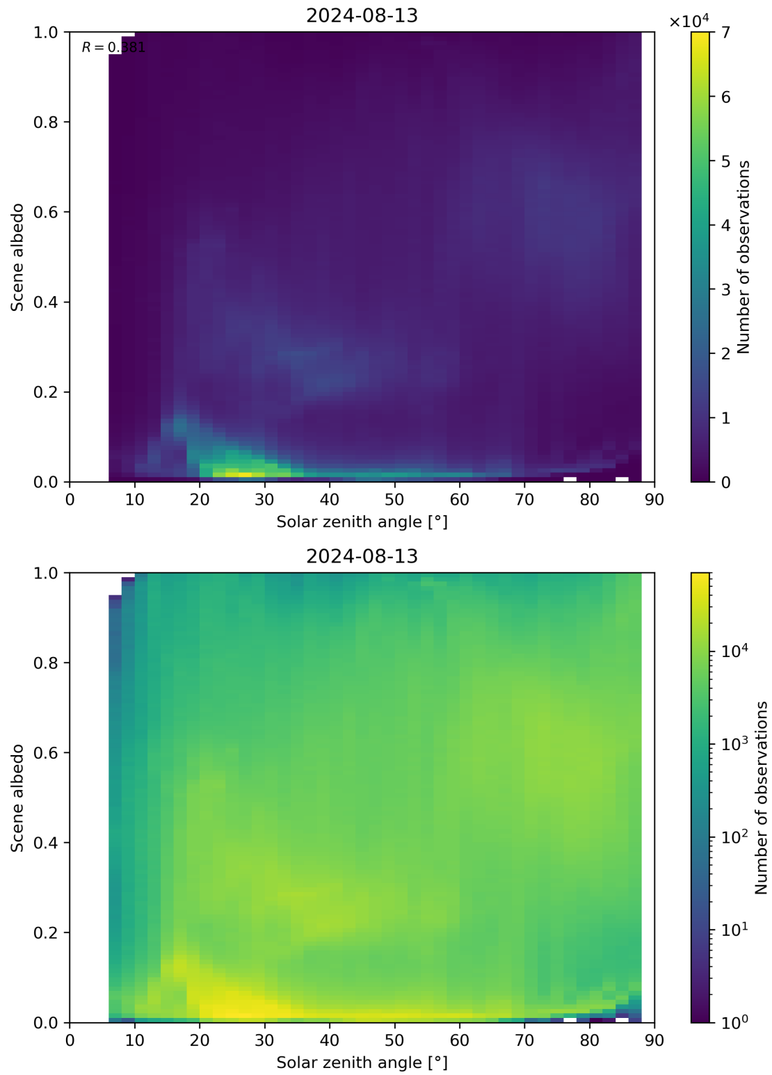
Figure 116: Scatter density plot of “Solar zenith angle” against “Scene albedo” for 2024-08-12 to 2024-08-14.
