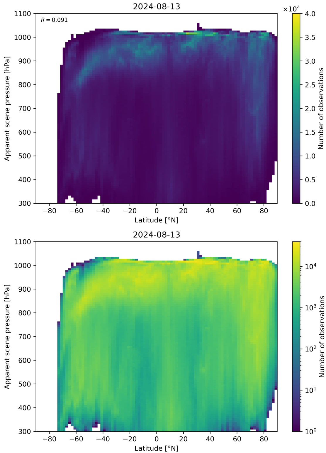
Figure 88: Scatter density plot of “Latitude” against “Apparent scene pressure” for 2024-08-12 to 2024-08-14.
