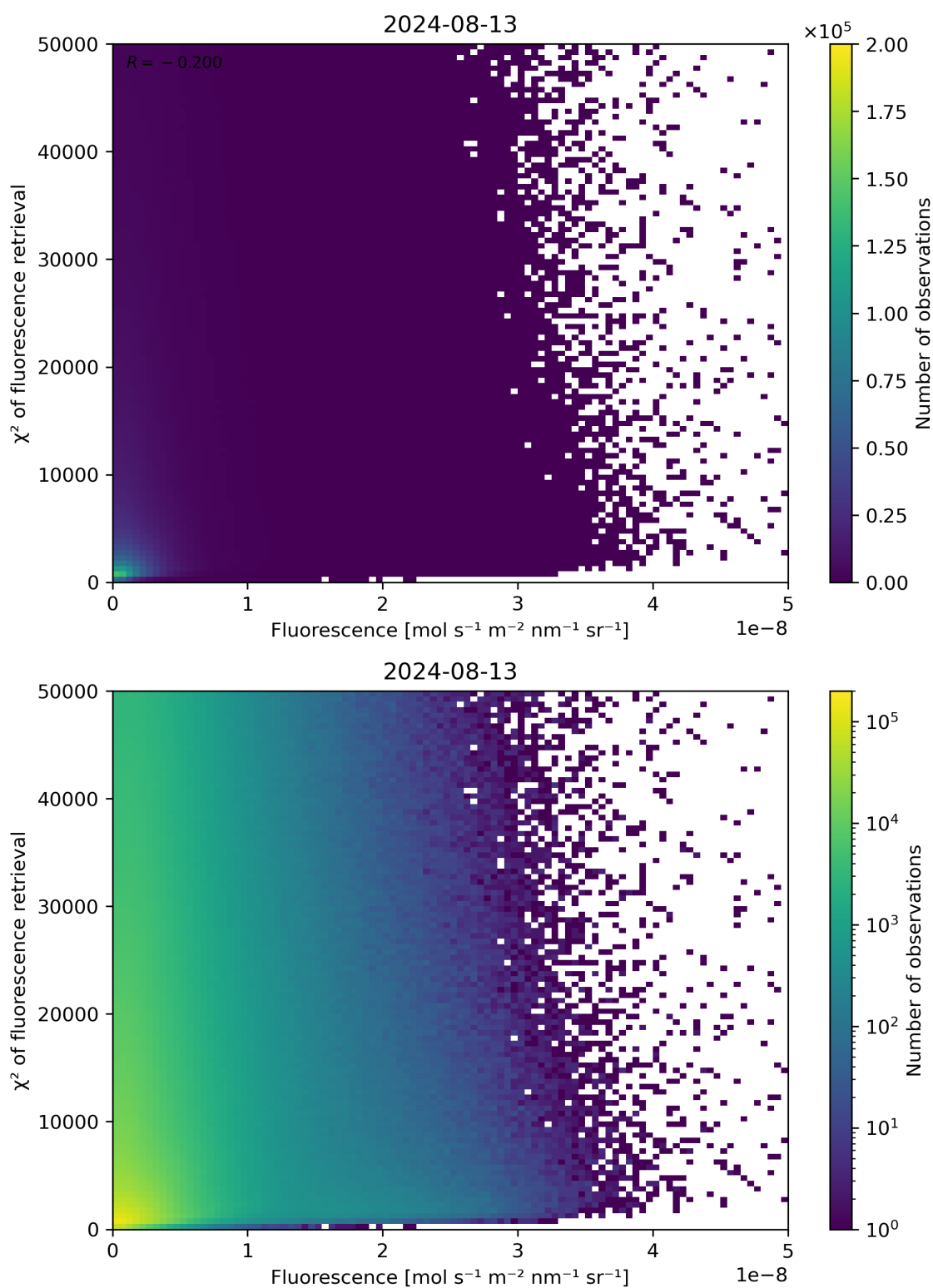
Figure 85: Scatter density plot of “Fluorescence” against “ \chi^2 of fluorescence retrieval” for 2024-08-12 to 2024-08-14.
