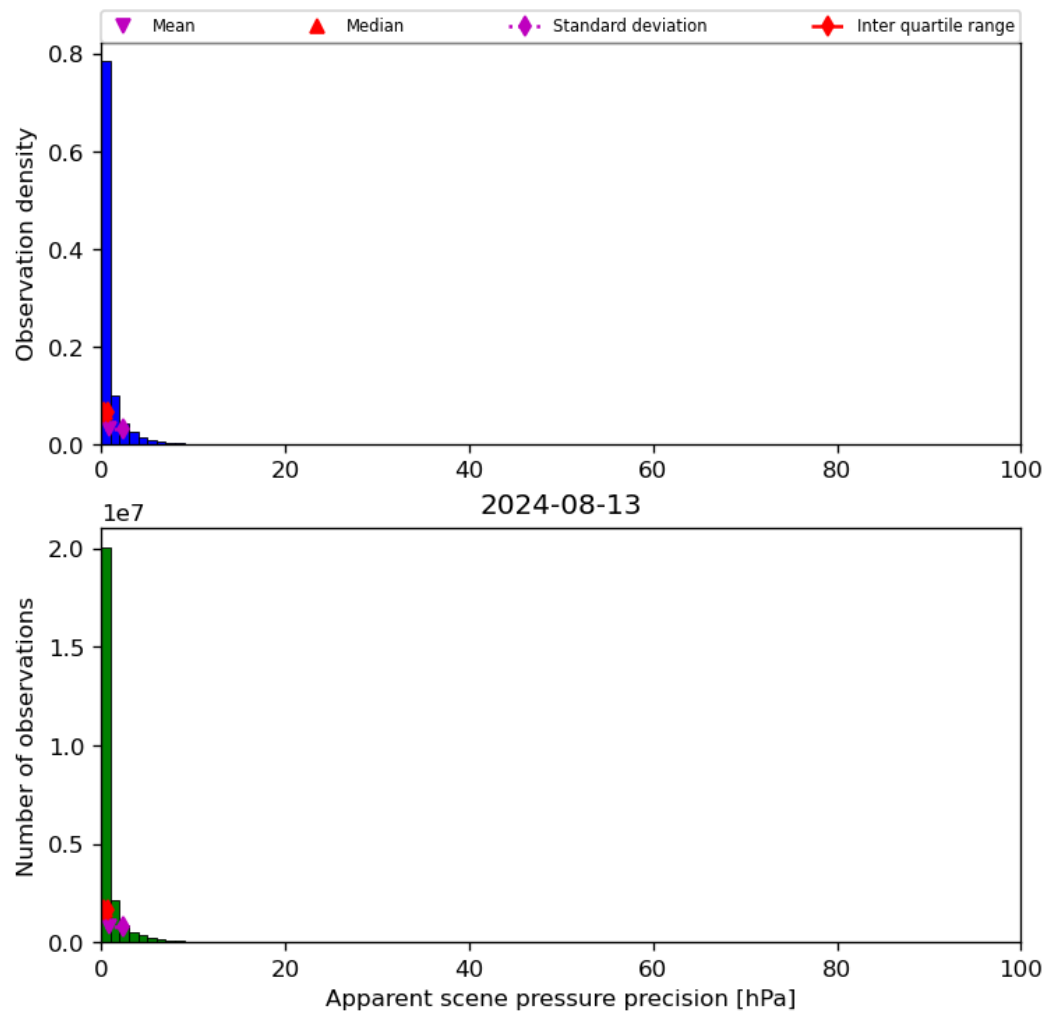
Figure 37: Histogram of “Apparent scene pressure precision” for 2024-08-12 to 2024-08-14
