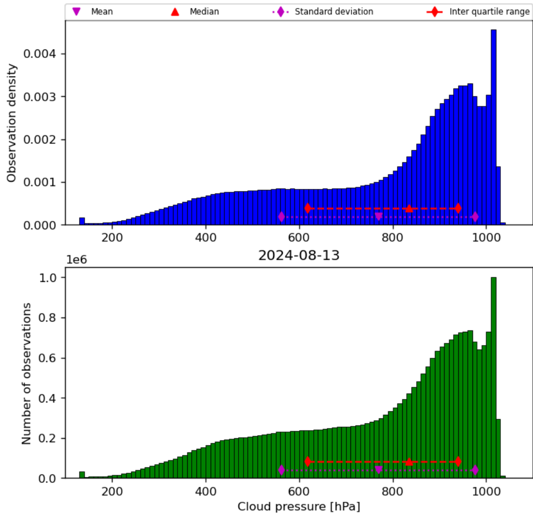
Figure 30: Histogram of “Cloud pressure” for 2024-08-12 to 2024-08-14
