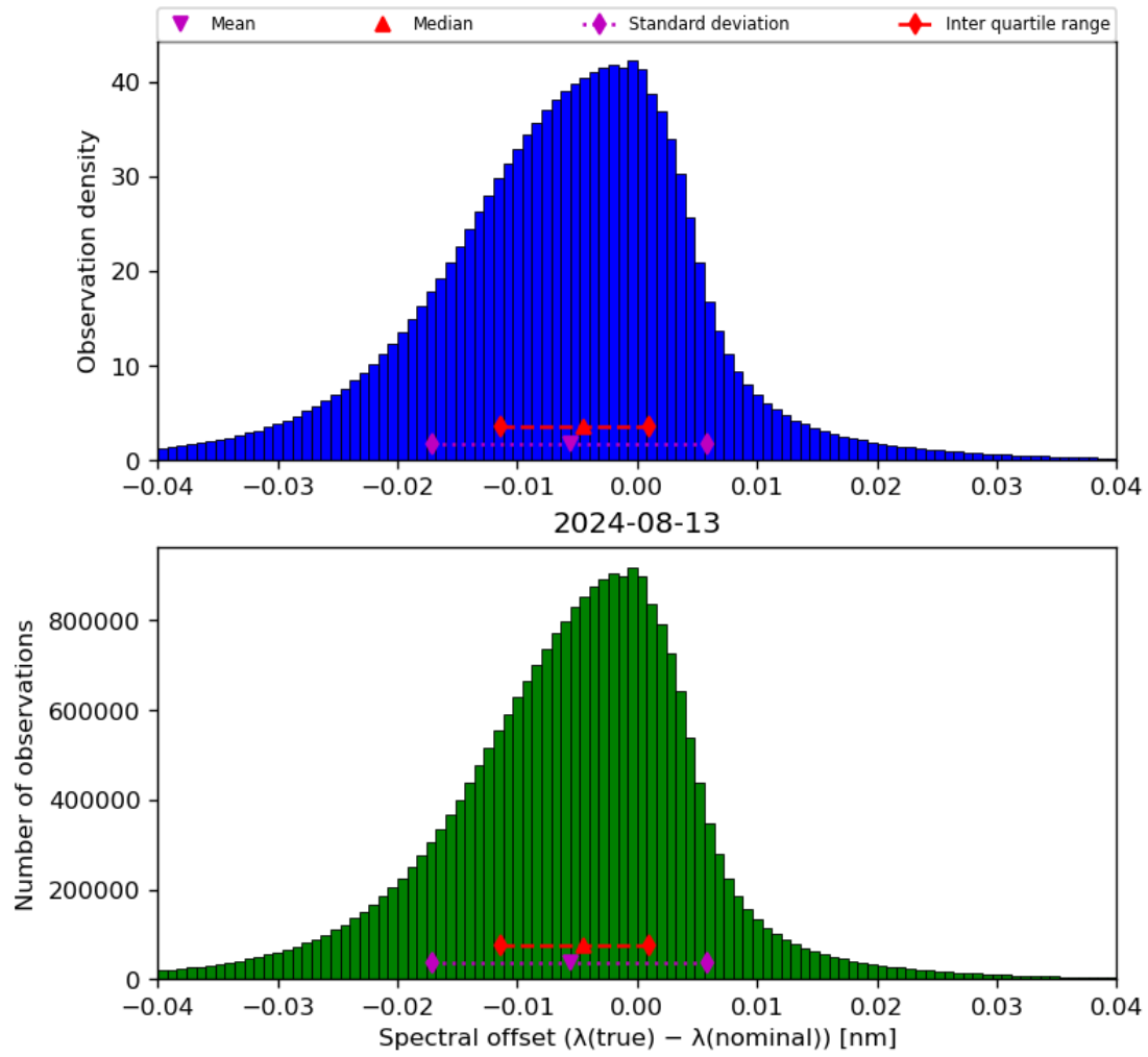
Figure 45: Histogram of “Spectral offset ( \lambda(\text{true}) - \lambda(\text{nominal}) )” for 2024-08-12 to 2024-08-14
