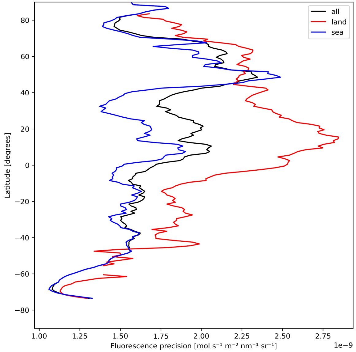
Figure 24: Zonal average of “Fluorescence precision” for 2024-08-12 to 2024-08-14.
