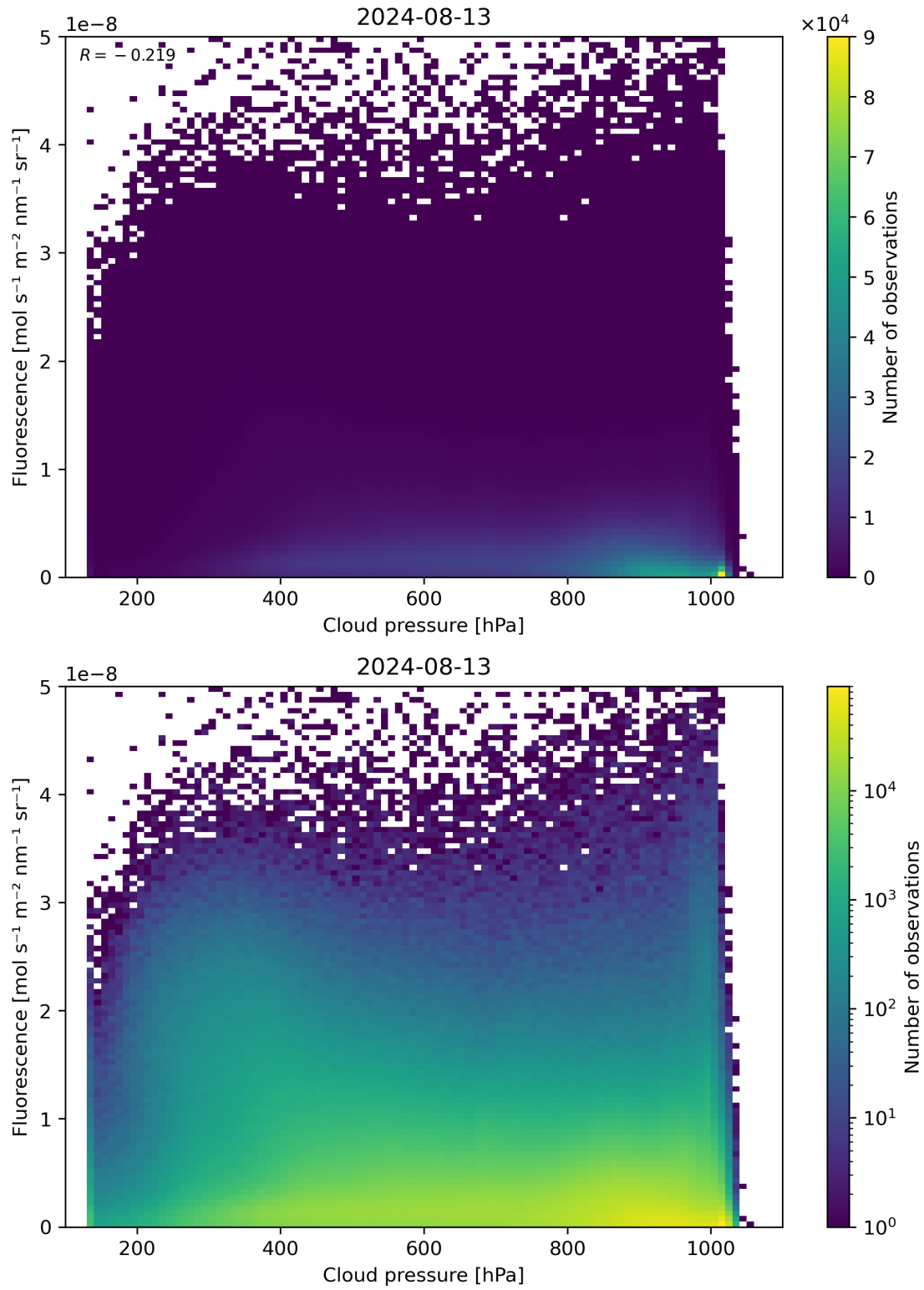
Figure 80: Scatter density plot of “Cloud pressure” against “Fluorescence” for 2024-08-12 to 2024-08-14.
