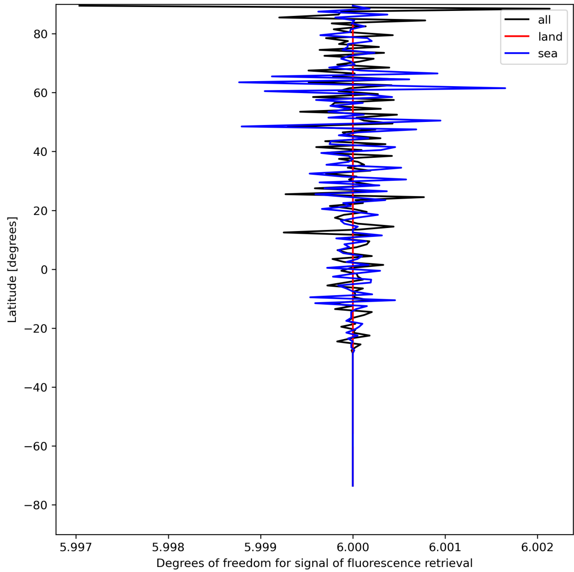
Figure 26: Zonal average of “Degrees of freedom for signal of fluorescence retrieval” for 2024-08-12 to 2024-08-14.
