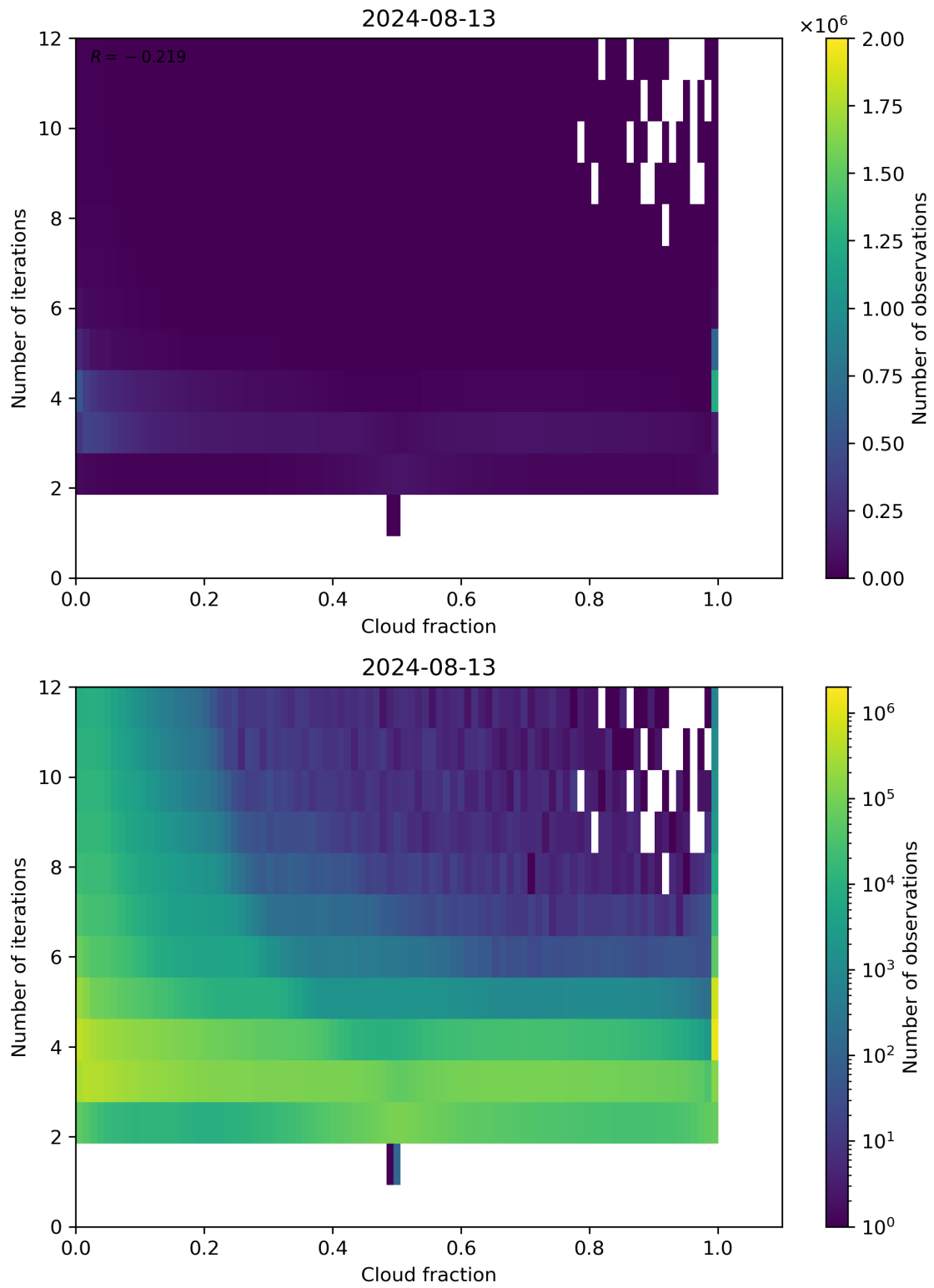
Figure 73: Scatter density plot of “Cloud fraction” against “Number of iterations” for 2024-08-12 to 2024-08-14.
