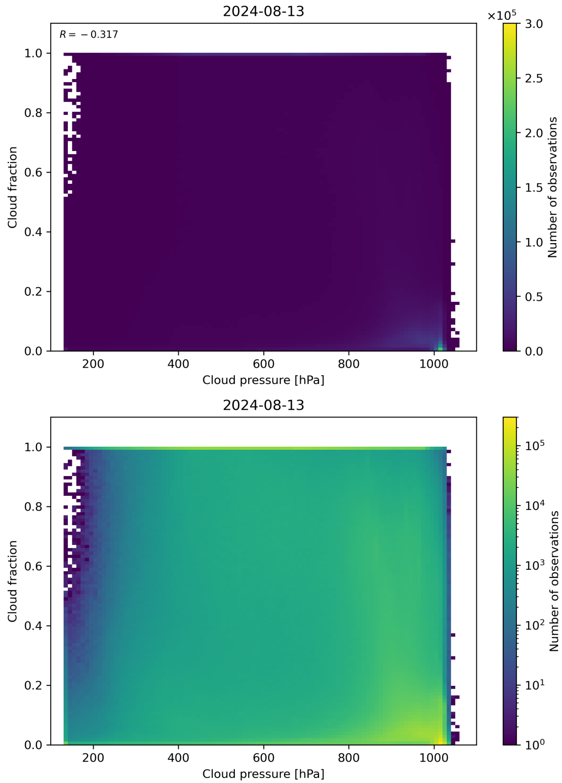
Figure 79: Scatter density plot of “Cloud pressure” against “Cloud fraction” for 2024-08-12 to 2024-08-14.
