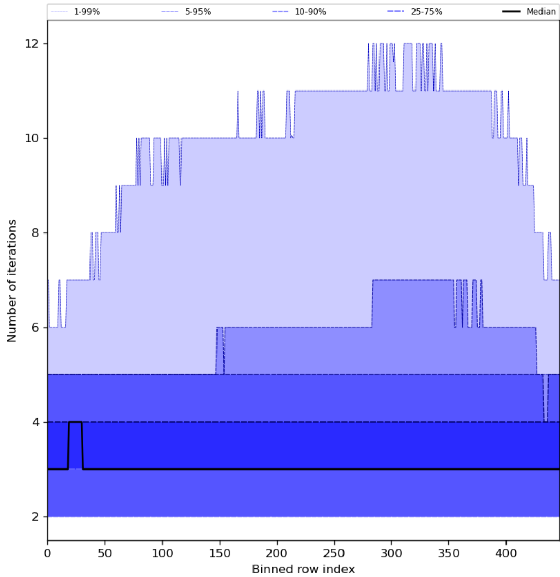
Figure 56: Along track statistics of “Number of iterations” for 2024-08-12 to 2024-08-14
