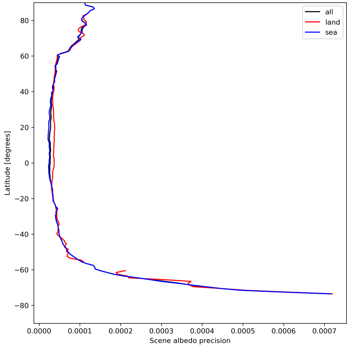
Figure 18: Zonal average of “Scene albedo precision” for 2024-08-12 to 2024-08-14.
