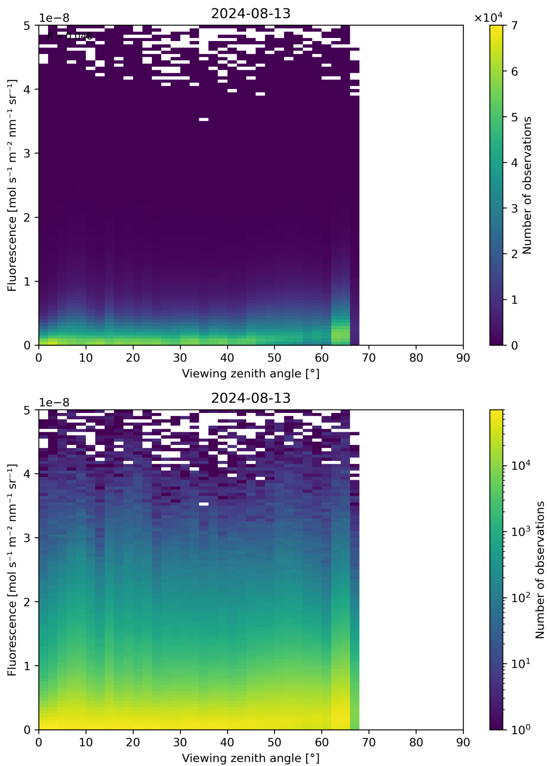
Figure 122: Scatter density plot of “Viewing zenith angle” against “Fluorescence” for 2024-08-12 to 2024-08-14.
