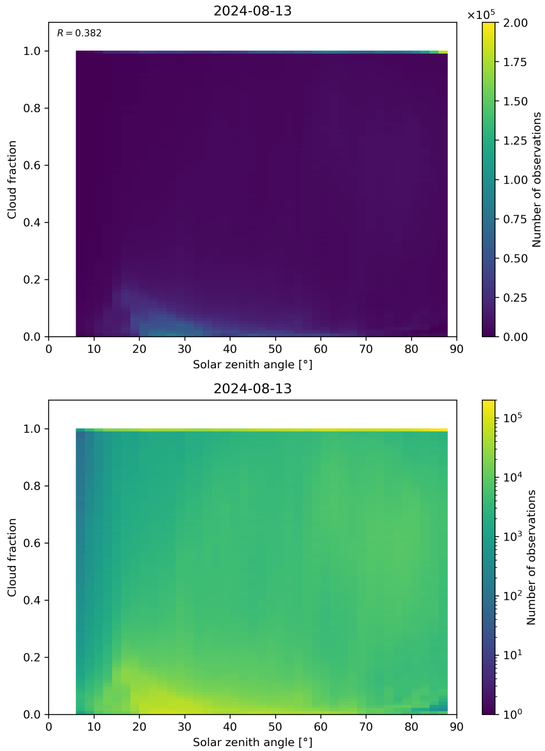
Figure 110: Scatter density plot of “Solar zenith angle” against “Cloud fraction” for 2024-08-12 to 2024-08-14.
