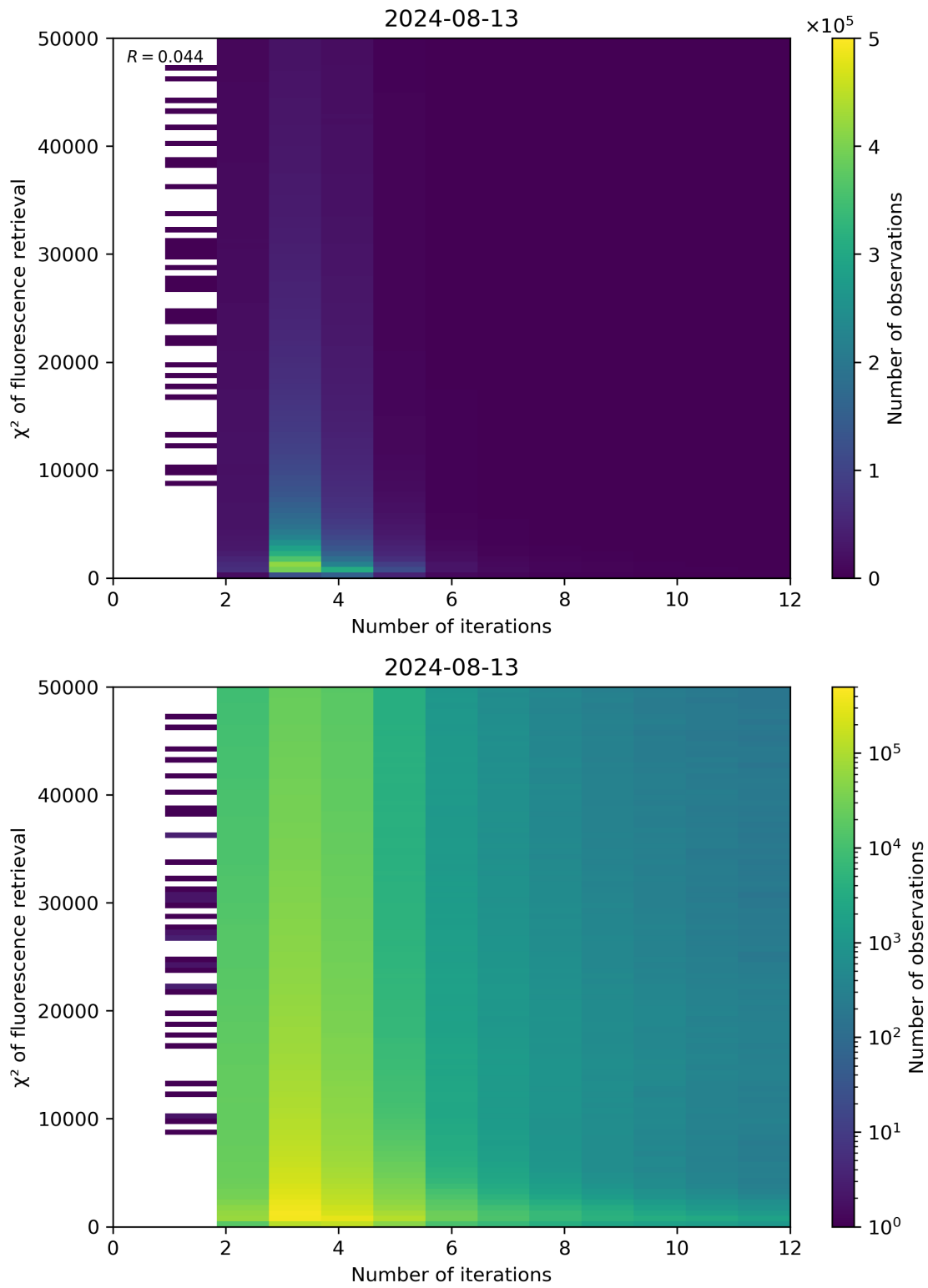
Figure 97: Scatter density plot of “Number of iterations” against “ \chi^2 of fluorescence retrieval” for 2024-08-12 to 2024-08-14.
