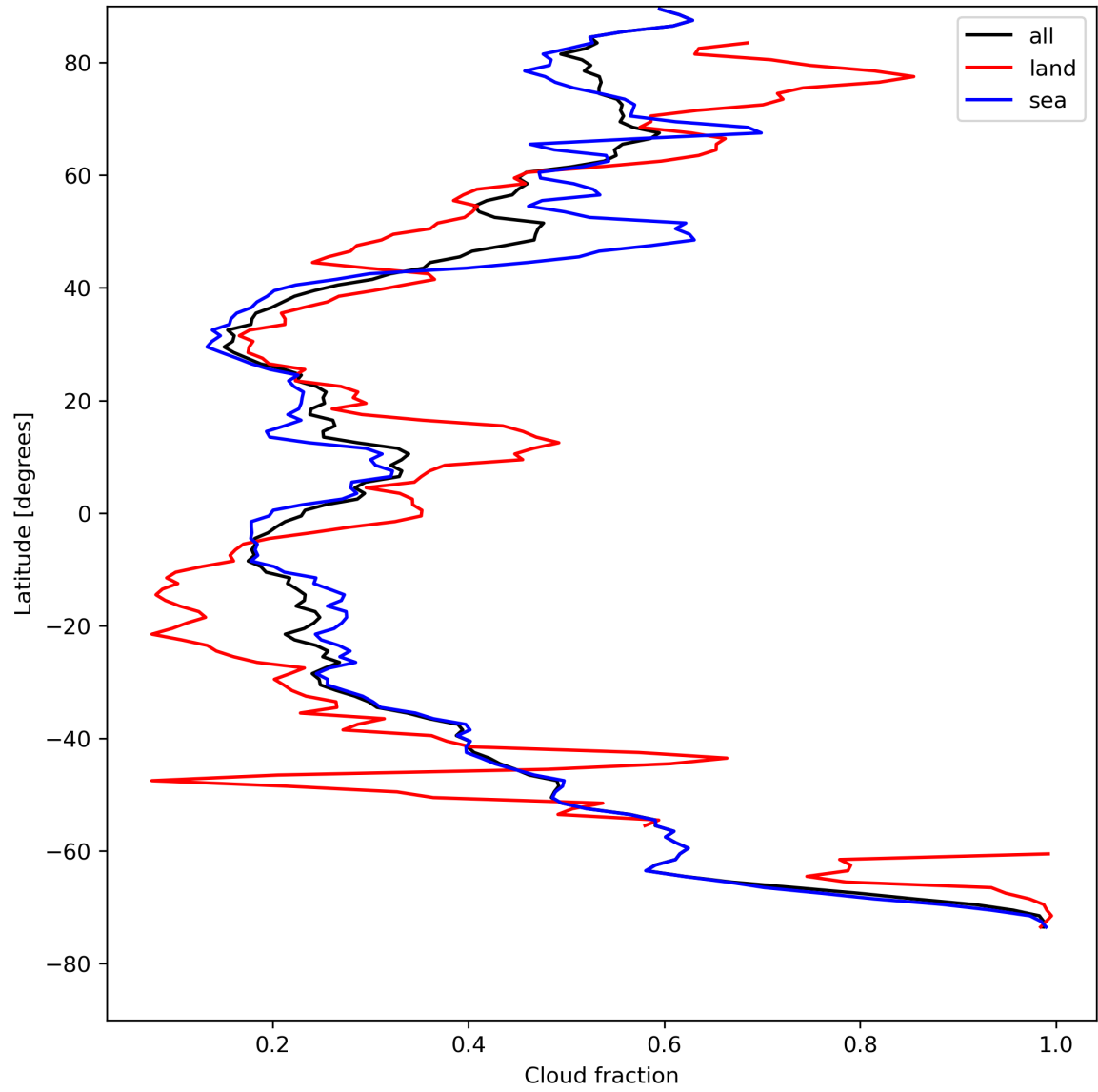
Figure 15: Zonal average of “Cloud fraction” for 2024-08-12 to 2024-08-14.
