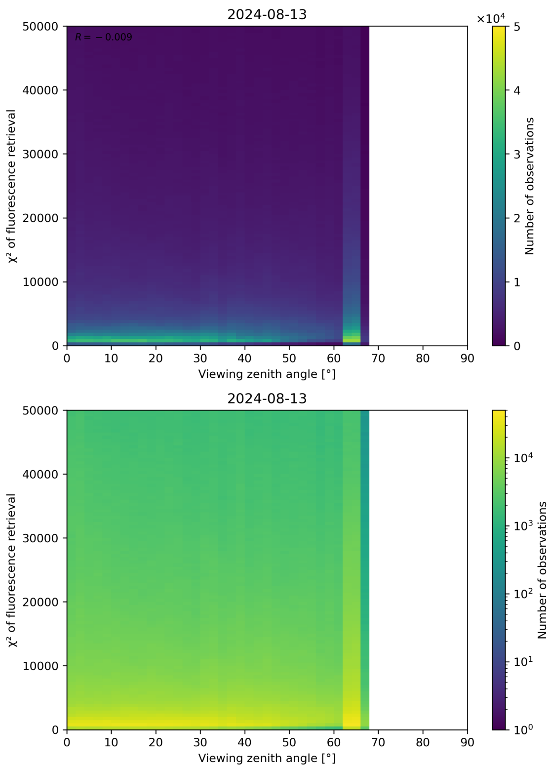
Figure 119: Scatter density plot of “Viewing zenith angle” against “ \chi^2 of fluorescence retrieval” for 2024-08-12 to 2024-08-14.
