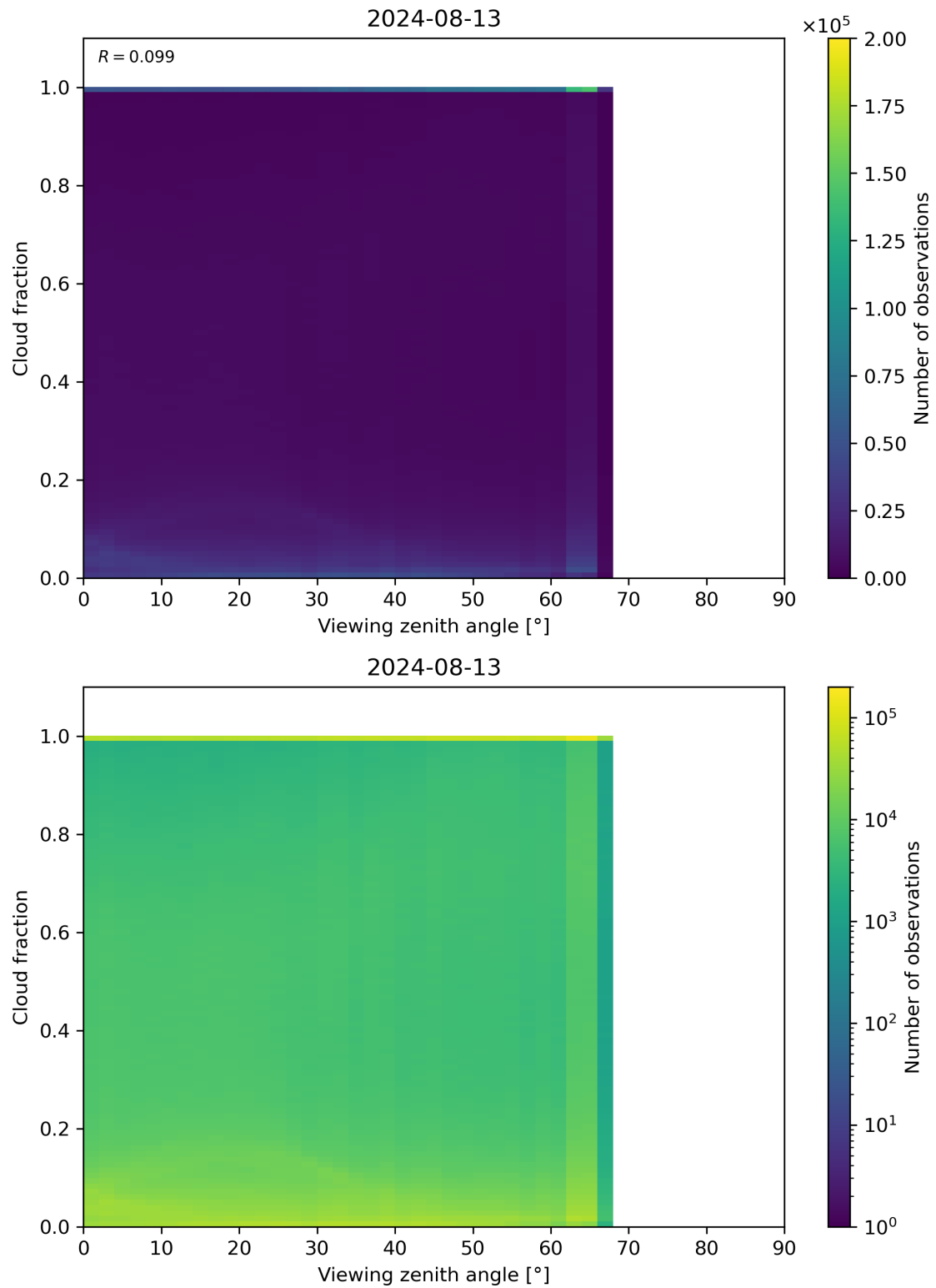
Figure 120: Scatter density plot of “Viewing zenith angle” against “Cloud fraction” for 2024-08-12 to 2024-08-14.
