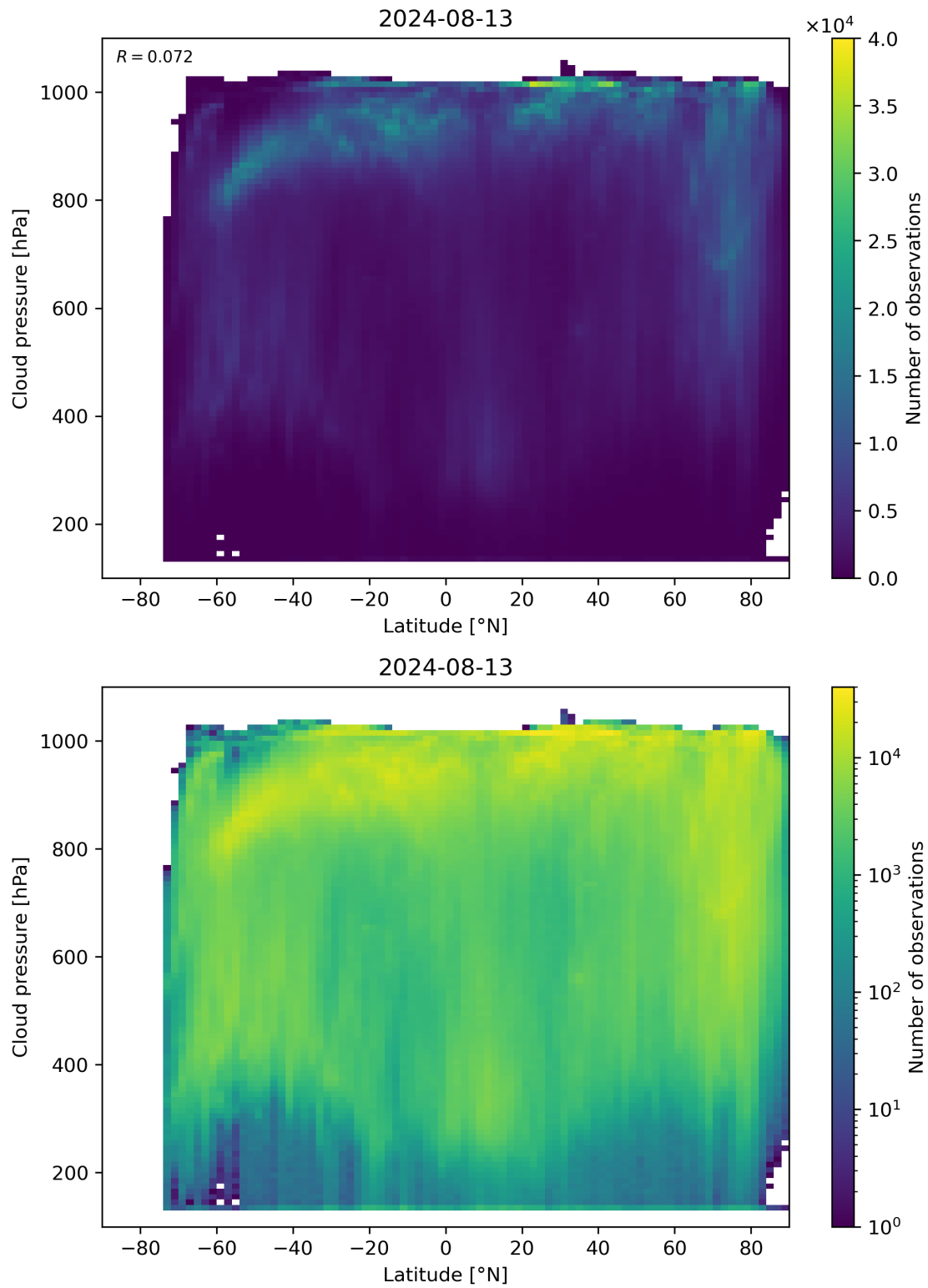
Figure 91: Scatter density plot of “Latitude” against “Cloud pressure” for 2024-08-12 to 2024-08-14.
