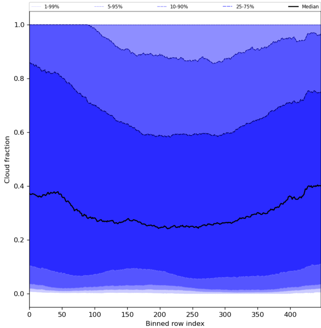
Figure 49: Along track statistics of “Cloud fraction” for 2024-08-12 to 2024-08-14
