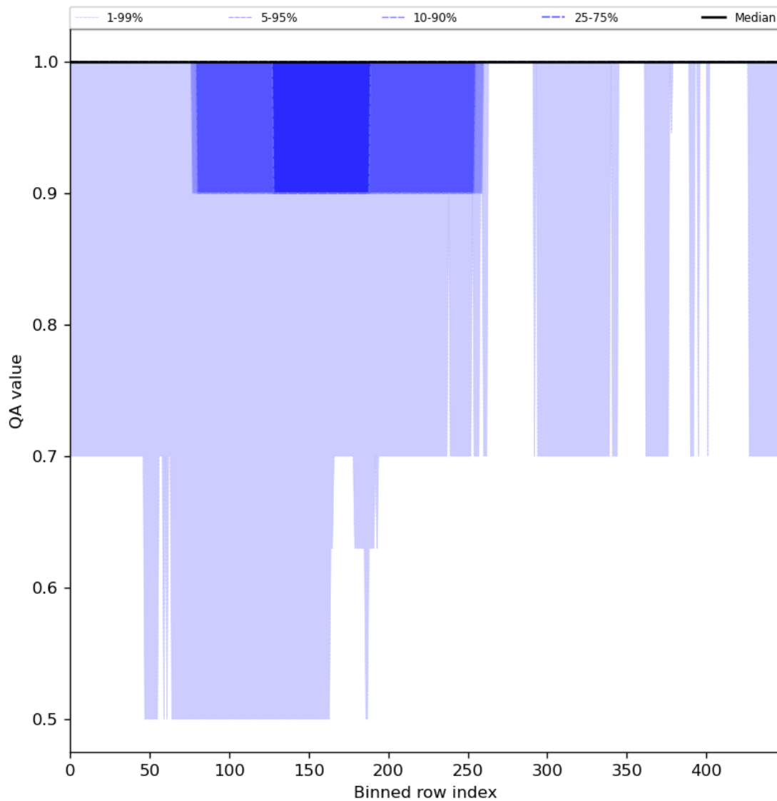
Figure 46: Along track statistics of “QA value” for 2024-08-12 to 2024-08-14
