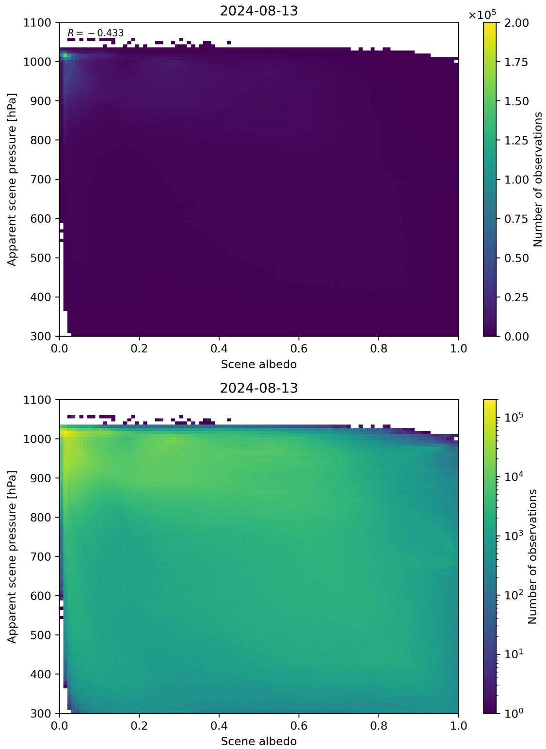
Figure 102: Scatter density plot of “Scene albedo” against “Apparent scene pressure” for 2024-08-12 to 2024-08-14.
