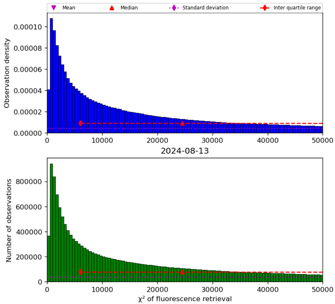
Figure 42: Histogram of “ \chi^2 of fluorescence retrieval” for 2024-08-12 to 2024-08-14
