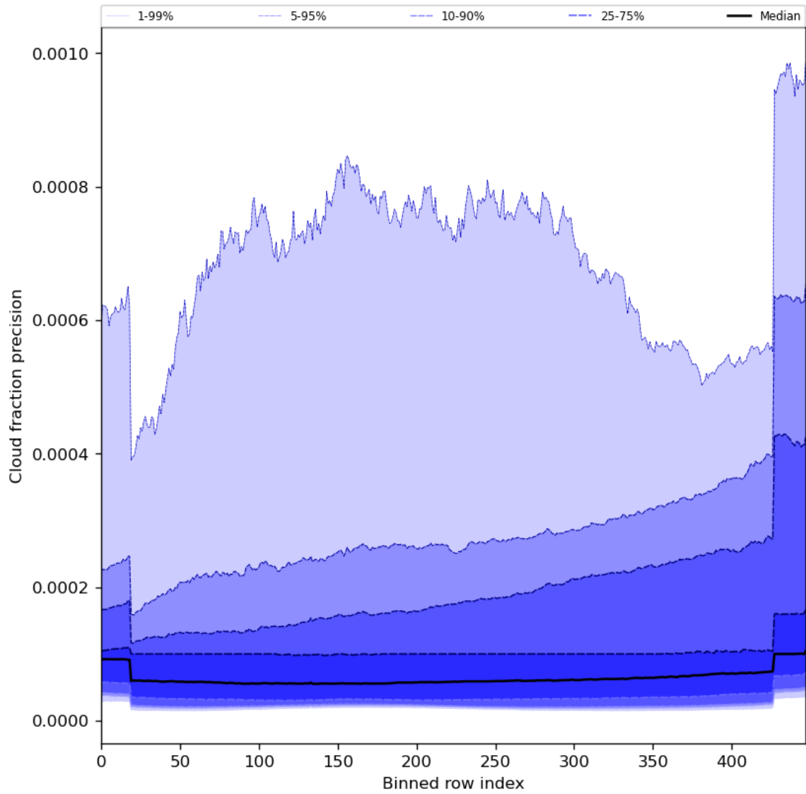
Figure 50: Along track statistics of “Cloud fraction precision” for 2024-08-12 to 2024-08-14
