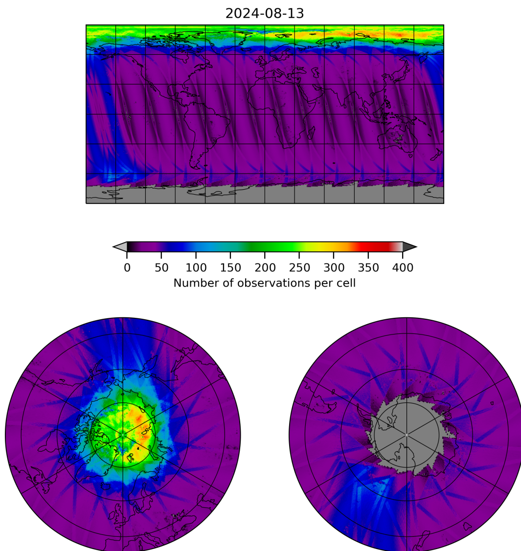
Figure 11: Map of the number of observations for 2024-08-12 to 2024-08-14
