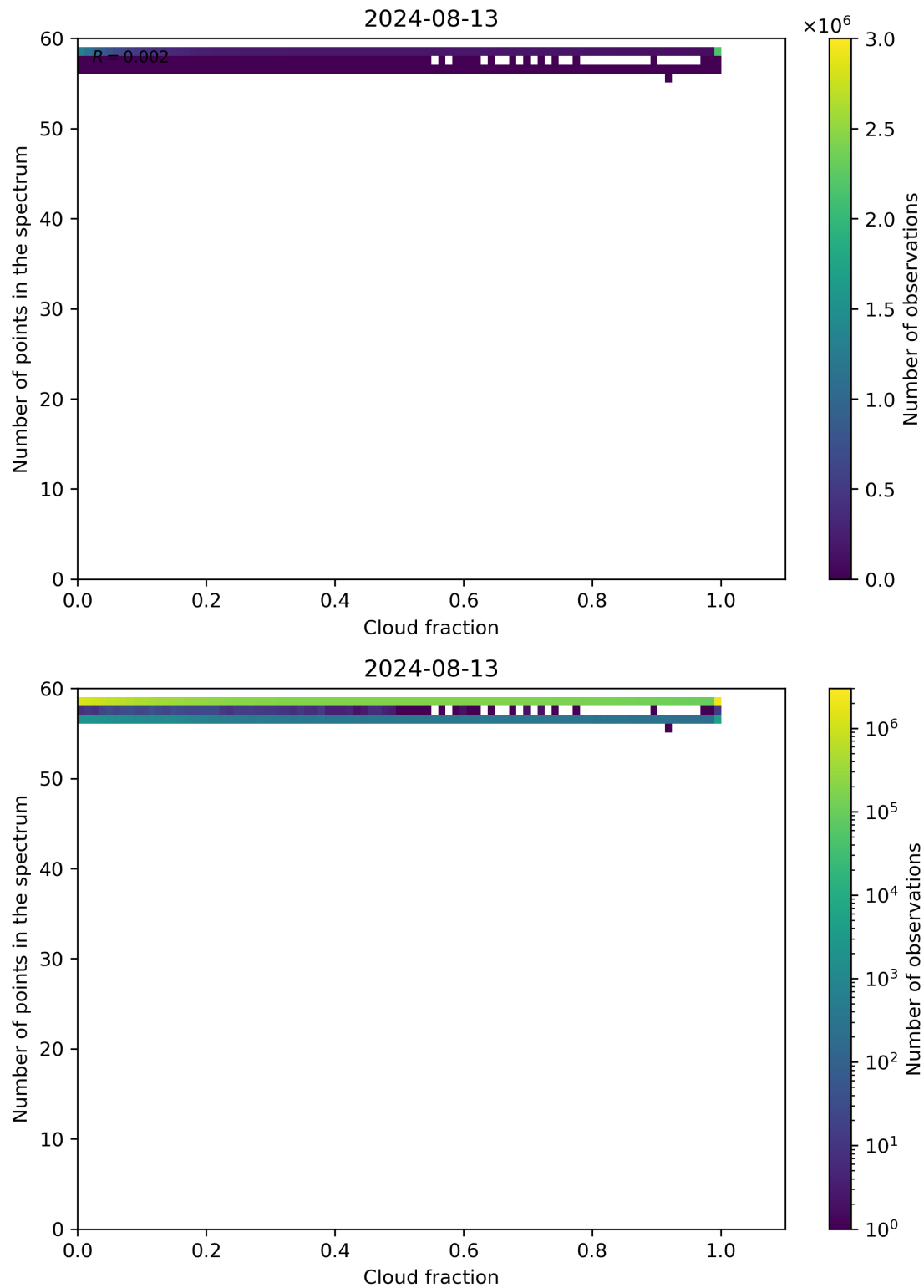
Figure 74: Scatter density plot of “Cloud fraction” against “Number of points in the spectrum” for 2024-08-12 to 2024-08-14.
