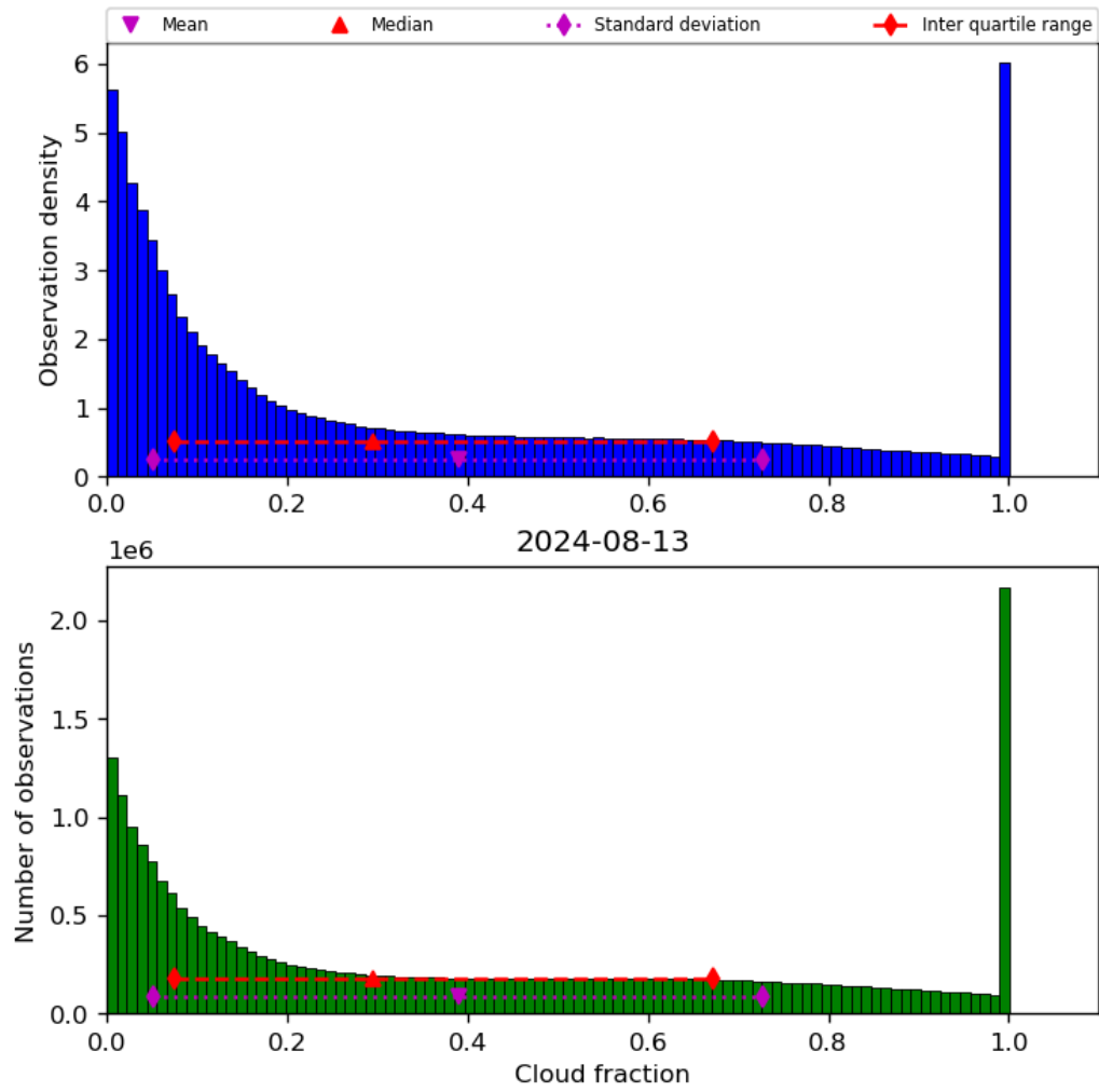
Figure 32: Histogram of “Cloud fraction” for 2024-08-12 to 2024-08-14
