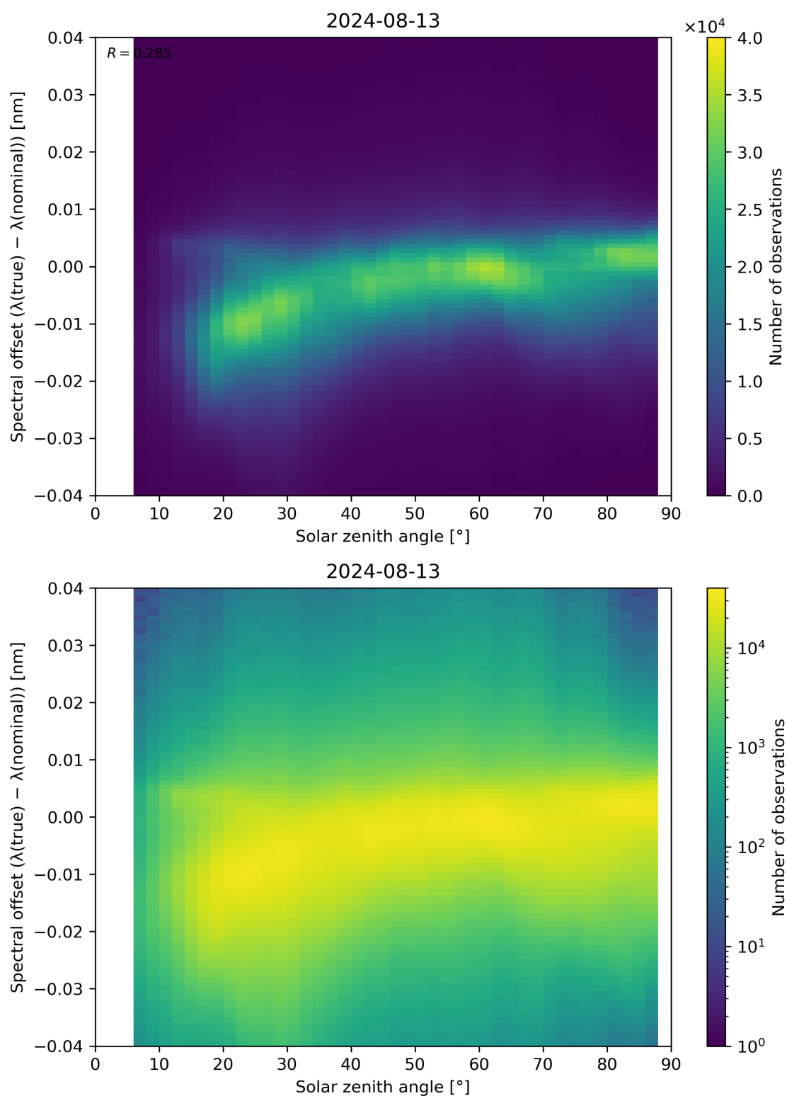
Figure 117: Scatter density plot of “Solar zenith angle” against “Spectral offset ( \lambda(\text{true}) - \lambda(\text{nominal}) )” for 2024-08-12 to 2024-08-14.
