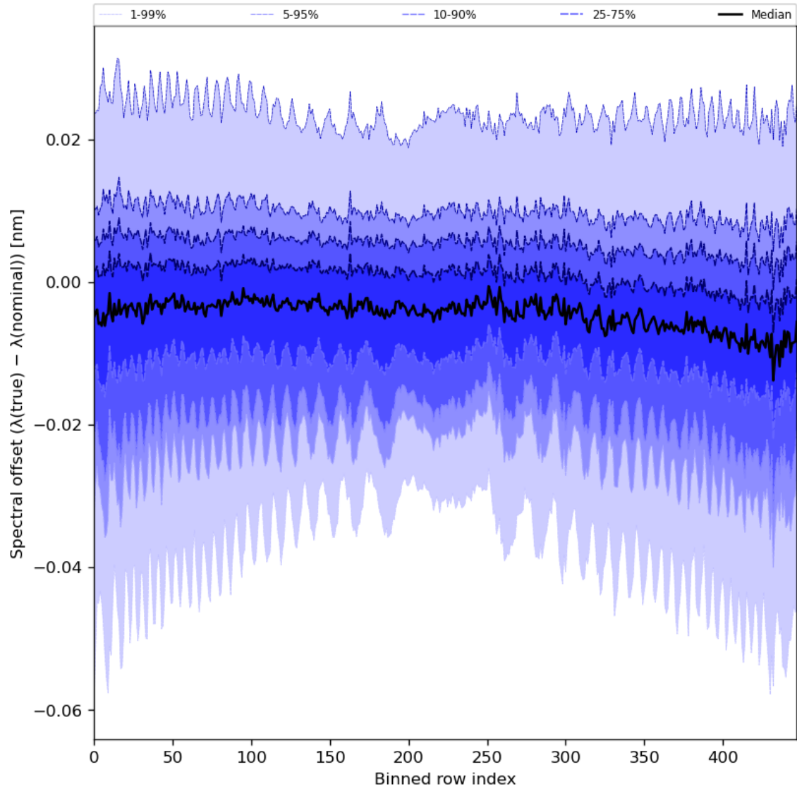
Figure 62: Along track statistics of “Spectral offset ( \lambda(\text{true}) - \lambda(\text{nominal}) )” for 2024-08-12 to 2024-08-14
