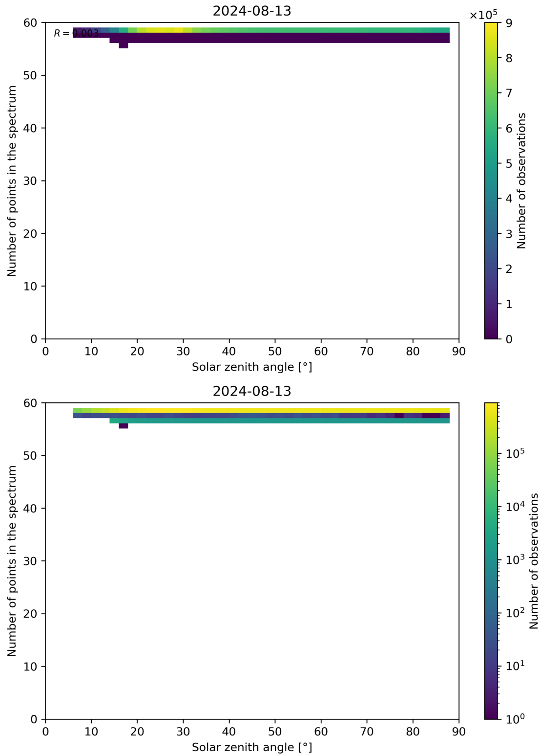
Figure 115: Scatter density plot of “Solar zenith angle” against “Number of points in the spectrum” for 2024-08-12 to 2024-08-14.
