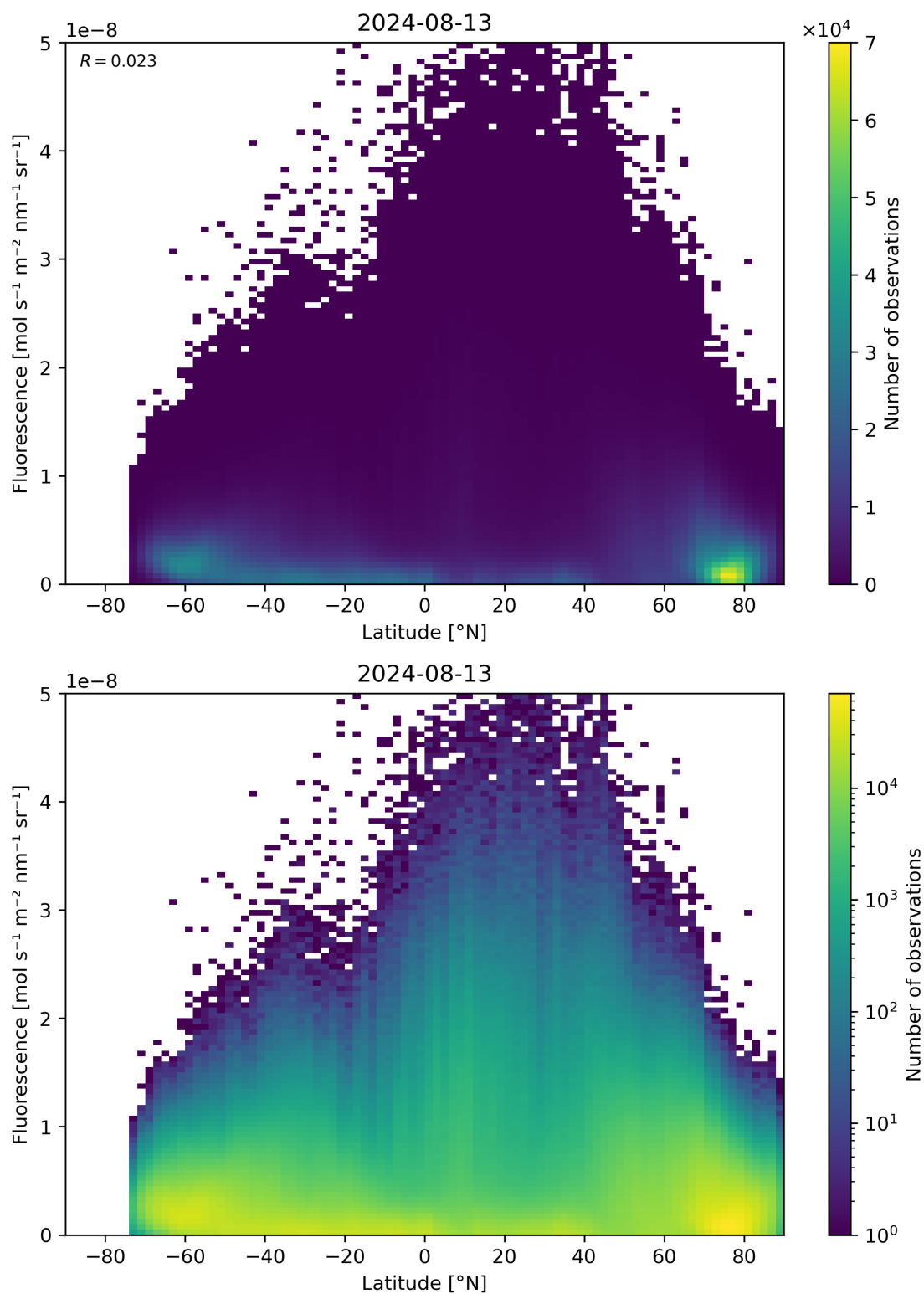
Figure 92: Scatter density plot of “Latitude” against “Fluorescence” for 2024-08-12 to 2024-08-14.
