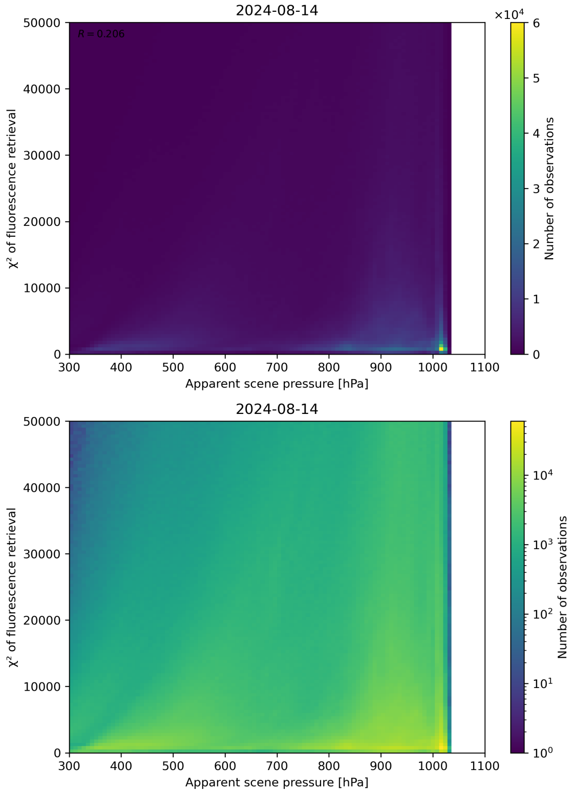
Figure 63: Scatter density plot of “Apparent scene pressure” against “ \chi^2 of fluorescence retrieval” for 2024-08-13 to 2024-08-15.
