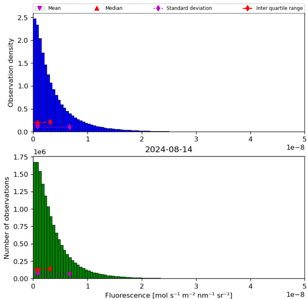
Figure 40: Histogram of “Fluorescence” for 2024-08-13 to 2024-08-15
