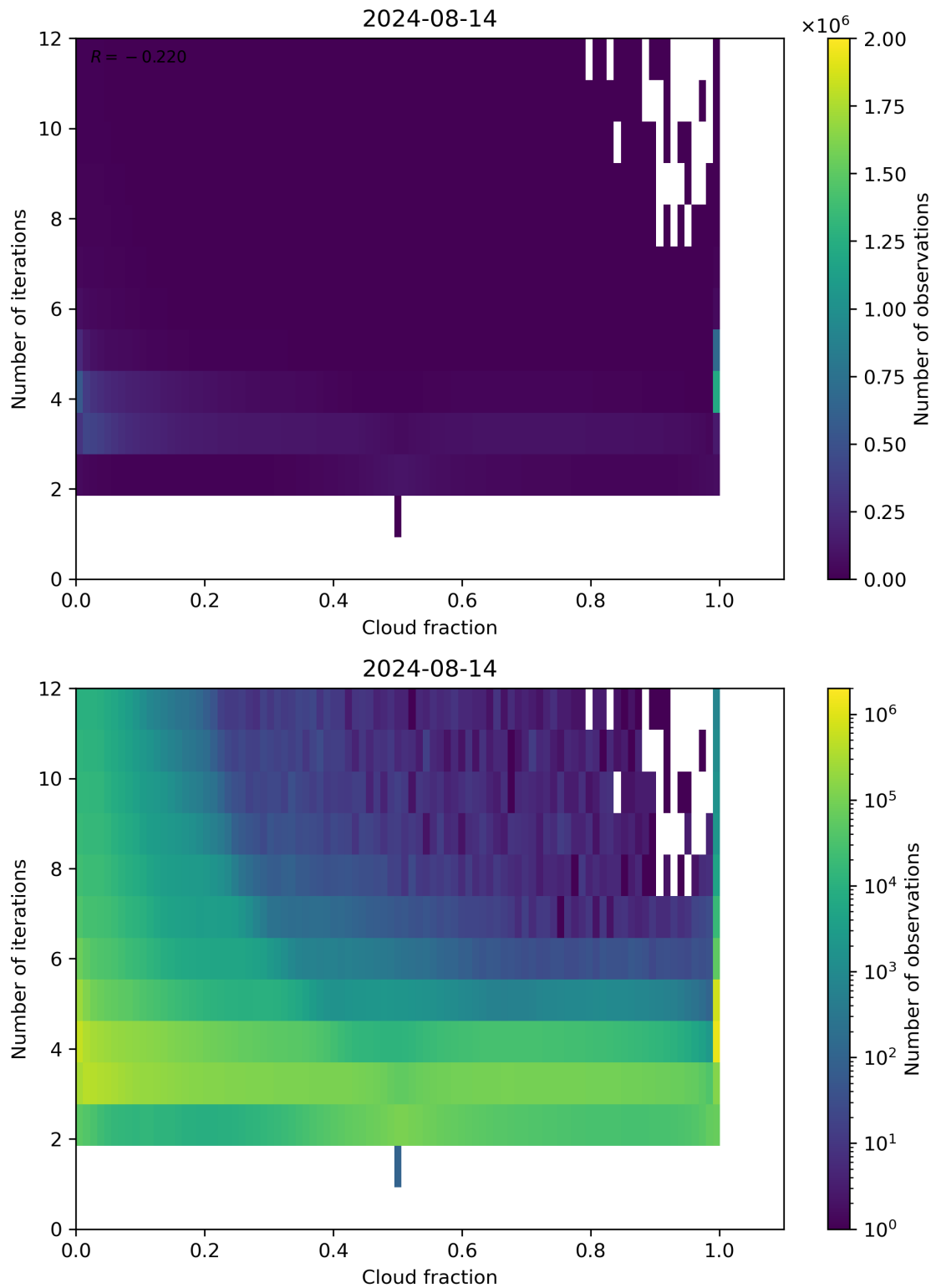
Figure 73: Scatter density plot of “Cloud fraction” against “Number of iterations” for 2024-08-13 to 2024-08-15.
