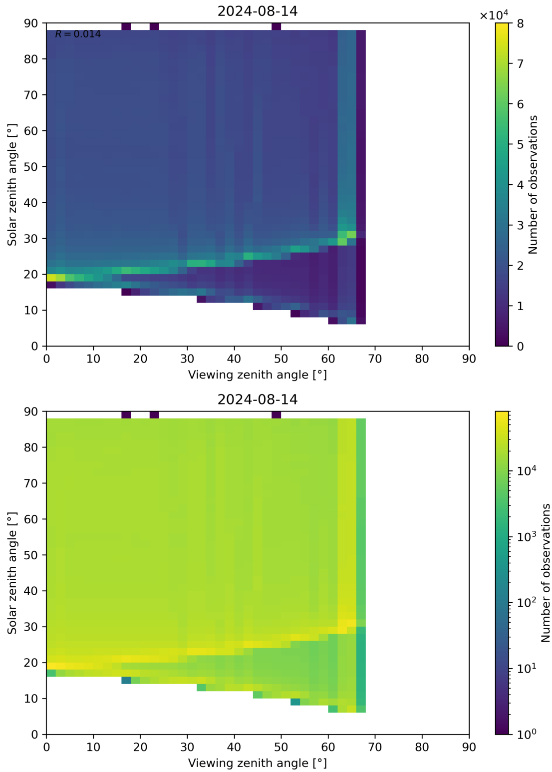
Figure 127: Scatter density plot of “Viewing zenith angle” against “Solar zenith angle” for 2024-08-13 to 2024-08-15.
