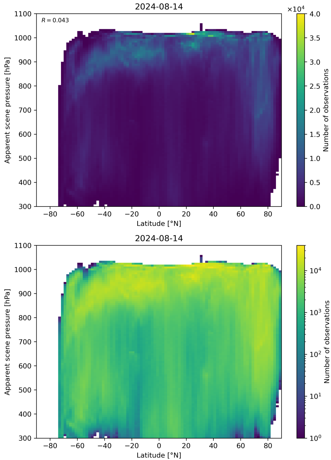
Figure 88: Scatter density plot of “Latitude” against “Apparent scene pressure” for 2024-08-13 to 2024-08-15.
