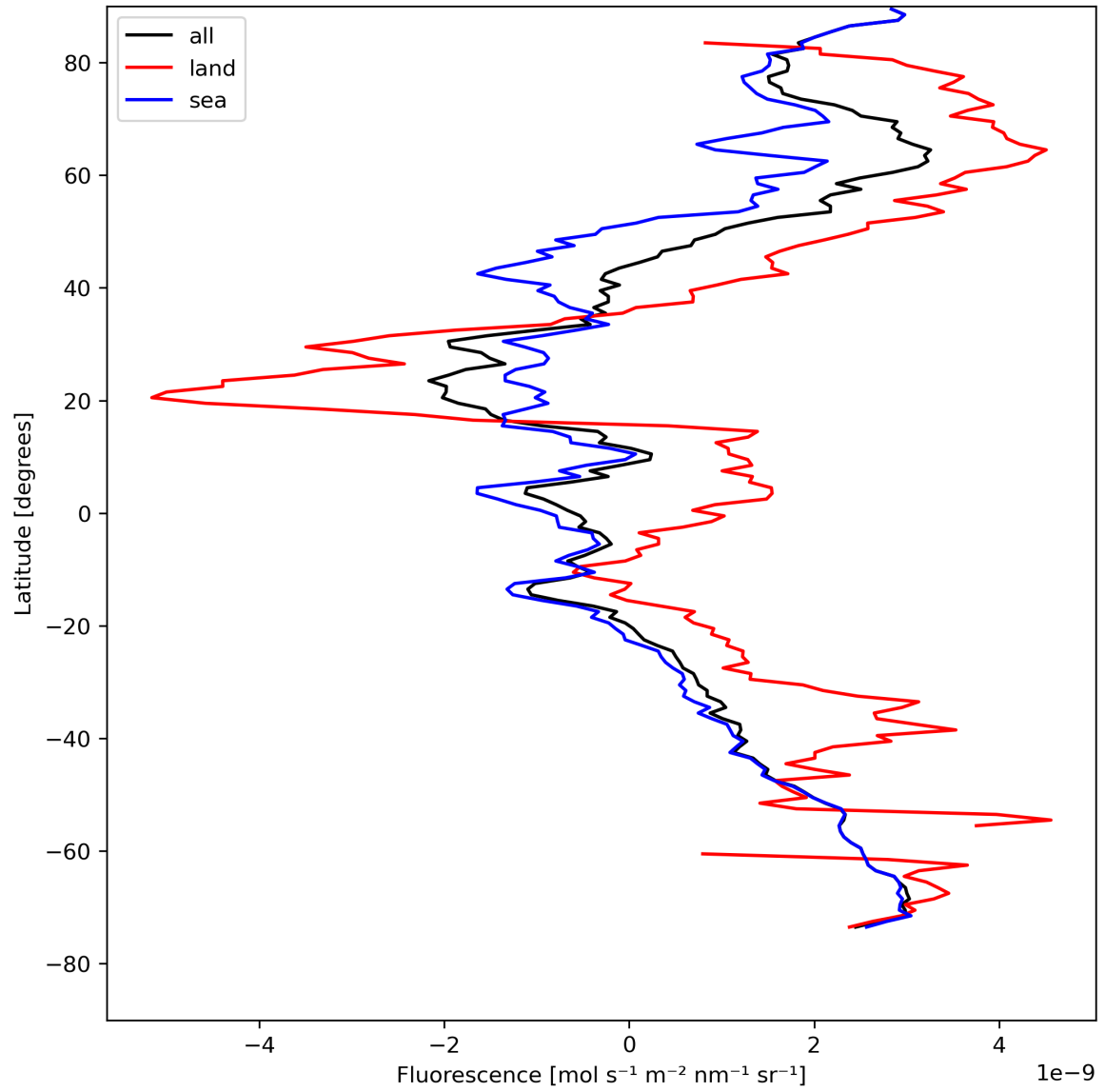
Figure 23: Zonal average of “Fluorescence” for 2024-08-13 to 2024-08-15.
