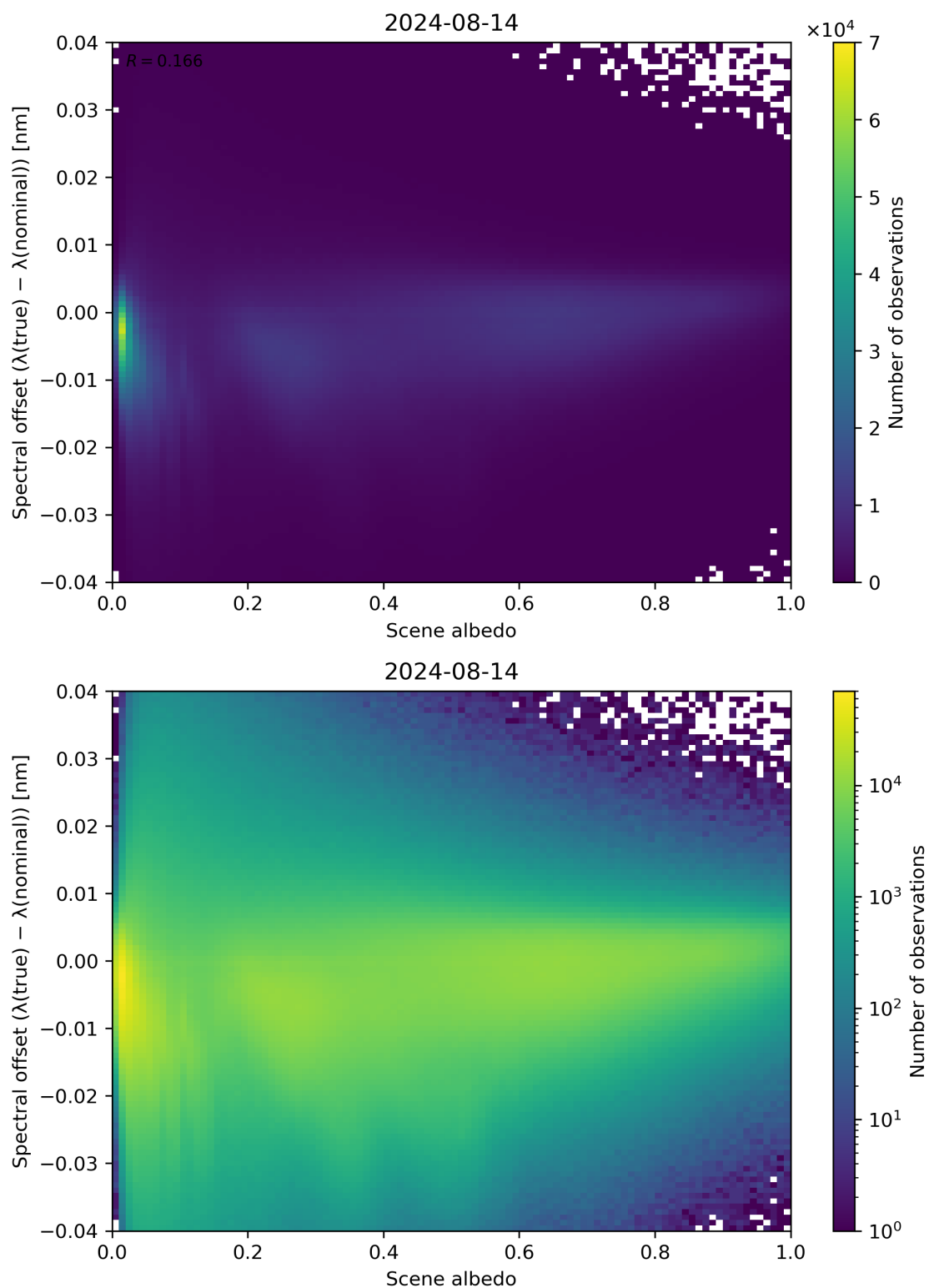
Figure 107: Scatter density plot of “Scene albedo” against “Spectral offset ( \lambda(\text{true}) - \lambda(\text{nominal}) )” for 2024-08-13 to 2024-08-15.
