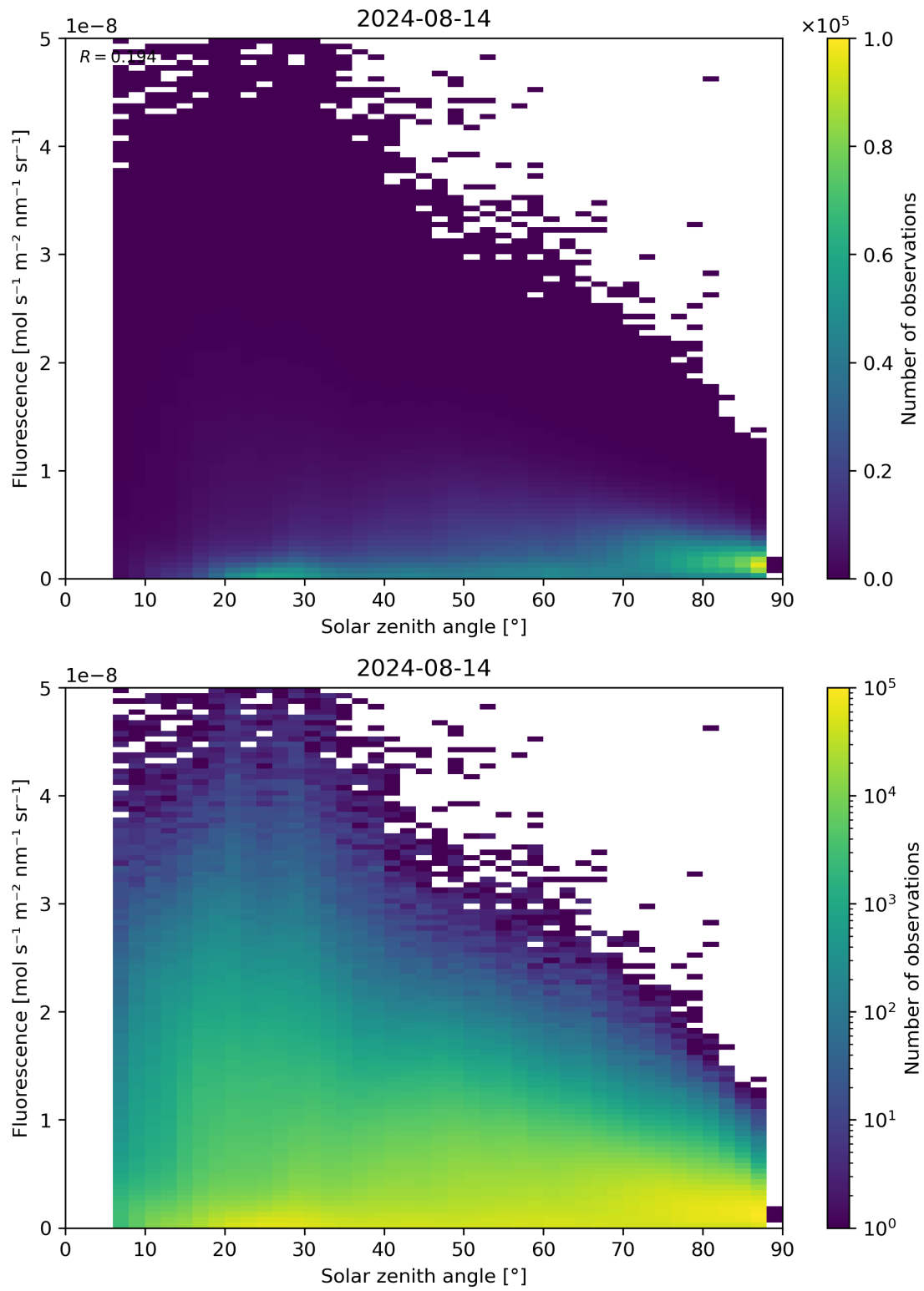
Figure 112: Scatter density plot of “Solar zenith angle” against “Fluorescence” for 2024-08-13 to 2024-08-15.
