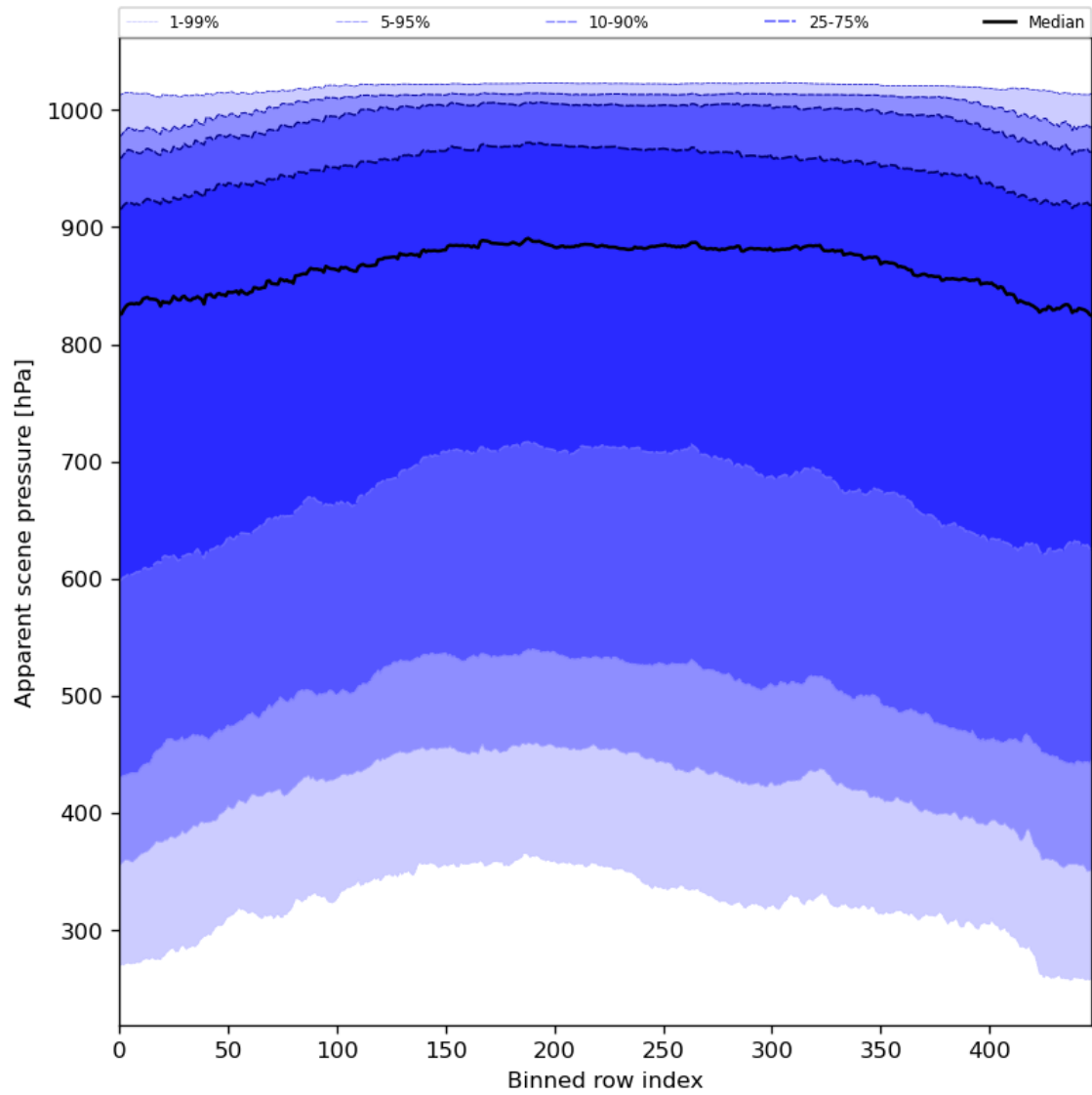
Figure 53: Along track statistics of “Apparent scene pressure” for 2024-08-13 to 2024-08-15
