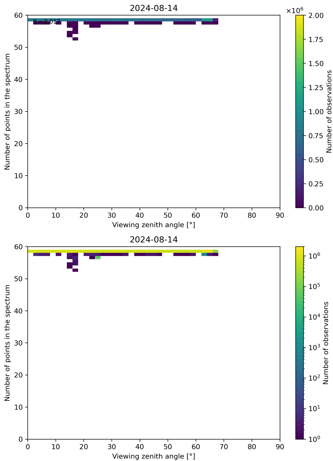
Figure 125: Scatter density plot of “Viewing zenith angle” against “Number of points in the spectrum” for 2024-08-13 to 2024-08-15.
