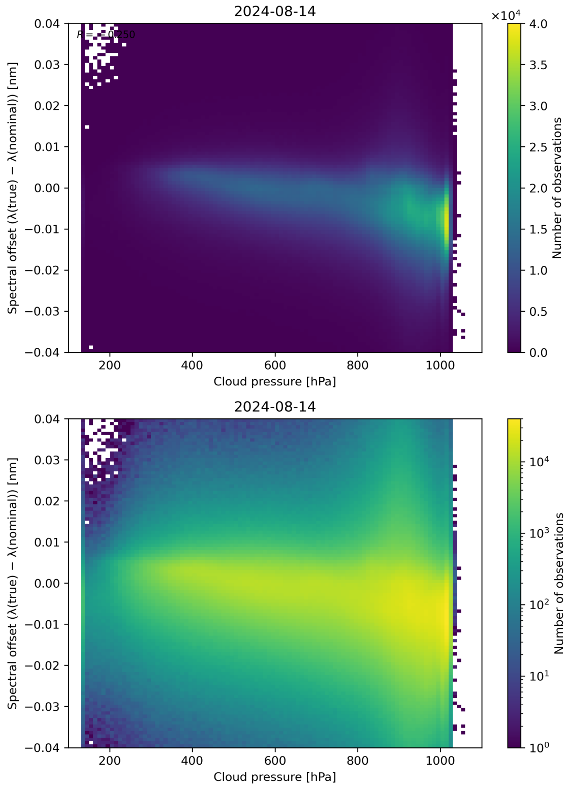
Figure 84: Scatter density plot of “Cloud pressure” against “Spectral offset ( \lambda(\text{true}) - \lambda(\text{nominal}) )” for 2024-08-13 to 2024-08-15.
