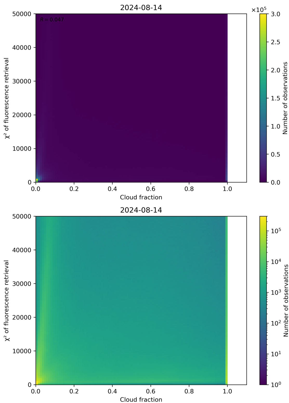
Figure 71: Scatter density plot of “Cloud fraction” against “ \chi^2 of fluorescence retrieval” for 2024-08-13 to 2024-08-15.
