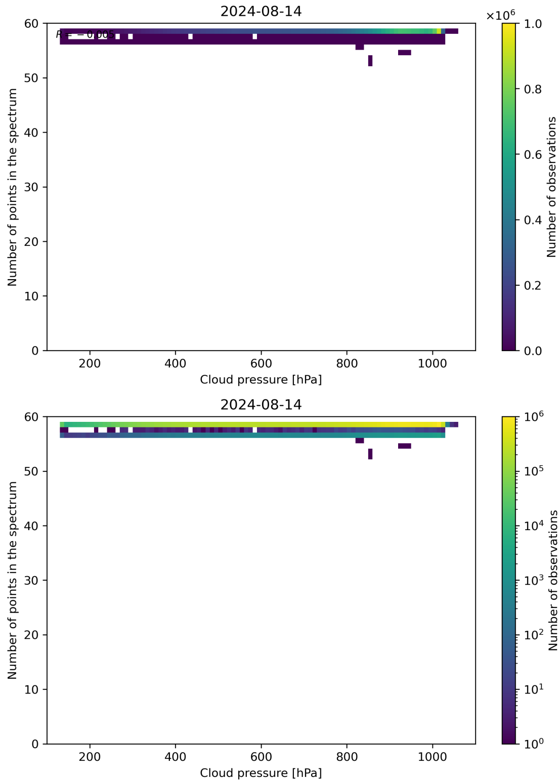
Figure 82: Scatter density plot of “Cloud pressure” against “Number of points in the spectrum” for 2024-08-13 to 2024-08-15.
