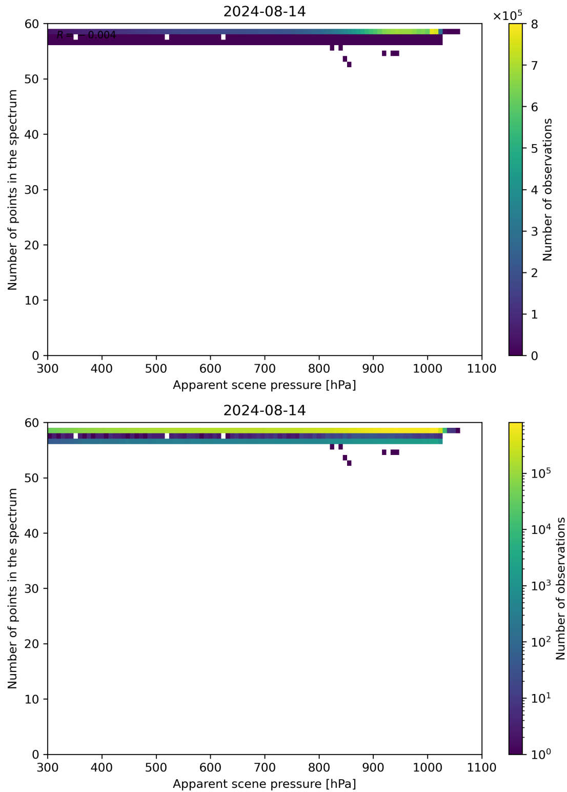
Figure 66: Scatter density plot of “Apparent scene pressure” against “Number of points in the spectrum” for 2024-08-13 to 2024-08-15.
