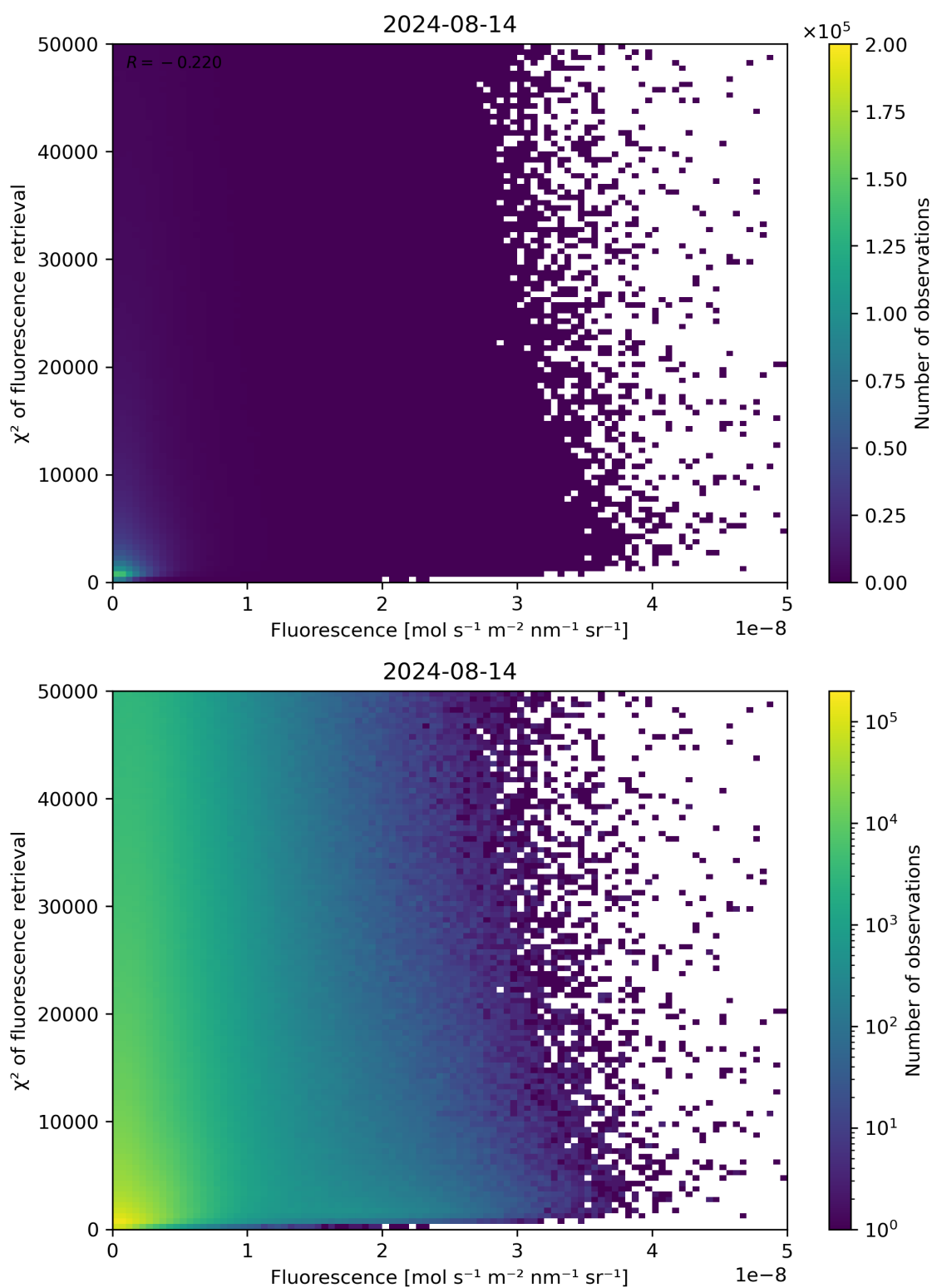
Figure 85: Scatter density plot of “Fluorescence” against “ \chi^2 of fluorescence retrieval” for 2024-08-13 to 2024-08-15.
