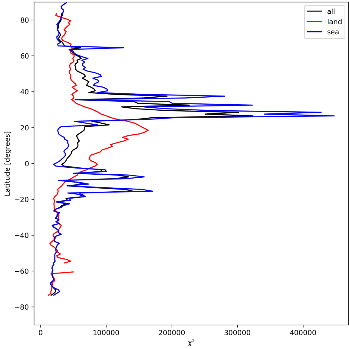
Figure 21: Zonal average of “ \chi^2 ” for 2024-08-13 to 2024-08-15.
