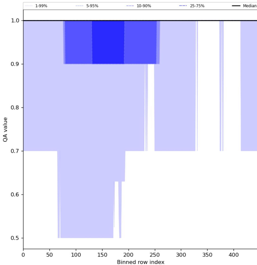
Figure 46: Along track statistics of “QA value” for 2024-08-13 to 2024-08-15
