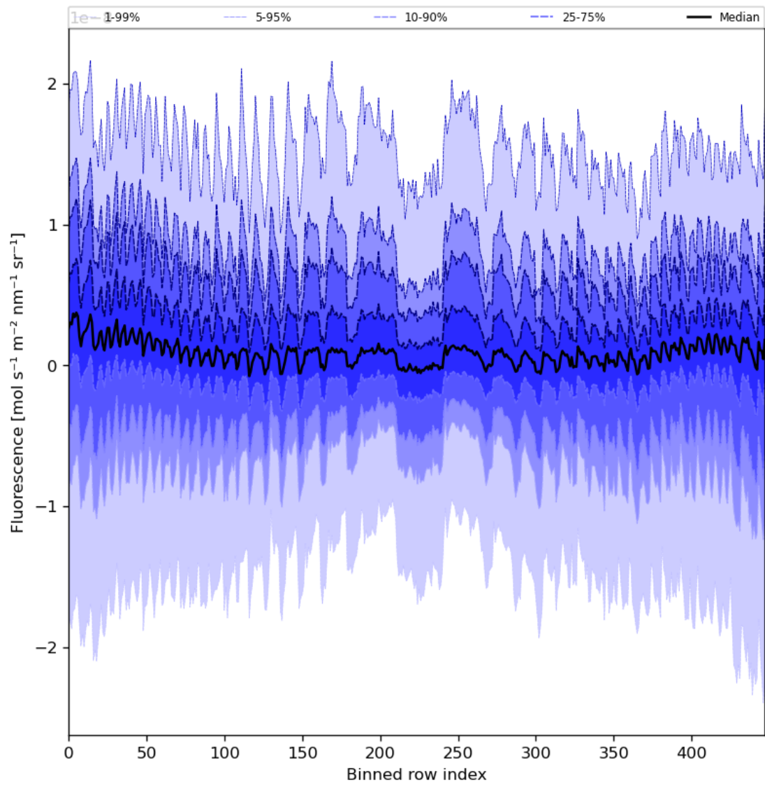
Figure 57: Along track statistics of "Fluorescence" for 2024-08-13 to 2024-08-15
