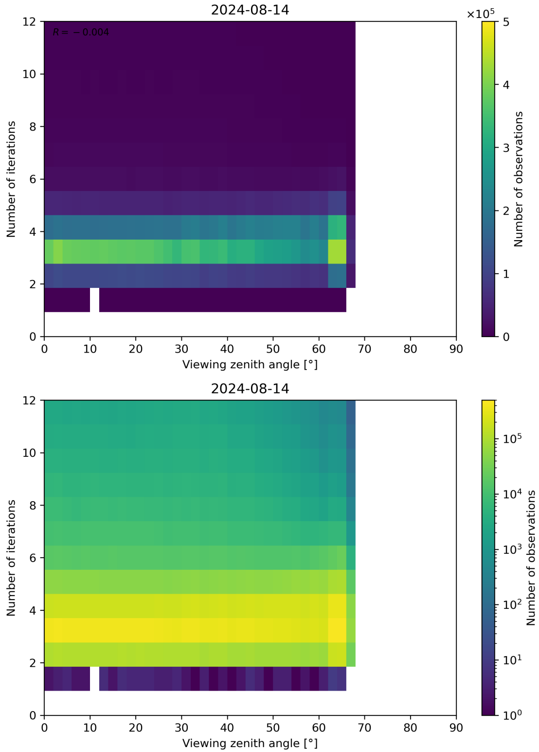
Figure 124: Scatter density plot of “Viewing zenith angle” against “Number of iterations” for 2024-08-13 to 2024-08-15.
