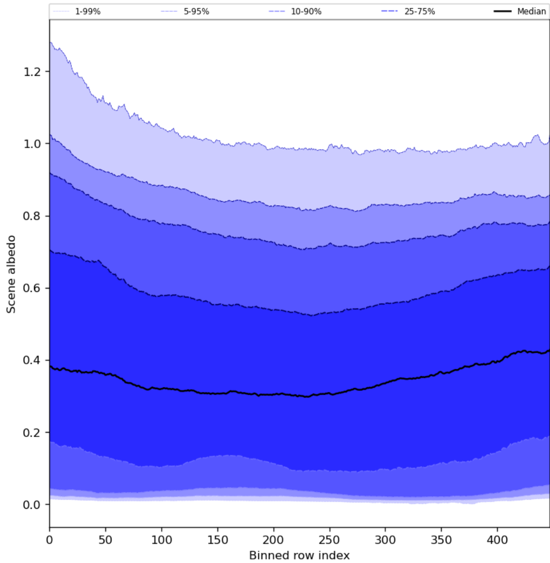
Figure 51: Along track statistics of “Scene albedo” for 2024-08-13 to 2024-08-15
