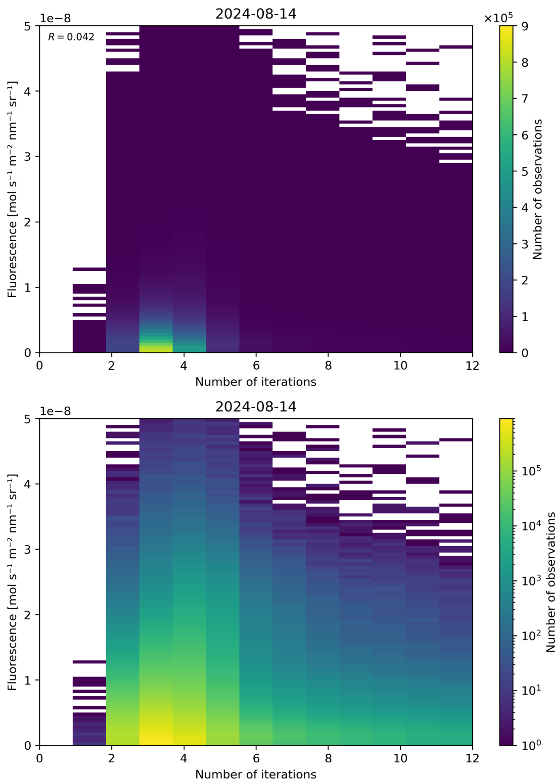
Figure 98: Scatter density plot of “Number of iterations” against “Fluorescence” for 2024-08-13 to 2024-08-15.
