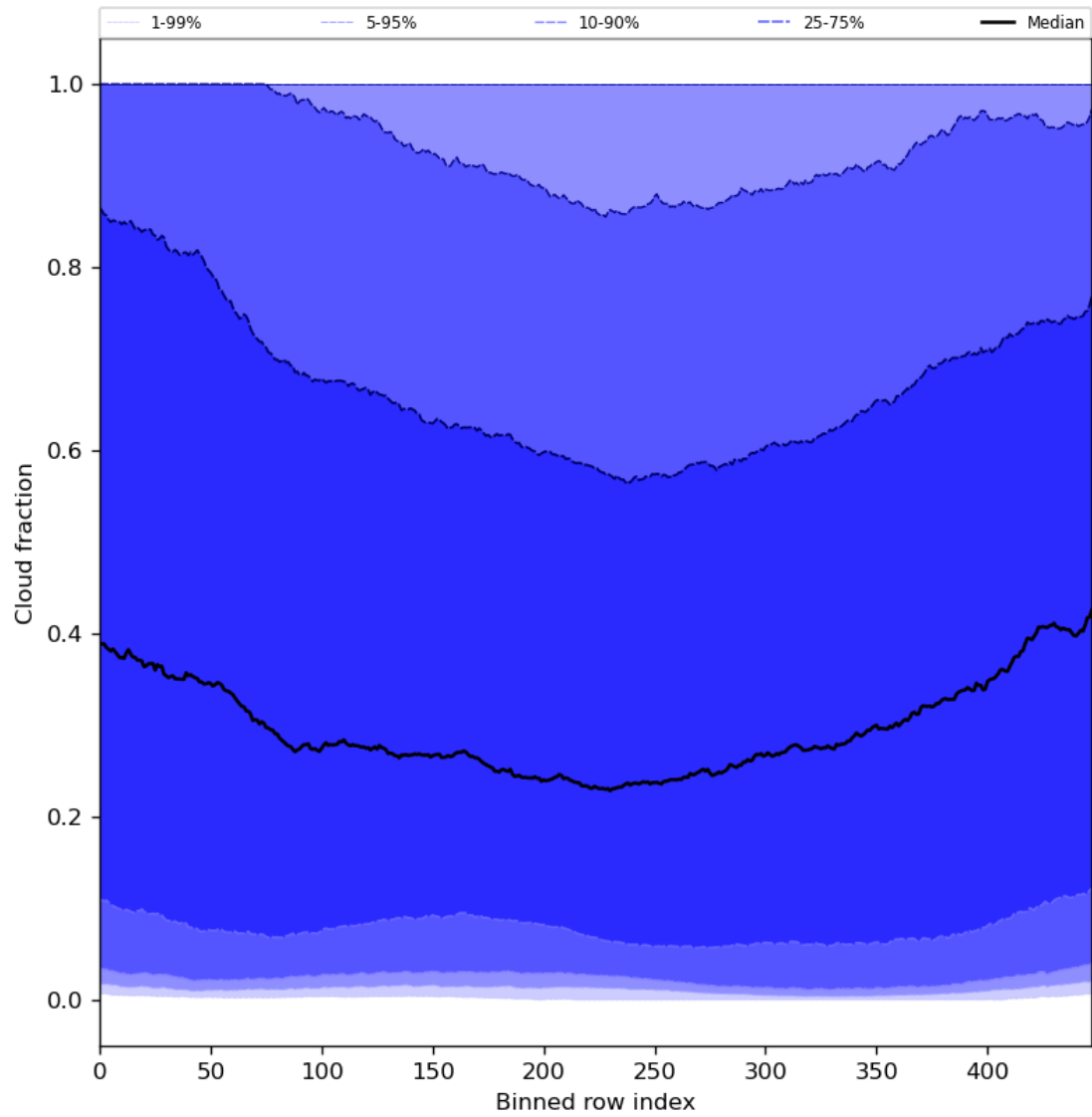
Figure 49: Along track statistics of “Cloud fraction” for 2024-08-13 to 2024-08-15
