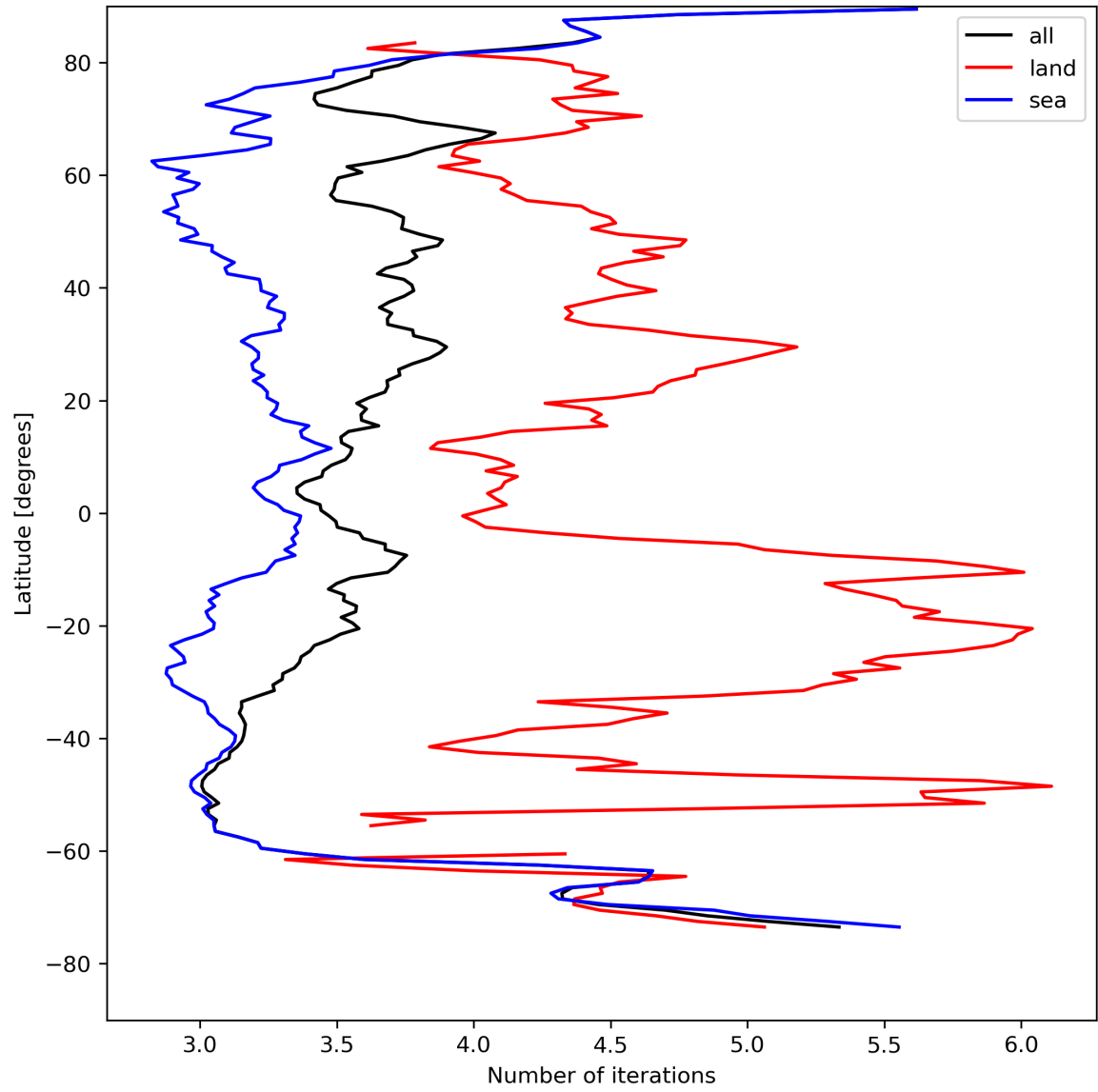
Figure 22: Zonal average of “Number of iterations” for 2024-08-13 to 2024-08-15.
