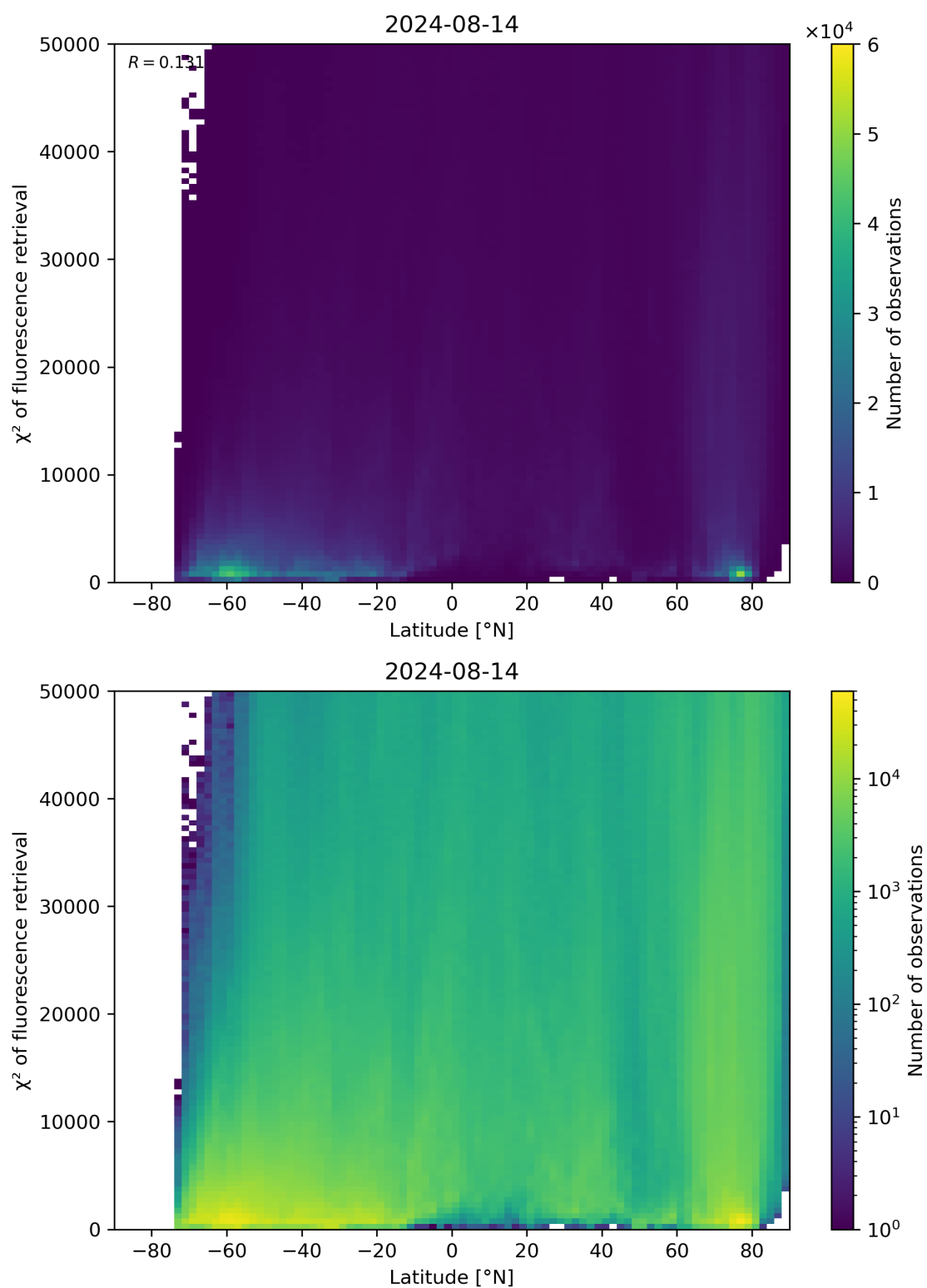
Figure 89: Scatter density plot of “Latitude” against “ \chi^2 of fluorescence retrieval” for 2024-08-13 to 2024-08-15.
