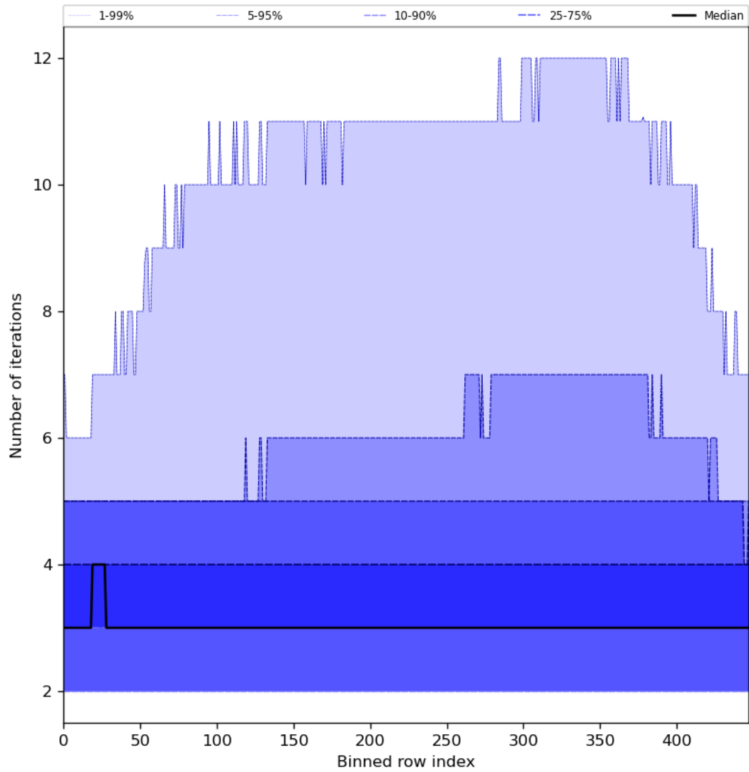
Figure 56: Along track statistics of “Number of iterations” for 2024-08-13 to 2024-08-15
