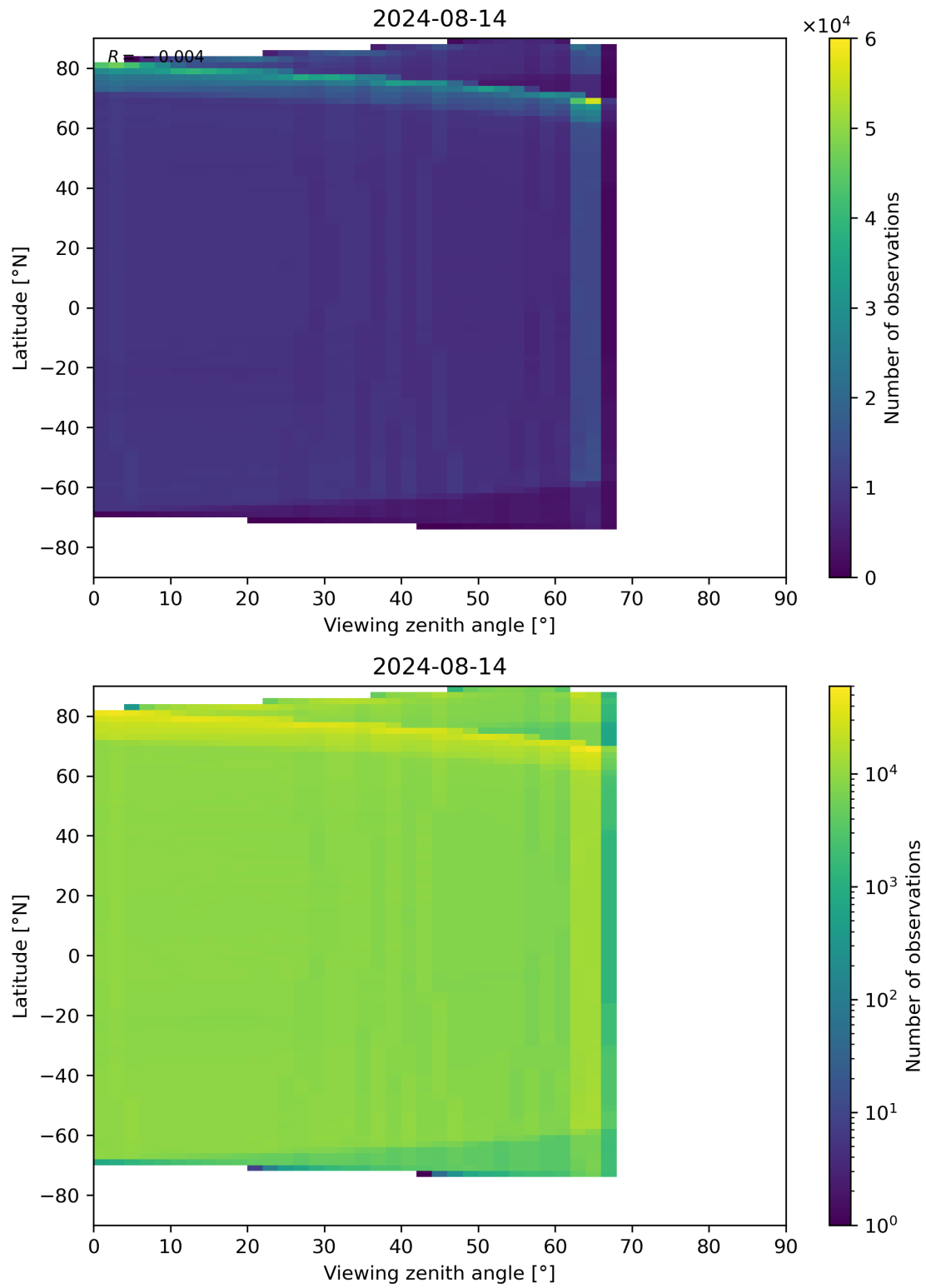
Figure 123: Scatter density plot of “Viewing zenith angle” against “Latitude” for 2024-08-13 to 2024-08-15.
