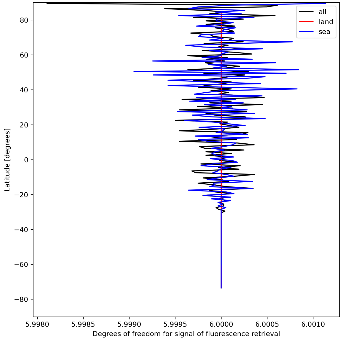
Figure 26: Zonal average of “Degrees of freedom for signal of fluorescence retrieval” for 2024-08-13 to 2024-08-15.
