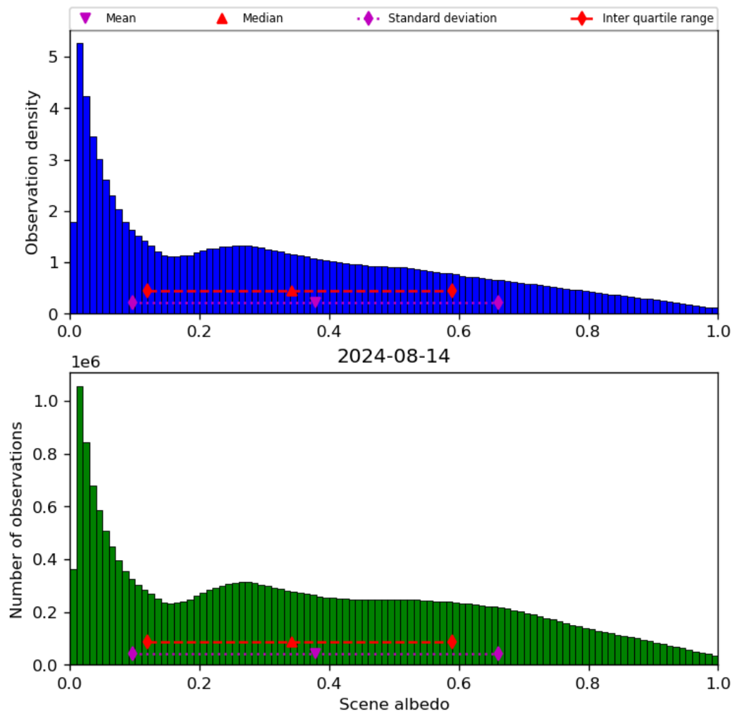
Figure 34: Histogram of “Scene albedo” for 2024-08-13 to 2024-08-15
