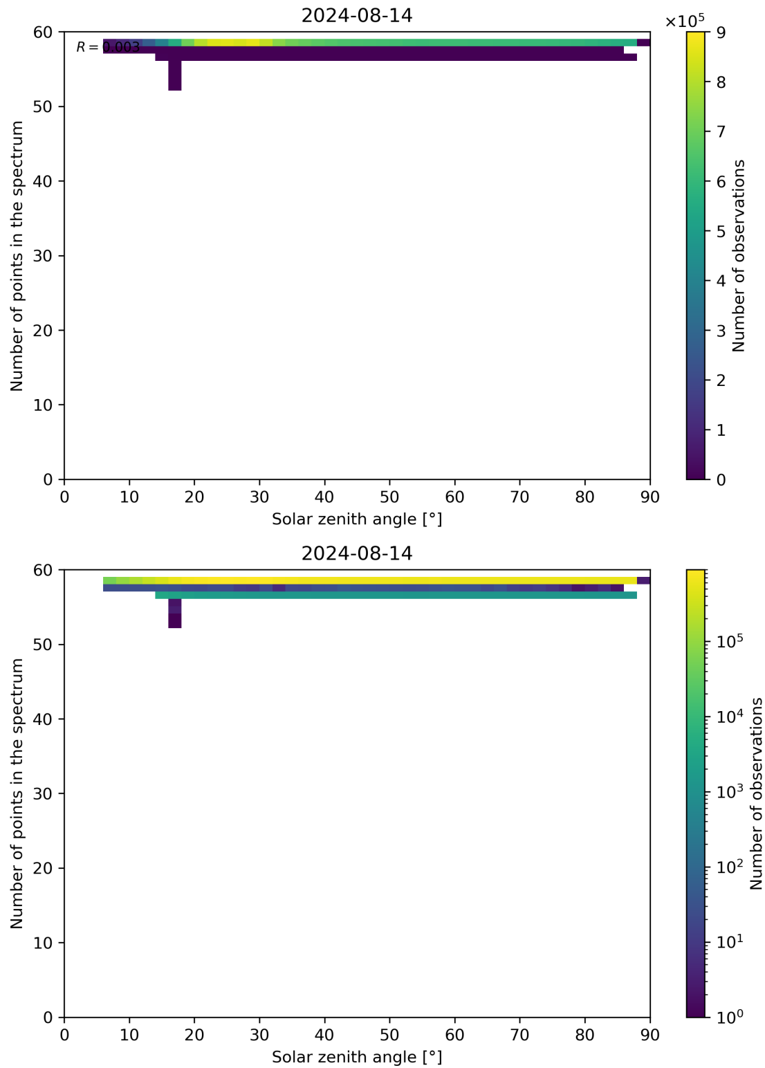
Figure 115: Scatter density plot of “Solar zenith angle” against “Number of points in the spectrum” for 2024-08-13 to 2024-08-15.
