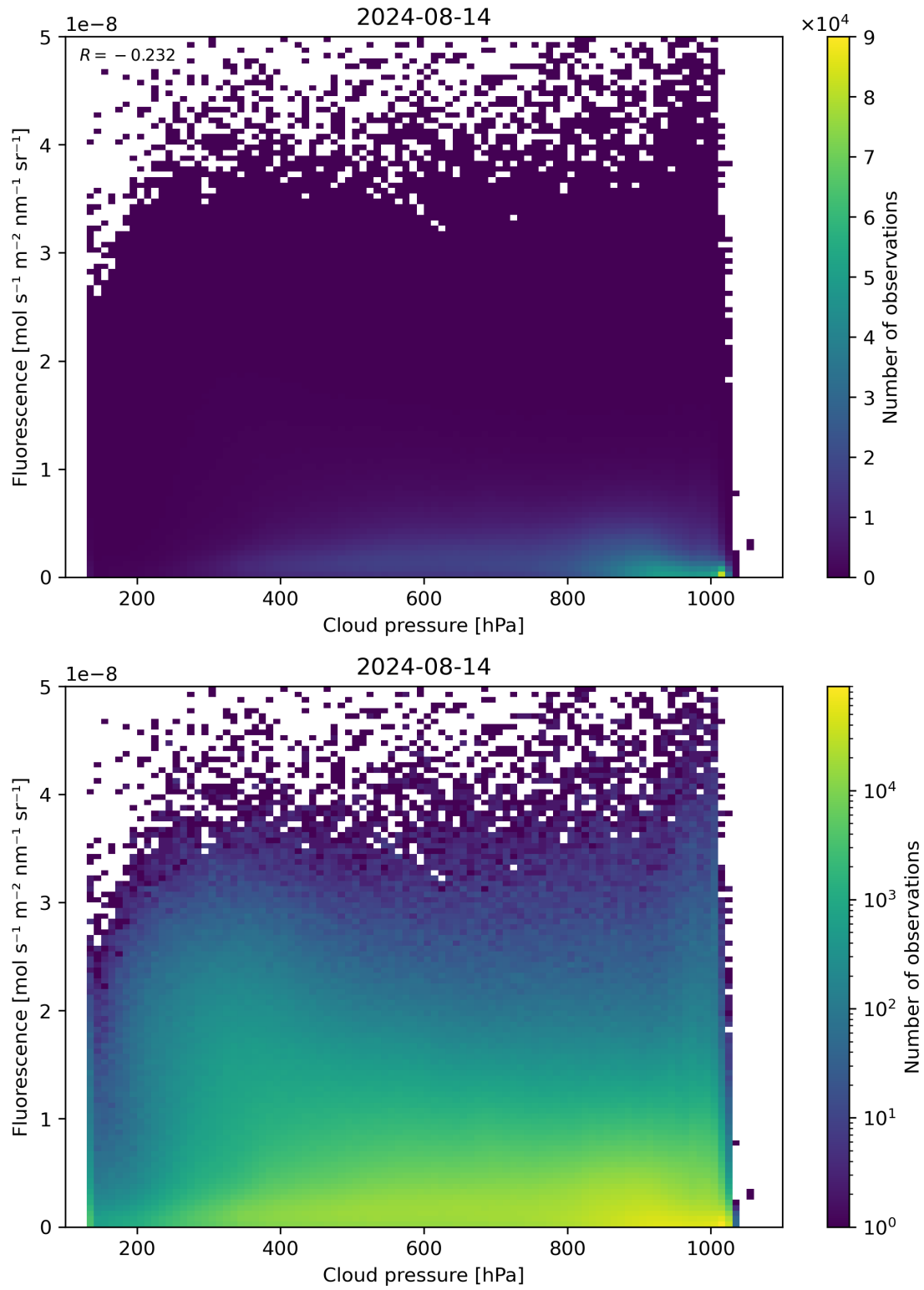
Figure 80: Scatter density plot of “Cloud pressure” against “Fluorescence” for 2024-08-13 to 2024-08-15.
