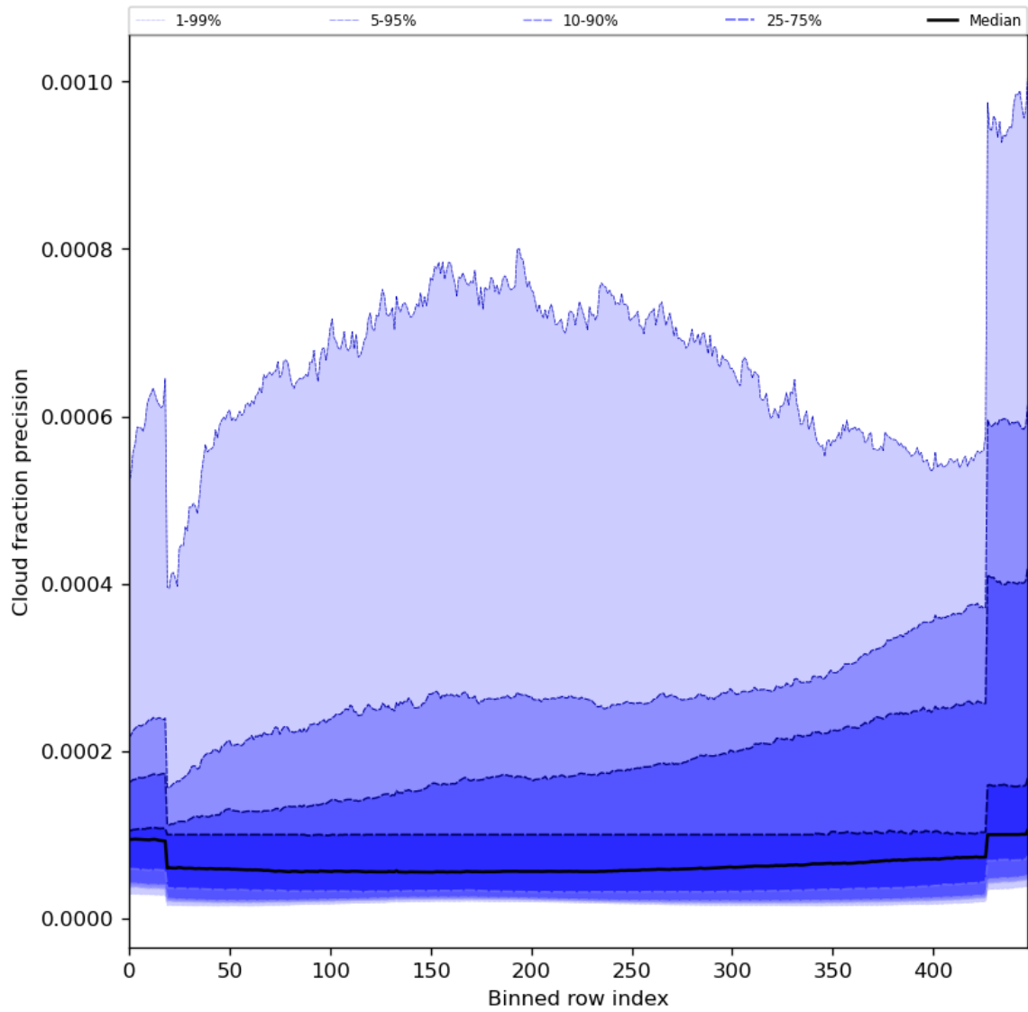
Figure 50: Along track statistics of “Cloud fraction precision” for 2024-08-13 to 2024-08-15
