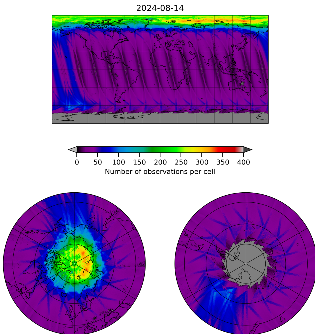
Figure 11: Map of the number of observations for 2024-08-13 to 2024-08-15
