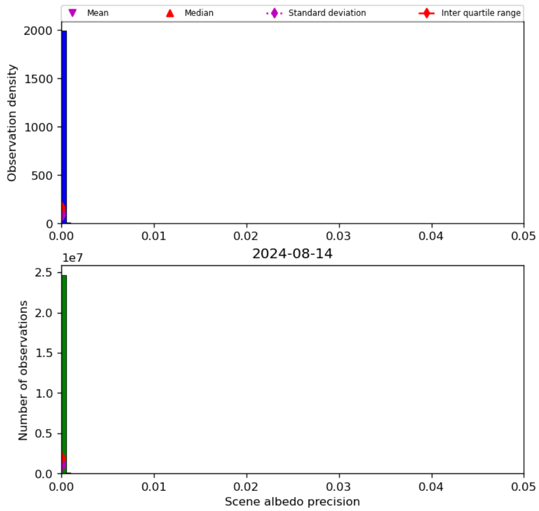
Figure 35: Histogram of “Scene albedo precision” for 2024-08-13 to 2024-08-15
