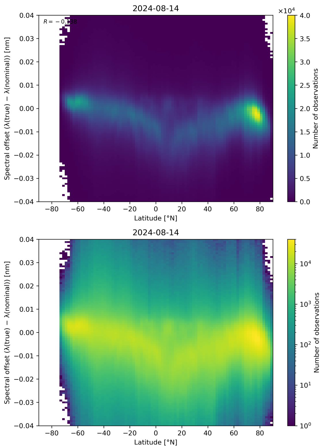
Figure 96: Scatter density plot of “Latitude” against “Spectral offset ( \lambda(\text{true}) - \lambda(\text{nominal}) )” for 2024-08-13 to 2024-08-15.
