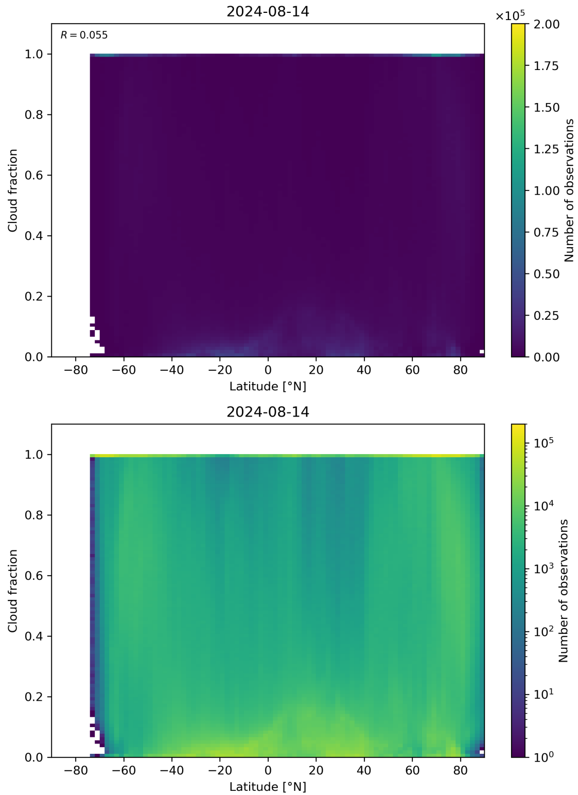
Figure 90: Scatter density plot of “Latitude” against “Cloud fraction” for 2024-08-13 to 2024-08-15.
