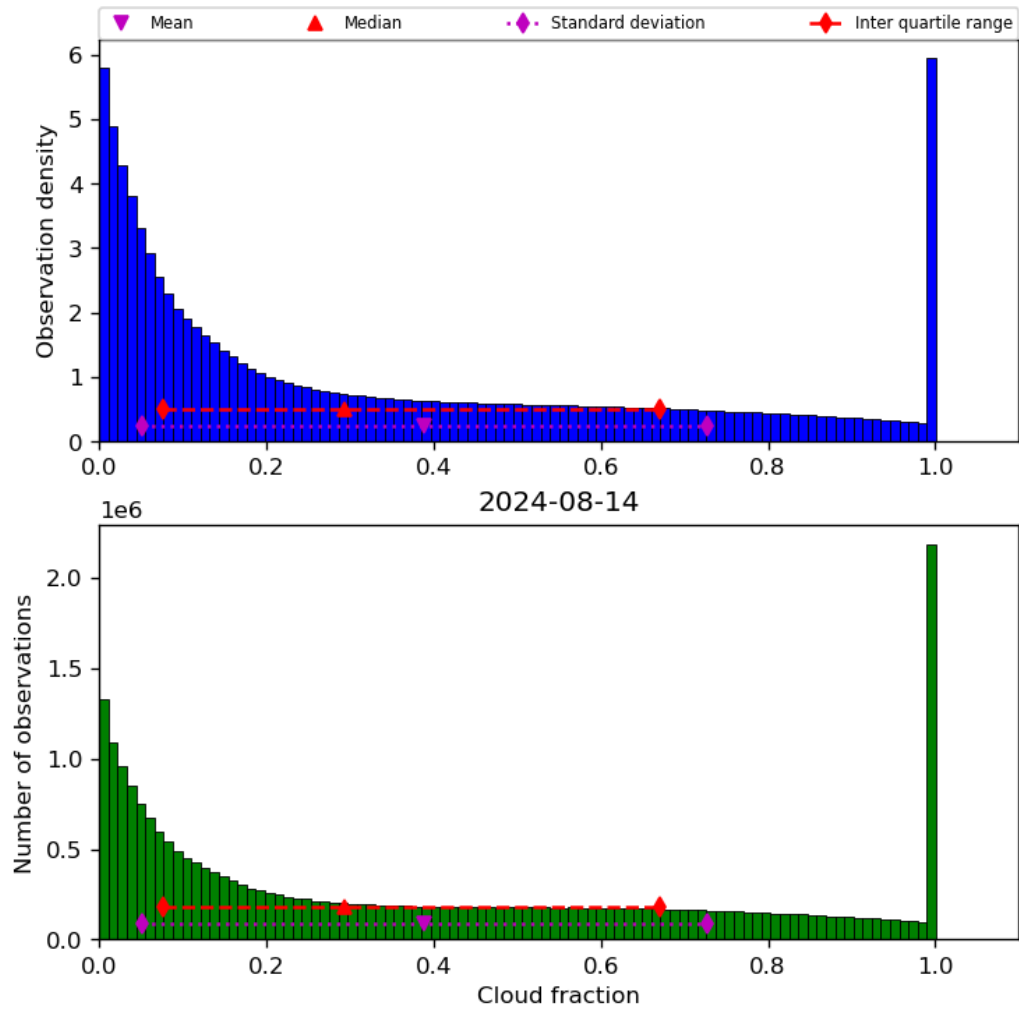
Figure 32: Histogram of “Cloud fraction” for 2024-08-13 to 2024-08-15
