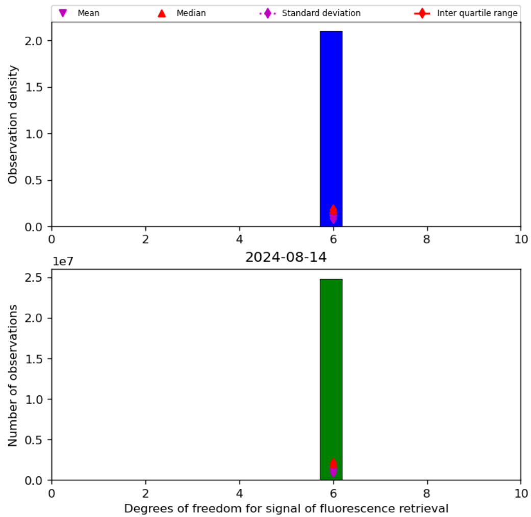
Figure 43: Histogram of “Degrees of freedom for signal of fluorescence retrieval” for 2024-08-13 to 2024-08-15
