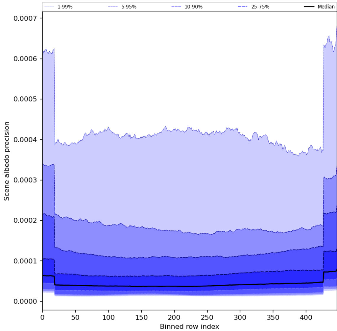
Figure 52: Along track statistics of “Scene albedo precision” for 2024-08-13 to 2024-08-15
