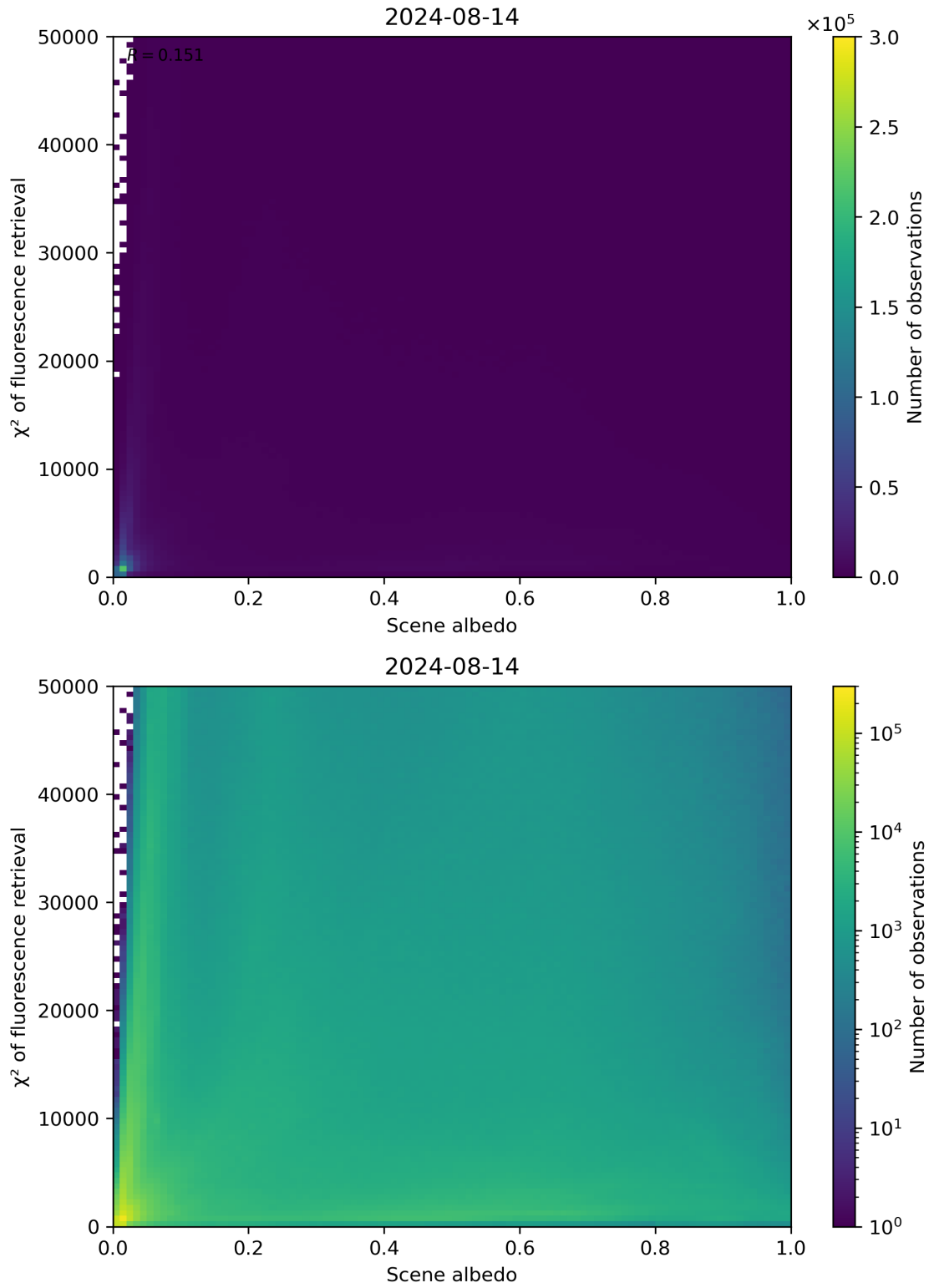
Figure 103: Scatter density plot of “Scene albedo” against “ \chi^2 of fluorescence retrieval” for 2024-08-13 to 2024-08-15.
