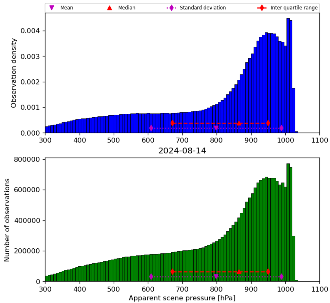
Figure 36: Histogram of “Apparent scene pressure” for 2024-08-13 to 2024-08-15
