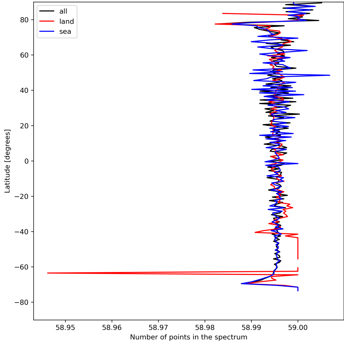
Figure 27: Zonal average of “Number of points in the spectrum” for 2024-08-13 to 2024-08-15.
