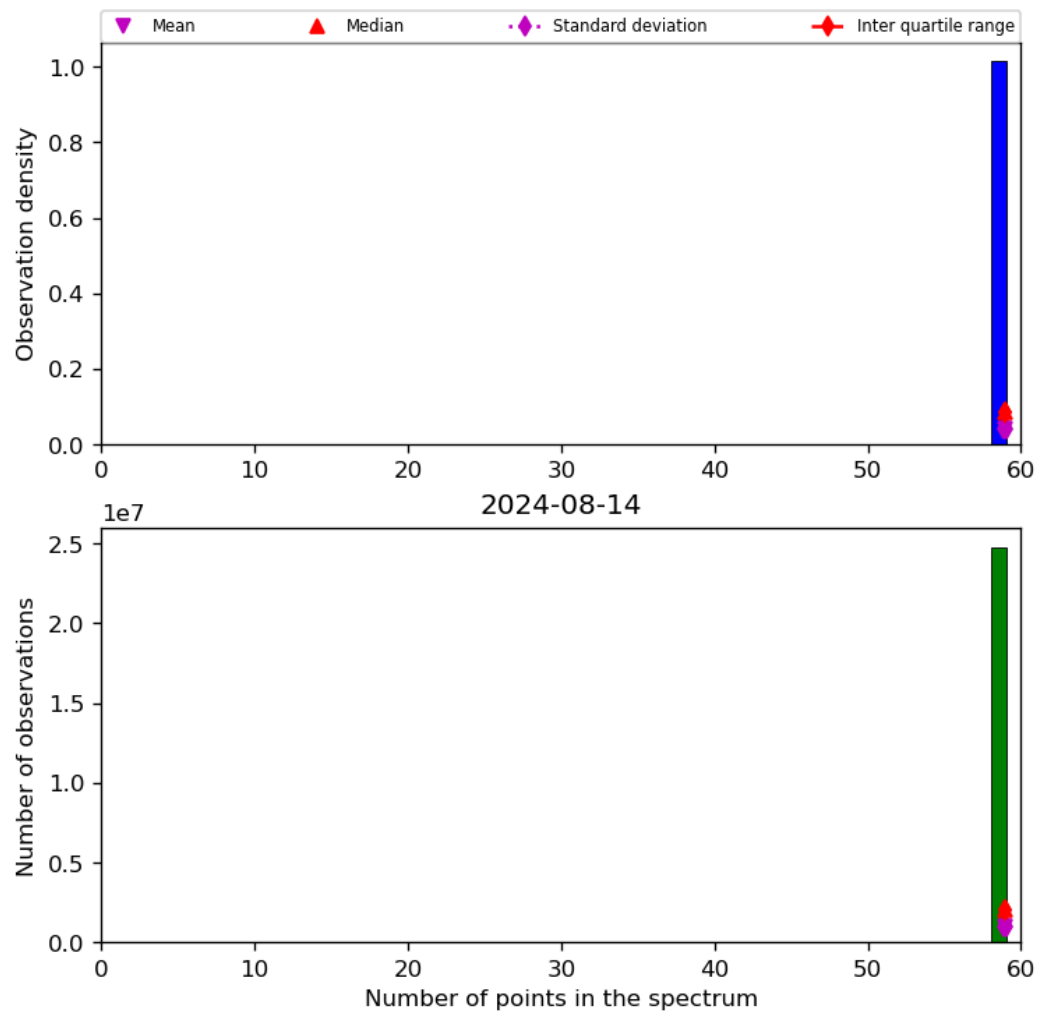
Figure 44: Histogram of “Number of points in the spectrum” for 2024-08-13 to 2024-08-15
