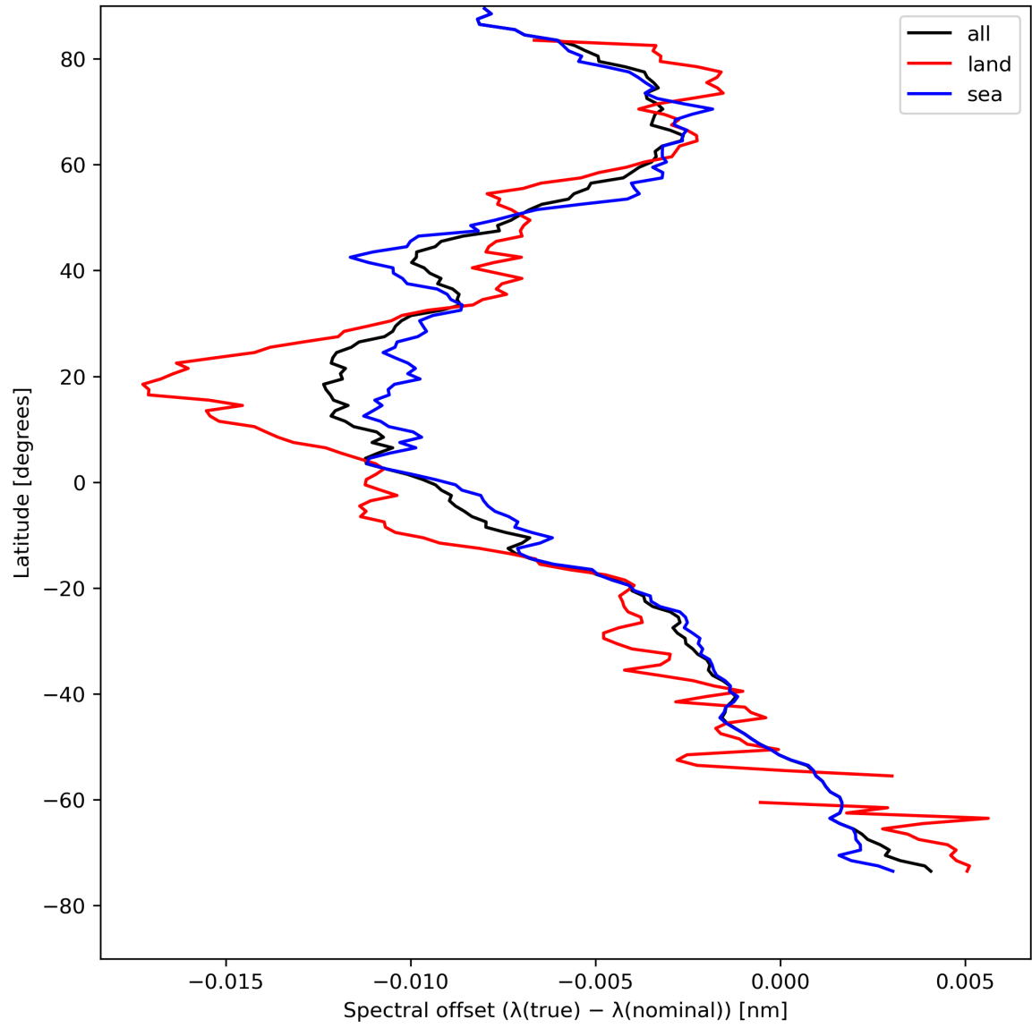
Figure 28: Zonal average of “Spectral offset ( \lambda(\text{true}) - \lambda(\text{nominal}) )” for 2024-08-13 to 2024-08-15.
