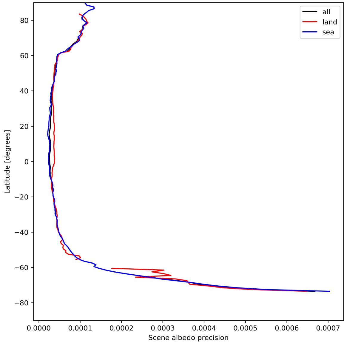
Figure 18: Zonal average of “Scene albedo precision” for 2024-08-13 to 2024-08-15.
