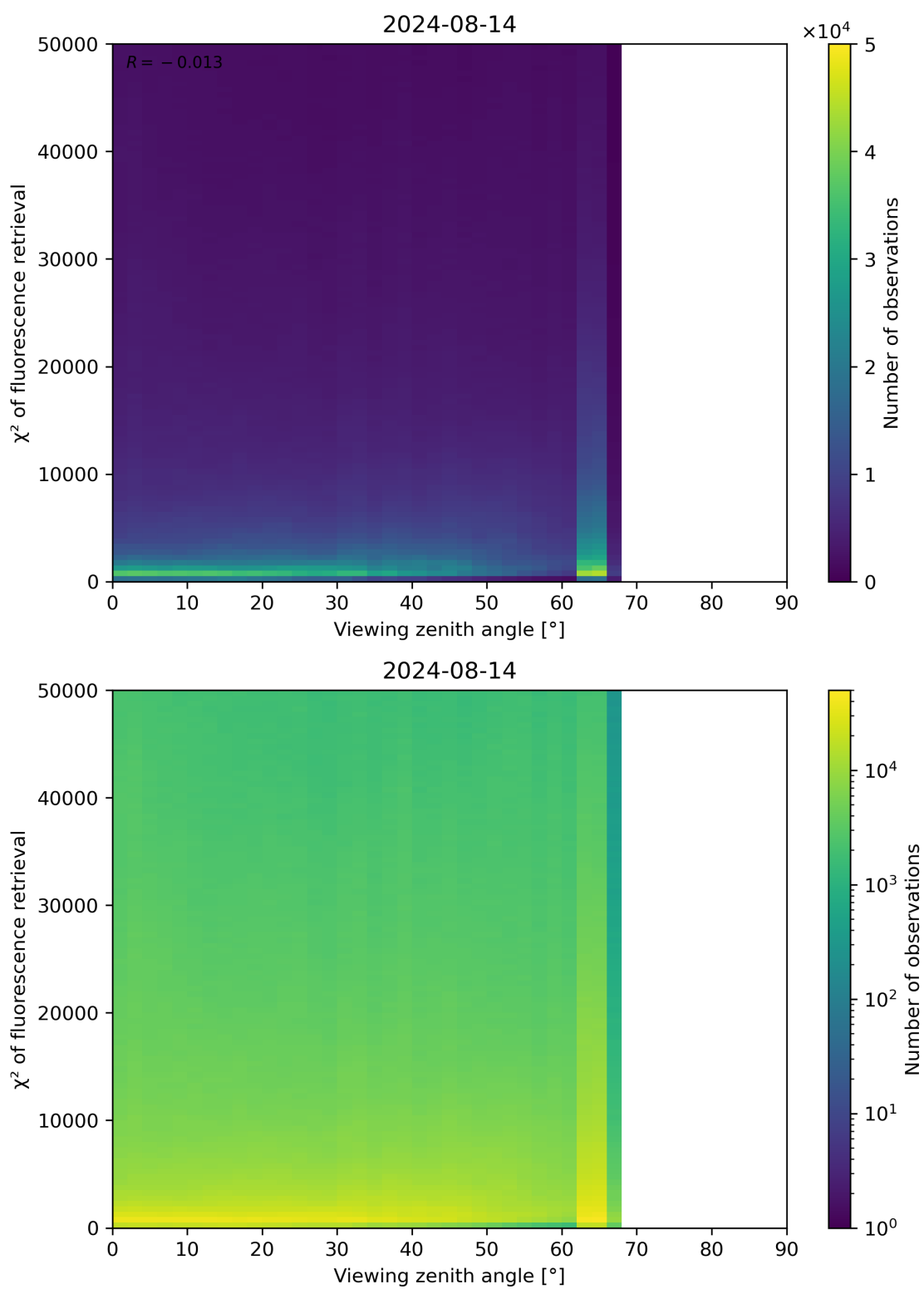
Figure 119: Scatter density plot of “Viewing zenith angle” against “ \chi^2 of fluorescence retrieval” for 2024-08-13 to 2024-08-15.
