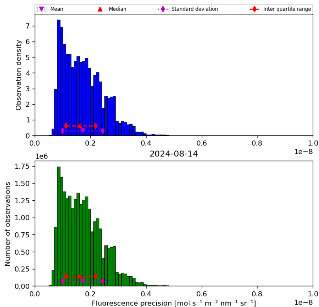
Figure 41: Histogram of “Fluorescence precision” for 2024-08-13 to 2024-08-15
