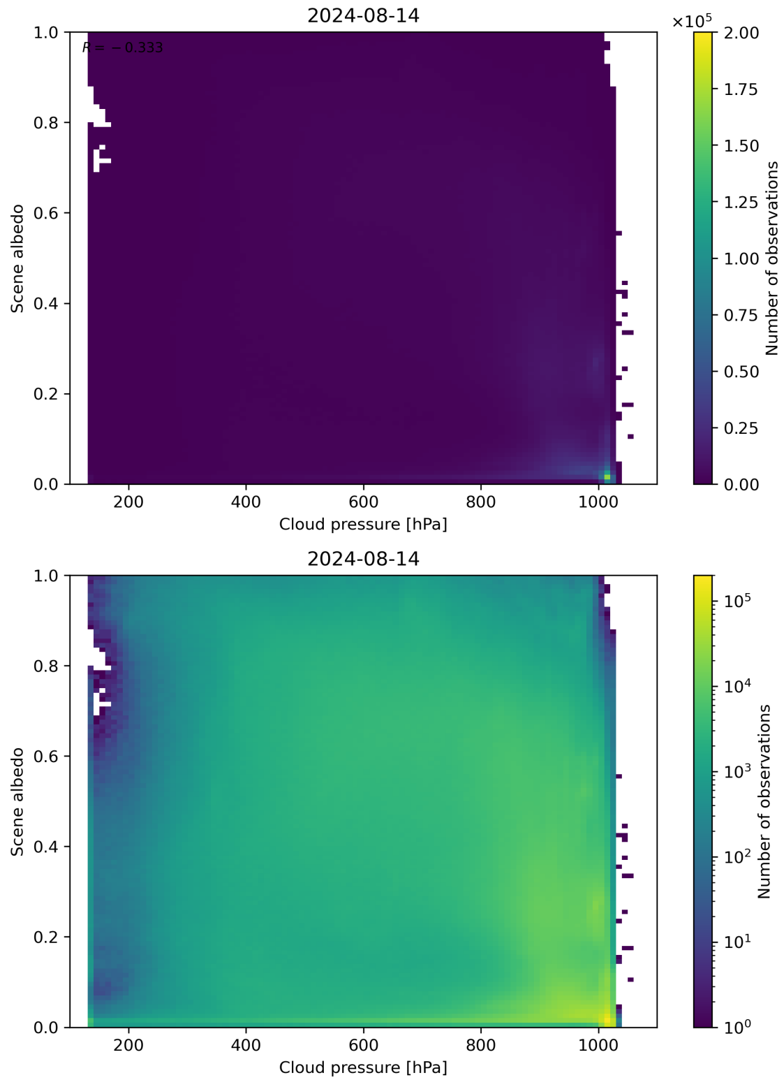
Figure 83: Scatter density plot of “Cloud pressure” against “Scene albedo” for 2024-08-13 to 2024-08-15.
