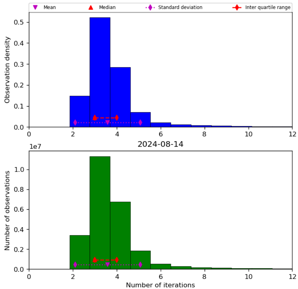
Figure 39: Histogram of “Number of iterations” for 2024-08-13 to 2024-08-15
