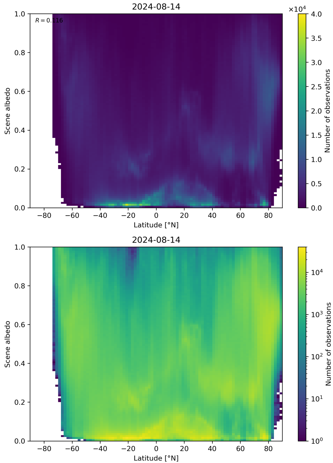
Figure 95: Scatter density plot of “Latitude” against “Scene albedo” for 2024-08-13 to 2024-08-15.
