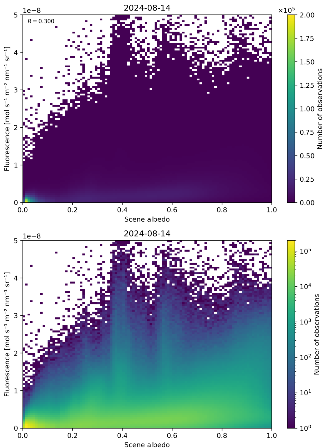
Figure 104: Scatter density plot of “Scene albedo” against “Fluorescence” for 2024-08-13 to 2024-08-15.
