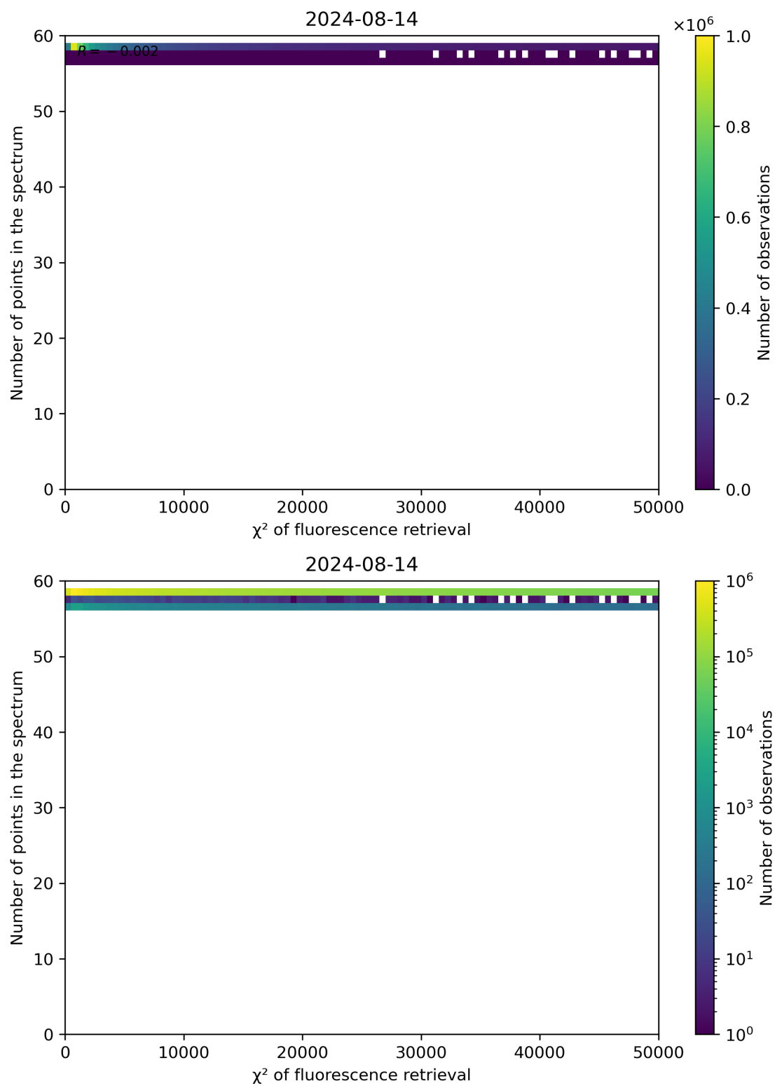
Figure 68: Scatter density plot of " \chi^2 of fluorescence retrieval" against "Number of points in the spectrum" for 2024-08-13 to 2024-08-15.
