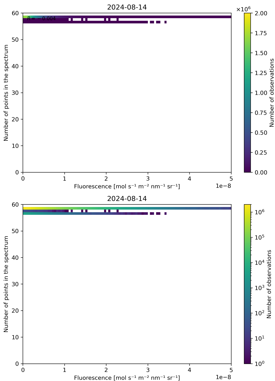
Figure 86: Scatter density plot of “Fluorescence” against “Number of points in the spectrum” for 2024-08-13 to 2024-08-15.
