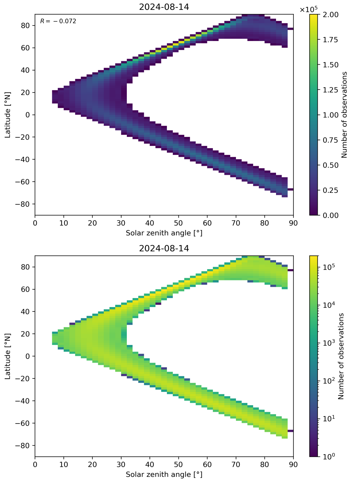
Figure 113: Scatter density plot of “Solar zenith angle” against “Latitude” for 2024-08-13 to 2024-08-15.
