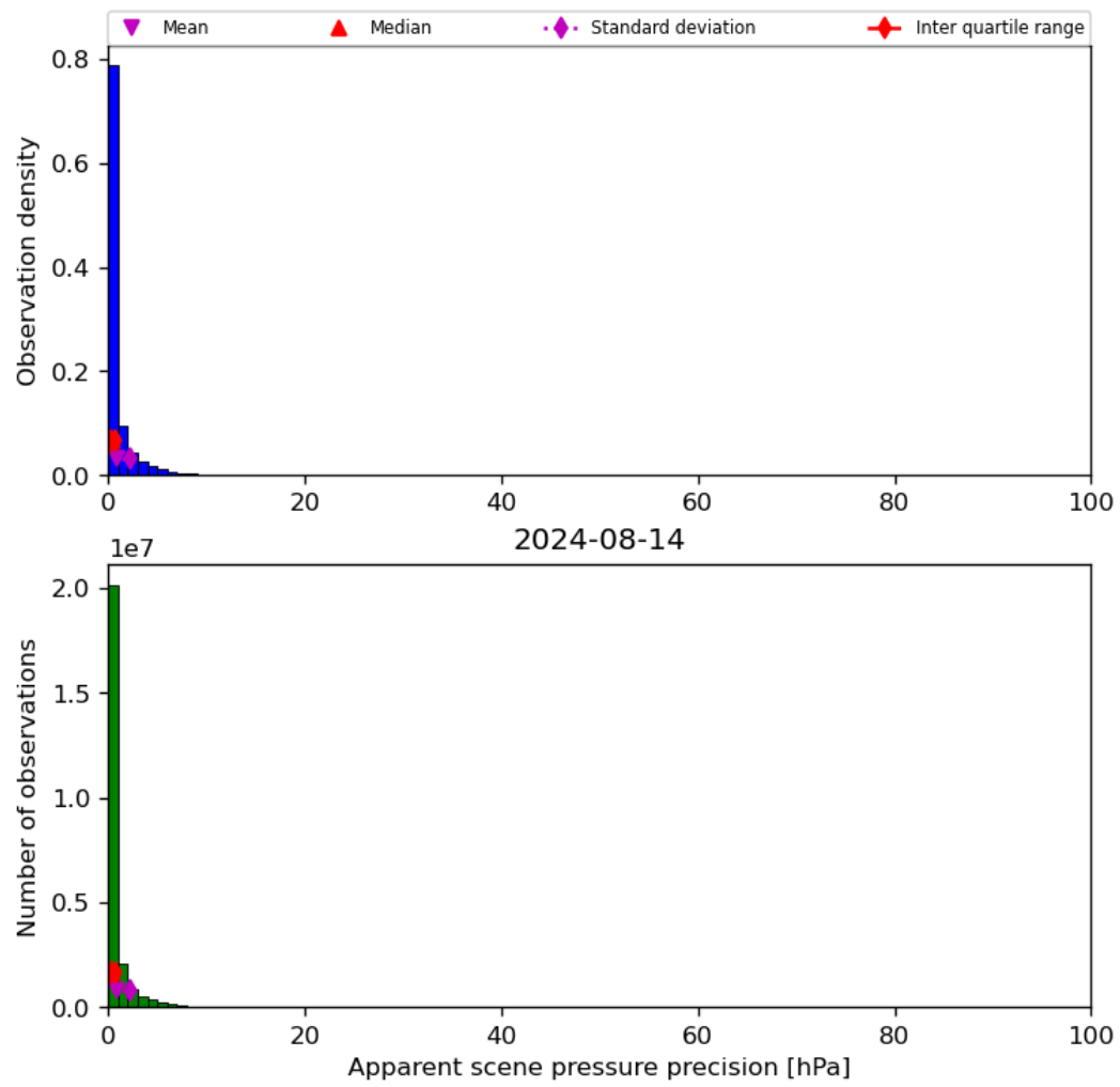
Figure 37: Histogram of “Apparent scene pressure precision” for 2024-08-13 to 2024-08-15
