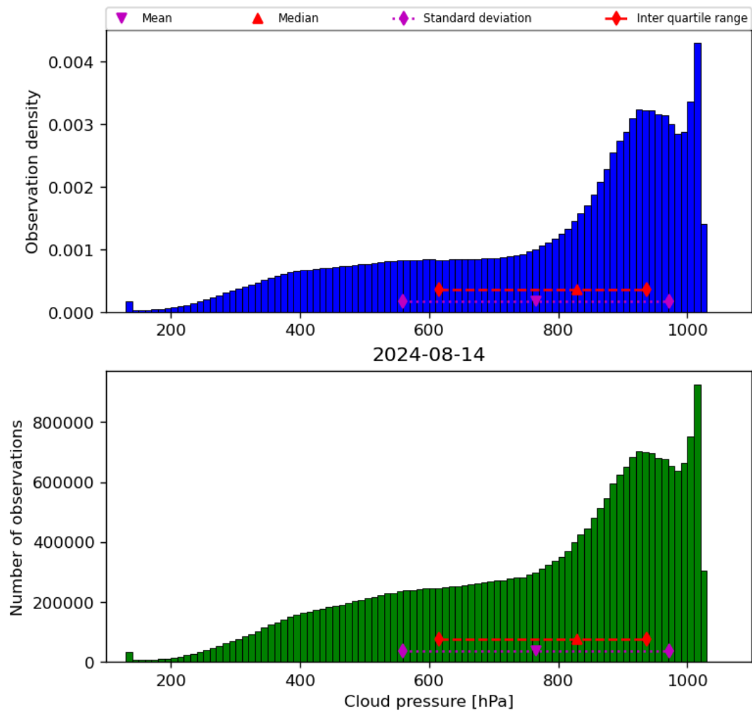
Figure 30: Histogram of “Cloud pressure” for 2024-08-13 to 2024-08-15
