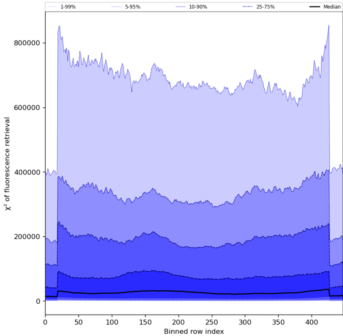
Figure 59: Along track statistics of “ \chi^2 of fluorescence retrieval” for 2024-08-13 to 2024-08-15
