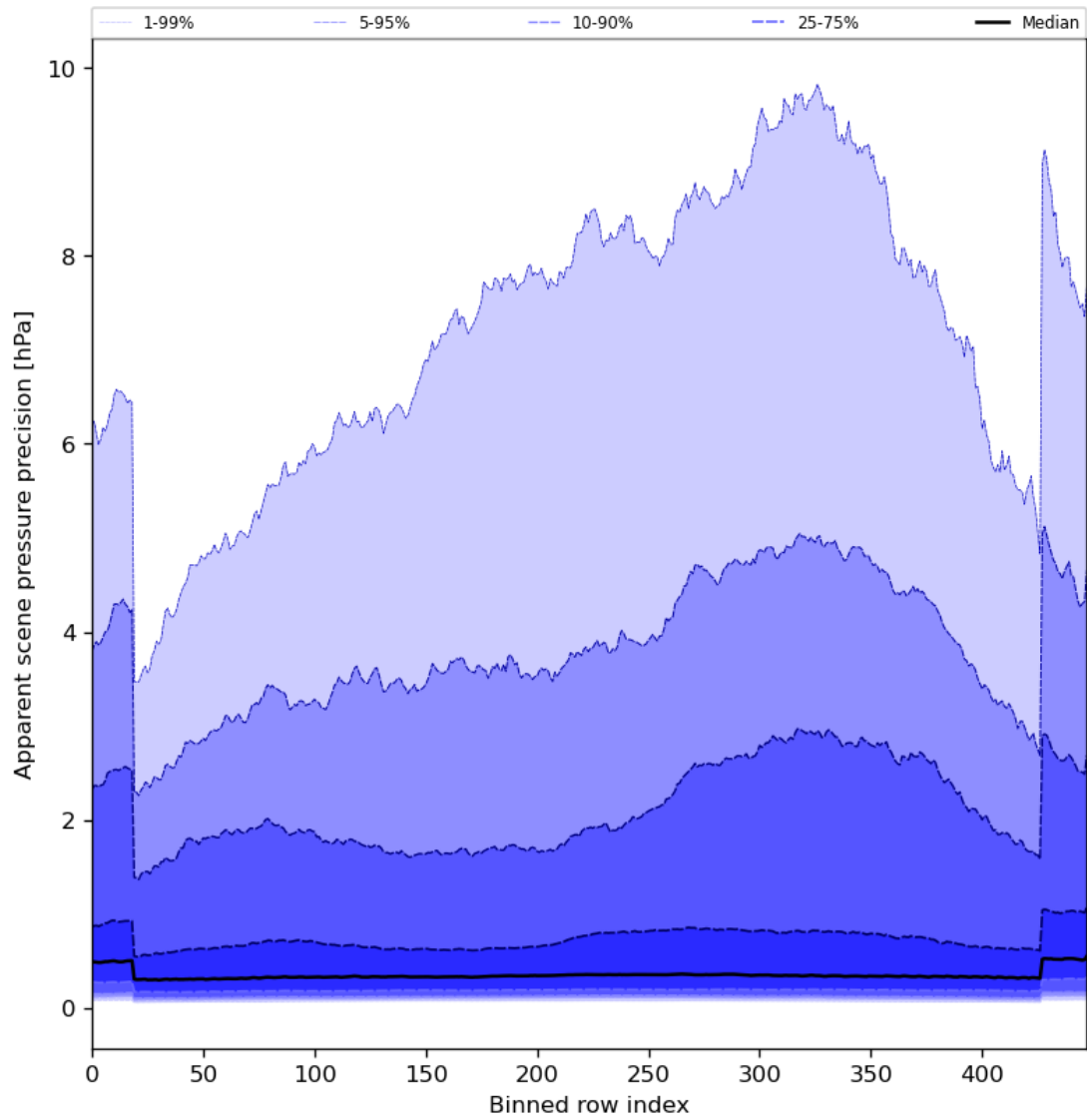
Figure 54: Along track statistics of “Apparent scene pressure precision” for 2024-08-13 to 2024-08-15
