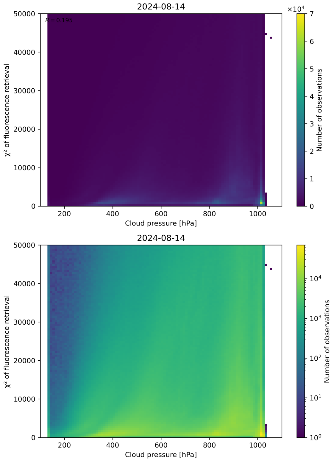
Figure 78: Scatter density plot of “Cloud pressure” against “ \chi^2 of fluorescence retrieval” for 2024-08-13 to 2024-08-15.
