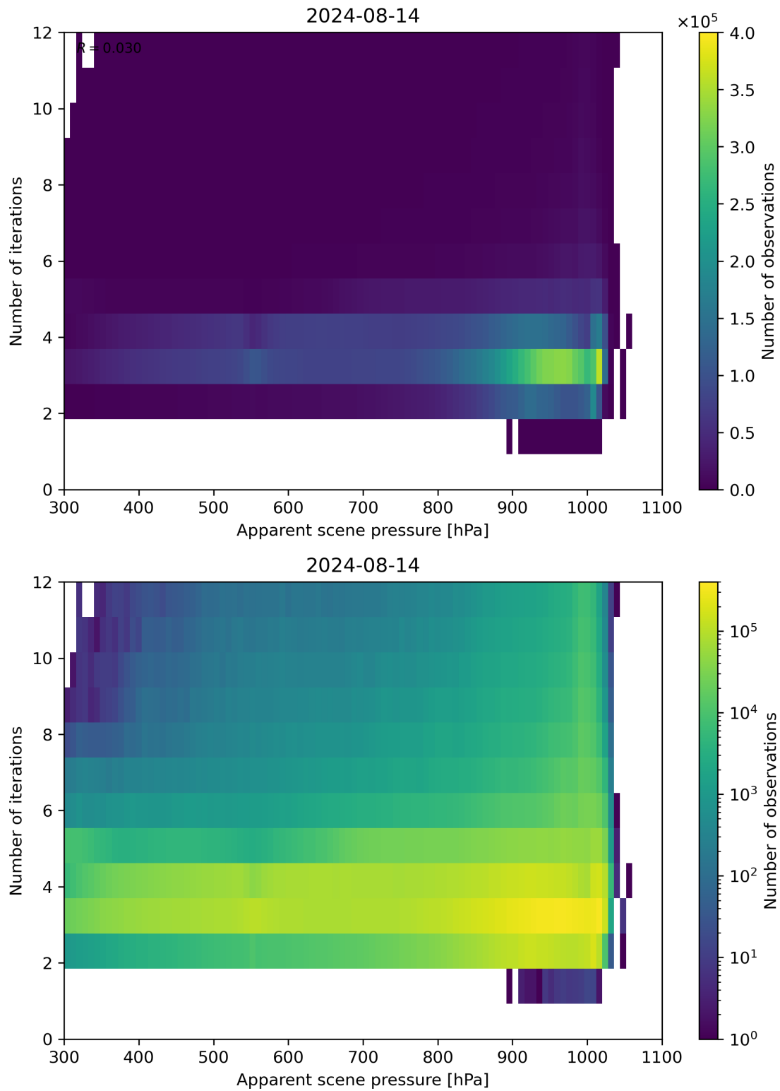
Figure 65: Scatter density plot of “Apparent scene pressure” against “Number of iterations” for 2024-08-13 to 2024-08-15.
