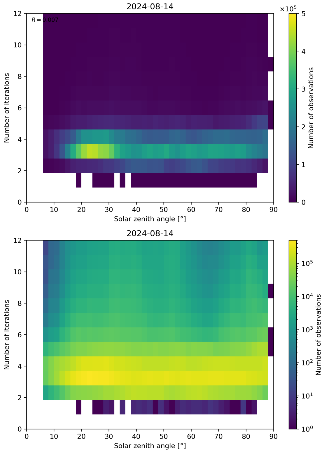
Figure 114: Scatter density plot of “Solar zenith angle” against “Number of iterations” for 2024-08-13 to 2024-08-15.
