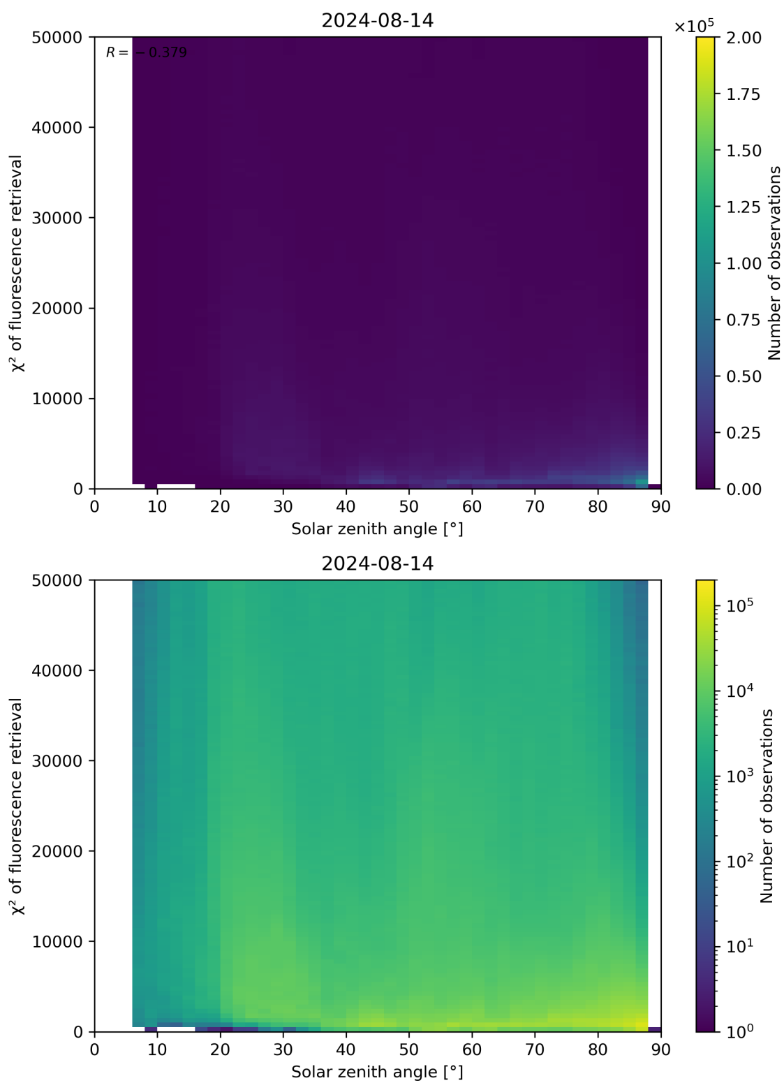
Figure 109: Scatter density plot of “Solar zenith angle” against “ \chi^2 of fluorescence retrieval” for 2024-08-13 to 2024-08-15.
