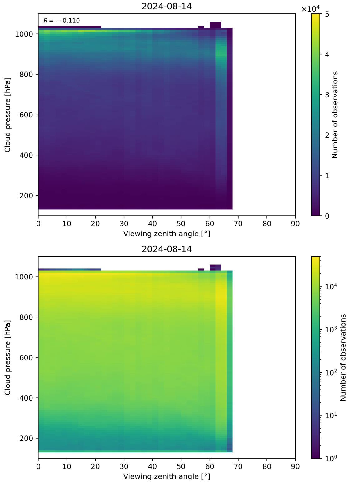
Figure 121: Scatter density plot of “Viewing zenith angle” against “Cloud pressure” for 2024-08-13 to 2024-08-15.
