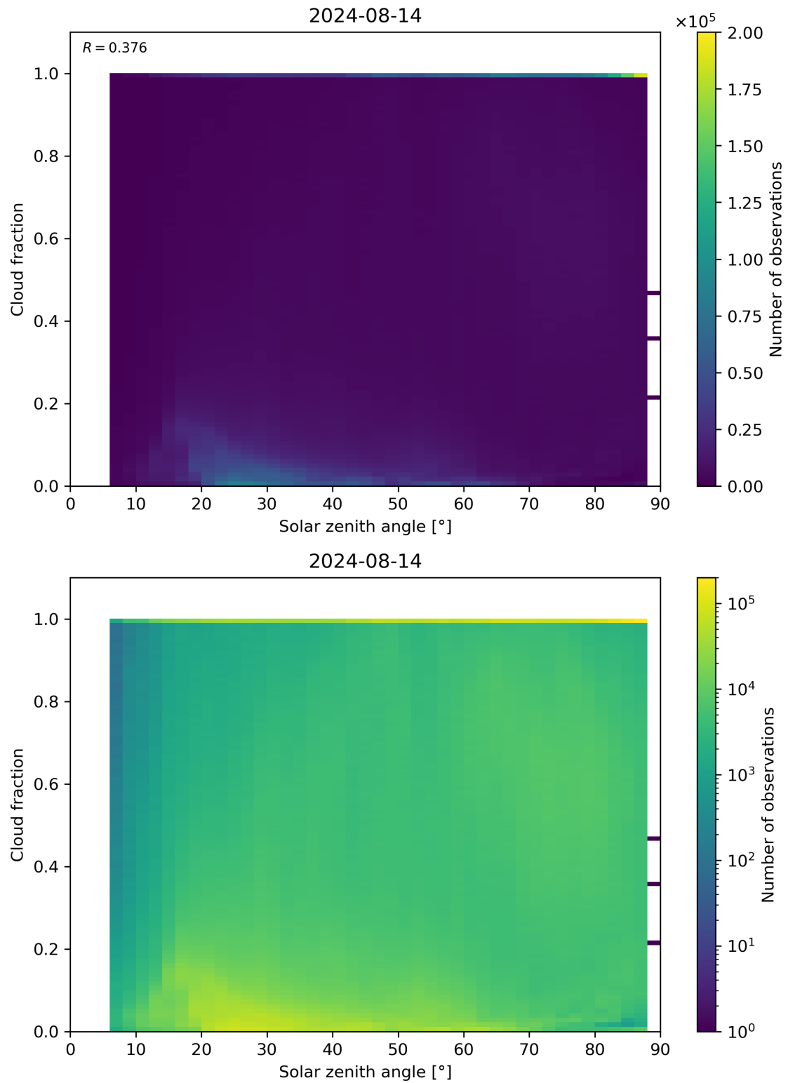
Figure 110: Scatter density plot of “Solar zenith angle” against “Cloud fraction” for 2024-08-13 to 2024-08-15.
