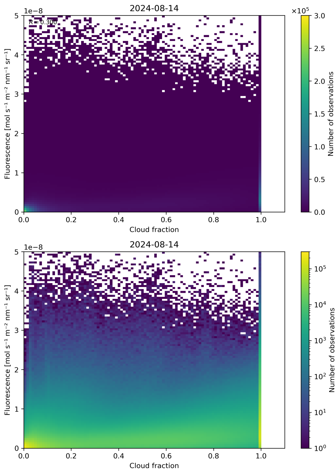
Figure 72: Scatter density plot of “Cloud fraction” against “Fluorescence” for 2024-08-13 to 2024-08-15.
