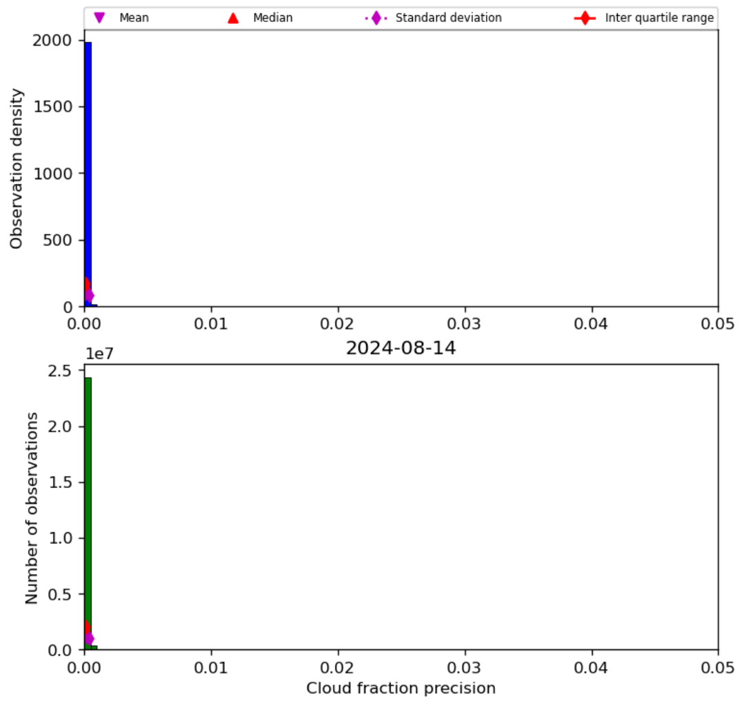
Figure 33: Histogram of “Cloud fraction precision” for 2024-08-13 to 2024-08-15
