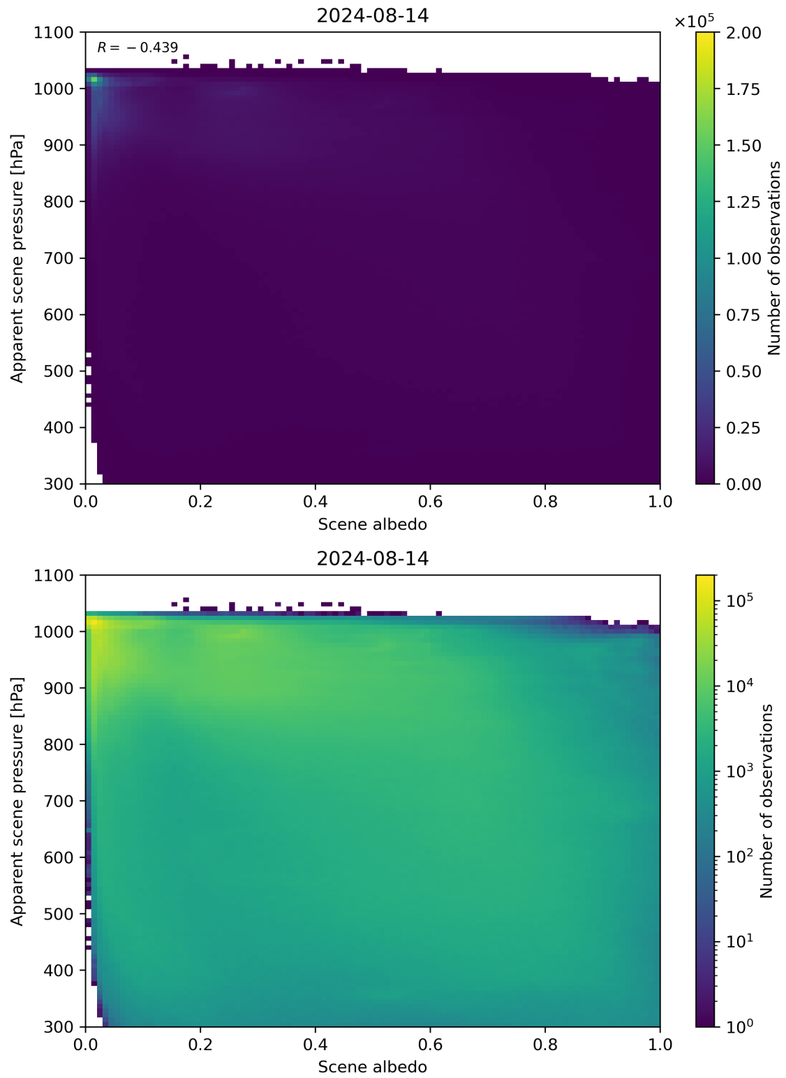
Figure 102: Scatter density plot of “Scene albedo” against “Apparent scene pressure” for 2024-08-13 to 2024-08-15.
