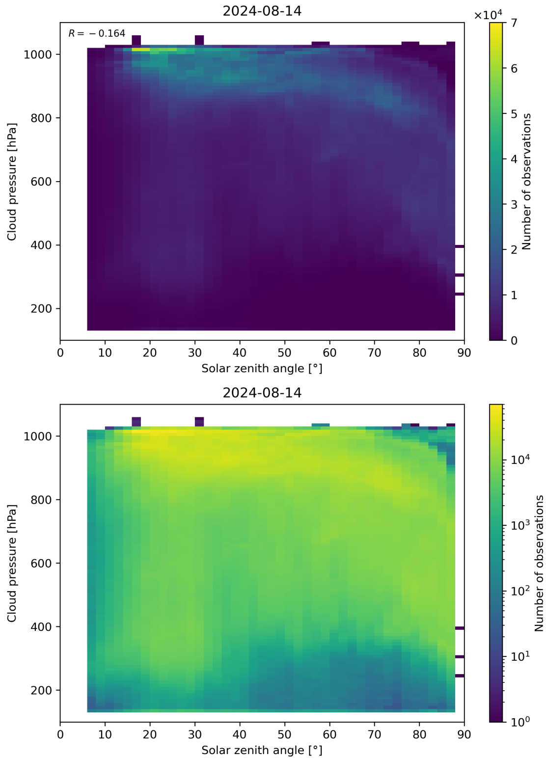
Figure 111: Scatter density plot of “Solar zenith angle” against “Cloud pressure” for 2024-08-13 to 2024-08-15.
