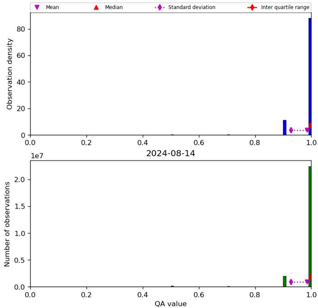
Figure 29: Histogram of “QA value” for 2024-08-13 to 2024-08-15
