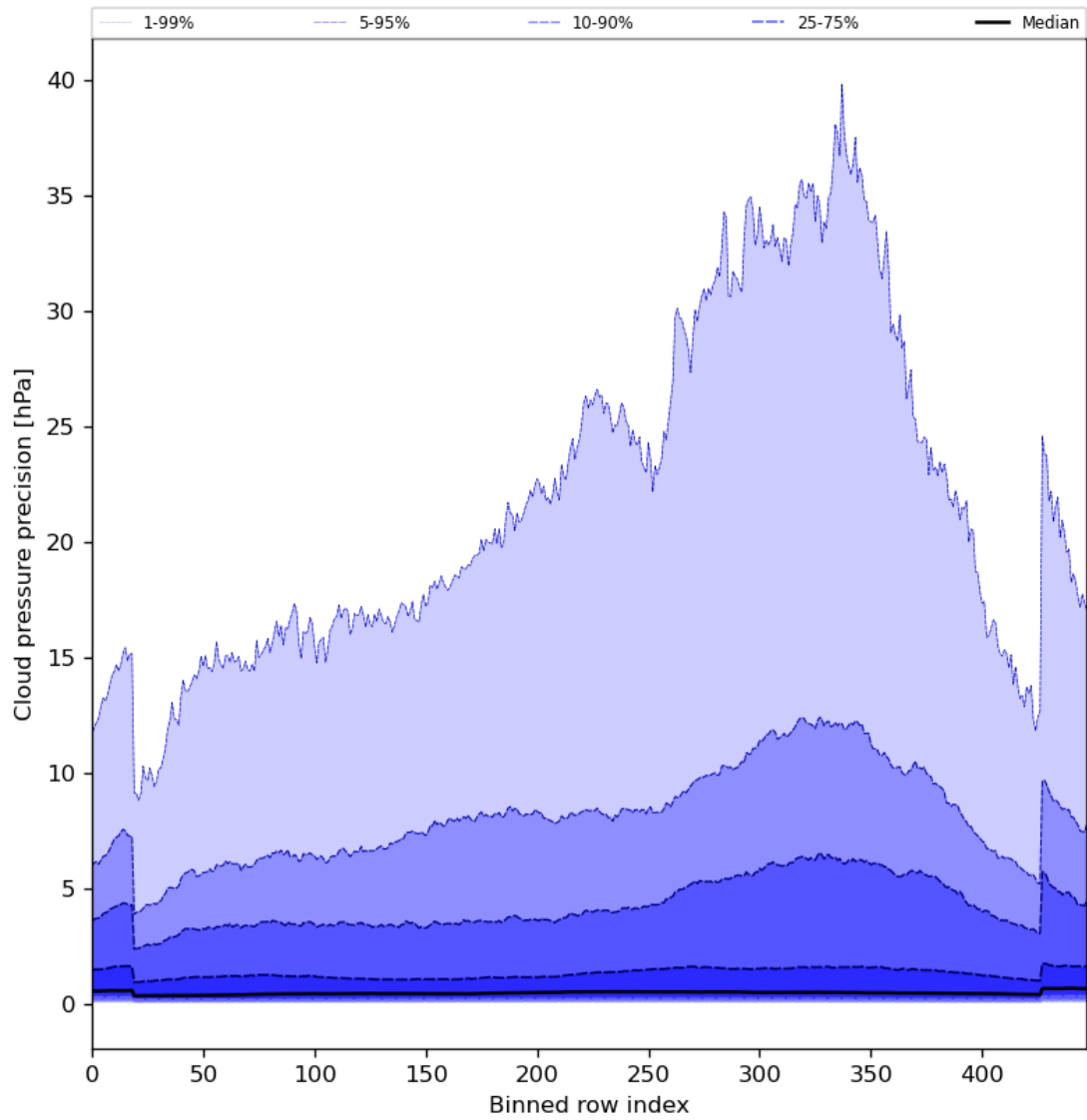
Figure 48: Along track statistics of “Cloud pressure precision” for 2024-08-13 to 2024-08-15
