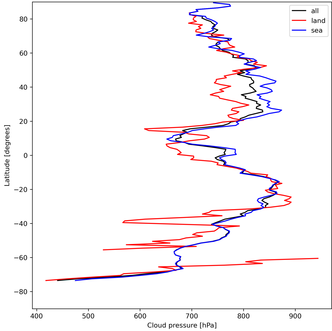
Figure 13: Zonal average of “Cloud pressure” for 2024-08-13 to 2024-08-15.
