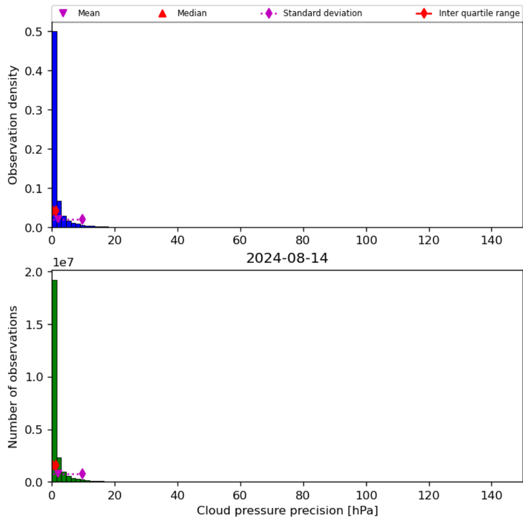
Figure 31: Histogram of “Cloud pressure precision” for 2024-08-13 to 2024-08-15
