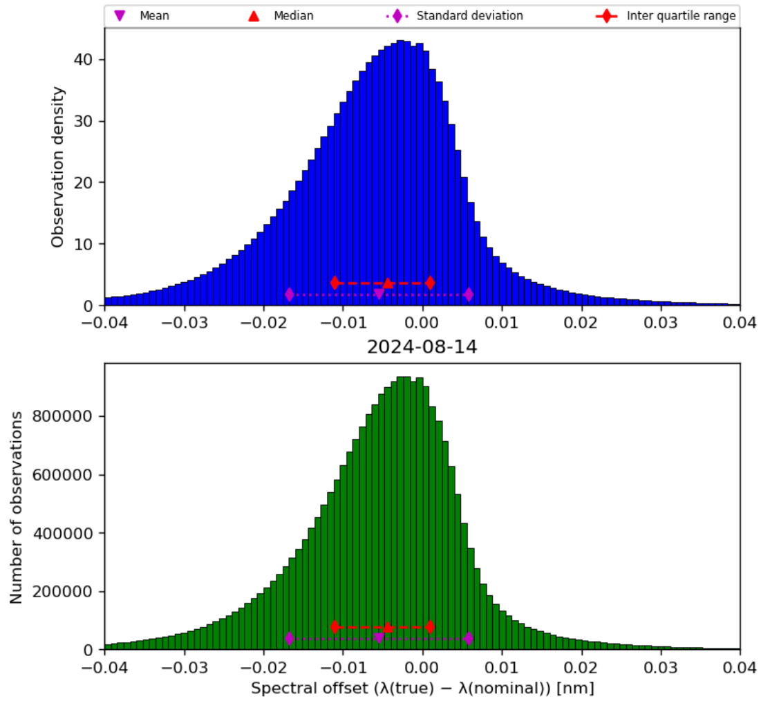
Figure 45: Histogram of “Spectral offset ( \lambda(\text{true}) - \lambda(\text{nominal}) )” for 2024-08-13 to 2024-08-15
