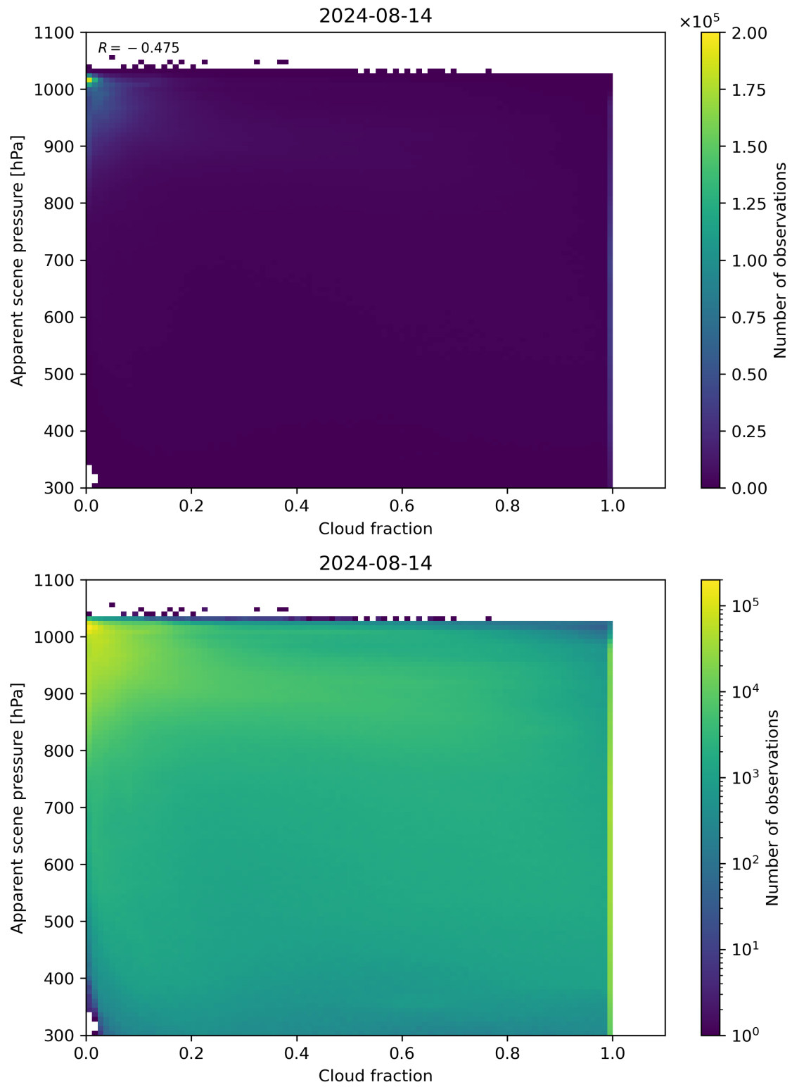
Figure 70: Scatter density plot of “Cloud fraction” against “Apparent scene pressure” for 2024-08-13 to 2024-08-15.
