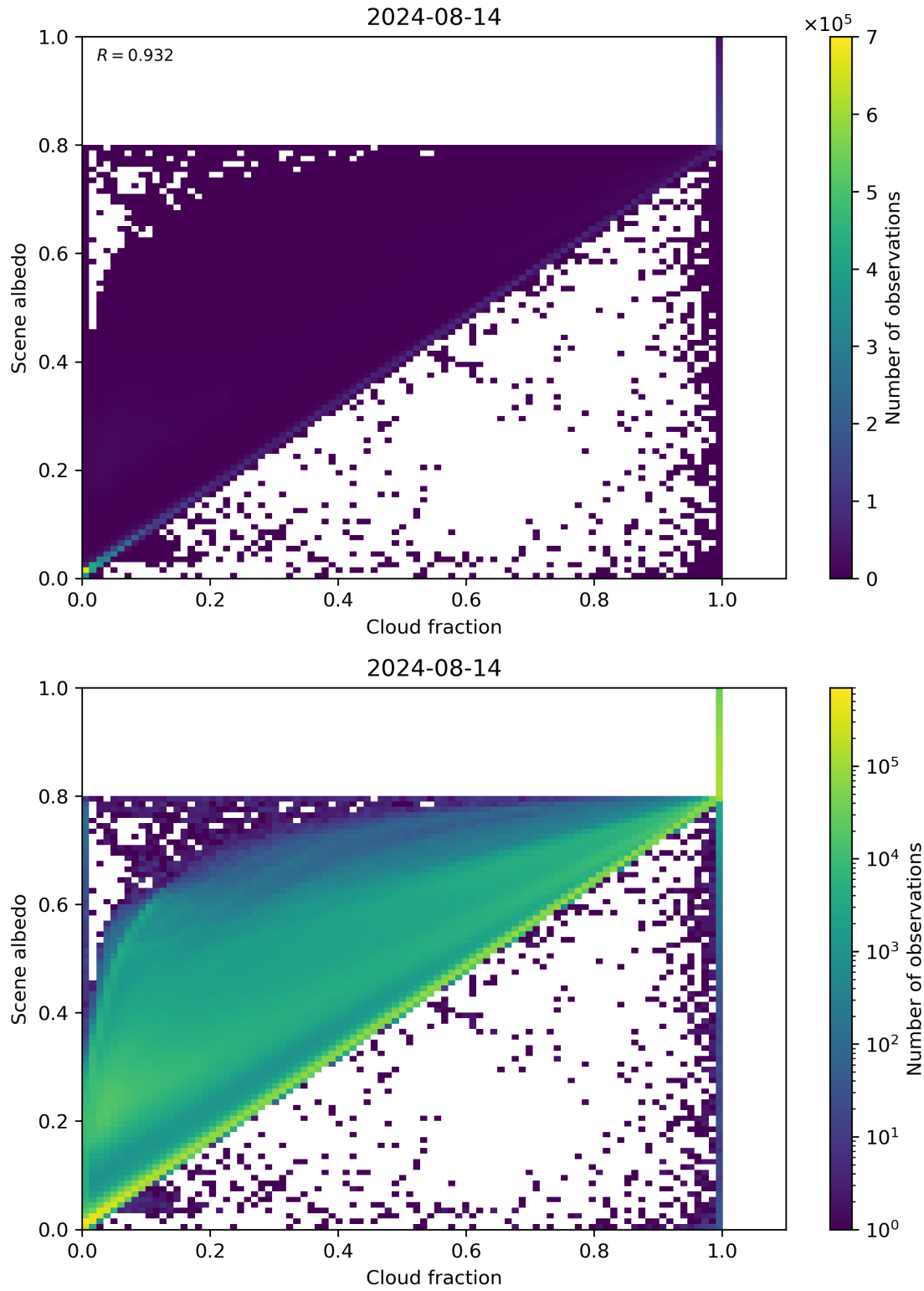
Figure 75: Scatter density plot of “Cloud fraction” against “Scene albedo” for 2024-08-13 to 2024-08-15.
