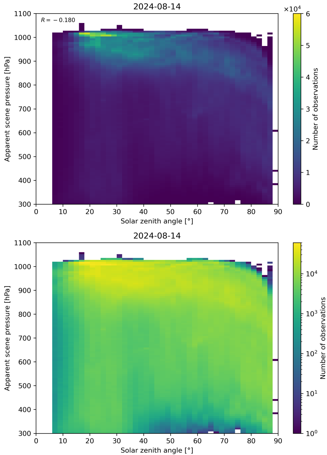
Figure 108: Scatter density plot of “Solar zenith angle” against “Apparent scene pressure” for 2024-08-13 to 2024-08-15.
