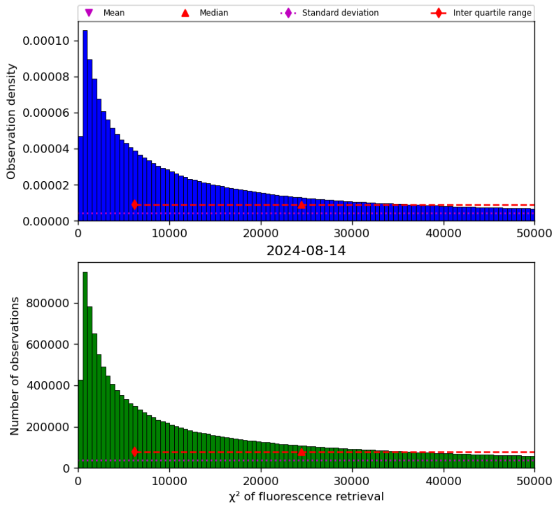
Figure 42: Histogram of “ \chi^2 of fluorescence retrieval” for 2024-08-13 to 2024-08-15
