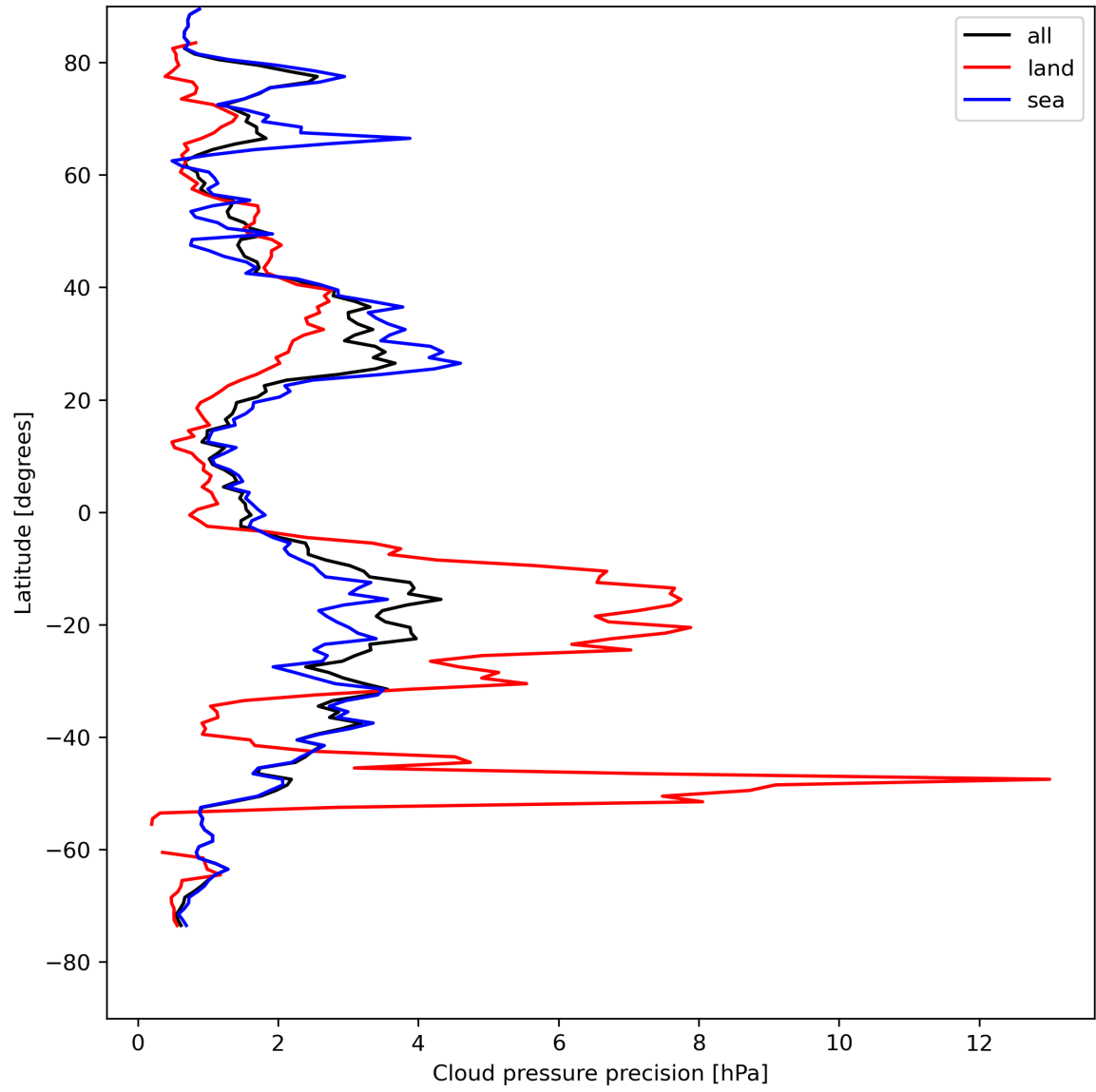
Figure 14: Zonal average of “Cloud pressure precision” for 2024-08-13 to 2024-08-15.
