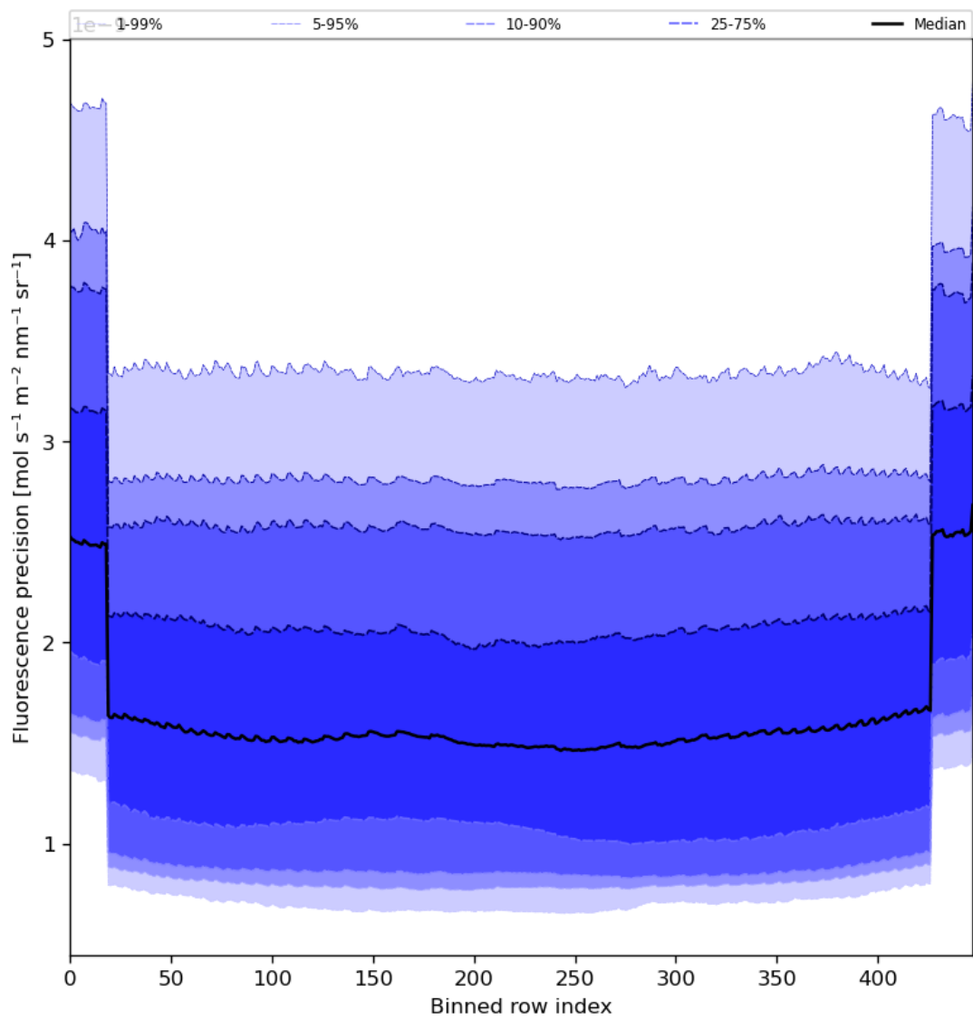
Figure 58: Along track statistics of “Fluorescence precision” for 2024-08-13 to 2024-08-15
