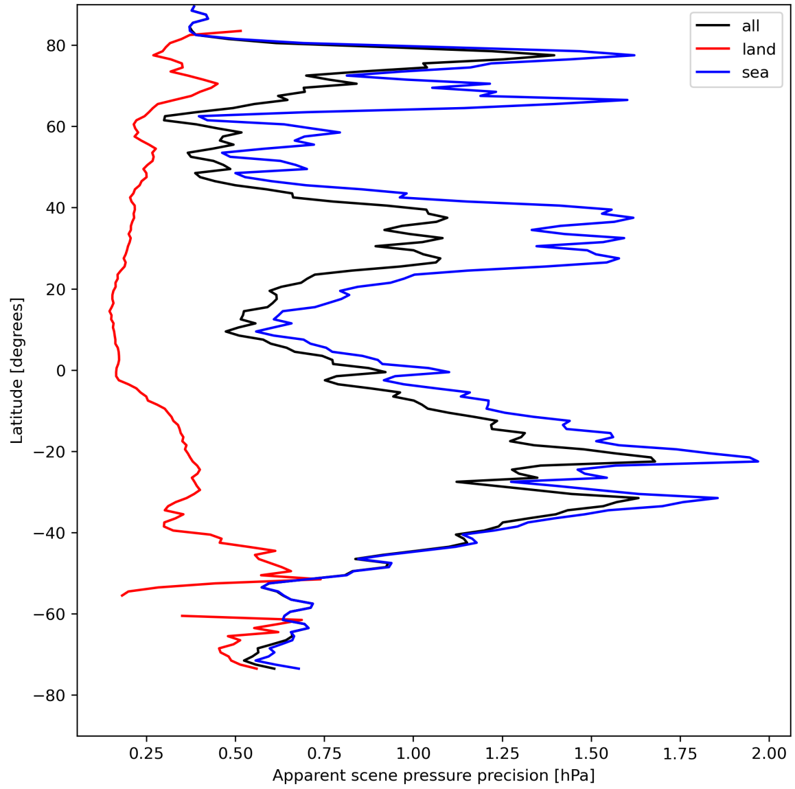
Figure 20: Zonal average of “Apparent scene pressure precision” for 2024-08-13 to 2024-08-15.
