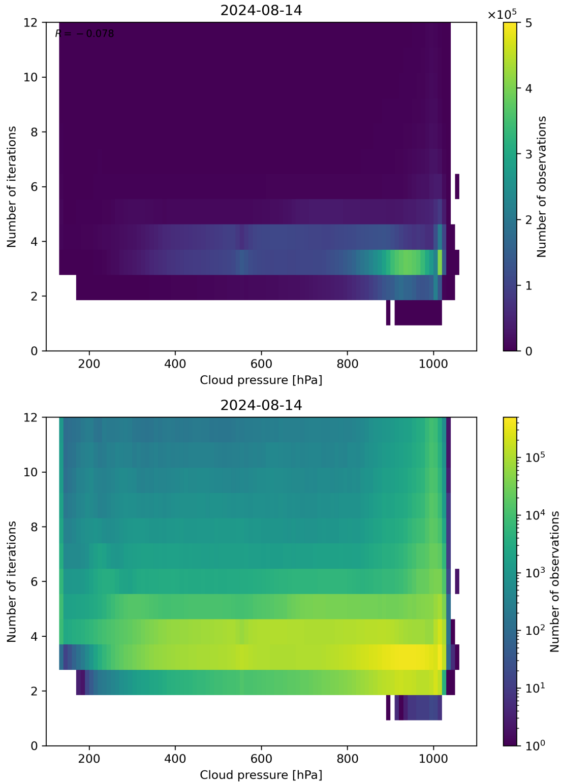
Figure 81: Scatter density plot of “Cloud pressure” against “Number of iterations” for 2024-08-13 to 2024-08-15.
