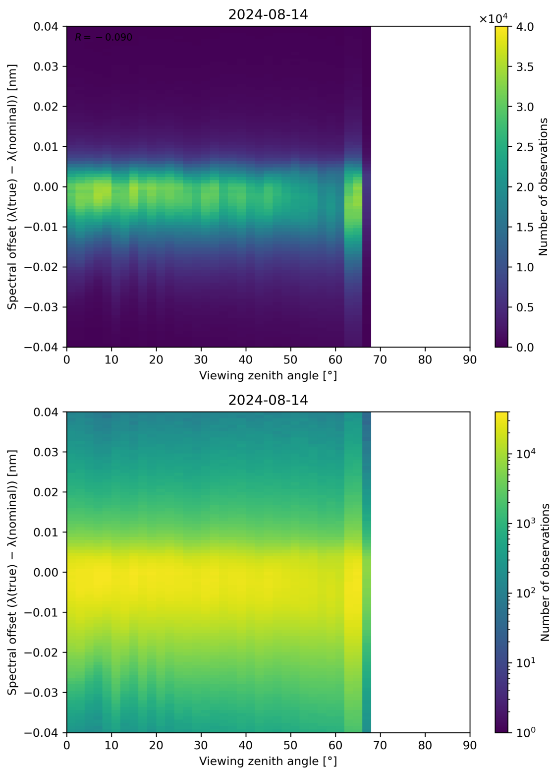
Figure 128: Scatter density plot of “Viewing zenith angle” against “Spectral offset ( \lambda(\text{true}) - \lambda(\text{nominal}) )” for 2024-08-13 to 2024-08-15.
