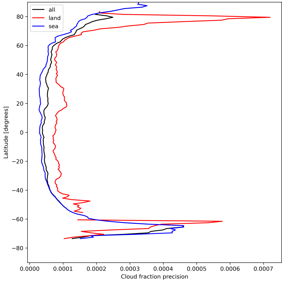
Figure 16: Zonal average of “Cloud fraction precision” for 2024-08-13 to 2024-08-15.
