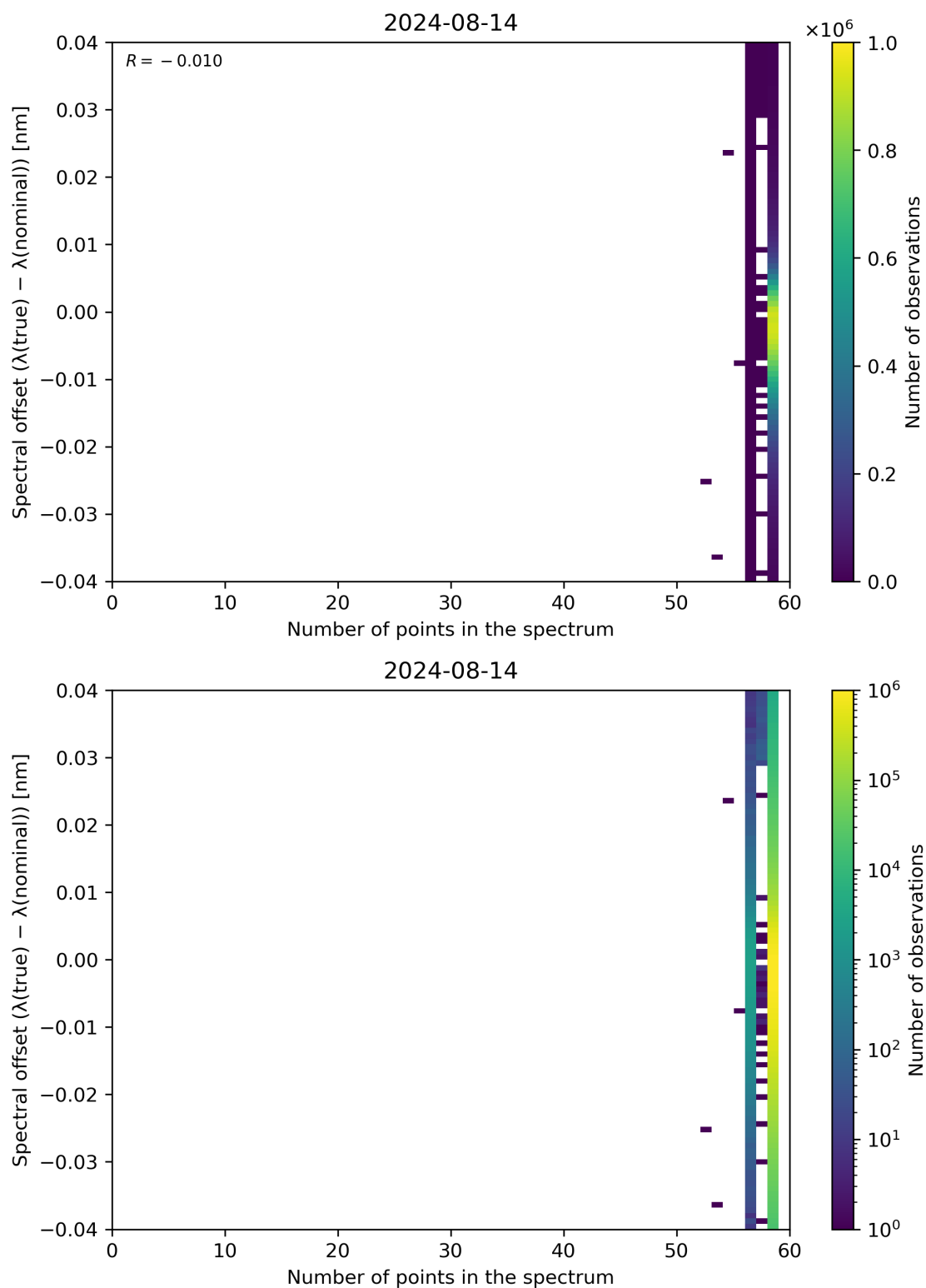
Figure 101: Scatter density plot of “Number of points in the spectrum” against “Spectral offset ( \lambda(\text{true}) - \lambda(\text{nominal}) )” for 2024-08-13 to 2024-08-15.
