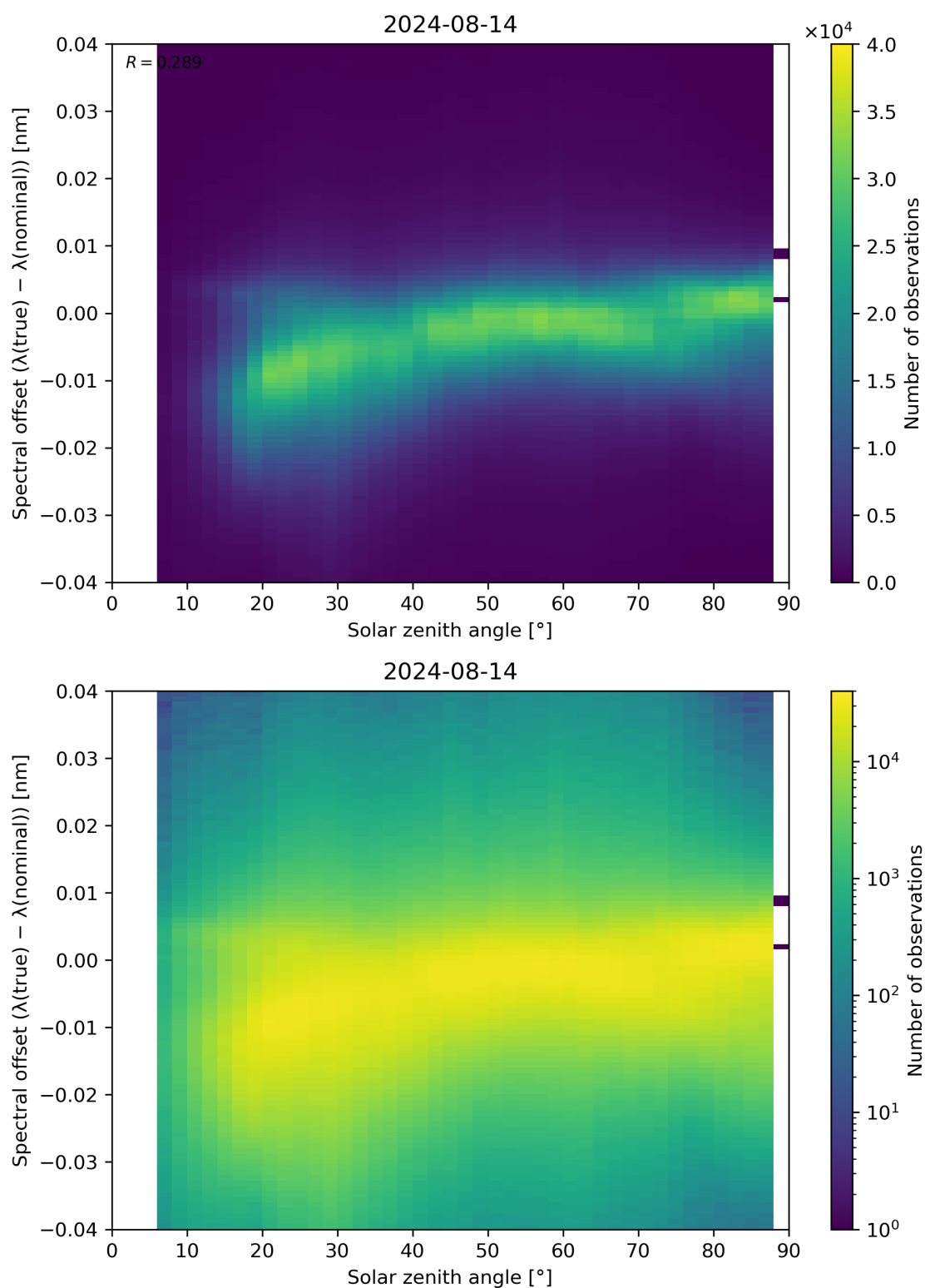
Figure 117: Scatter density plot of “Solar zenith angle” against “Spectral offset ( \lambda(\text{true}) - \lambda(\text{nominal}) )” for 2024-08-13 to 2024-08-15.
