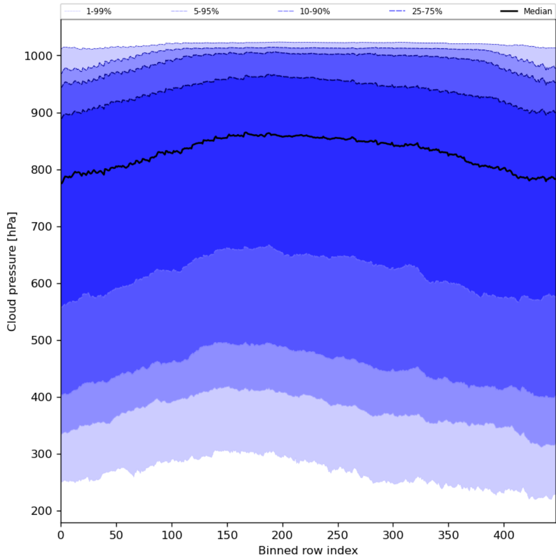
Figure 47: Along track statistics of “Cloud pressure” for 2024-08-13 to 2024-08-15
