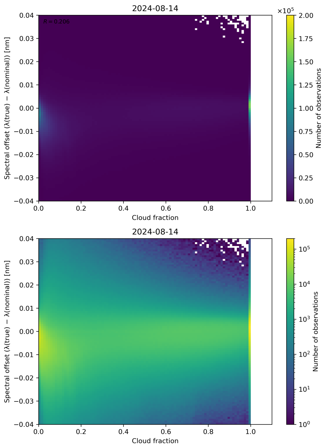
Figure 76: Scatter density plot of “Cloud fraction” against “Spectral offset ( \lambda(\text{true}) - \lambda(\text{nominal}) )” for 2024-08-13 to 2024-08-15.
