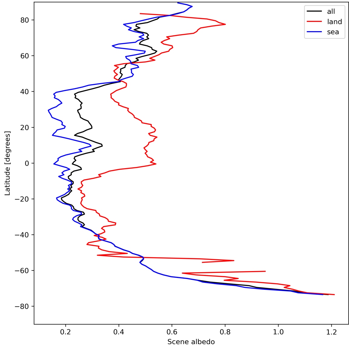
Figure 17: Zonal average of “Scene albedo” for 2024-08-13 to 2024-08-15.
