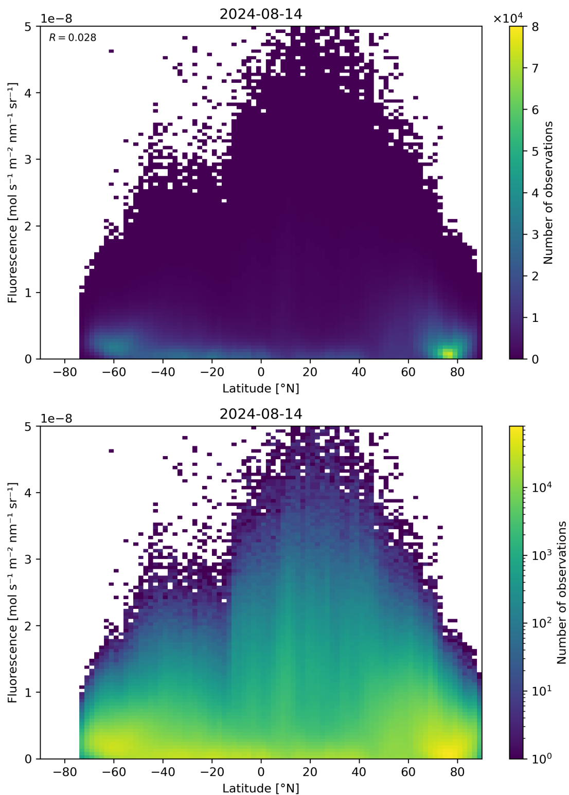
Figure 92: Scatter density plot of “Latitude” against “Fluorescence” for 2024-08-13 to 2024-08-15.
