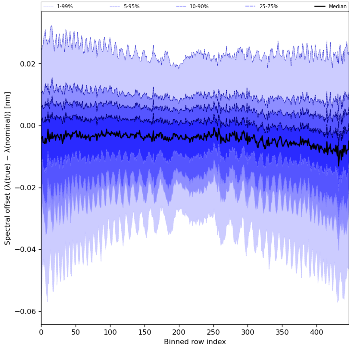
Figure 62: Along track statistics of “Spectral offset ( \lambda(\text{true}) - \lambda(\text{nominal}) )” for 2024-08-13 to 2024-08-15
