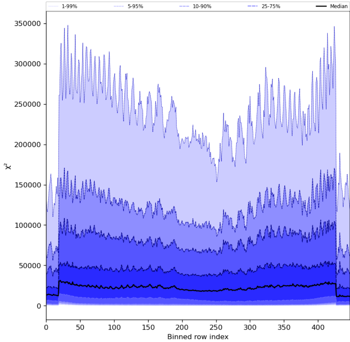
Figure 55: Along track statistics of “ \chi^2 ” for 2024-08-13 to 2024-08-15
