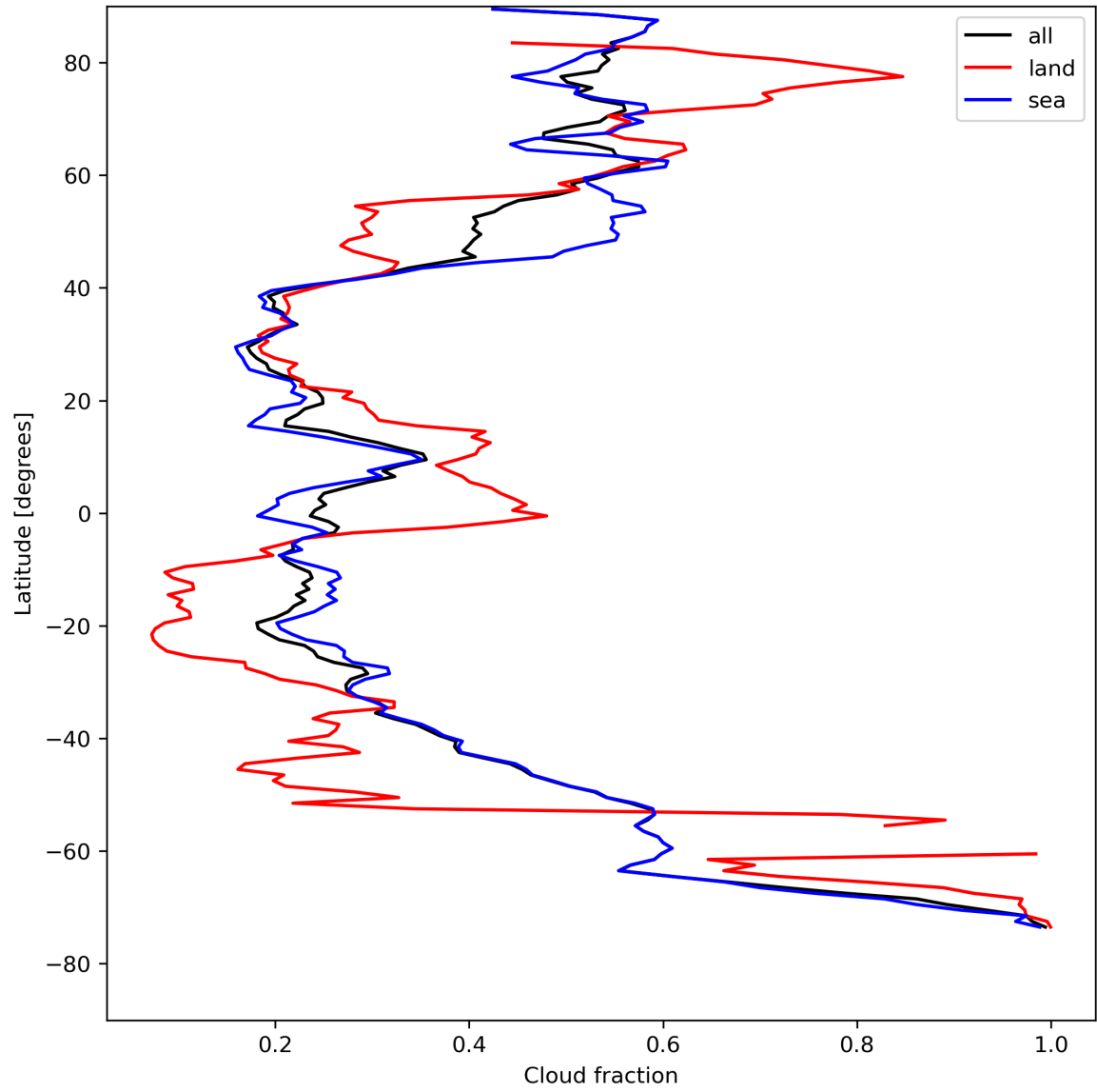
Figure 15: Zonal average of “Cloud fraction” for 2024-08-13 to 2024-08-15.
