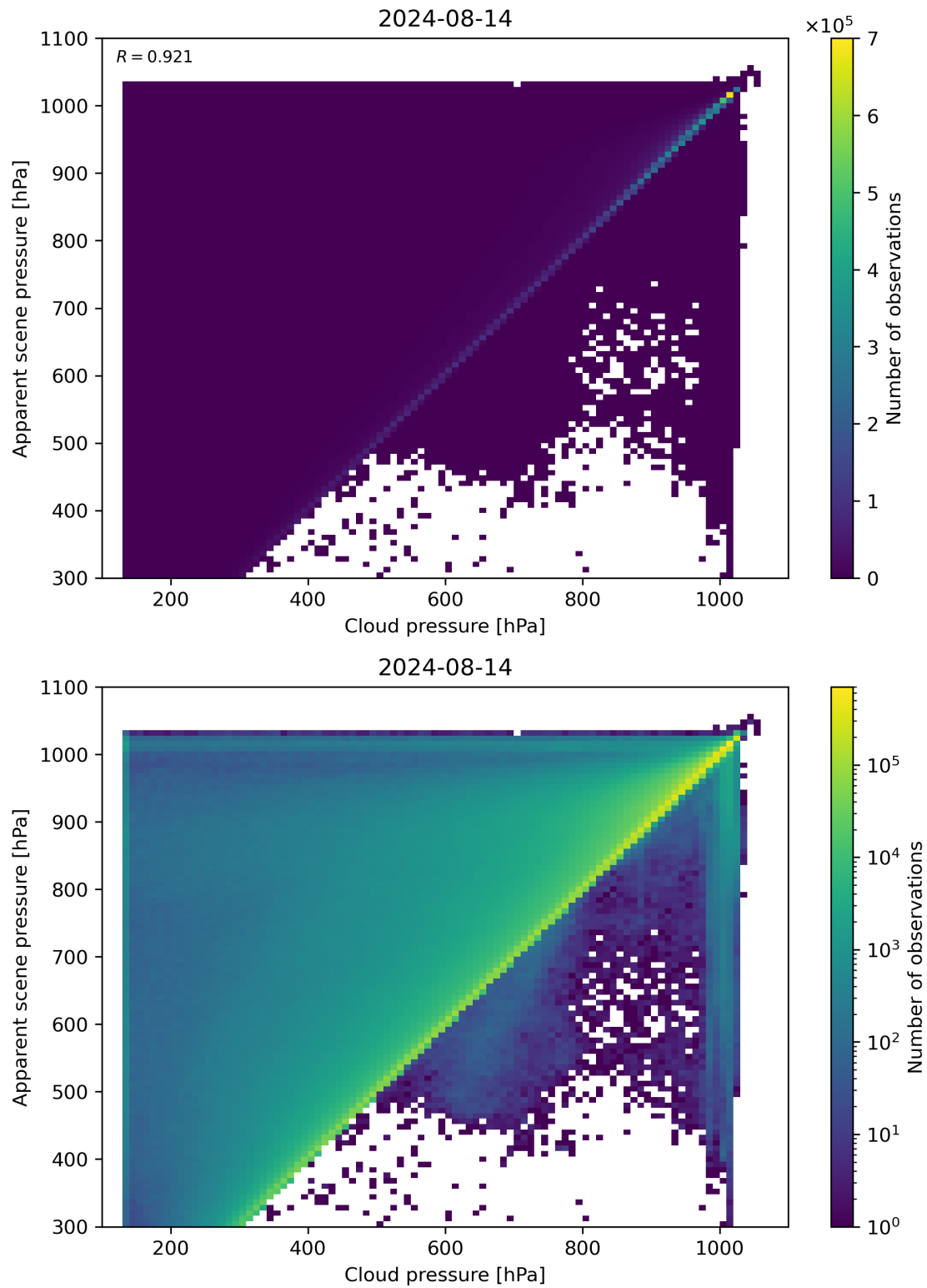
Figure 77: Scatter density plot of “Cloud pressure” against “Apparent scene pressure” for 2024-08-13 to 2024-08-15.
