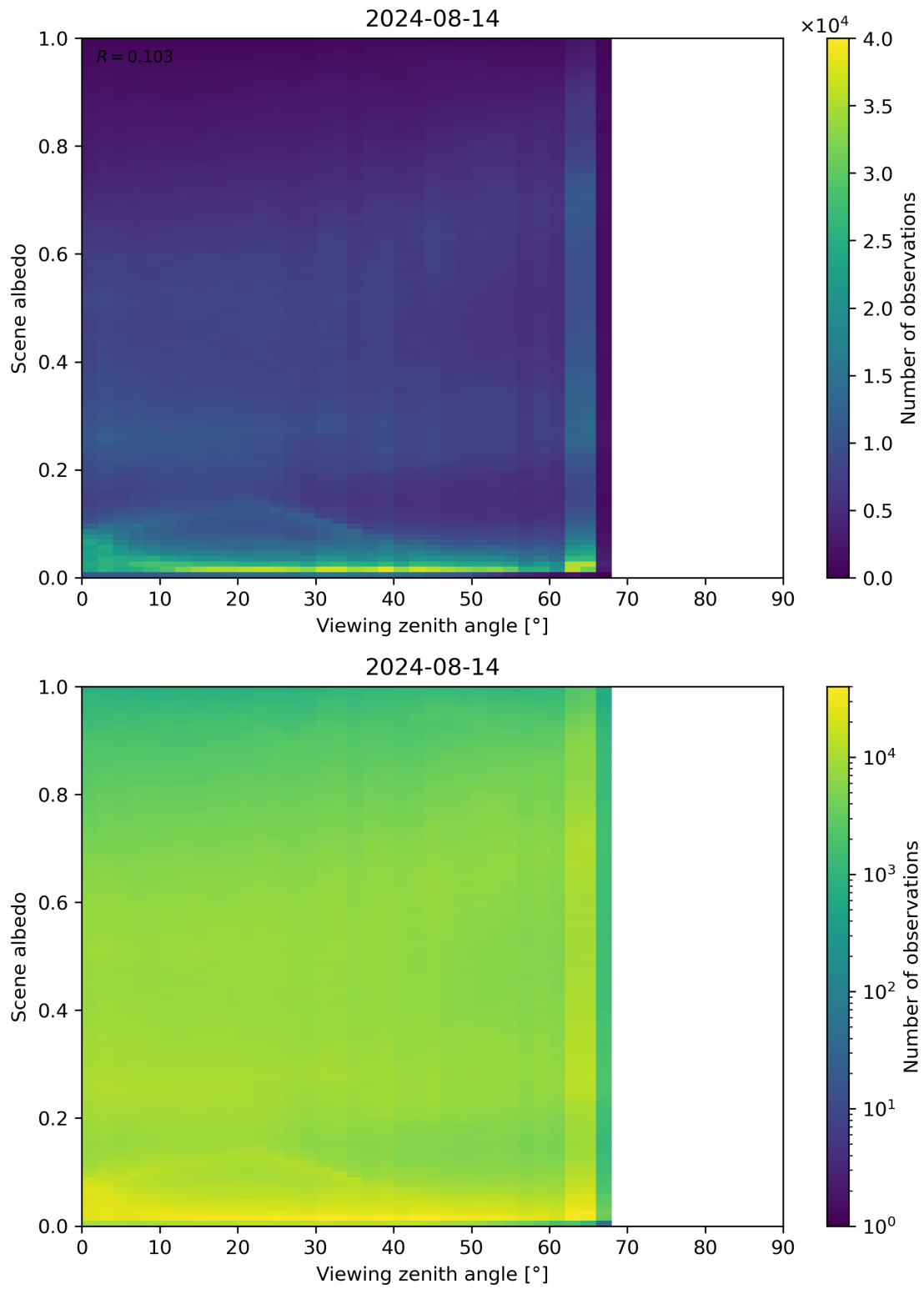
Figure 126: Scatter density plot of “Viewing zenith angle” against “Scene albedo” for 2024-08-13 to 2024-08-15.
