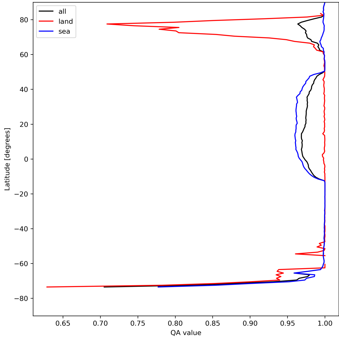
Figure 12: Zonal average of “QA value” for 2024-08-13 to 2024-08-15.
