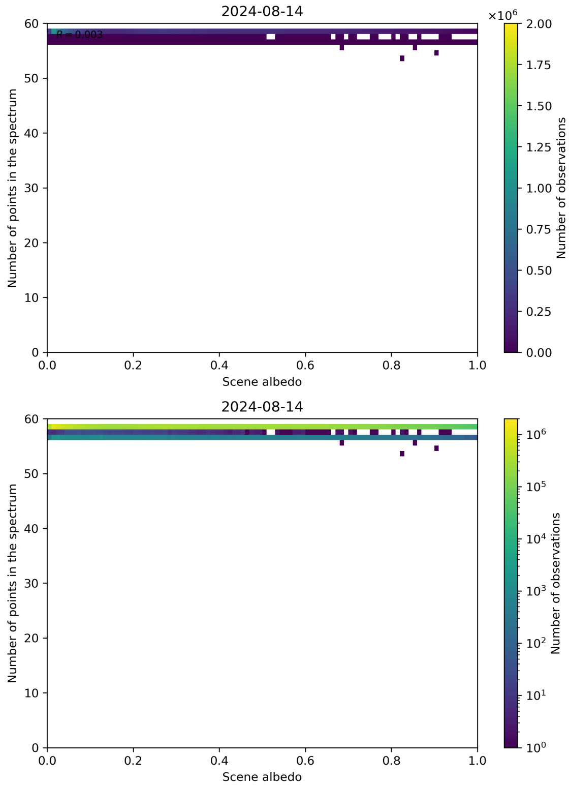
Figure 106: Scatter density plot of “Scene albedo” against “Number of points in the spectrum” for 2024-08-13 to 2024-08-15.
