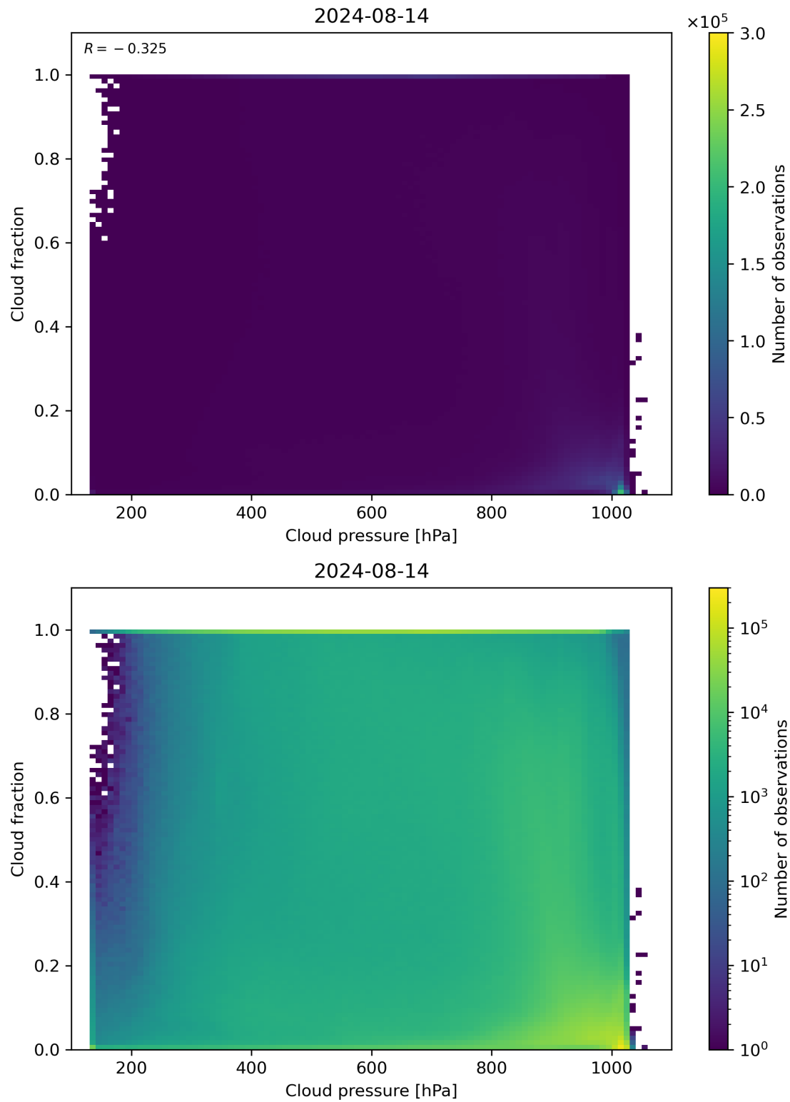
Figure 79: Scatter density plot of “Cloud pressure” against “Cloud fraction” for 2024-08-13 to 2024-08-15.
