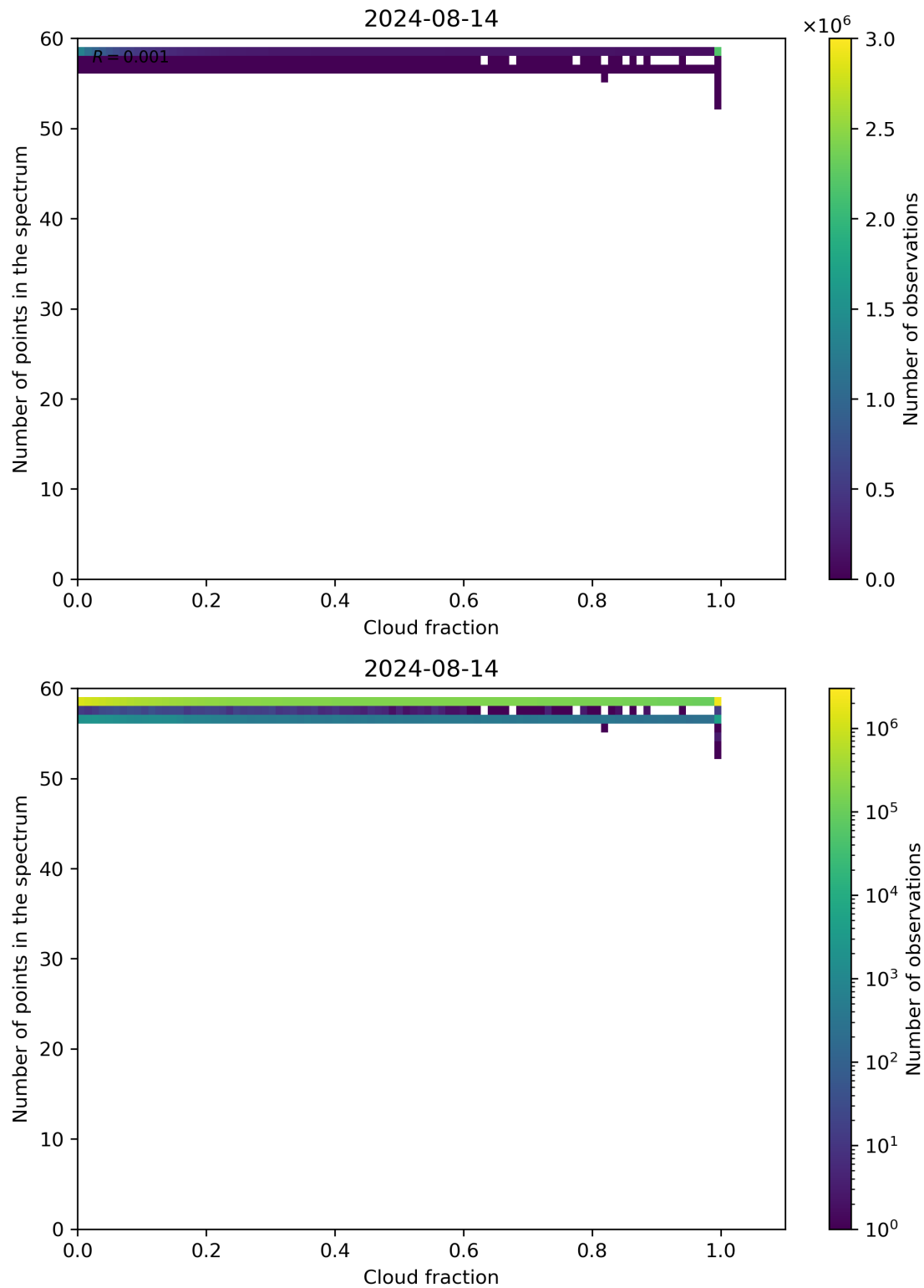
Figure 74: Scatter density plot of “Cloud fraction” against “Number of points in the spectrum” for 2024-08-13 to 2024-08-15.
