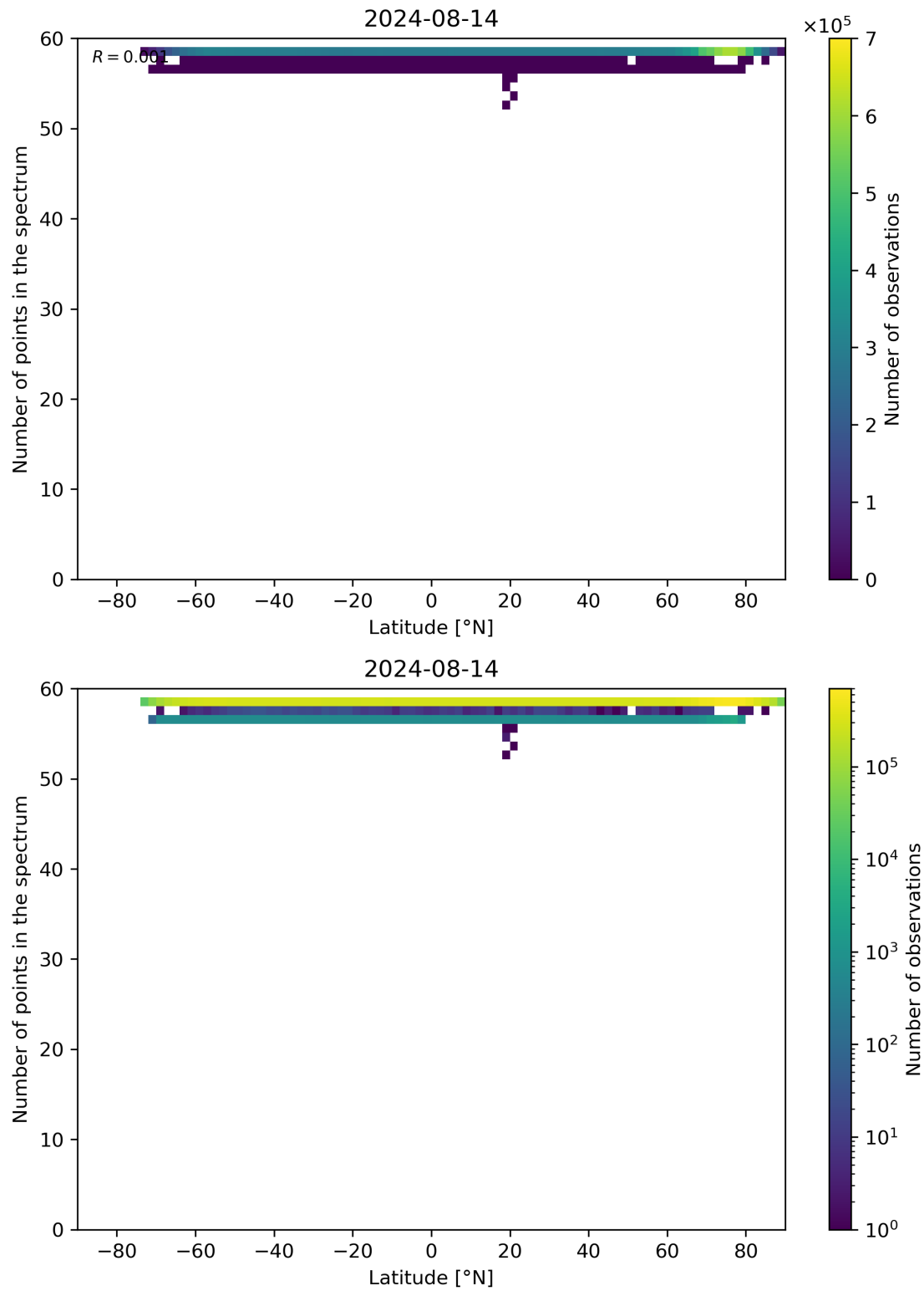
Figure 94: Scatter density plot of “Latitude” against “Number of points in the spectrum” for 2024-08-13 to 2024-08-15.
