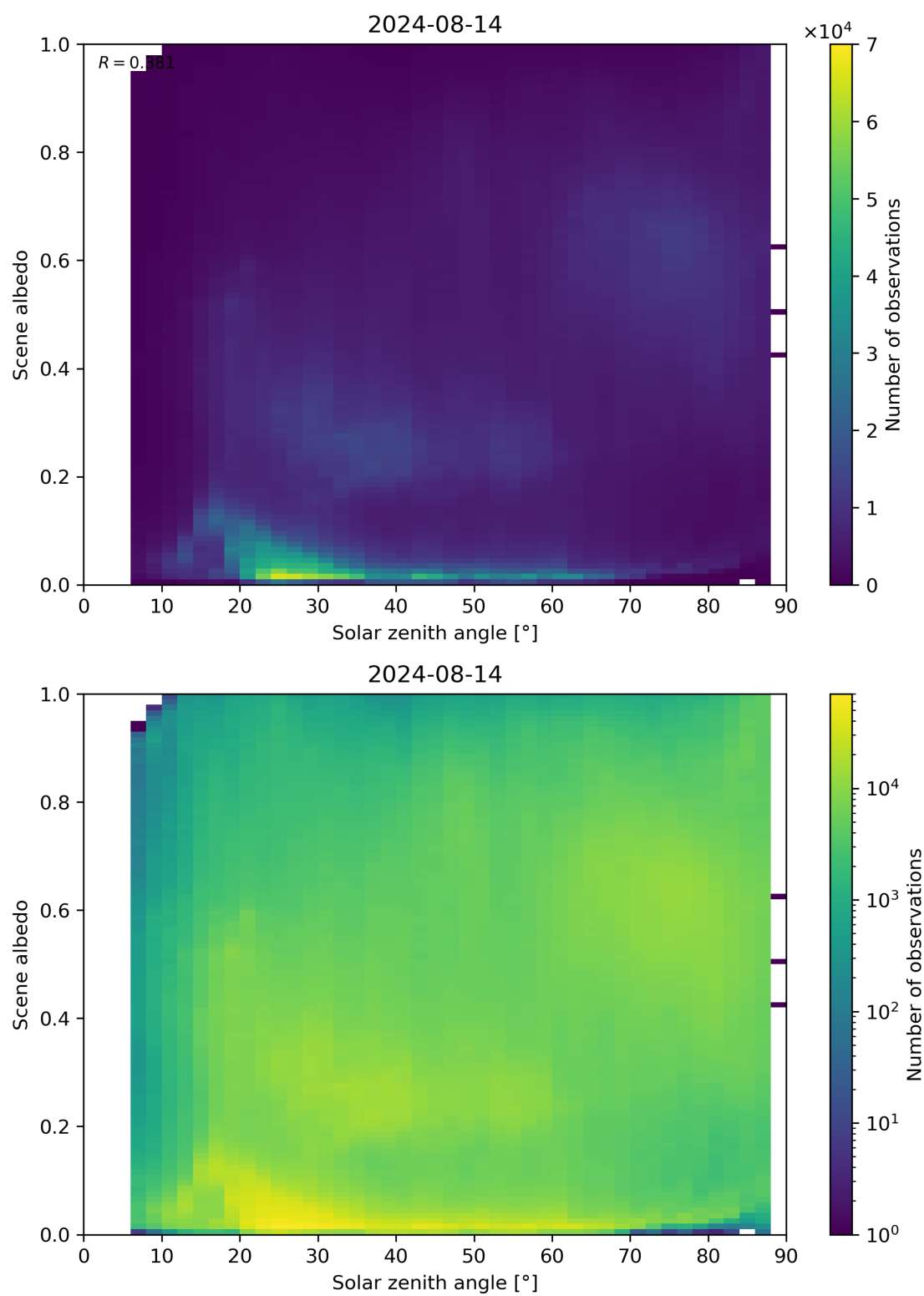
Figure 116: Scatter density plot of “Solar zenith angle” against “Scene albedo” for 2024-08-13 to 2024-08-15.
