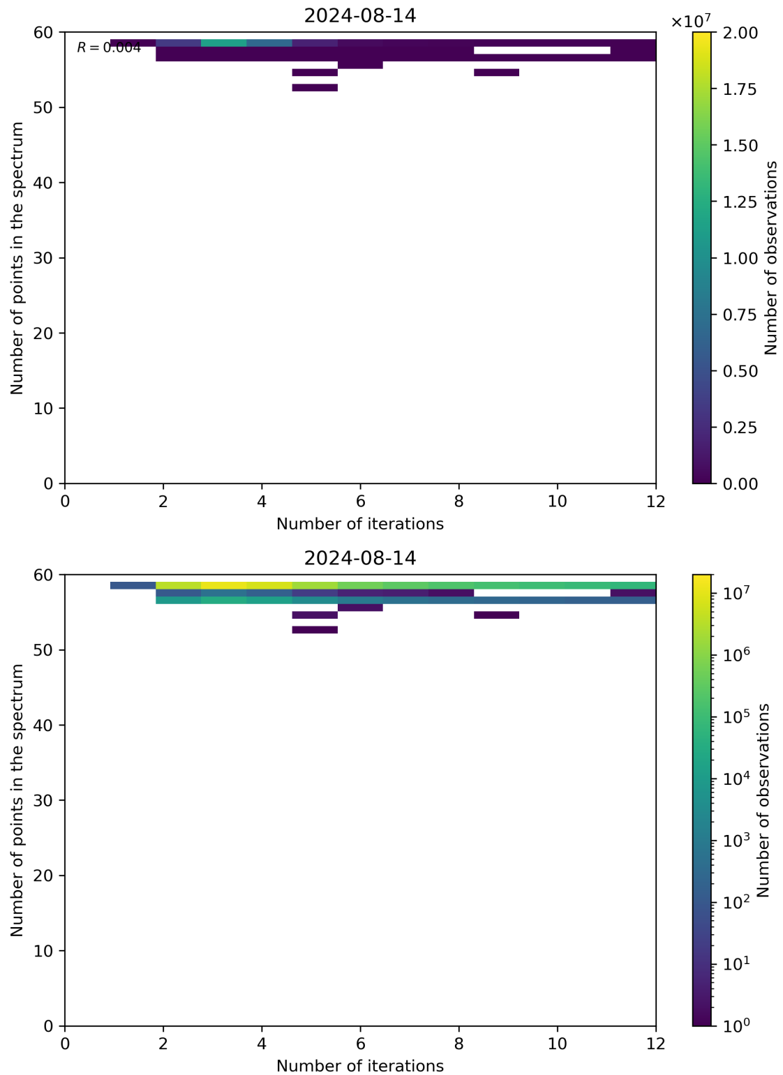
Figure 99: Scatter density plot of “Number of iterations” against “Number of points in the spectrum” for 2024-08-13 to 2024-08-15.
