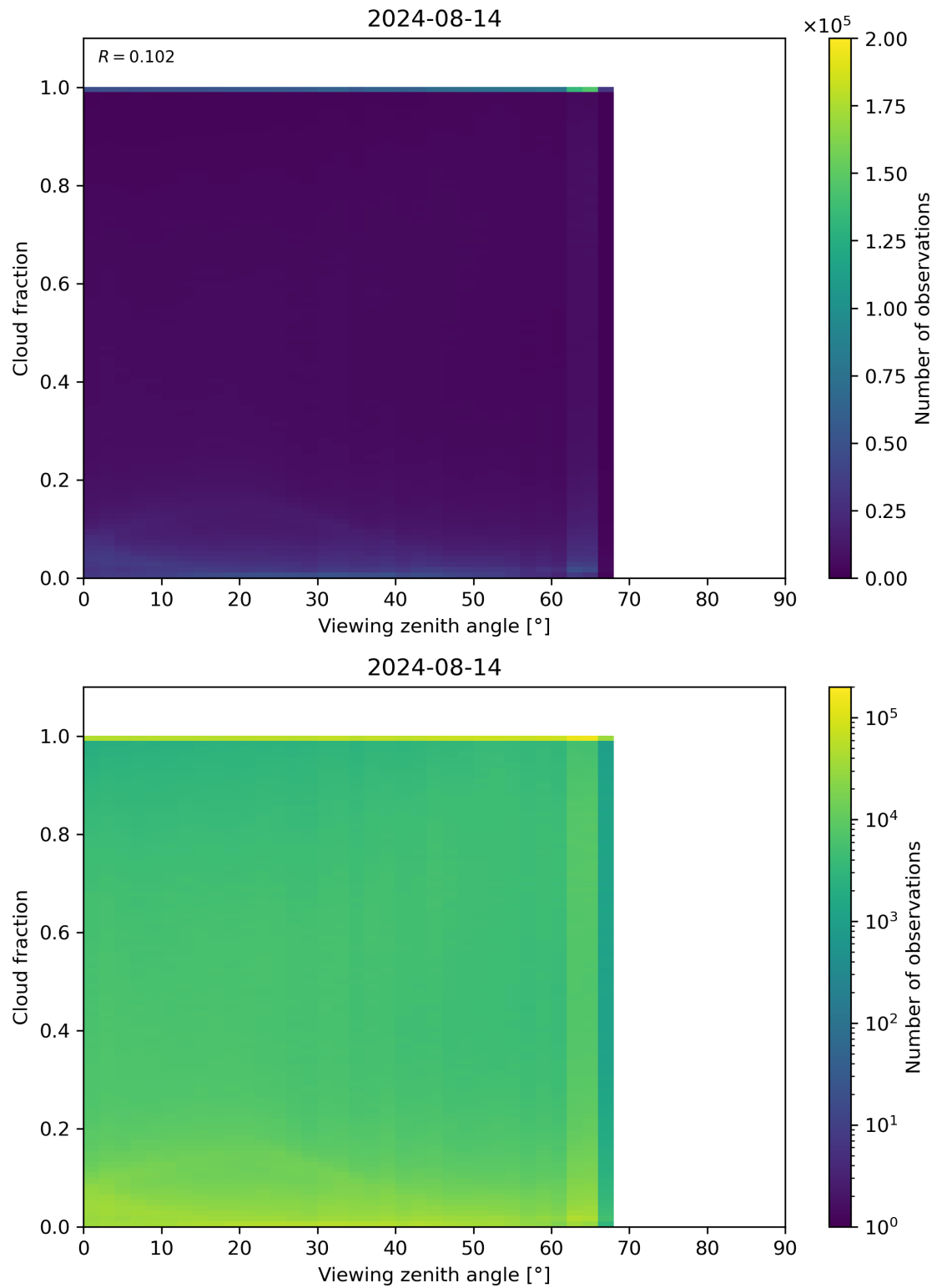
Figure 120: Scatter density plot of “Viewing zenith angle” against “Cloud fraction” for 2024-08-13 to 2024-08-15.
