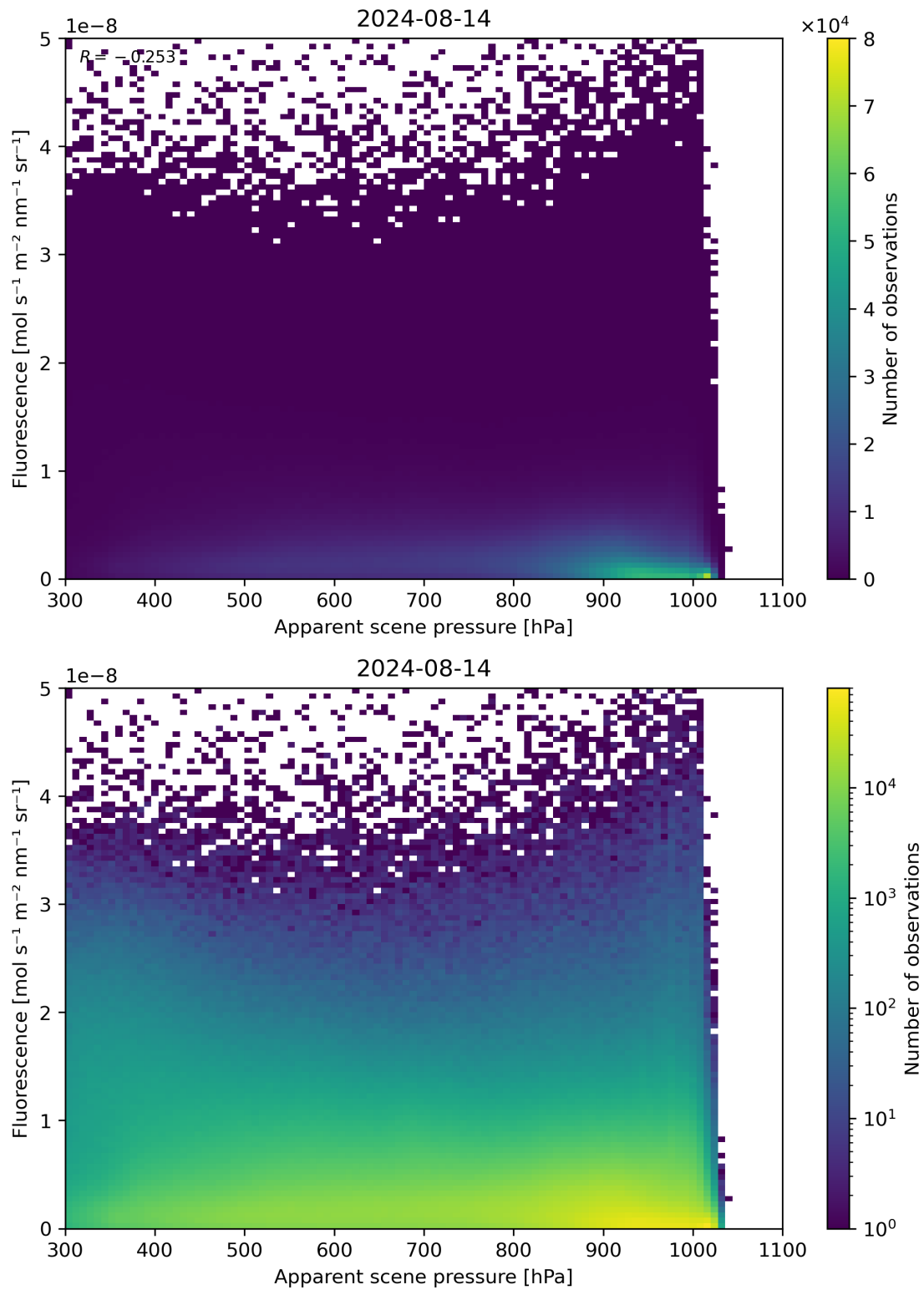
Figure 64: Scatter density plot of “Apparent scene pressure” against “Fluorescence” for 2024-08-13 to 2024-08-15.
