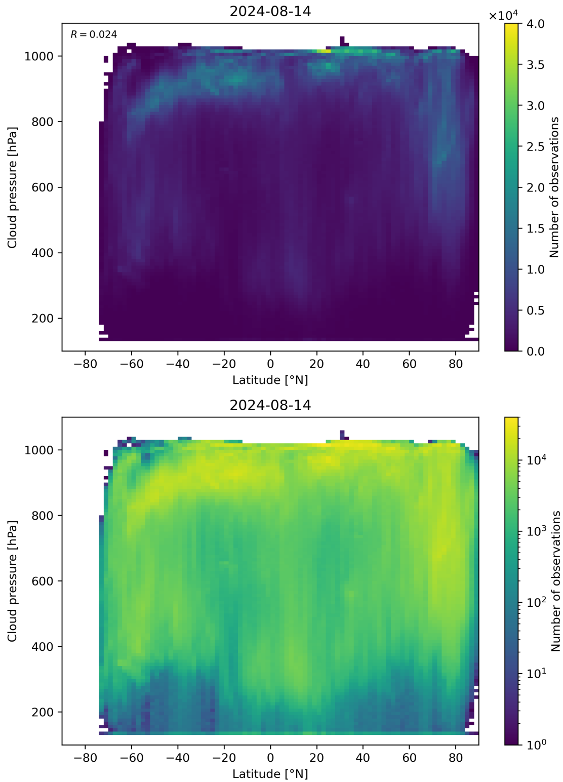
Figure 91: Scatter density plot of “Latitude” against “Cloud pressure” for 2024-08-13 to 2024-08-15.
