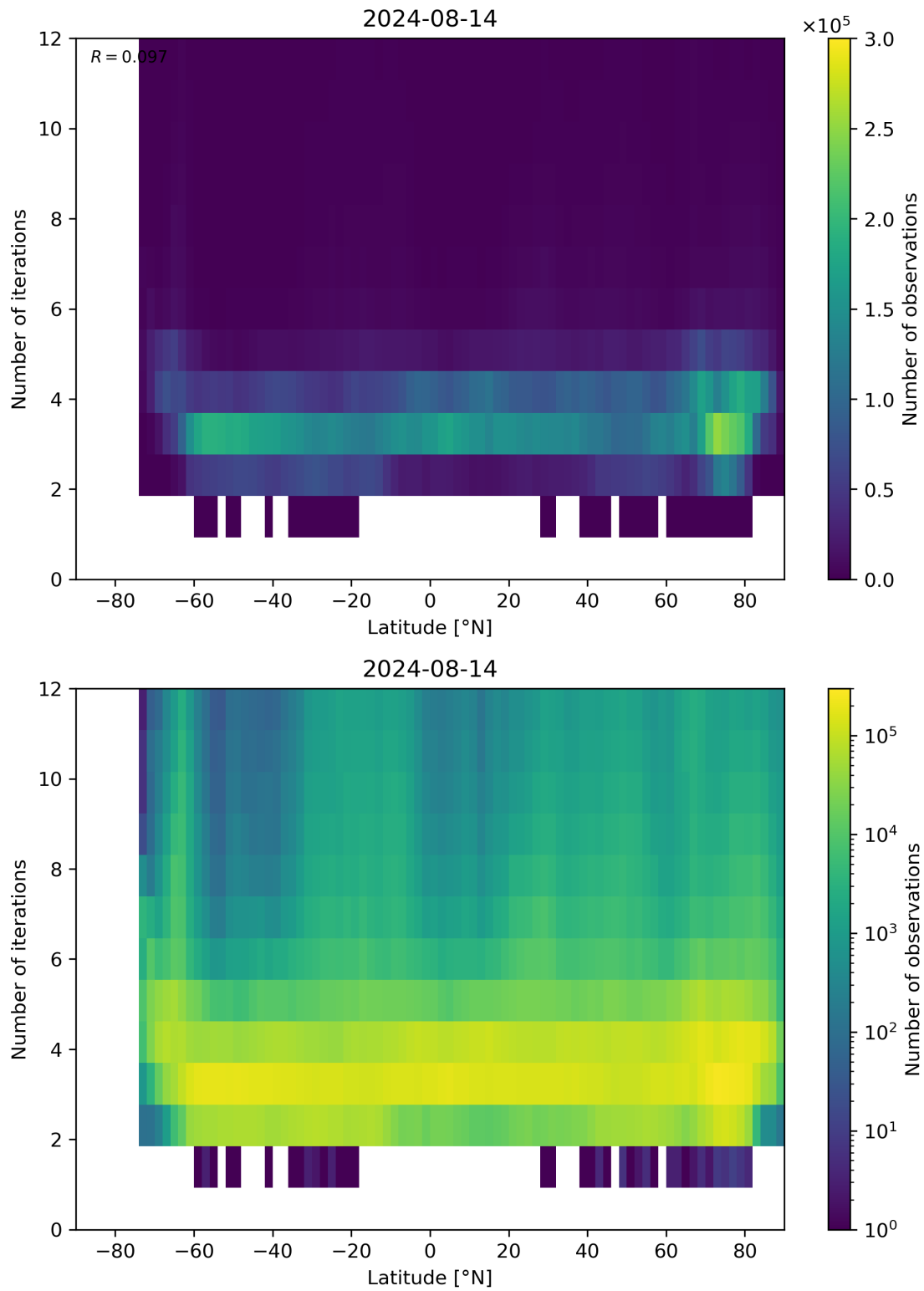
Figure 93: Scatter density plot of “Latitude” against “Number of iterations” for 2024-08-13 to 2024-08-15.
