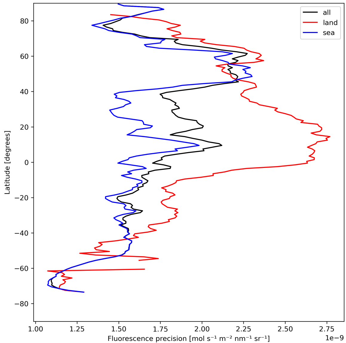
Figure 24: Zonal average of “Fluorescence precision” for 2024-08-13 to 2024-08-15.
