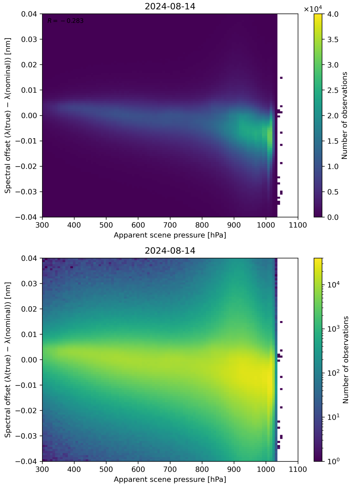
Figure 67: Scatter density plot of “Apparent scene pressure” against “Spectral offset ( \lambda(\text{true}) - \lambda(\text{nominal}) )” for 2024-08-13 to 2024-08-15.
