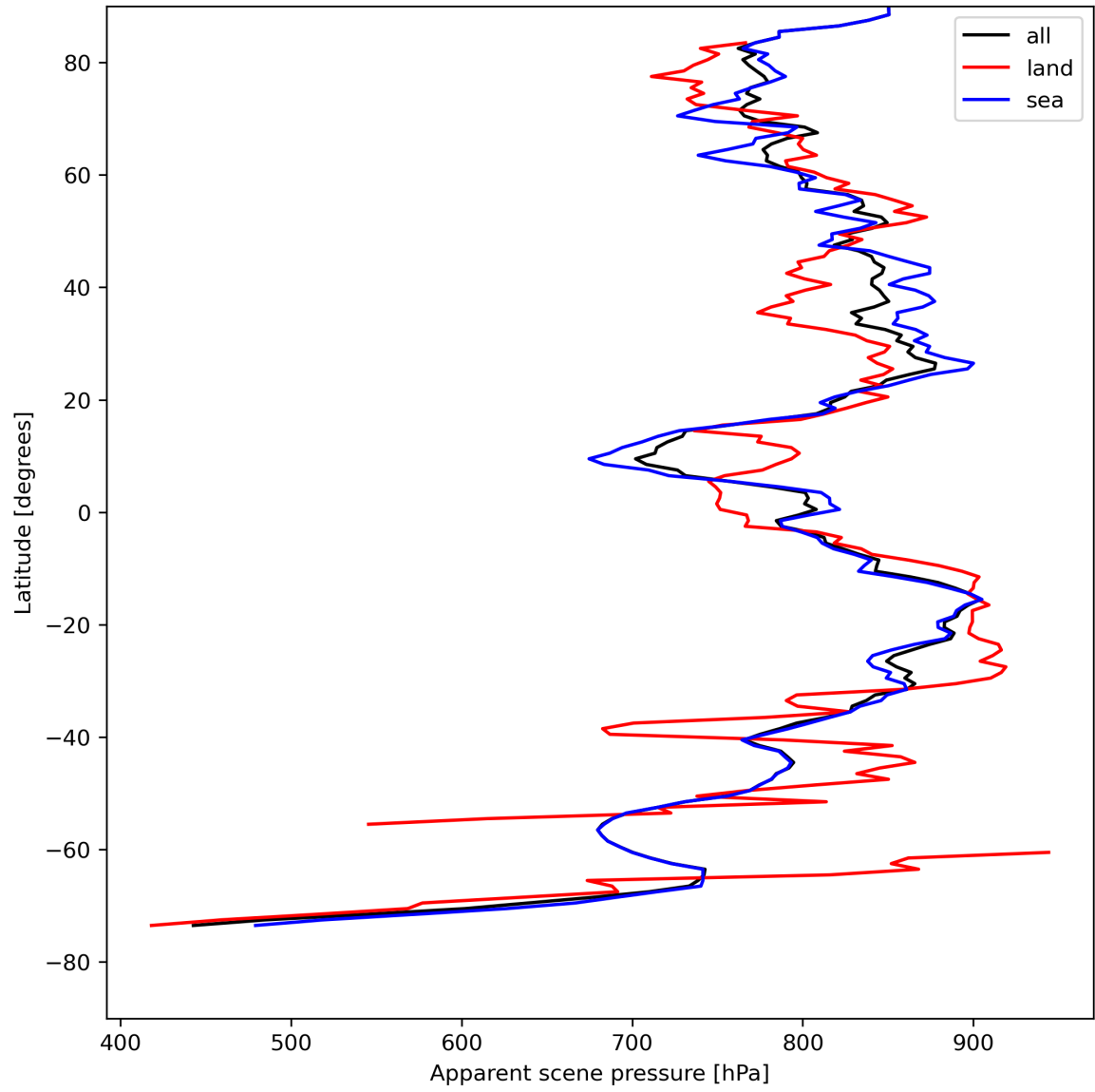
Figure 19: Zonal average of “Apparent scene pressure” for 2024-08-13 to 2024-08-15.
