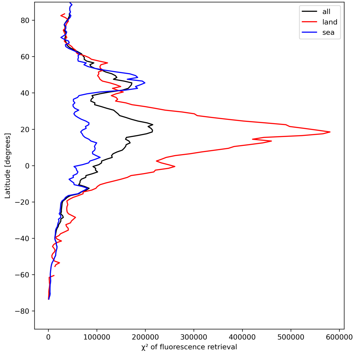
Figure 25: Zonal average of “ \chi^2 of fluorescence retrieval” for 2024-08-13 to 2024-08-15.
