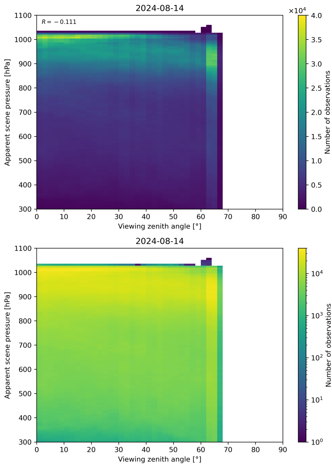
Figure 118: Scatter density plot of “Viewing zenith angle” against “Apparent scene pressure” for 2024-08-13 to 2024-08-15.
