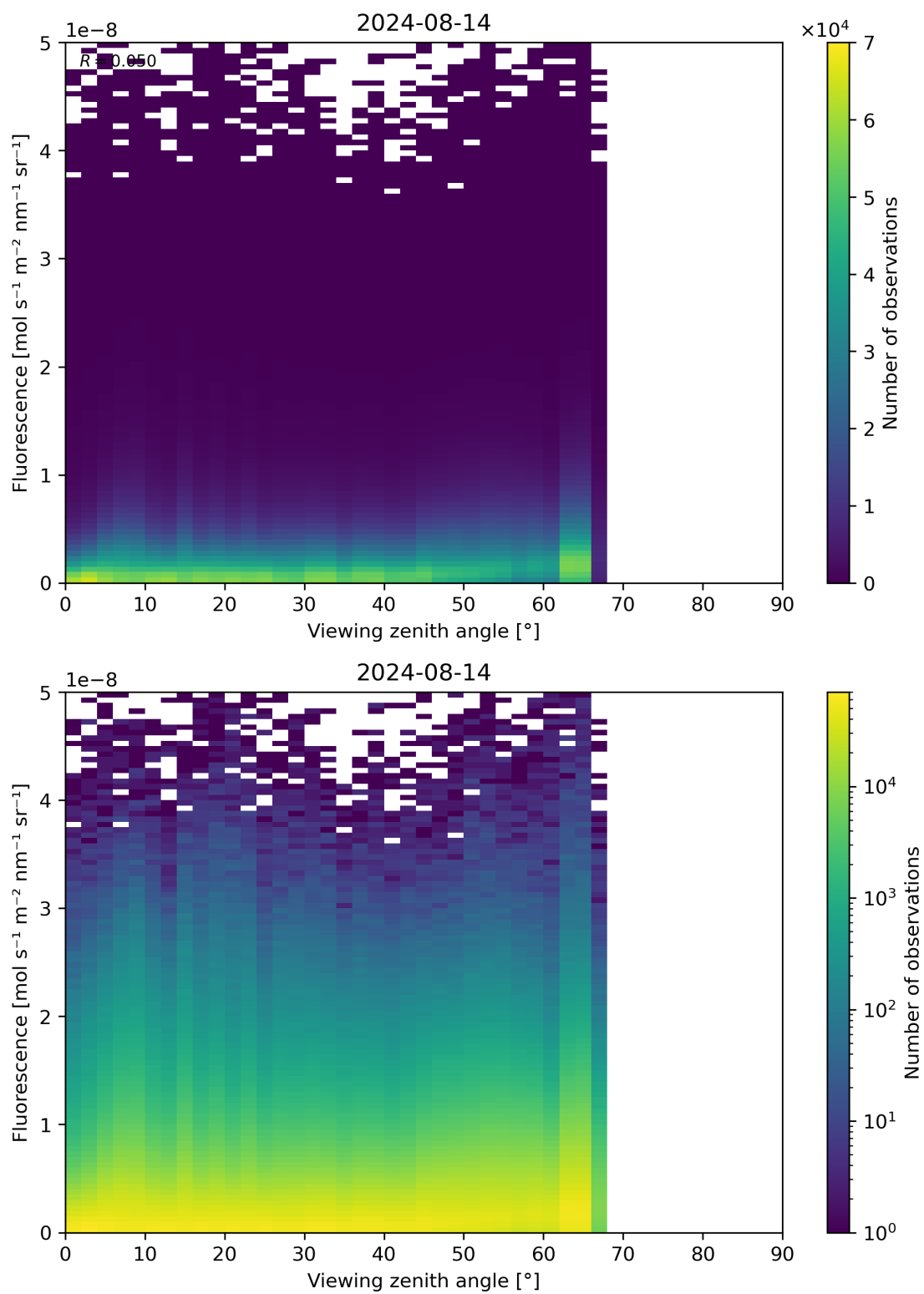
Figure 122: Scatter density plot of “Viewing zenith angle” against “Fluorescence” for 2024-08-13 to 2024-08-15.
