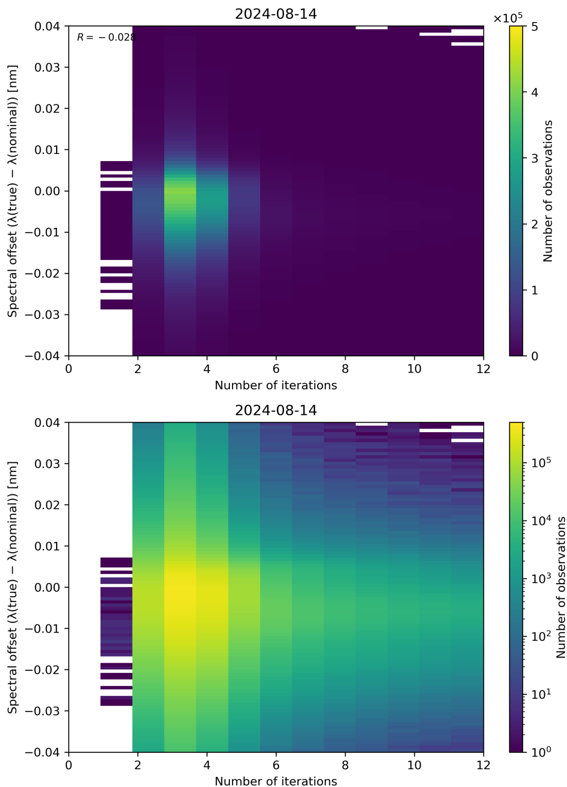
Figure 100: Scatter density plot of “Number of iterations” against “Spectral offset ( \lambda(\text{true}) - \lambda(\text{nominal}) )” for 2024-08-13 to 2024-08-15.
