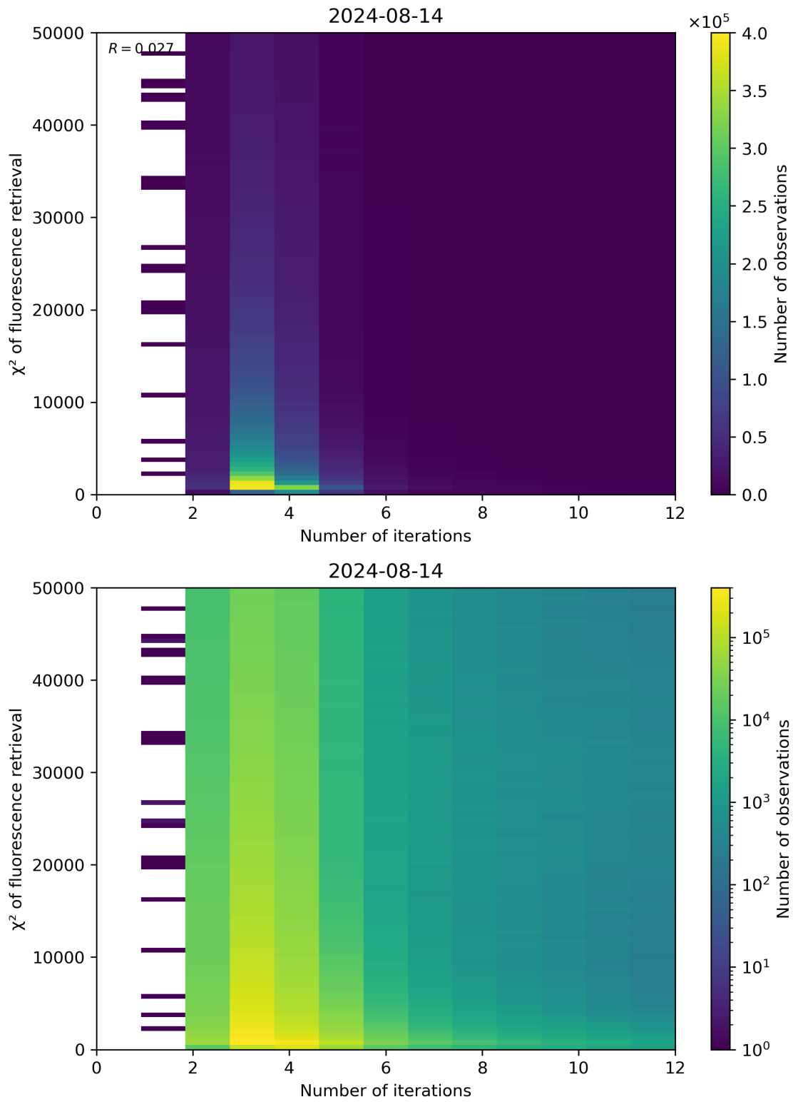
Figure 97: Scatter density plot of “Number of iterations” against “ \chi^2 of fluorescence retrieval” for 2024-08-13 to 2024-08-15.
