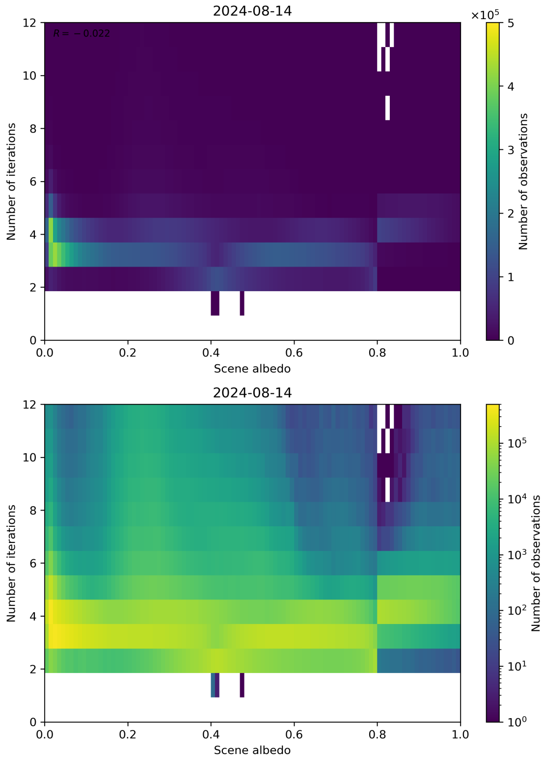
Figure 105: Scatter density plot of “Scene albedo” against “Number of iterations” for 2024-08-13 to 2024-08-15.
