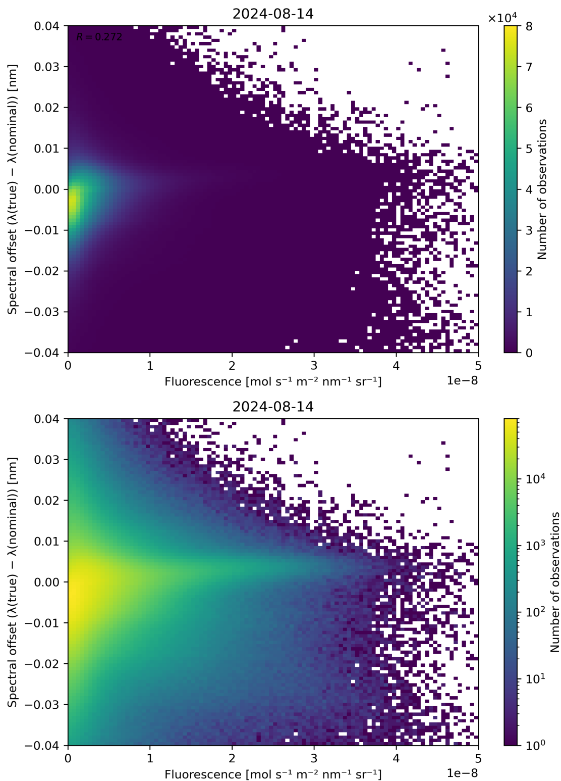
Figure 87: Scatter density plot of “Fluorescence” against “Spectral offset ( \lambda(\text{true}) - \lambda(\text{nominal}) )” for 2024-08-13 to 2024-08-15.
