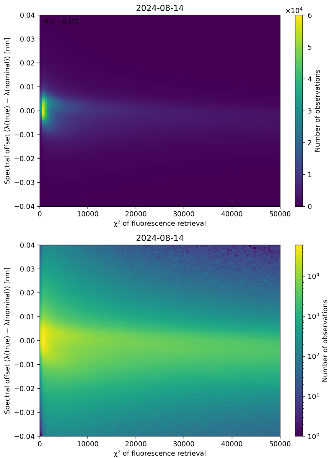
Figure 69: Scatter density plot of " \chi^2 of fluorescence retrieval" against "Spectral offset ( \lambda(\text{true}) - \lambda(\text{nominal}) )" for 2024-08-13 to 2024-08-15.
