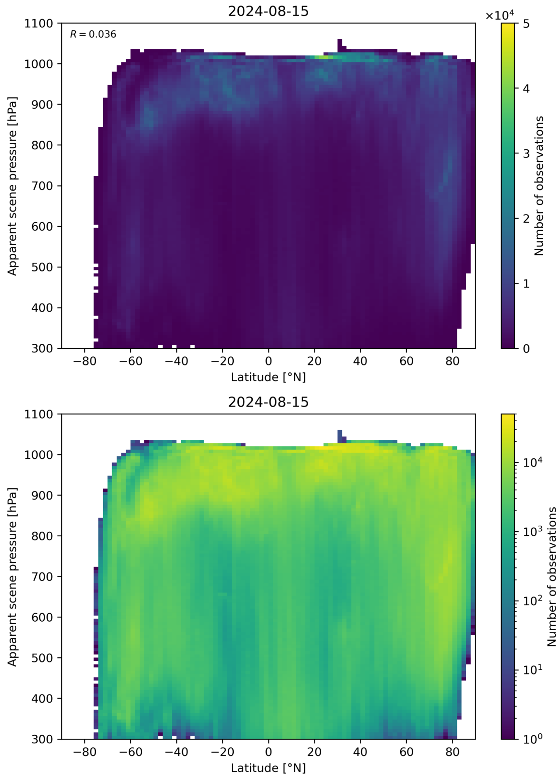
Figure 88: Scatter density plot of “Latitude” against “Apparent scene pressure” for 2024-08-14 to 2024-08-16.
