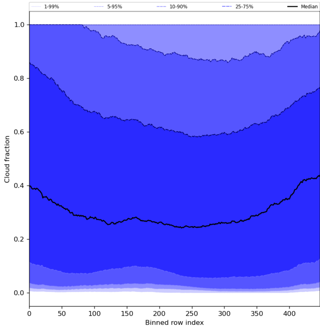
Figure 49: Along track statistics of “Cloud fraction” for 2024-08-14 to 2024-08-16
