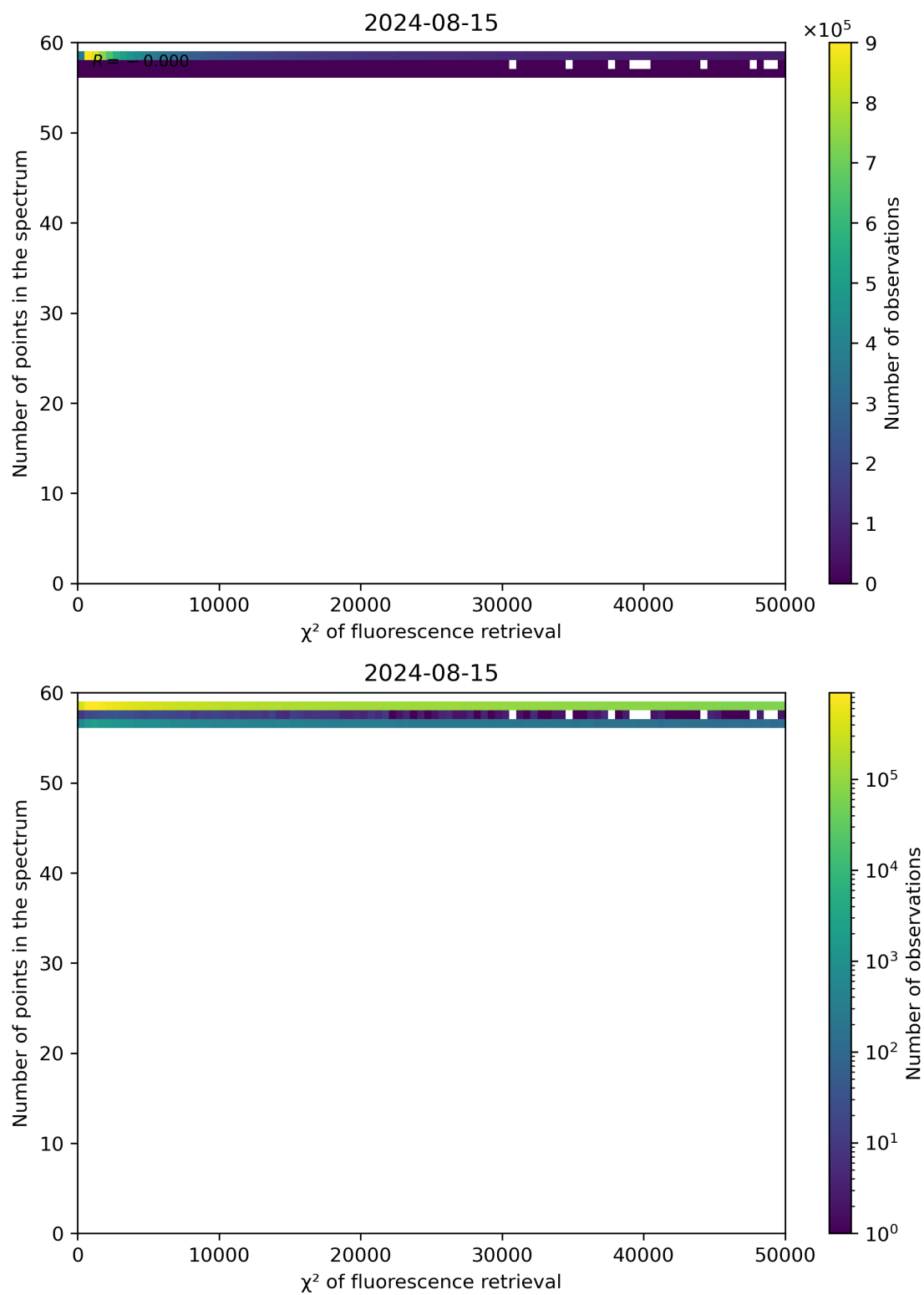
Figure 68: Scatter density plot of " \chi^2 of fluorescence retrieval" against "Number of points in the spectrum" for 2024-08-14 to 2024-08-16.
