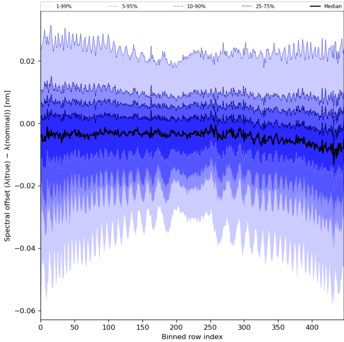
Figure 62: Along track statistics of “Spectral offset ( \lambda(\text{true}) - \lambda(\text{nominal}) )” for 2024-08-14 to 2024-08-16
