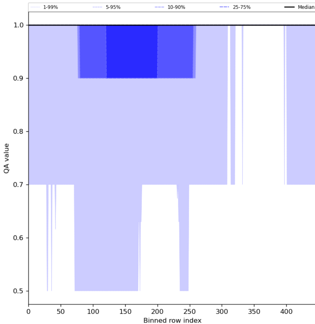
Figure 46: Along track statistics of “QA value” for 2024-08-14 to 2024-08-16
