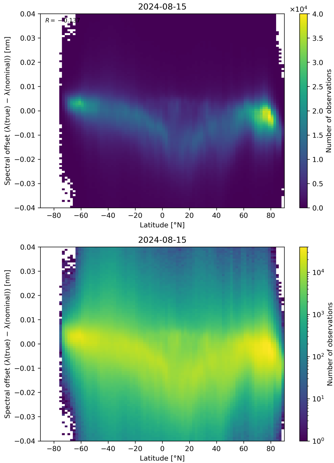
Figure 96: Scatter density plot of “Latitude” against “Spectral offset ( \lambda(\text{true}) - \lambda(\text{nominal}) )” for 2024-08-14 to 2024-08-16.
