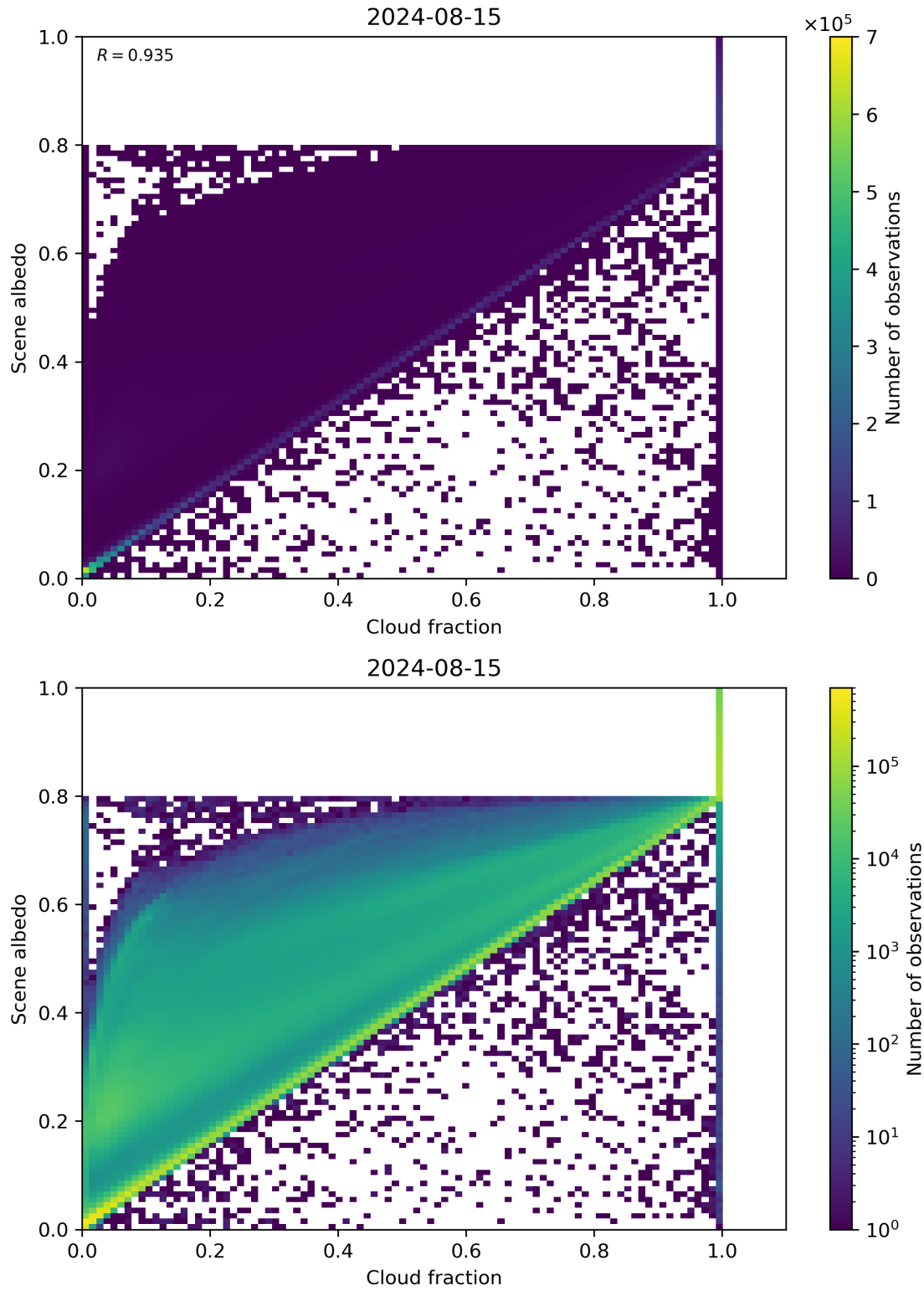
Figure 75: Scatter density plot of “Cloud fraction” against “Scene albedo” for 2024-08-14 to 2024-08-16.
