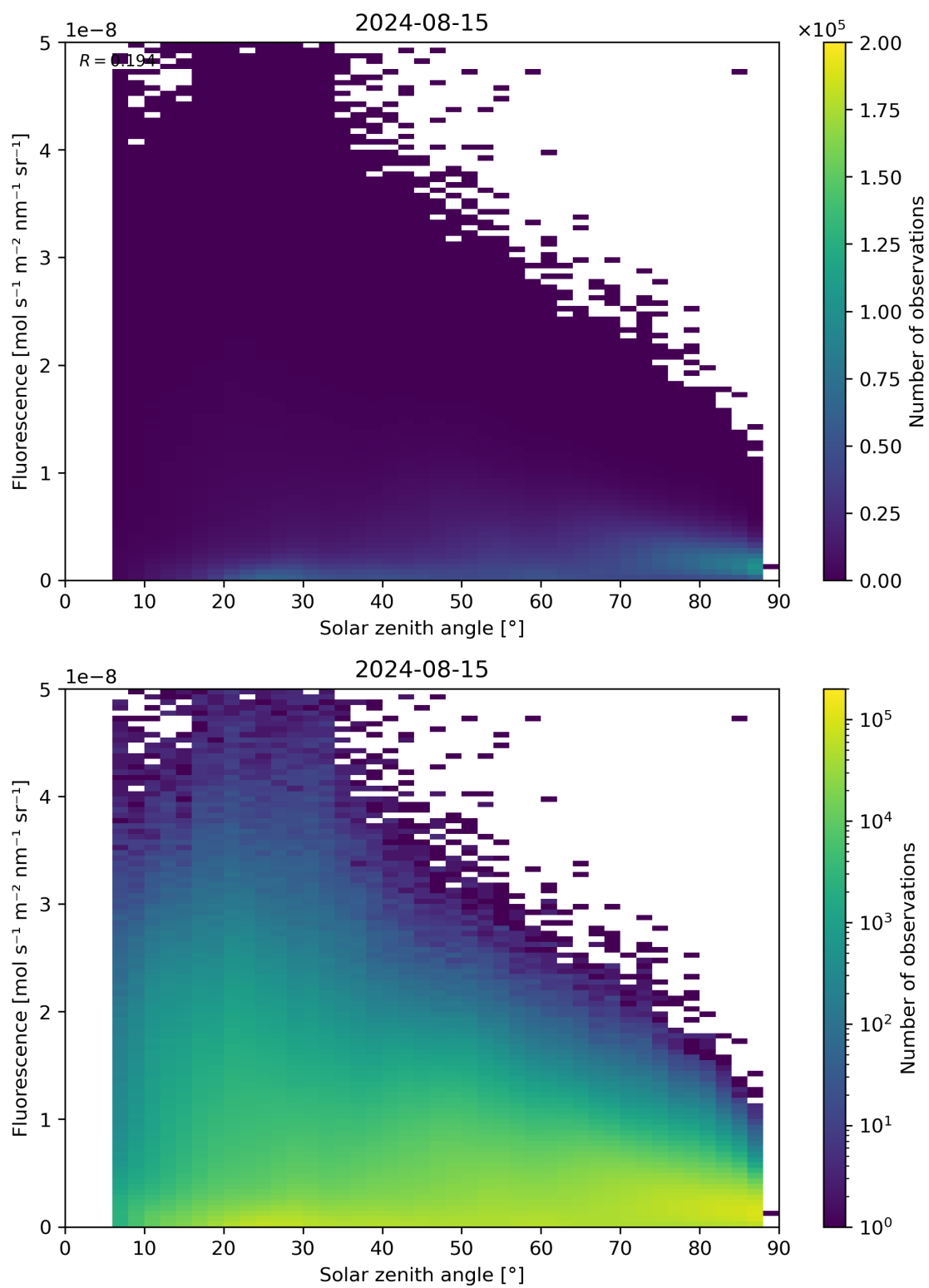
Figure 112: Scatter density plot of “Solar zenith angle” against “Fluorescence” for 2024-08-14 to 2024-08-16.
