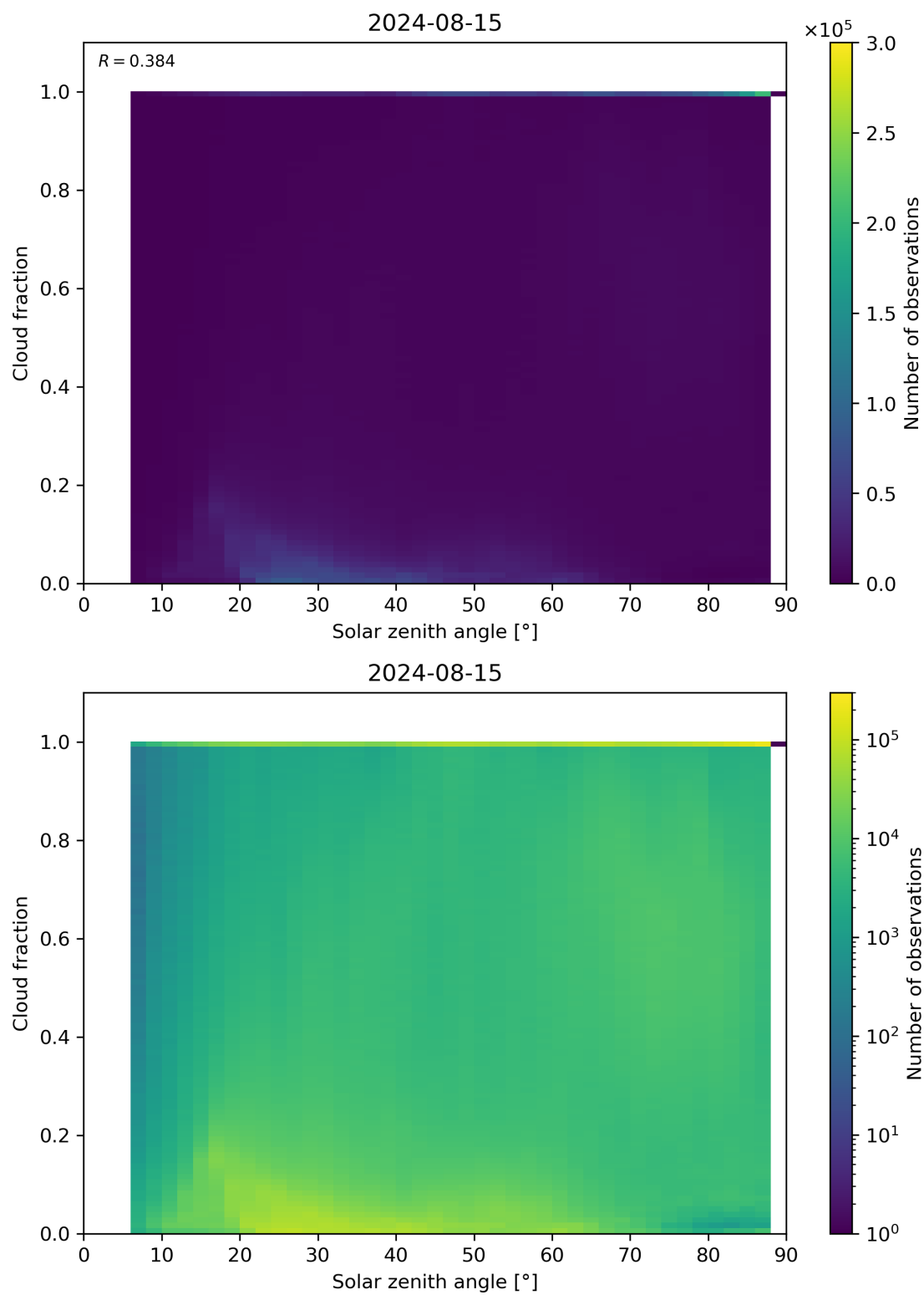
Figure 110: Scatter density plot of “Solar zenith angle” against “Cloud fraction” for 2024-08-14 to 2024-08-16.
