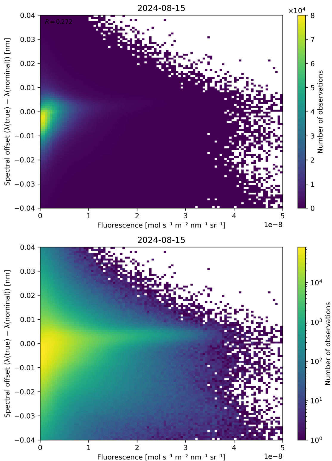
Figure 87: Scatter density plot of “Fluorescence” against “Spectral offset ( \lambda(\text{true}) - \lambda(\text{nominal}) )” for 2024-08-14 to 2024-08-16.
