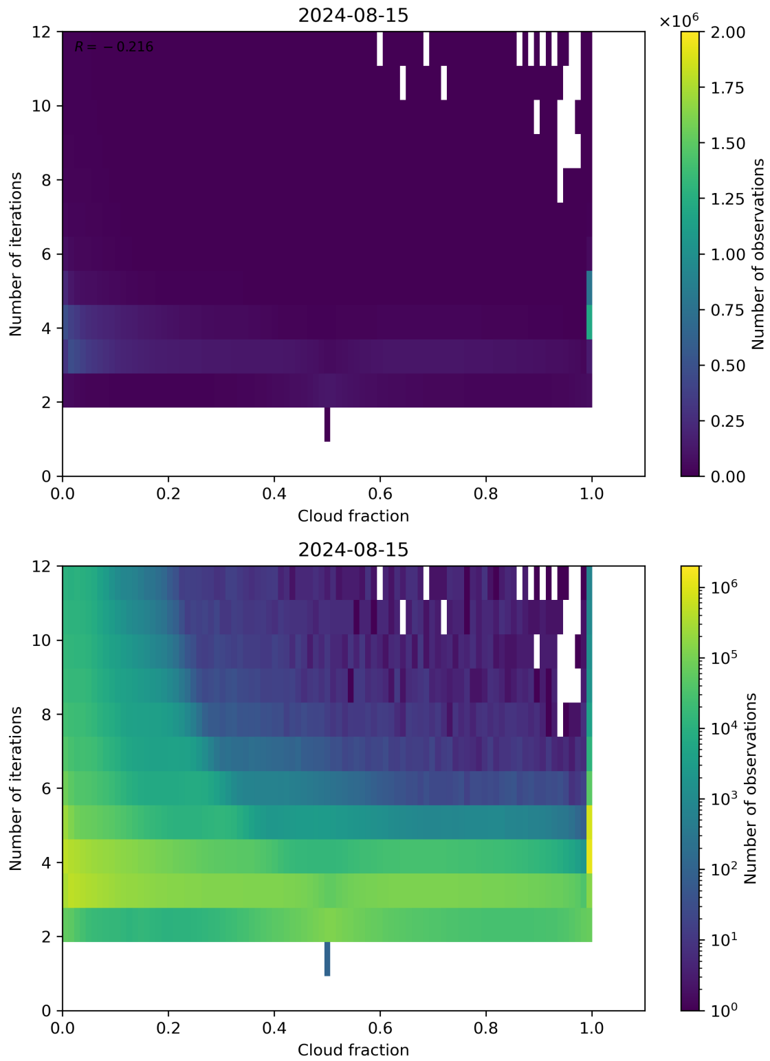
Figure 73: Scatter density plot of “Cloud fraction” against “Number of iterations” for 2024-08-14 to 2024-08-16.
