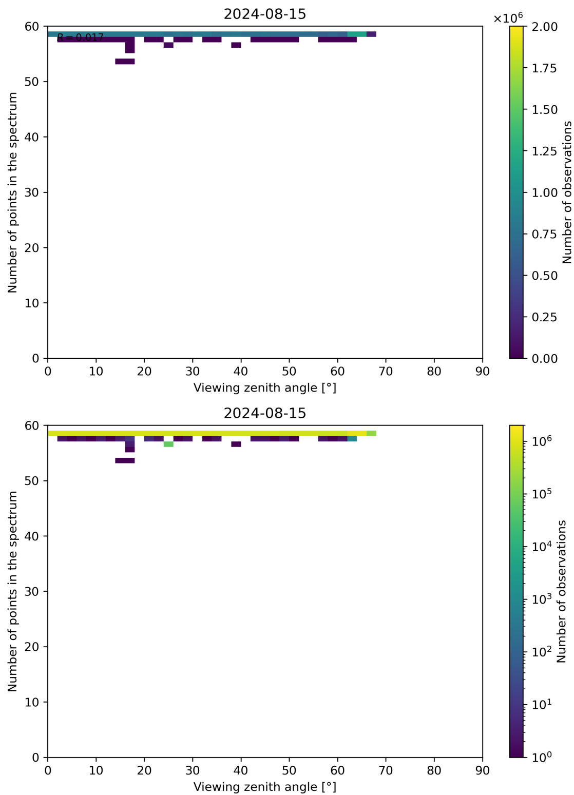
Figure 125: Scatter density plot of “Viewing zenith angle” against “Number of points in the spectrum” for 2024-08-14 to 2024-08-16.
