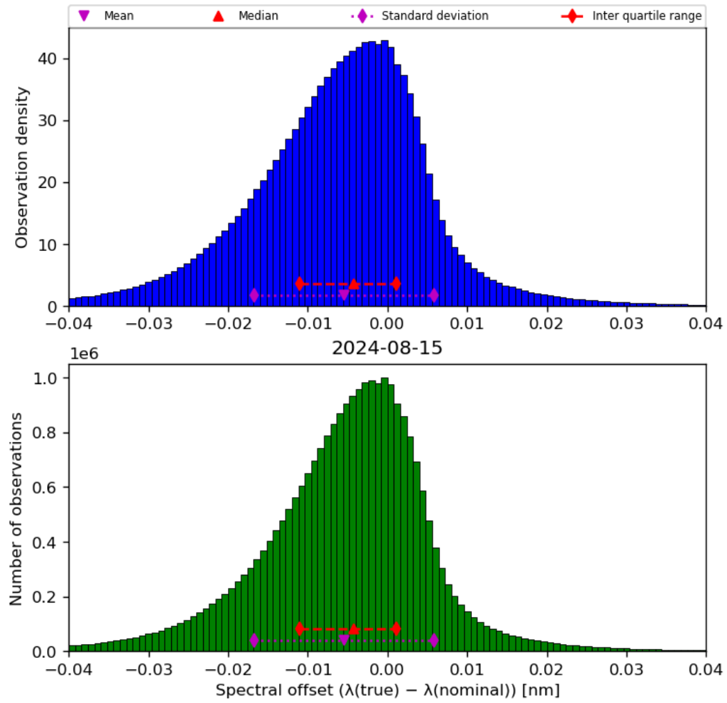
Figure 45: Histogram of “Spectral offset ( \lambda(\text{true}) - \lambda(\text{nominal}) )” for 2024-08-14 to 2024-08-16
