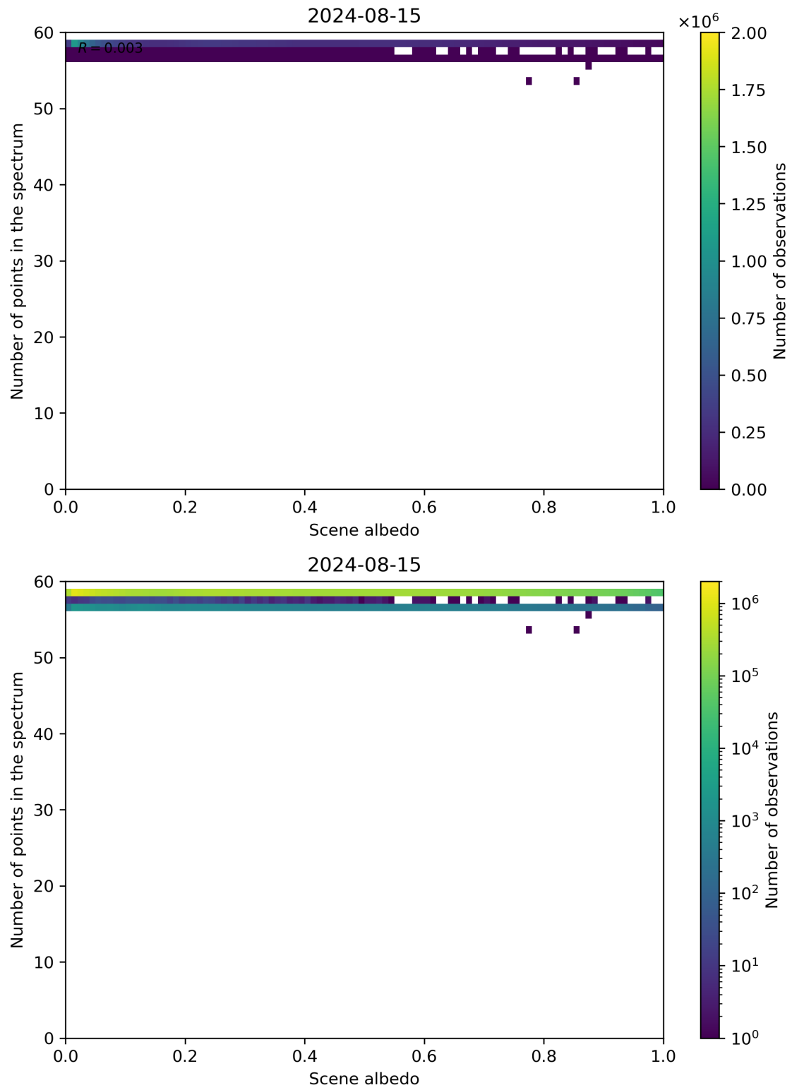
Figure 106: Scatter density plot of “Scene albedo” against “Number of points in the spectrum” for 2024-08-14 to 2024-08-16.
