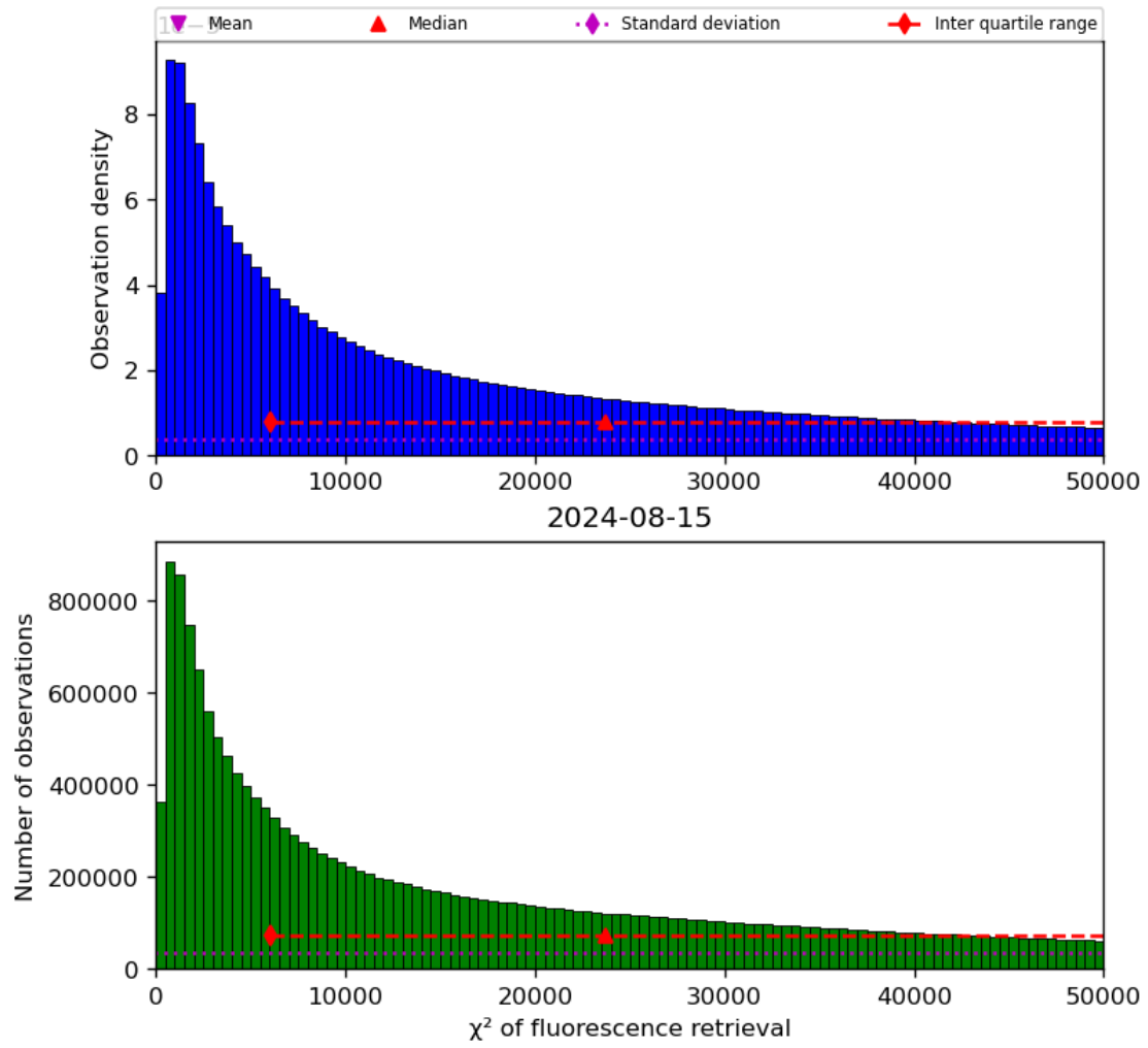
Figure 42: Histogram of “ \chi^2 of fluorescence retrieval” for 2024-08-14 to 2024-08-16
