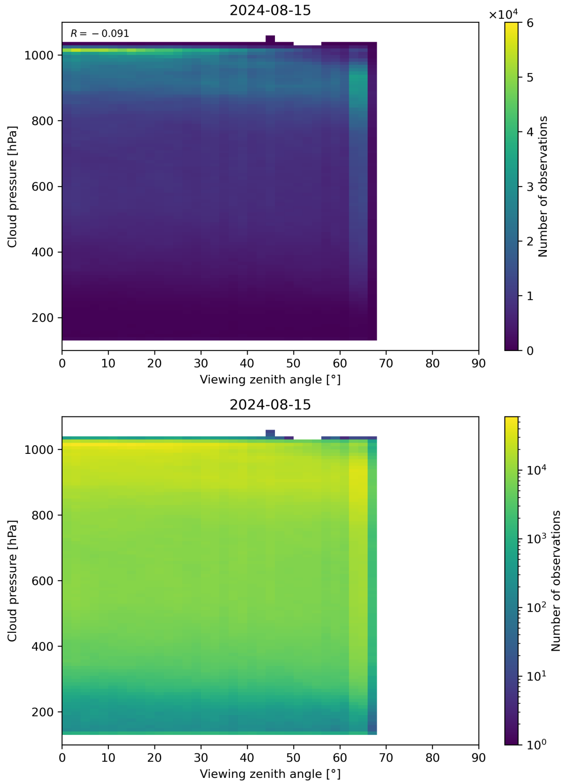
Figure 121: Scatter density plot of “Viewing zenith angle” against “Cloud pressure” for 2024-08-14 to 2024-08-16.
