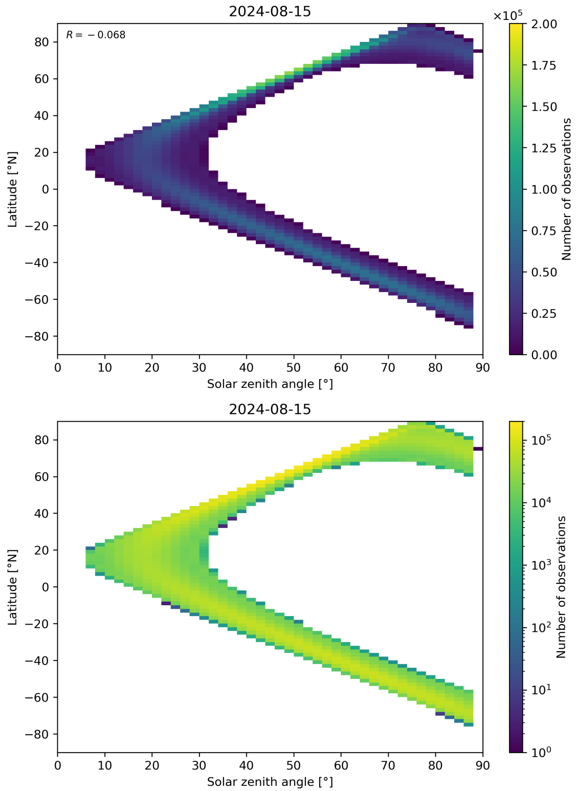
Figure 113: Scatter density plot of “Solar zenith angle” against “Latitude” for 2024-08-14 to 2024-08-16.
