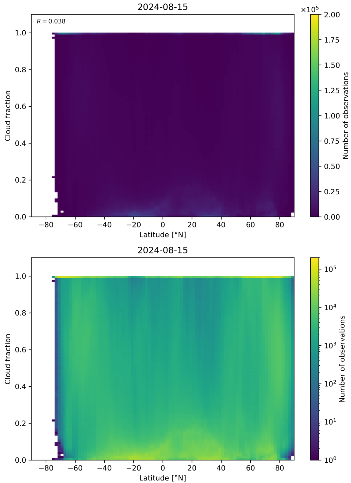
Figure 90: Scatter density plot of “Latitude” against “Cloud fraction” for 2024-08-14 to 2024-08-16.
