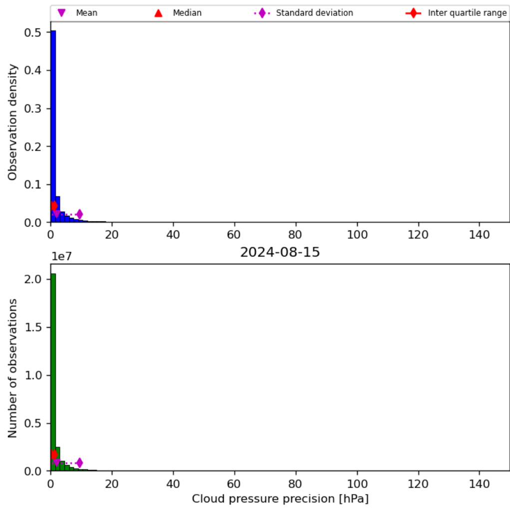
Figure 31: Histogram of “Cloud pressure precision” for 2024-08-14 to 2024-08-16
