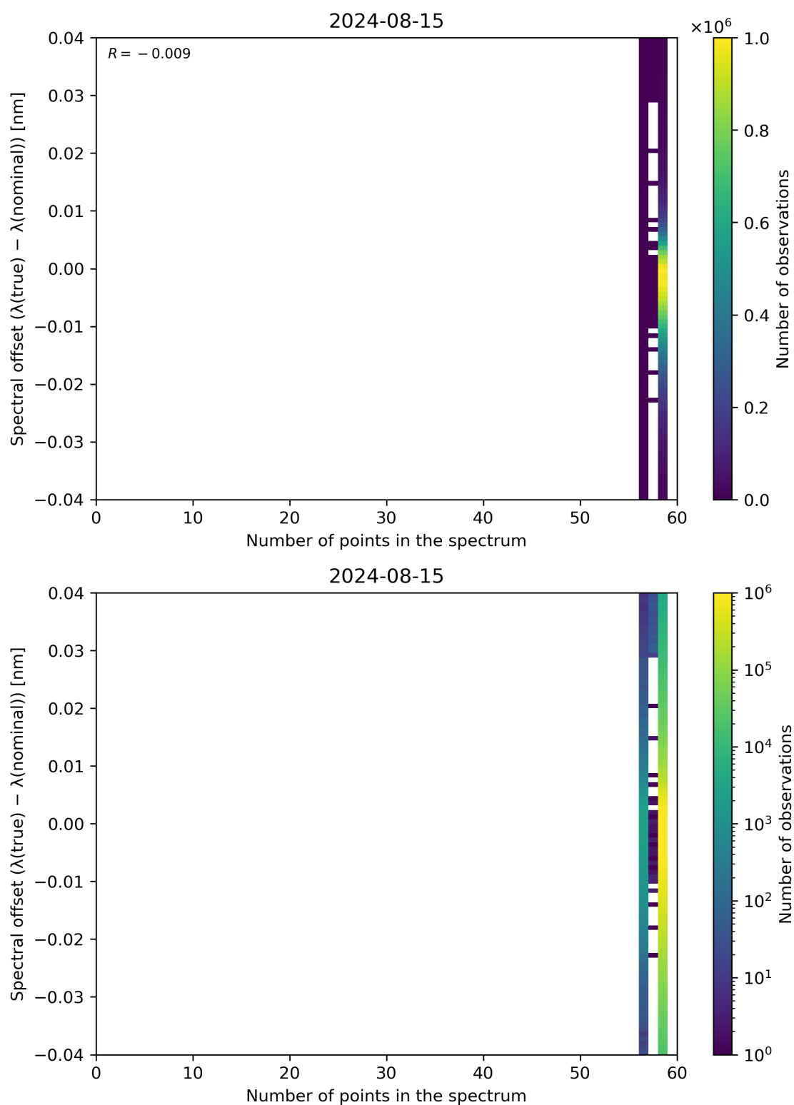
Figure 101: Scatter density plot of “Number of points in the spectrum” against “Spectral offset ( \lambda(\text{true}) - \lambda(\text{nominal}) )” for 2024-08-14 to 2024-08-16.
