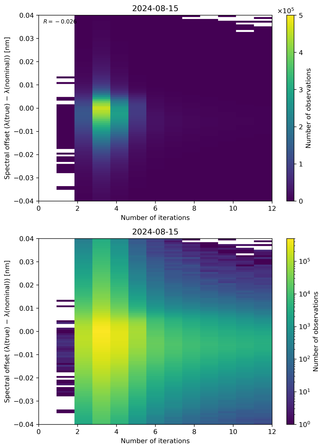
Figure 100: Scatter density plot of “Number of iterations” against “Spectral offset ( \lambda(\text{true}) - \lambda(\text{nominal}) )” for 2024-08-14 to 2024-08-16.
