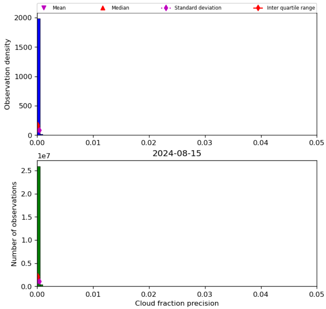
Figure 33: Histogram of “Cloud fraction precision” for 2024-08-14 to 2024-08-16
