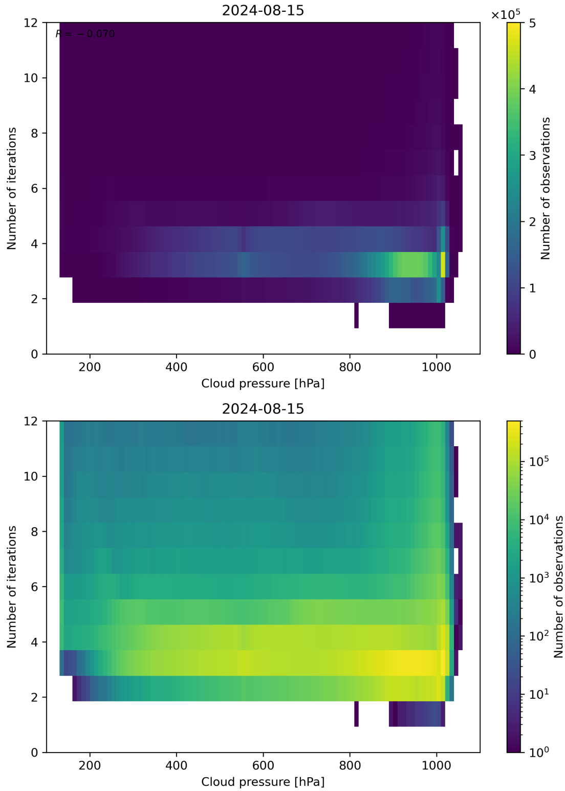
Figure 81: Scatter density plot of “Cloud pressure” against “Number of iterations” for 2024-08-14 to 2024-08-16.
