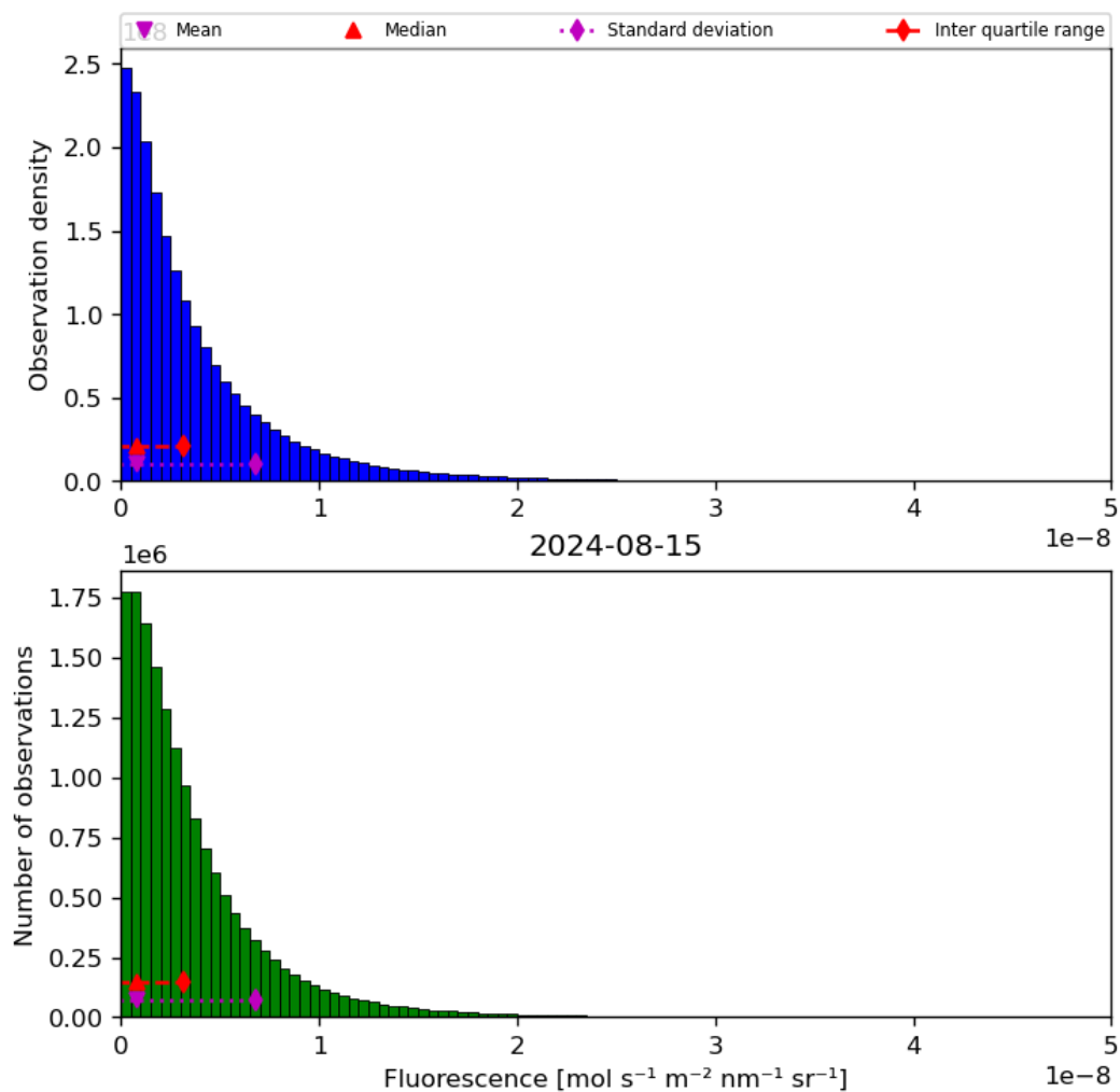
Figure 40: Histogram of “Fluorescence” for 2024-08-14 to 2024-08-16
