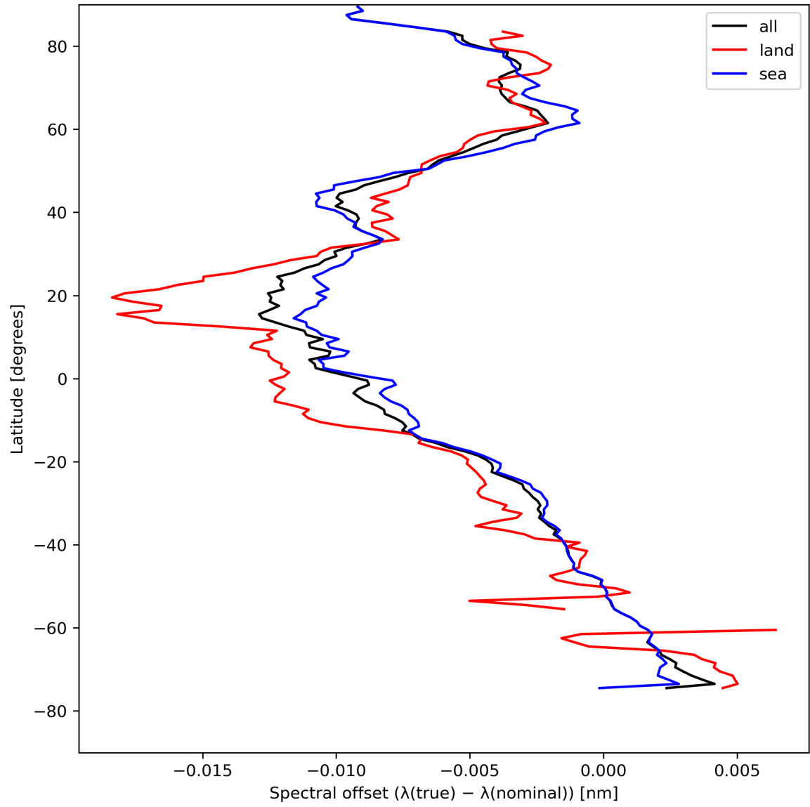
Figure 28: Zonal average of “Spectral offset ( \lambda(\text{true}) - \lambda(\text{nominal}) )” for 2024-08-14 to 2024-08-16.
