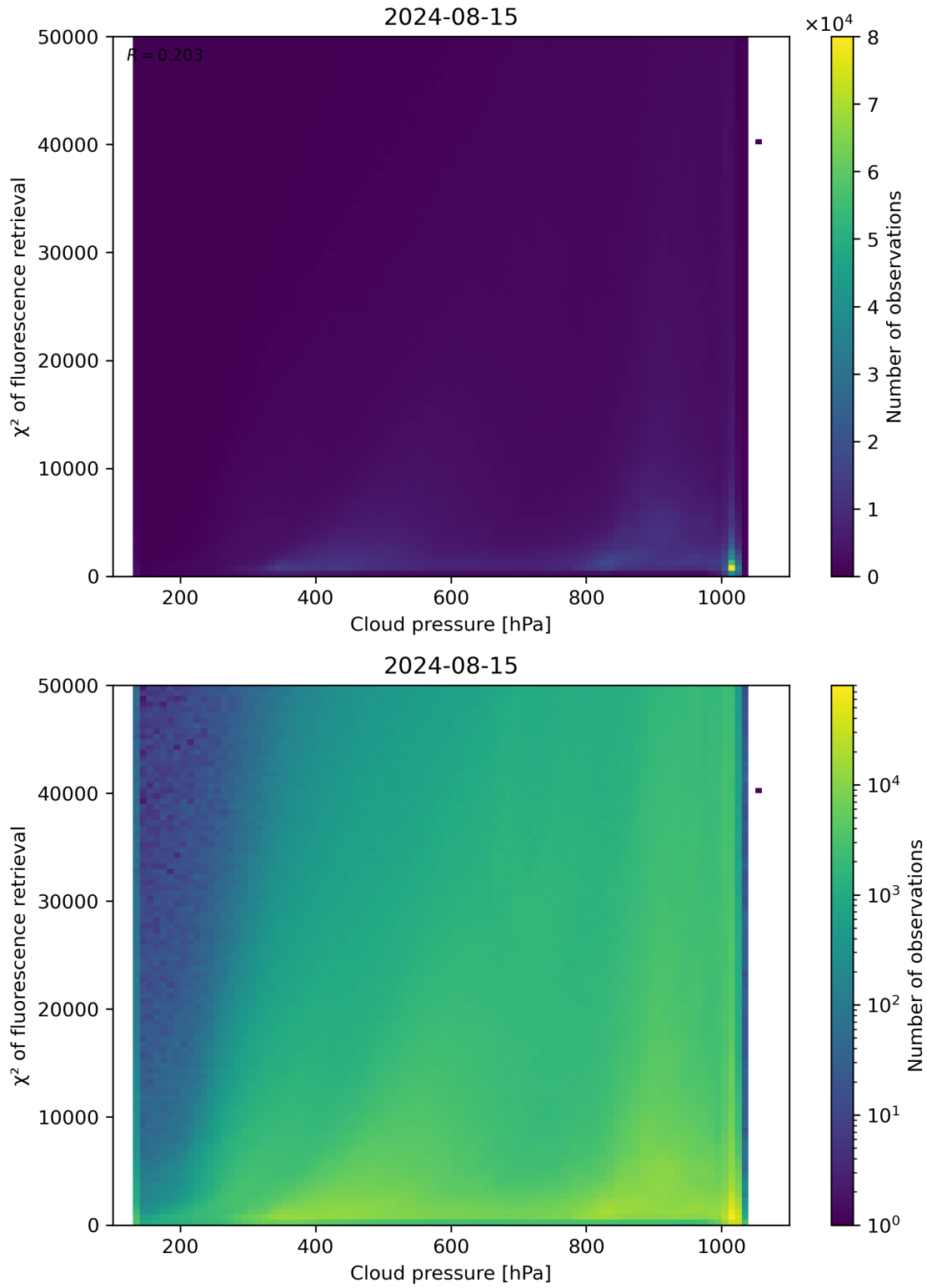
Figure 78: Scatter density plot of “Cloud pressure” against “ \chi^2 of fluorescence retrieval” for 2024-08-14 to 2024-08-16.
