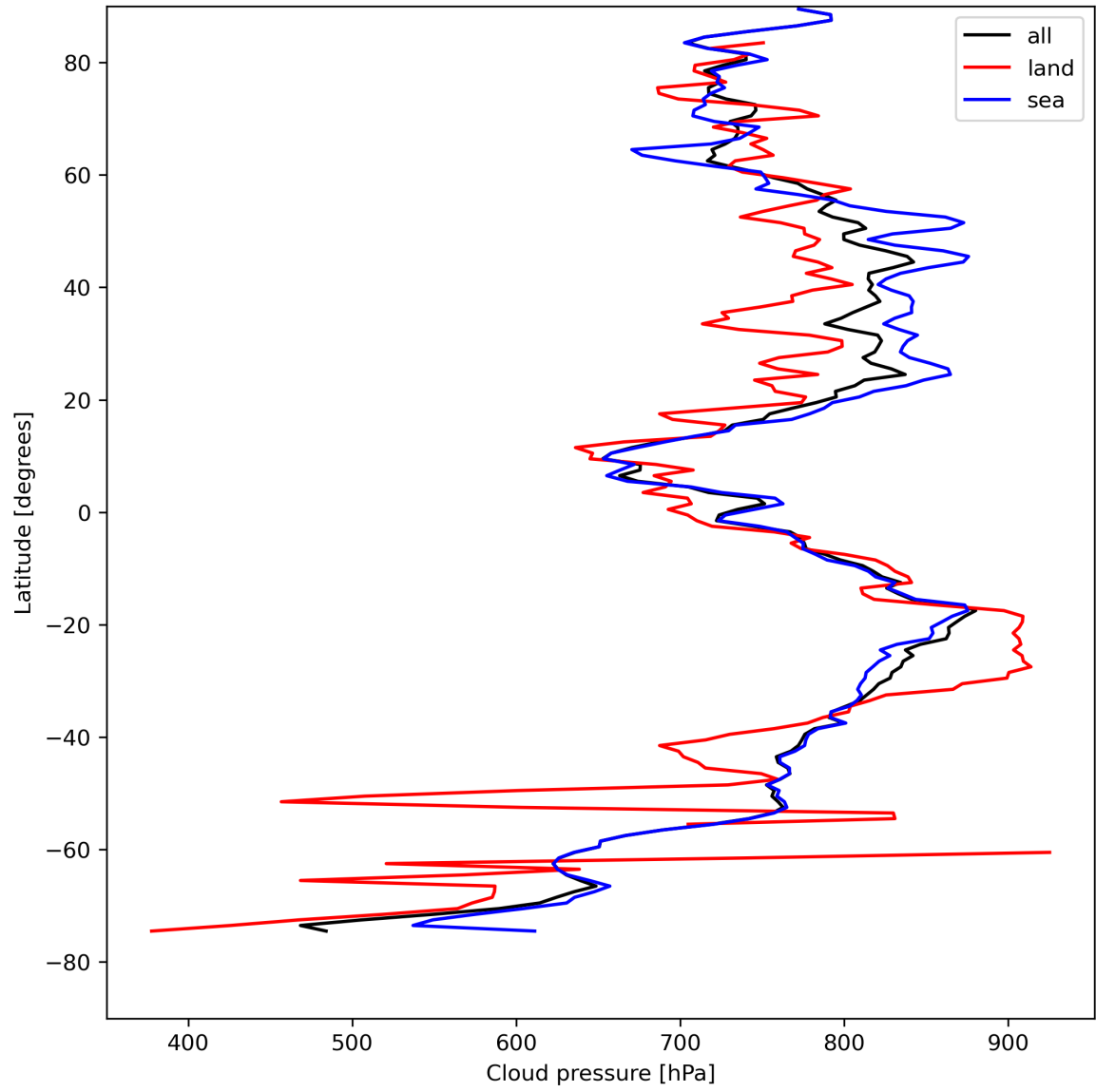
Figure 13: Zonal average of “Cloud pressure” for 2024-08-14 to 2024-08-16.
