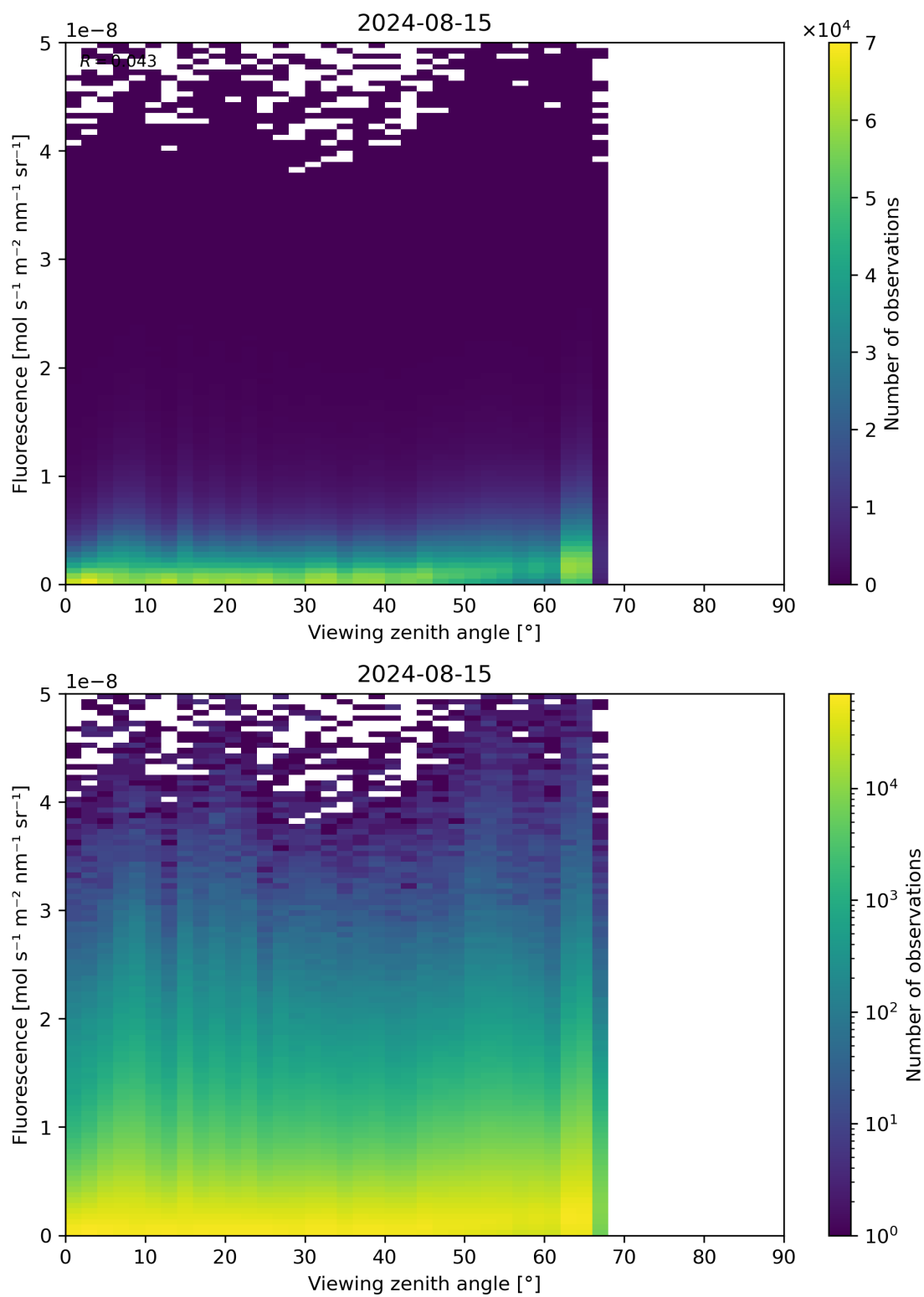
Figure 122: Scatter density plot of “Viewing zenith angle” against “Fluorescence” for 2024-08-14 to 2024-08-16.
