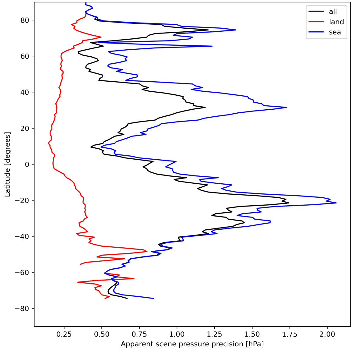
Figure 20: Zonal average of “Apparent scene pressure precision” for 2024-08-14 to 2024-08-16.
