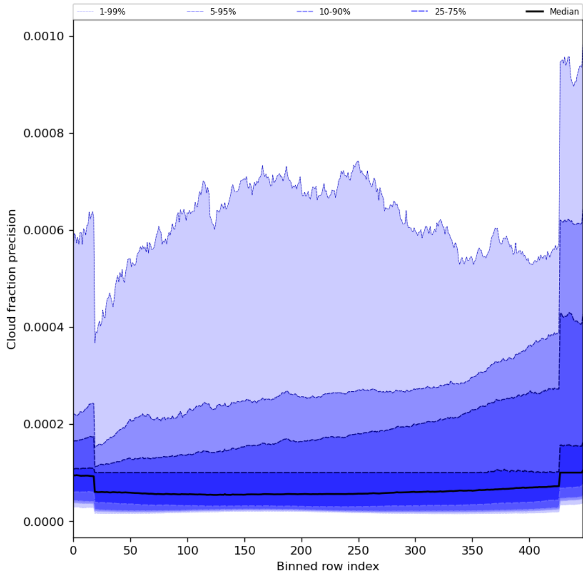
Figure 50: Along track statistics of “Cloud fraction precision” for 2024-08-14 to 2024-08-16
