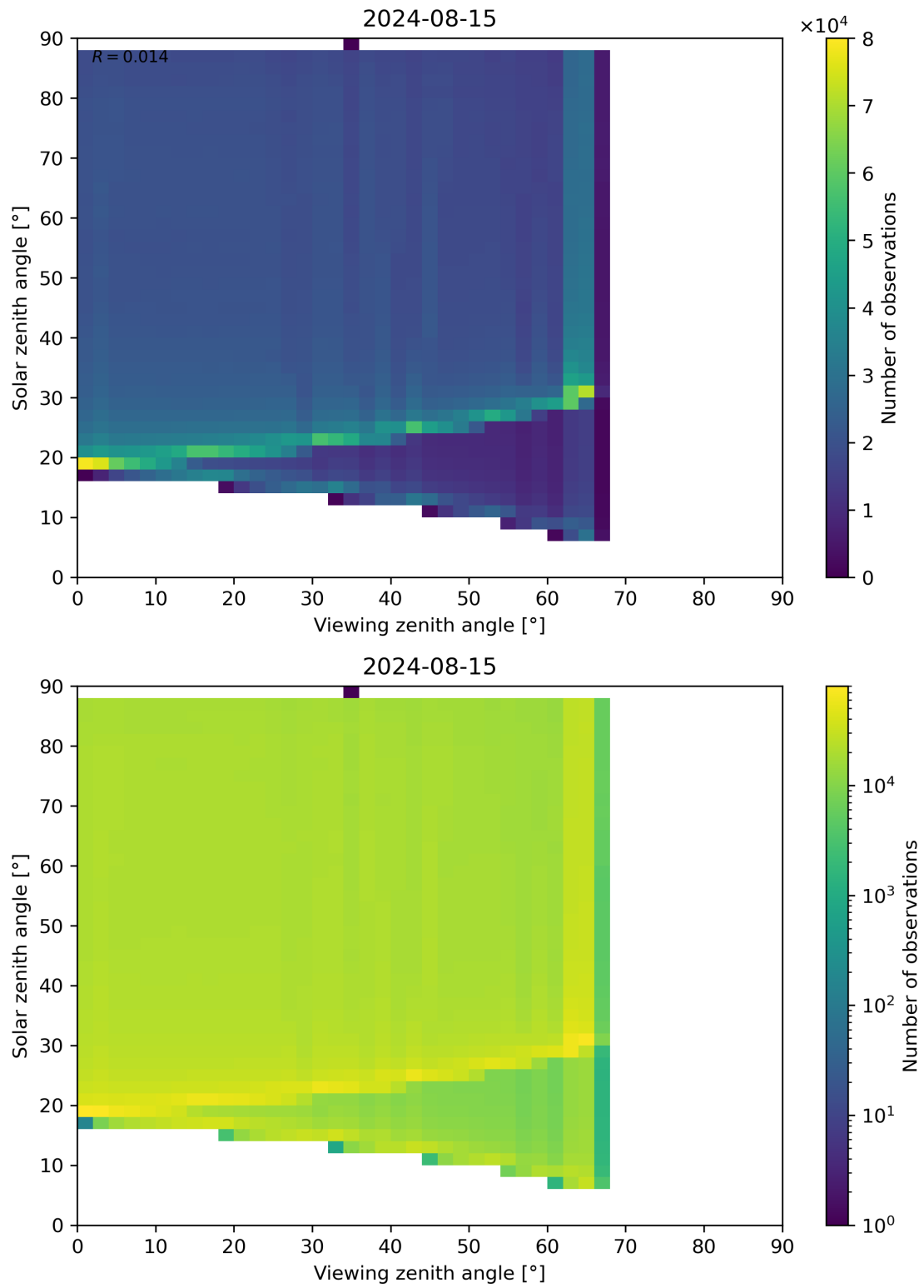
Figure 127: Scatter density plot of “Viewing zenith angle” against “Solar zenith angle” for 2024-08-14 to 2024-08-16.
