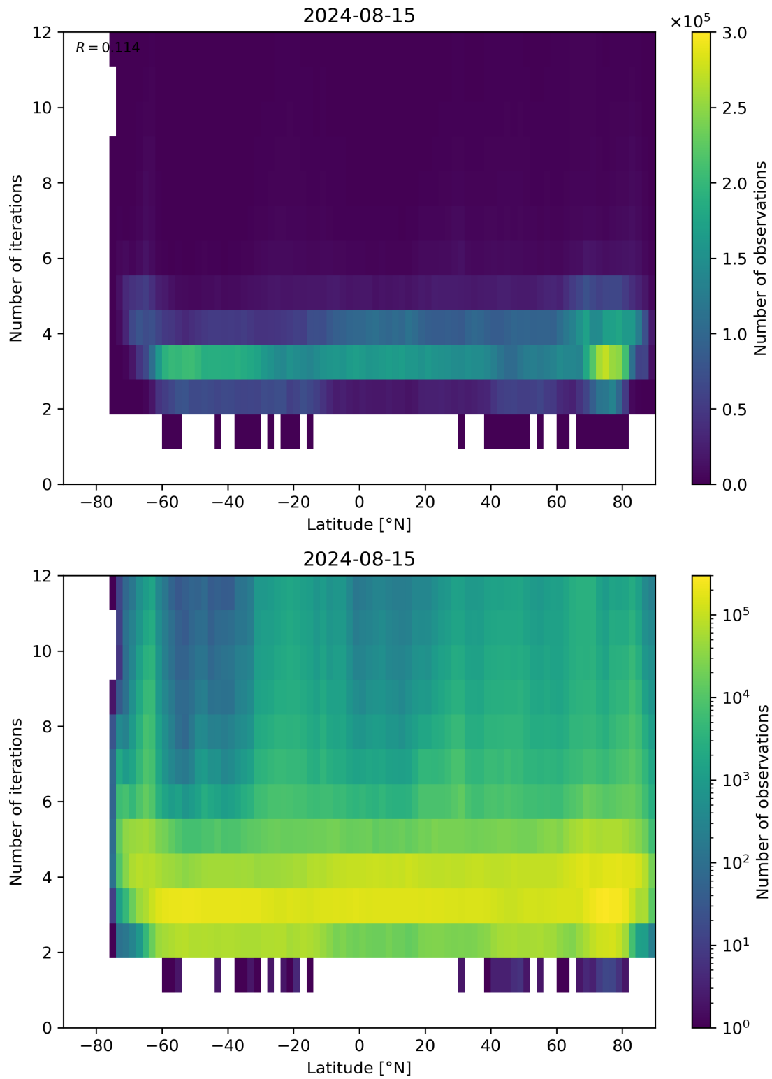
Figure 93: Scatter density plot of “Latitude” against “Number of iterations” for 2024-08-14 to 2024-08-16.
