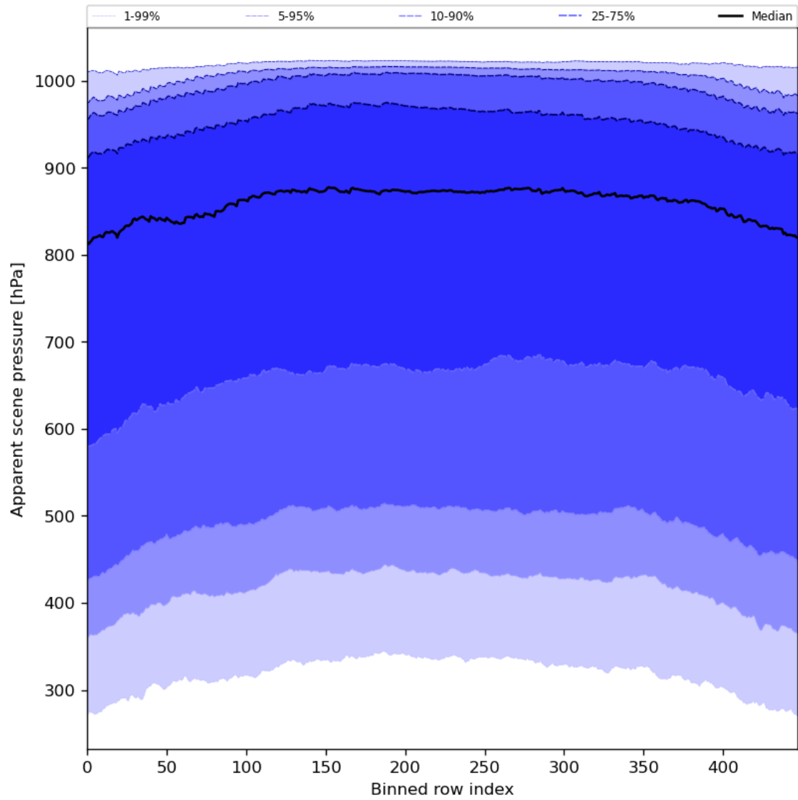
Figure 53: Along track statistics of “Apparent scene pressure” for 2024-08-14 to 2024-08-16
