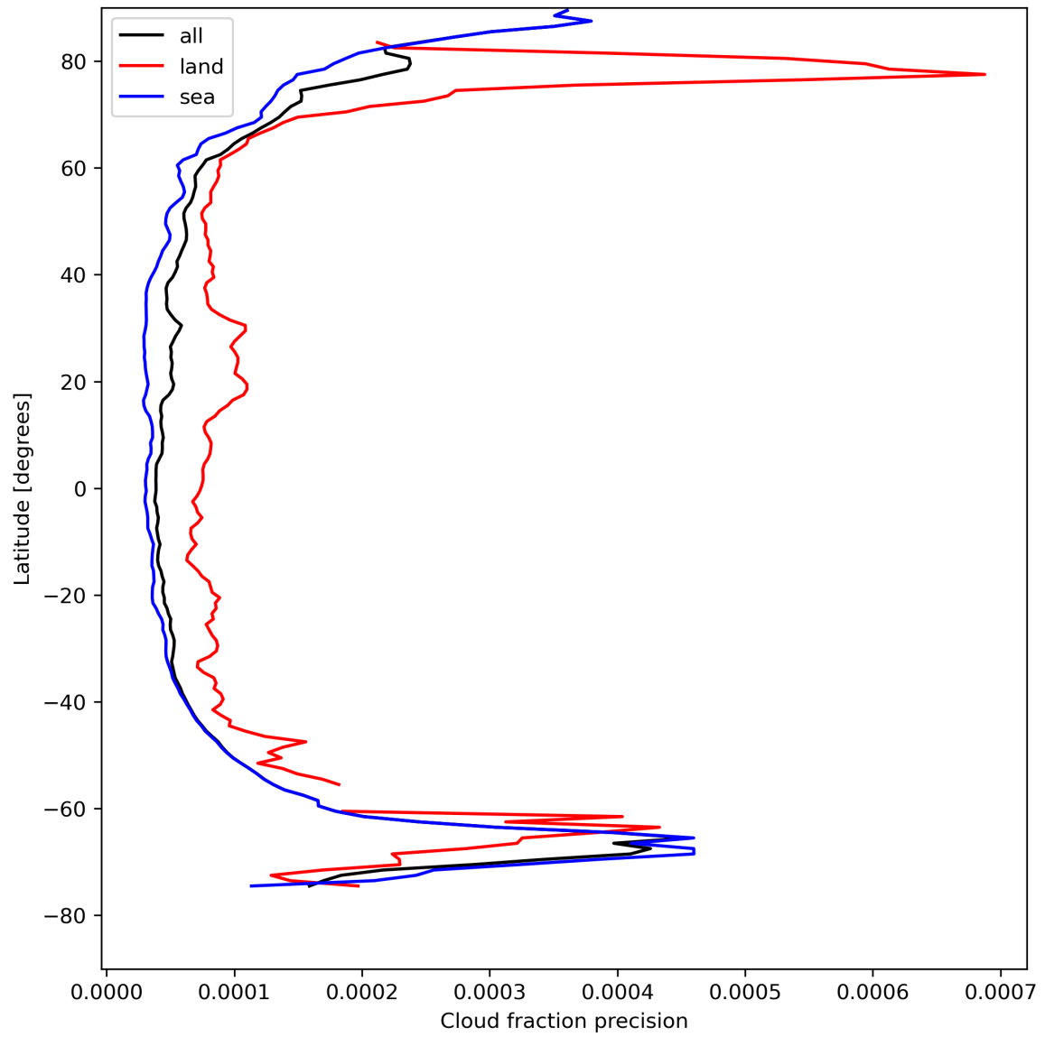
Figure 16: Zonal average of “Cloud fraction precision” for 2024-08-14 to 2024-08-16.
