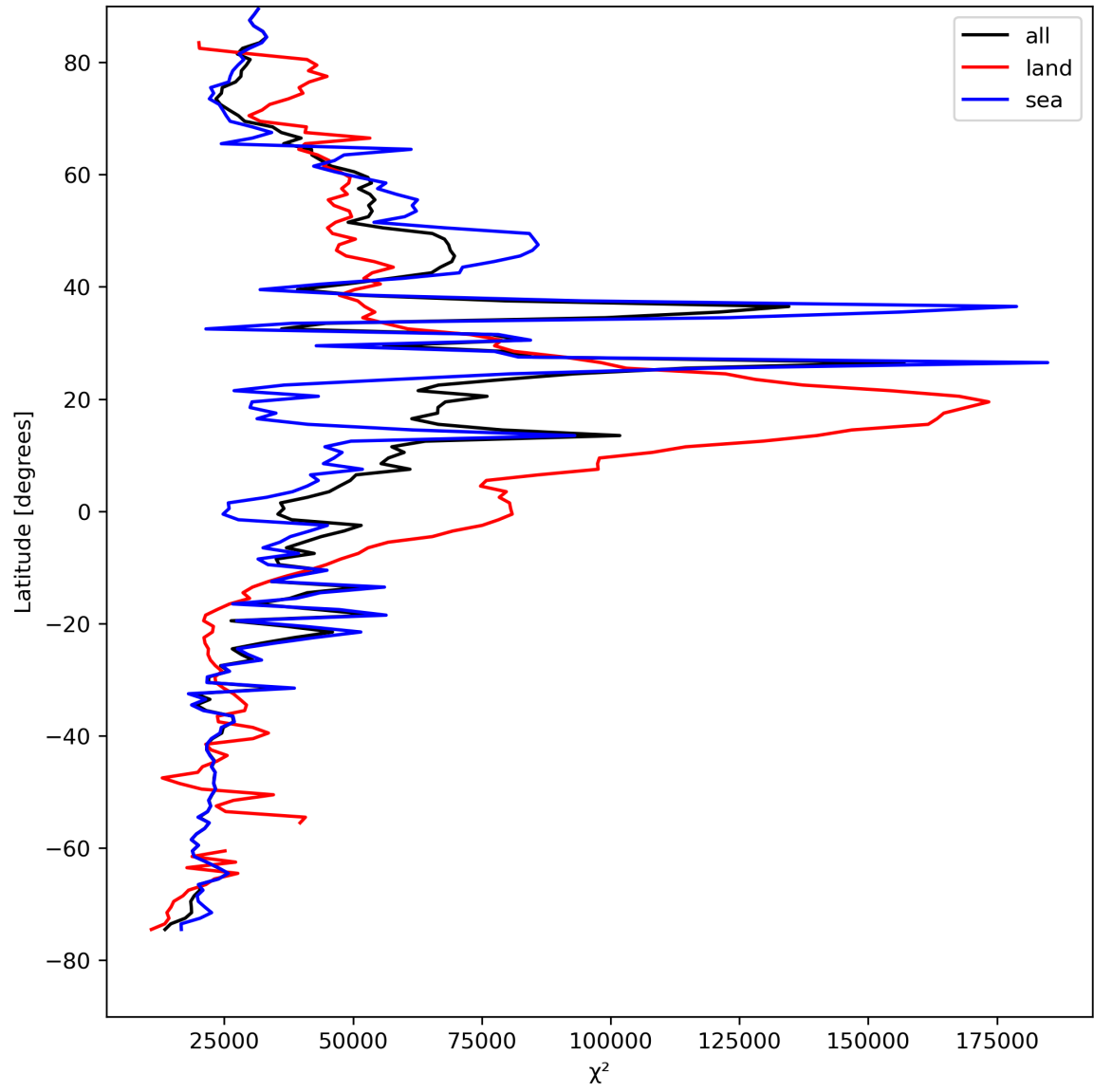
Figure 21: Zonal average of “ \chi^2 ” for 2024-08-14 to 2024-08-16.
