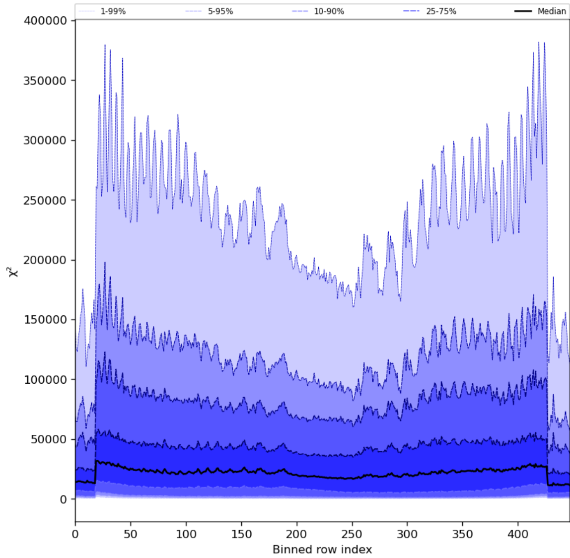
Figure 55: Along track statistics of “ \chi^2 ” for 2024-08-14 to 2024-08-16
