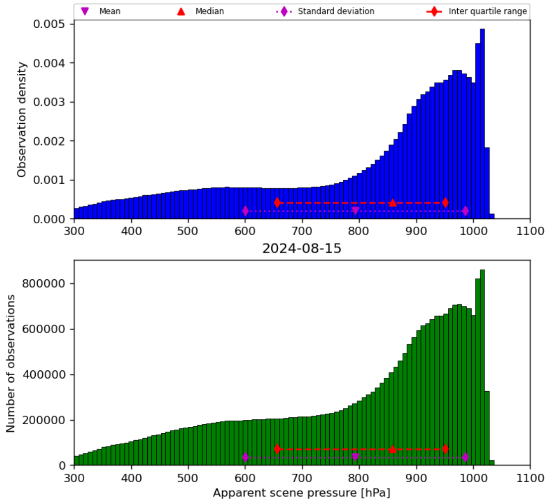
Figure 36: Histogram of “Apparent scene pressure” for 2024-08-14 to 2024-08-16
