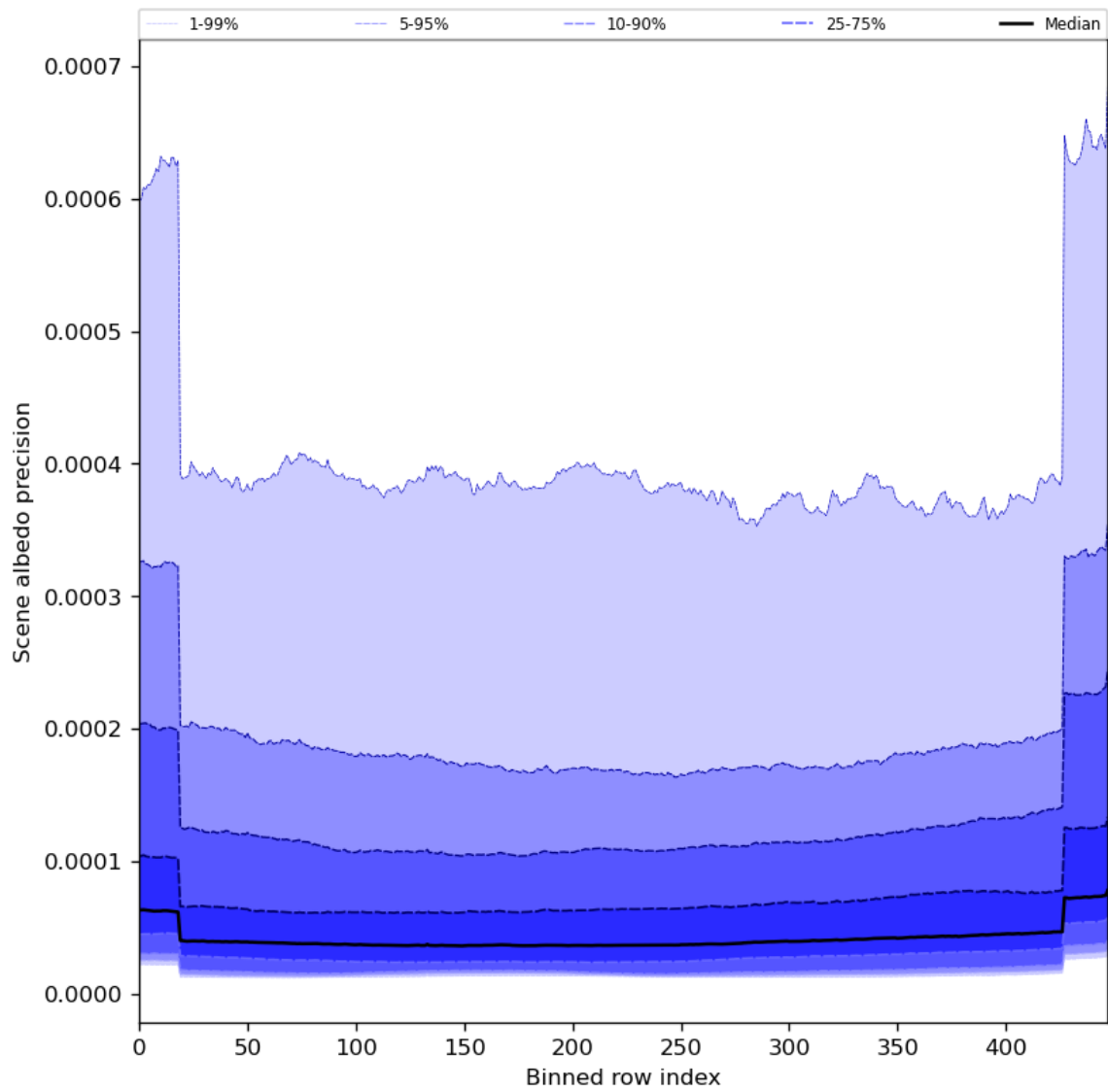
Figure 52: Along track statistics of “Scene albedo precision” for 2024-08-14 to 2024-08-16
