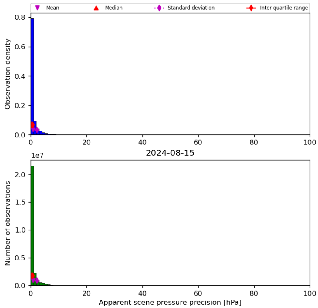
Figure 37: Histogram of “Apparent scene pressure precision” for 2024-08-14 to 2024-08-16
