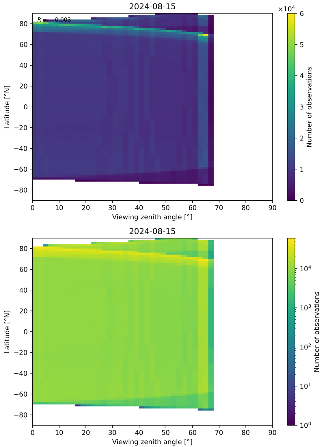
Figure 123: Scatter density plot of “Viewing zenith angle” against “Latitude” for 2024-08-14 to 2024-08-16.
