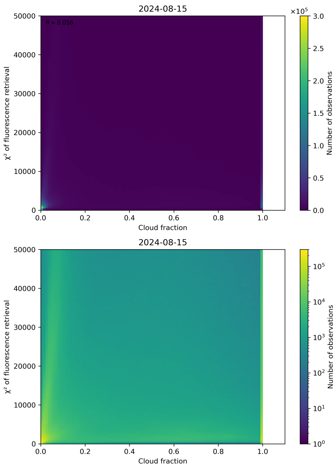
Figure 71: Scatter density plot of “Cloud fraction” against “ \chi^2 of fluorescence retrieval” for 2024-08-14 to 2024-08-16.
