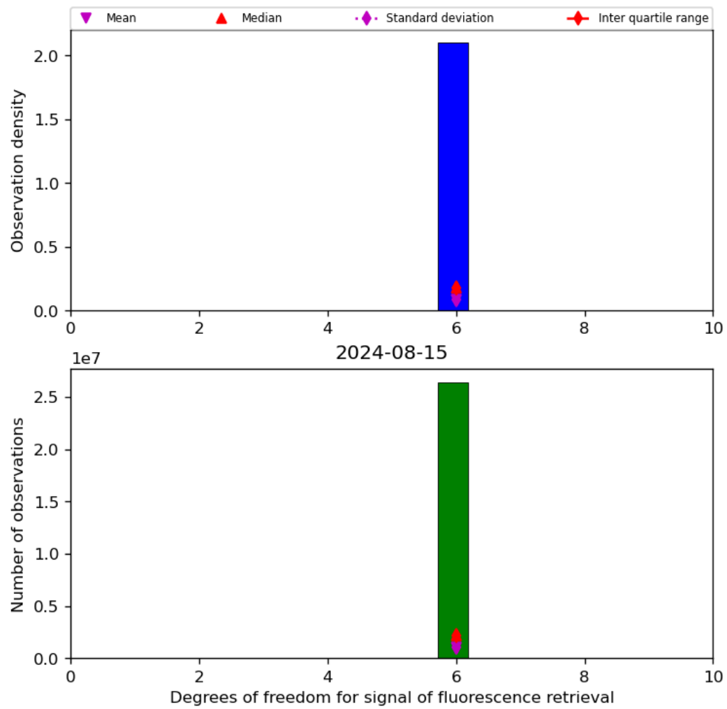
Figure 43: Histogram of “Degrees of freedom for signal of fluorescence retrieval” for 2024-08-14 to 2024-08-16
