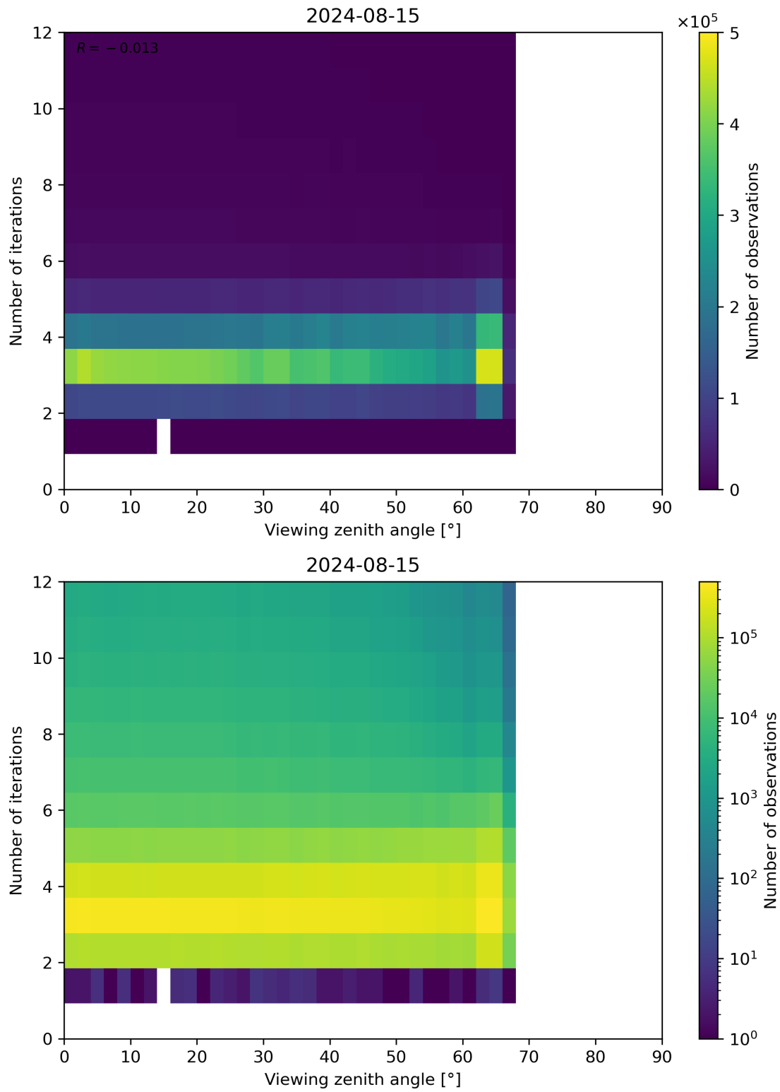
Figure 124: Scatter density plot of “Viewing zenith angle” against “Number of iterations” for 2024-08-14 to 2024-08-16.
