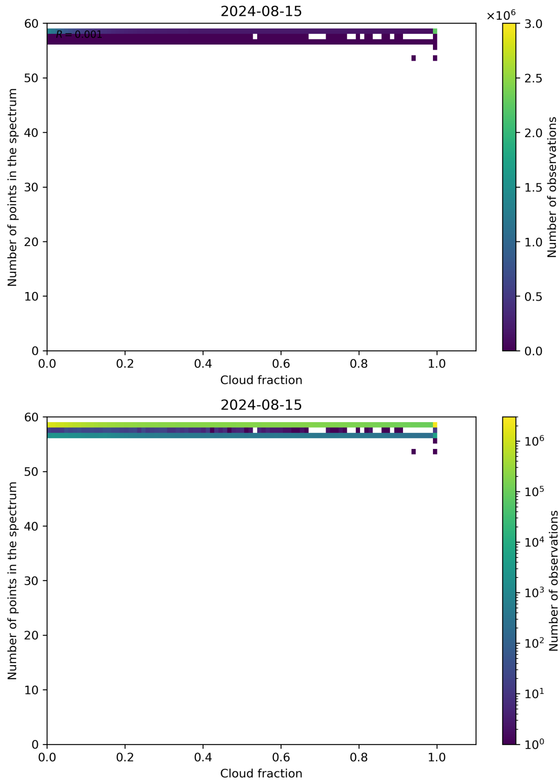
Figure 74: Scatter density plot of “Cloud fraction” against “Number of points in the spectrum” for 2024-08-14 to 2024-08-16.
