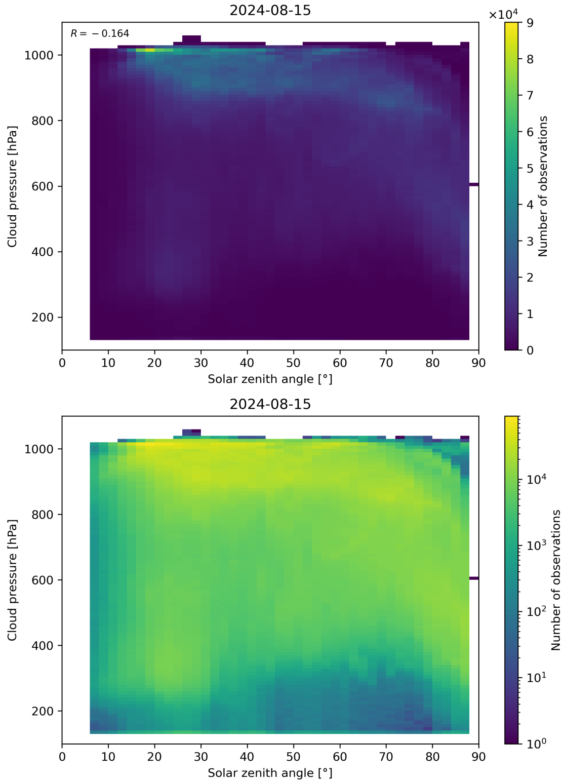
Figure 111: Scatter density plot of “Solar zenith angle” against “Cloud pressure” for 2024-08-14 to 2024-08-16.
