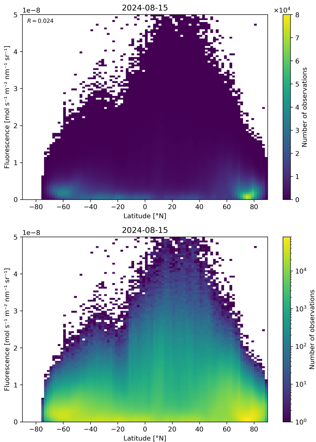
Figure 92: Scatter density plot of “Latitude” against “Fluorescence” for 2024-08-14 to 2024-08-16.
