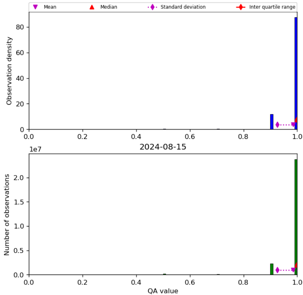
Figure 29: Histogram of “QA value” for 2024-08-14 to 2024-08-16
