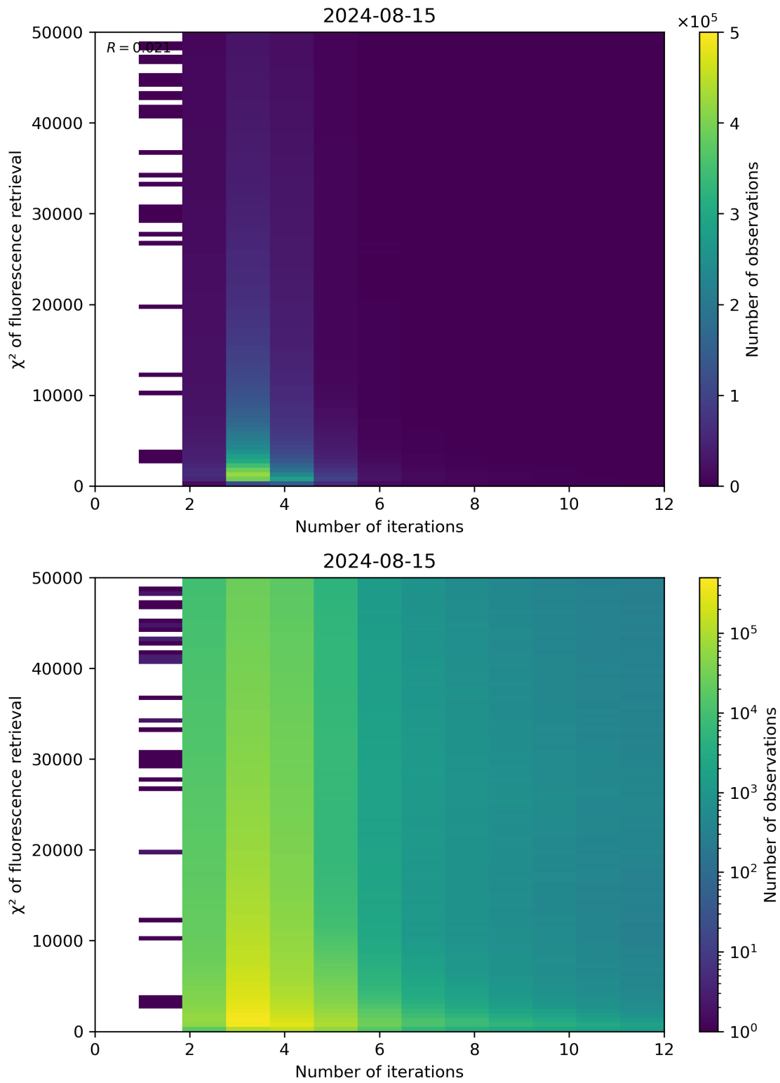
Figure 97: Scatter density plot of “Number of iterations” against “ \chi^2 of fluorescence retrieval” for 2024-08-14 to 2024-08-16.
