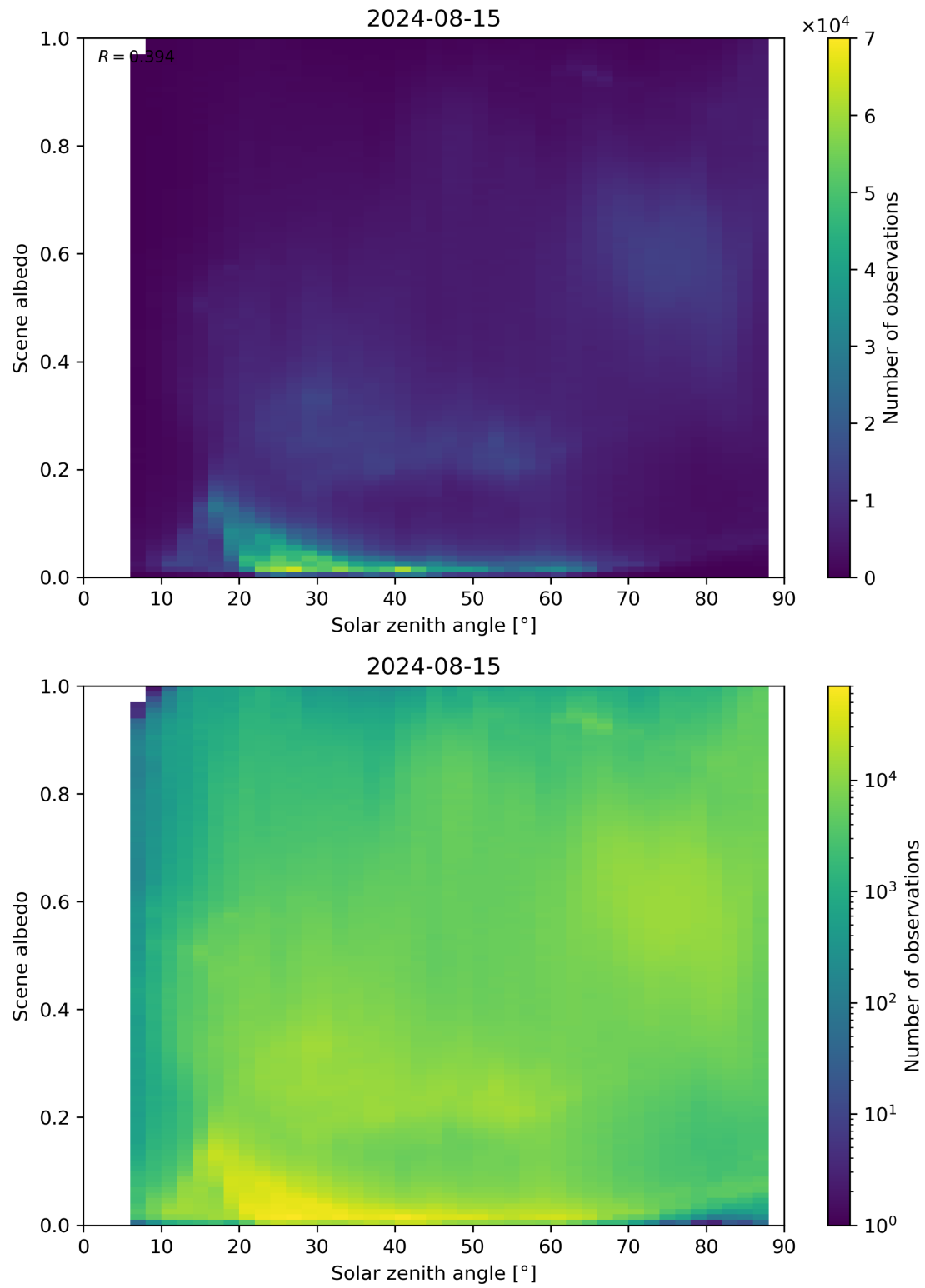
Figure 116: Scatter density plot of “Solar zenith angle” against “Scene albedo” for 2024-08-14 to 2024-08-16.
