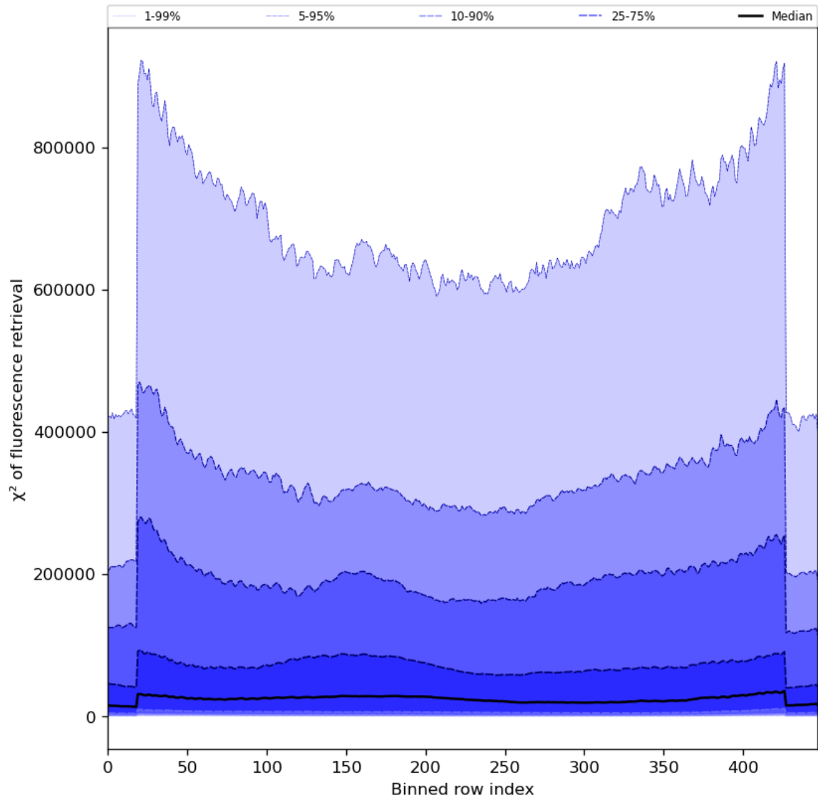
Figure 59: Along track statistics of “ \chi^2 of fluorescence retrieval” for 2024-08-14 to 2024-08-16
