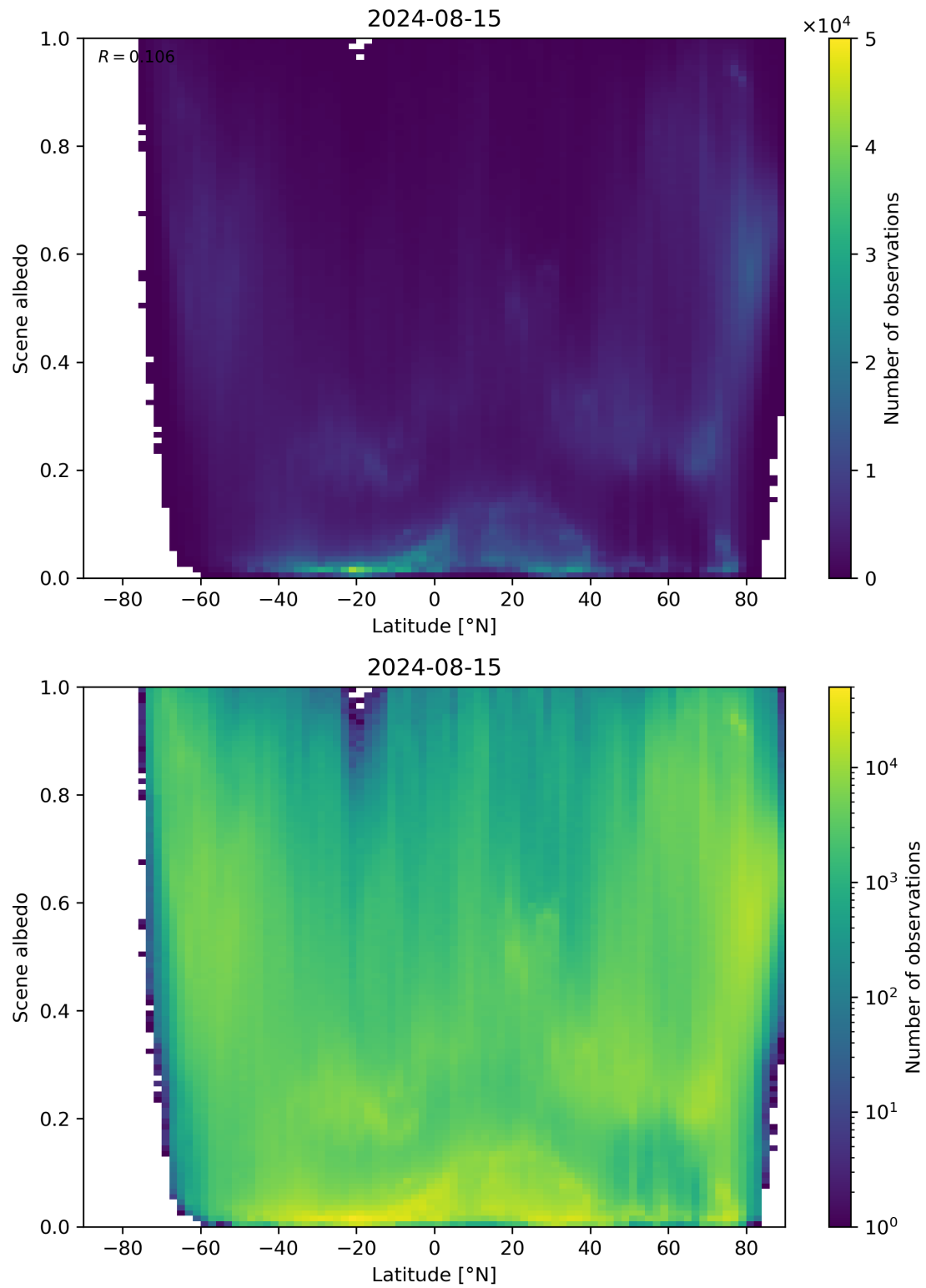
Figure 95: Scatter density plot of “Latitude” against “Scene albedo” for 2024-08-14 to 2024-08-16.
