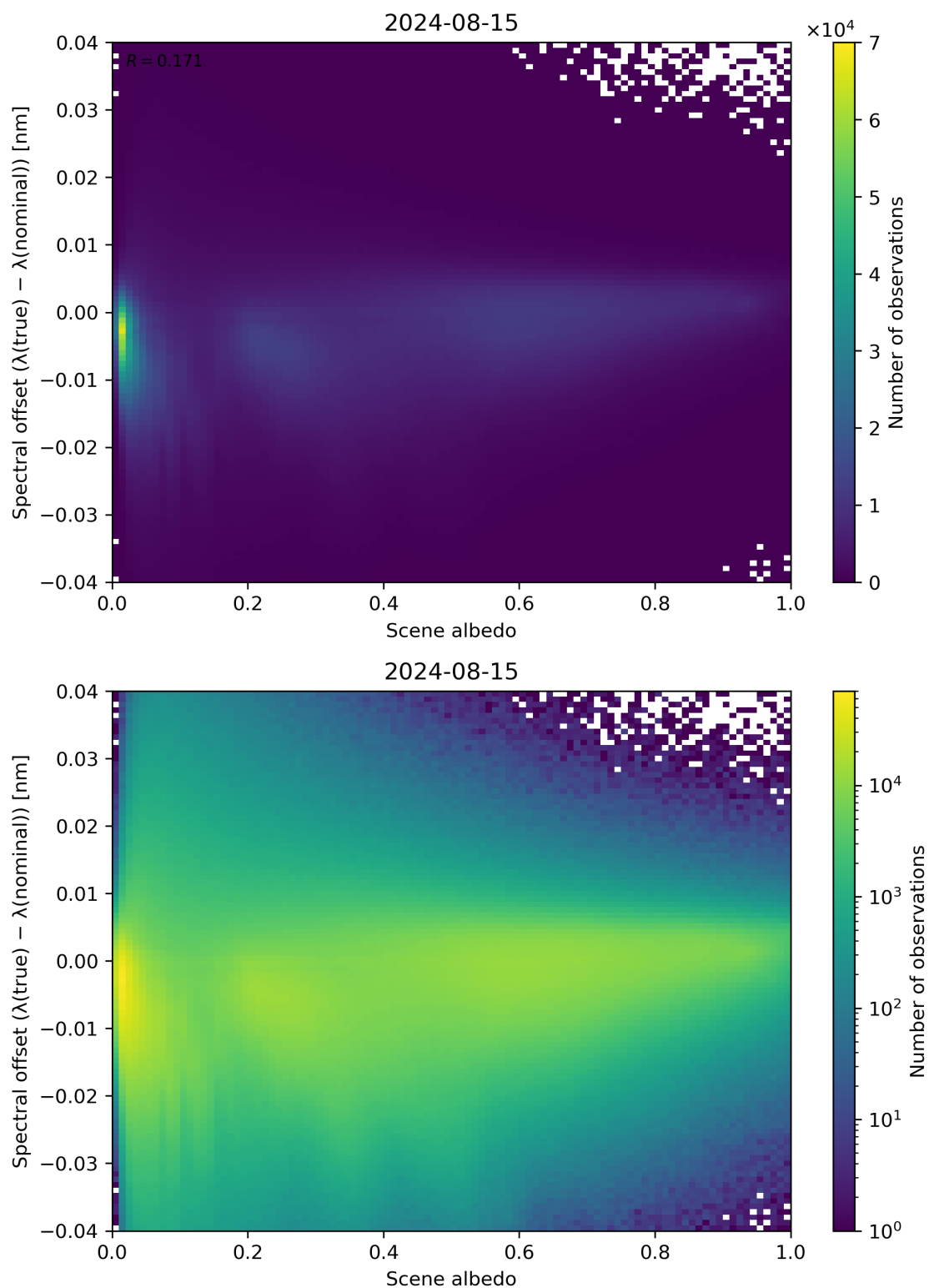
Figure 107: Scatter density plot of “Scene albedo” against “Spectral offset ( \lambda(\text{true}) - \lambda(\text{nominal}) )” for 2024-08-14 to 2024-08-16.
