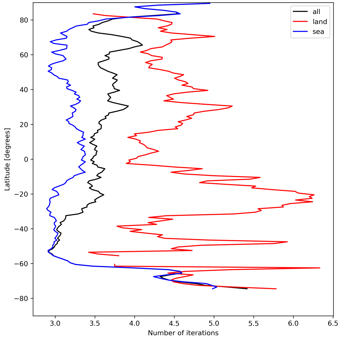
Figure 22: Zonal average of “Number of iterations” for 2024-08-14 to 2024-08-16.
