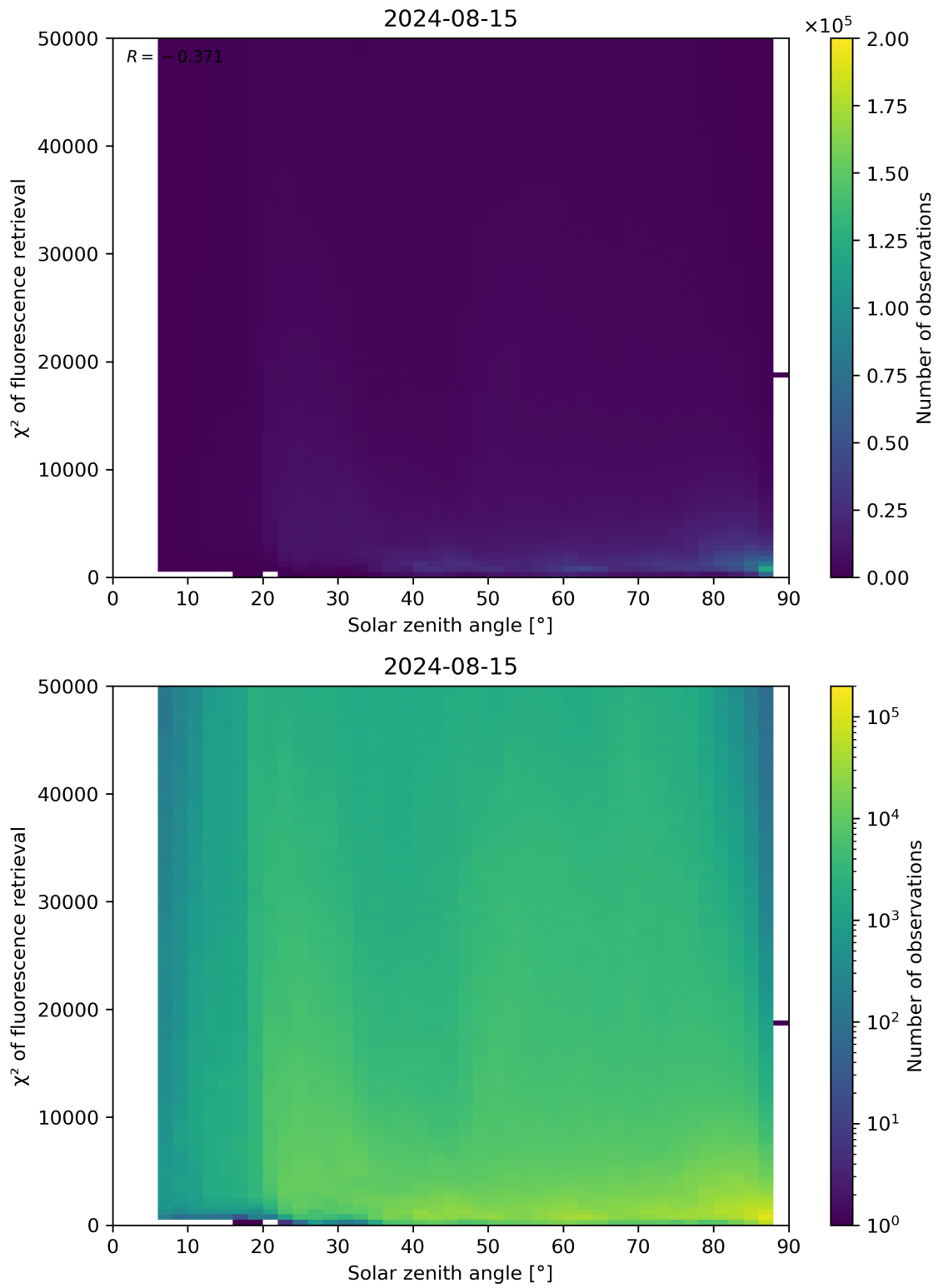
Figure 109: Scatter density plot of “Solar zenith angle” against “ \chi^2 of fluorescence retrieval” for 2024-08-14 to 2024-08-16.
