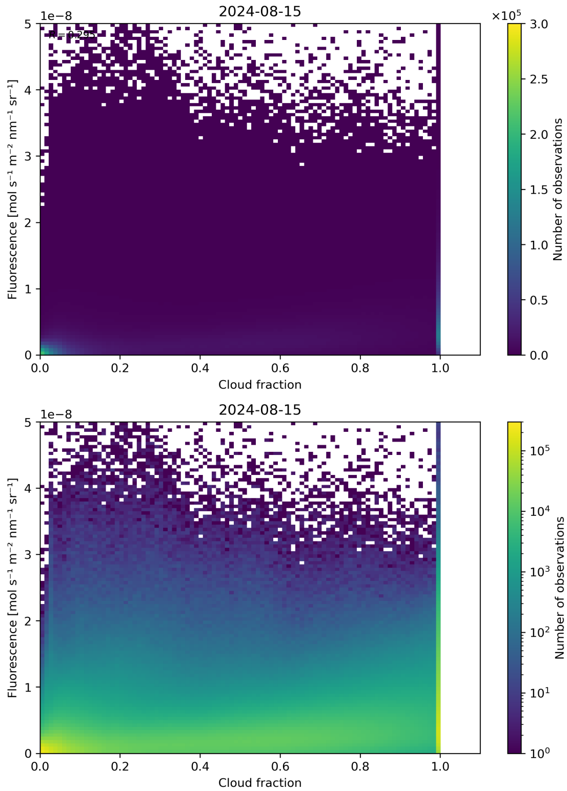
Figure 72: Scatter density plot of “Cloud fraction” against “Fluorescence” for 2024-08-14 to 2024-08-16.
