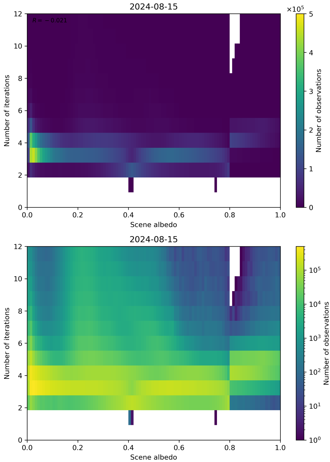
Figure 105: Scatter density plot of “Scene albedo” against “Number of iterations” for 2024-08-14 to 2024-08-16.
