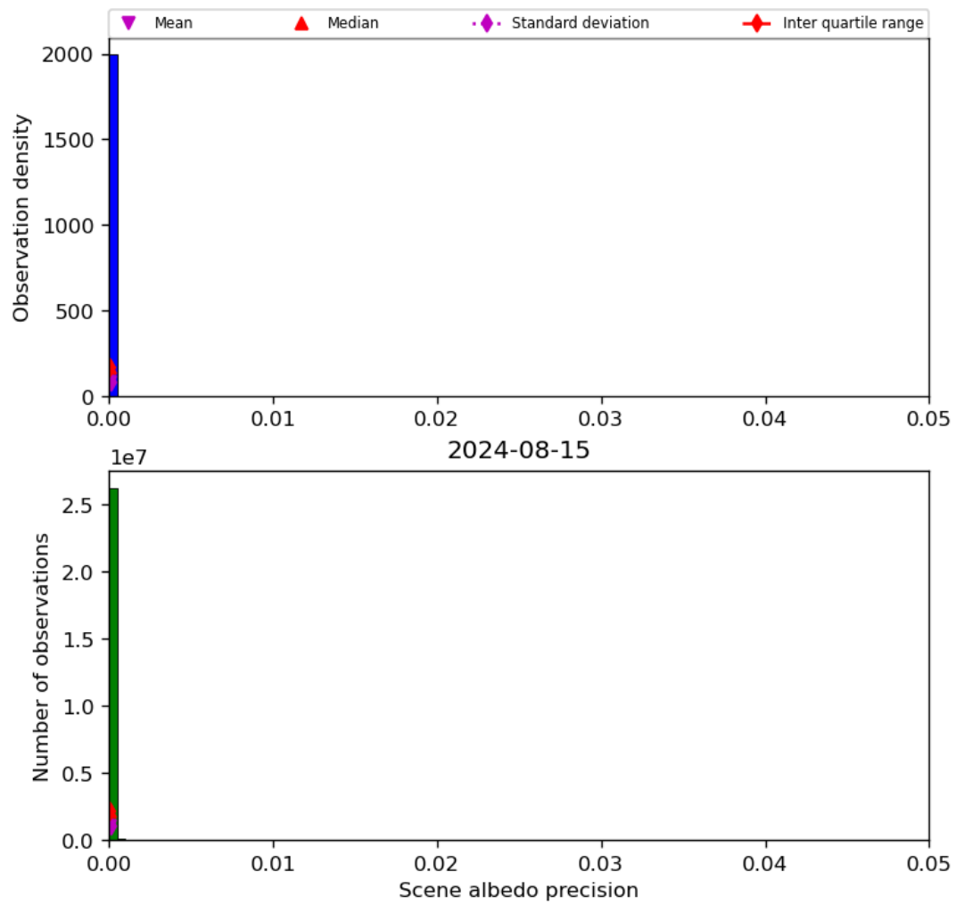
Figure 35: Histogram of “Scene albedo precision” for 2024-08-14 to 2024-08-16
