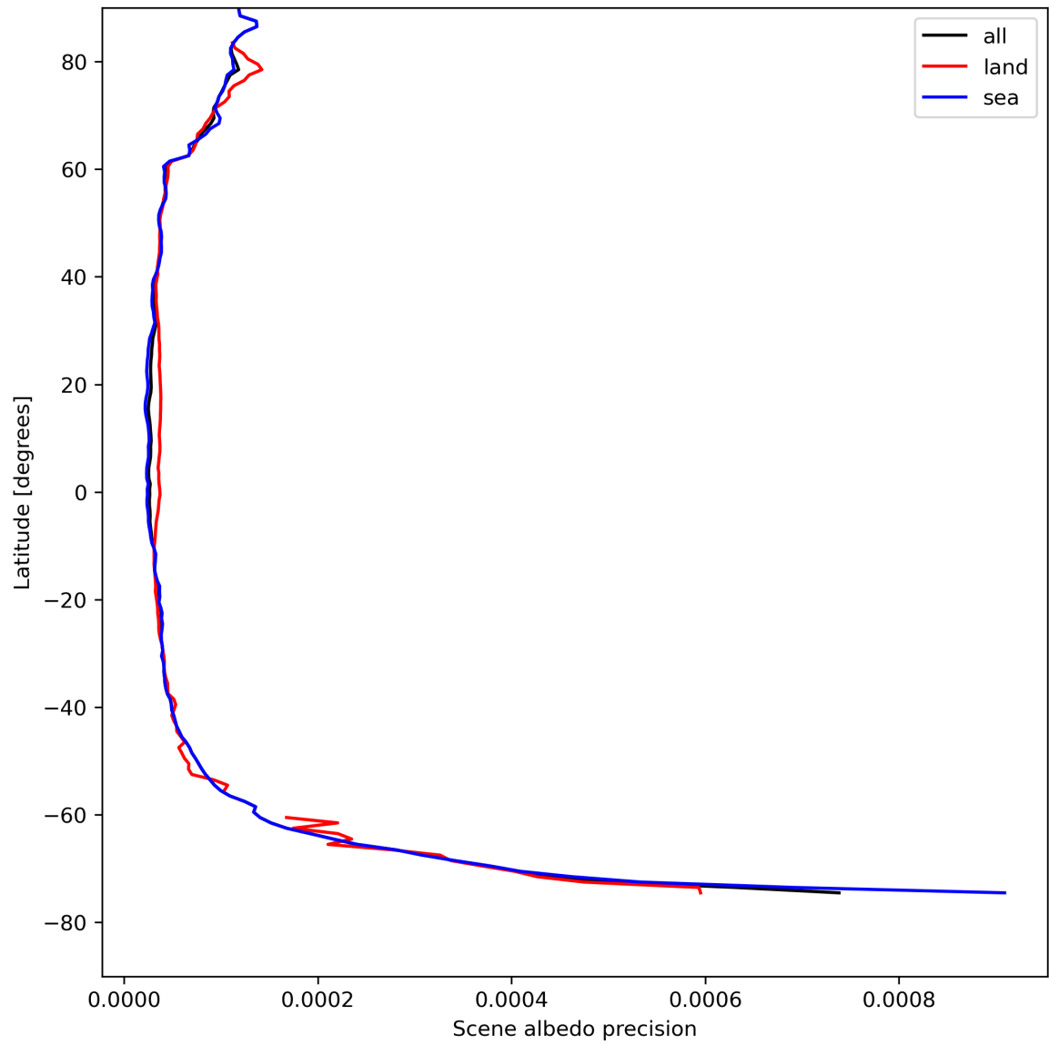
Figure 18: Zonal average of “Scene albedo precision” for 2024-08-14 to 2024-08-16.
