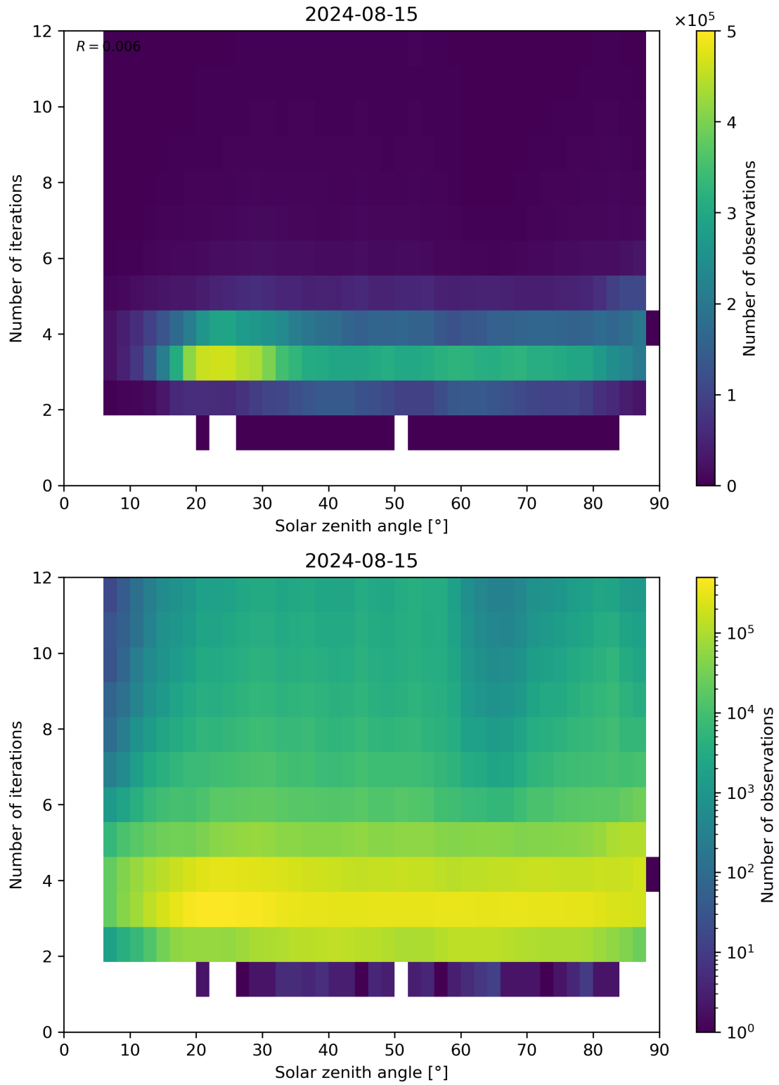
Figure 114: Scatter density plot of “Solar zenith angle” against “Number of iterations” for 2024-08-14 to 2024-08-16.
