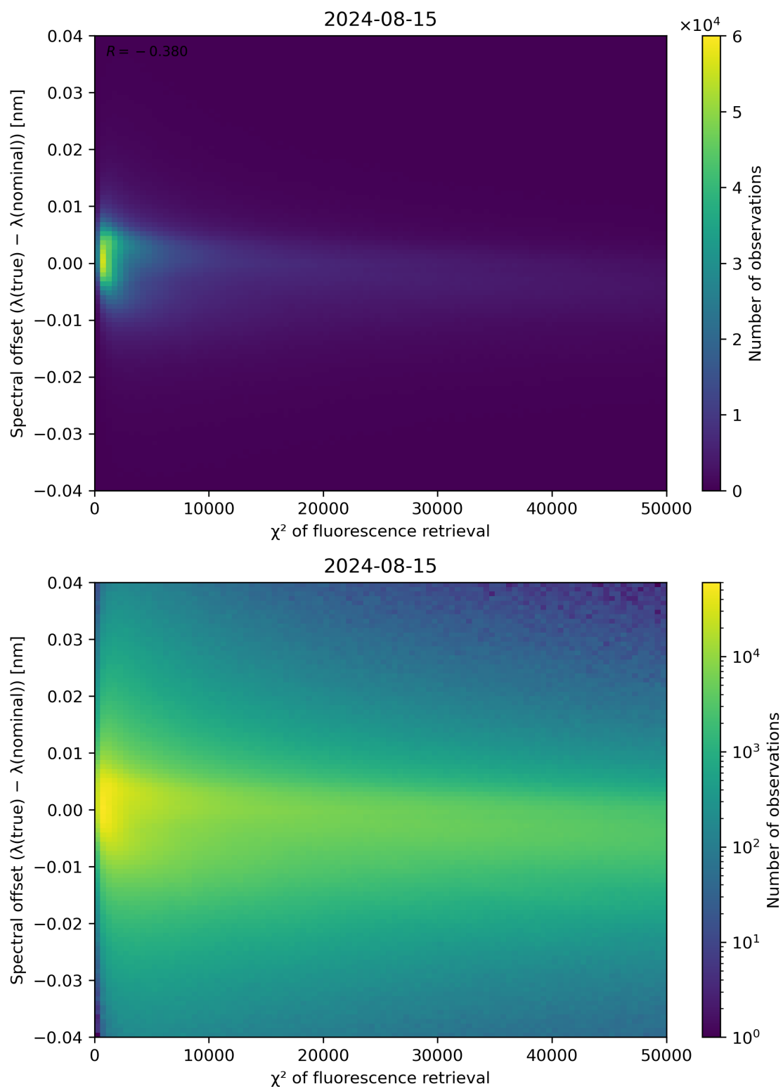
Figure 69: Scatter density plot of “ \chi^2 of fluorescence retrieval” against “Spectral offset ( \lambda(\text{true}) - \lambda(\text{nominal}) )” for 2024-08-14 to 2024-08-16.
