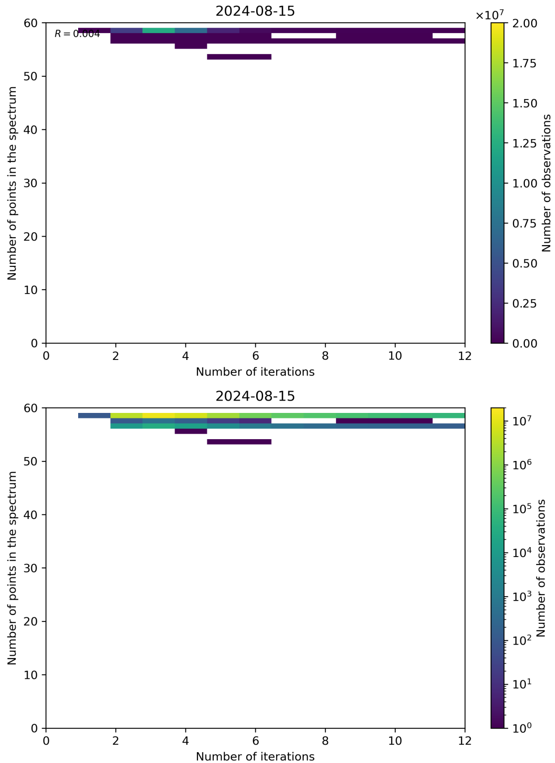
Figure 99: Scatter density plot of “Number of iterations” against “Number of points in the spectrum” for 2024-08-14 to 2024-08-16.
