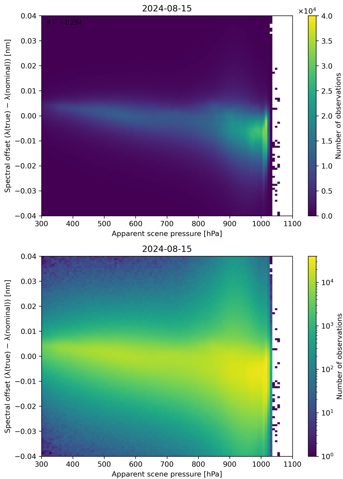
Figure 67: Scatter density plot of “Apparent scene pressure” against “Spectral offset ( \lambda(\text{true}) - \lambda(\text{nominal}) )” for 2024-08-14 to 2024-08-16.
