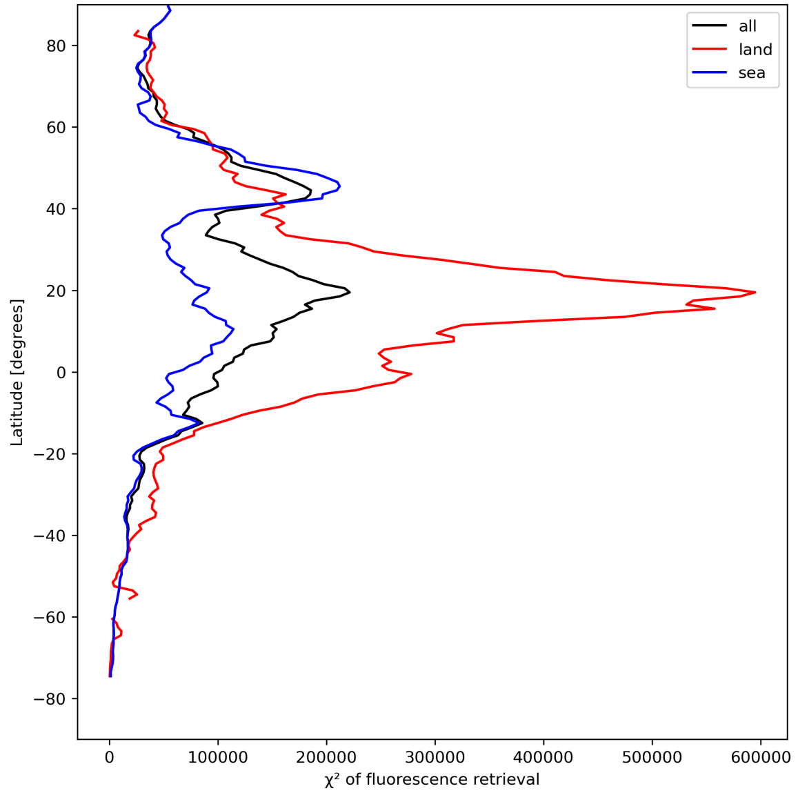
Figure 25: Zonal average of “ \chi^2 of fluorescence retrieval” for 2024-08-14 to 2024-08-16.
