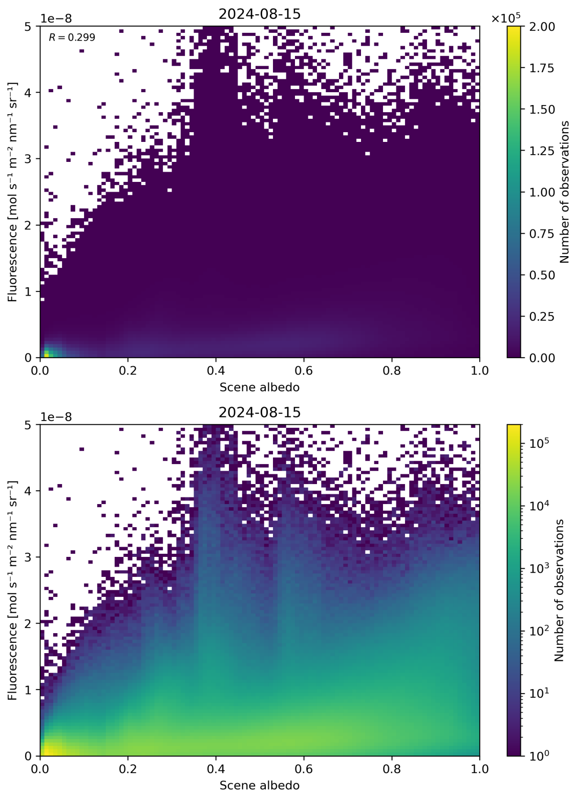
Figure 104: Scatter density plot of “Scene albedo” against “Fluorescence” for 2024-08-14 to 2024-08-16.
