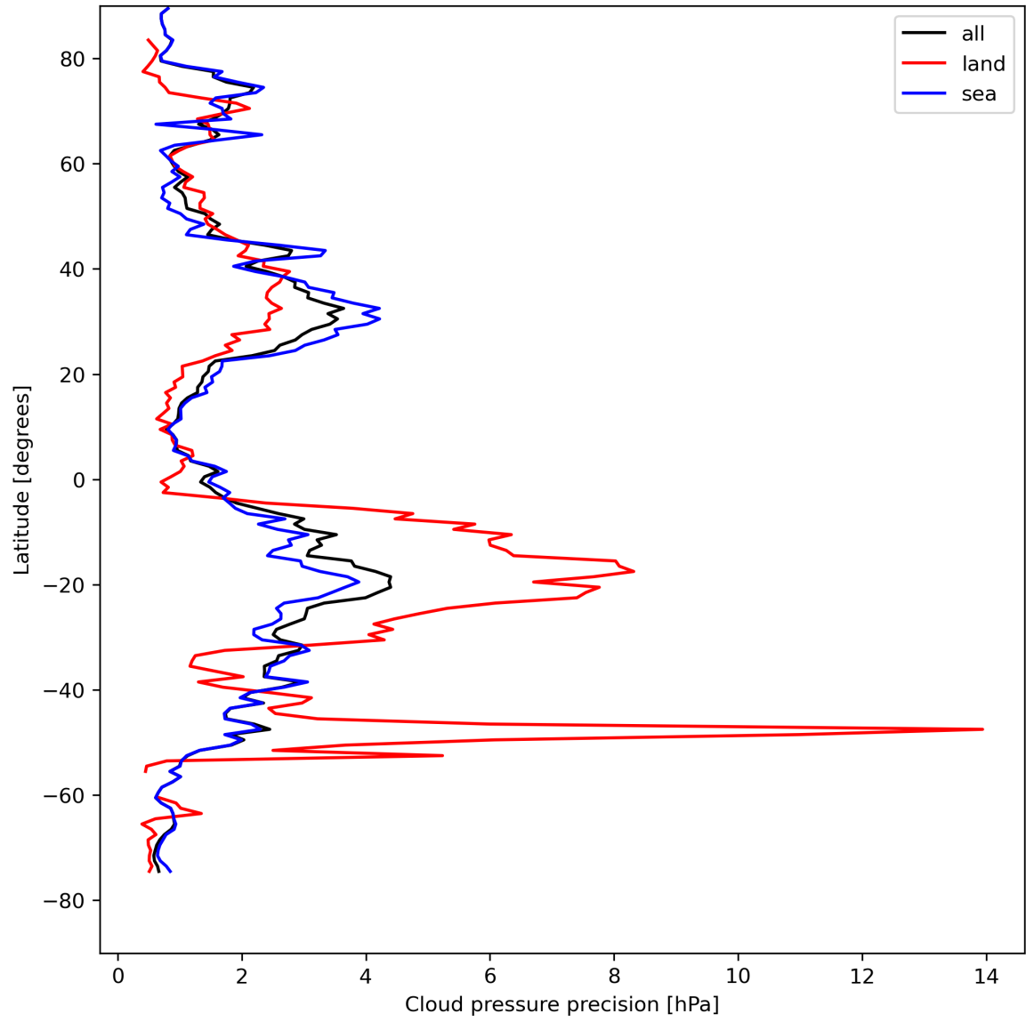
Figure 14: Zonal average of “Cloud pressure precision” for 2024-08-14 to 2024-08-16.
