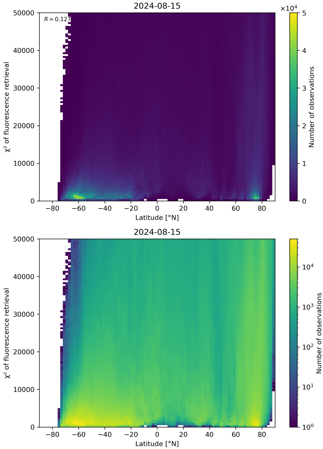
Figure 89: Scatter density plot of “Latitude” against “ \chi^2 of fluorescence retrieval” for 2024-08-14 to 2024-08-16.
