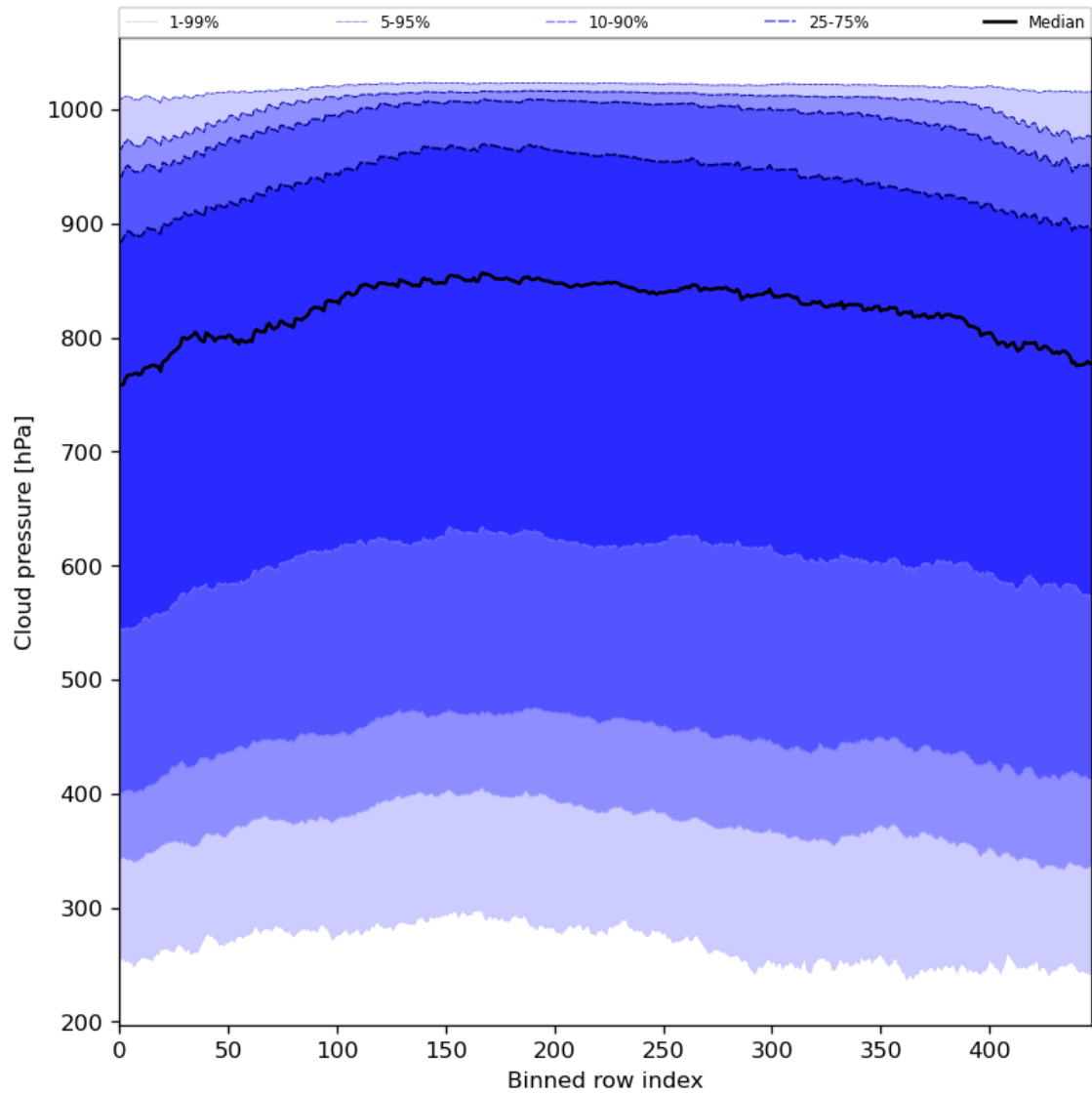
Figure 47: Along track statistics of “Cloud pressure” for 2024-08-14 to 2024-08-16
