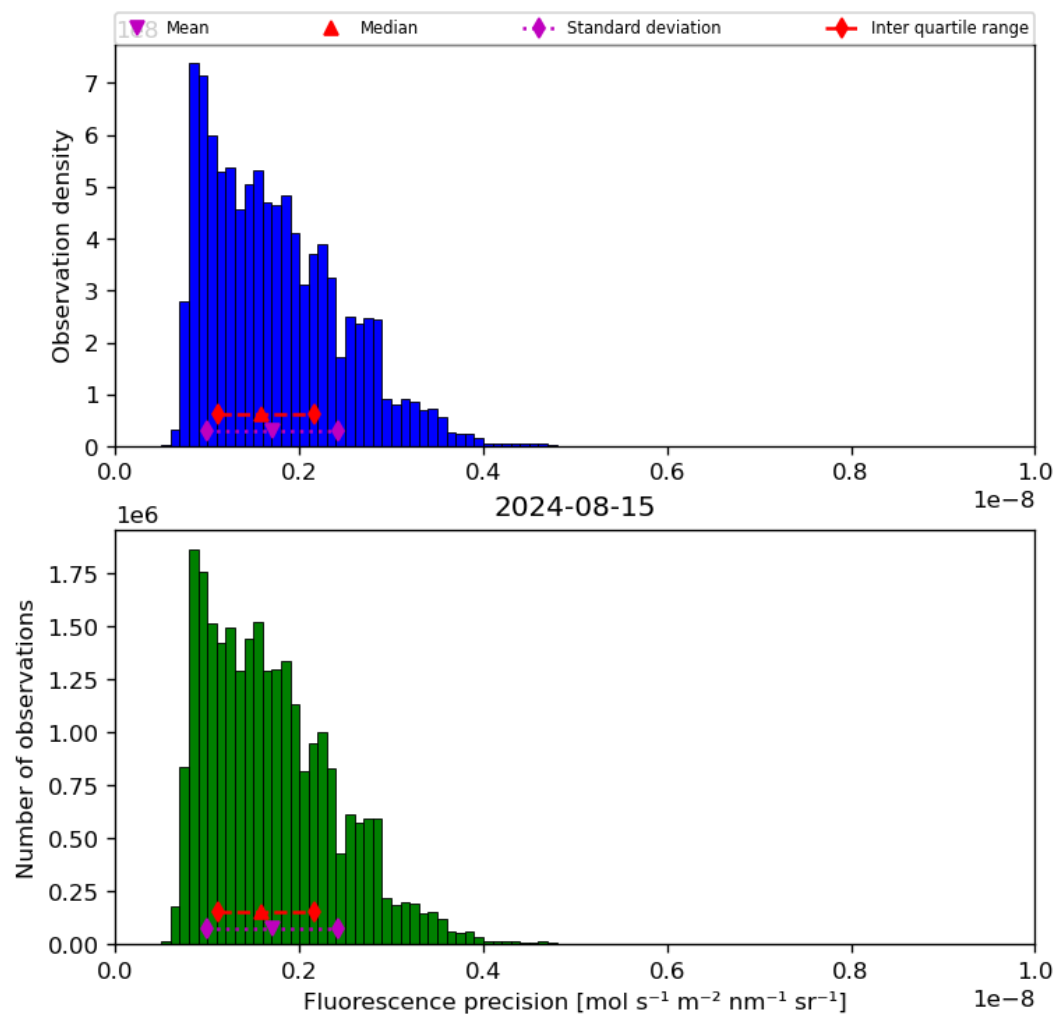
Figure 41: Histogram of “Fluorescence precision” for 2024-08-14 to 2024-08-16
