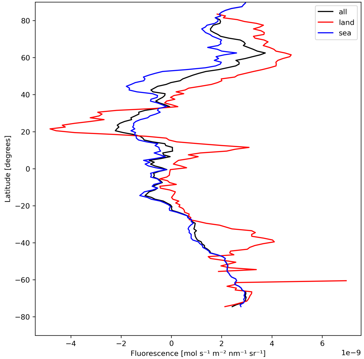
Figure 23: Zonal average of “Fluorescence” for 2024-08-14 to 2024-08-16.
