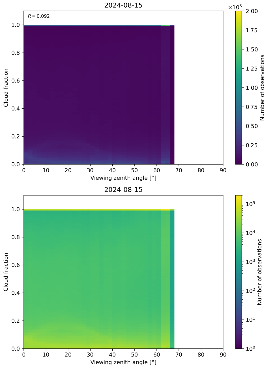
Figure 120: Scatter density plot of “Viewing zenith angle” against “Cloud fraction” for 2024-08-14 to 2024-08-16.
