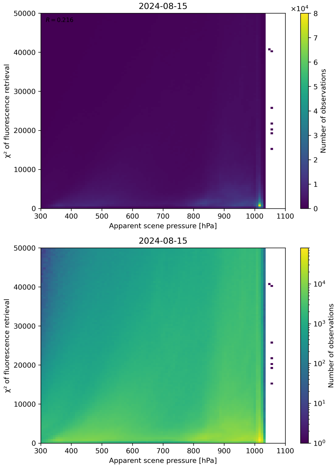
Figure 63: Scatter density plot of “Apparent scene pressure” against “ \chi^2 of fluorescence retrieval” for 2024-08-14 to 2024-08-16.
