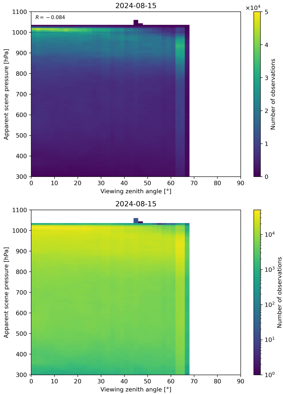
Figure 118: Scatter density plot of “Viewing zenith angle” against “Apparent scene pressure” for 2024-08-14 to 2024-08-16.
