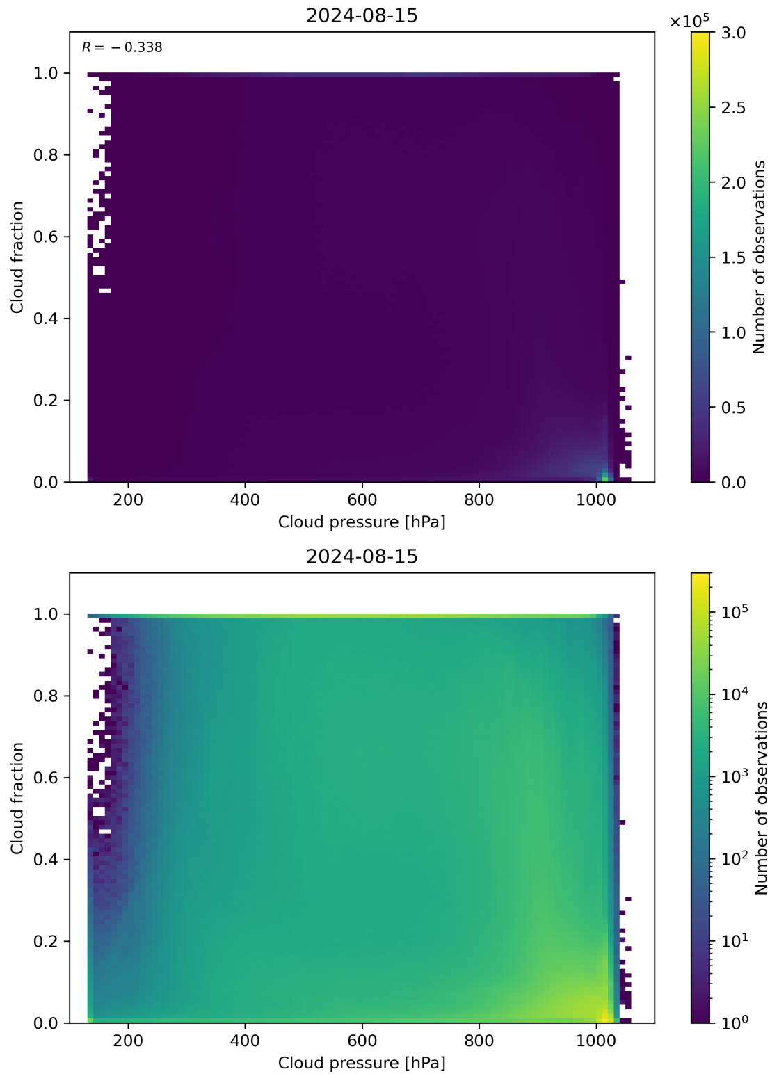
Figure 79: Scatter density plot of “Cloud pressure” against “Cloud fraction” for 2024-08-14 to 2024-08-16.
