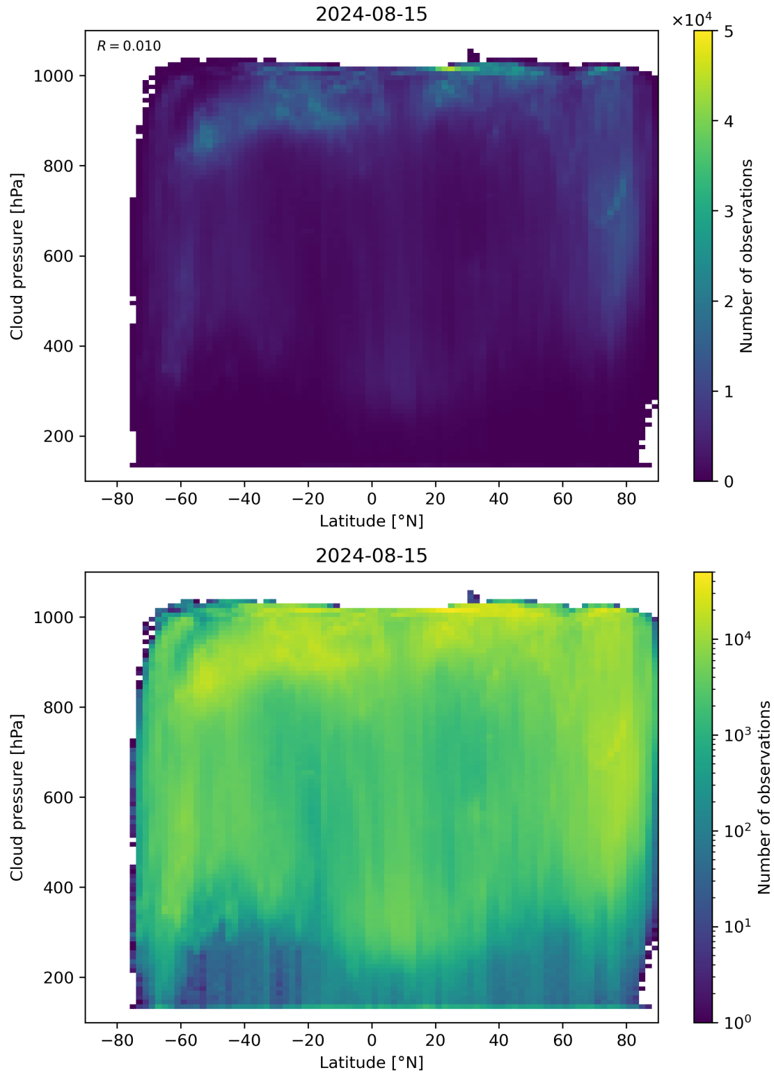
Figure 91: Scatter density plot of “Latitude” against “Cloud pressure” for 2024-08-14 to 2024-08-16.
