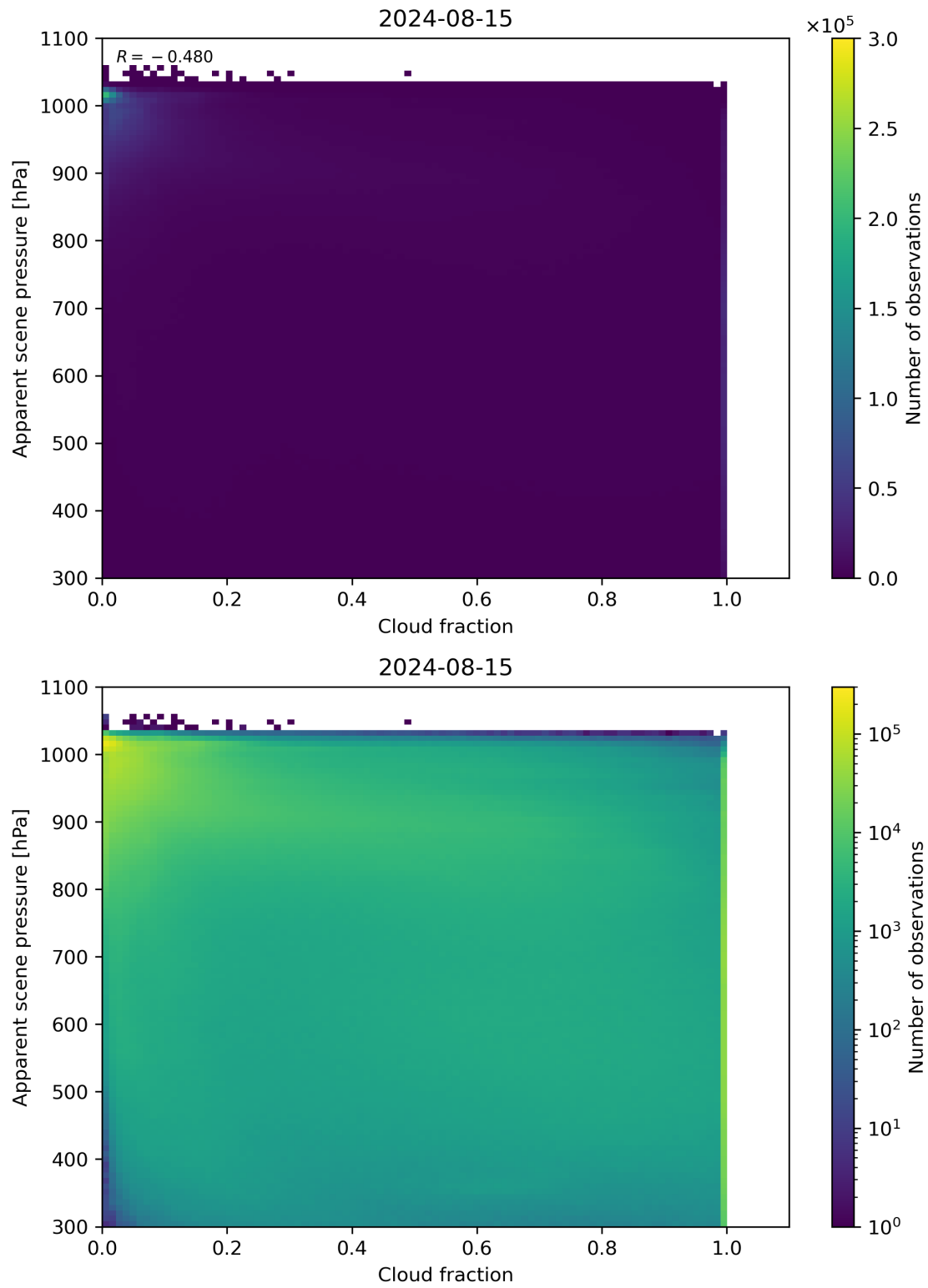
Figure 70: Scatter density plot of “Cloud fraction” against “Apparent scene pressure” for 2024-08-14 to 2024-08-16.
