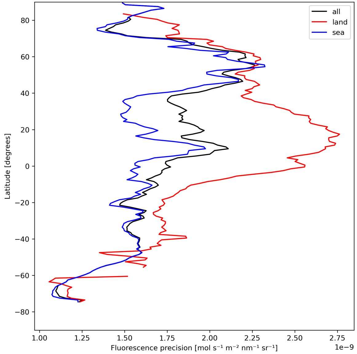
Figure 24: Zonal average of “Fluorescence precision” for 2024-08-14 to 2024-08-16.
