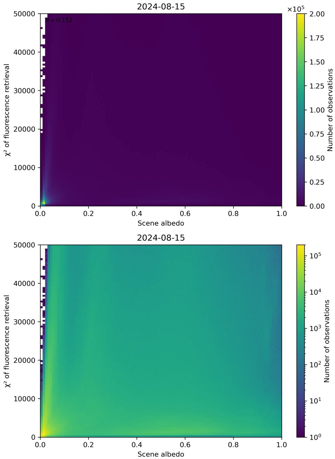
Figure 103: Scatter density plot of “Scene albedo” against “ \chi^2 of fluorescence retrieval” for 2024-08-14 to 2024-08-16.
