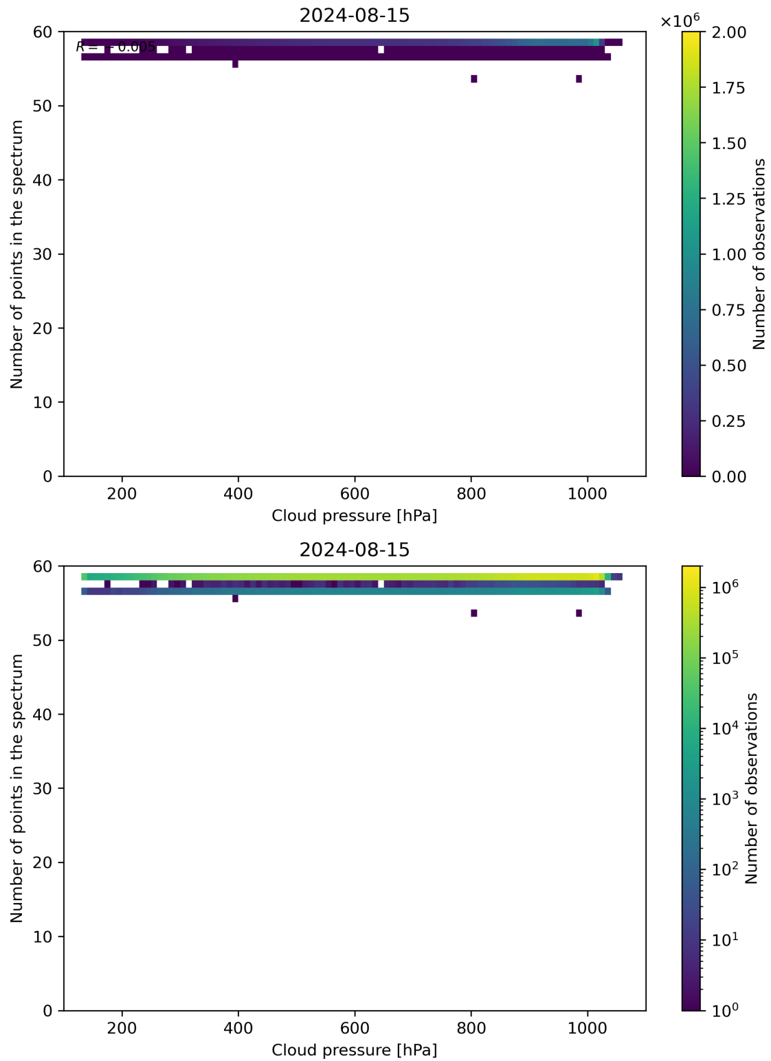
Figure 82: Scatter density plot of “Cloud pressure” against “Number of points in the spectrum” for 2024-08-14 to 2024-08-16.
