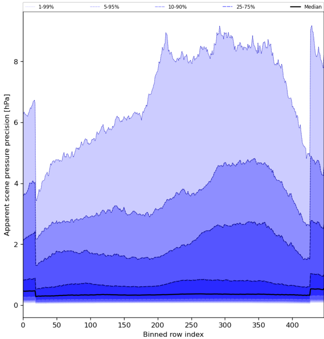
Figure 54: Along track statistics of “Apparent scene pressure precision” for 2024-08-14 to 2024-08-16
