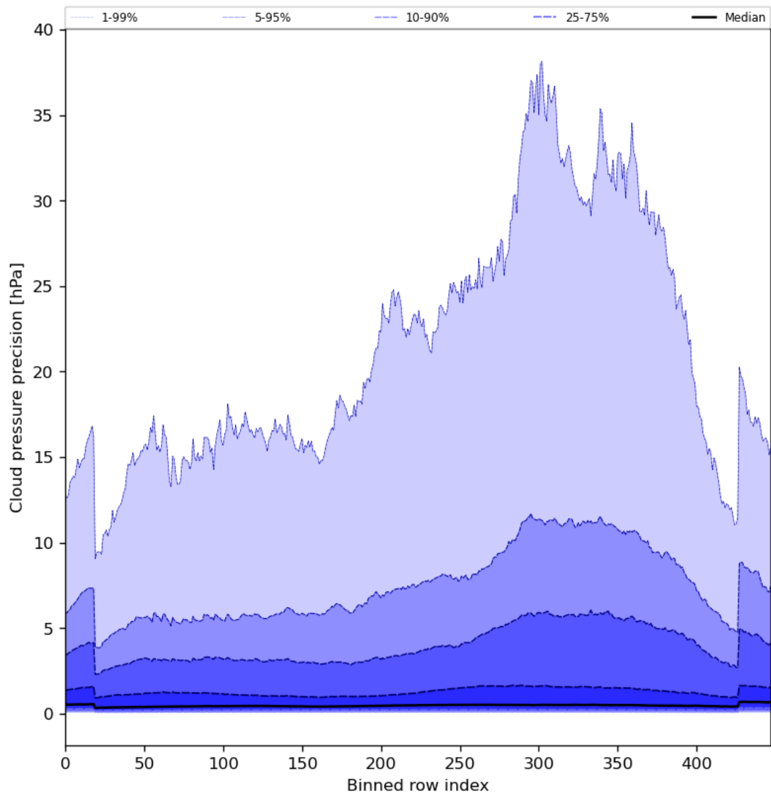
Figure 48: Along track statistics of “Cloud pressure precision” for 2024-08-14 to 2024-08-16
