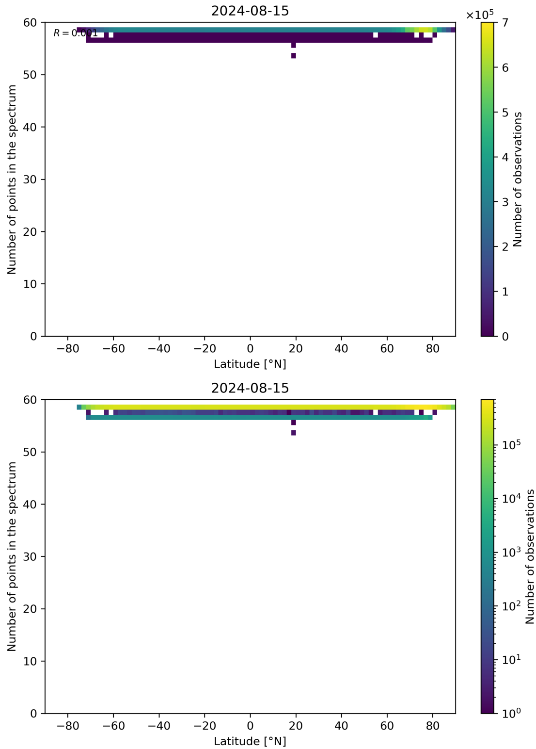
Figure 94: Scatter density plot of “Latitude” against “Number of points in the spectrum” for 2024-08-14 to 2024-08-16.
