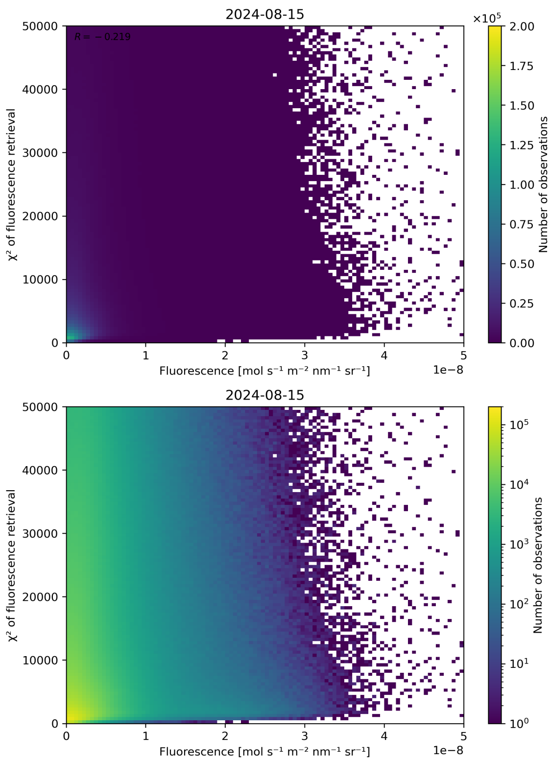
Figure 85: Scatter density plot of “Fluorescence” against “ \chi^2 of fluorescence retrieval” for 2024-08-14 to 2024-08-16.
