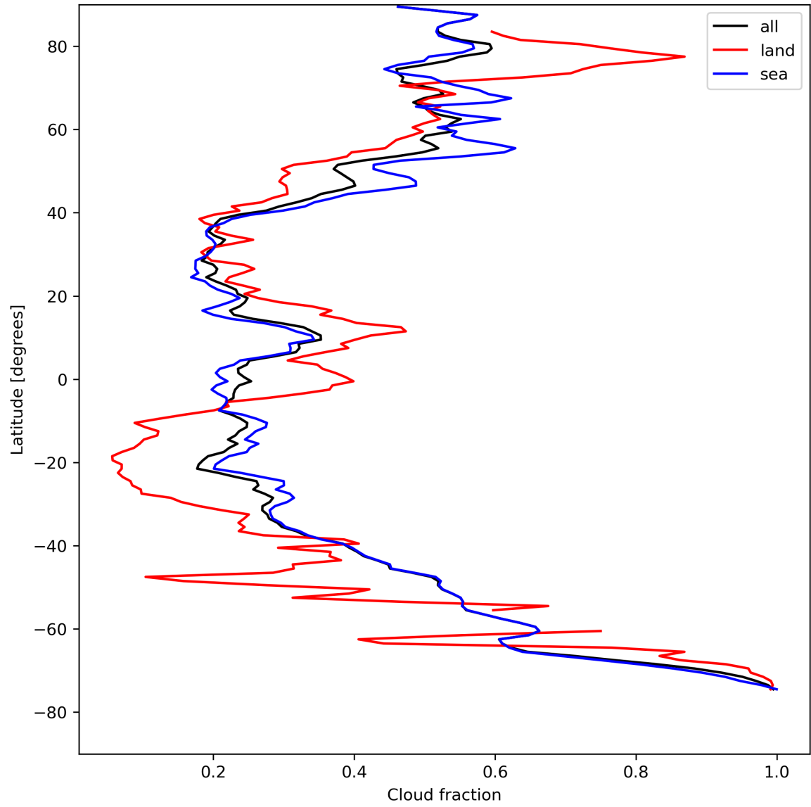
Figure 15: Zonal average of “Cloud fraction” for 2024-08-14 to 2024-08-16.
