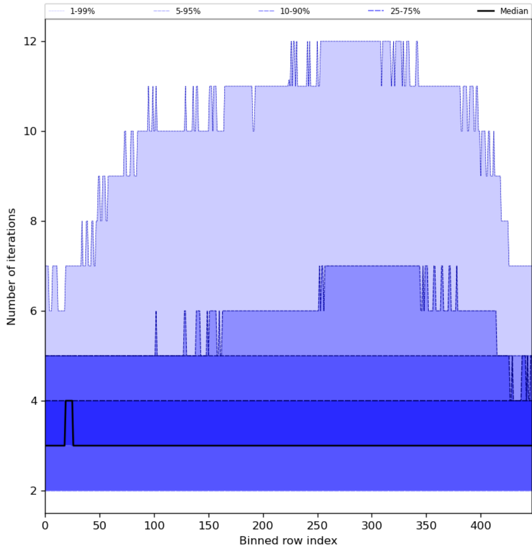
Figure 56: Along track statistics of “Number of iterations” for 2024-08-14 to 2024-08-16
