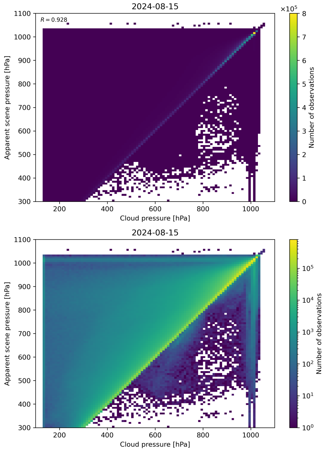
Figure 77: Scatter density plot of “Cloud pressure” against “Apparent scene pressure” for 2024-08-14 to 2024-08-16.
