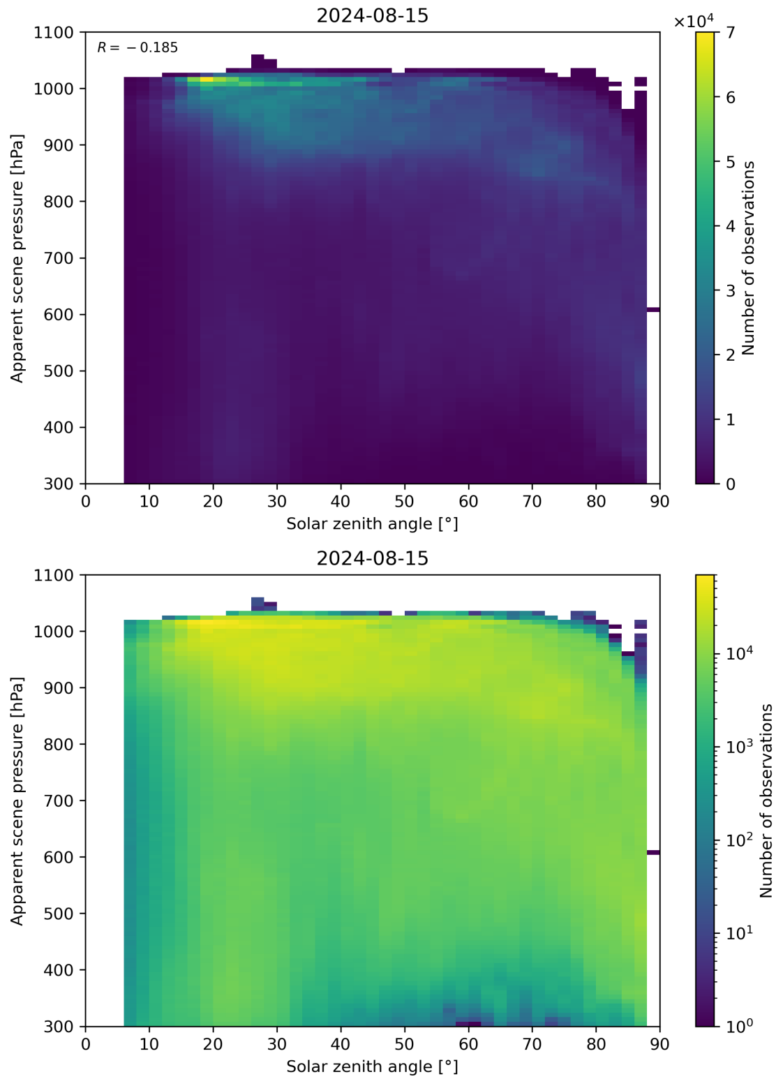
Figure 108: Scatter density plot of “Solar zenith angle” against “Apparent scene pressure” for 2024-08-14 to 2024-08-16.
