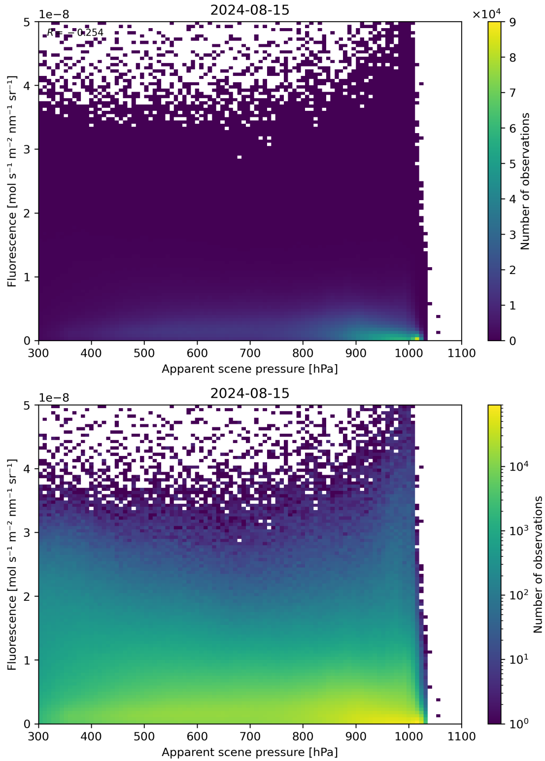
Figure 64: Scatter density plot of “Apparent scene pressure” against “Fluorescence” for 2024-08-14 to 2024-08-16.
