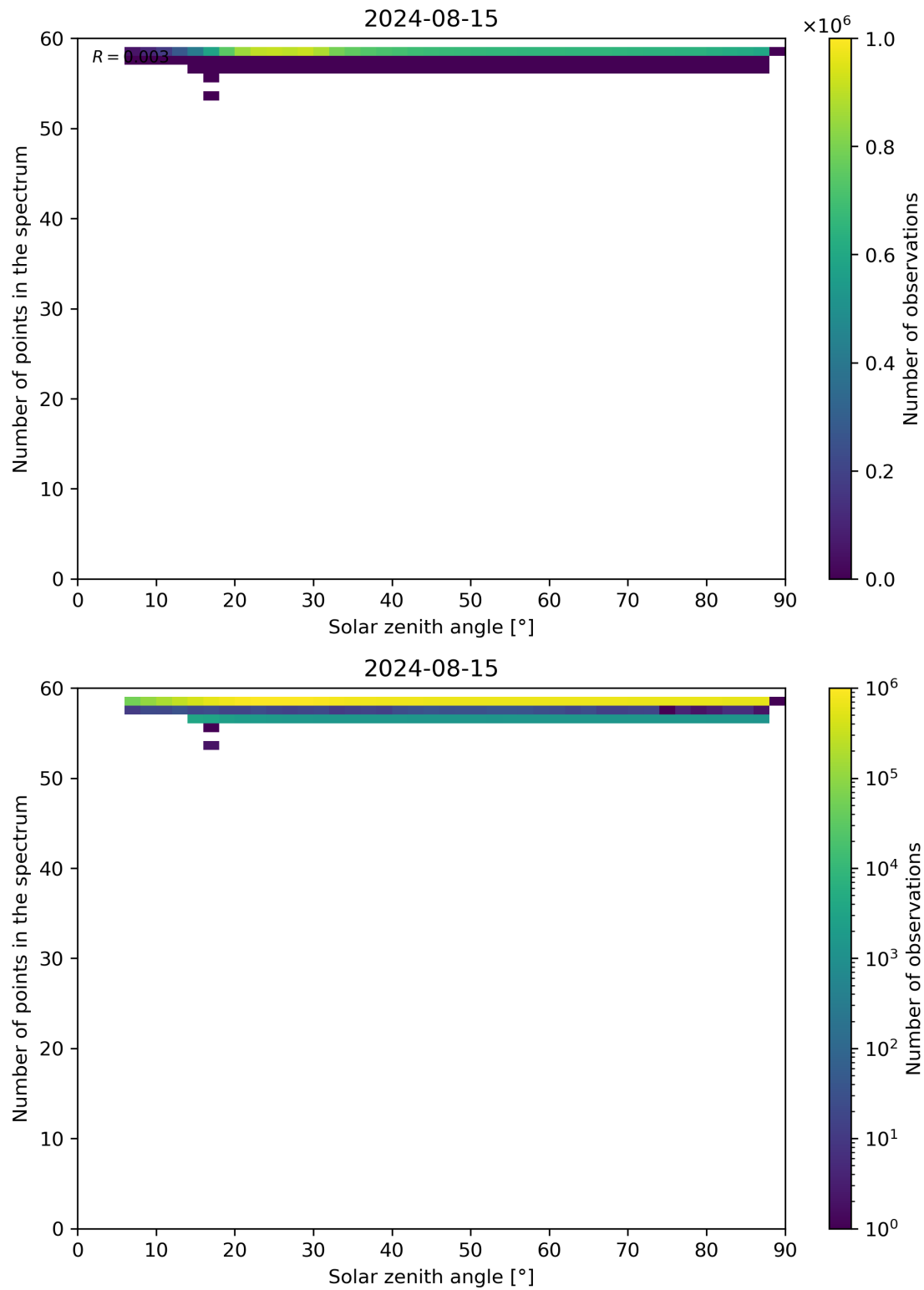
Figure 115: Scatter density plot of “Solar zenith angle” against “Number of points in the spectrum” for 2024-08-14 to 2024-08-16.
