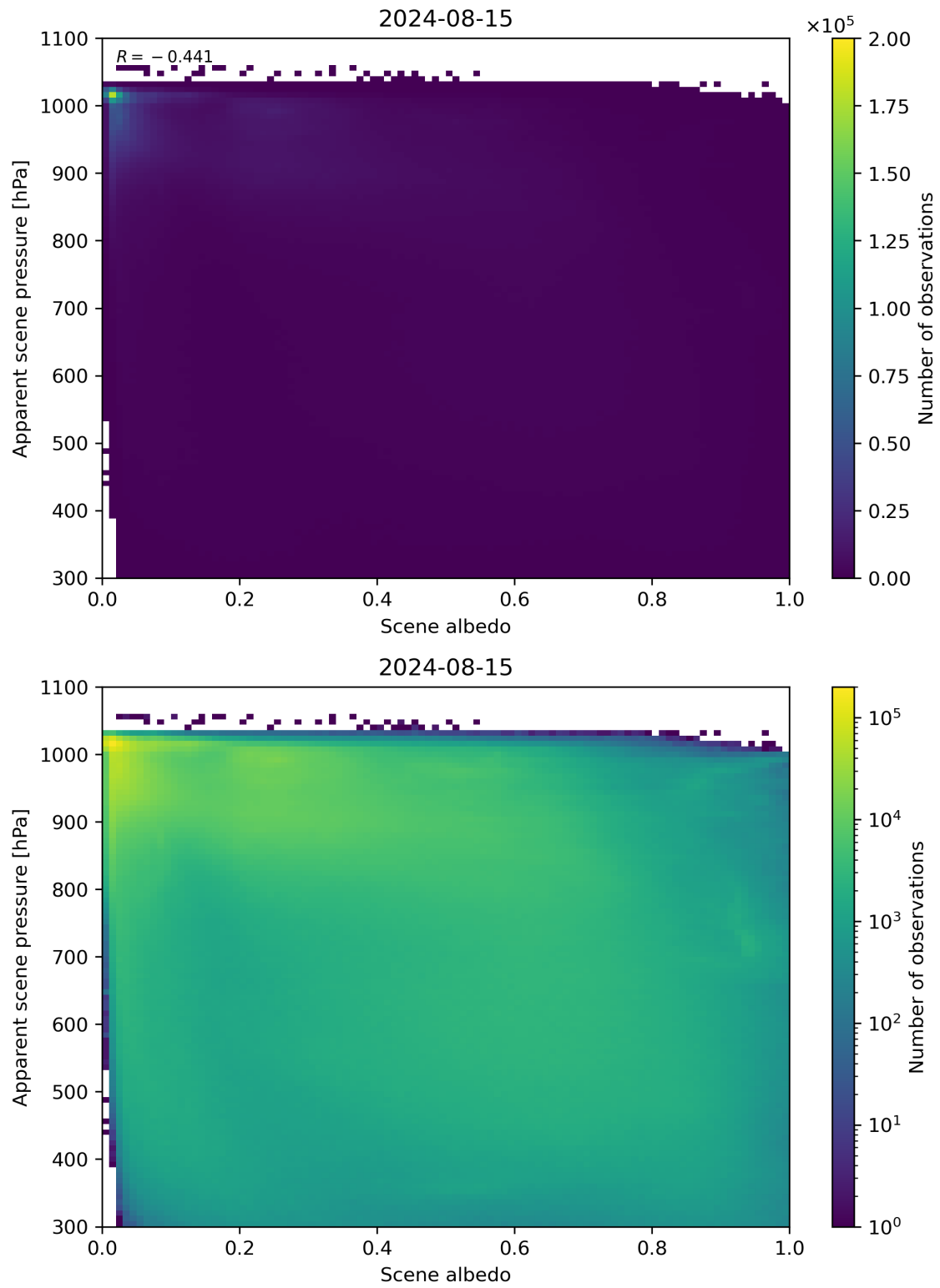
Figure 102: Scatter density plot of “Scene albedo” against “Apparent scene pressure” for 2024-08-14 to 2024-08-16.
