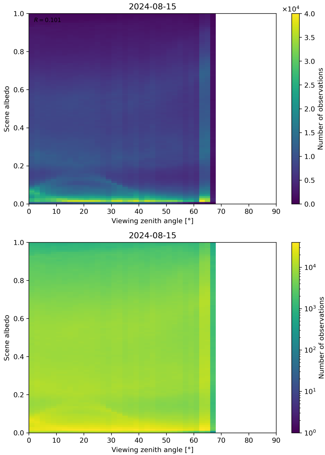
Figure 126: Scatter density plot of “Viewing zenith angle” against “Scene albedo” for 2024-08-14 to 2024-08-16.
