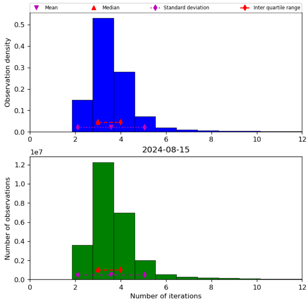
Figure 39: Histogram of “Number of iterations” for 2024-08-14 to 2024-08-16
