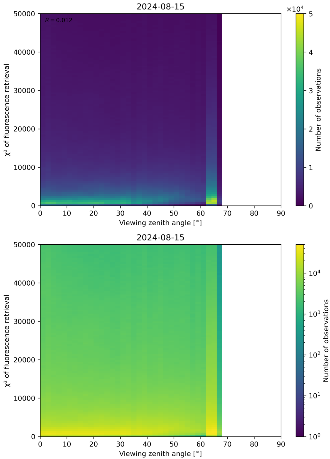
Figure 119: Scatter density plot of “Viewing zenith angle” against “ \chi^2 of fluorescence retrieval” for 2024-08-14 to 2024-08-16.
