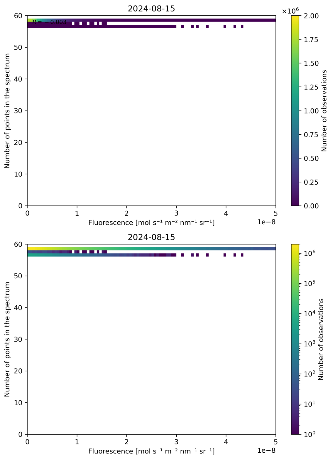
Figure 86: Scatter density plot of “Fluorescence” against “Number of points in the spectrum” for 2024-08-14 to 2024-08-16.
