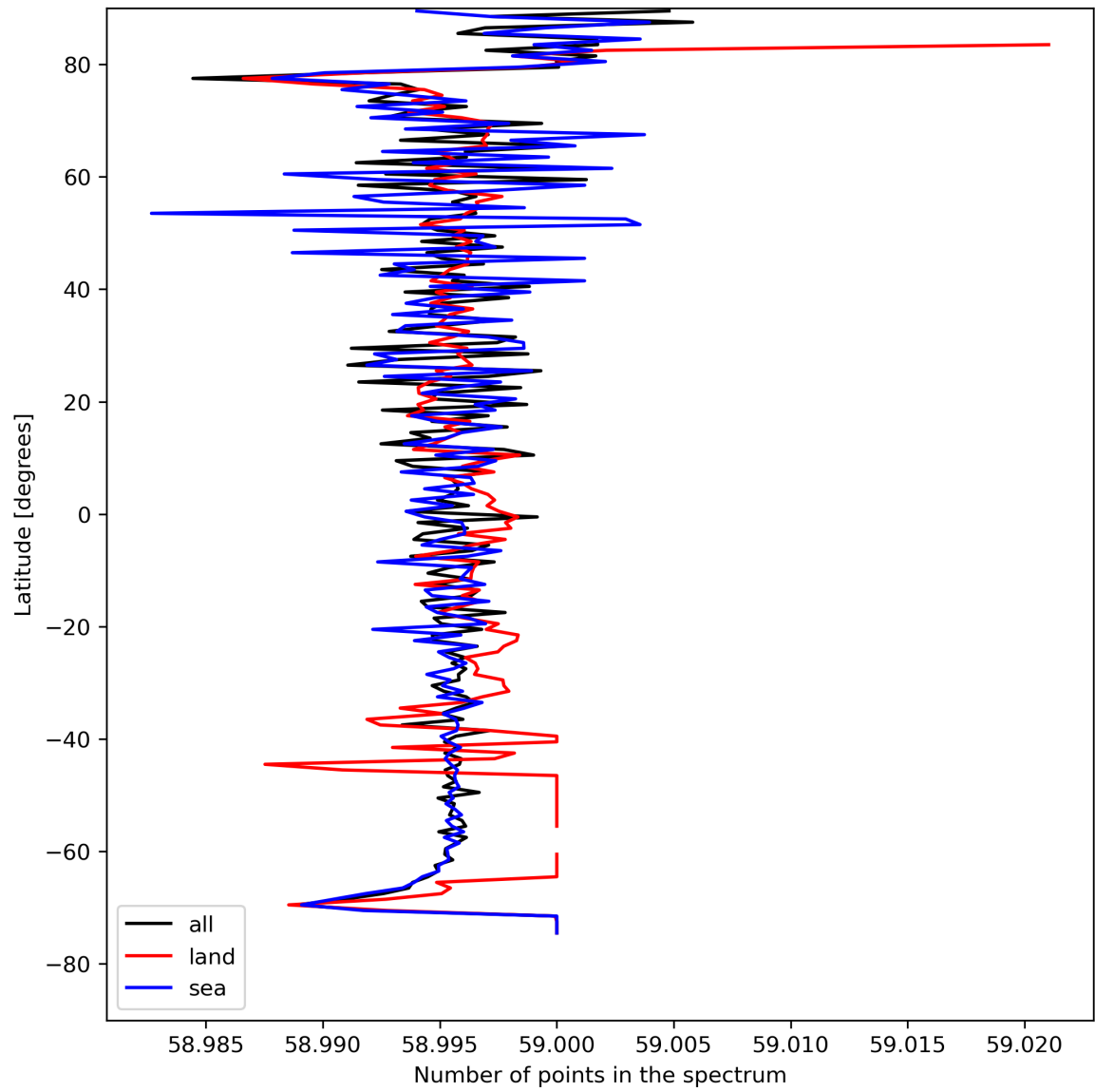
Figure 27: Zonal average of “Number of points in the spectrum” for 2024-08-14 to 2024-08-16.
