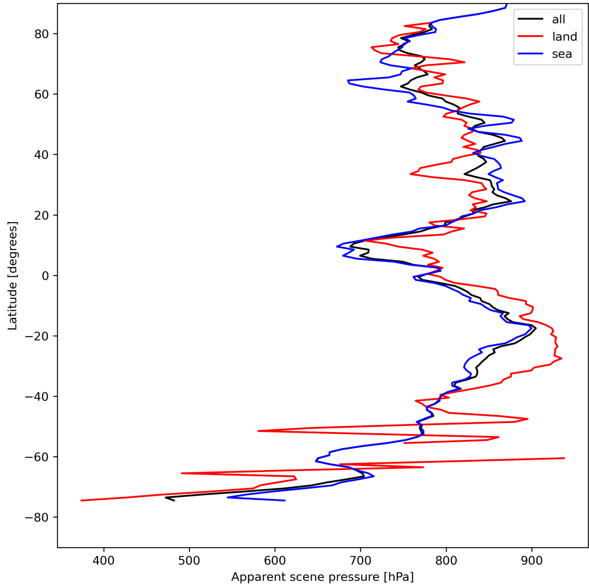
Figure 19: Zonal average of “Apparent scene pressure” for 2024-08-14 to 2024-08-16.
