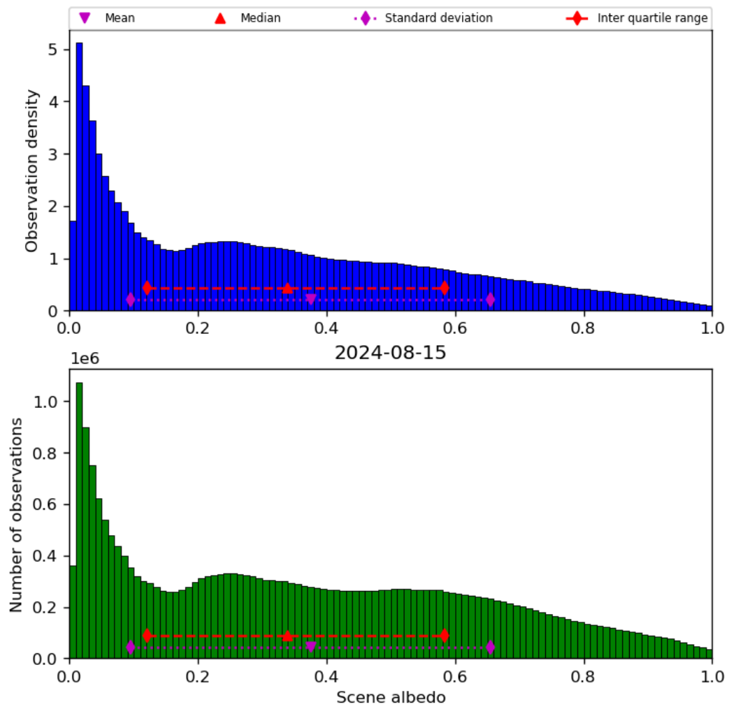
Figure 34: Histogram of “Scene albedo” for 2024-08-14 to 2024-08-16
