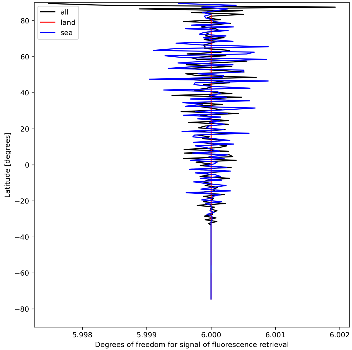
Figure 26: Zonal average of “Degrees of freedom for signal of fluorescence retrieval” for 2024-08-14 to 2024-08-16.
