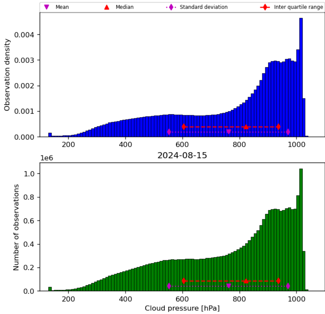
Figure 30: Histogram of “Cloud pressure” for 2024-08-14 to 2024-08-16
