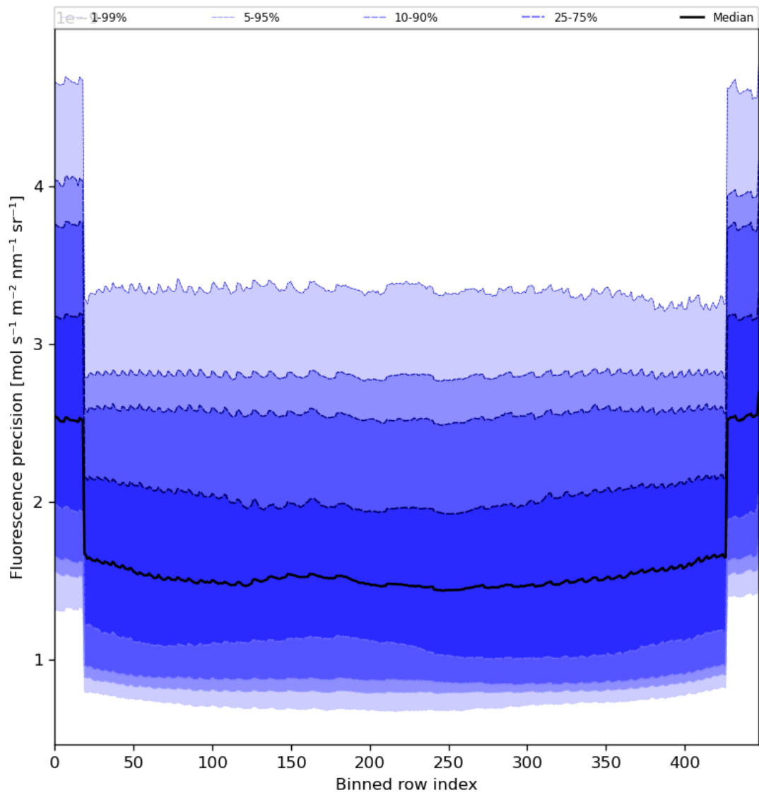
Figure 58: Along track statistics of “Fluorescence precision” for 2024-08-14 to 2024-08-16
