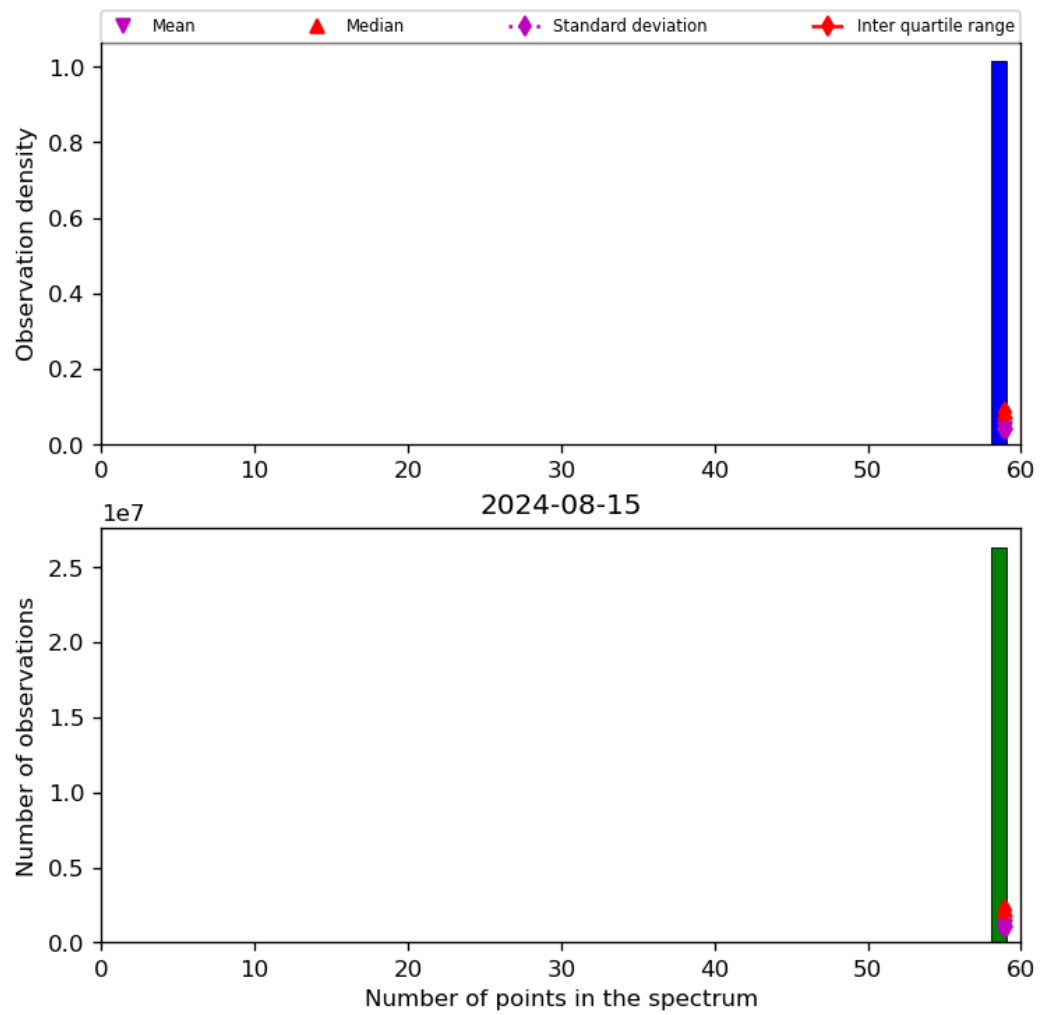
Figure 44: Histogram of “Number of points in the spectrum” for 2024-08-14 to 2024-08-16
