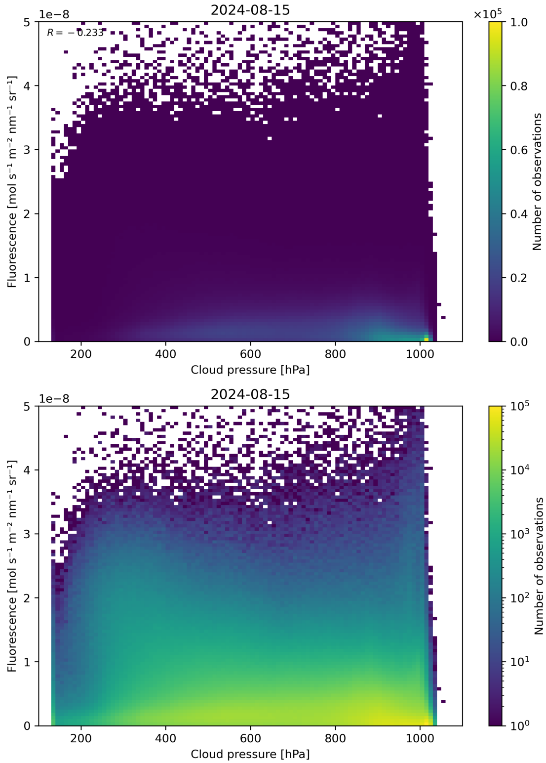
Figure 80: Scatter density plot of “Cloud pressure” against “Fluorescence” for 2024-08-14 to 2024-08-16.
