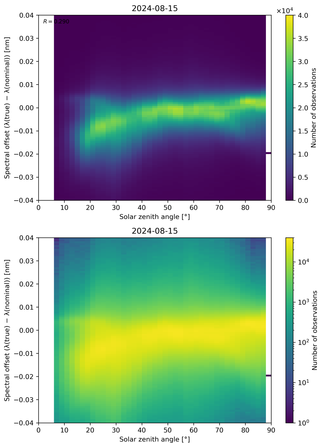
Figure 117: Scatter density plot of “Solar zenith angle” against “Spectral offset ( \lambda(\text{true}) - \lambda(\text{nominal}) )” for 2024-08-14 to 2024-08-16.
