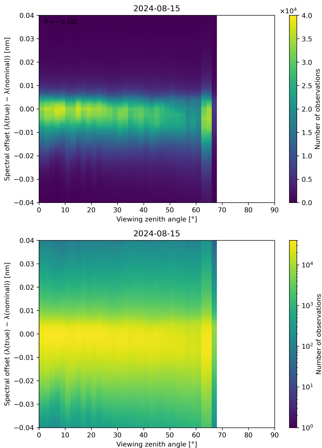
Figure 128: Scatter density plot of “Viewing zenith angle” against “Spectral offset ( \lambda(\text{true}) - \lambda(\text{nominal}) )” for 2024-08-14 to 2024-08-16.
