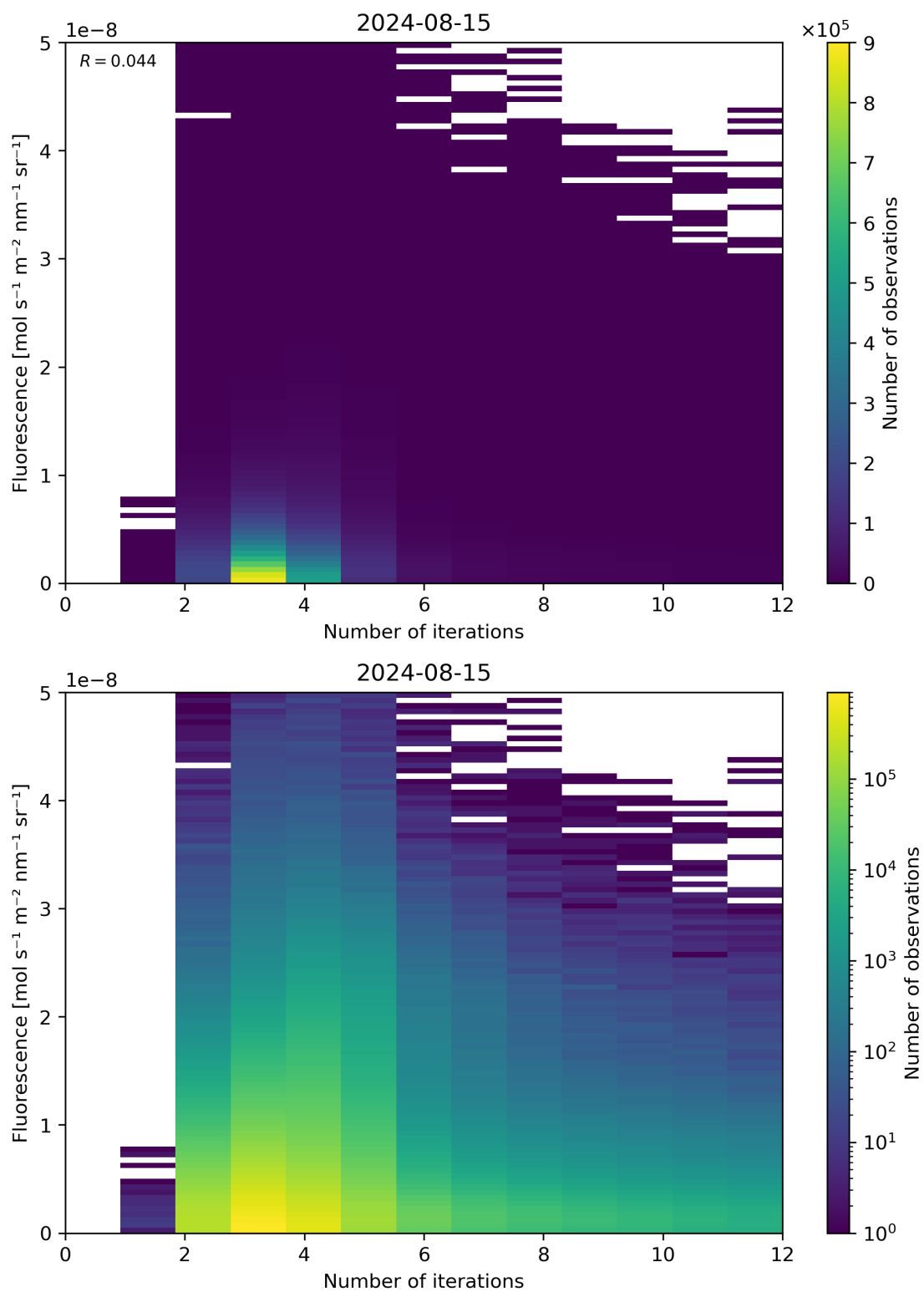
Figure 98: Scatter density plot of “Number of iterations” against “Fluorescence” for 2024-08-14 to 2024-08-16.
