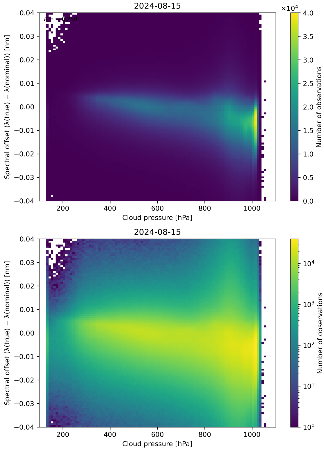
Figure 84: Scatter density plot of “Cloud pressure” against “Spectral offset ( \lambda(\text{true}) - \lambda(\text{nominal}) )” for 2024-08-14 to 2024-08-16.
