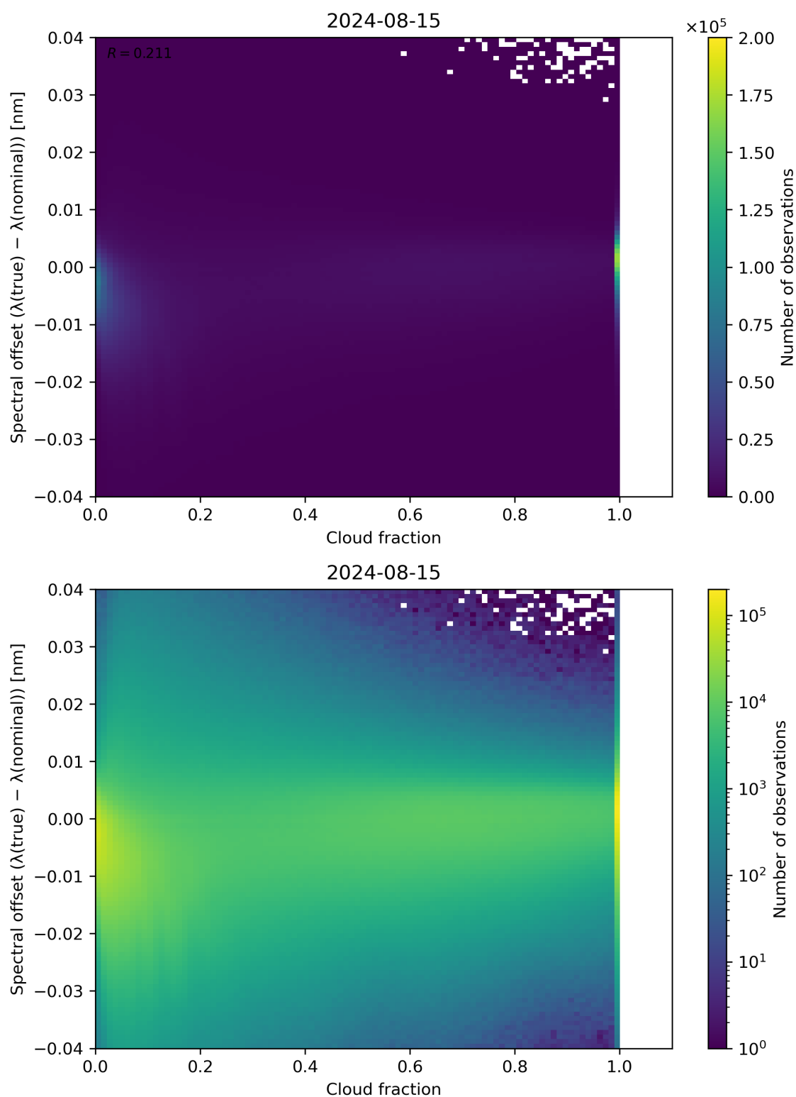
Figure 76: Scatter density plot of “Cloud fraction” against “Spectral offset ( \lambda(\text{true}) - \lambda(\text{nominal}) )” for 2024-08-14 to 2024-08-16.
