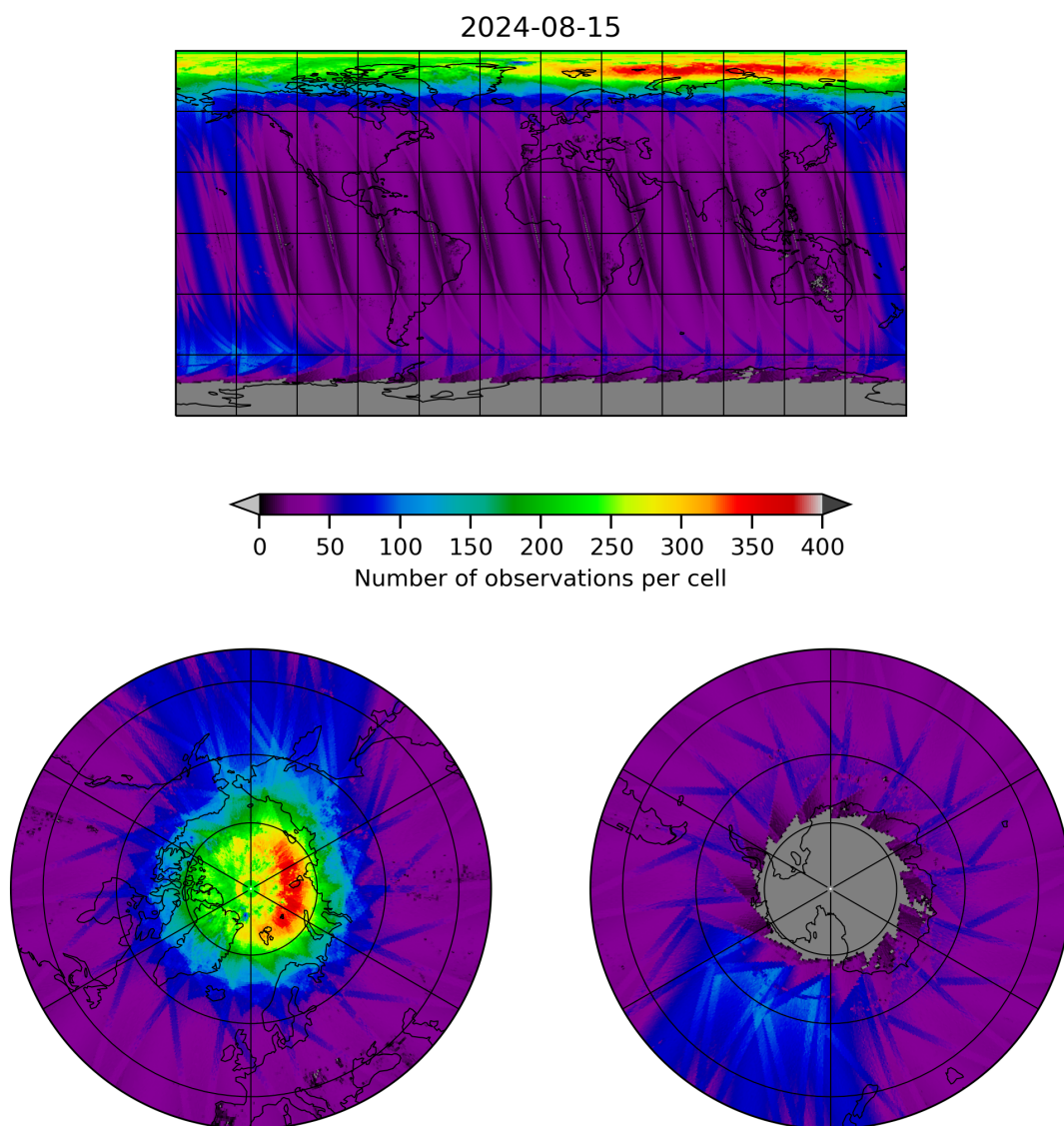
Figure 11: Map of the number of observations for 2024-08-14 to 2024-08-16
