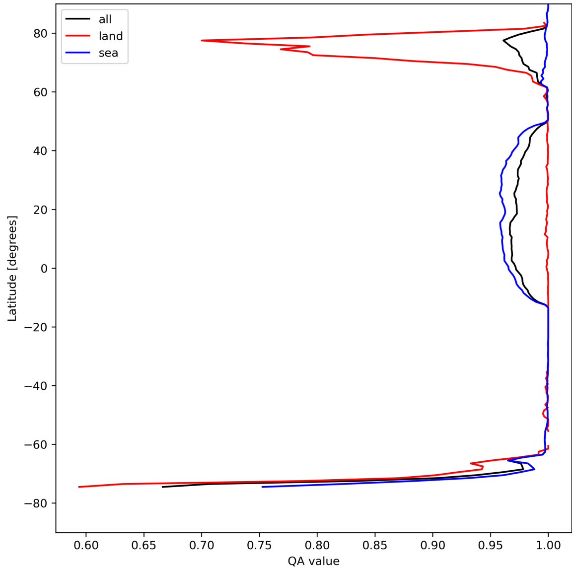
Figure 12: Zonal average of “QA value” for 2024-08-14 to 2024-08-16.
