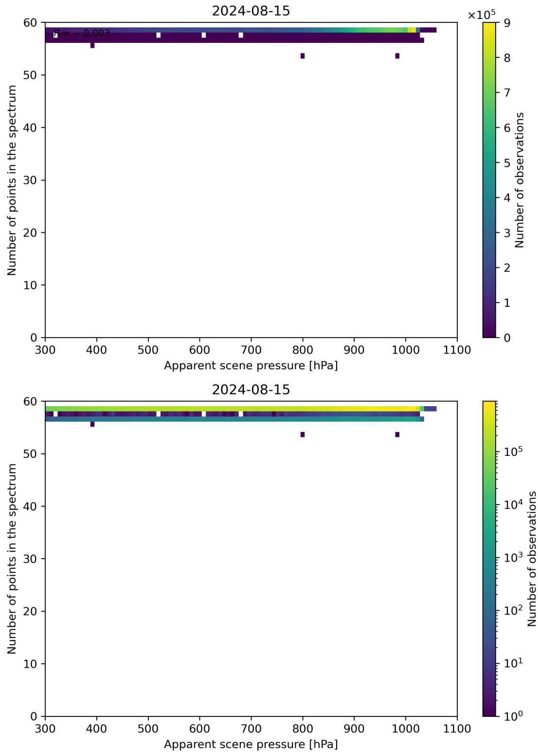
Figure 66: Scatter density plot of “Apparent scene pressure” against “Number of points in the spectrum” for 2024-08-14 to 2024-08-16.
