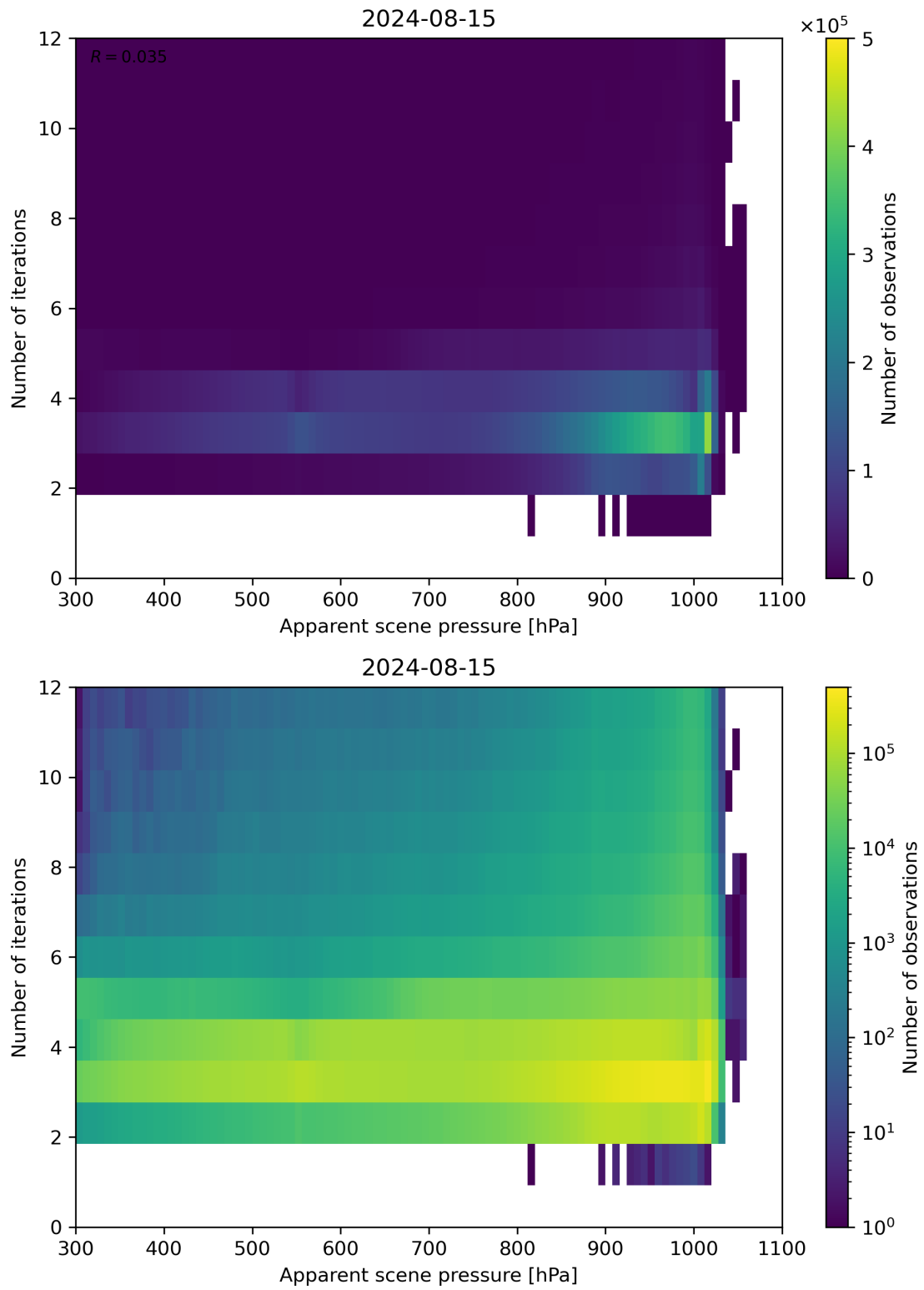
Figure 65: Scatter density plot of “Apparent scene pressure” against “Number of iterations” for 2024-08-14 to 2024-08-16.
