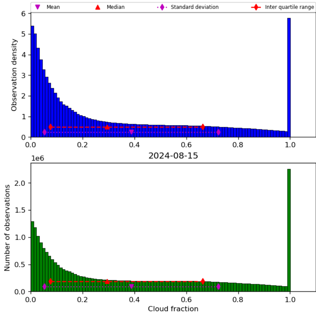
Figure 32: Histogram of “Cloud fraction” for 2024-08-14 to 2024-08-16
