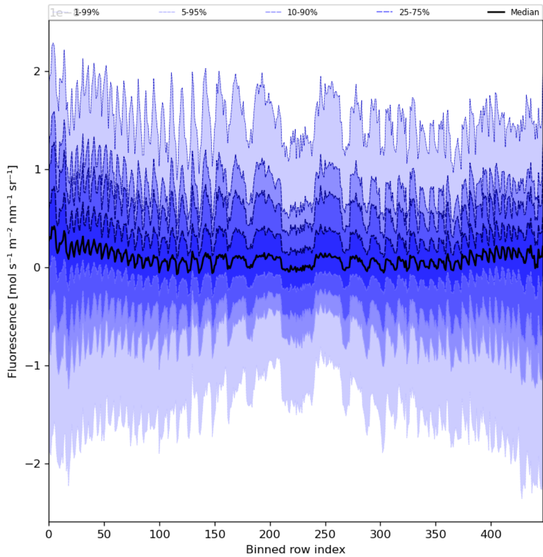
Figure 57: Along track statistics of “Fluorescence” for 2024-08-14 to 2024-08-16
