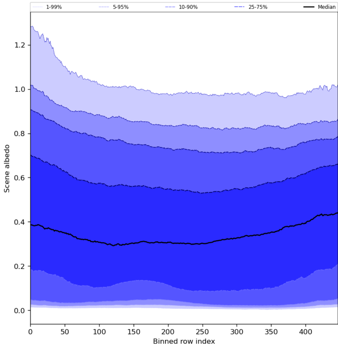
Figure 51: Along track statistics of “Scene albedo” for 2024-08-14 to 2024-08-16
