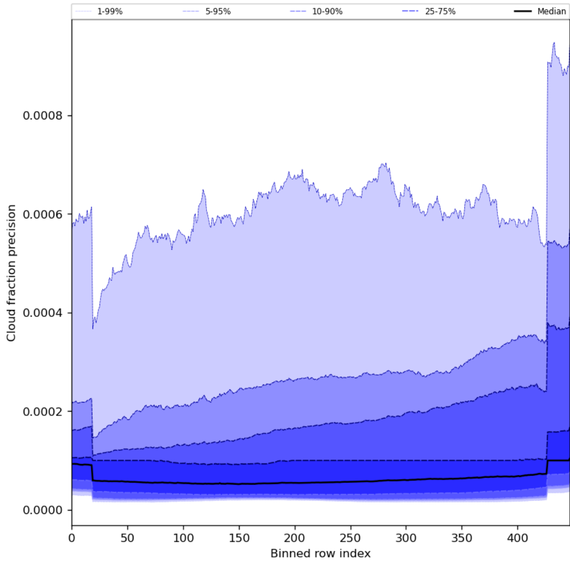
Figure 50: Along track statistics of “Cloud fraction precision” for 2024-08-16 to 2024-08-17
