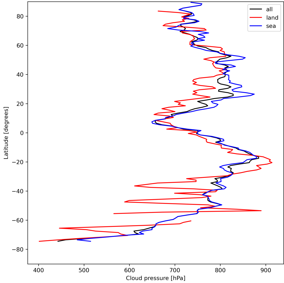
Figure 13: Zonal average of “Cloud pressure” for 2024-08-16 to 2024-08-17.
