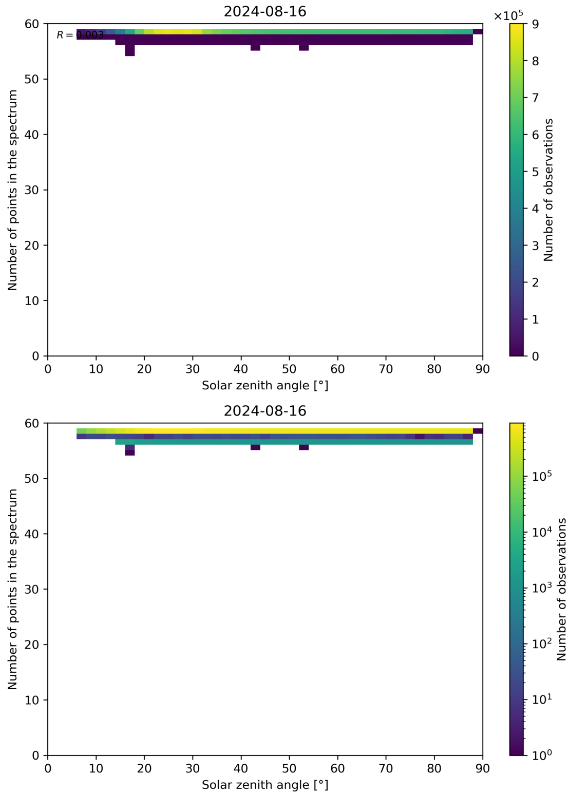
Figure 115: Scatter density plot of “Solar zenith angle” against “Number of points in the spectrum” for 2024-08-16 to 2024-08-17.
