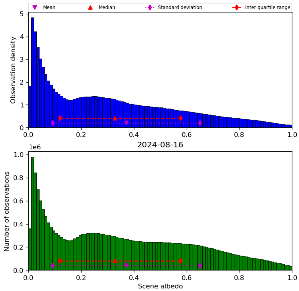
Figure 34: Histogram of “Scene albedo” for 2024-08-16 to 2024-08-17
