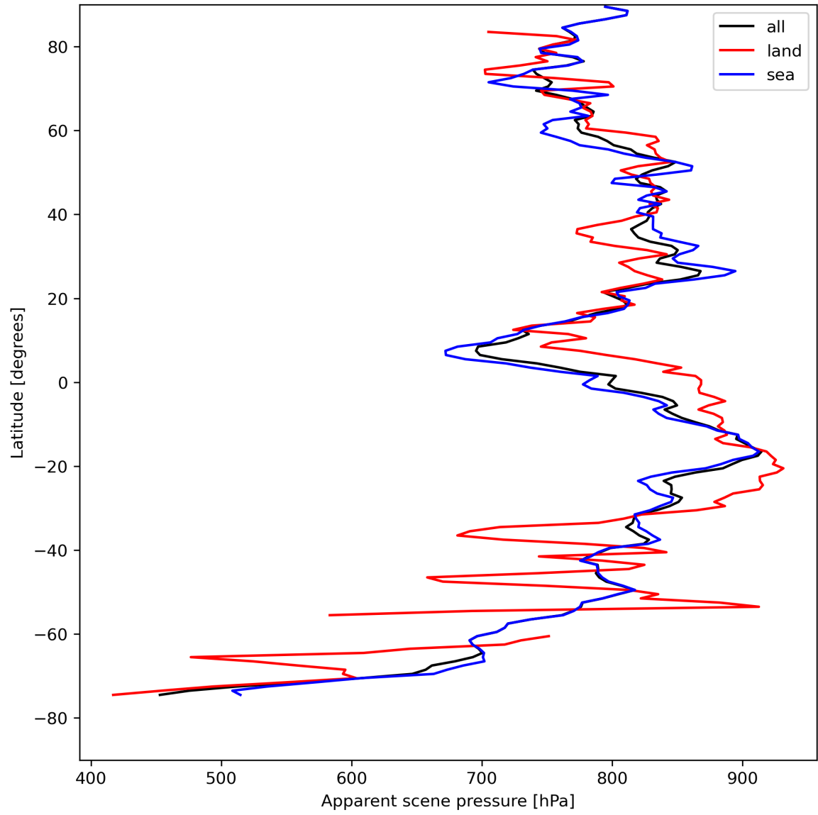
Figure 19: Zonal average of “Apparent scene pressure” for 2024-08-16 to 2024-08-17.
