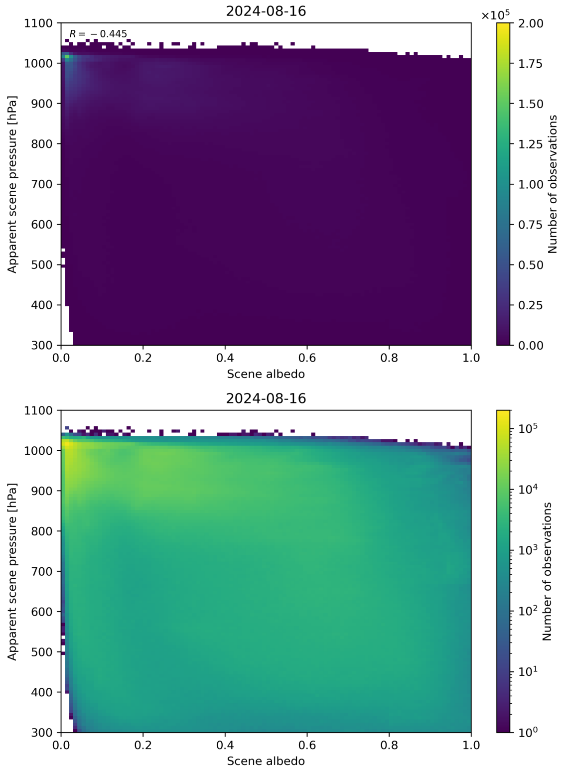
Figure 102: Scatter density plot of “Scene albedo” against “Apparent scene pressure” for 2024-08-16 to 2024-08-17.
