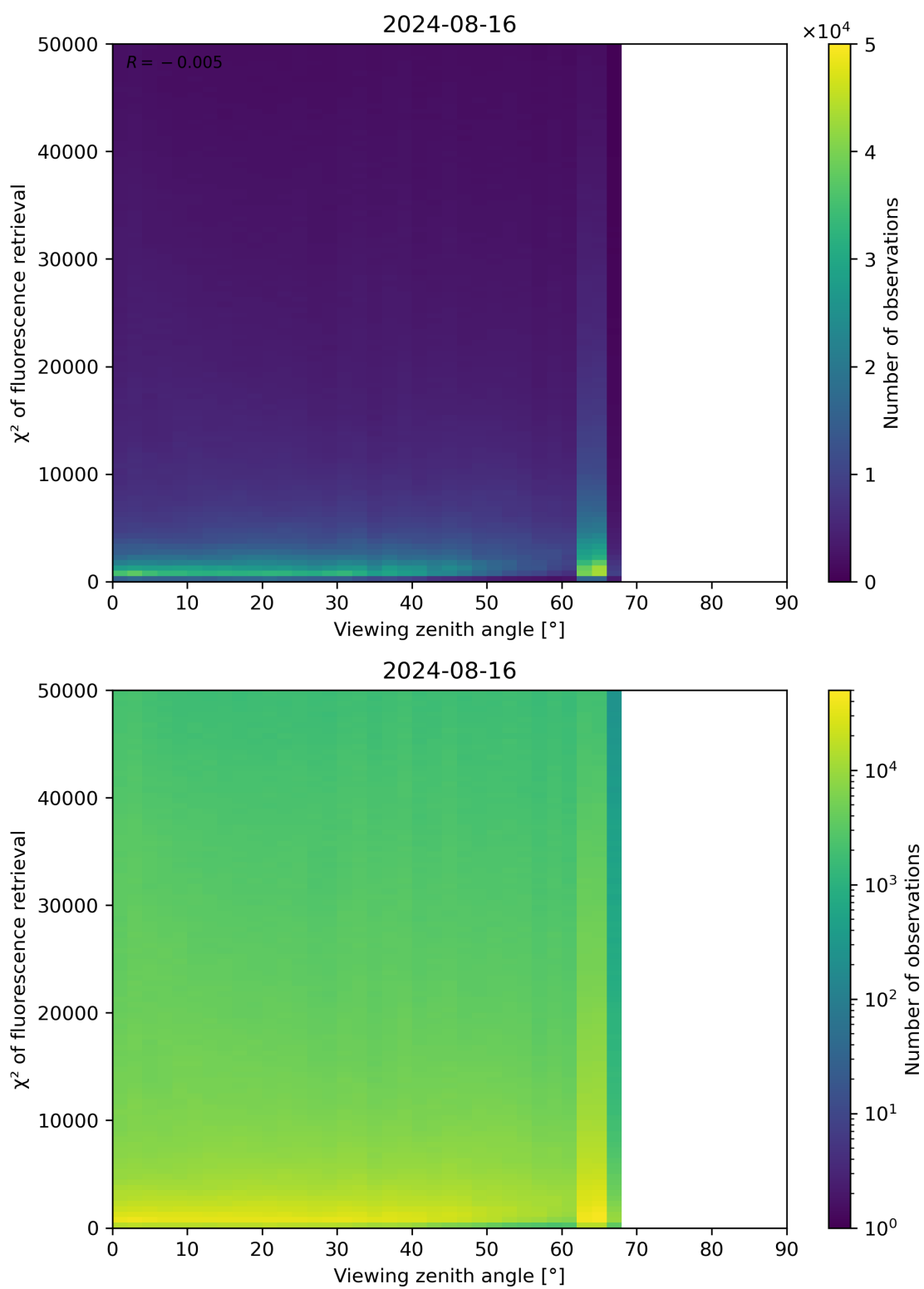
Figure 119: Scatter density plot of “Viewing zenith angle” against “ \chi^2 of fluorescence retrieval” for 2024-08-16 to 2024-08-17.
