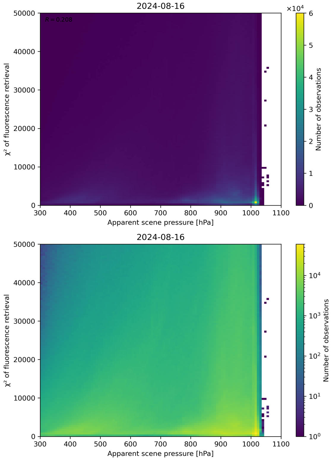
Figure 63: Scatter density plot of “Apparent scene pressure” against “ \chi^2 of fluorescence retrieval” for 2024-08-16 to 2024-08-17.
