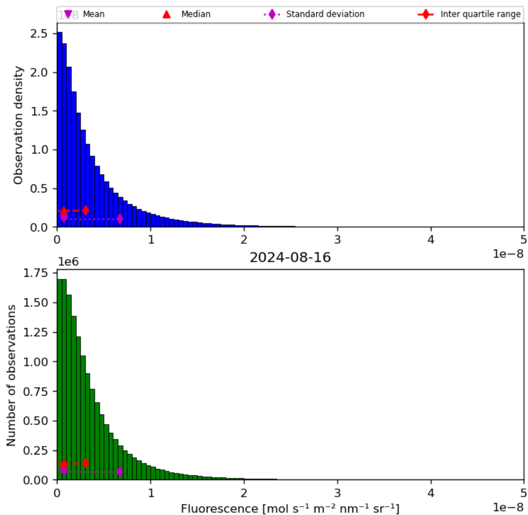
Figure 40: Histogram of “Fluorescence” for 2024-08-16 to 2024-08-17
