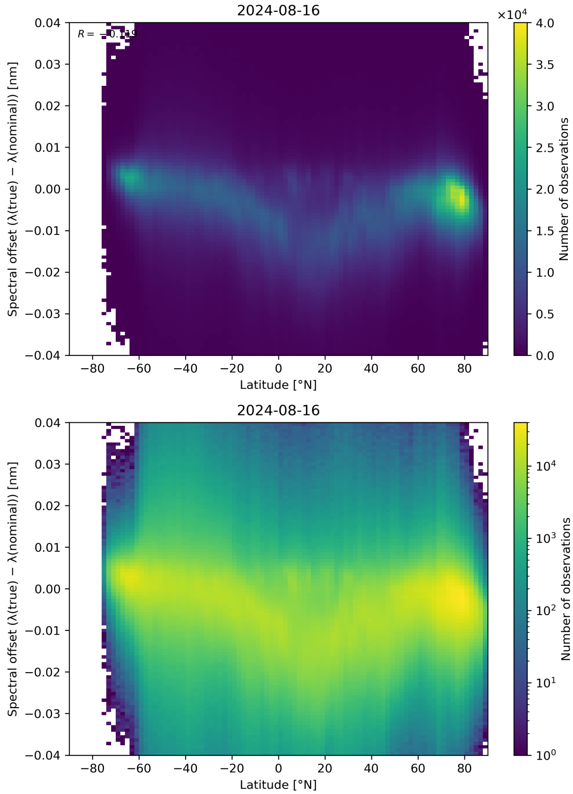
Figure 96: Scatter density plot of “Latitude” against “Spectral offset ( \lambda(\text{true}) - \lambda(\text{nominal}) )” for 2024-08-16 to 2024-08-17.
