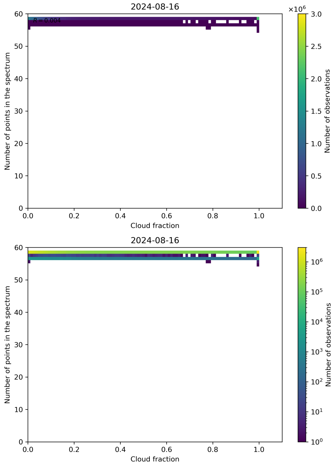
Figure 74: Scatter density plot of “Cloud fraction” against “Number of points in the spectrum” for 2024-08-16 to 2024-08-17.
