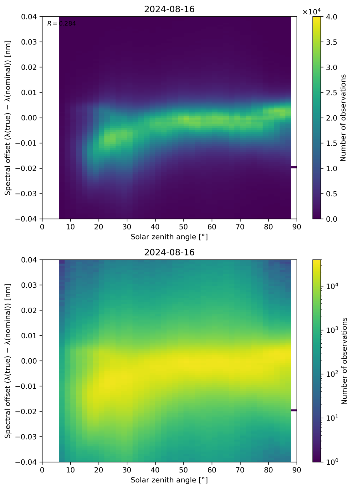
Figure 117: Scatter density plot of “Solar zenith angle” against “Spectral offset ( \lambda(\text{true}) - \lambda(\text{nominal}) )” for 2024-08-16 to 2024-08-17.
