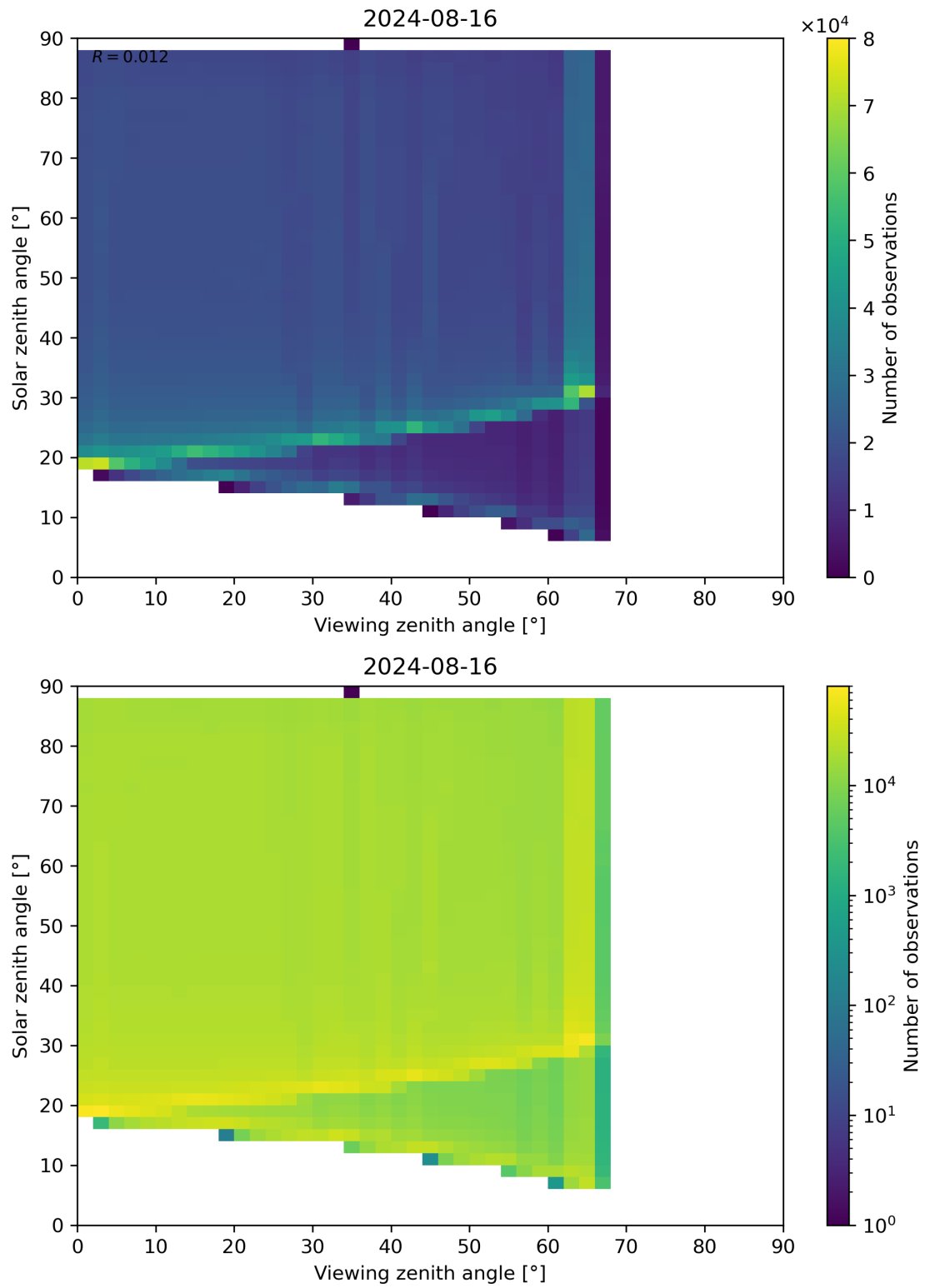
Figure 127: Scatter density plot of “Viewing zenith angle” against “Solar zenith angle” for 2024-08-16 to 2024-08-17.
