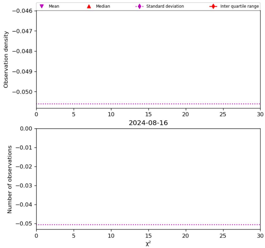
Figure 38: Histogram of " \chi^2 " for 2024-08-16 to 2024-08-17
