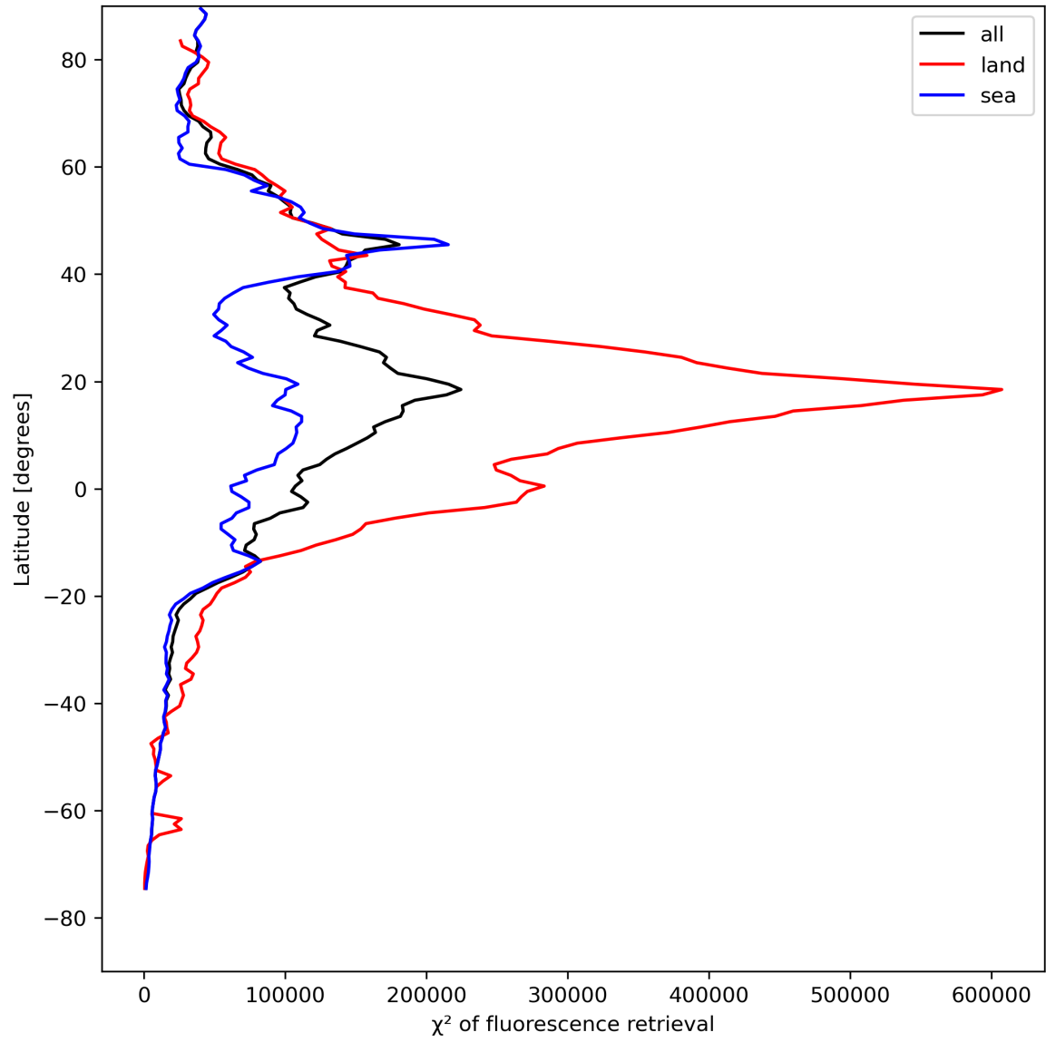
Figure 25: Zonal average of “ \chi^2 of fluorescence retrieval” for 2024-08-16 to 2024-08-17.
