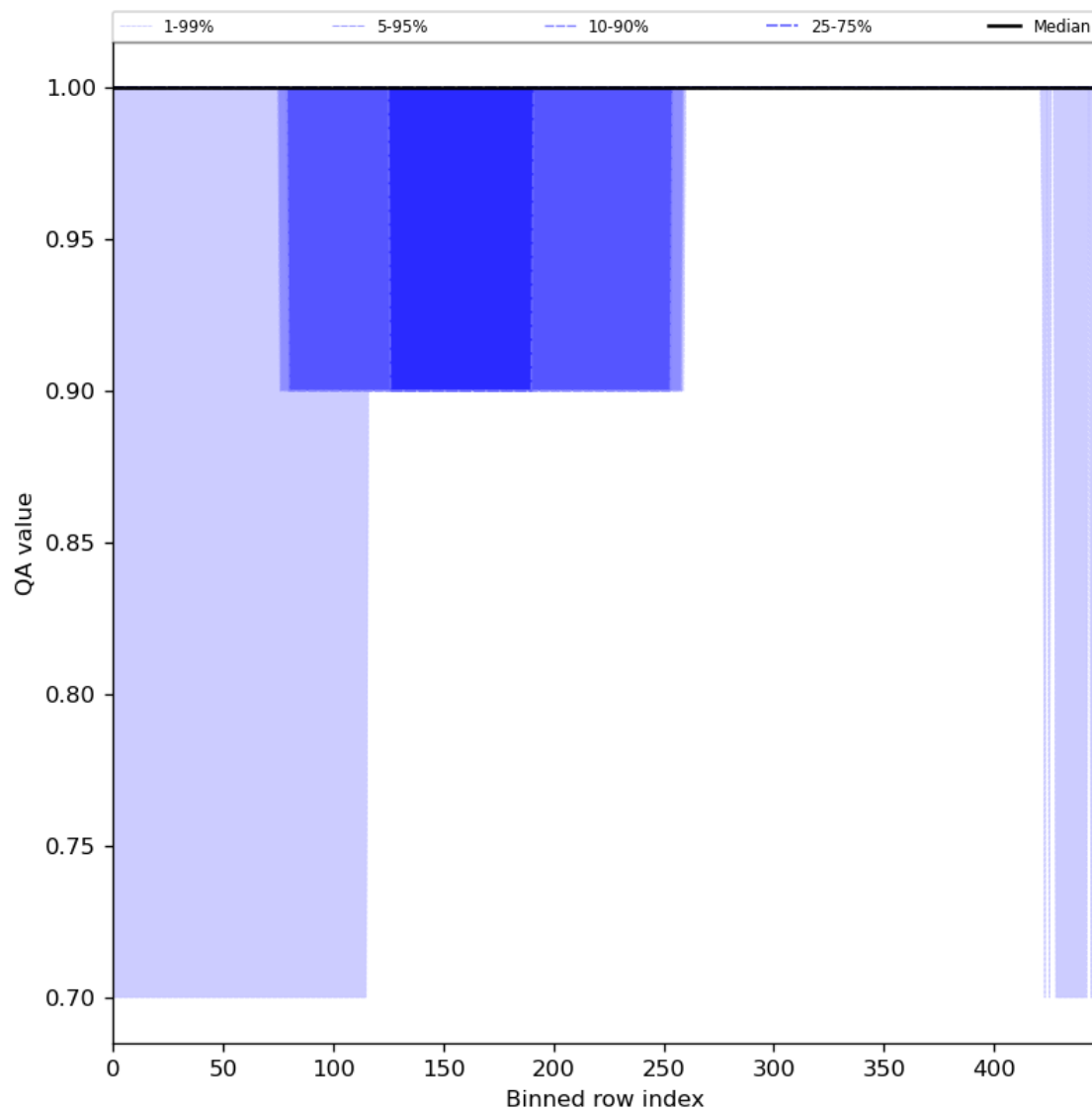
Figure 46: Along track statistics of “QA value” for 2024-08-16 to 2024-08-17
