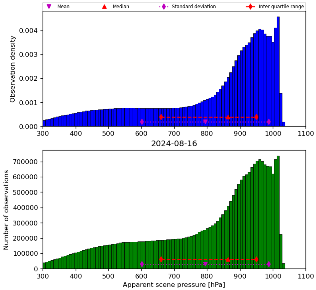
Figure 36: Histogram of “Apparent scene pressure” for 2024-08-16 to 2024-08-17
