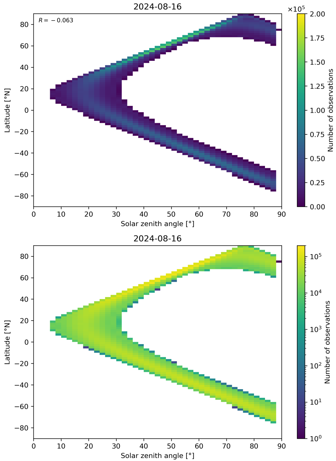
Figure 113: Scatter density plot of “Solar zenith angle” against “Latitude” for 2024-08-16 to 2024-08-17.
