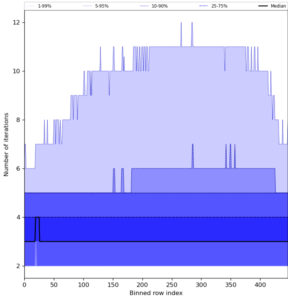
Figure 56: Along track statistics of “Number of iterations” for 2024-08-16 to 2024-08-17
