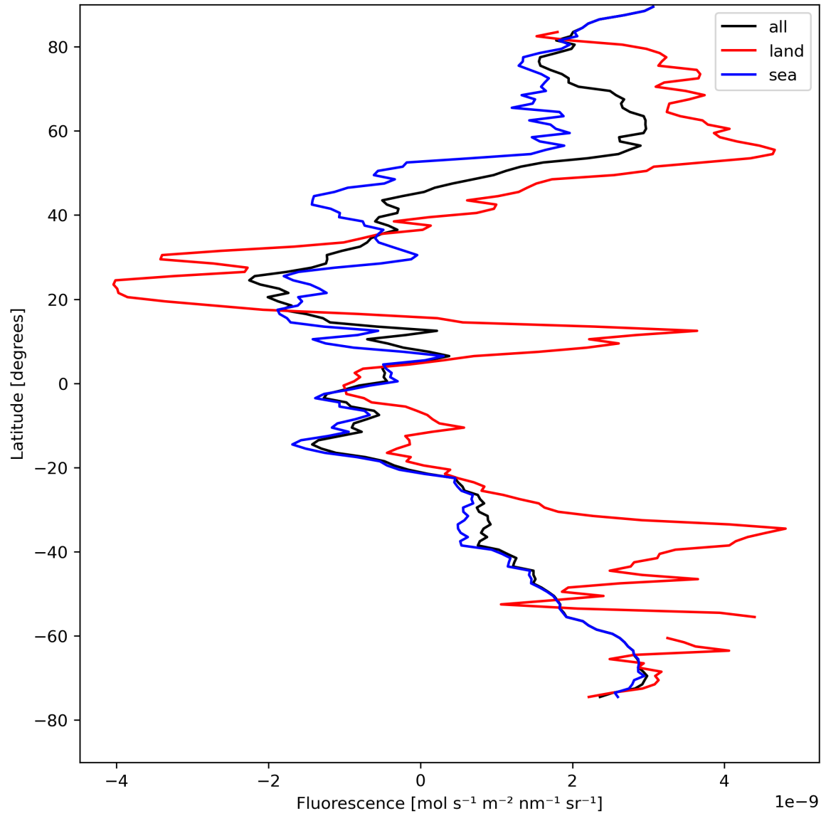
Figure 23: Zonal average of “Fluorescence” for 2024-08-16 to 2024-08-17.
