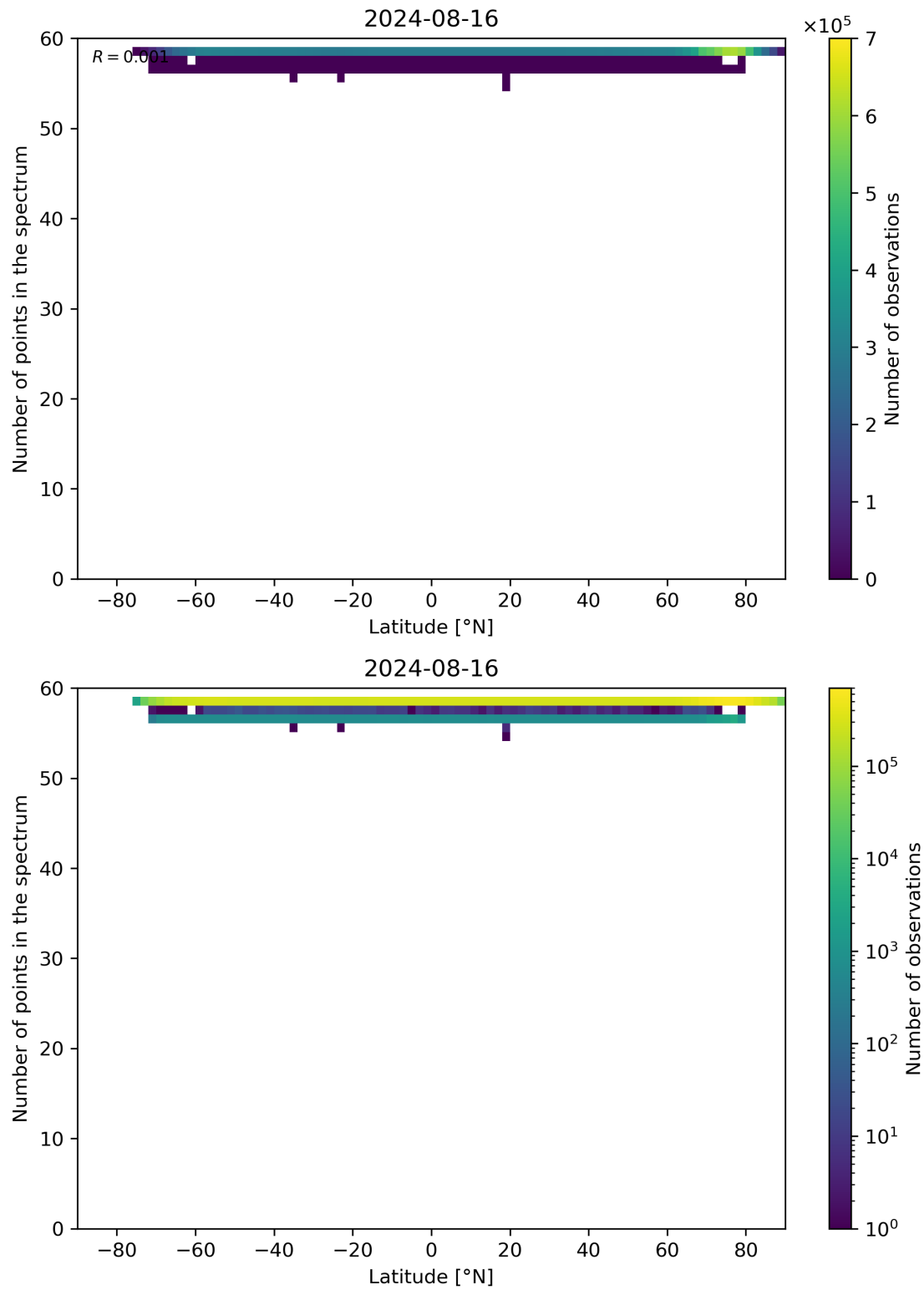
Figure 94: Scatter density plot of “Latitude” against “Number of points in the spectrum” for 2024-08-16 to 2024-08-17.
