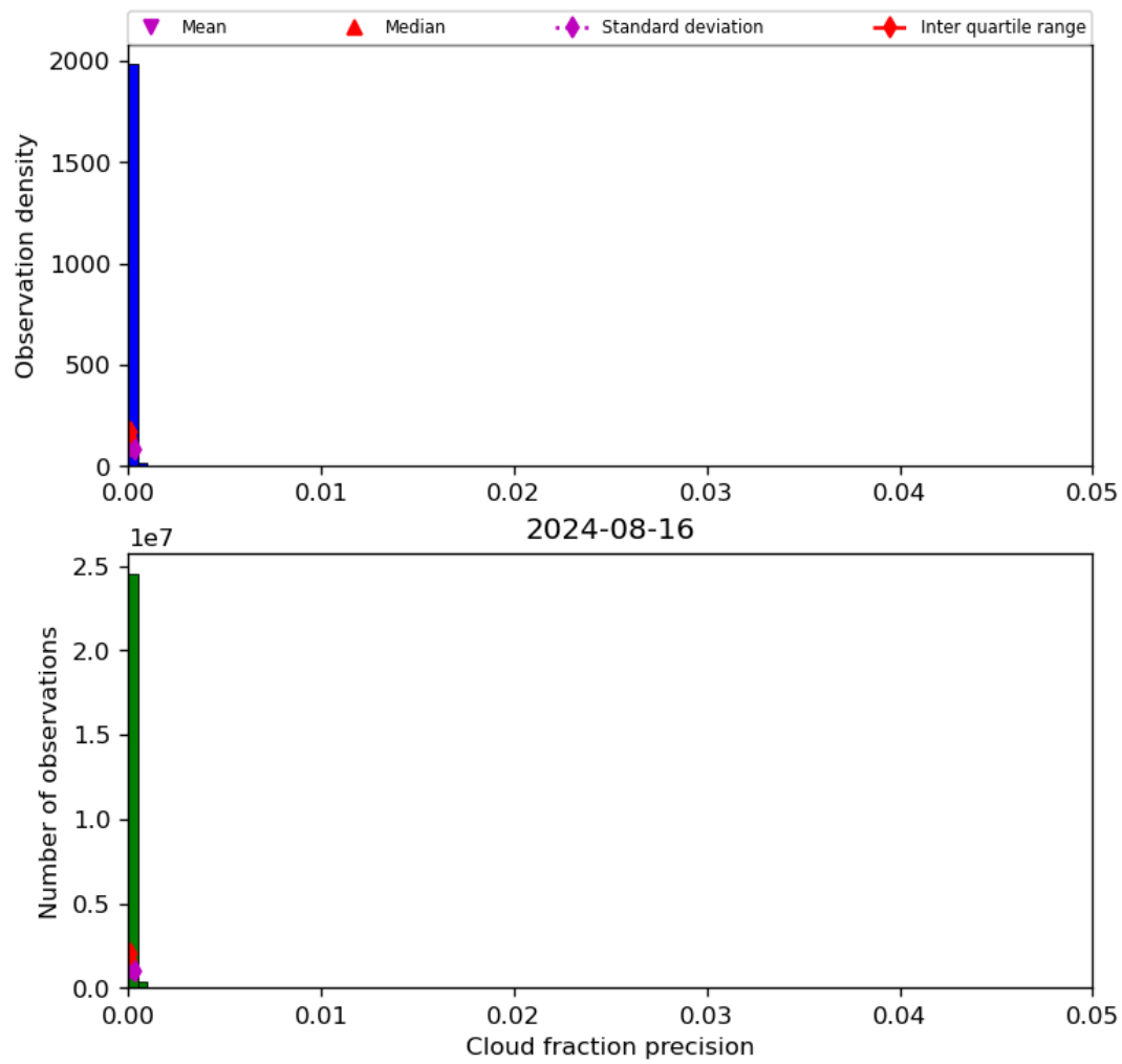
Figure 33: Histogram of “Cloud fraction precision” for 2024-08-16 to 2024-08-17
