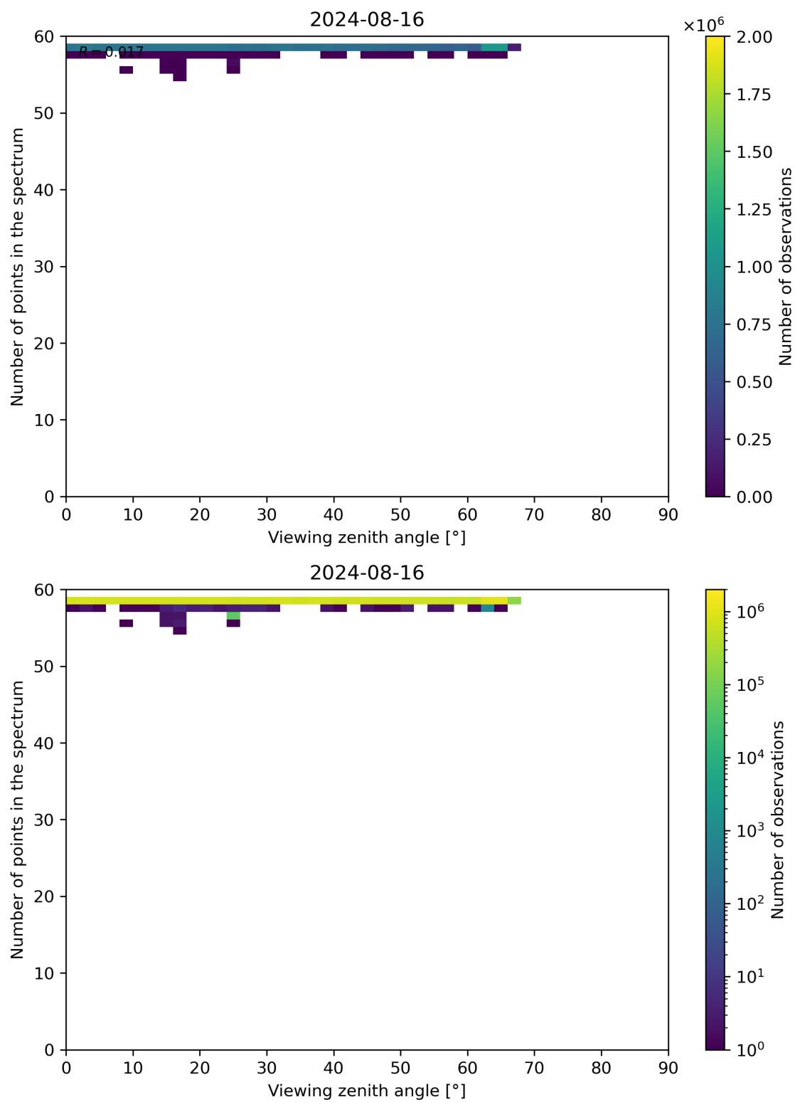
Figure 125: Scatter density plot of “Viewing zenith angle” against “Number of points in the spectrum” for 2024-08-16 to 2024-08-17.
