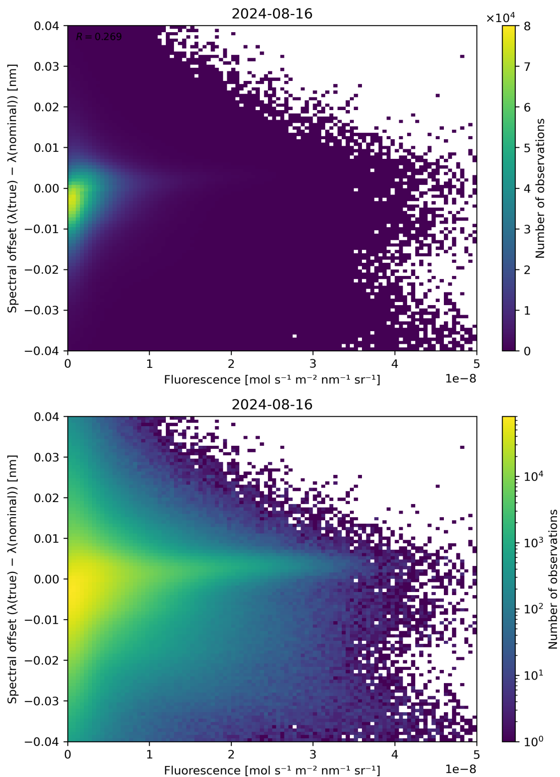
Figure 87: Scatter density plot of “Fluorescence” against “Spectral offset ( \lambda(\text{true}) - \lambda(\text{nominal}) )” for 2024-08-16 to 2024-08-17.
