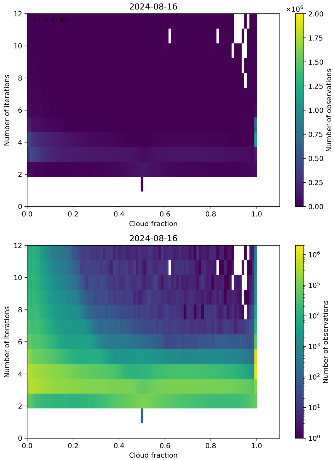
Figure 73: Scatter density plot of “Cloud fraction” against “Number of iterations” for 2024-08-16 to 2024-08-17.
