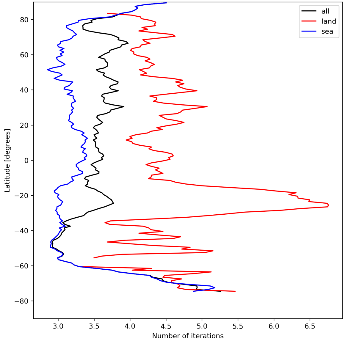
Figure 22: Zonal average of “Number of iterations” for 2024-08-16 to 2024-08-17.
