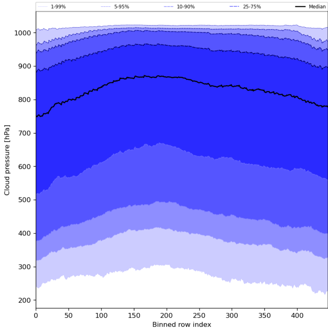
Figure 47: Along track statistics of “Cloud pressure” for 2024-08-16 to 2024-08-17
