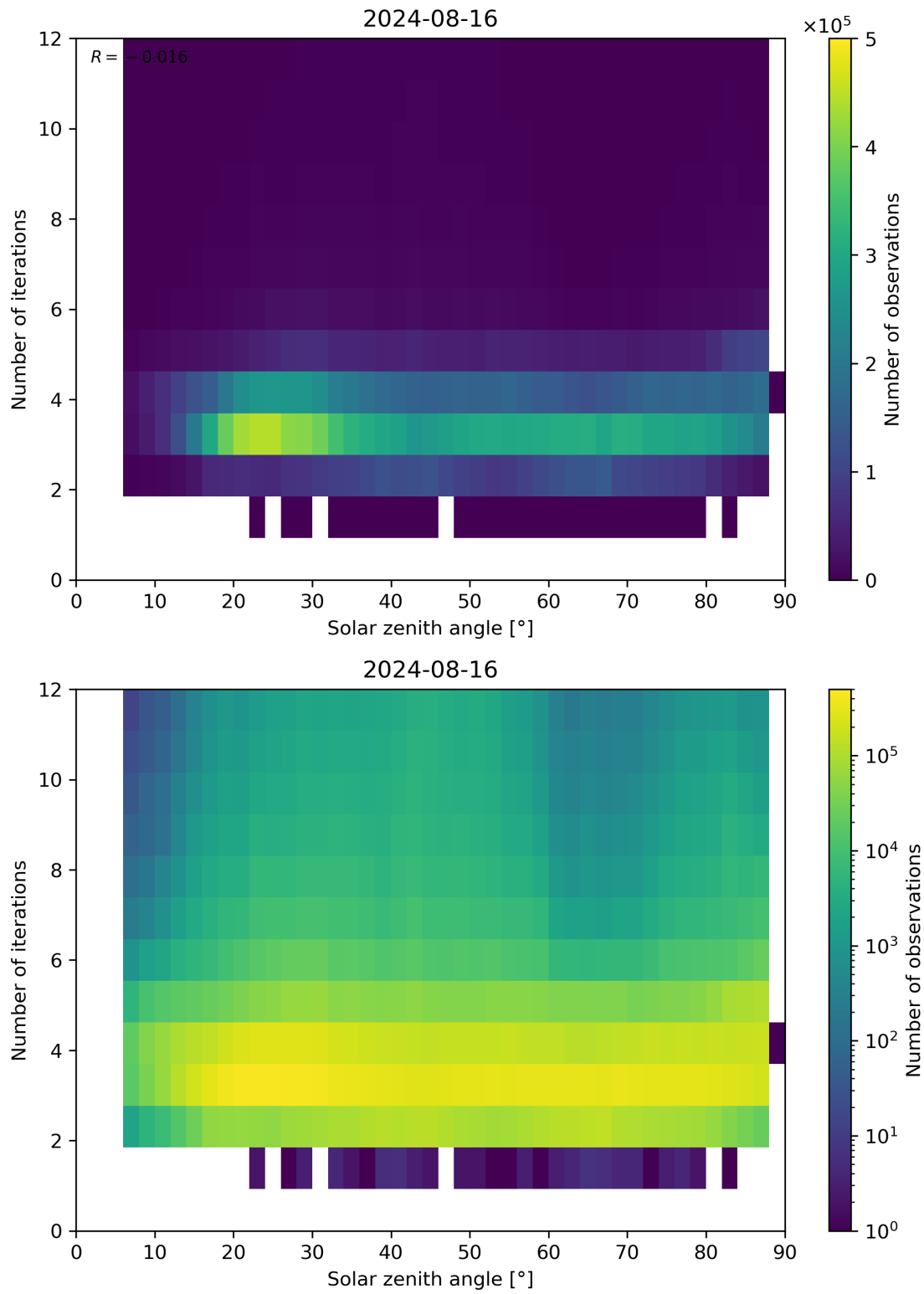
Figure 114: Scatter density plot of “Solar zenith angle” against “Number of iterations” for 2024-08-16 to 2024-08-17.
