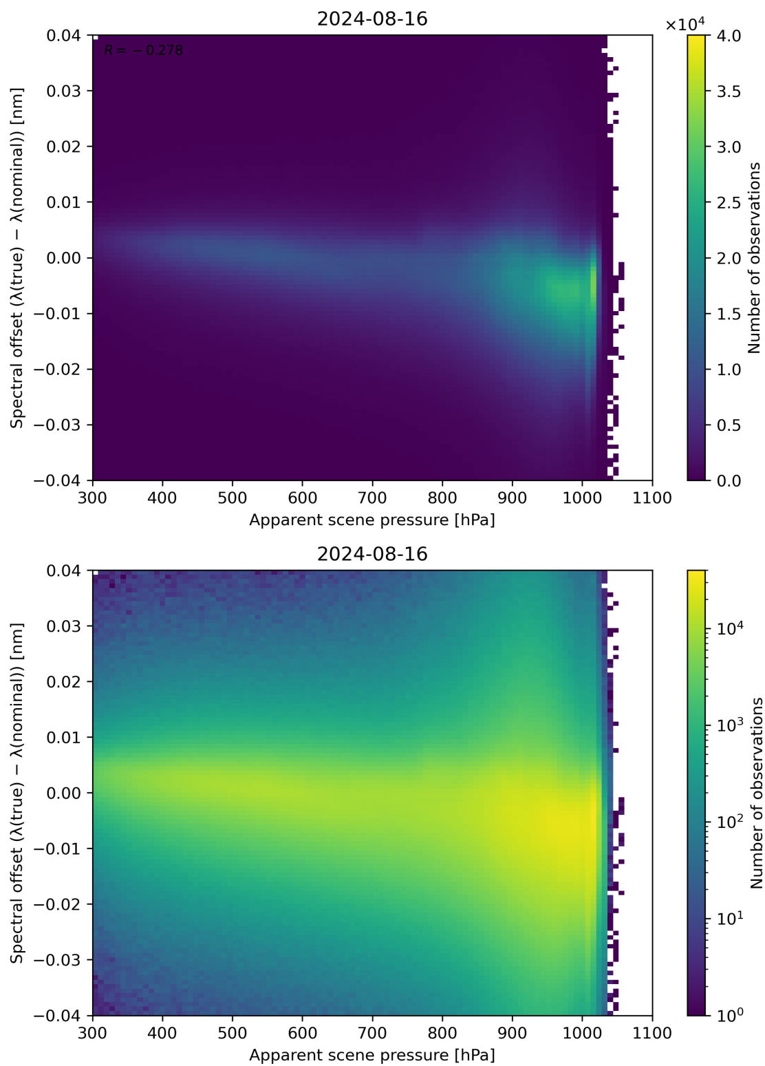
Figure 67: Scatter density plot of “Apparent scene pressure” against “Spectral offset ( \lambda(\text{true}) - \lambda(\text{nominal}) )” for 2024-08-16 to 2024-08-17.
