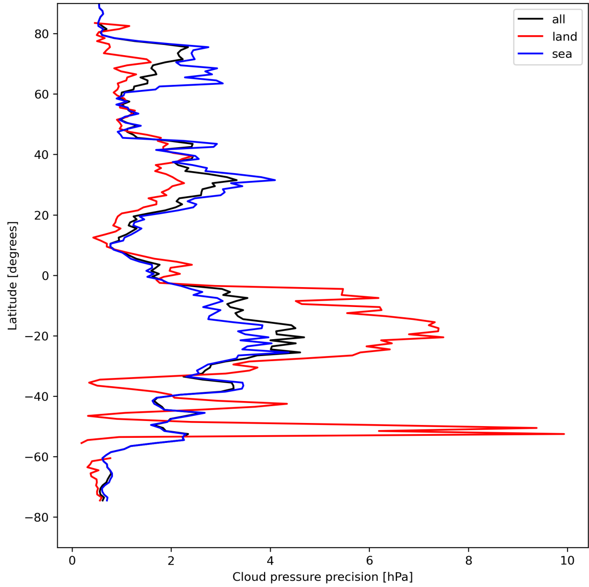
Figure 14: Zonal average of “Cloud pressure precision” for 2024-08-16 to 2024-08-17.
