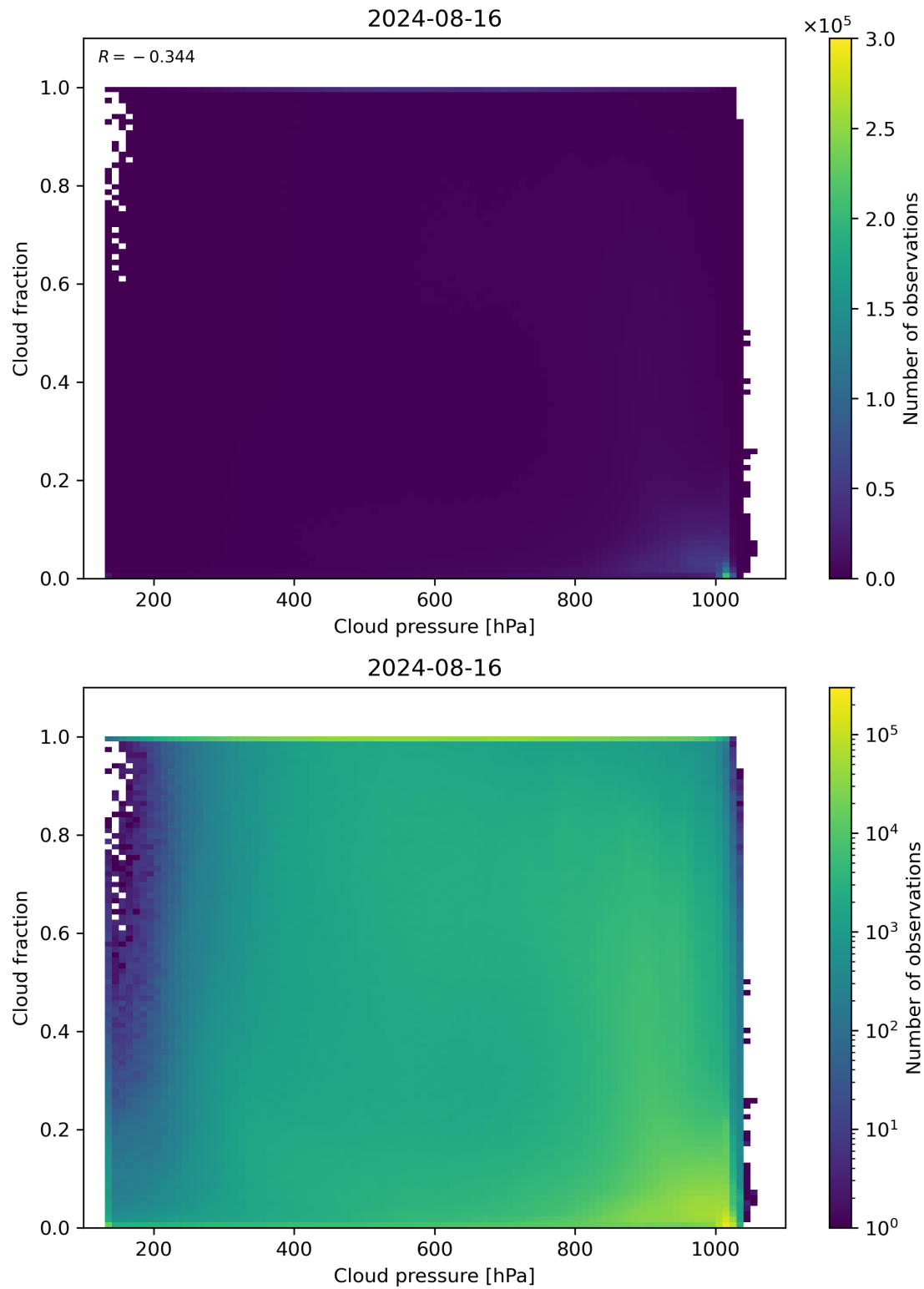
Figure 79: Scatter density plot of “Cloud pressure” against “Cloud fraction” for 2024-08-16 to 2024-08-17.
