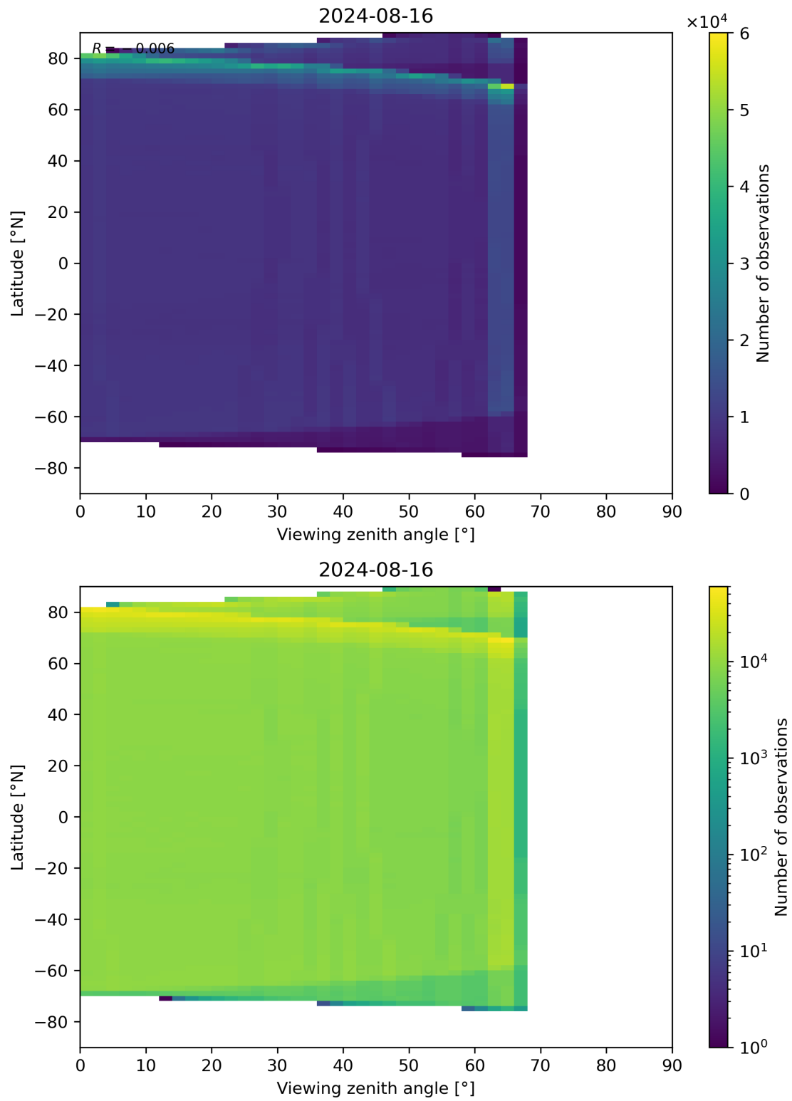
Figure 123: Scatter density plot of “Viewing zenith angle” against “Latitude” for 2024-08-16 to 2024-08-17.
