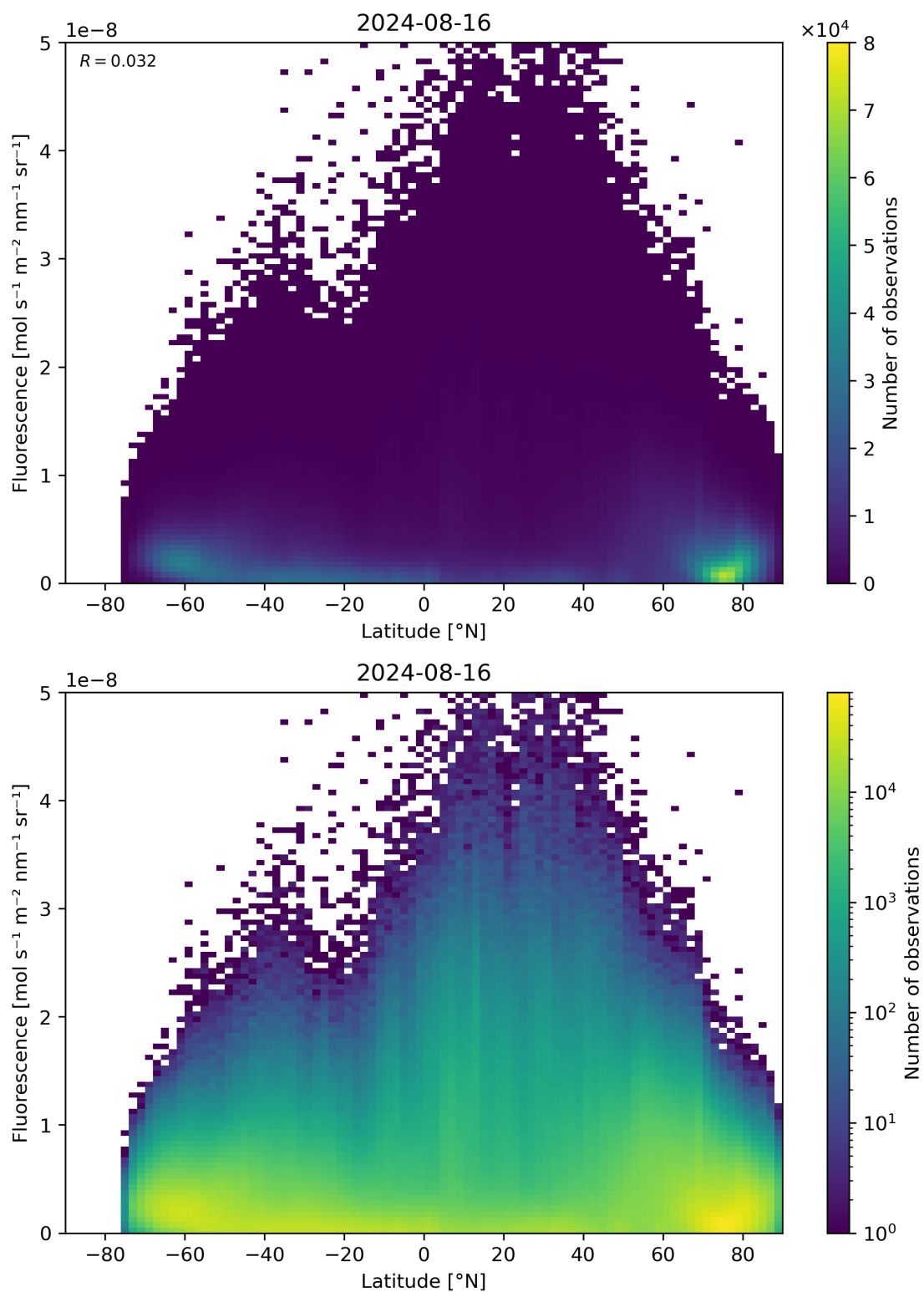
Figure 92: Scatter density plot of “Latitude” against “Fluorescence” for 2024-08-16 to 2024-08-17.
