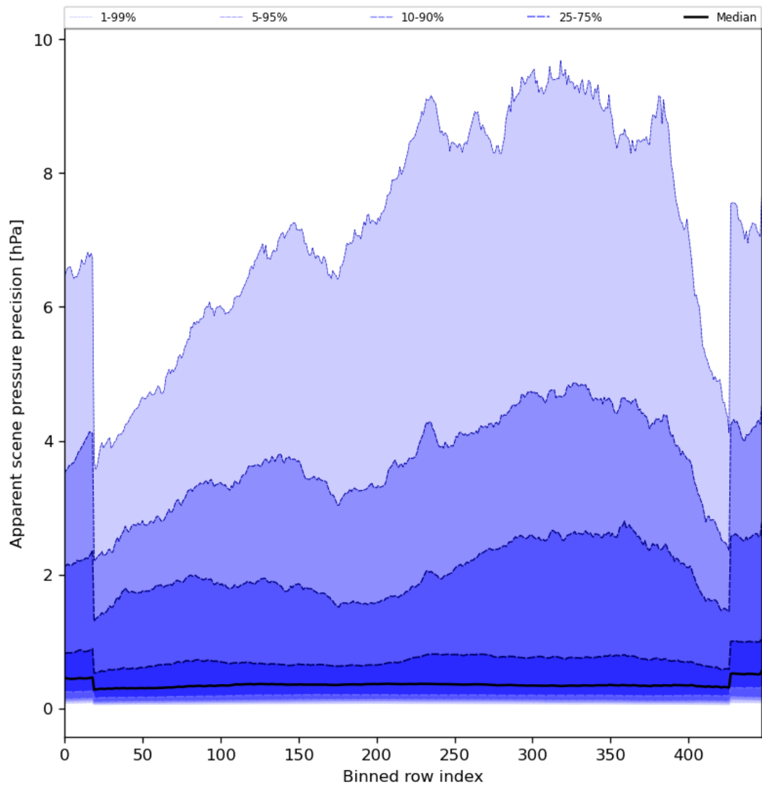
Figure 54: Along track statistics of “Apparent scene pressure precision” for 2024-08-16 to 2024-08-17
