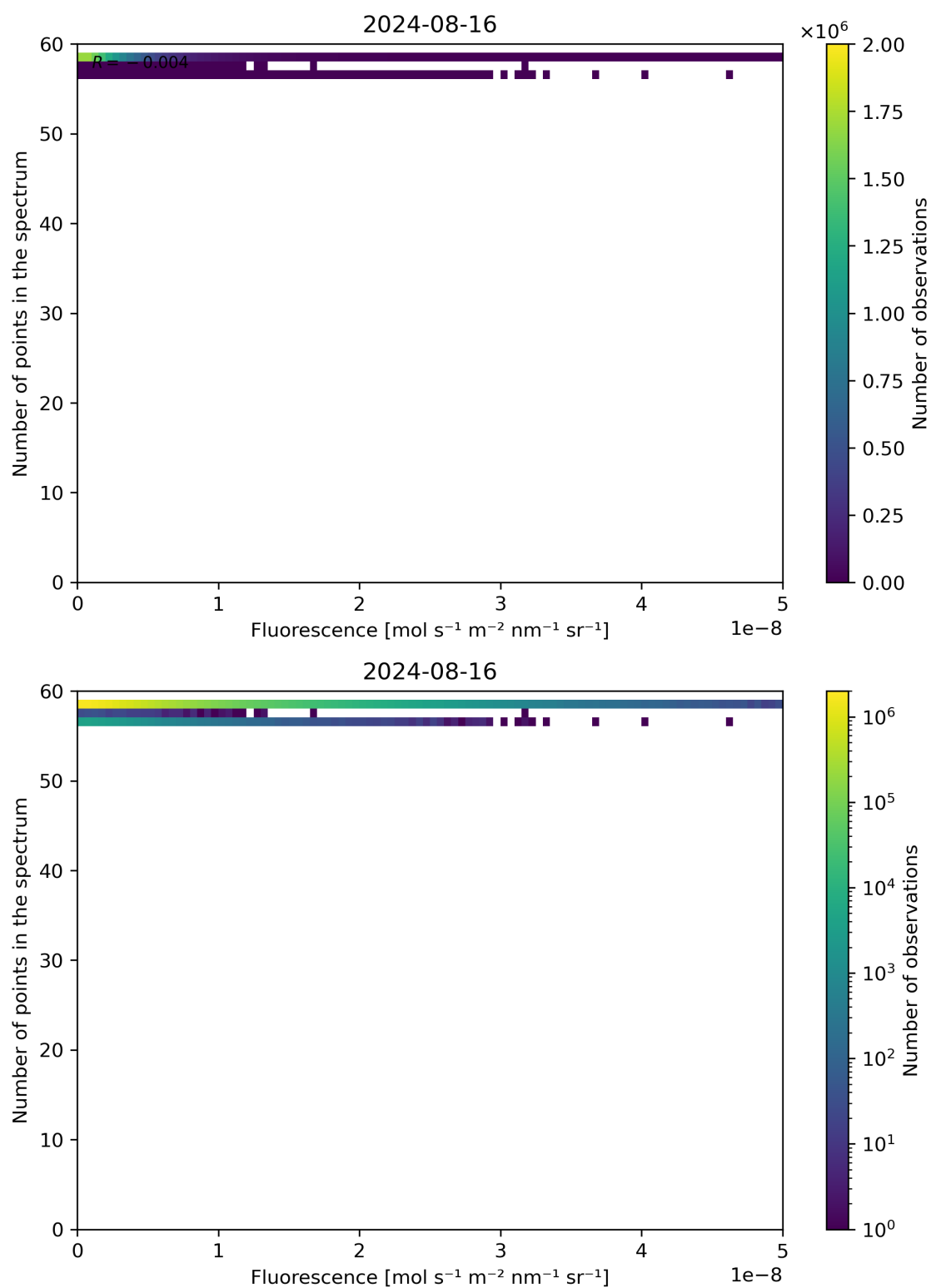
Figure 86: Scatter density plot of “Fluorescence” against “Number of points in the spectrum” for 2024-08-16 to 2024-08-17.
