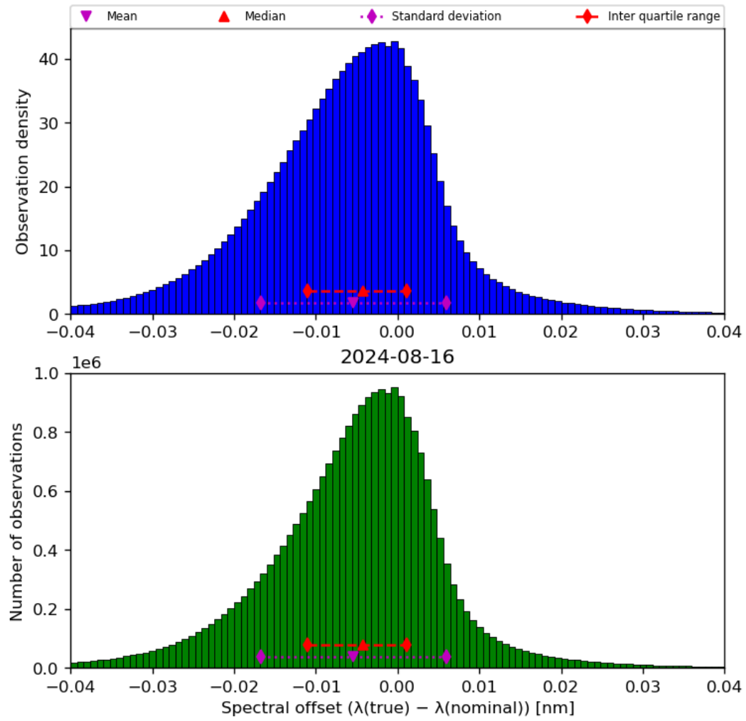
Figure 45: Histogram of “Spectral offset ( \lambda(\text{true}) - \lambda(\text{nominal}) )” for 2024-08-16 to 2024-08-17
