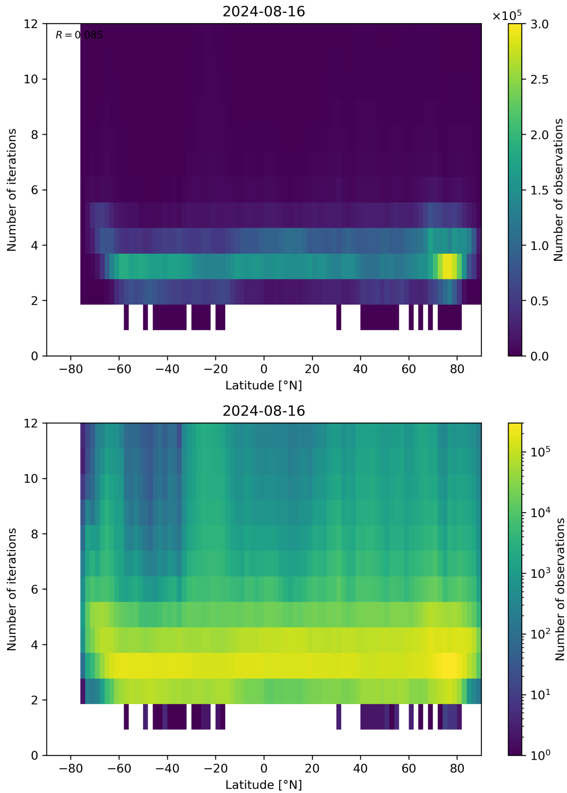
Figure 93: Scatter density plot of “Latitude” against “Number of iterations” for 2024-08-16 to 2024-08-17.
