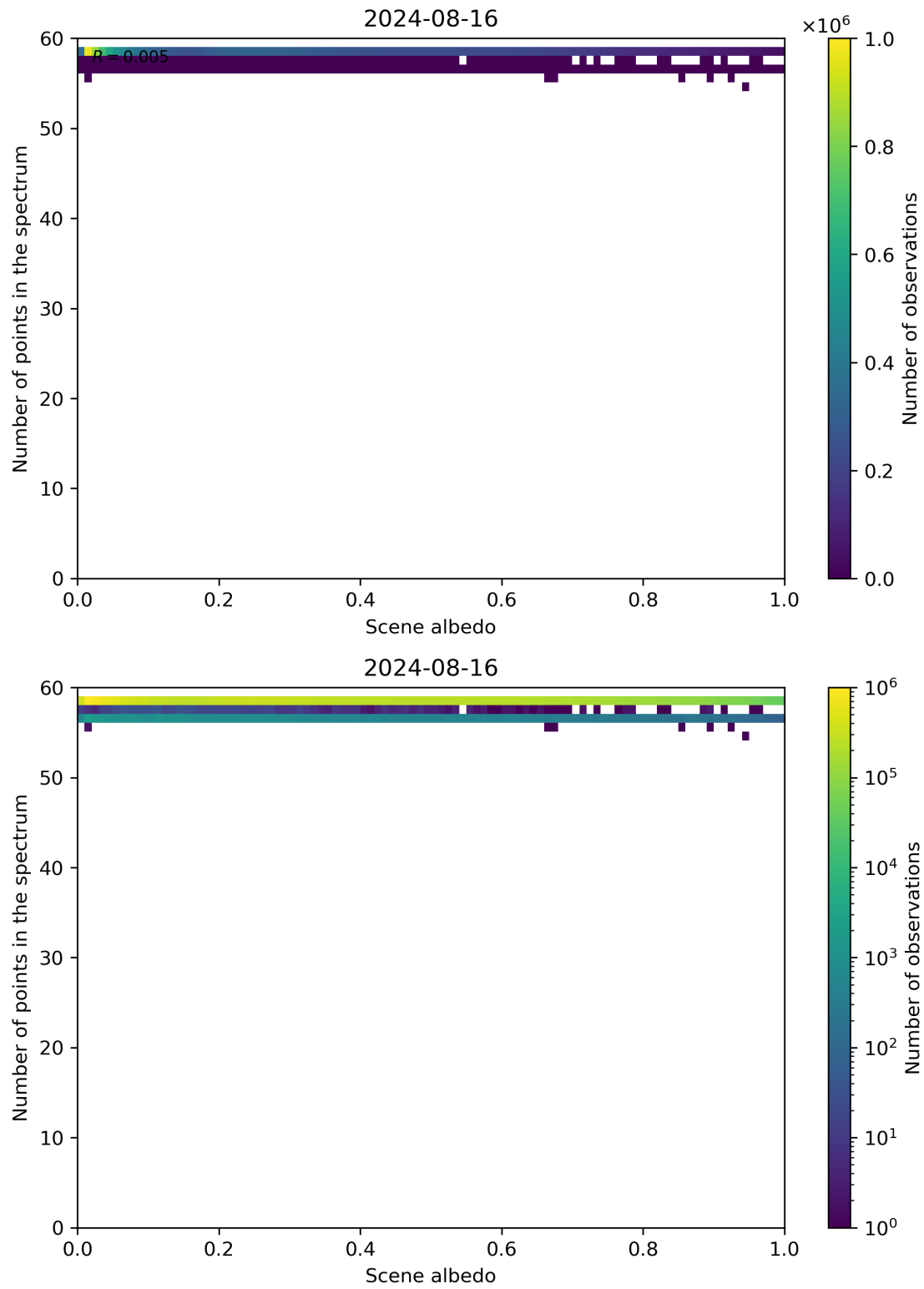
Figure 106: Scatter density plot of “Scene albedo” against “Number of points in the spectrum” for 2024-08-16 to 2024-08-17.
