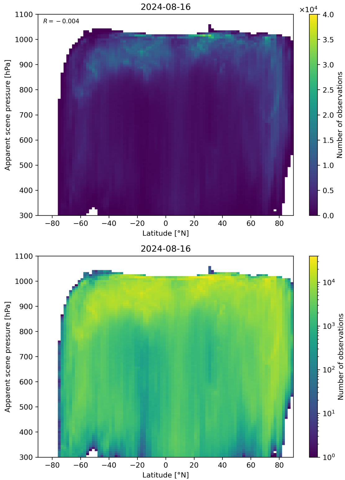
Figure 88: Scatter density plot of “Latitude” against “Apparent scene pressure” for 2024-08-16 to 2024-08-17.
