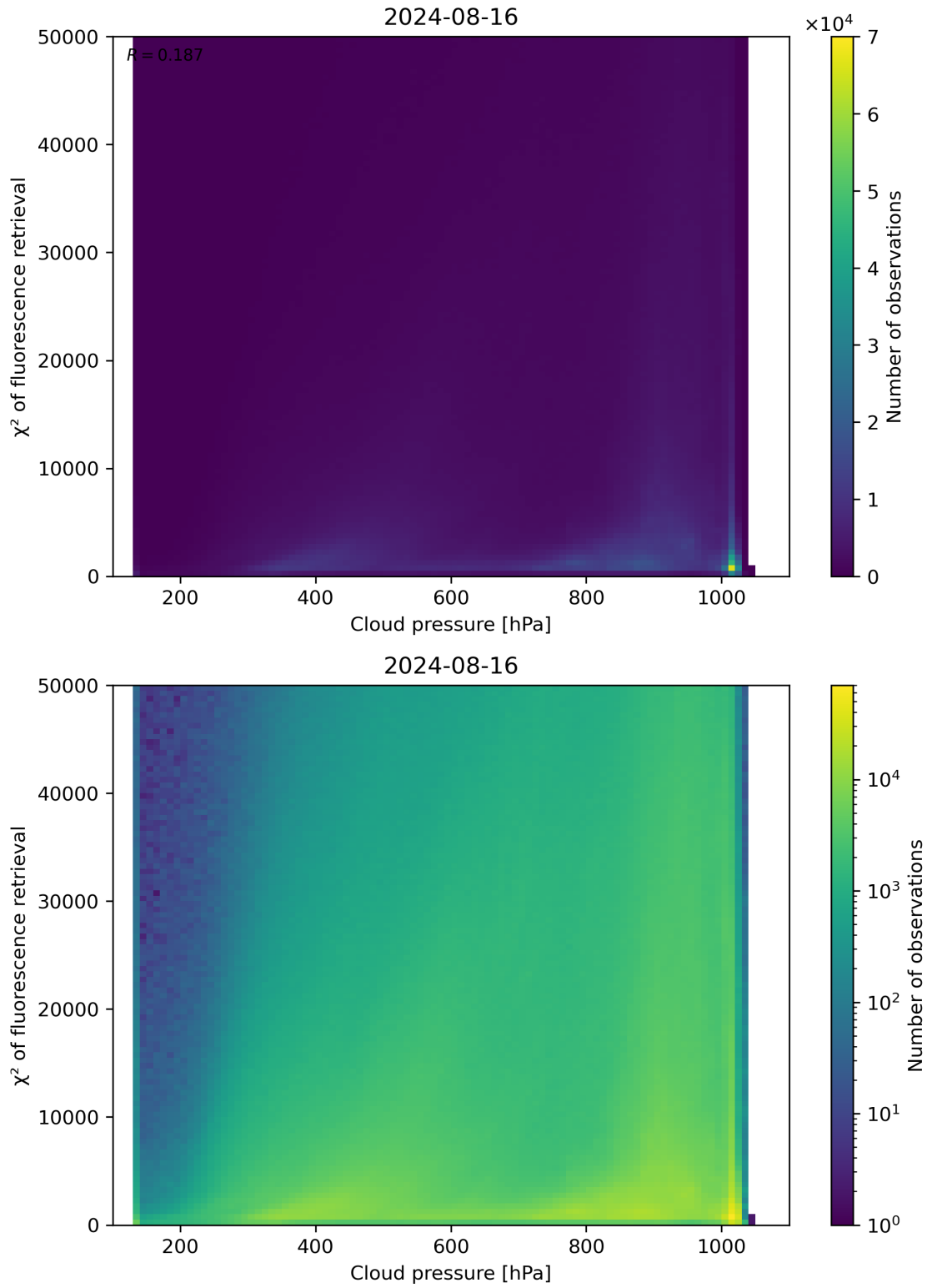
Figure 78: Scatter density plot of “Cloud pressure” against “ \chi^2 of fluorescence retrieval” for 2024-08-16 to 2024-08-17.
