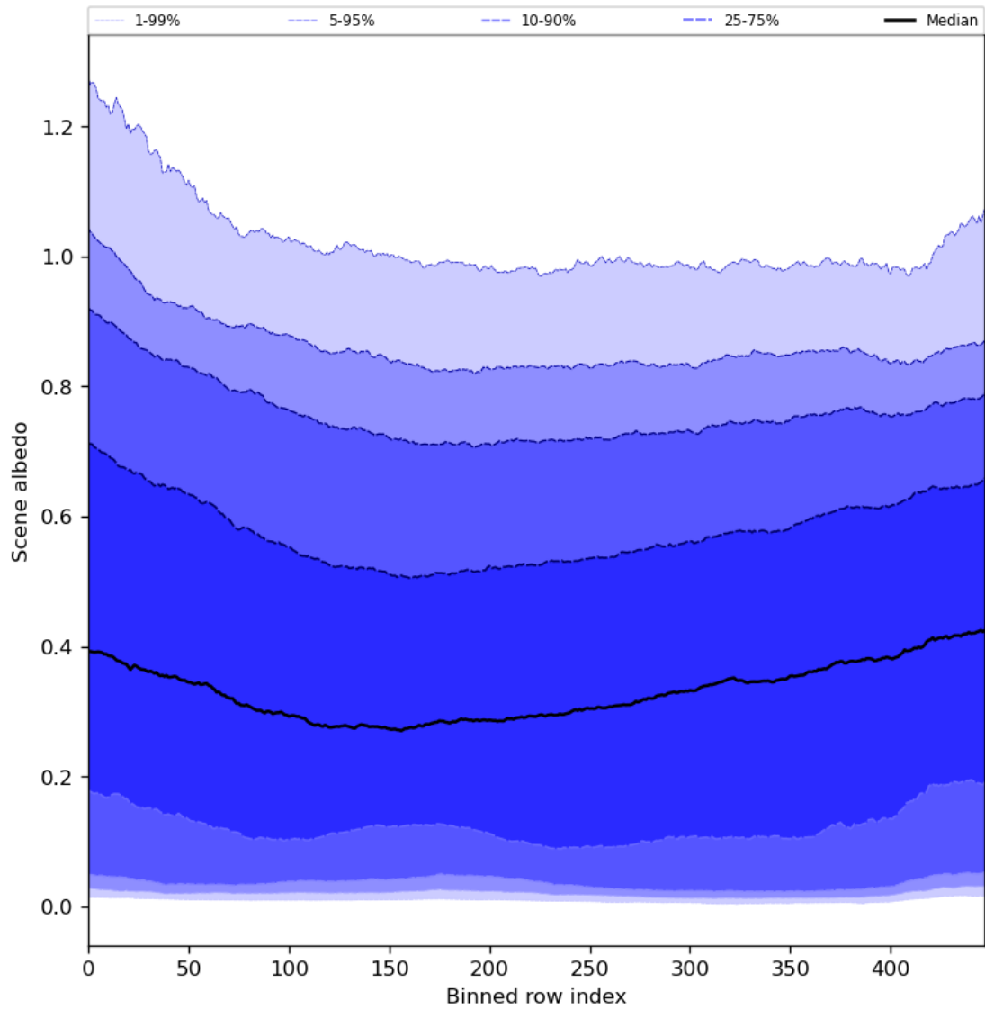
Figure 51: Along track statistics of “Scene albedo” for 2024-08-16 to 2024-08-17
