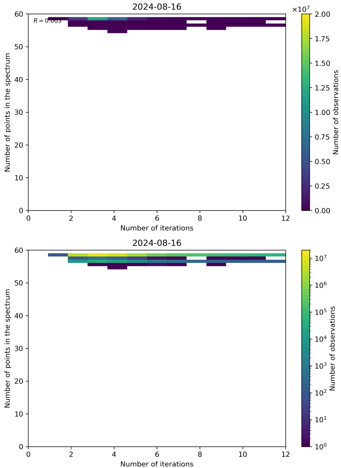
Figure 99: Scatter density plot of “Number of iterations” against “Number of points in the spectrum” for 2024-08-16 to 2024-08-17.
