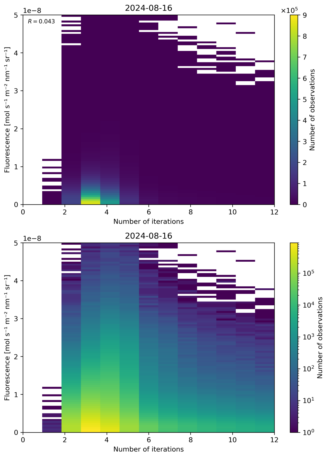
Figure 98: Scatter density plot of “Number of iterations” against “Fluorescence” for 2024-08-16 to 2024-08-17.
