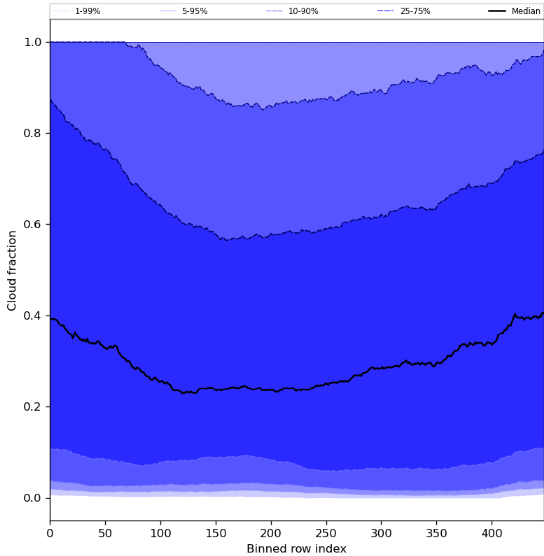
Figure 49: Along track statistics of “Cloud fraction” for 2024-08-16 to 2024-08-17
