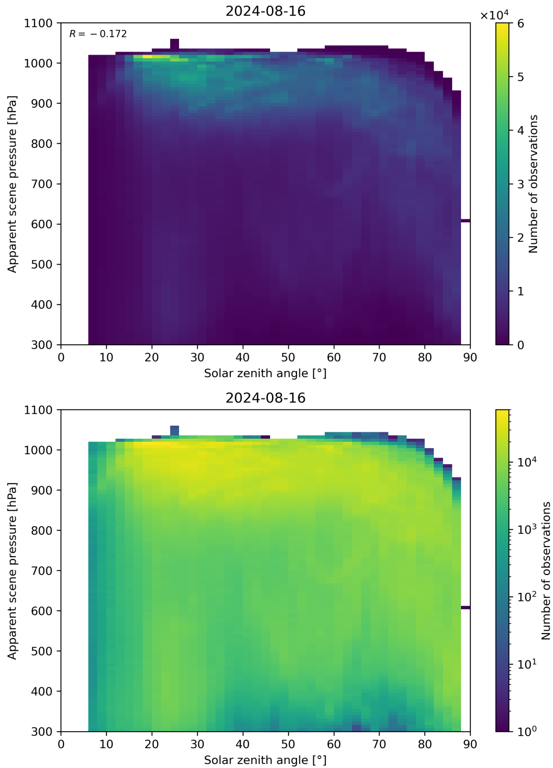
Figure 108: Scatter density plot of “Solar zenith angle” against “Apparent scene pressure” for 2024-08-16 to 2024-08-17.
