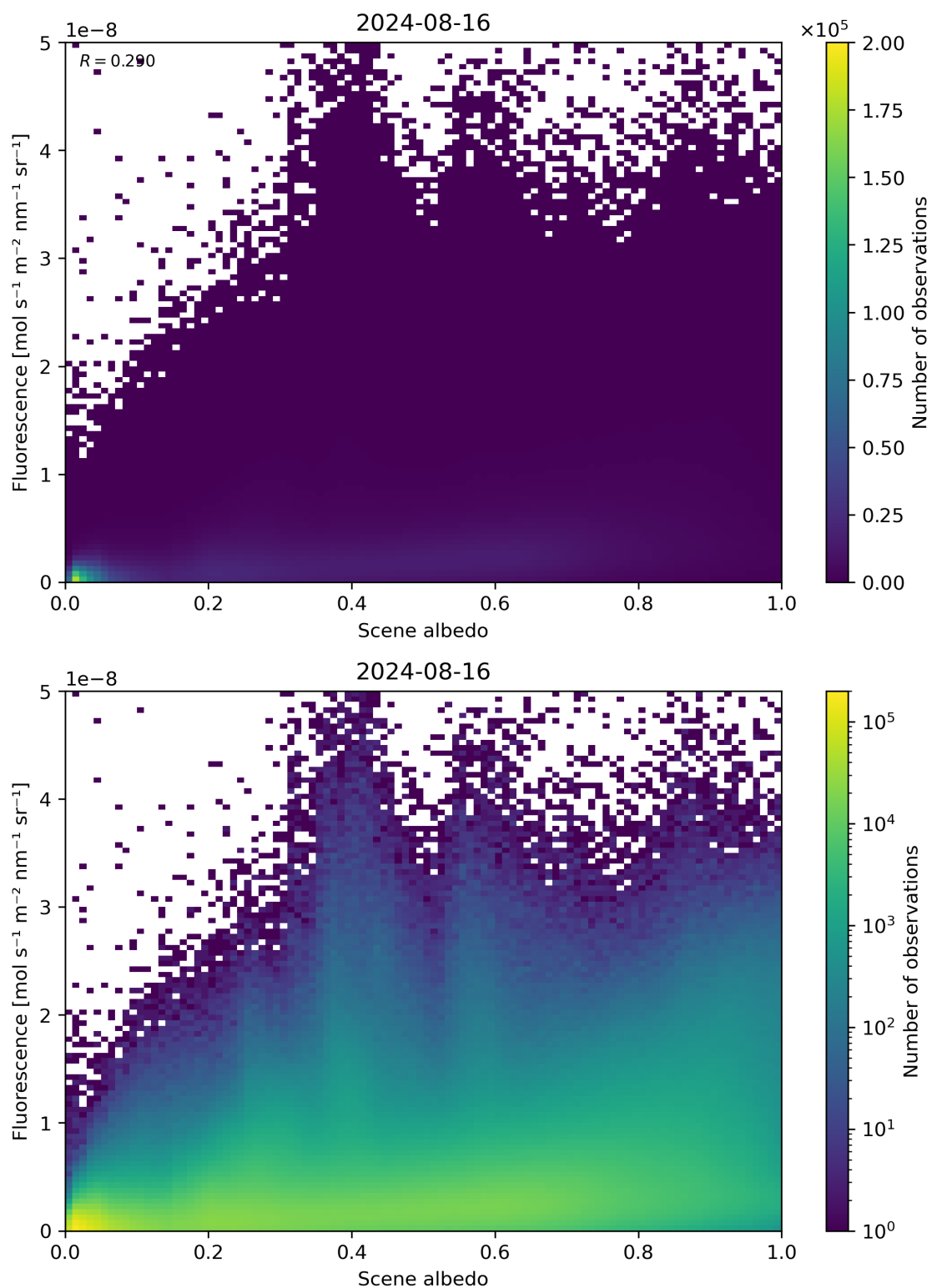
Figure 104: Scatter density plot of “Scene albedo” against “Fluorescence” for 2024-08-16 to 2024-08-17.
