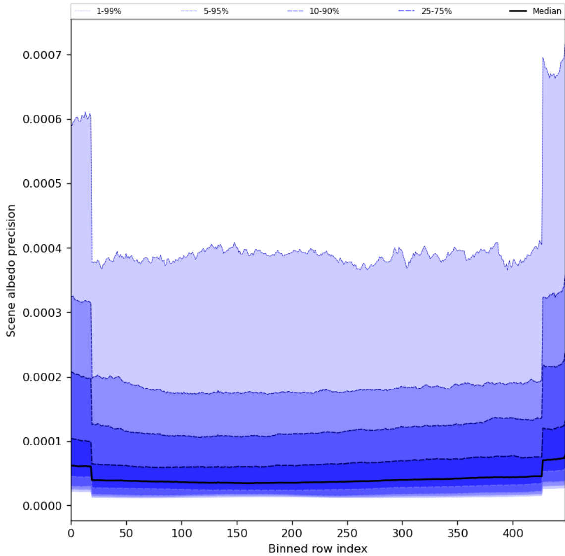
Figure 52: Along track statistics of “Scene albedo precision” for 2024-08-16 to 2024-08-17
