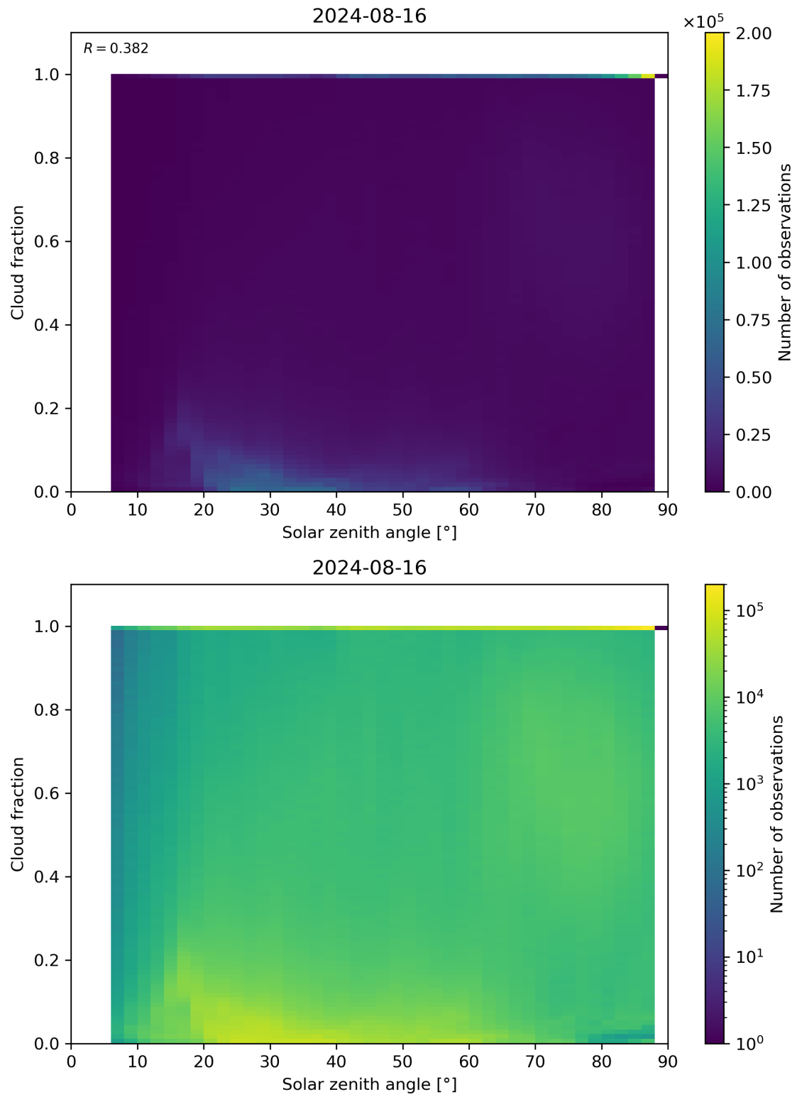
Figure 110: Scatter density plot of “Solar zenith angle” against “Cloud fraction” for 2024-08-16 to 2024-08-17.
