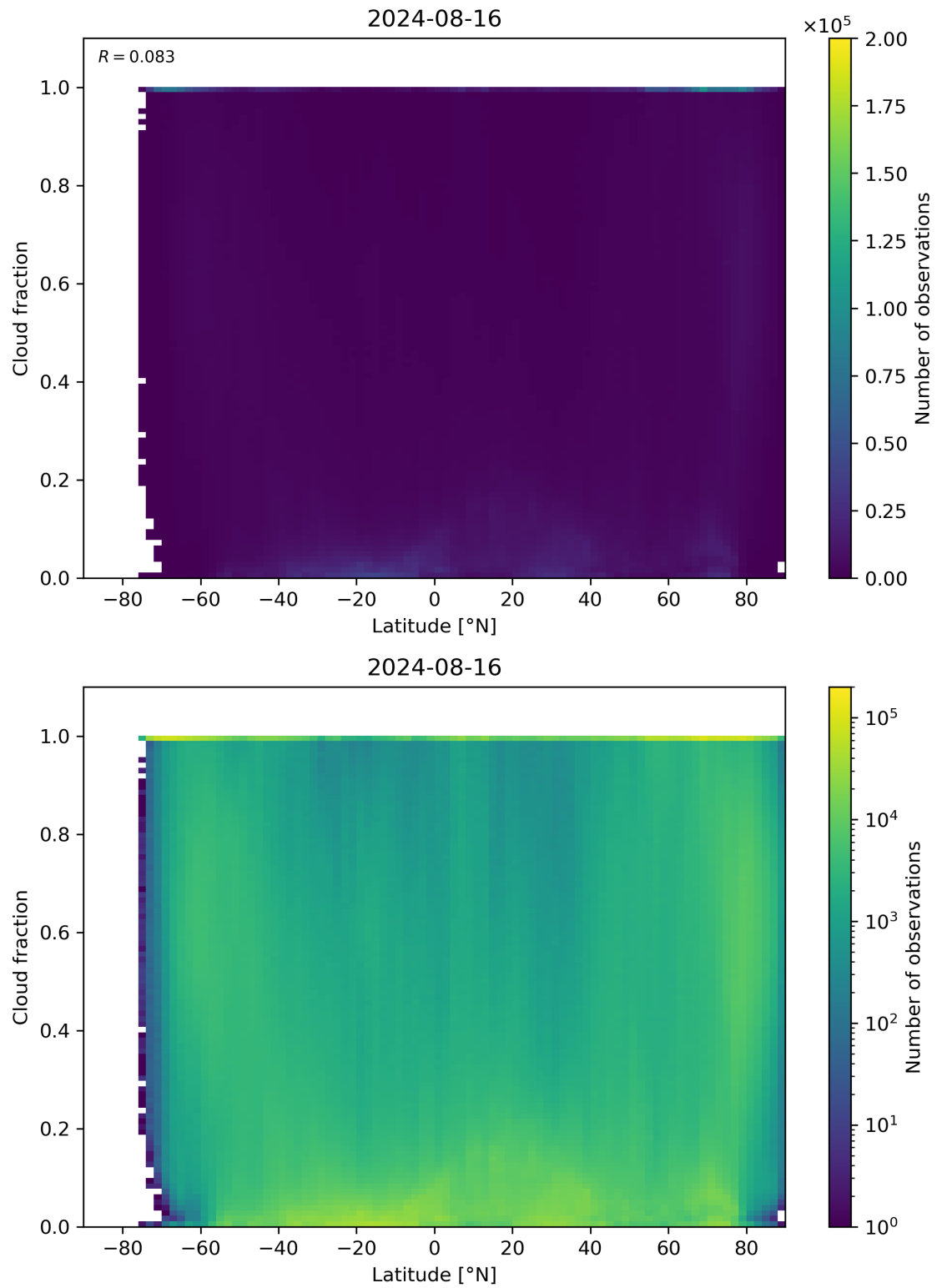
Figure 90: Scatter density plot of “Latitude” against “Cloud fraction” for 2024-08-16 to 2024-08-17.
