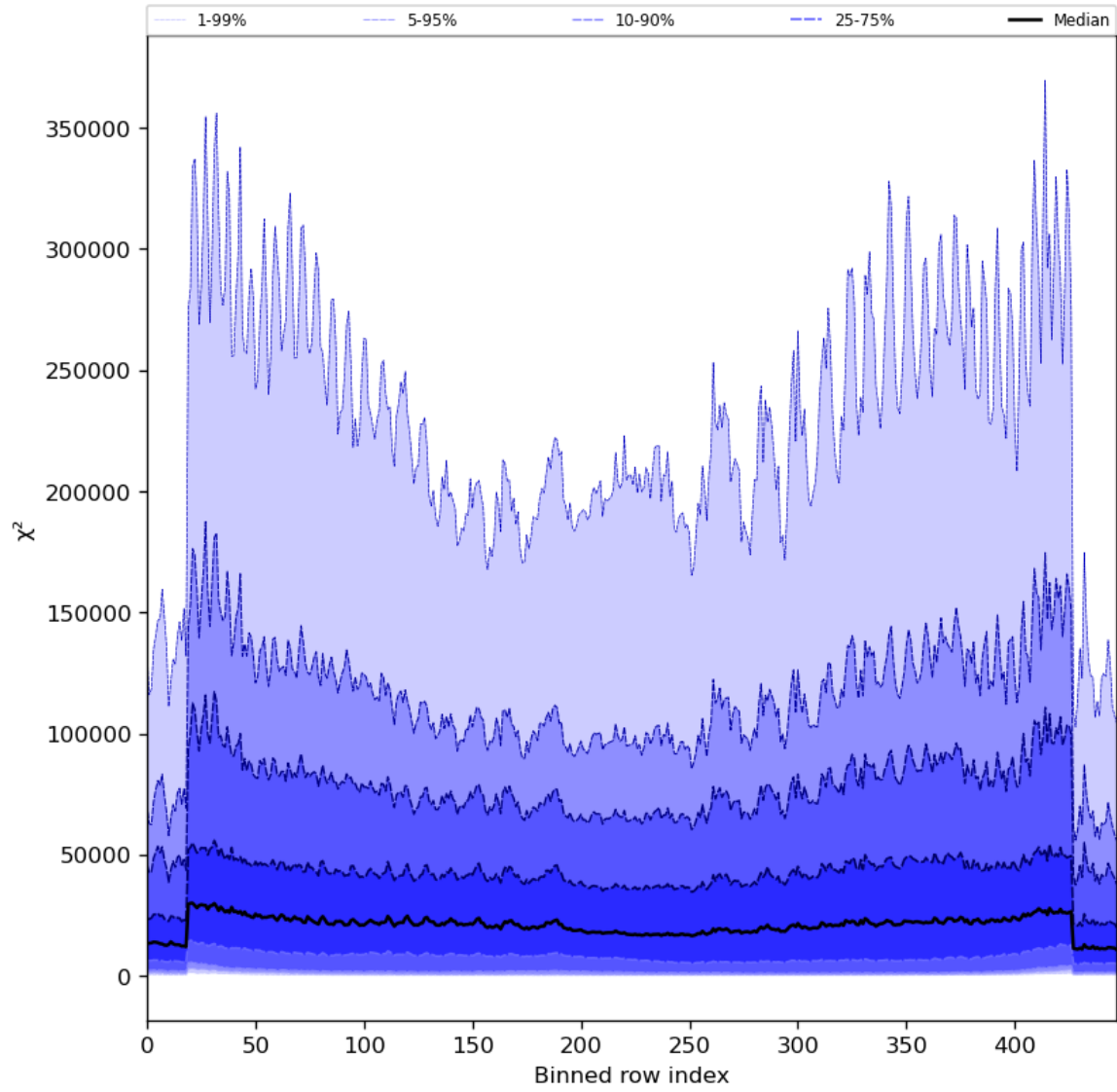
Figure 55: Along track statistics of “ \chi^2 ” for 2024-08-16 to 2024-08-17
