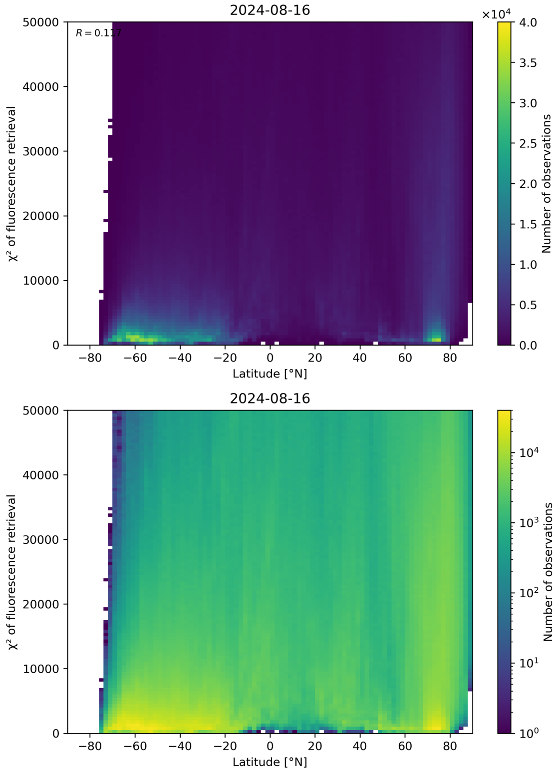
Figure 89: Scatter density plot of “Latitude” against “ \chi^2 of fluorescence retrieval” for 2024-08-16 to 2024-08-17.
