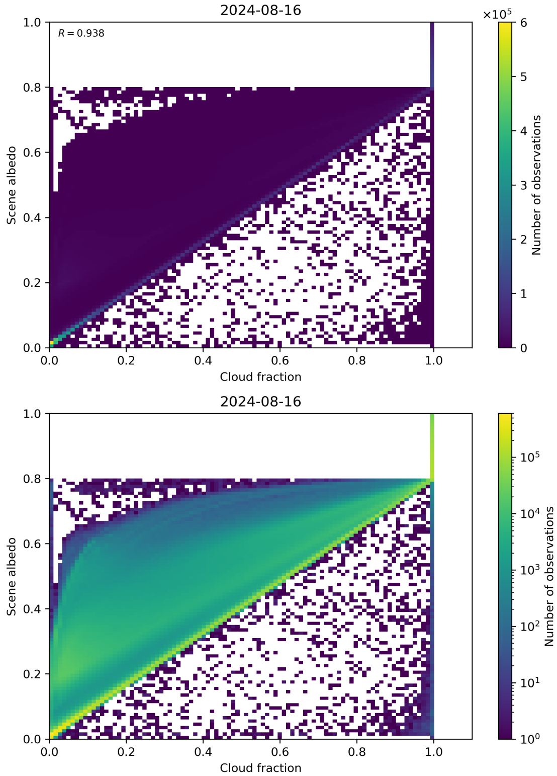
Figure 75: Scatter density plot of “Cloud fraction” against “Scene albedo” for 2024-08-16 to 2024-08-17.
