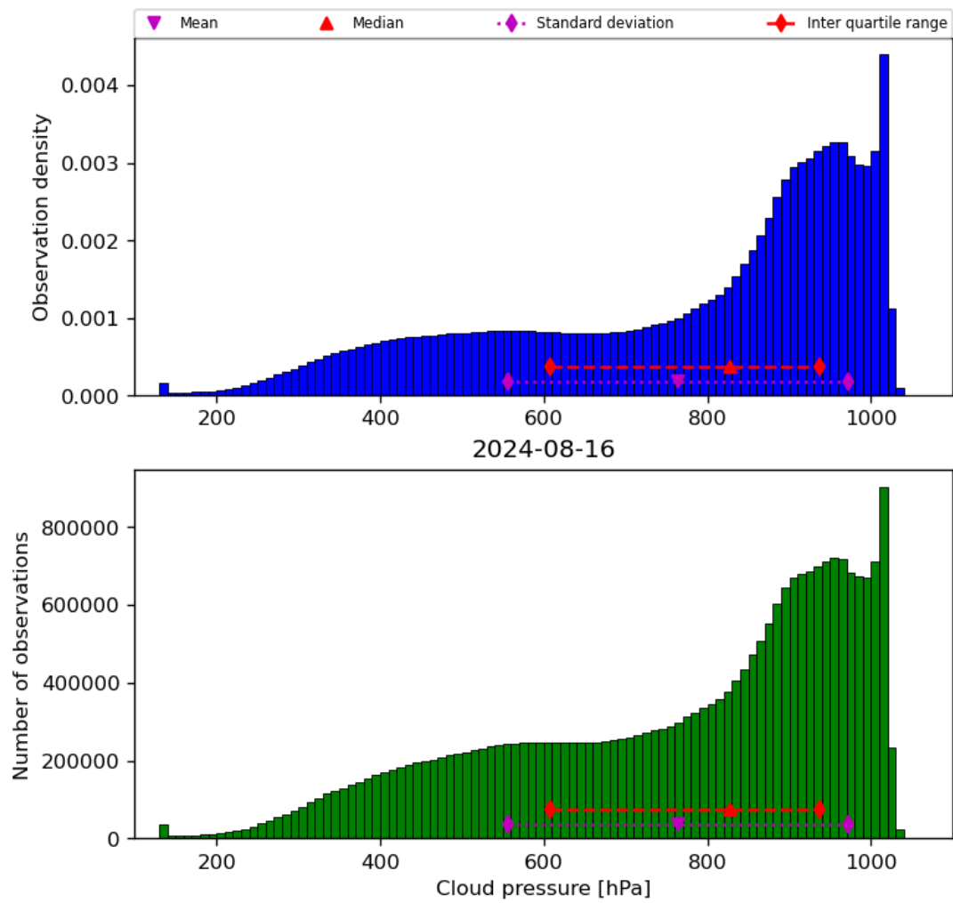
Figure 30: Histogram of “Cloud pressure” for 2024-08-16 to 2024-08-17
