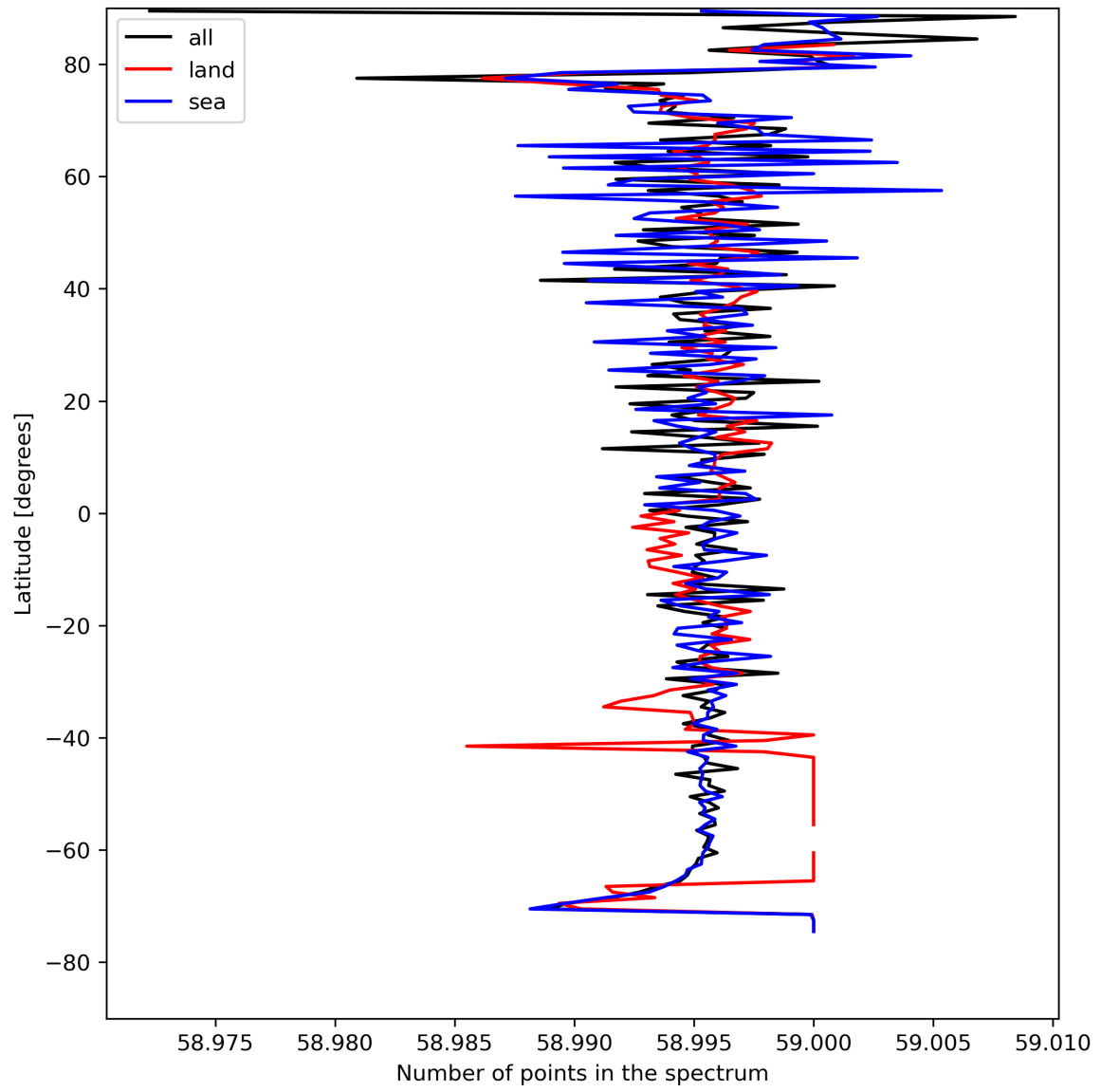
Figure 27: Zonal average of “Number of points in the spectrum” for 2024-08-16 to 2024-08-17.
