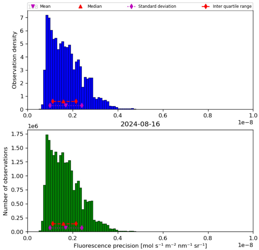
Figure 41: Histogram of “Fluorescence precision” for 2024-08-16 to 2024-08-17
