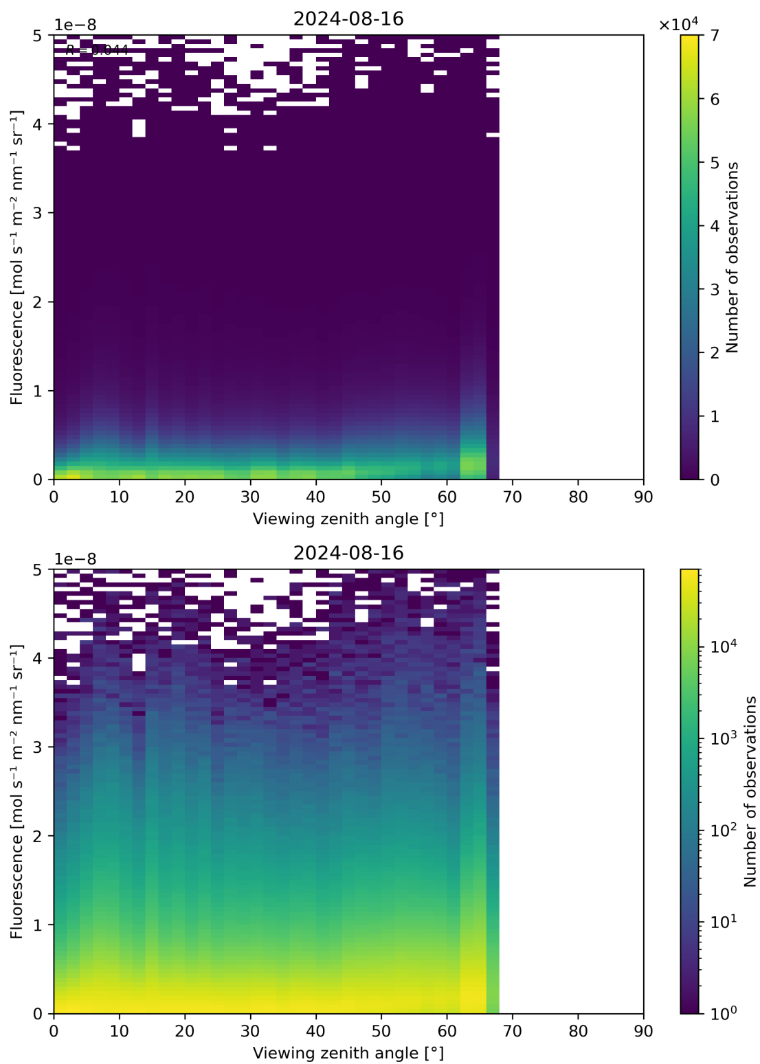
Figure 122: Scatter density plot of “Viewing zenith angle” against “Fluorescence” for 2024-08-16 to 2024-08-17.
