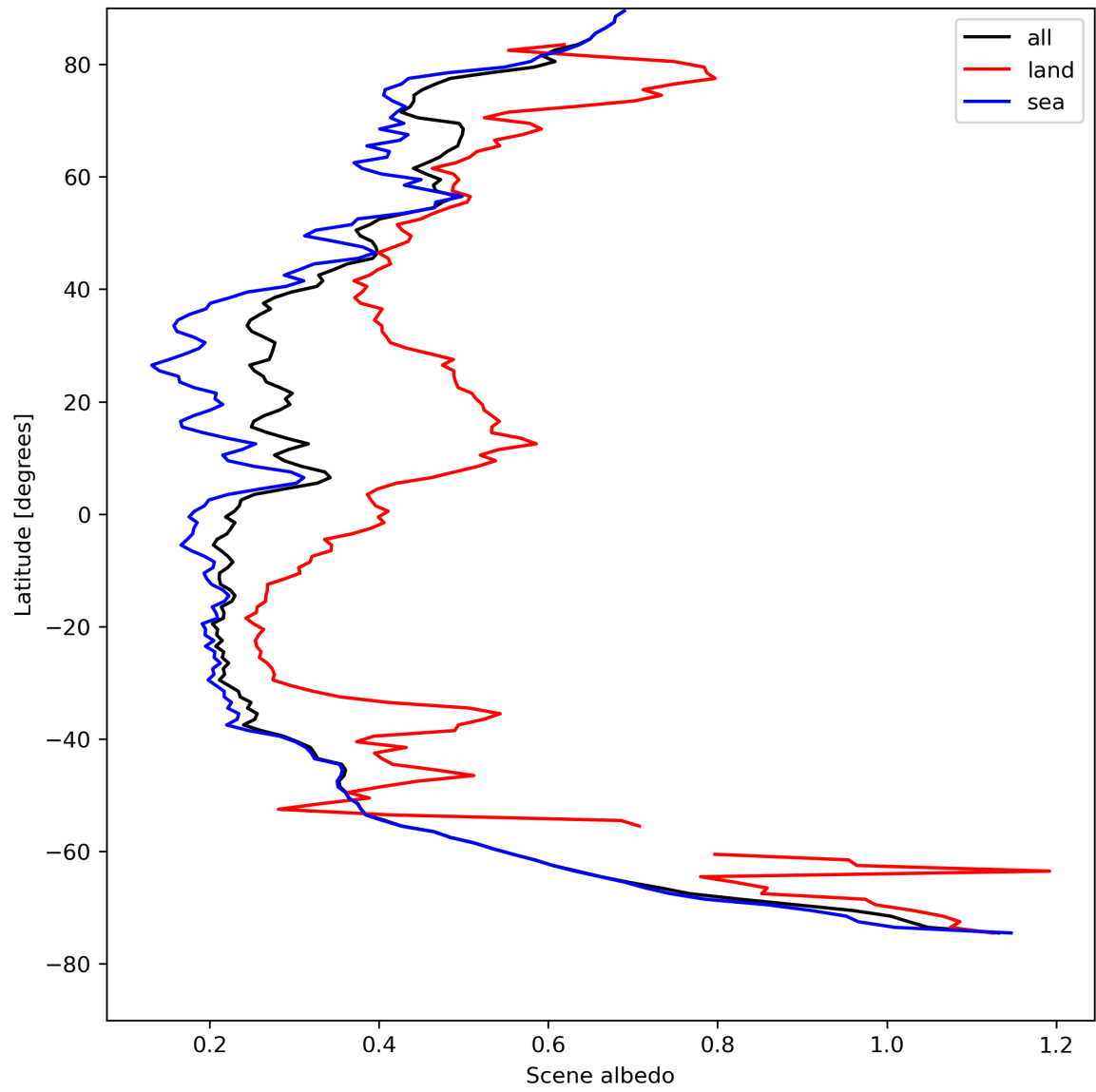
Figure 17: Zonal average of “Scene albedo” for 2024-08-16 to 2024-08-17.
