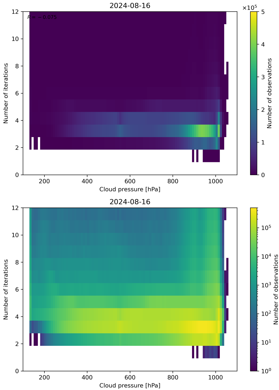
Figure 81: Scatter density plot of “Cloud pressure” against “Number of iterations” for 2024-08-16 to 2024-08-17.
