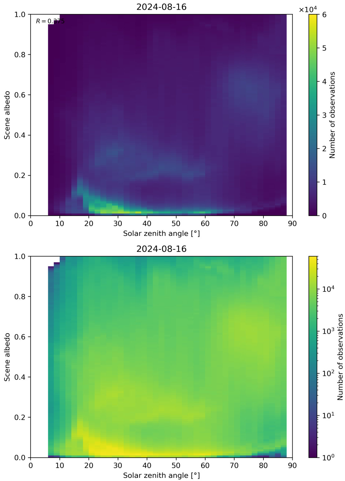
Figure 116: Scatter density plot of “Solar zenith angle” against “Scene albedo” for 2024-08-16 to 2024-08-17.
