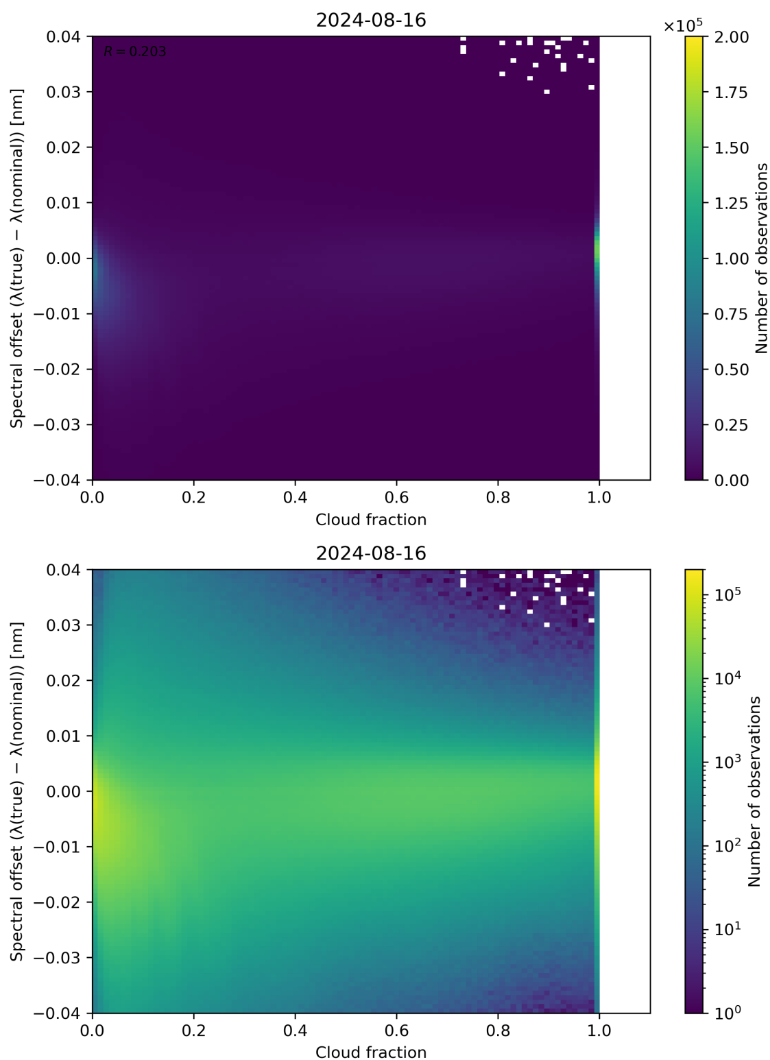
Figure 76: Scatter density plot of “Cloud fraction” against “Spectral offset ( \lambda(\text{true}) - \lambda(\text{nominal}) )” for 2024-08-16 to 2024-08-17.
