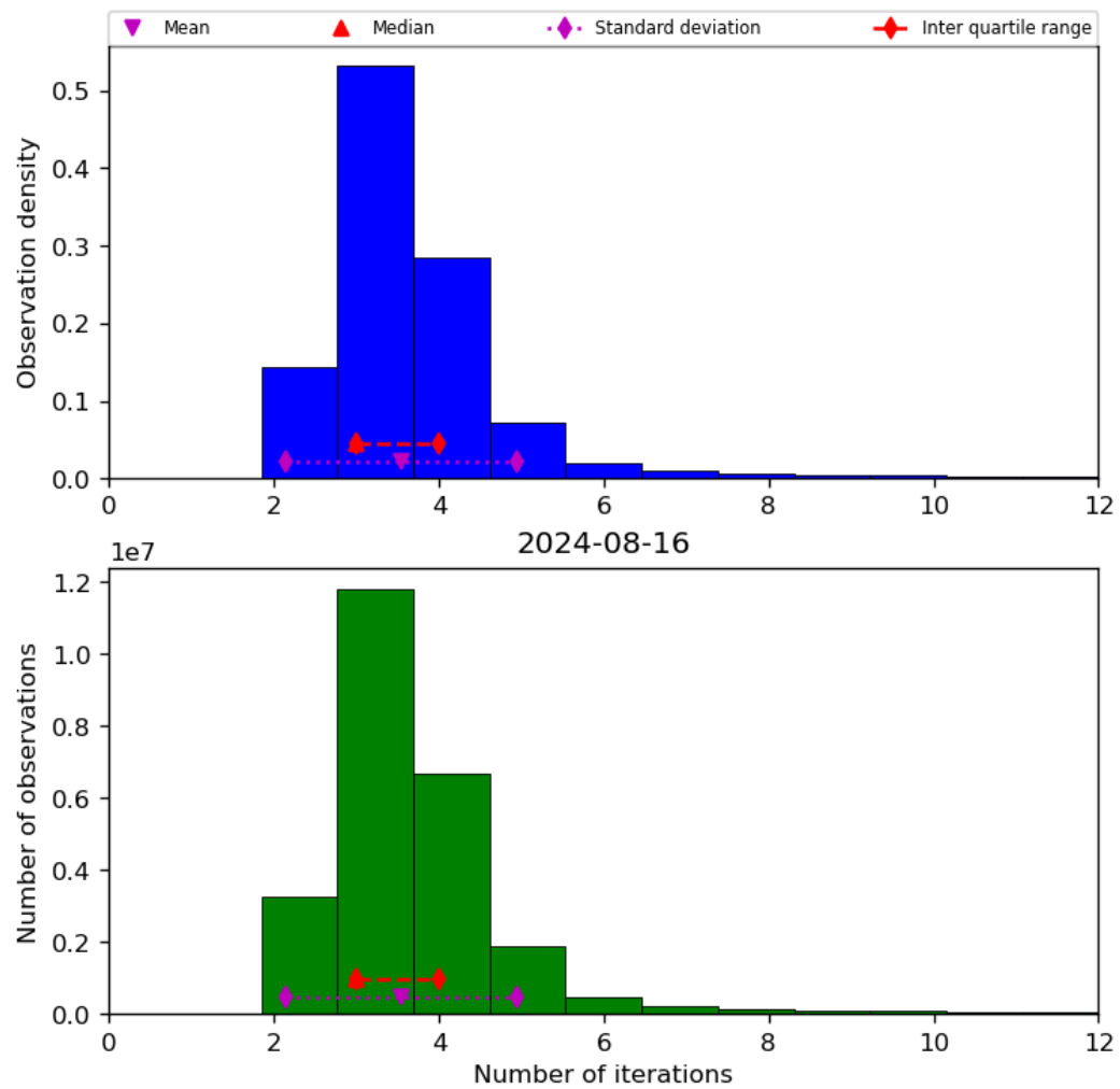
Figure 39: Histogram of “Number of iterations” for 2024-08-16 to 2024-08-17
