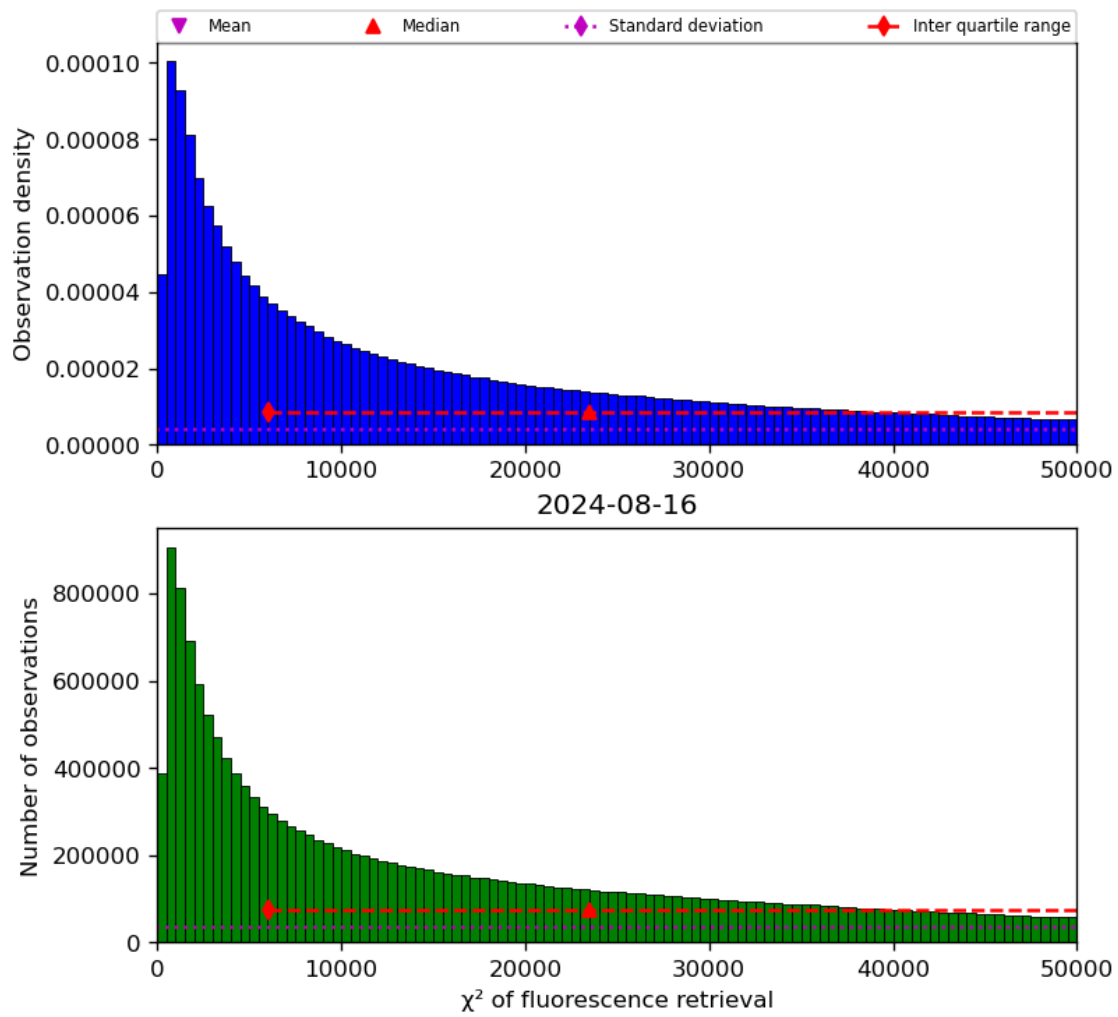
Figure 42: Histogram of “ \chi^2 of fluorescence retrieval” for 2024-08-16 to 2024-08-17
