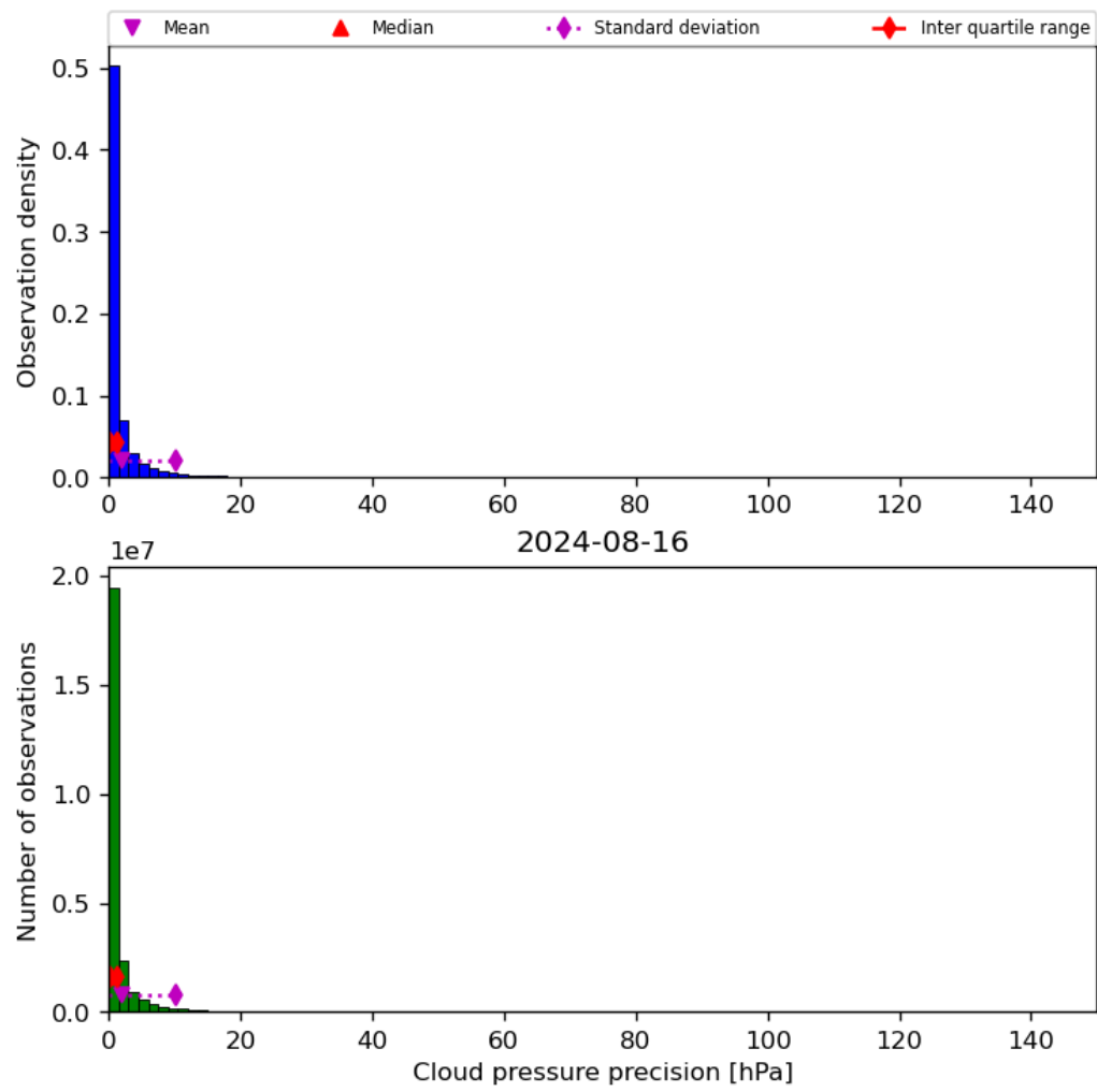
Figure 31: Histogram of “Cloud pressure precision” for 2024-08-16 to 2024-08-17
