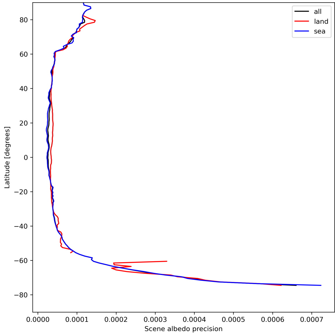
Figure 18: Zonal average of “Scene albedo precision” for 2024-08-16 to 2024-08-17.
