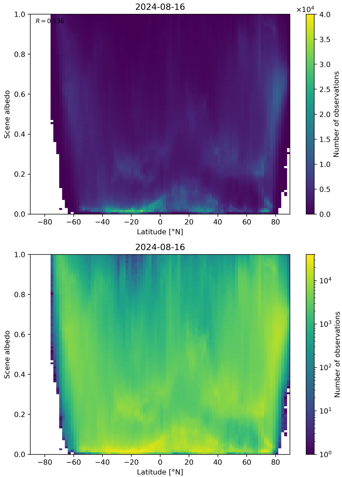
Figure 95: Scatter density plot of “Latitude” against “Scene albedo” for 2024-08-16 to 2024-08-17.
