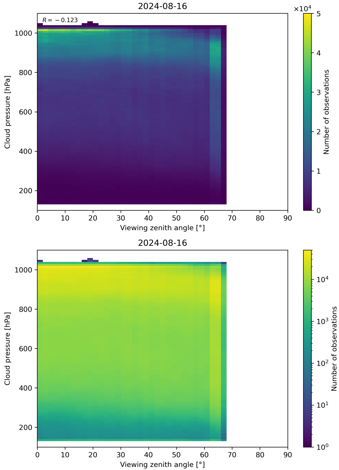
Figure 121: Scatter density plot of “Viewing zenith angle” against “Cloud pressure” for 2024-08-16 to 2024-08-17.
