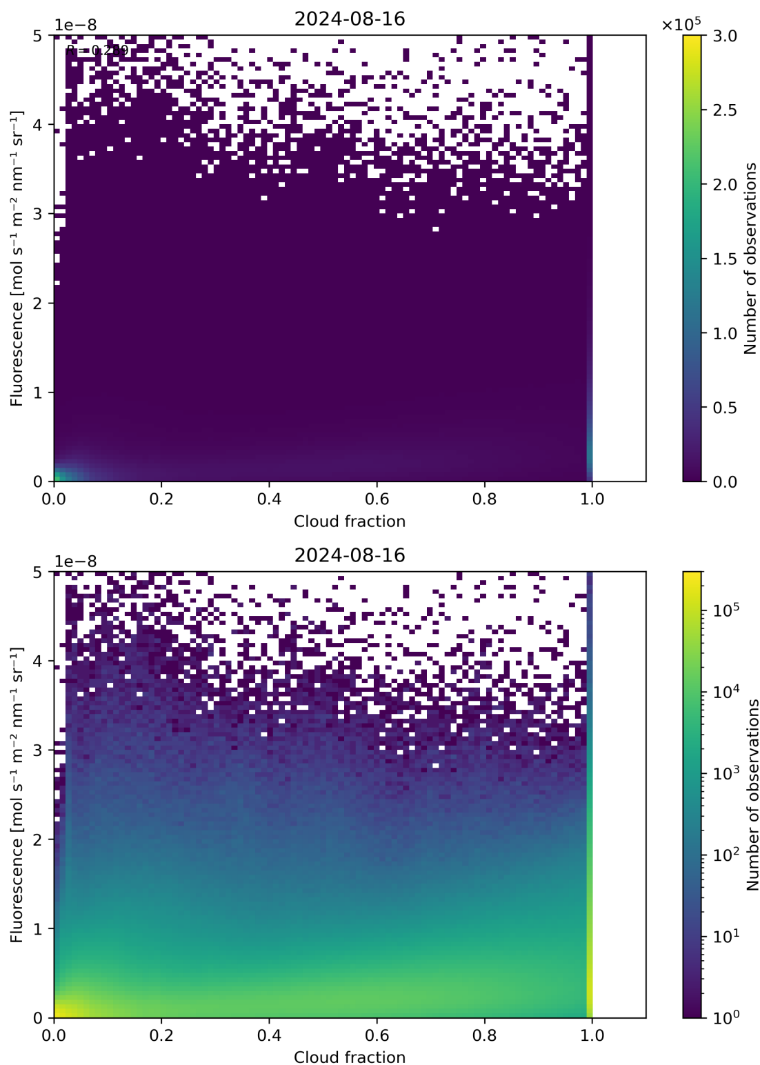
Figure 72: Scatter density plot of “Cloud fraction” against “Fluorescence” for 2024-08-16 to 2024-08-17.
