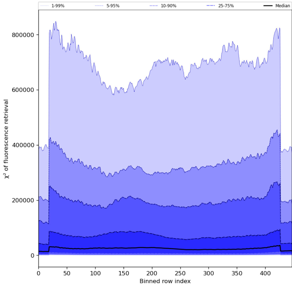
Figure 59: Along track statistics of “ \chi^2 of fluorescence retrieval” for 2024-08-16 to 2024-08-17
