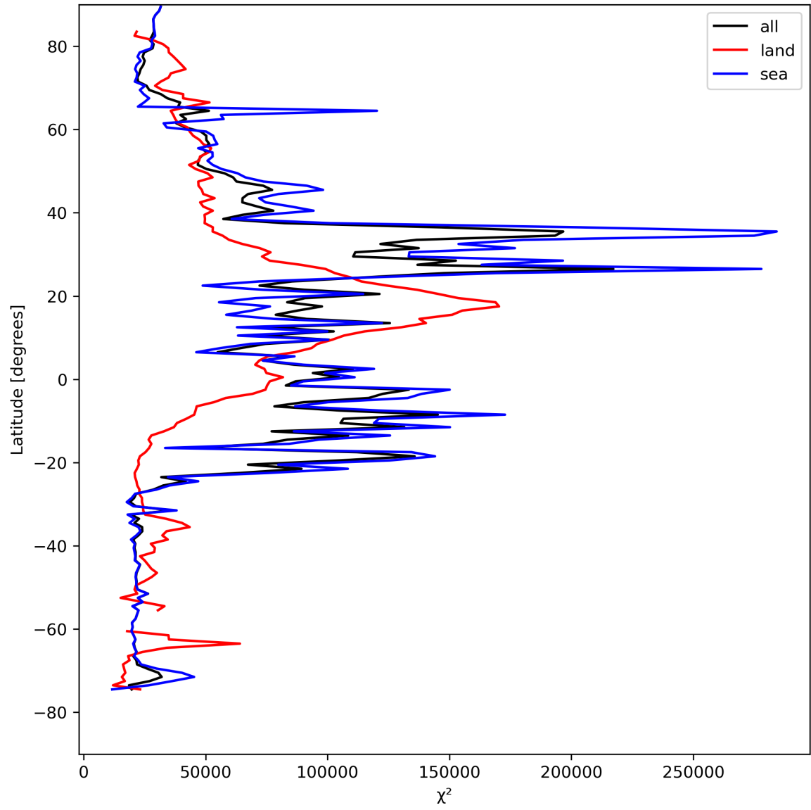
Figure 21: Zonal average of “ \chi^2 ” for 2024-08-16 to 2024-08-17.
