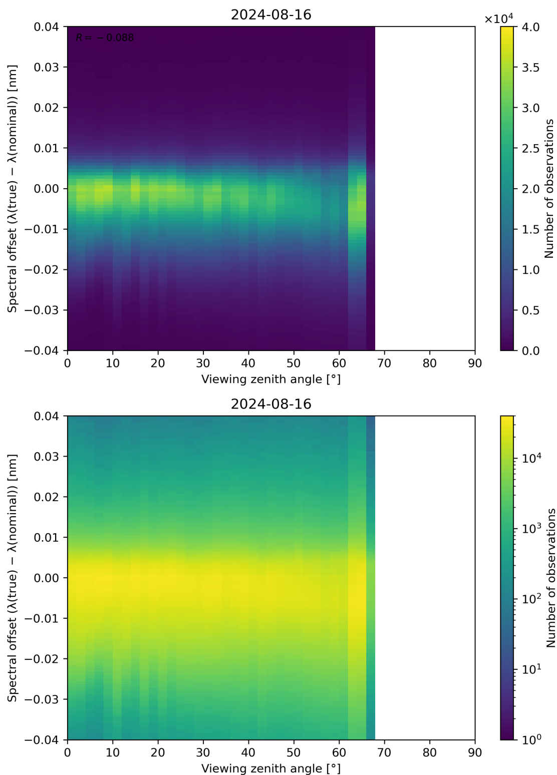
Figure 128: Scatter density plot of “Viewing zenith angle” against “Spectral offset ( \lambda(\text{true}) - \lambda(\text{nominal}) )” for 2024-08-16 to 2024-08-17.
