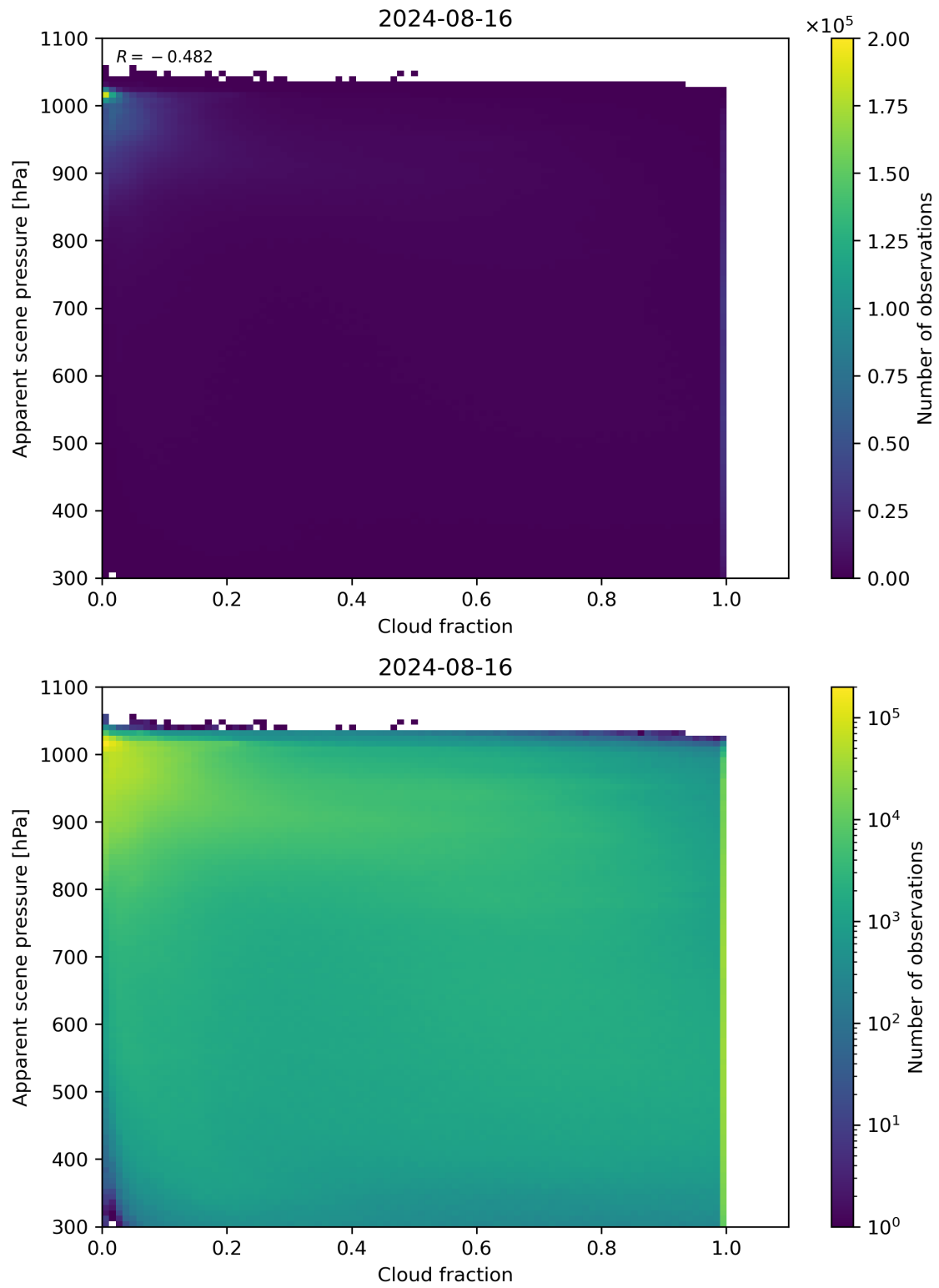
Figure 70: Scatter density plot of “Cloud fraction” against “Apparent scene pressure” for 2024-08-16 to 2024-08-17.
