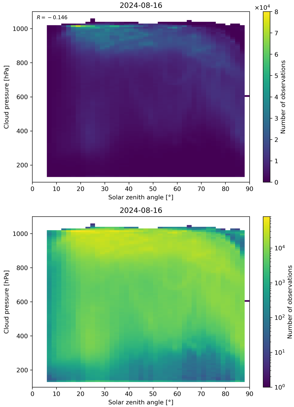
Figure 111: Scatter density plot of “Solar zenith angle” against “Cloud pressure” for 2024-08-16 to 2024-08-17.
