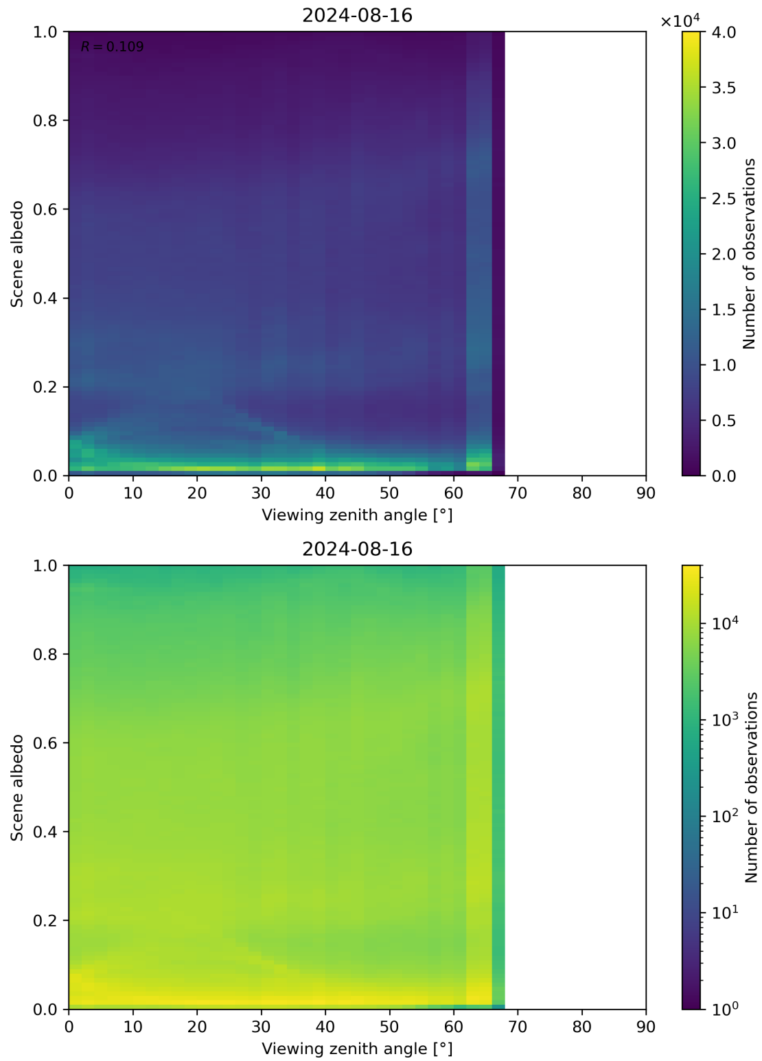
Figure 126: Scatter density plot of “Viewing zenith angle” against “Scene albedo” for 2024-08-16 to 2024-08-17.
