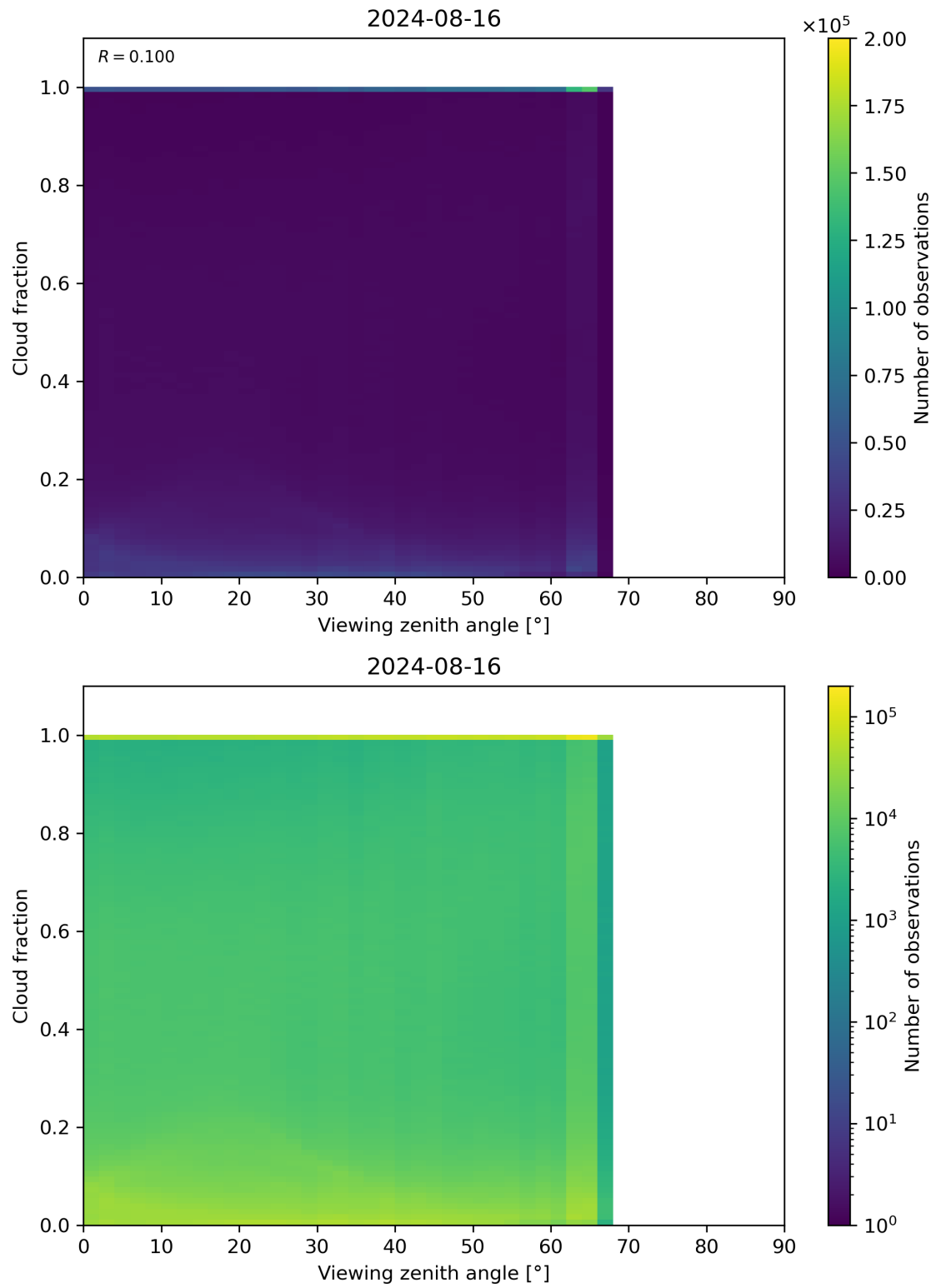
Figure 120: Scatter density plot of “Viewing zenith angle” against “Cloud fraction” for 2024-08-16 to 2024-08-17.
