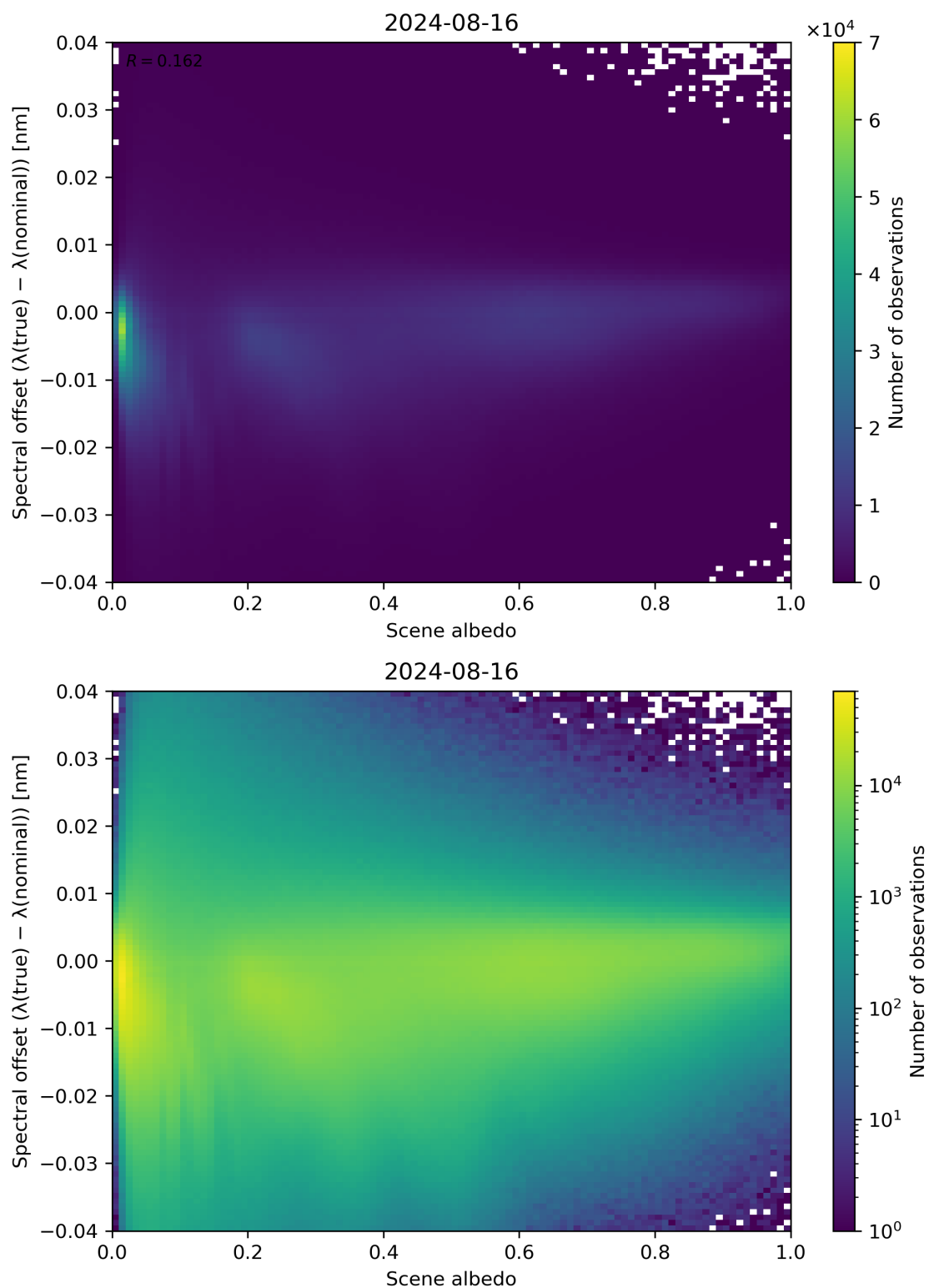
Figure 107: Scatter density plot of “Scene albedo” against “Spectral offset ( \lambda(\text{true}) - \lambda(\text{nominal}) )” for 2024-08-16 to 2024-08-17.
