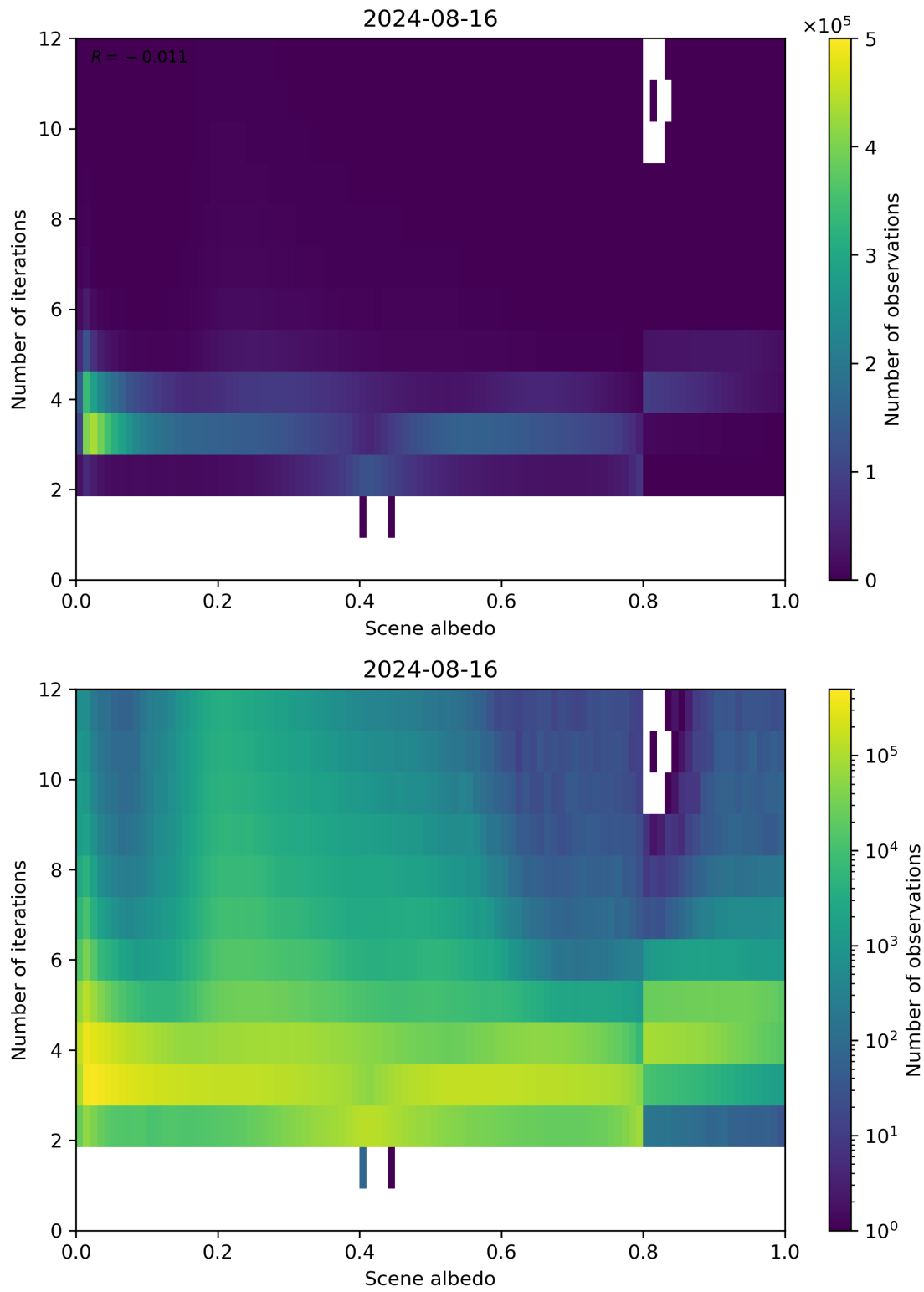
Figure 105: Scatter density plot of “Scene albedo” against “Number of iterations” for 2024-08-16 to 2024-08-17.
