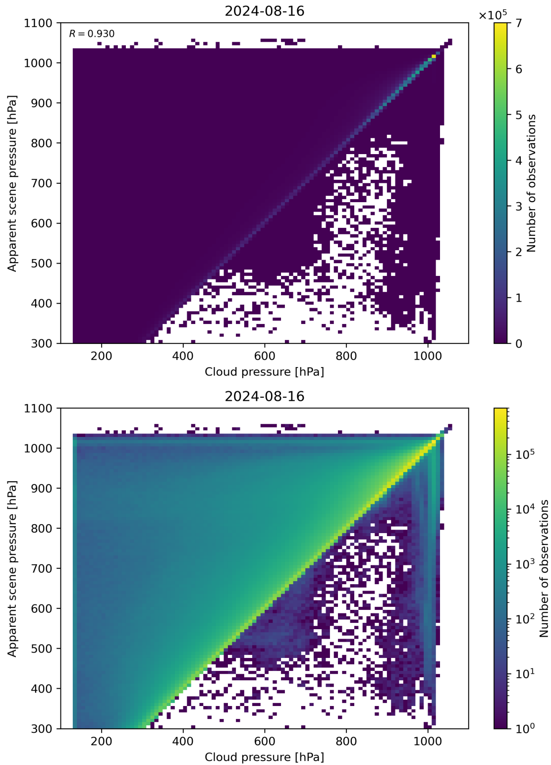
Figure 77: Scatter density plot of “Cloud pressure” against “Apparent scene pressure” for 2024-08-16 to 2024-08-17.
