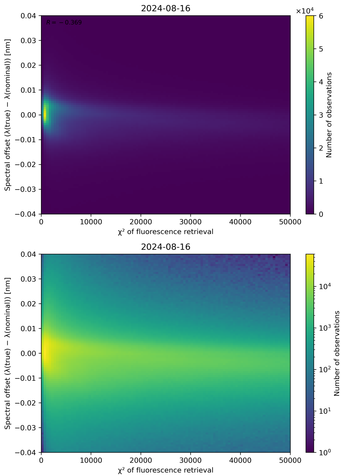
Figure 69: Scatter density plot of " \chi^2 of fluorescence retrieval" against "Spectral offset ( \lambda(\text{true}) - \lambda(\text{nominal})) " for 2024-08-16 to 2024-08-17.
