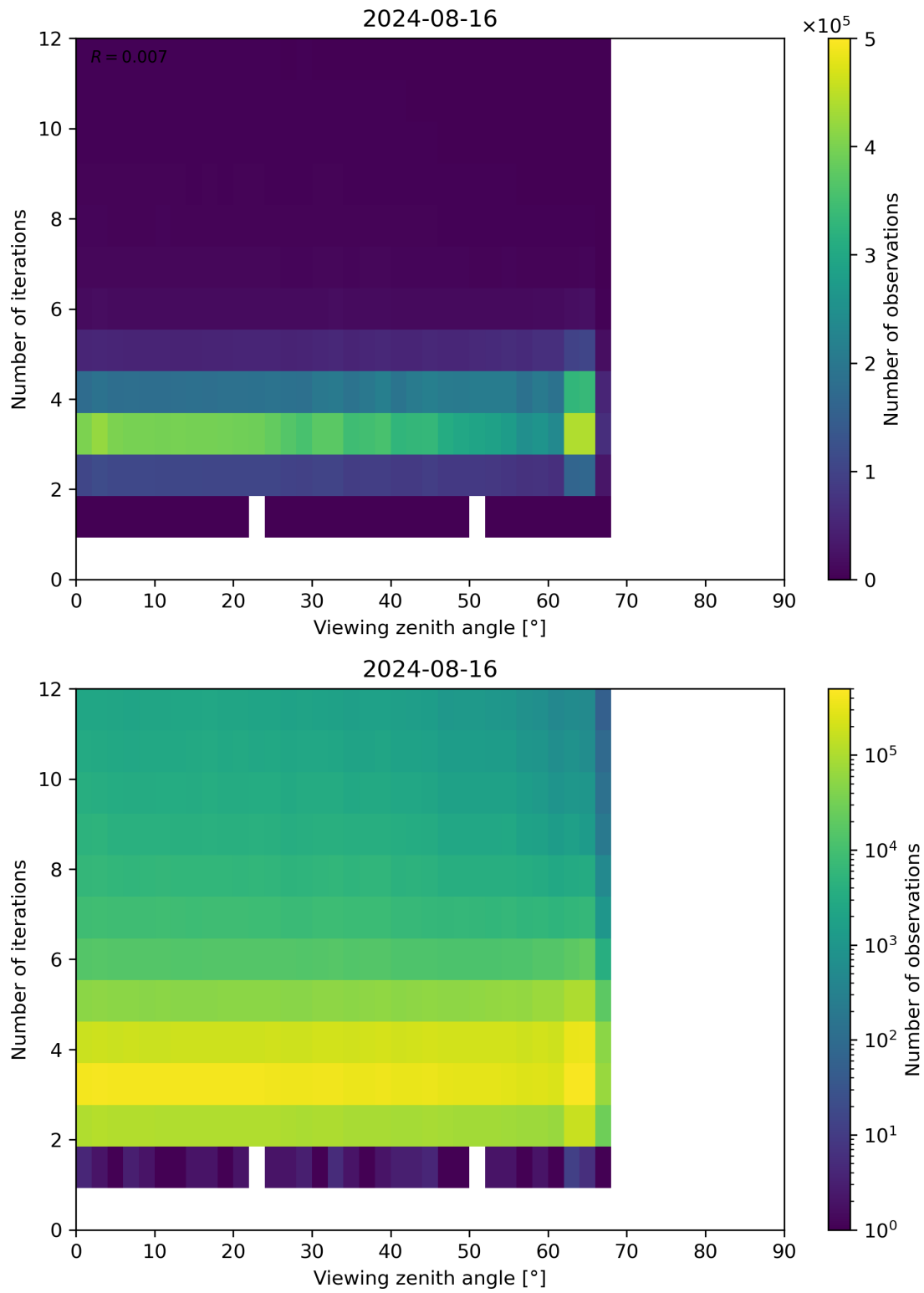
Figure 124: Scatter density plot of “Viewing zenith angle” against “Number of iterations” for 2024-08-16 to 2024-08-17.
