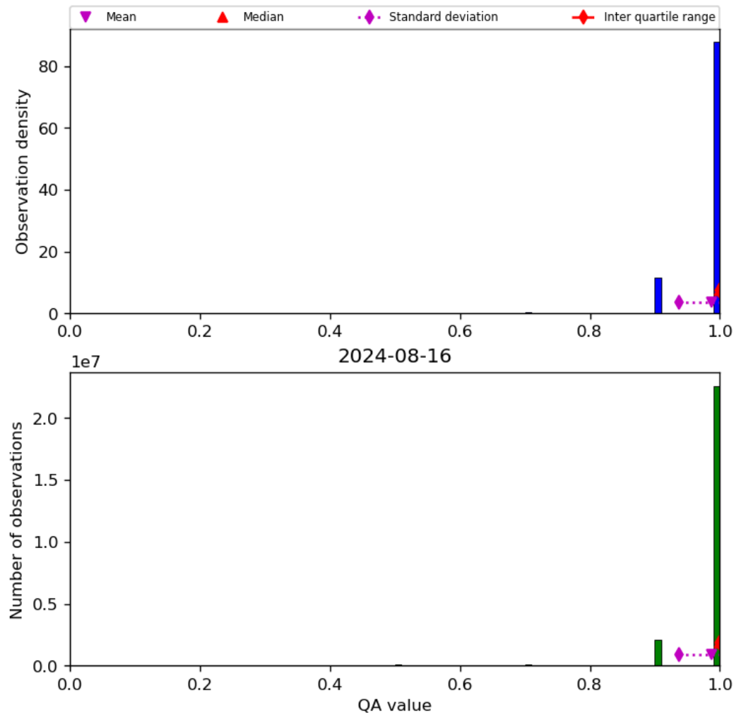
Figure 29: Histogram of “QA value” for 2024-08-16 to 2024-08-17
