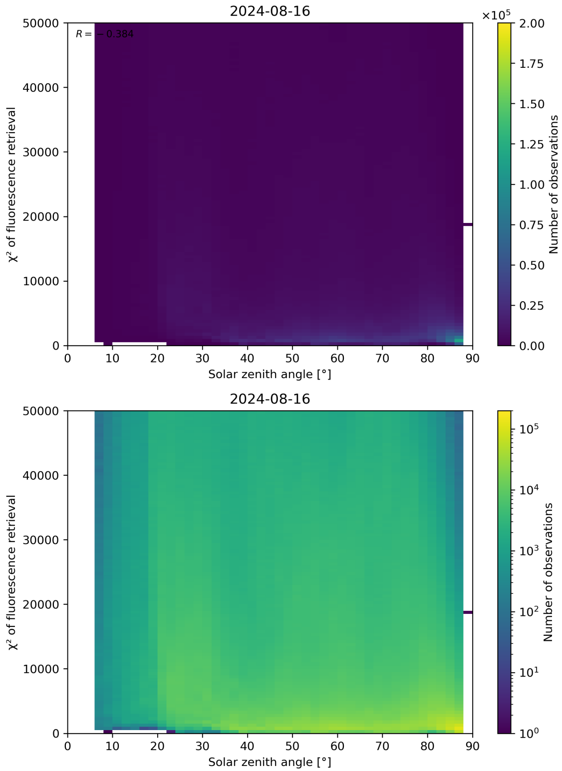
Figure 109: Scatter density plot of “Solar zenith angle” against “ \chi^2 of fluorescence retrieval” for 2024-08-16 to 2024-08-17.
