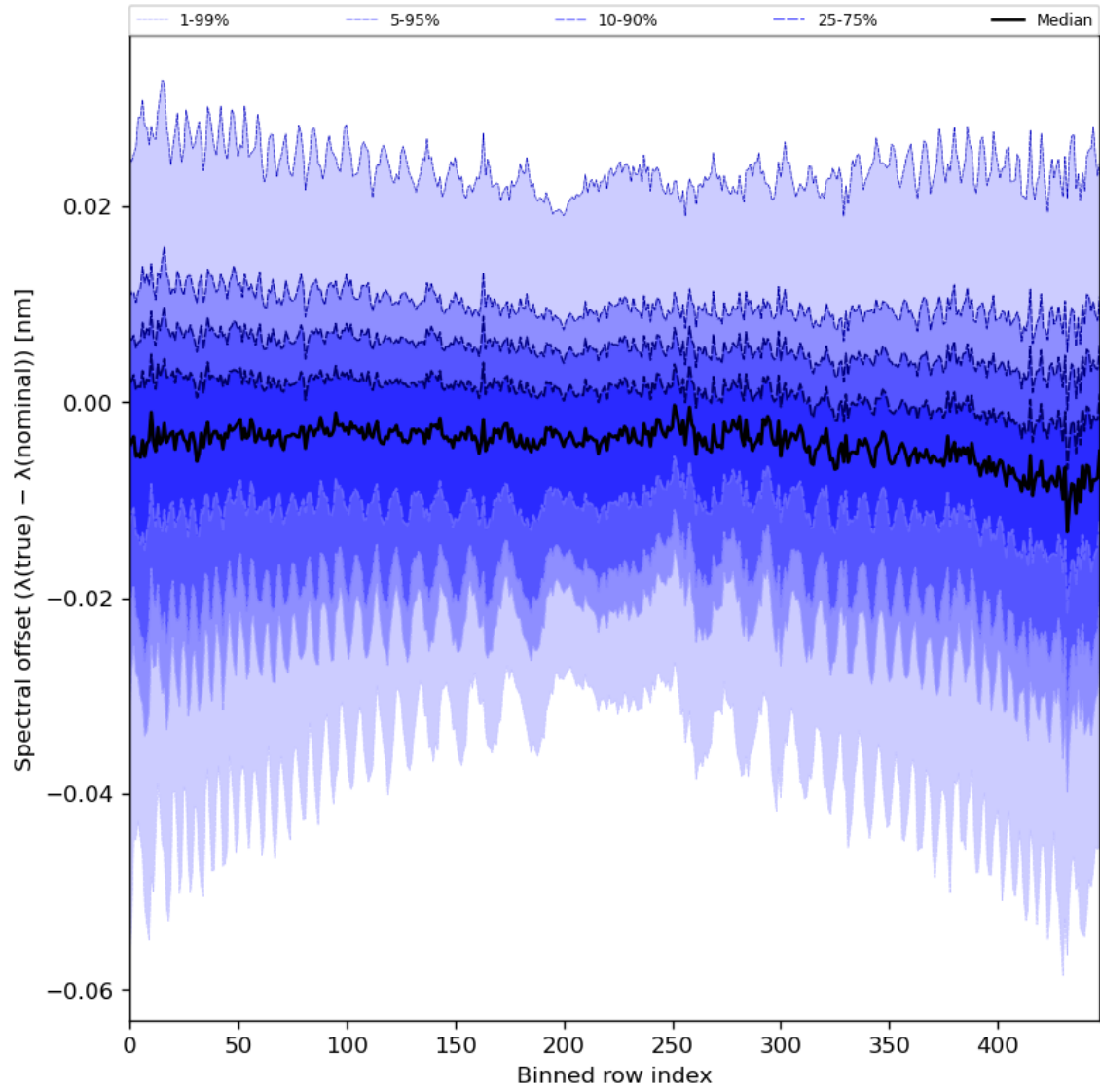
Figure 62: Along track statistics of “Spectral offset ( \lambda(\text{true}) - \lambda(\text{nominal}) )” for 2024-08-16 to 2024-08-17
