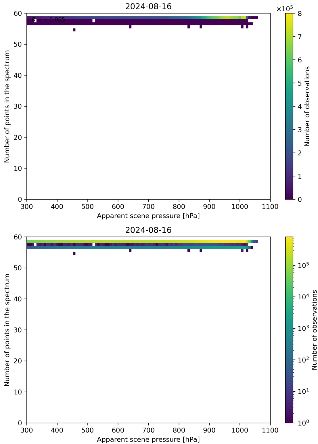
Figure 66: Scatter density plot of “Apparent scene pressure” against “Number of points in the spectrum” for 2024-08-16 to 2024-08-17.
