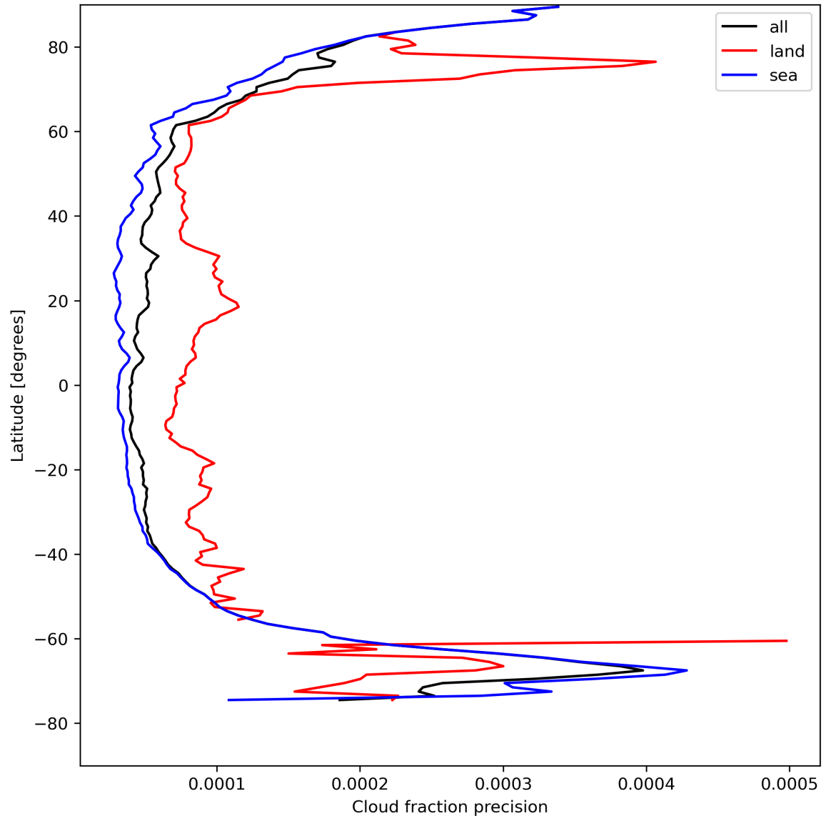
Figure 16: Zonal average of “Cloud fraction precision” for 2024-08-16 to 2024-08-17.
