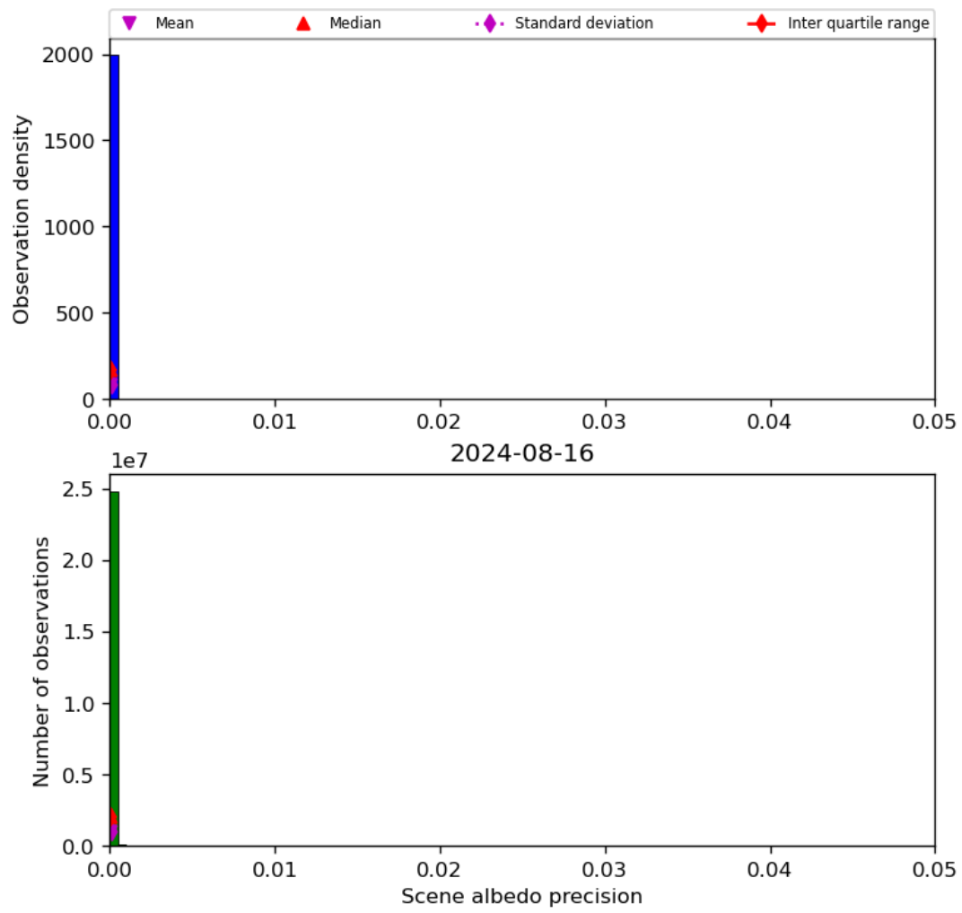
Figure 35: Histogram of “Scene albedo precision” for 2024-08-16 to 2024-08-17
