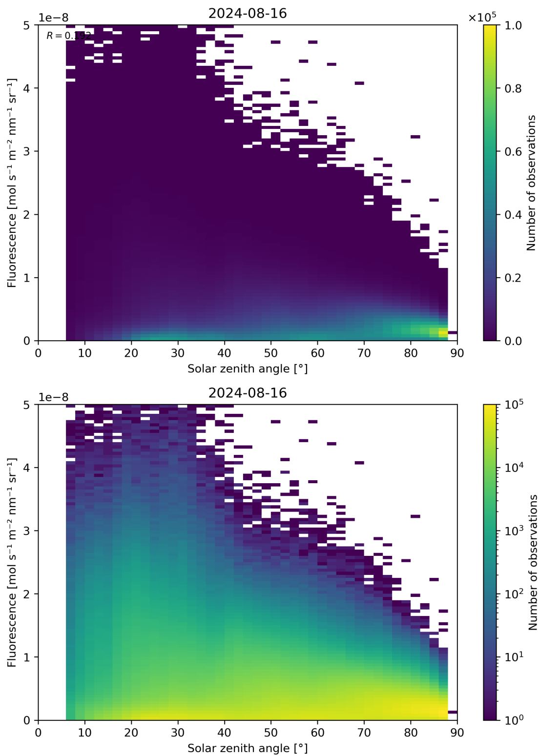
Figure 112: Scatter density plot of “Solar zenith angle” against “Fluorescence” for 2024-08-16 to 2024-08-17.
