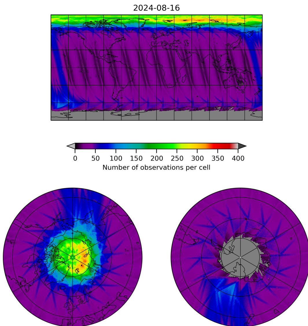
Figure 11: Map of the number of observations for 2024-08-16 to 2024-08-17
