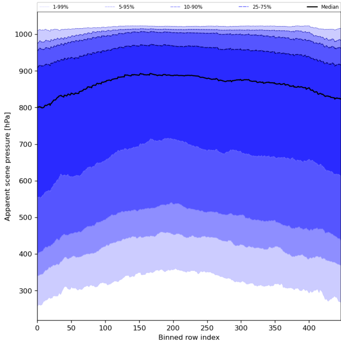
Figure 53: Along track statistics of “Apparent scene pressure” for 2024-08-16 to 2024-08-17
