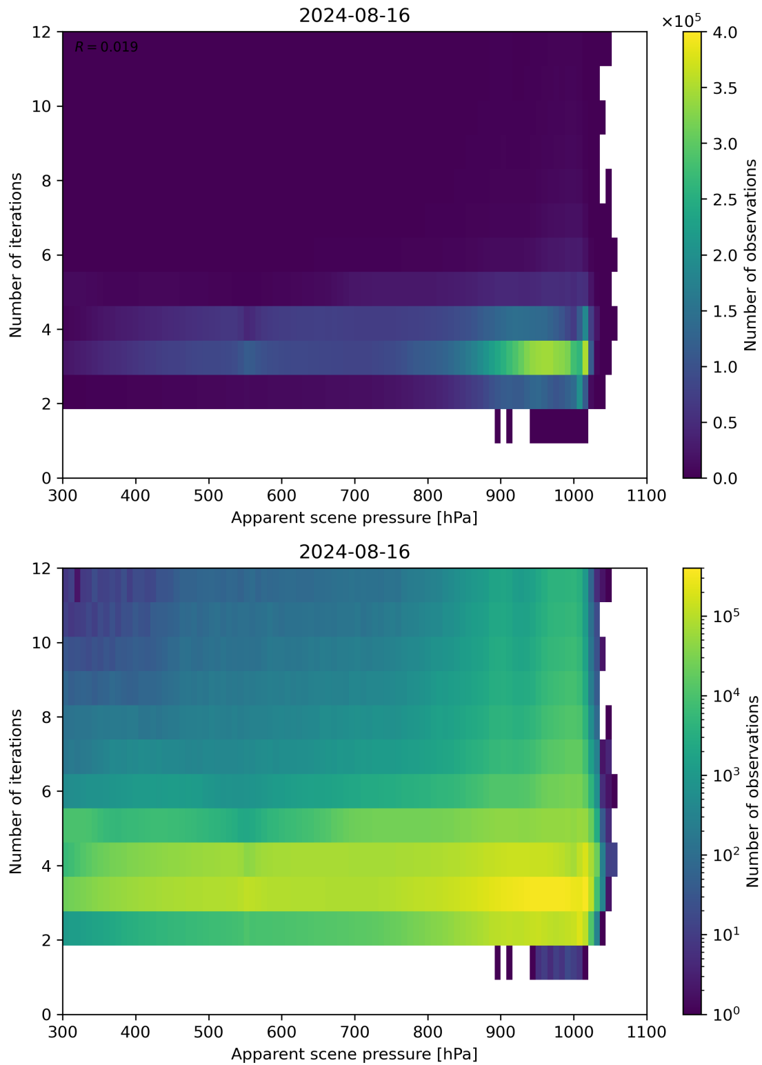
Figure 65: Scatter density plot of “Apparent scene pressure” against “Number of iterations” for 2024-08-16 to 2024-08-17.
