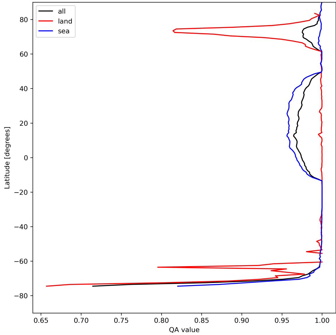
Figure 12: Zonal average of “QA value” for 2024-08-16 to 2024-08-17.
