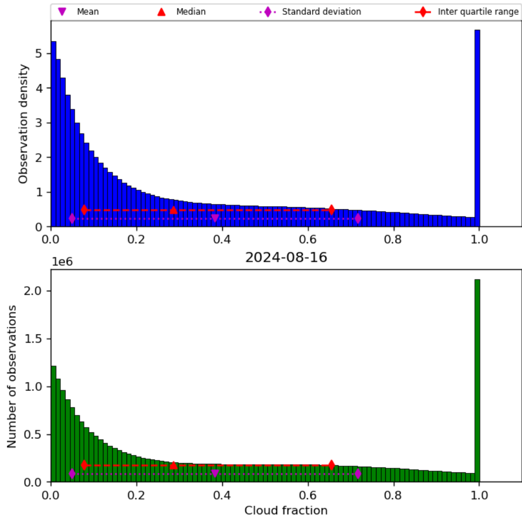
Figure 32: Histogram of “Cloud fraction” for 2024-08-16 to 2024-08-17
