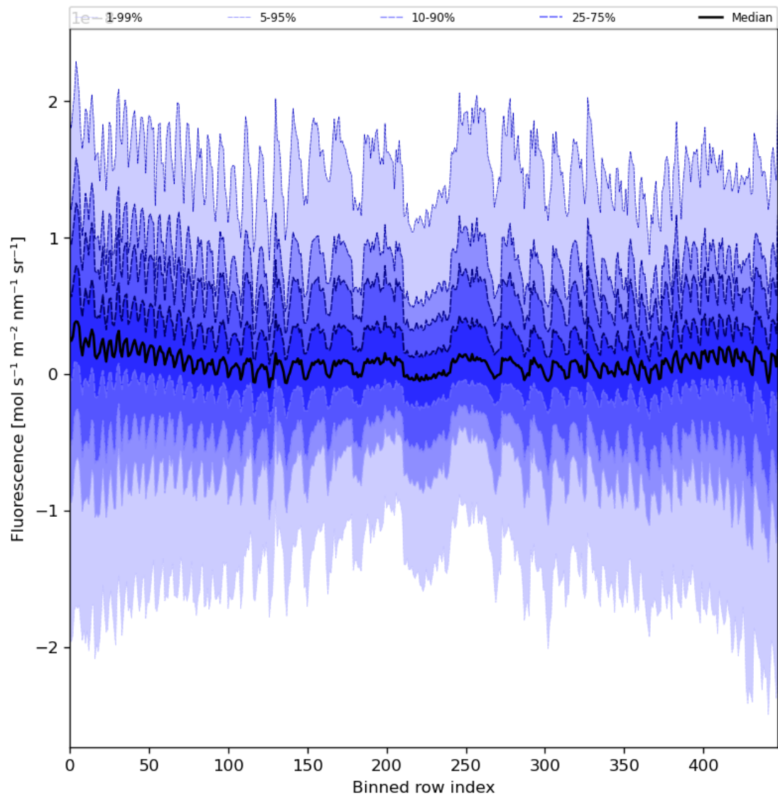
Figure 57: Along track statistics of “Fluorescence” for 2024-08-16 to 2024-08-17
