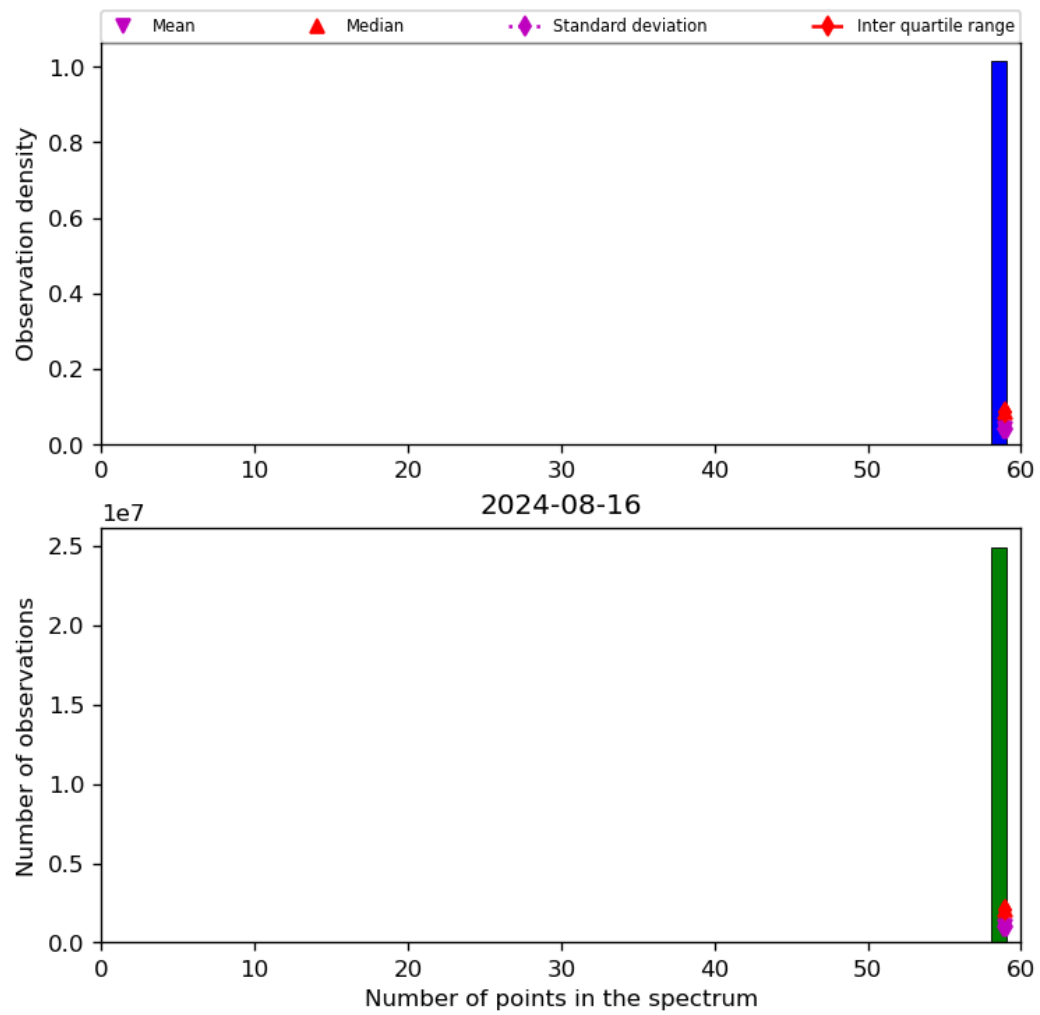
Figure 44: Histogram of “Number of points in the spectrum” for 2024-08-16 to 2024-08-17
