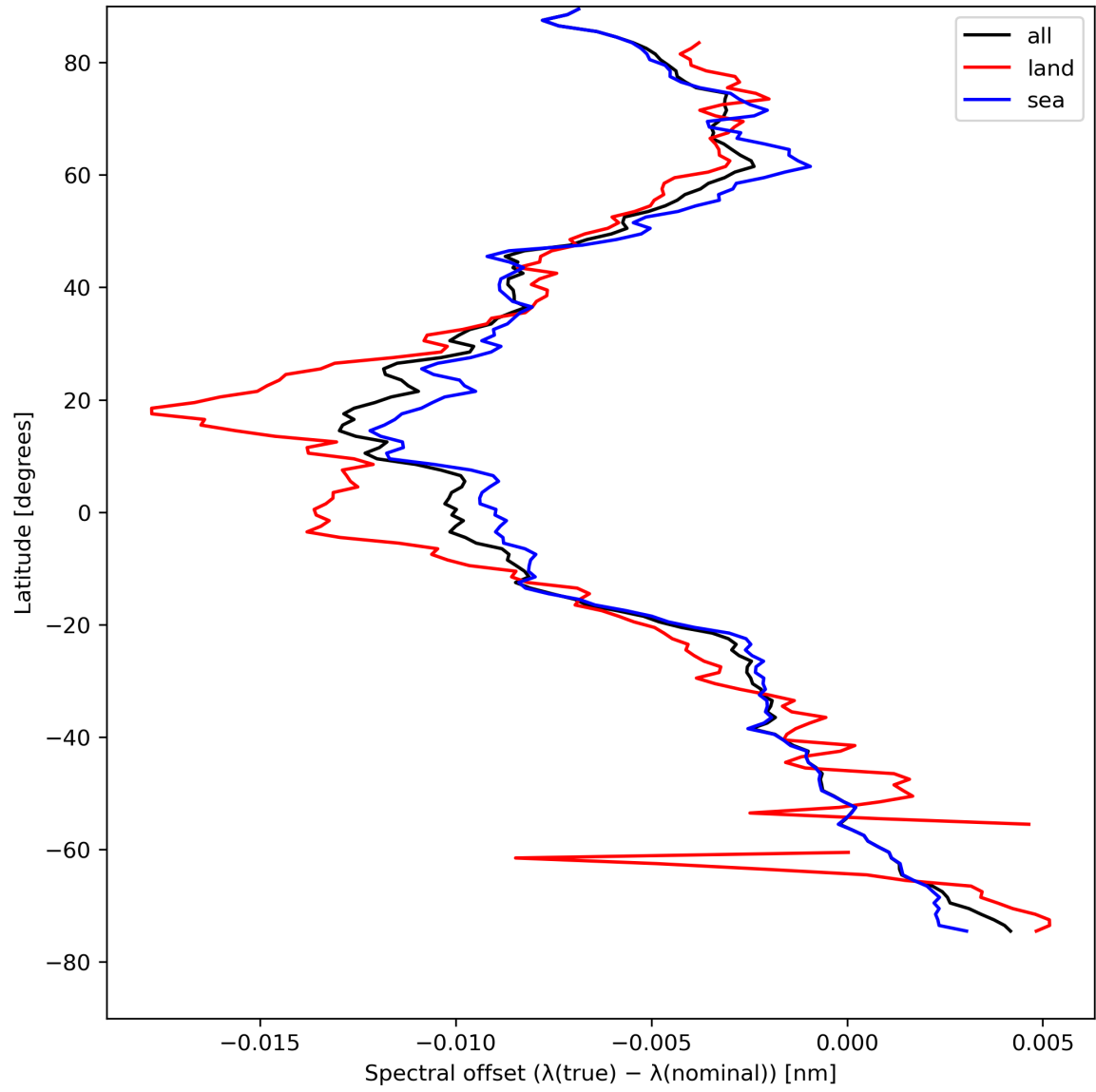
Figure 28: Zonal average of “Spectral offset ( \lambda(\text{true}) - \lambda(\text{nominal}) )” for 2024-08-16 to 2024-08-17.
