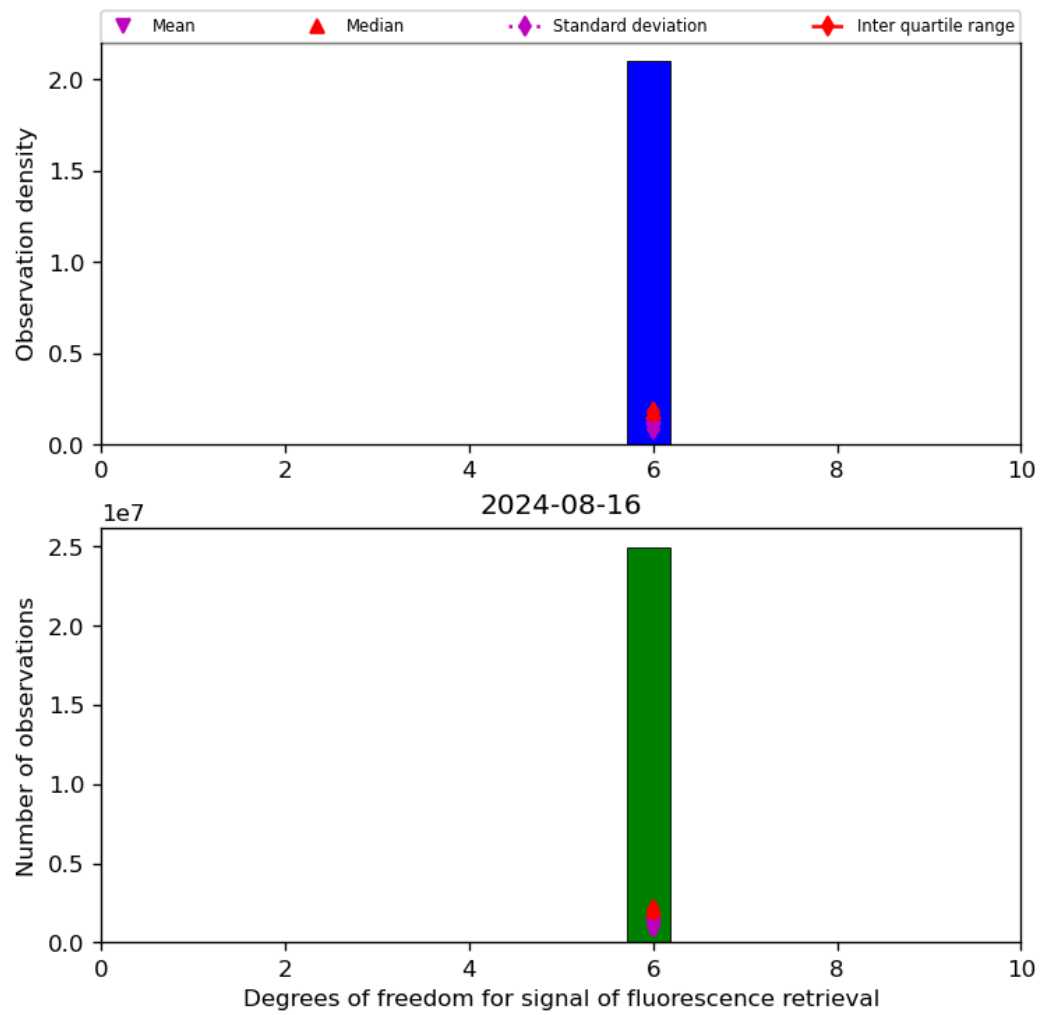
Figure 43: Histogram of “Degrees of freedom for signal of fluorescence retrieval” for 2024-08-16 to 2024-08-17
