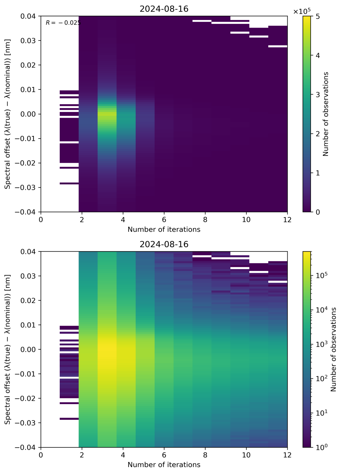
Figure 100: Scatter density plot of “Number of iterations” against “Spectral offset ( \lambda(\text{true}) - \lambda(\text{nominal}) )” for 2024-08-16 to 2024-08-17.
