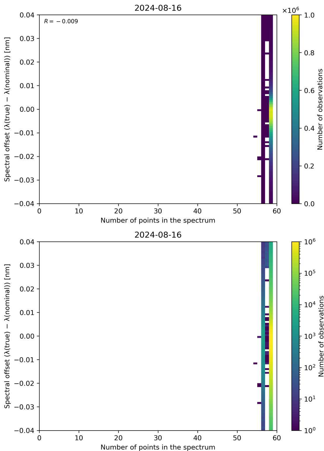
Figure 101: Scatter density plot of “Number of points in the spectrum” against “Spectral offset ( \lambda(\text{true}) - \lambda(\text{nominal}) )” for 2024-08-16 to 2024-08-17.
