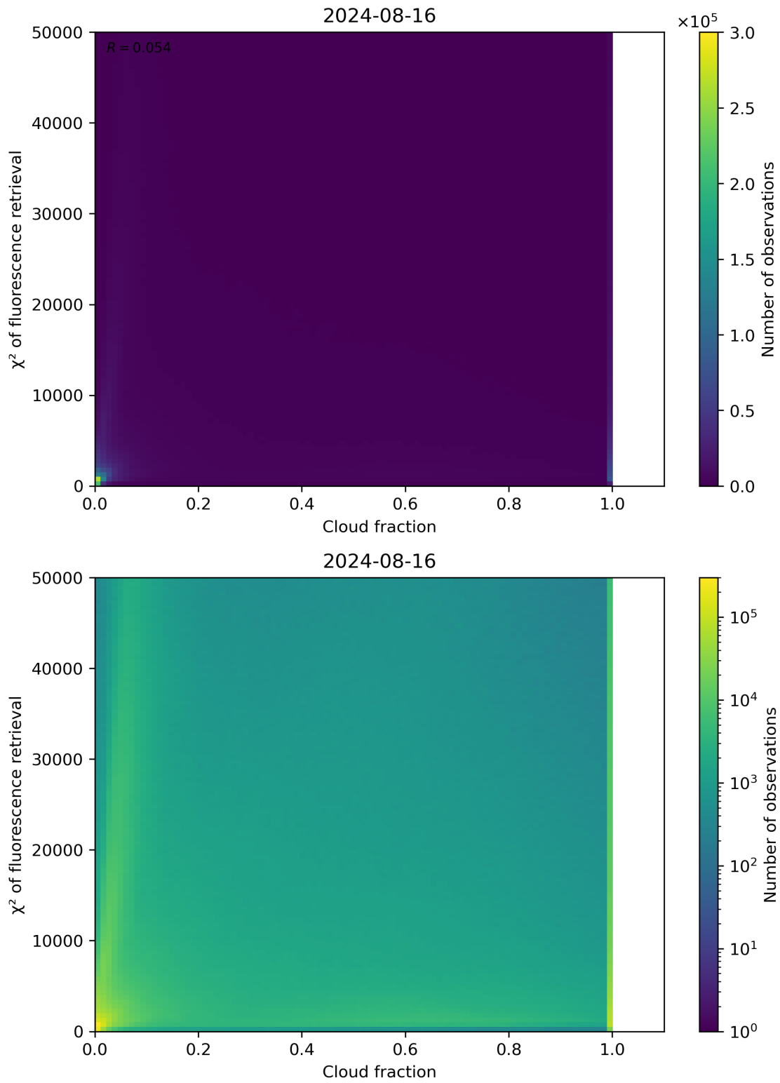
Figure 71: Scatter density plot of “Cloud fraction” against “ \chi^2 of fluorescence retrieval” for 2024-08-16 to 2024-08-17.
