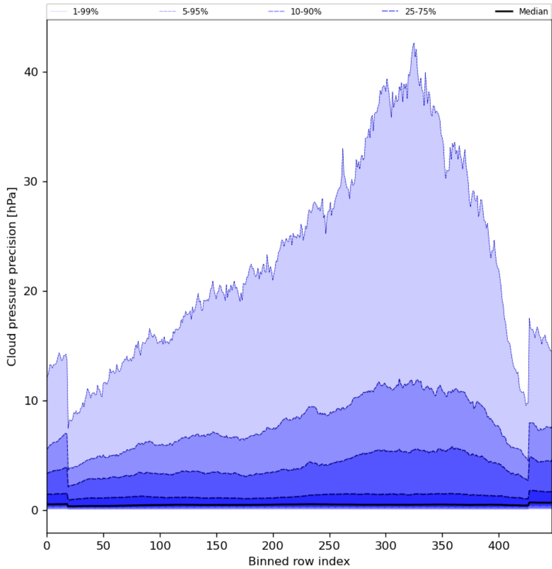
Figure 48: Along track statistics of “Cloud pressure precision” for 2024-08-16 to 2024-08-17
