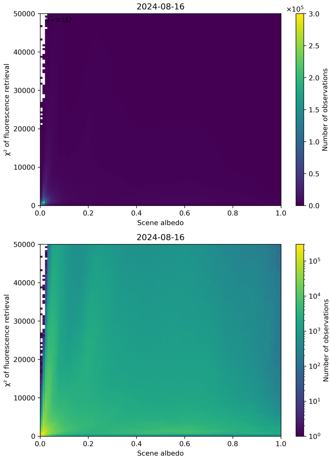
Figure 103: Scatter density plot of “Scene albedo” against “ \chi^2 of fluorescence retrieval” for 2024-08-16 to 2024-08-17.
