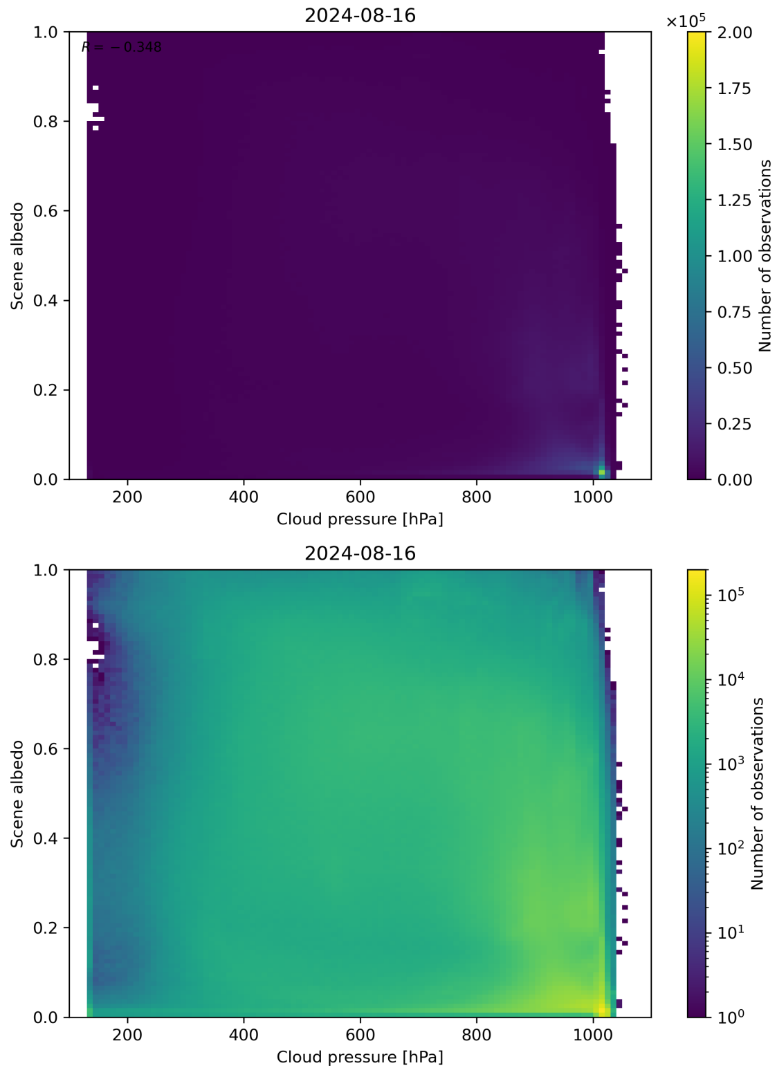
Figure 83: Scatter density plot of “Cloud pressure” against “Scene albedo” for 2024-08-16 to 2024-08-17.
