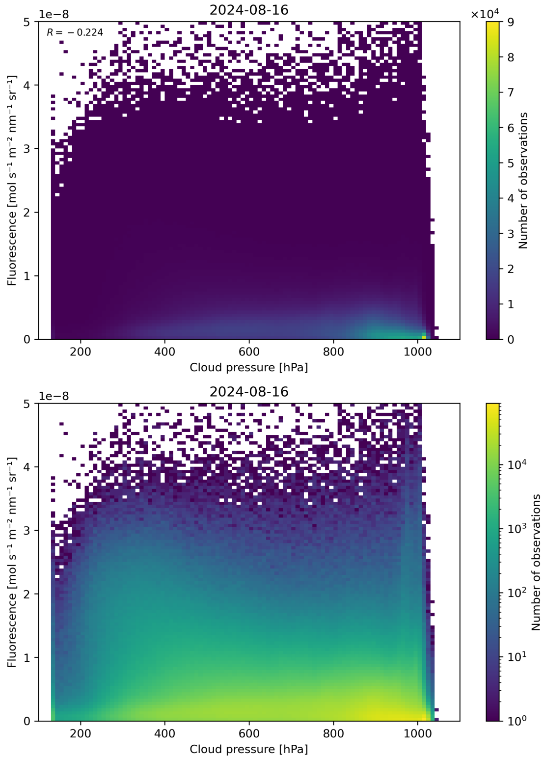
Figure 80: Scatter density plot of “Cloud pressure” against “Fluorescence” for 2024-08-16 to 2024-08-17.
