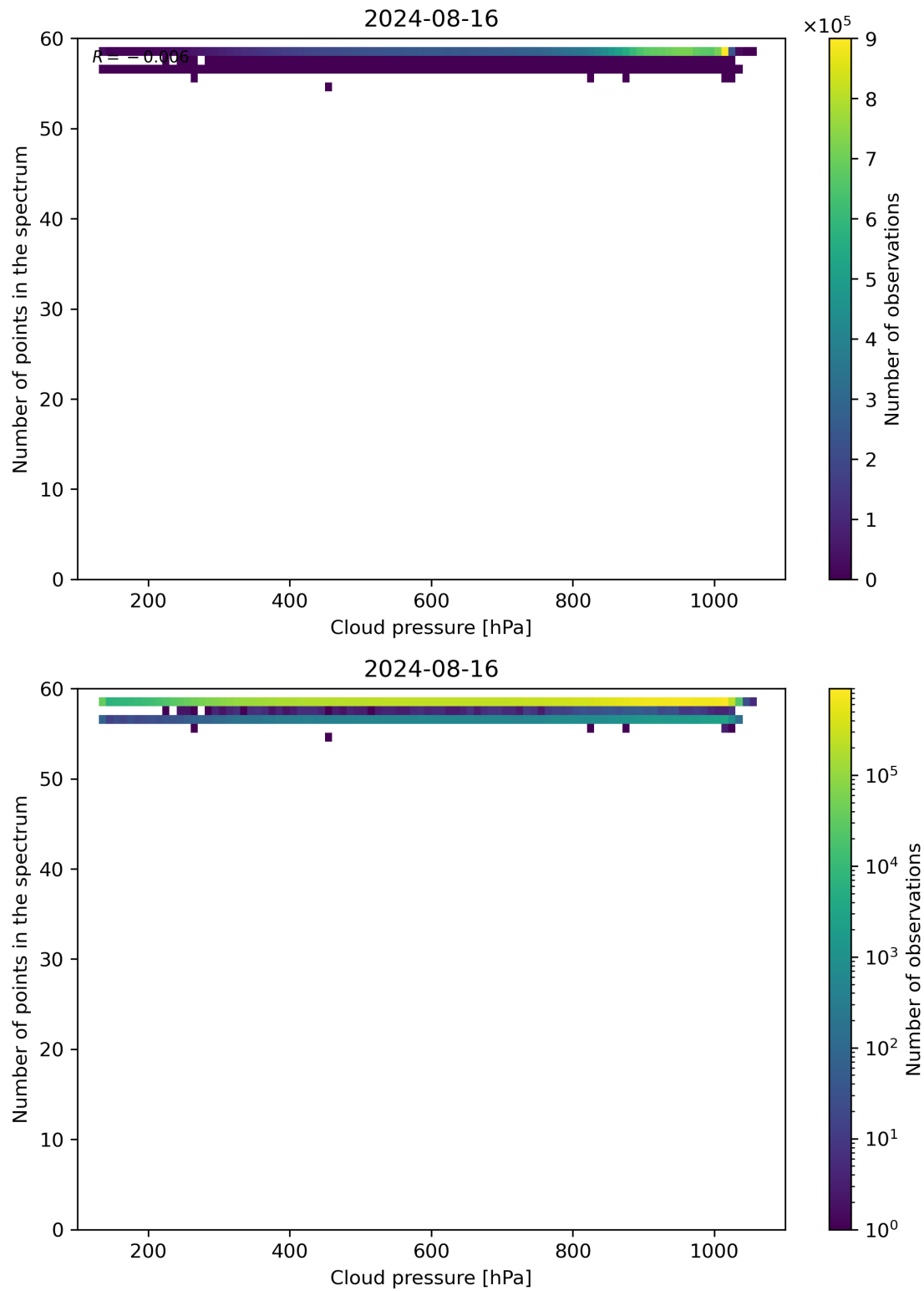
Figure 82: Scatter density plot of “Cloud pressure” against “Number of points in the spectrum” for 2024-08-16 to 2024-08-17.
