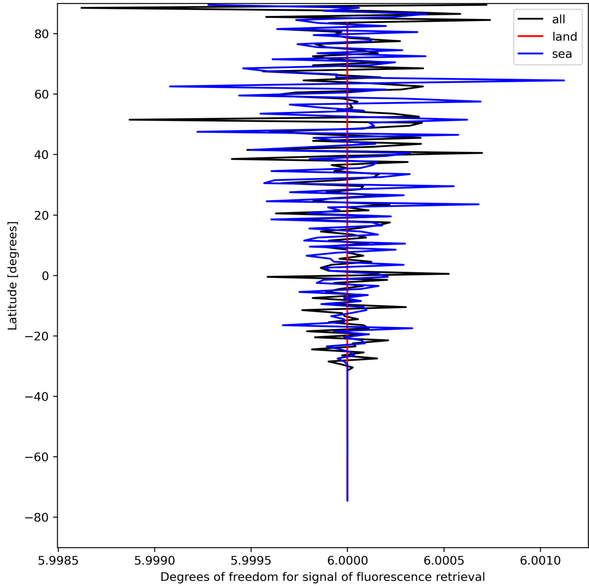
Figure 26: Zonal average of “Degrees of freedom for signal of fluorescence retrieval” for 2024-08-16 to 2024-08-17.
