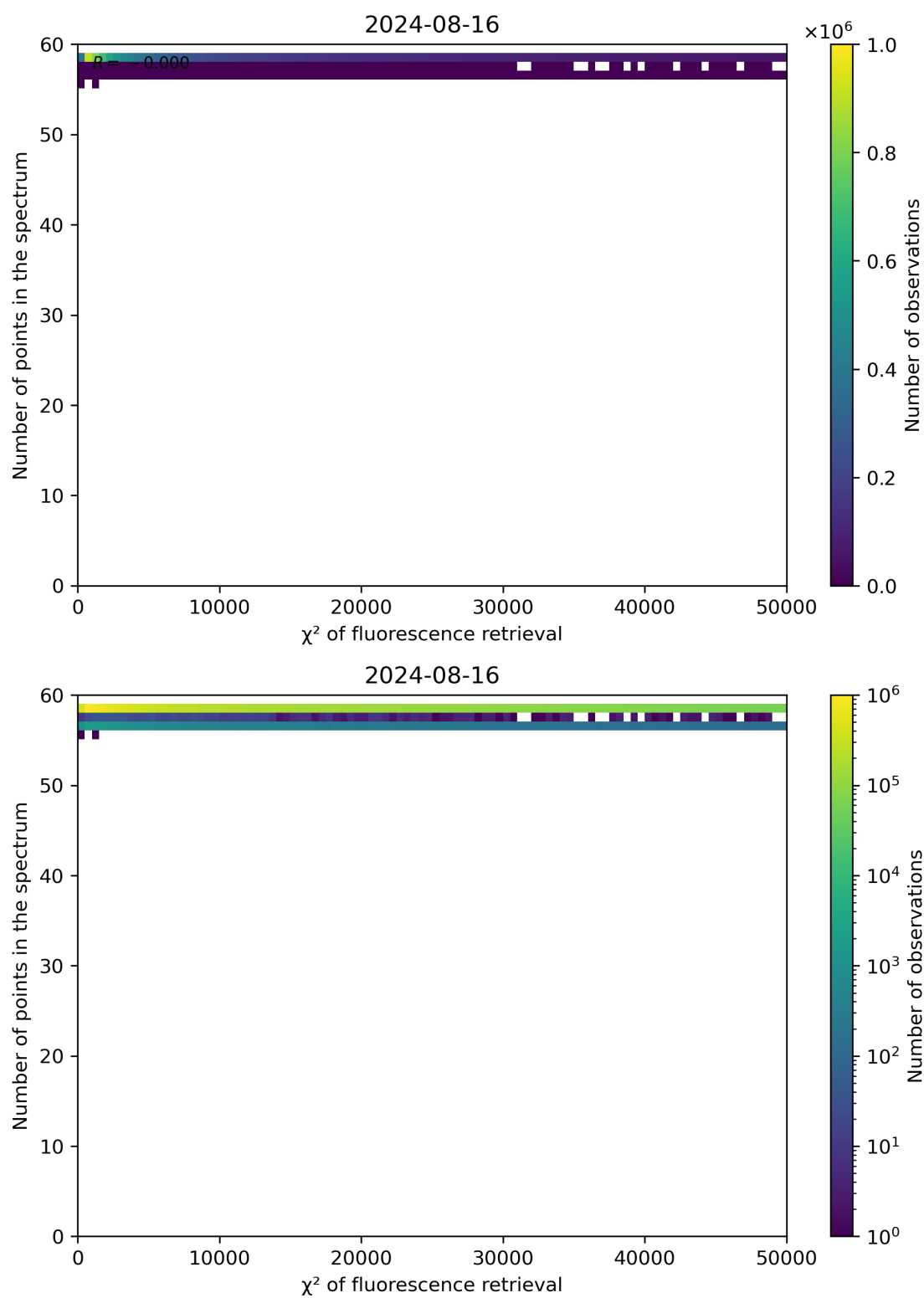
Figure 68: Scatter density plot of " \chi^2 of fluorescence retrieval" against "Number of points in the spectrum" for 2024-08-16 to 2024-08-17.
