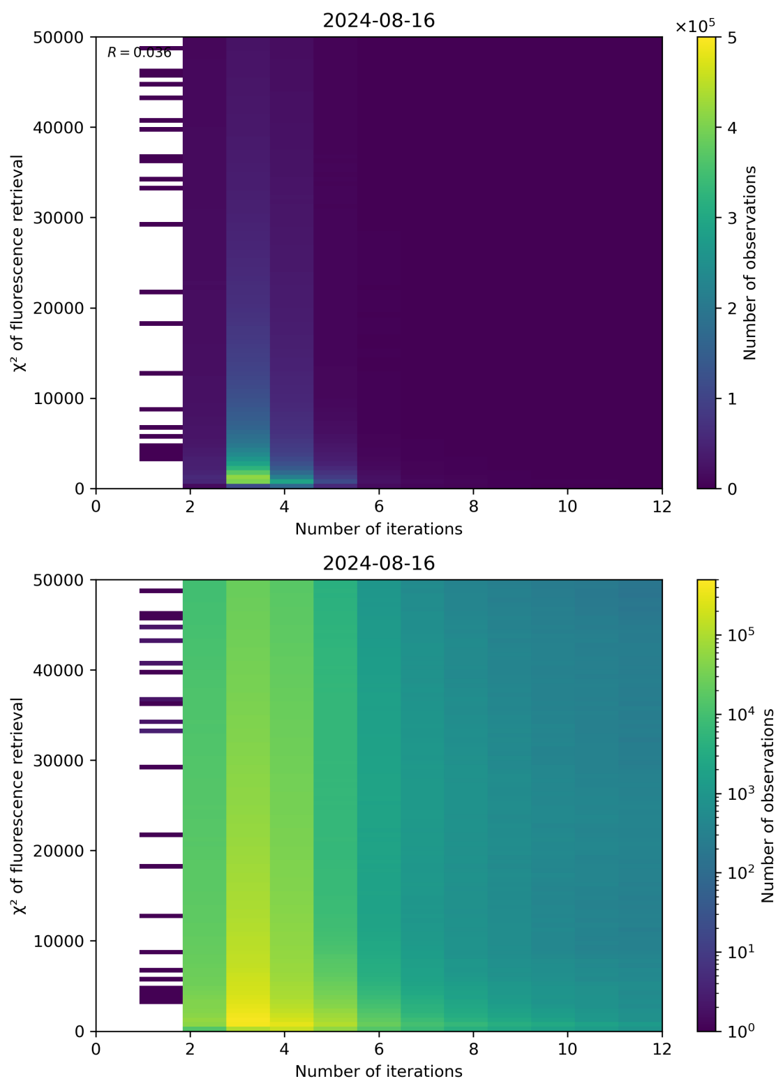
Figure 97: Scatter density plot of “Number of iterations” against “ \chi^2 of fluorescence retrieval” for 2024-08-16 to 2024-08-17.
