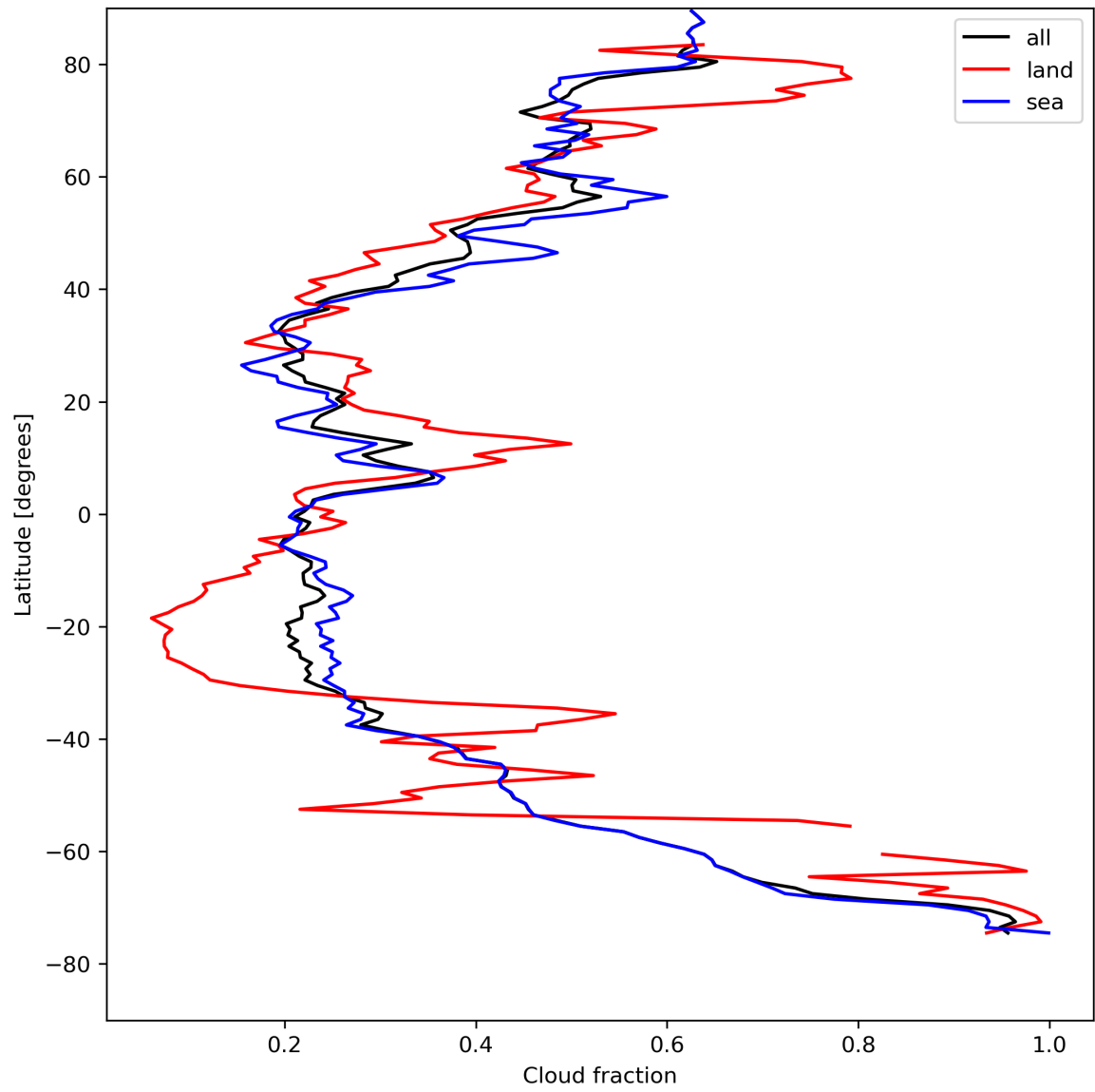
Figure 15: Zonal average of “Cloud fraction” for 2024-08-16 to 2024-08-17.
