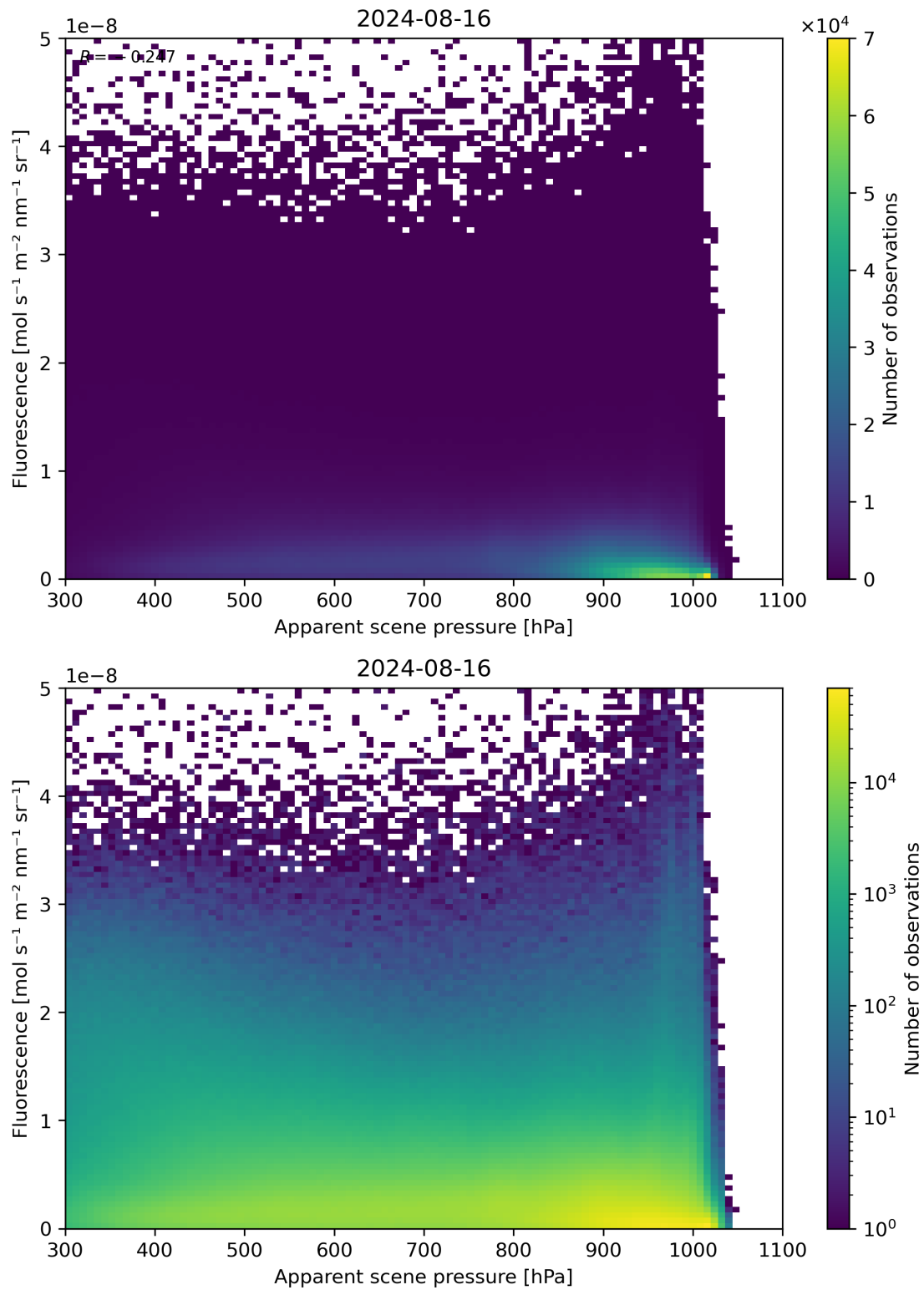
Figure 64: Scatter density plot of “Apparent scene pressure” against “Fluorescence” for 2024-08-16 to 2024-08-17.
