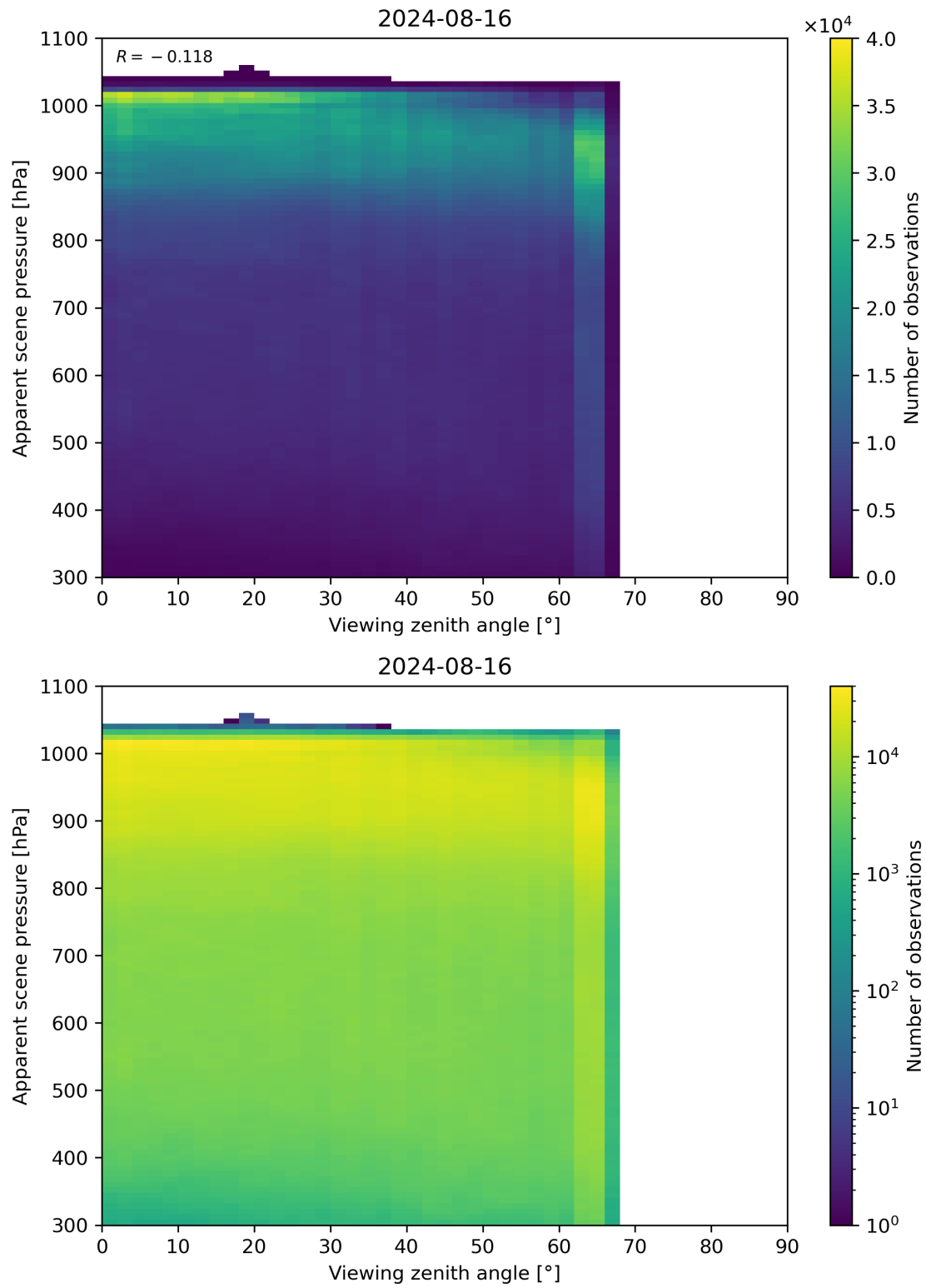
Figure 118: Scatter density plot of “Viewing zenith angle” against “Apparent scene pressure” for 2024-08-16 to 2024-08-17.
