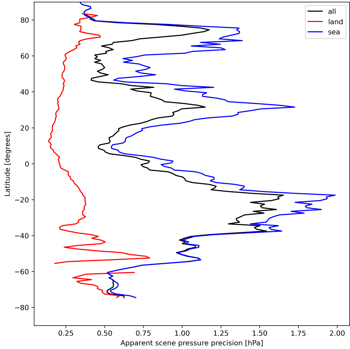
Figure 20: Zonal average of “Apparent scene pressure precision” for 2024-08-16 to 2024-08-17.
