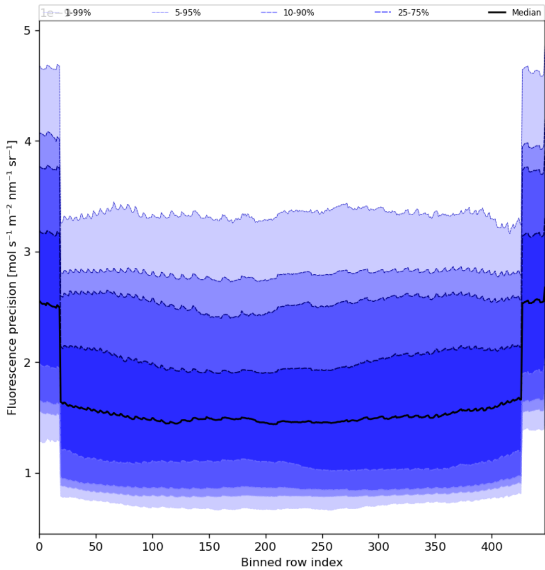
Figure 58: Along track statistics of “Fluorescence precision” for 2024-08-16 to 2024-08-17
