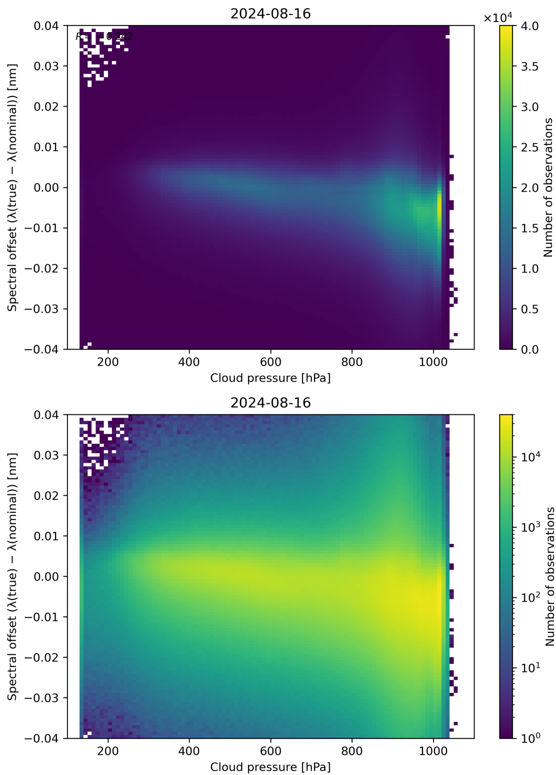
Figure 84: Scatter density plot of “Cloud pressure” against “Spectral offset ( \lambda(\text{true}) - \lambda(\text{nominal}) )” for 2024-08-16 to 2024-08-17.
