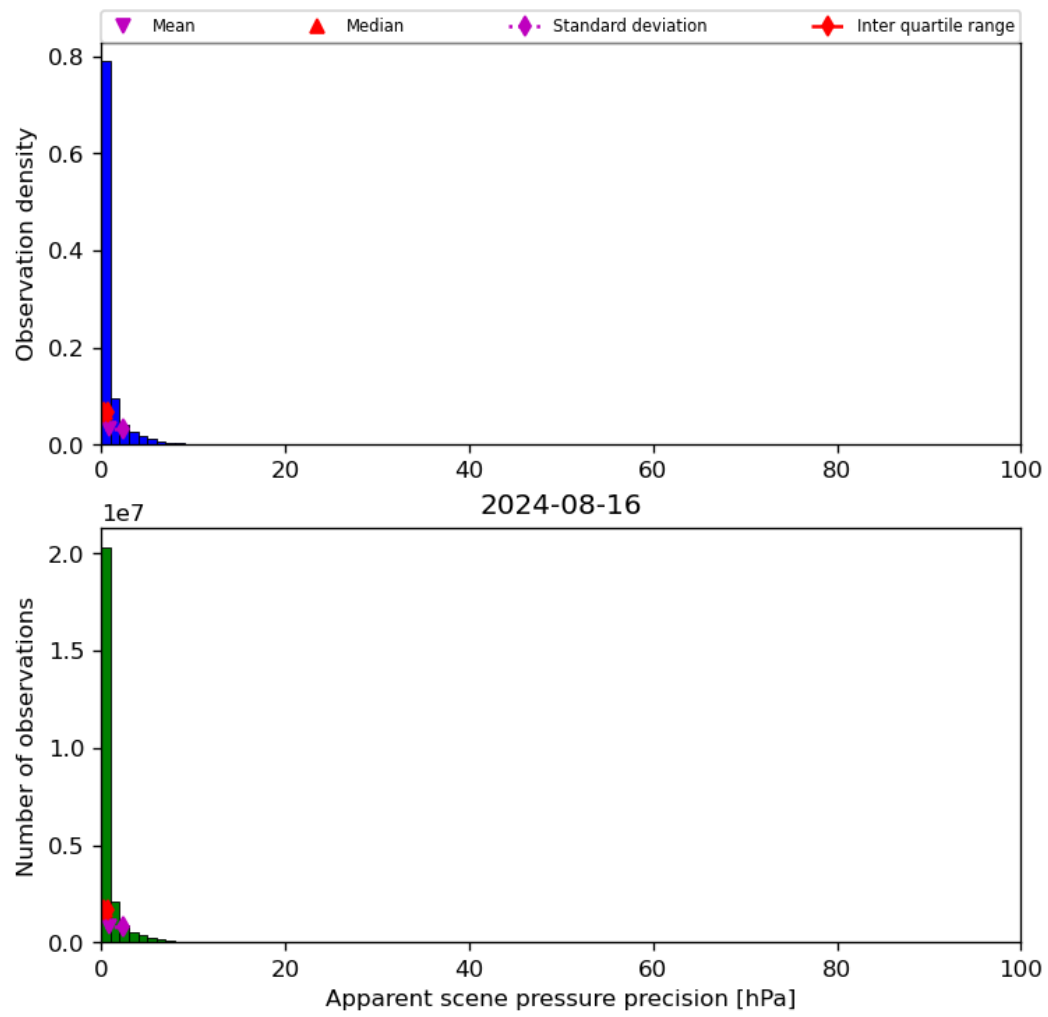
Figure 37: Histogram of “Apparent scene pressure precision” for 2024-08-16 to 2024-08-17
