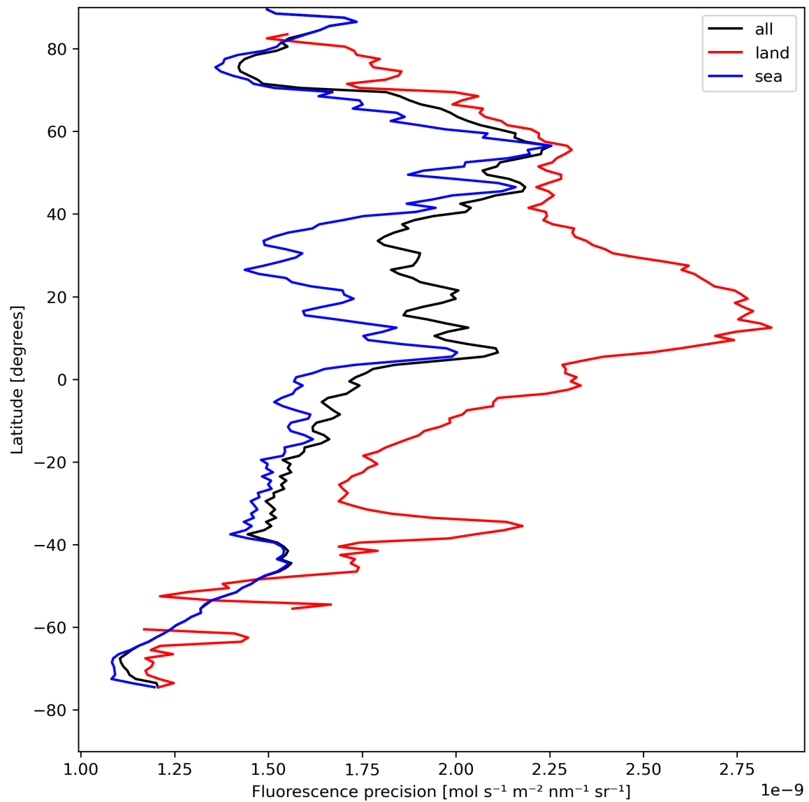
Figure 24: Zonal average of “Fluorescence precision” for 2024-08-16 to 2024-08-17.
