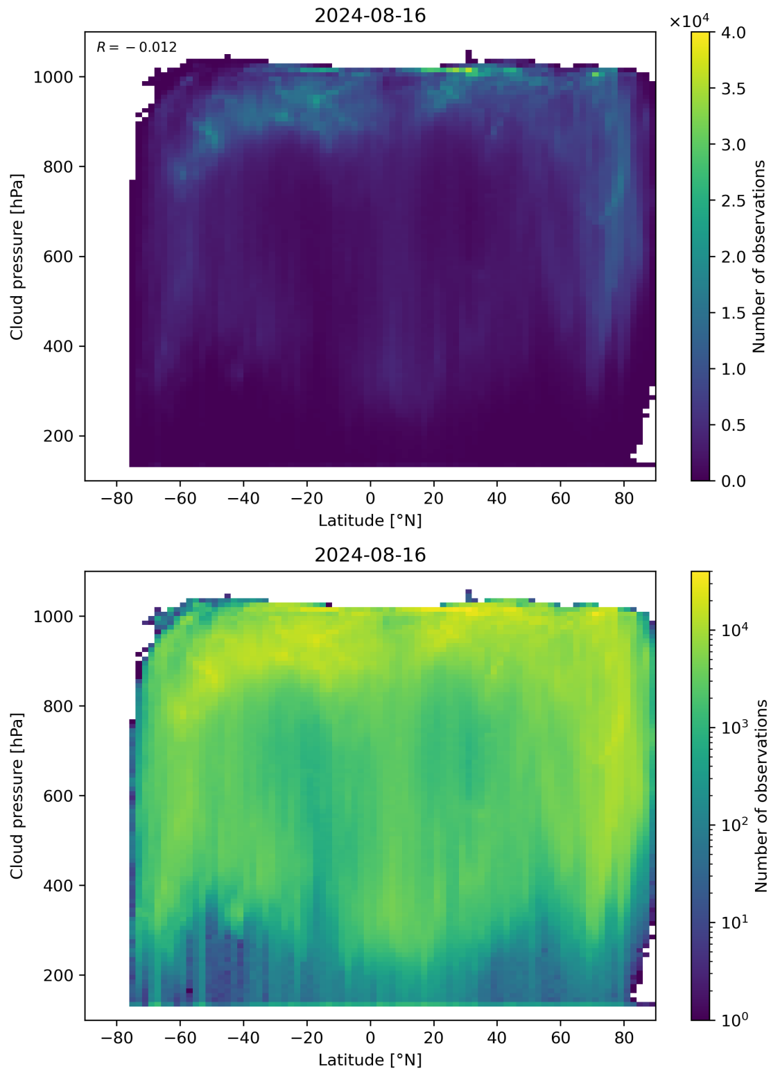
Figure 91: Scatter density plot of “Latitude” against “Cloud pressure” for 2024-08-16 to 2024-08-17.
