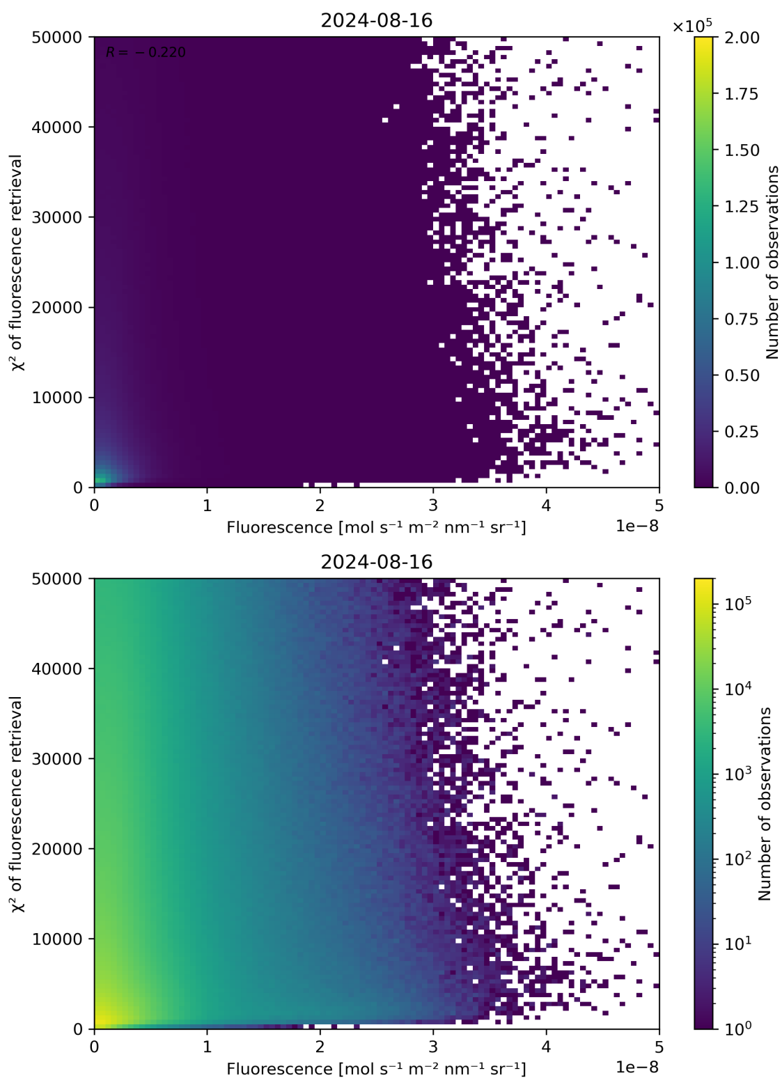
Figure 85: Scatter density plot of “Fluorescence” against “ \chi^2 of fluorescence retrieval” for 2024-08-16 to 2024-08-17.
