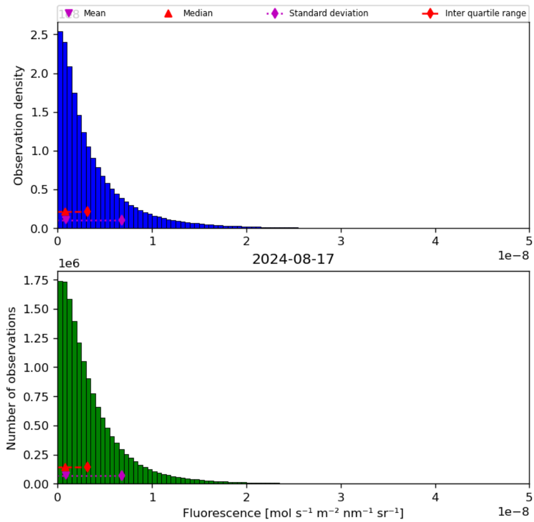
Figure 40: Histogram of “Fluorescence” for 2024-08-16 to 2024-08-18
