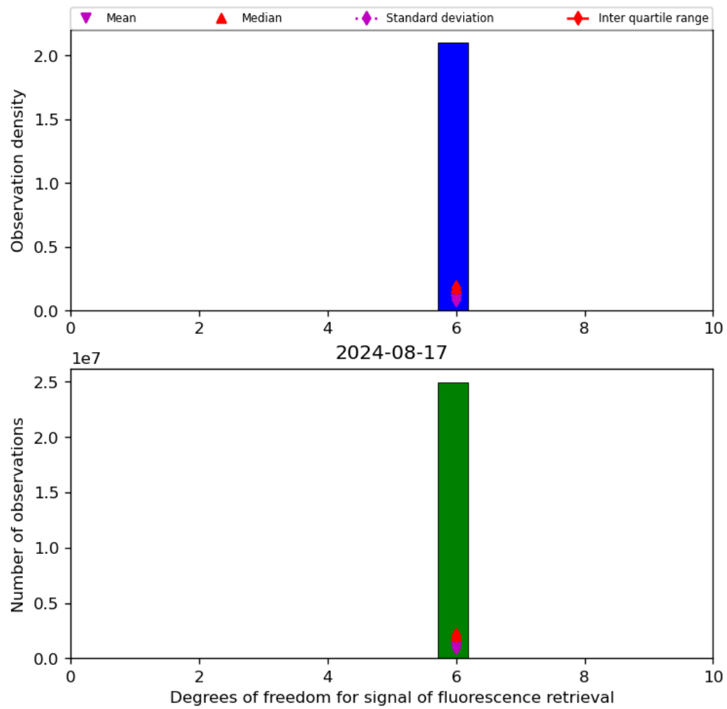
Figure 43: Histogram of “Degrees of freedom for signal of fluorescence retrieval” for 2024-08-16 to 2024-08-18
