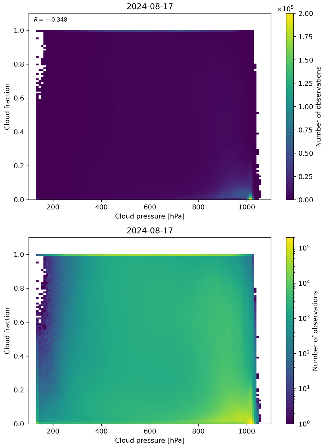
Figure 79: Scatter density plot of “Cloud pressure” against “Cloud fraction” for 2024-08-16 to 2024-08-18.
