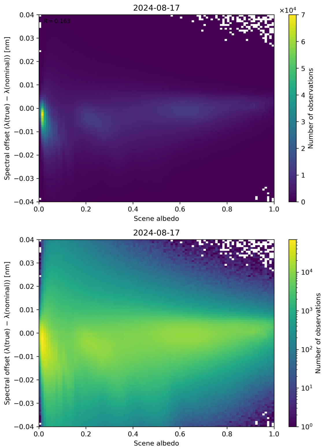
Figure 107: Scatter density plot of “Scene albedo” against “Spectral offset ( \lambda(\text{true}) - \lambda(\text{nominal}) )” for 2024-08-16 to 2024-08-18.
