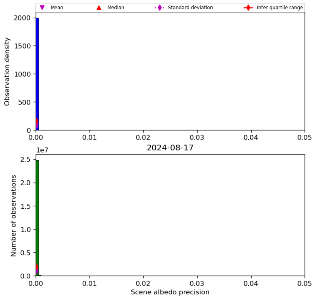
Figure 35: Histogram of “Scene albedo precision” for 2024-08-16 to 2024-08-18
