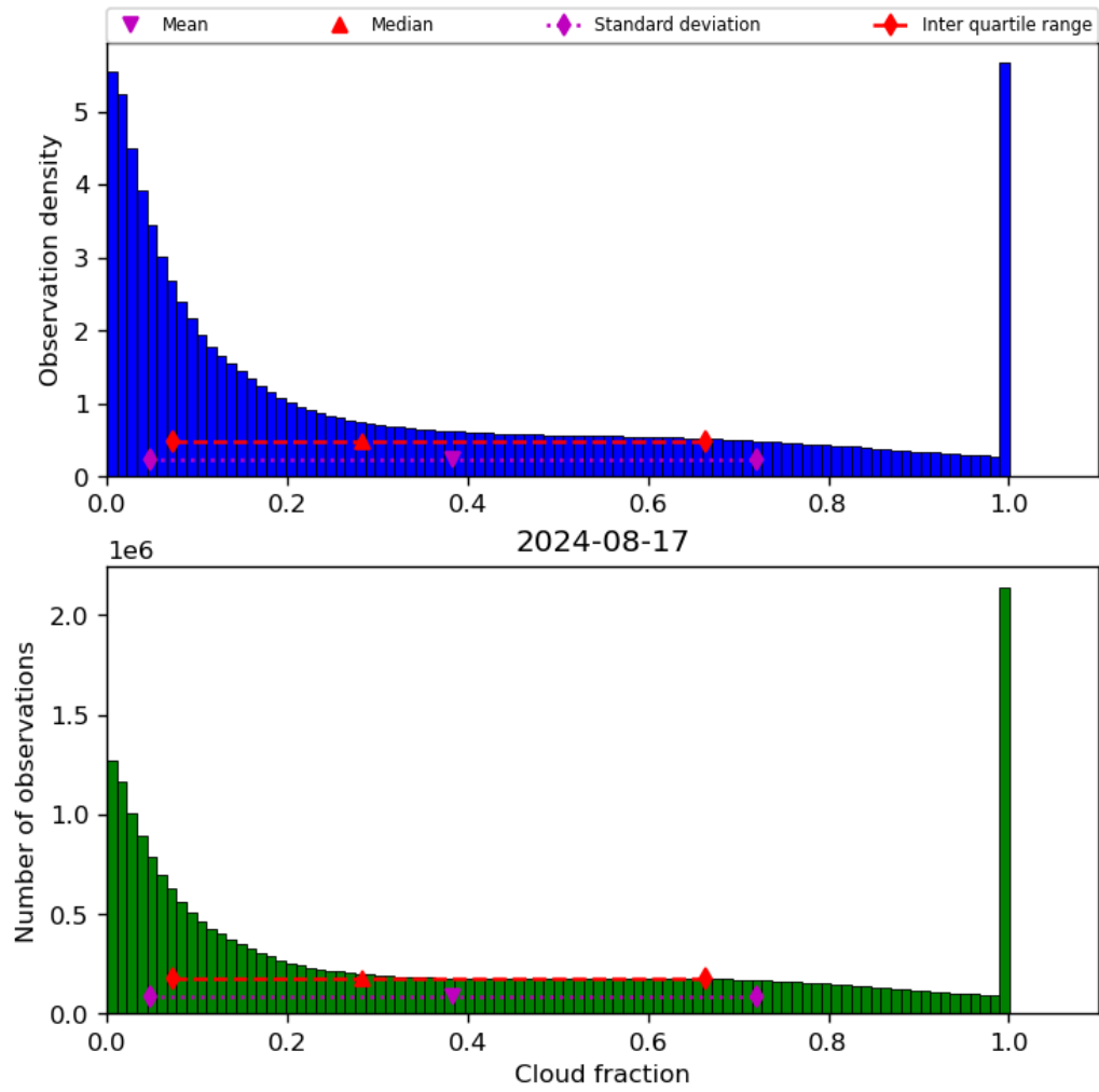
Figure 32: Histogram of “Cloud fraction” for 2024-08-16 to 2024-08-18
