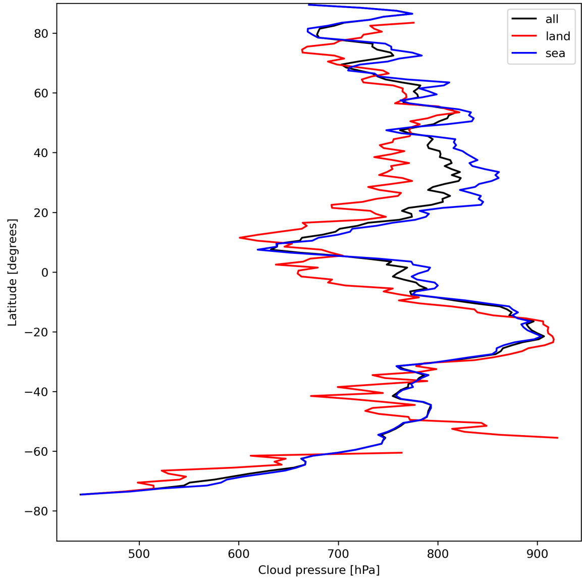
Figure 13: Zonal average of “Cloud pressure” for 2024-08-16 to 2024-08-18.
