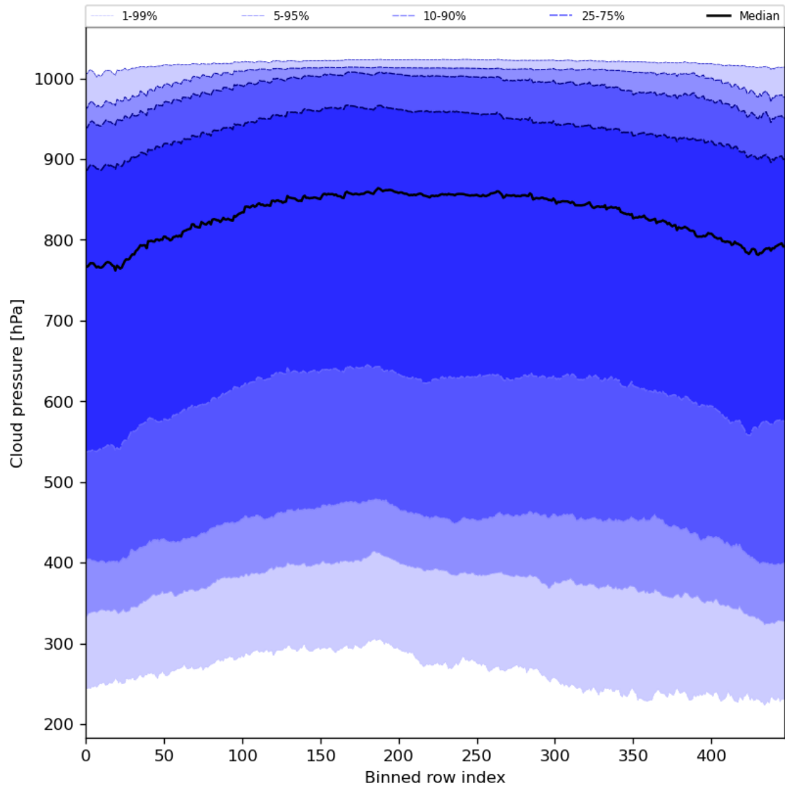
Figure 47: Along track statistics of “Cloud pressure” for 2024-08-16 to 2024-08-18
