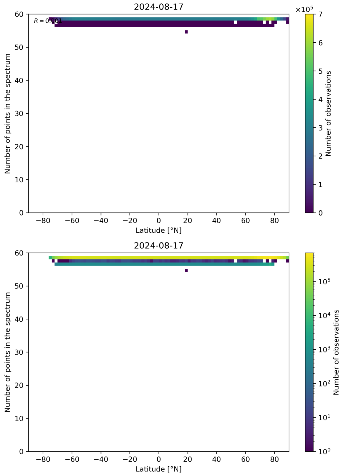
Figure 94: Scatter density plot of “Latitude” against “Number of points in the spectrum” for 2024-08-16 to 2024-08-18.
