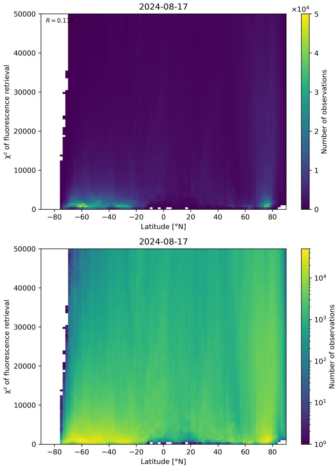
Figure 89: Scatter density plot of “Latitude” against “ \chi^2 of fluorescence retrieval” for 2024-08-16 to 2024-08-18.
