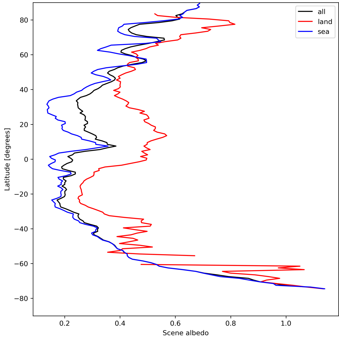
Figure 17: Zonal average of “Scene albedo” for 2024-08-16 to 2024-08-18.
