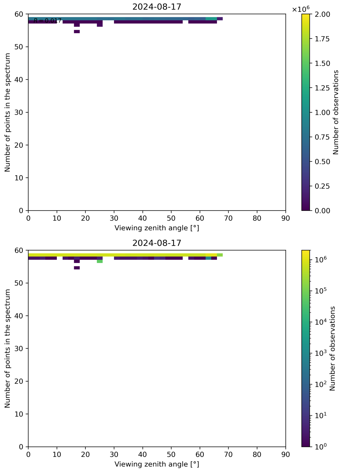
Figure 125: Scatter density plot of “Viewing zenith angle” against “Number of points in the spectrum” for 2024-08-16 to 2024-08-18.
