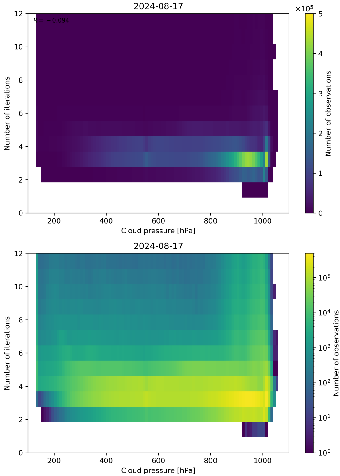
Figure 81: Scatter density plot of “Cloud pressure” against “Number of iterations” for 2024-08-16 to 2024-08-18.
