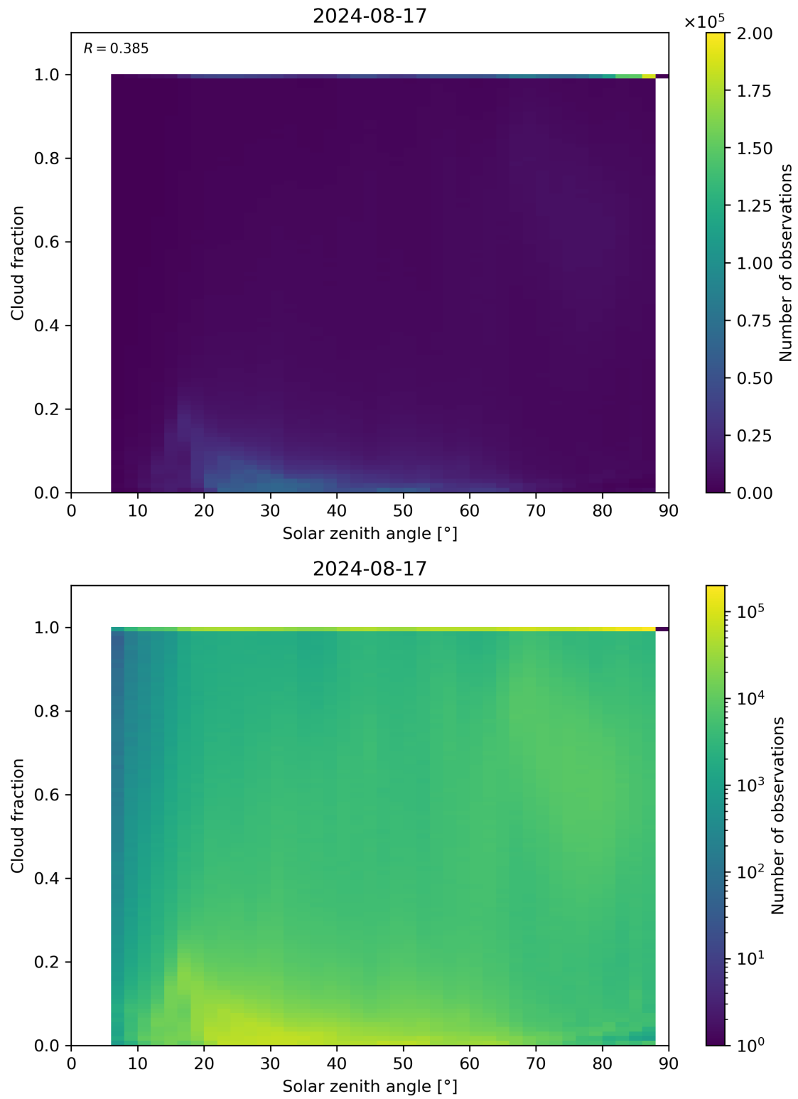
Figure 110: Scatter density plot of “Solar zenith angle” against “Cloud fraction” for 2024-08-16 to 2024-08-18.
