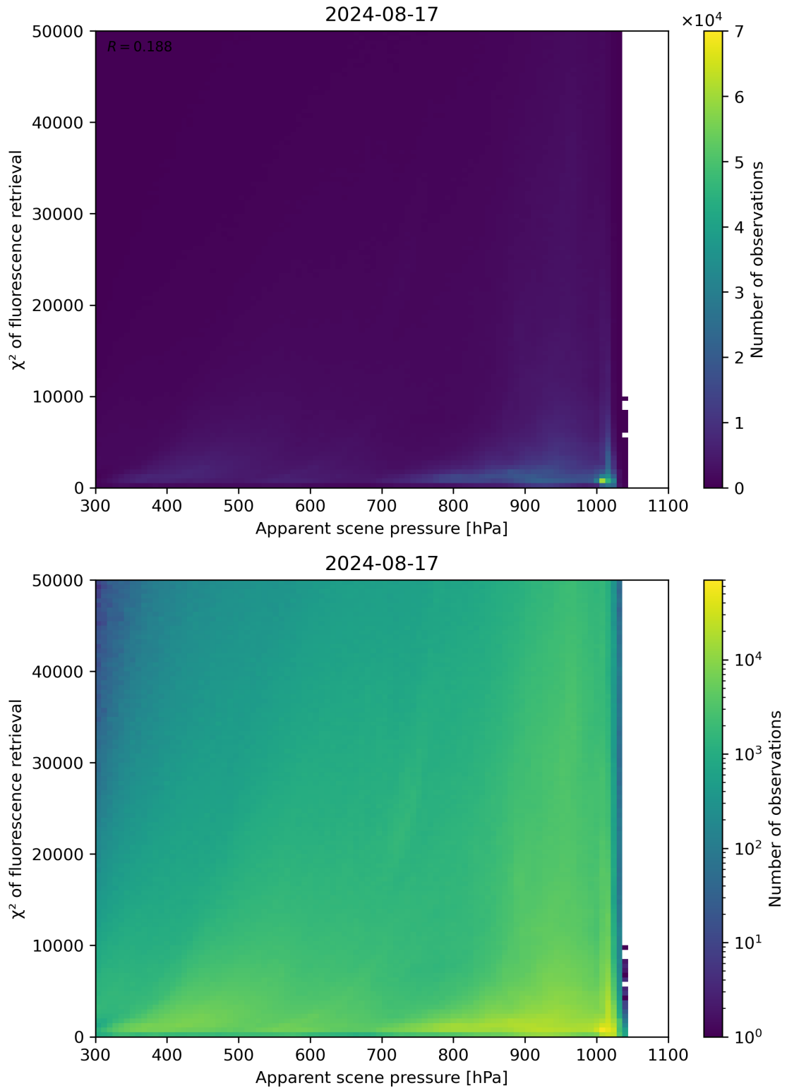
Figure 63: Scatter density plot of “Apparent scene pressure” against “ \chi^2 of fluorescence retrieval” for 2024-08-16 to 2024-08-18.
