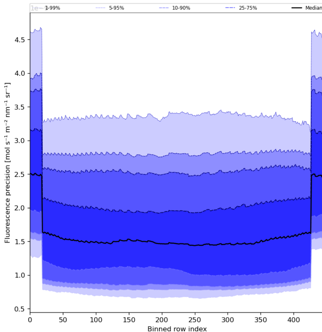
Figure 58: Along track statistics of “Fluorescence precision” for 2024-08-16 to 2024-08-18
