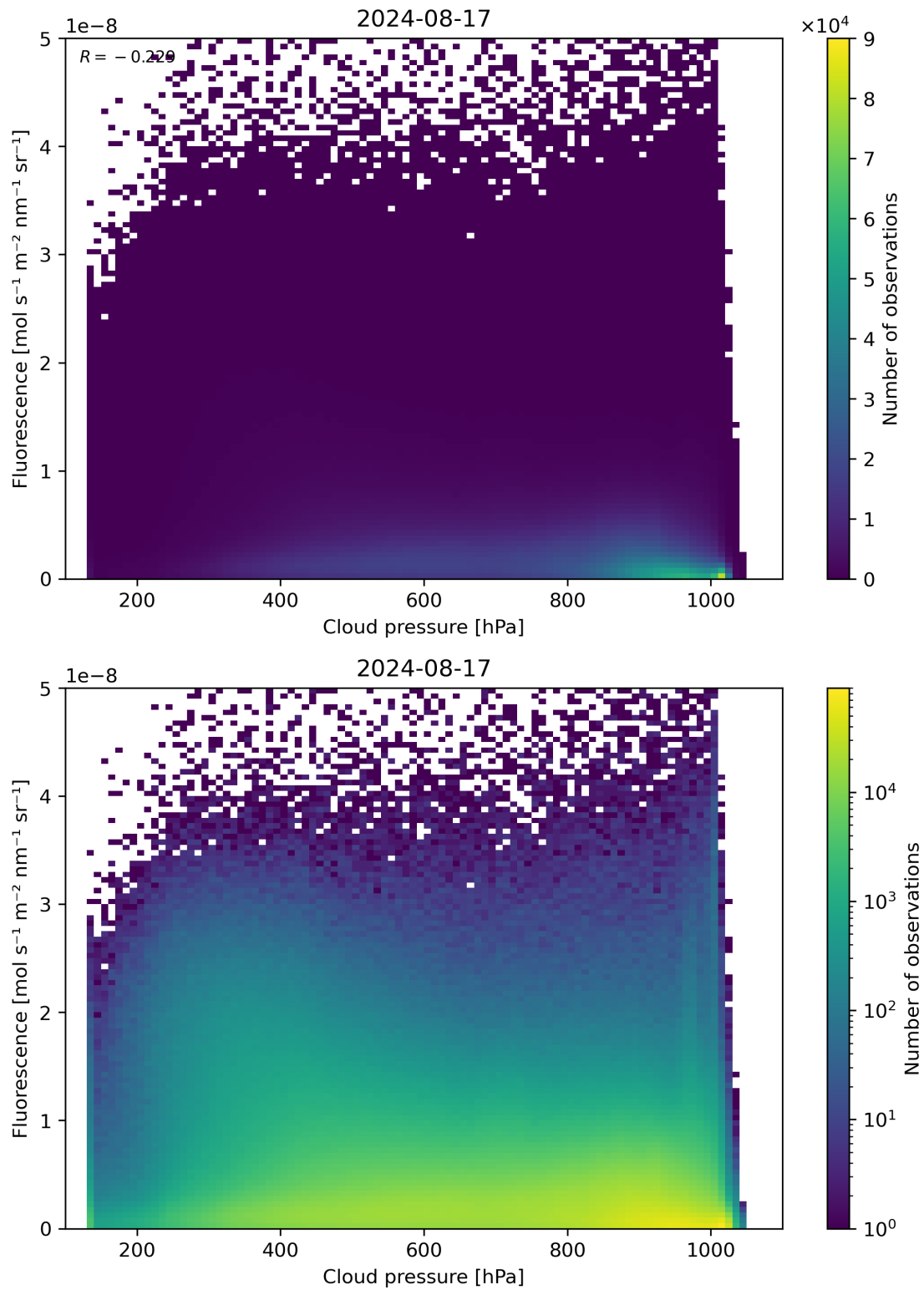
Figure 80: Scatter density plot of “Cloud pressure” against “Fluorescence” for 2024-08-16 to 2024-08-18.
