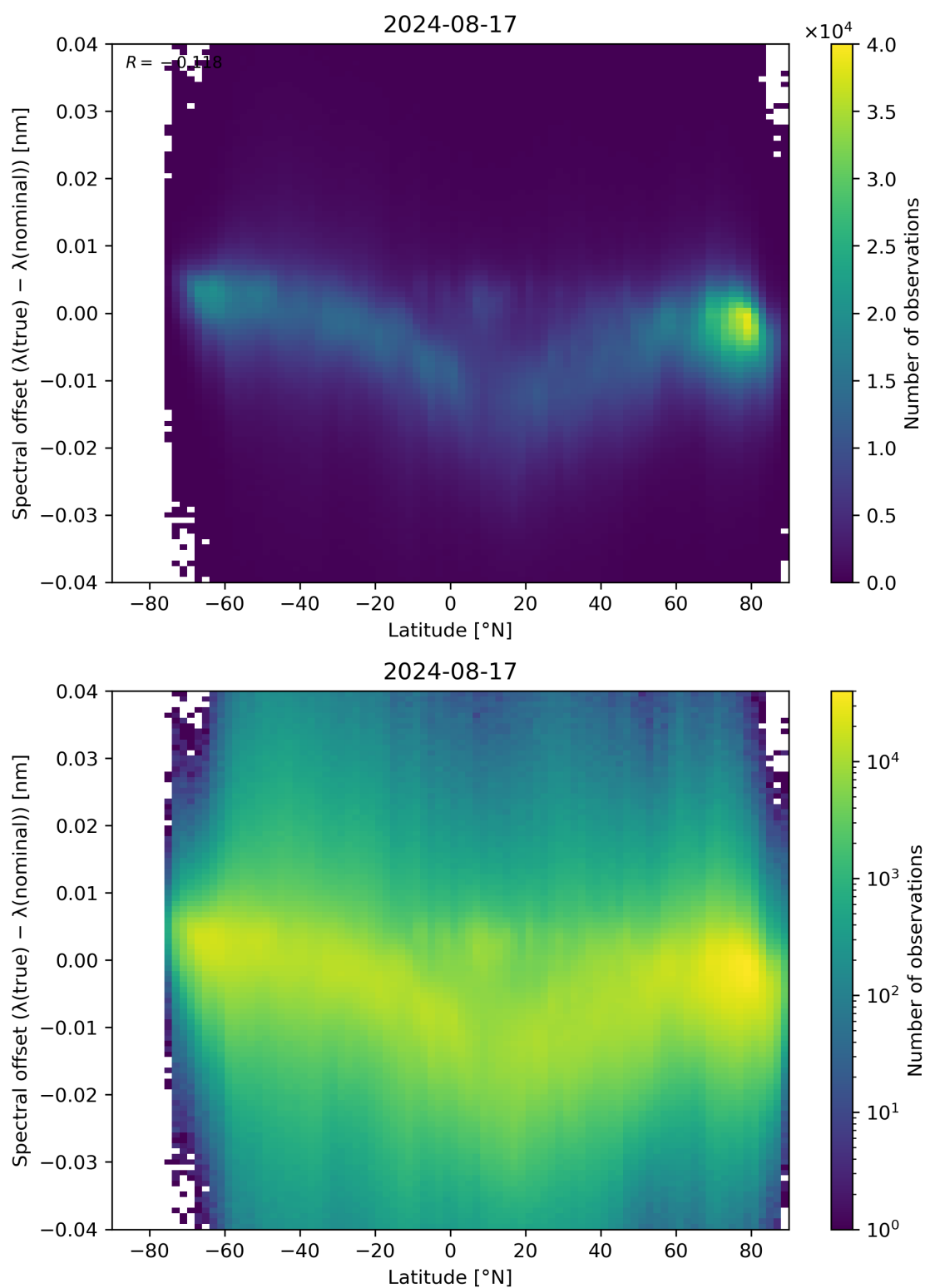
Figure 96: Scatter density plot of “Latitude” against “Spectral offset ( \lambda(\text{true}) - \lambda(\text{nominal}) )” for 2024-08-16 to 2024-08-18.
