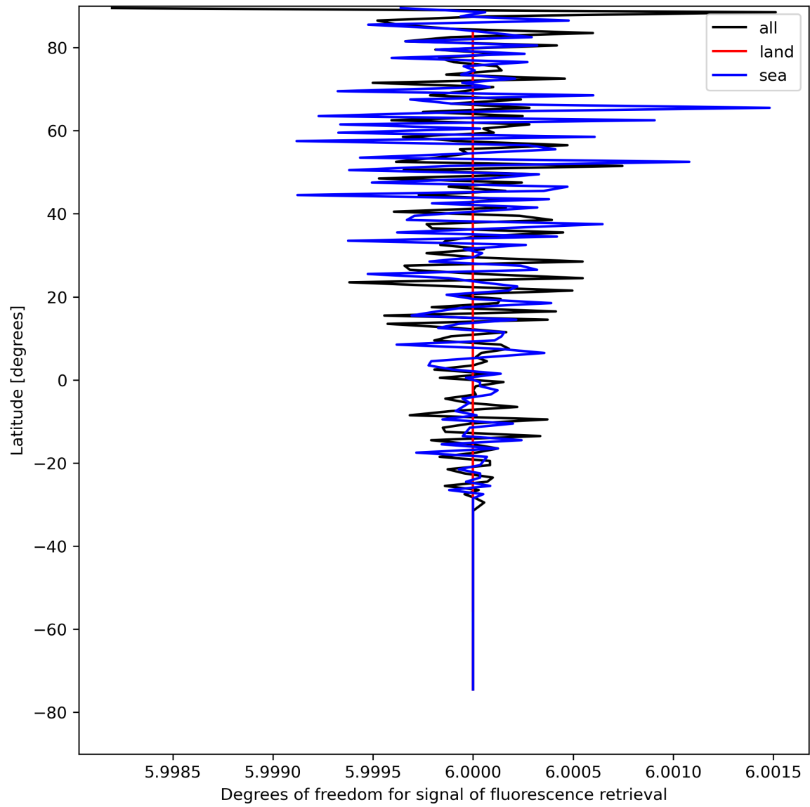
Figure 26: Zonal average of “Degrees of freedom for signal of fluorescence retrieval” for 2024-08-16 to 2024-08-18.
