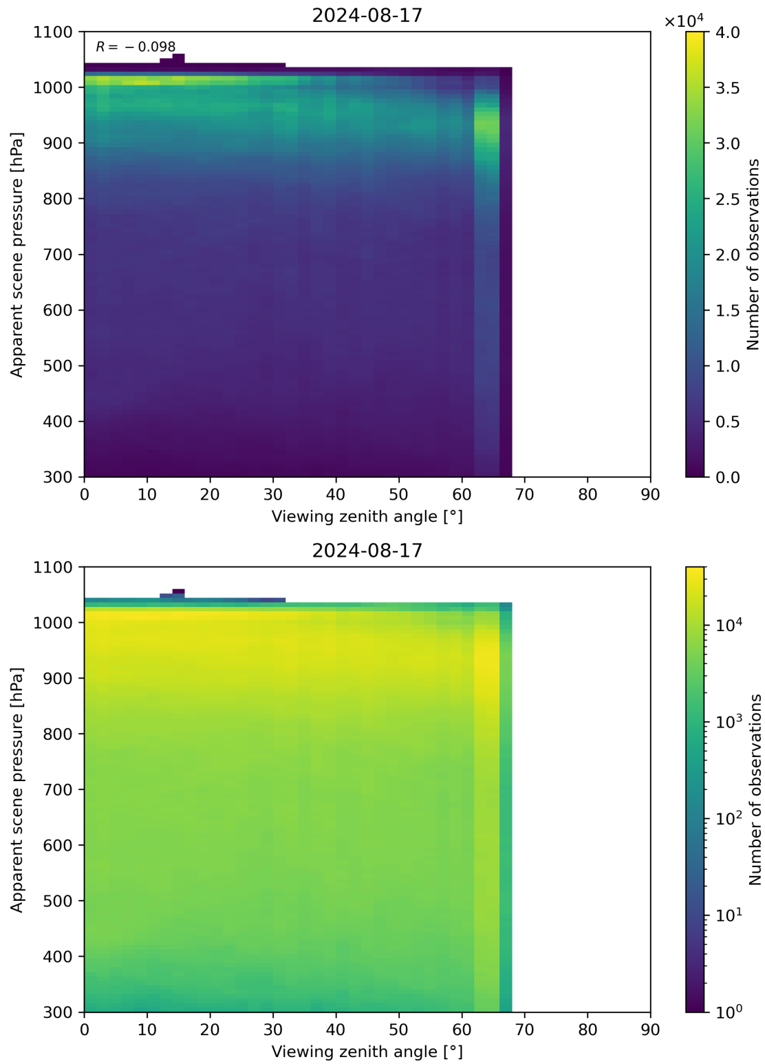
Figure 118: Scatter density plot of “Viewing zenith angle” against “Apparent scene pressure” for 2024-08-16 to 2024-08-18.
