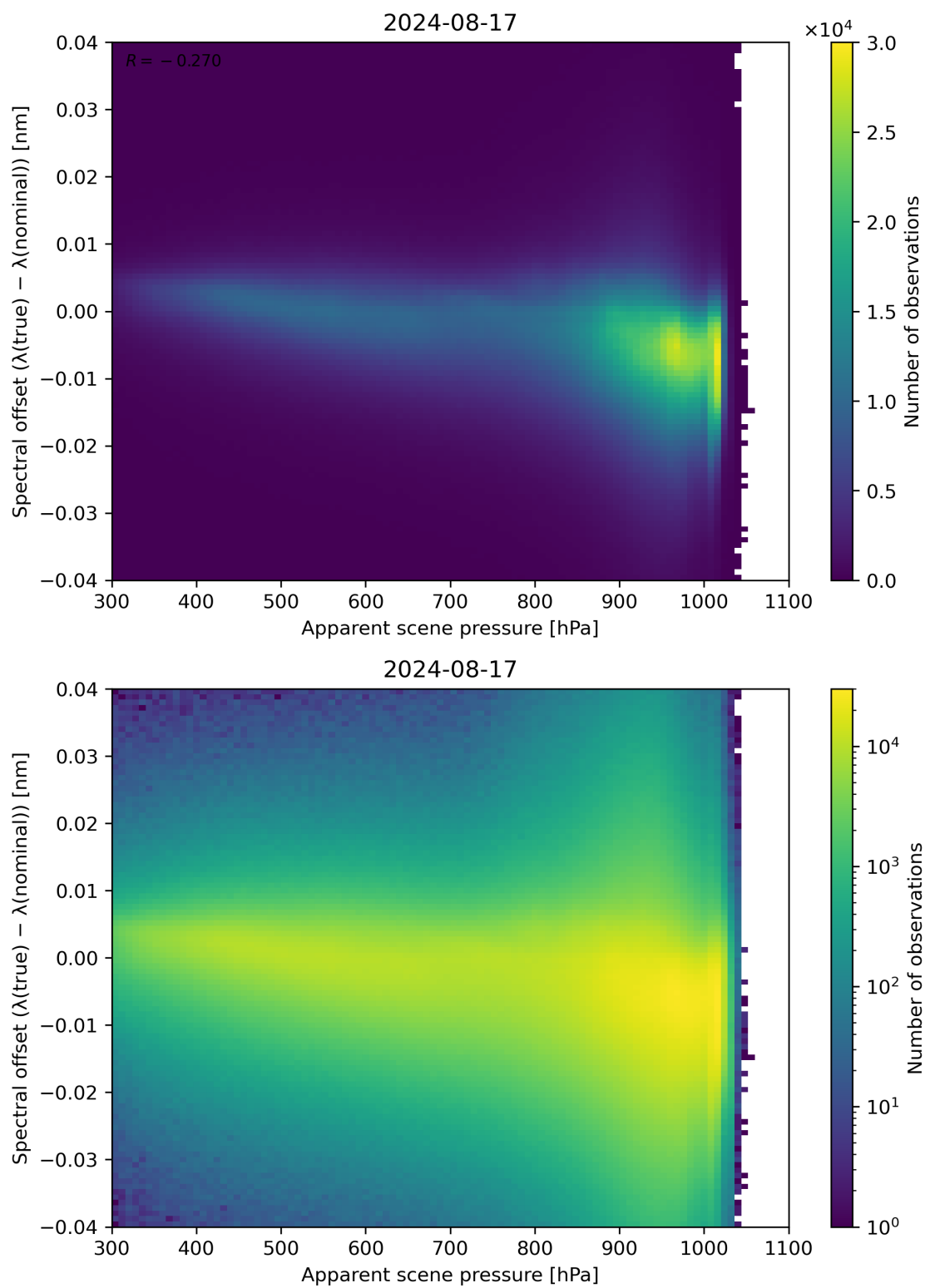
Figure 67: Scatter density plot of “Apparent scene pressure” against “Spectral offset ( \lambda(\text{true}) - \lambda(\text{nominal}) )” for 2024-08-16 to 2024-08-18.
