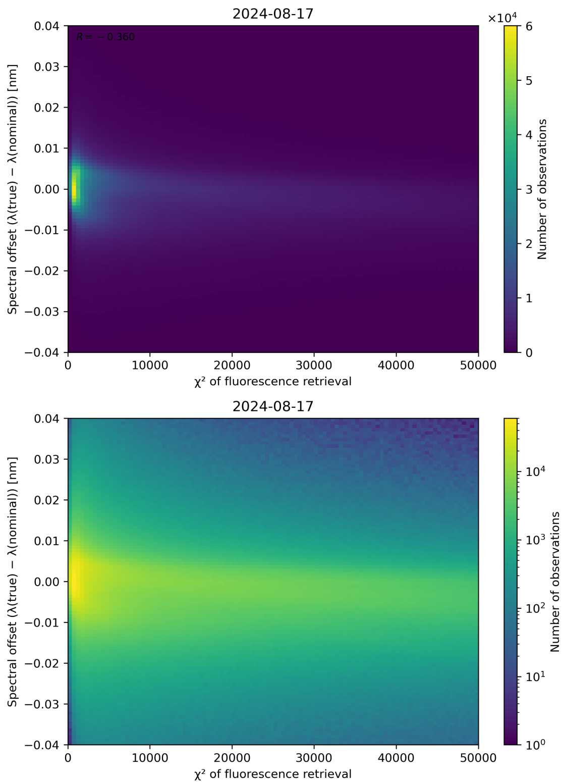
Figure 69: Scatter density plot of " \chi^2 of fluorescence retrieval" against "Spectral offset ( \lambda(\text{true}) - \lambda(\text{nominal})) " for 2024-08-16 to 2024-08-18.
