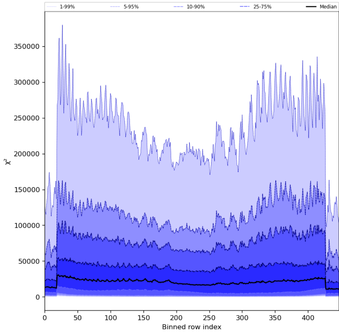
Figure 55: Along track statistics of “ \chi^2 ” for 2024-08-16 to 2024-08-18
