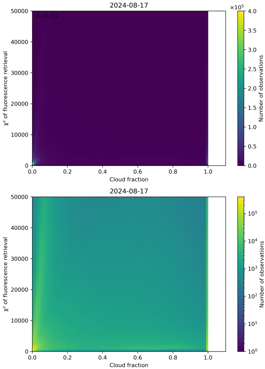
Figure 71: Scatter density plot of “Cloud fraction” against “ \chi^2 of fluorescence retrieval” for 2024-08-16 to 2024-08-18.
