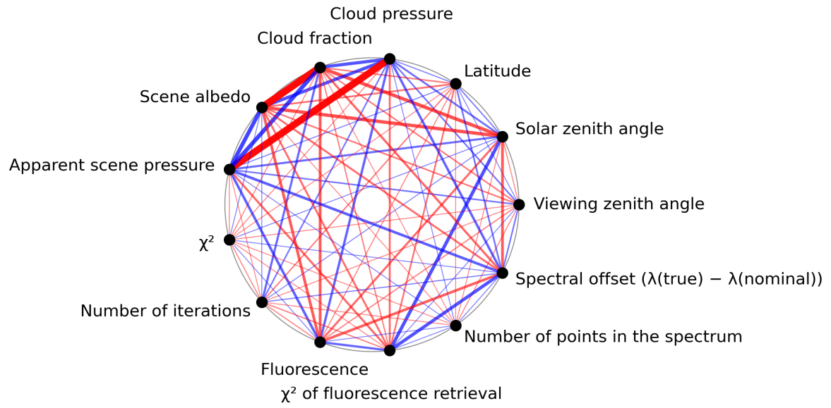
Figure 1: Map of correlation graph for 2024-08-16 to 2024-08-18.
