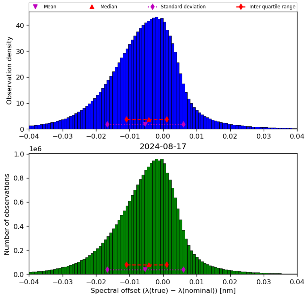
Figure 45: Histogram of “Spectral offset ( \lambda(\text{true}) - \lambda(\text{nominal}) )” for 2024-08-16 to 2024-08-18
