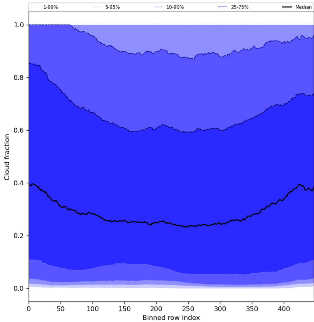
Figure 49: Along track statistics of “Cloud fraction” for 2024-08-16 to 2024-08-18
