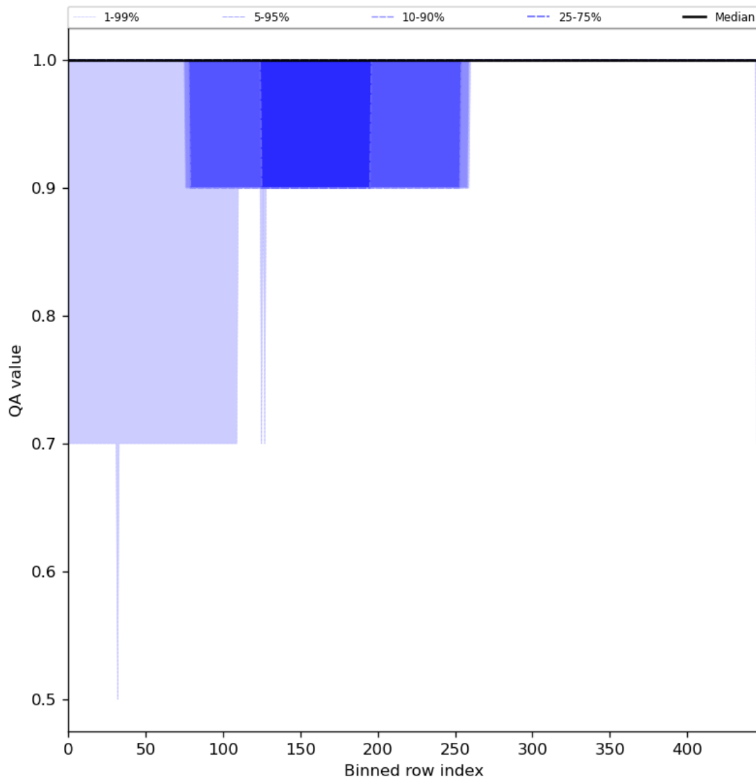
Figure 46: Along track statistics of “QA value” for 2024-08-16 to 2024-08-18
