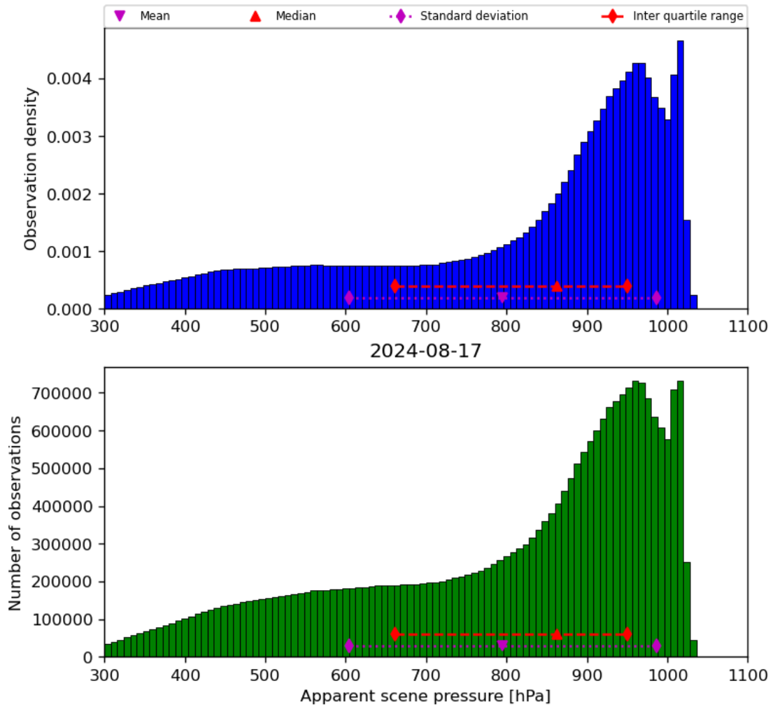
Figure 36: Histogram of “Apparent scene pressure” for 2024-08-16 to 2024-08-18
