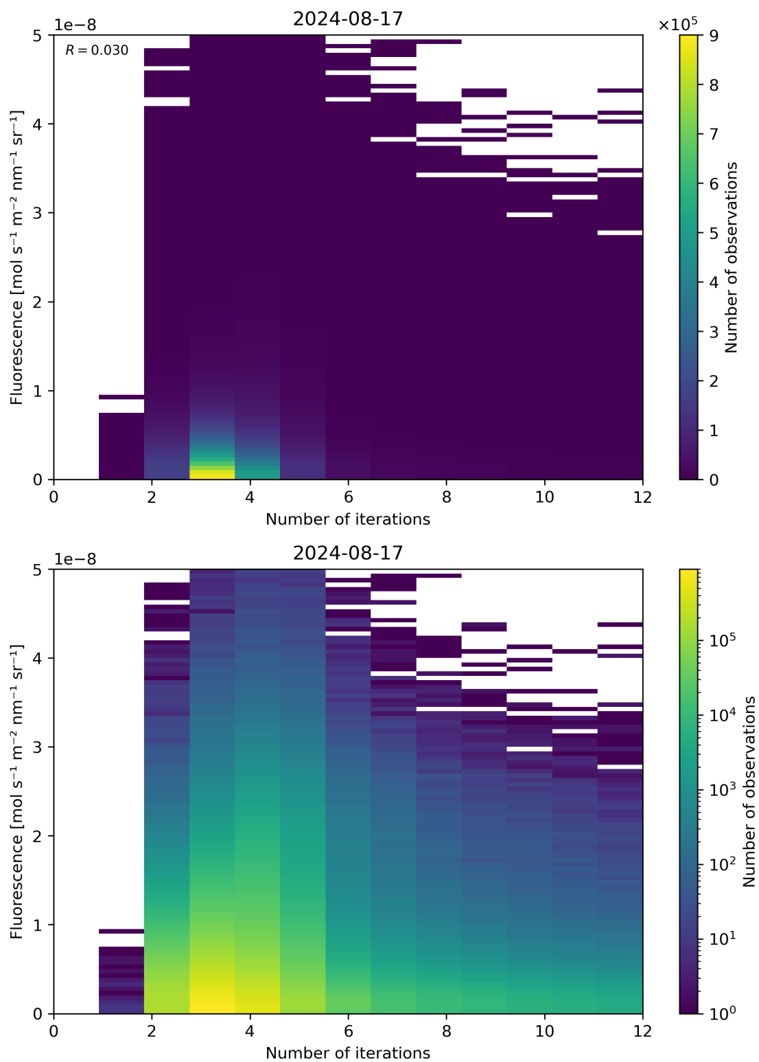
Figure 98: Scatter density plot of “Number of iterations” against “Fluorescence” for 2024-08-16 to 2024-08-18.
