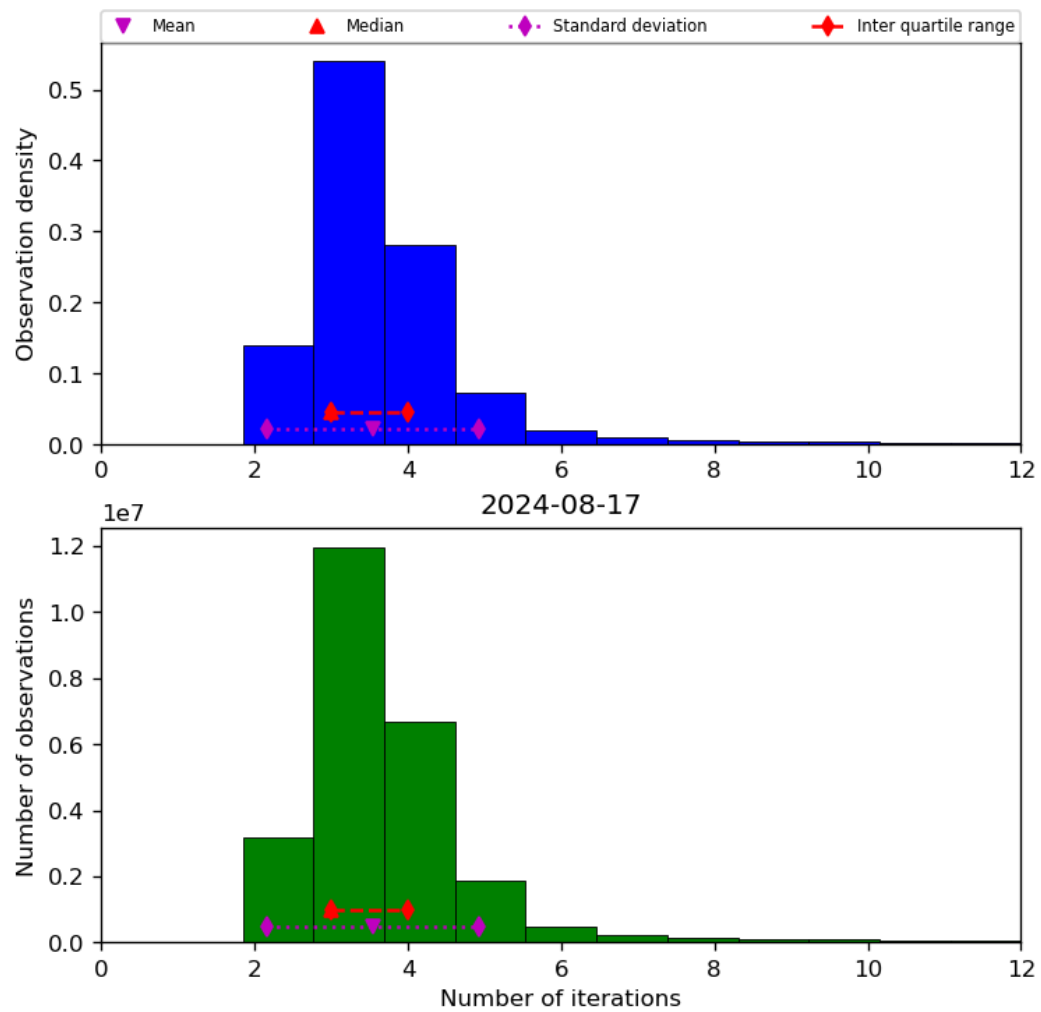
Figure 39: Histogram of “Number of iterations” for 2024-08-16 to 2024-08-18
