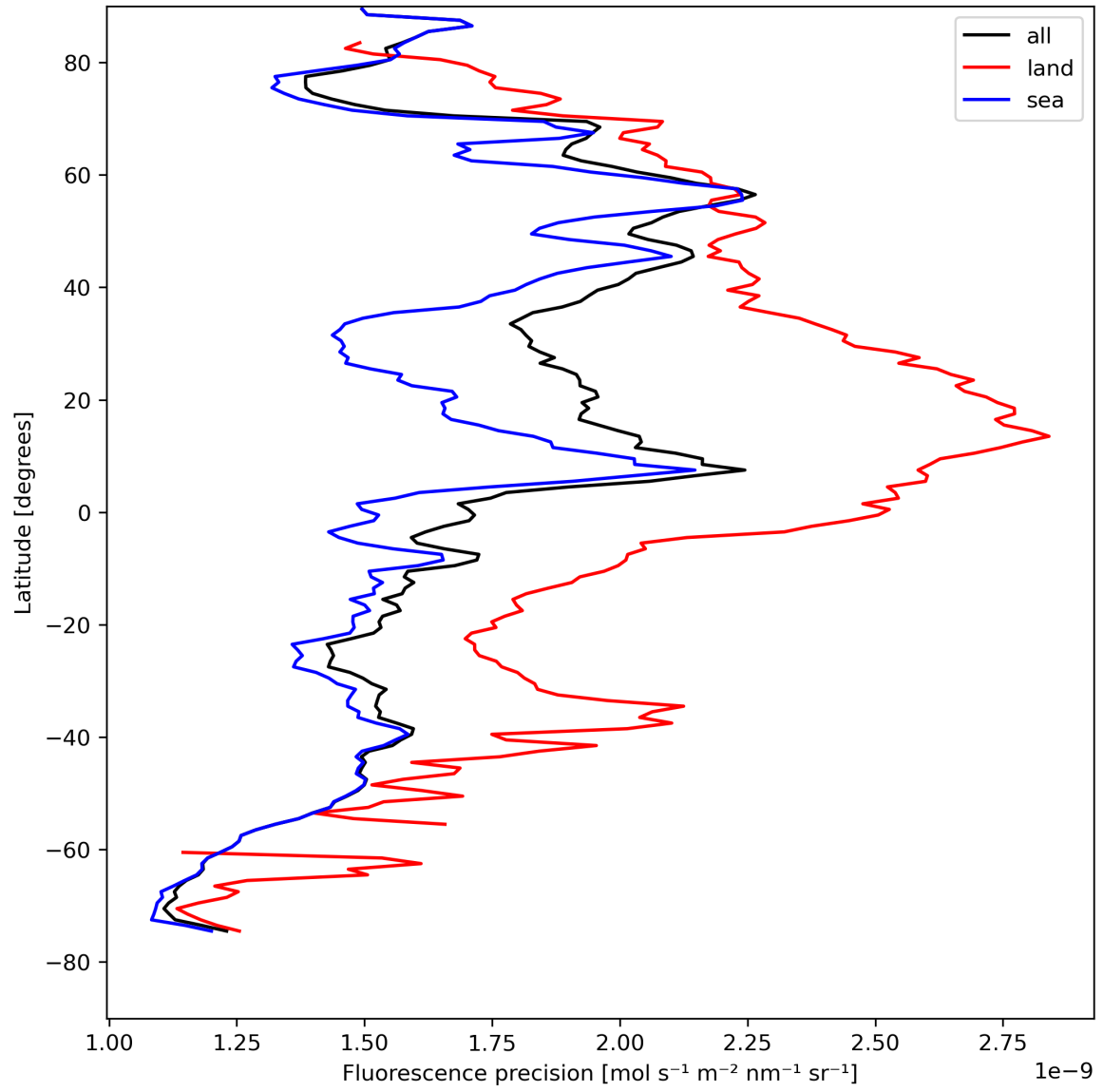
Figure 24: Zonal average of “Fluorescence precision” for 2024-08-16 to 2024-08-18.
