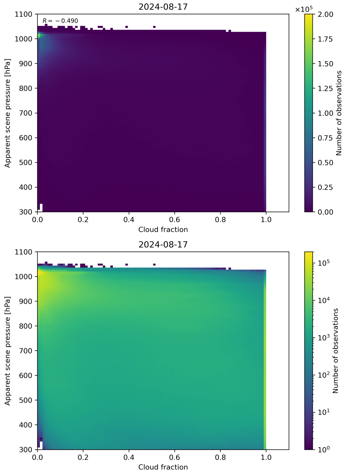
Figure 70: Scatter density plot of “Cloud fraction” against “Apparent scene pressure” for 2024-08-16 to 2024-08-18.
