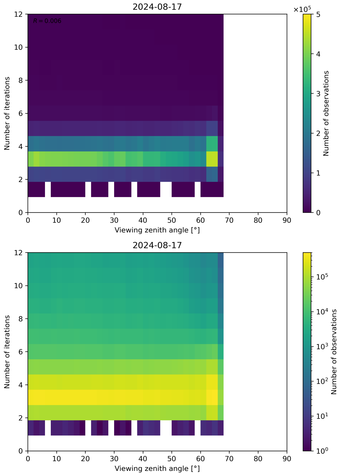
Figure 124: Scatter density plot of “Viewing zenith angle” against “Number of iterations” for 2024-08-16 to 2024-08-18.
