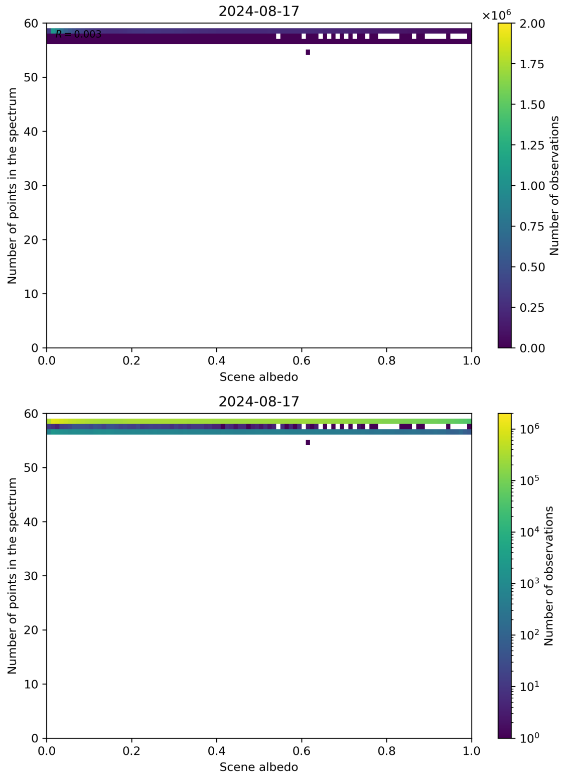
Figure 106: Scatter density plot of “Scene albedo” against “Number of points in the spectrum” for 2024-08-16 to 2024-08-18.
