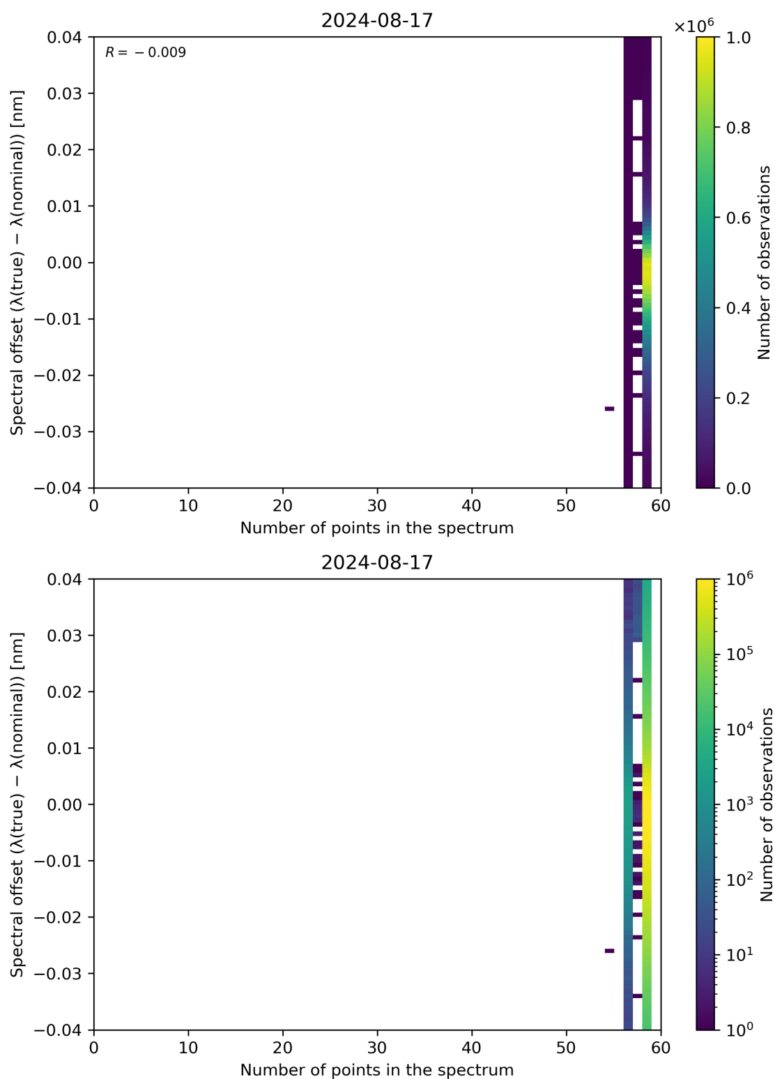
Figure 101: Scatter density plot of “Number of points in the spectrum” against “Spectral offset ( \lambda(\text{true}) - \lambda(\text{nominal}) )” for 2024-08-16 to 2024-08-18.
