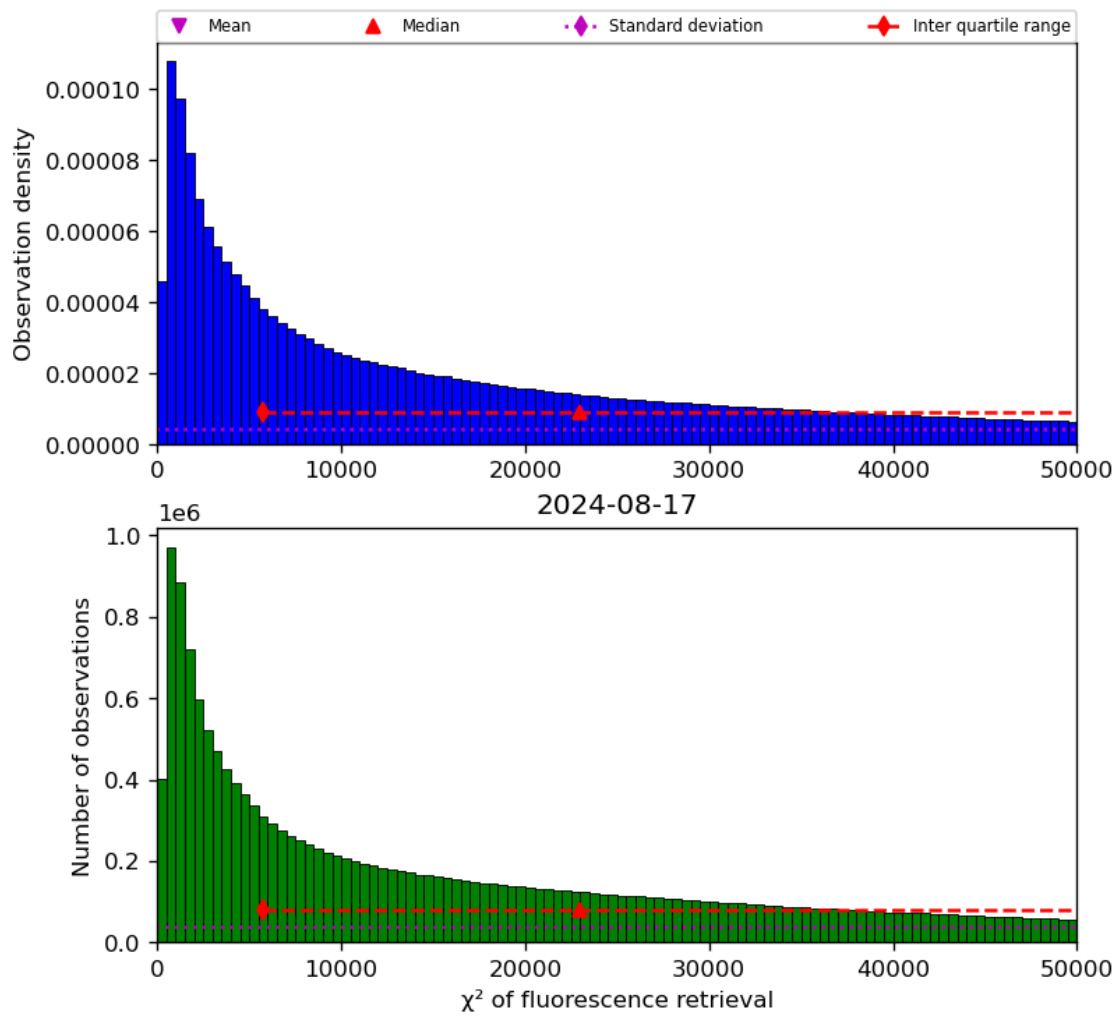
Figure 42: Histogram of “ \chi^2 of fluorescence retrieval” for 2024-08-16 to 2024-08-18
