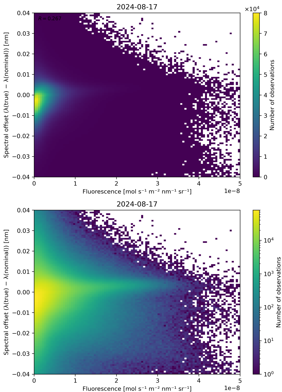
Figure 87: Scatter density plot of “Fluorescence” against “Spectral offset ( \lambda(\text{true}) - \lambda(\text{nominal}) )” for 2024-08-16 to 2024-08-18.
