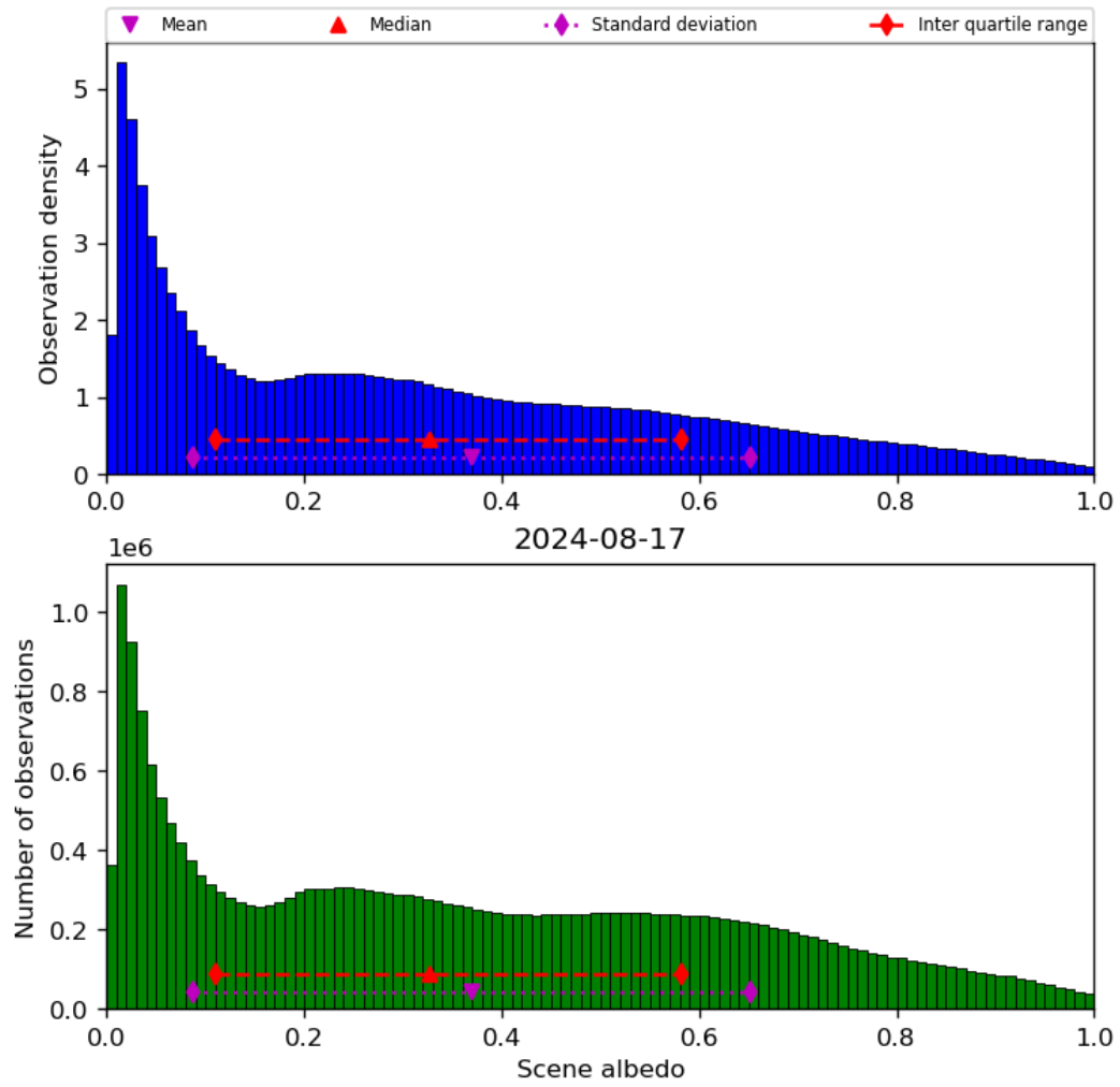
Figure 34: Histogram of “Scene albedo” for 2024-08-16 to 2024-08-18
