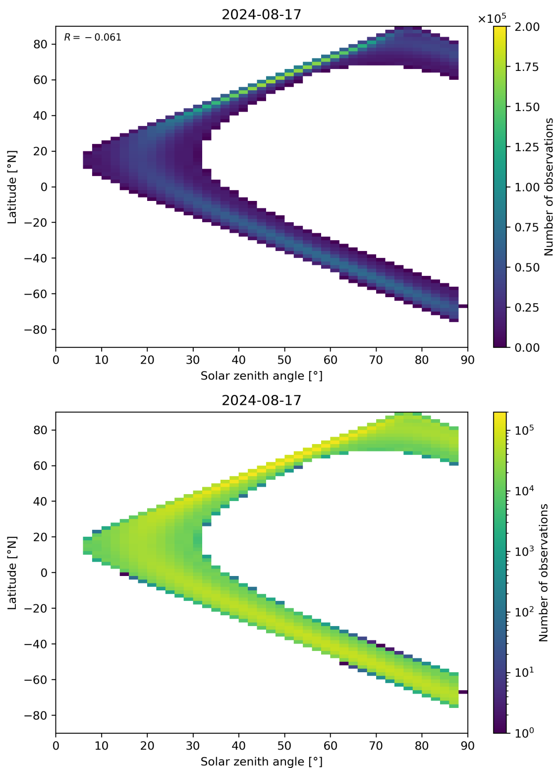
Figure 113: Scatter density plot of “Solar zenith angle” against “Latitude” for 2024-08-16 to 2024-08-18.
