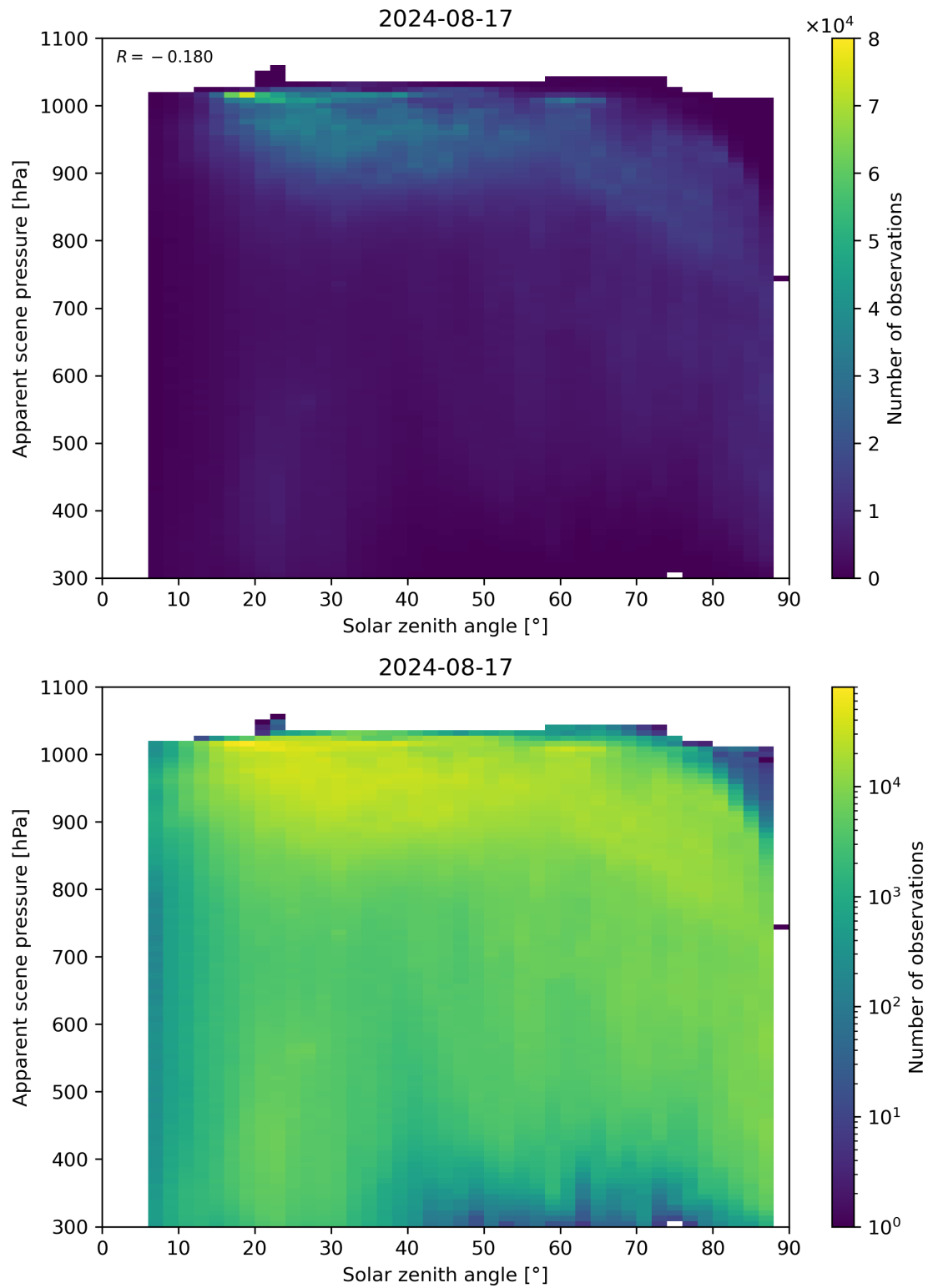
Figure 108: Scatter density plot of “Solar zenith angle” against “Apparent scene pressure” for 2024-08-16 to 2024-08-18.
