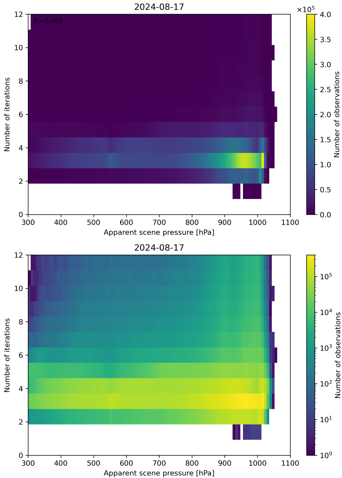
Figure 65: Scatter density plot of “Apparent scene pressure” against “Number of iterations” for 2024-08-16 to 2024-08-18.
