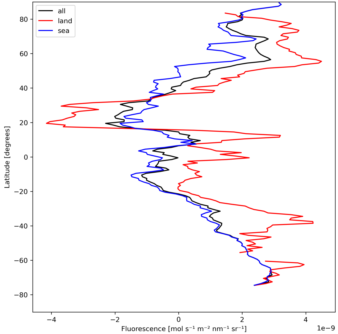
Figure 23: Zonal average of “Fluorescence” for 2024-08-16 to 2024-08-18.
