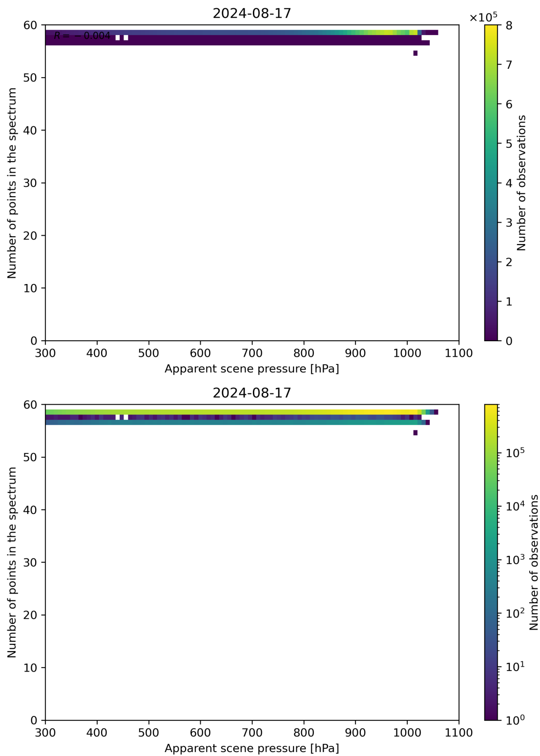
Figure 66: Scatter density plot of “Apparent scene pressure” against “Number of points in the spectrum” for 2024-08-16 to 2024-08-18.
