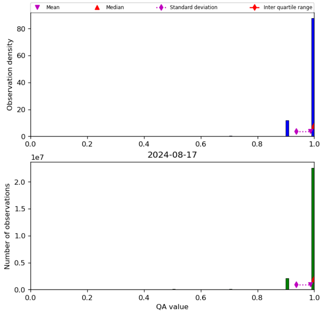
Figure 29: Histogram of “QA value” for 2024-08-16 to 2024-08-18
