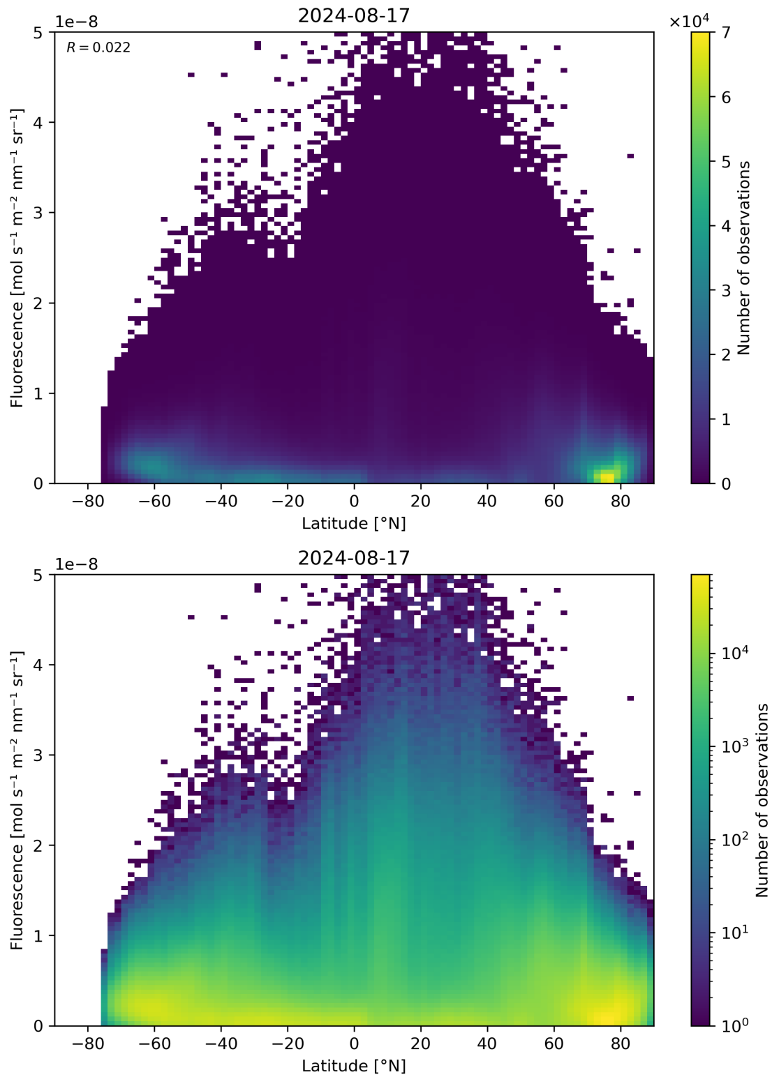
Figure 92: Scatter density plot of “Latitude” against “Fluorescence” for 2024-08-16 to 2024-08-18.
