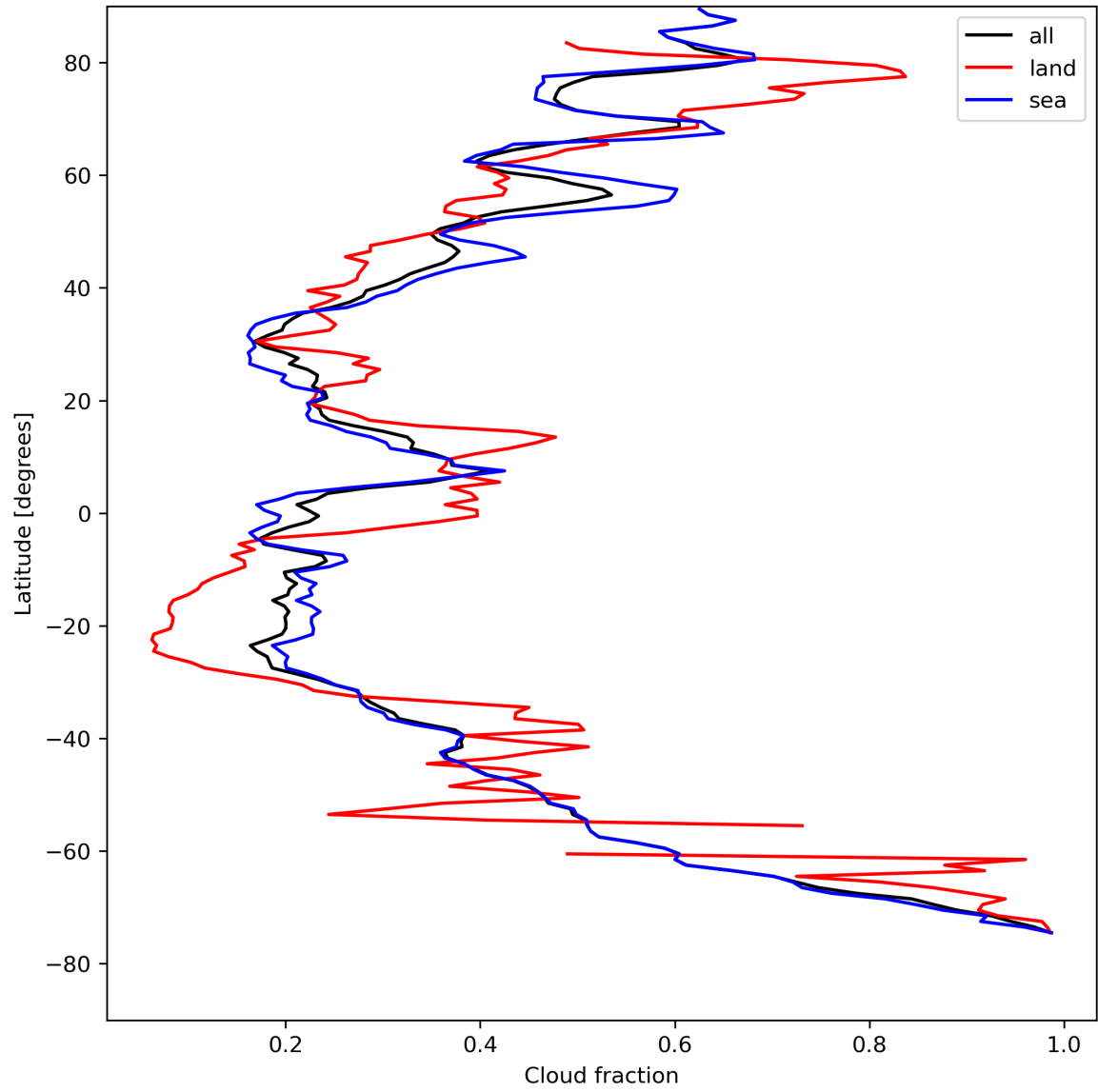
Figure 15: Zonal average of “Cloud fraction” for 2024-08-16 to 2024-08-18.
