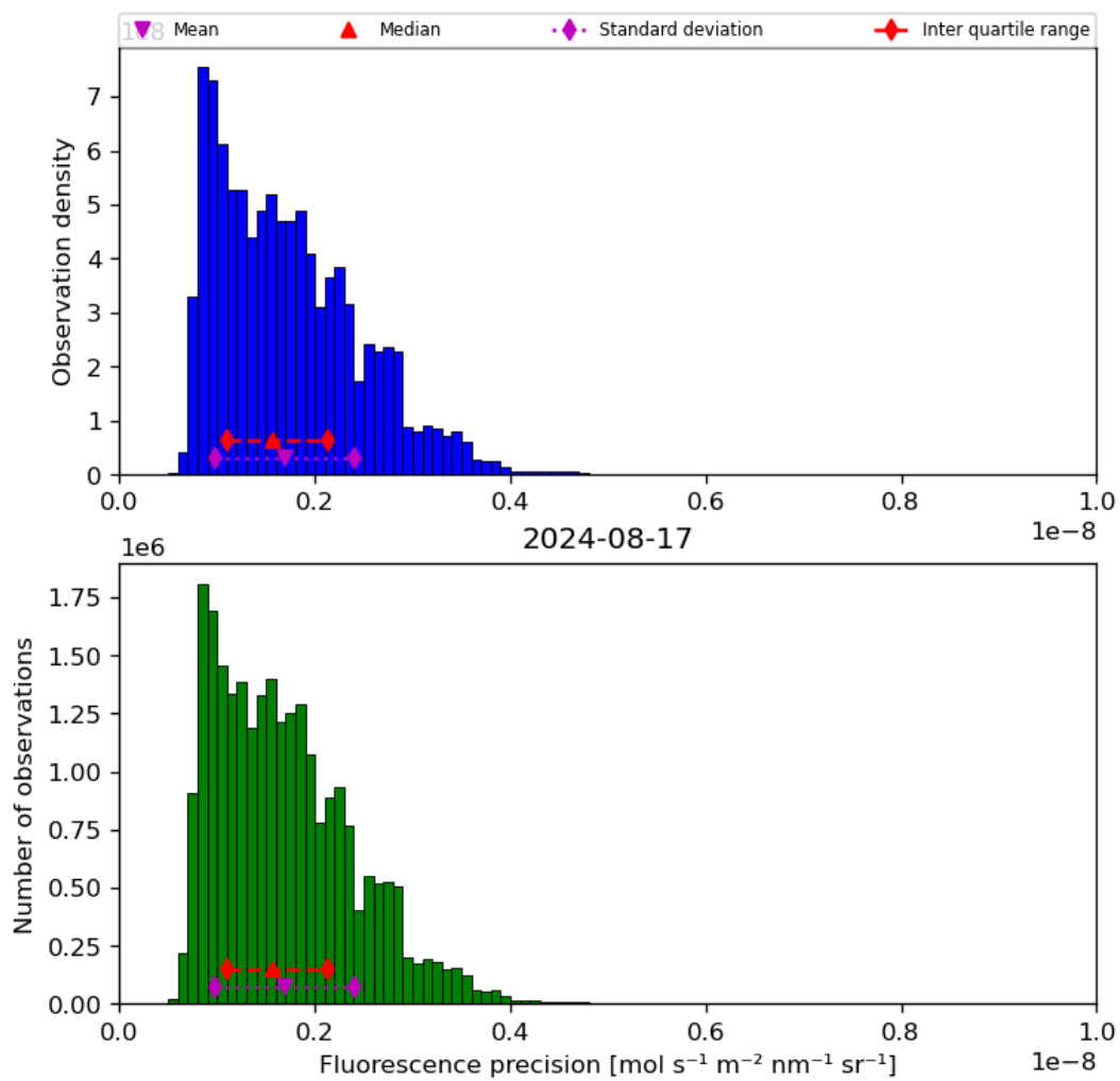
Figure 41: Histogram of “Fluorescence precision” for 2024-08-16 to 2024-08-18
