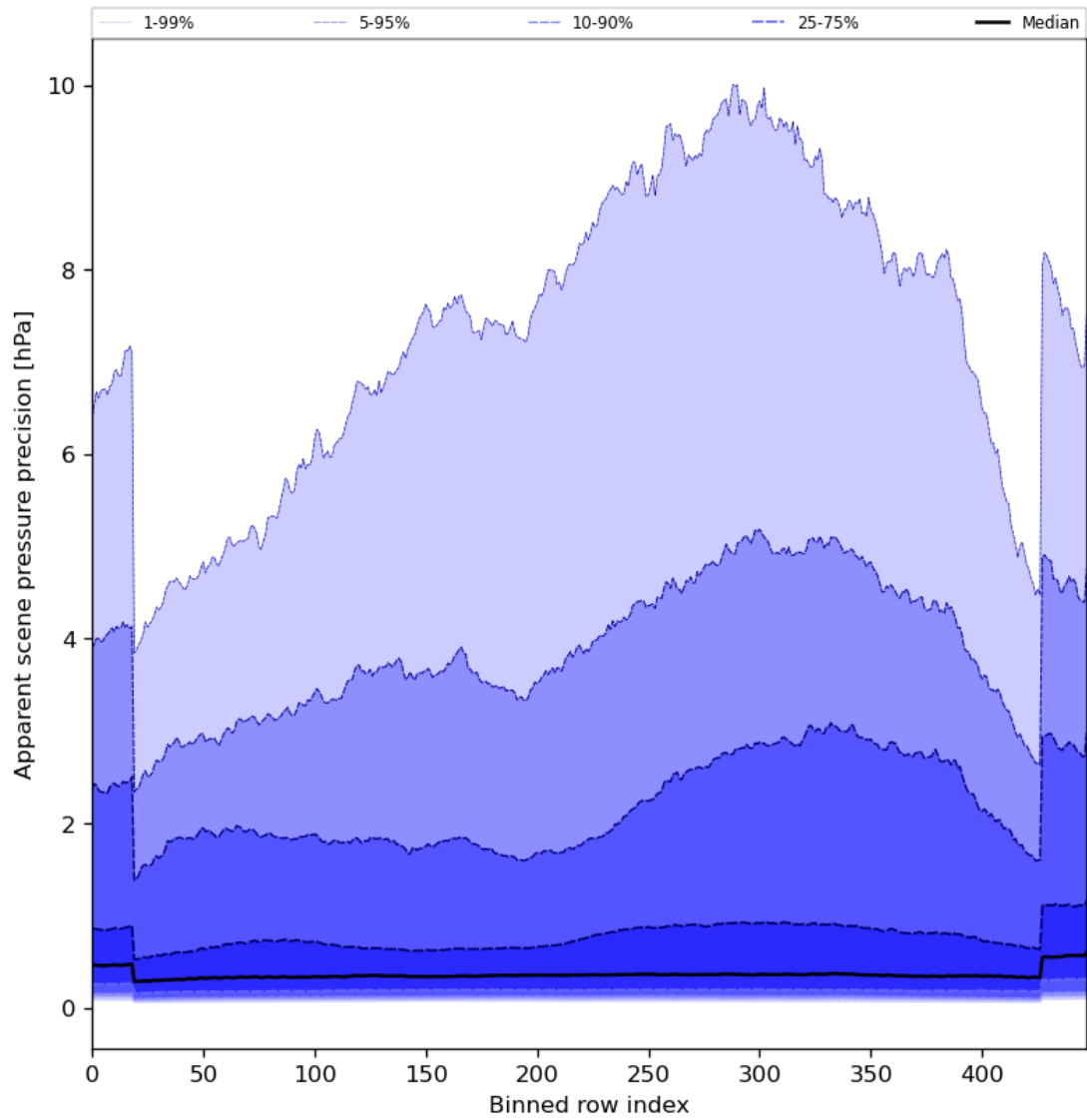
Figure 54: Along track statistics of “Apparent scene pressure precision” for 2024-08-16 to 2024-08-18
