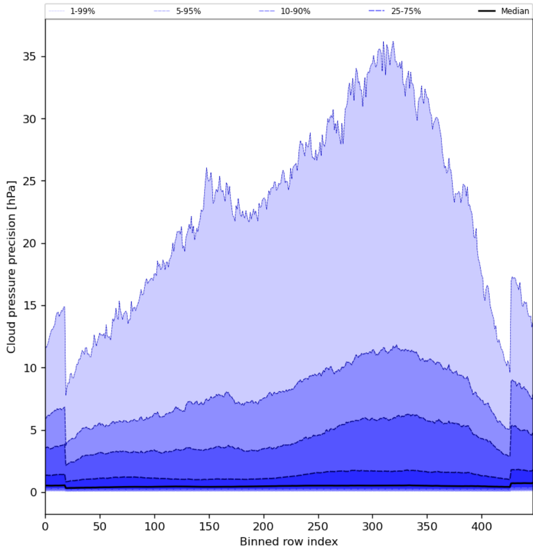
Figure 48: Along track statistics of “Cloud pressure precision” for 2024-08-16 to 2024-08-18
