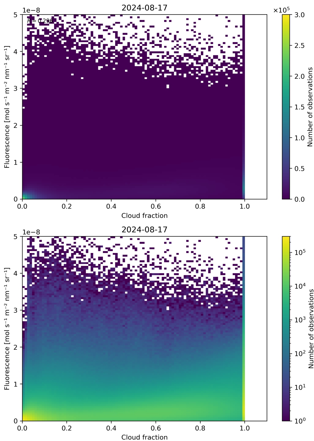
Figure 72: Scatter density plot of “Cloud fraction” against “Fluorescence” for 2024-08-16 to 2024-08-18.
