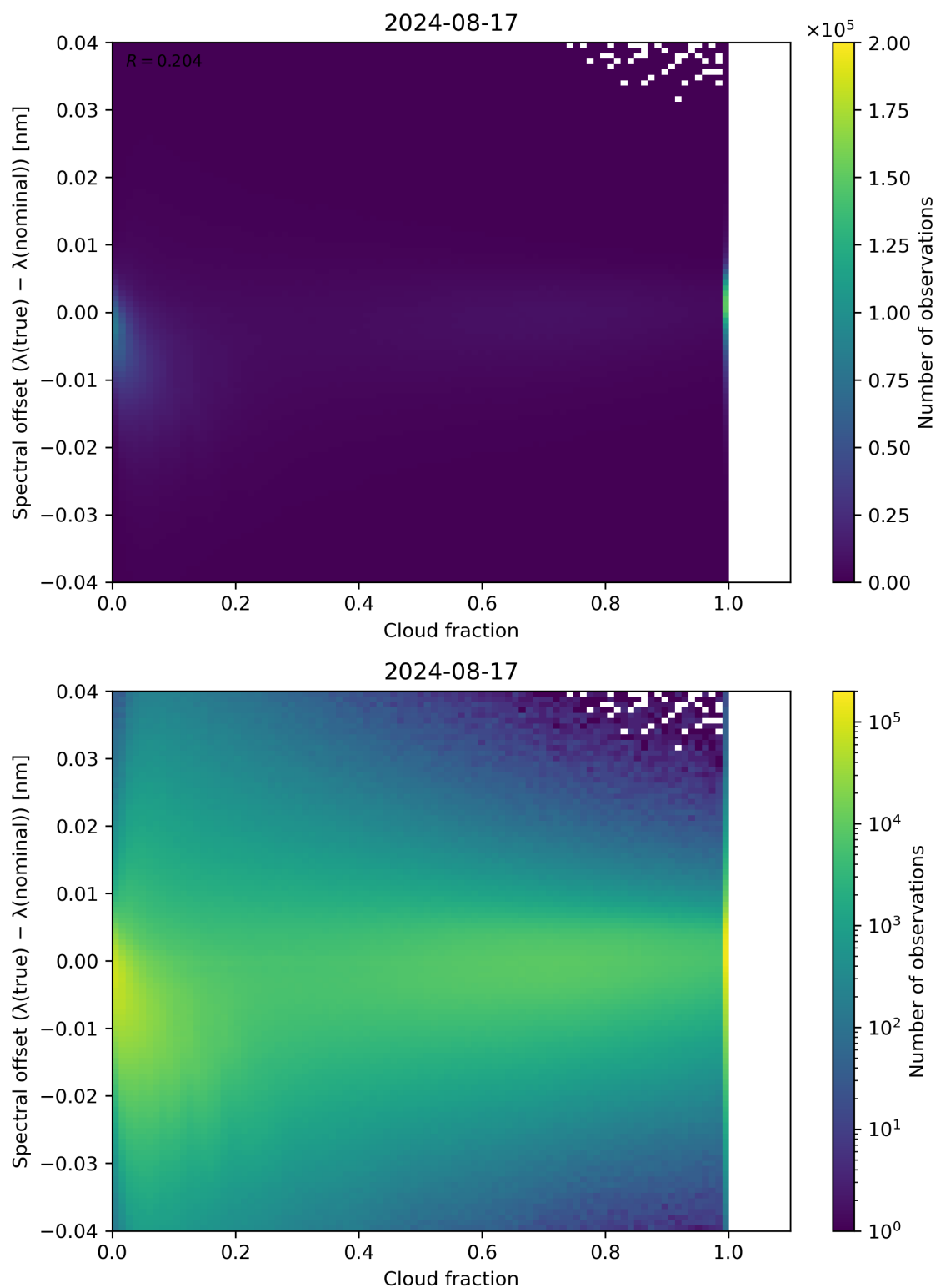
Figure 76: Scatter density plot of “Cloud fraction” against “Spectral offset ( \lambda(\text{true}) - \lambda(\text{nominal}) )” for 2024-08-16 to 2024-08-18.
