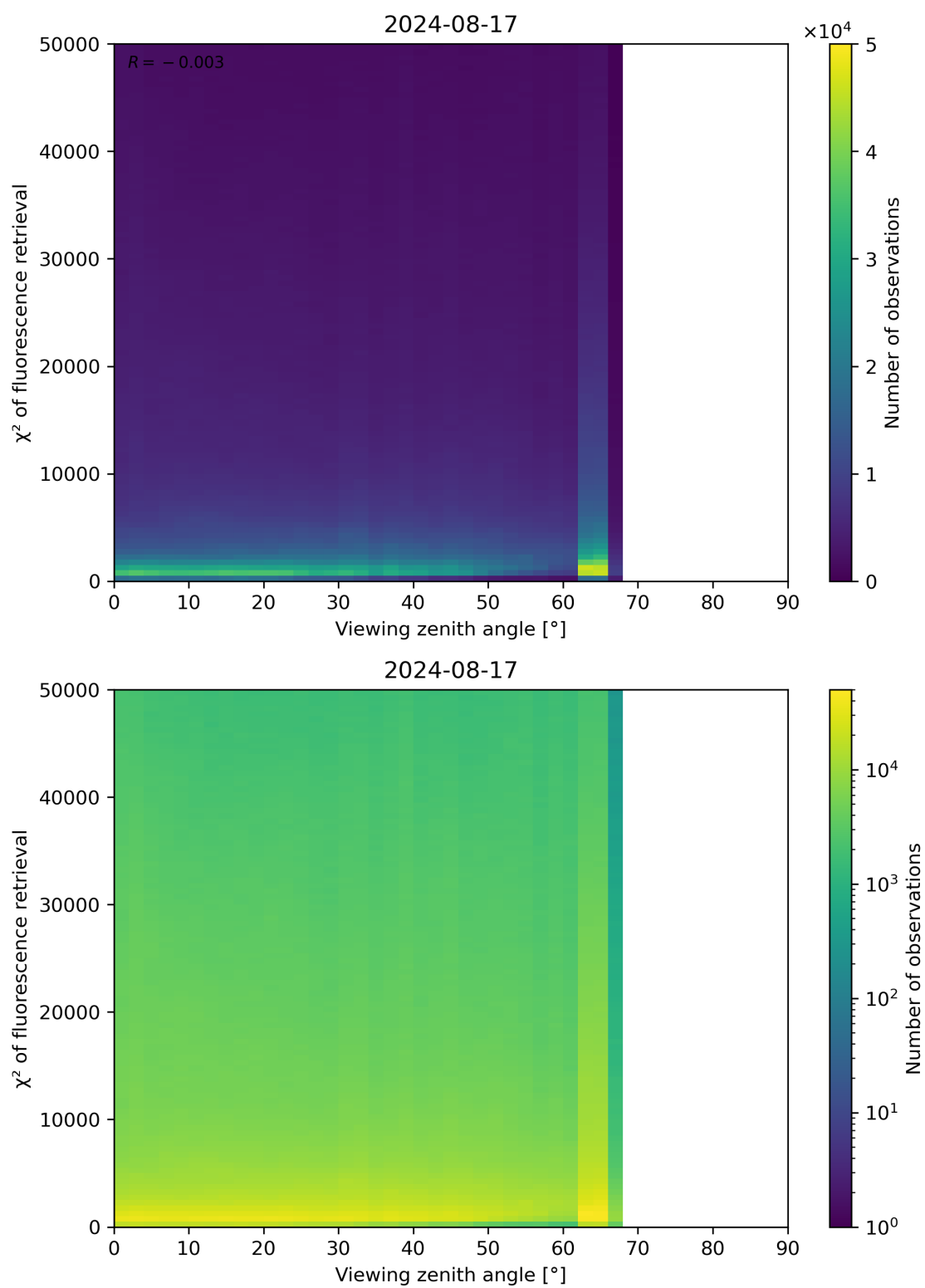
Figure 119: Scatter density plot of “Viewing zenith angle” against “ \chi^2 of fluorescence retrieval” for 2024-08-16 to 2024-08-18.
