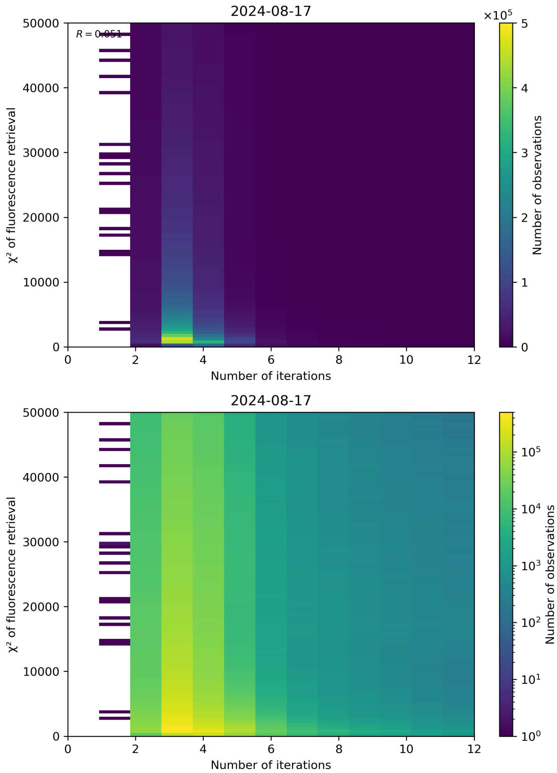
Figure 97: Scatter density plot of “Number of iterations” against “ \chi^2 of fluorescence retrieval” for 2024-08-16 to 2024-08-18.
