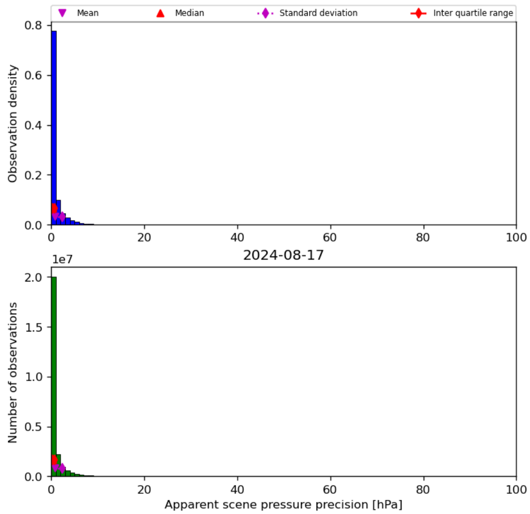
Figure 37: Histogram of “Apparent scene pressure precision” for 2024-08-16 to 2024-08-18
