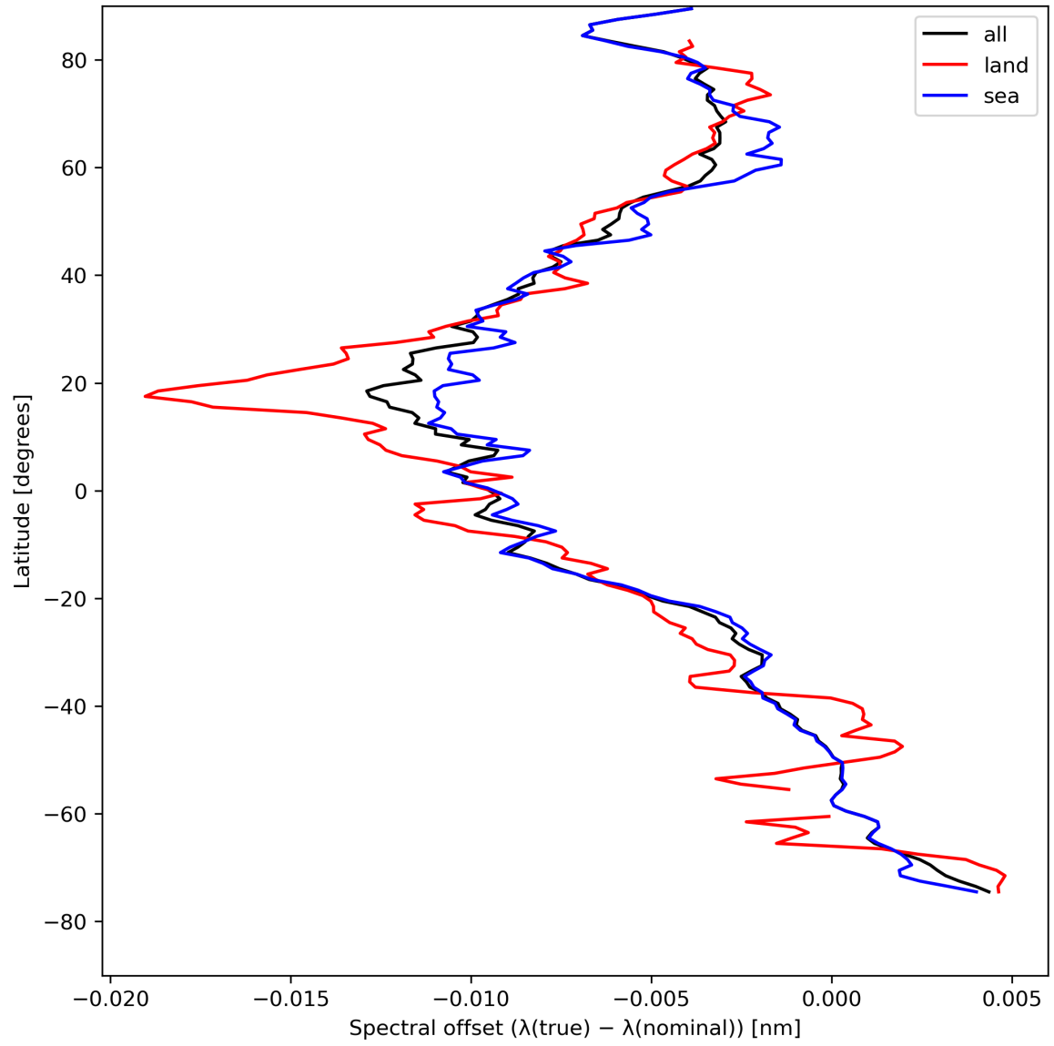
Figure 28: Zonal average of “Spectral offset ( \lambda(\text{true}) - \lambda(\text{nominal}) )” for 2024-08-16 to 2024-08-18.
