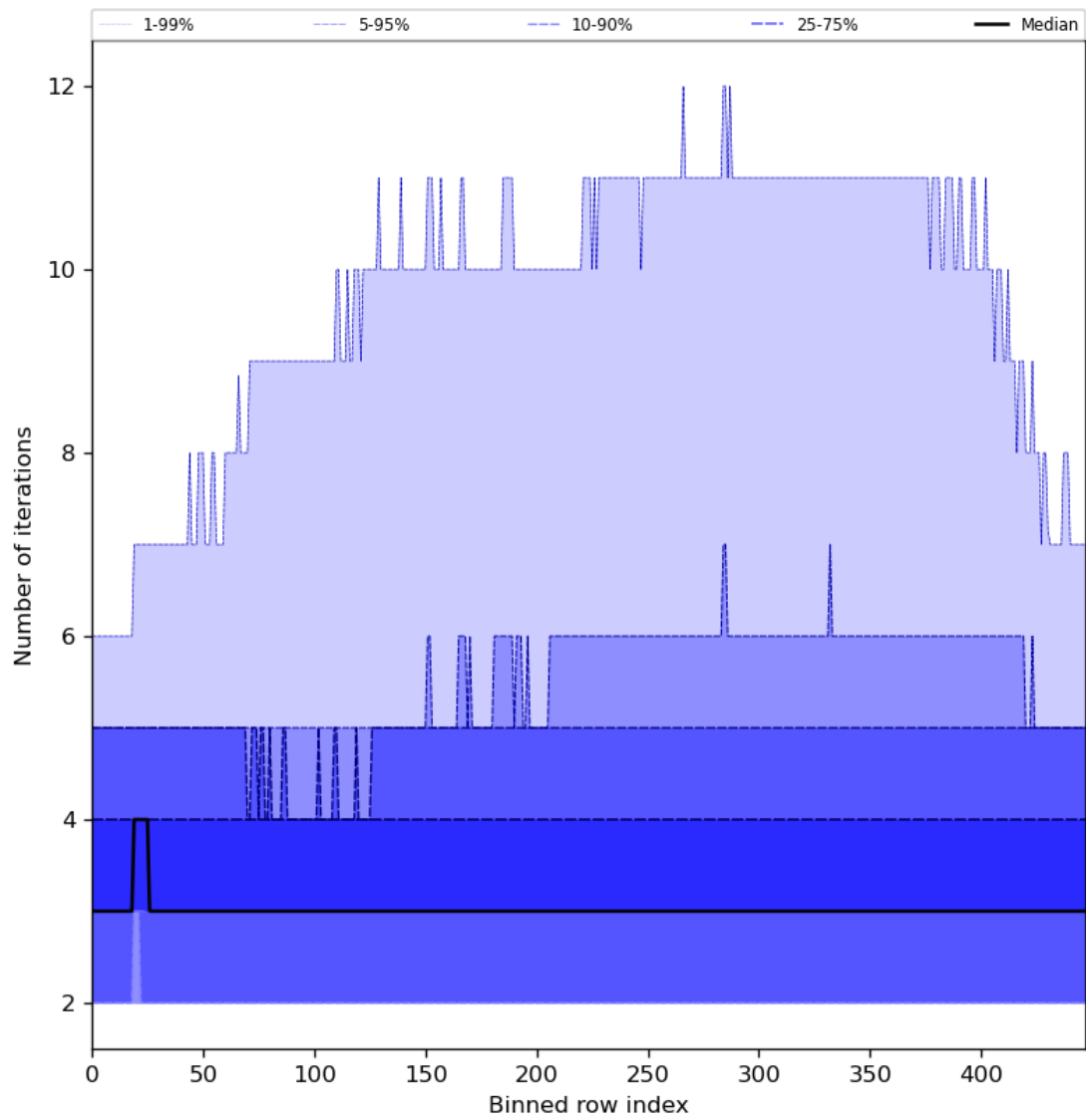
Figure 56: Along track statistics of “Number of iterations” for 2024-08-16 to 2024-08-18
