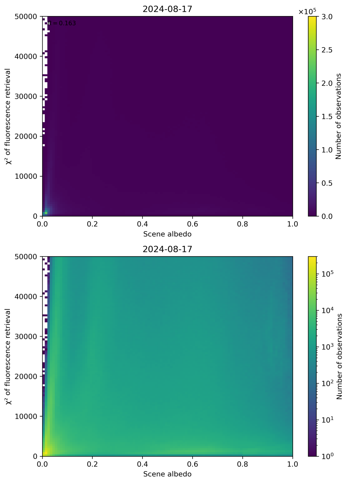
Figure 103: Scatter density plot of “Scene albedo” against “ \chi^2 of fluorescence retrieval” for 2024-08-16 to 2024-08-18.
