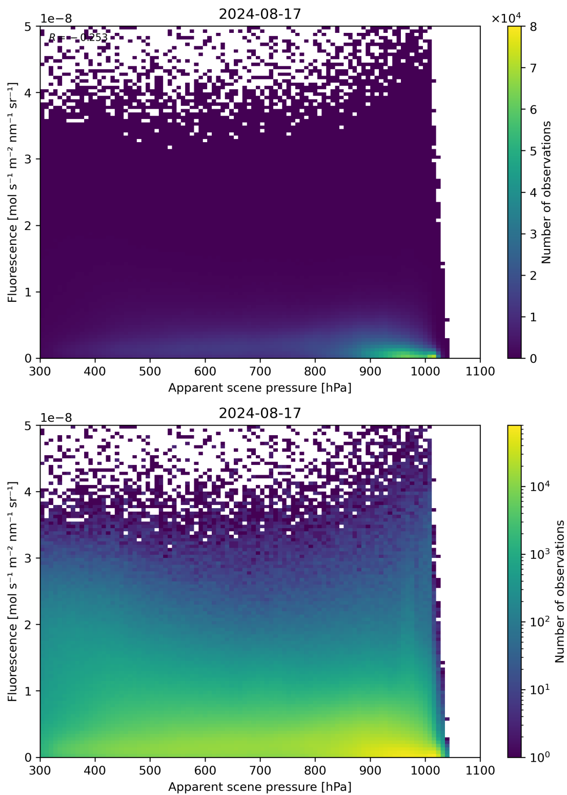
Figure 64: Scatter density plot of “Apparent scene pressure” against “Fluorescence” for 2024-08-16 to 2024-08-18.
