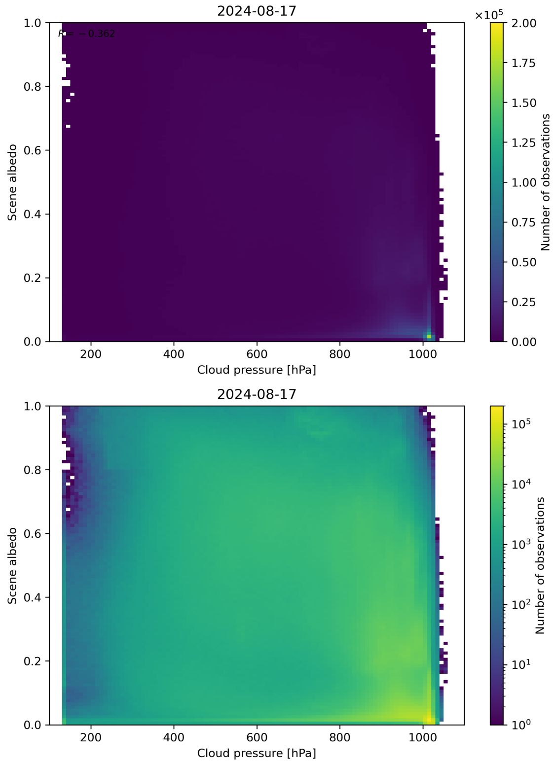
Figure 83: Scatter density plot of “Cloud pressure” against “Scene albedo” for 2024-08-16 to 2024-08-18.
