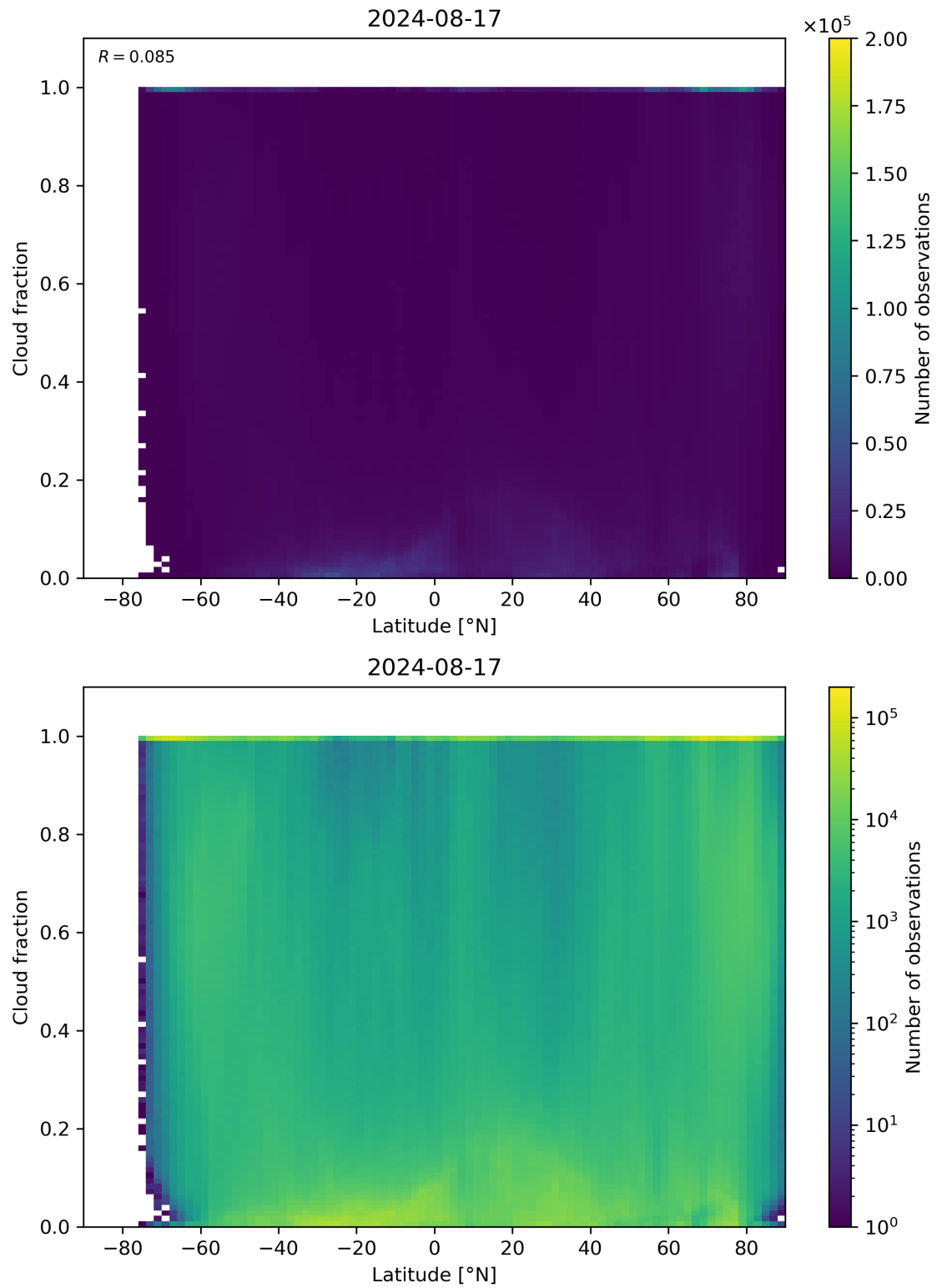
Figure 90: Scatter density plot of “Latitude” against “Cloud fraction” for 2024-08-16 to 2024-08-18.
