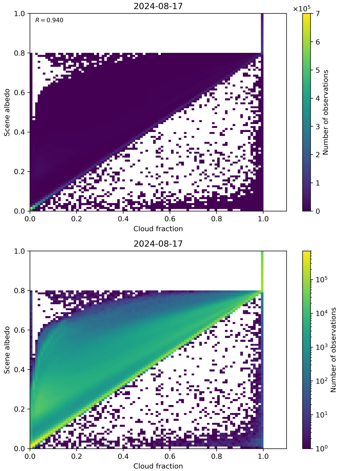
Figure 75: Scatter density plot of “Cloud fraction” against “Scene albedo” for 2024-08-16 to 2024-08-18.
