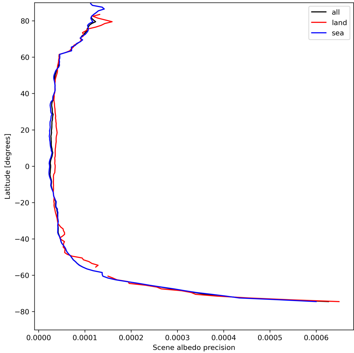
Figure 18: Zonal average of “Scene albedo precision” for 2024-08-16 to 2024-08-18.
