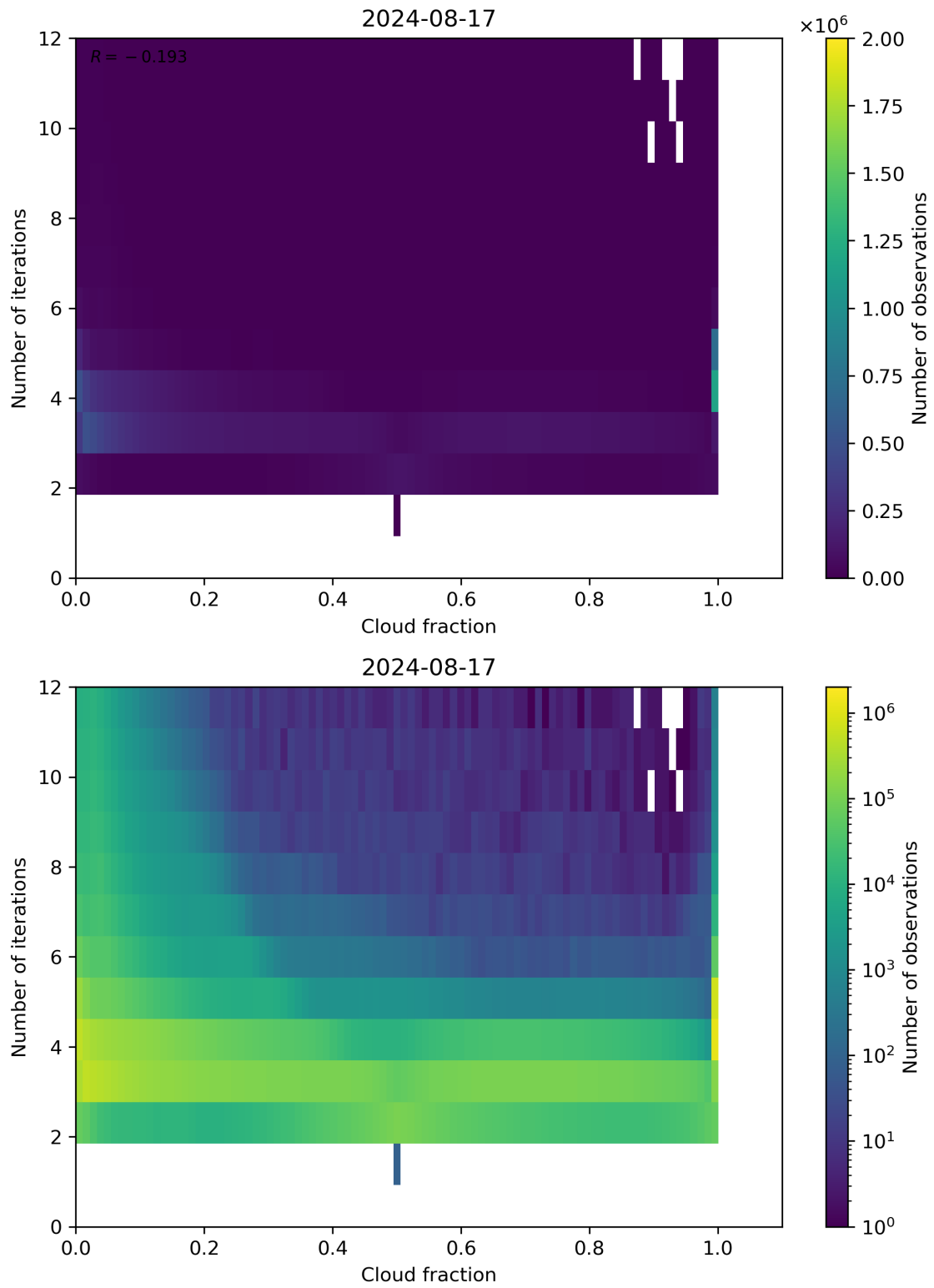
Figure 73: Scatter density plot of “Cloud fraction” against “Number of iterations” for 2024-08-16 to 2024-08-18.
