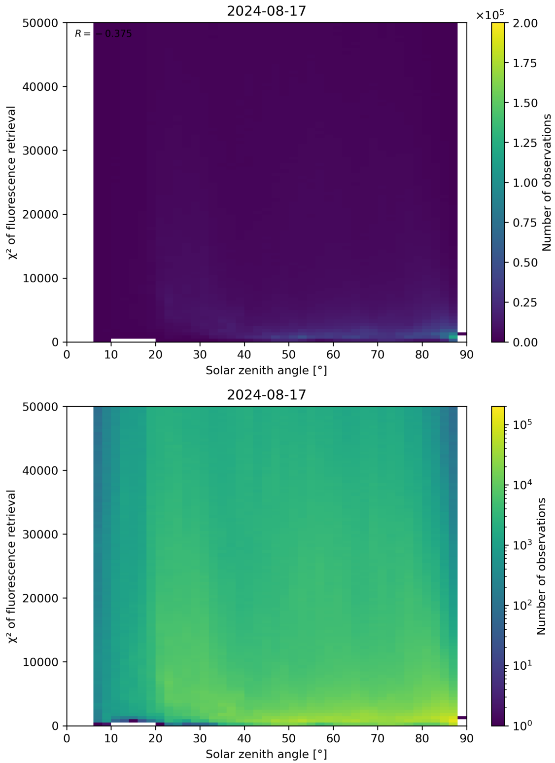
Figure 109: Scatter density plot of “Solar zenith angle” against “ \chi^2 of fluorescence retrieval” for 2024-08-16 to 2024-08-18.
