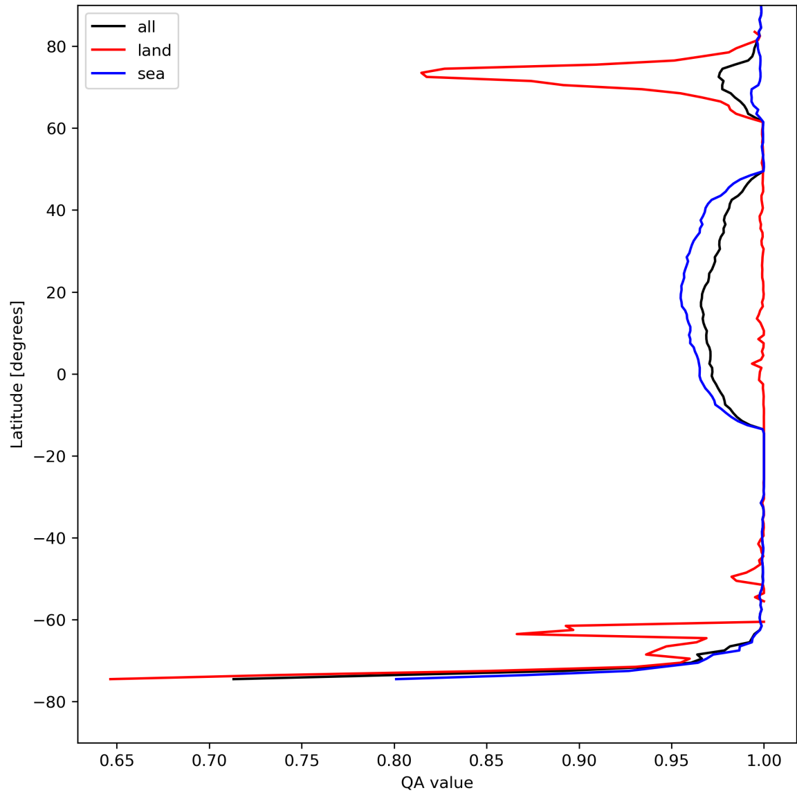
Figure 12: Zonal average of “QA value” for 2024-08-16 to 2024-08-18.
