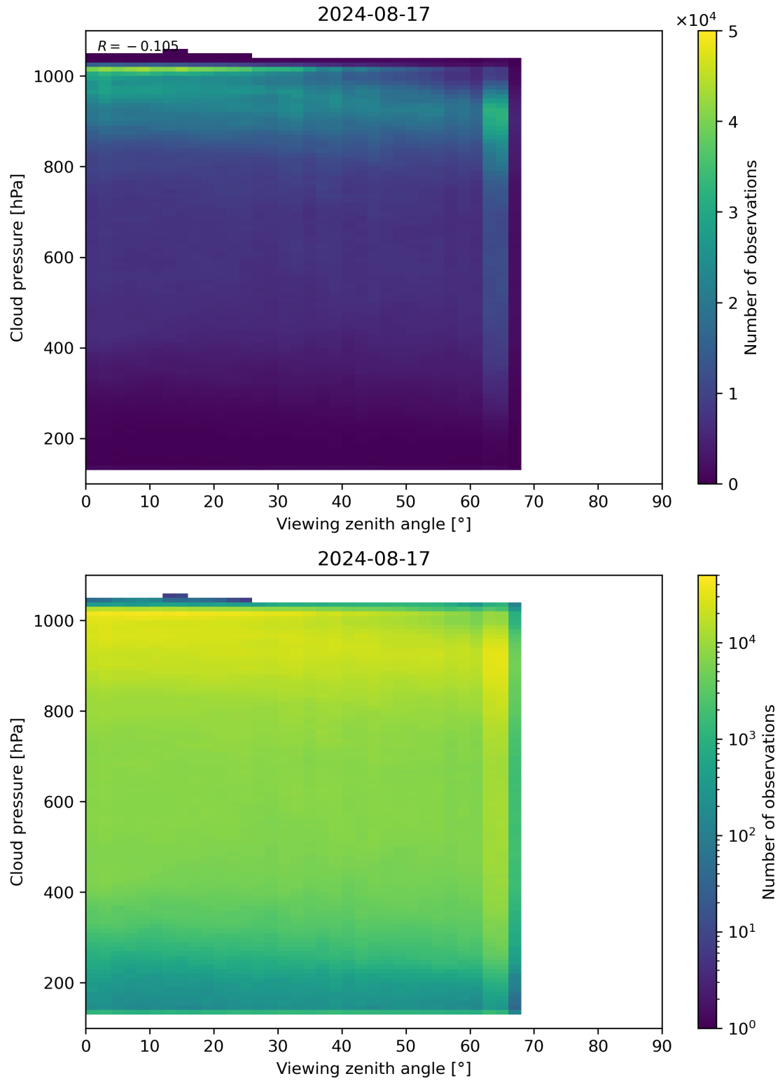
Figure 121: Scatter density plot of “Viewing zenith angle” against “Cloud pressure” for 2024-08-16 to 2024-08-18.
