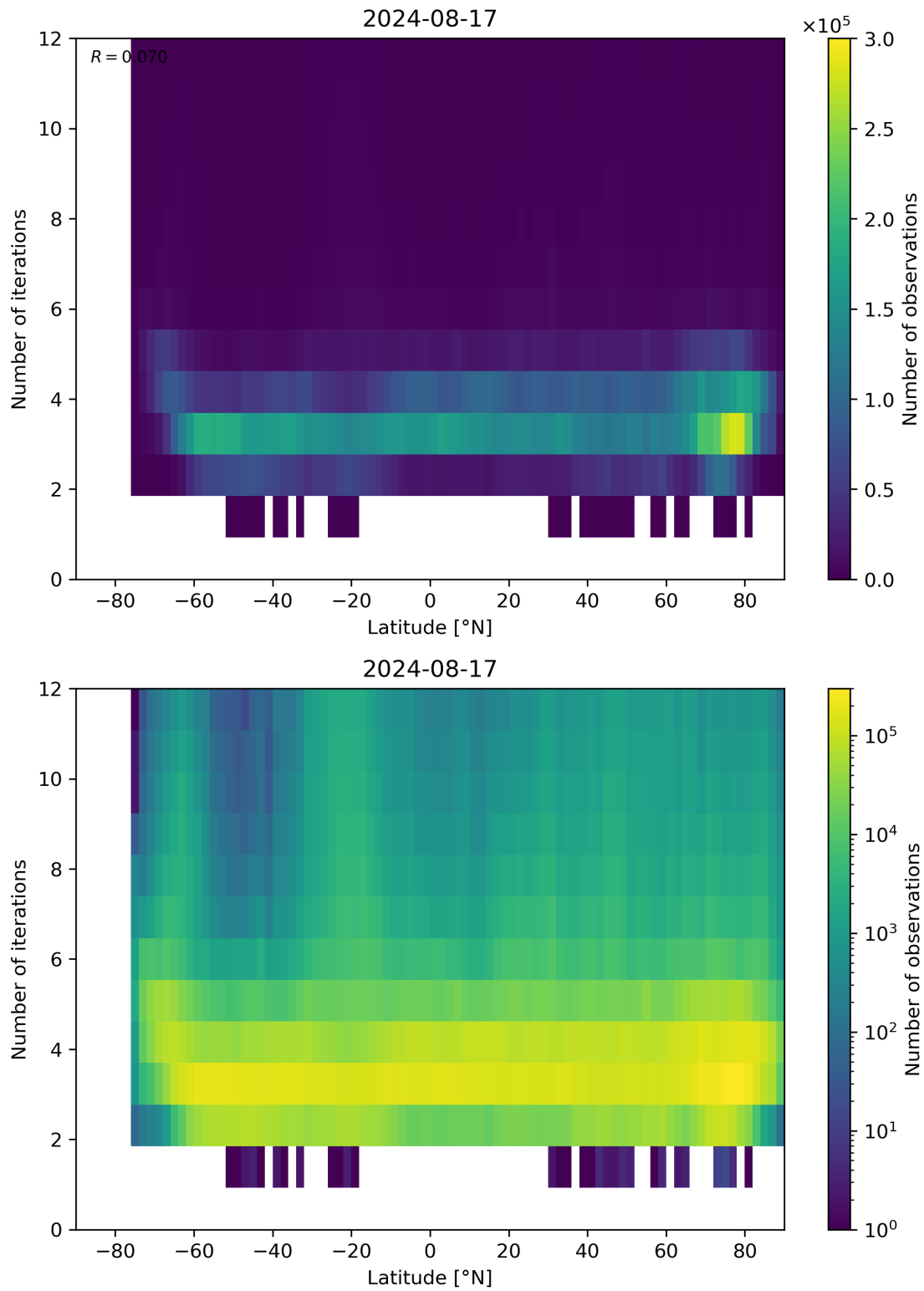
Figure 93: Scatter density plot of “Latitude” against “Number of iterations” for 2024-08-16 to 2024-08-18.
