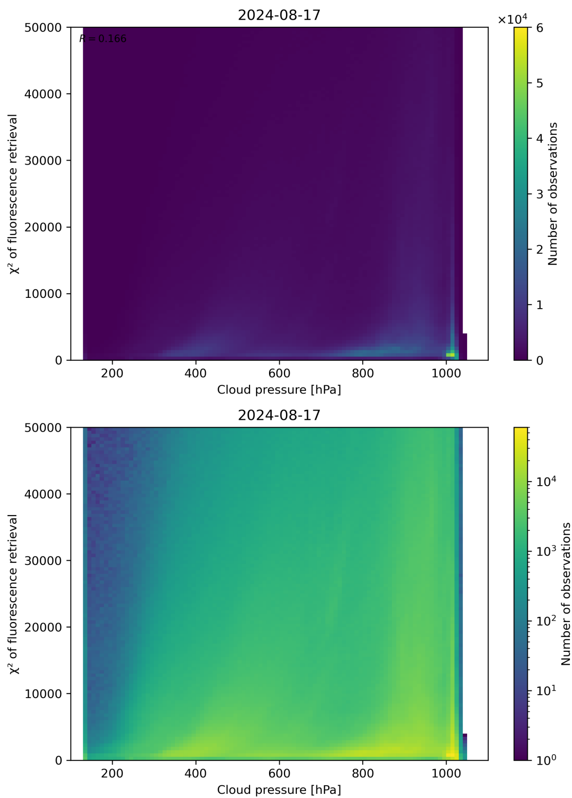
Figure 78: Scatter density plot of “Cloud pressure” against “ \chi^2 of fluorescence retrieval” for 2024-08-16 to 2024-08-18.
