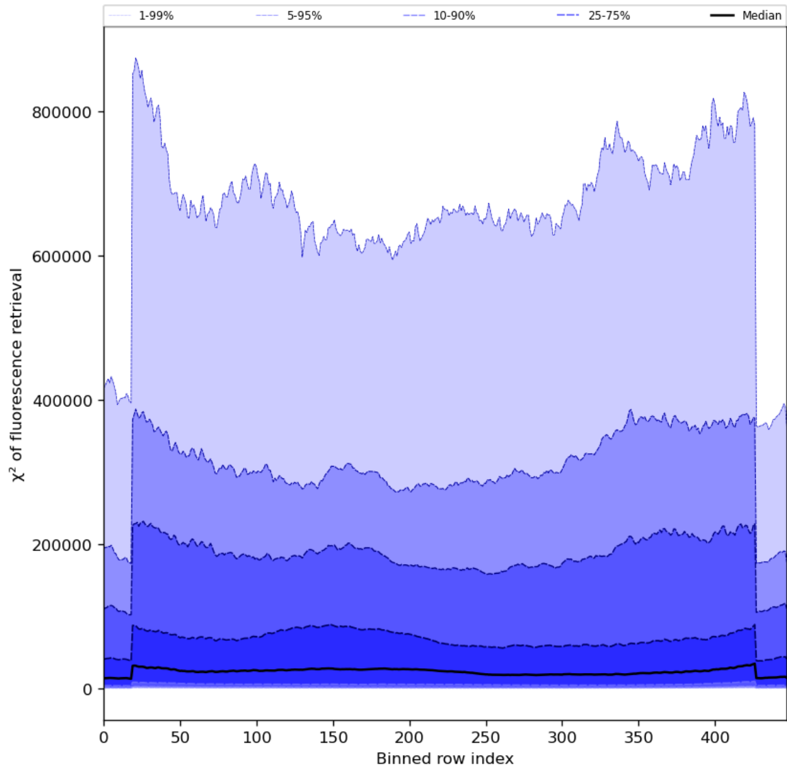
Figure 59: Along track statistics of “ \chi^2 of fluorescence retrieval” for 2024-08-16 to 2024-08-18
