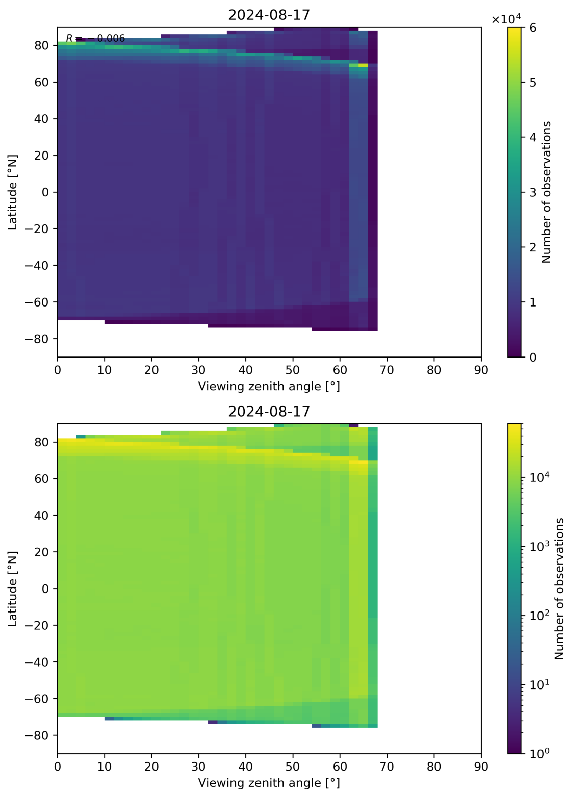
Figure 123: Scatter density plot of “Viewing zenith angle” against “Latitude” for 2024-08-16 to 2024-08-18.
