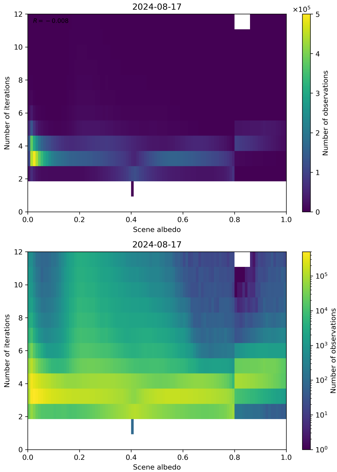
Figure 105: Scatter density plot of “Scene albedo” against “Number of iterations” for 2024-08-16 to 2024-08-18.
