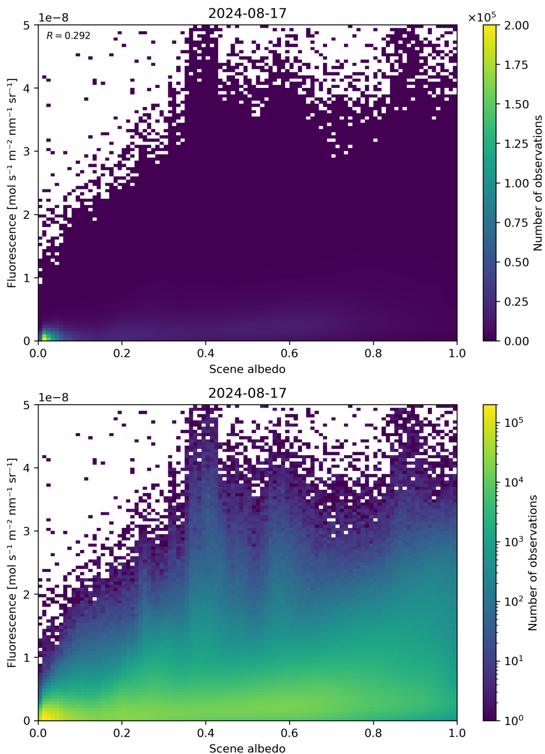
Figure 104: Scatter density plot of “Scene albedo” against “Fluorescence” for 2024-08-16 to 2024-08-18.
