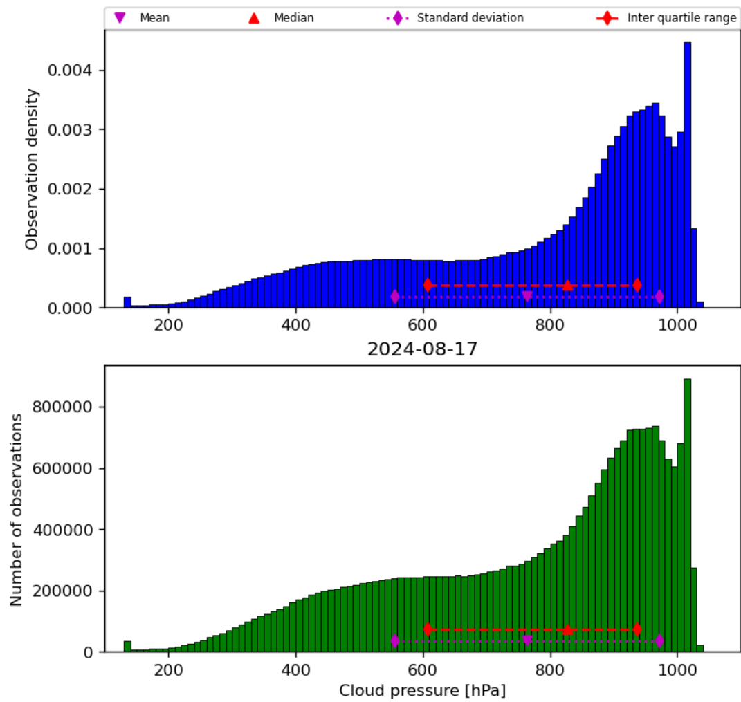
Figure 30: Histogram of “Cloud pressure” for 2024-08-16 to 2024-08-18
