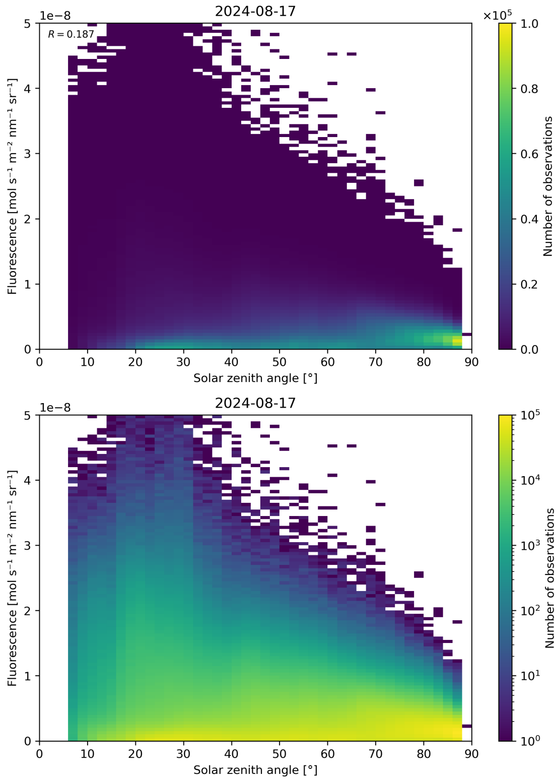
Figure 112: Scatter density plot of “Solar zenith angle” against “Fluorescence” for 2024-08-16 to 2024-08-18.
