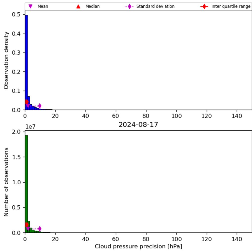
Figure 31: Histogram of “Cloud pressure precision” for 2024-08-16 to 2024-08-18
