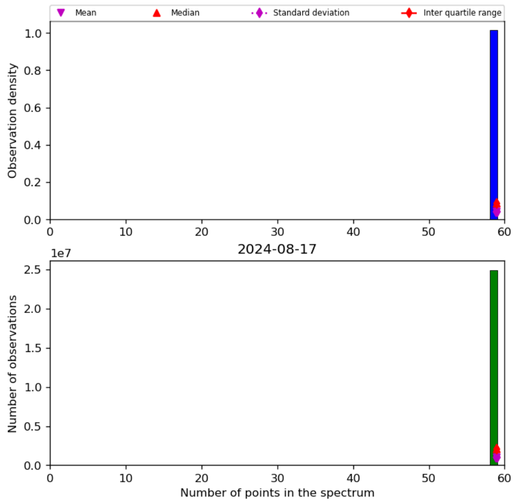
Figure 44: Histogram of “Number of points in the spectrum” for 2024-08-16 to 2024-08-18
