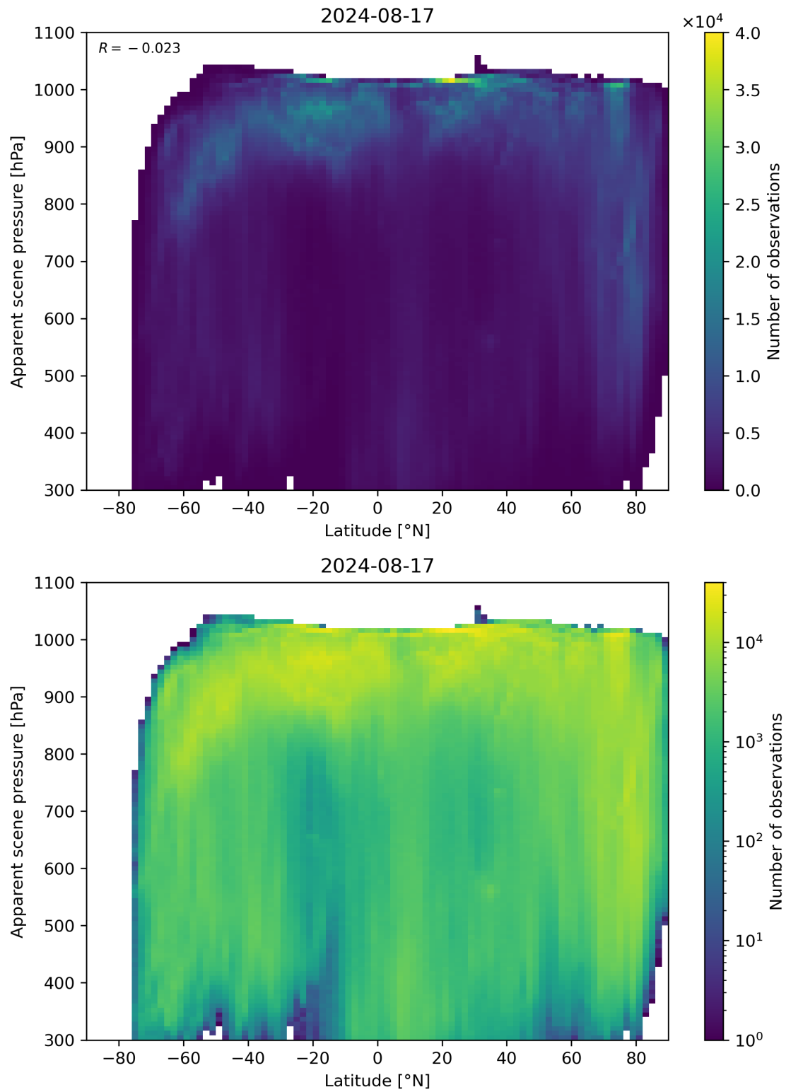
Figure 88: Scatter density plot of “Latitude” against “Apparent scene pressure” for 2024-08-16 to 2024-08-18.
