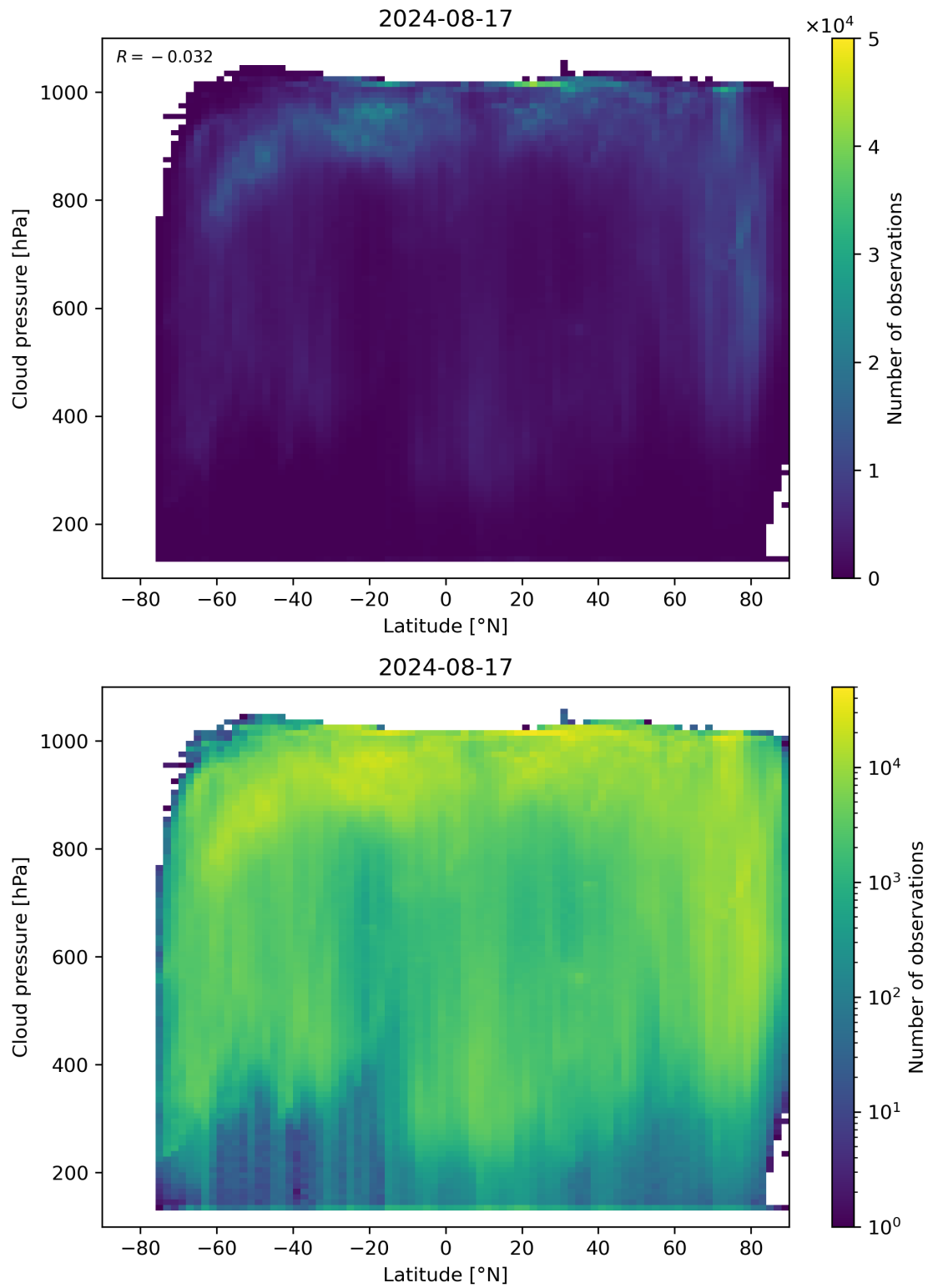
Figure 91: Scatter density plot of “Latitude” against “Cloud pressure” for 2024-08-16 to 2024-08-18.
