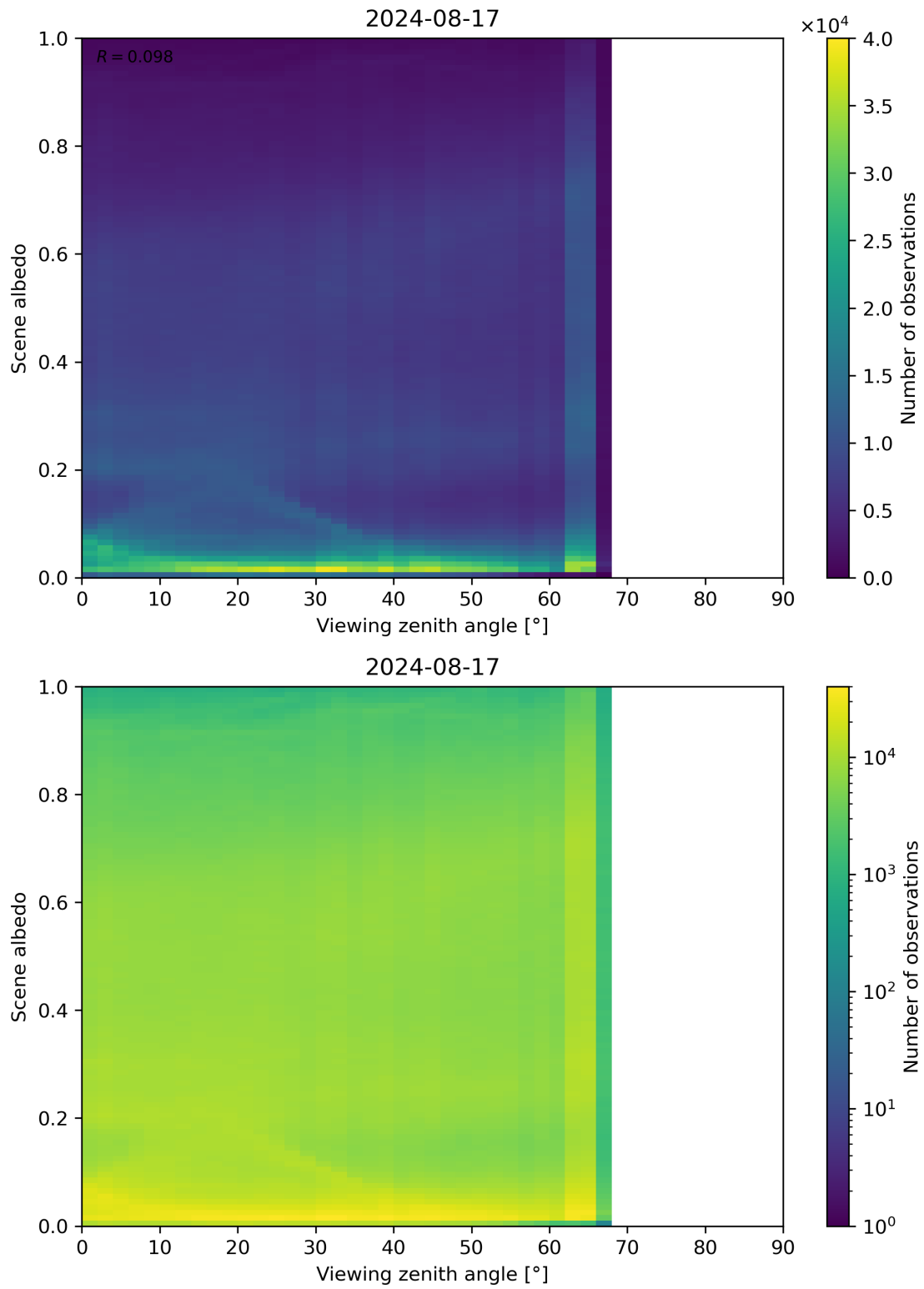
Figure 126: Scatter density plot of “Viewing zenith angle” against “Scene albedo” for 2024-08-16 to 2024-08-18.
