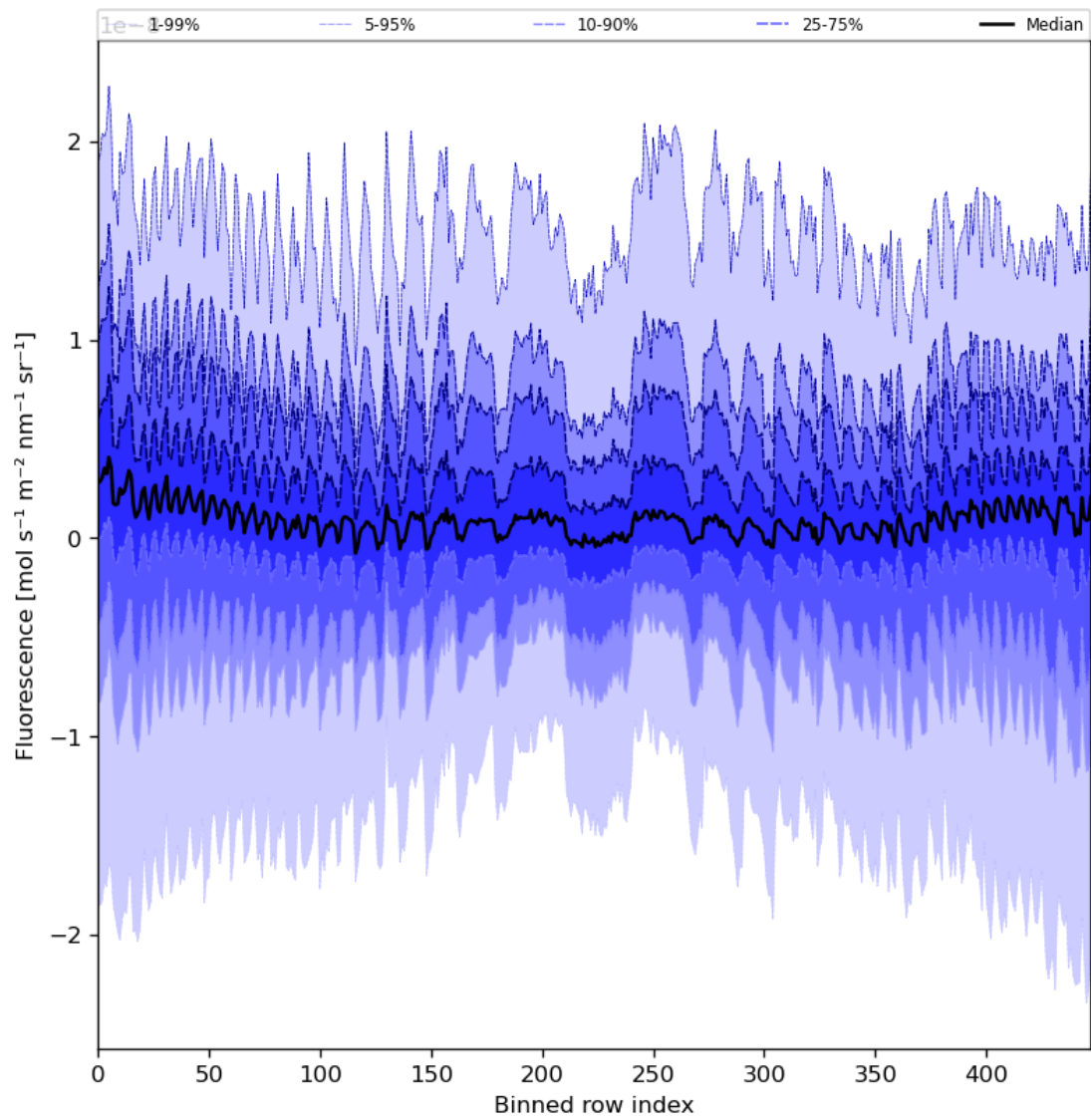
Figure 57: Along track statistics of “Fluorescence” for 2024-08-16 to 2024-08-18
