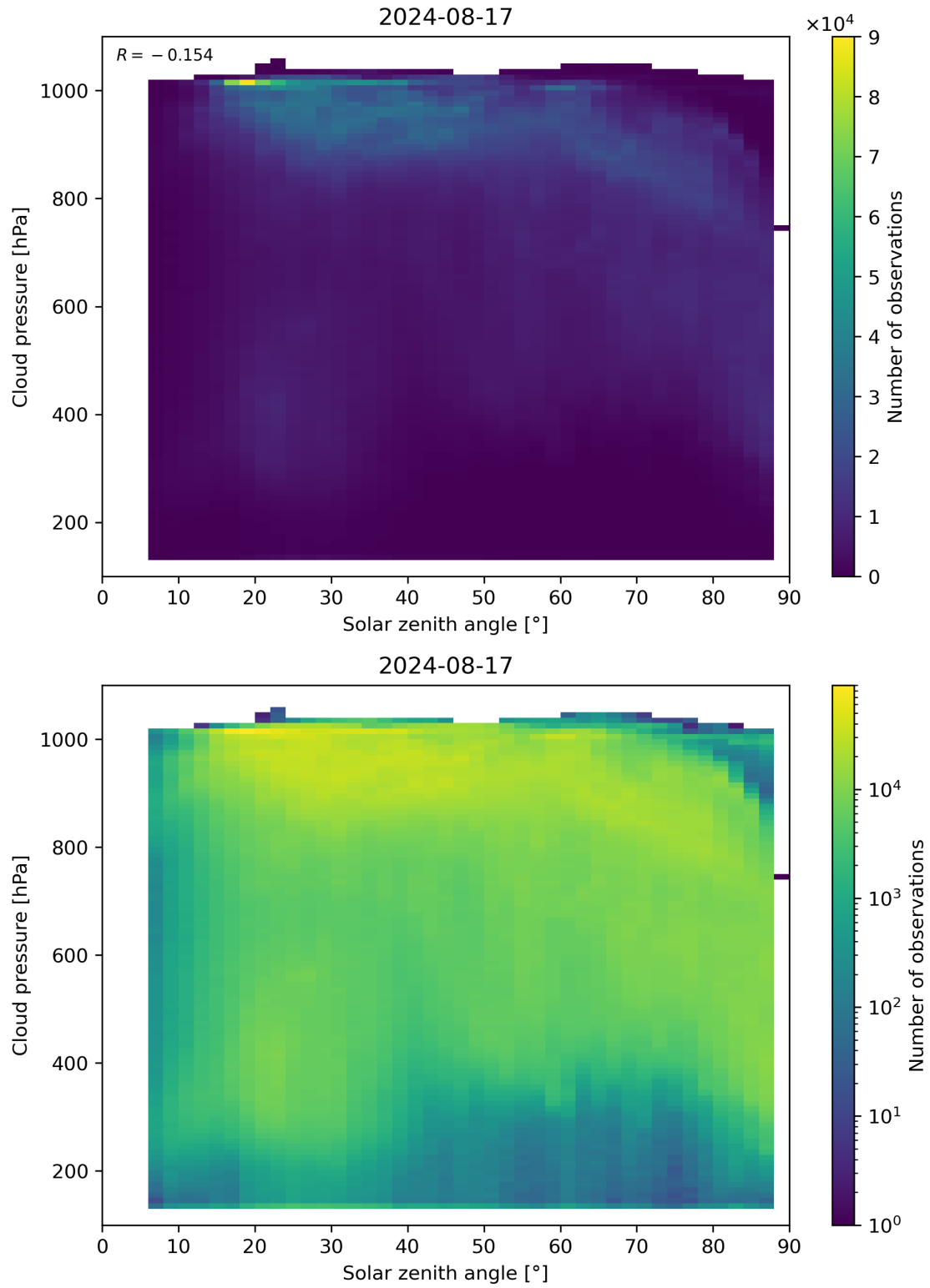
Figure 111: Scatter density plot of “Solar zenith angle” against “Cloud pressure” for 2024-08-16 to 2024-08-18.
