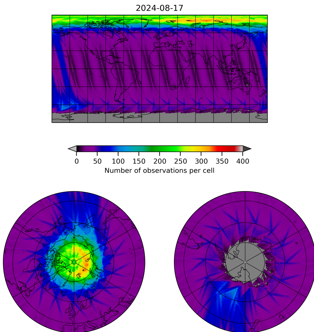
Figure 11: Map of the number of observations for 2024-08-16 to 2024-08-18
