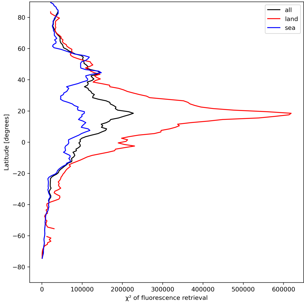
Figure 25: Zonal average of “ \chi^2 of fluorescence retrieval” for 2024-08-16 to 2024-08-18.
