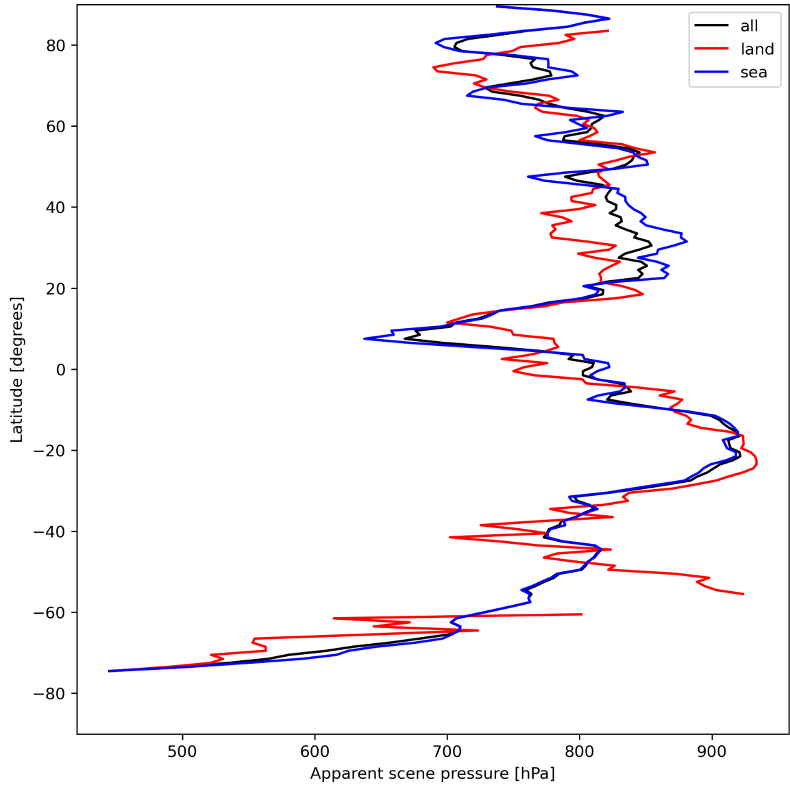
Figure 19: Zonal average of “Apparent scene pressure” for 2024-08-16 to 2024-08-18.
