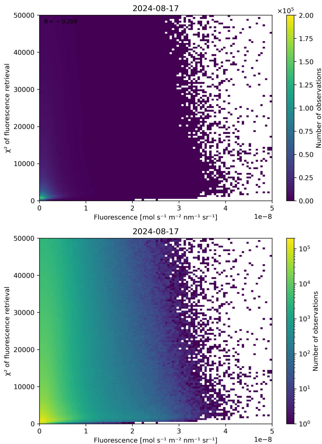
Figure 85: Scatter density plot of “Fluorescence” against “ \chi^2 of fluorescence retrieval” for 2024-08-16 to 2024-08-18.
