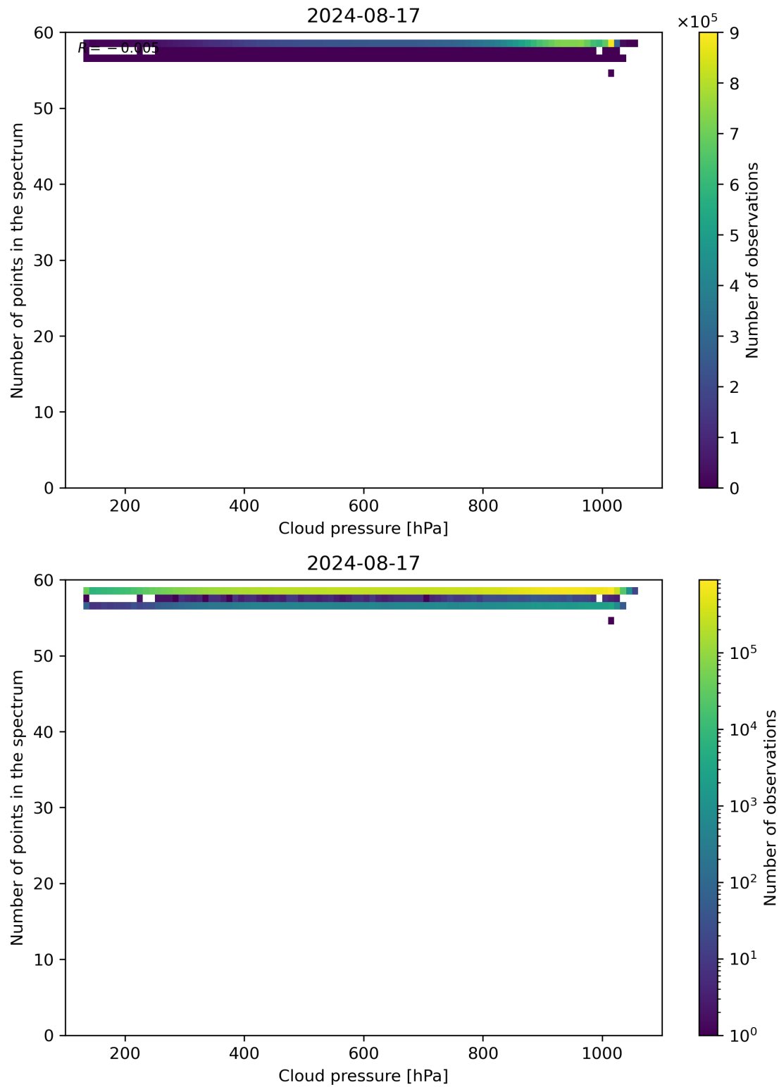
Figure 82: Scatter density plot of “Cloud pressure” against “Number of points in the spectrum” for 2024-08-16 to 2024-08-18.
