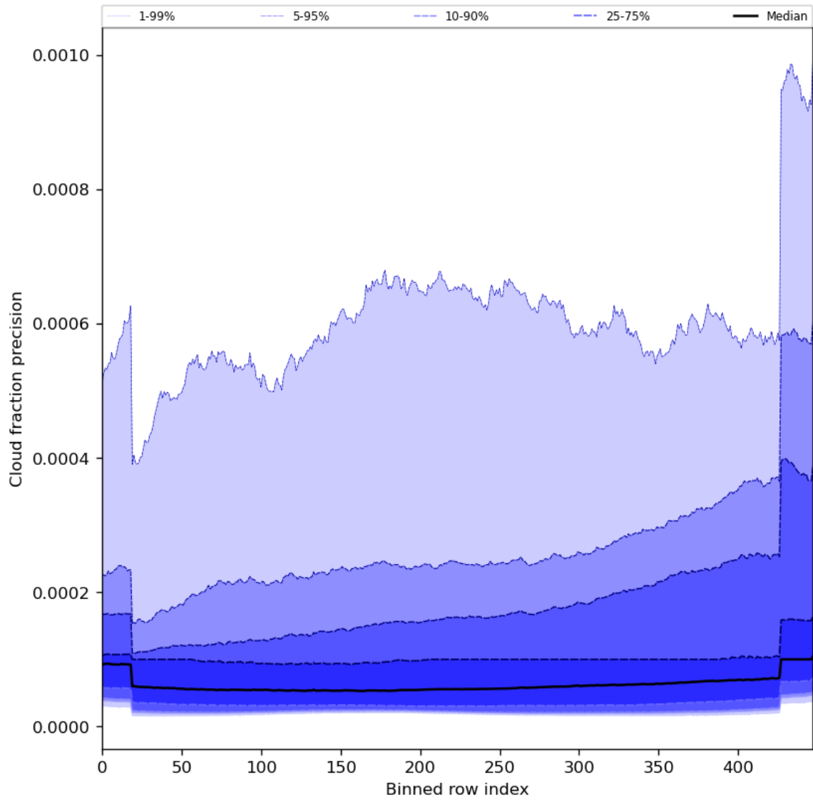
Figure 50: Along track statistics of “Cloud fraction precision” for 2024-08-16 to 2024-08-18
