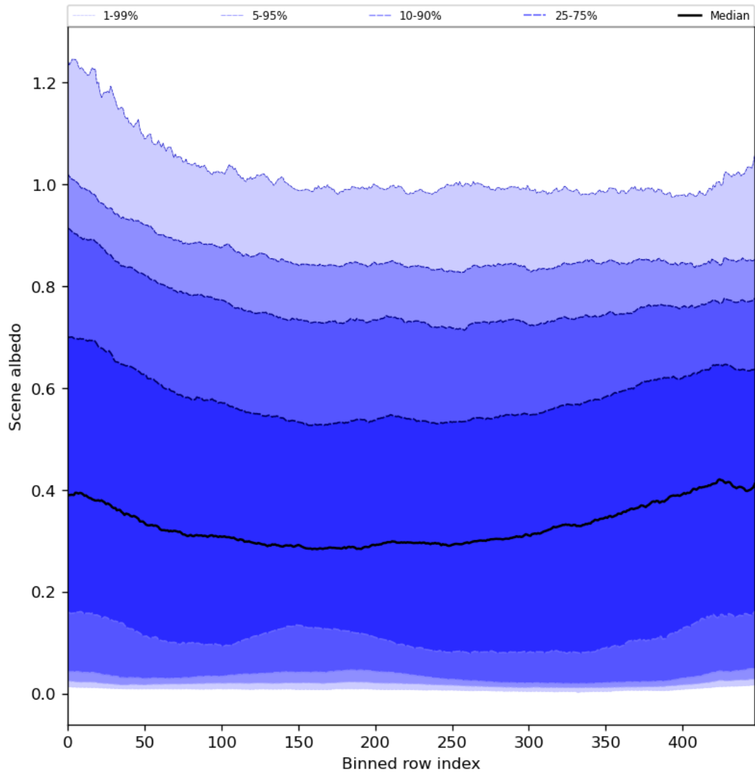
Figure 51: Along track statistics of “Scene albedo” for 2024-08-16 to 2024-08-18
