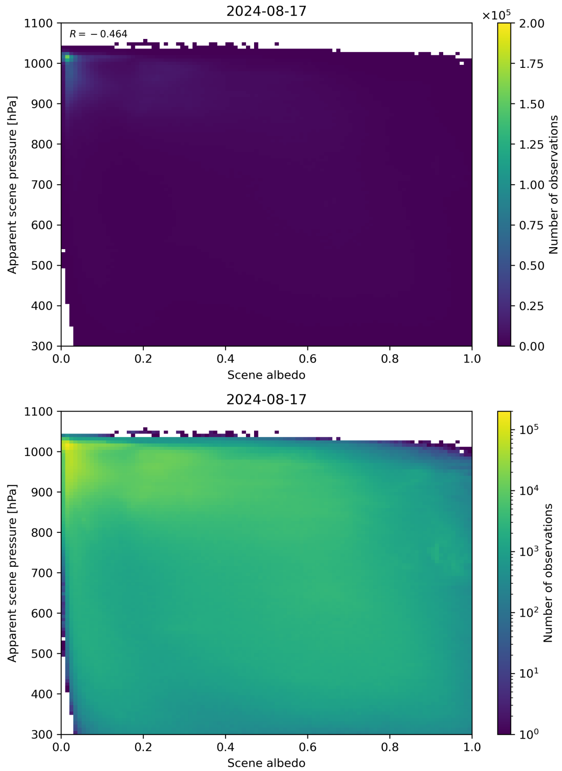
Figure 102: Scatter density plot of “Scene albedo” against “Apparent scene pressure” for 2024-08-16 to 2024-08-18.
