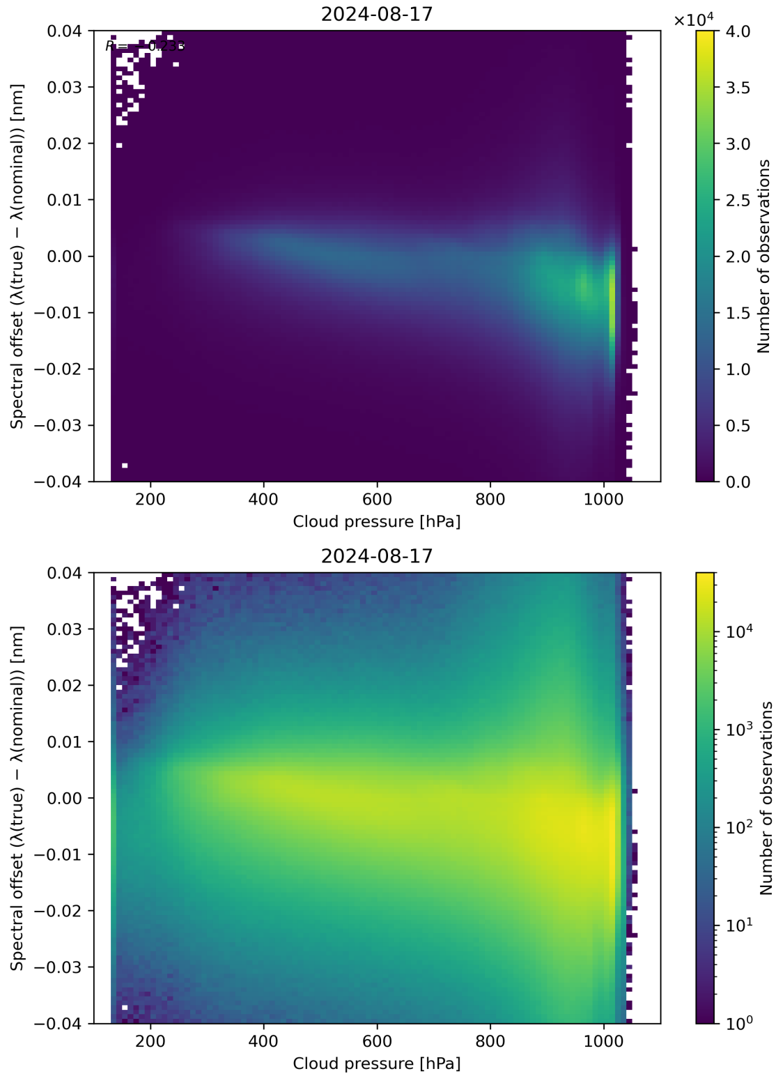
Figure 84: Scatter density plot of “Cloud pressure” against “Spectral offset ( \lambda(\text{true}) - \lambda(\text{nominal}) )” for 2024-08-16 to 2024-08-18.
