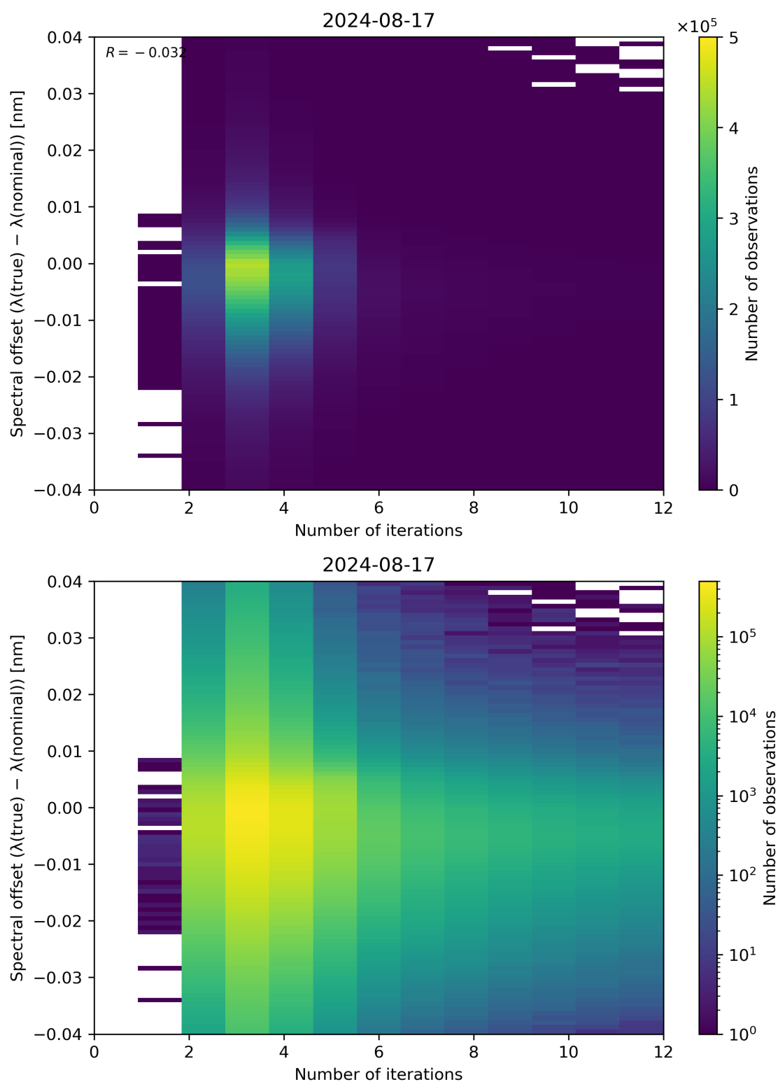
Figure 100: Scatter density plot of “Number of iterations” against “Spectral offset ( \lambda(\text{true}) - \lambda(\text{nominal}) )” for 2024-08-16 to 2024-08-18.
