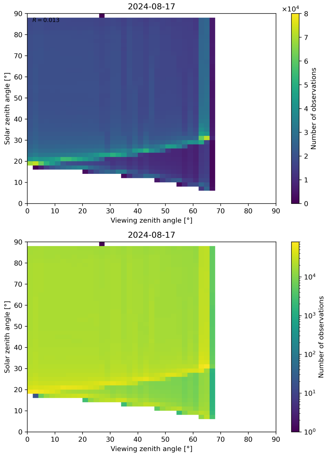
Figure 127: Scatter density plot of “Viewing zenith angle” against “Solar zenith angle” for 2024-08-16 to 2024-08-18.
