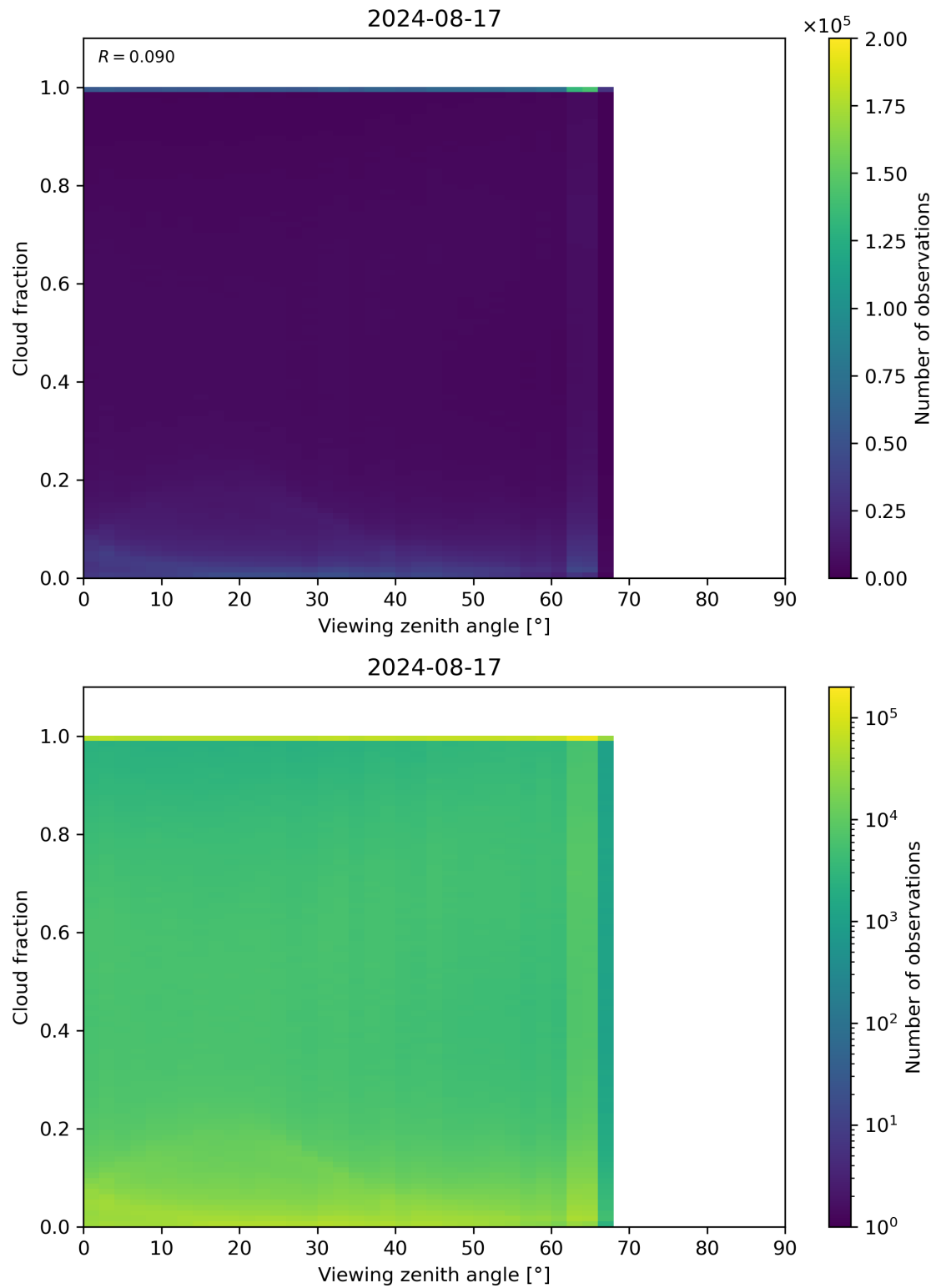
Figure 120: Scatter density plot of “Viewing zenith angle” against “Cloud fraction” for 2024-08-16 to 2024-08-18.
