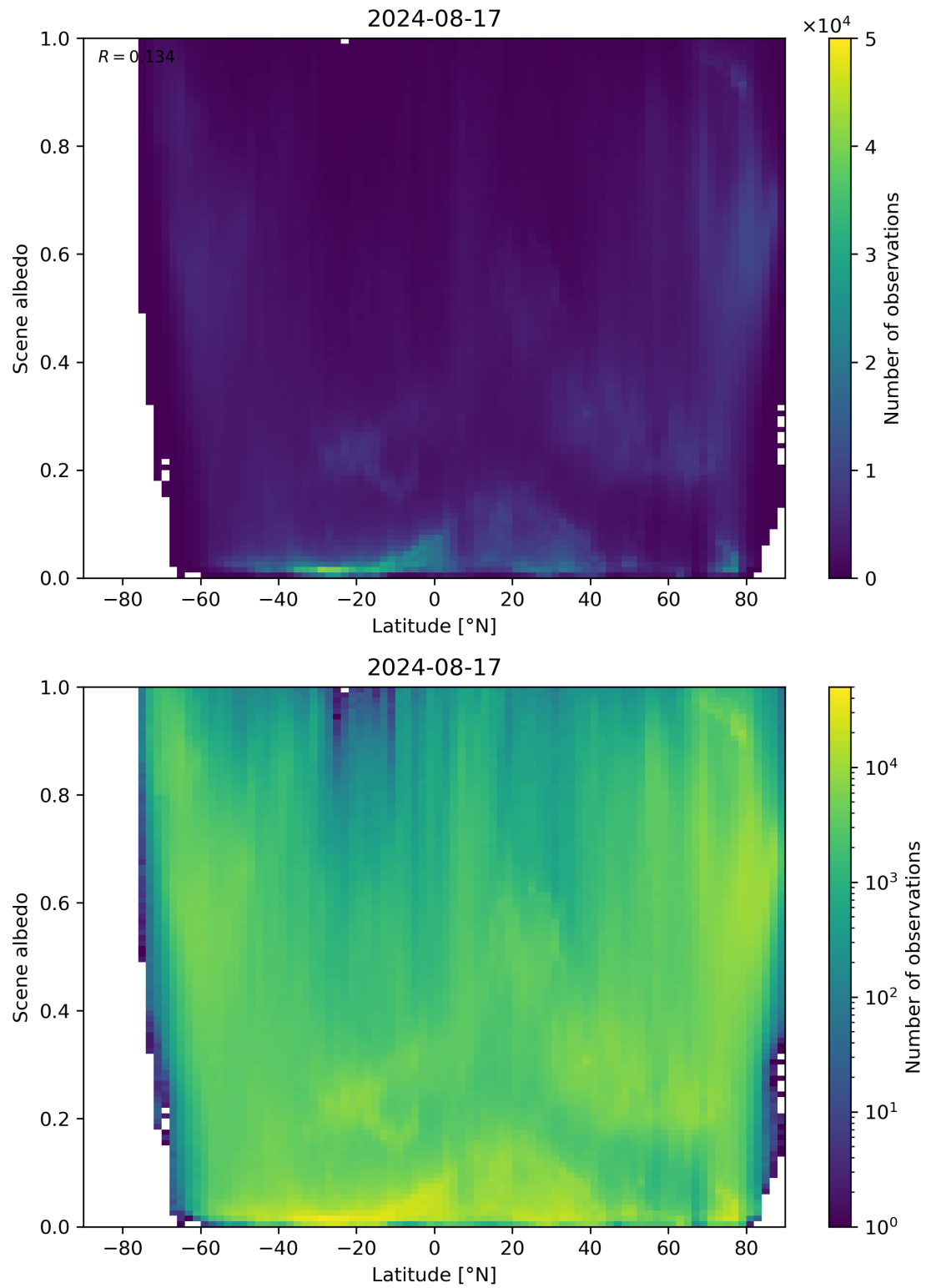
Figure 95: Scatter density plot of “Latitude” against “Scene albedo” for 2024-08-16 to 2024-08-18.
