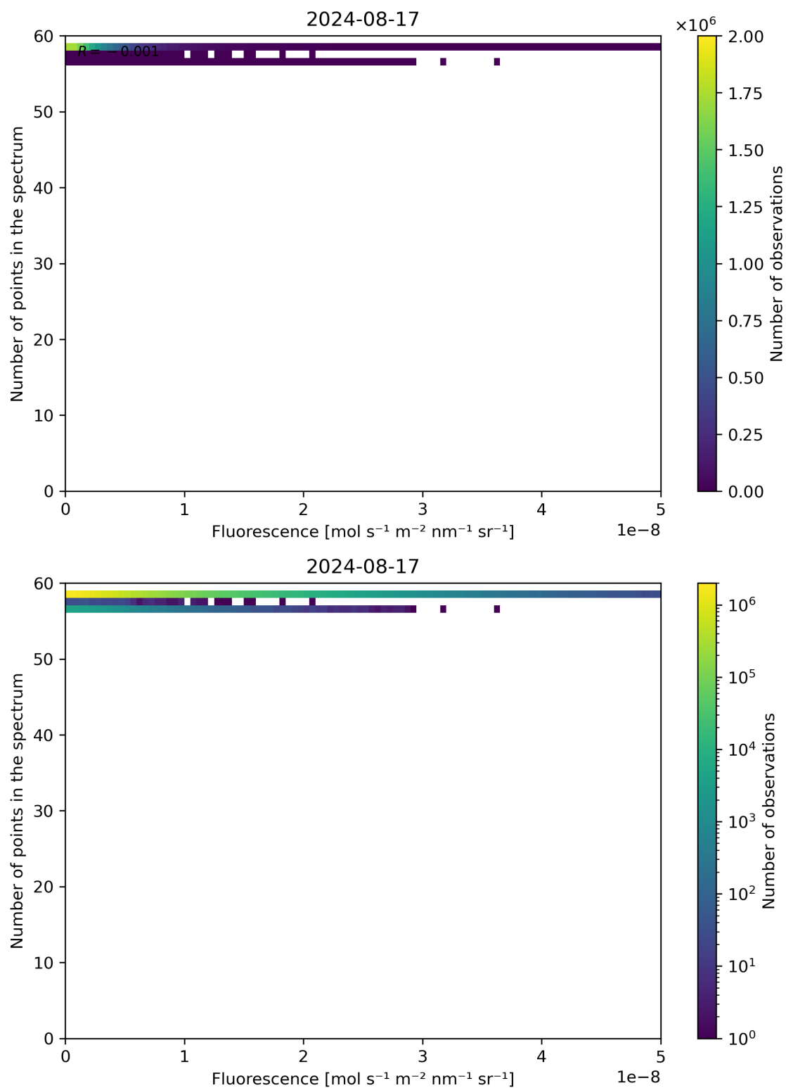
Figure 86: Scatter density plot of “Fluorescence” against “Number of points in the spectrum” for 2024-08-16 to 2024-08-18.
