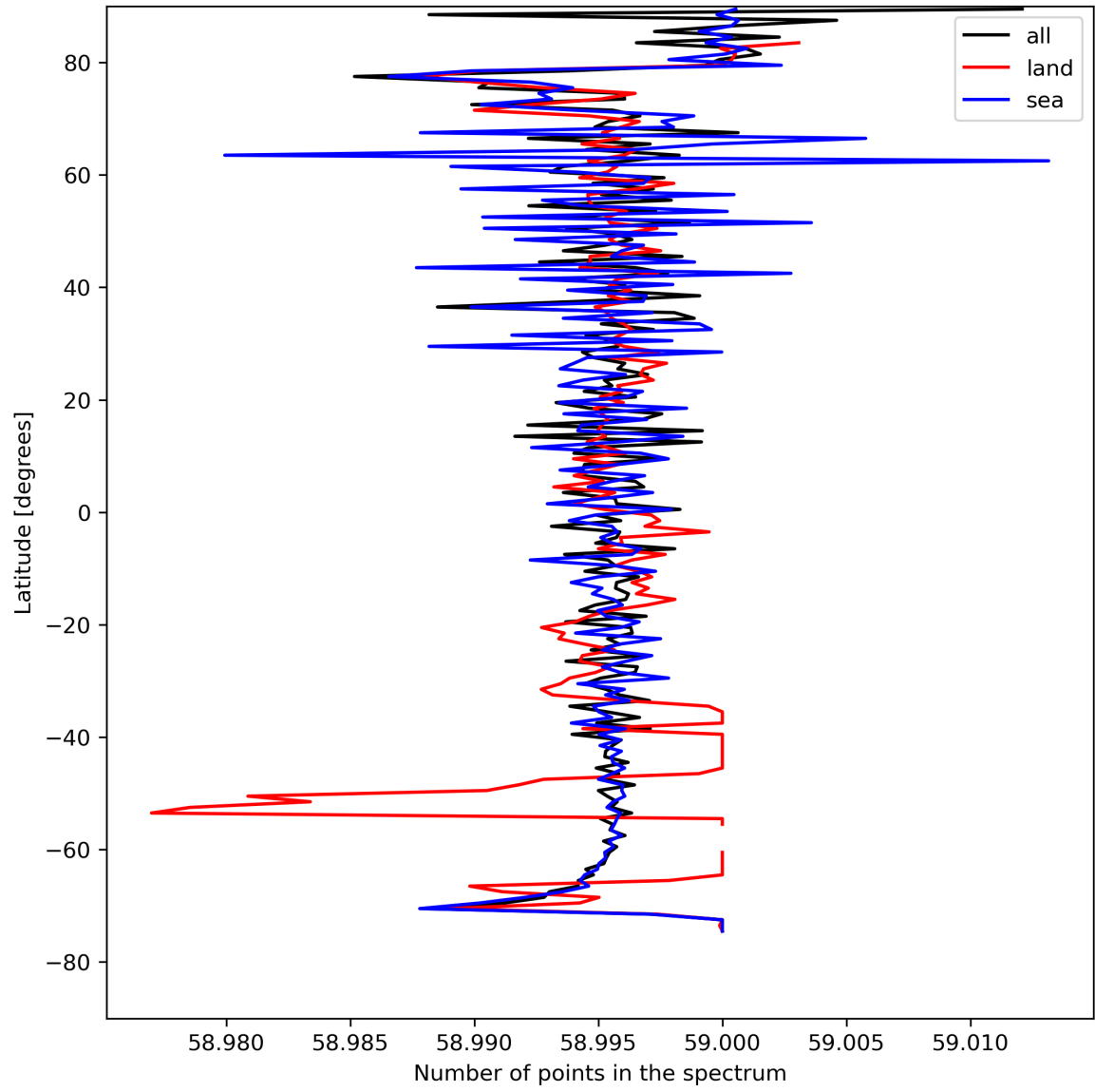
Figure 27: Zonal average of “Number of points in the spectrum” for 2024-08-16 to 2024-08-18.
