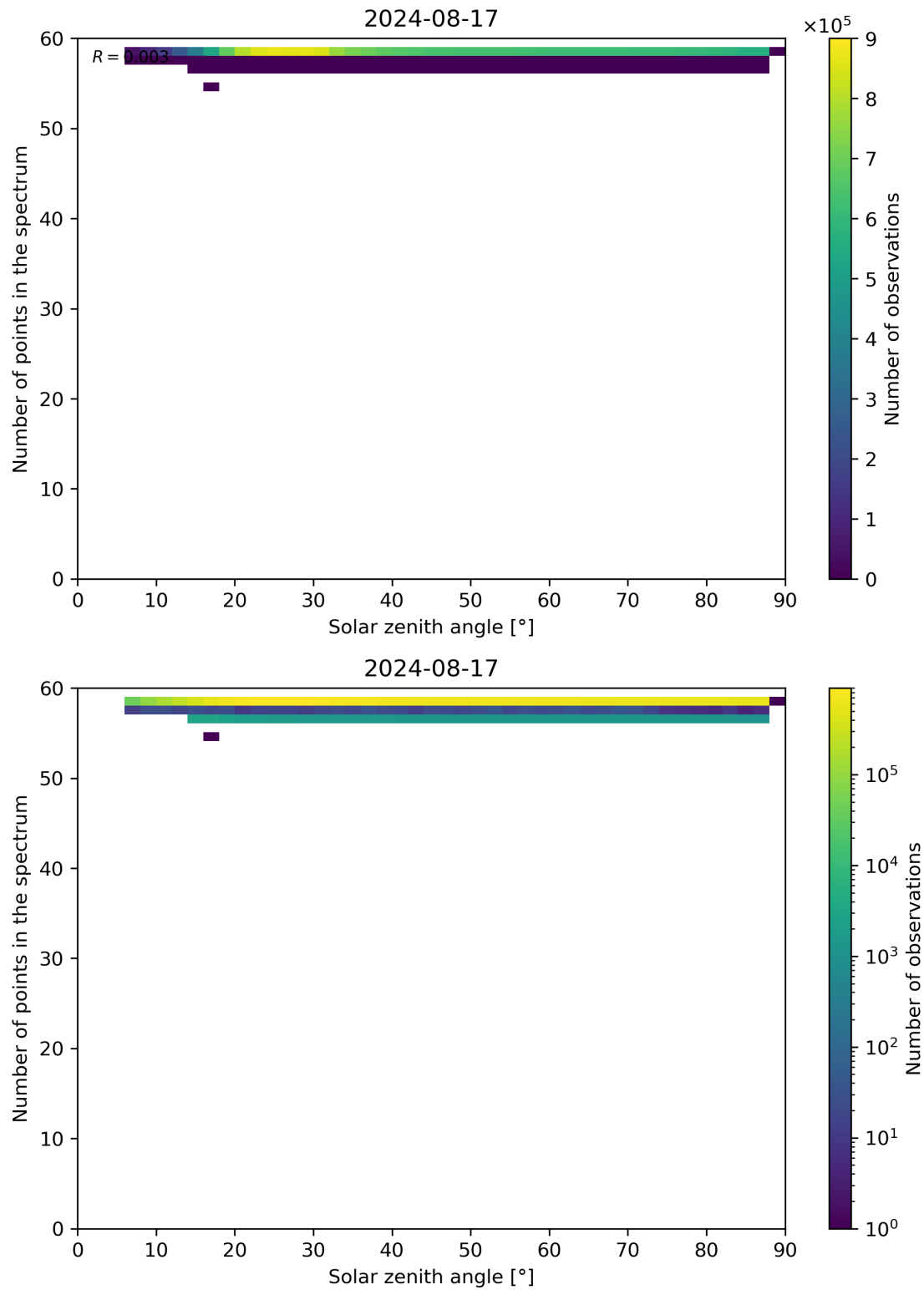
Figure 115: Scatter density plot of “Solar zenith angle” against “Number of points in the spectrum” for 2024-08-16 to 2024-08-18.
