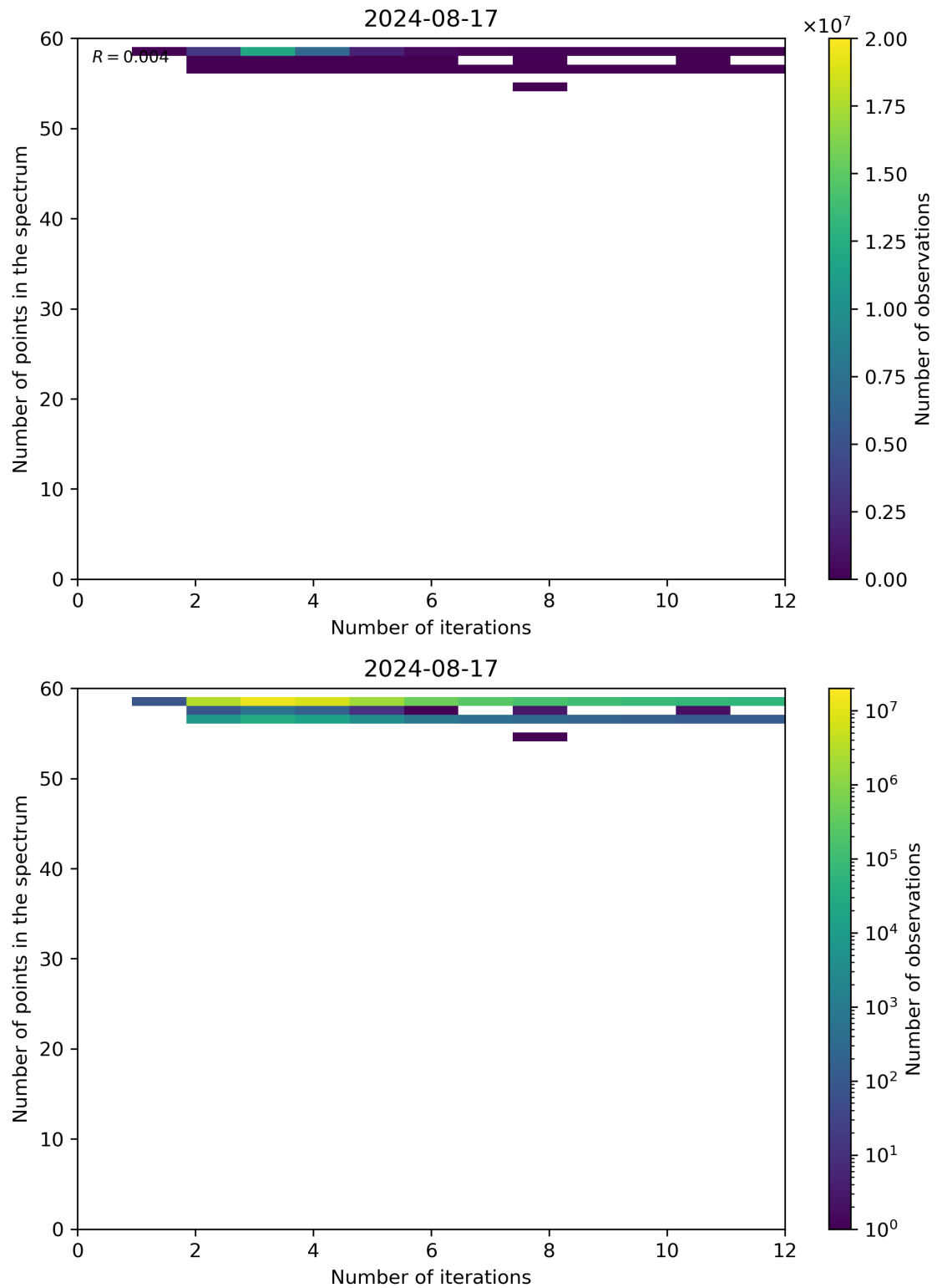
Figure 99: Scatter density plot of “Number of iterations” against “Number of points in the spectrum” for 2024-08-16 to 2024-08-18.
