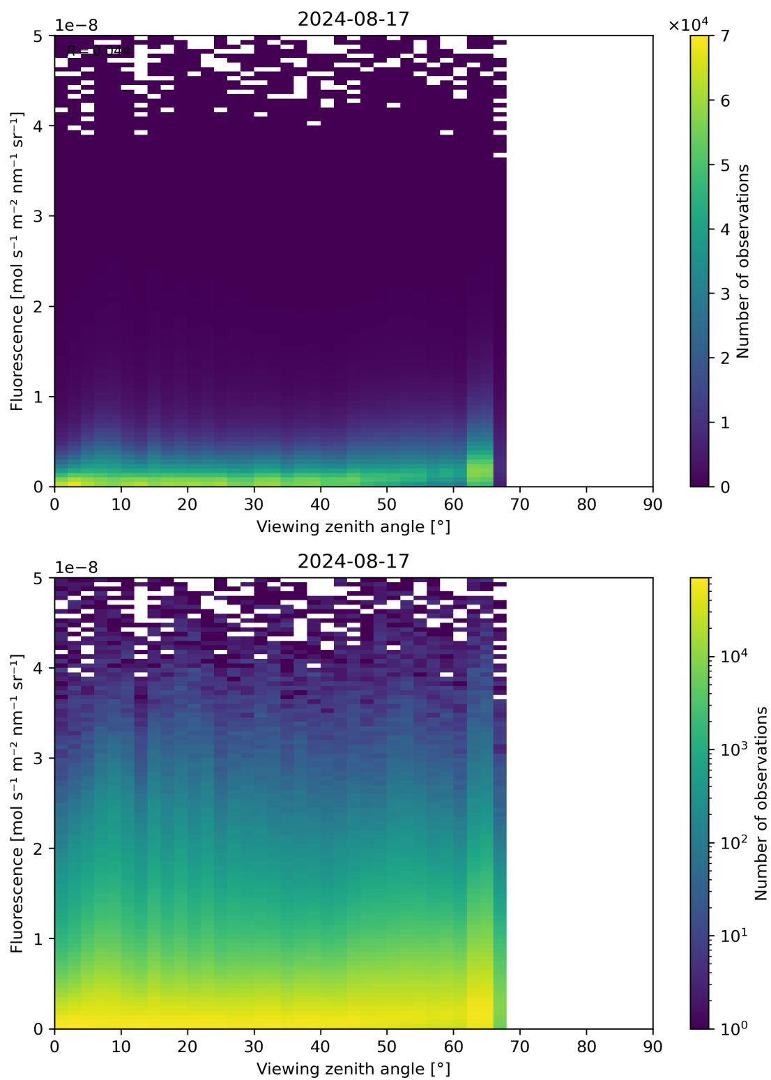
Figure 122: Scatter density plot of “Viewing zenith angle” against “Fluorescence” for 2024-08-16 to 2024-08-18.
