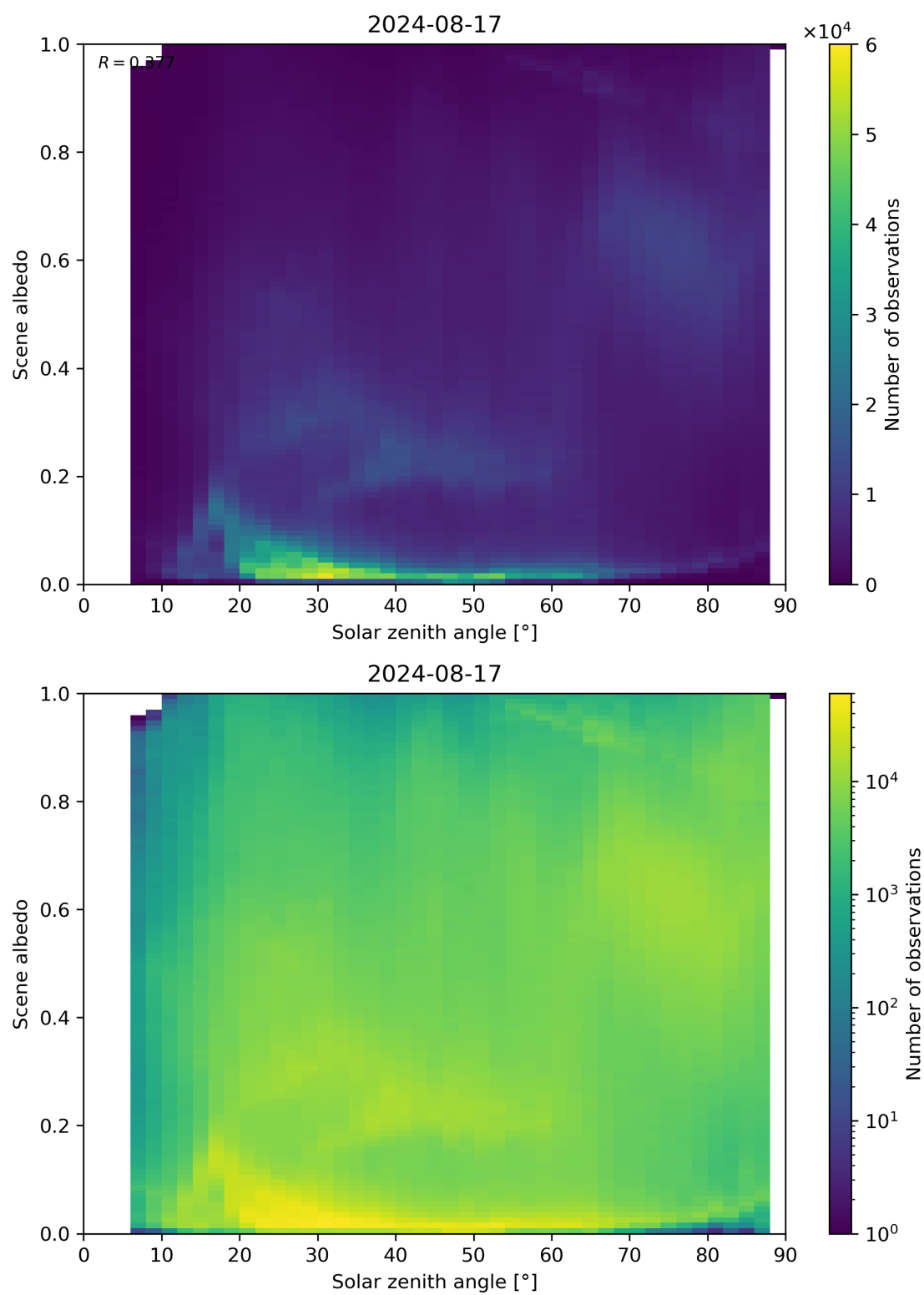
Figure 116: Scatter density plot of “Solar zenith angle” against “Scene albedo” for 2024-08-16 to 2024-08-18.
