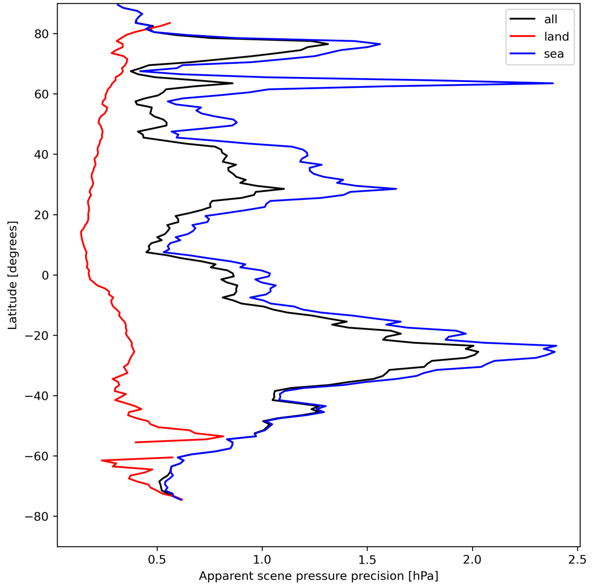
Figure 20: Zonal average of “Apparent scene pressure precision” for 2024-08-16 to 2024-08-18.
