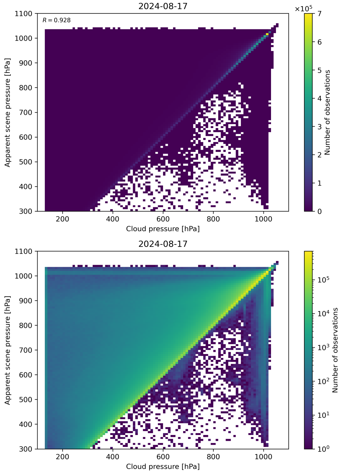
Figure 77: Scatter density plot of “Cloud pressure” against “Apparent scene pressure” for 2024-08-16 to 2024-08-18.
