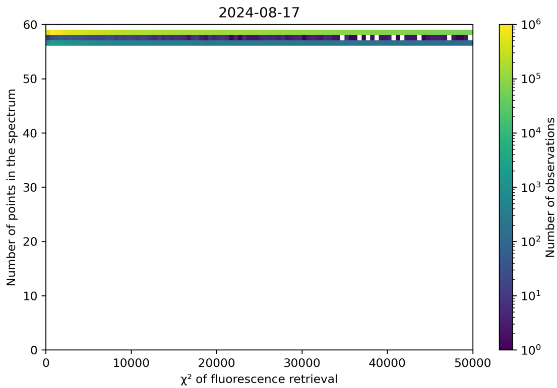
Figure 68: Scatter density plot of “ \chi^2 of fluorescence retrieval” against “Number of points in the spectrum” for 2024-08-16 to 2024-08-18.
