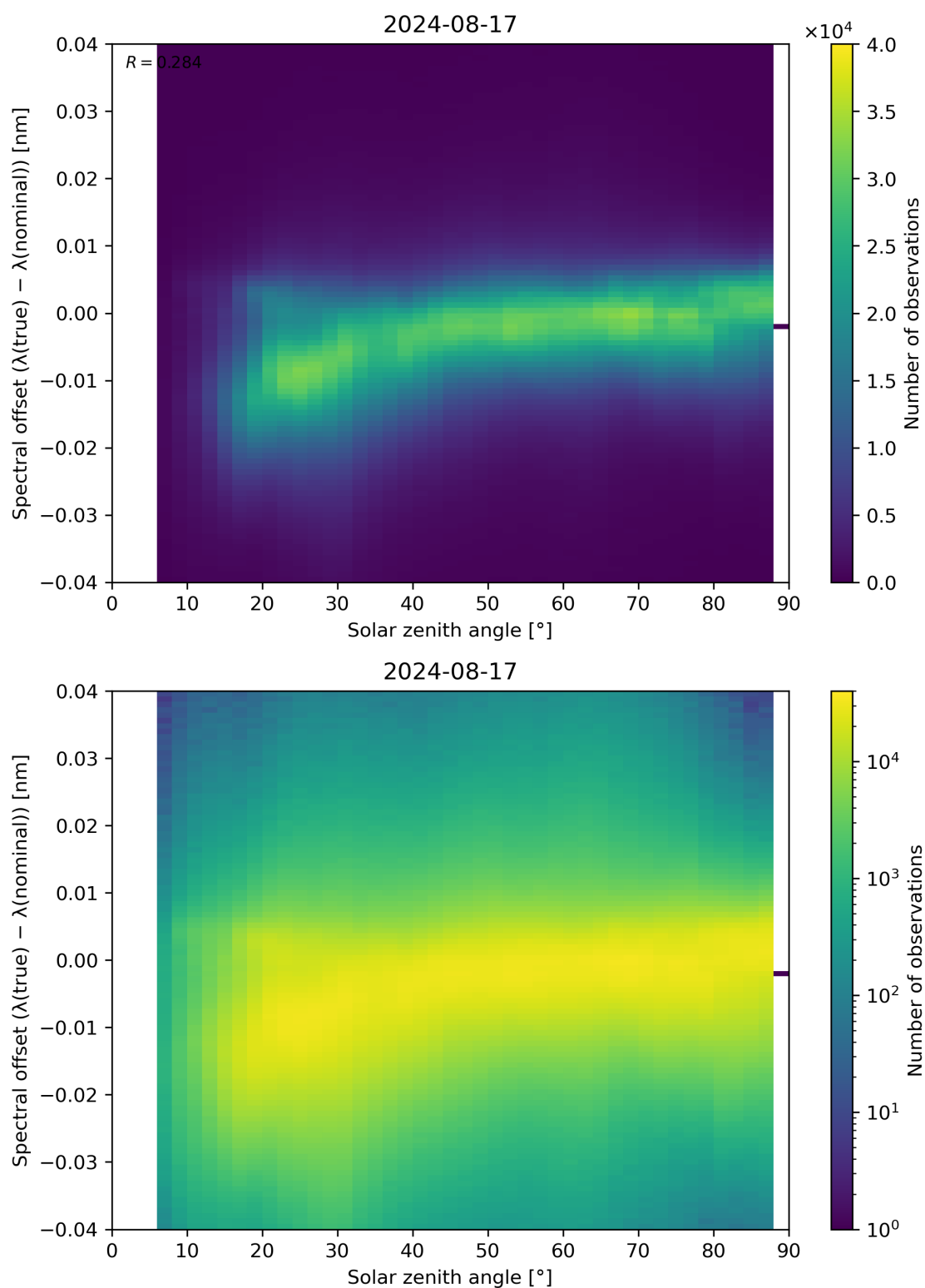
Figure 117: Scatter density plot of “Solar zenith angle” against “Spectral offset ( \lambda(\text{true}) - \lambda(\text{nominal}) )” for 2024-08-16 to 2024-08-18.
