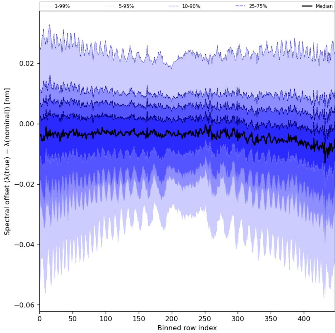
Figure 62: Along track statistics of “Spectral offset ( \lambda(\text{true}) - \lambda(\text{nominal}) )” for 2024-08-16 to 2024-08-18
