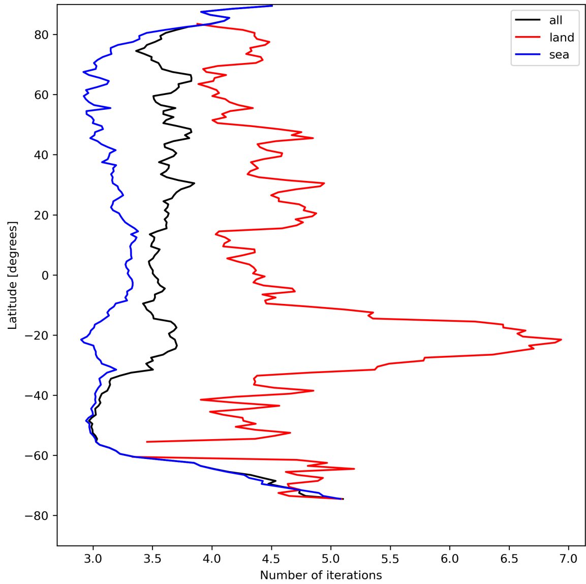
Figure 22: Zonal average of “Number of iterations” for 2024-08-16 to 2024-08-18.
