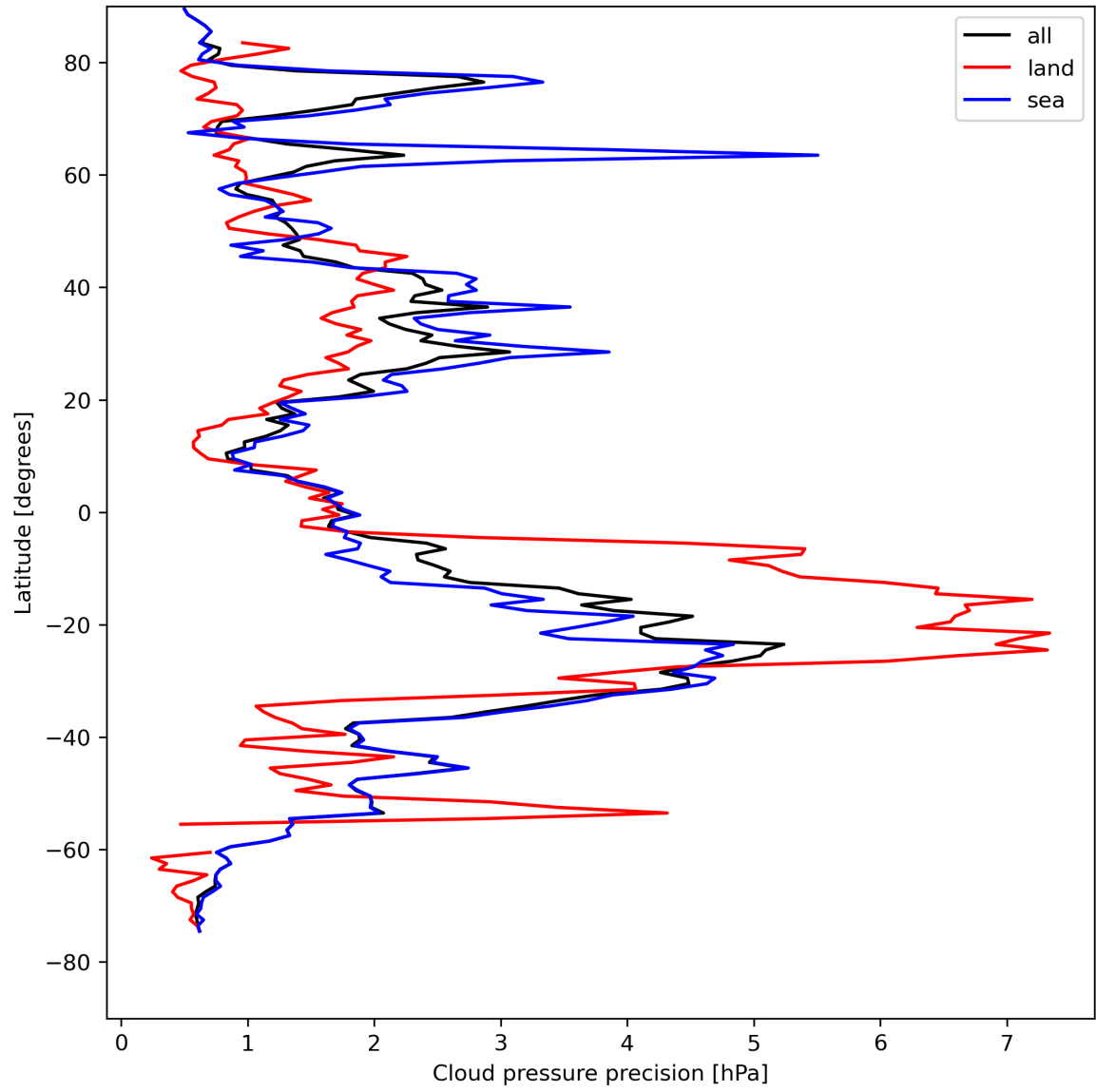
Figure 14: Zonal average of “Cloud pressure precision” for 2024-08-16 to 2024-08-18.
