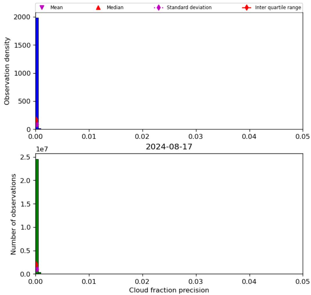
Figure 33: Histogram of “Cloud fraction precision” for 2024-08-16 to 2024-08-18
