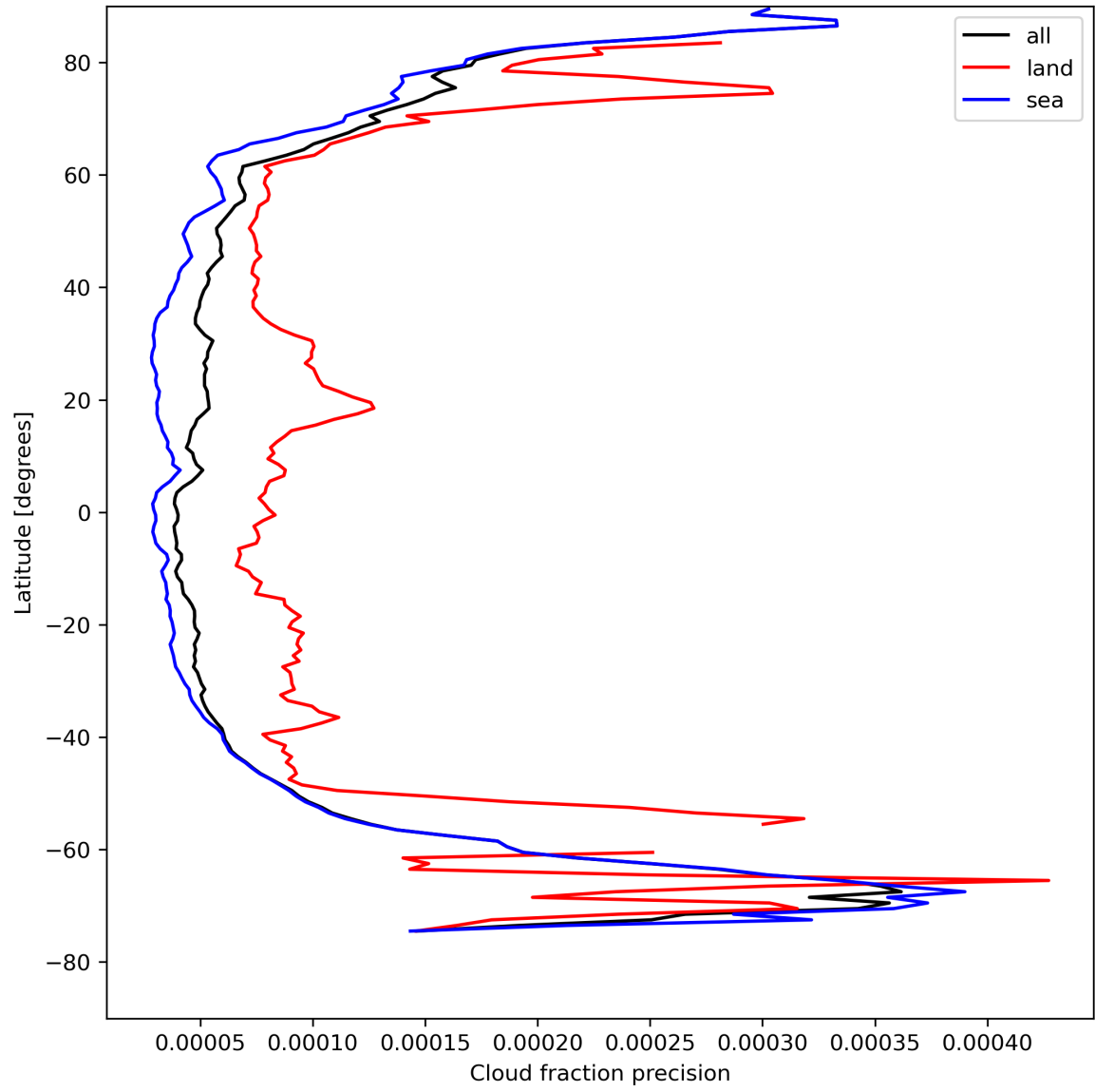
Figure 16: Zonal average of “Cloud fraction precision” for 2024-08-16 to 2024-08-18.
