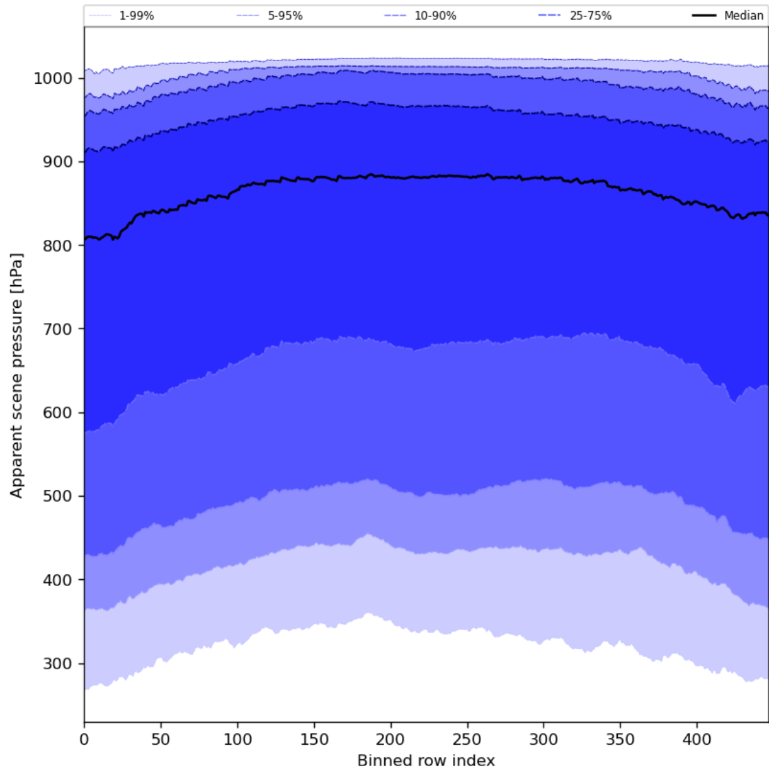
Figure 53: Along track statistics of “Apparent scene pressure” for 2024-08-16 to 2024-08-18
