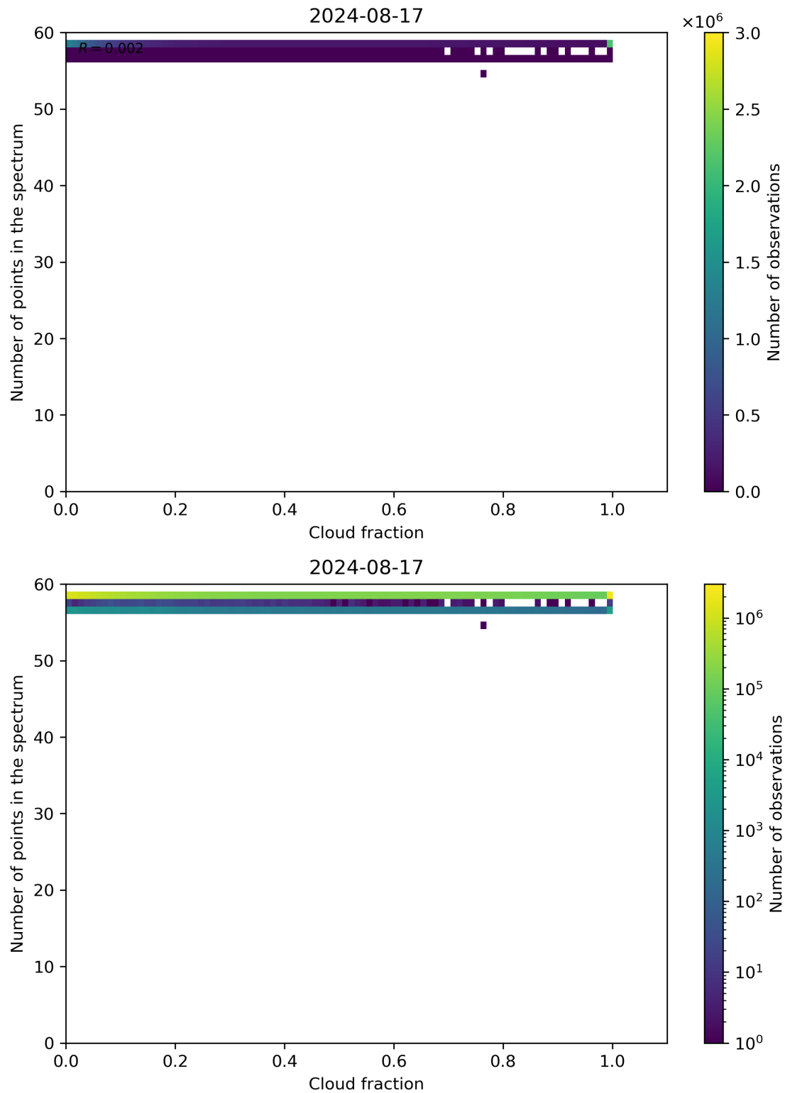
Figure 74: Scatter density plot of “Cloud fraction” against “Number of points in the spectrum” for 2024-08-16 to 2024-08-18.
