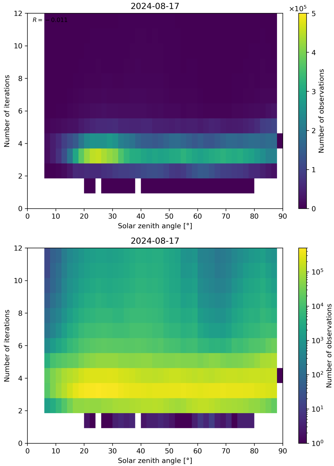
Figure 114: Scatter density plot of “Solar zenith angle” against “Number of iterations” for 2024-08-16 to 2024-08-18.
