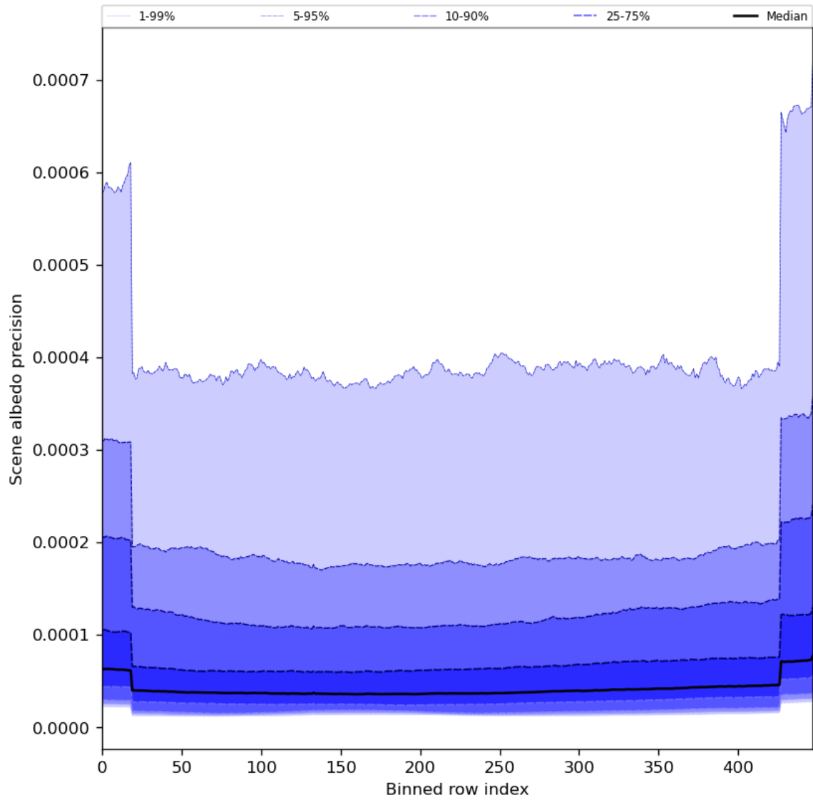
Figure 52: Along track statistics of “Scene albedo precision” for 2024-08-16 to 2024-08-18
