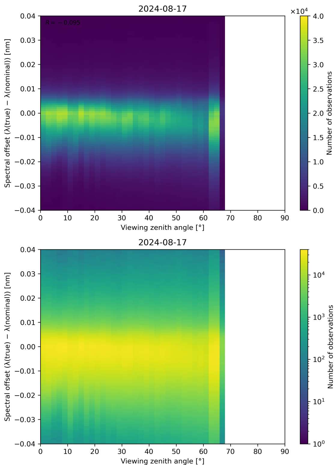
Figure 128: Scatter density plot of “Viewing zenith angle” against “Spectral offset ( \lambda(\text{true}) - \lambda(\text{nominal}) )” for 2024-08-16 to 2024-08-18.
