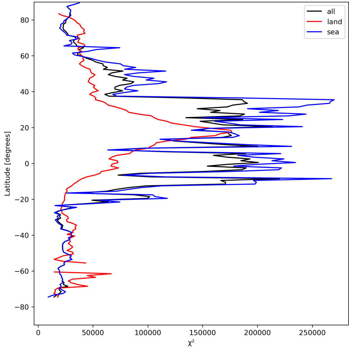
Figure 21: Zonal average of “ \chi^2 ” for 2024-08-16 to 2024-08-18.
