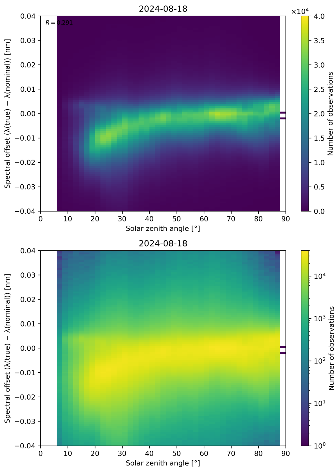
Figure 117: Scatter density plot of “Solar zenith angle” against “Spectral offset ( \lambda(\text{true}) - \lambda(\text{nominal}) )” for 2024-08-17 to 2024-08-19.
