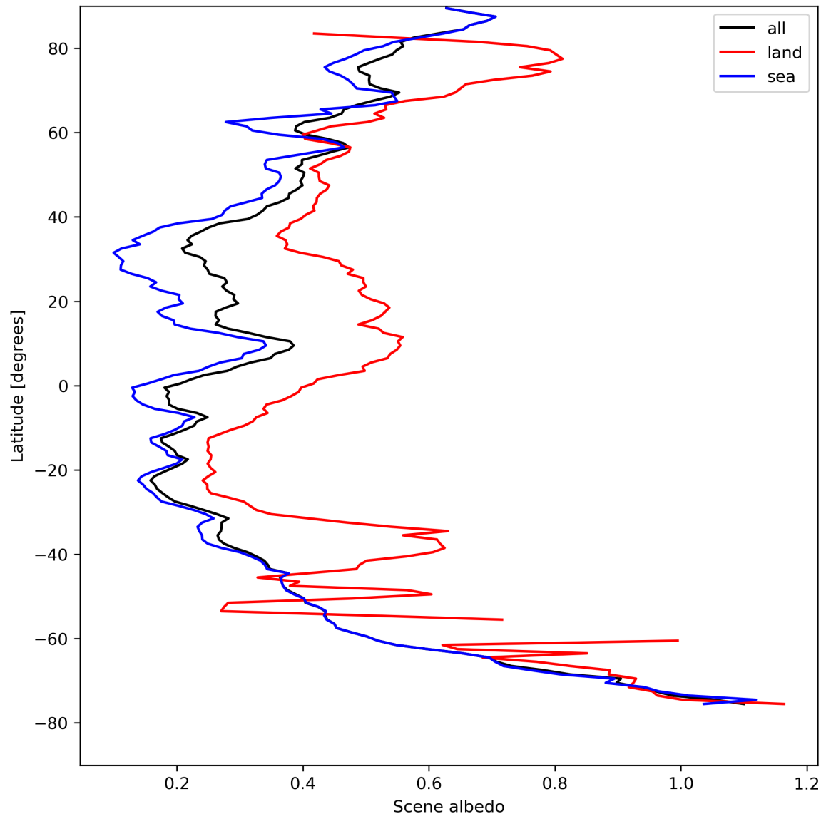
Figure 17: Zonal average of “Scene albedo” for 2024-08-17 to 2024-08-19.
