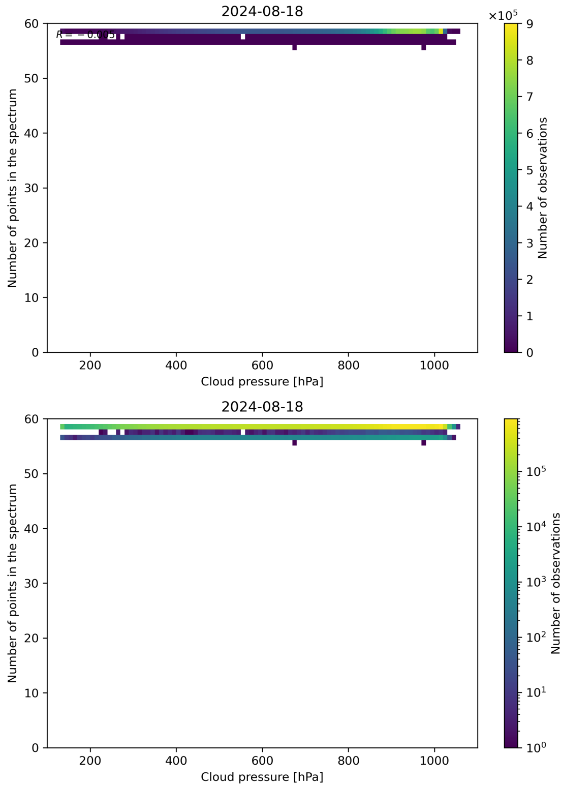
Figure 82: Scatter density plot of “Cloud pressure” against “Number of points in the spectrum” for 2024-08-17 to 2024-08-19.
