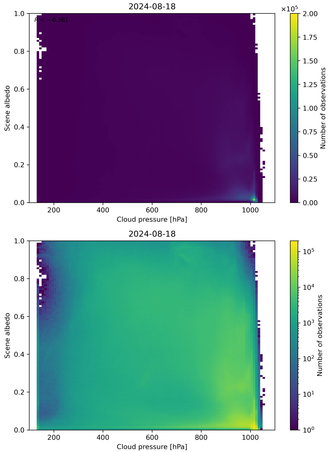
Figure 83: Scatter density plot of “Cloud pressure” against “Scene albedo” for 2024-08-17 to 2024-08-19.
