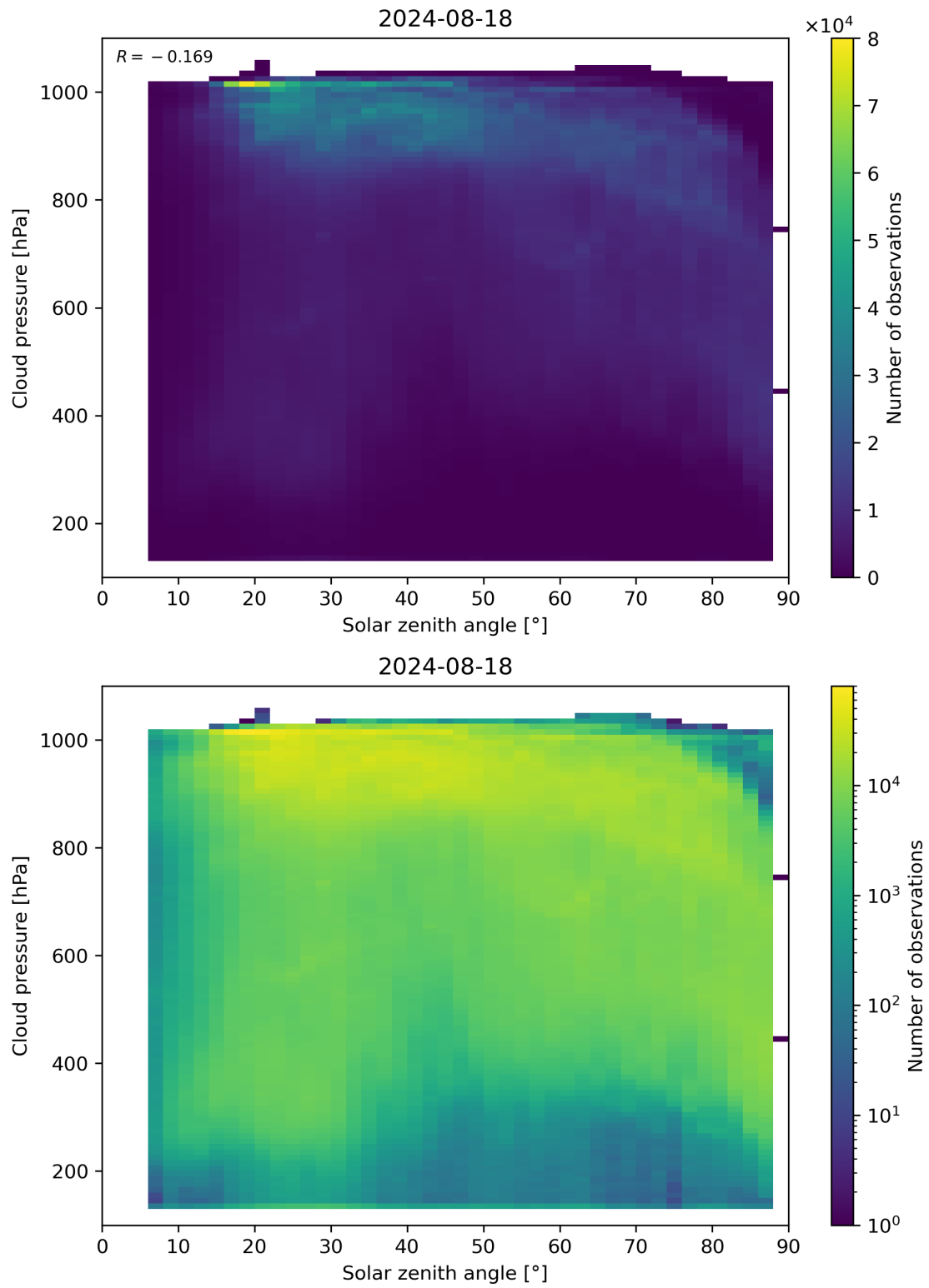
Figure 111: Scatter density plot of “Solar zenith angle” against “Cloud pressure” for 2024-08-17 to 2024-08-19.
