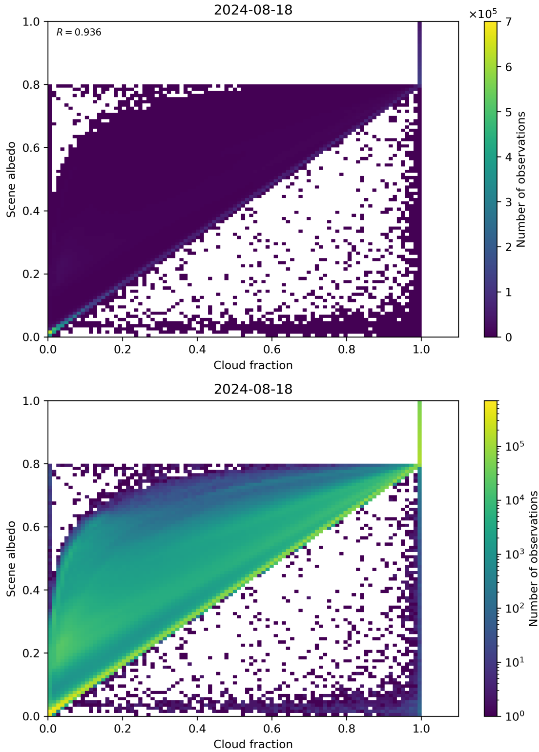
Figure 75: Scatter density plot of “Cloud fraction” against “Scene albedo” for 2024-08-17 to 2024-08-19.
