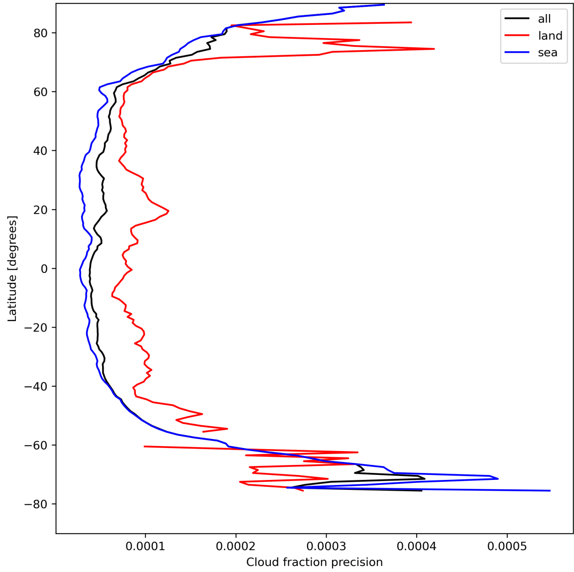
Figure 16: Zonal average of “Cloud fraction precision” for 2024-08-17 to 2024-08-19.
