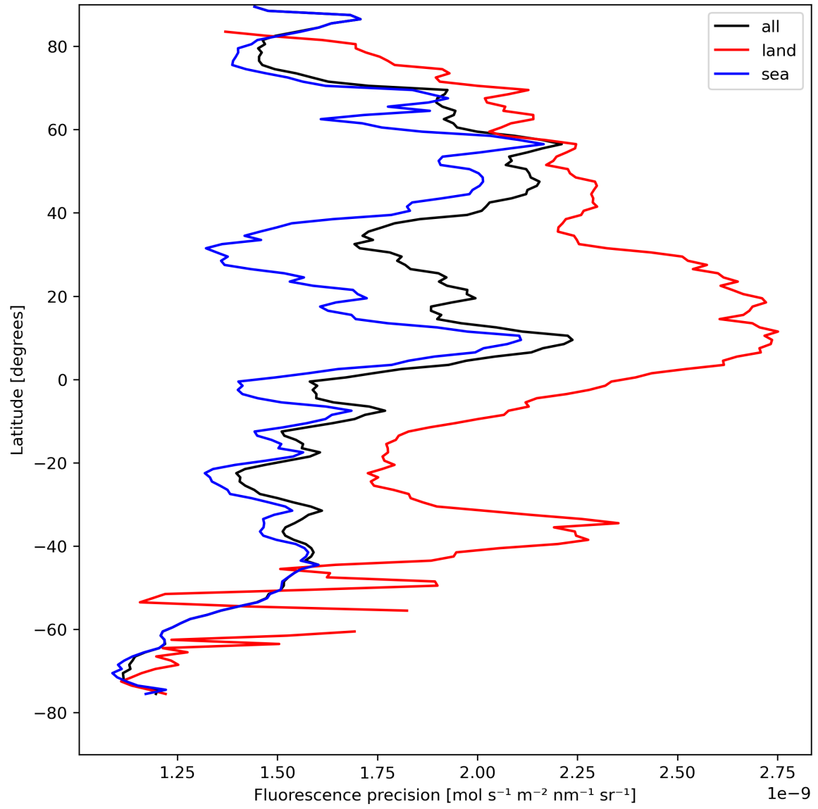
Figure 24: Zonal average of “Fluorescence precision” for 2024-08-17 to 2024-08-19.
