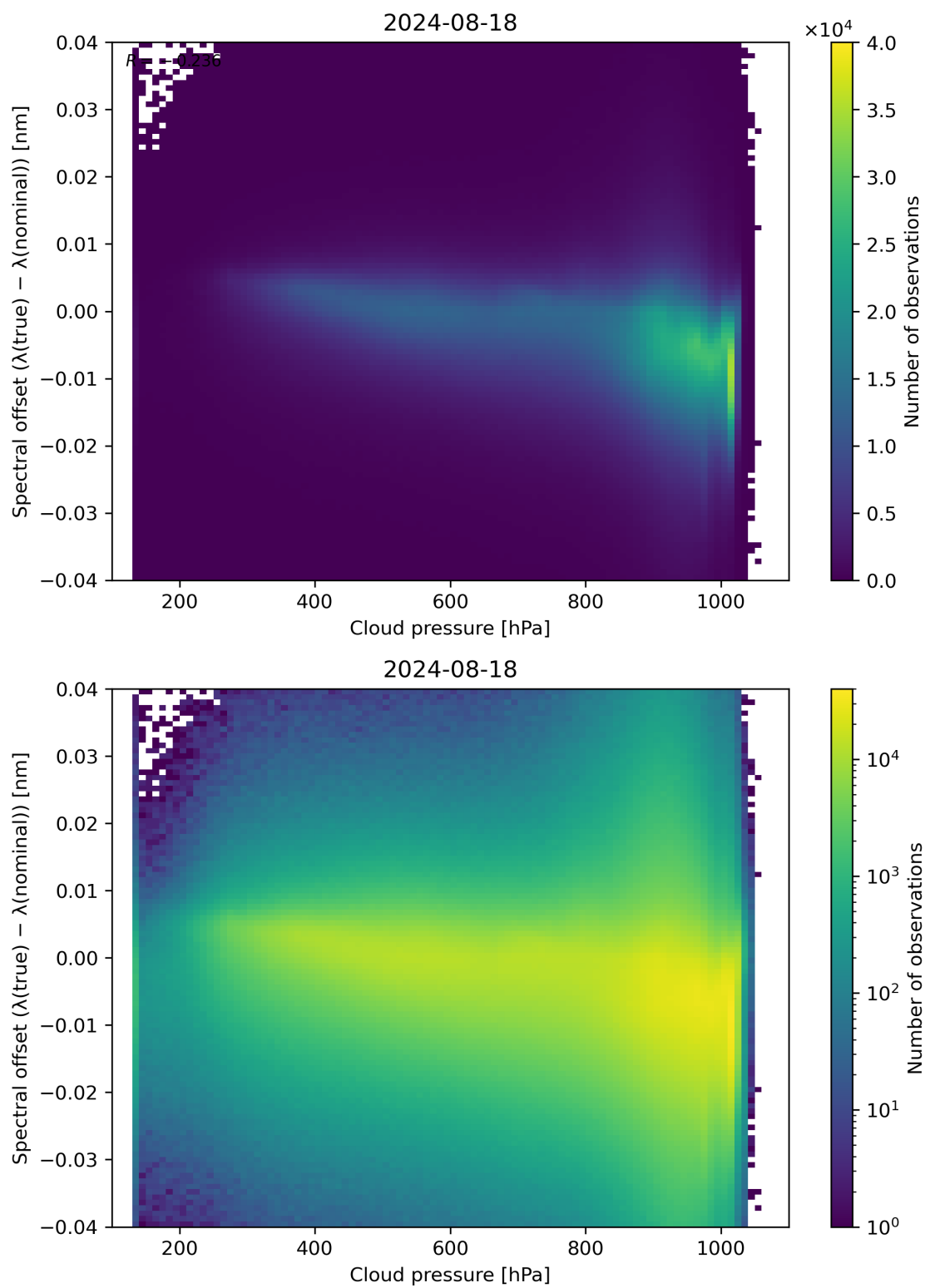
Figure 84: Scatter density plot of “Cloud pressure” against “Spectral offset ( \lambda(\text{true}) - \lambda(\text{nominal}) )” for 2024-08-17 to 2024-08-19.
