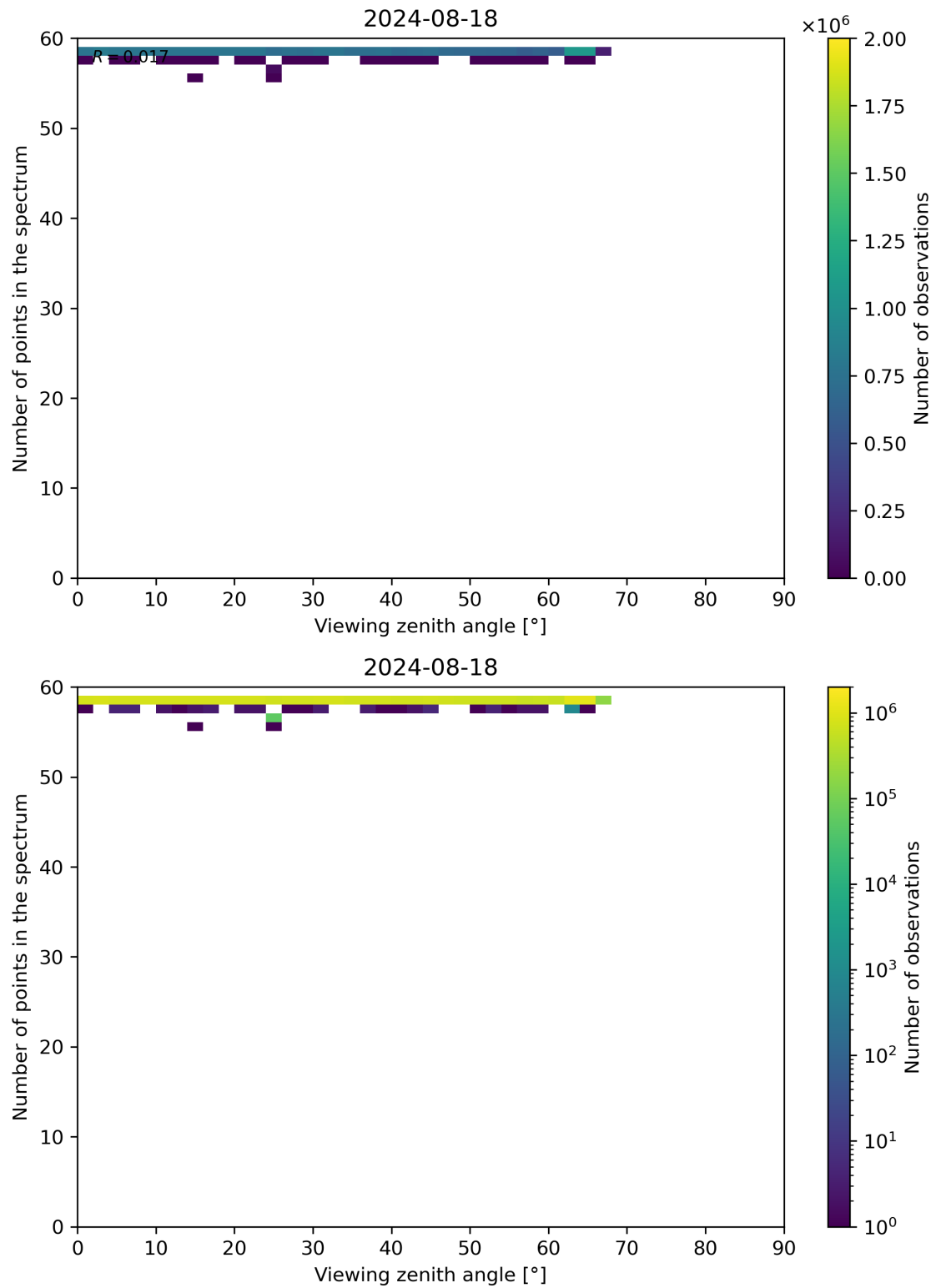
Figure 125: Scatter density plot of “Viewing zenith angle” against “Number of points in the spectrum” for 2024-08-17 to 2024-08-19.
