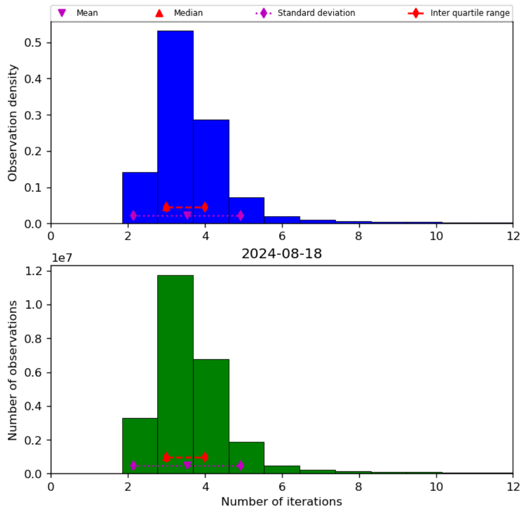
Figure 39: Histogram of “Number of iterations” for 2024-08-17 to 2024-08-19
