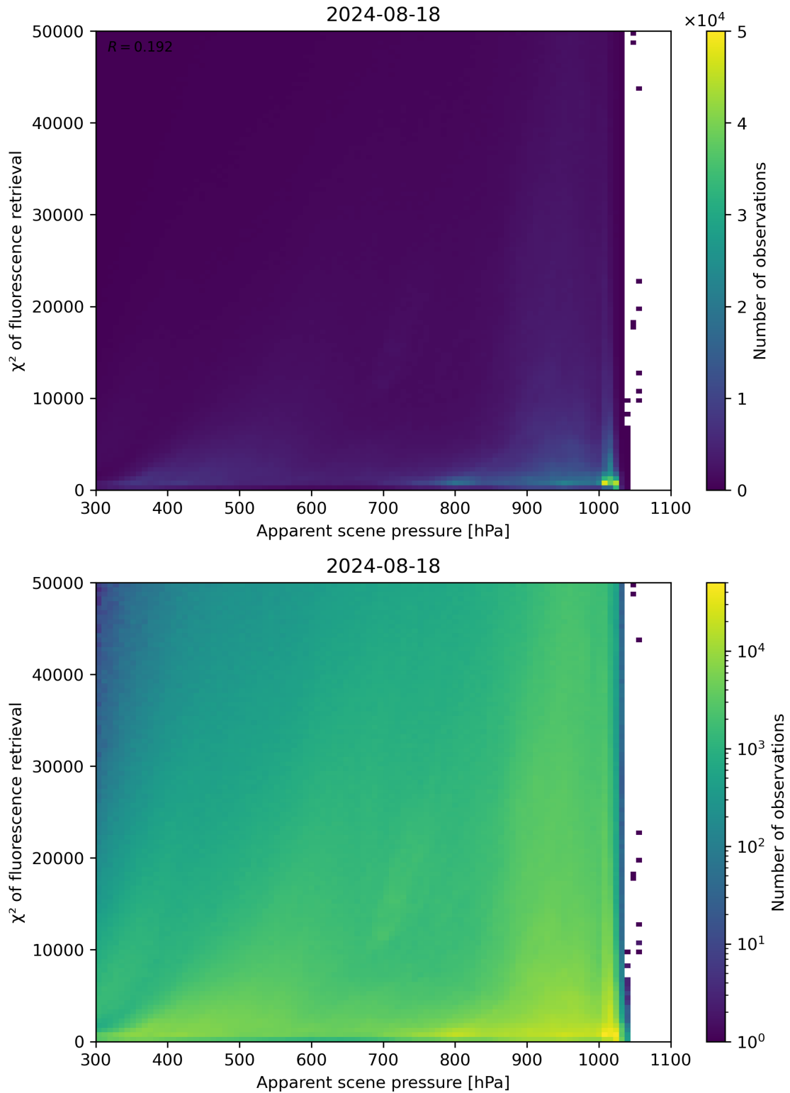
Figure 63: Scatter density plot of “Apparent scene pressure” against “ \chi^2 of fluorescence retrieval” for 2024-08-17 to 2024-08-19.
