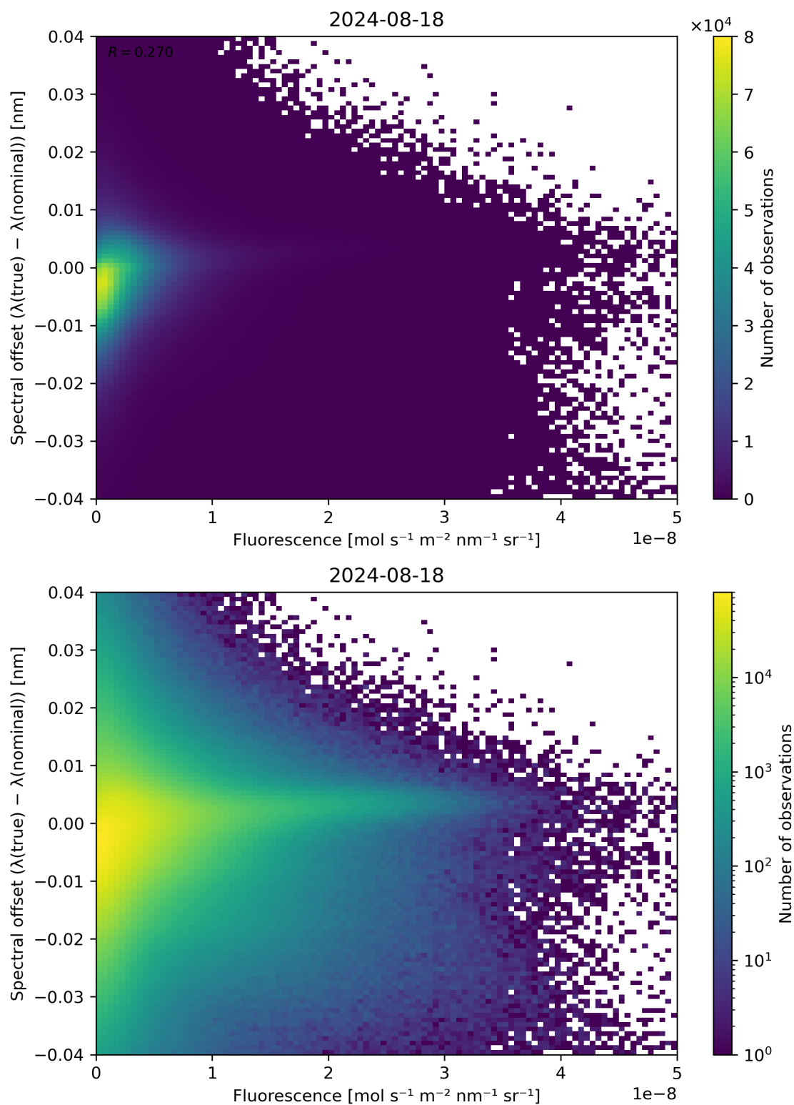
Figure 87: Scatter density plot of “Fluorescence” against “Spectral offset ( \lambda(\text{true}) - \lambda(\text{nominal}) )” for 2024-08-17 to 2024-08-19.
