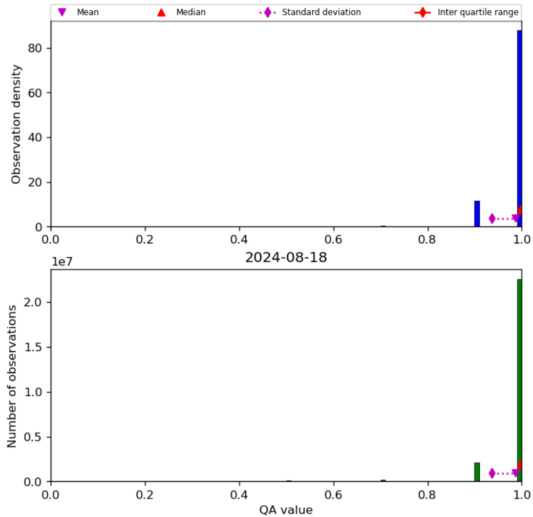
Figure 29: Histogram of “QA value” for 2024-08-17 to 2024-08-19
