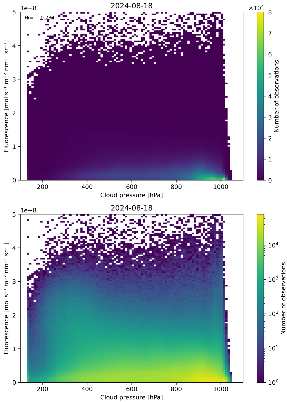
Figure 80: Scatter density plot of “Cloud pressure” against “Fluorescence” for 2024-08-17 to 2024-08-19.
