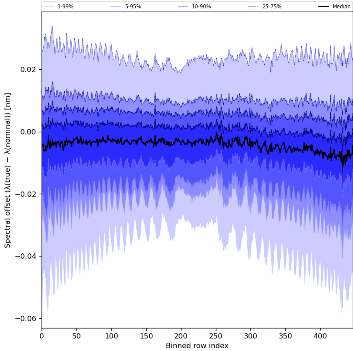
Figure 62: Along track statistics of “Spectral offset ( \lambda(\text{true}) - \lambda(\text{nominal}) )” for 2024-08-17 to 2024-08-19
