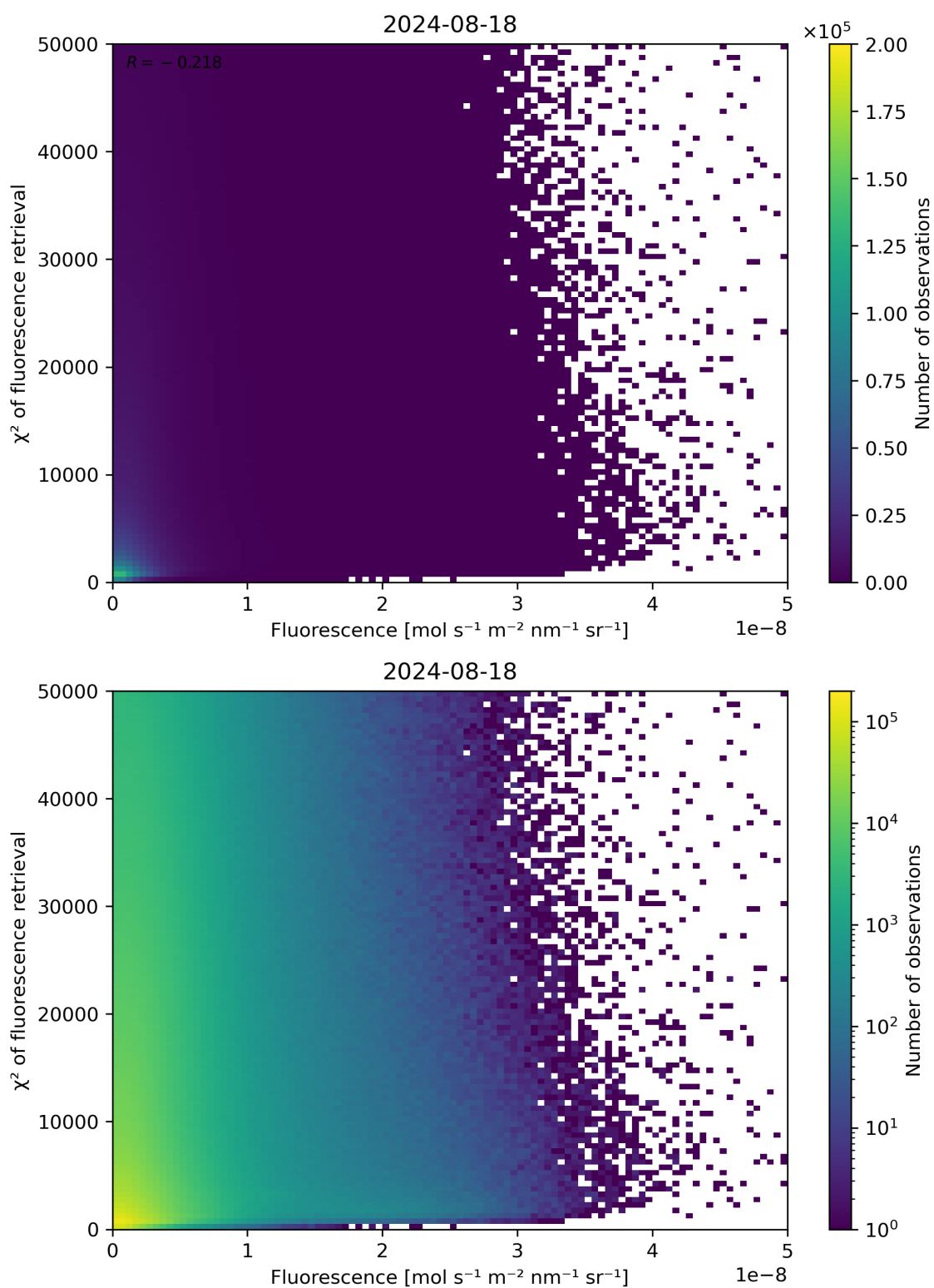
Figure 85: Scatter density plot of “Fluorescence” against “ \chi^2 of fluorescence retrieval” for 2024-08-17 to 2024-08-19.
