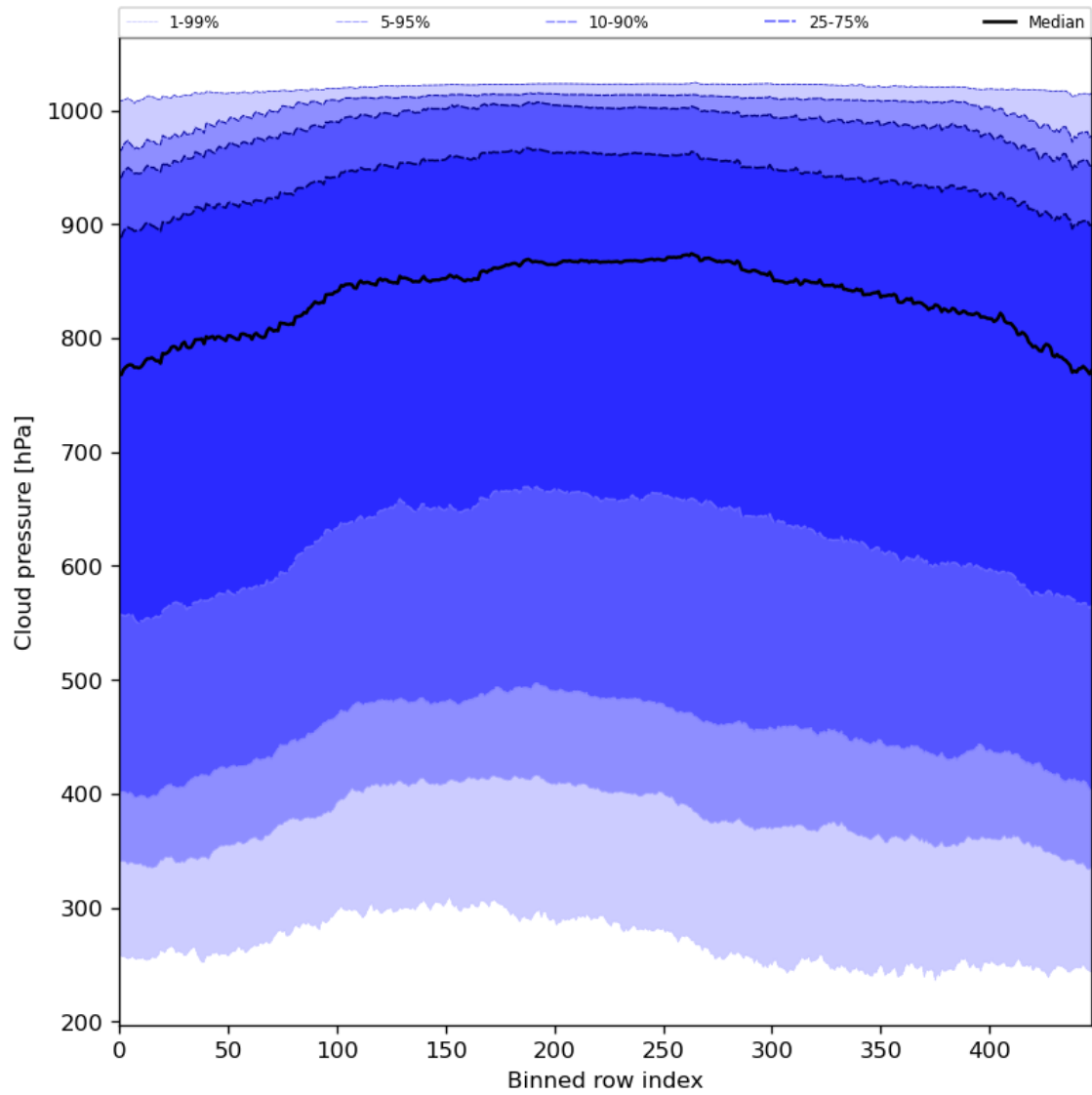
Figure 47: Along track statistics of “Cloud pressure” for 2024-08-17 to 2024-08-19
