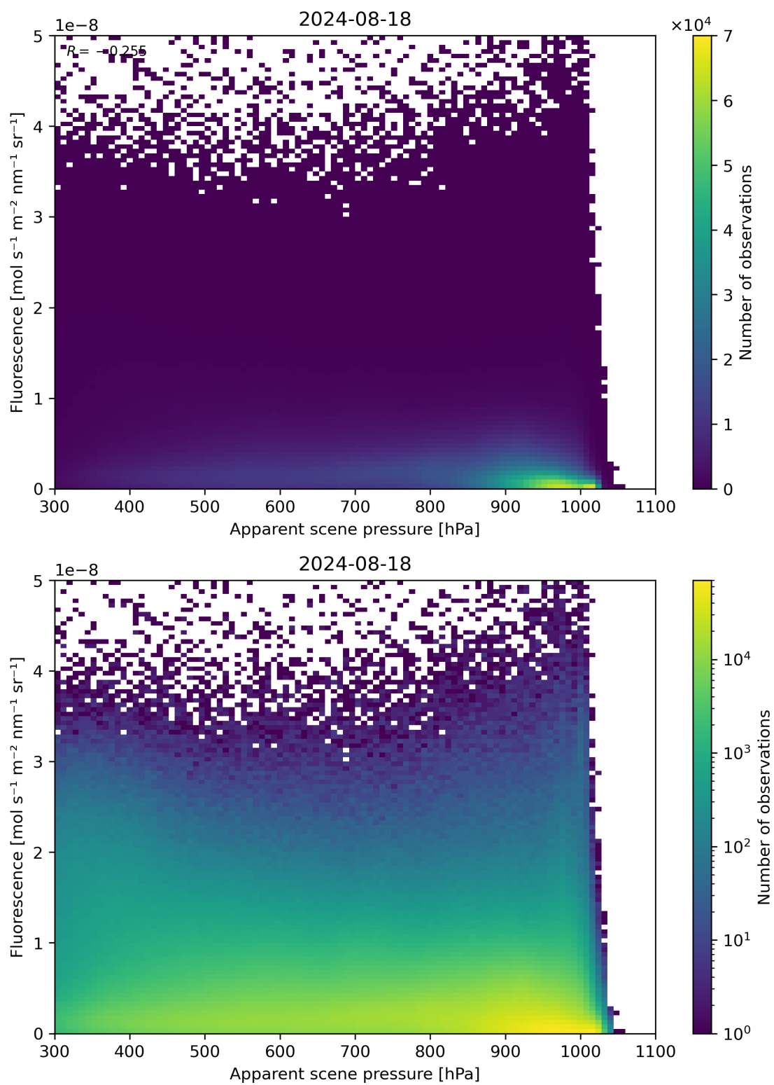
Figure 64: Scatter density plot of “Apparent scene pressure” against “Fluorescence” for 2024-08-17 to 2024-08-19.
