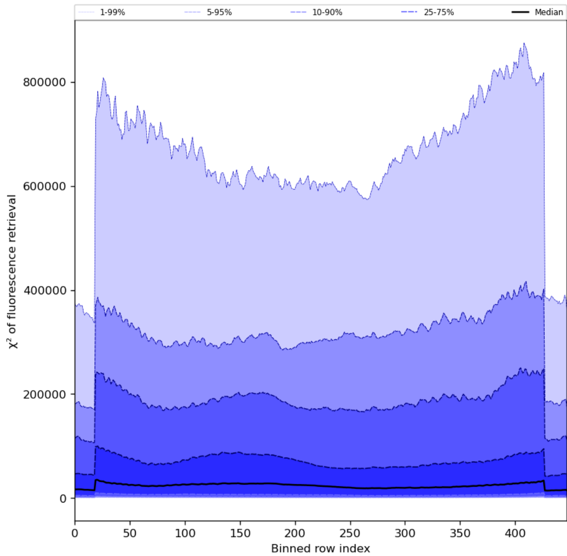
Figure 59: Along track statistics of “ \chi^2 of fluorescence retrieval” for 2024-08-17 to 2024-08-19
