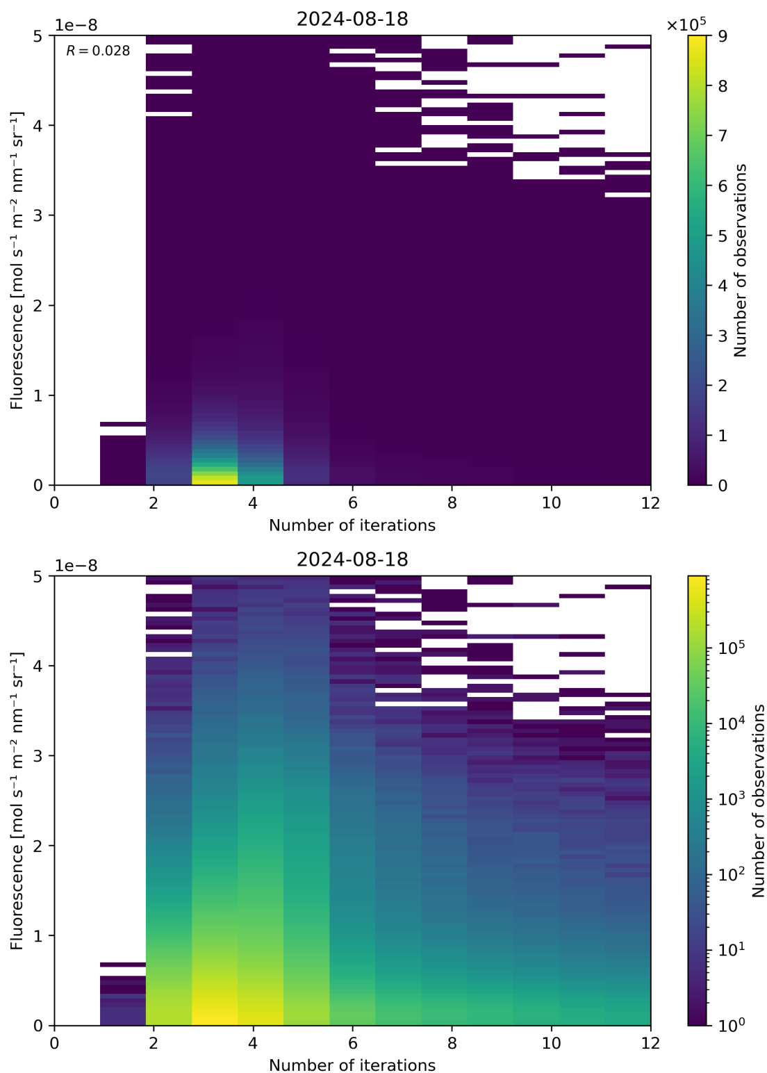
Figure 98: Scatter density plot of “Number of iterations” against “Fluorescence” for 2024-08-17 to 2024-08-19.
