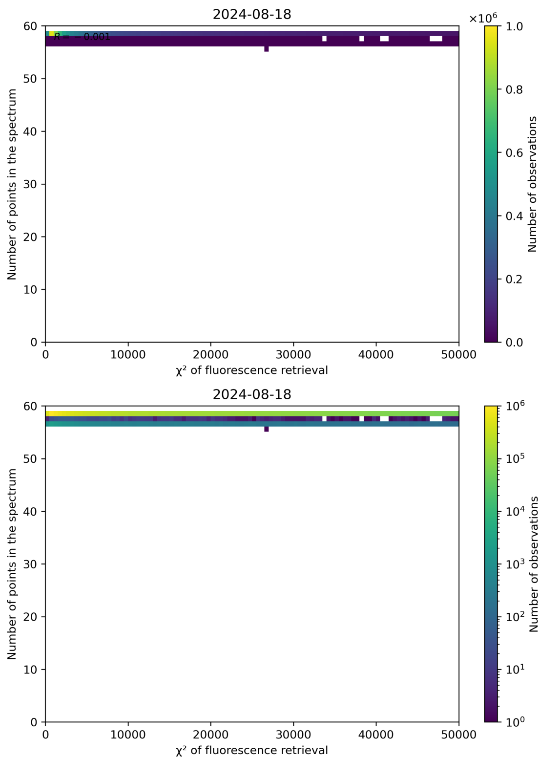
Figure 68: Scatter density plot of “ \chi^2 of fluorescence retrieval” against “Number of points in the spectrum” for 2024-08-17 to 2024-08-19.
