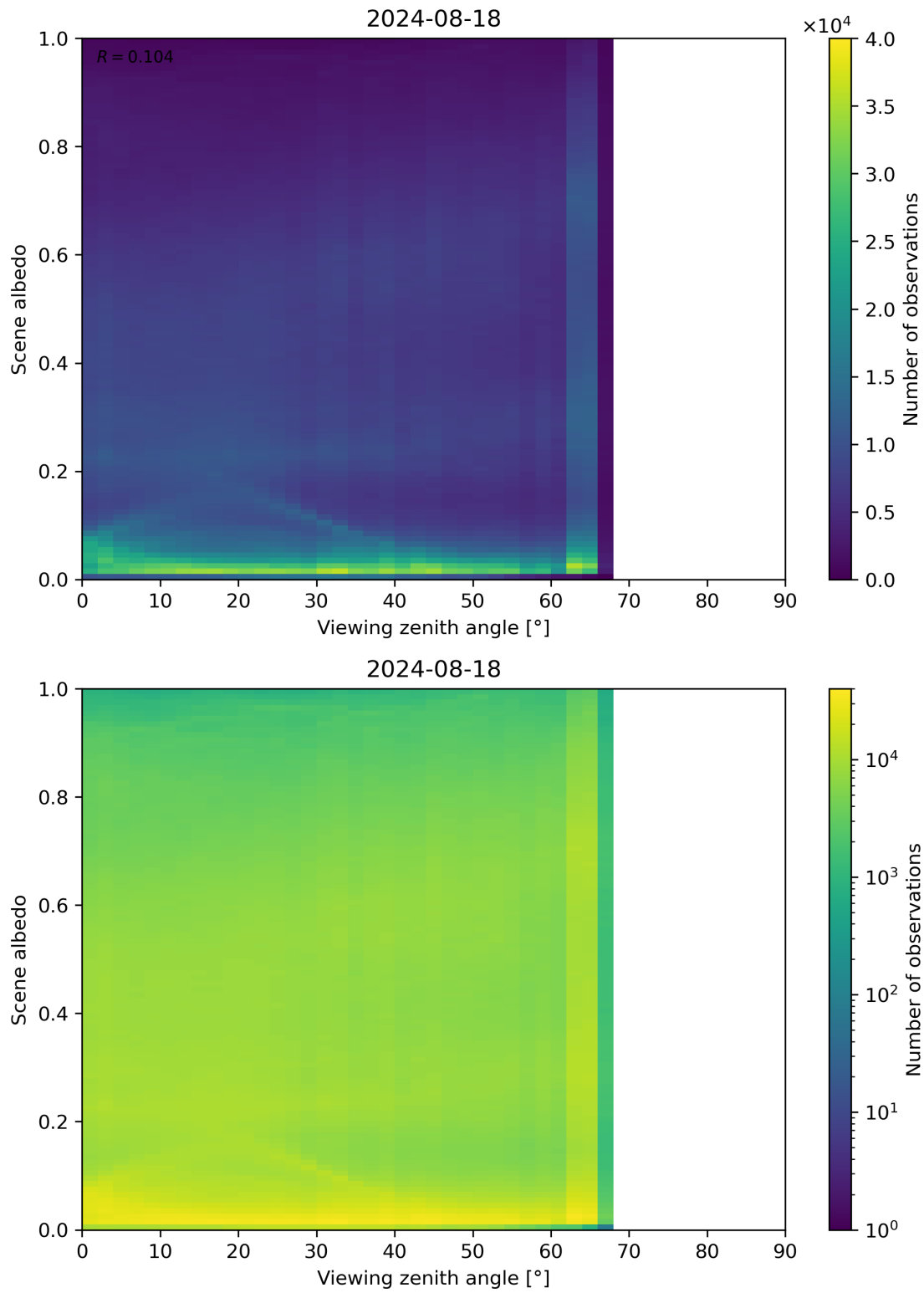
Figure 126: Scatter density plot of “Viewing zenith angle” against “Scene albedo” for 2024-08-17 to 2024-08-19.
