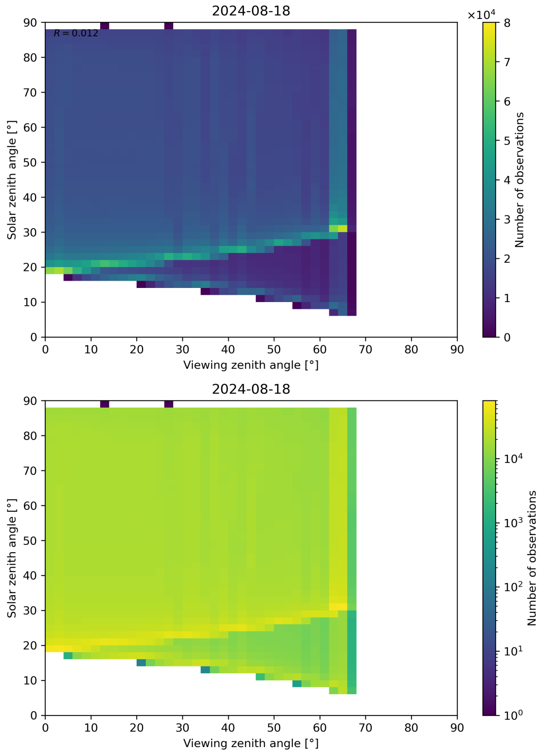
Figure 127: Scatter density plot of “Viewing zenith angle” against “Solar zenith angle” for 2024-08-17 to 2024-08-19.
