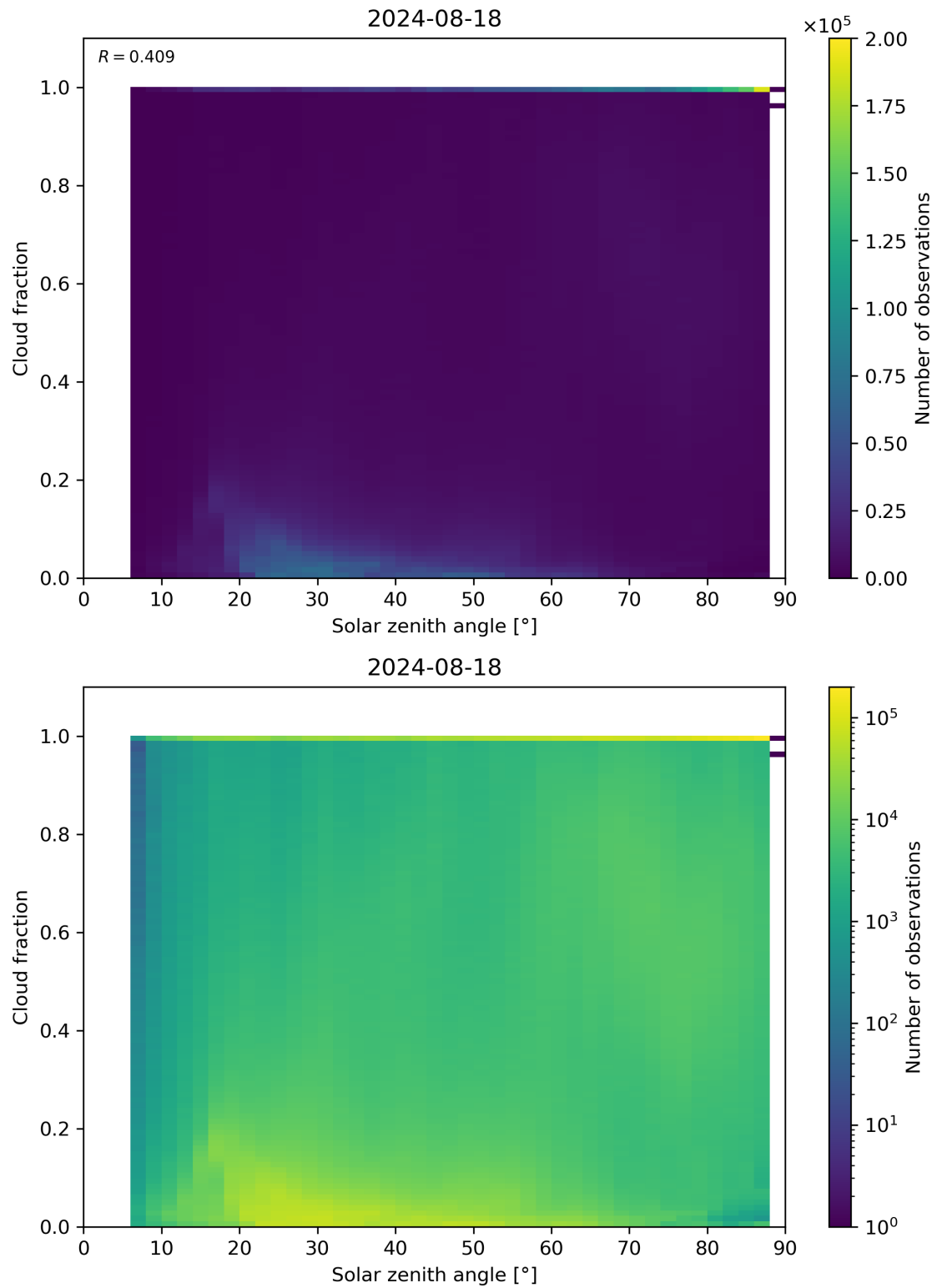
Figure 110: Scatter density plot of “Solar zenith angle” against “Cloud fraction” for 2024-08-17 to 2024-08-19.
