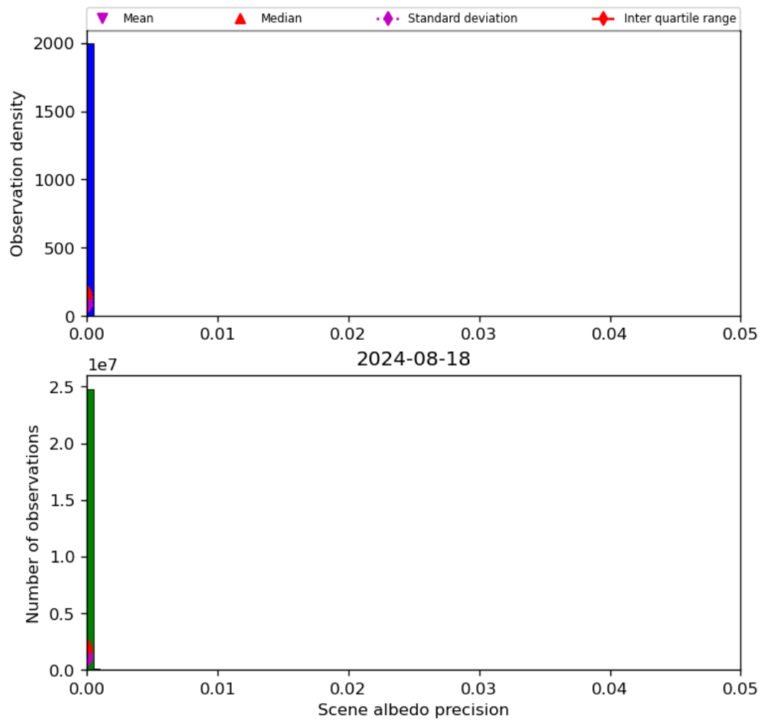
Figure 35: Histogram of “Scene albedo precision” for 2024-08-17 to 2024-08-19
