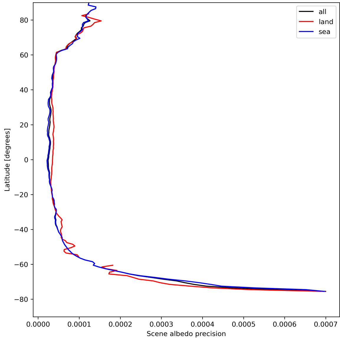
Figure 18: Zonal average of “Scene albedo precision” for 2024-08-17 to 2024-08-19.
