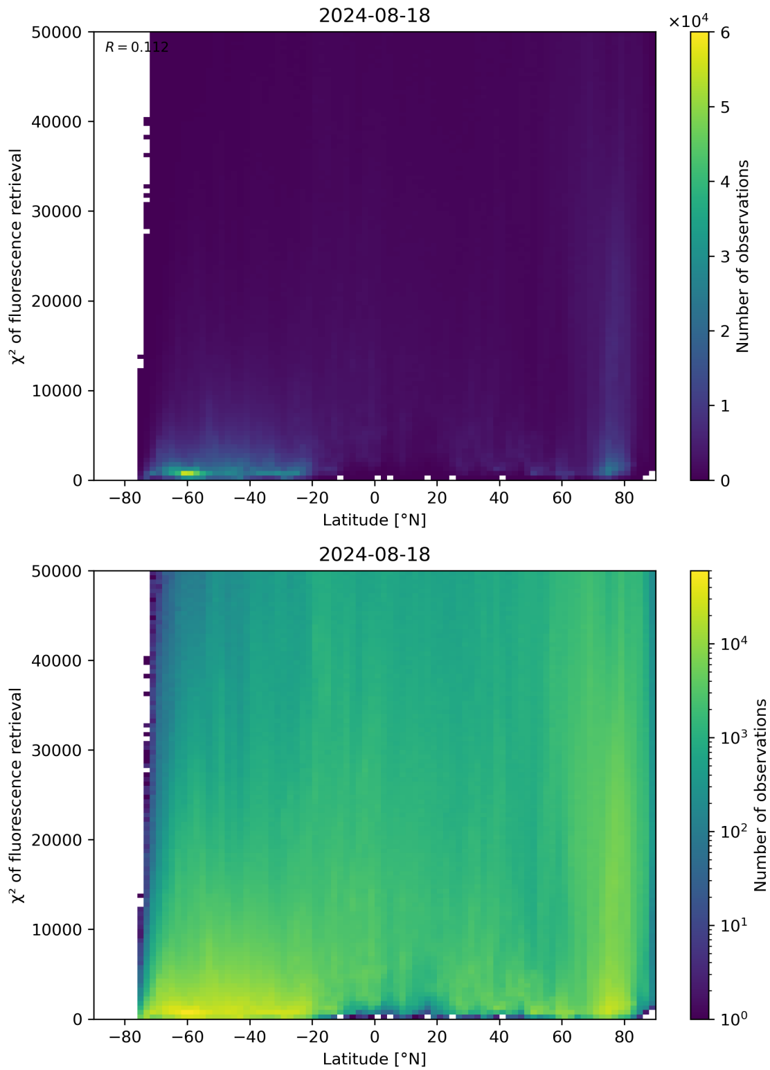
Figure 89: Scatter density plot of “Latitude” against “ \chi^2 of fluorescence retrieval” for 2024-08-17 to 2024-08-19.
