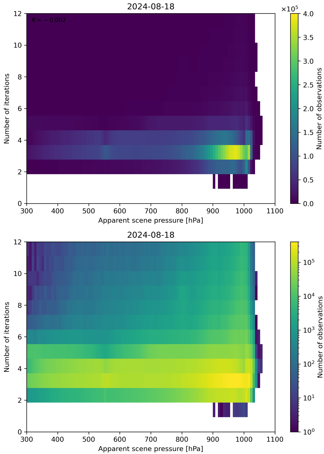
Figure 65: Scatter density plot of “Apparent scene pressure” against “Number of iterations” for 2024-08-17 to 2024-08-19.
