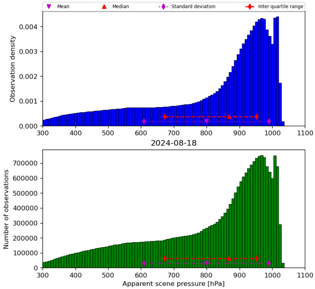
Figure 36: Histogram of “Apparent scene pressure” for 2024-08-17 to 2024-08-19
