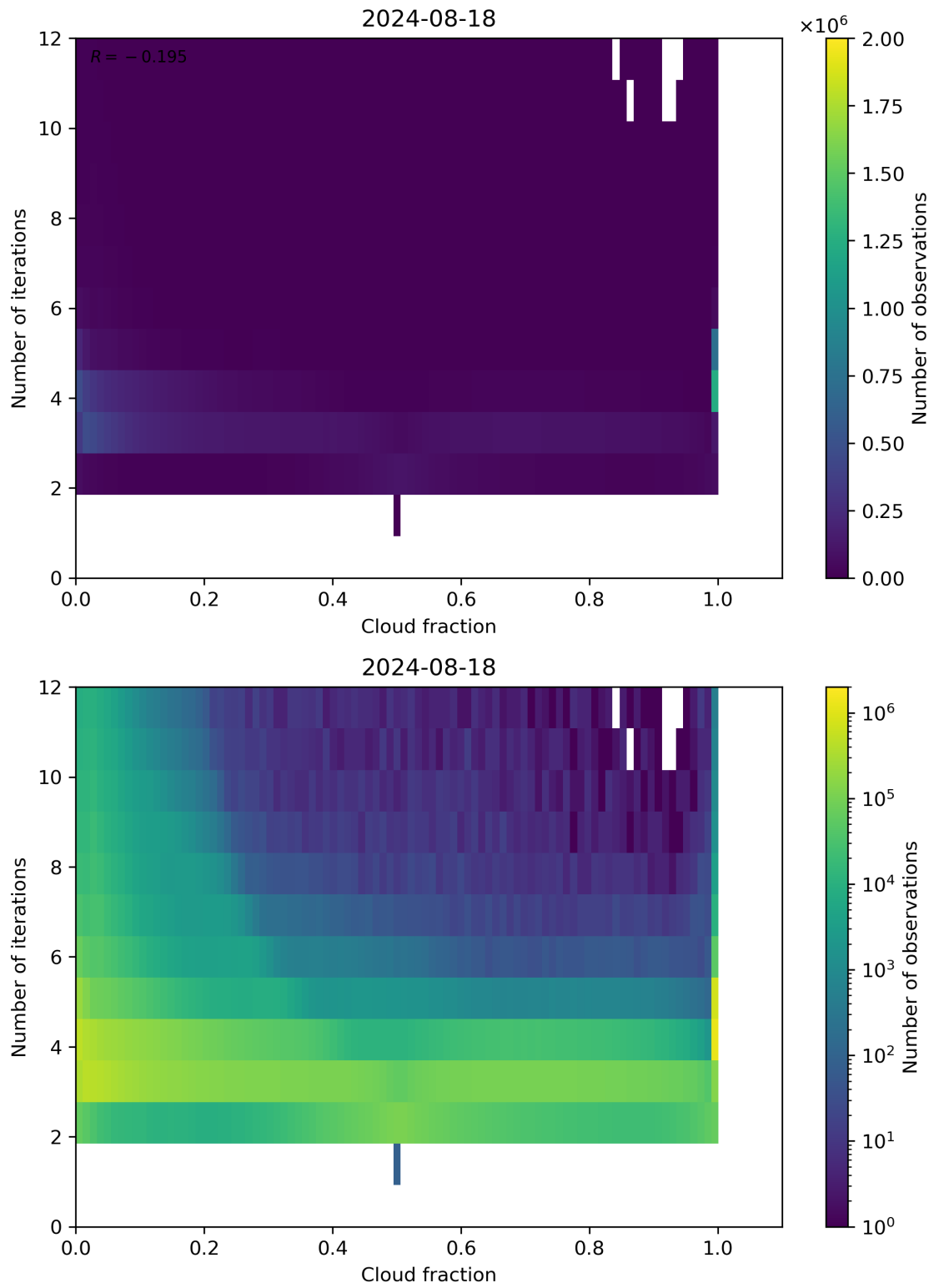
Figure 73: Scatter density plot of “Cloud fraction” against “Number of iterations” for 2024-08-17 to 2024-08-19.
