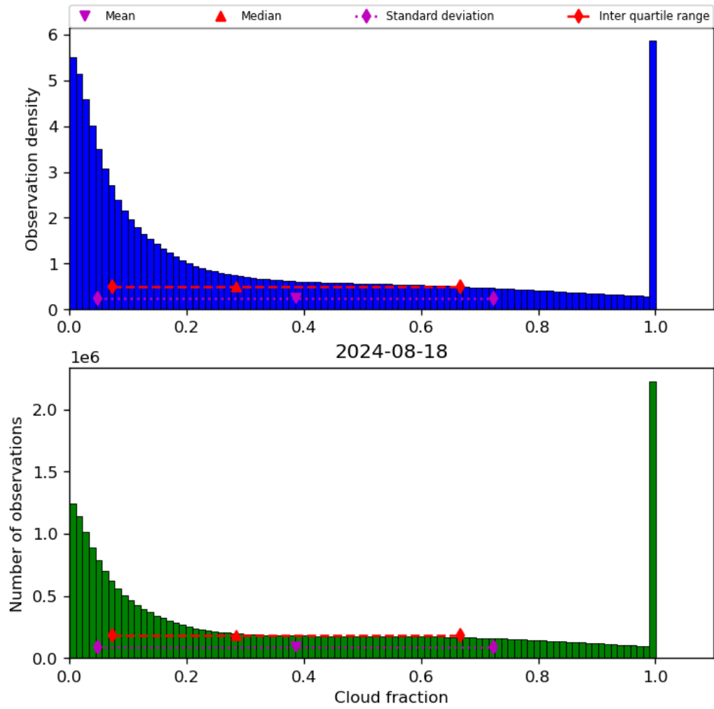
Figure 32: Histogram of “Cloud fraction” for 2024-08-17 to 2024-08-19
