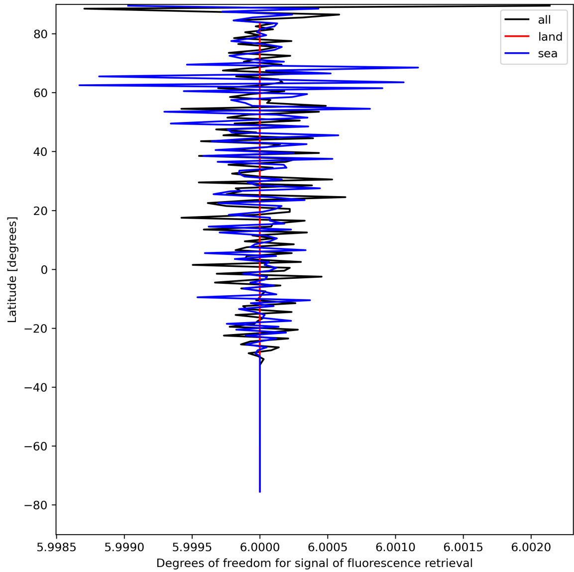
Figure 26: Zonal average of “Degrees of freedom for signal of fluorescence retrieval” for 2024-08-17 to 2024-08-19.
