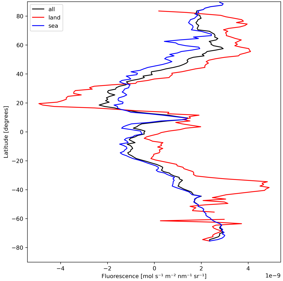
Figure 23: Zonal average of “Fluorescence” for 2024-08-17 to 2024-08-19.
