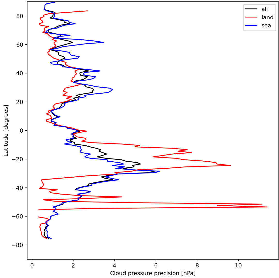
Figure 14: Zonal average of “Cloud pressure precision” for 2024-08-17 to 2024-08-19.
