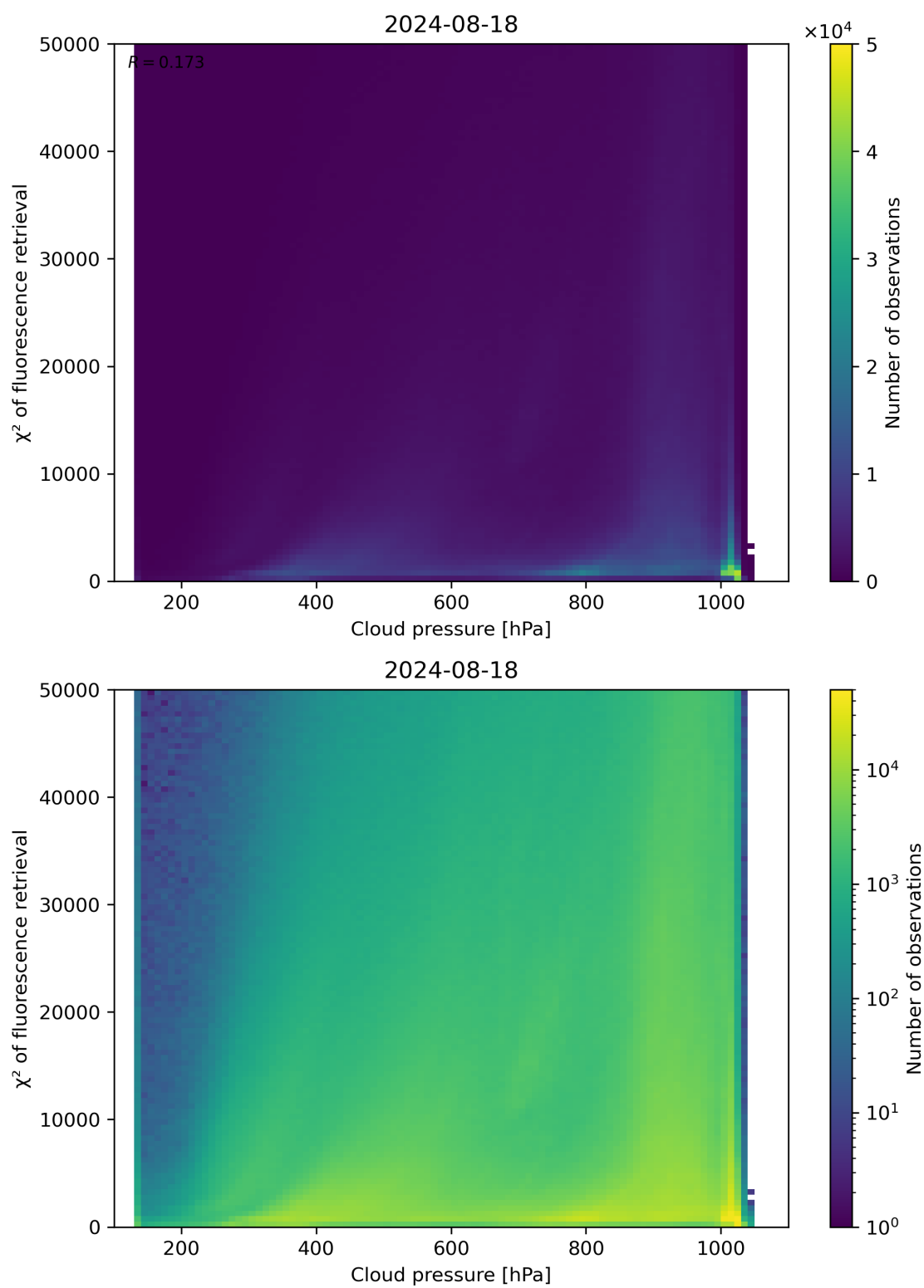
Figure 78: Scatter density plot of “Cloud pressure” against “ \chi^2 of fluorescence retrieval” for 2024-08-17 to 2024-08-19.
