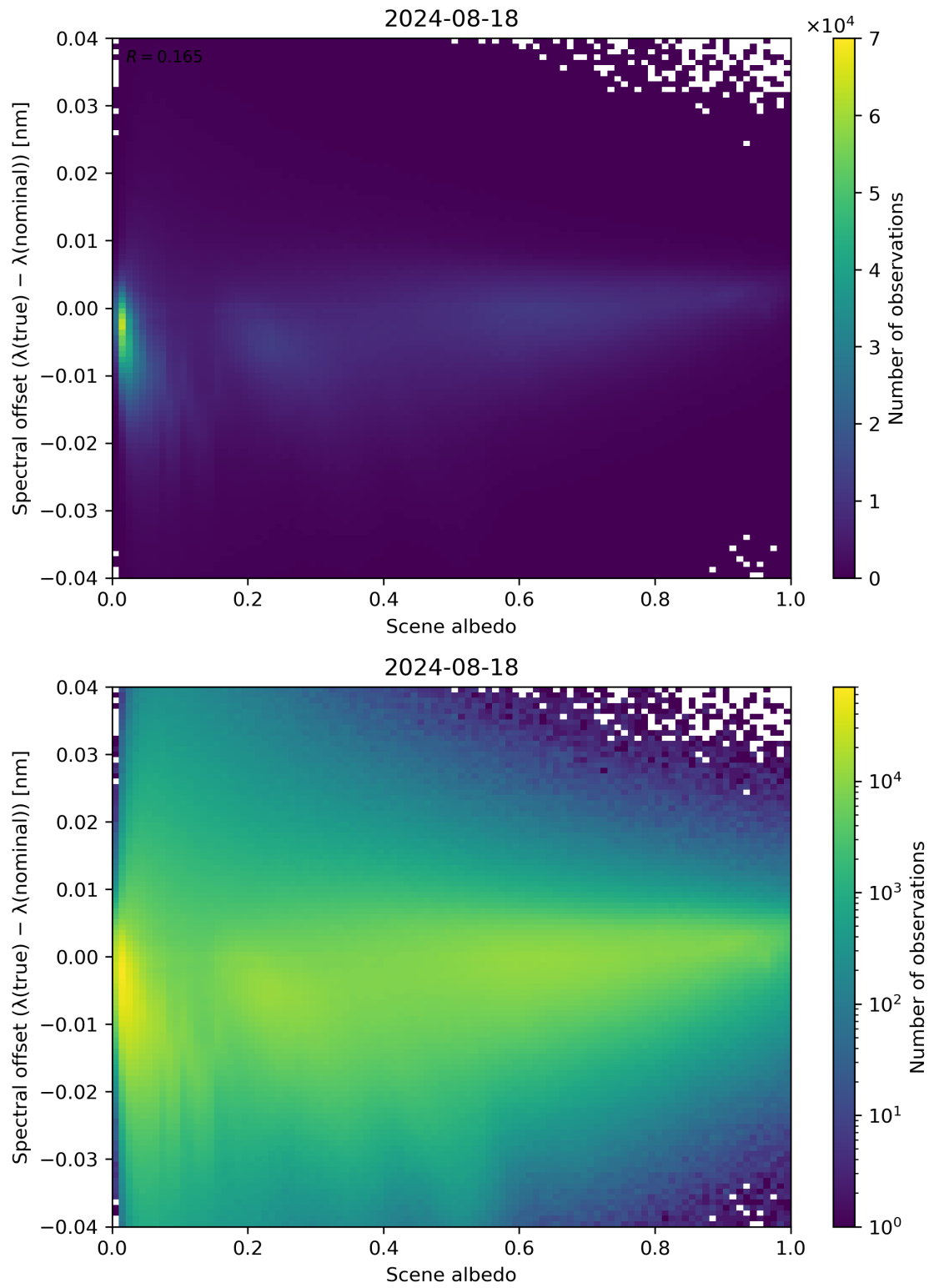
Figure 107: Scatter density plot of “Scene albedo” against “Spectral offset ( \lambda(\text{true}) - \lambda(\text{nominal}) )” for 2024-08-17 to 2024-08-19.
