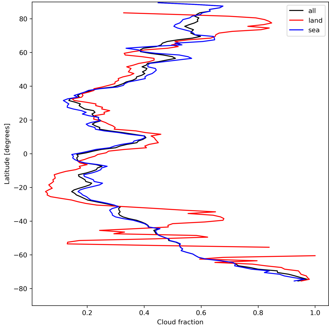
Figure 15: Zonal average of “Cloud fraction” for 2024-08-17 to 2024-08-19.
