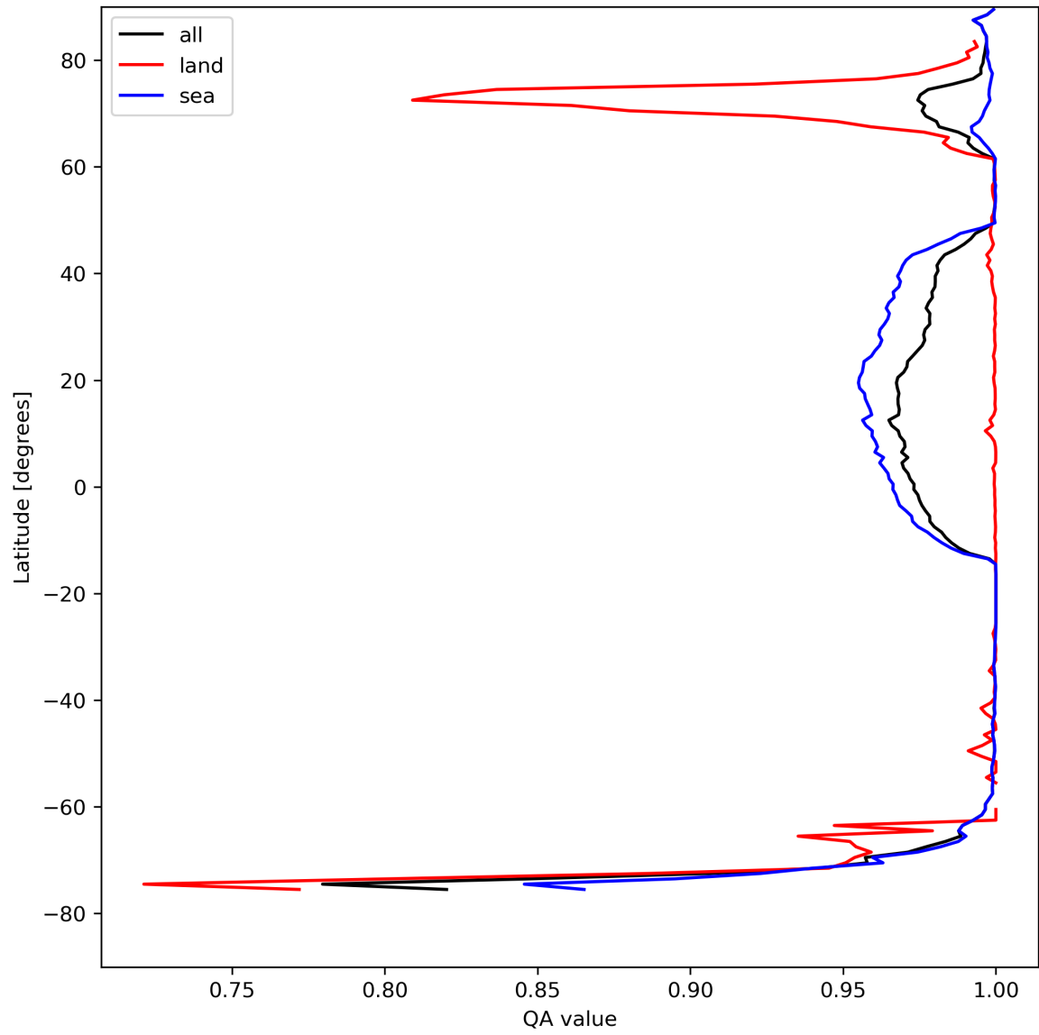
Figure 12: Zonal average of “QA value” for 2024-08-17 to 2024-08-19.
