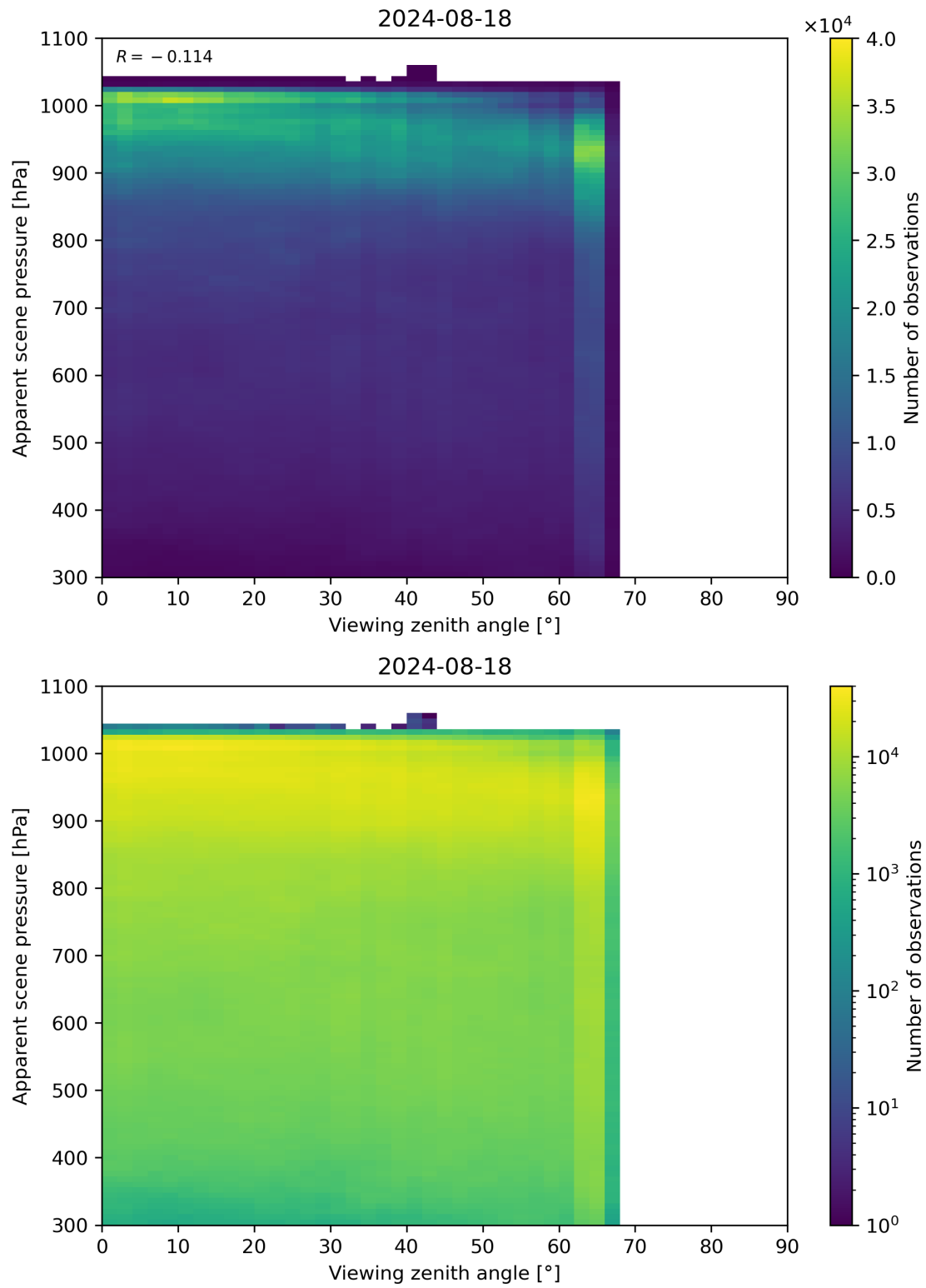
Figure 118: Scatter density plot of “Viewing zenith angle” against “Apparent scene pressure” for 2024-08-17 to 2024-08-19.
