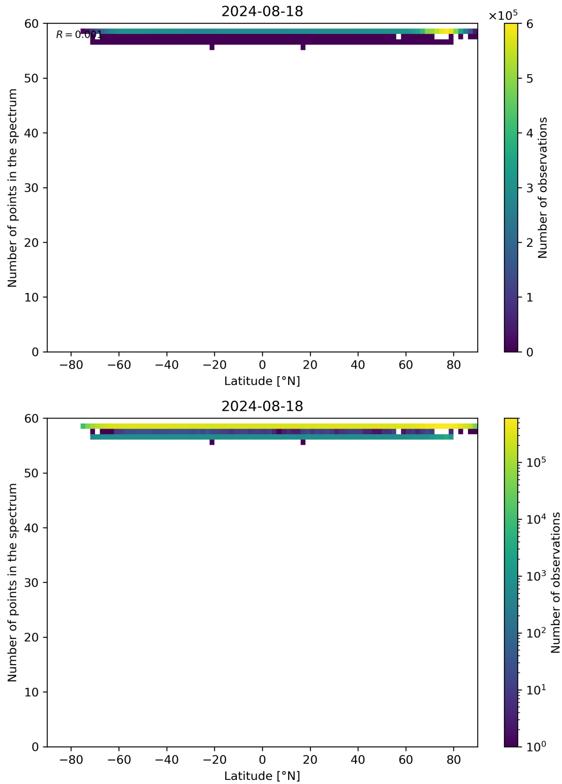
Figure 94: Scatter density plot of “Latitude” against “Number of points in the spectrum” for 2024-08-17 to 2024-08-19.
