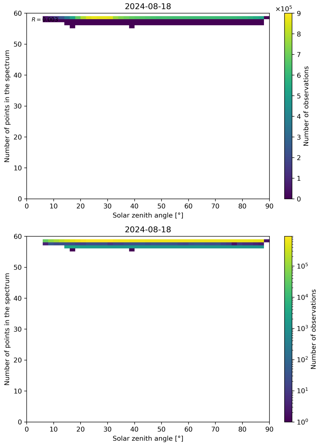
Figure 115: Scatter density plot of “Solar zenith angle” against “Number of points in the spectrum” for 2024-08-17 to 2024-08-19.
