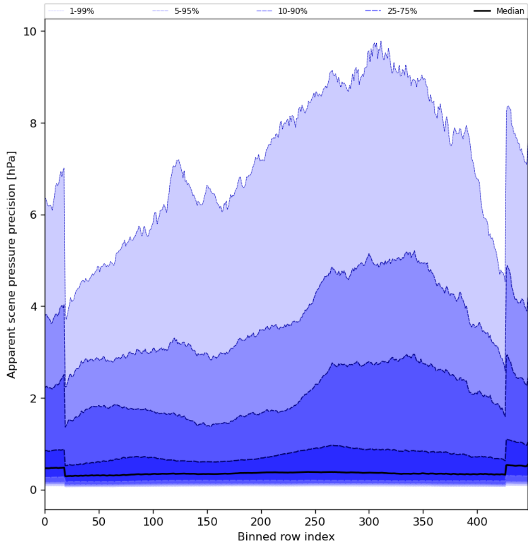
Figure 54: Along track statistics of “Apparent scene pressure precision” for 2024-08-17 to 2024-08-19
