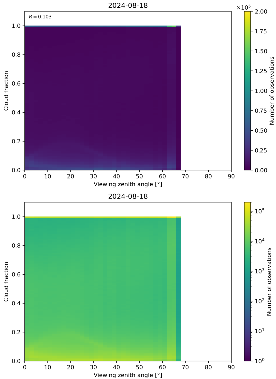
Figure 120: Scatter density plot of “Viewing zenith angle” against “Cloud fraction” for 2024-08-17 to 2024-08-19.
