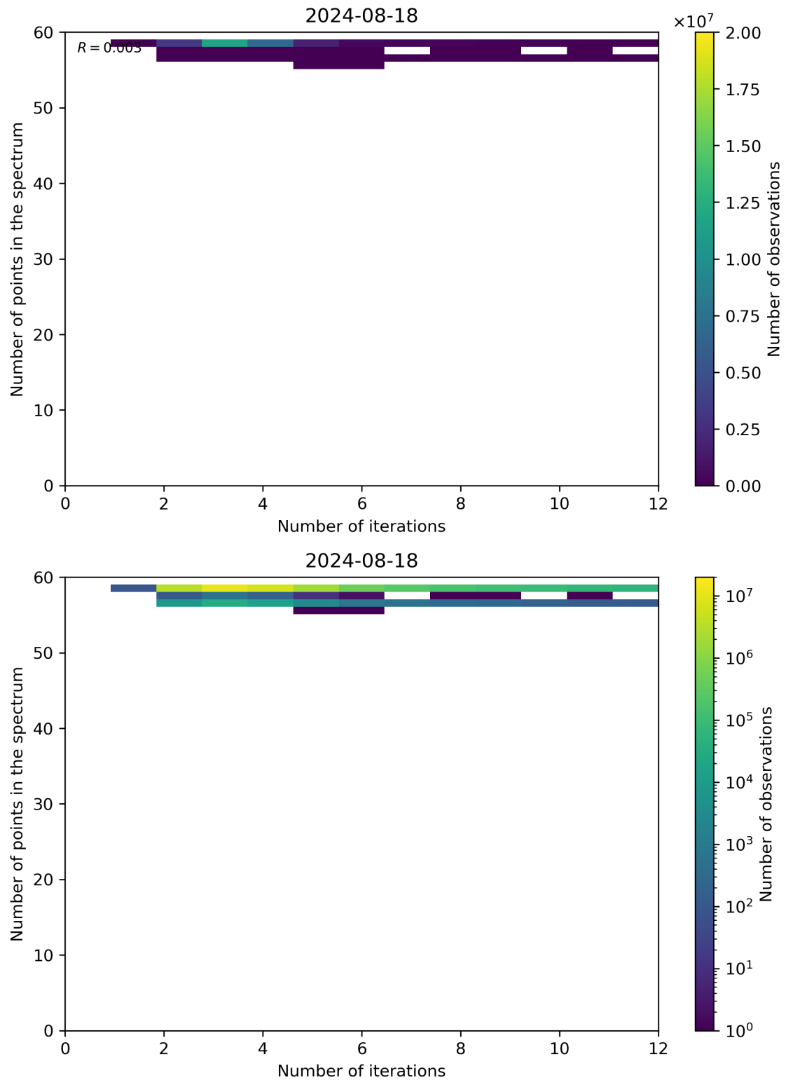
Figure 99: Scatter density plot of “Number of iterations” against “Number of points in the spectrum” for 2024-08-17 to 2024-08-19.
