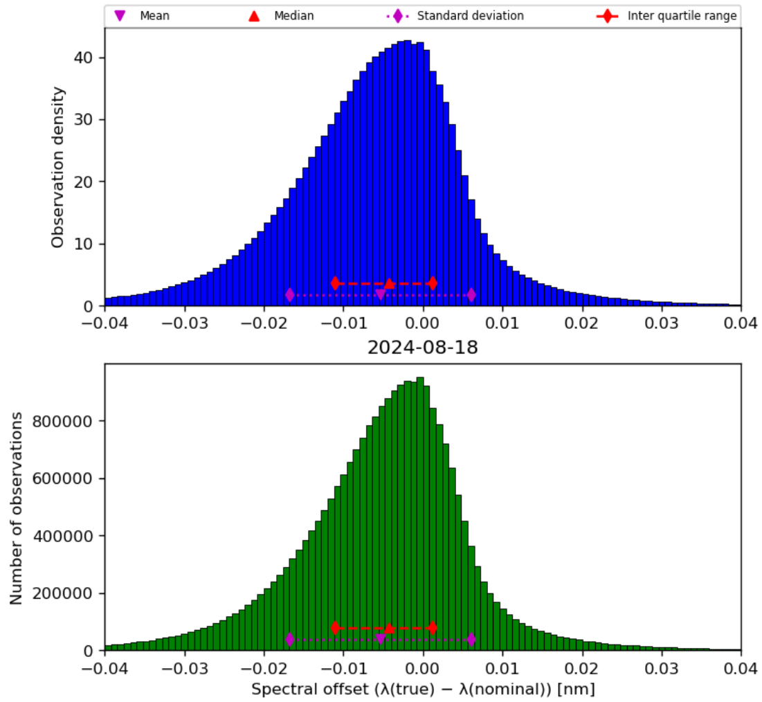
Figure 45: Histogram of “Spectral offset ( \lambda(\text{true}) - \lambda(\text{nominal}) )” for 2024-08-17 to 2024-08-19
