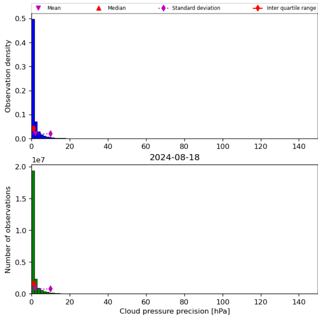
Figure 31: Histogram of “Cloud pressure precision” for 2024-08-17 to 2024-08-19
