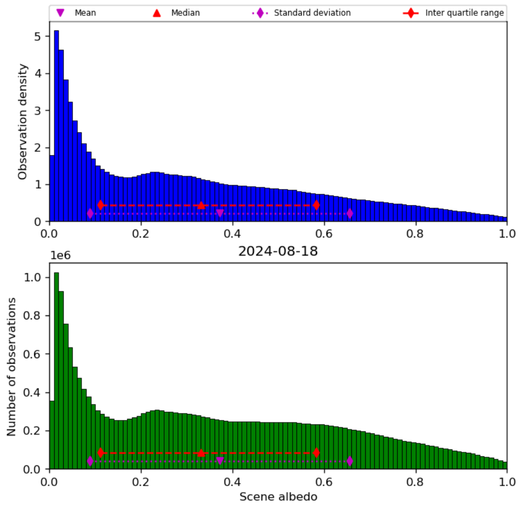
Figure 34: Histogram of “Scene albedo” for 2024-08-17 to 2024-08-19
