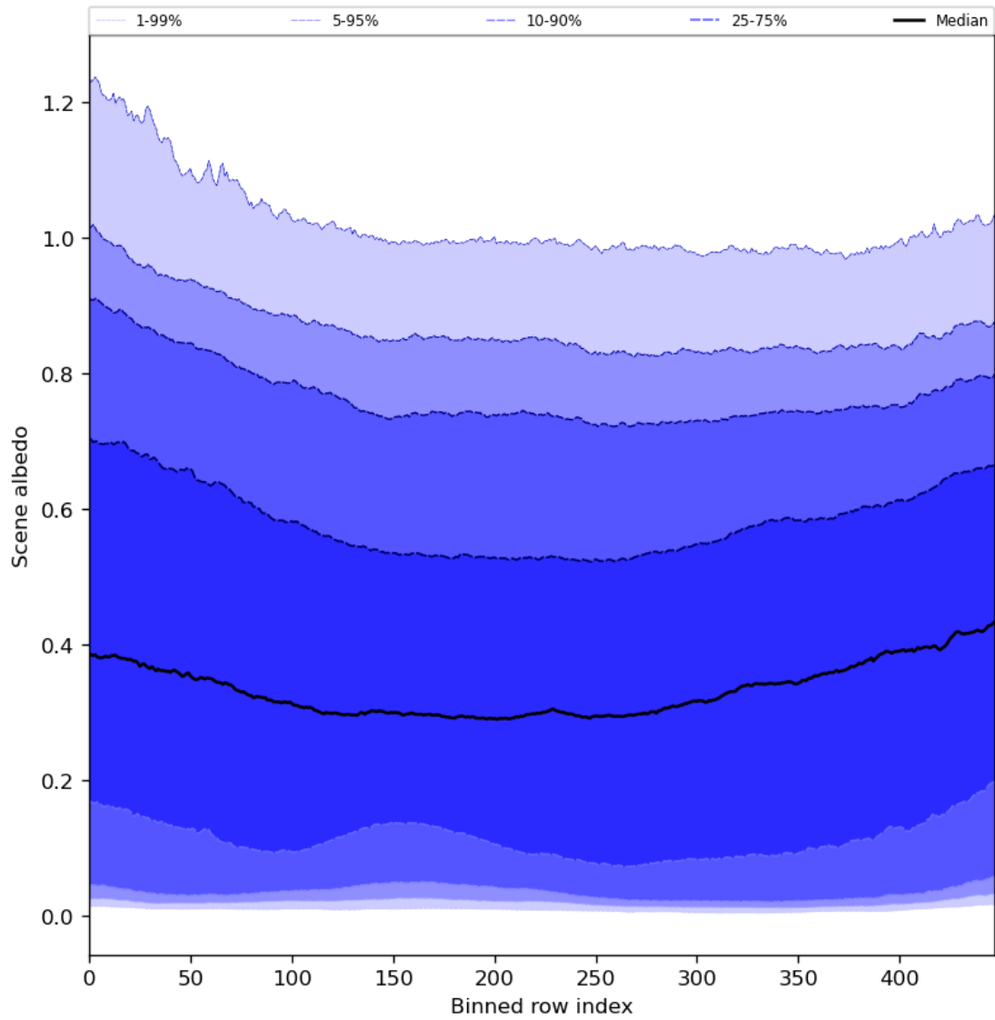
Figure 51: Along track statistics of “Scene albedo” for 2024-08-17 to 2024-08-19
