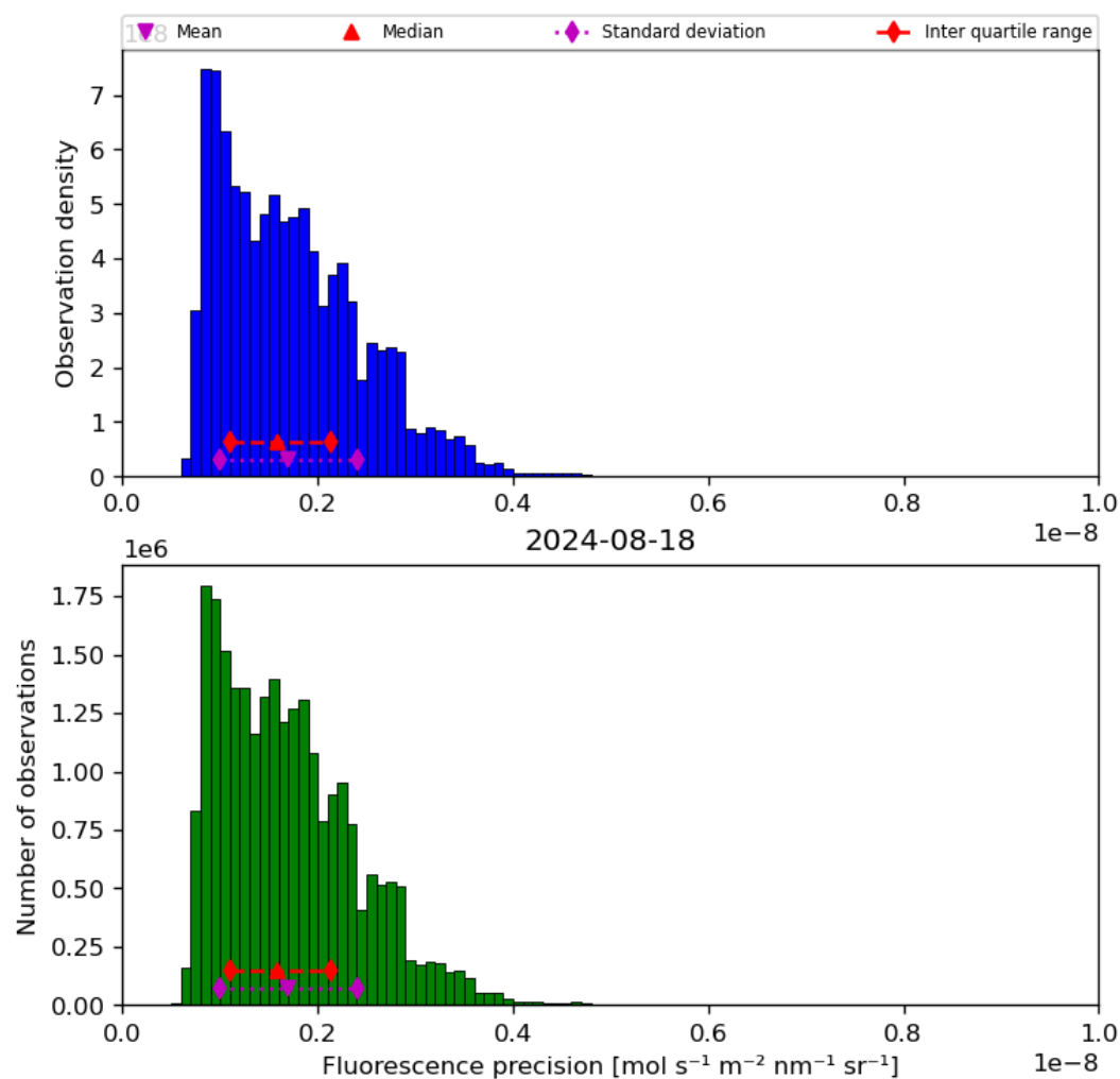
Figure 41: Histogram of “Fluorescence precision” for 2024-08-17 to 2024-08-19
