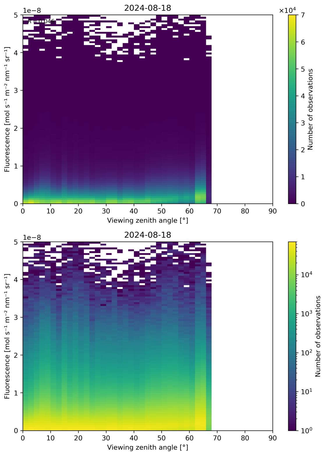
Figure 122: Scatter density plot of “Viewing zenith angle” against “Fluorescence” for 2024-08-17 to 2024-08-19.
