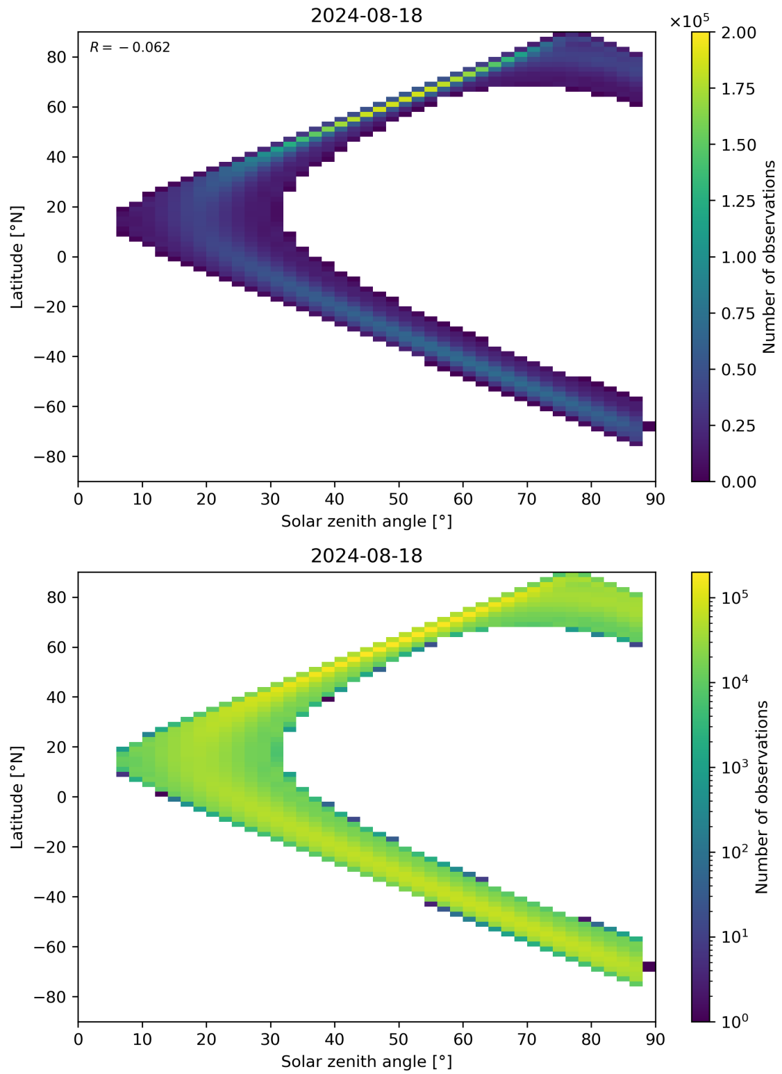
Figure 113: Scatter density plot of “Solar zenith angle” against “Latitude” for 2024-08-17 to 2024-08-19.
