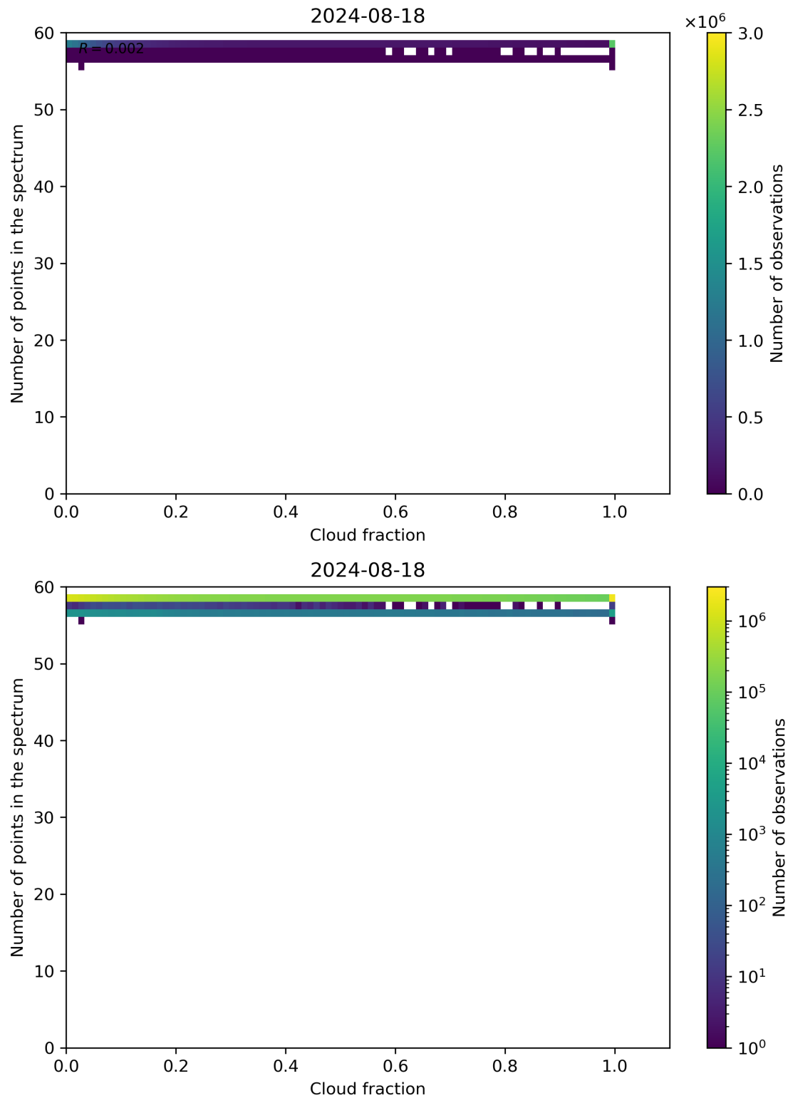
Figure 74: Scatter density plot of “Cloud fraction” against “Number of points in the spectrum” for 2024-08-17 to 2024-08-19.
