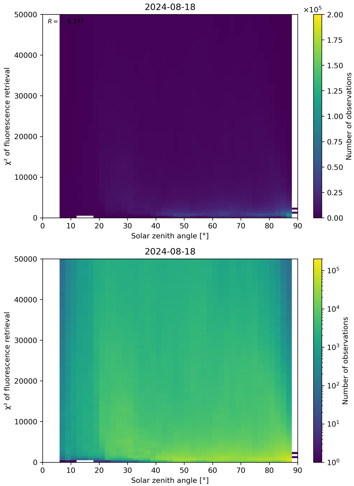
Figure 109: Scatter density plot of “Solar zenith angle” against “ \chi^2 of fluorescence retrieval” for 2024-08-17 to 2024-08-19.
