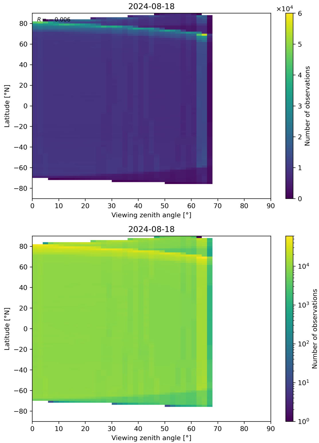
Figure 123: Scatter density plot of “Viewing zenith angle” against “Latitude” for 2024-08-17 to 2024-08-19.
