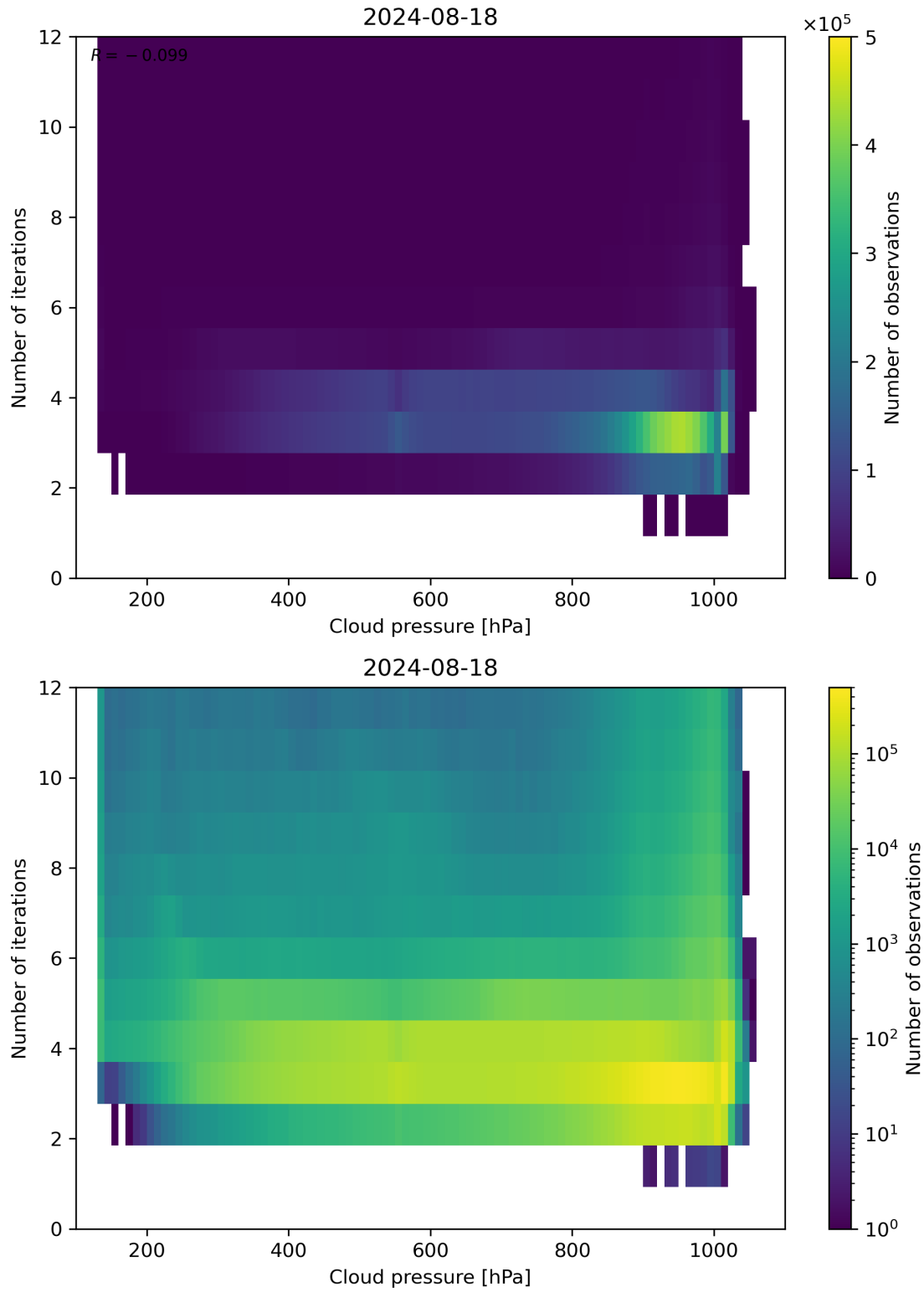
Figure 81: Scatter density plot of “Cloud pressure” against “Number of iterations” for 2024-08-17 to 2024-08-19.
