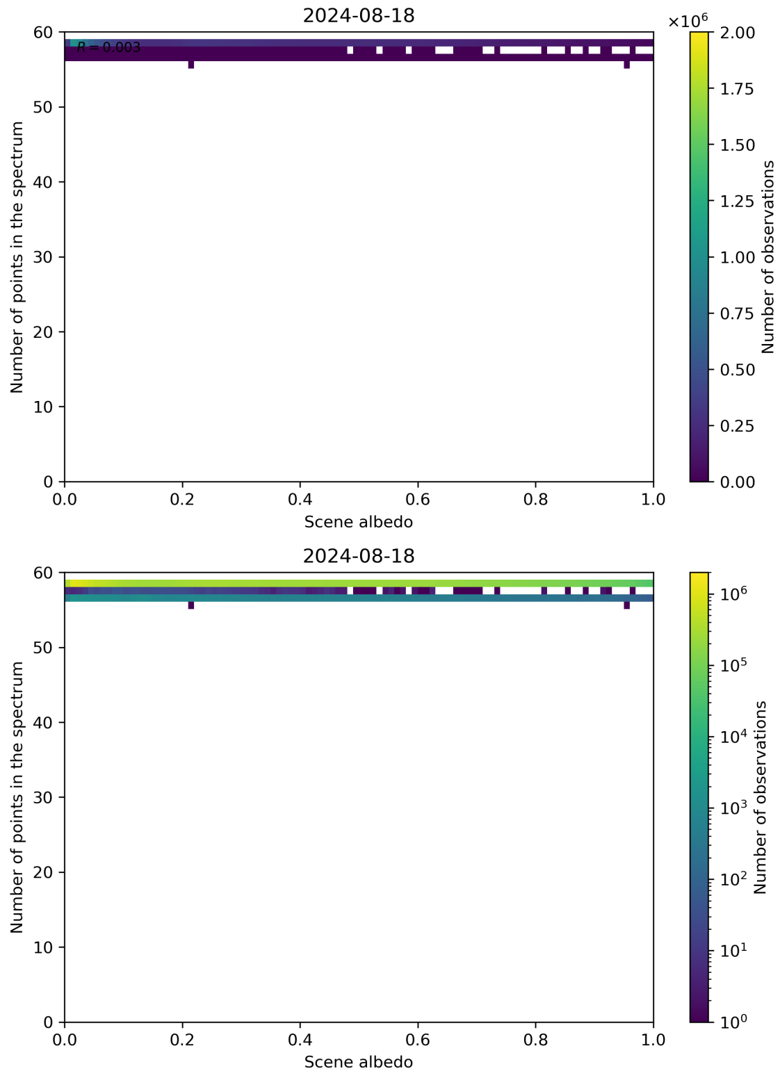
Figure 106: Scatter density plot of “Scene albedo” against “Number of points in the spectrum” for 2024-08-17 to 2024-08-19.
