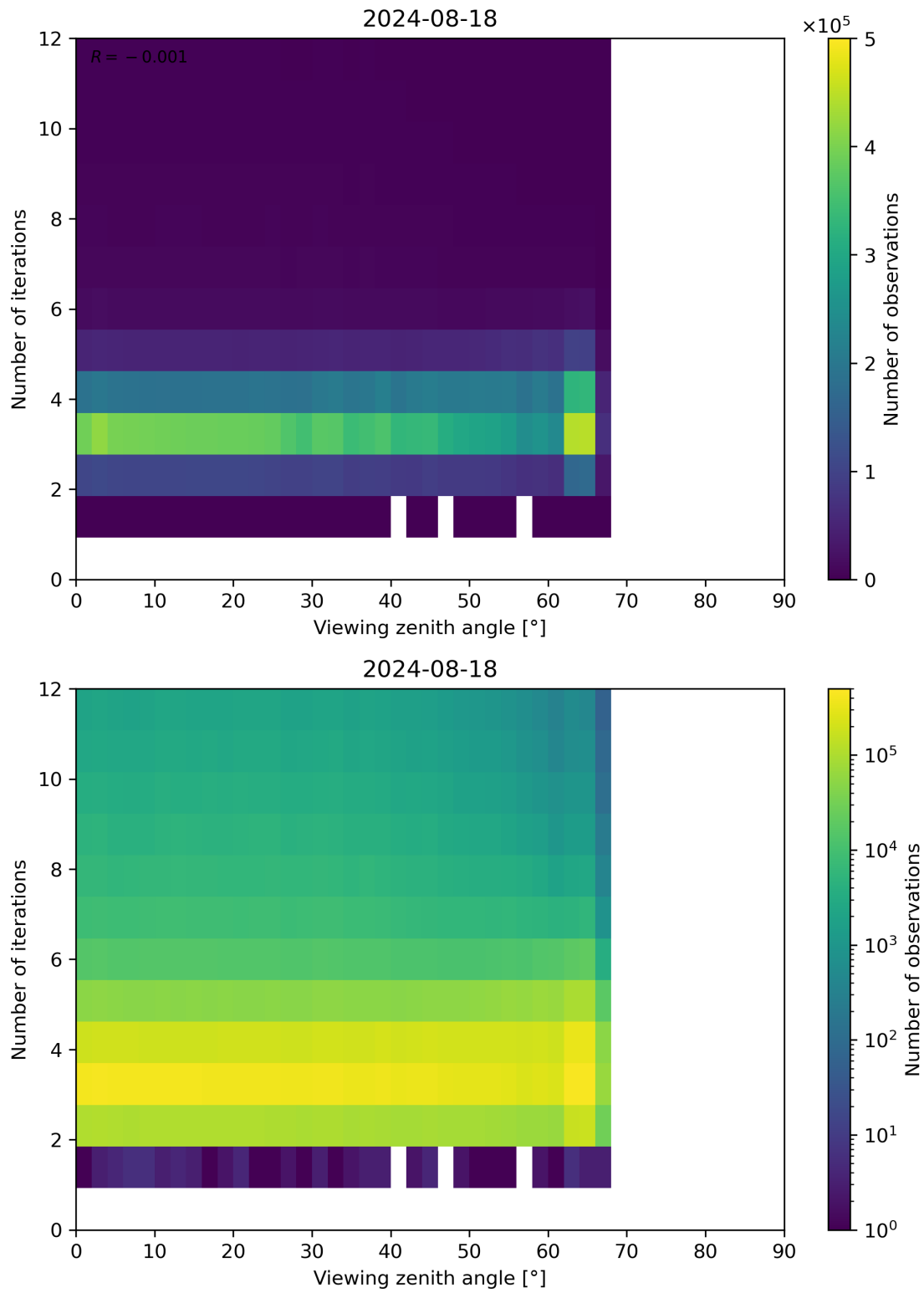
Figure 124: Scatter density plot of “Viewing zenith angle” against “Number of iterations” for 2024-08-17 to 2024-08-19.
