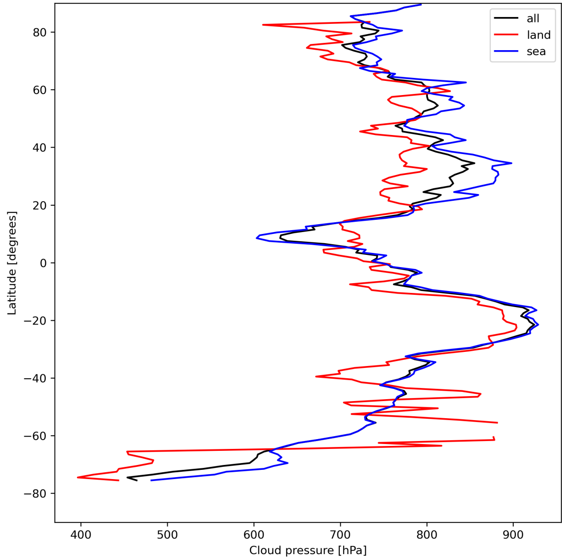
Figure 13: Zonal average of “Cloud pressure” for 2024-08-17 to 2024-08-19.
