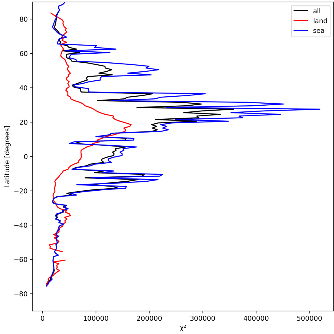
Figure 21: Zonal average of “ \chi^2 ” for 2024-08-17 to 2024-08-19.
