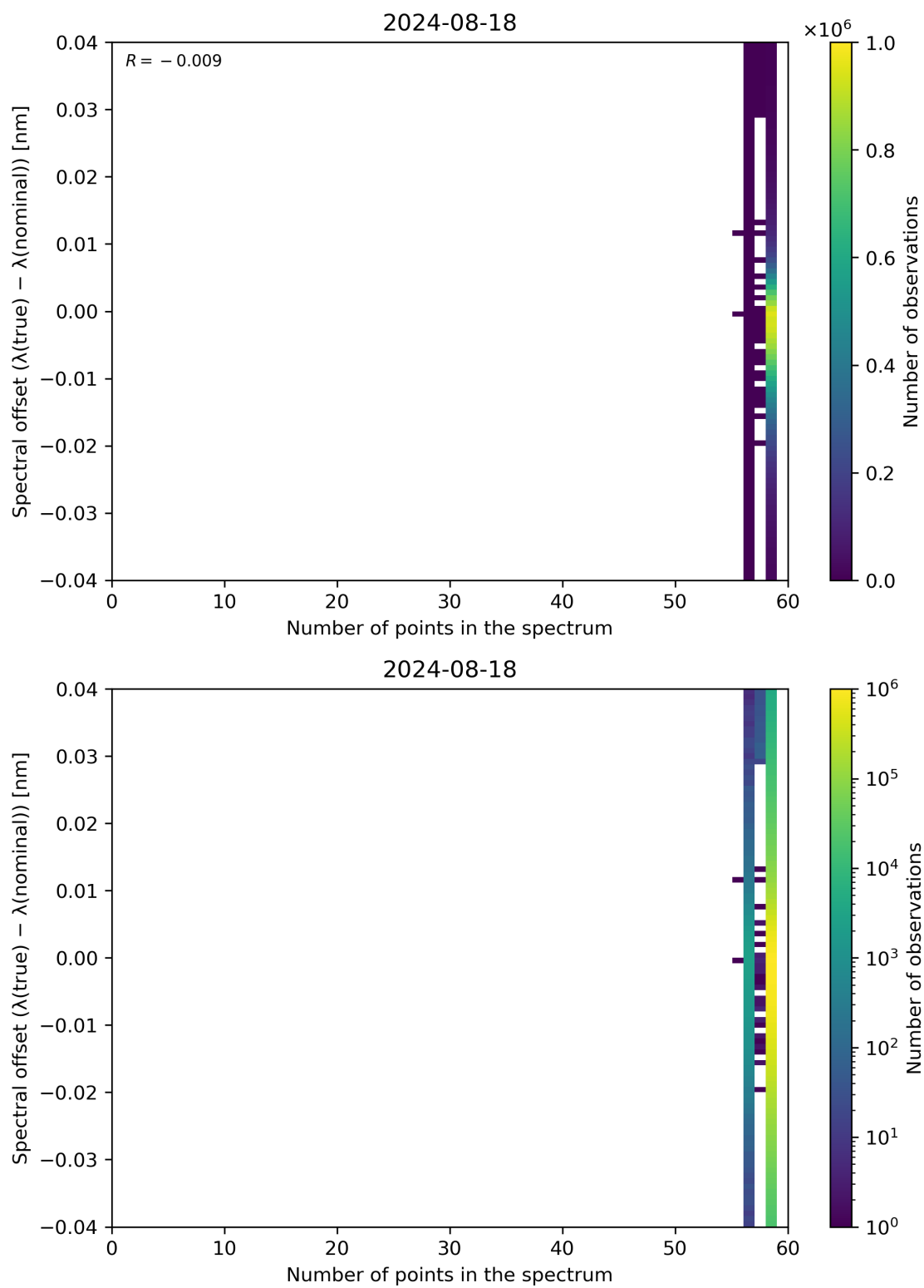
Figure 101: Scatter density plot of “Number of points in the spectrum” against “Spectral offset ( \lambda(\text{true}) - \lambda(\text{nominal}) )” for 2024-08-17 to 2024-08-19.
