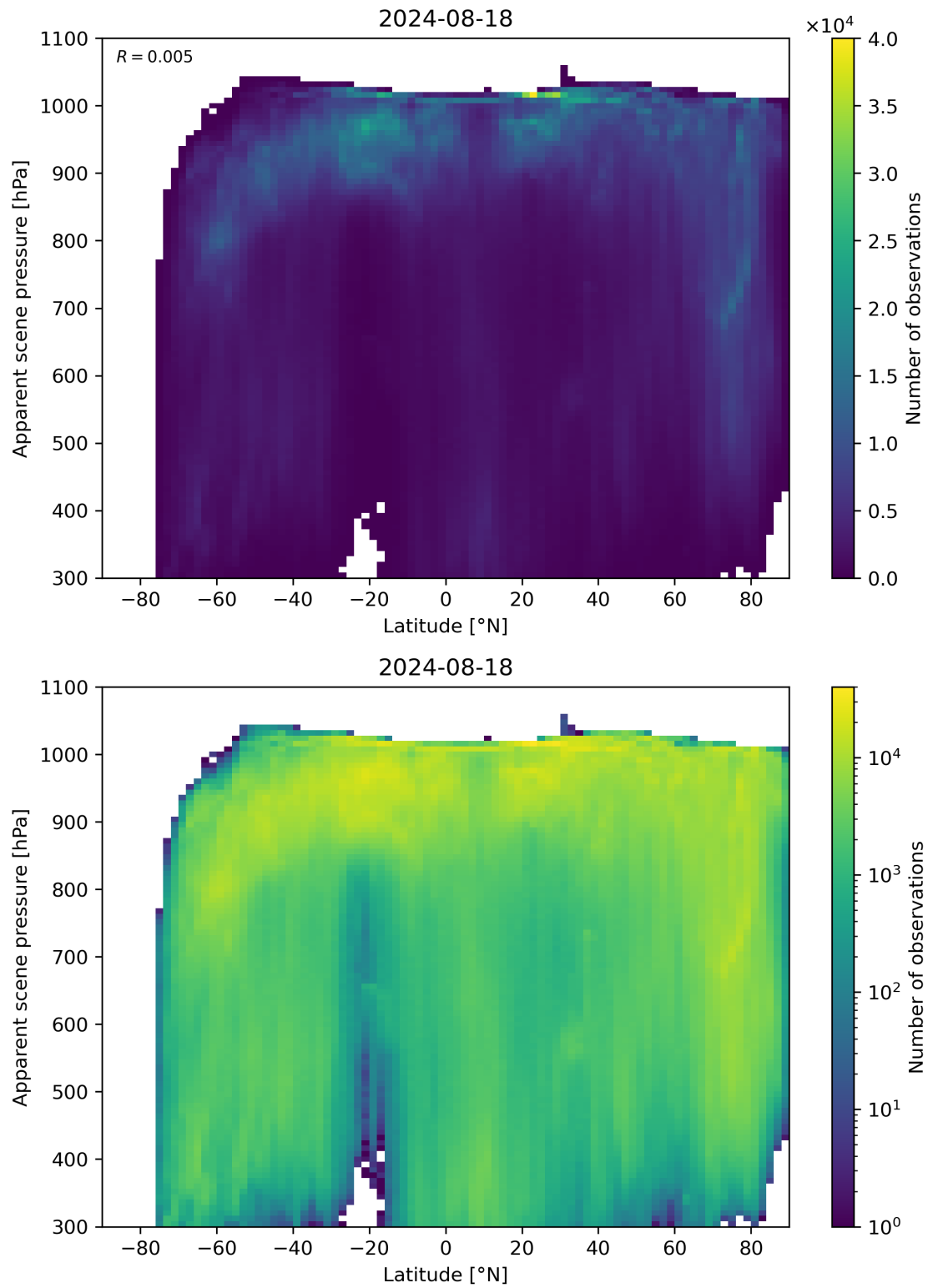
Figure 88: Scatter density plot of “Latitude” against “Apparent scene pressure” for 2024-08-17 to 2024-08-19.
