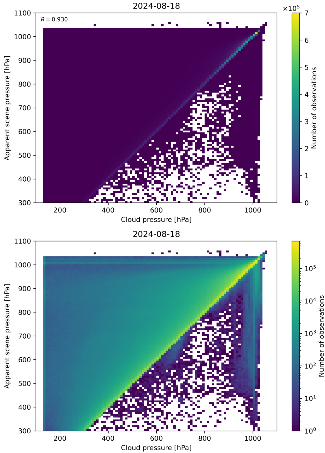
Figure 77: Scatter density plot of “Cloud pressure” against “Apparent scene pressure” for 2024-08-17 to 2024-08-19.
