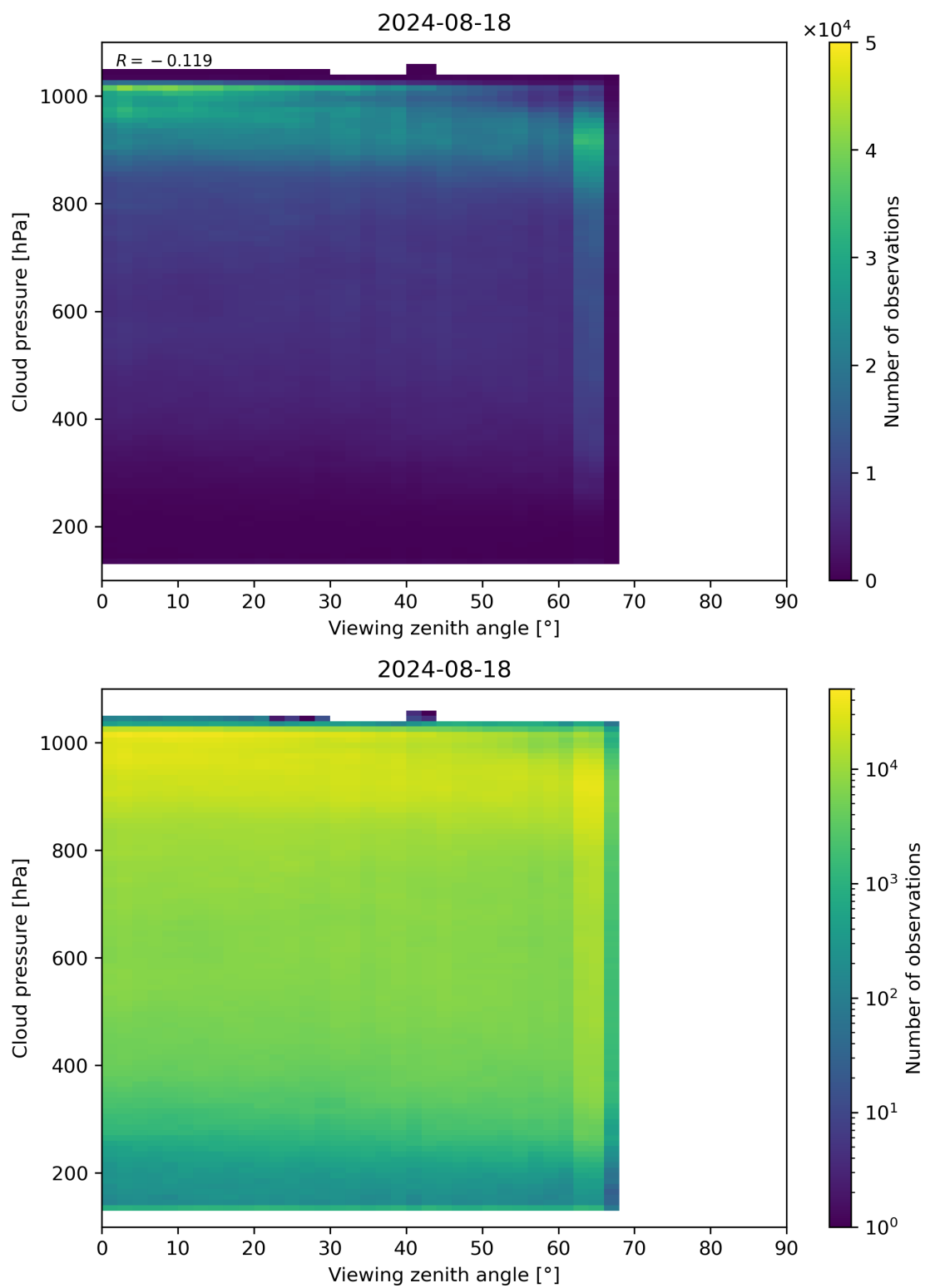
Figure 121: Scatter density plot of “Viewing zenith angle” against “Cloud pressure” for 2024-08-17 to 2024-08-19.
