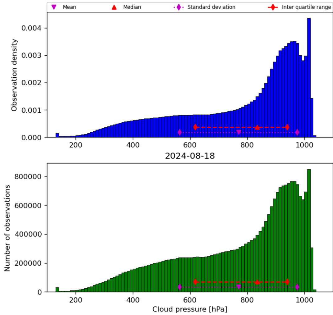
Figure 30: Histogram of “Cloud pressure” for 2024-08-17 to 2024-08-19
