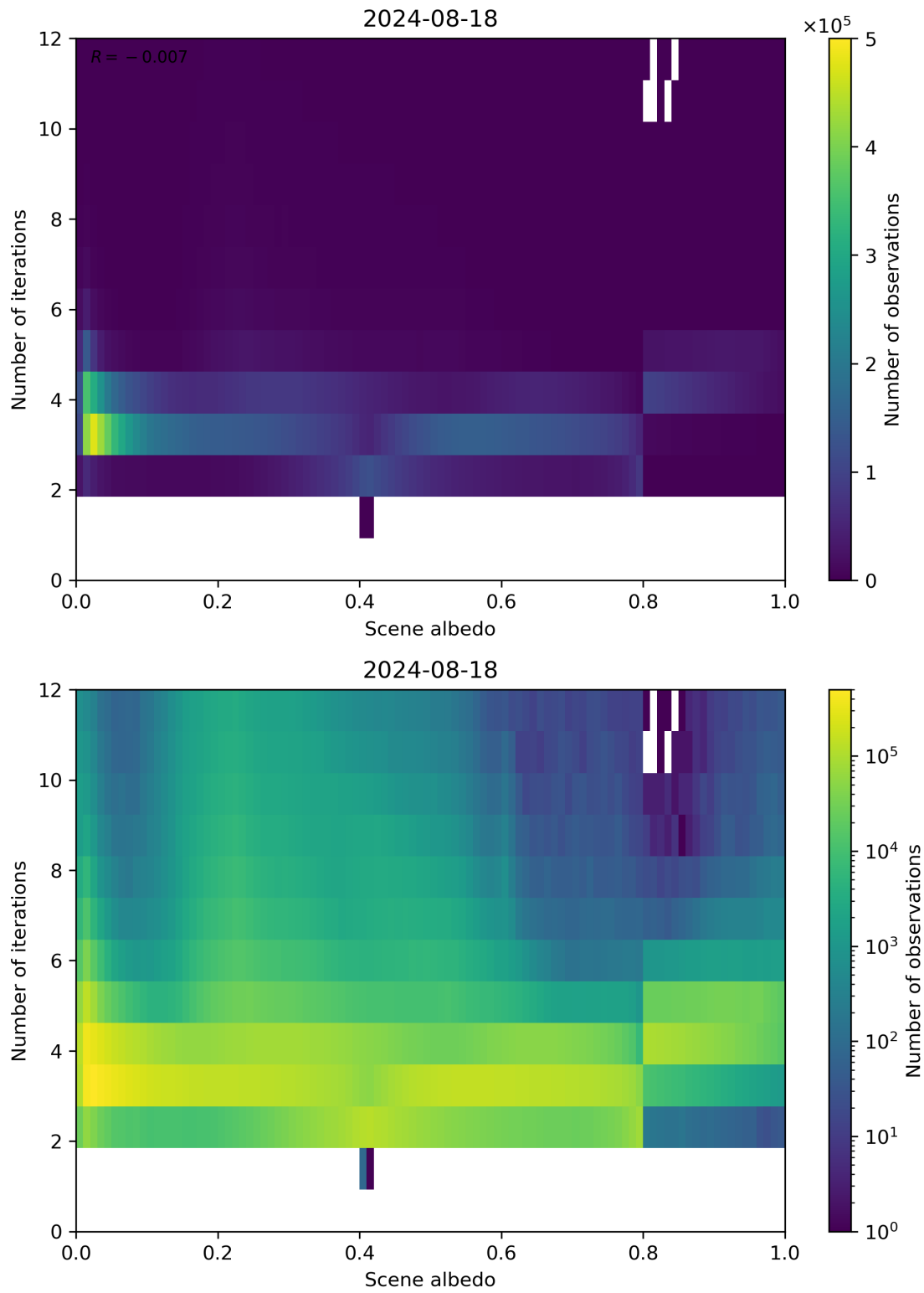
Figure 105: Scatter density plot of “Scene albedo” against “Number of iterations” for 2024-08-17 to 2024-08-19.
