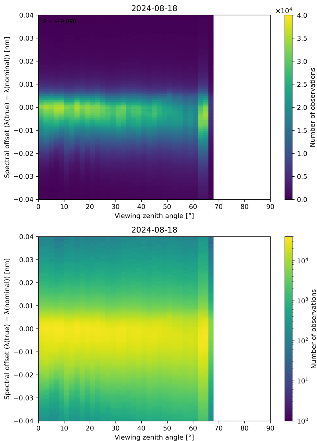
Figure 128: Scatter density plot of “Viewing zenith angle” against “Spectral offset ( \lambda(\text{true}) - \lambda(\text{nominal}) )” for 2024-08-17 to 2024-08-19.
