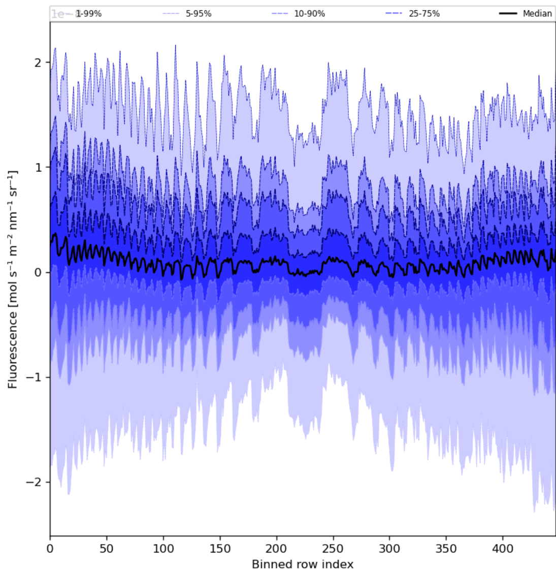
Figure 57: Along track statistics of “Fluorescence” for 2024-08-17 to 2024-08-19
