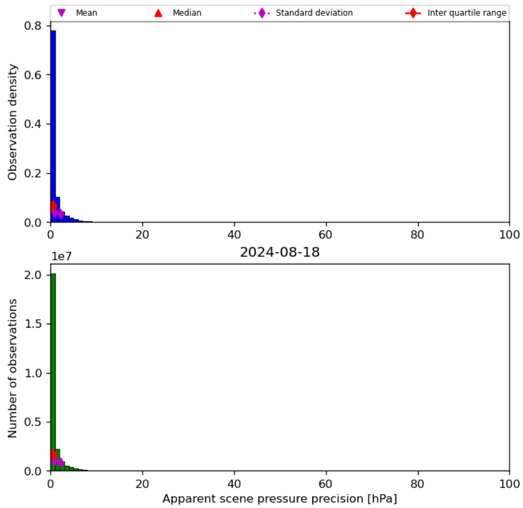
Figure 37: Histogram of “Apparent scene pressure precision” for 2024-08-17 to 2024-08-19
