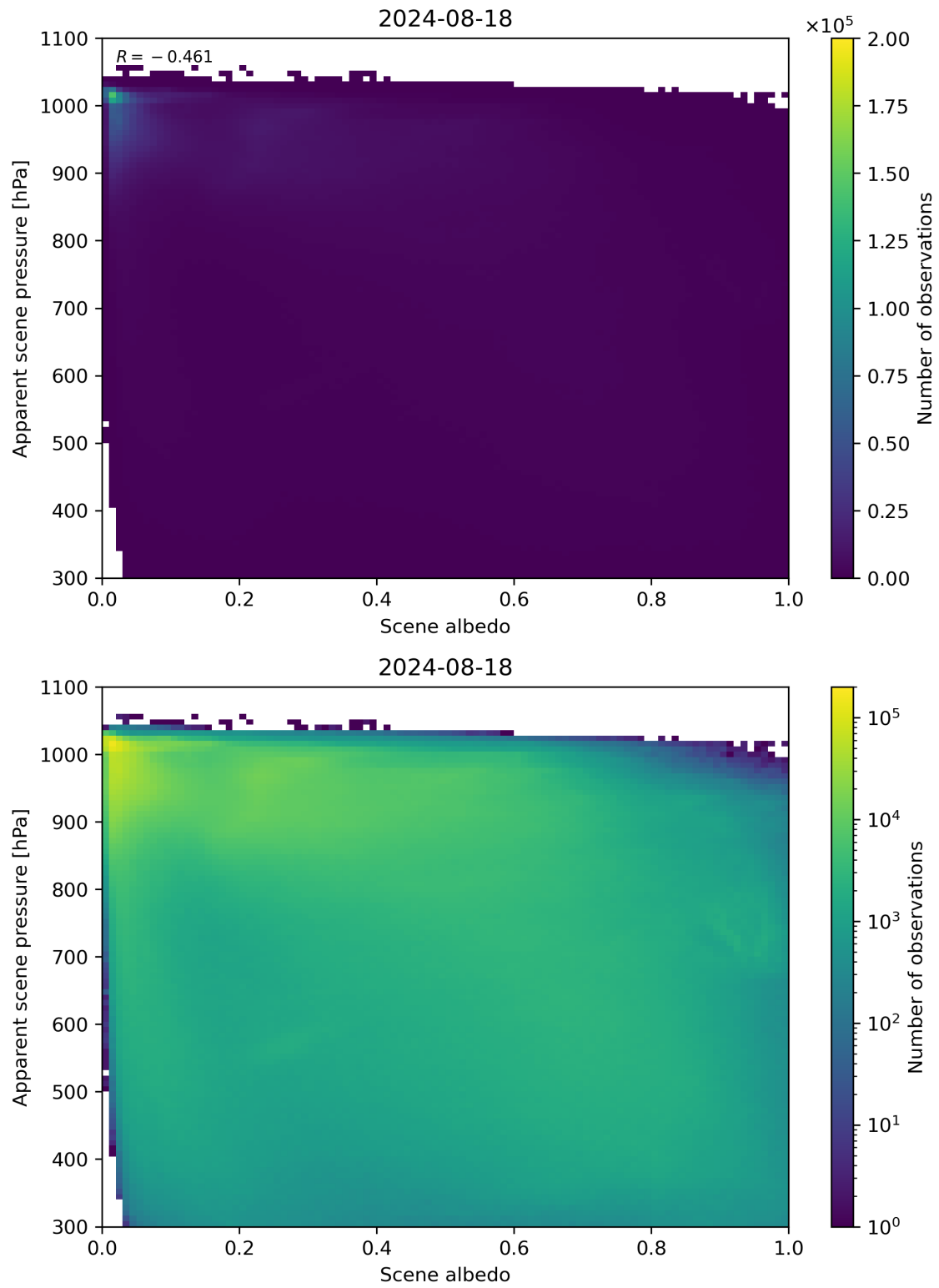
Figure 102: Scatter density plot of “Scene albedo” against “Apparent scene pressure” for 2024-08-17 to 2024-08-19.
