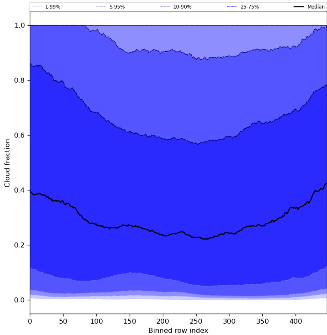
Figure 49: Along track statistics of “Cloud fraction” for 2024-08-17 to 2024-08-19
