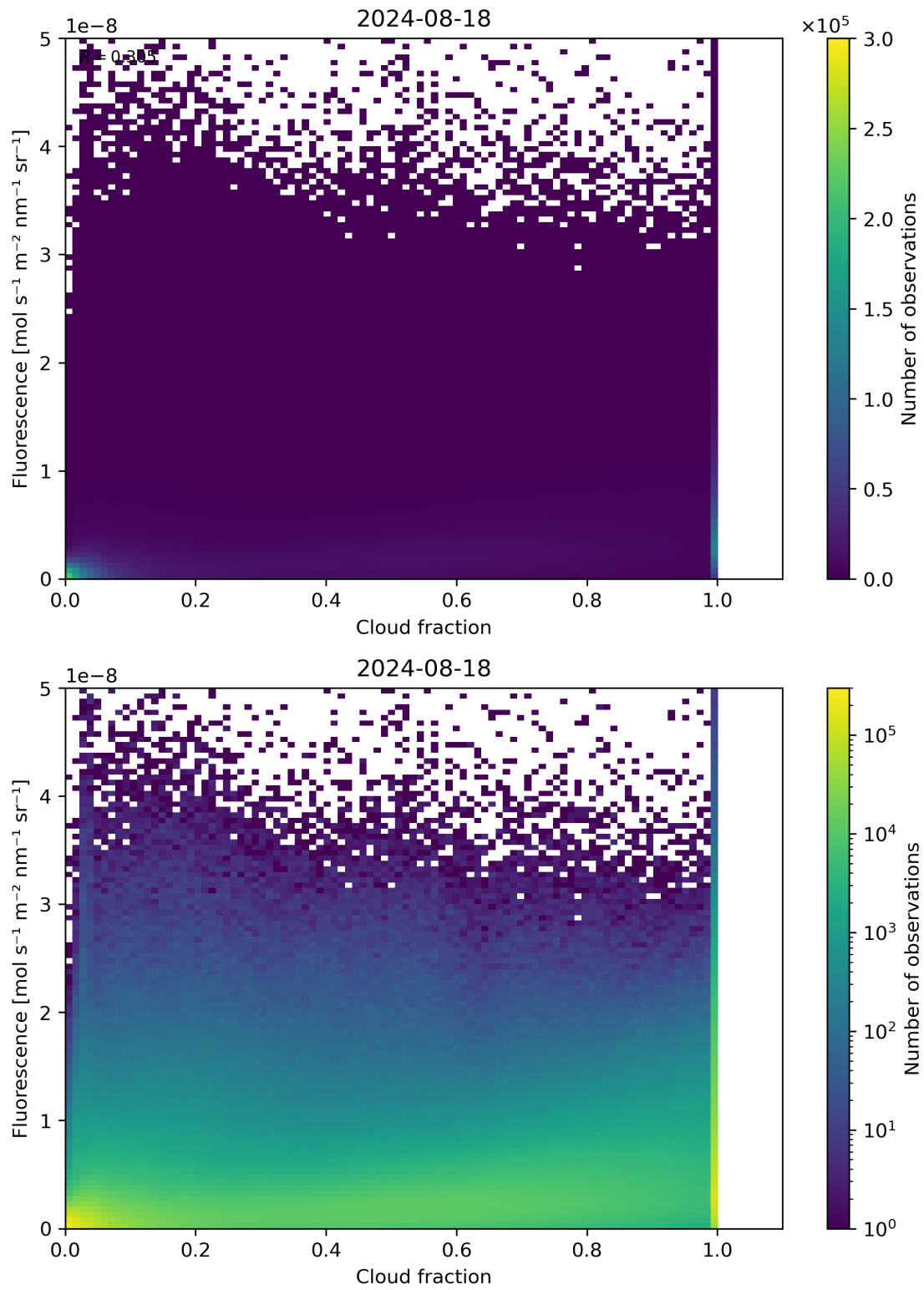
Figure 72: Scatter density plot of “Cloud fraction” against “Fluorescence” for 2024-08-17 to 2024-08-19.
