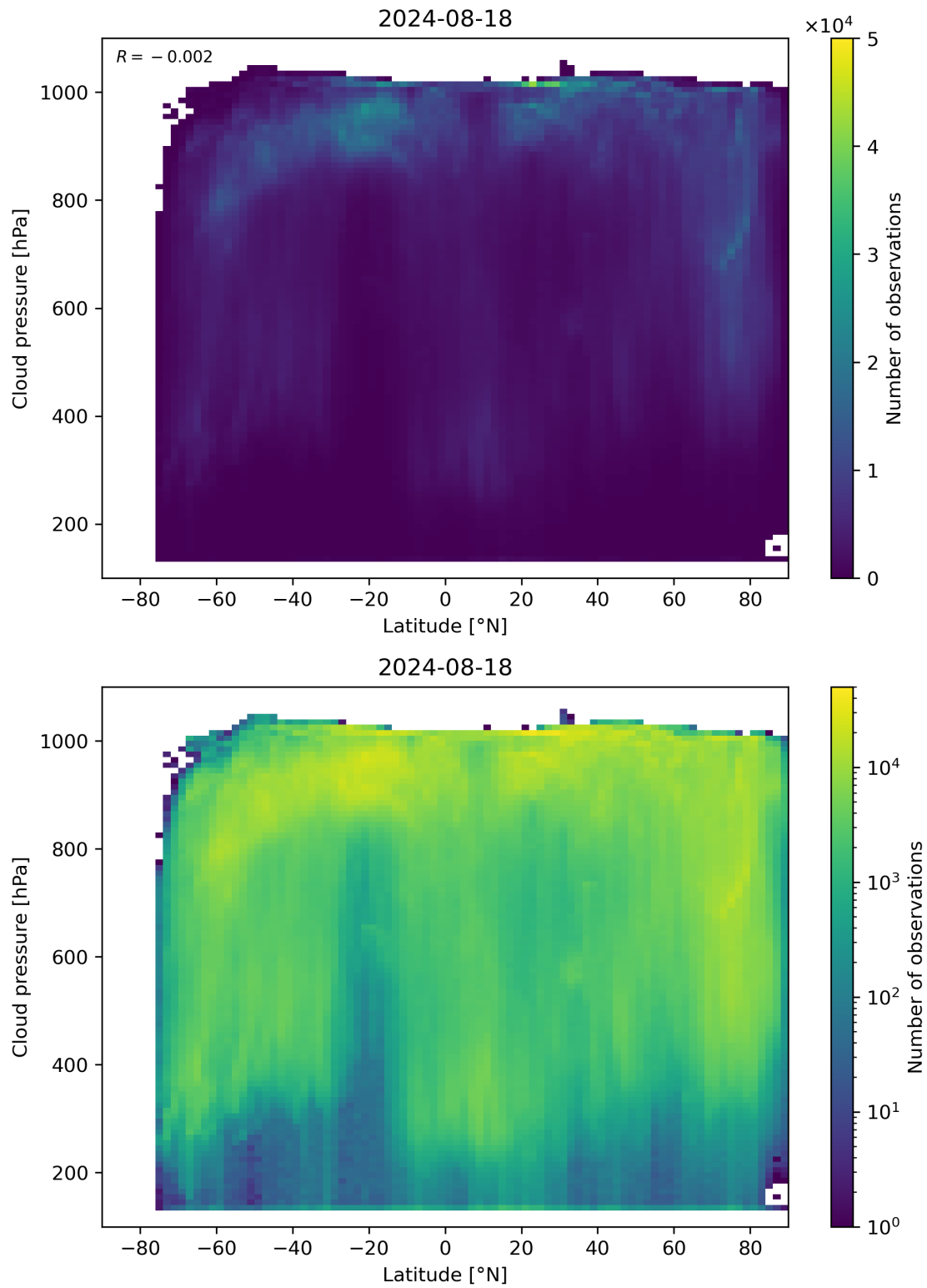
Figure 91: Scatter density plot of “Latitude” against “Cloud pressure” for 2024-08-17 to 2024-08-19.
