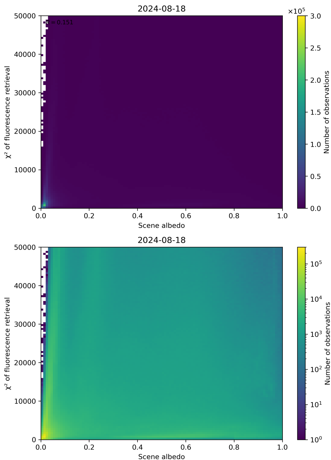
Figure 103: Scatter density plot of “Scene albedo” against “ \chi^2 of fluorescence retrieval” for 2024-08-17 to 2024-08-19.
