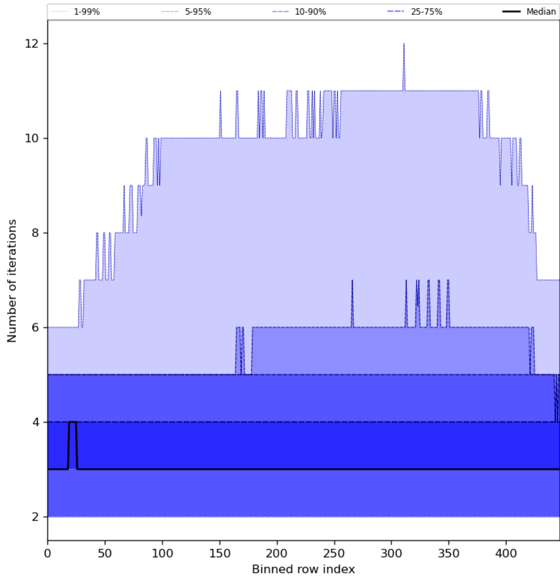
Figure 56: Along track statistics of “Number of iterations” for 2024-08-17 to 2024-08-19
