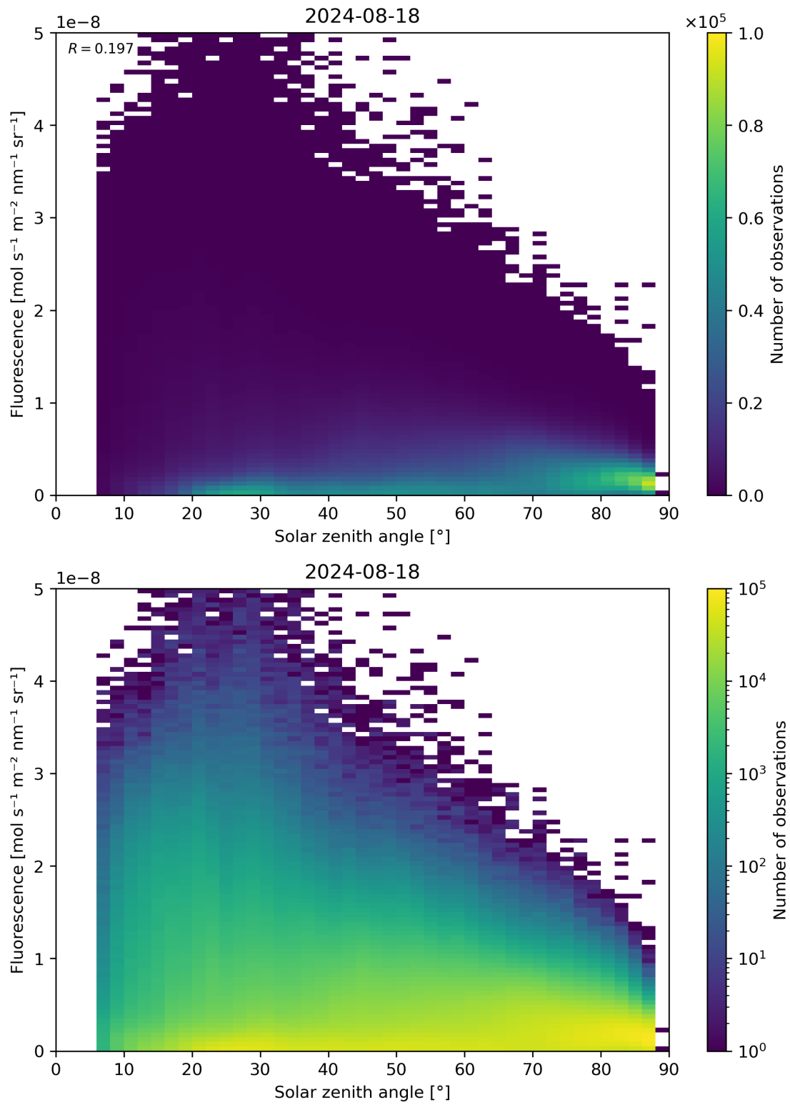
Figure 112: Scatter density plot of “Solar zenith angle” against “Fluorescence” for 2024-08-17 to 2024-08-19.
