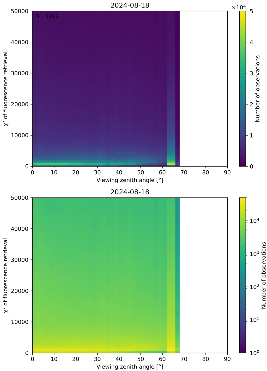
Figure 119: Scatter density plot of “Viewing zenith angle” against “ \chi^2 of fluorescence retrieval” for 2024-08-17 to 2024-08-19.
