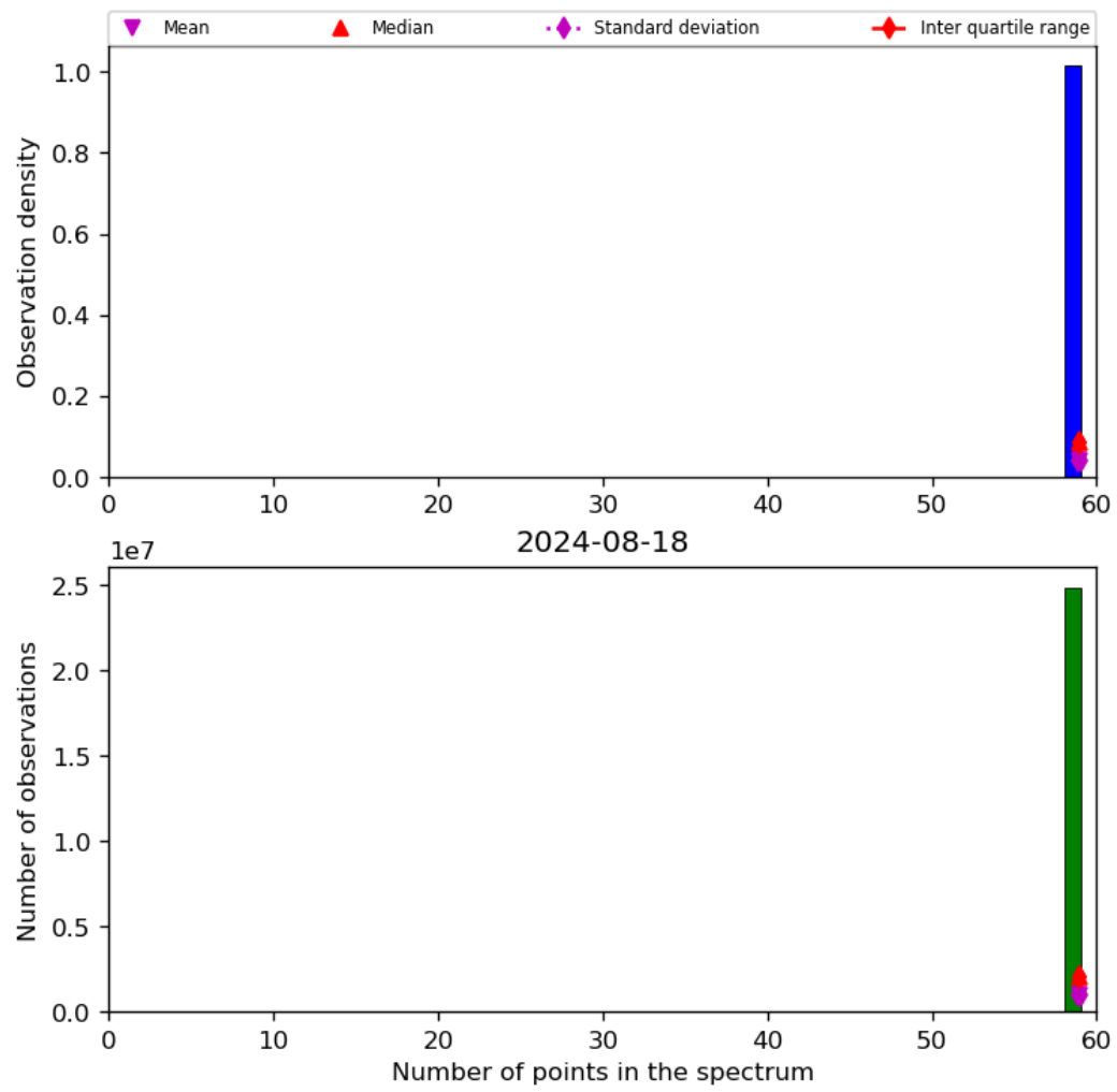
Figure 44: Histogram of “Number of points in the spectrum” for 2024-08-17 to 2024-08-19
