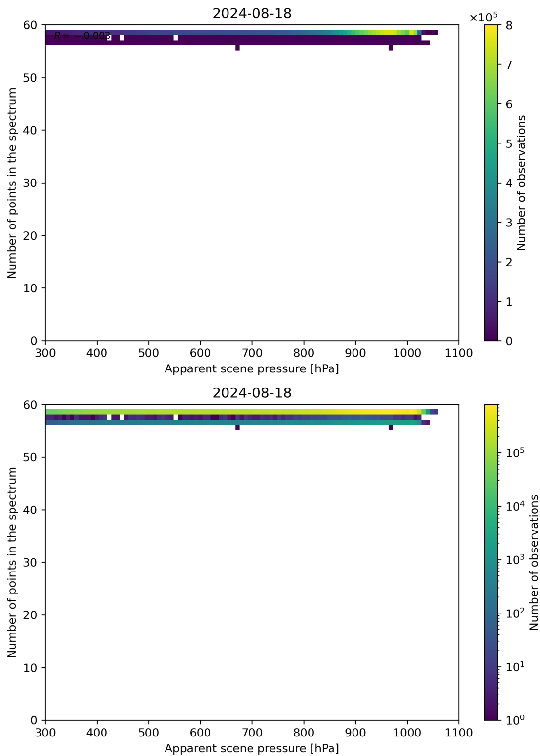
Figure 66: Scatter density plot of “Apparent scene pressure” against “Number of points in the spectrum” for 2024-08-17 to 2024-08-19.
