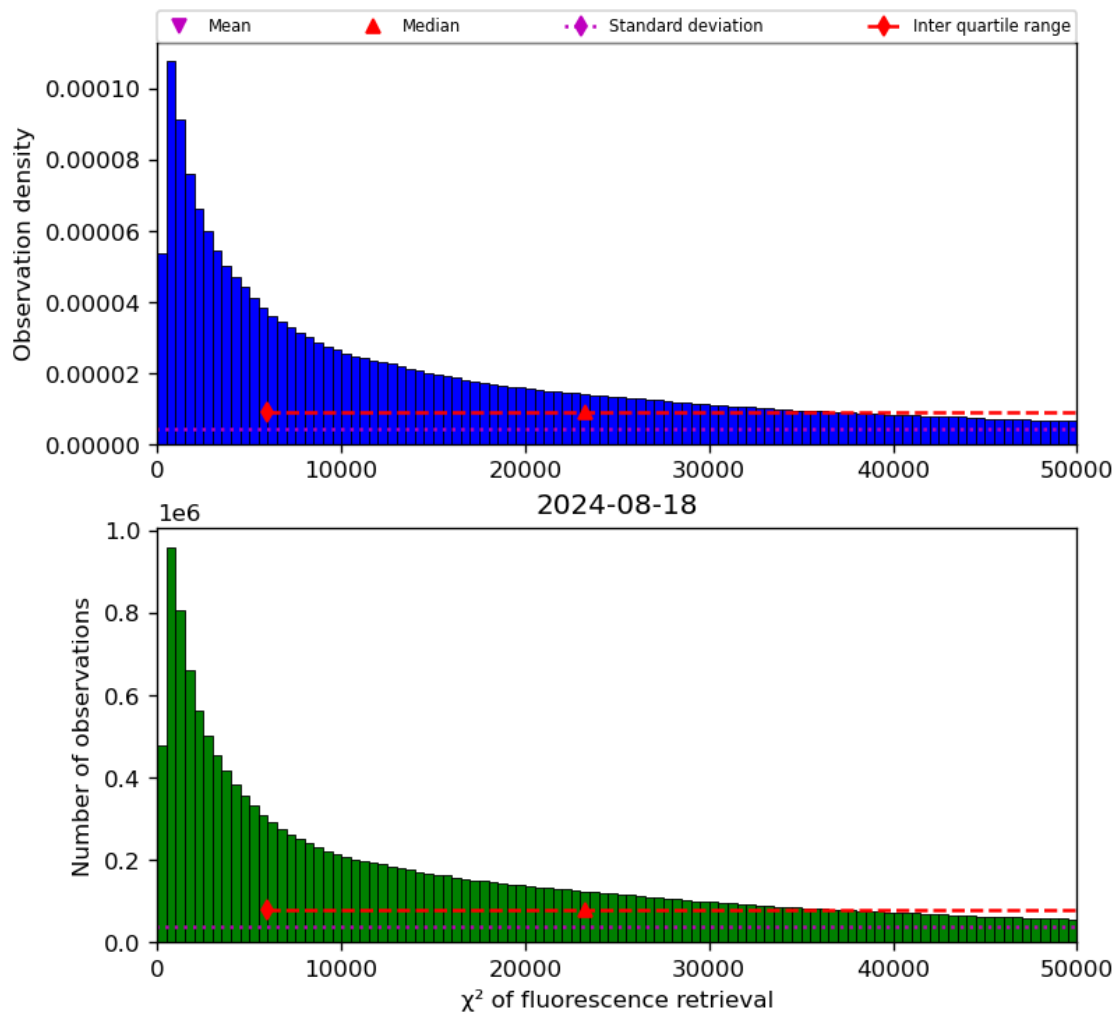
Figure 42: Histogram of “ \chi^2 of fluorescence retrieval” for 2024-08-17 to 2024-08-19
