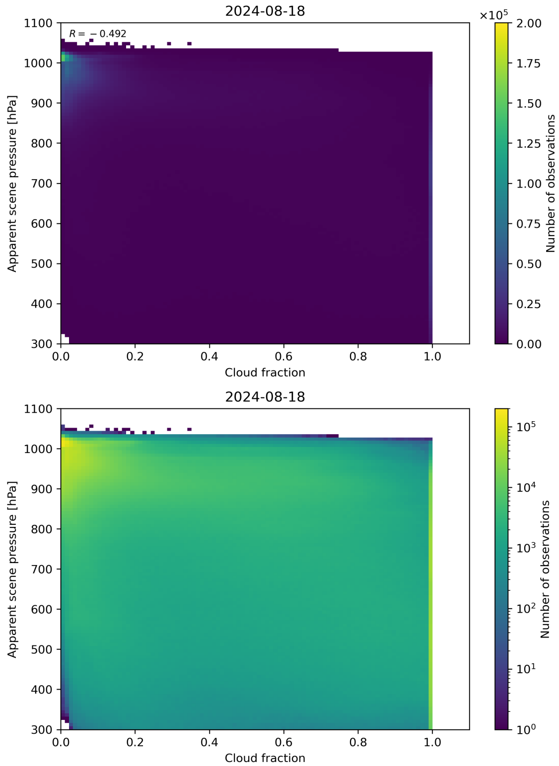
Figure 70: Scatter density plot of “Cloud fraction” against “Apparent scene pressure” for 2024-08-17 to 2024-08-19.
