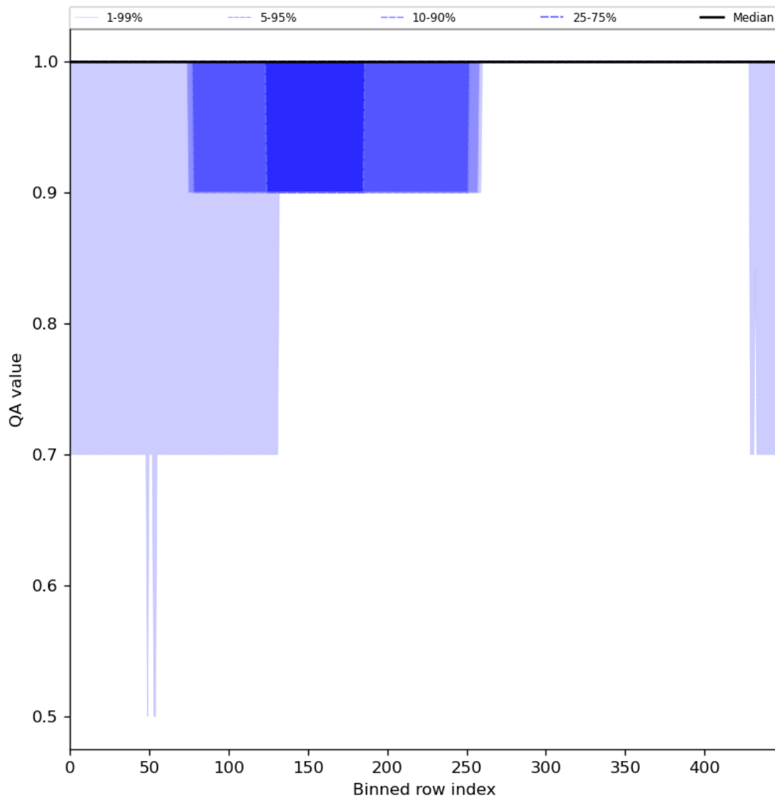
Figure 46: Along track statistics of “QA value” for 2024-08-17 to 2024-08-19
