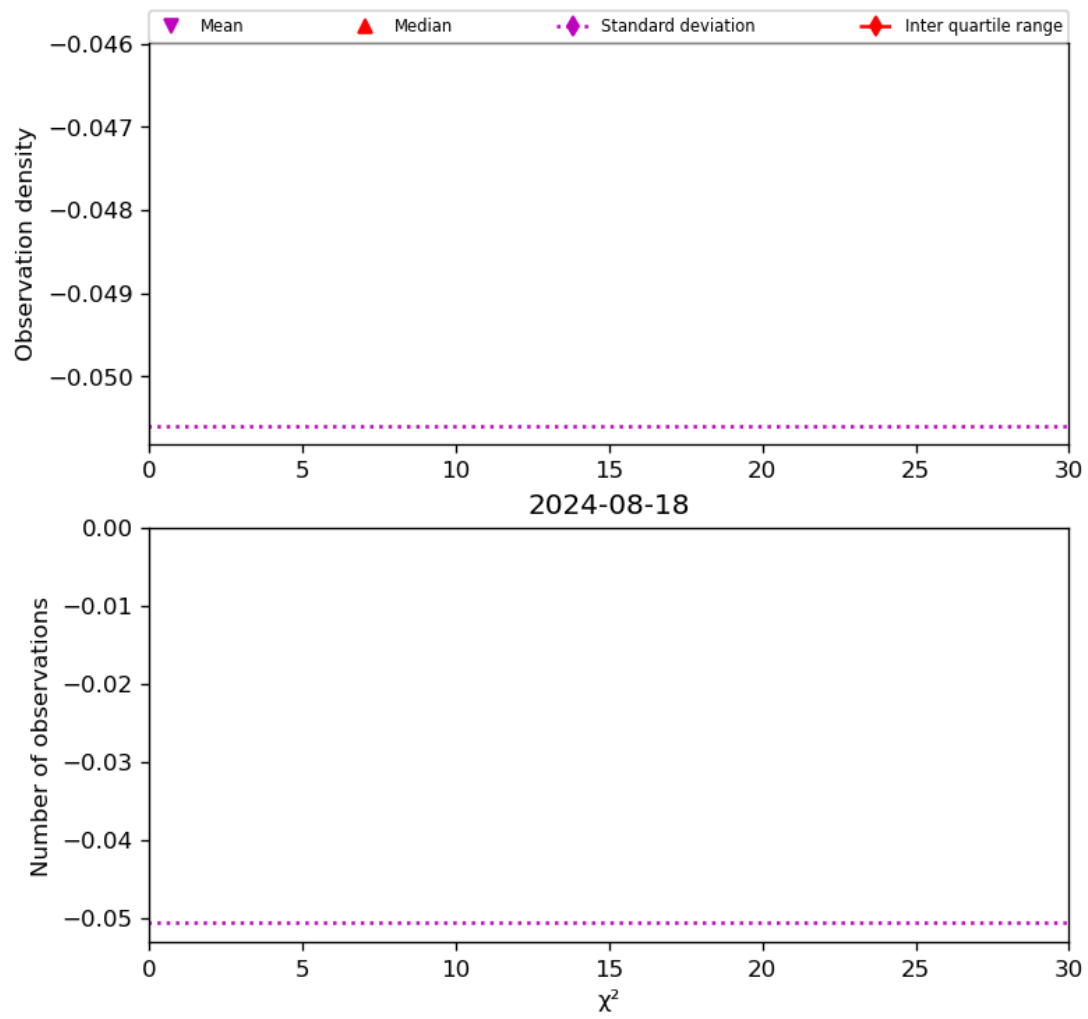
Figure 38: Histogram of " \chi^2 " for 2024-08-17 to 2024-08-19
