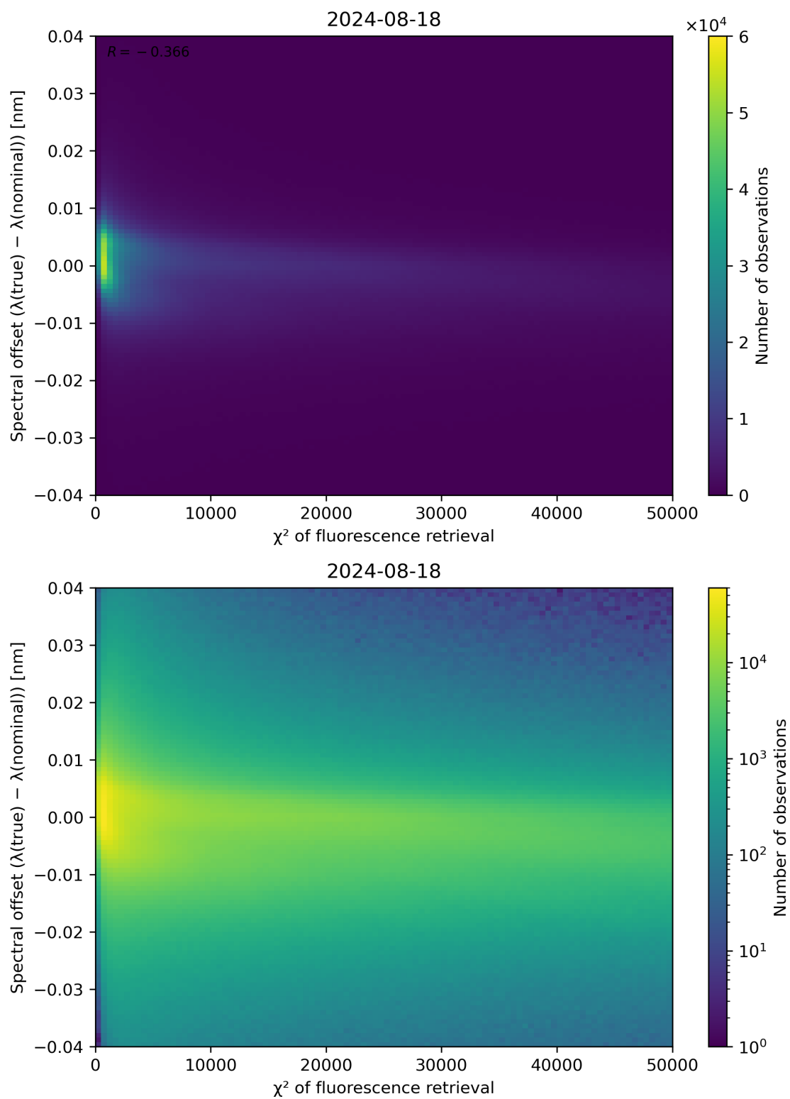
Figure 69: Scatter density plot of " \chi^2 of fluorescence retrieval" against "Spectral offset ( \lambda(\text{true}) - \lambda(\text{nominal}) )" for 2024-08-17 to 2024-08-19.
