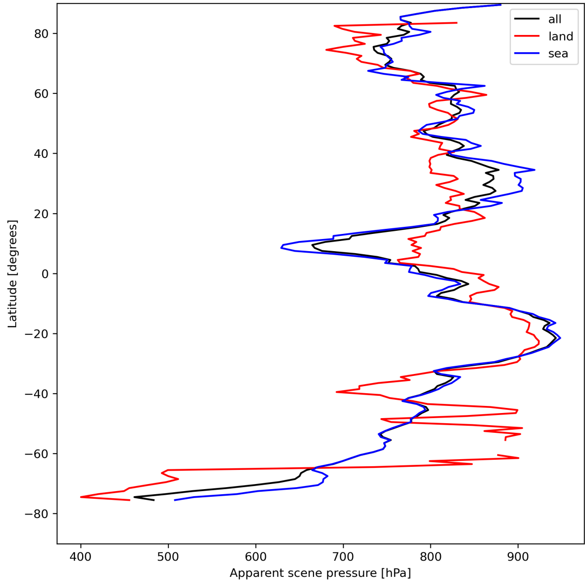
Figure 19: Zonal average of “Apparent scene pressure” for 2024-08-17 to 2024-08-19.
