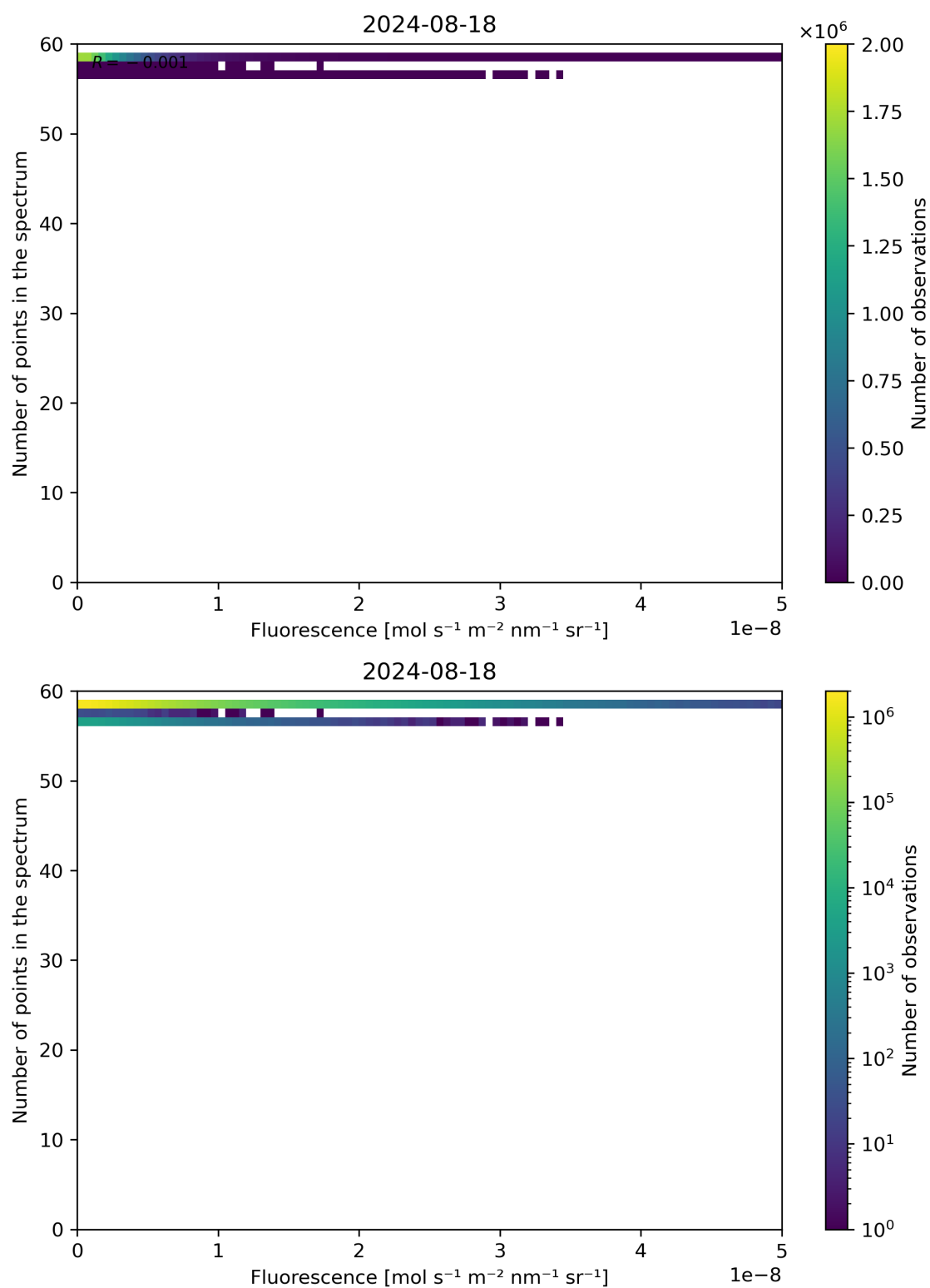
Figure 86: Scatter density plot of “Fluorescence” against “Number of points in the spectrum” for 2024-08-17 to 2024-08-19.
