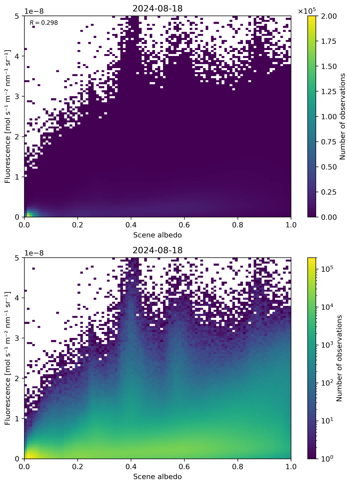
Figure 104: Scatter density plot of “Scene albedo” against “Fluorescence” for 2024-08-17 to 2024-08-19.
