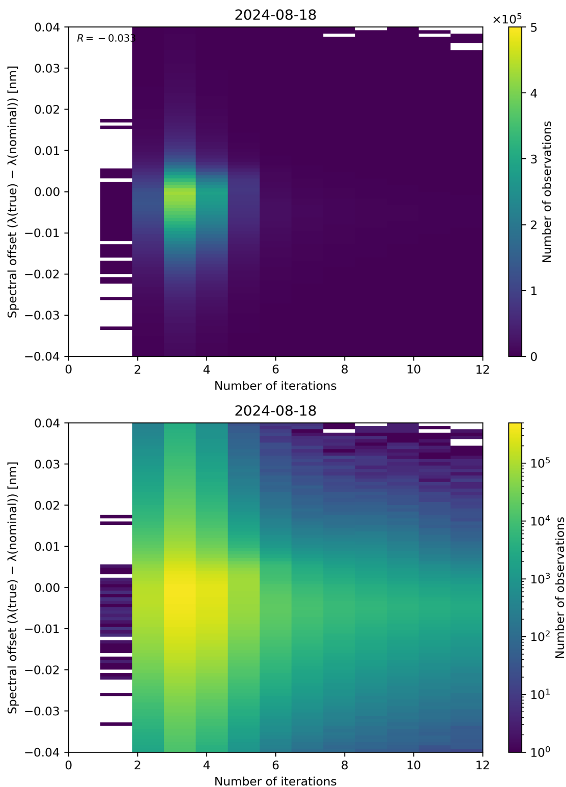
Figure 100: Scatter density plot of “Number of iterations” against “Spectral offset ( \lambda(\text{true}) - \lambda(\text{nominal}) )” for 2024-08-17 to 2024-08-19.
