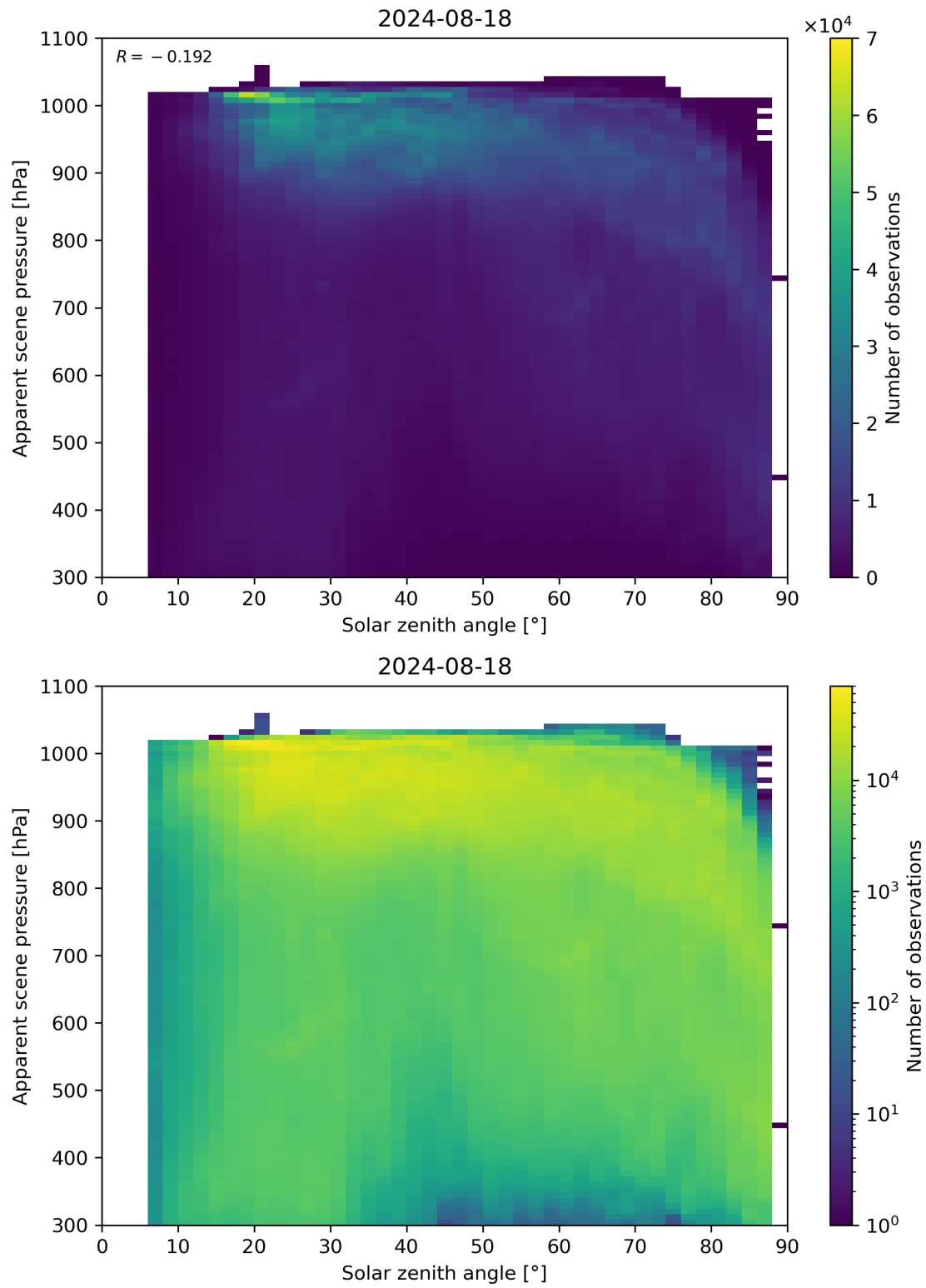
Figure 108: Scatter density plot of “Solar zenith angle” against “Apparent scene pressure” for 2024-08-17 to 2024-08-19.
