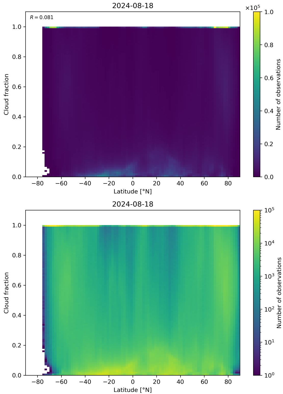
Figure 90: Scatter density plot of “Latitude” against “Cloud fraction” for 2024-08-17 to 2024-08-19.
