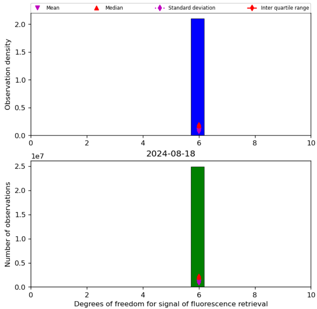
Figure 43: Histogram of “Degrees of freedom for signal of fluorescence retrieval” for 2024-08-17 to 2024-08-19
