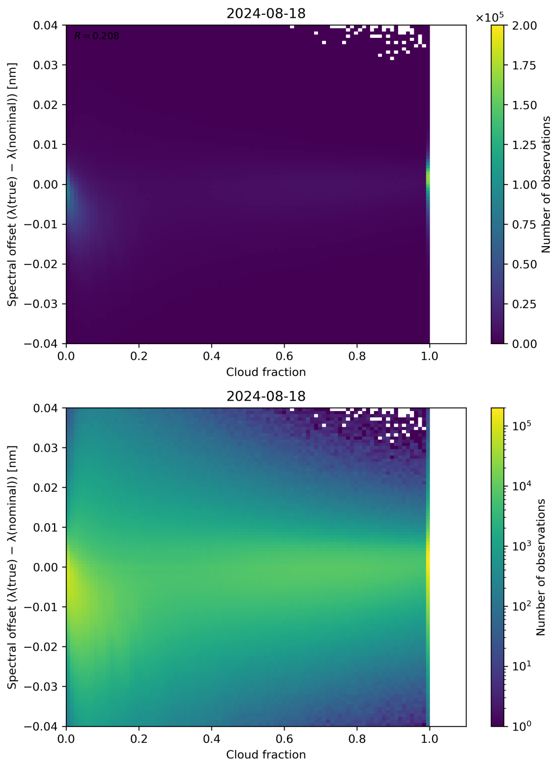
Figure 76: Scatter density plot of “Cloud fraction” against “Spectral offset ( \lambda(\text{true}) - \lambda(\text{nominal}) )” for 2024-08-17 to 2024-08-19.
