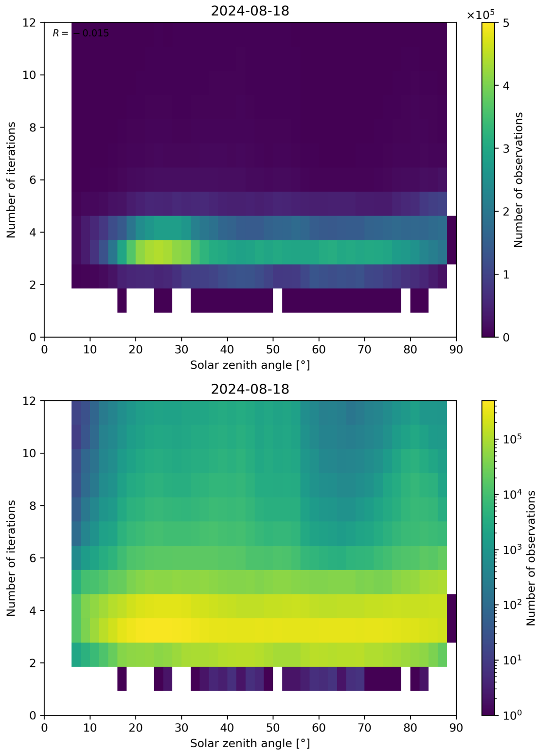
Figure 114: Scatter density plot of “Solar zenith angle” against “Number of iterations” for 2024-08-17 to 2024-08-19.
