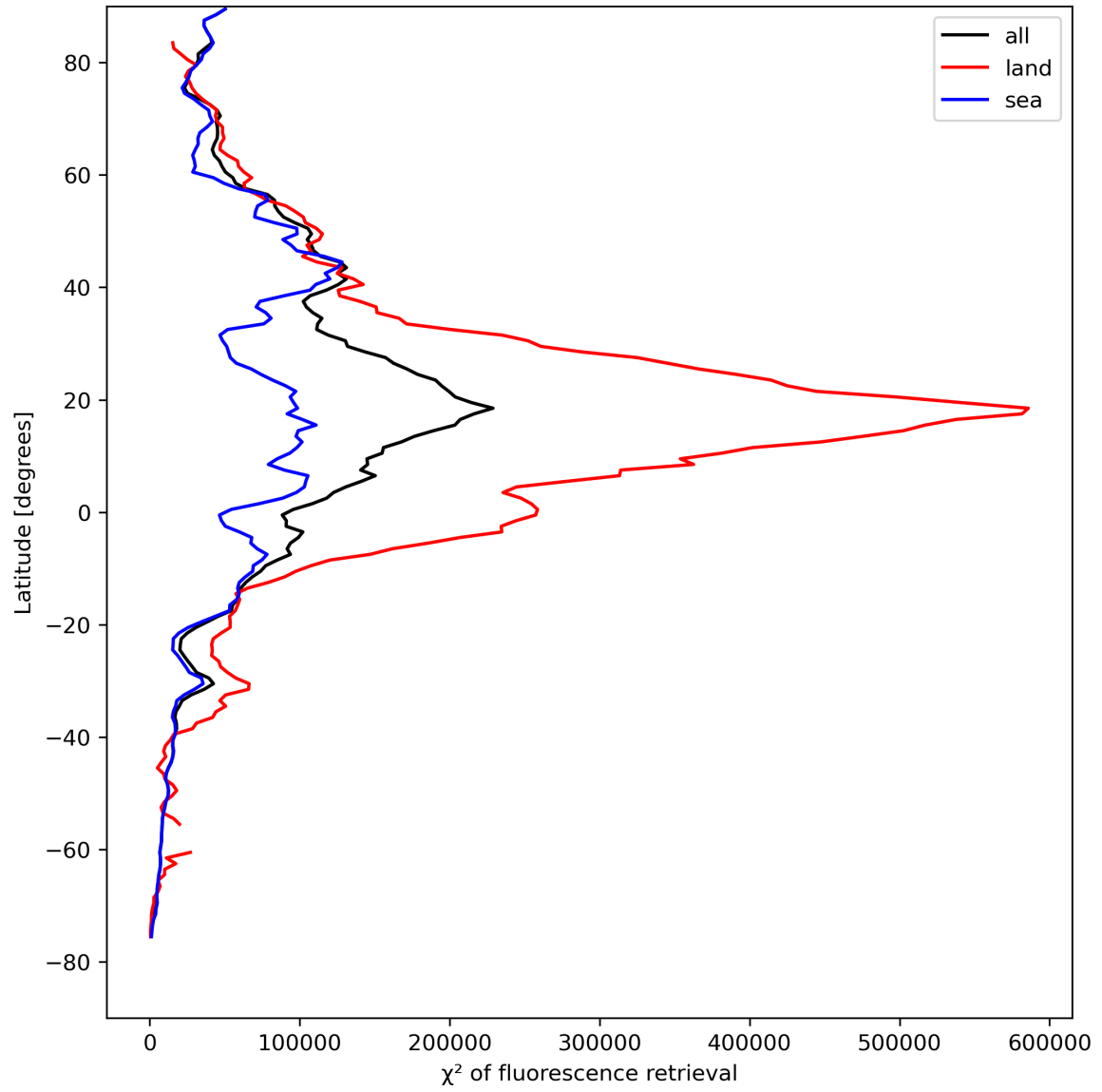
Figure 25: Zonal average of “ \chi^2 of fluorescence retrieval” for 2024-08-17 to 2024-08-19.
