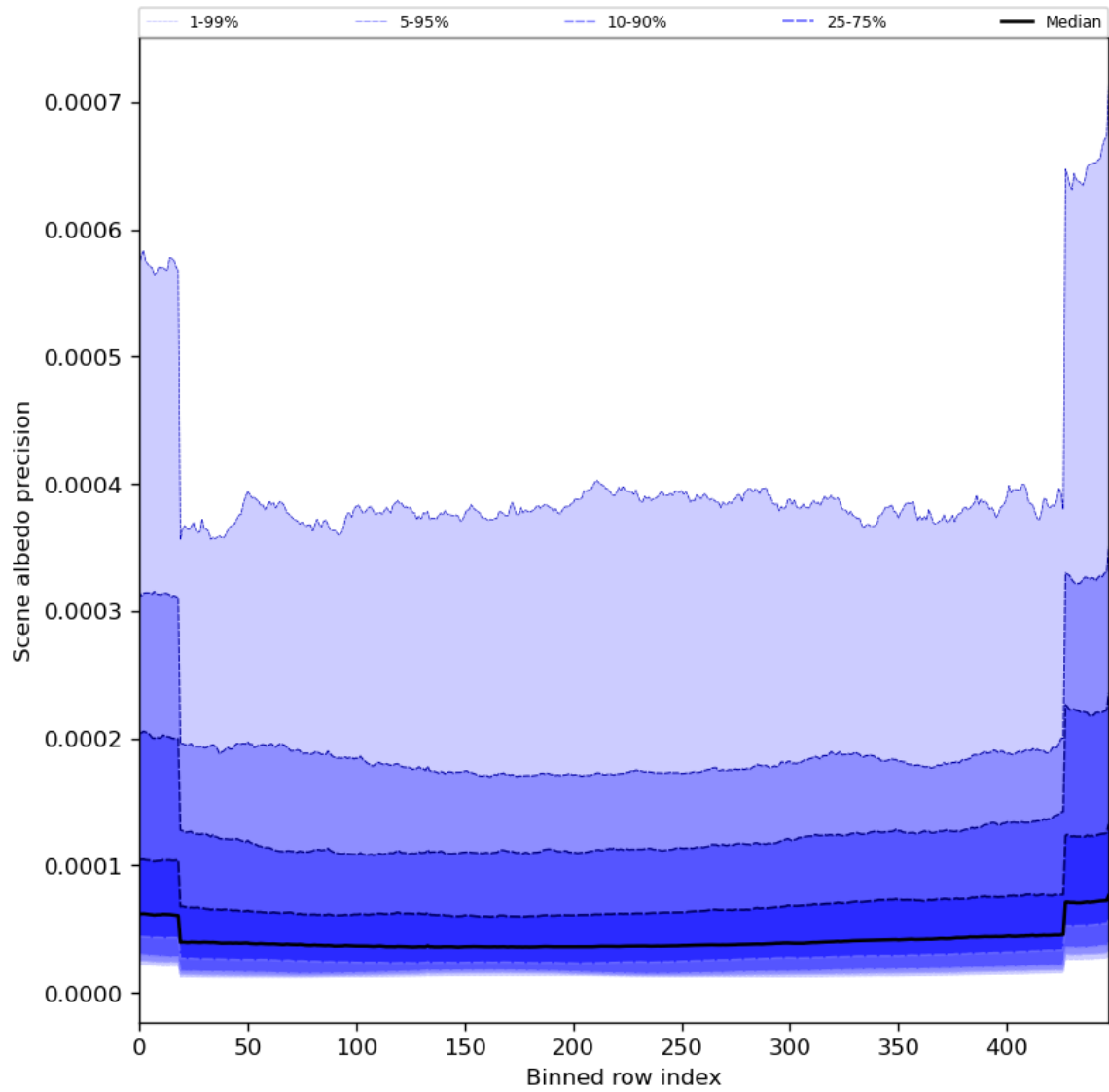
Figure 52: Along track statistics of “Scene albedo precision” for 2024-08-17 to 2024-08-19
