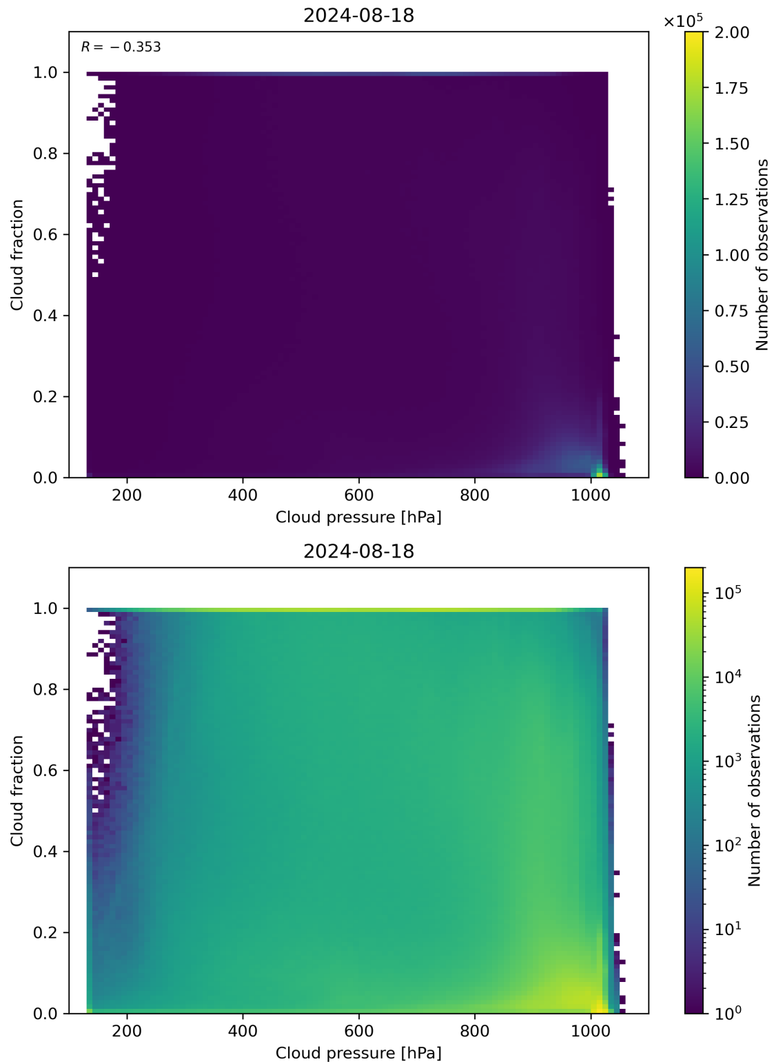
Figure 79: Scatter density plot of “Cloud pressure” against “Cloud fraction” for 2024-08-17 to 2024-08-19.
