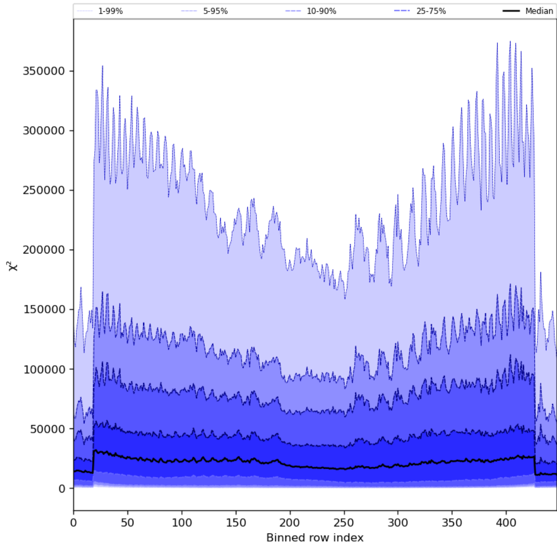
Figure 55: Along track statistics of “ \chi^2 ” for 2024-08-17 to 2024-08-19
