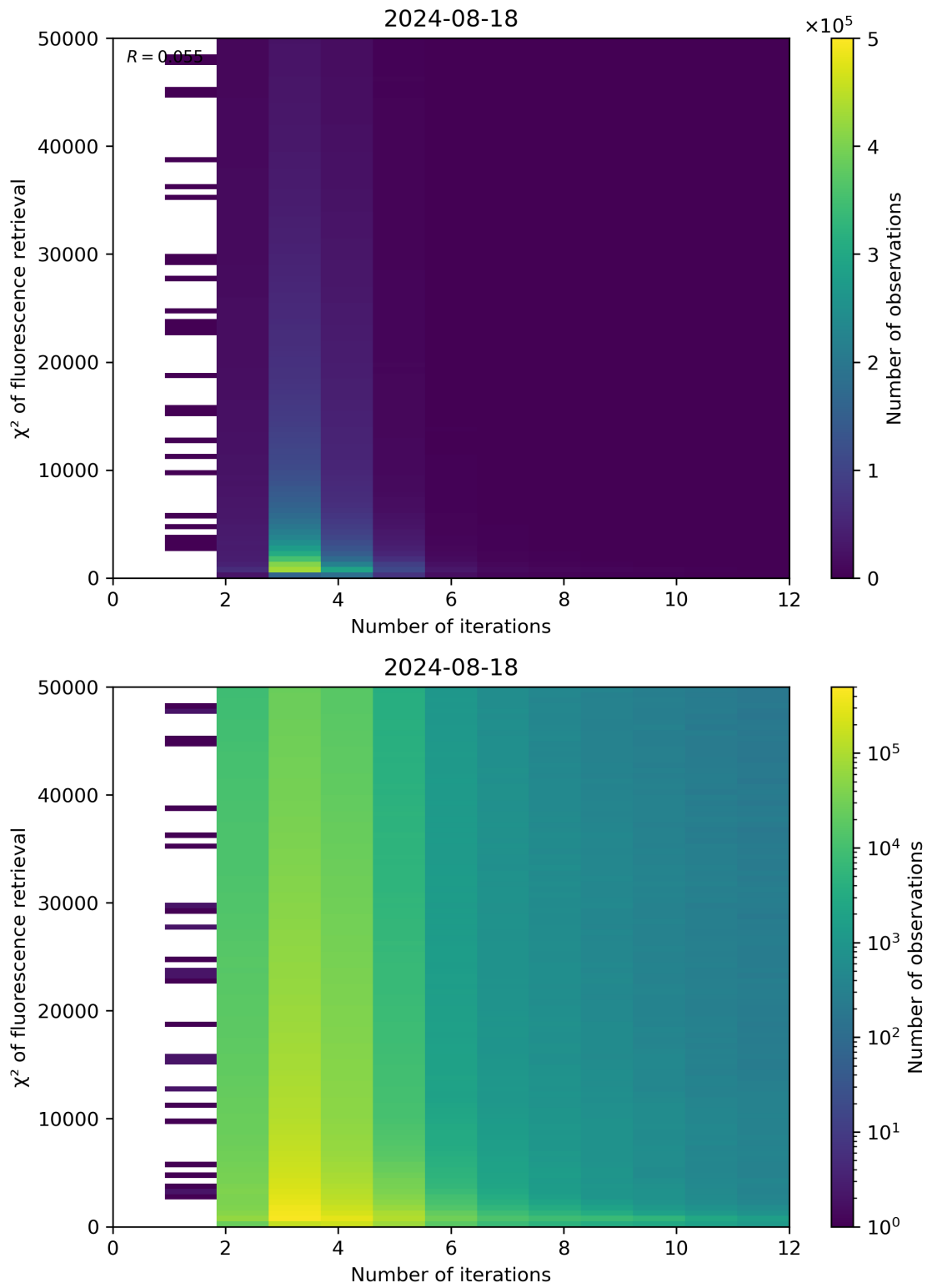
Figure 97: Scatter density plot of “Number of iterations” against “ \chi^2 of fluorescence retrieval” for 2024-08-17 to 2024-08-19.
