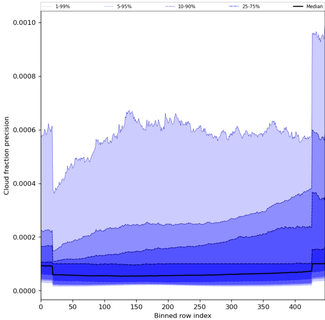
Figure 50: Along track statistics of “Cloud fraction precision” for 2024-08-17 to 2024-08-19
