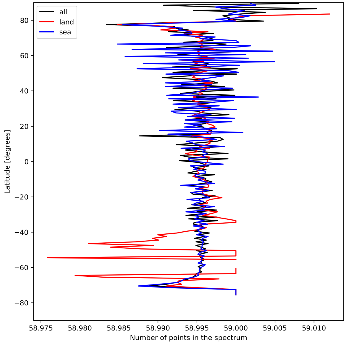
Figure 27: Zonal average of “Number of points in the spectrum” for 2024-08-17 to 2024-08-19.
