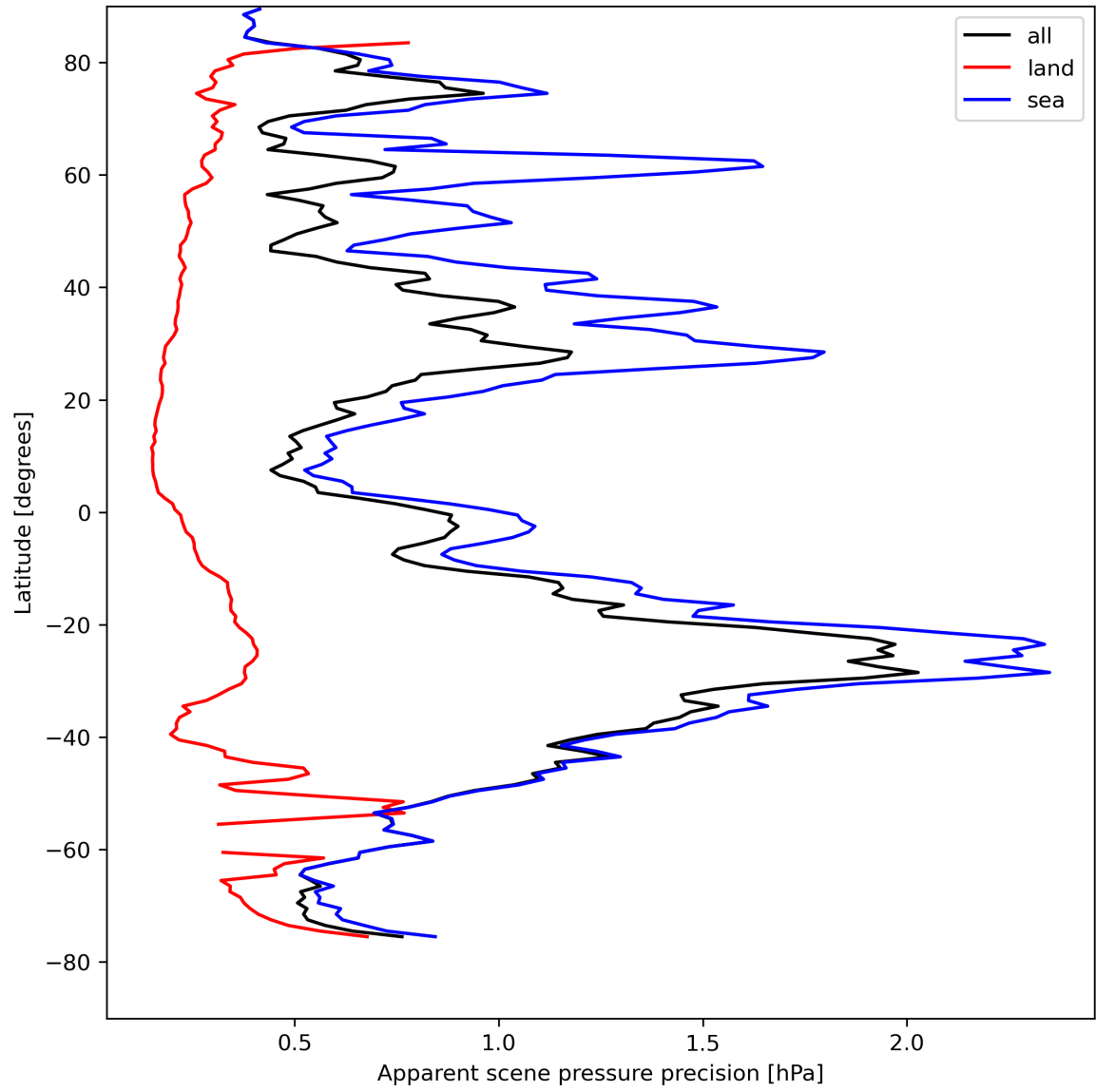
Figure 20: Zonal average of “Apparent scene pressure precision” for 2024-08-17 to 2024-08-19.
