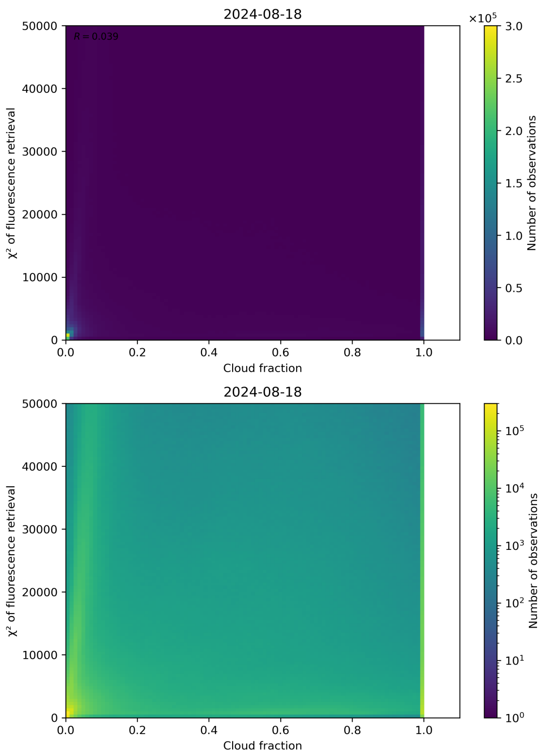
Figure 71: Scatter density plot of “Cloud fraction” against “ \chi^2 of fluorescence retrieval” for 2024-08-17 to 2024-08-19.
