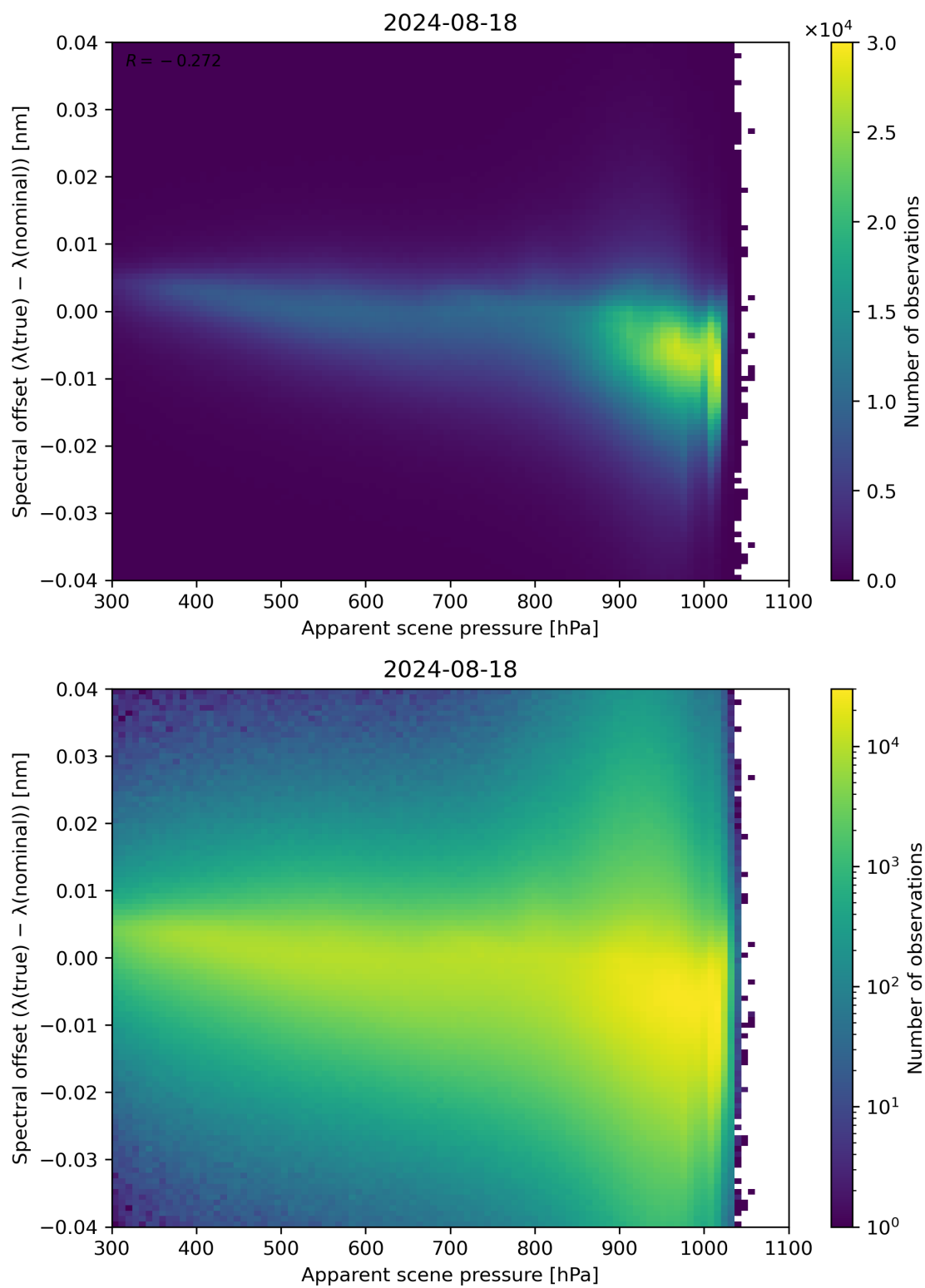
Figure 67: Scatter density plot of “Apparent scene pressure” against “Spectral offset ( \lambda(\text{true}) - \lambda(\text{nominal}) )” for 2024-08-17 to 2024-08-19.
