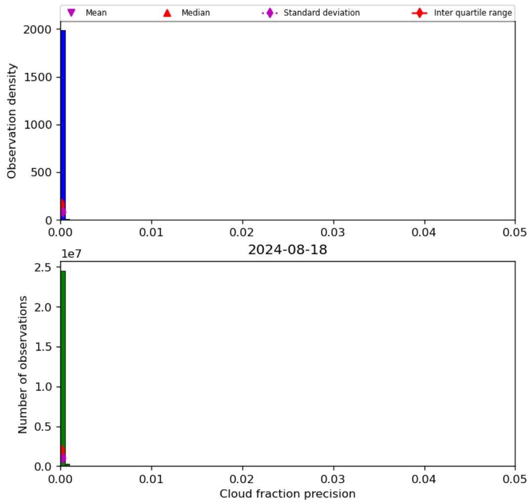
Figure 33: Histogram of “Cloud fraction precision” for 2024-08-17 to 2024-08-19
