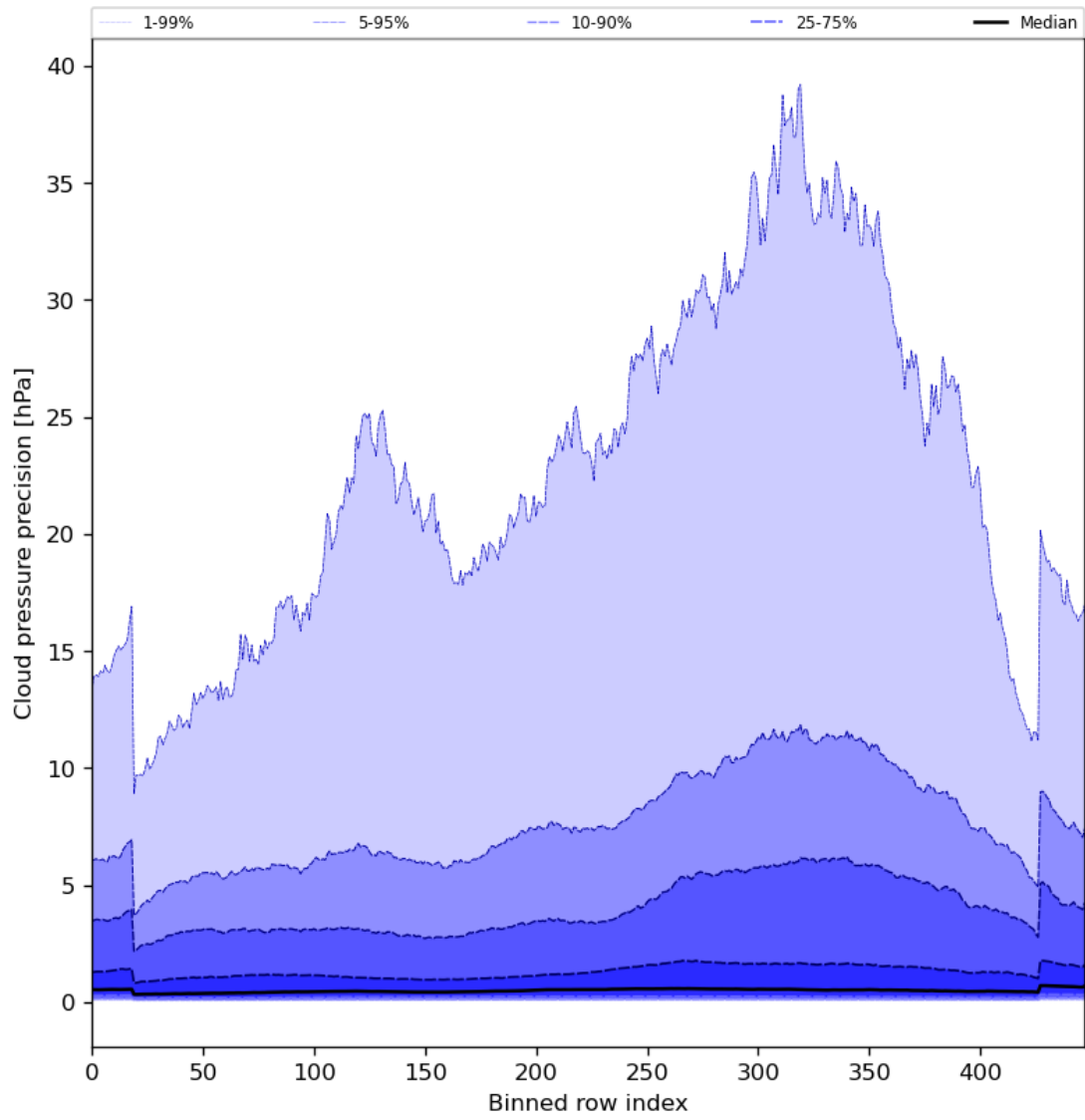
Figure 48: Along track statistics of “Cloud pressure precision” for 2024-08-17 to 2024-08-19
