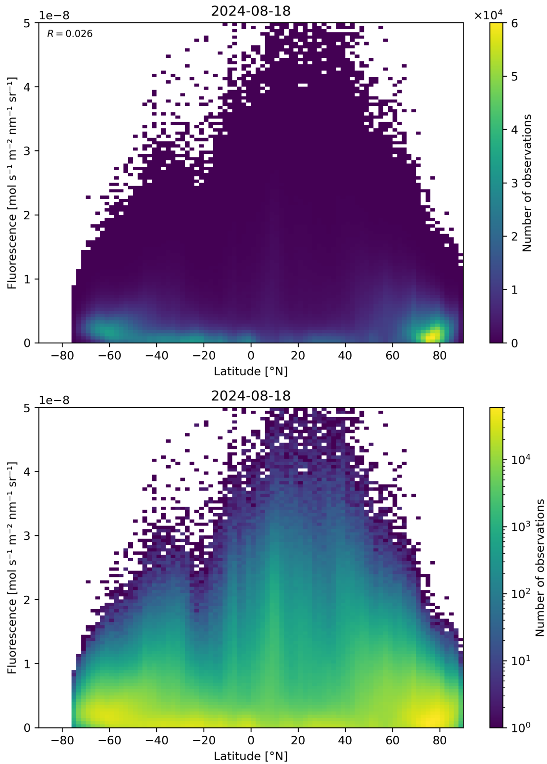
Figure 92: Scatter density plot of “Latitude” against “Fluorescence” for 2024-08-17 to 2024-08-19.
