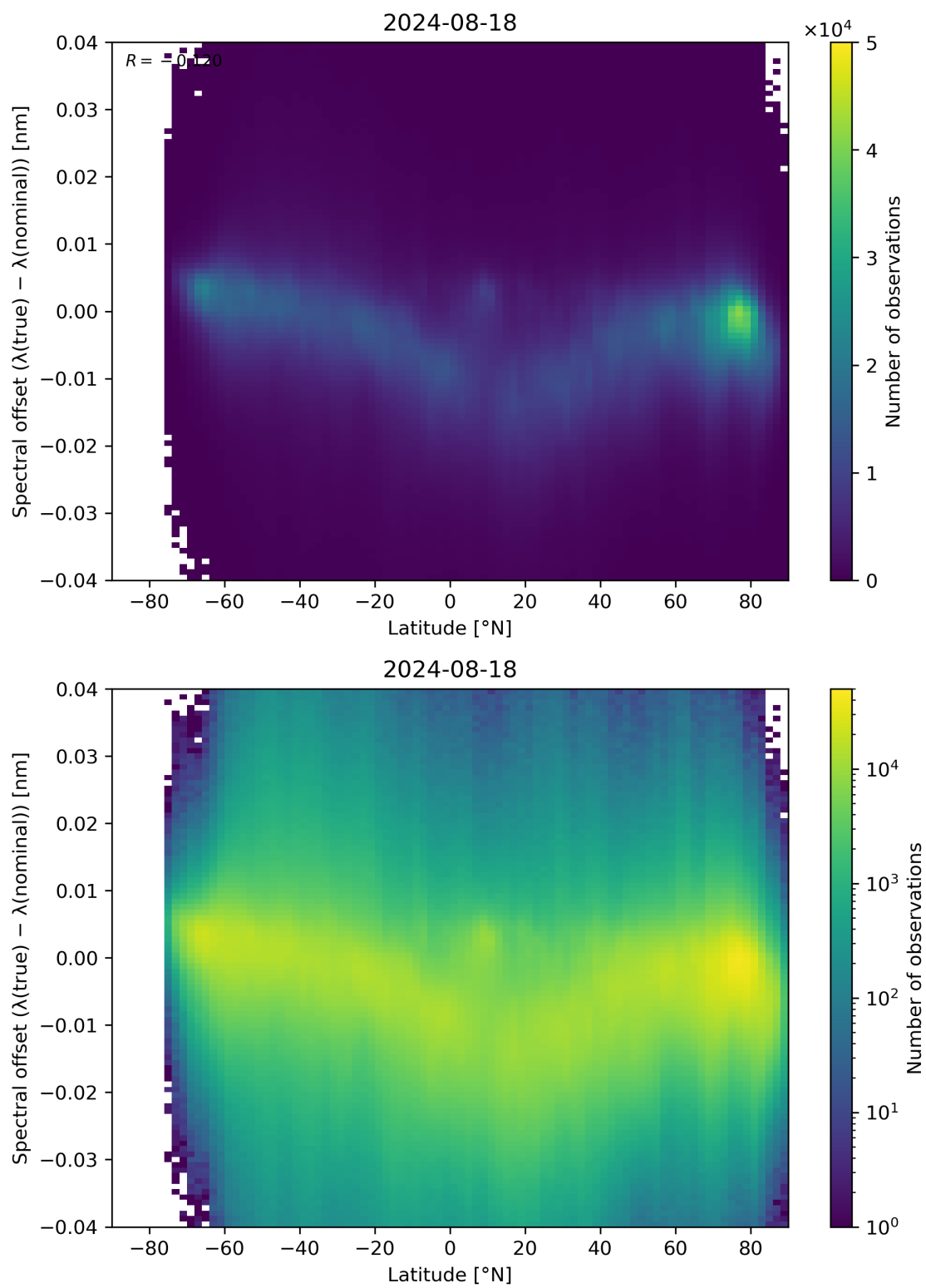
Figure 96: Scatter density plot of “Latitude” against “Spectral offset ( \lambda(\text{true}) - \lambda(\text{nominal}) )” for 2024-08-17 to 2024-08-19.
