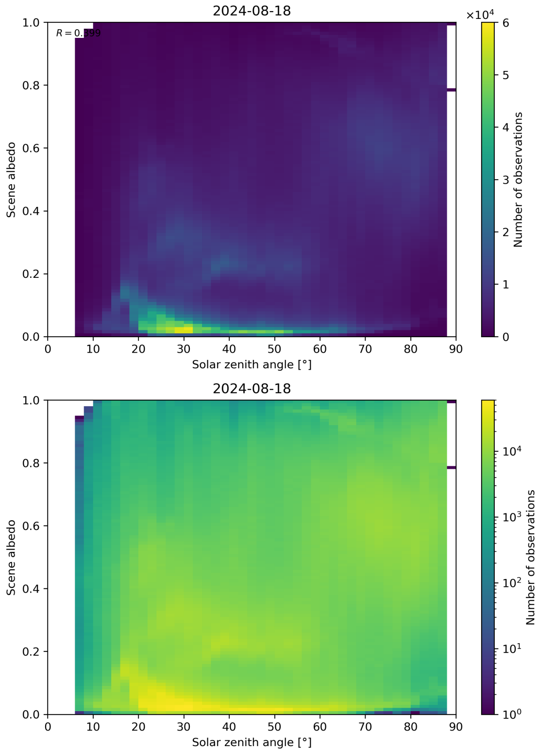
Figure 116: Scatter density plot of “Solar zenith angle” against “Scene albedo” for 2024-08-17 to 2024-08-19.
