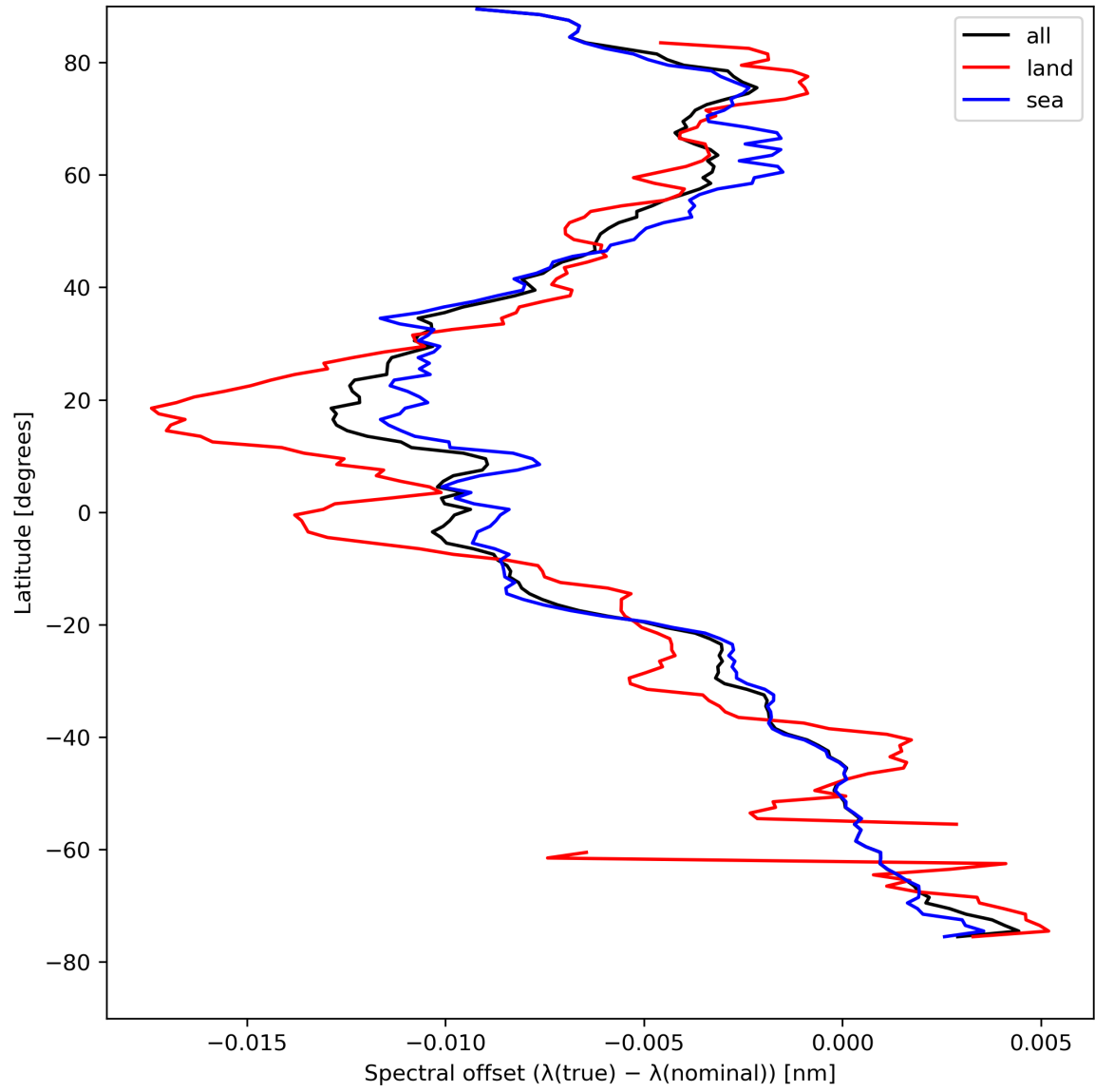
Figure 28: Zonal average of “Spectral offset ( \lambda(\text{true}) - \lambda(\text{nominal}) )” for 2024-08-17 to 2024-08-19.
