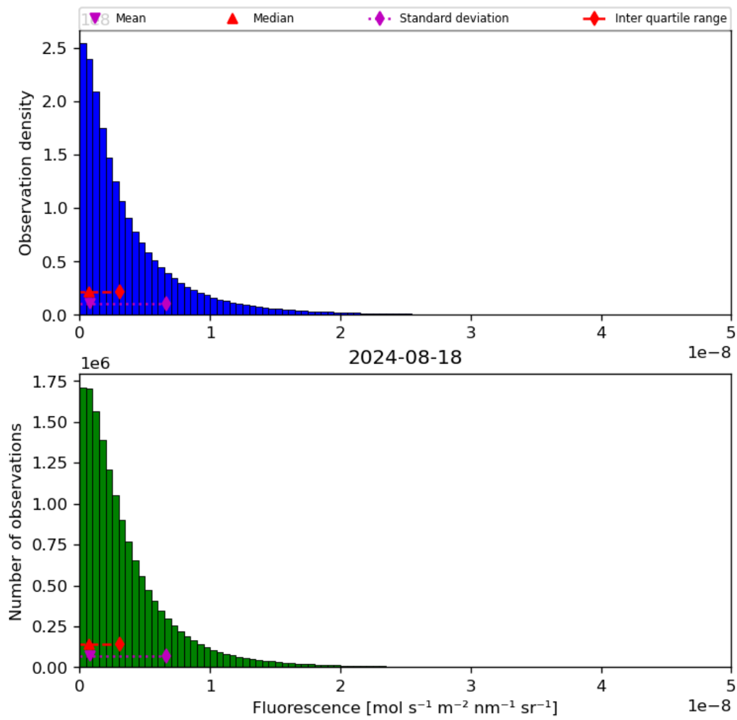
Figure 40: Histogram of “Fluorescence” for 2024-08-17 to 2024-08-19
