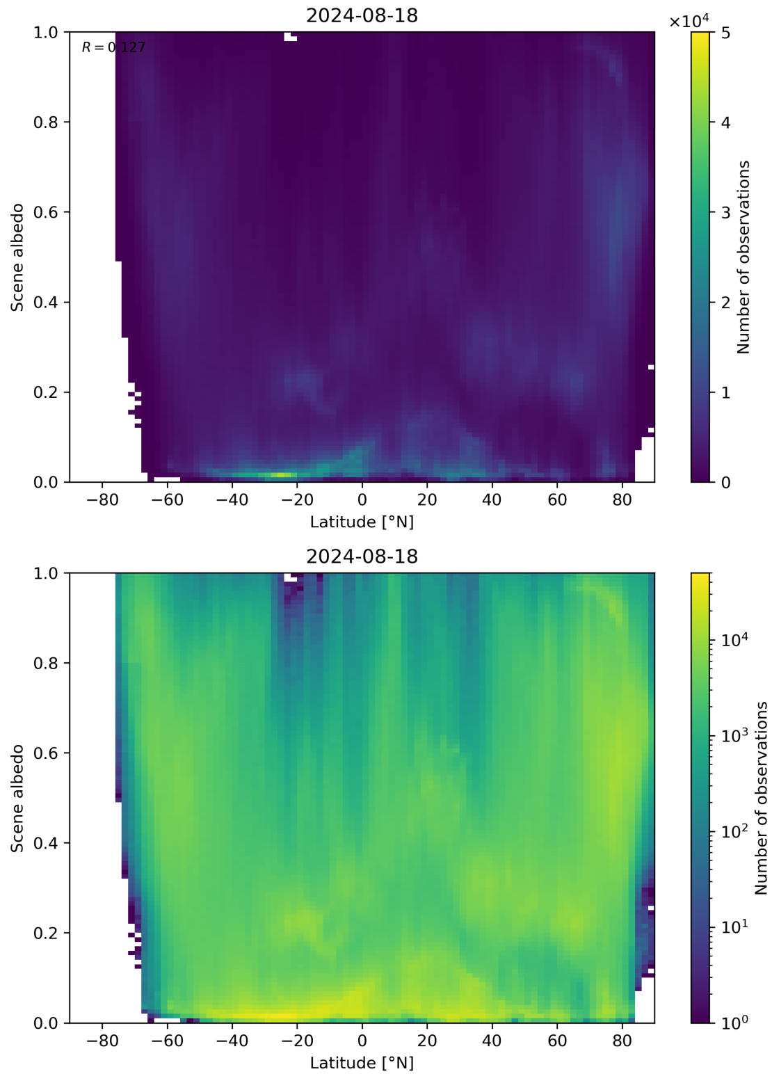
Figure 95: Scatter density plot of “Latitude” against “Scene albedo” for 2024-08-17 to 2024-08-19.
