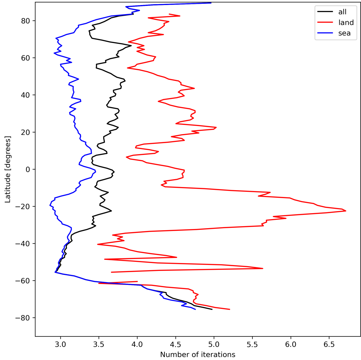
Figure 22: Zonal average of “Number of iterations” for 2024-08-17 to 2024-08-19.
