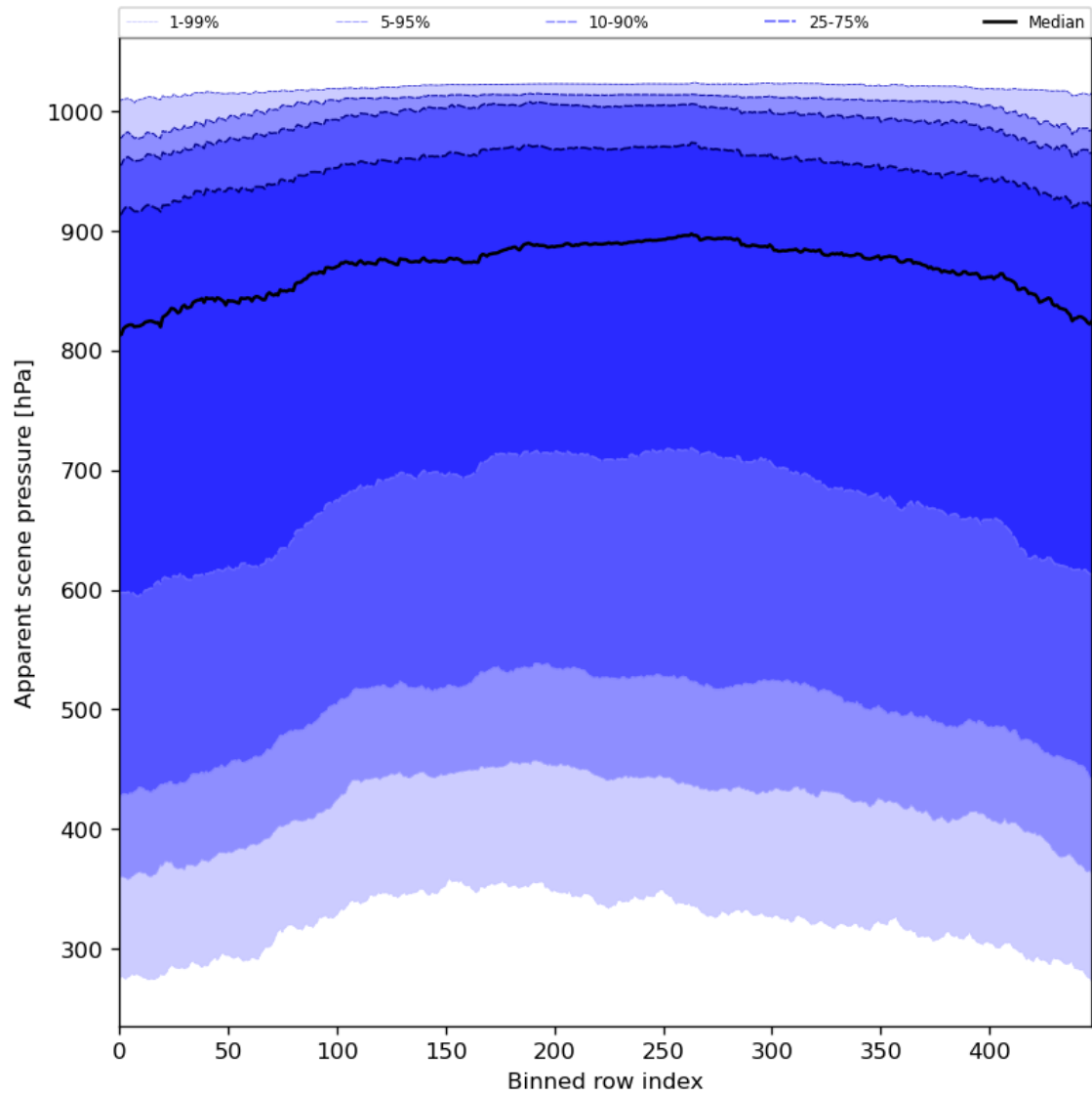
Figure 53: Along track statistics of “Apparent scene pressure” for 2024-08-17 to 2024-08-19
