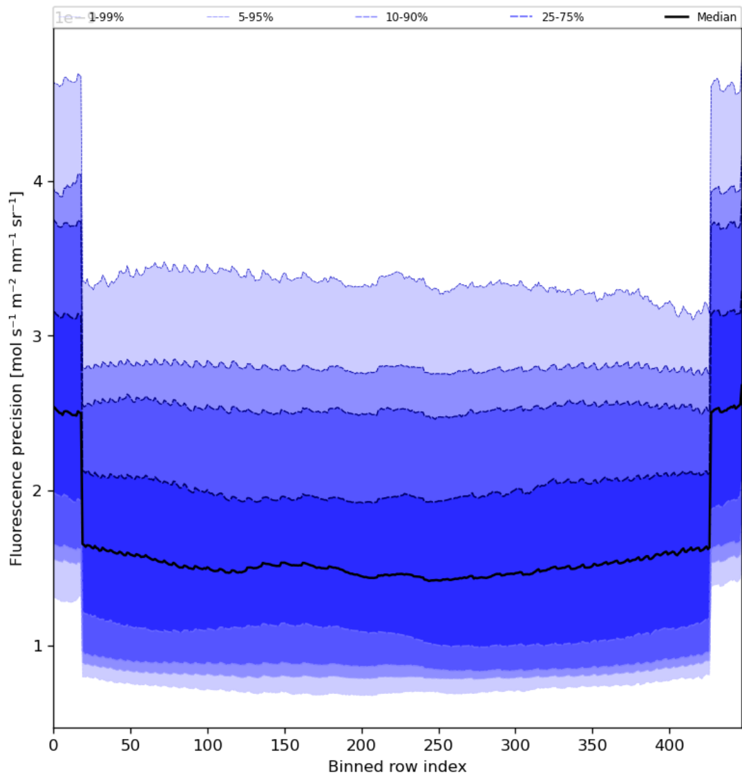
Figure 58: Along track statistics of “Fluorescence precision” for 2024-08-17 to 2024-08-19
