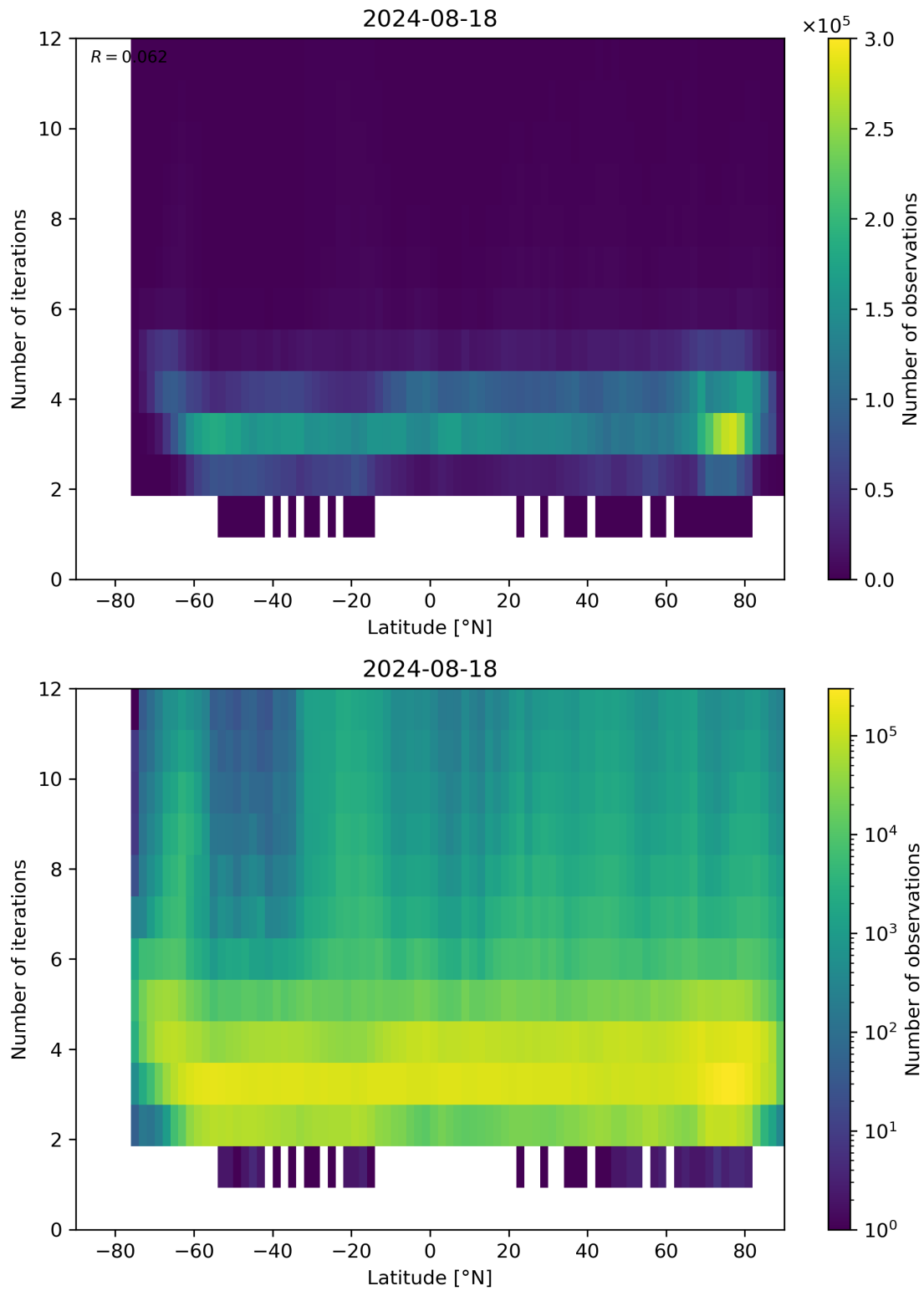
Figure 93: Scatter density plot of “Latitude” against “Number of iterations” for 2024-08-17 to 2024-08-19.
