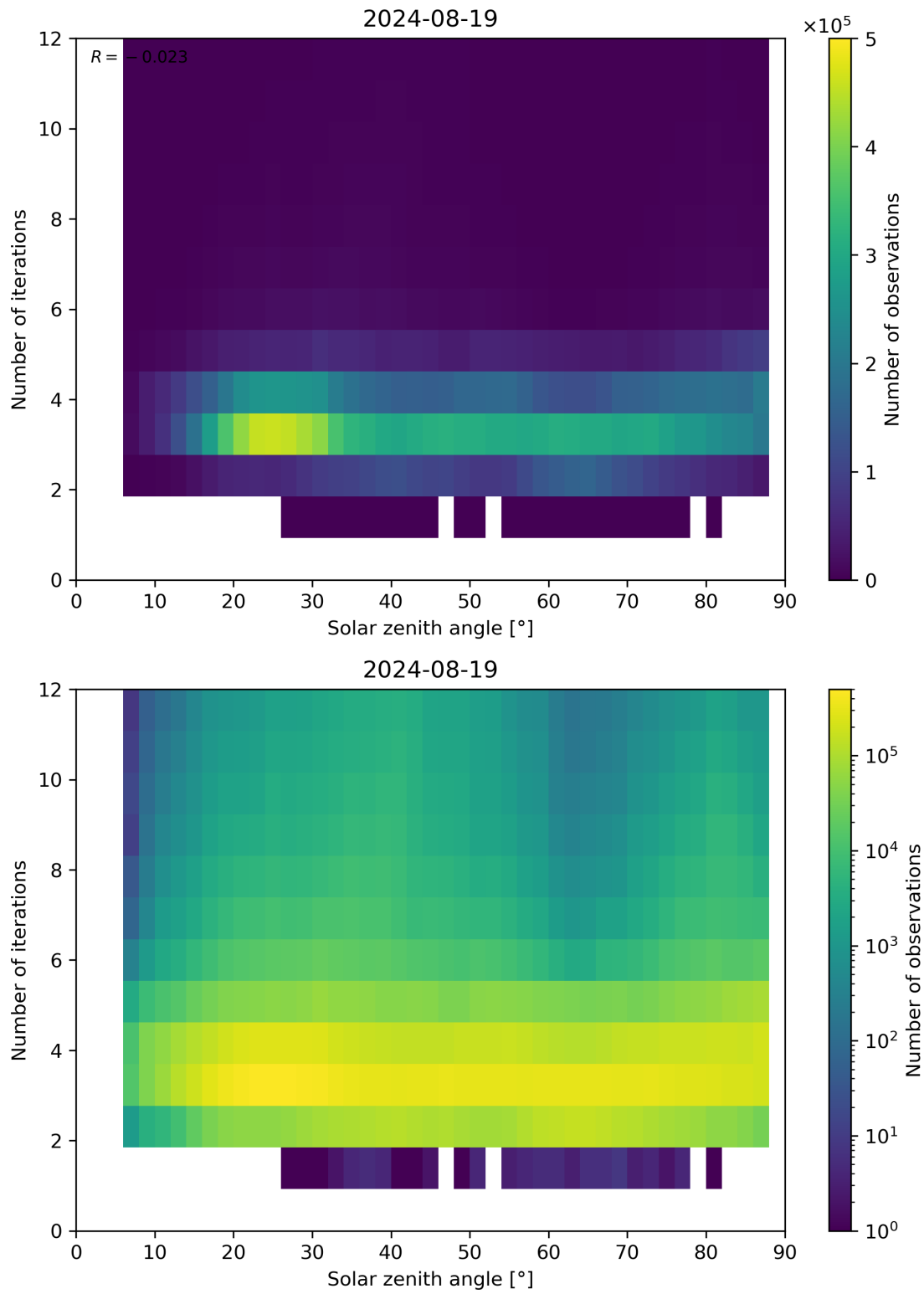
Figure 114: Scatter density plot of “Solar zenith angle” against “Number of iterations” for 2024-08-18 to 2024-08-20.
