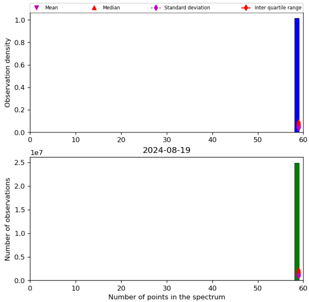
Figure 44: Histogram of “Number of points in the spectrum” for 2024-08-18 to 2024-08-20
