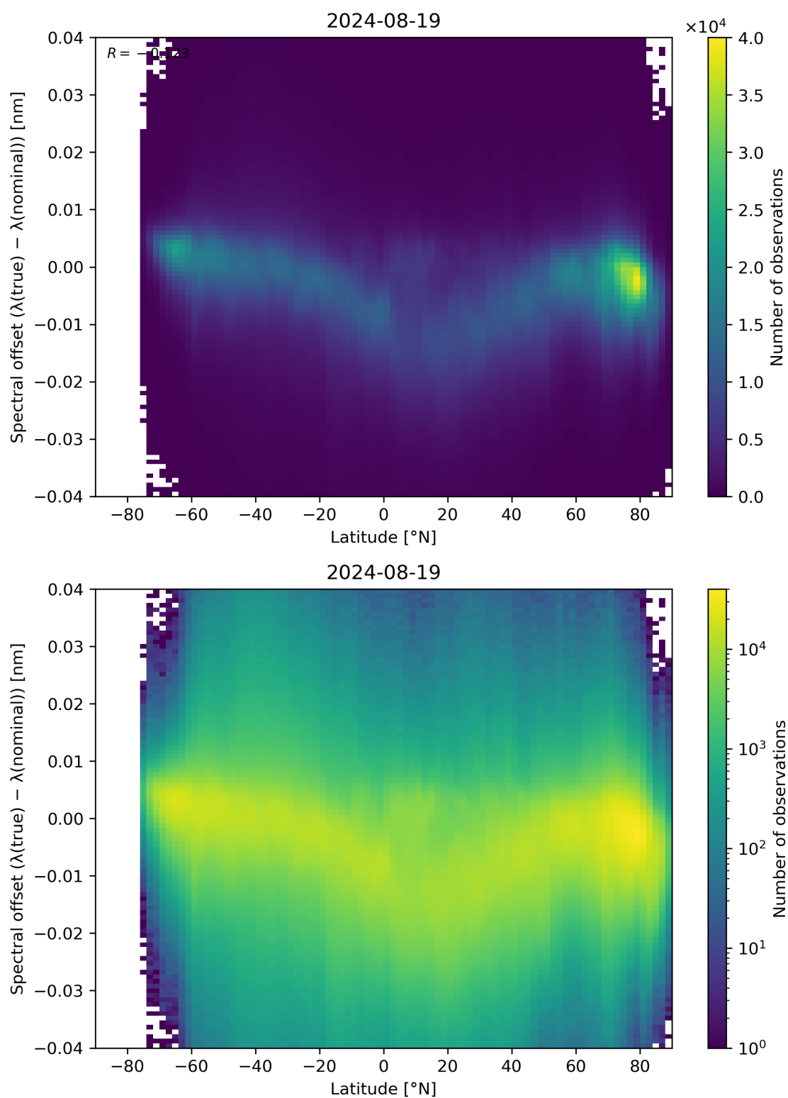
Figure 96: Scatter density plot of “Latitude” against “Spectral offset ( \lambda(\text{true}) - \lambda(\text{nominal}) )” for 2024-08-18 to 2024-08-20.
