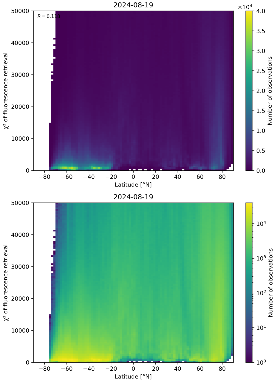
Figure 89: Scatter density plot of “Latitude” against “ \chi^2 of fluorescence retrieval” for 2024-08-18 to 2024-08-20.
