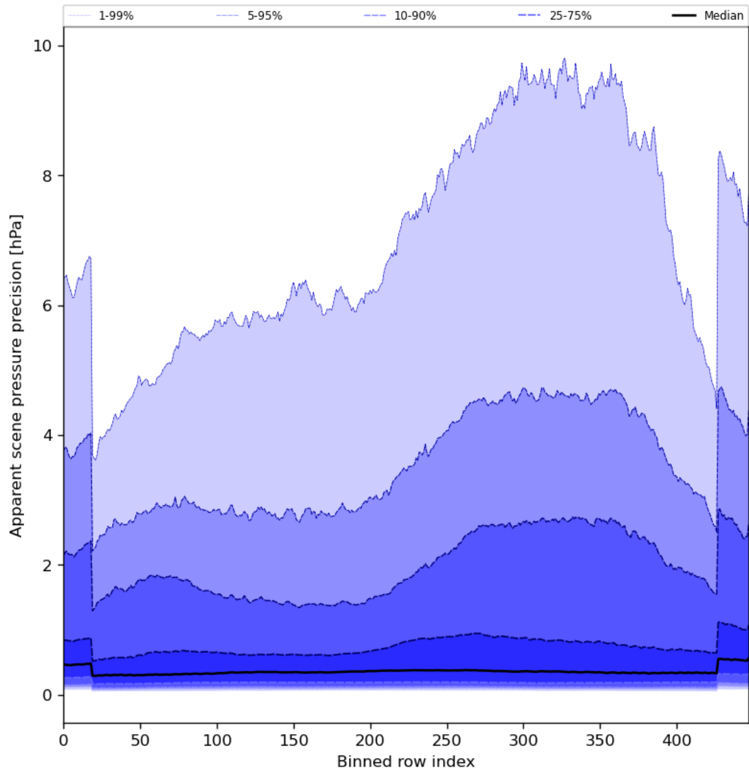
Figure 54: Along track statistics of “Apparent scene pressure precision” for 2024-08-18 to 2024-08-20
