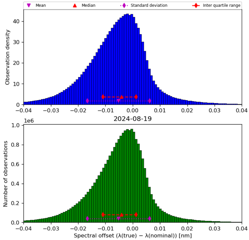
Figure 45: Histogram of “Spectral offset ( \lambda(\text{true}) - \lambda(\text{nominal}) )” for 2024-08-18 to 2024-08-20
