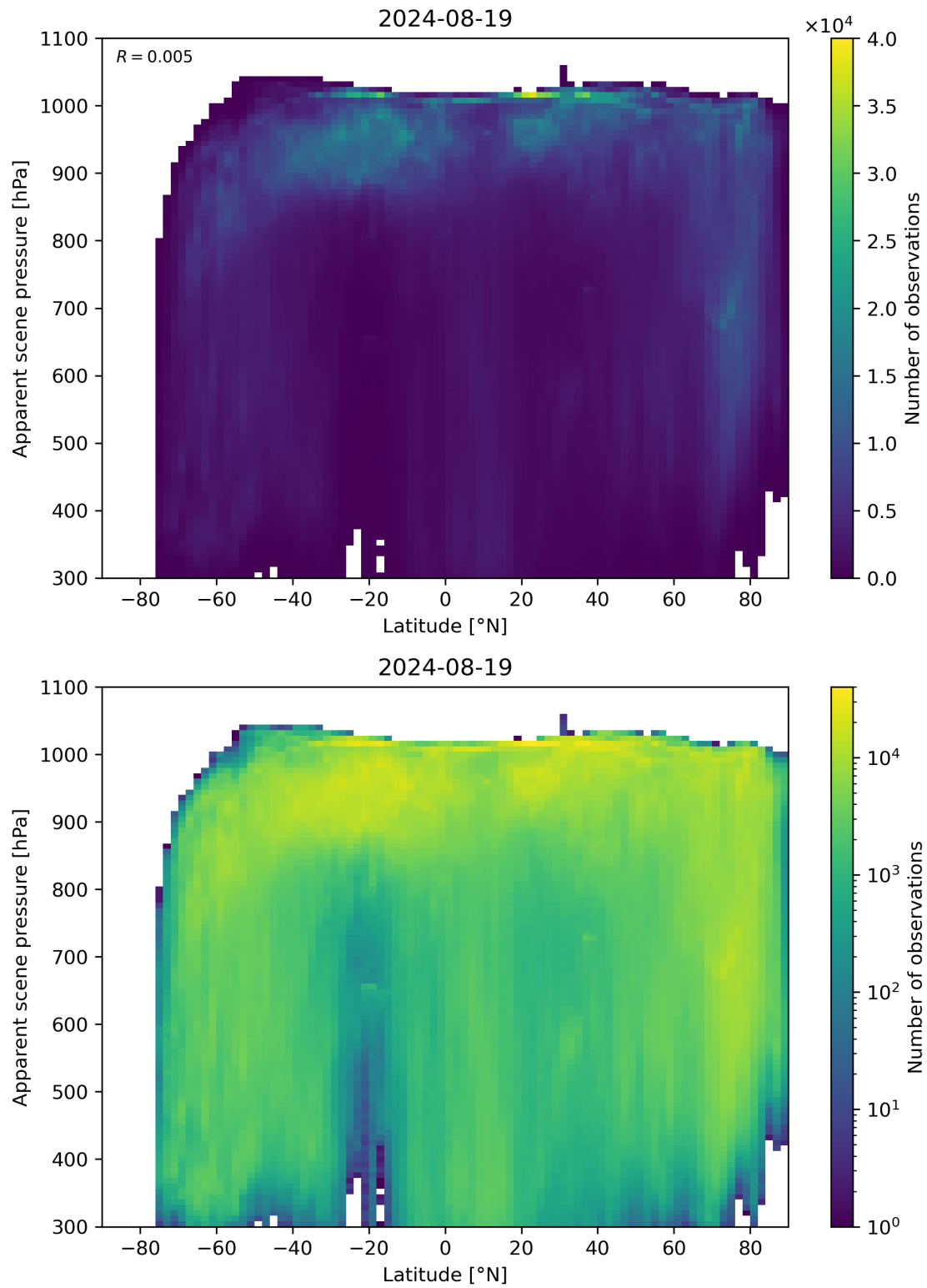
Figure 88: Scatter density plot of “Latitude” against “Apparent scene pressure” for 2024-08-18 to 2024-08-20.
