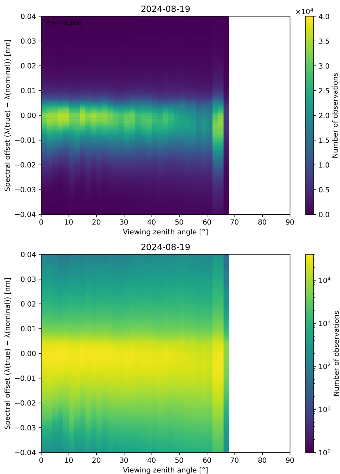
Figure 128: Scatter density plot of “Viewing zenith angle” against “Spectral offset ( \lambda(\text{true}) - \lambda(\text{nominal}) )” for 2024-08-18 to 2024-08-20.
