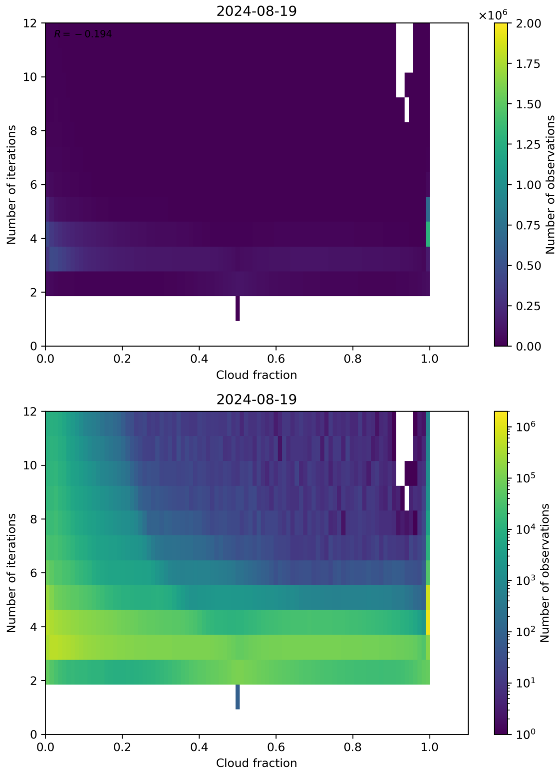
Figure 73: Scatter density plot of “Cloud fraction” against “Number of iterations” for 2024-08-18 to 2024-08-20.
