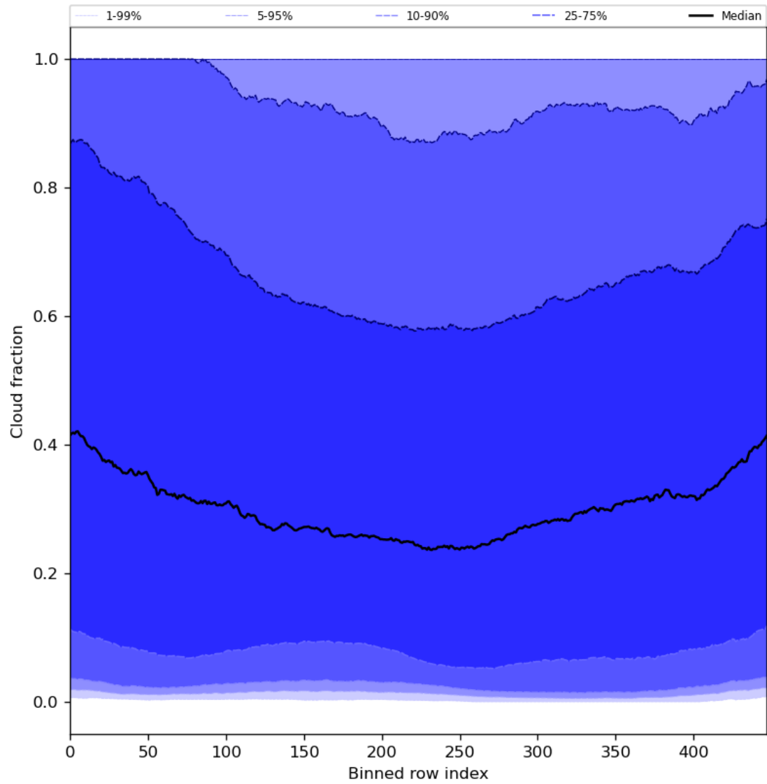
Figure 49: Along track statistics of “Cloud fraction” for 2024-08-18 to 2024-08-20
