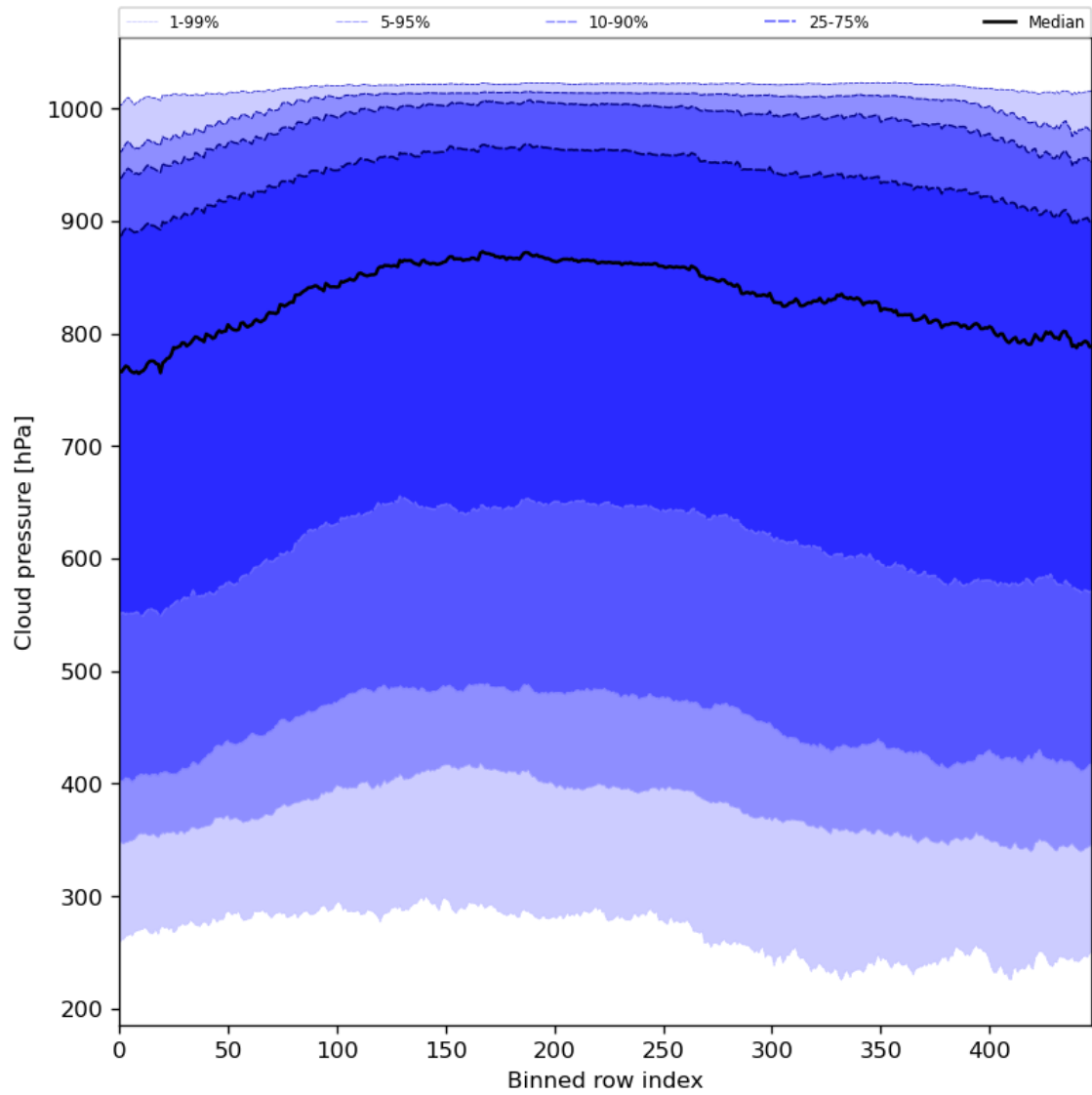
Figure 47: Along track statistics of “Cloud pressure” for 2024-08-18 to 2024-08-20
