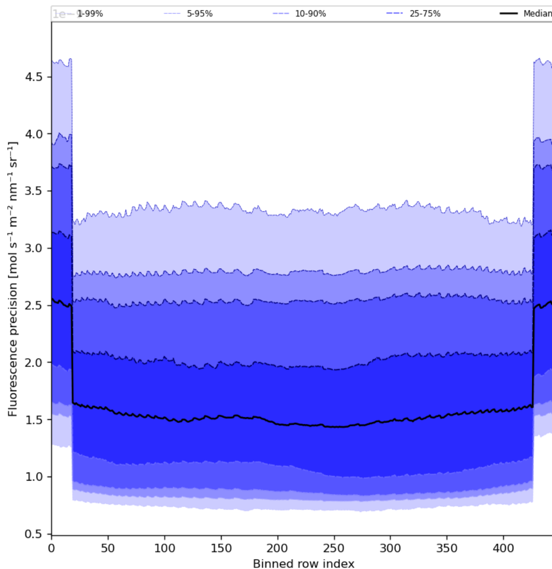
Figure 58: Along track statistics of “Fluorescence precision” for 2024-08-18 to 2024-08-20
