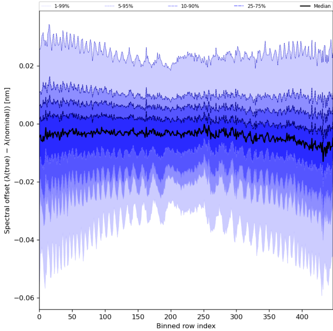
Figure 62: Along track statistics of “Spectral offset ( \lambda(\text{true}) - \lambda(\text{nominal}) )” for 2024-08-18 to 2024-08-20
