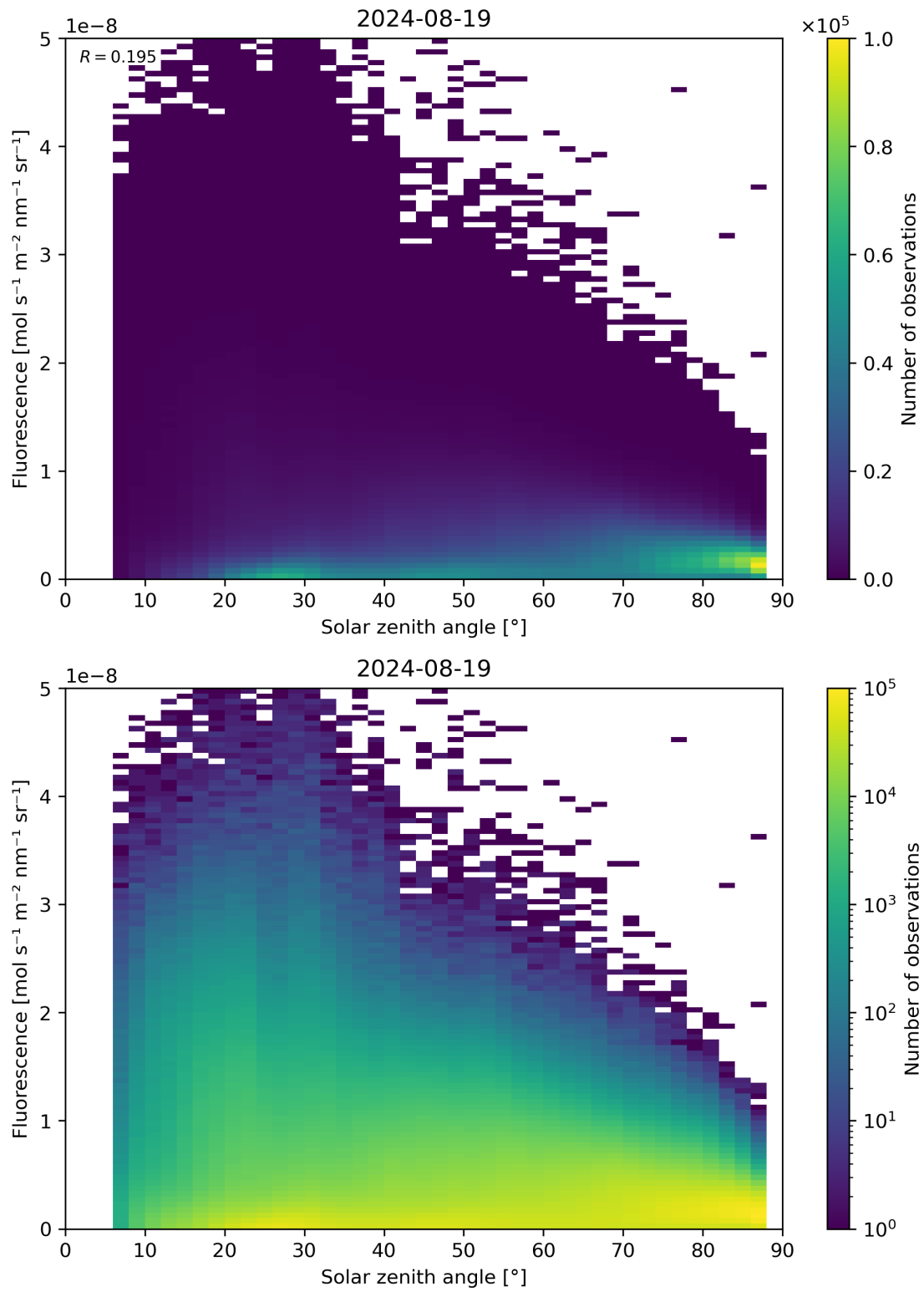
Figure 112: Scatter density plot of “Solar zenith angle” against “Fluorescence” for 2024-08-18 to 2024-08-20.
