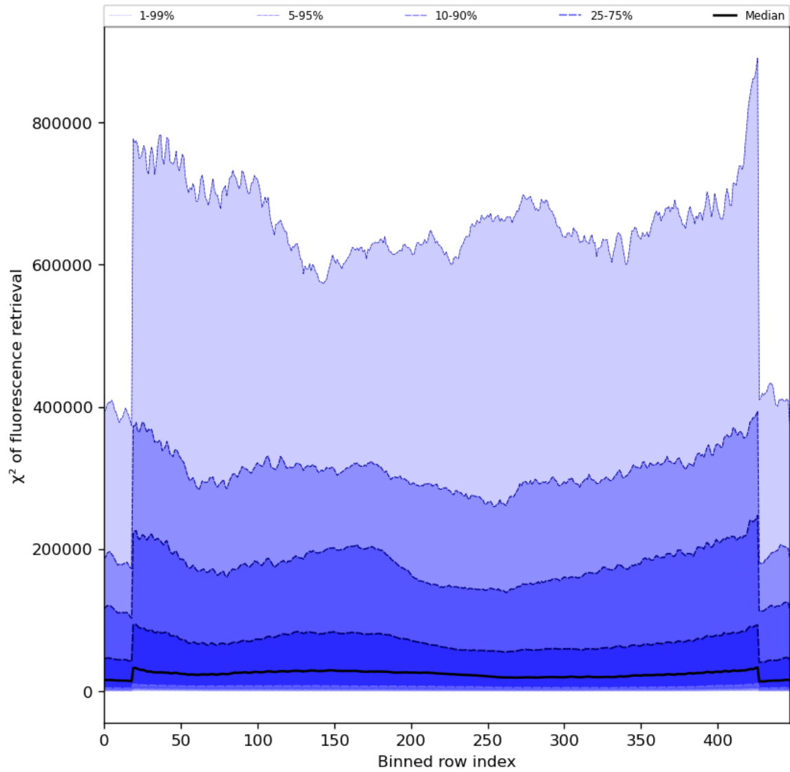
Figure 59: Along track statistics of “ \chi^2 of fluorescence retrieval” for 2024-08-18 to 2024-08-20
