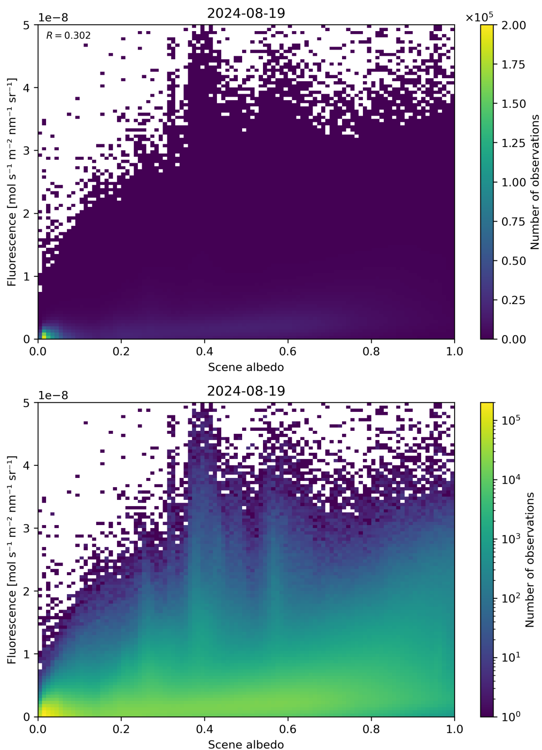
Figure 104: Scatter density plot of “Scene albedo” against “Fluorescence” for 2024-08-18 to 2024-08-20.
