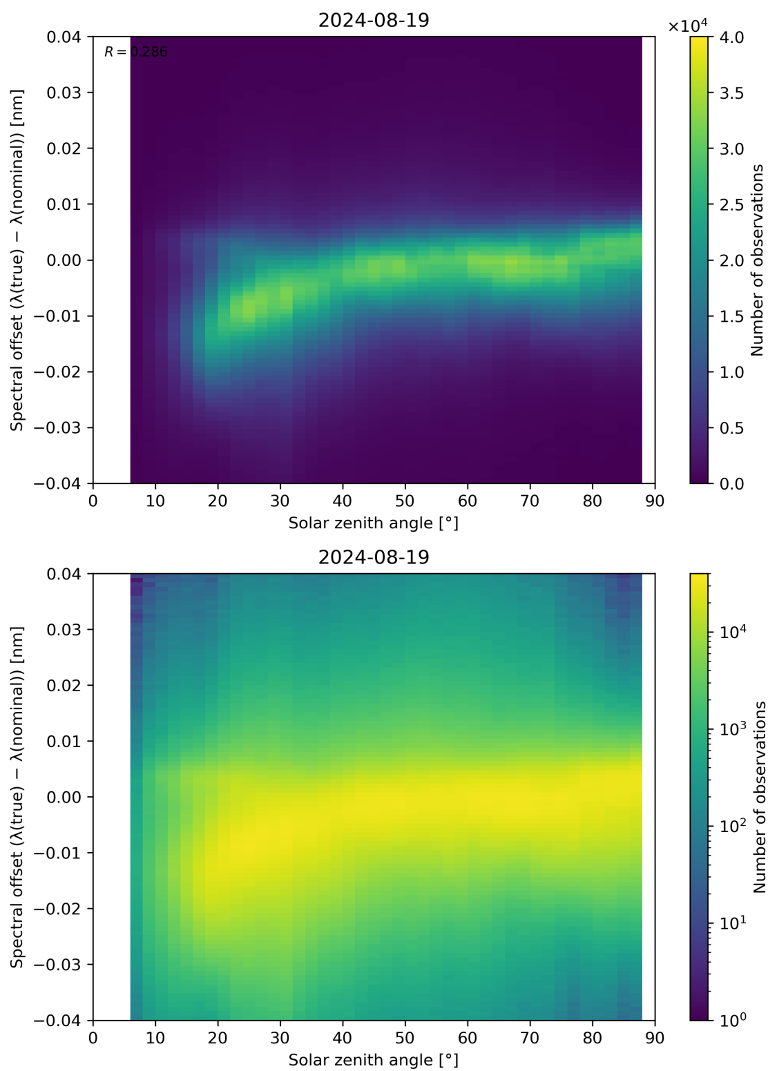
Figure 117: Scatter density plot of “Solar zenith angle” against “Spectral offset ( \lambda(\text{true}) - \lambda(\text{nominal}) )” for 2024-08-18 to 2024-08-20.
