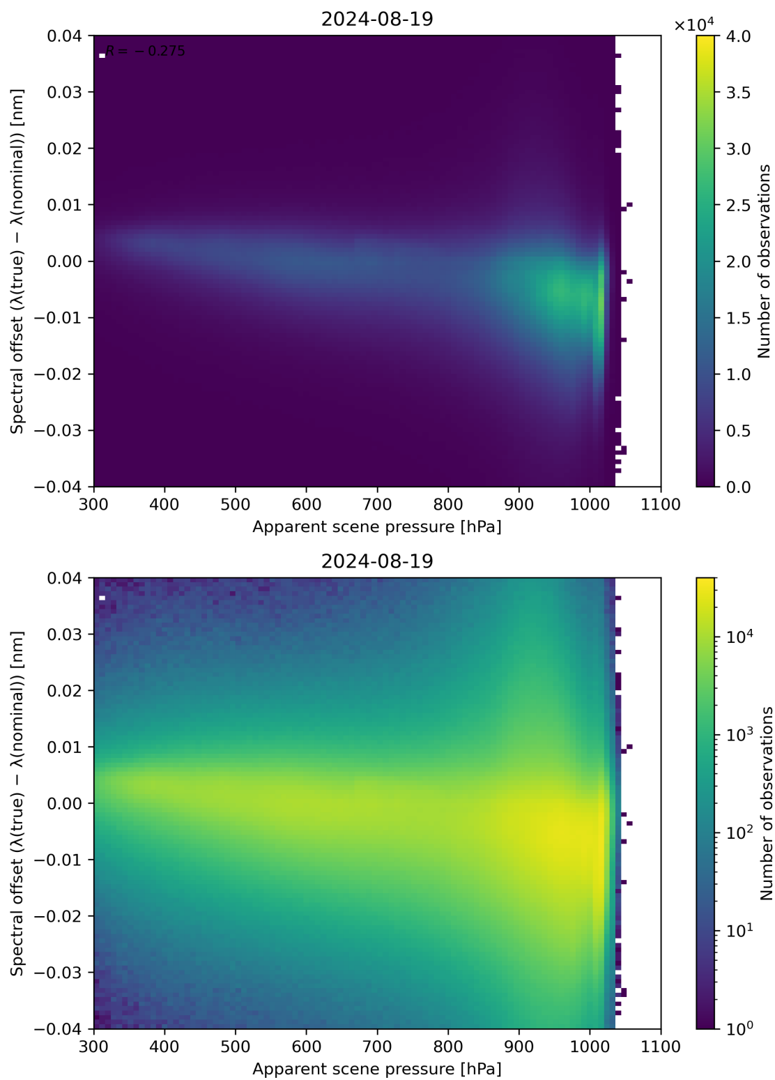
Figure 67: Scatter density plot of “Apparent scene pressure” against “Spectral offset ( \lambda(\text{true}) - \lambda(\text{nominal}) )” for 2024-08-18 to 2024-08-20.
