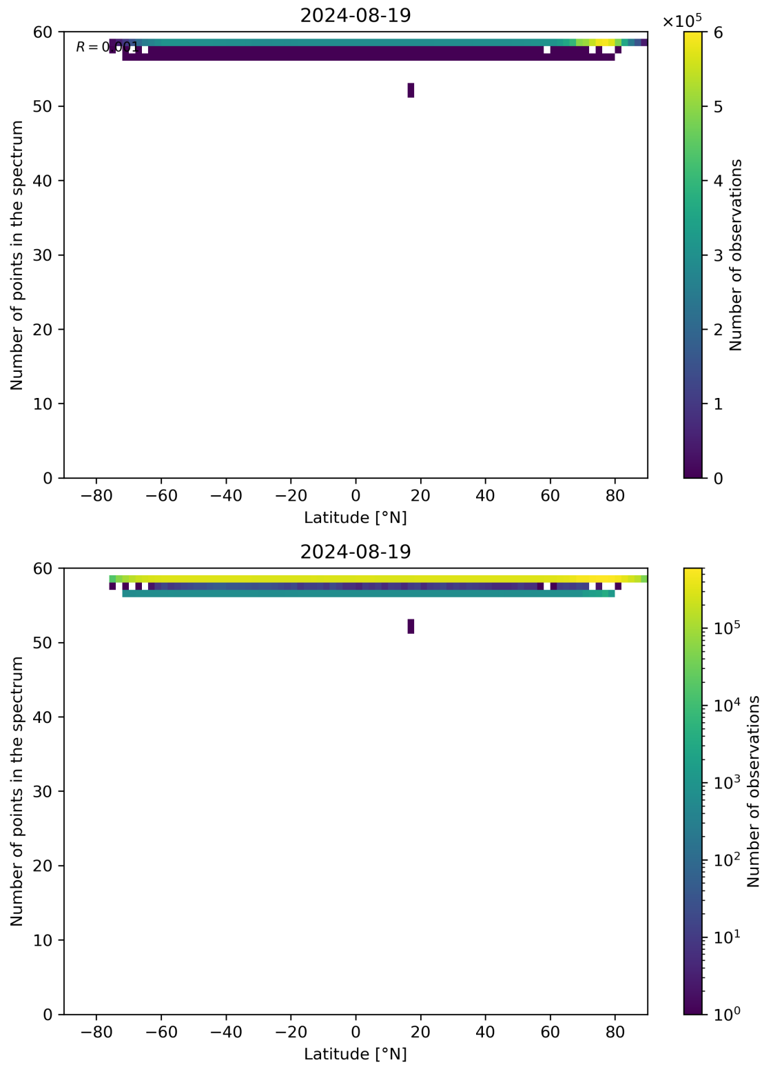
Figure 94: Scatter density plot of “Latitude” against “Number of points in the spectrum” for 2024-08-18 to 2024-08-20.
