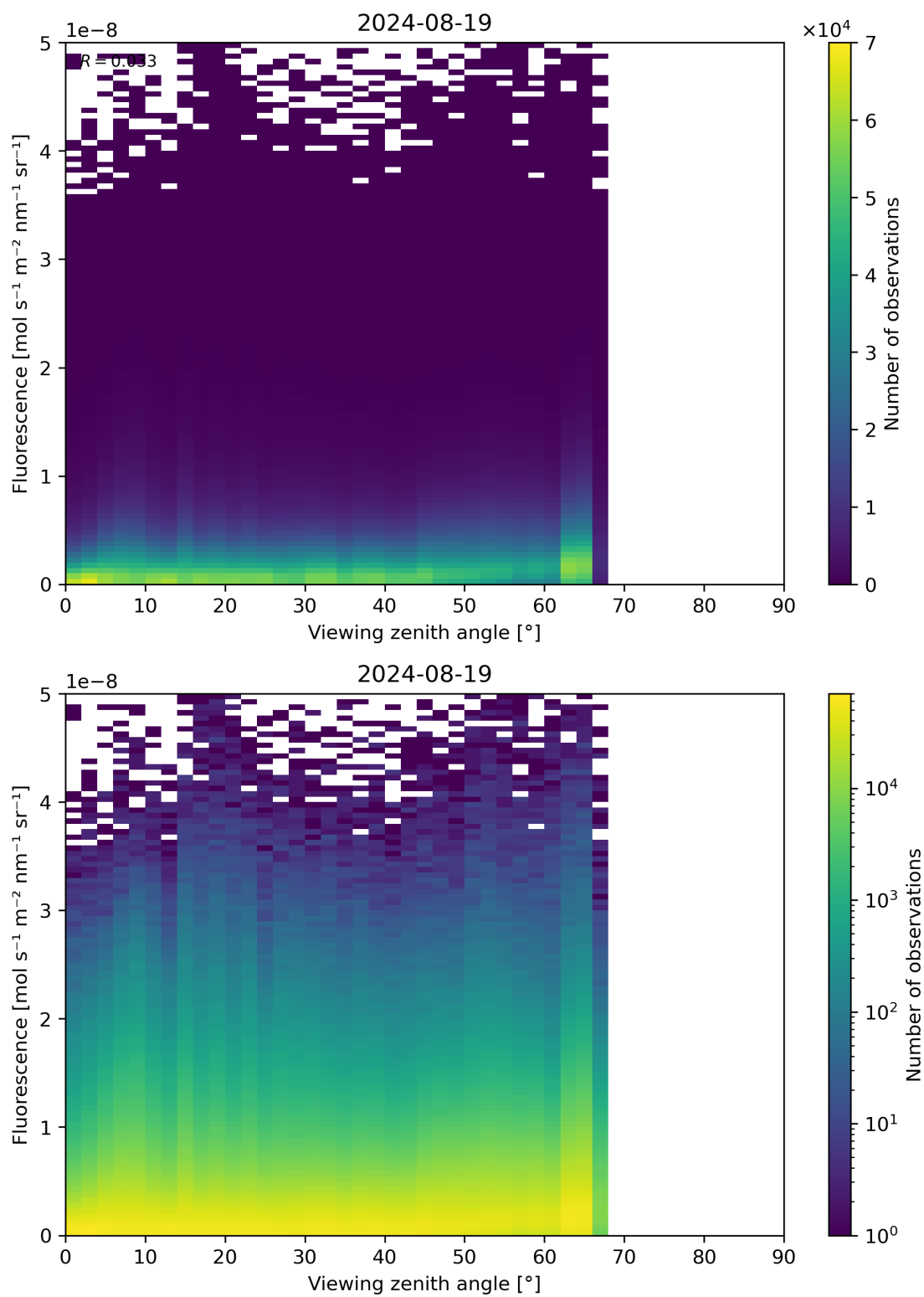
Figure 122: Scatter density plot of “Viewing zenith angle” against “Fluorescence” for 2024-08-18 to 2024-08-20.
