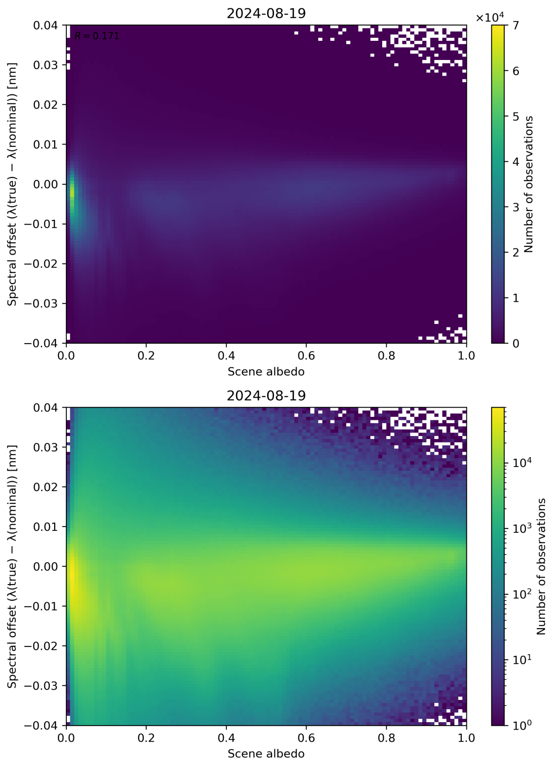
Figure 107: Scatter density plot of “Scene albedo” against “Spectral offset ( \lambda(\text{true}) - \lambda(\text{nominal}) )” for 2024-08-18 to 2024-08-20.
