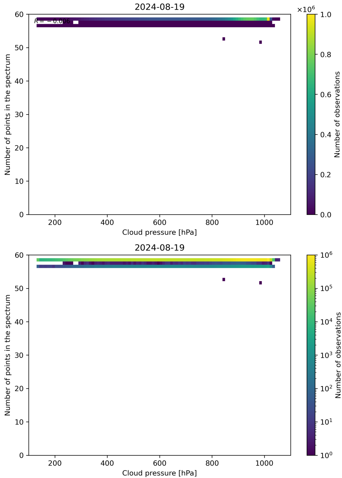
Figure 82: Scatter density plot of “Cloud pressure” against “Number of points in the spectrum” for 2024-08-18 to 2024-08-20.
