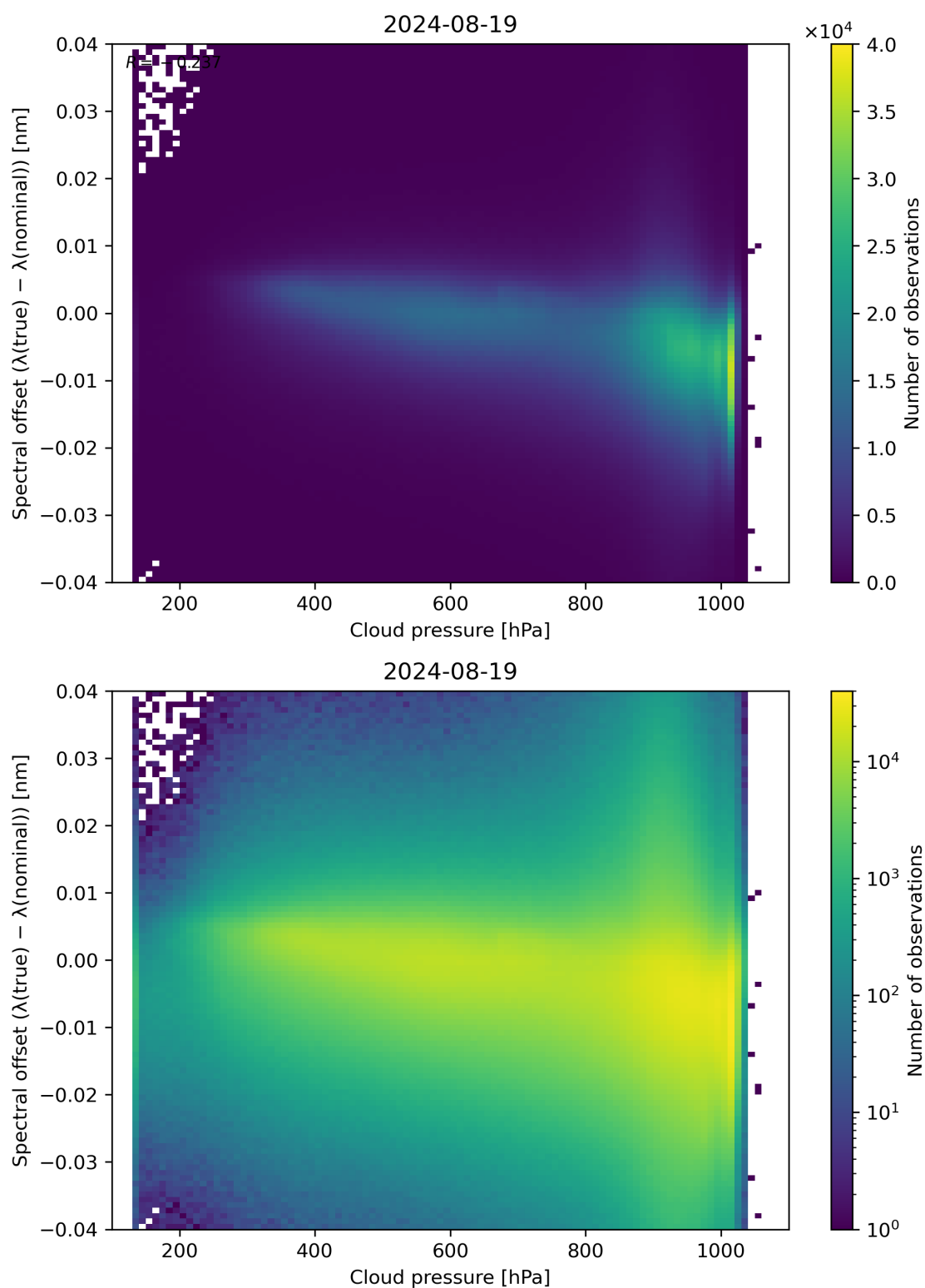
Figure 84: Scatter density plot of “Cloud pressure” against “Spectral offset ( \lambda(\text{true}) - \lambda(\text{nominal}) )” for 2024-08-18 to 2024-08-20.
