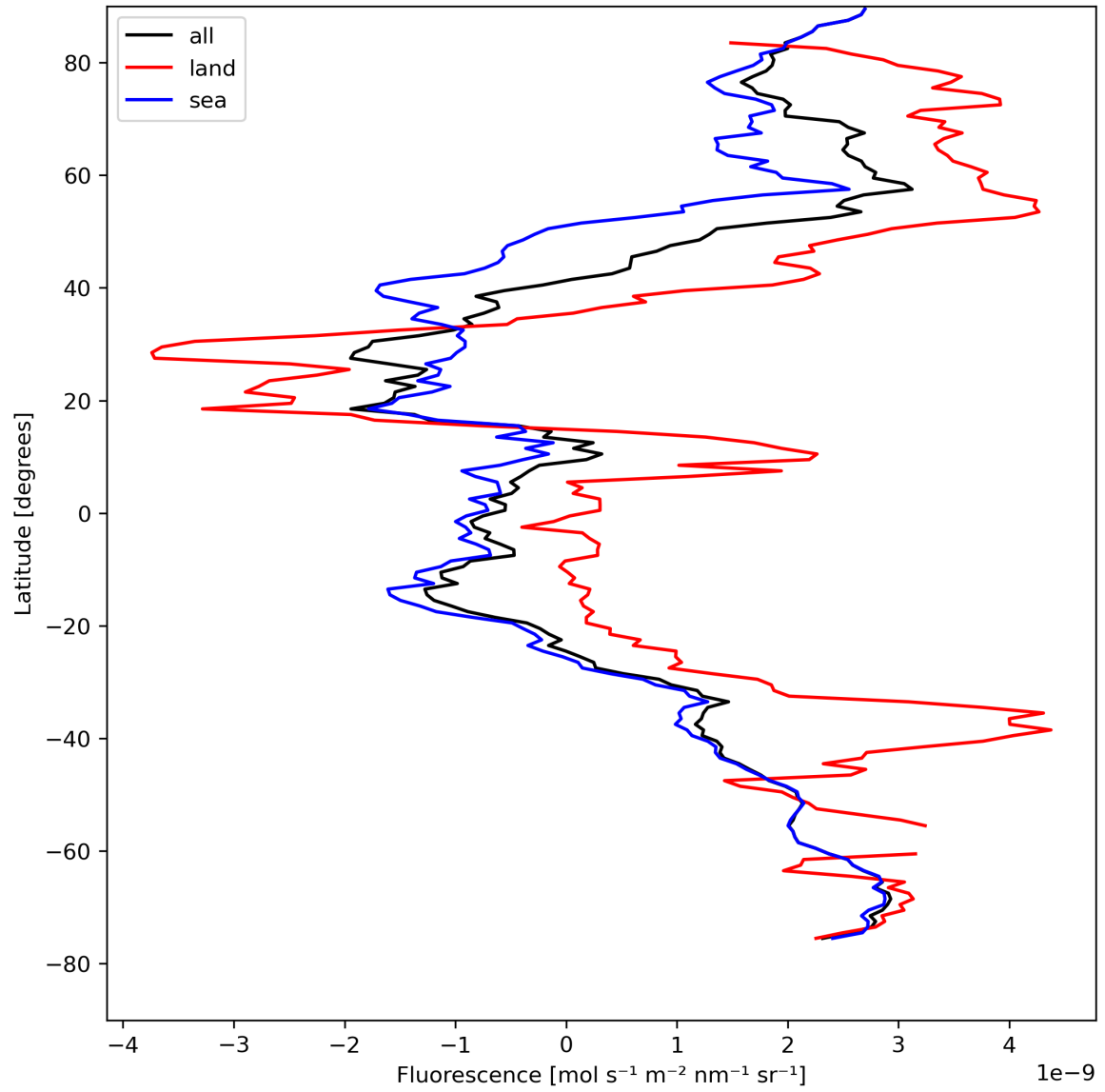
Figure 23: Zonal average of “Fluorescence” for 2024-08-18 to 2024-08-20.
