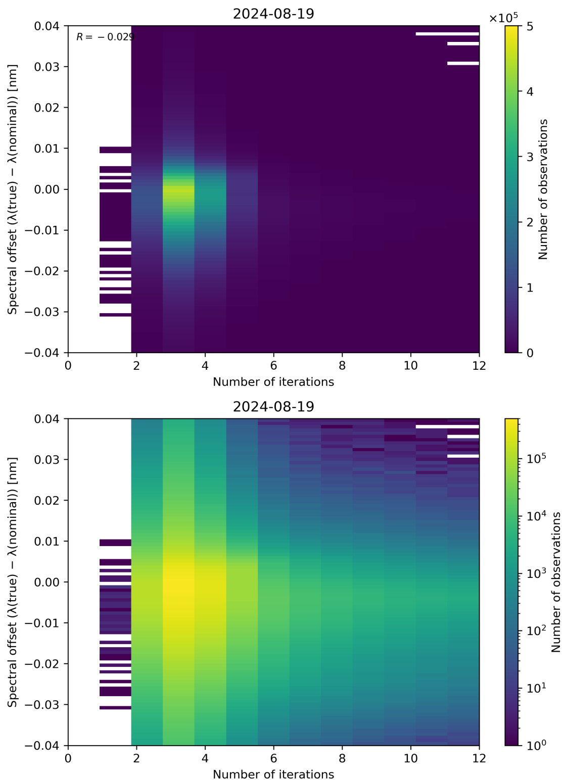
Figure 100: Scatter density plot of “Number of iterations” against “Spectral offset ( \lambda(\text{true}) - \lambda(\text{nominal}) )” for 2024-08-18 to 2024-08-20.
