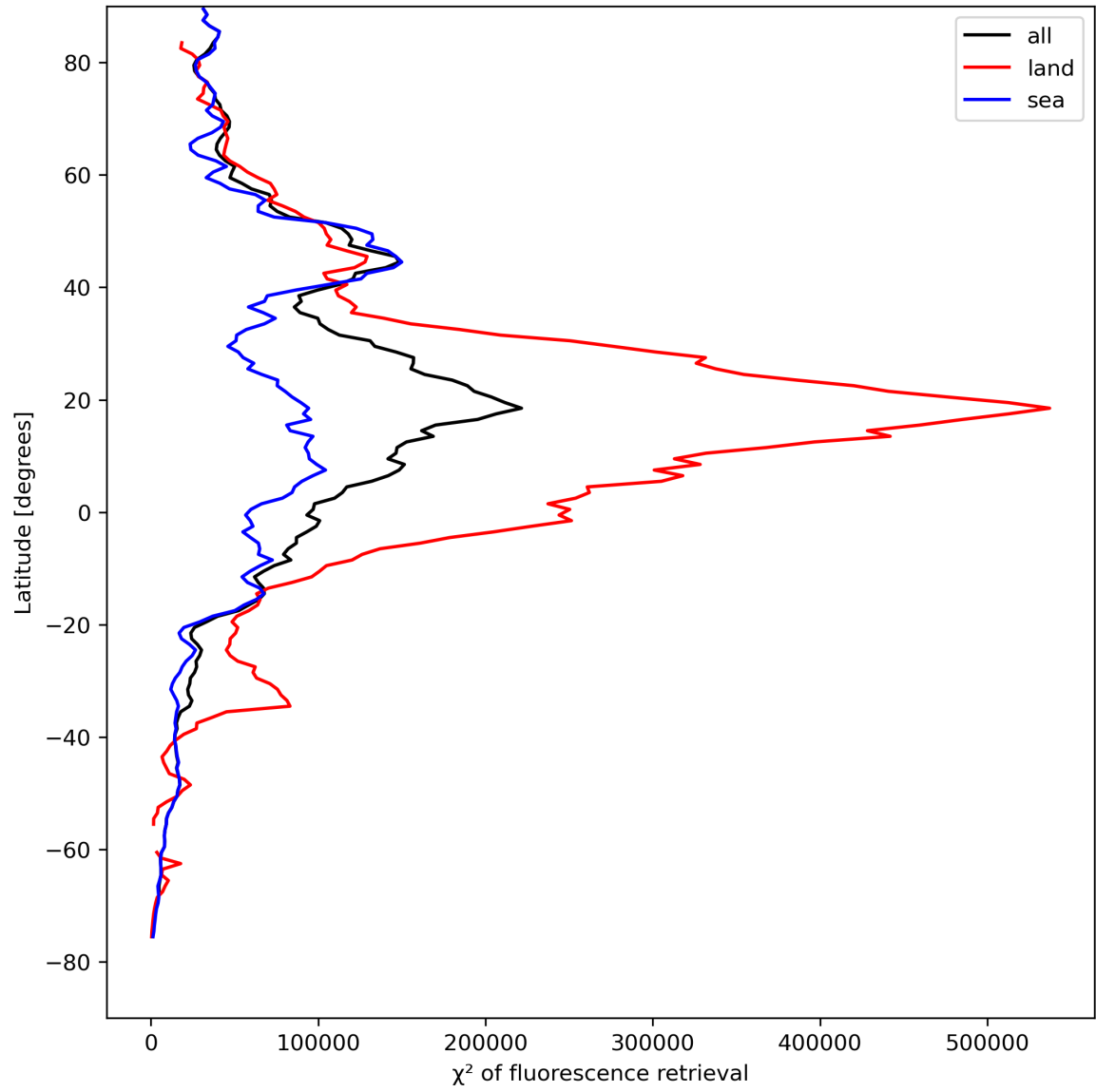
Figure 25: Zonal average of “ \chi^2 of fluorescence retrieval” for 2024-08-18 to 2024-08-20.
