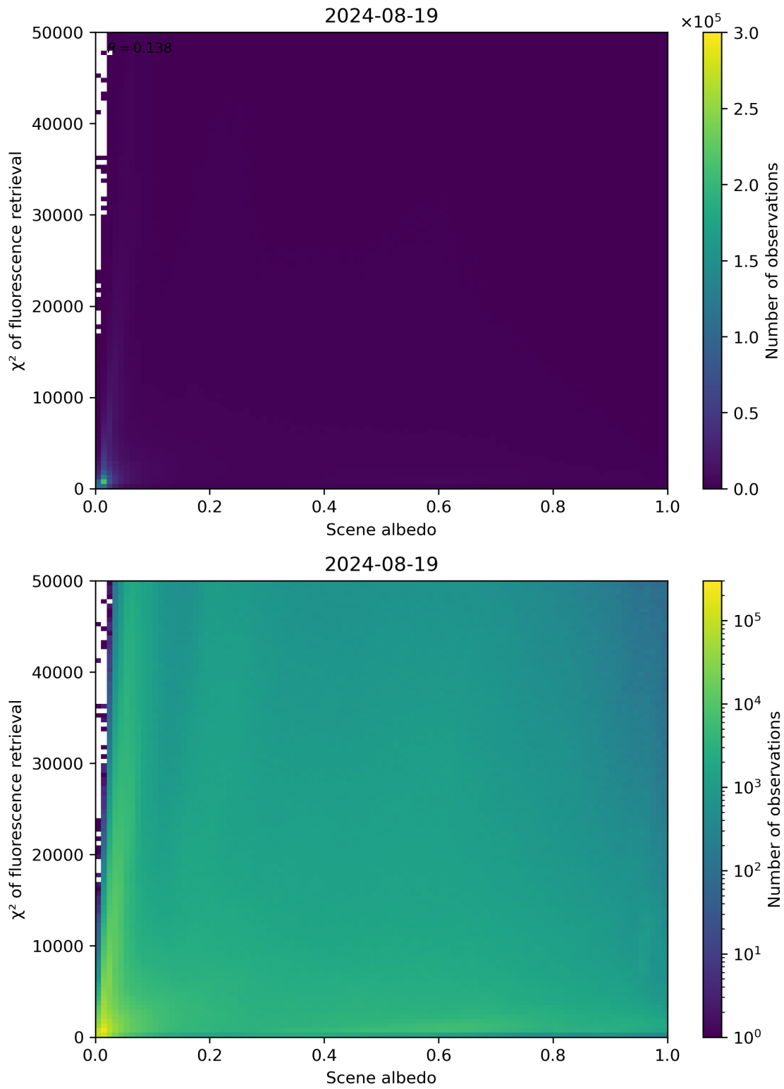
Figure 103: Scatter density plot of “Scene albedo” against “ \chi^2 of fluorescence retrieval” for 2024-08-18 to 2024-08-20.
