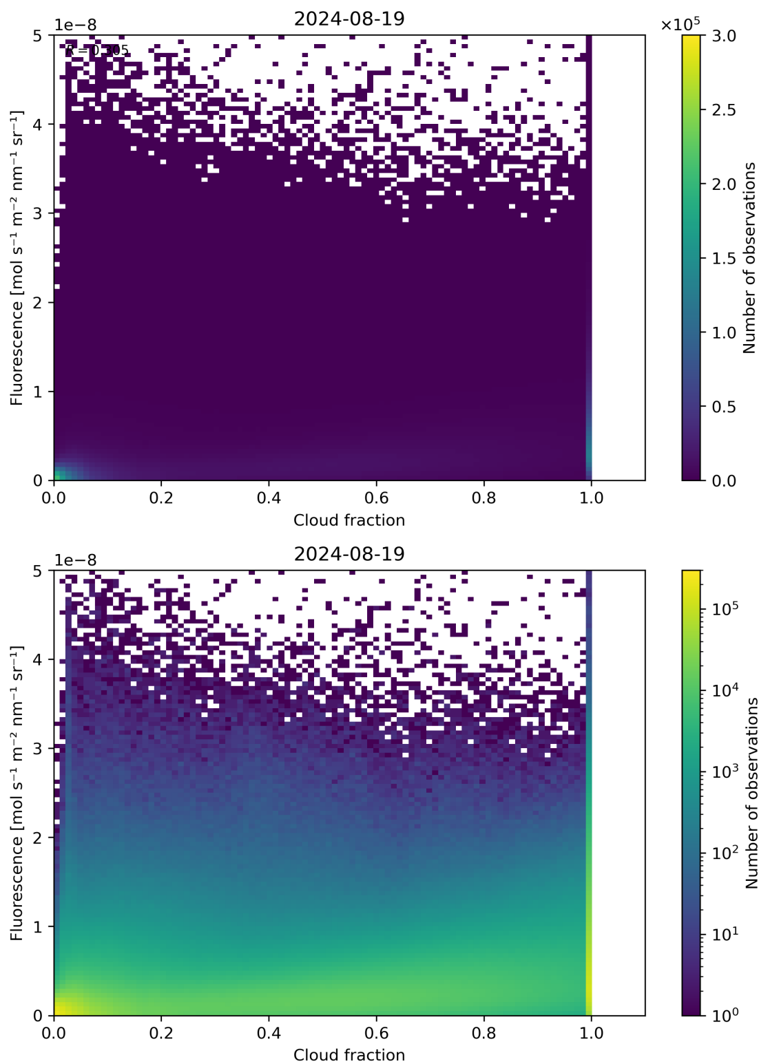
Figure 72: Scatter density plot of “Cloud fraction” against “Fluorescence” for 2024-08-18 to 2024-08-20.
