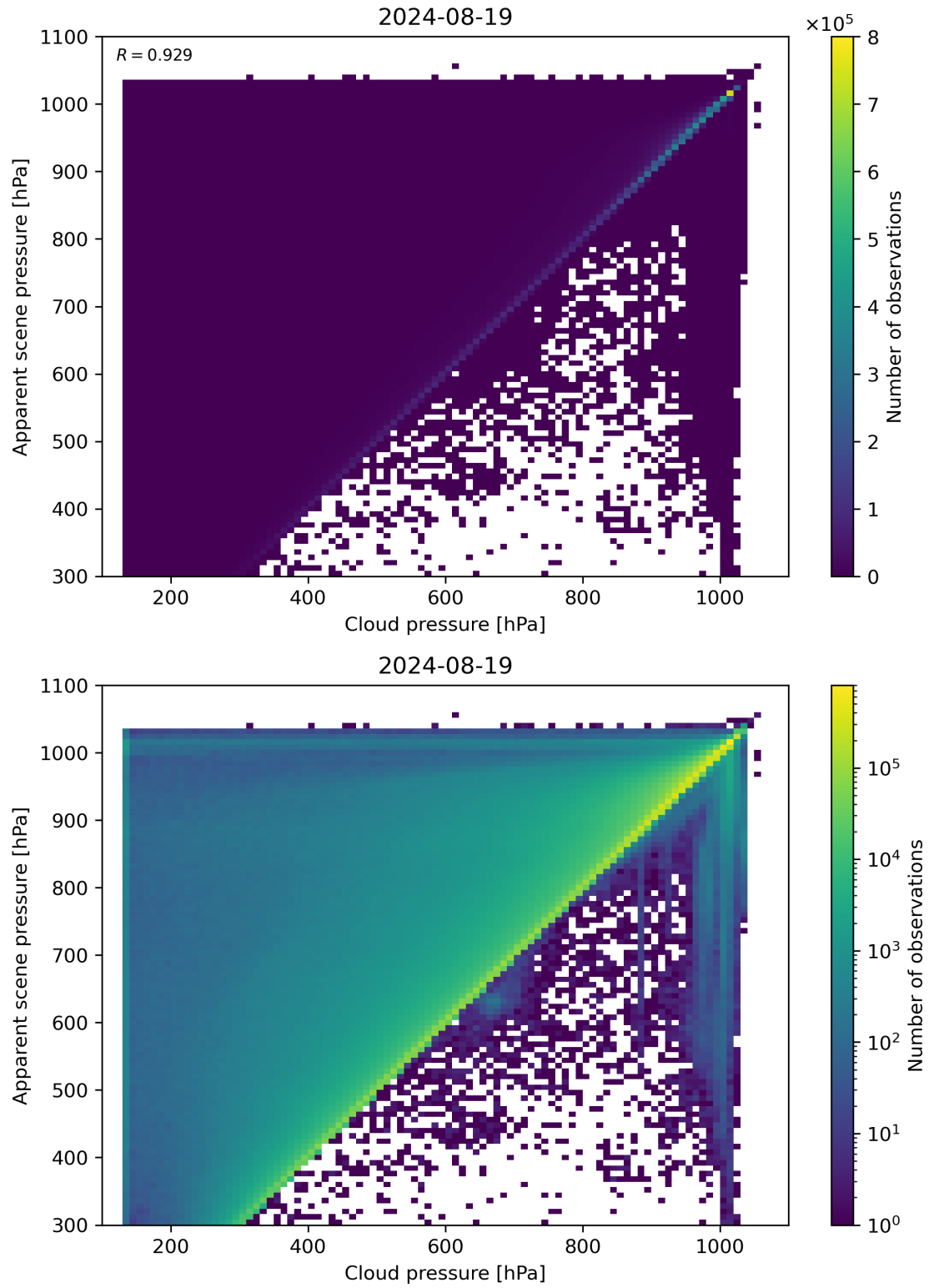
Figure 77: Scatter density plot of “Cloud pressure” against “Apparent scene pressure” for 2024-08-18 to 2024-08-20.
