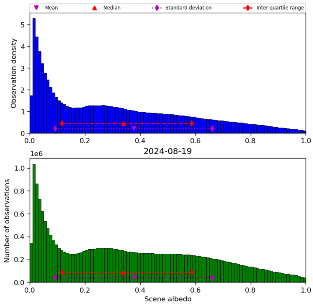
Figure 34: Histogram of “Scene albedo” for 2024-08-18 to 2024-08-20
