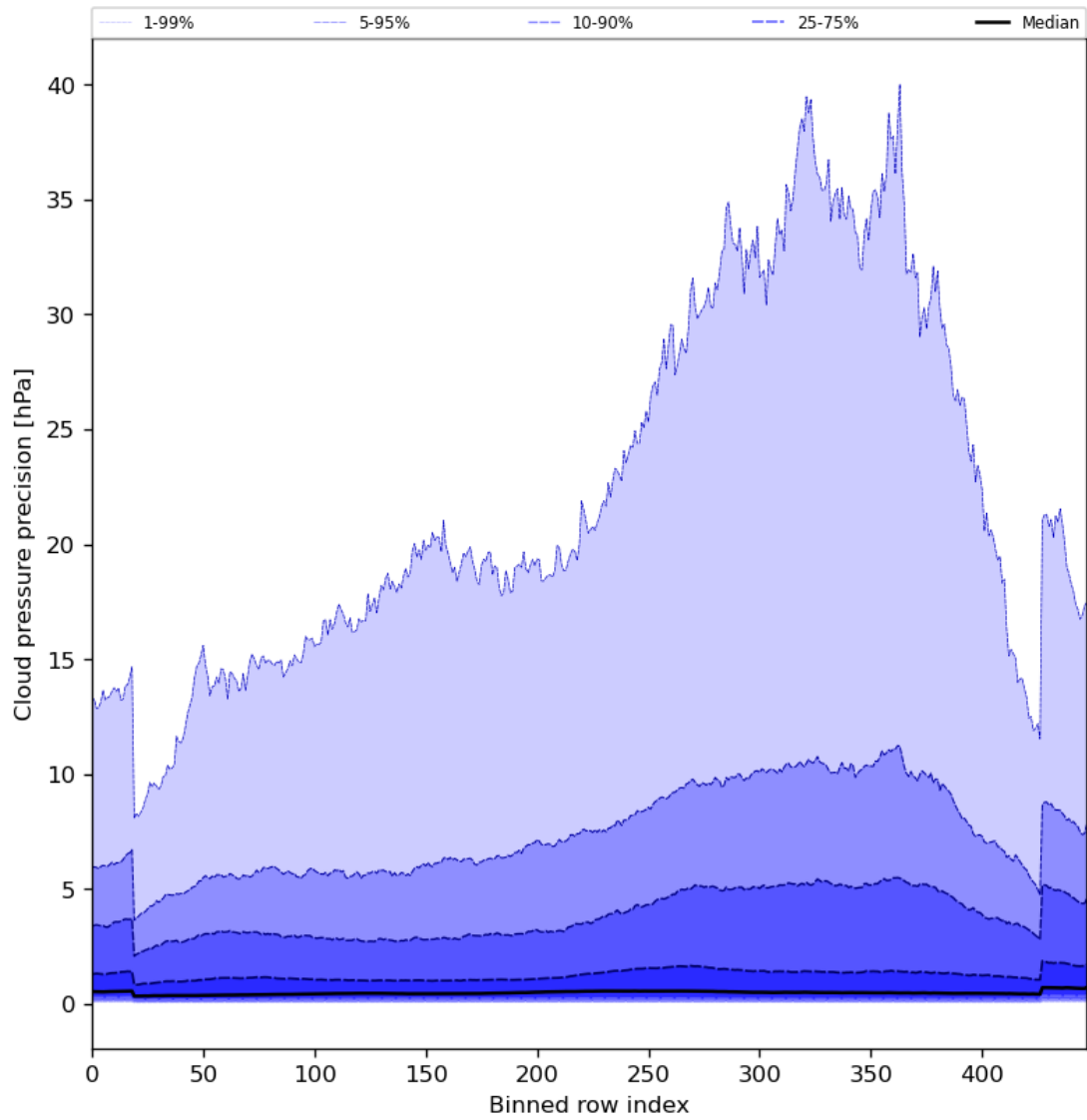
Figure 48: Along track statistics of “Cloud pressure precision” for 2024-08-18 to 2024-08-20
