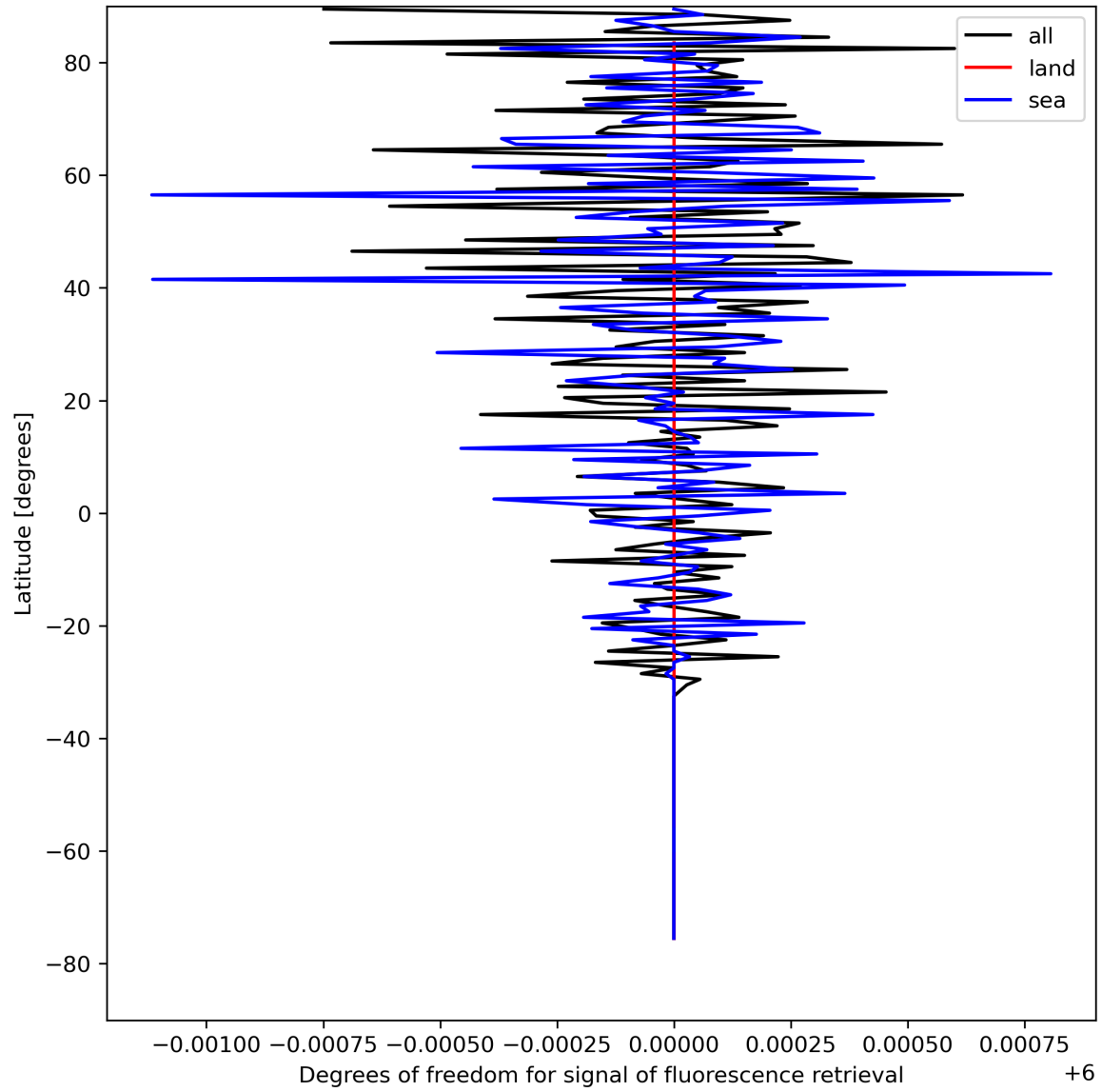
Figure 26: Zonal average of “Degrees of freedom for signal of fluorescence retrieval” for 2024-08-18 to 2024-08-20.
