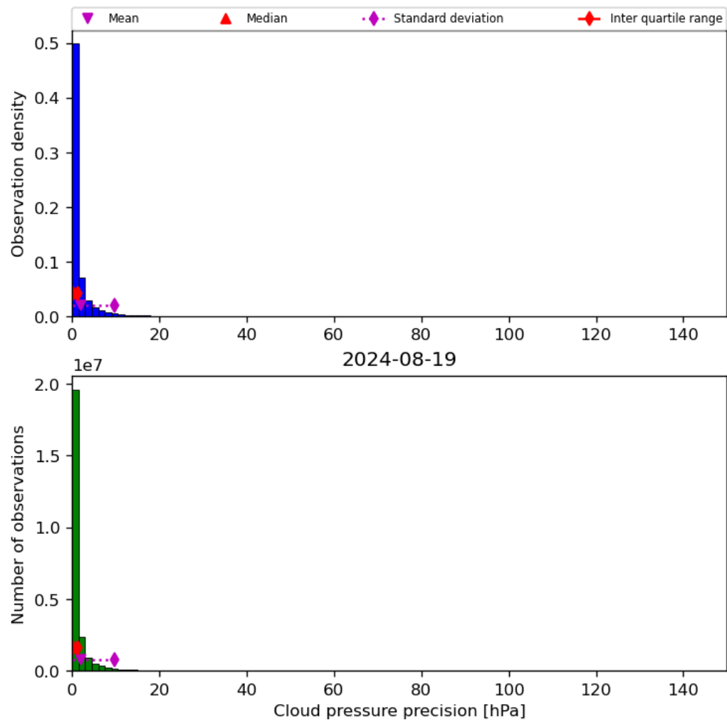
Figure 31: Histogram of “Cloud pressure precision” for 2024-08-18 to 2024-08-20
