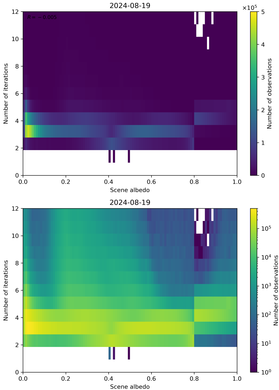
Figure 105: Scatter density plot of “Scene albedo” against “Number of iterations” for 2024-08-18 to 2024-08-20.
