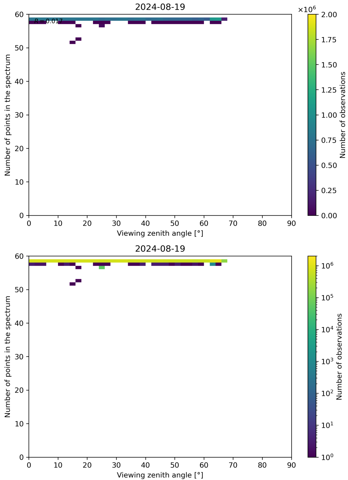
Figure 125: Scatter density plot of “Viewing zenith angle” against “Number of points in the spectrum” for 2024-08-18 to 2024-08-20.
