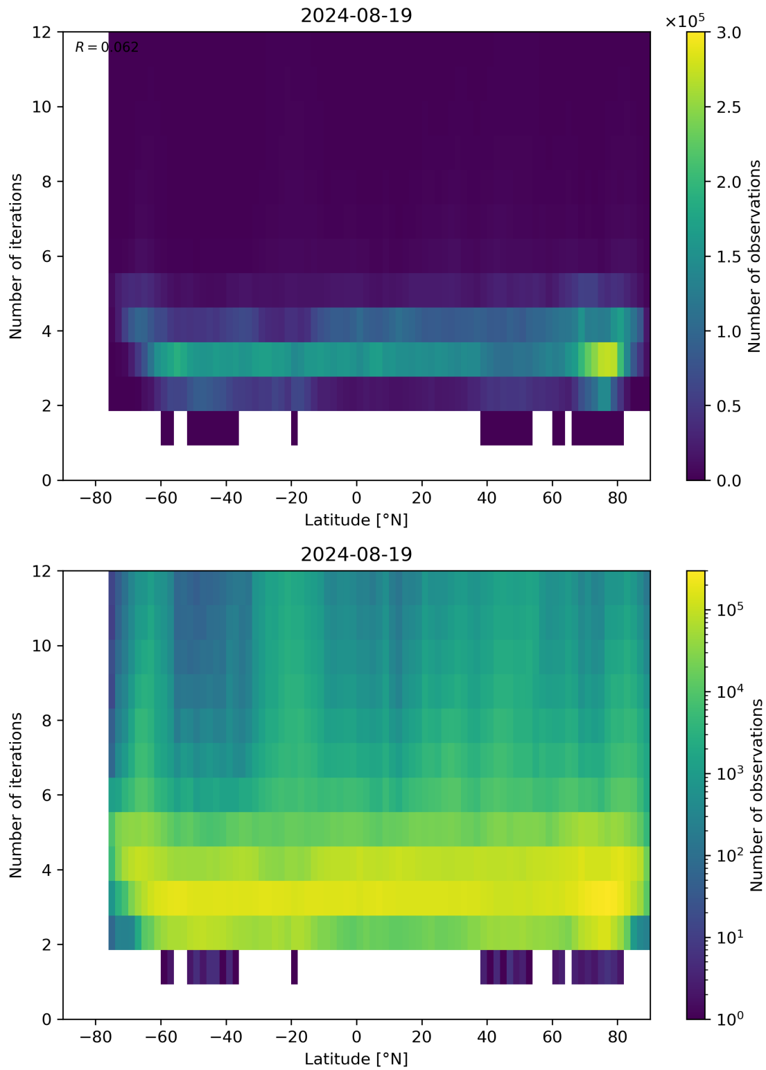
Figure 93: Scatter density plot of “Latitude” against “Number of iterations” for 2024-08-18 to 2024-08-20.
