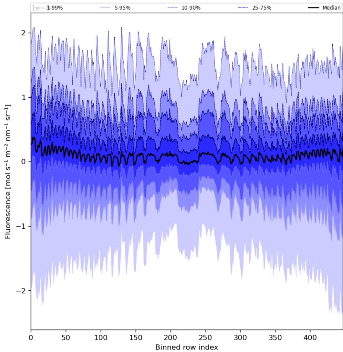
Figure 57: Along track statistics of “Fluorescence” for 2024-08-18 to 2024-08-20
