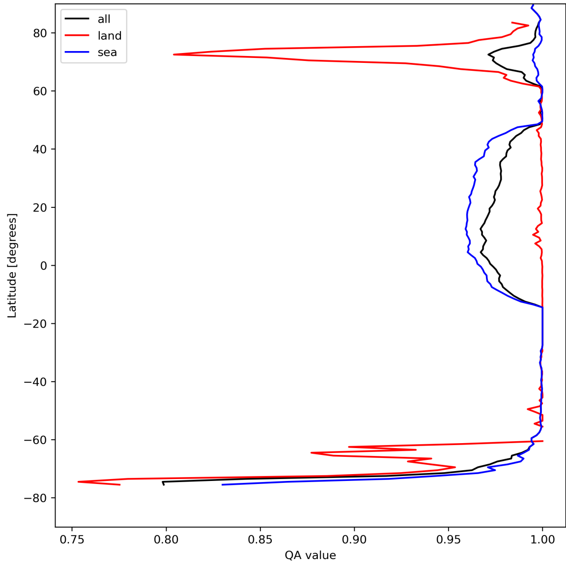
Figure 12: Zonal average of “QA value” for 2024-08-18 to 2024-08-20.
