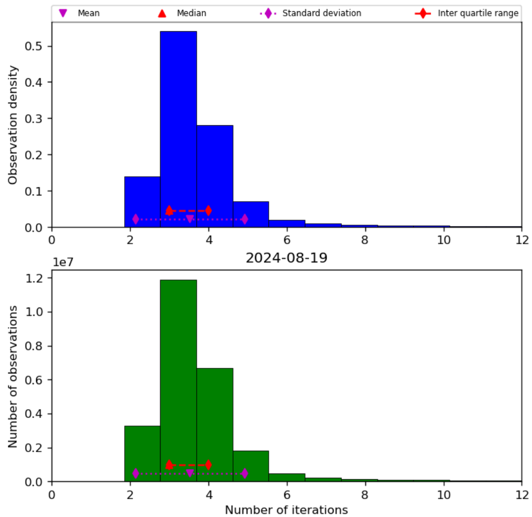
Figure 39: Histogram of “Number of iterations” for 2024-08-18 to 2024-08-20
