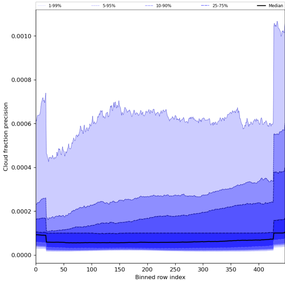
Figure 50: Along track statistics of “Cloud fraction precision” for 2024-08-18 to 2024-08-20
