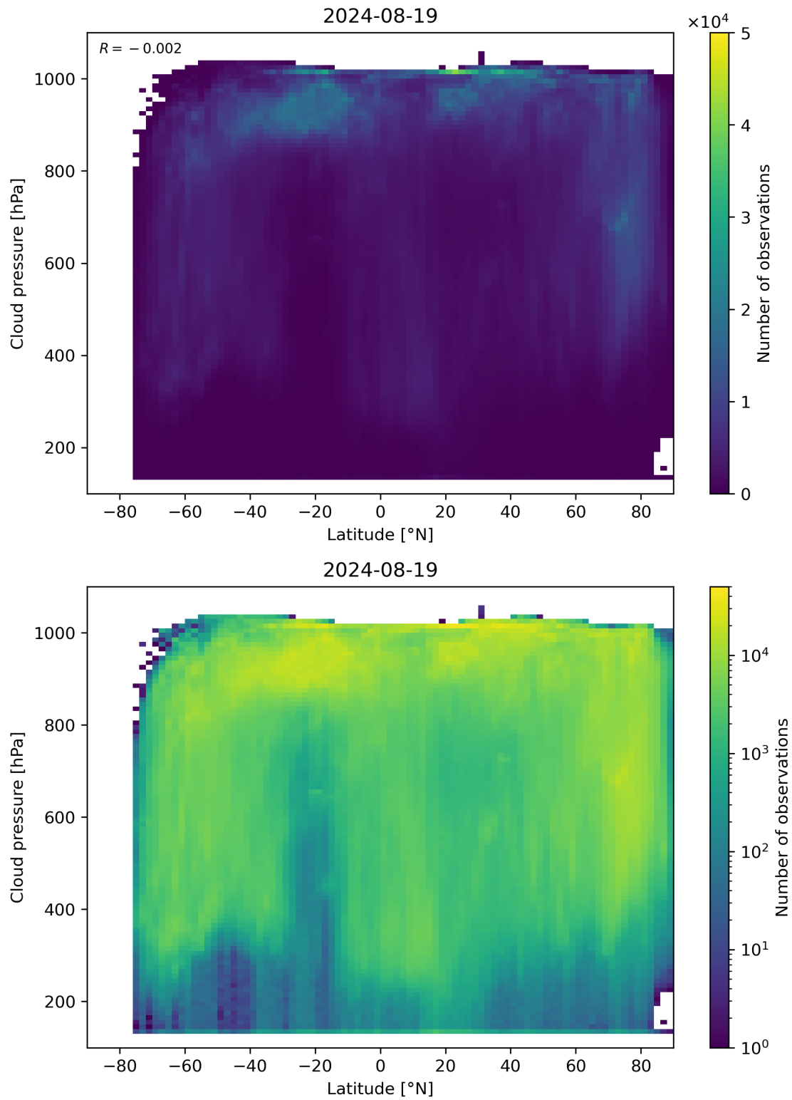
Figure 91: Scatter density plot of “Latitude” against “Cloud pressure” for 2024-08-18 to 2024-08-20.
