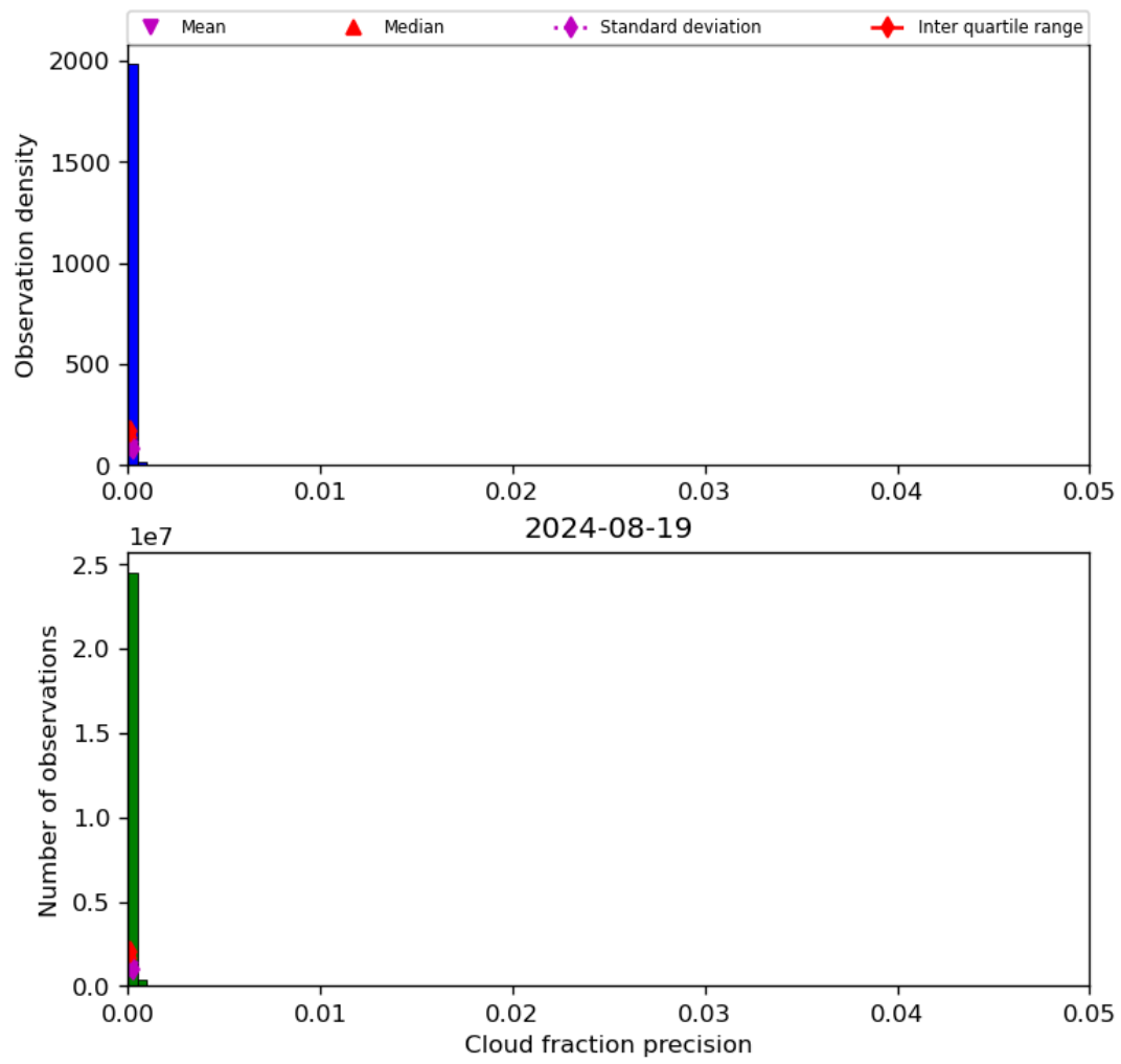
Figure 33: Histogram of “Cloud fraction precision” for 2024-08-18 to 2024-08-20
