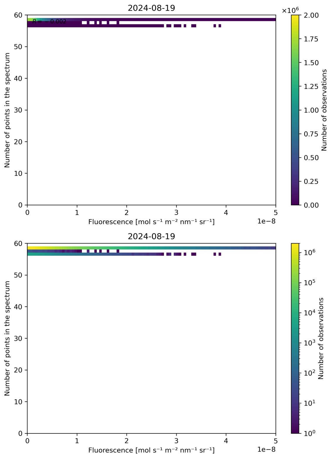
Figure 86: Scatter density plot of “Fluorescence” against “Number of points in the spectrum” for 2024-08-18 to 2024-08-20.
