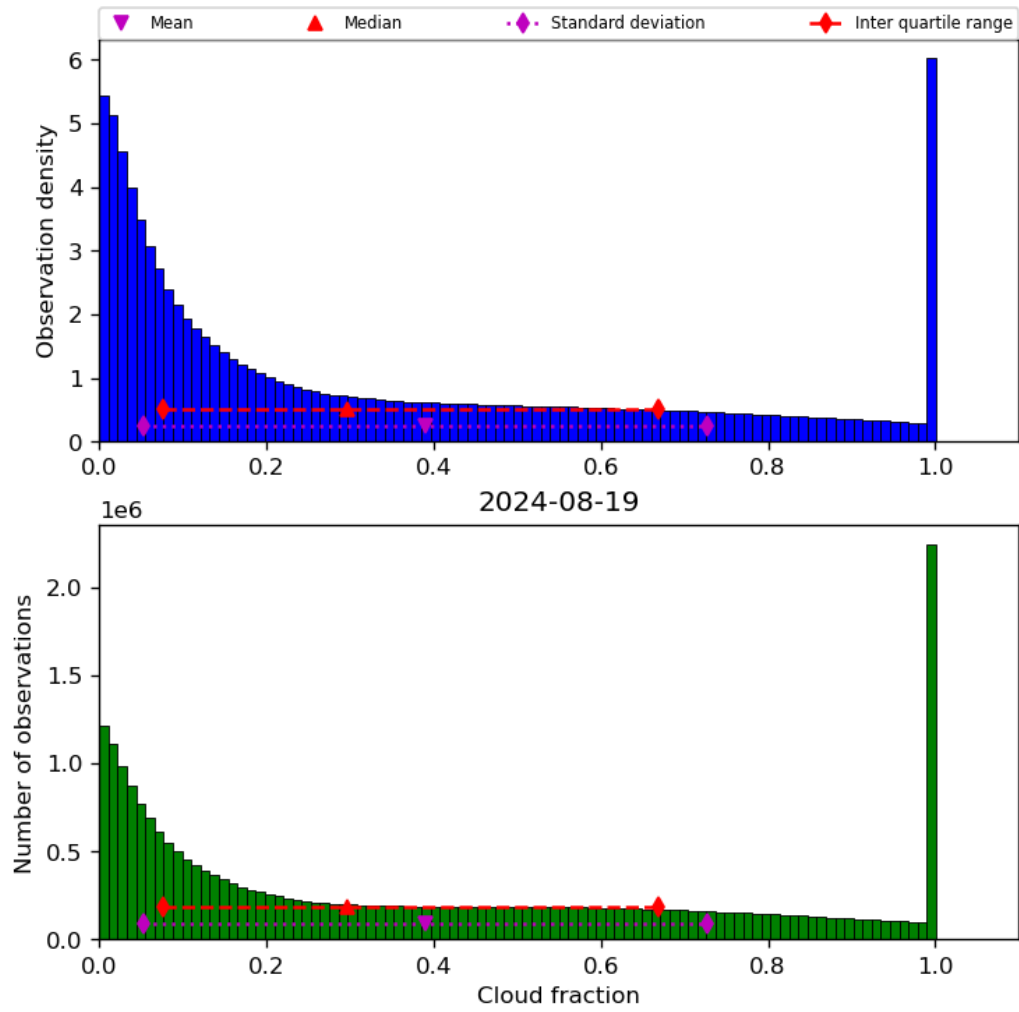
Figure 32: Histogram of “Cloud fraction” for 2024-08-18 to 2024-08-20
