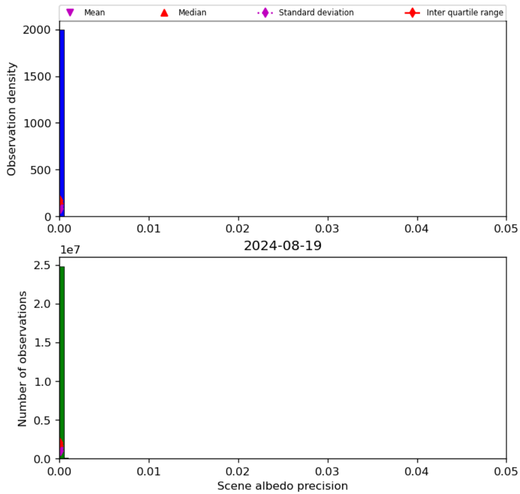
Figure 35: Histogram of “Scene albedo precision” for 2024-08-18 to 2024-08-20
