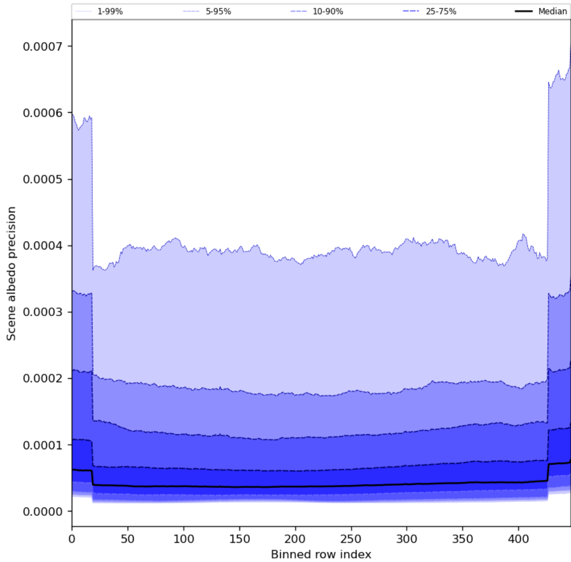
Figure 52: Along track statistics of “Scene albedo precision” for 2024-08-18 to 2024-08-20
