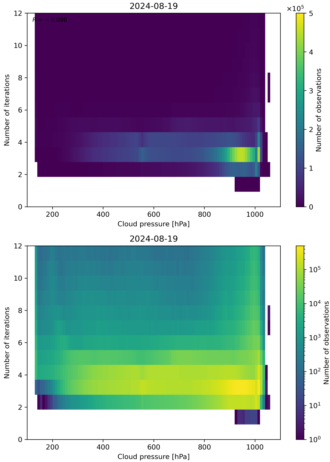
Figure 81: Scatter density plot of “Cloud pressure” against “Number of iterations” for 2024-08-18 to 2024-08-20.
