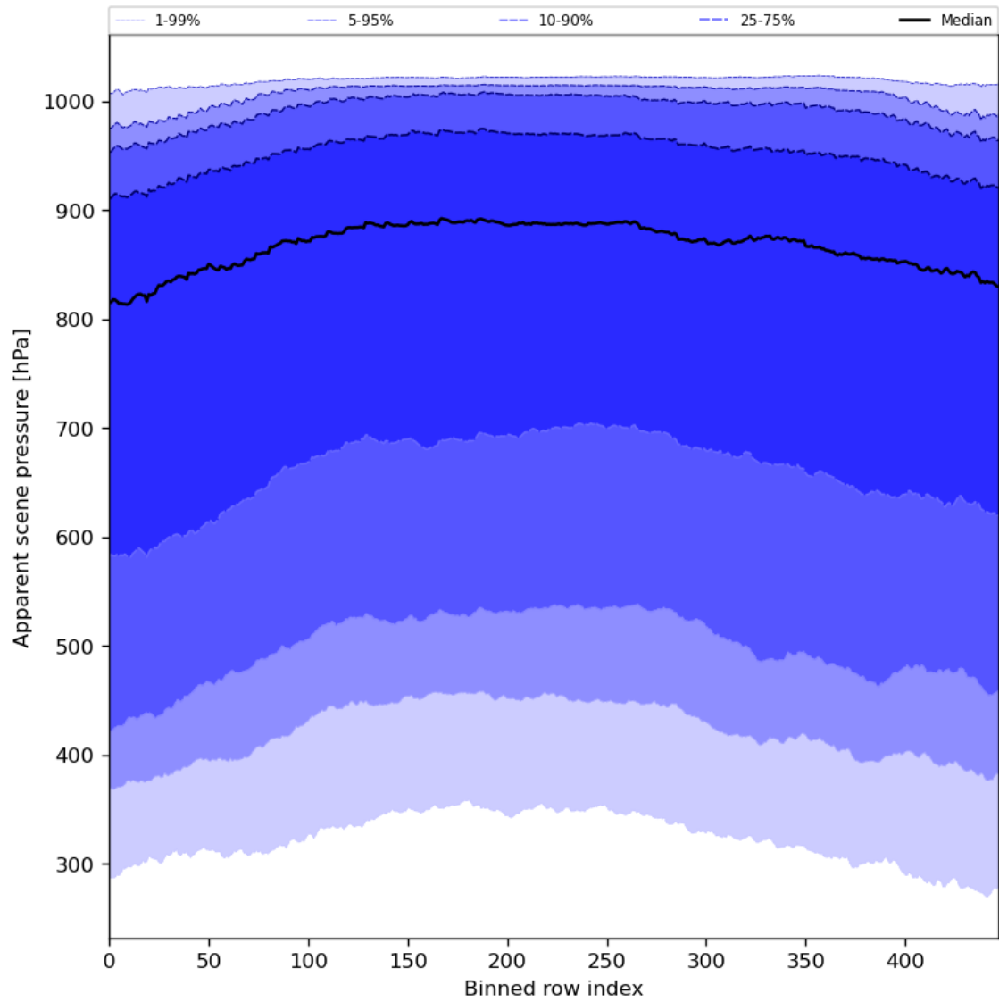
Figure 53: Along track statistics of “Apparent scene pressure” for 2024-08-18 to 2024-08-20
