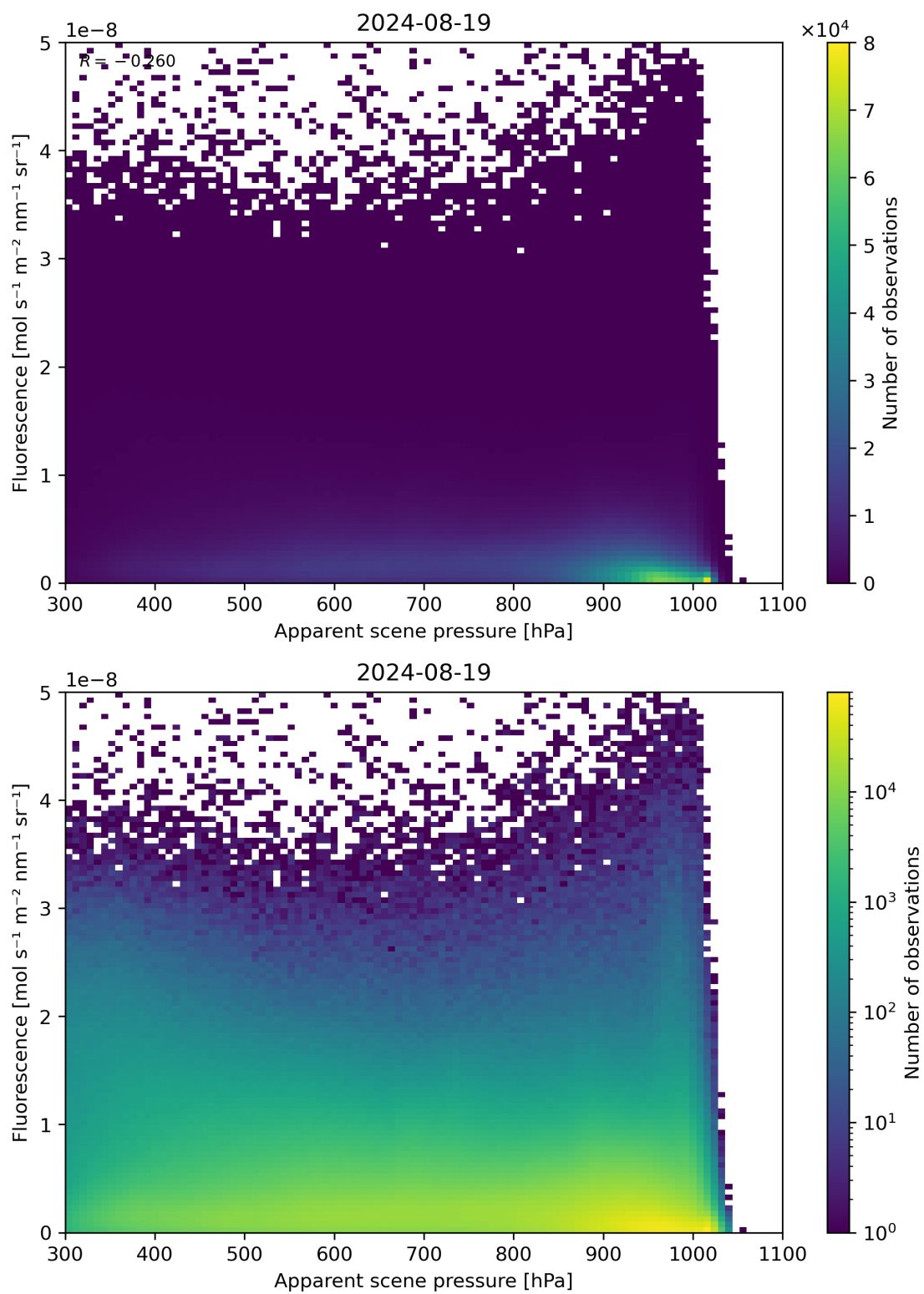
Figure 64: Scatter density plot of “Apparent scene pressure” against “Fluorescence” for 2024-08-18 to 2024-08-20.
