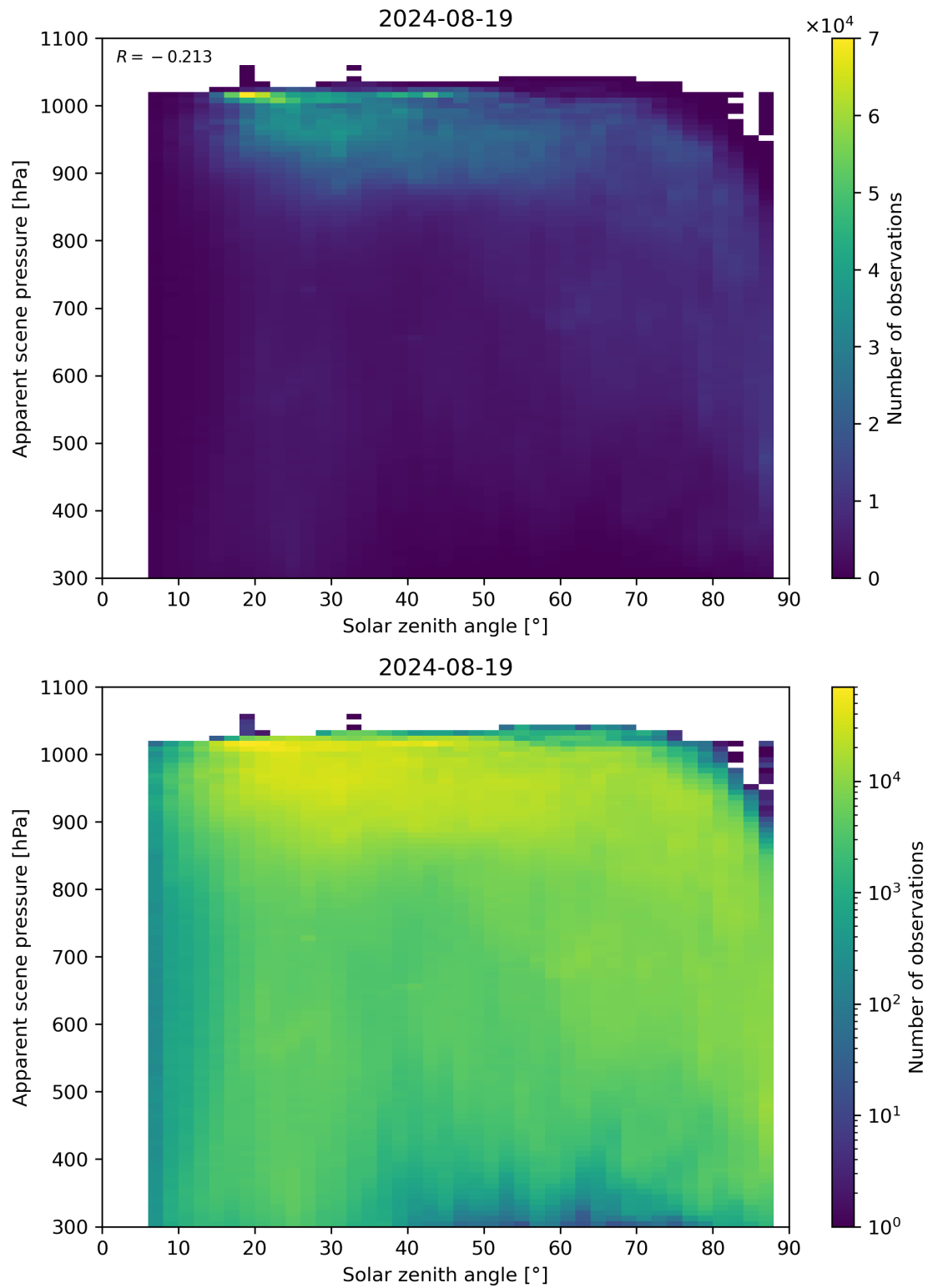
Figure 108: Scatter density plot of “Solar zenith angle” against “Apparent scene pressure” for 2024-08-18 to 2024-08-20.
