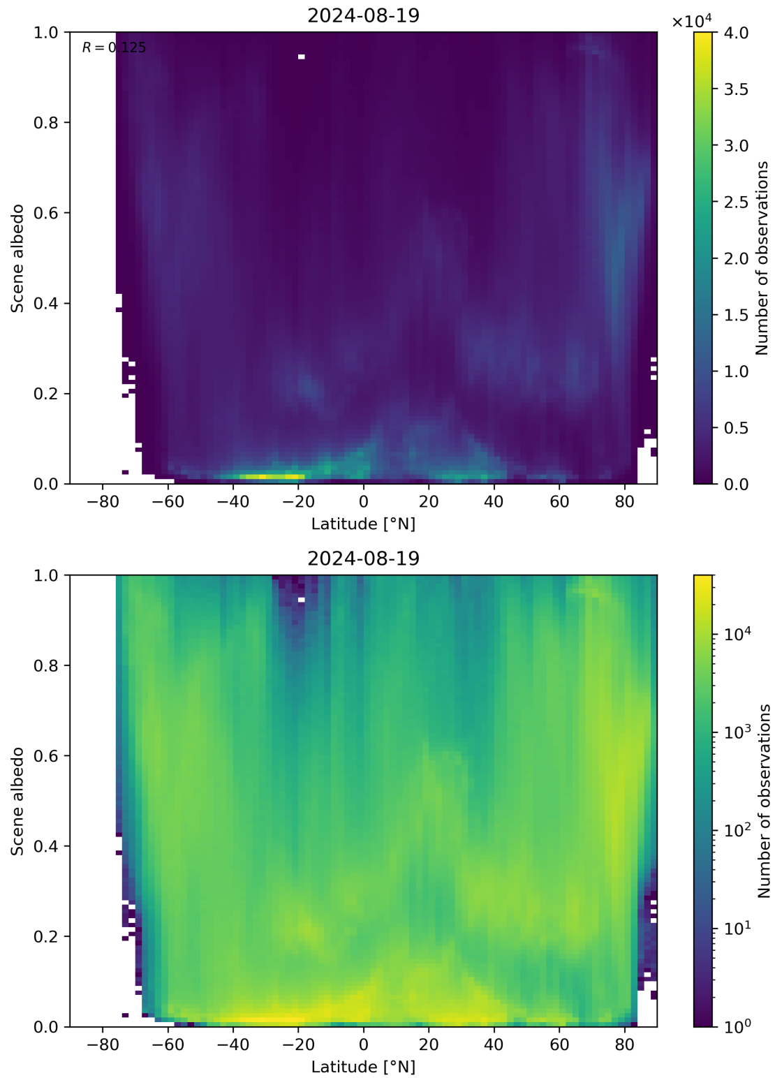
Figure 95: Scatter density plot of “Latitude” against “Scene albedo” for 2024-08-18 to 2024-08-20.
