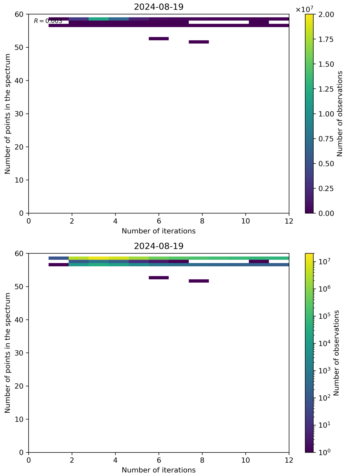
Figure 99: Scatter density plot of “Number of iterations” against “Number of points in the spectrum” for 2024-08-18 to 2024-08-20.
