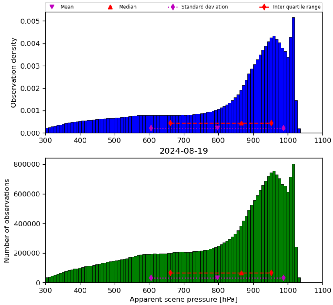
Figure 36: Histogram of “Apparent scene pressure” for 2024-08-18 to 2024-08-20
