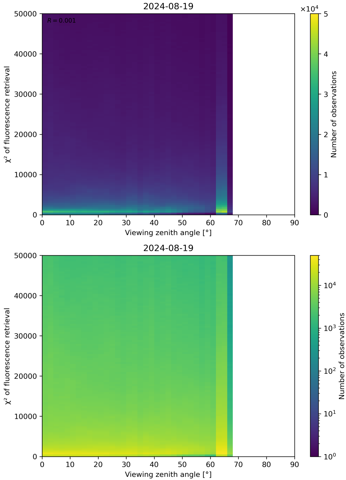
Figure 119: Scatter density plot of “Viewing zenith angle” against “ \chi^2 of fluorescence retrieval” for 2024-08-18 to 2024-08-20.
