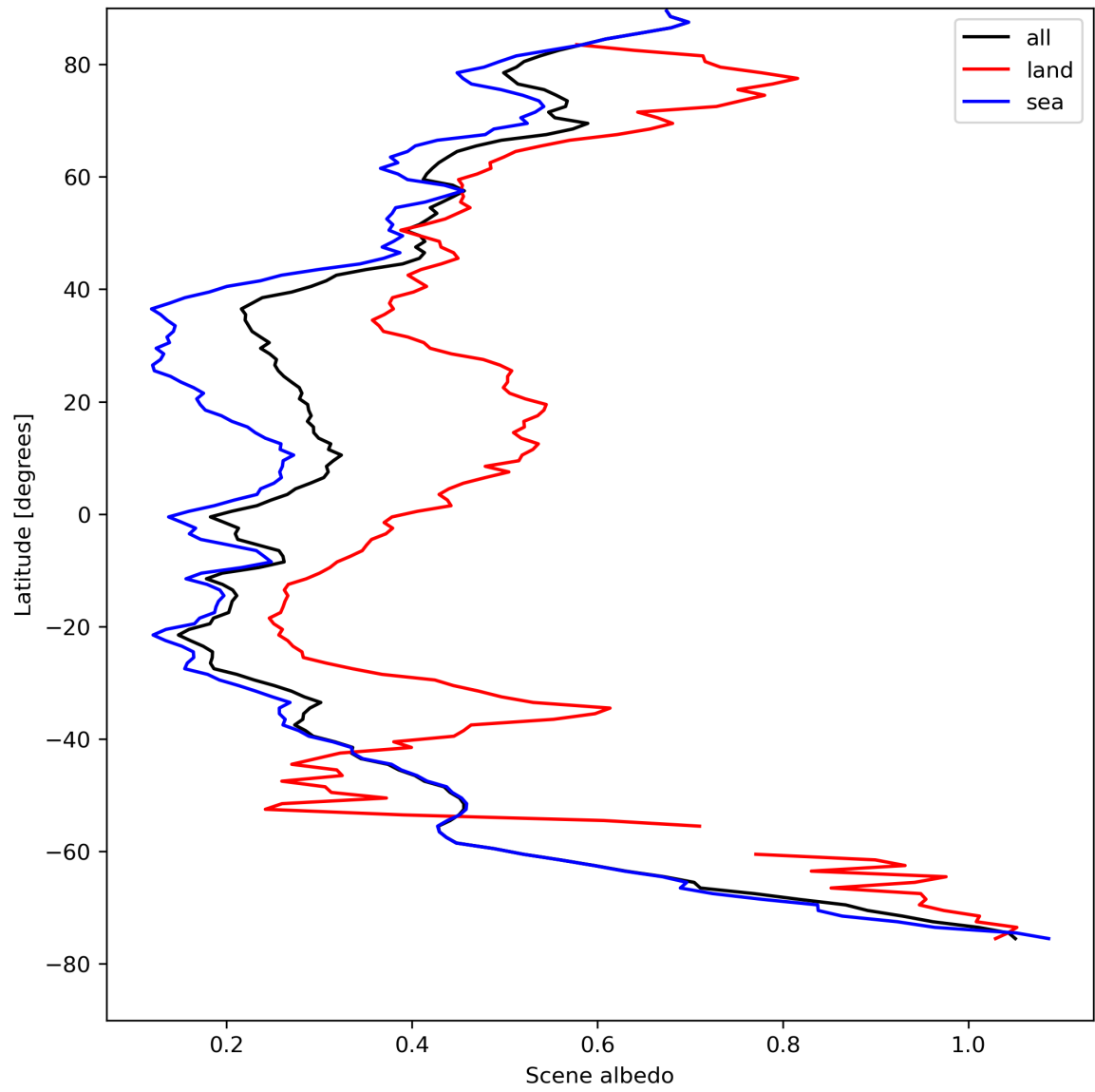
Figure 17: Zonal average of “Scene albedo” for 2024-08-18 to 2024-08-20.
