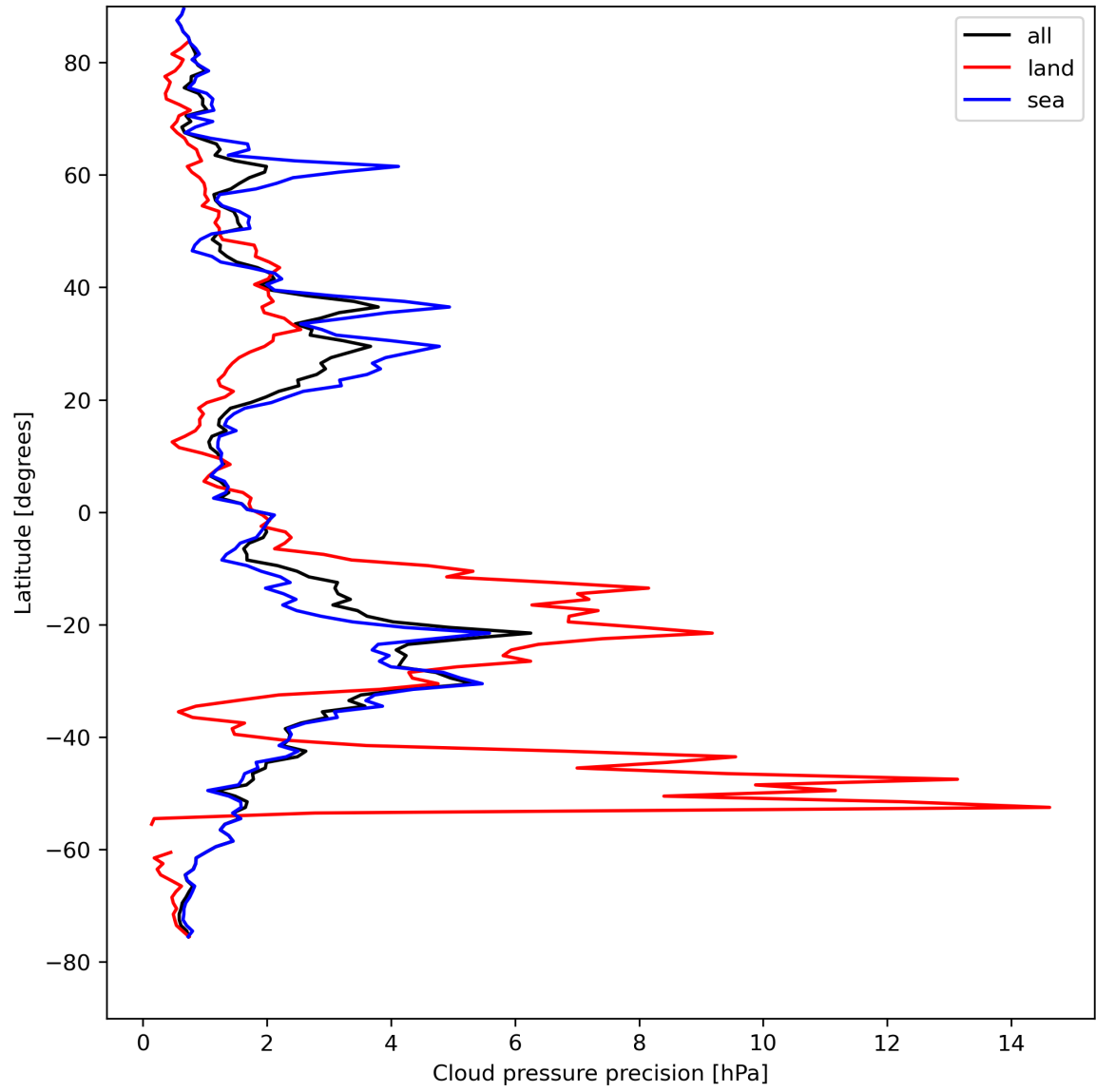
Figure 14: Zonal average of “Cloud pressure precision” for 2024-08-18 to 2024-08-20.
