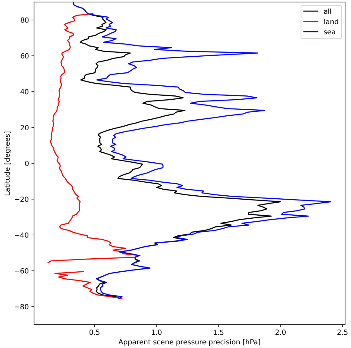
Figure 20: Zonal average of “Apparent scene pressure precision” for 2024-08-18 to 2024-08-20.
