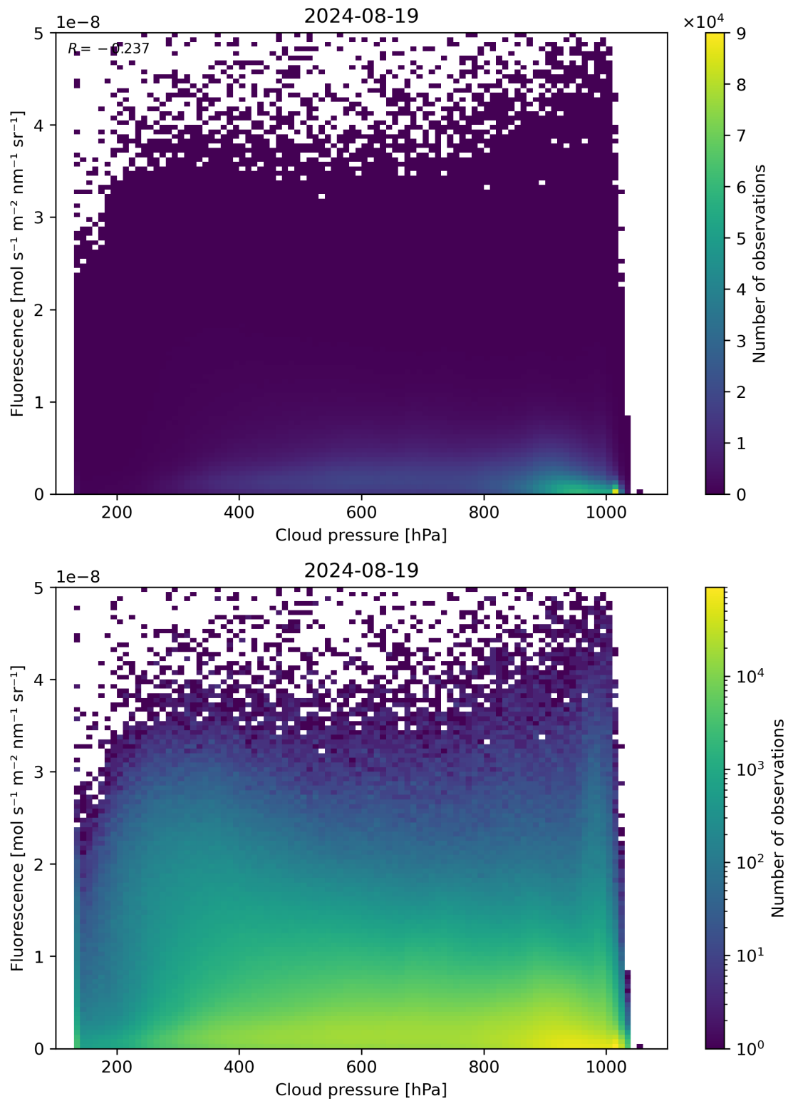
Figure 80: Scatter density plot of “Cloud pressure” against “Fluorescence” for 2024-08-18 to 2024-08-20.
