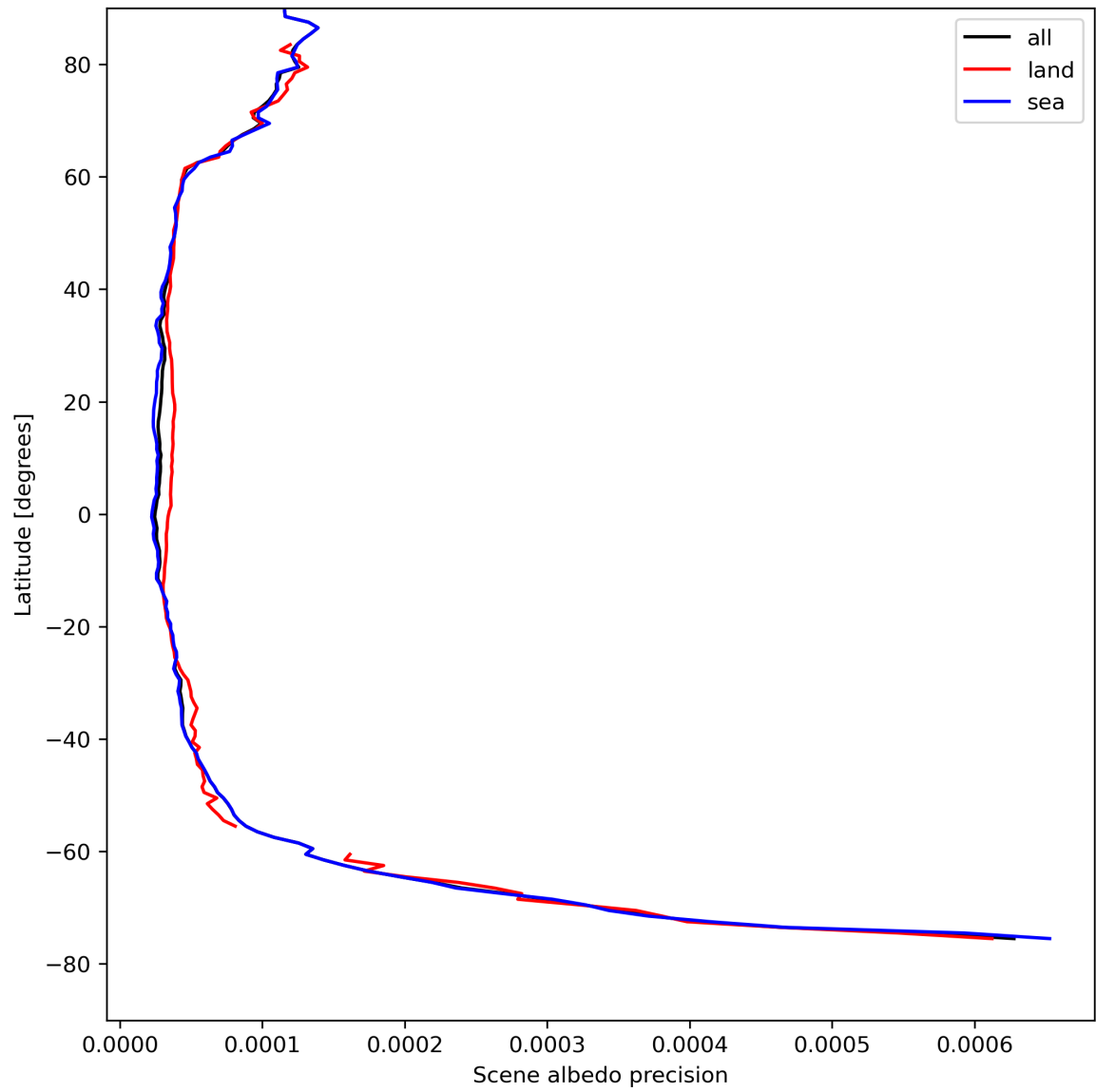
Figure 18: Zonal average of “Scene albedo precision” for 2024-08-18 to 2024-08-20.
