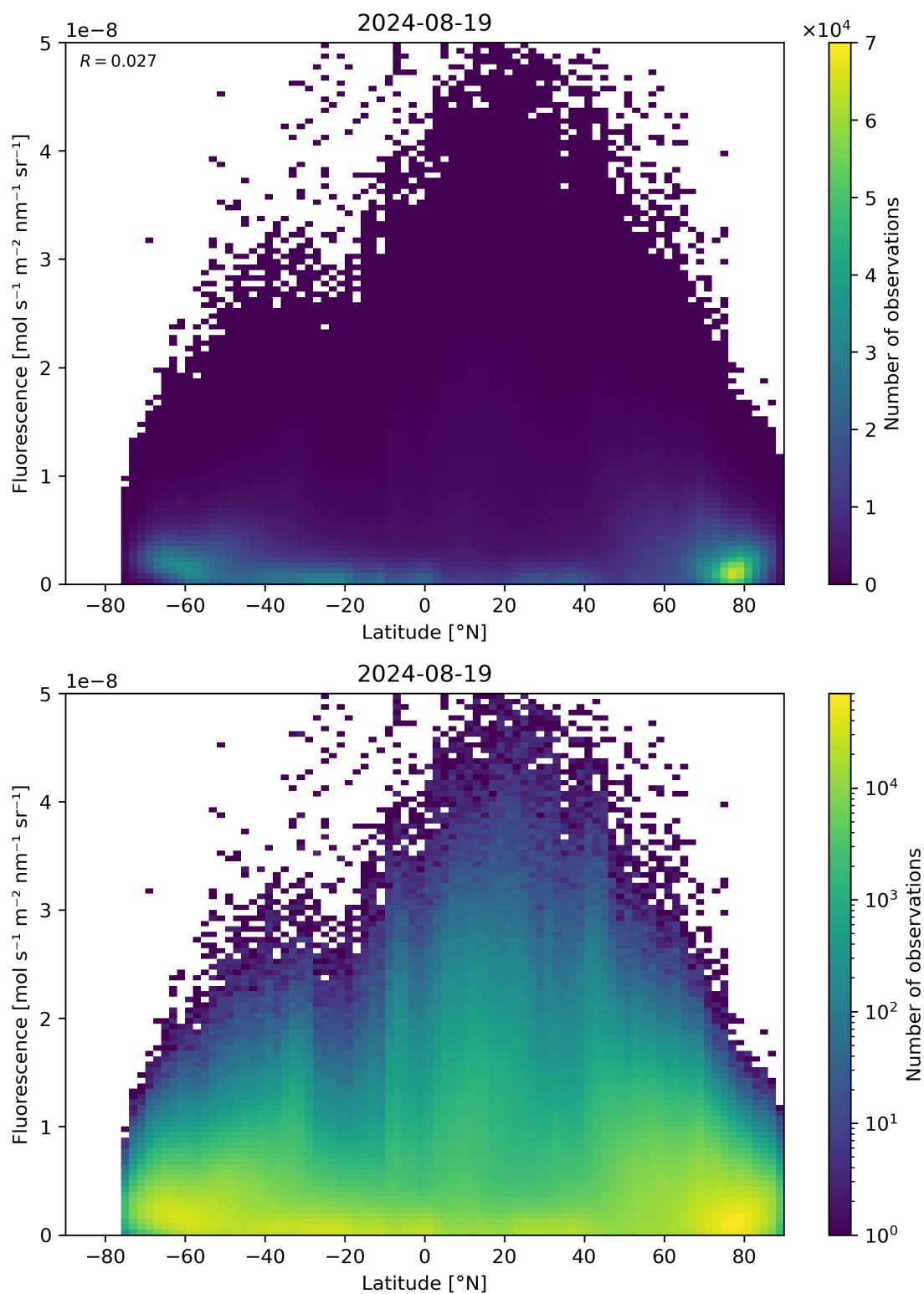
Figure 92: Scatter density plot of “Latitude” against “Fluorescence” for 2024-08-18 to 2024-08-20.
