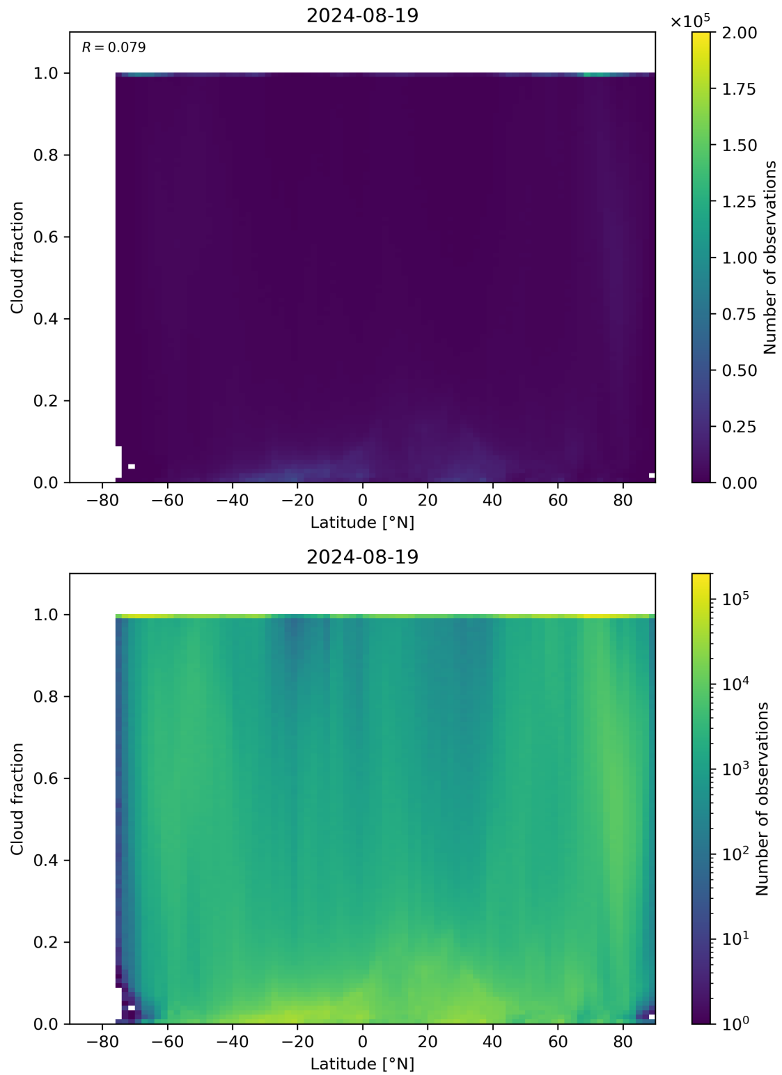
Figure 90: Scatter density plot of “Latitude” against “Cloud fraction” for 2024-08-18 to 2024-08-20.
