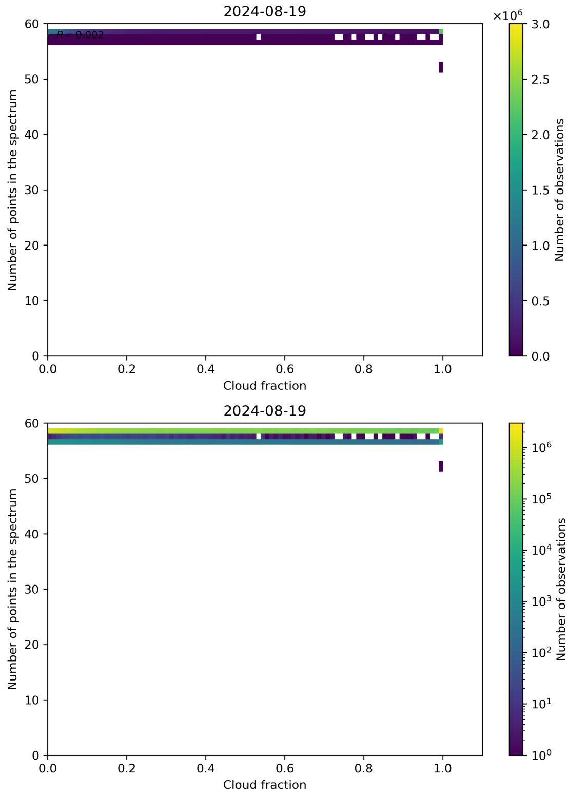
Figure 74: Scatter density plot of “Cloud fraction” against “Number of points in the spectrum” for 2024-08-18 to 2024-08-20.
