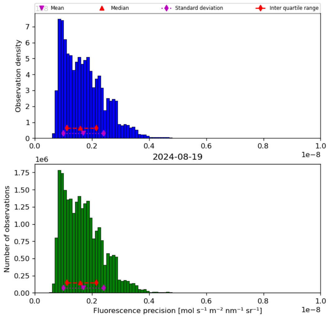
Figure 41: Histogram of “Fluorescence precision” for 2024-08-18 to 2024-08-20
