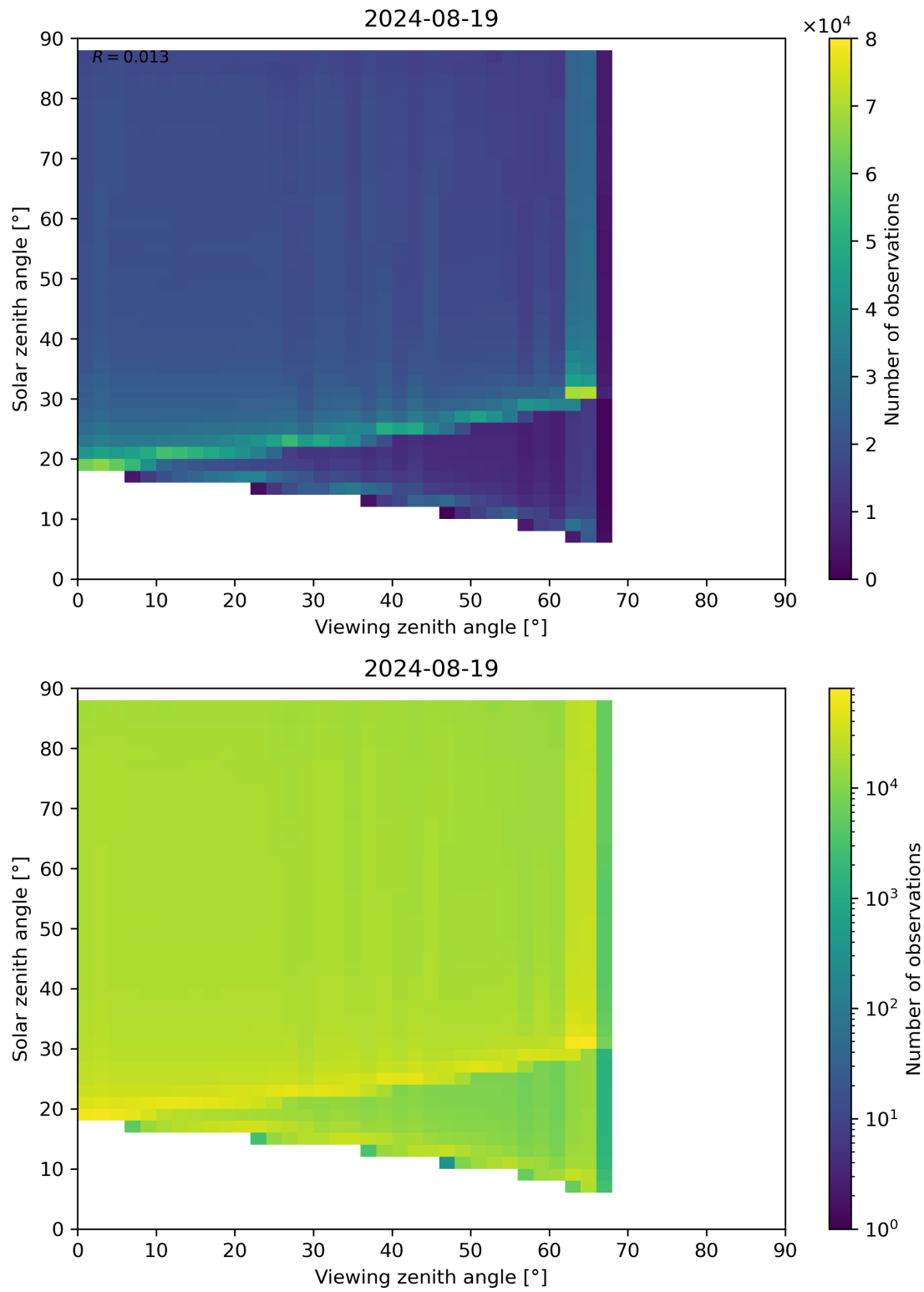
Figure 127: Scatter density plot of “Viewing zenith angle” against “Solar zenith angle” for 2024-08-18 to 2024-08-20.
