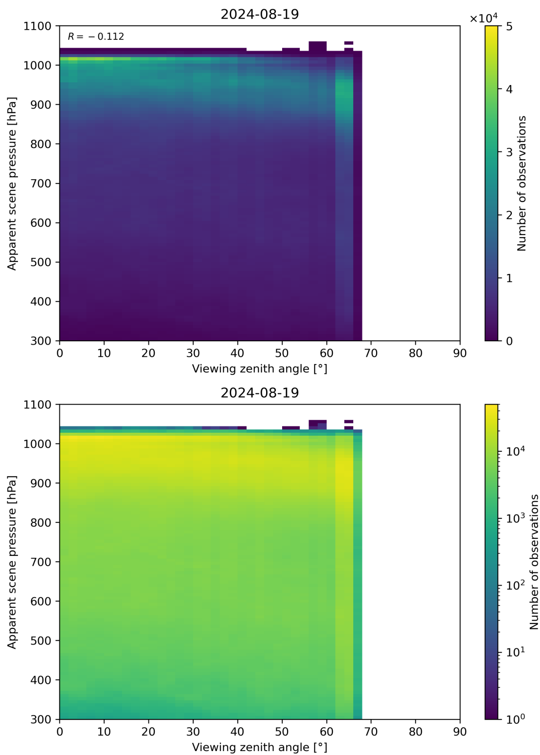
Figure 118: Scatter density plot of “Viewing zenith angle” against “Apparent scene pressure” for 2024-08-18 to 2024-08-20.
