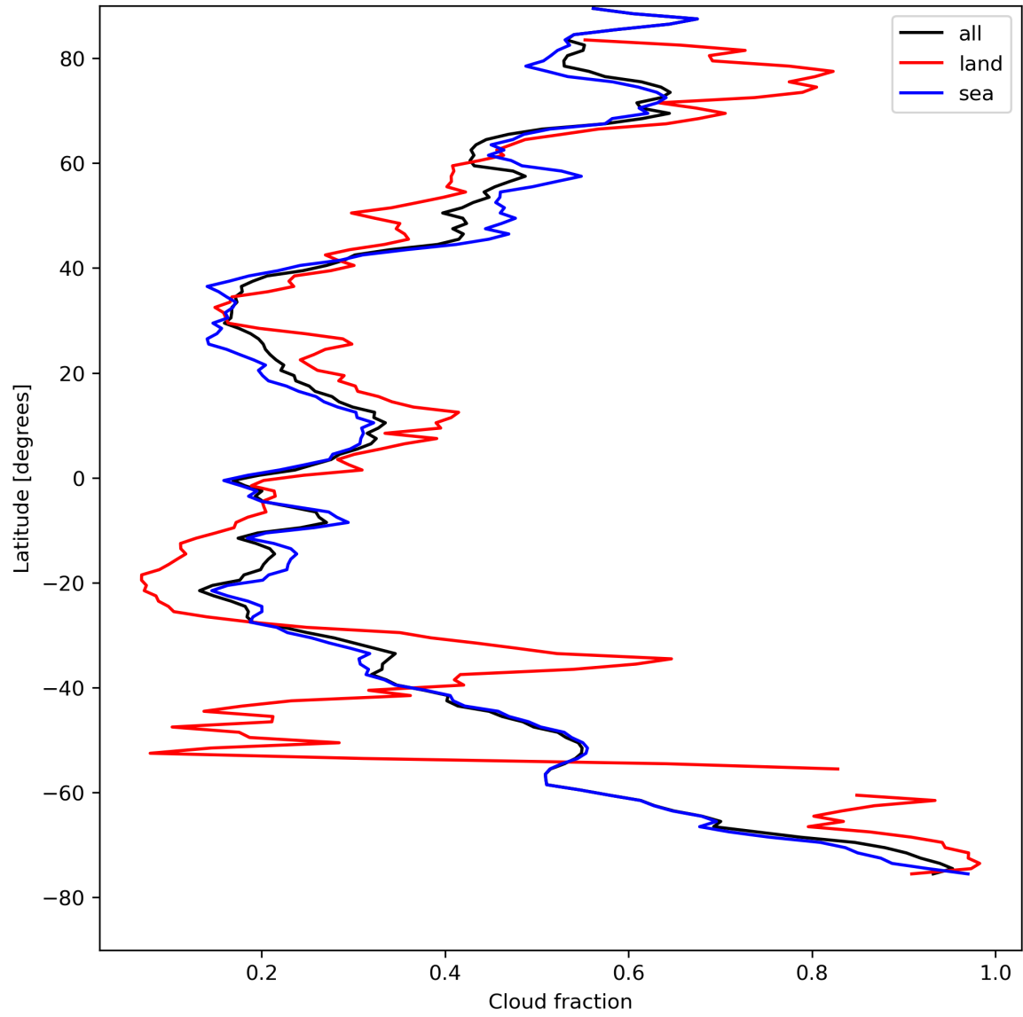
Figure 15: Zonal average of “Cloud fraction” for 2024-08-18 to 2024-08-20.
