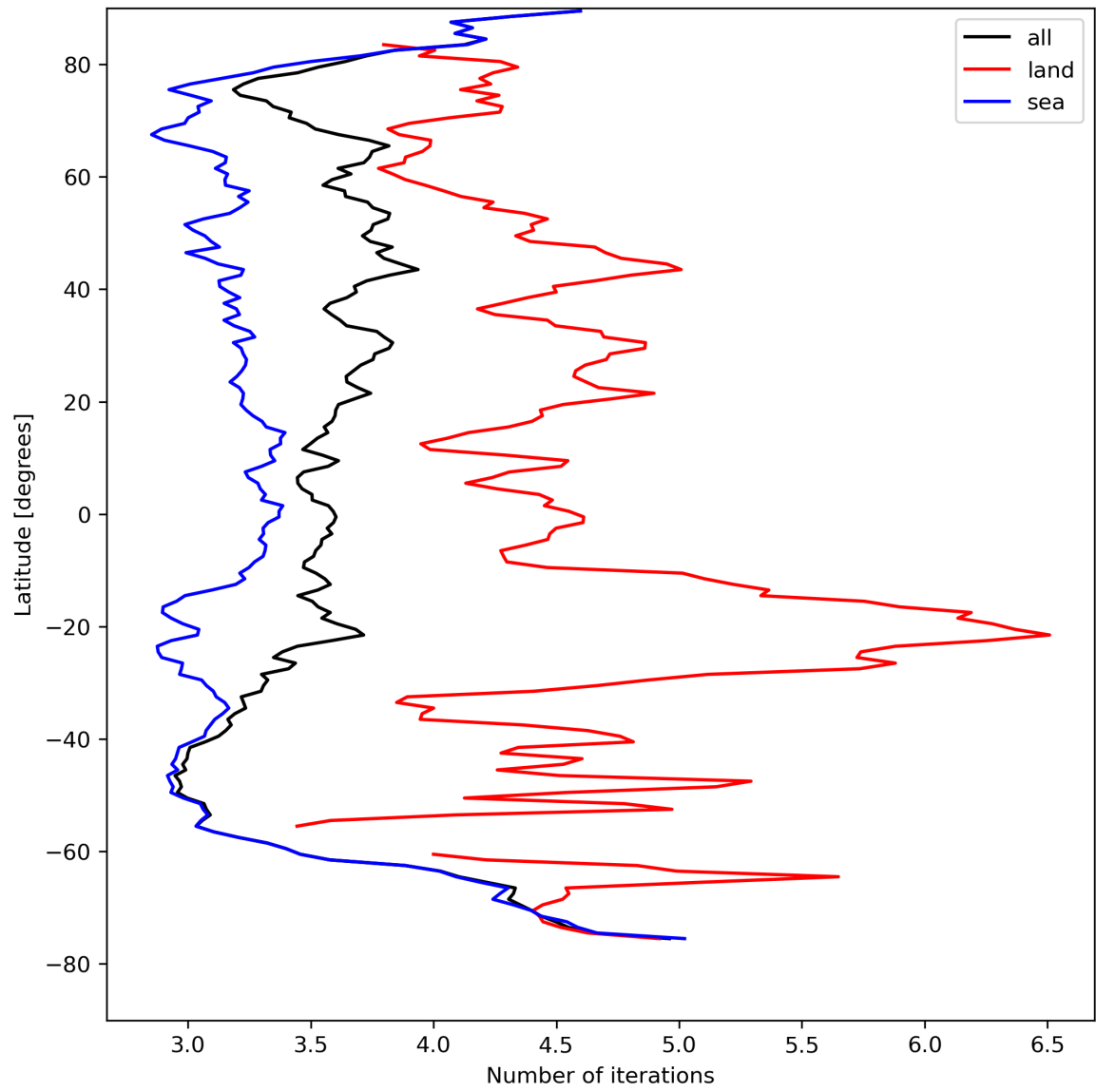
Figure 22: Zonal average of “Number of iterations” for 2024-08-18 to 2024-08-20.
