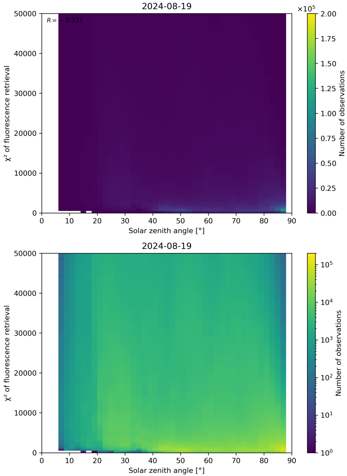
Figure 109: Scatter density plot of “Solar zenith angle” against “ \chi^2 of fluorescence retrieval” for 2024-08-18 to 2024-08-20.
