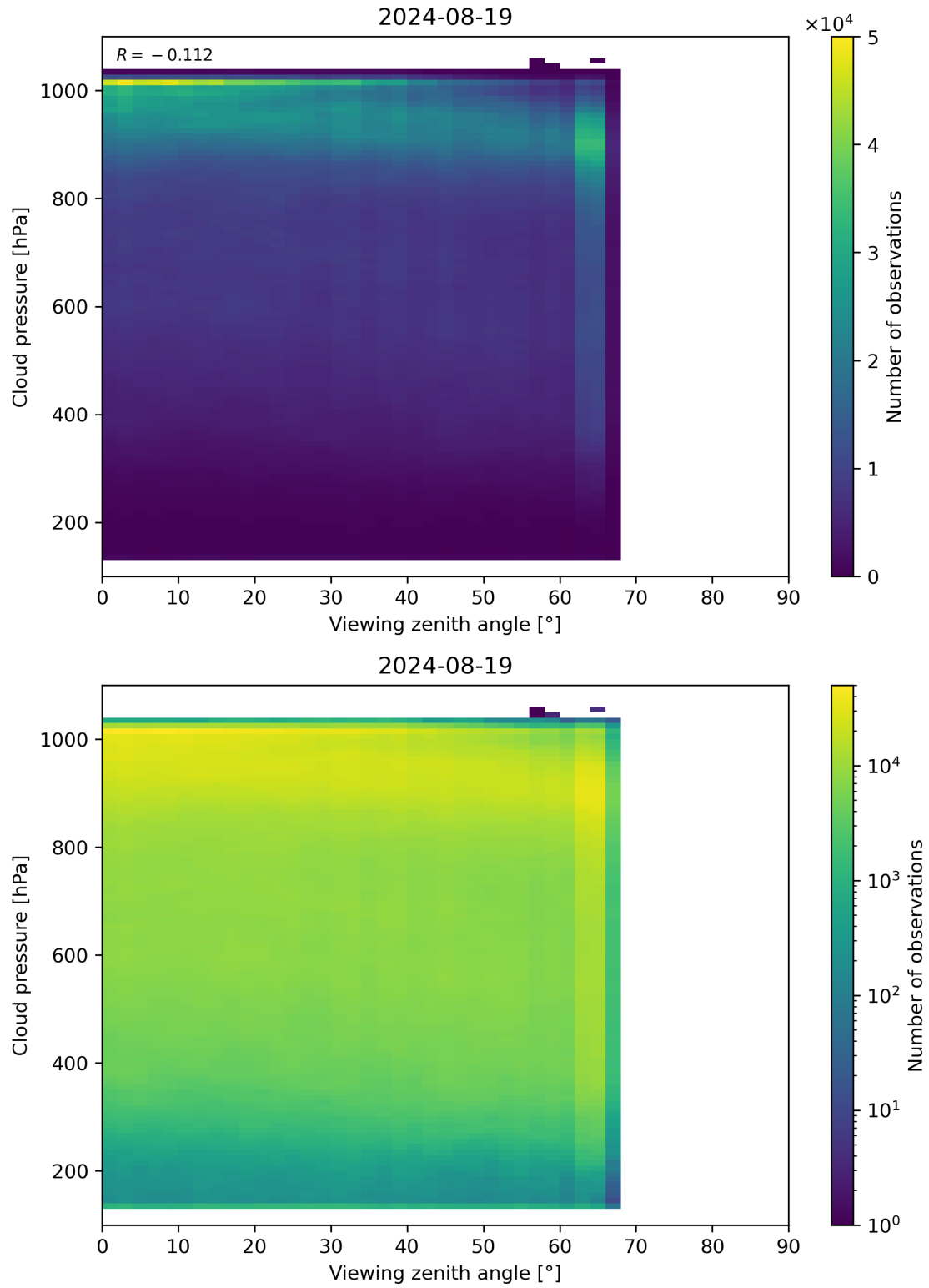
Figure 121: Scatter density plot of “Viewing zenith angle” against “Cloud pressure” for 2024-08-18 to 2024-08-20.
