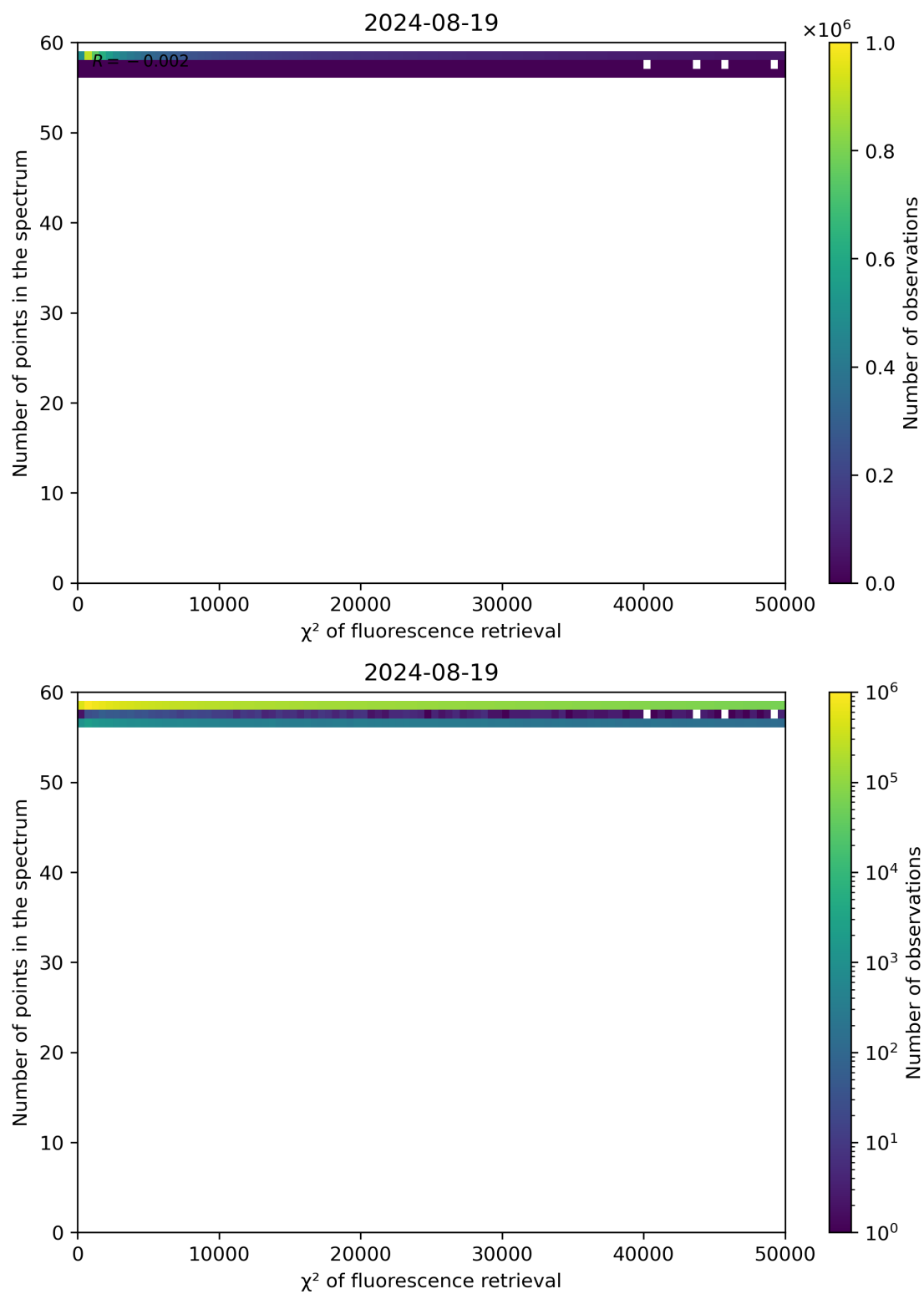
Figure 68: Scatter density plot of " \chi^2 of fluorescence retrieval" against "Number of points in the spectrum" for 2024-08-18 to 2024-08-20.
