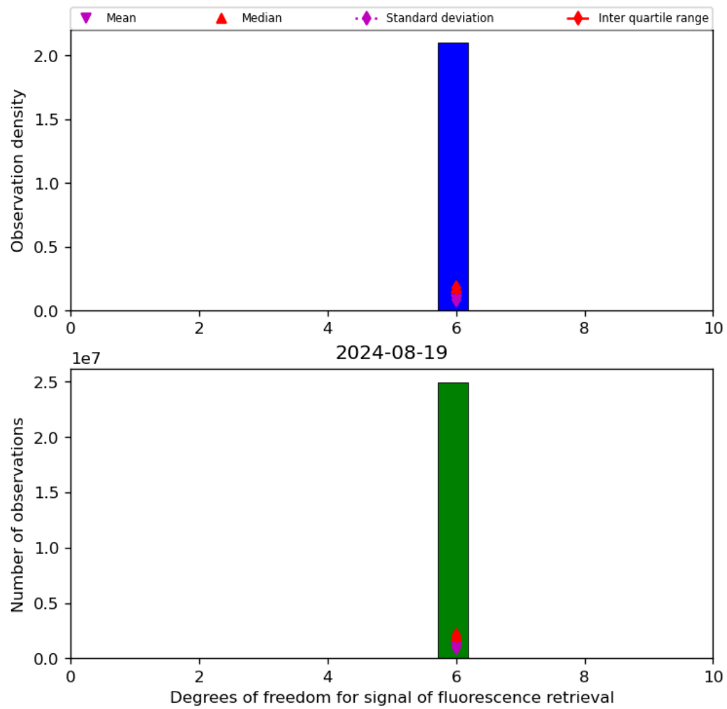
Figure 43: Histogram of “Degrees of freedom for signal of fluorescence retrieval” for 2024-08-18 to 2024-08-20
