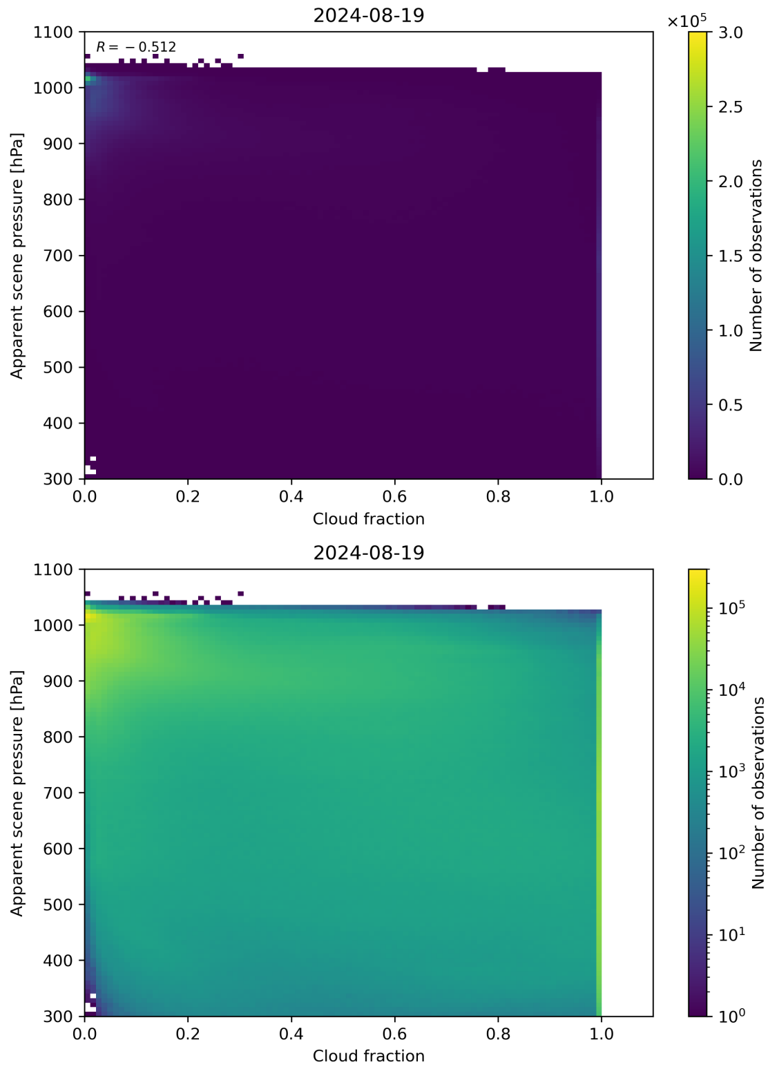
Figure 70: Scatter density plot of “Cloud fraction” against “Apparent scene pressure” for 2024-08-18 to 2024-08-20.
