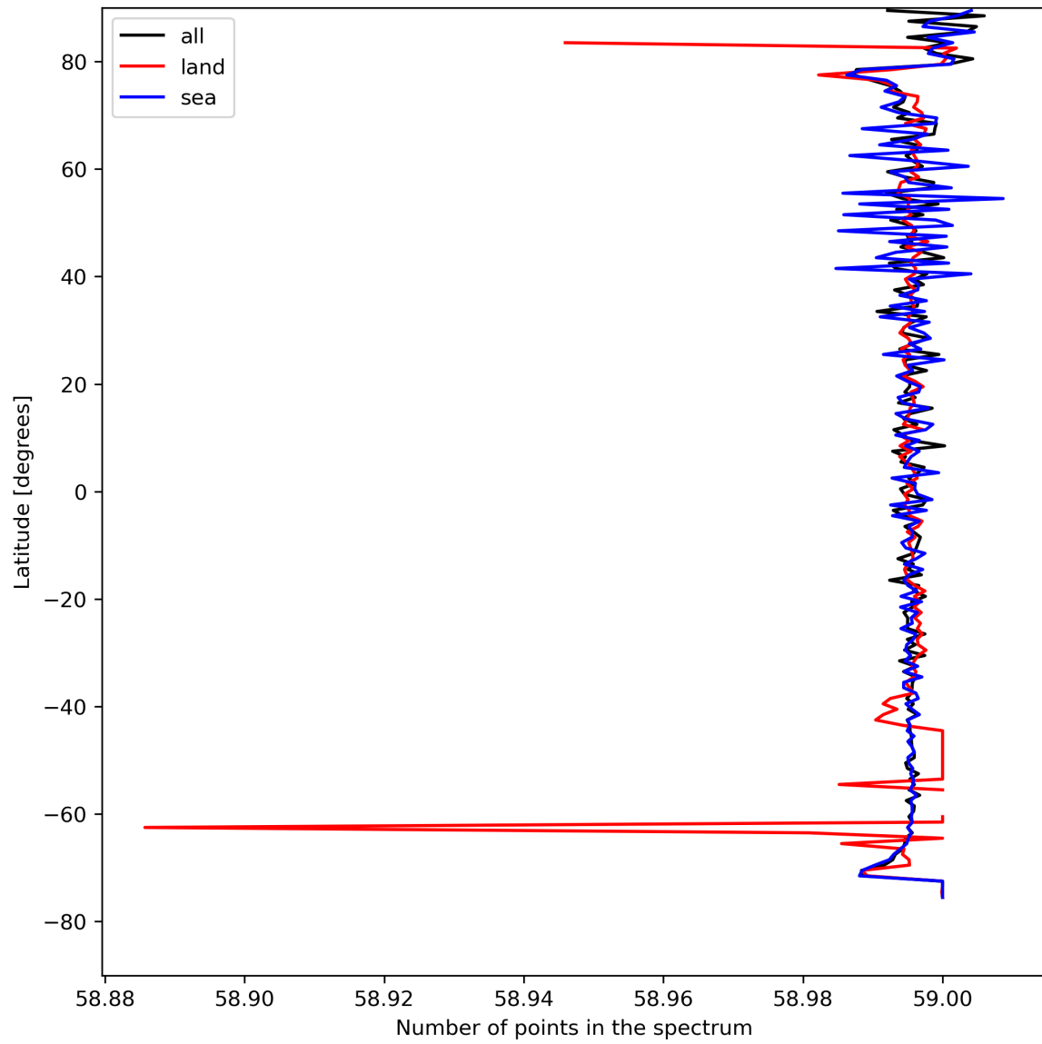
Figure 27: Zonal average of “Number of points in the spectrum” for 2024-08-18 to 2024-08-20.
