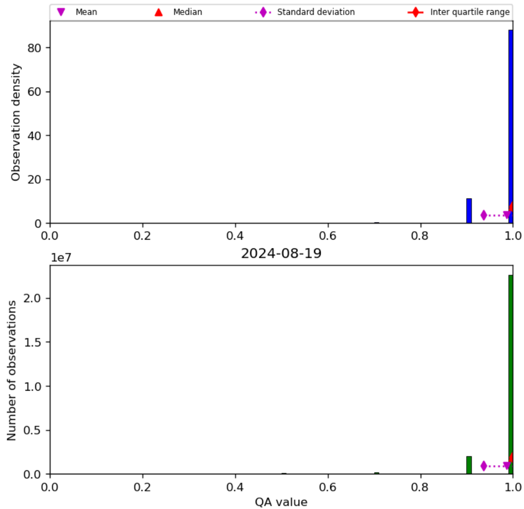
Figure 29: Histogram of “QA value” for 2024-08-18 to 2024-08-20
