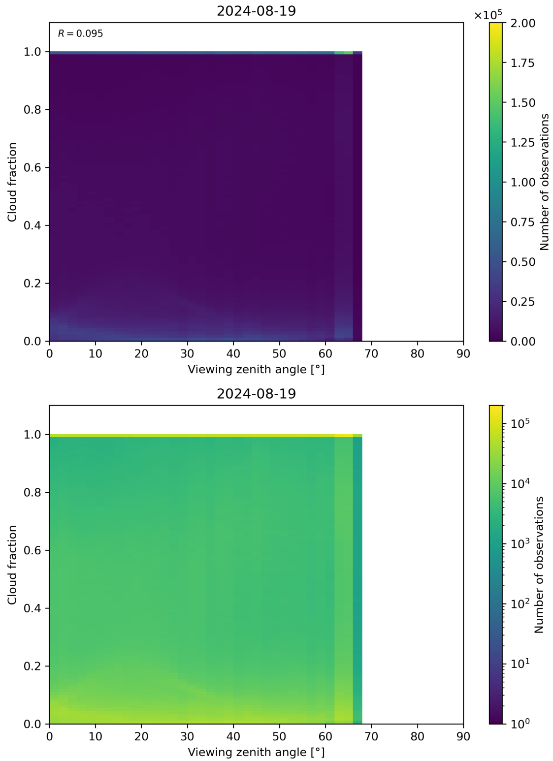
Figure 120: Scatter density plot of “Viewing zenith angle” against “Cloud fraction” for 2024-08-18 to 2024-08-20.
