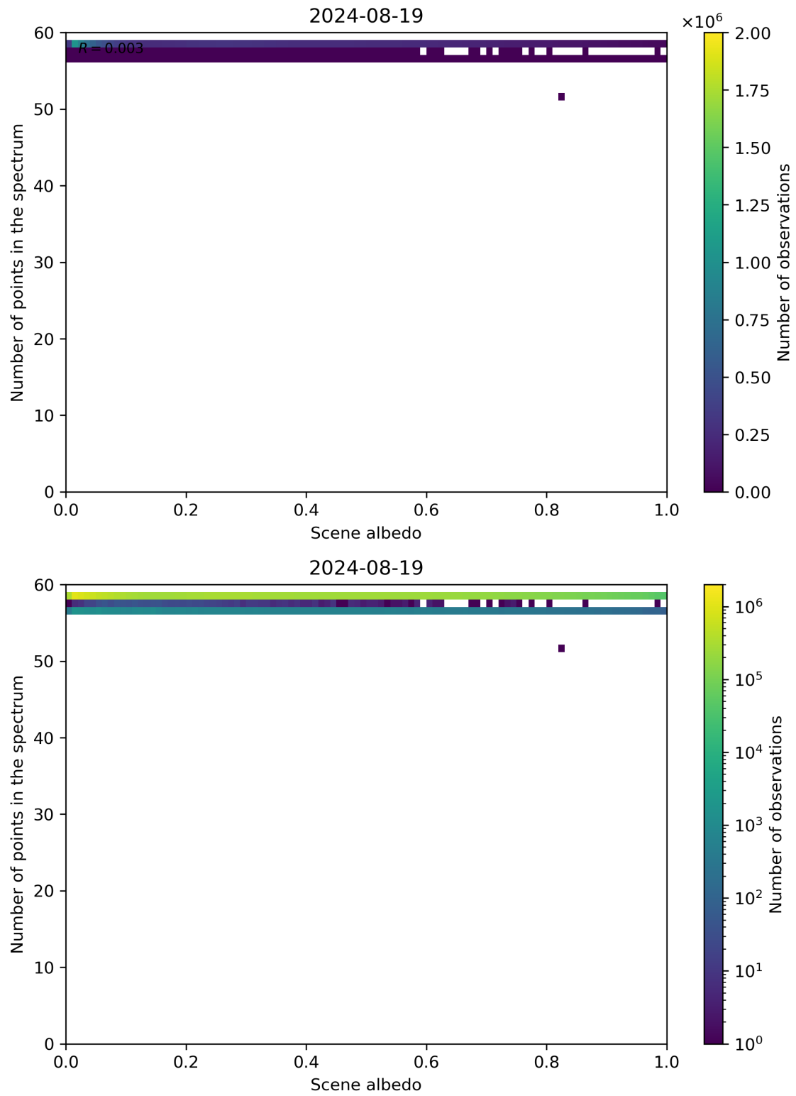
Figure 106: Scatter density plot of “Scene albedo” against “Number of points in the spectrum” for 2024-08-18 to 2024-08-20.
