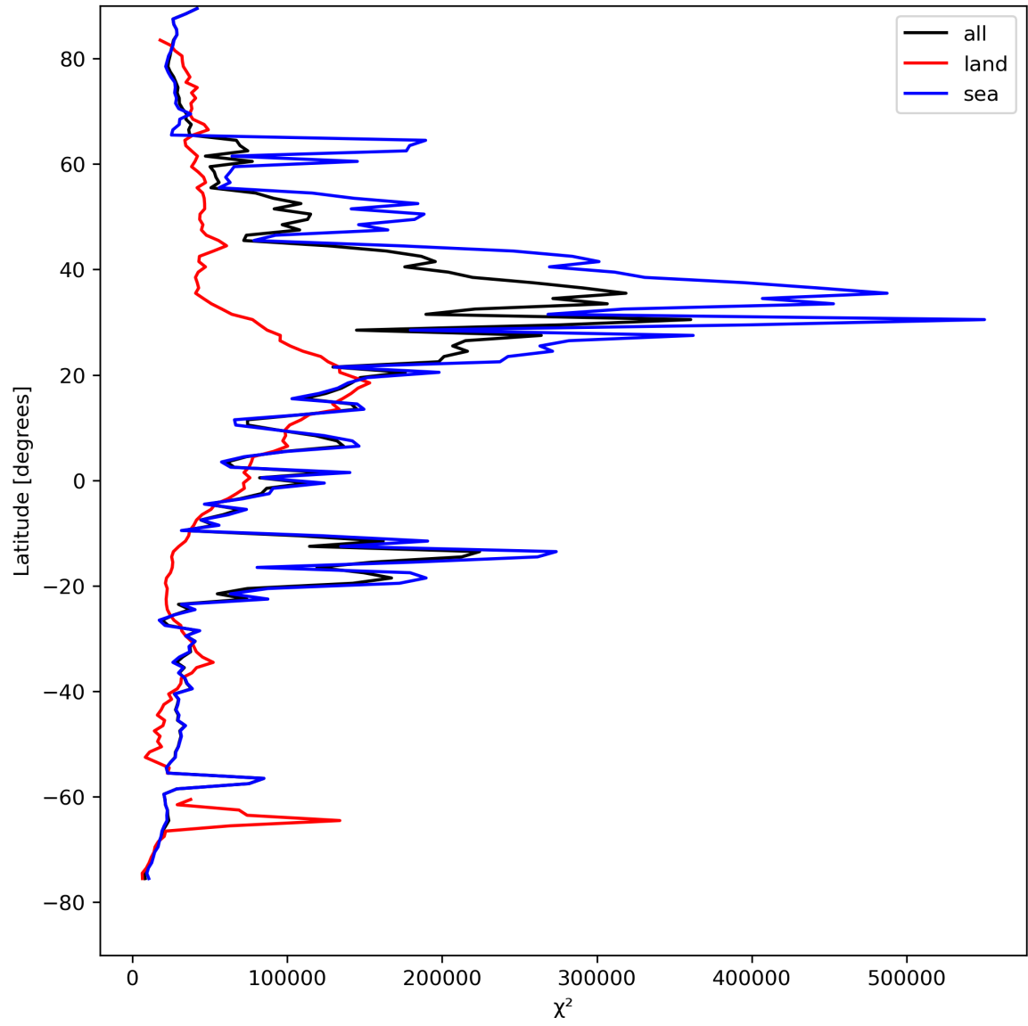
Figure 21: Zonal average of “ \chi^2 ” for 2024-08-18 to 2024-08-20.
