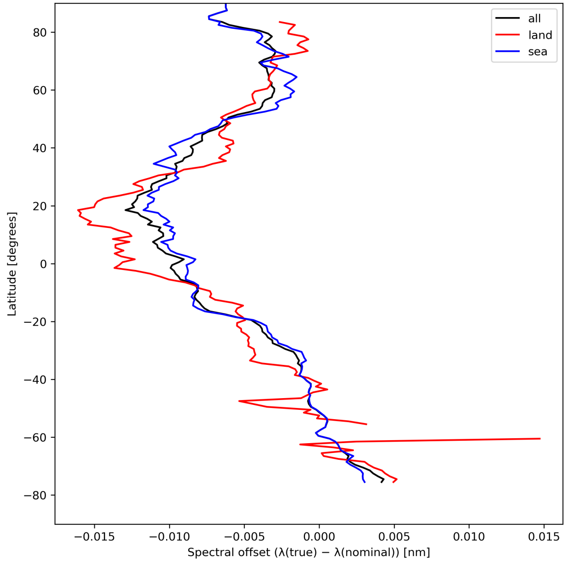
Figure 28: Zonal average of “Spectral offset ( \lambda(\text{true}) - \lambda(\text{nominal}) )” for 2024-08-18 to 2024-08-20.
