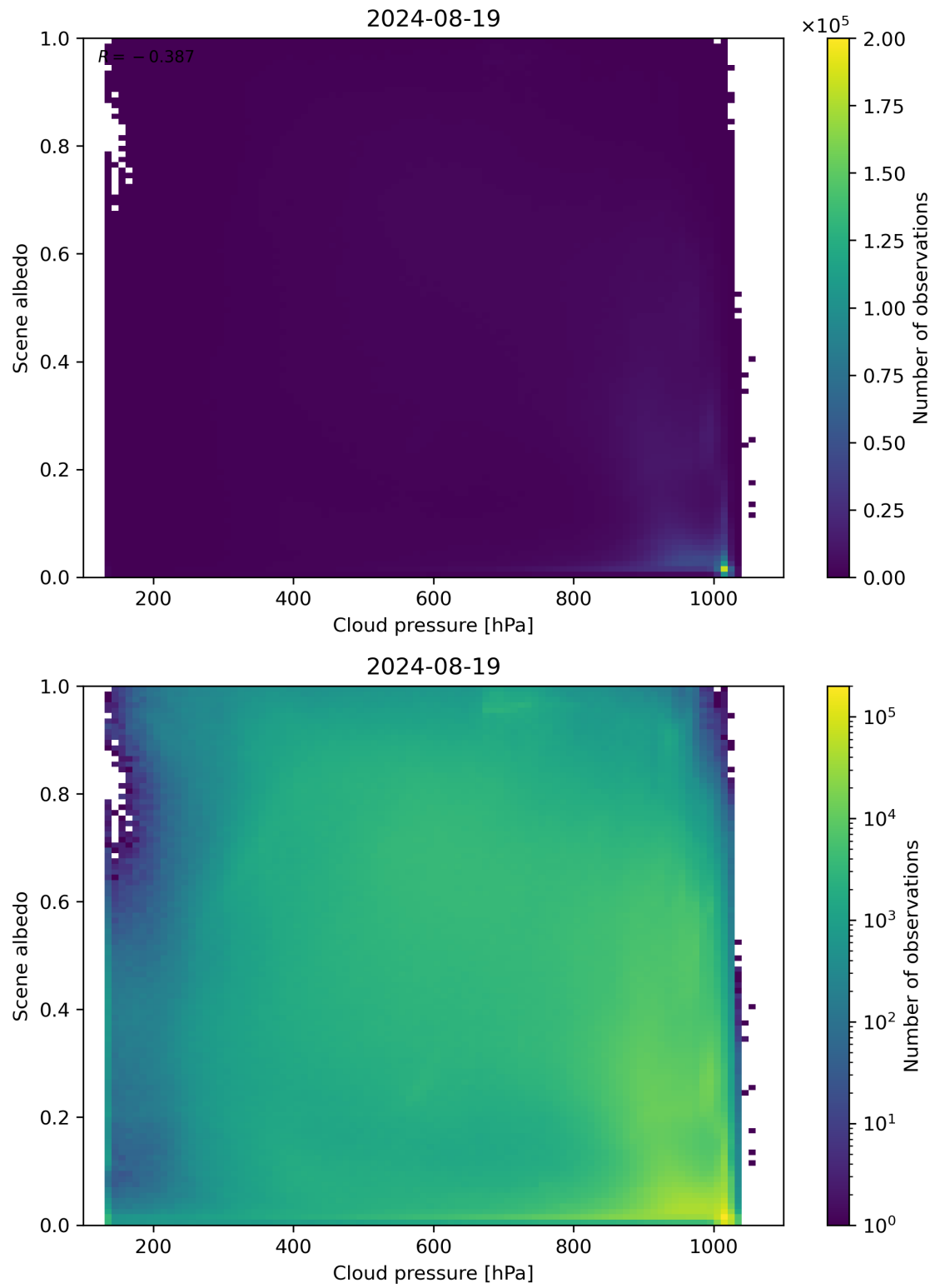
Figure 83: Scatter density plot of “Cloud pressure” against “Scene albedo” for 2024-08-18 to 2024-08-20.
