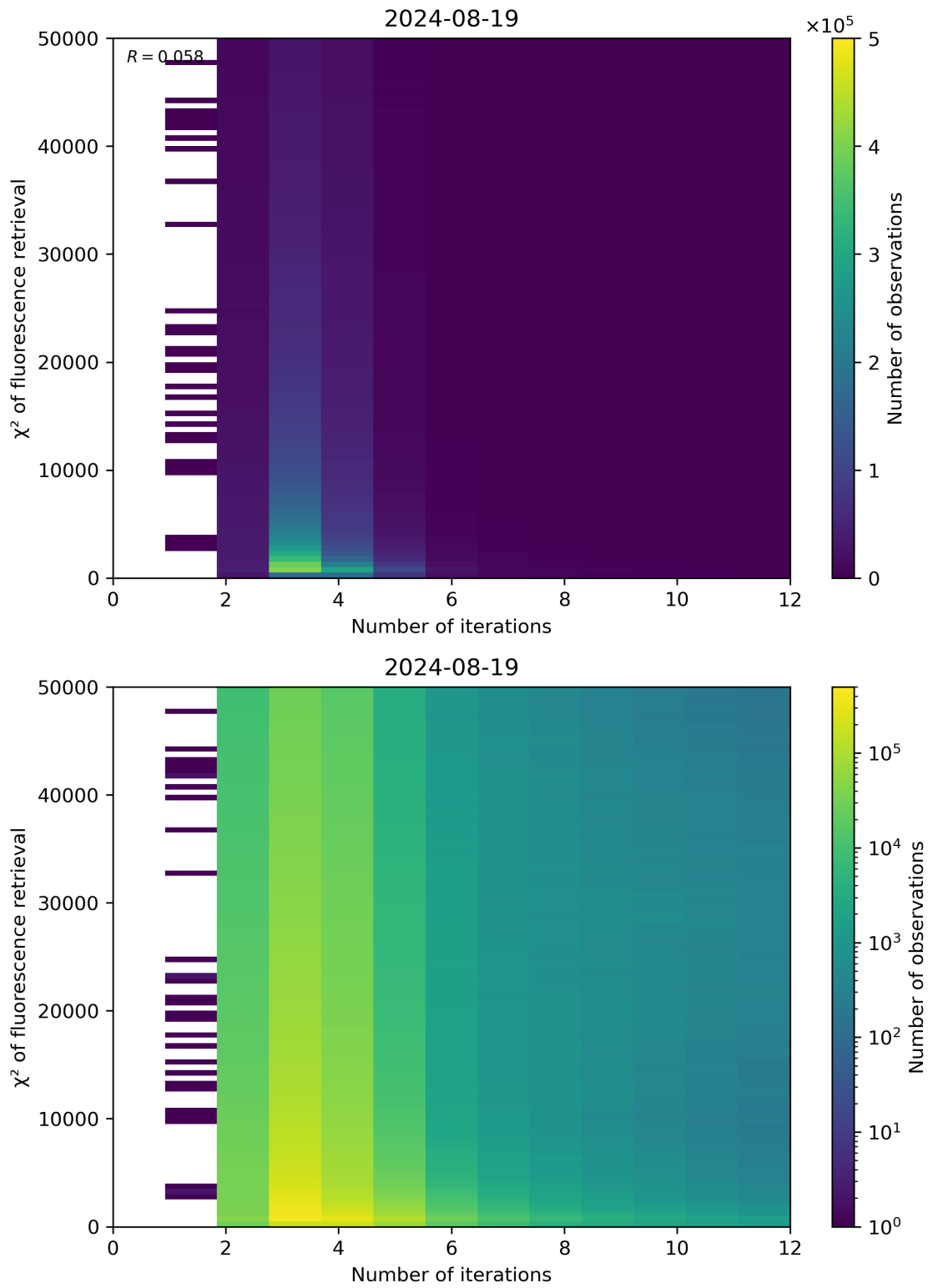
Figure 97: Scatter density plot of “Number of iterations” against “ \chi^2 of fluorescence retrieval” for 2024-08-18 to 2024-08-20.
