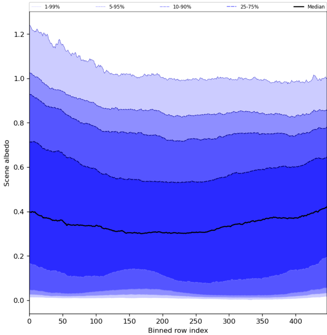
Figure 51: Along track statistics of “Scene albedo” for 2024-08-18 to 2024-08-20
