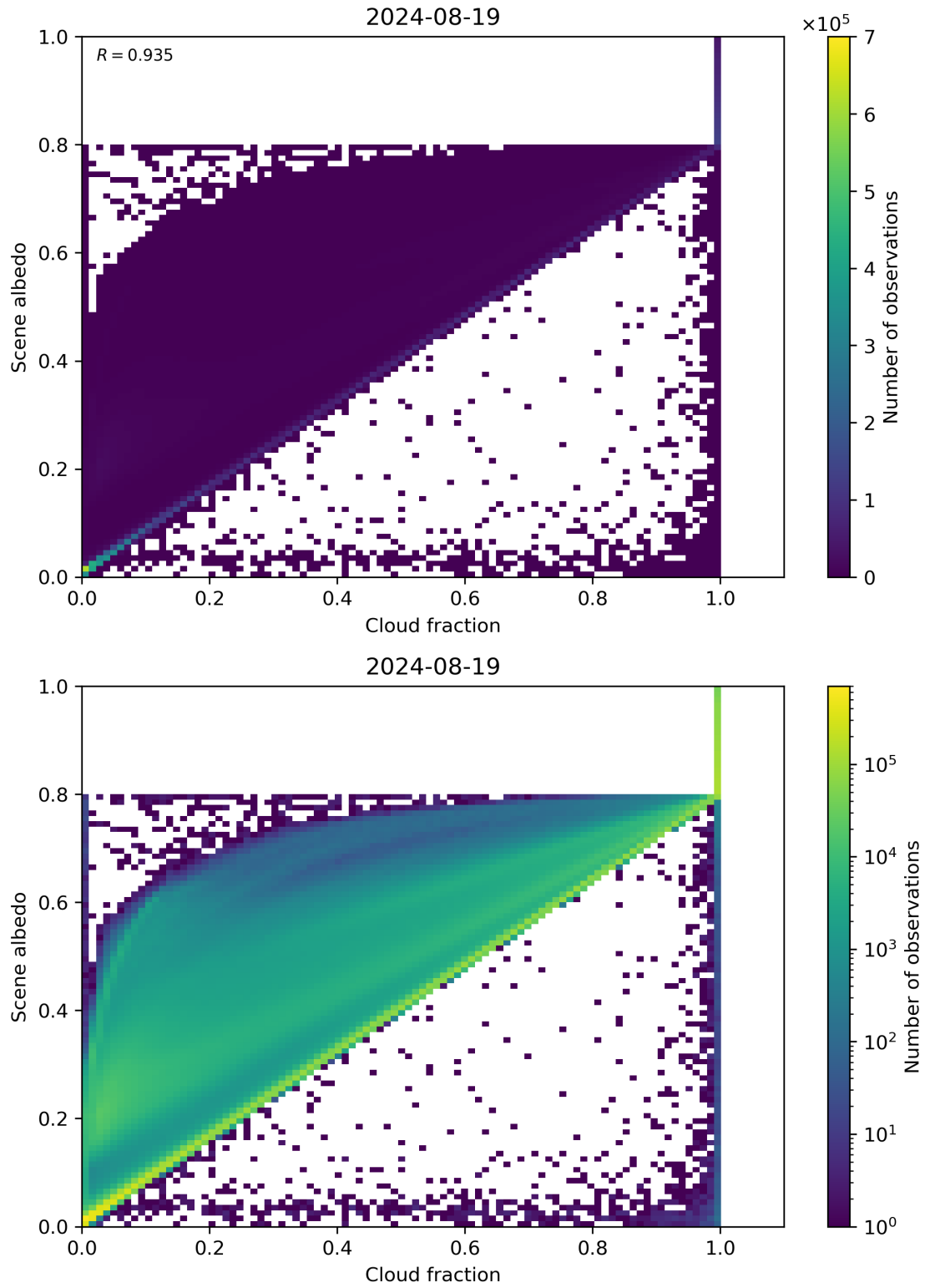
Figure 75: Scatter density plot of “Cloud fraction” against “Scene albedo” for 2024-08-18 to 2024-08-20.
