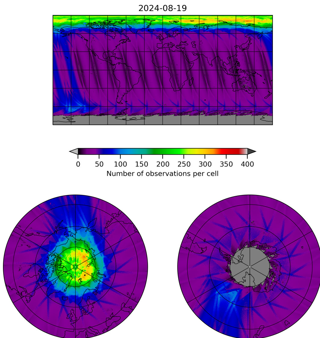
Figure 11: Map of the number of observations for 2024-08-18 to 2024-08-20
