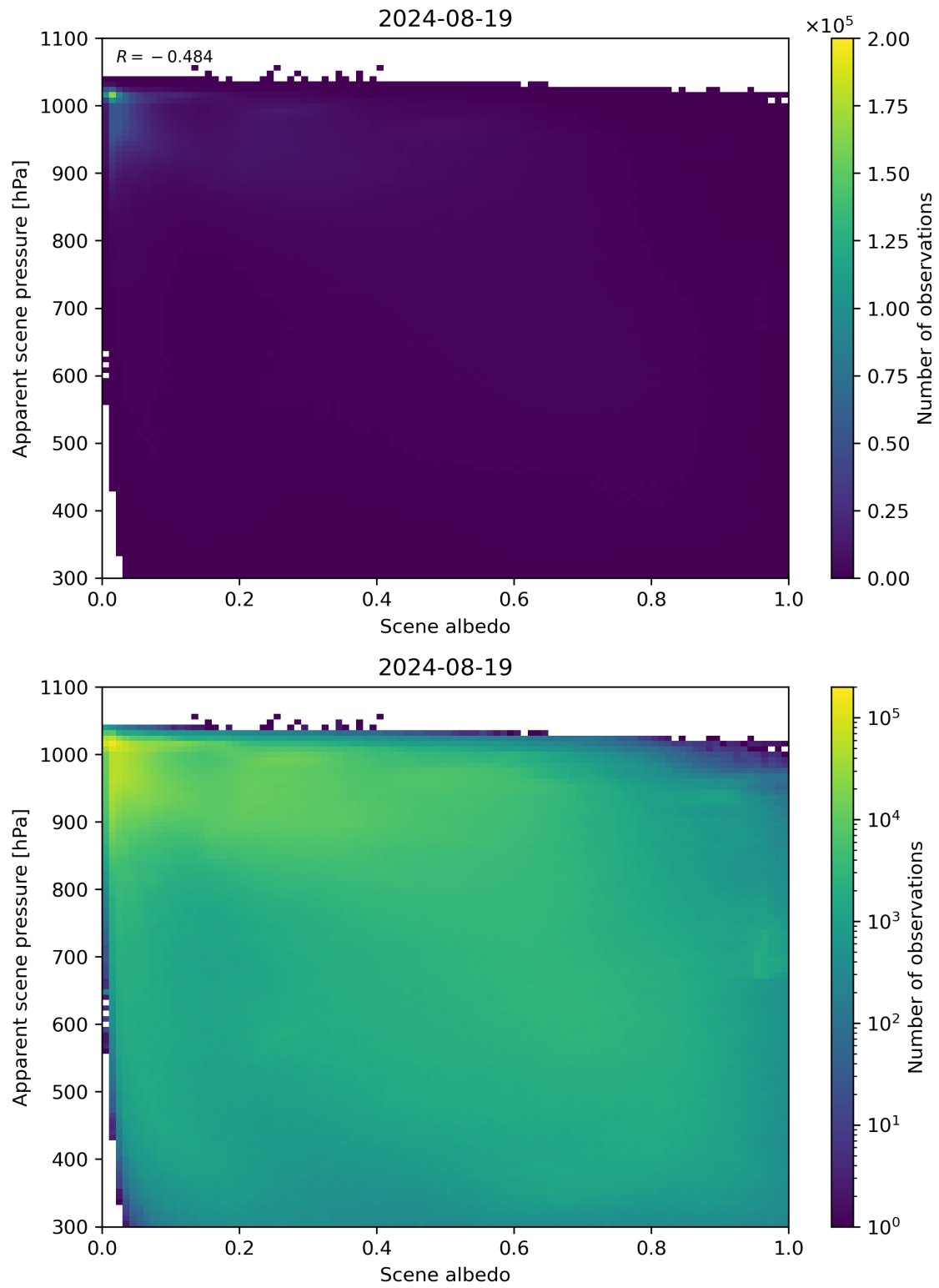
Figure 102: Scatter density plot of “Scene albedo” against “Apparent scene pressure” for 2024-08-18 to 2024-08-20.
