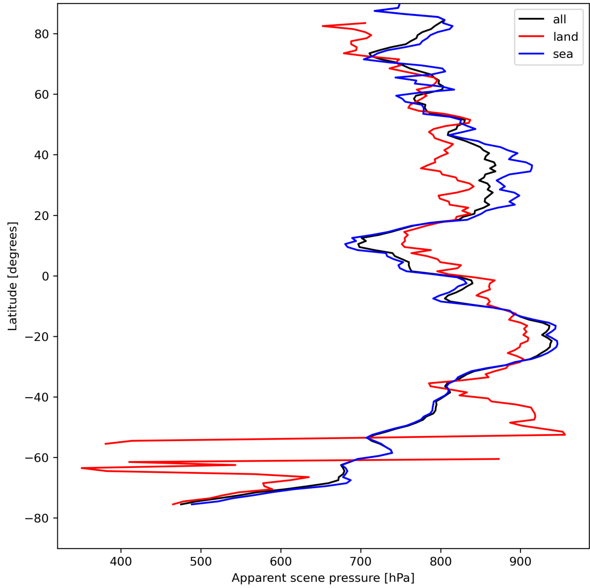
Figure 19: Zonal average of “Apparent scene pressure” for 2024-08-18 to 2024-08-20.
