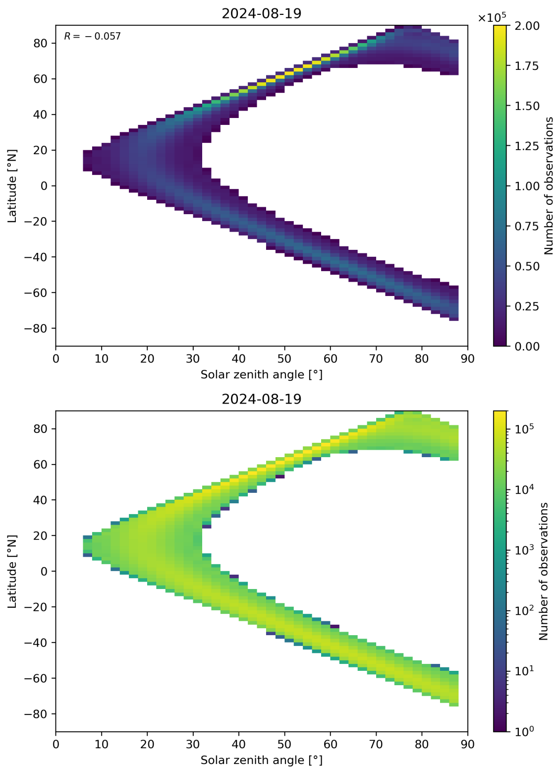
Figure 113: Scatter density plot of “Solar zenith angle” against “Latitude” for 2024-08-18 to 2024-08-20.
