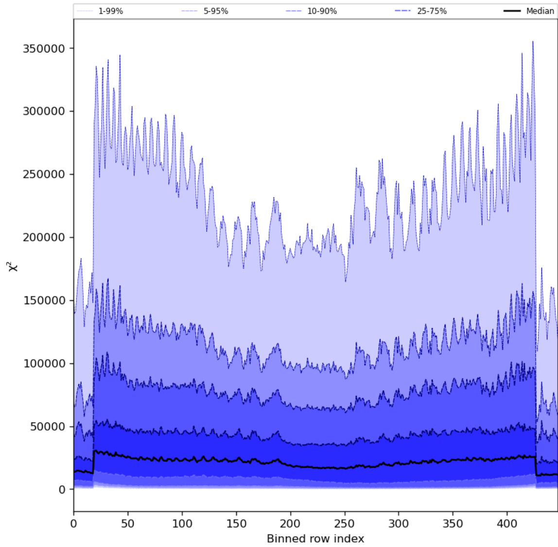
Figure 55: Along track statistics of “ \chi^2 ” for 2024-08-18 to 2024-08-20
