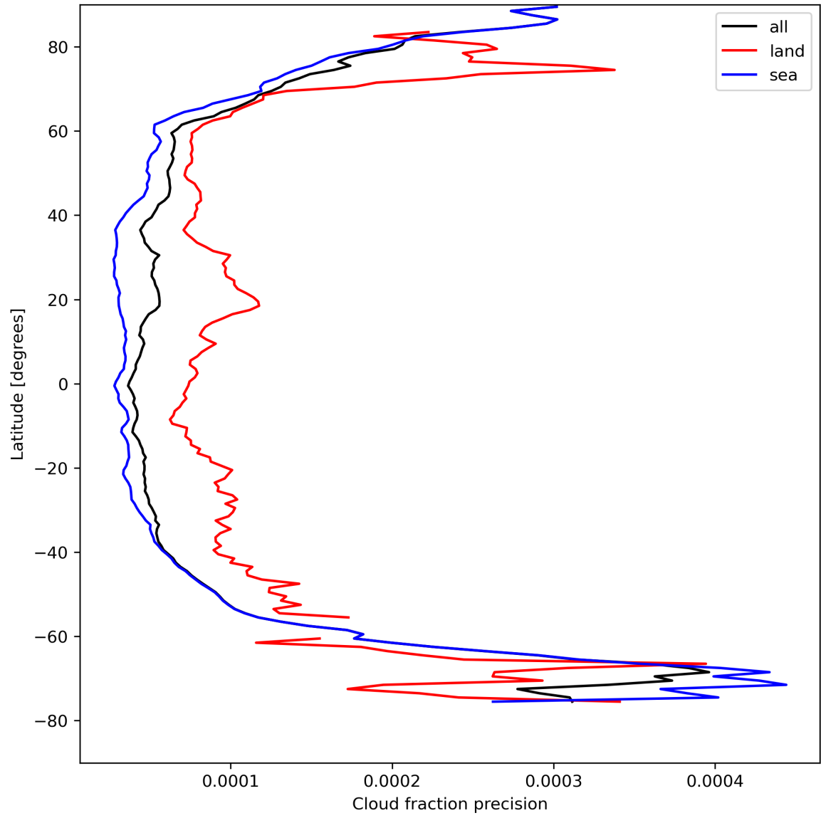
Figure 16: Zonal average of “Cloud fraction precision” for 2024-08-18 to 2024-08-20.
