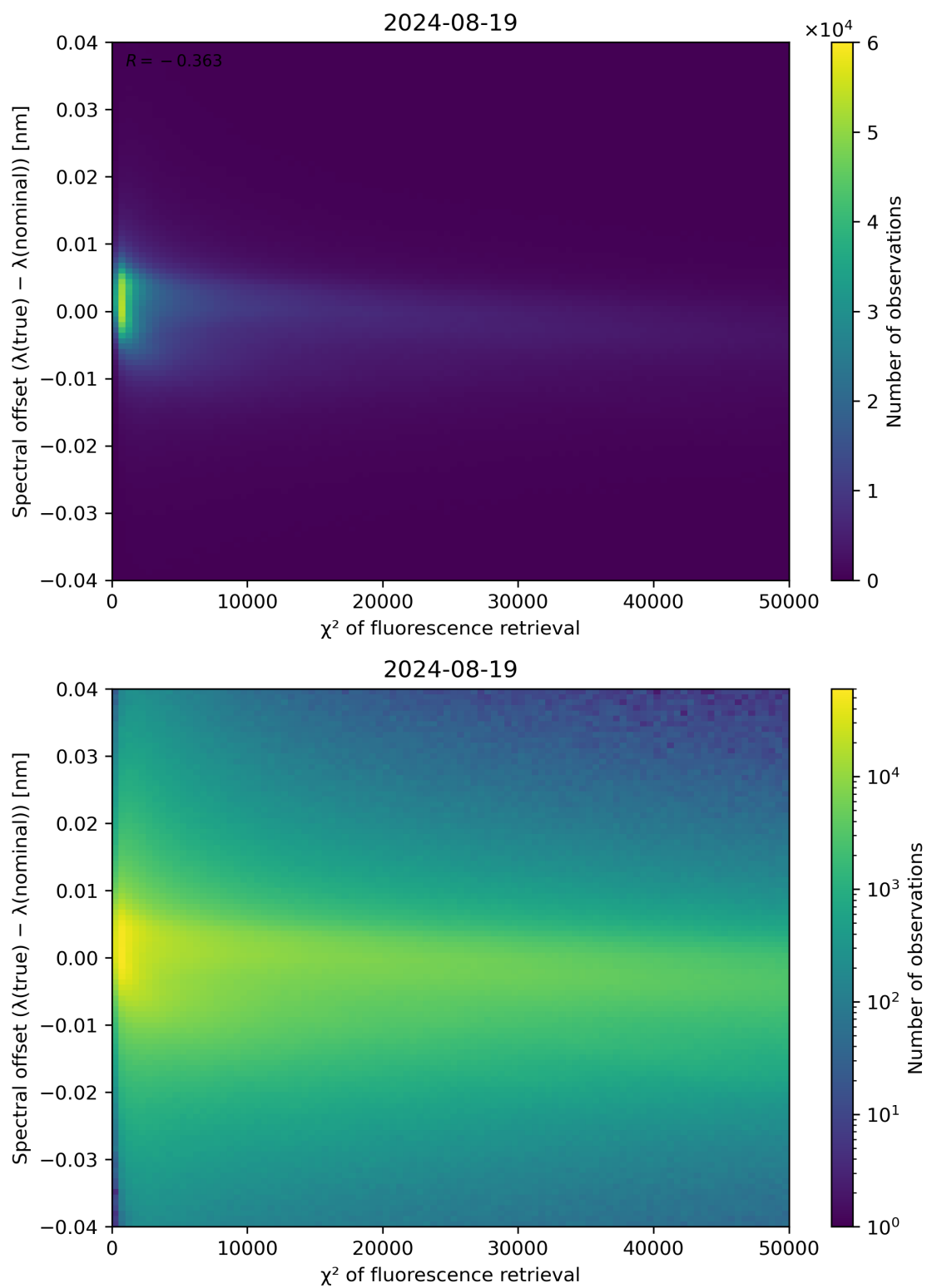
Figure 69: Scatter density plot of “ \chi^2 of fluorescence retrieval” against “Spectral offset ( \lambda(\text{true}) - \lambda(\text{nominal}) )” for 2024-08-18 to 2024-08-20.
