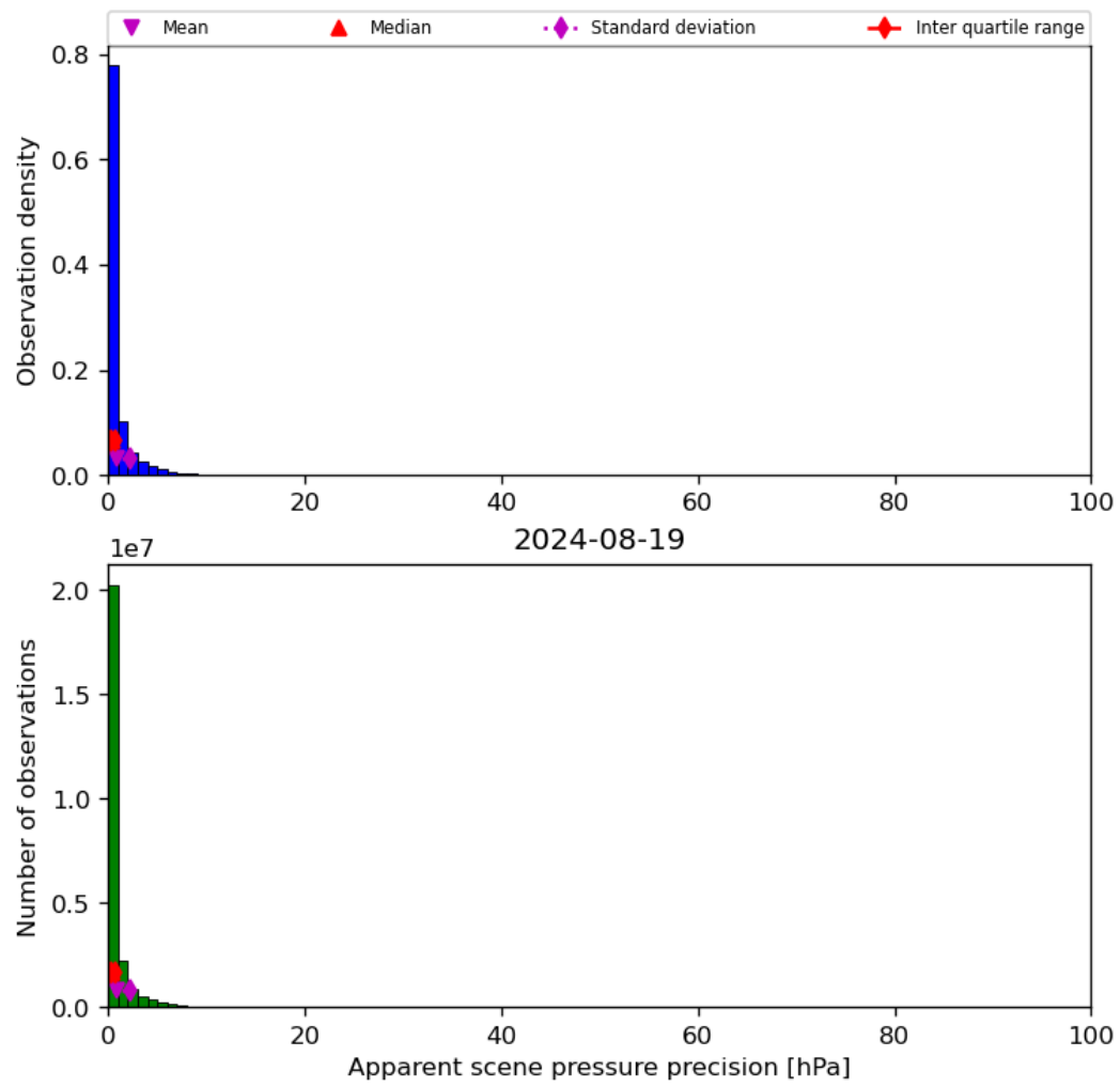
Figure 37: Histogram of “Apparent scene pressure precision” for 2024-08-18 to 2024-08-20
