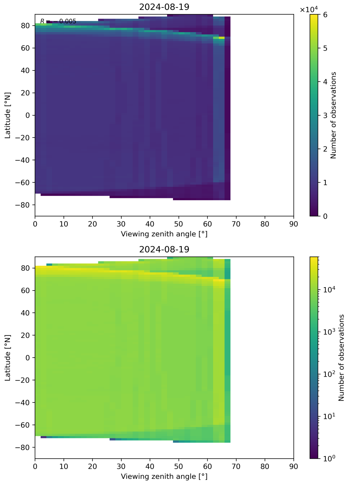
Figure 123: Scatter density plot of “Viewing zenith angle” against “Latitude” for 2024-08-18 to 2024-08-20.
