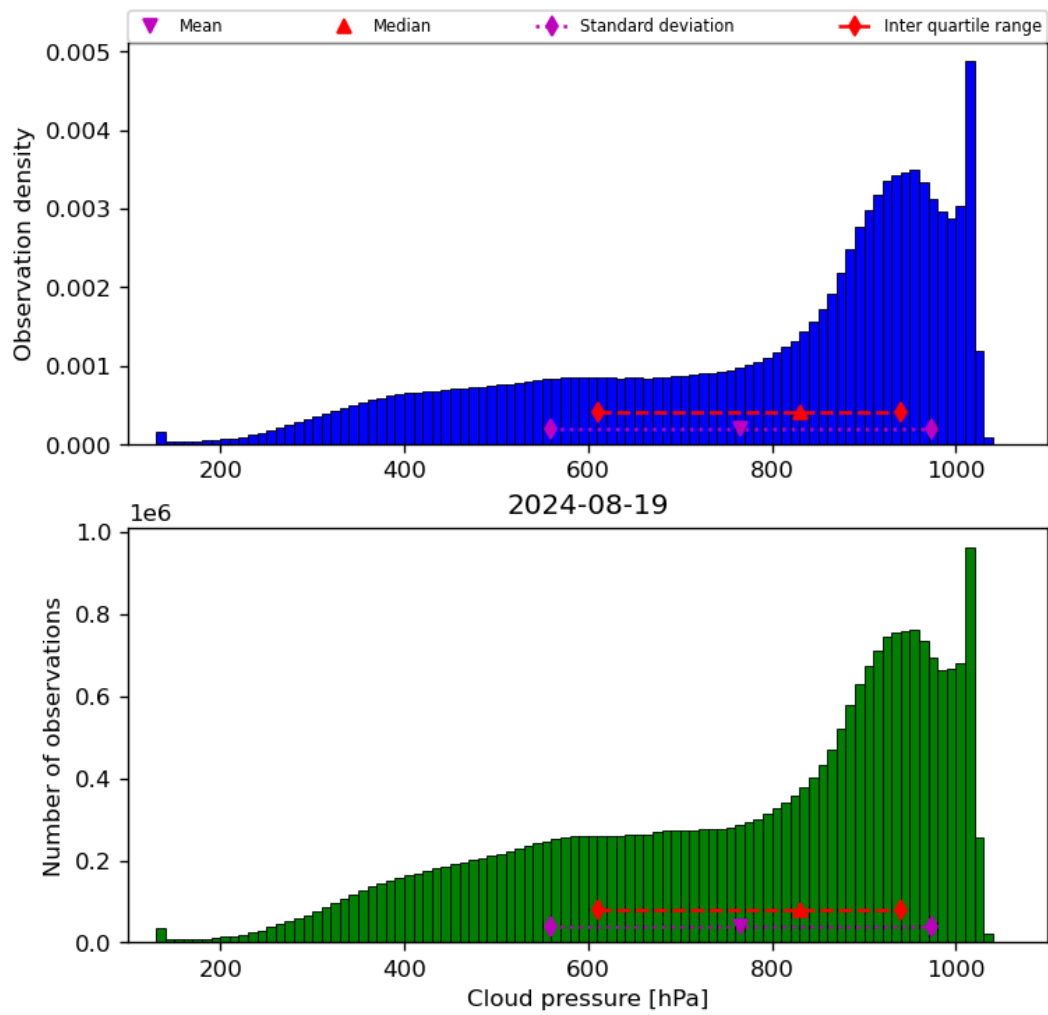
Figure 30: Histogram of “Cloud pressure” for 2024-08-18 to 2024-08-20
