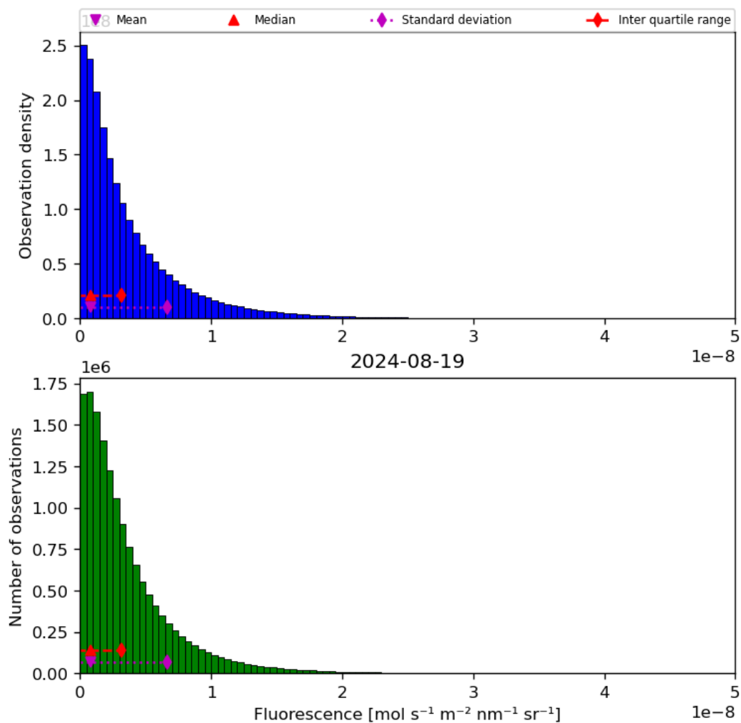
Figure 40: Histogram of “Fluorescence” for 2024-08-18 to 2024-08-20
