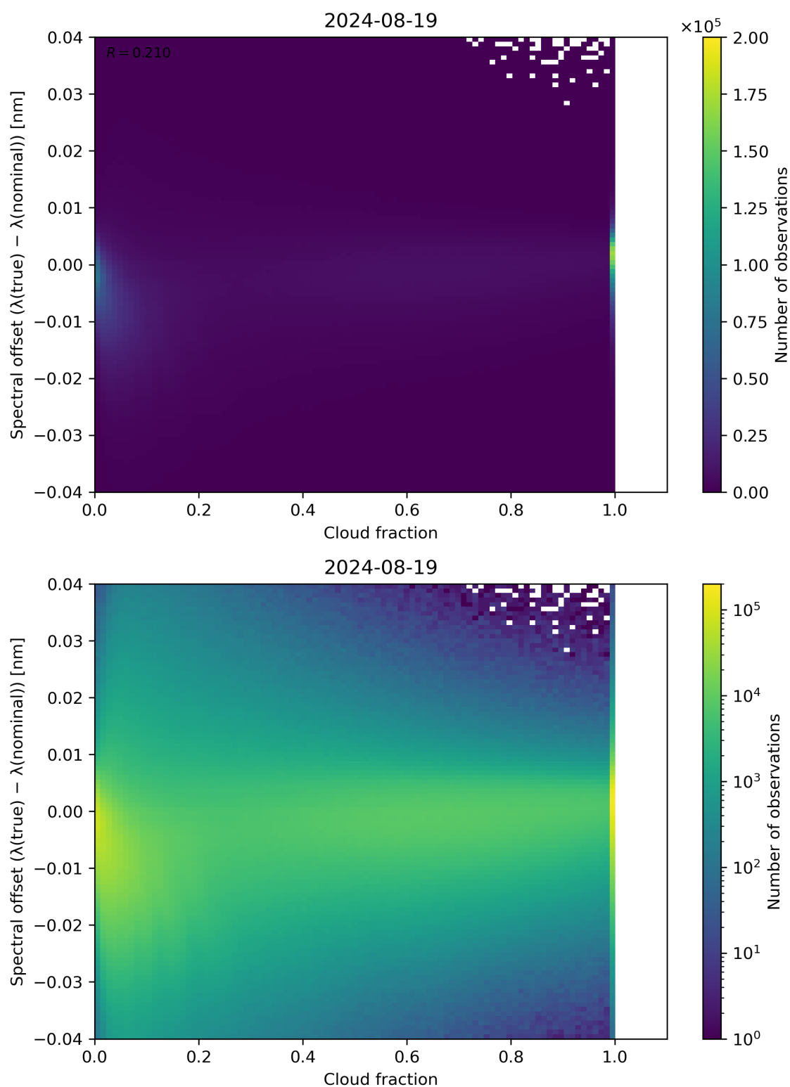
Figure 76: Scatter density plot of “Cloud fraction” against “Spectral offset ( \lambda(\text{true}) - \lambda(\text{nominal}) )” for 2024-08-18 to 2024-08-20.
