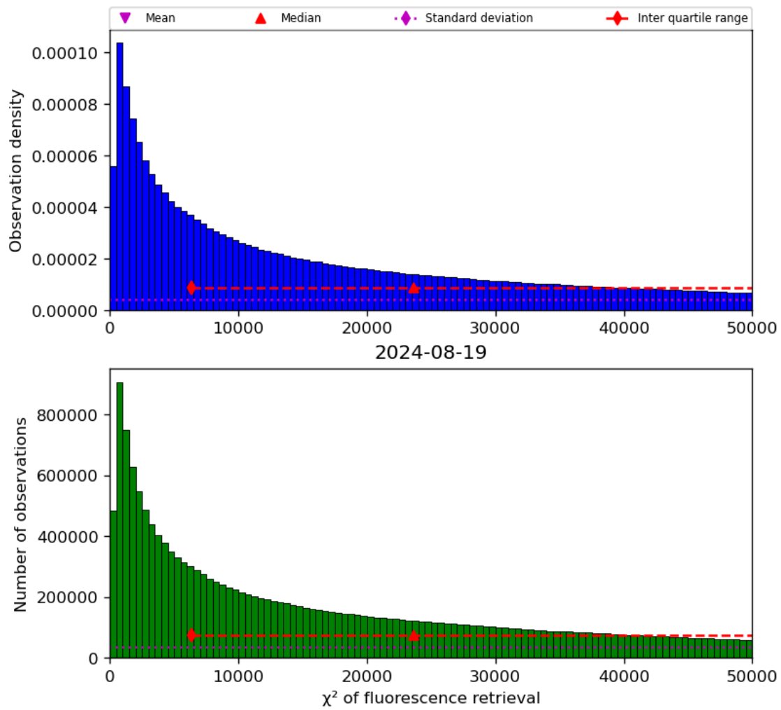
Figure 42: Histogram of “ \chi^2 of fluorescence retrieval” for 2024-08-18 to 2024-08-20
