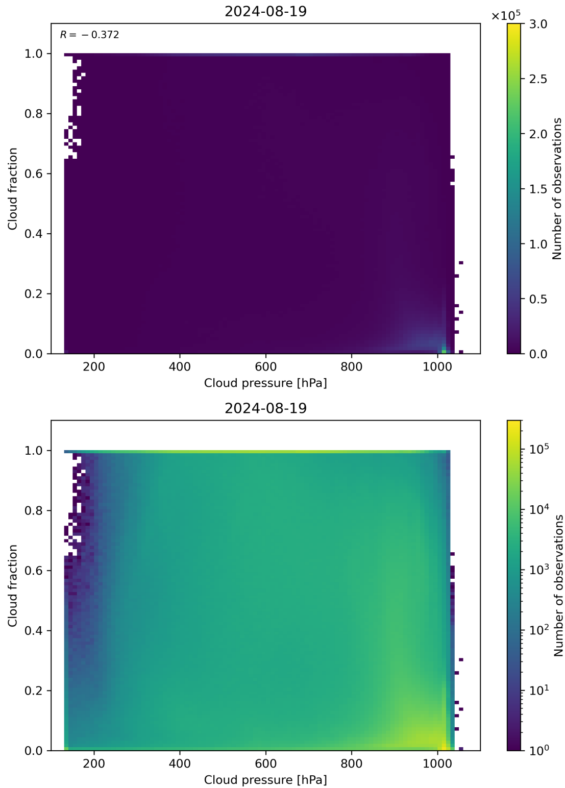
Figure 79: Scatter density plot of “Cloud pressure” against “Cloud fraction” for 2024-08-18 to 2024-08-20.
