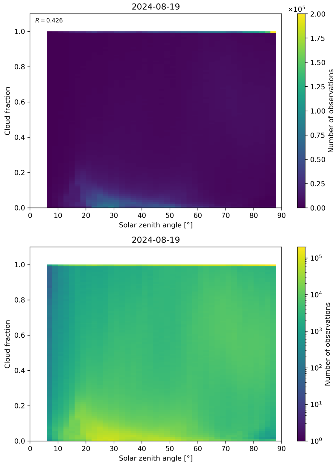
Figure 110: Scatter density plot of “Solar zenith angle” against “Cloud fraction” for 2024-08-18 to 2024-08-20.
