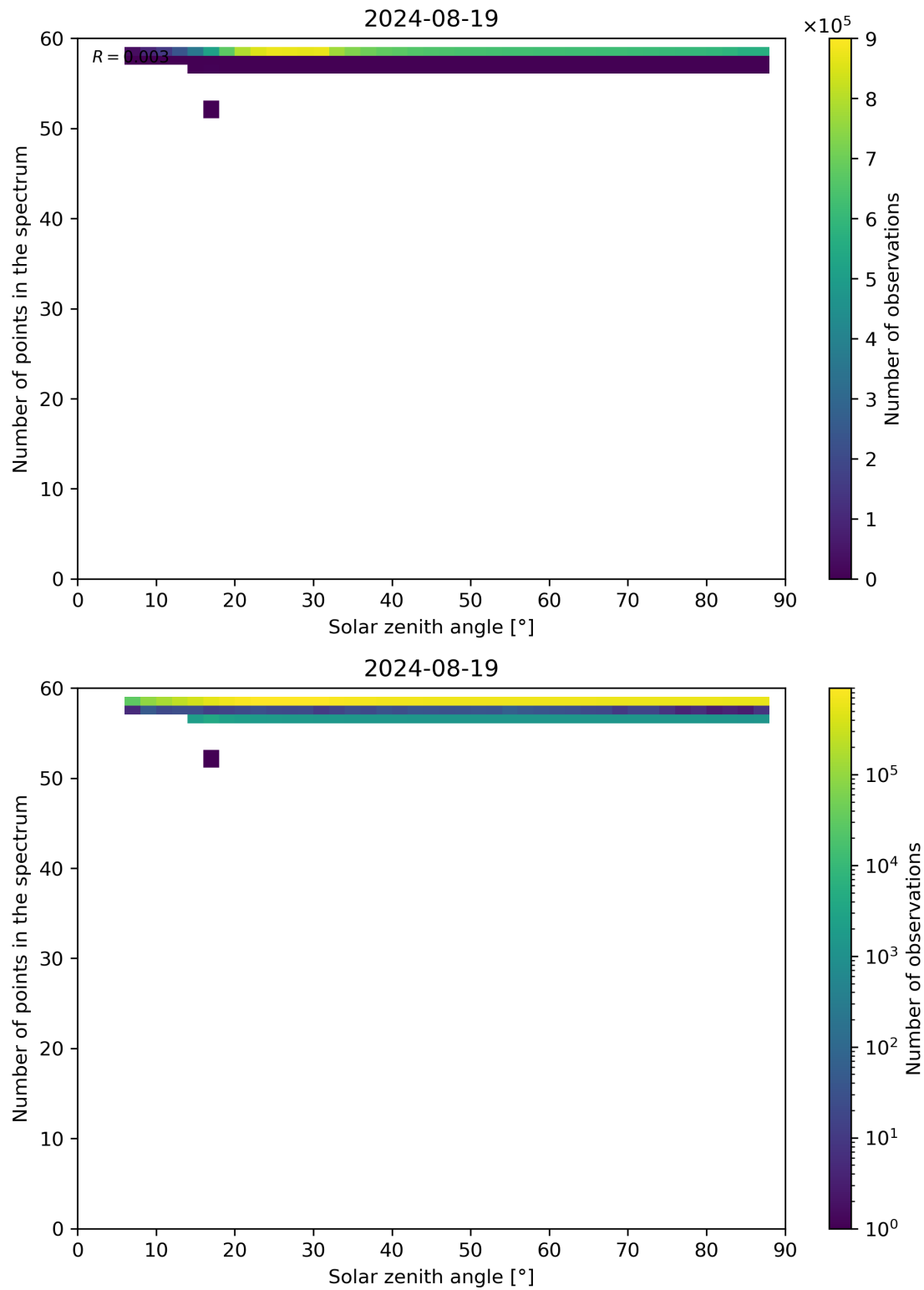
Figure 115: Scatter density plot of “Solar zenith angle” against “Number of points in the spectrum” for 2024-08-18 to 2024-08-20.
