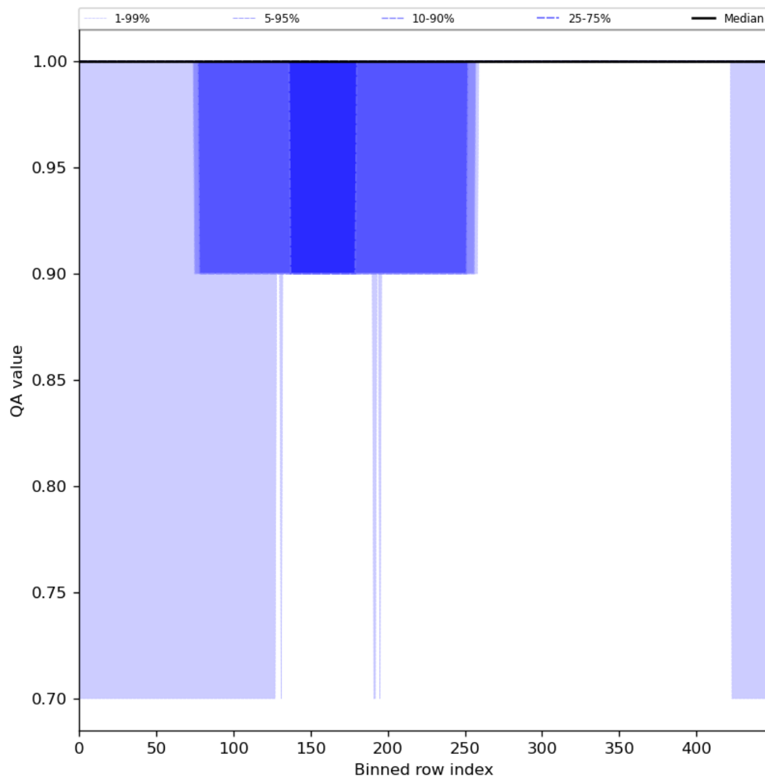
Figure 46: Along track statistics of “QA value” for 2024-08-18 to 2024-08-20
