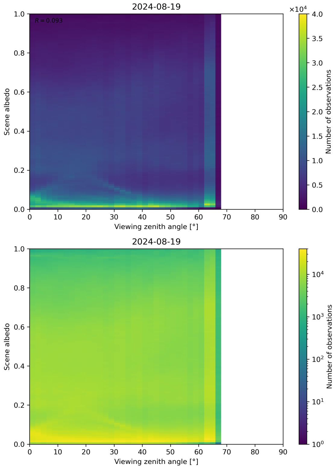
Figure 126: Scatter density plot of “Viewing zenith angle” against “Scene albedo” for 2024-08-18 to 2024-08-20.
