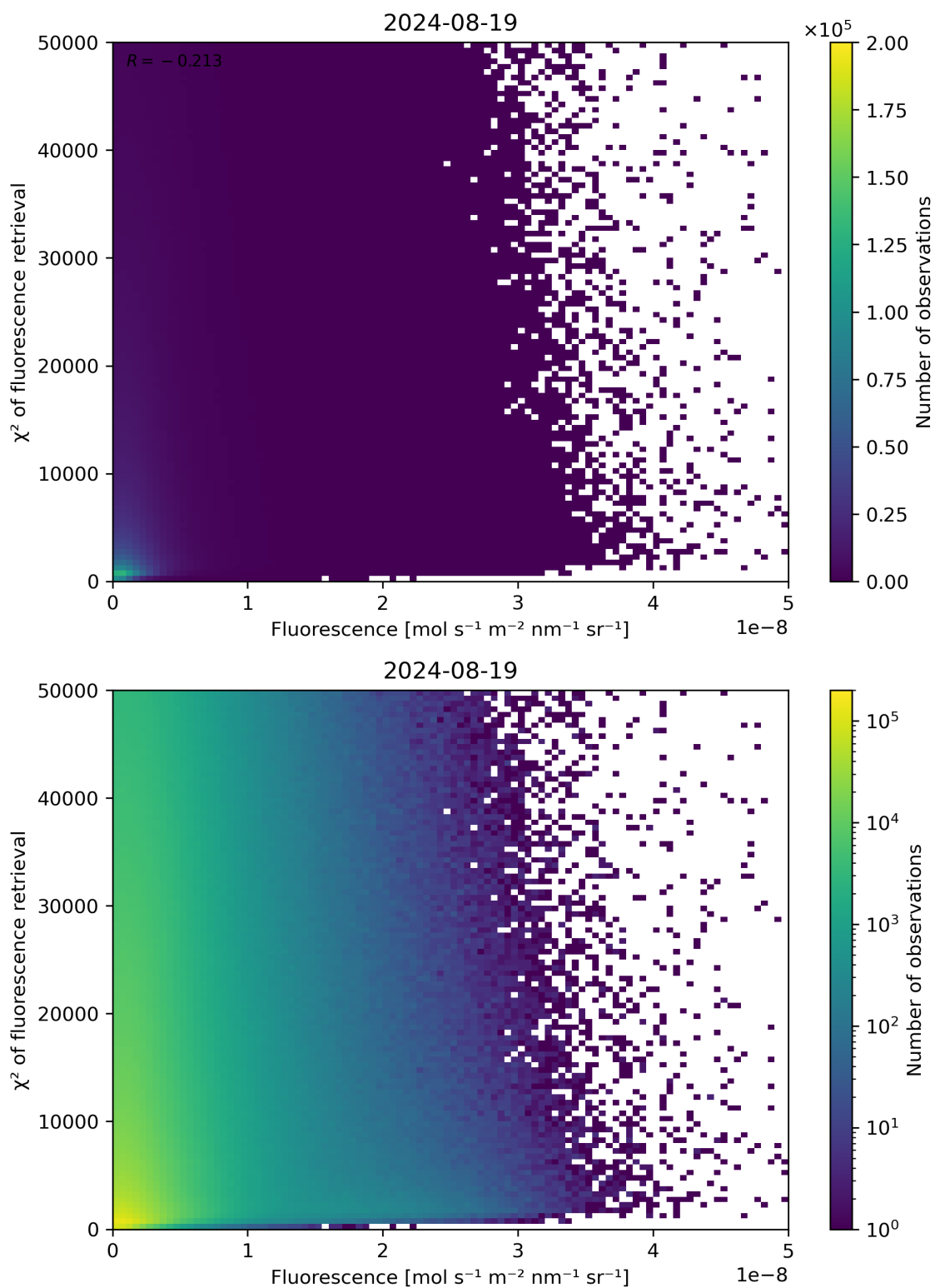
Figure 85: Scatter density plot of “Fluorescence” against “ \chi^2 of fluorescence retrieval” for 2024-08-18 to 2024-08-20.
