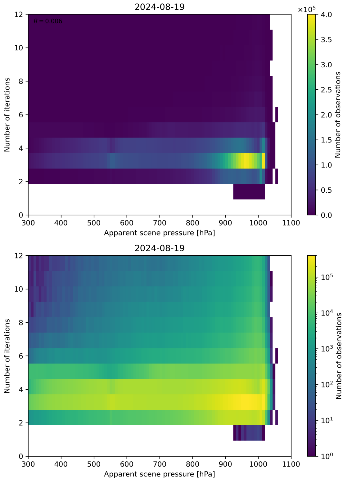
Figure 65: Scatter density plot of “Apparent scene pressure” against “Number of iterations” for 2024-08-18 to 2024-08-20.
