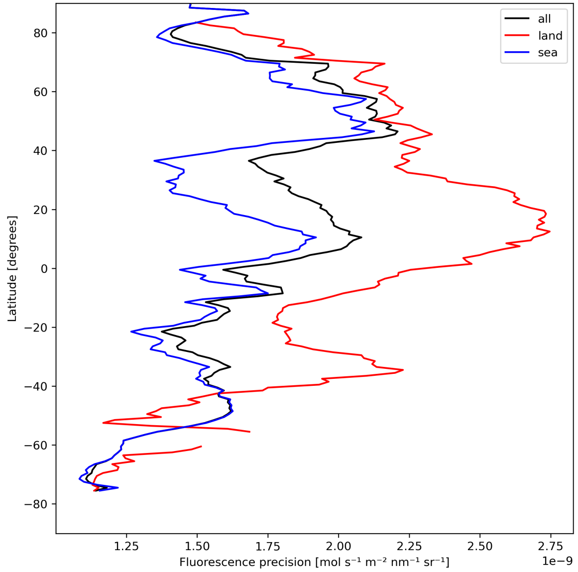
Figure 24: Zonal average of “Fluorescence precision” for 2024-08-18 to 2024-08-20.
