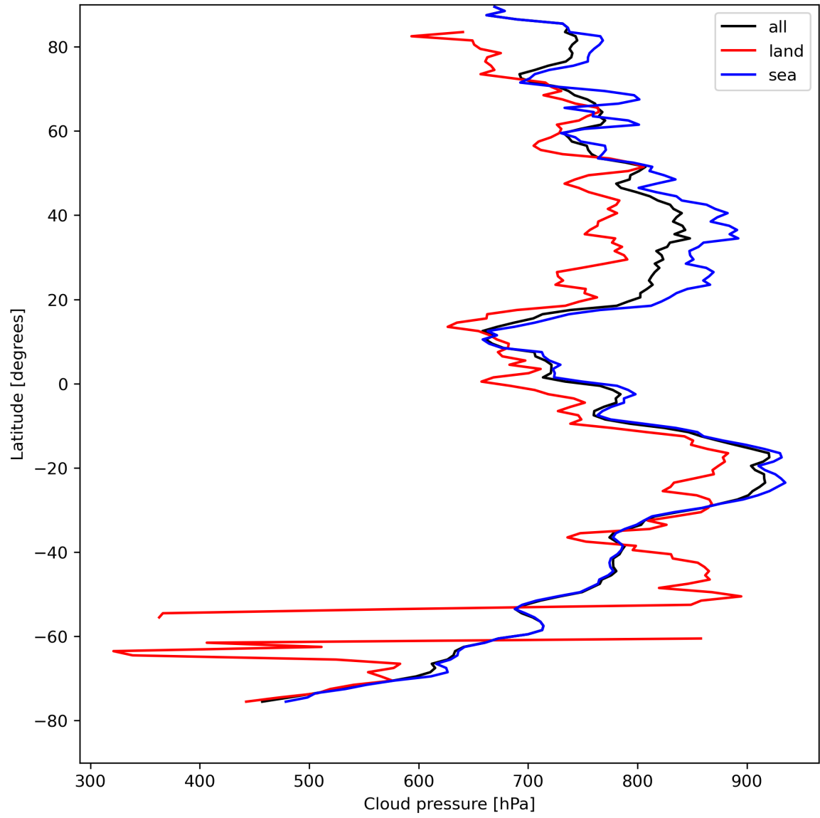
Figure 13: Zonal average of “Cloud pressure” for 2024-08-18 to 2024-08-20.
