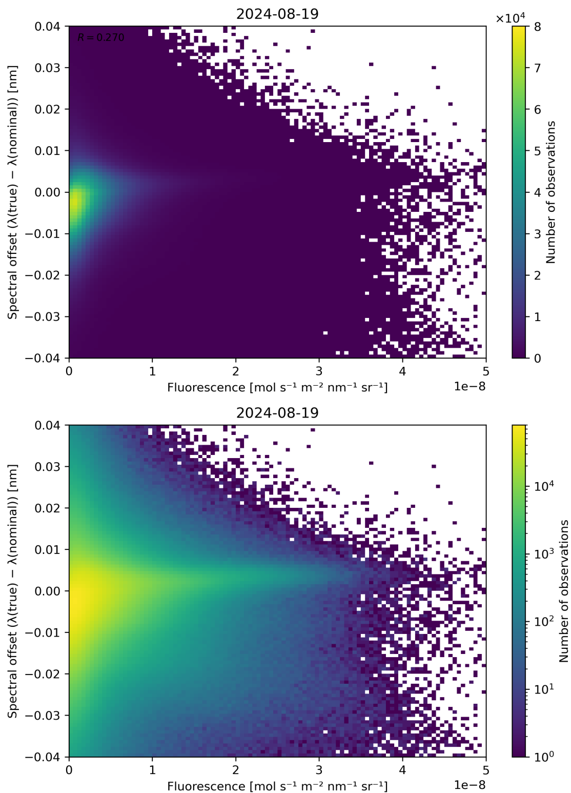
Figure 87: Scatter density plot of “Fluorescence” against “Spectral offset ( \lambda(\text{true}) - \lambda(\text{nominal}) )” for 2024-08-18 to 2024-08-20.
