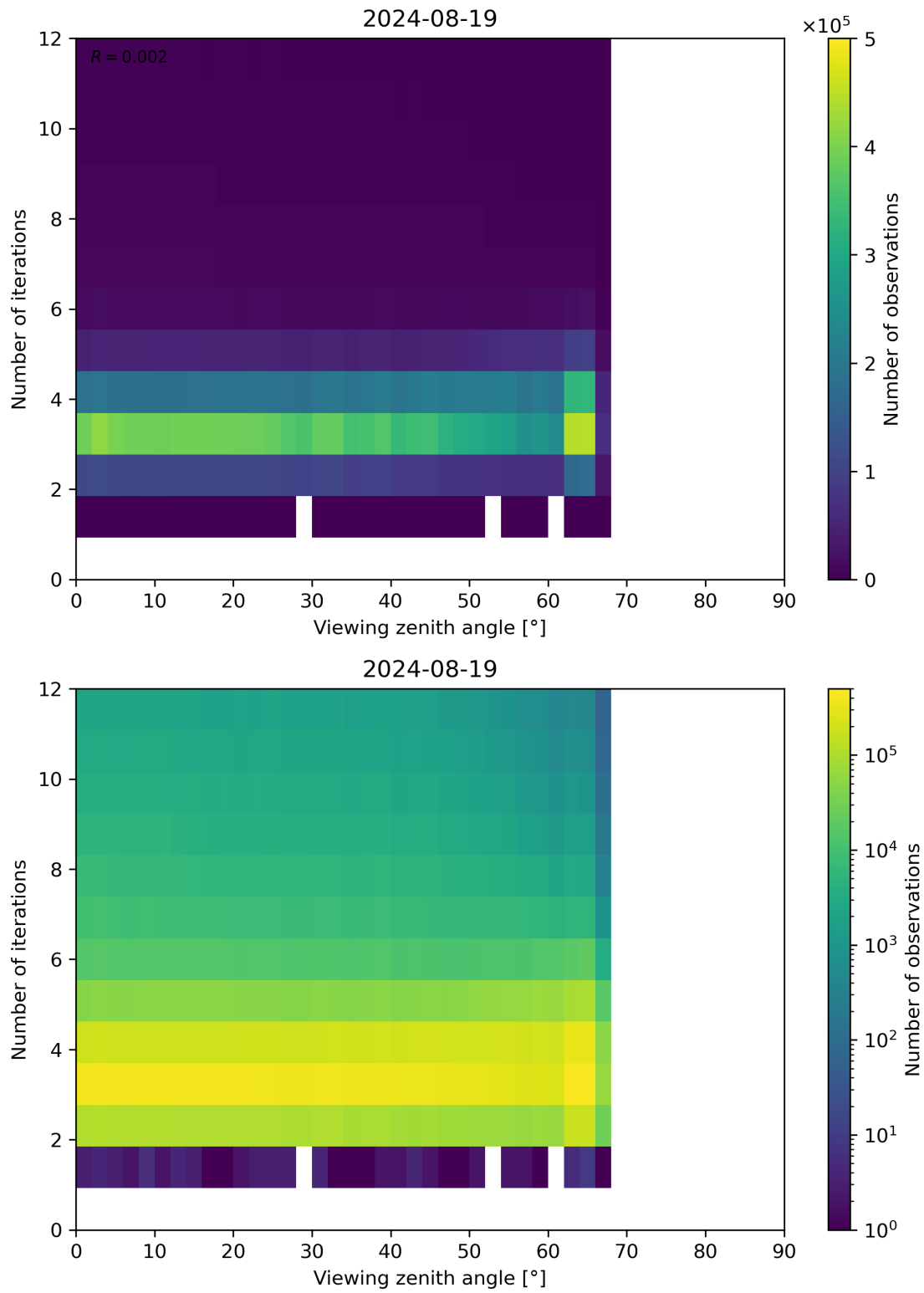
Figure 124: Scatter density plot of “Viewing zenith angle” against “Number of iterations” for 2024-08-18 to 2024-08-20.
