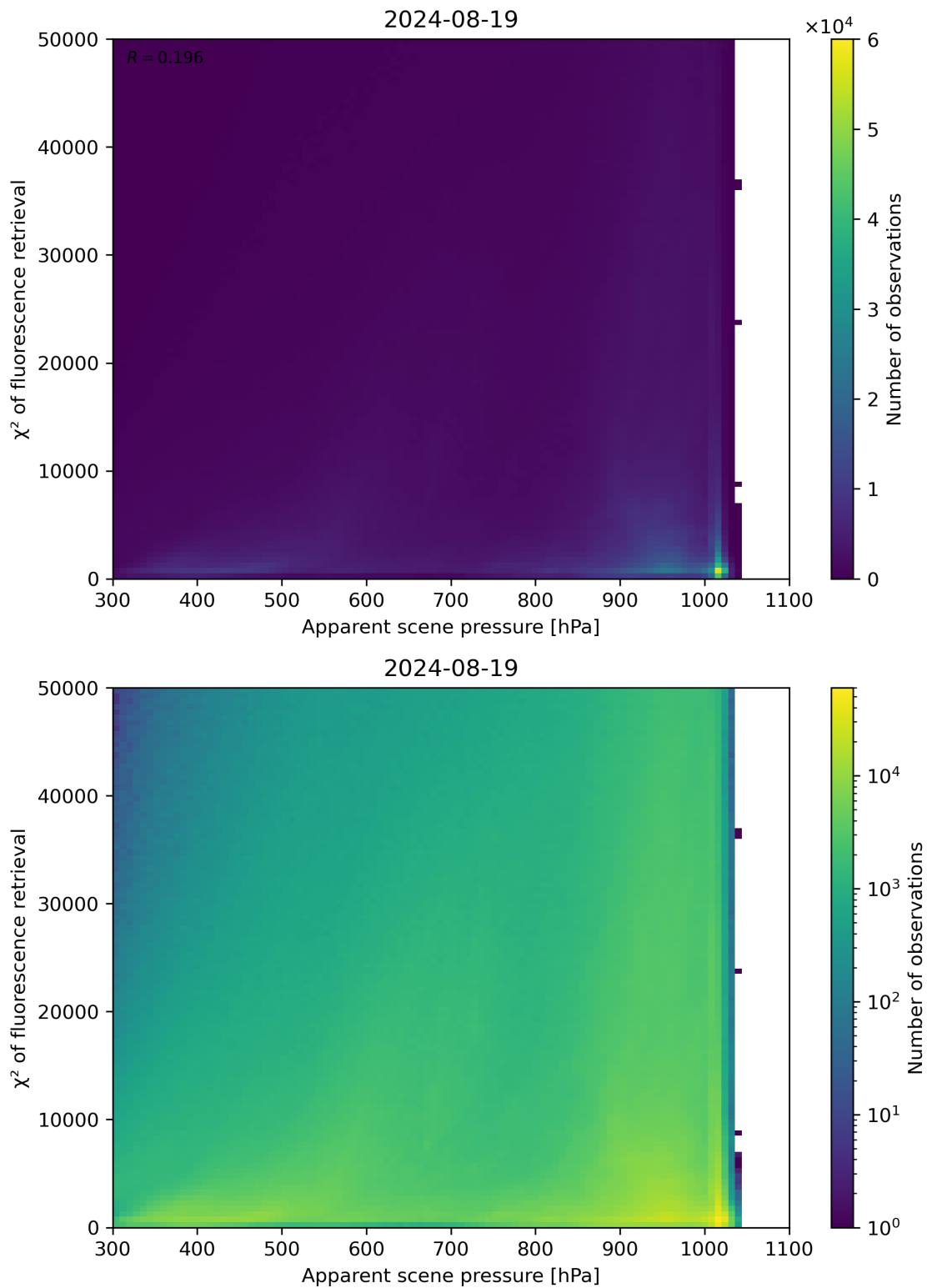
Figure 63: Scatter density plot of “Apparent scene pressure” against “ \chi^2 of fluorescence retrieval” for 2024-08-18 to 2024-08-20.
