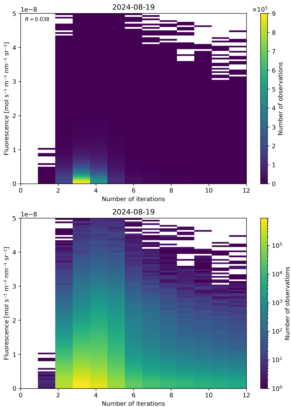
Figure 98: Scatter density plot of “Number of iterations” against “Fluorescence” for 2024-08-18 to 2024-08-20.
