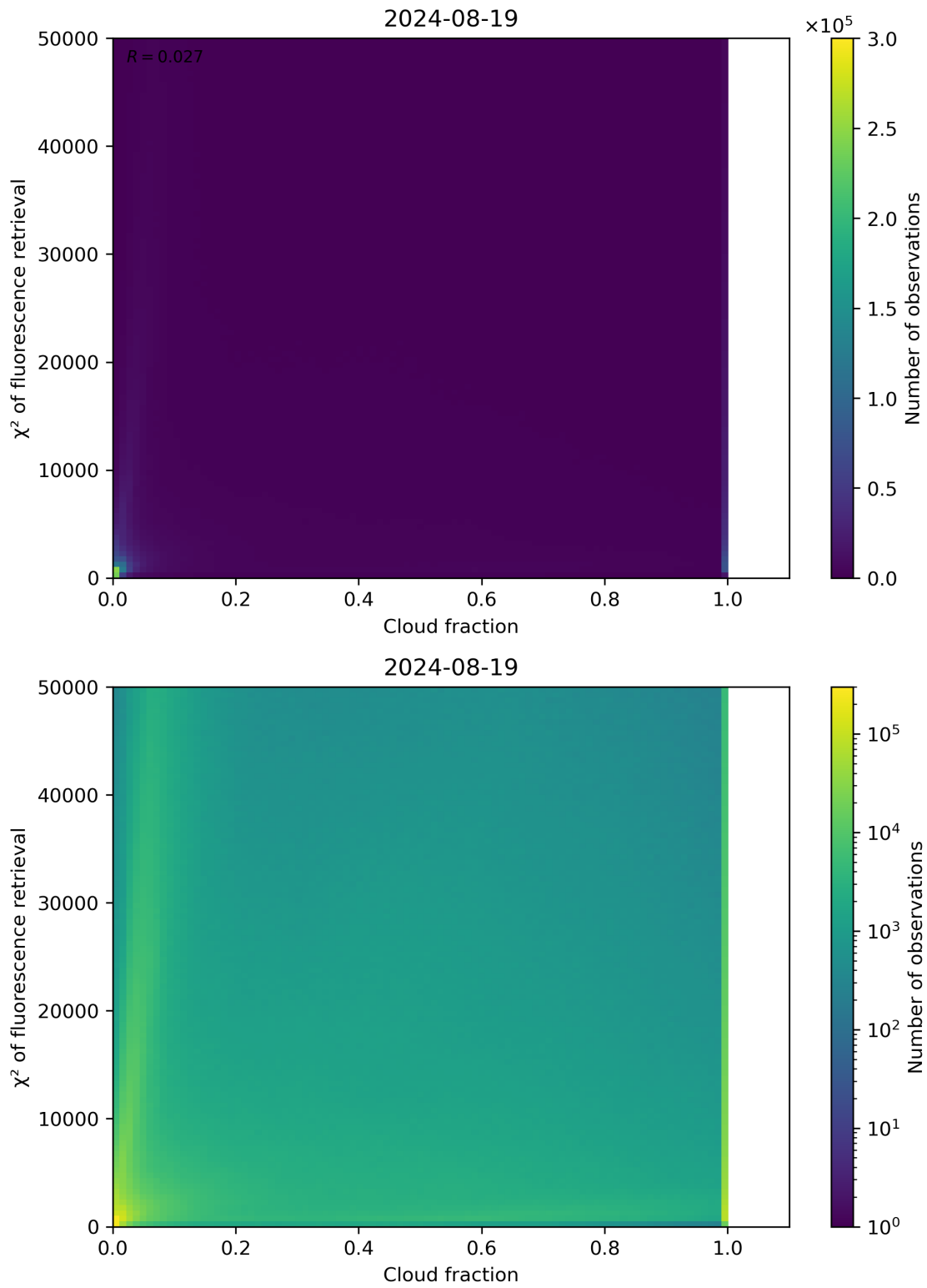
Figure 71: Scatter density plot of “Cloud fraction” against “ \chi^2 of fluorescence retrieval” for 2024-08-18 to 2024-08-20.
