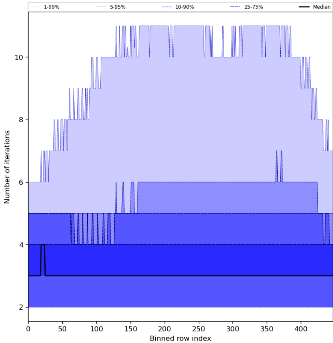
Figure 56: Along track statistics of “Number of iterations” for 2024-08-18 to 2024-08-20
