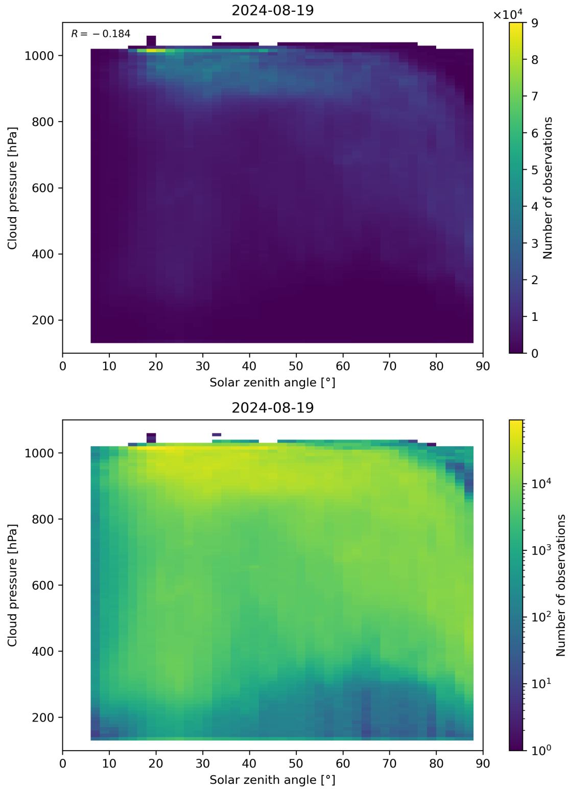
Figure 111: Scatter density plot of “Solar zenith angle” against “Cloud pressure” for 2024-08-18 to 2024-08-20.
