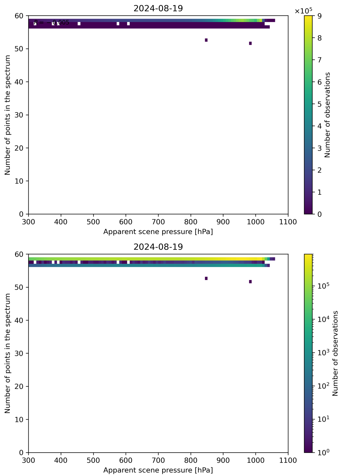
Figure 66: Scatter density plot of “Apparent scene pressure” against “Number of points in the spectrum” for 2024-08-18 to 2024-08-20.
