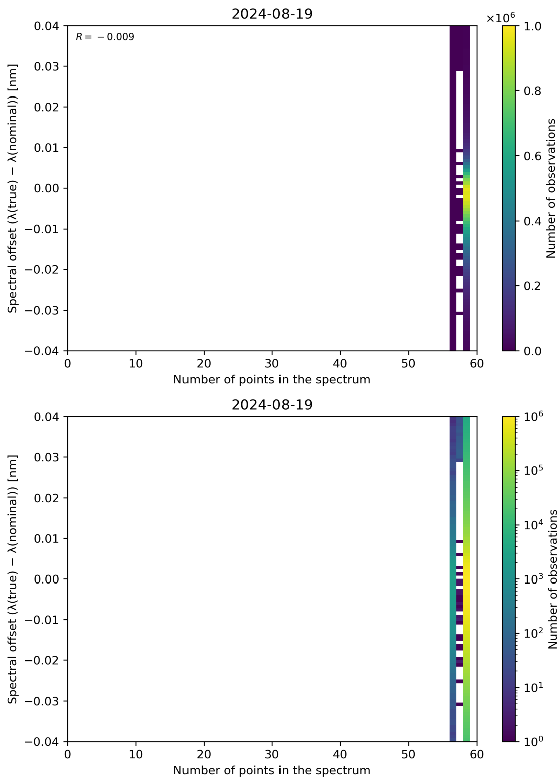
Figure 101: Scatter density plot of “Number of points in the spectrum” against “Spectral offset ( \lambda(\text{true}) - \lambda(\text{nominal}) )” for 2024-08-18 to 2024-08-20.
