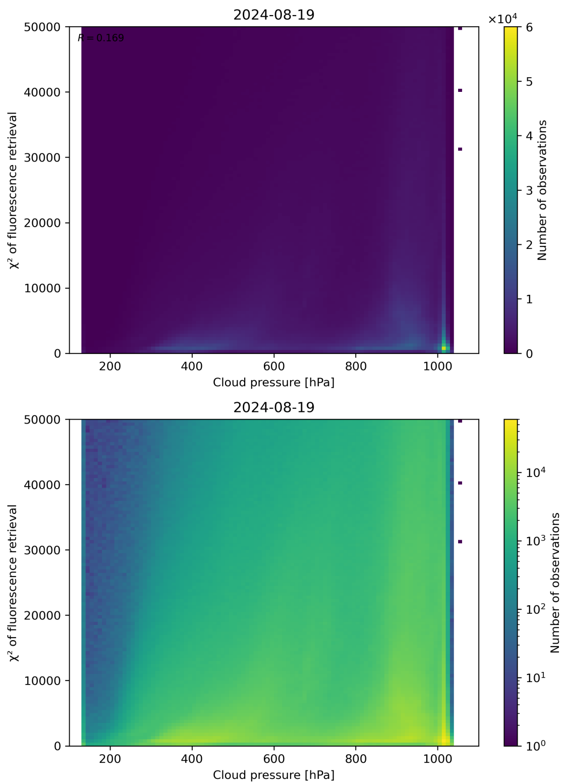
Figure 78: Scatter density plot of “Cloud pressure” against “ \chi^2 of fluorescence retrieval” for 2024-08-18 to 2024-08-20.
