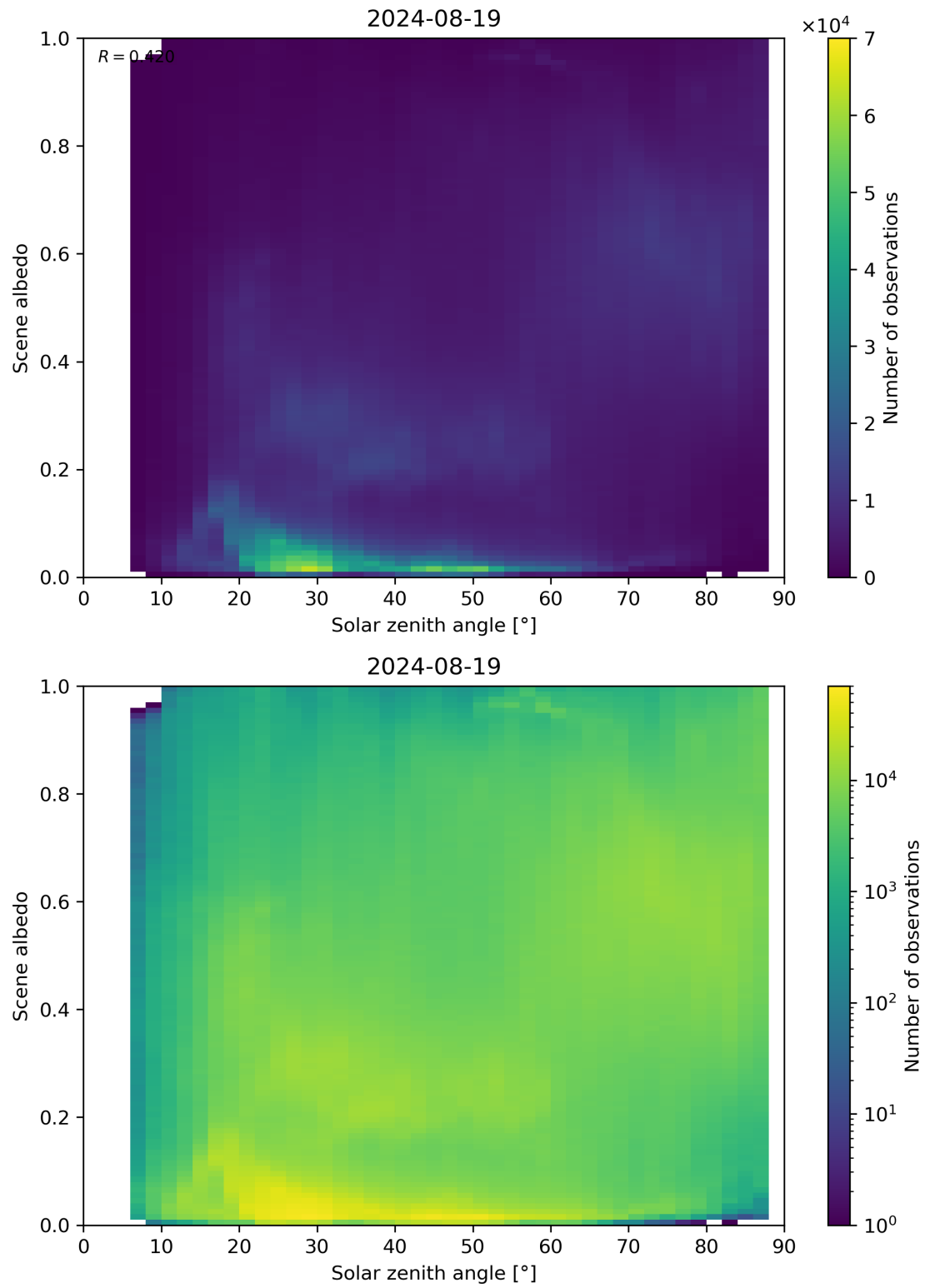
Figure 116: Scatter density plot of “Solar zenith angle” against “Scene albedo” for 2024-08-18 to 2024-08-20.
