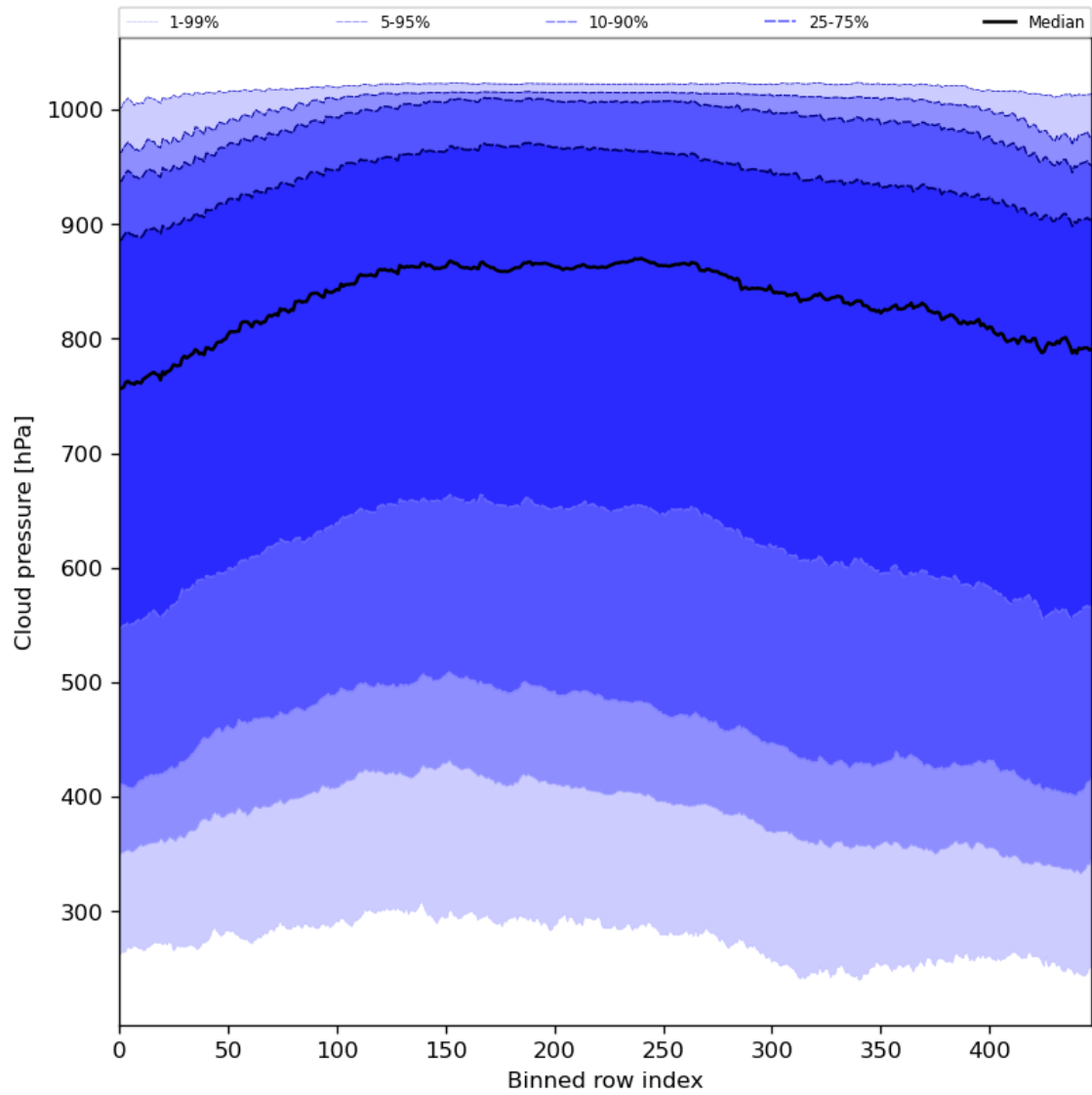
Figure 47: Along track statistics of “Cloud pressure” for 2024-08-19 to 2024-08-21
