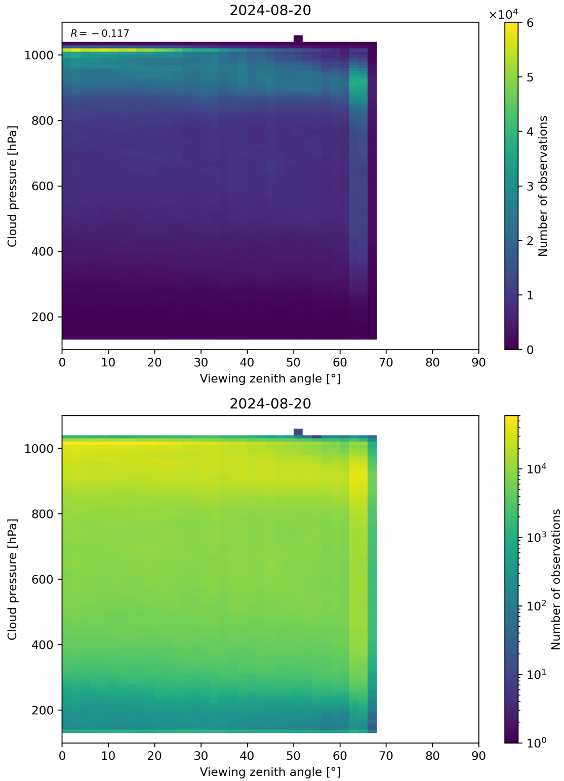
Figure 121: Scatter density plot of “Viewing zenith angle” against “Cloud pressure” for 2024-08-19 to 2024-08-21.
