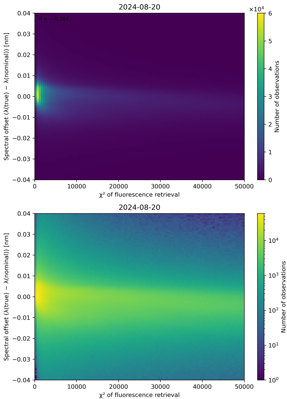
Figure 69: Scatter density plot of " \chi^2 of fluorescence retrieval" against "Spectral offset ( \lambda(\text{true}) - \lambda(\text{nominal})) " for 2024-08-19 to 2024-08-21.
