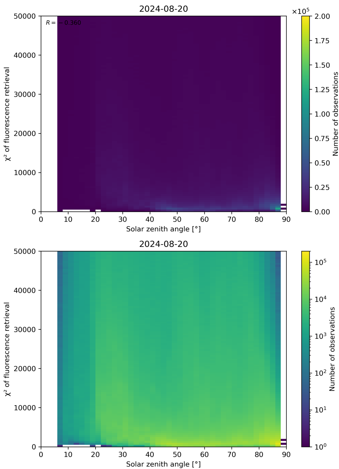
Figure 109: Scatter density plot of “Solar zenith angle” against “ \chi^2 of fluorescence retrieval” for 2024-08-19 to 2024-08-21.
