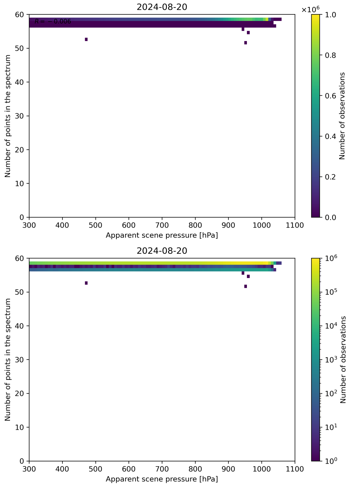
Figure 66: Scatter density plot of “Apparent scene pressure” against “Number of points in the spectrum” for 2024-08-19 to 2024-08-21.
