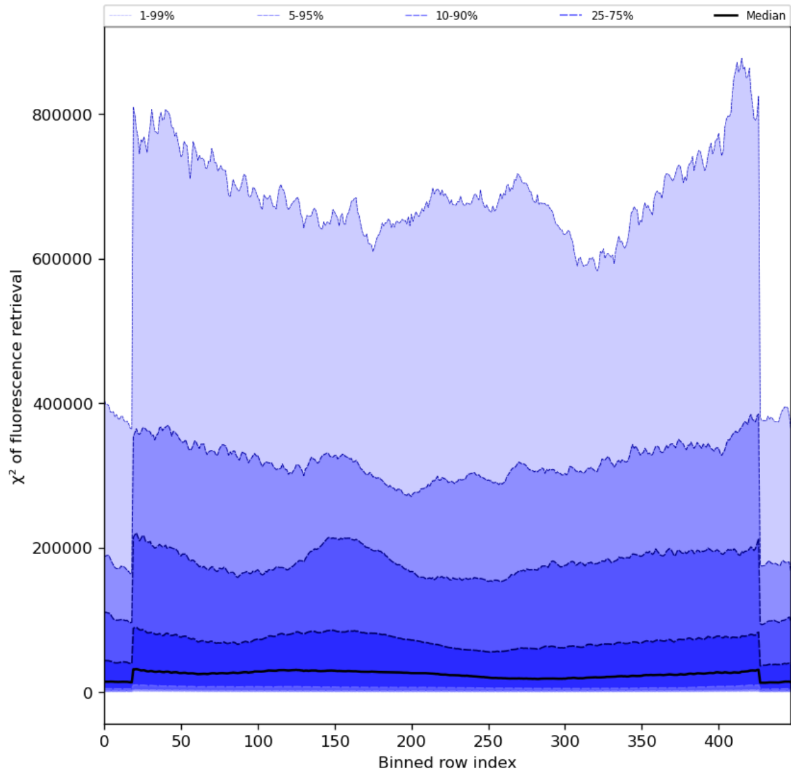
Figure 59: Along track statistics of “ \chi^2 of fluorescence retrieval” for 2024-08-19 to 2024-08-21
