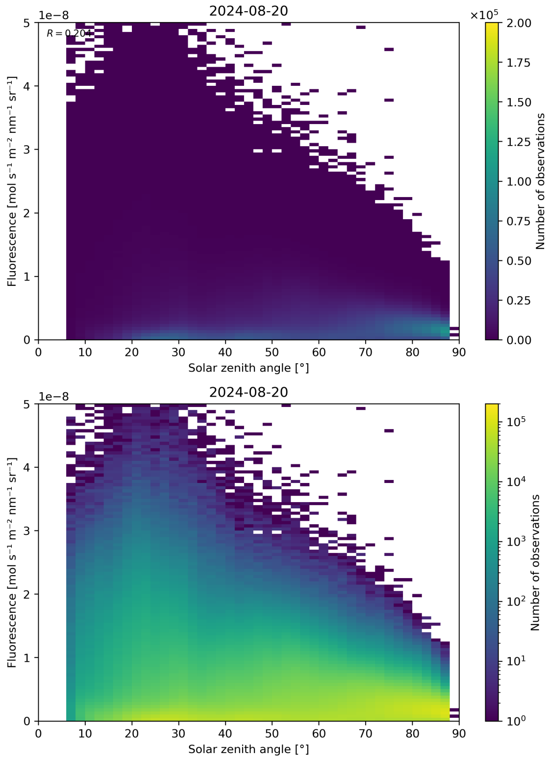
Figure 112: Scatter density plot of “Solar zenith angle” against “Fluorescence” for 2024-08-19 to 2024-08-21.
