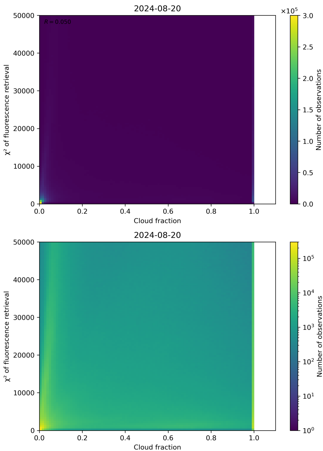
Figure 71: Scatter density plot of “Cloud fraction” against “ \chi^2 of fluorescence retrieval” for 2024-08-19 to 2024-08-21.
