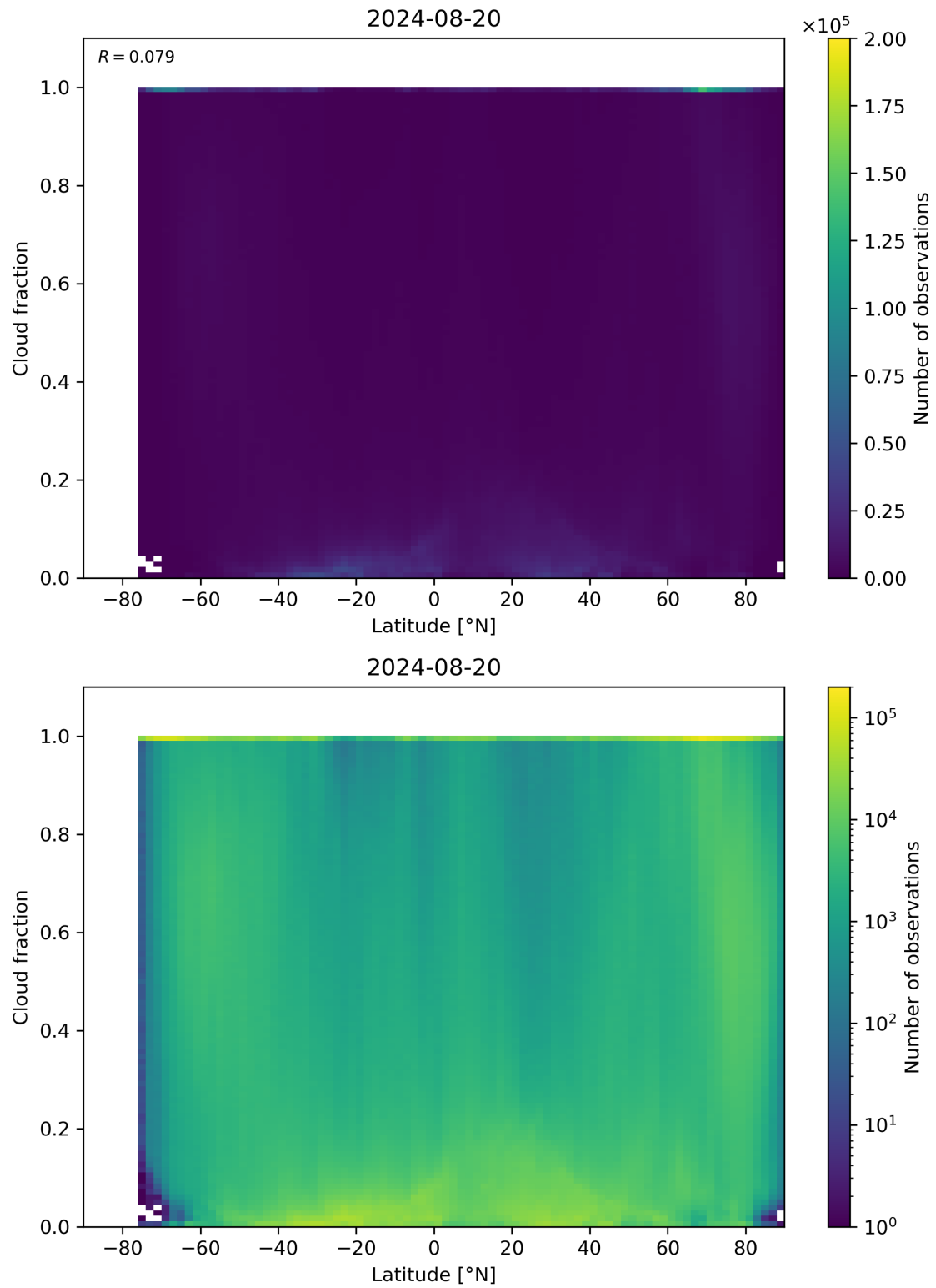
Figure 90: Scatter density plot of “Latitude” against “Cloud fraction” for 2024-08-19 to 2024-08-21.
