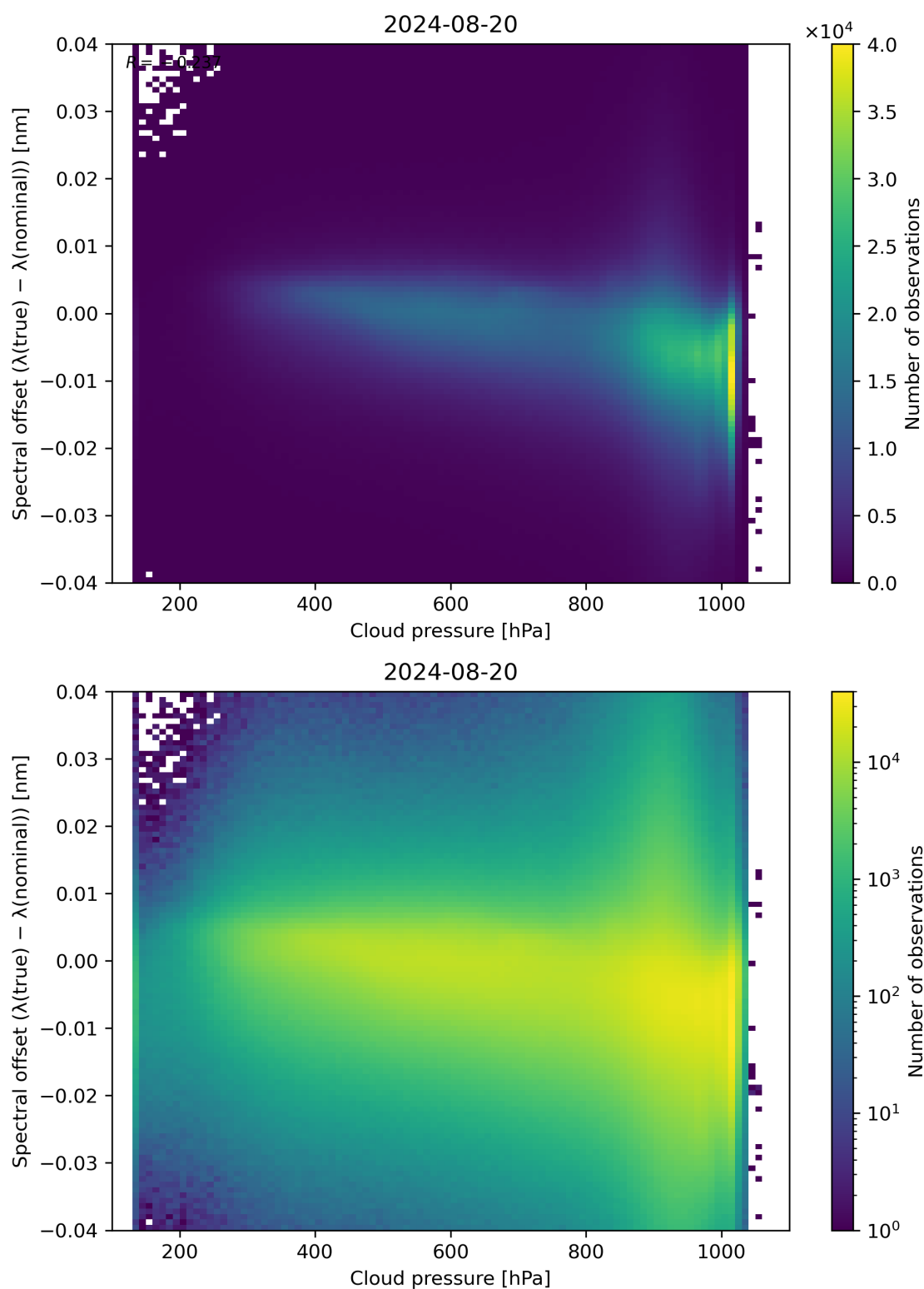
Figure 84: Scatter density plot of “Cloud pressure” against “Spectral offset ( \lambda(\text{true}) - \lambda(\text{nominal}) )” for 2024-08-19 to 2024-08-21.
