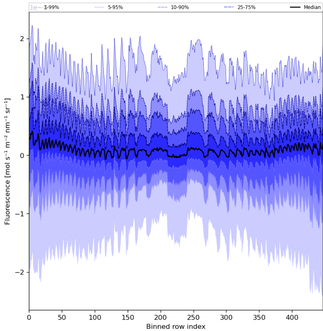
Figure 57: Along track statistics of “Fluorescence” for 2024-08-19 to 2024-08-21
