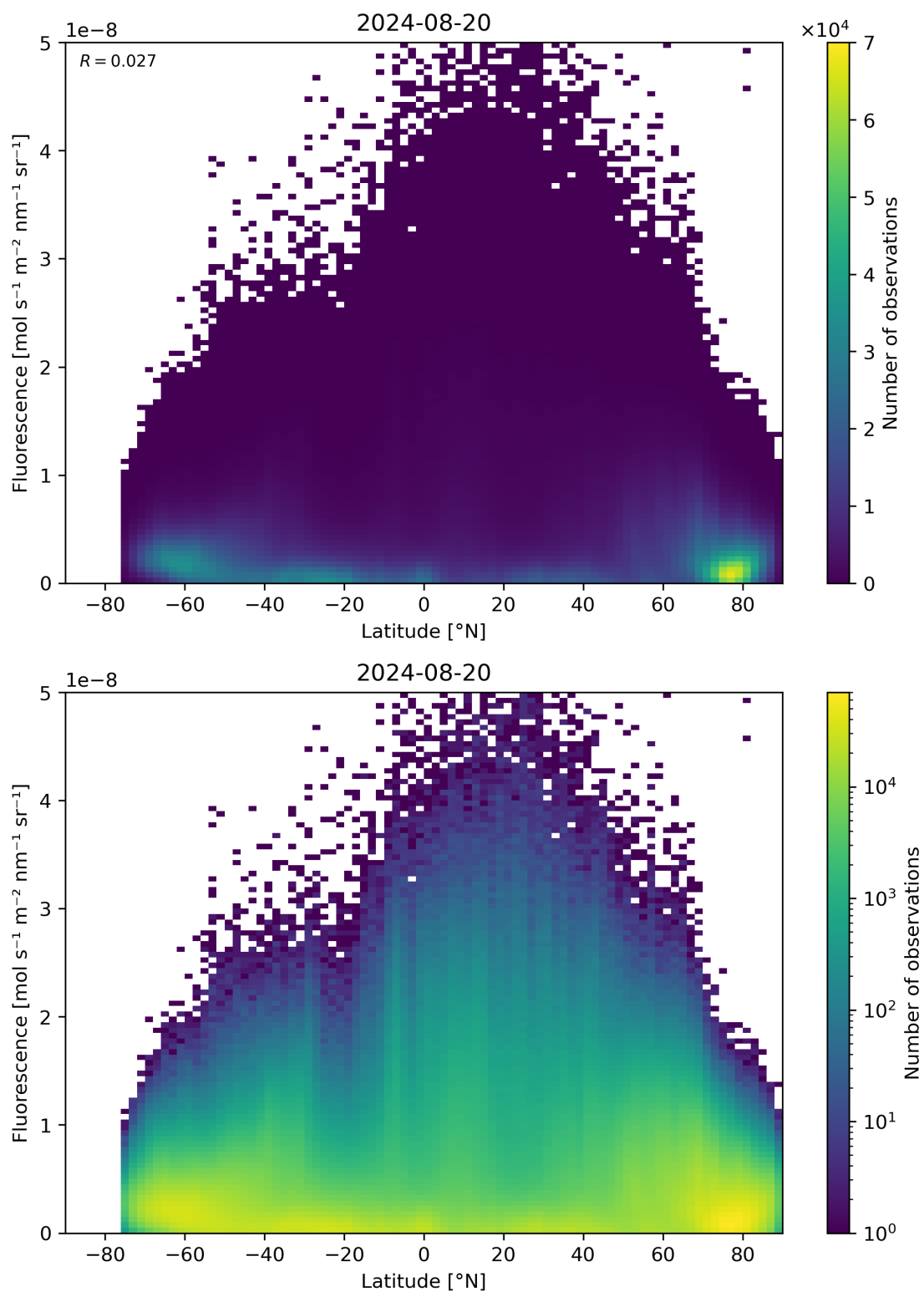
Figure 92: Scatter density plot of “Latitude” against “Fluorescence” for 2024-08-19 to 2024-08-21.
