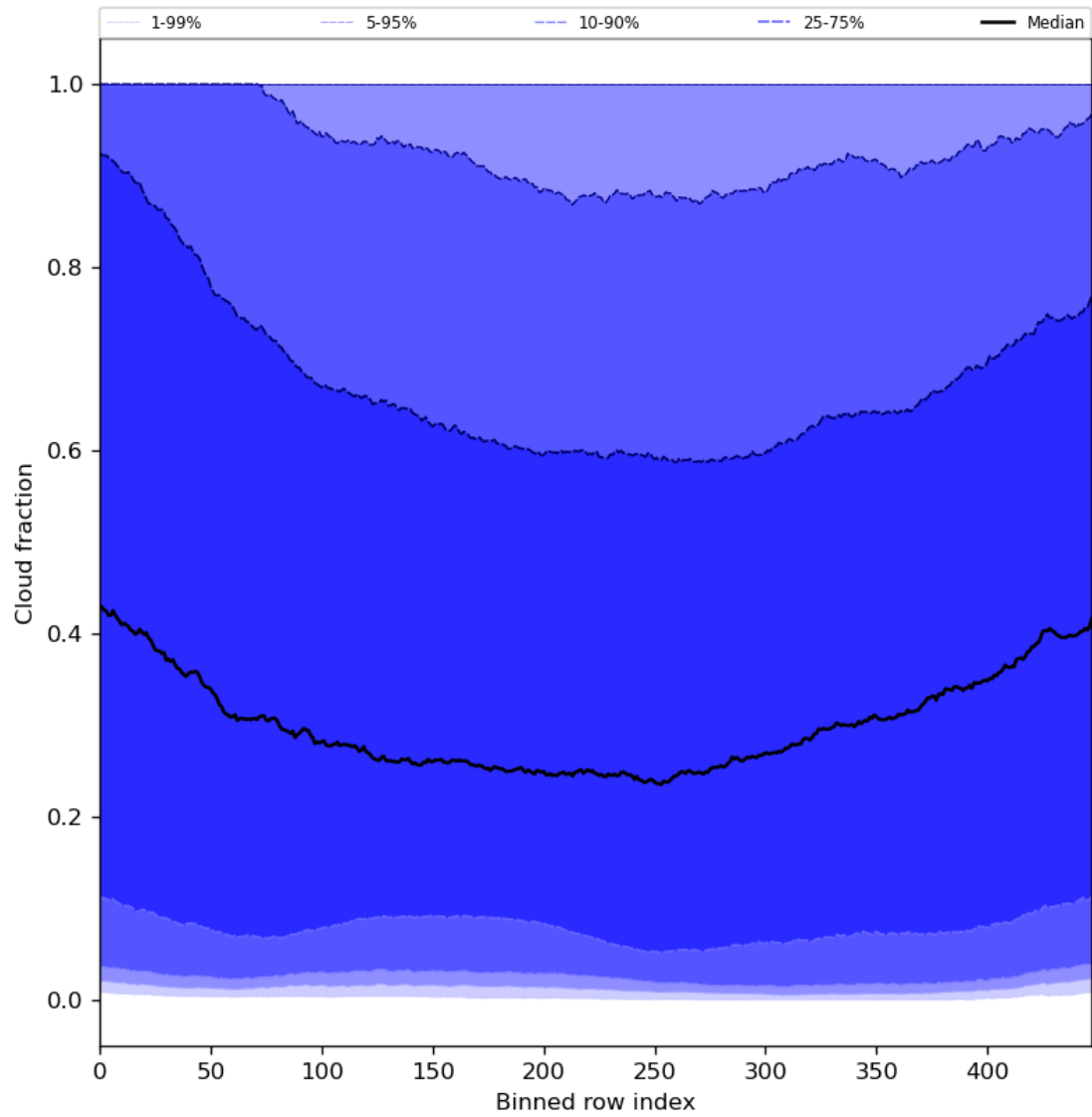
Figure 49: Along track statistics of “Cloud fraction” for 2024-08-19 to 2024-08-21
