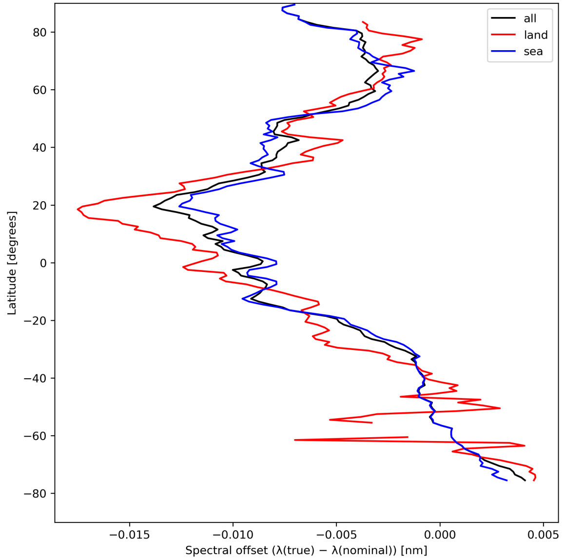
Figure 28: Zonal average of “Spectral offset ( \lambda(\text{true}) - \lambda(\text{nominal}) )” for 2024-08-19 to 2024-08-21.
