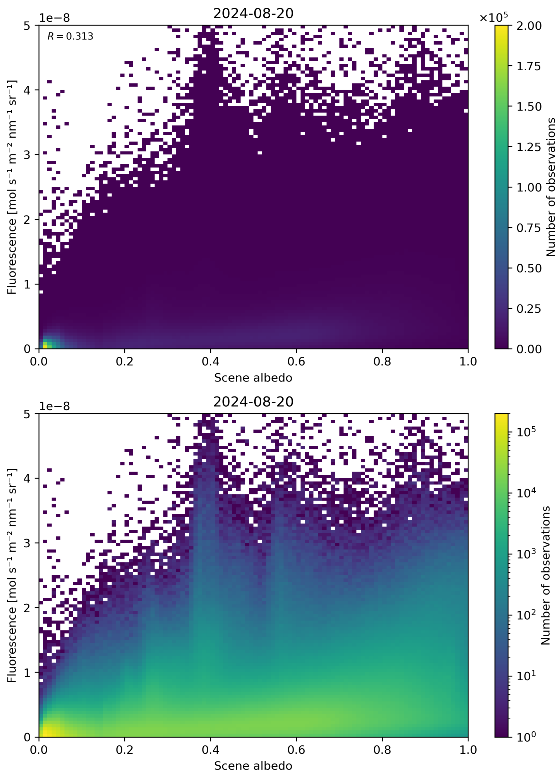
Figure 104: Scatter density plot of “Scene albedo” against “Fluorescence” for 2024-08-19 to 2024-08-21.
