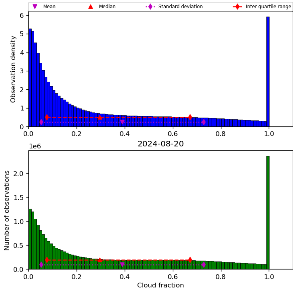
Figure 32: Histogram of “Cloud fraction” for 2024-08-19 to 2024-08-21
