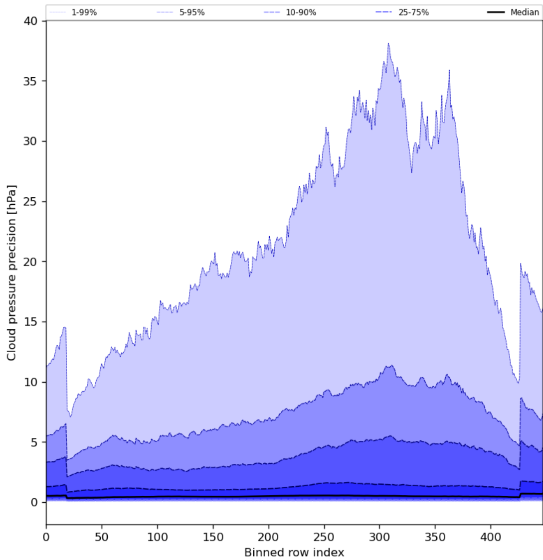
Figure 48: Along track statistics of “Cloud pressure precision” for 2024-08-19 to 2024-08-21
