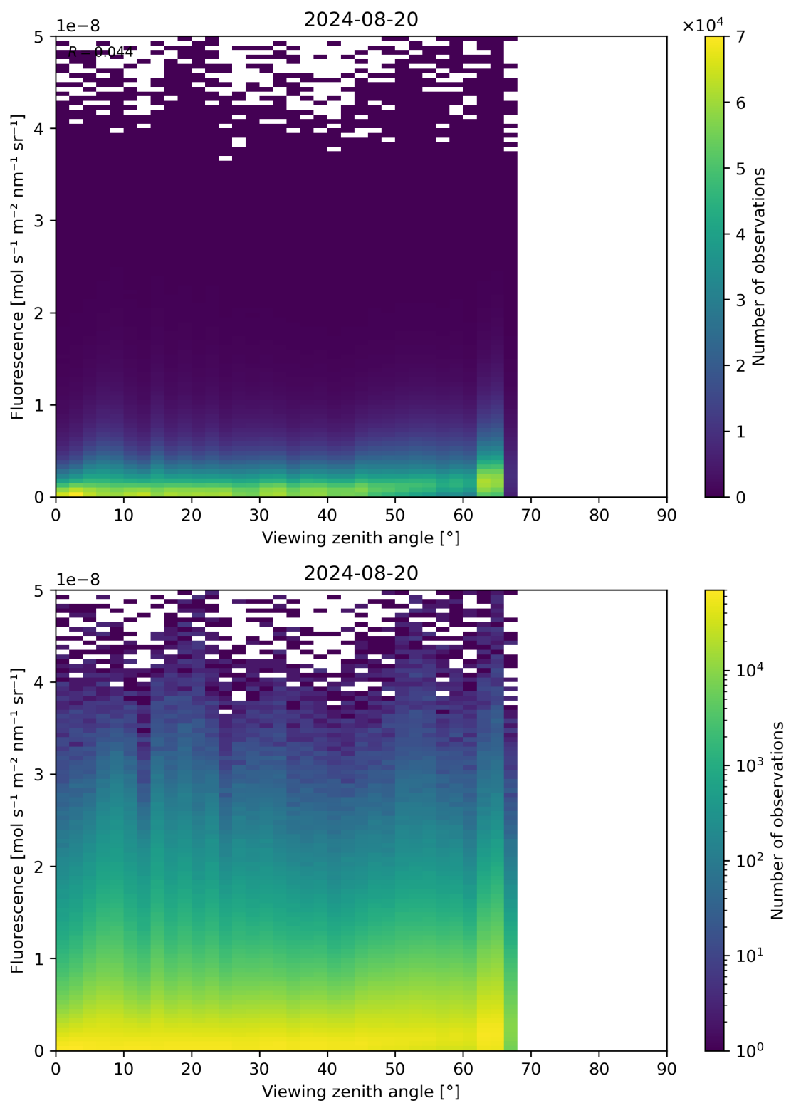
Figure 122: Scatter density plot of “Viewing zenith angle” against “Fluorescence” for 2024-08-19 to 2024-08-21.
