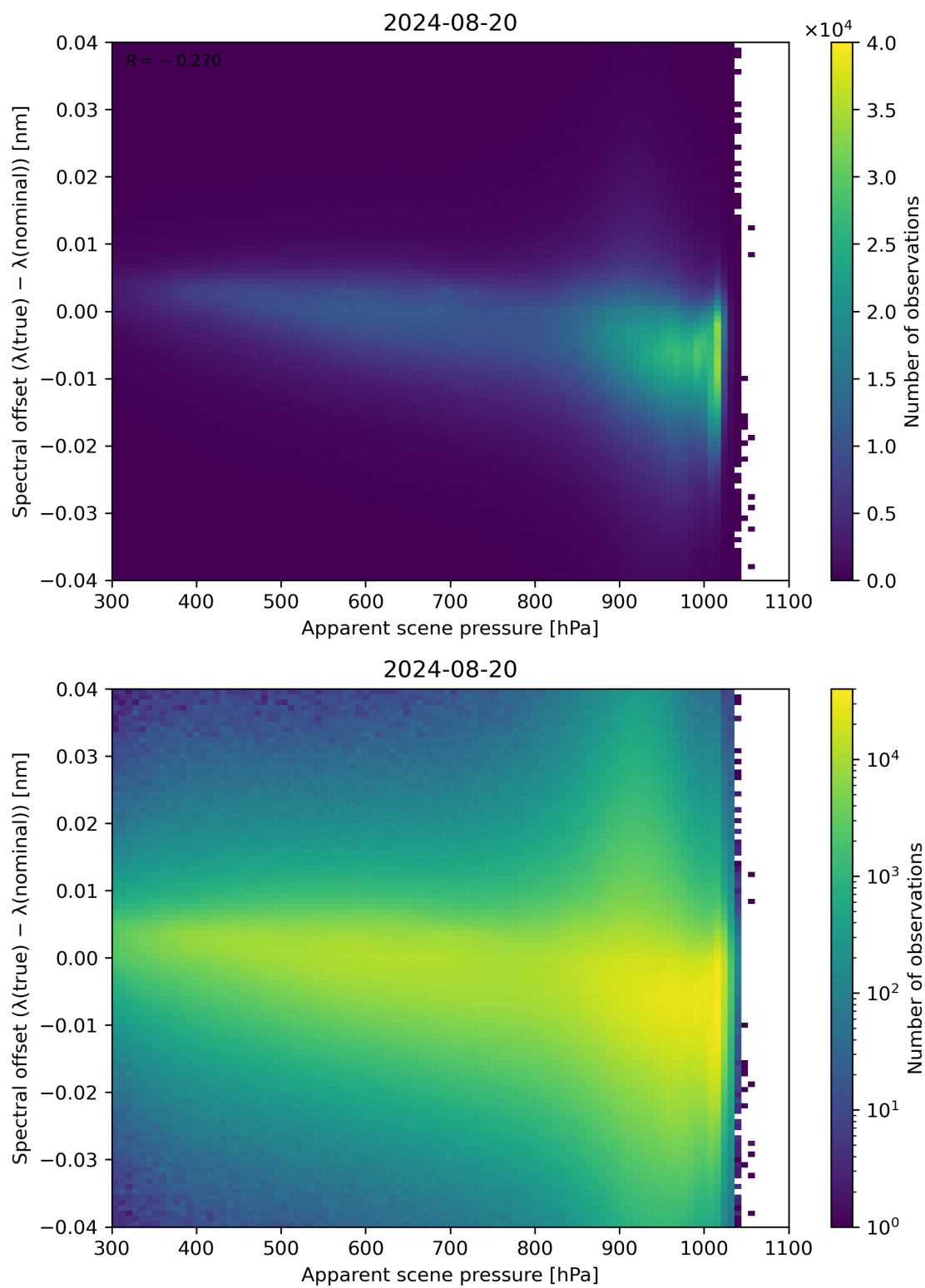
Figure 67: Scatter density plot of “Apparent scene pressure” against “Spectral offset ( \lambda(\text{true}) - \lambda(\text{nominal}) )” for 2024-08-19 to 2024-08-21.
