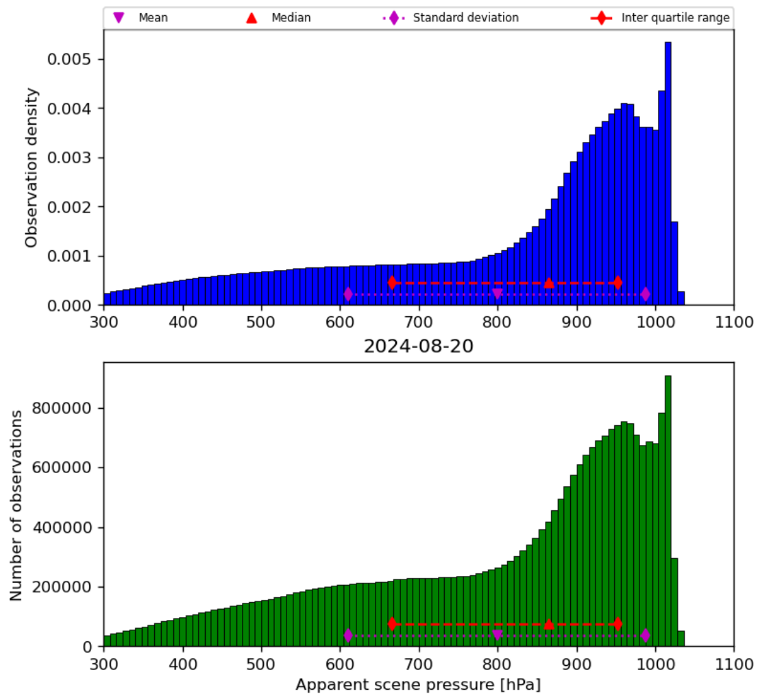
Figure 36: Histogram of “Apparent scene pressure” for 2024-08-19 to 2024-08-21
