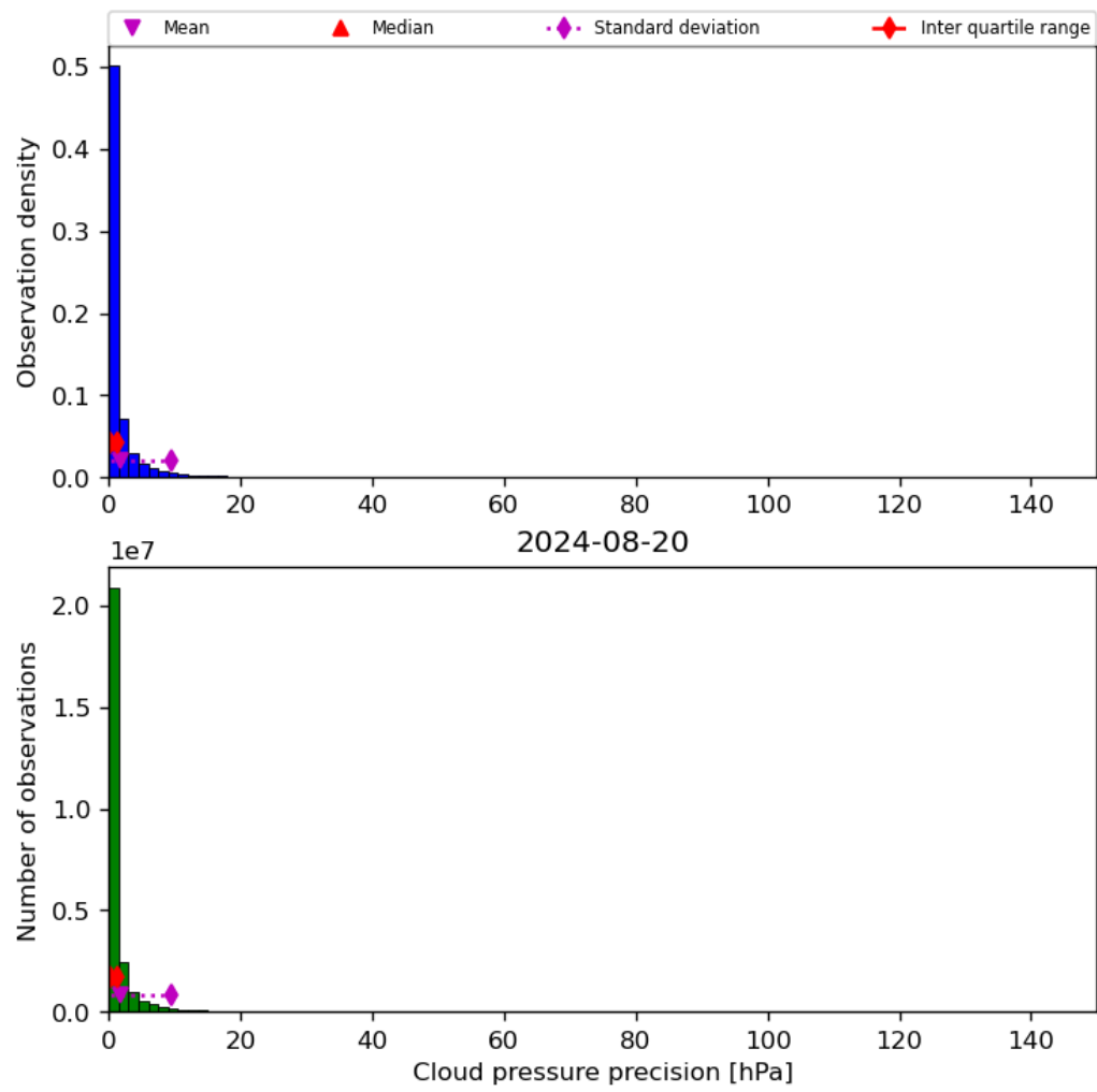
Figure 31: Histogram of “Cloud pressure precision” for 2024-08-19 to 2024-08-21
