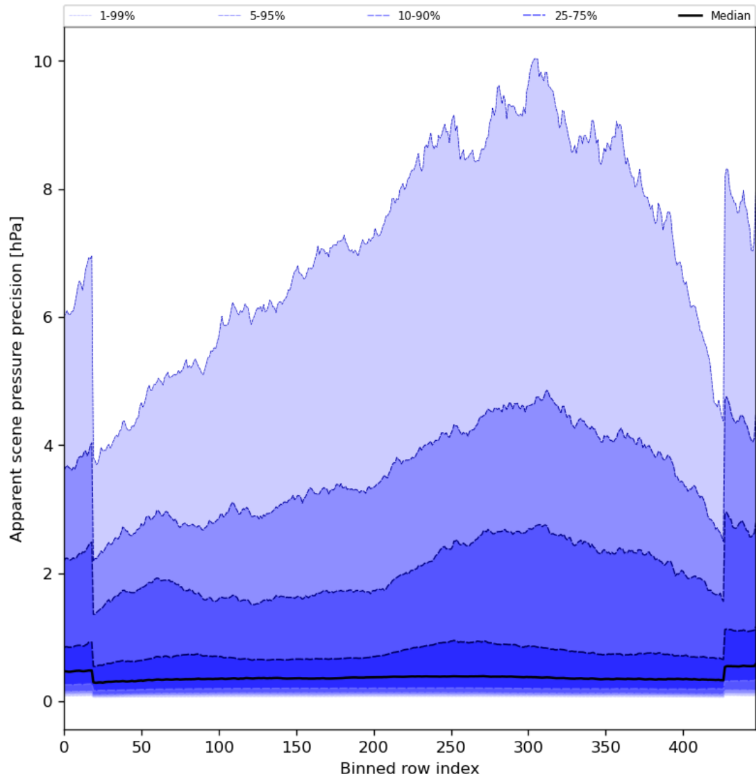
Figure 54: Along track statistics of “Apparent scene pressure precision” for 2024-08-19 to 2024-08-21
