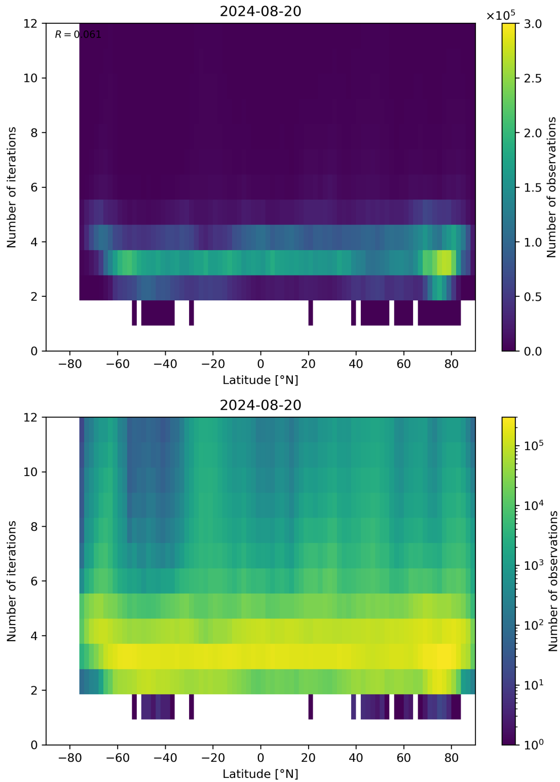
Figure 93: Scatter density plot of “Latitude” against “Number of iterations” for 2024-08-19 to 2024-08-21.
