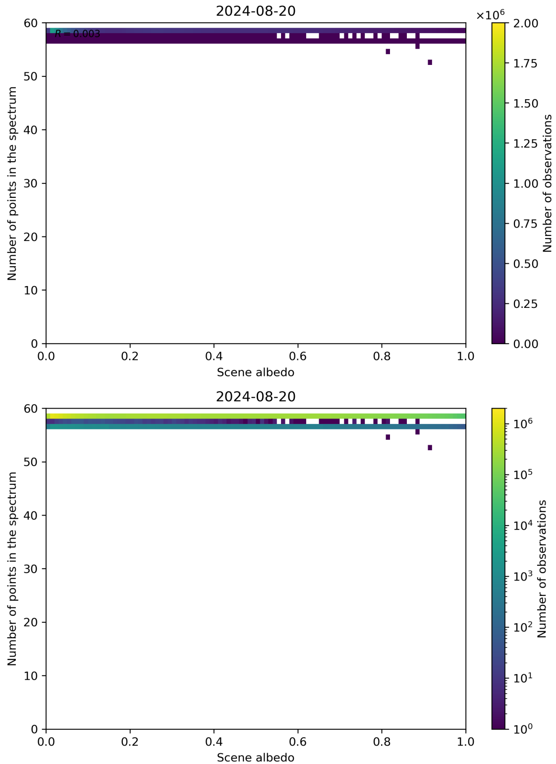
Figure 106: Scatter density plot of “Scene albedo” against “Number of points in the spectrum” for 2024-08-19 to 2024-08-21.
