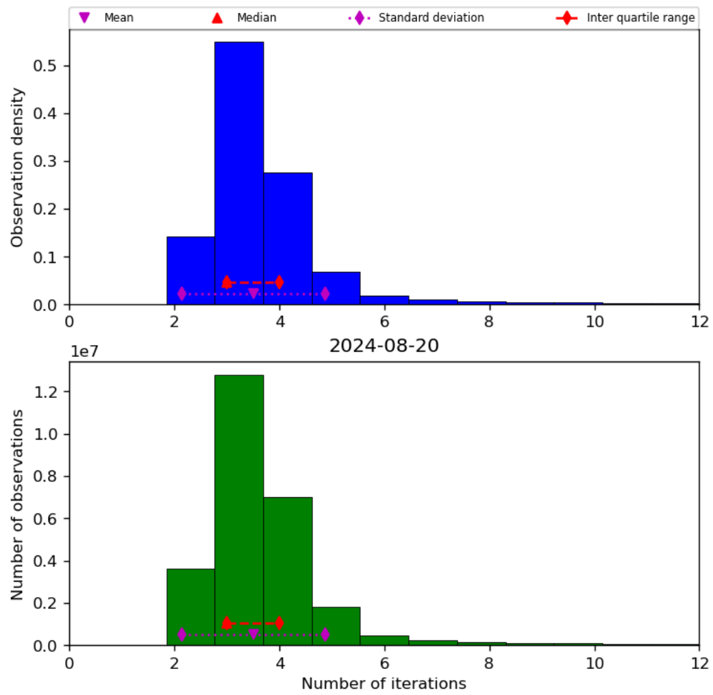
Figure 39: Histogram of “Number of iterations” for 2024-08-19 to 2024-08-21
