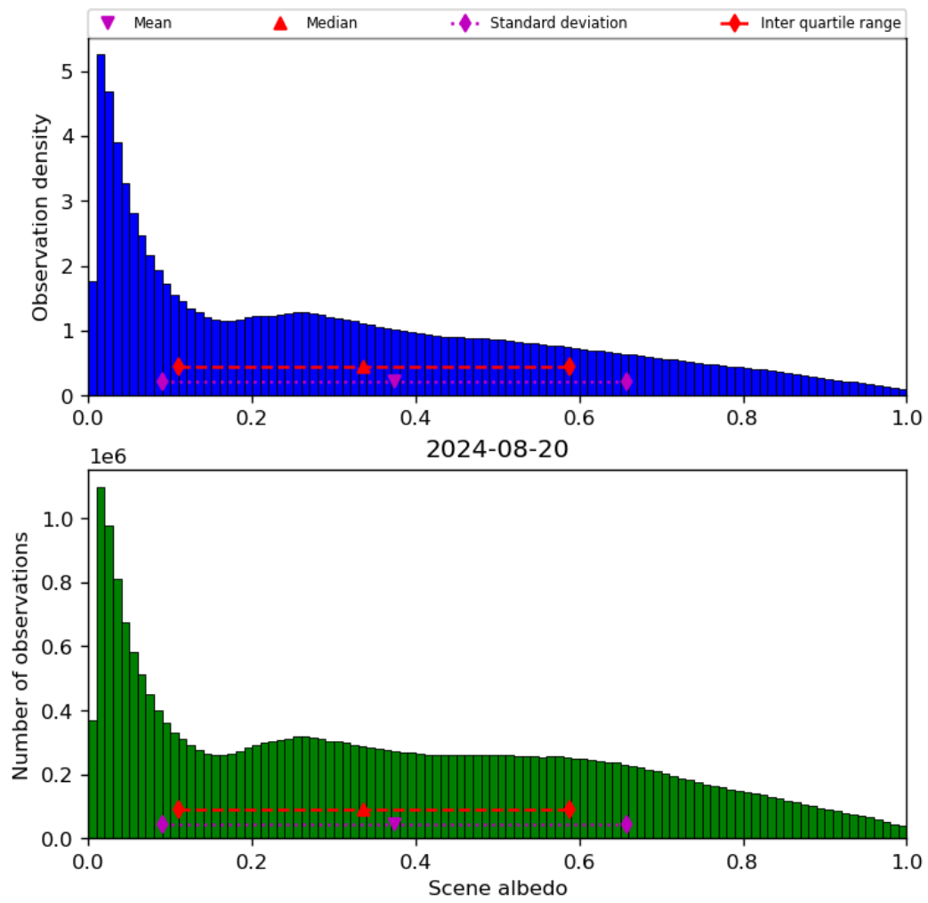
Figure 34: Histogram of “Scene albedo” for 2024-08-19 to 2024-08-21
