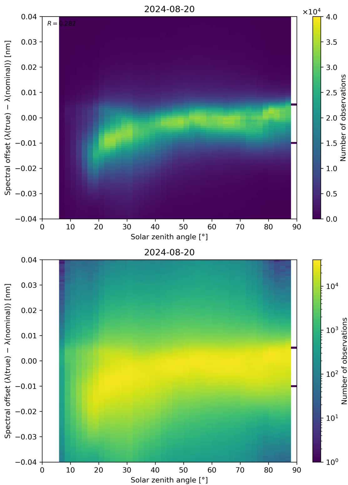
Figure 117: Scatter density plot of “Solar zenith angle” against “Spectral offset ( \lambda(\text{true}) - \lambda(\text{nominal}) )” for 2024-08-19 to 2024-08-21.
