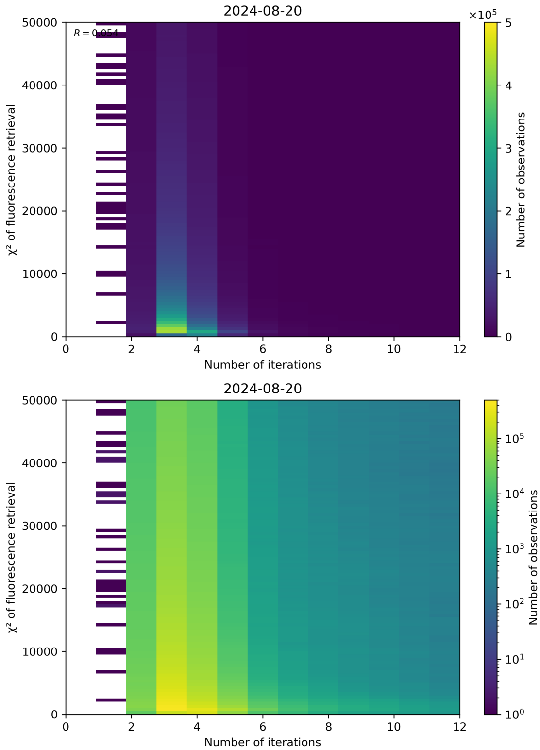
Figure 97: Scatter density plot of “Number of iterations” against “ \chi^2 of fluorescence retrieval” for 2024-08-19 to 2024-08-21.
