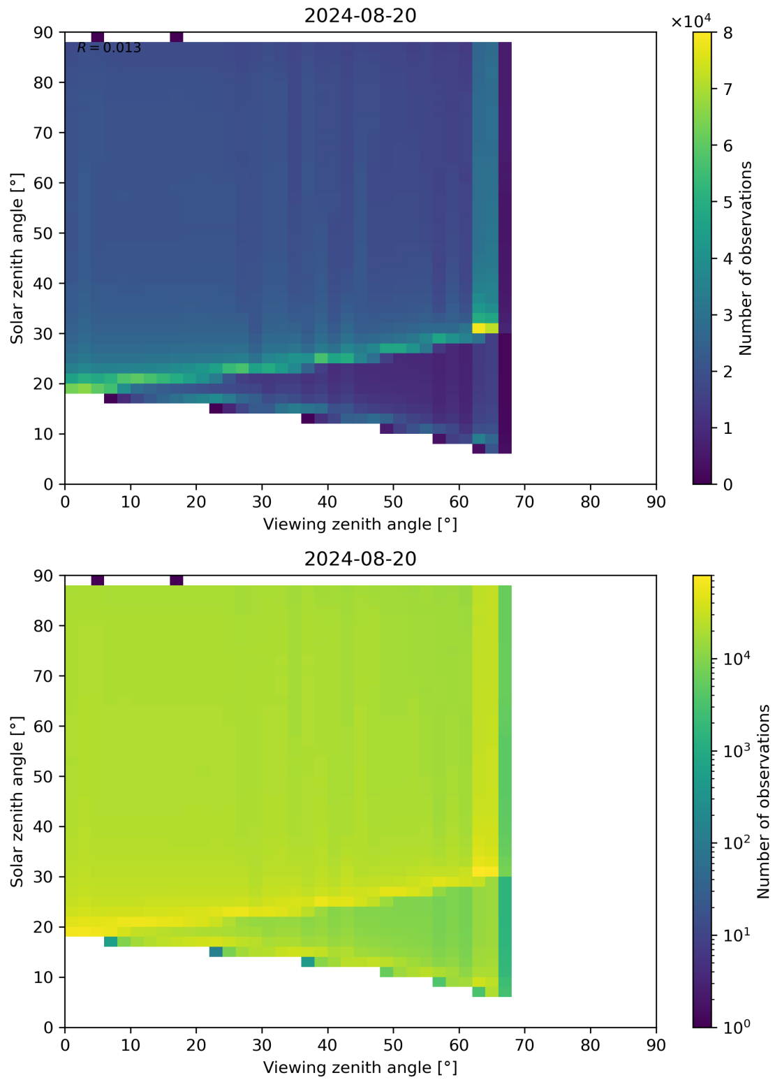
Figure 127: Scatter density plot of “Viewing zenith angle” against “Solar zenith angle” for 2024-08-19 to 2024-08-21.
