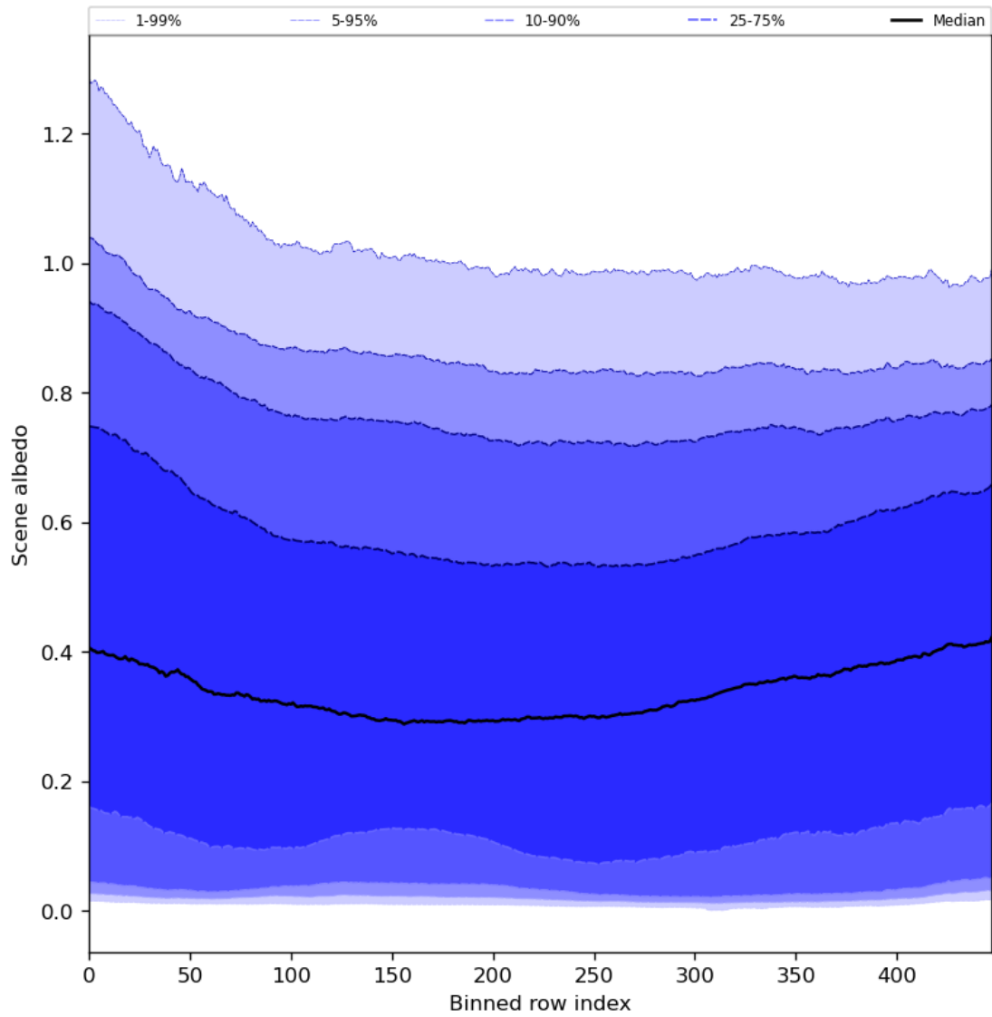
Figure 51: Along track statistics of “Scene albedo” for 2024-08-19 to 2024-08-21
