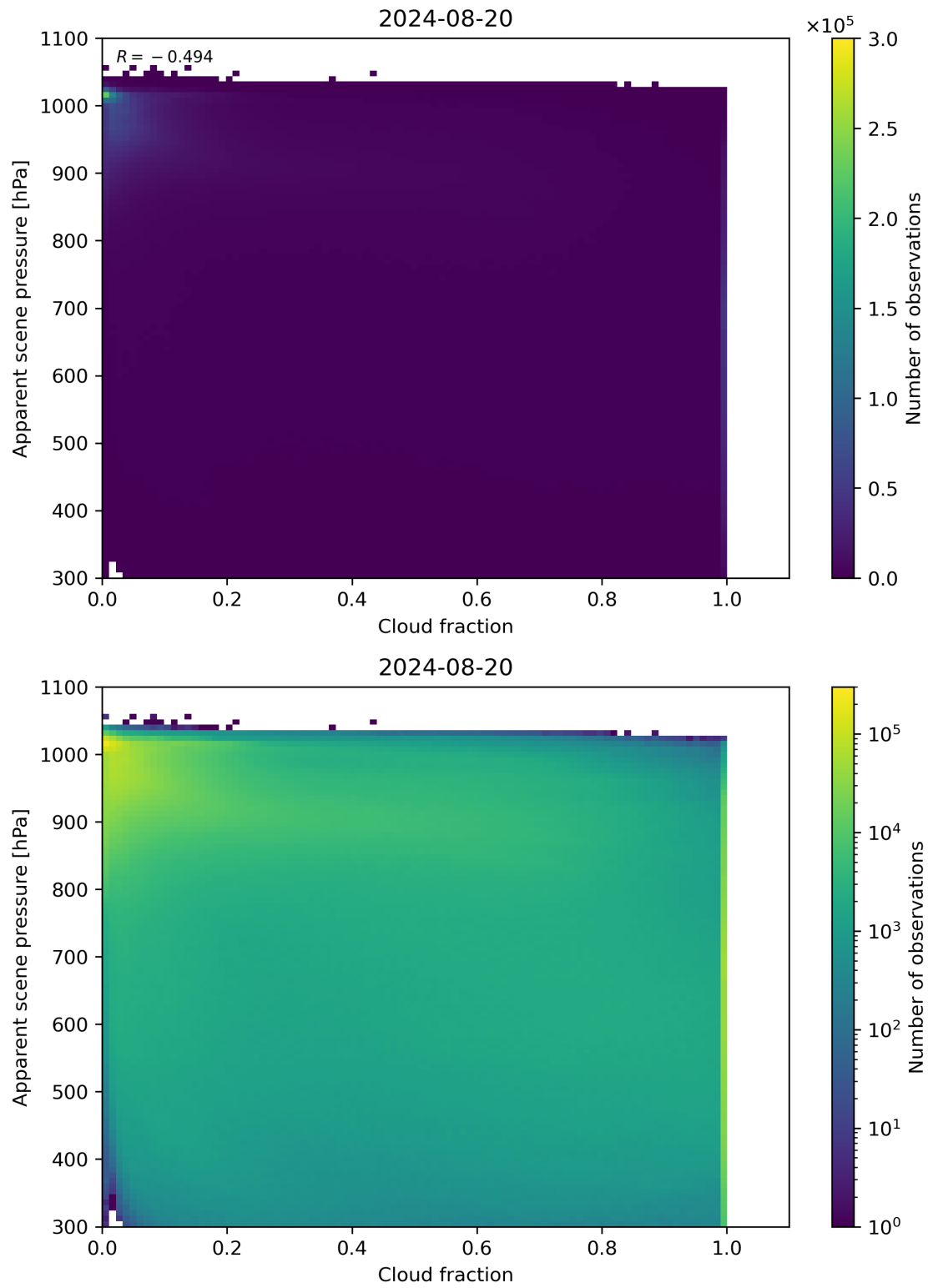
Figure 70: Scatter density plot of “Cloud fraction” against “Apparent scene pressure” for 2024-08-19 to 2024-08-21.
