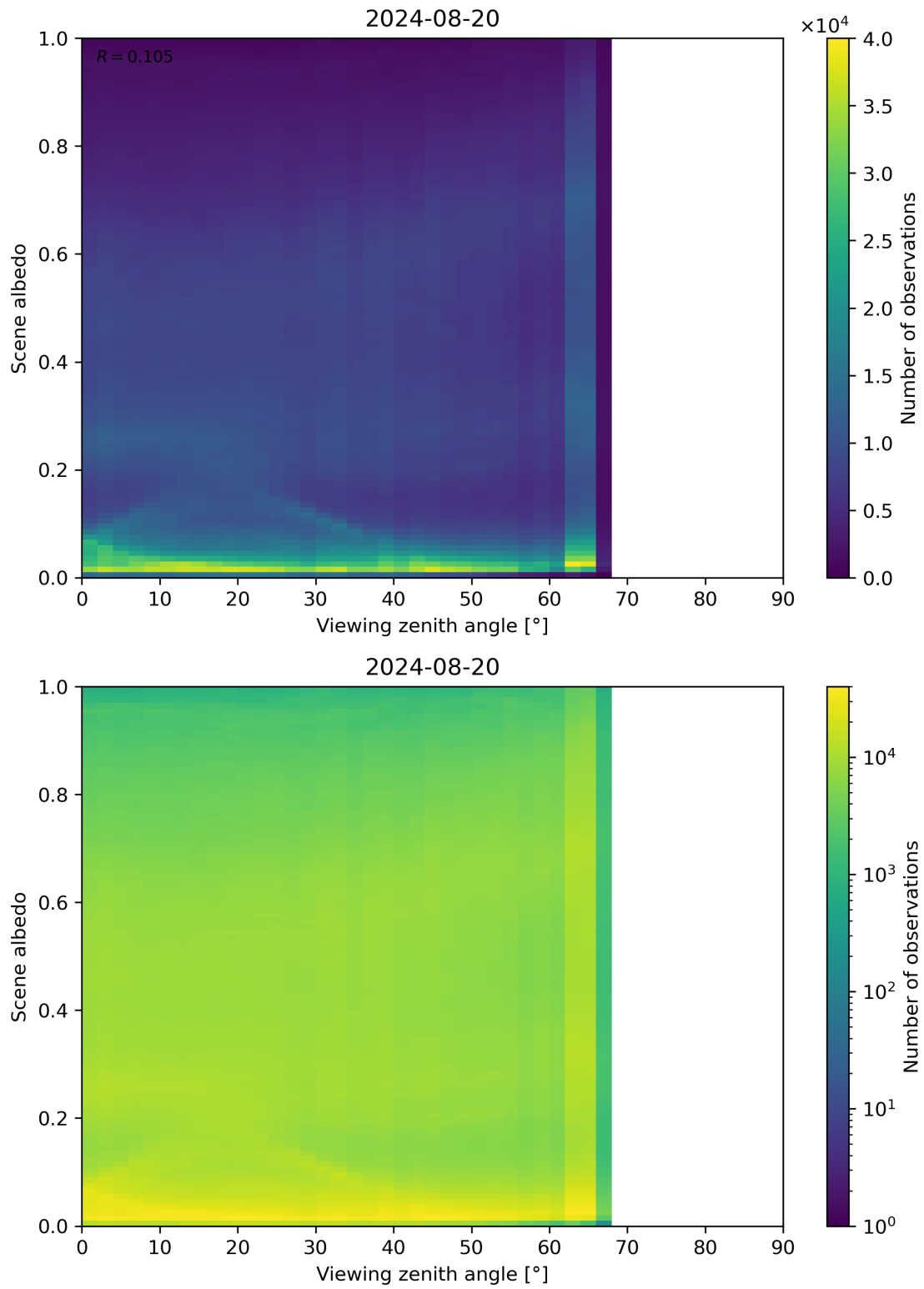
Figure 126: Scatter density plot of “Viewing zenith angle” against “Scene albedo” for 2024-08-19 to 2024-08-21.
