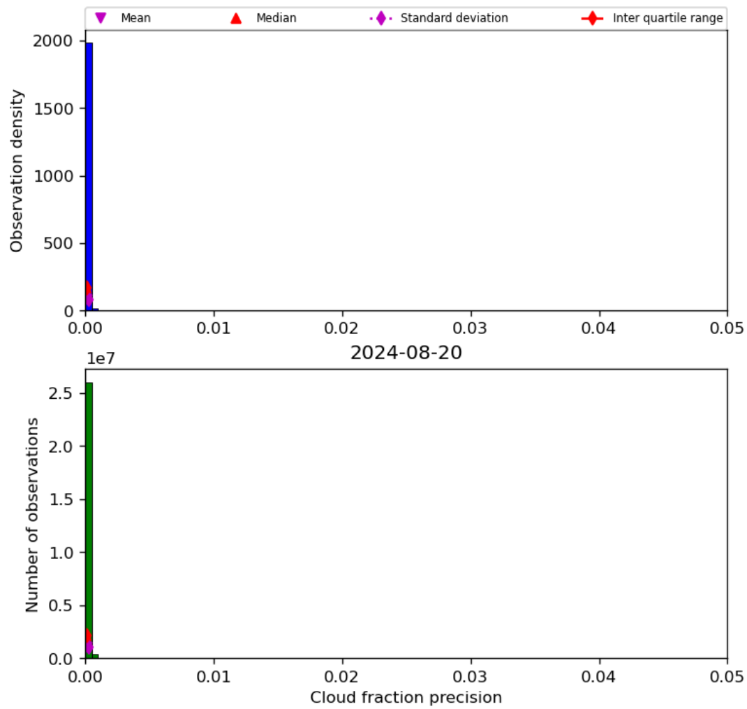
Figure 33: Histogram of “Cloud fraction precision” for 2024-08-19 to 2024-08-21
