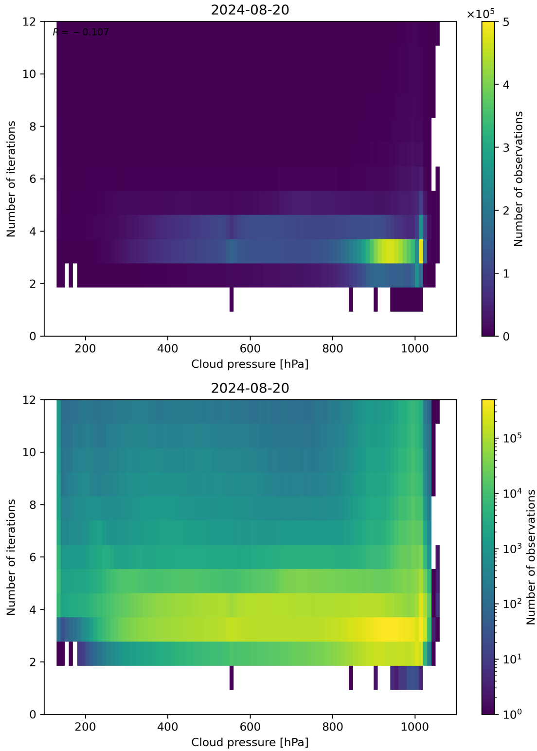
Figure 81: Scatter density plot of “Cloud pressure” against “Number of iterations” for 2024-08-19 to 2024-08-21.
