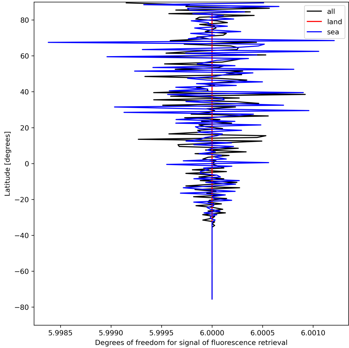
Figure 26: Zonal average of “Degrees of freedom for signal of fluorescence retrieval” for 2024-08-19 to 2024-08-21.
