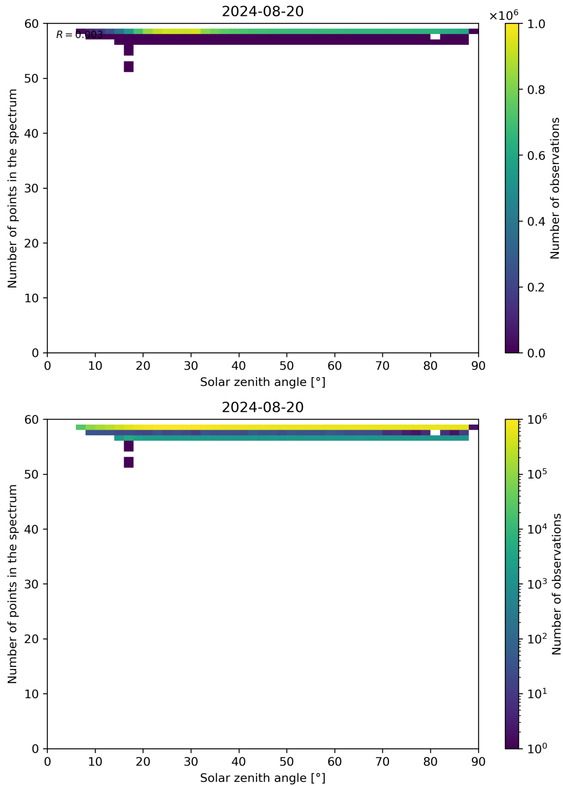
Figure 115: Scatter density plot of “Solar zenith angle” against “Number of points in the spectrum” for 2024-08-19 to 2024-08-21.
