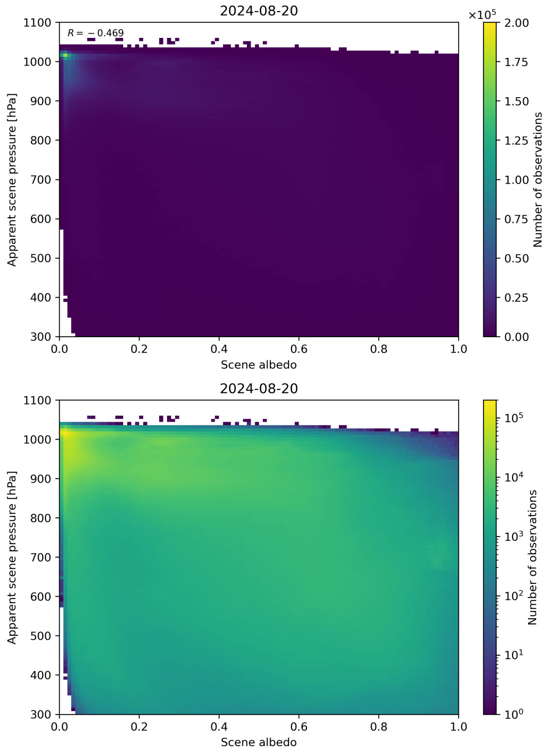
Figure 102: Scatter density plot of “Scene albedo” against “Apparent scene pressure” for 2024-08-19 to 2024-08-21.
