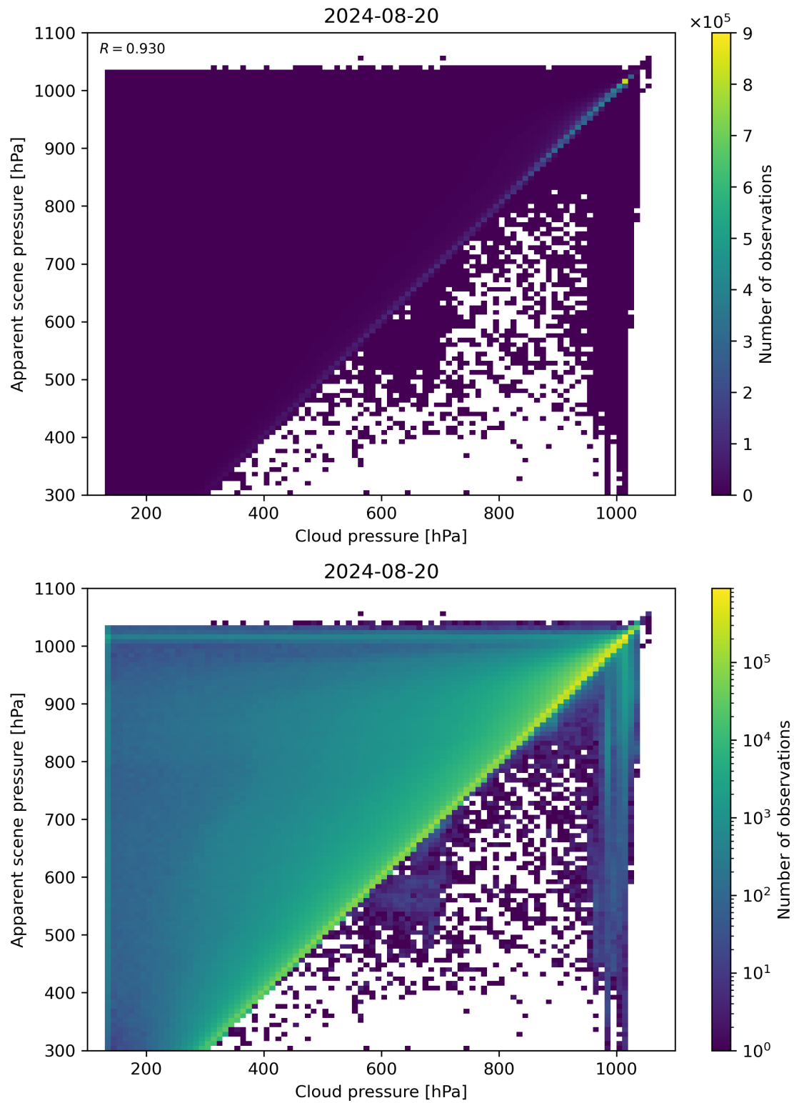
Figure 77: Scatter density plot of “Cloud pressure” against “Apparent scene pressure” for 2024-08-19 to 2024-08-21.
