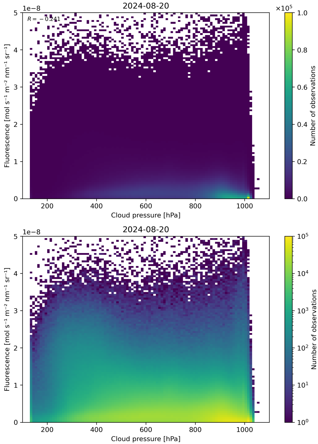
Figure 80: Scatter density plot of “Cloud pressure” against “Fluorescence” for 2024-08-19 to 2024-08-21.
