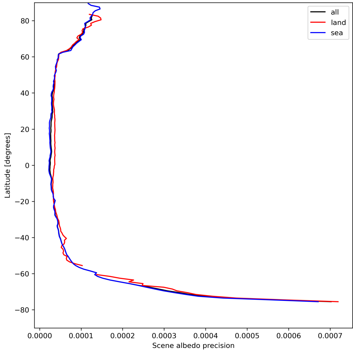
Figure 18: Zonal average of “Scene albedo precision” for 2024-08-19 to 2024-08-21.
