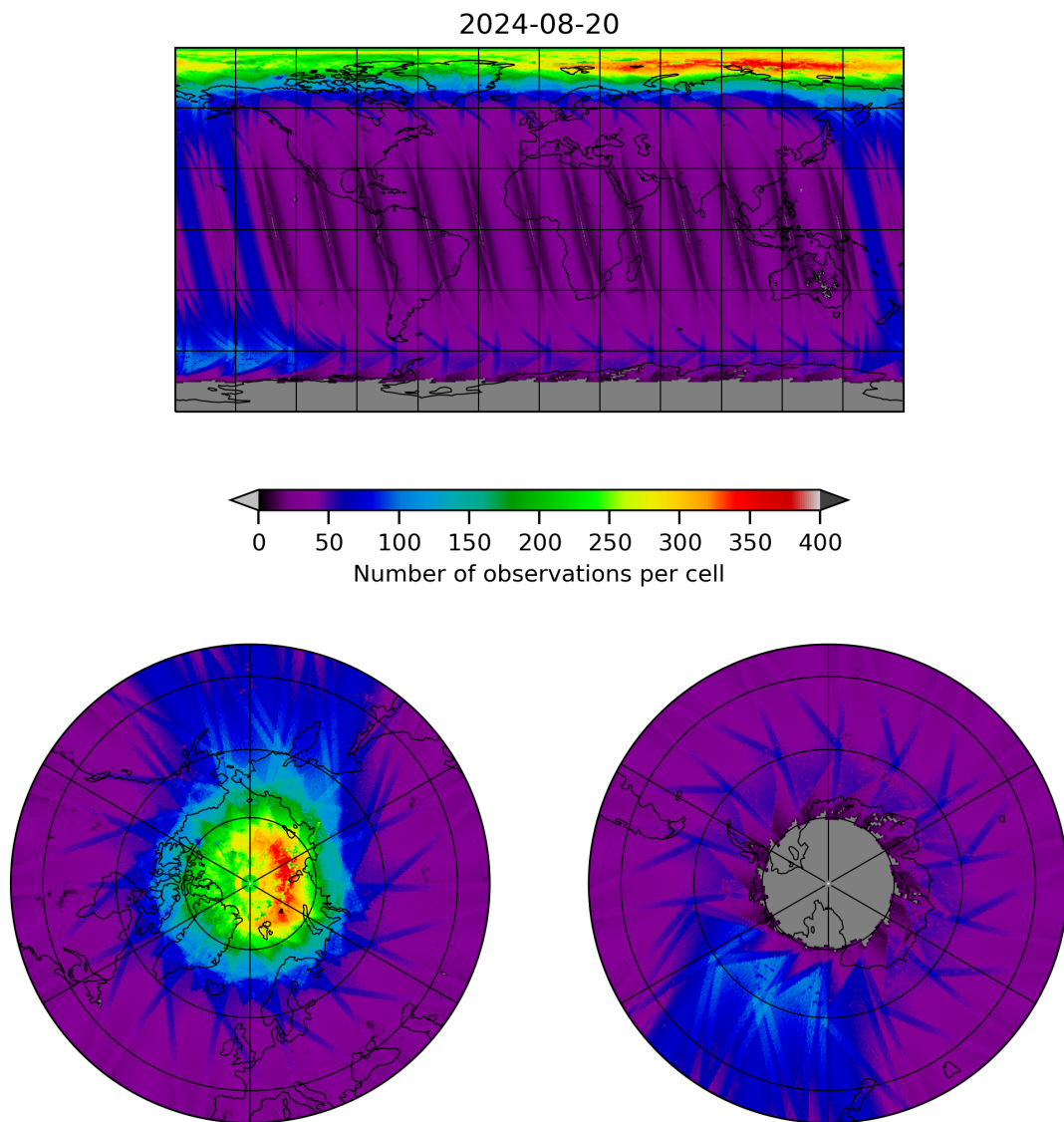
Figure 11: Map of the number of observations for 2024-08-19 to 2024-08-21
