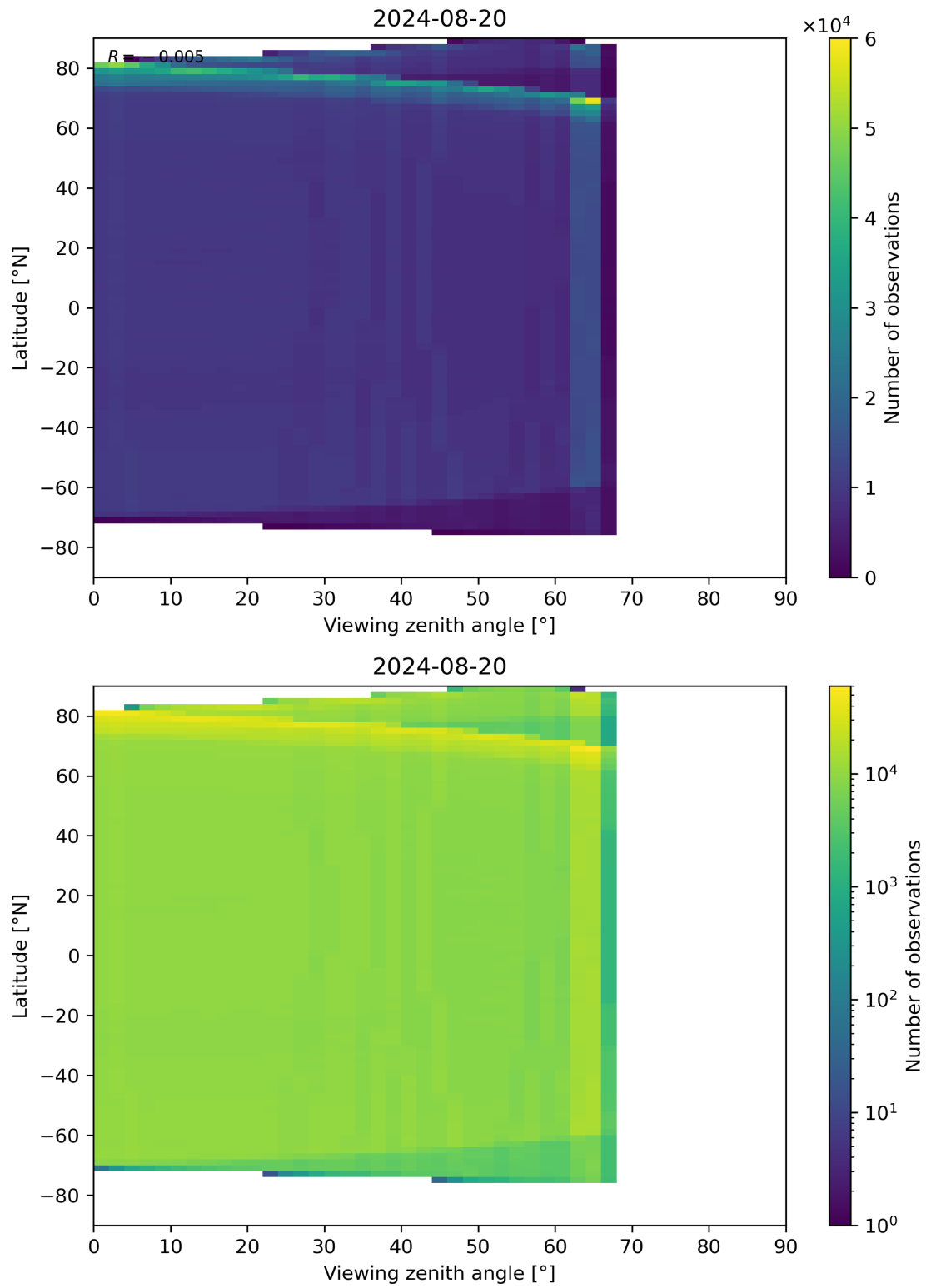
Figure 123: Scatter density plot of “Viewing zenith angle” against “Latitude” for 2024-08-19 to 2024-08-21.
