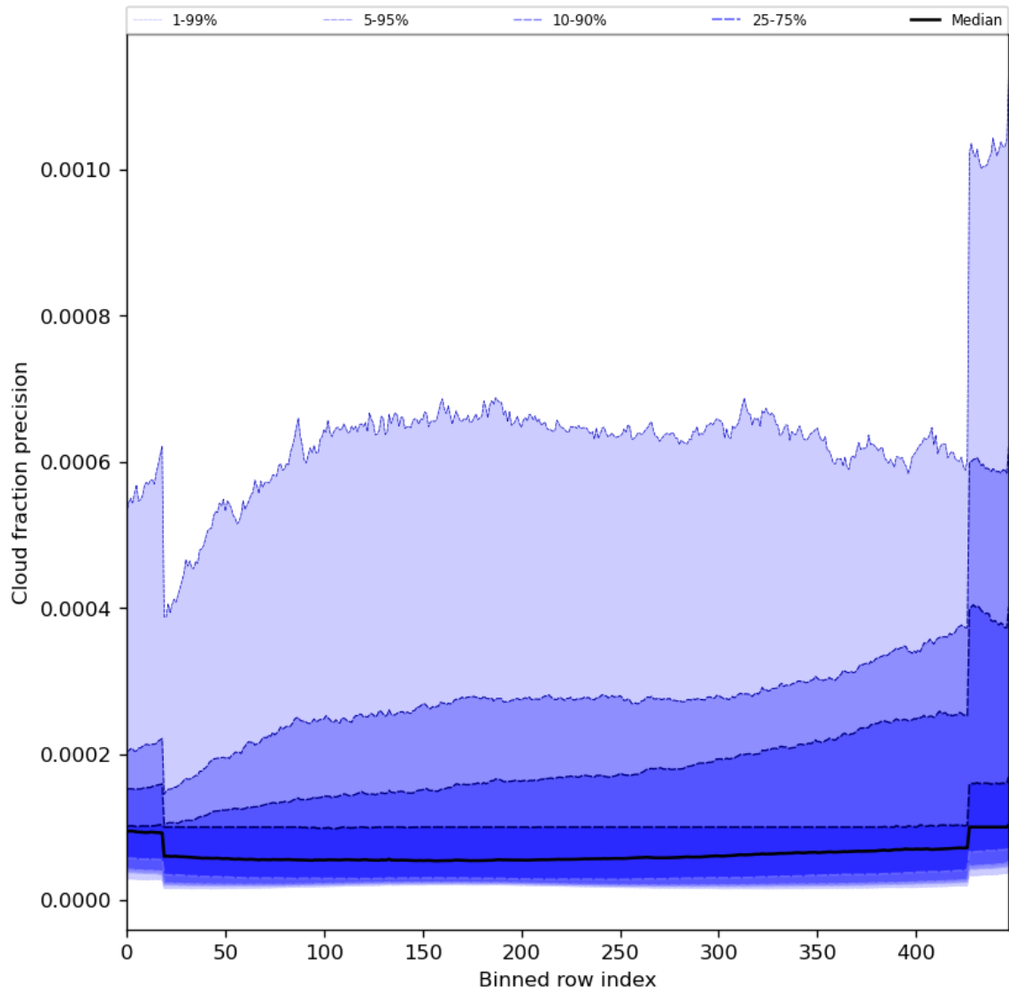
Figure 50: Along track statistics of “Cloud fraction precision” for 2024-08-19 to 2024-08-21
