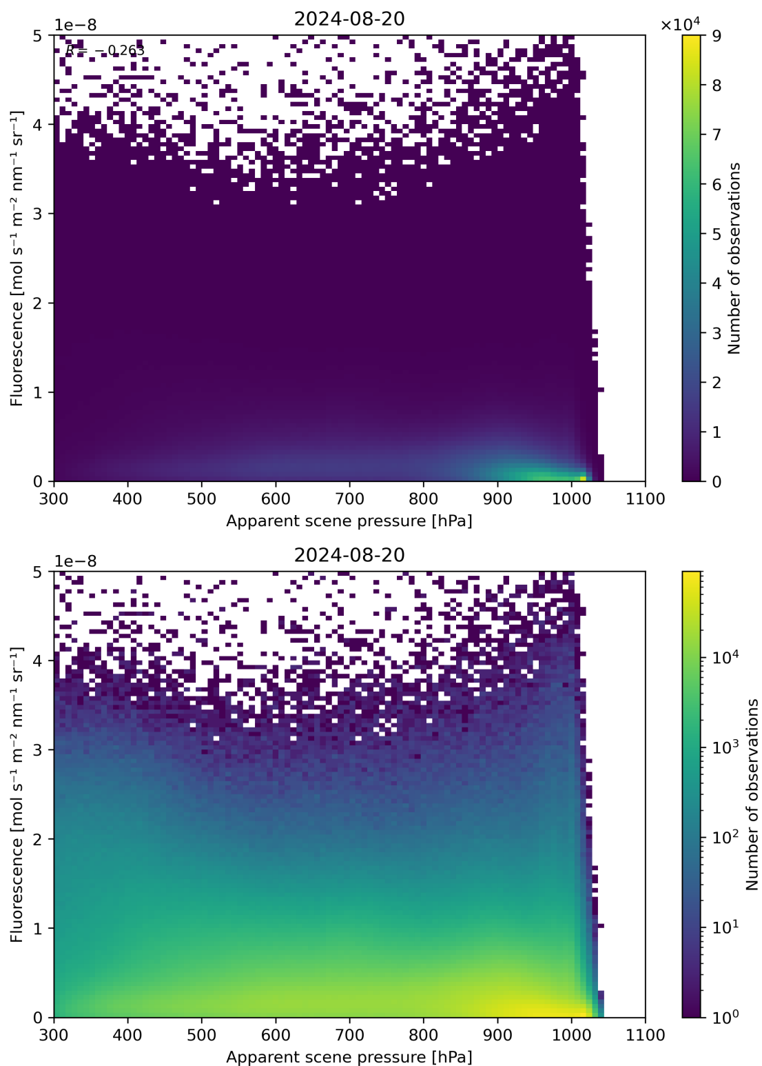
Figure 64: Scatter density plot of “Apparent scene pressure” against “Fluorescence” for 2024-08-19 to 2024-08-21.
