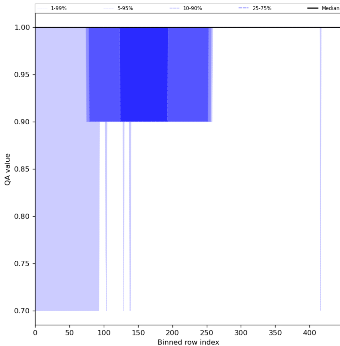
Figure 46: Along track statistics of “QA value” for 2024-08-19 to 2024-08-21
