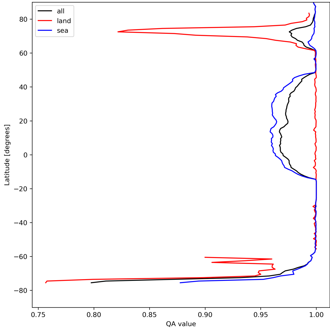
Figure 12: Zonal average of “QA value” for 2024-08-19 to 2024-08-21.
