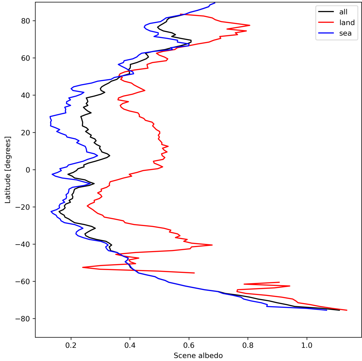
Figure 17: Zonal average of “Scene albedo” for 2024-08-19 to 2024-08-21.
