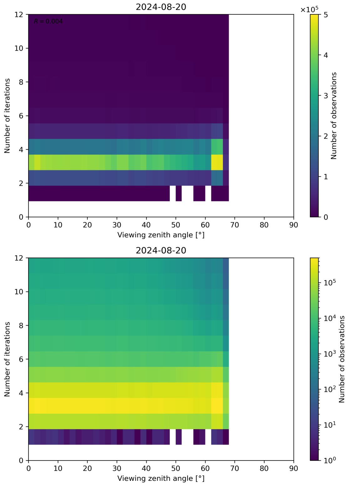
Figure 124: Scatter density plot of “Viewing zenith angle” against “Number of iterations” for 2024-08-19 to 2024-08-21.
