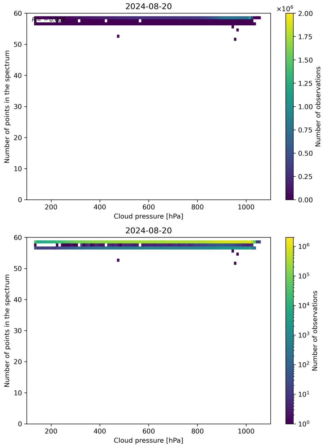
Figure 82: Scatter density plot of “Cloud pressure” against “Number of points in the spectrum” for 2024-08-19 to 2024-08-21.
