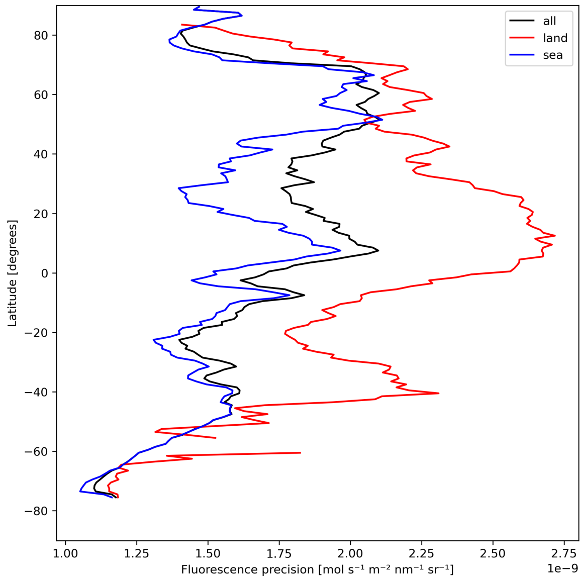
Figure 24: Zonal average of “Fluorescence precision” for 2024-08-19 to 2024-08-21.
