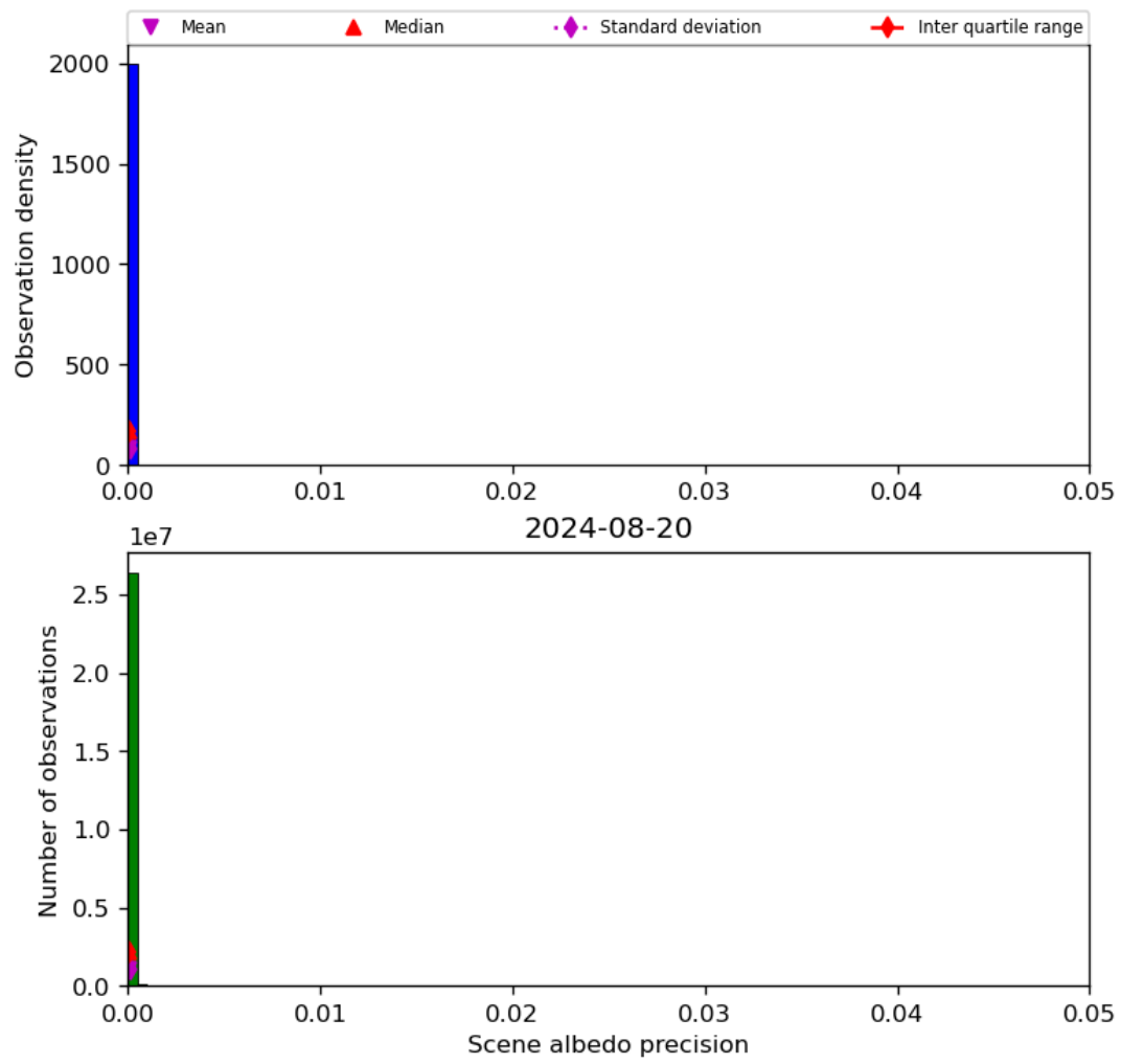
Figure 35: Histogram of “Scene albedo precision” for 2024-08-19 to 2024-08-21
