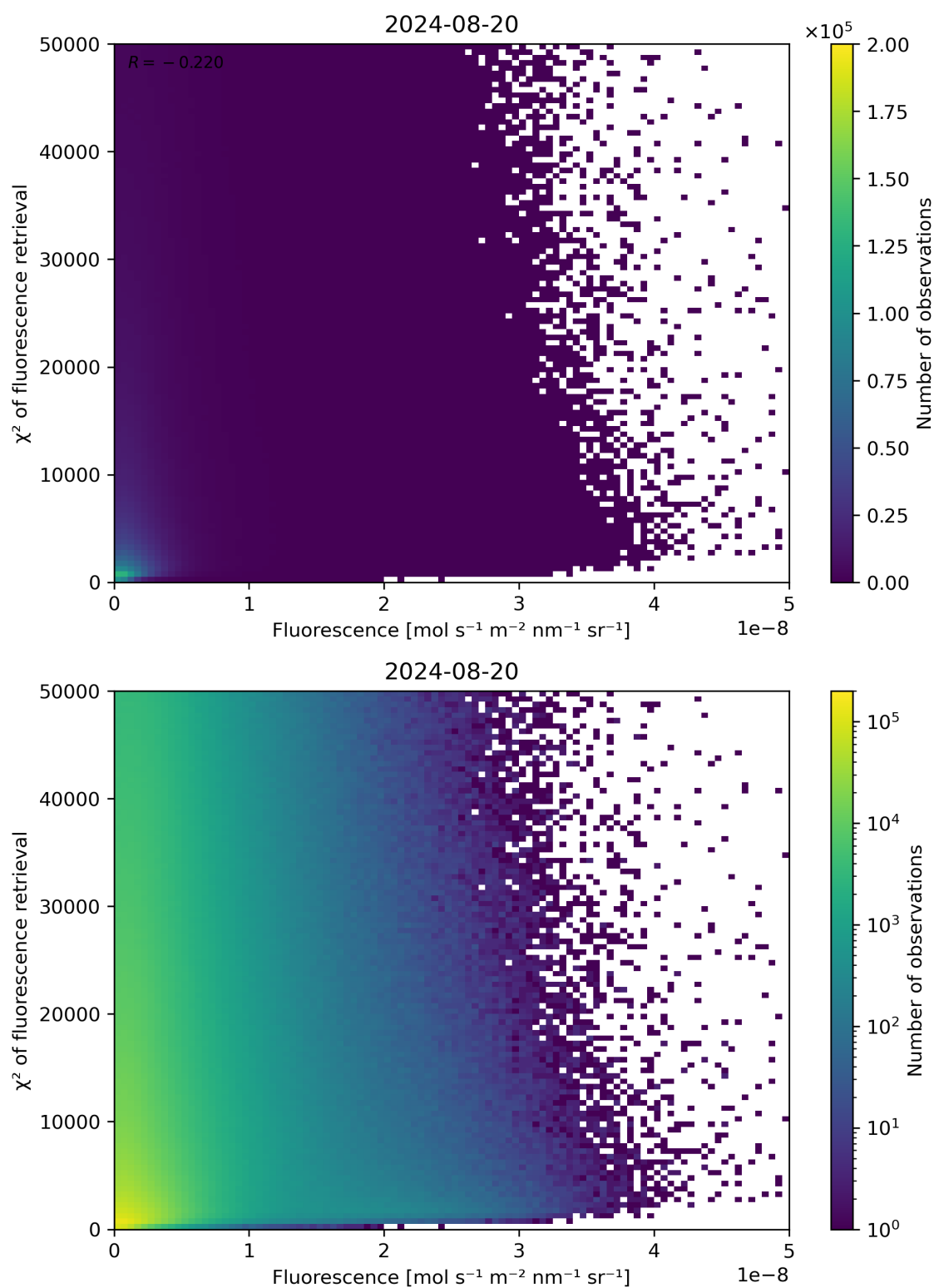
Figure 85: Scatter density plot of “Fluorescence” against “ \chi^2 of fluorescence retrieval” for 2024-08-19 to 2024-08-21.
