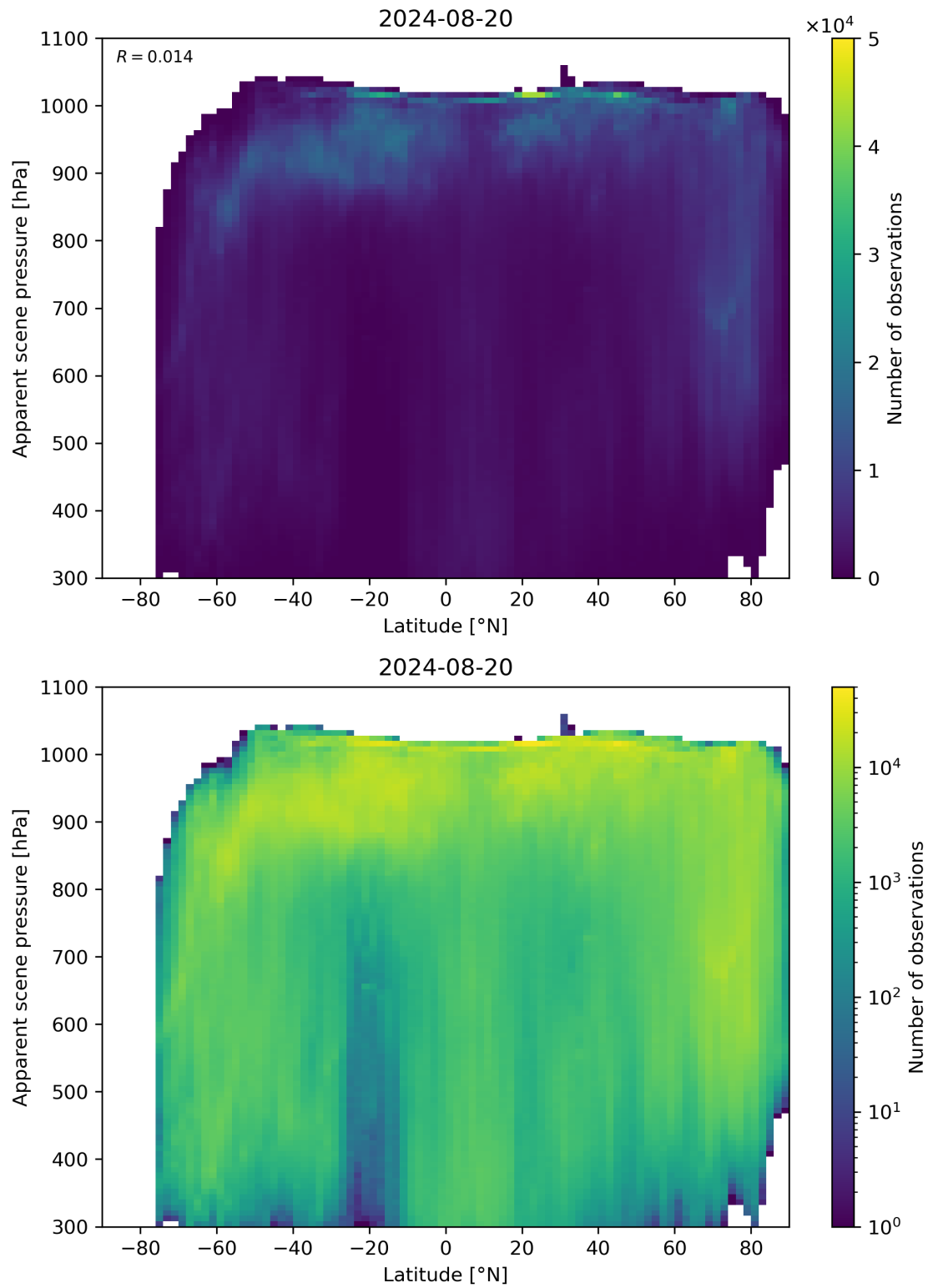
Figure 88: Scatter density plot of “Latitude” against “Apparent scene pressure” for 2024-08-19 to 2024-08-21.
