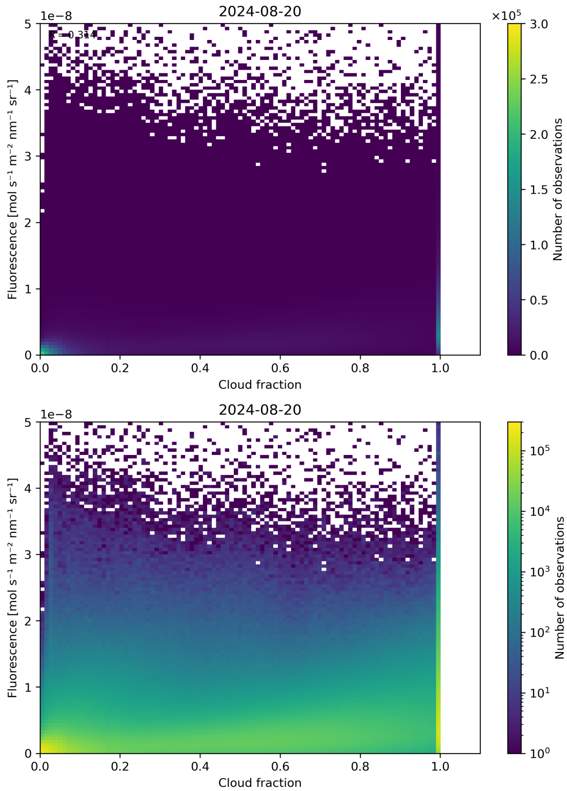
Figure 72: Scatter density plot of “Cloud fraction” against “Fluorescence” for 2024-08-19 to 2024-08-21.
