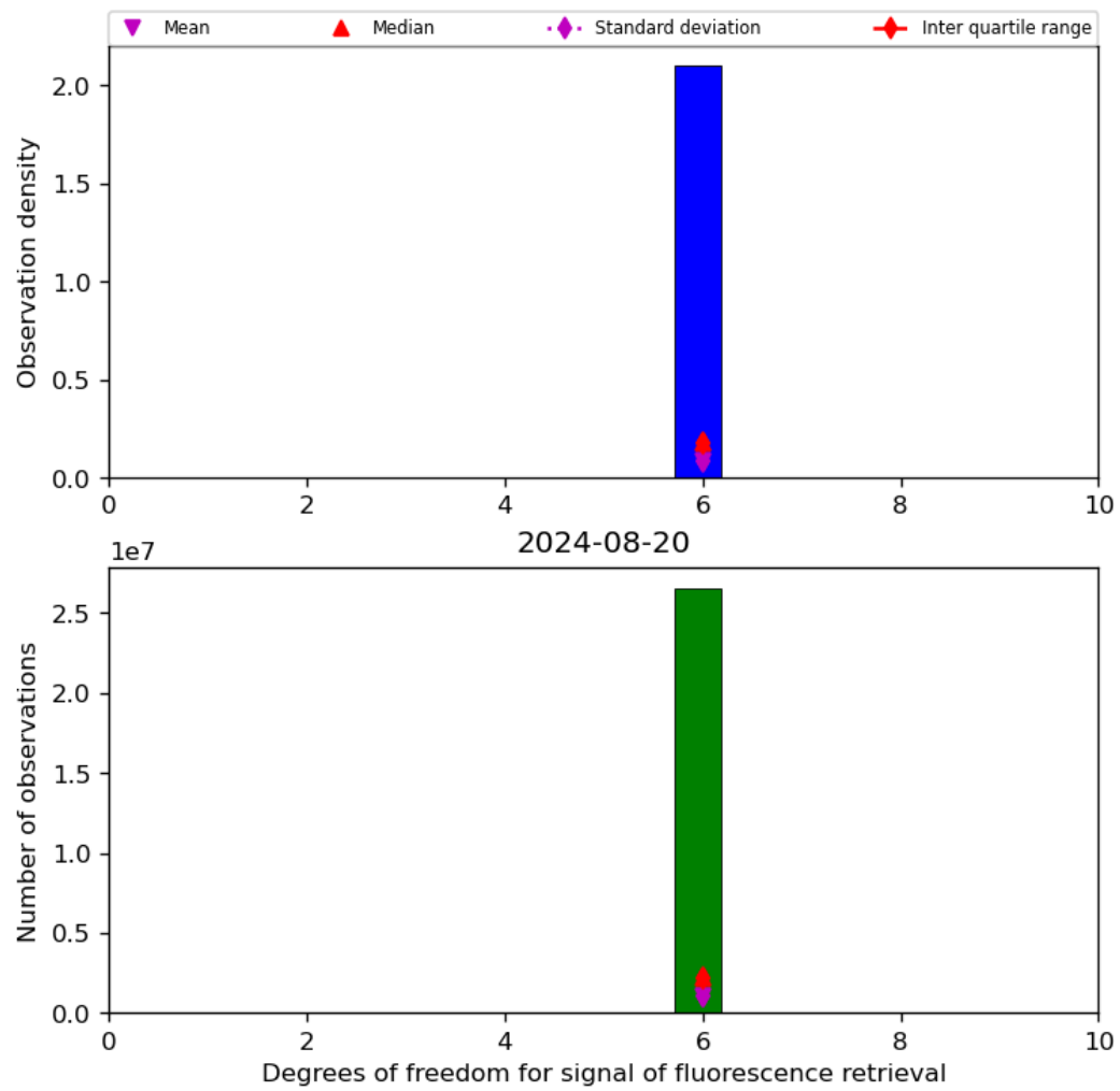
Figure 43: Histogram of “Degrees of freedom for signal of fluorescence retrieval” for 2024-08-19 to 2024-08-21
