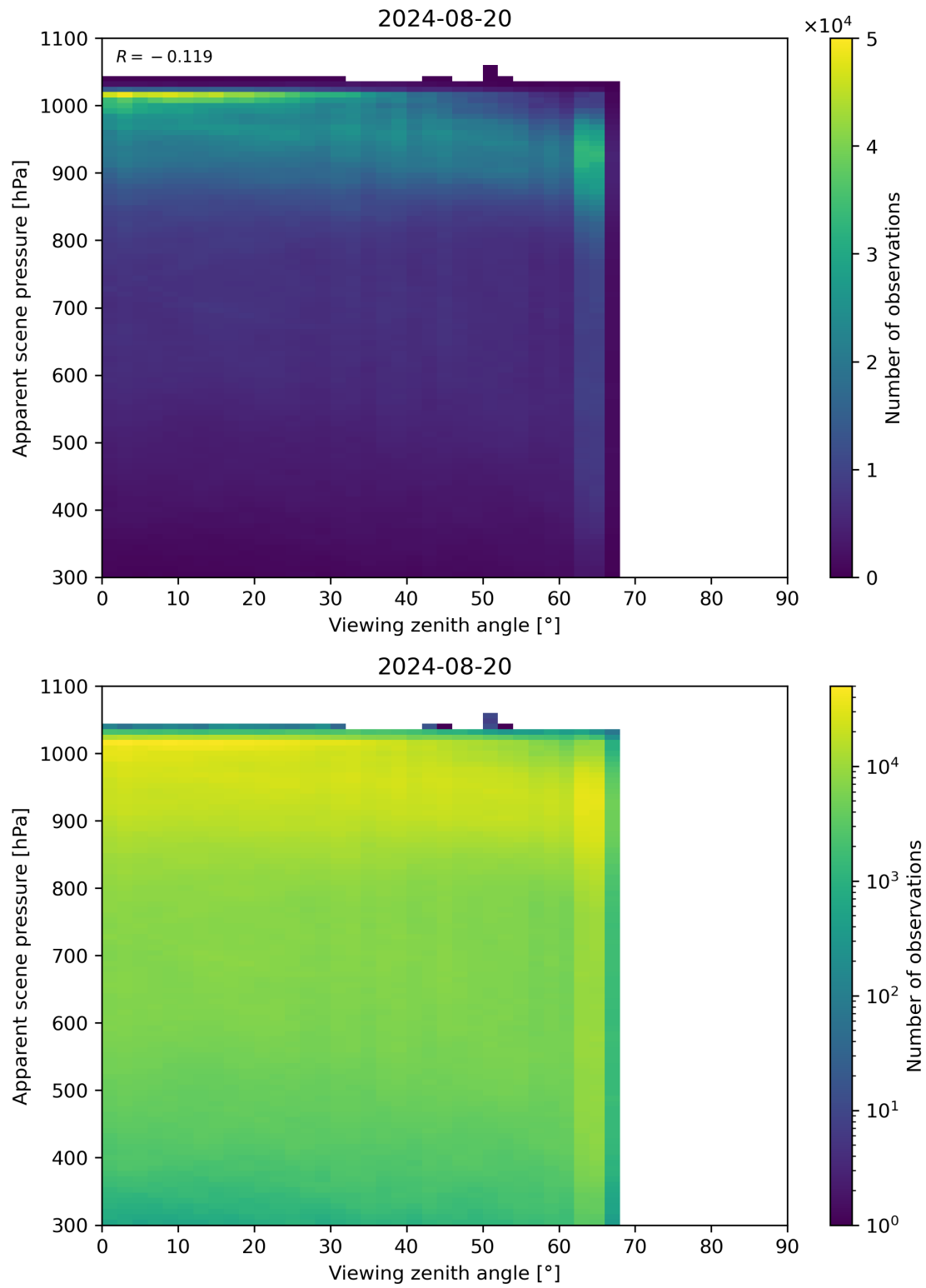
Figure 118: Scatter density plot of “Viewing zenith angle” against “Apparent scene pressure” for 2024-08-19 to 2024-08-21.
