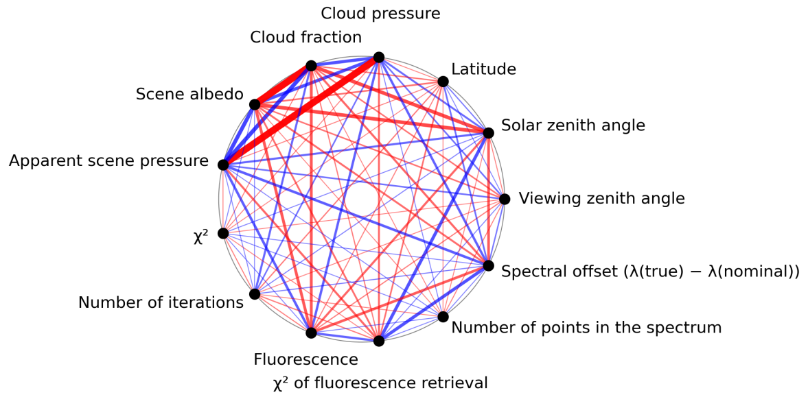
Figure 1: Map of correlation graph for 2024-08-19 to 2024-08-21.
