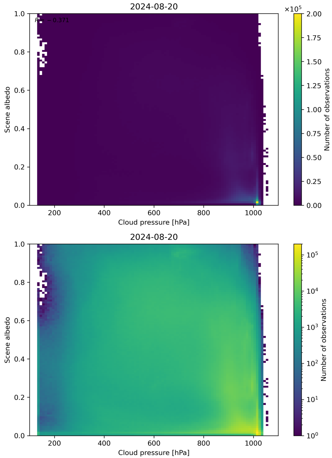
Figure 83: Scatter density plot of “Cloud pressure” against “Scene albedo” for 2024-08-19 to 2024-08-21.
