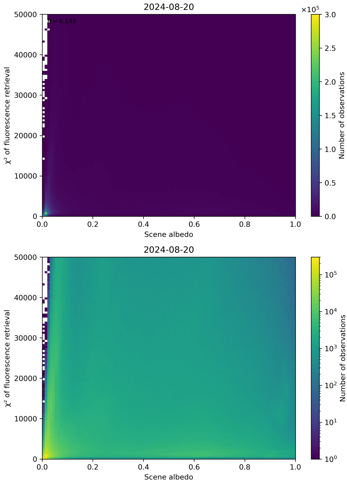
Figure 103: Scatter density plot of “Scene albedo” against “ \chi^2 of fluorescence retrieval” for 2024-08-19 to 2024-08-21.
