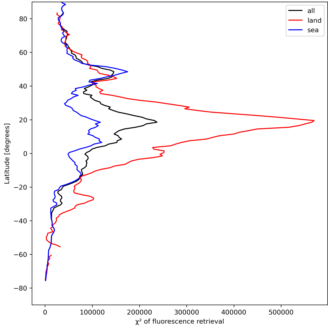
Figure 25: Zonal average of “ \chi^2 of fluorescence retrieval” for 2024-08-19 to 2024-08-21.
