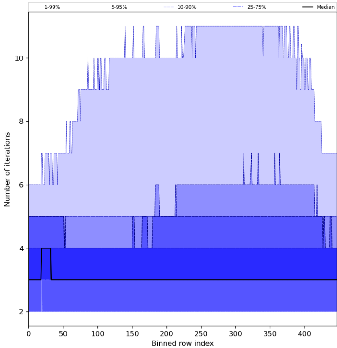
Figure 56: Along track statistics of “Number of iterations” for 2024-08-19 to 2024-08-21
