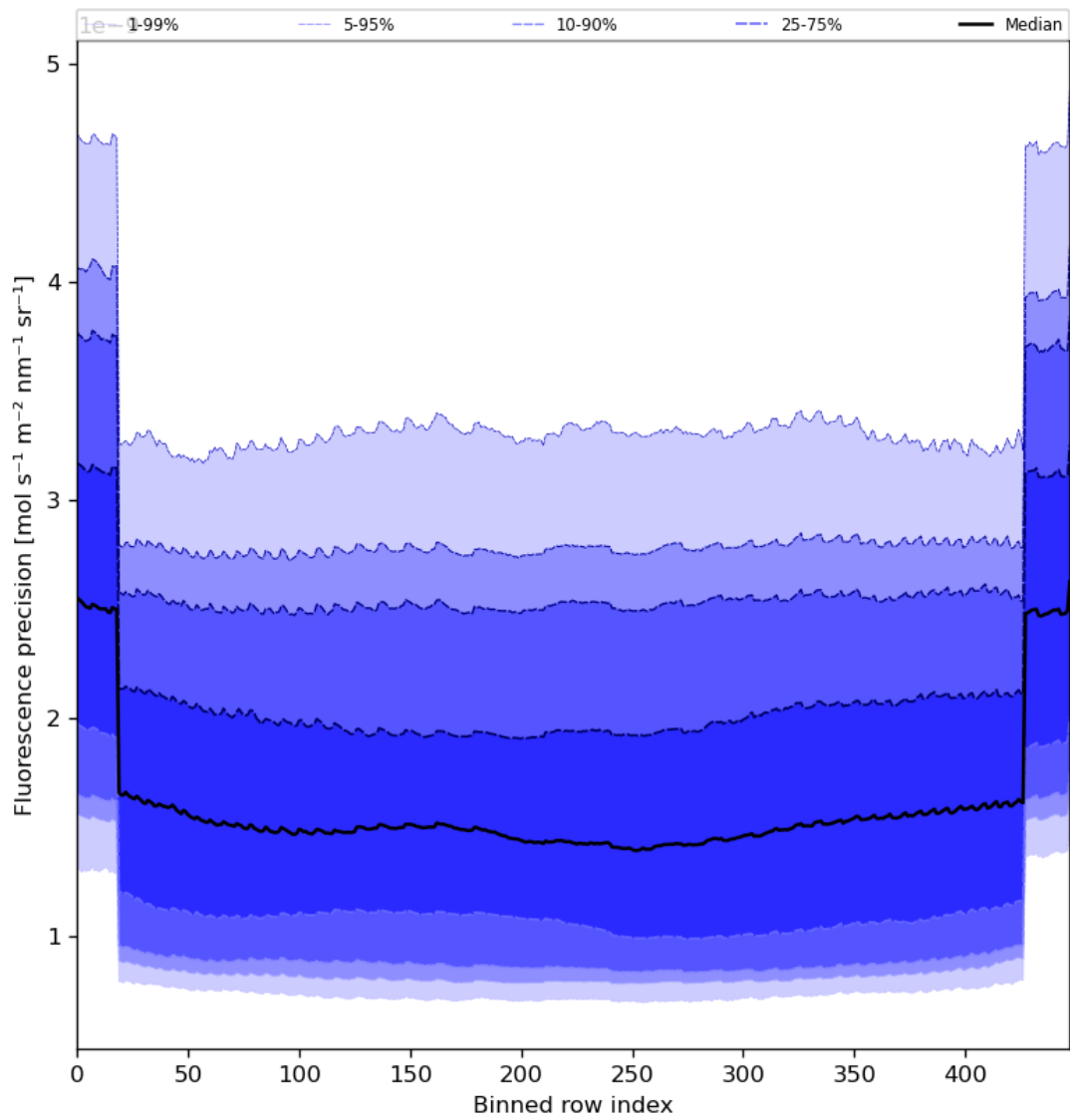
Figure 58: Along track statistics of “Fluorescence precision” for 2024-08-19 to 2024-08-21
