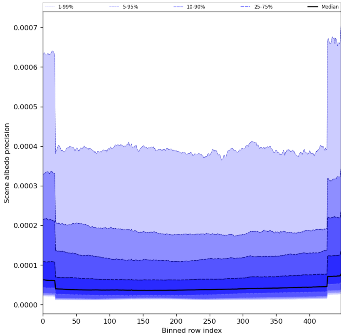
Figure 52: Along track statistics of “Scene albedo precision” for 2024-08-19 to 2024-08-21
