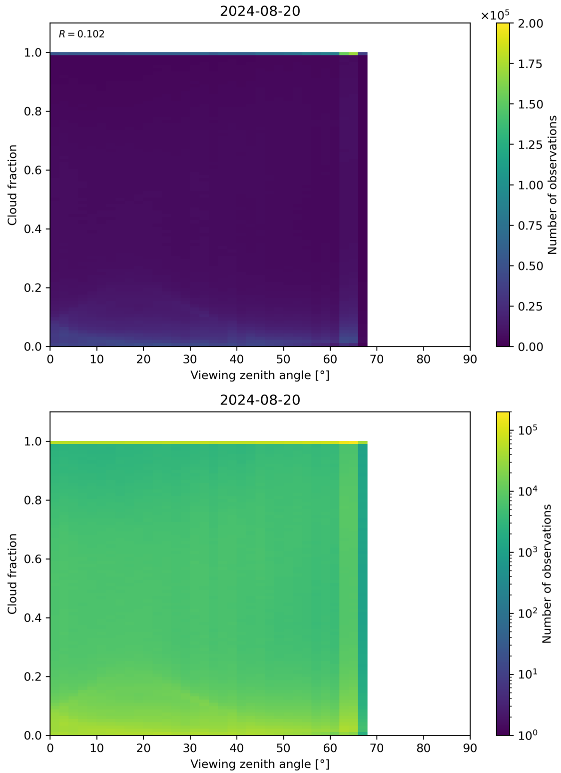
Figure 120: Scatter density plot of “Viewing zenith angle” against “Cloud fraction” for 2024-08-19 to 2024-08-21.
