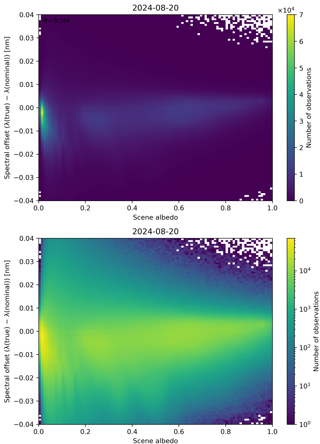
Figure 107: Scatter density plot of “Scene albedo” against “Spectral offset ( \lambda(\text{true}) - \lambda(\text{nominal}) )” for 2024-08-19 to 2024-08-21.
