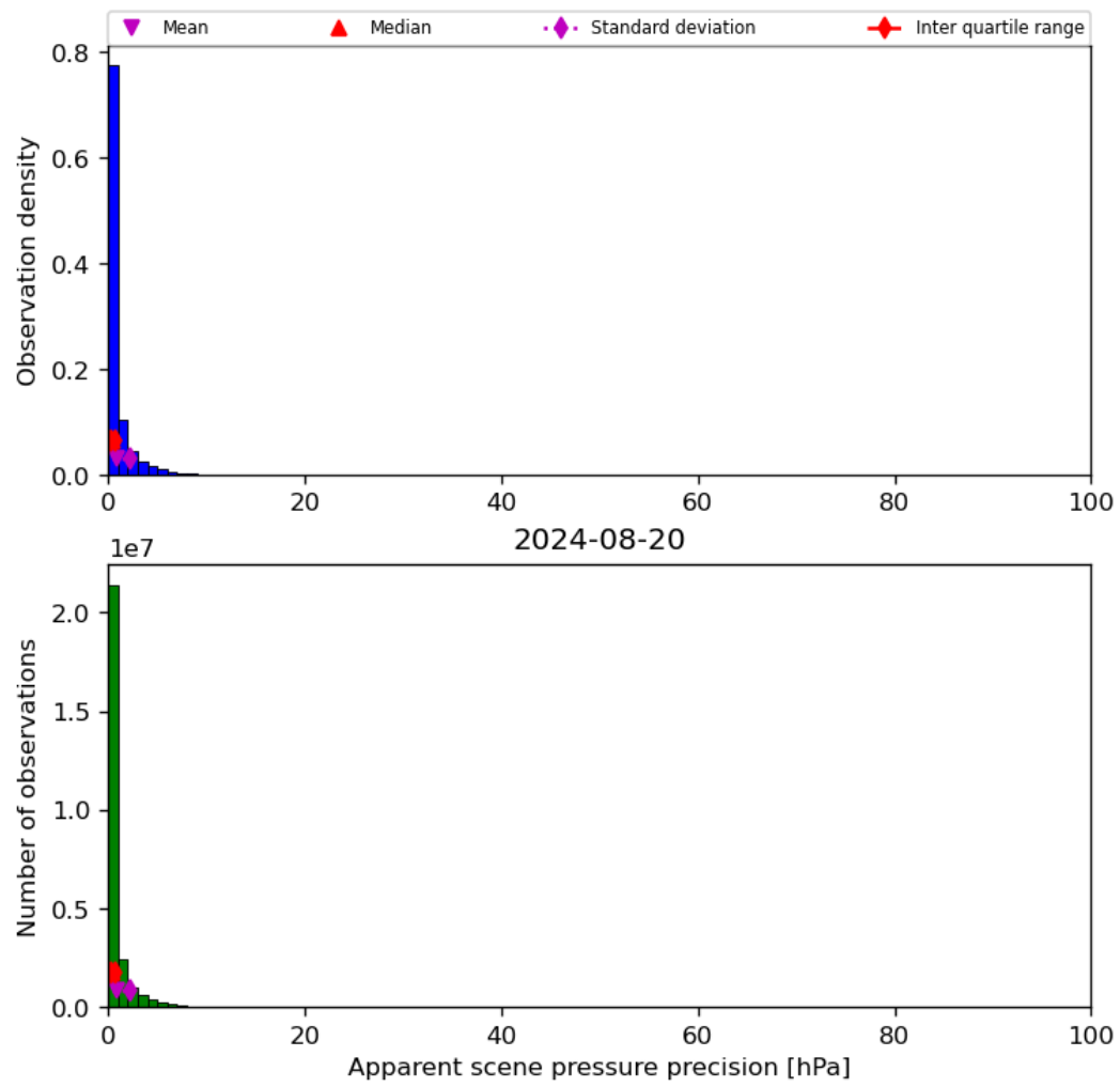
Figure 37: Histogram of “Apparent scene pressure precision” for 2024-08-19 to 2024-08-21
