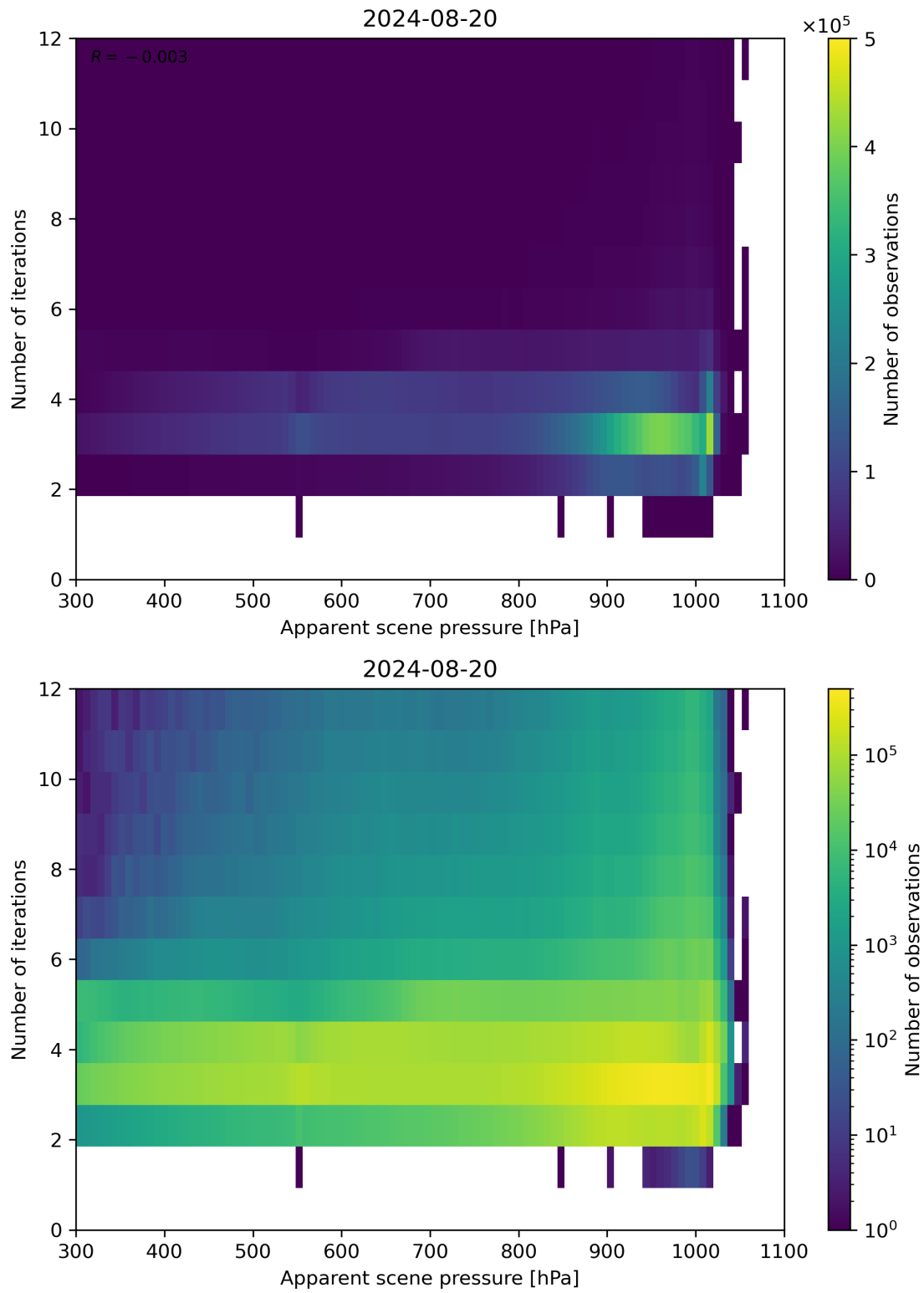
Figure 65: Scatter density plot of “Apparent scene pressure” against “Number of iterations” for 2024-08-19 to 2024-08-21.
