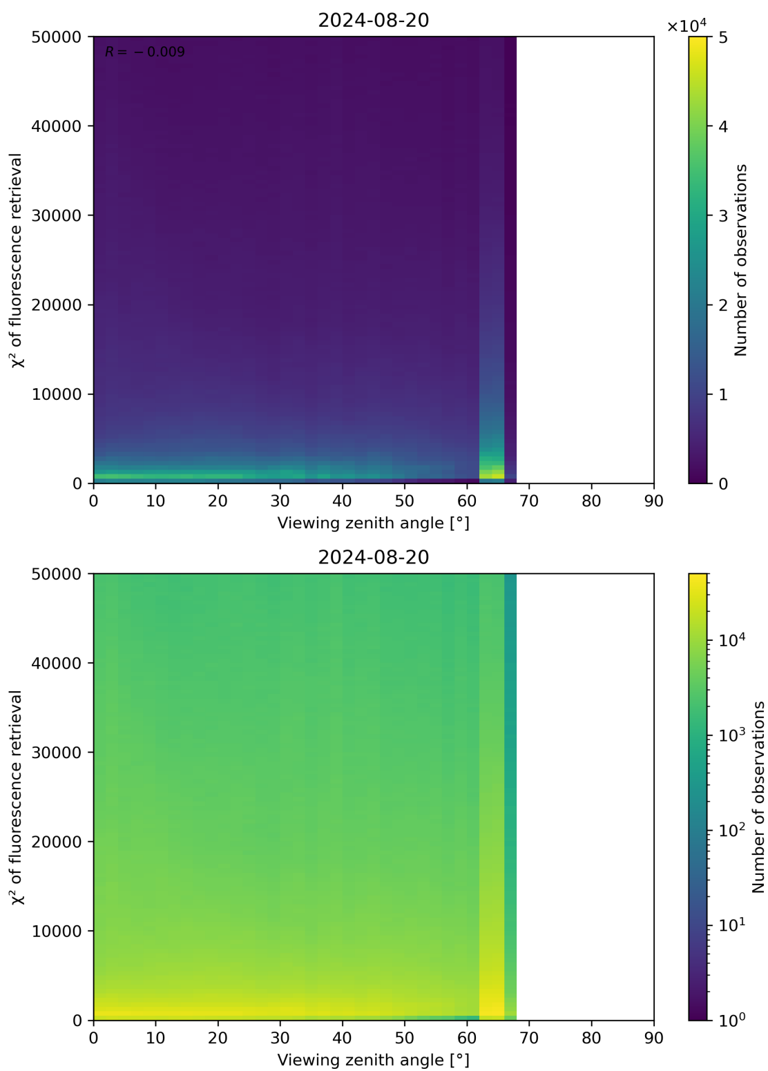
Figure 119: Scatter density plot of “Viewing zenith angle” against “ \chi^2 of fluorescence retrieval” for 2024-08-19 to 2024-08-21.
