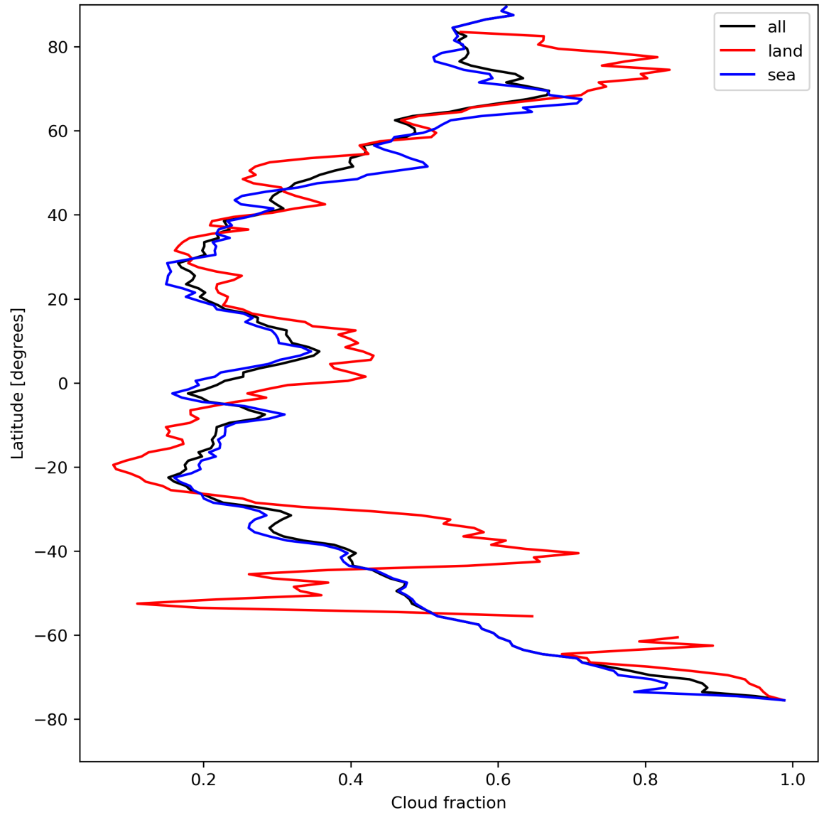
Figure 15: Zonal average of “Cloud fraction” for 2024-08-19 to 2024-08-21.
