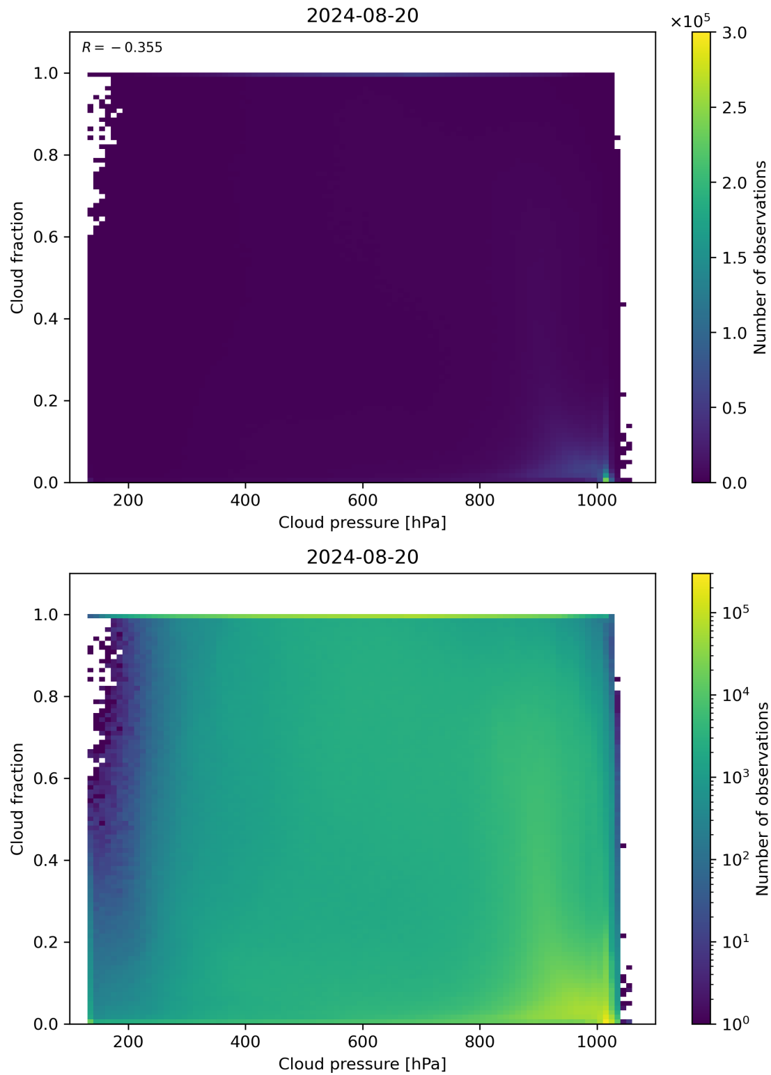
Figure 79: Scatter density plot of “Cloud pressure” against “Cloud fraction” for 2024-08-19 to 2024-08-21.
