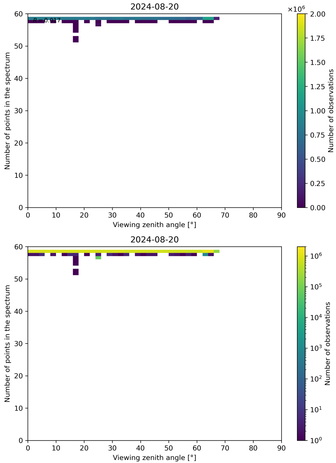
Figure 125: Scatter density plot of “Viewing zenith angle” against “Number of points in the spectrum” for 2024-08-19 to 2024-08-21.
