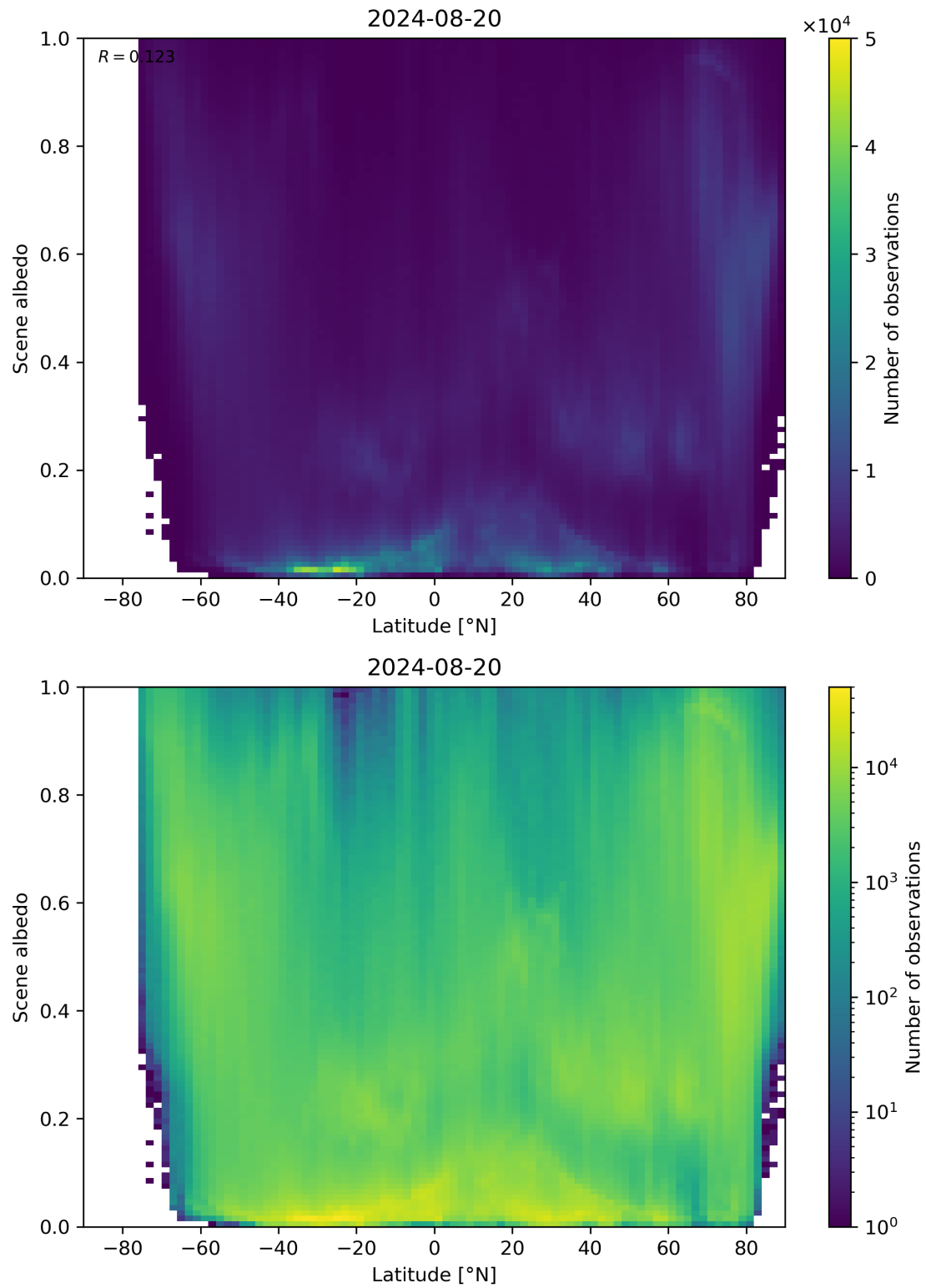
Figure 95: Scatter density plot of “Latitude” against “Scene albedo” for 2024-08-19 to 2024-08-21.
