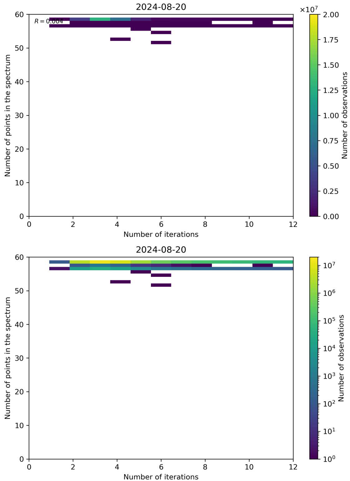
Figure 99: Scatter density plot of “Number of iterations” against “Number of points in the spectrum” for 2024-08-19 to 2024-08-21.
