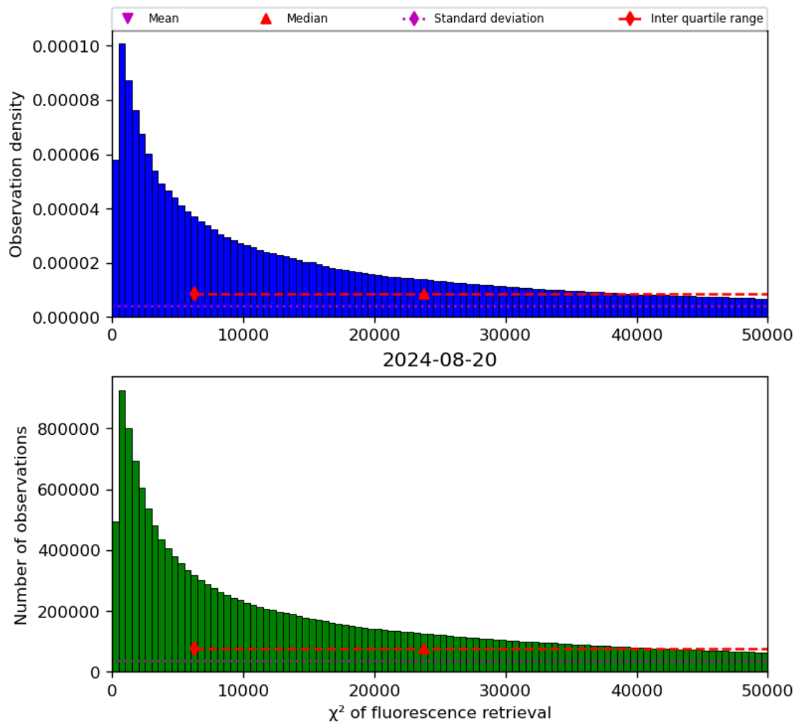
Figure 42: Histogram of “ \chi^2 of fluorescence retrieval” for 2024-08-19 to 2024-08-21
