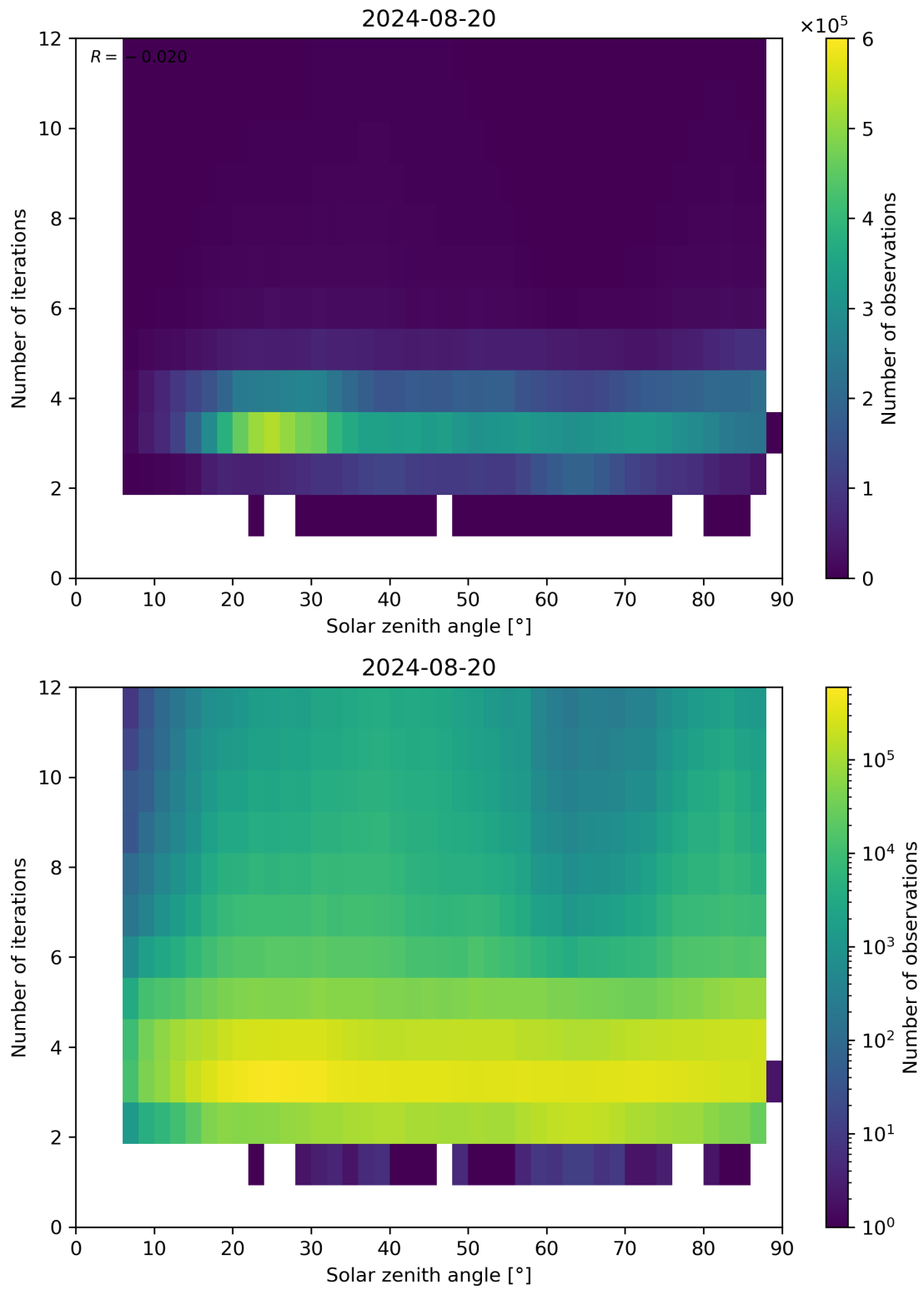
Figure 114: Scatter density plot of “Solar zenith angle” against “Number of iterations” for 2024-08-19 to 2024-08-21.
