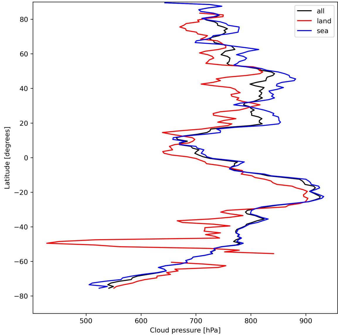
Figure 13: Zonal average of “Cloud pressure” for 2024-08-19 to 2024-08-21.
