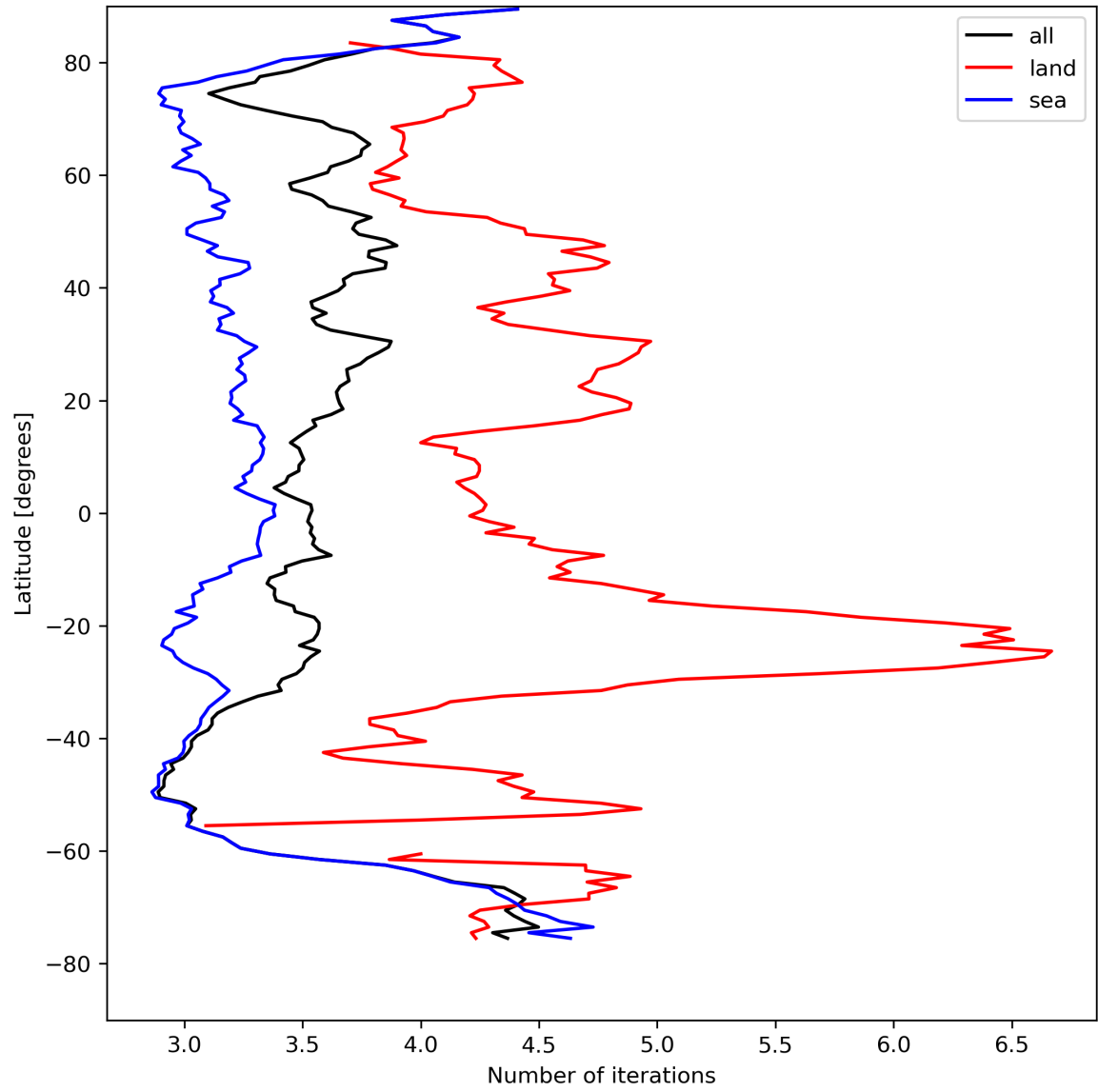
Figure 22: Zonal average of “Number of iterations” for 2024-08-19 to 2024-08-21.
