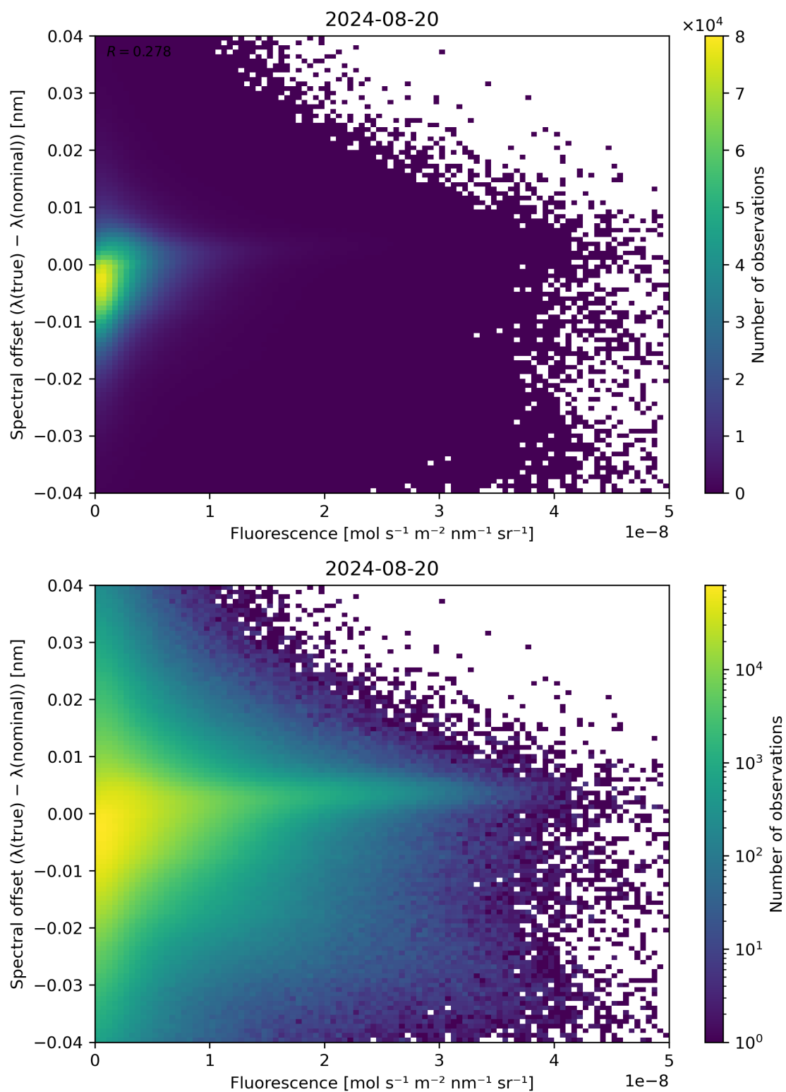
Figure 87: Scatter density plot of “Fluorescence” against “Spectral offset ( \lambda(\text{true}) - \lambda(\text{nominal}) )” for 2024-08-19 to 2024-08-21.
