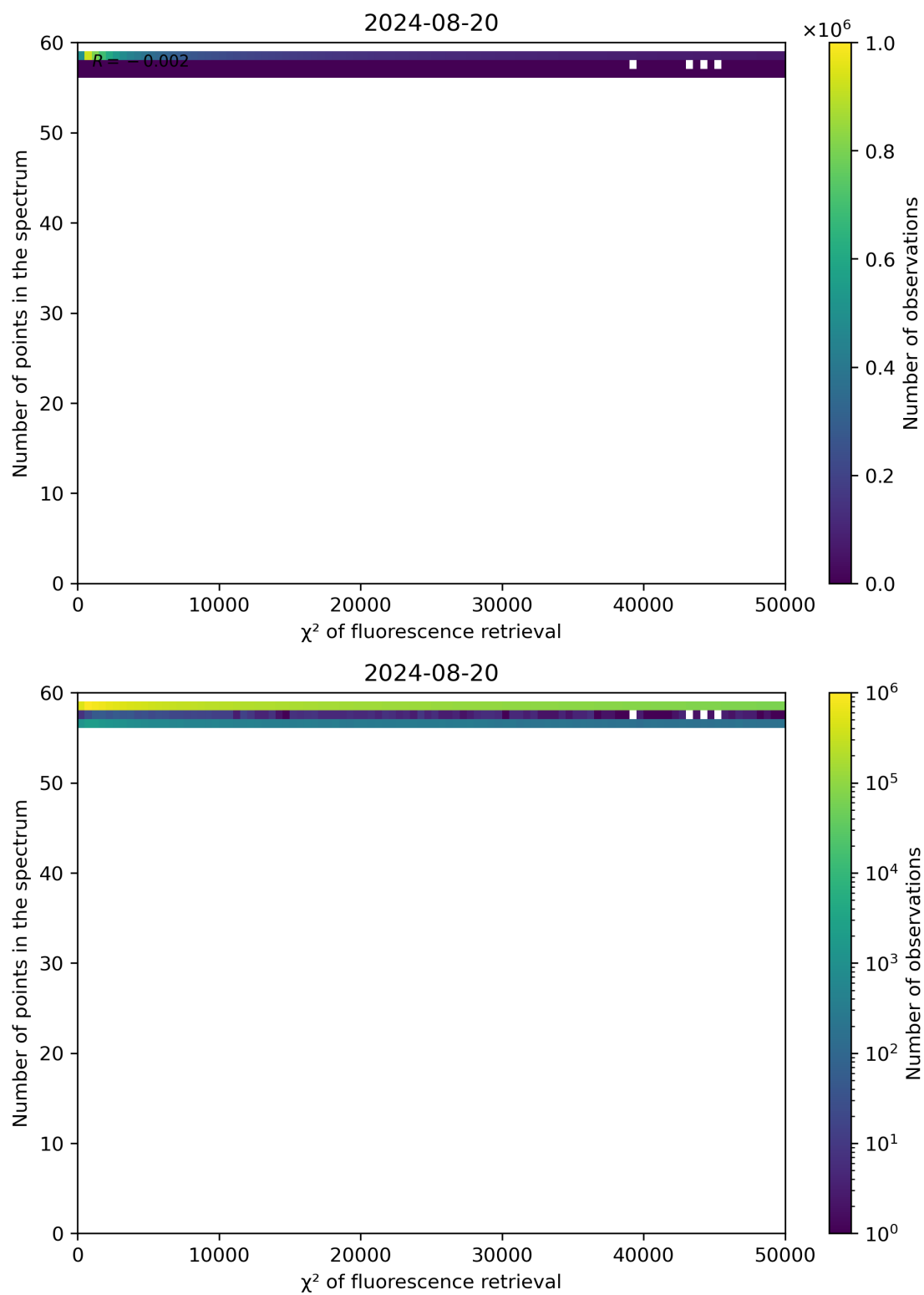
Figure 68: Scatter density plot of " \chi^2 of fluorescence retrieval" against "Number of points in the spectrum" for 2024-08-19 to 2024-08-21.
