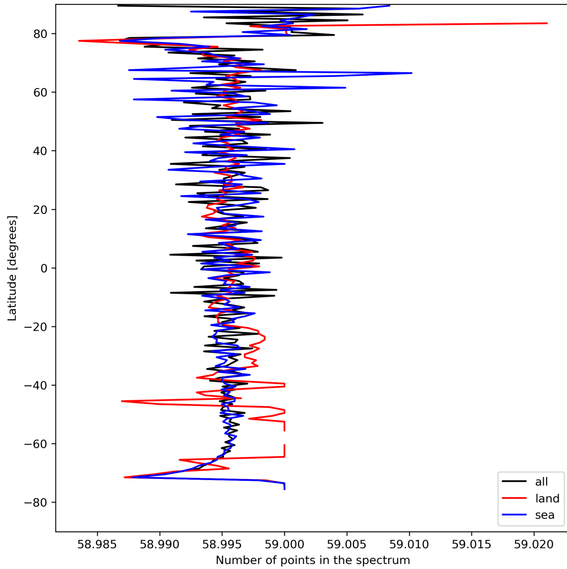
Figure 27: Zonal average of “Number of points in the spectrum” for 2024-08-19 to 2024-08-21.
