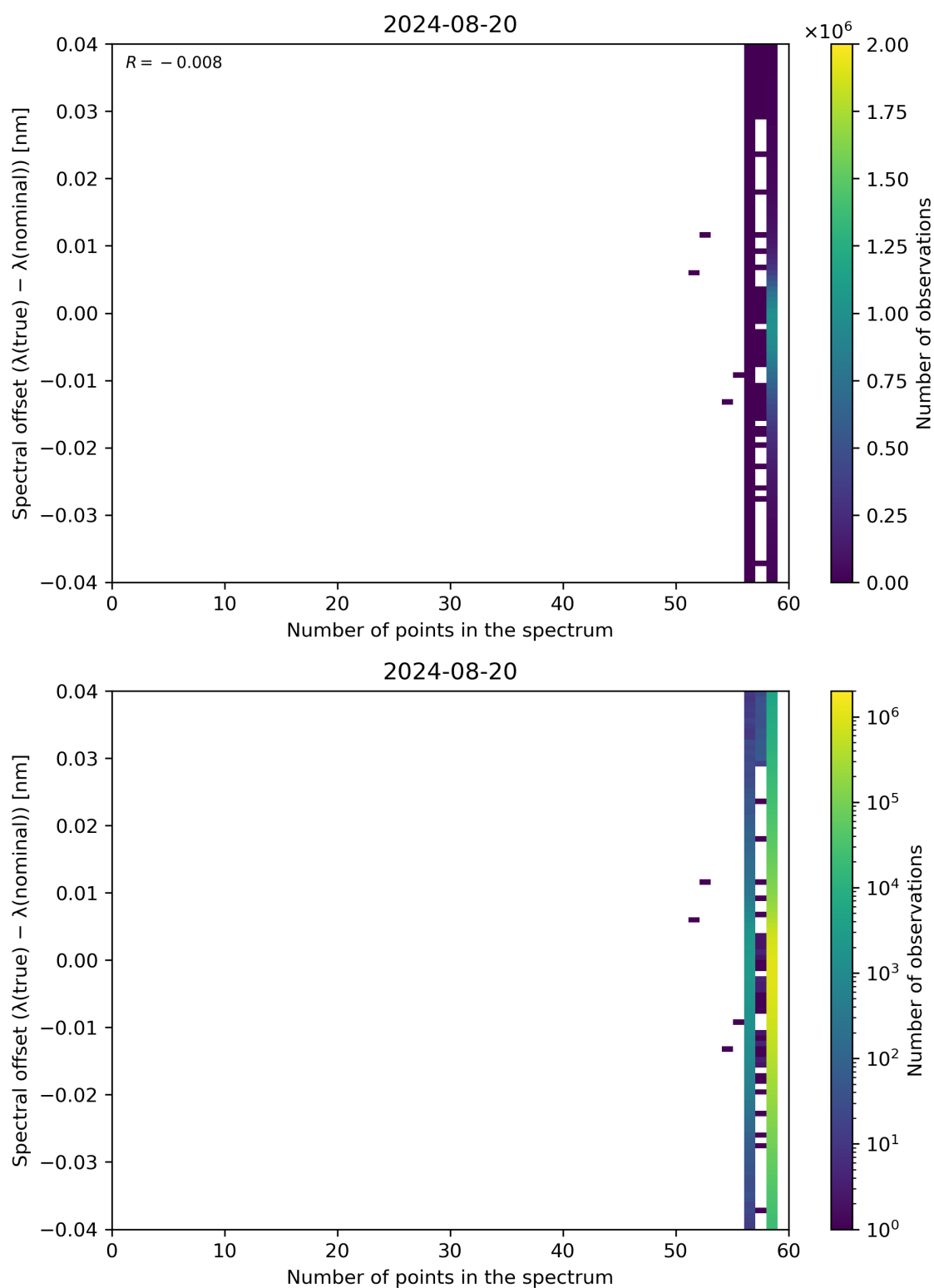
Figure 101: Scatter density plot of “Number of points in the spectrum” against “Spectral offset ( \lambda(\text{true}) - \lambda(\text{nominal}) )” for 2024-08-19 to 2024-08-21.
