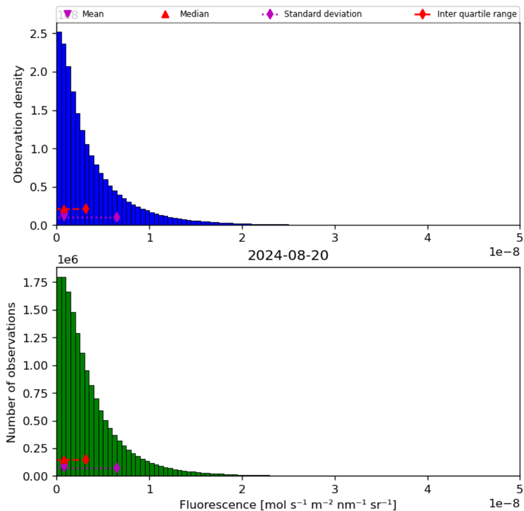
Figure 40: Histogram of “Fluorescence” for 2024-08-19 to 2024-08-21
