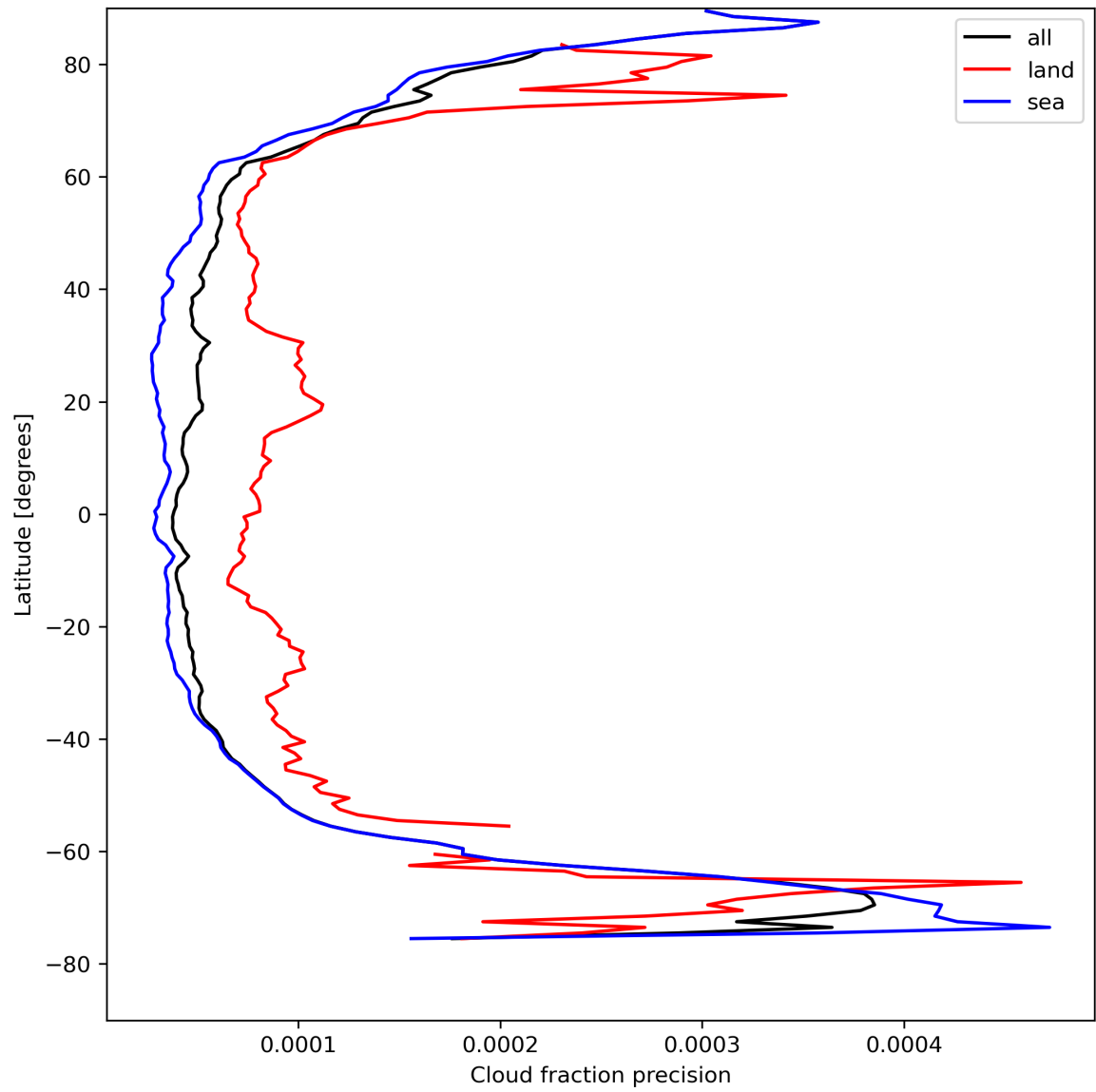
Figure 16: Zonal average of “Cloud fraction precision” for 2024-08-19 to 2024-08-21.
