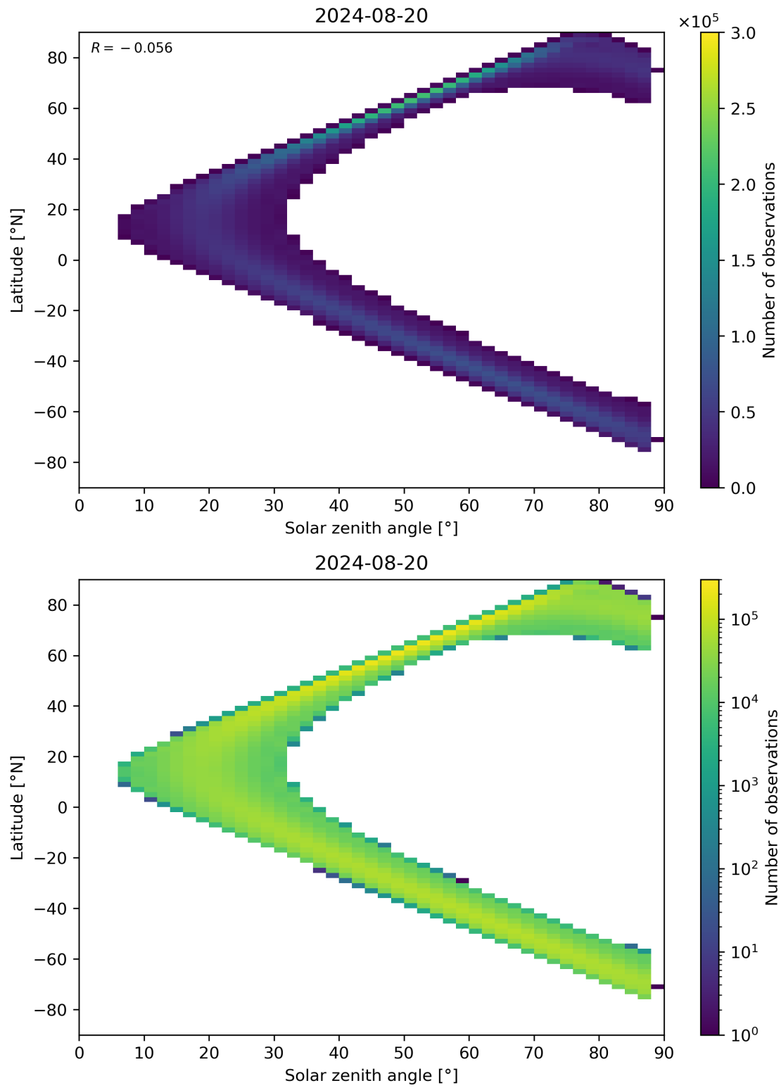
Figure 113: Scatter density plot of “Solar zenith angle” against “Latitude” for 2024-08-19 to 2024-08-21.
