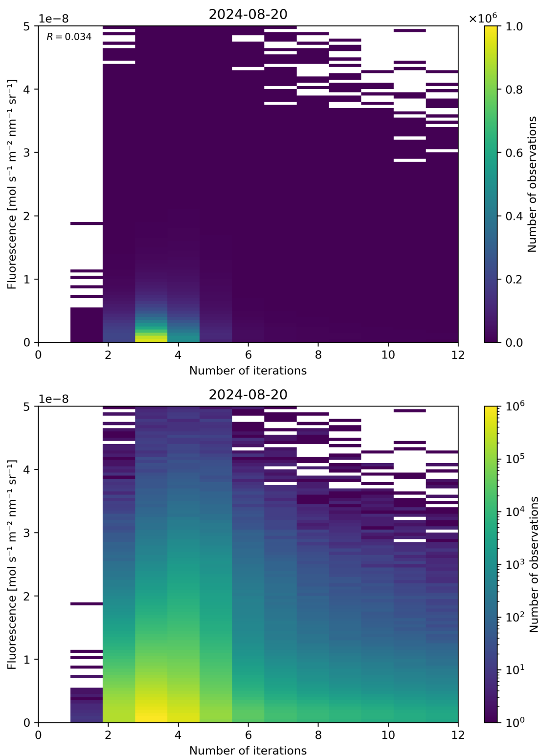
Figure 98: Scatter density plot of “Number of iterations” against “Fluorescence” for 2024-08-19 to 2024-08-21.
