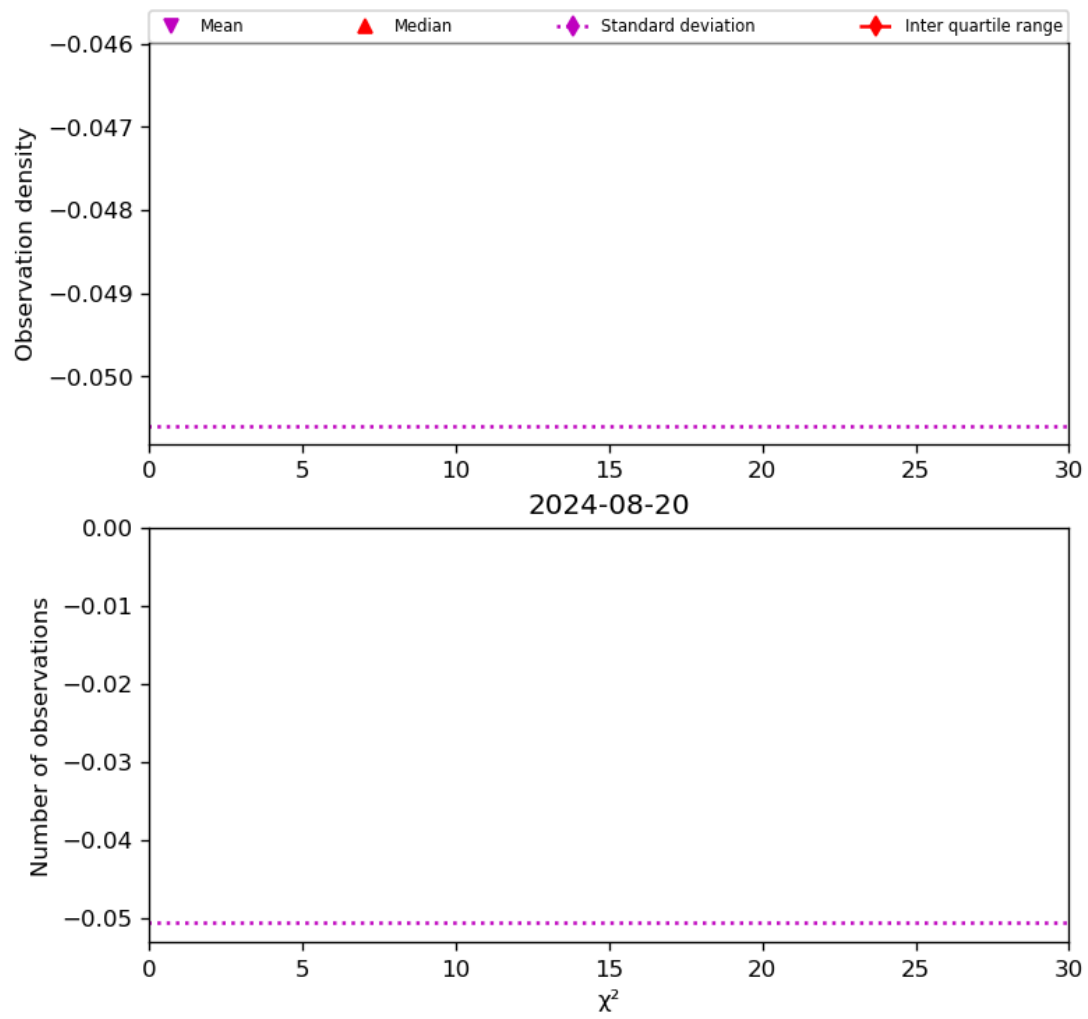
Figure 38: Histogram of " \chi^2 " for 2024-08-19 to 2024-08-21
