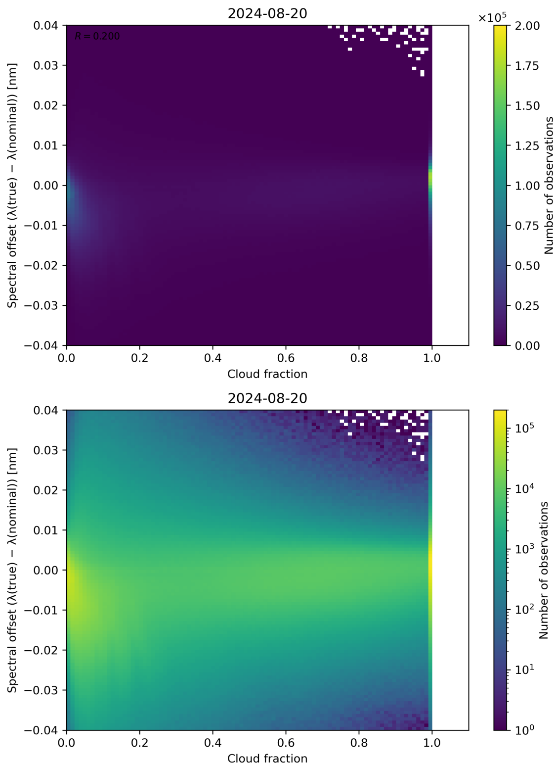
Figure 76: Scatter density plot of “Cloud fraction” against “Spectral offset ( \lambda(\text{true}) - \lambda(\text{nominal}) )” for 2024-08-19 to 2024-08-21.
