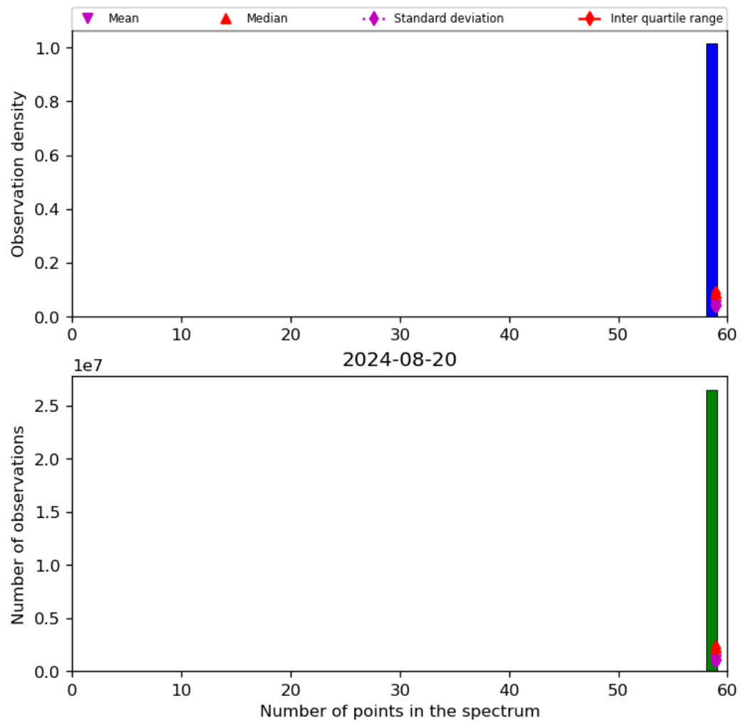
Figure 44: Histogram of "Number of points in the spectrum" for 2024-08-19 to 2024-08-21
