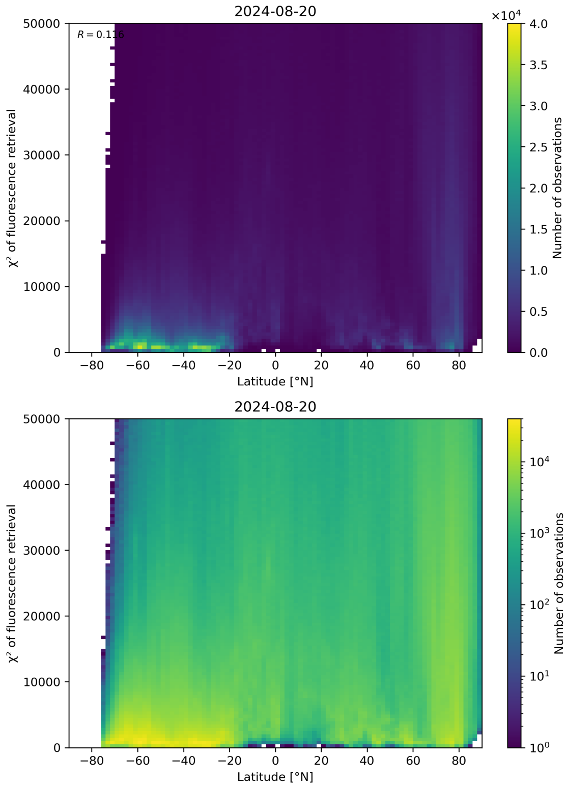
Figure 89: Scatter density plot of “Latitude” against “ \chi^2 of fluorescence retrieval” for 2024-08-19 to 2024-08-21.
