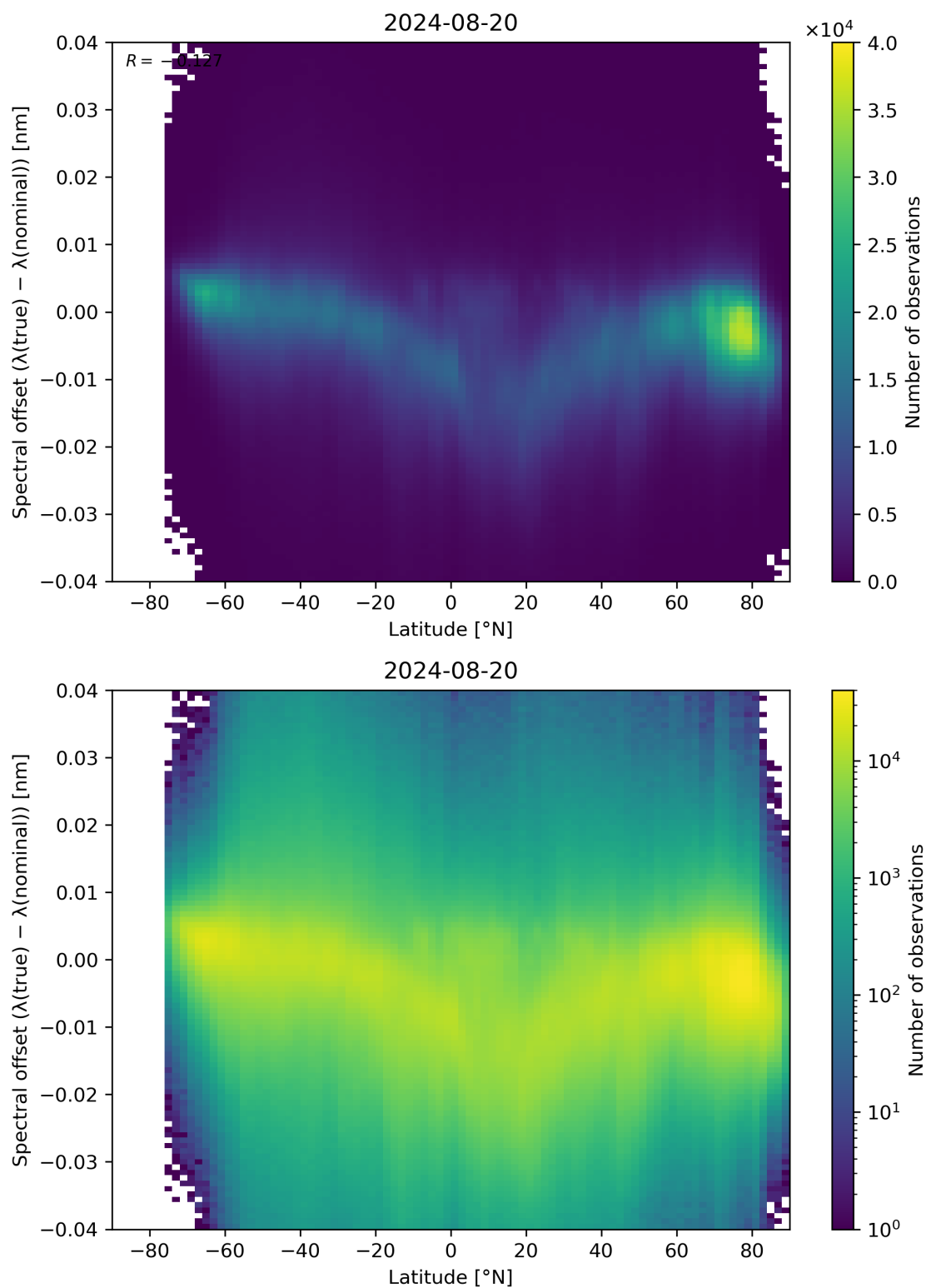
Figure 96: Scatter density plot of “Latitude” against “Spectral offset ( \lambda(\text{true}) - \lambda(\text{nominal}) )” for 2024-08-19 to 2024-08-21.
