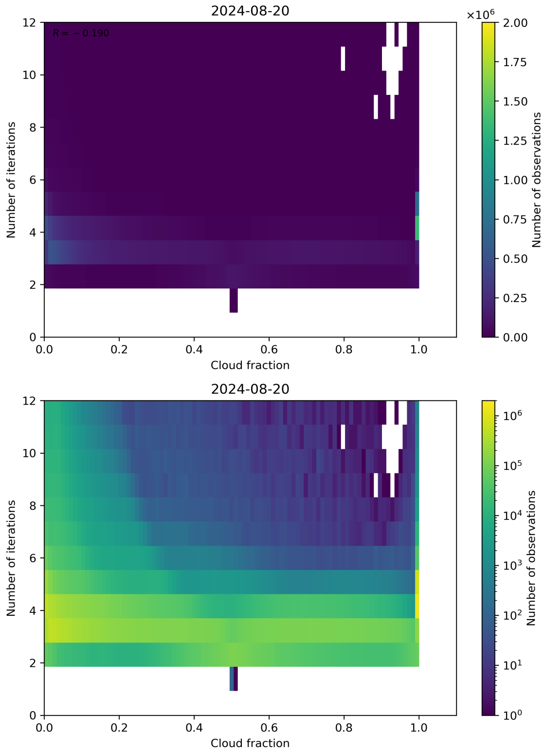
Figure 73: Scatter density plot of “Cloud fraction” against “Number of iterations” for 2024-08-19 to 2024-08-21.
