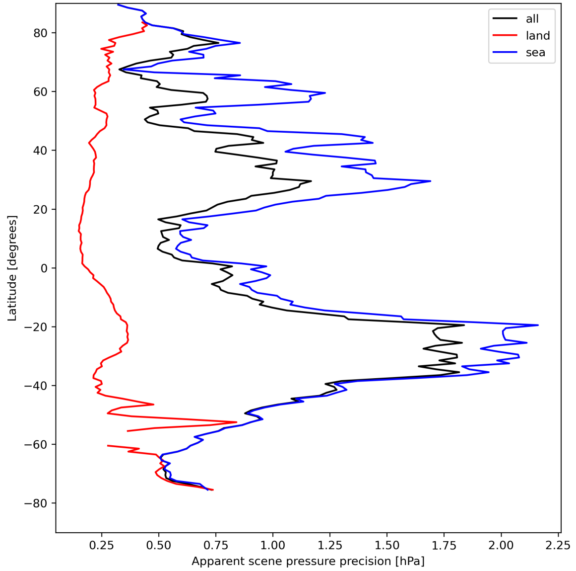
Figure 20: Zonal average of “Apparent scene pressure precision” for 2024-08-19 to 2024-08-21.
