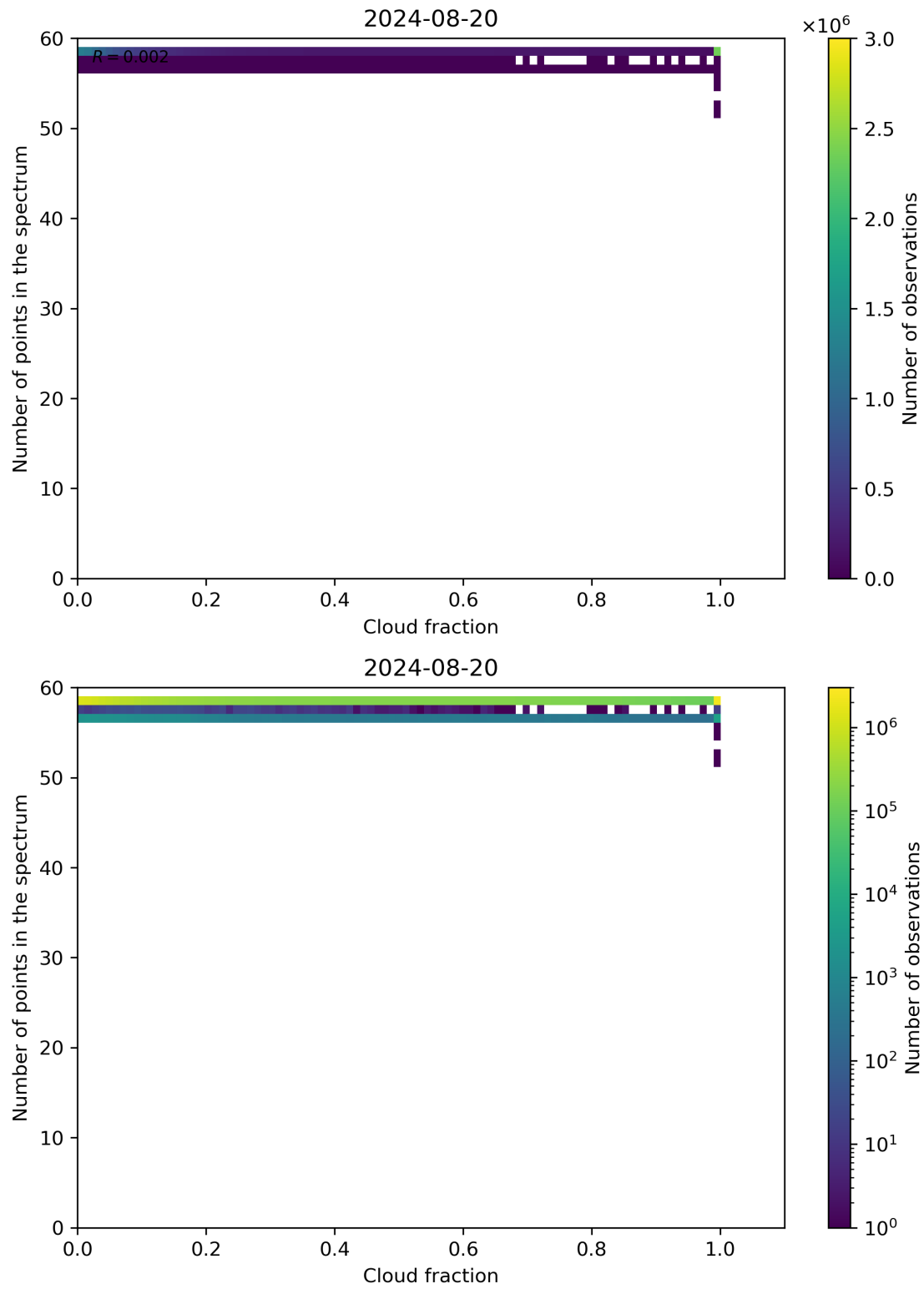
Figure 74: Scatter density plot of “Cloud fraction” against “Number of points in the spectrum” for 2024-08-19 to 2024-08-21.
