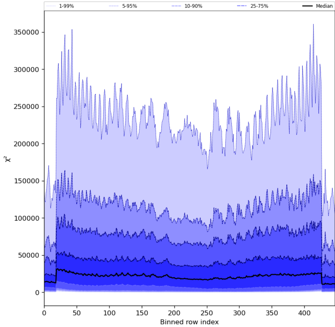
Figure 55: Along track statistics of “ \chi^2 ” for 2024-08-19 to 2024-08-21
