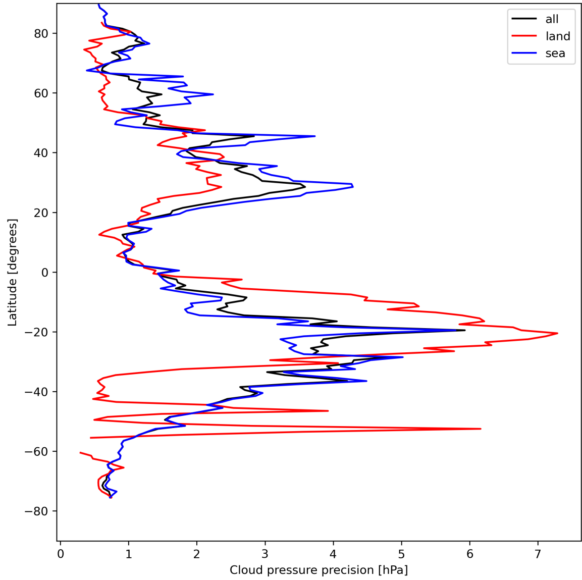
Figure 14: Zonal average of “Cloud pressure precision” for 2024-08-19 to 2024-08-21.
