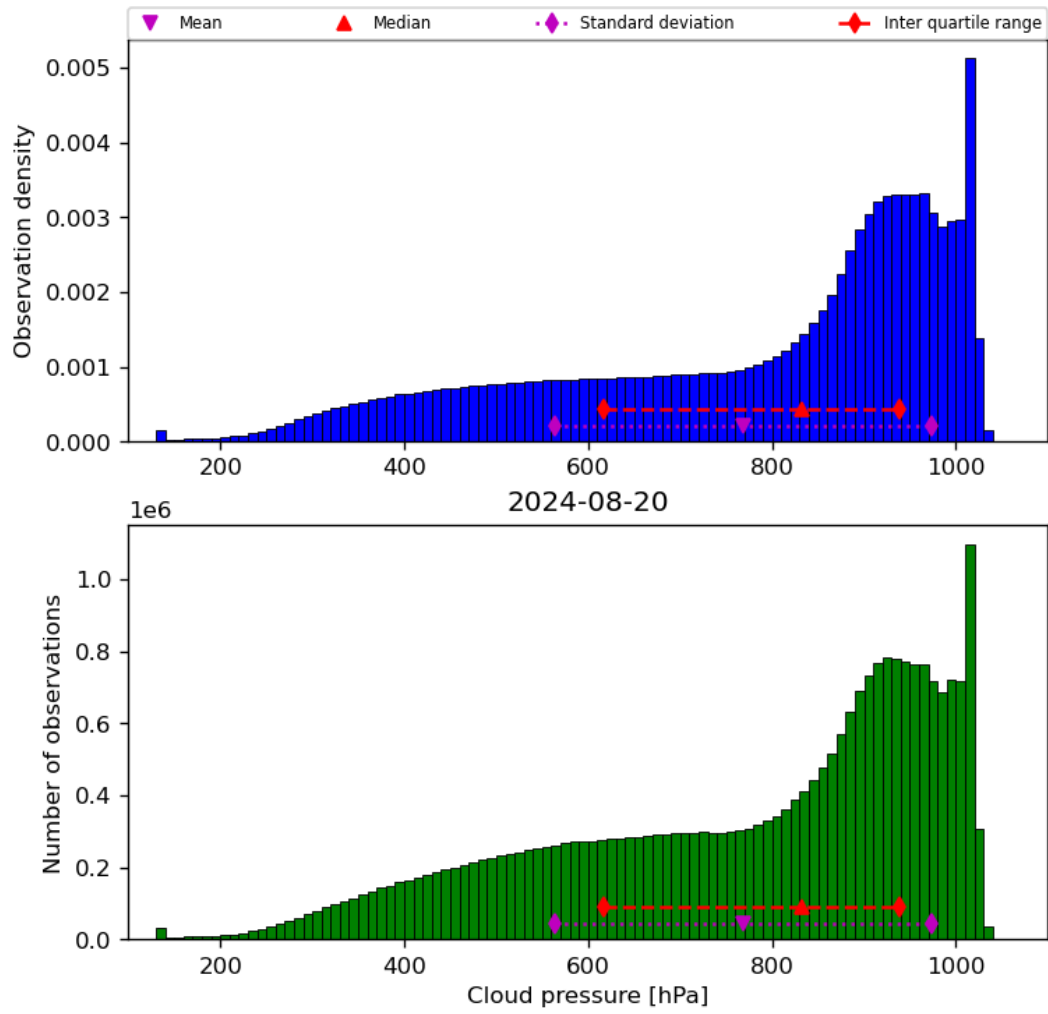
Figure 30: Histogram of “Cloud pressure” for 2024-08-19 to 2024-08-21
