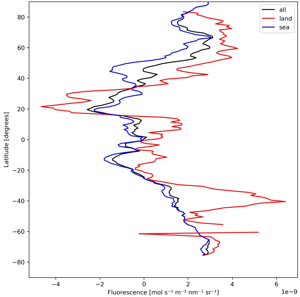
Figure 23: Zonal average of “Fluorescence” for 2024-08-19 to 2024-08-21.
