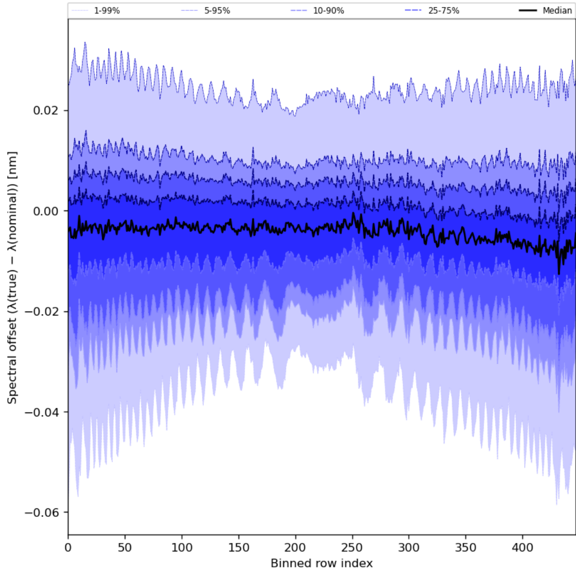
Figure 62: Along track statistics of “Spectral offset ( \lambda(\text{true}) - \lambda(\text{nominal}) )” for 2024-08-19 to 2024-08-21
