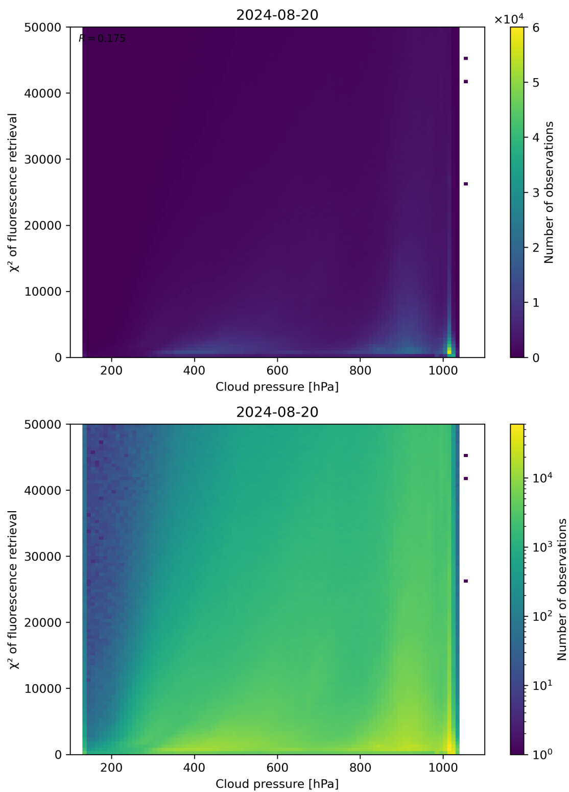
Figure 78: Scatter density plot of “Cloud pressure” against “ \chi^2 of fluorescence retrieval” for 2024-08-19 to 2024-08-21.
