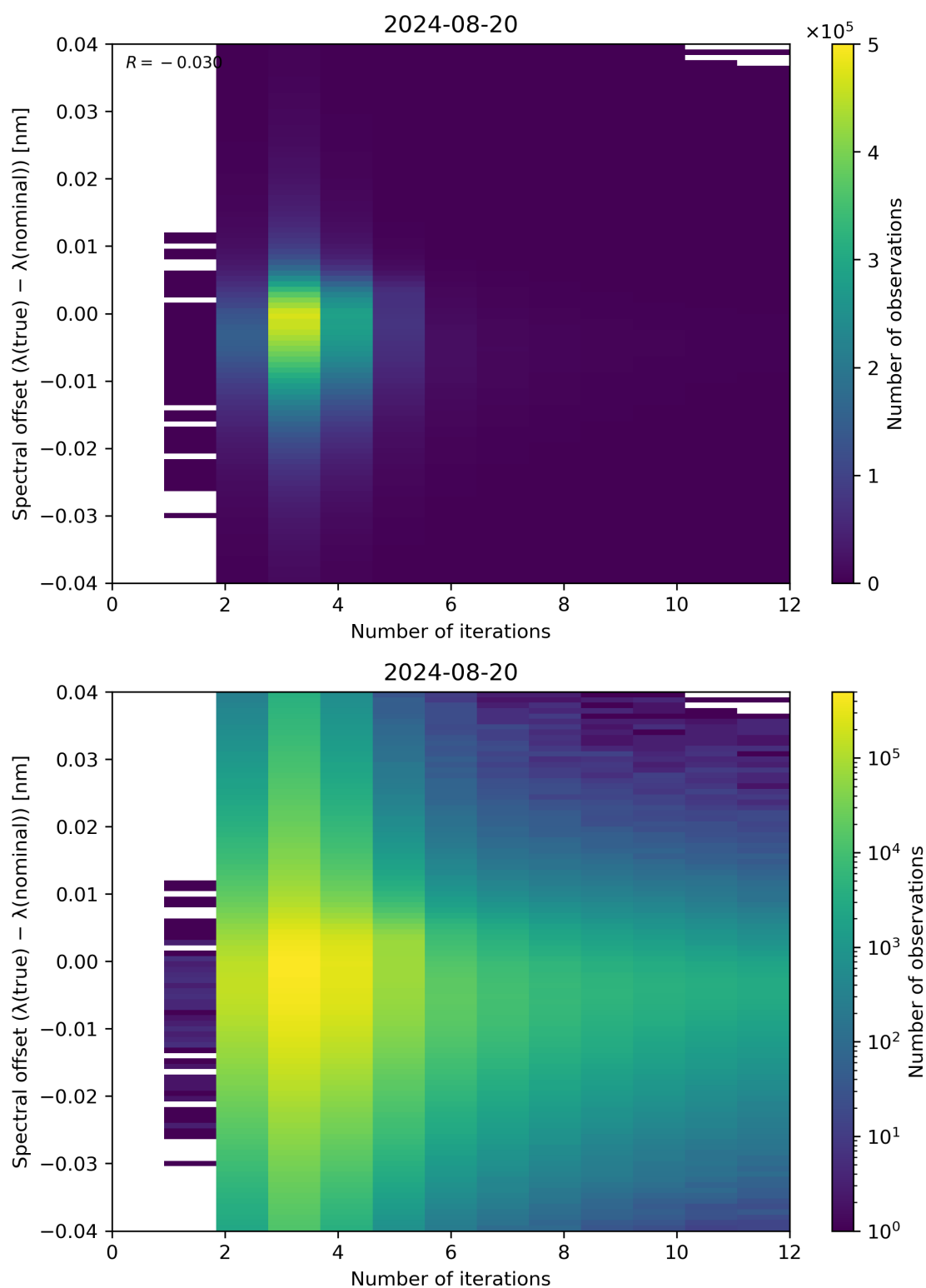
Figure 100: Scatter density plot of “Number of iterations” against “Spectral offset ( \lambda(\text{true}) - \lambda(\text{nominal}) )” for 2024-08-19 to 2024-08-21.
