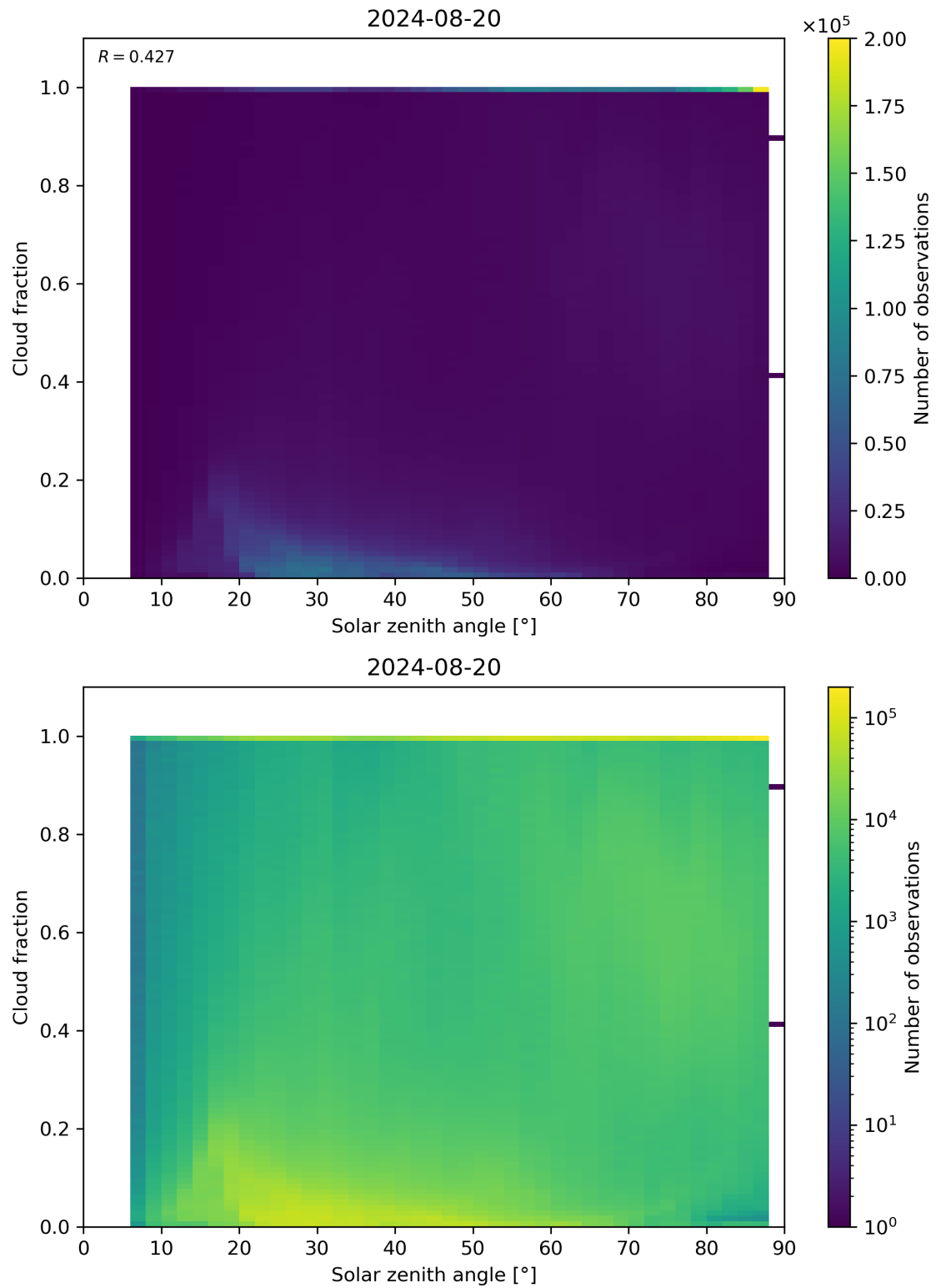
Figure 110: Scatter density plot of “Solar zenith angle” against “Cloud fraction” for 2024-08-19 to 2024-08-21.
