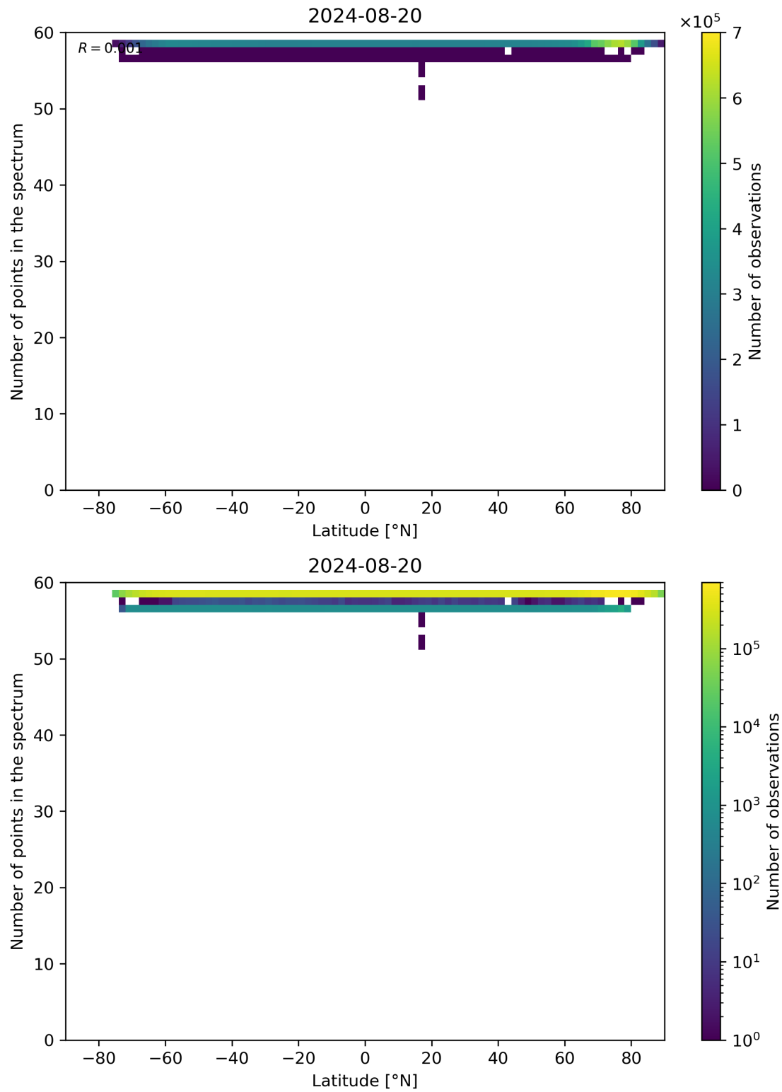
Figure 94: Scatter density plot of “Latitude” against “Number of points in the spectrum” for 2024-08-19 to 2024-08-21.
