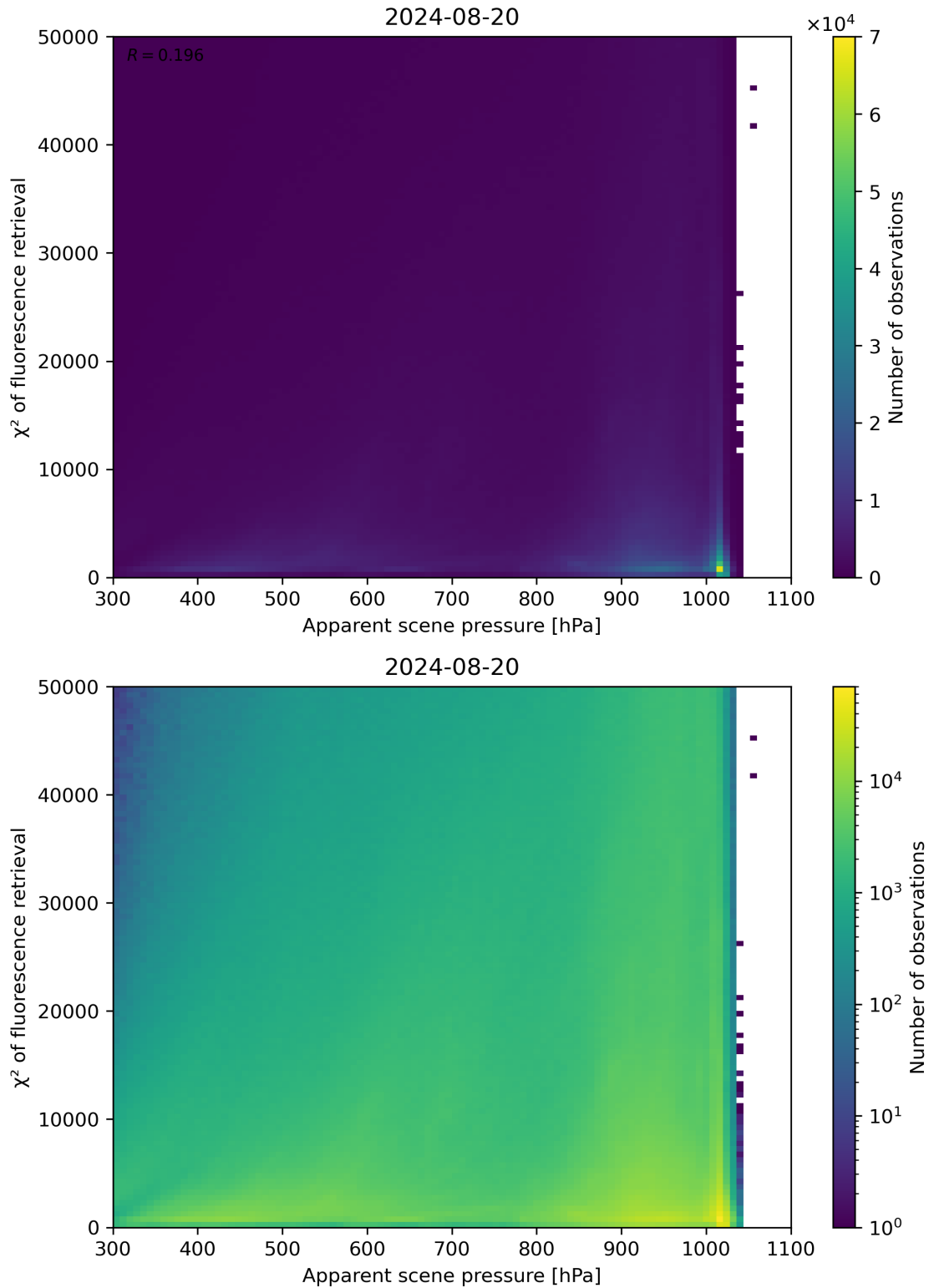
Figure 63: Scatter density plot of “Apparent scene pressure” against “ \chi^2 of fluorescence retrieval” for 2024-08-19 to 2024-08-21.
