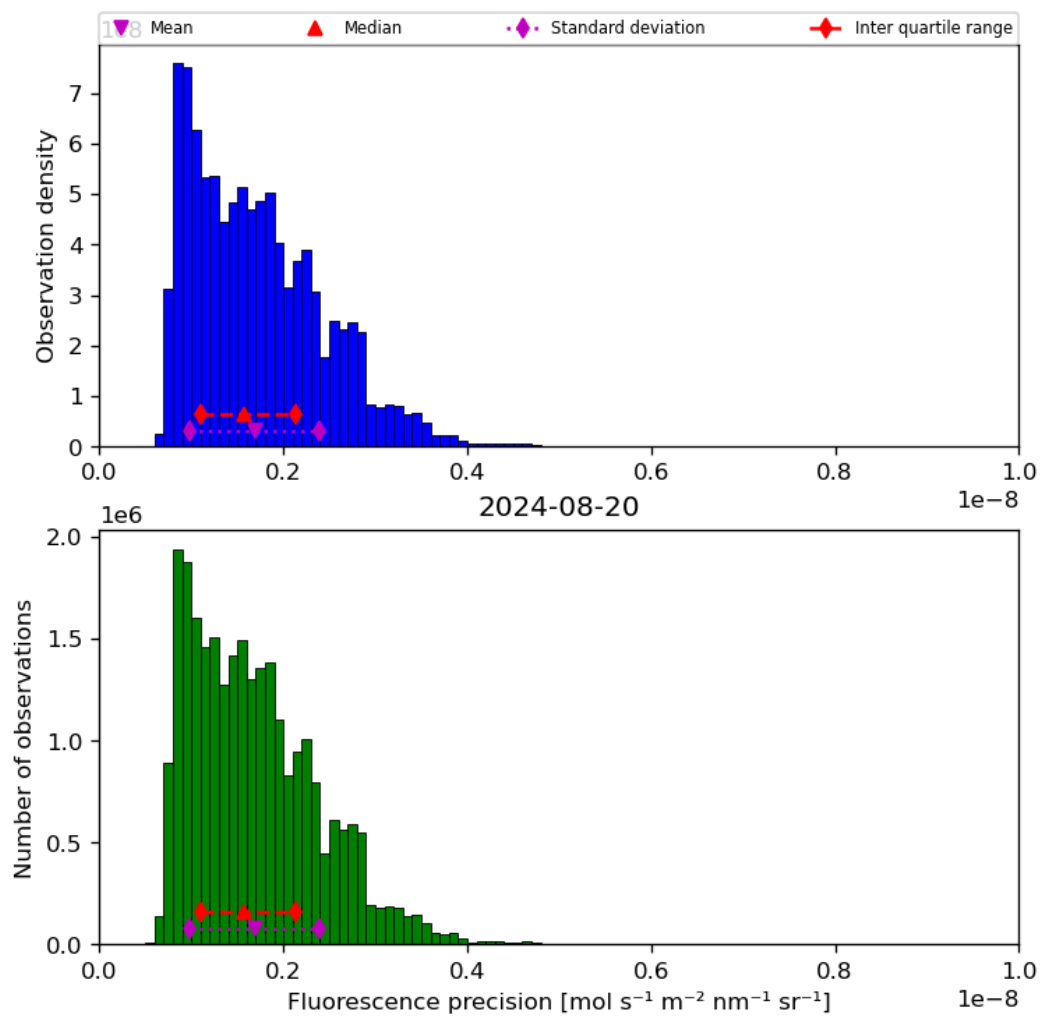
Figure 41: Histogram of “Fluorescence precision” for 2024-08-19 to 2024-08-21
