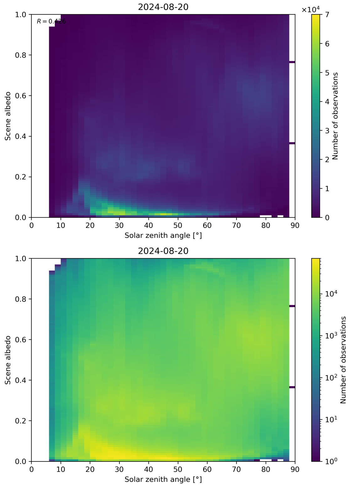
Figure 116: Scatter density plot of “Solar zenith angle” against “Scene albedo” for 2024-08-19 to 2024-08-21.
