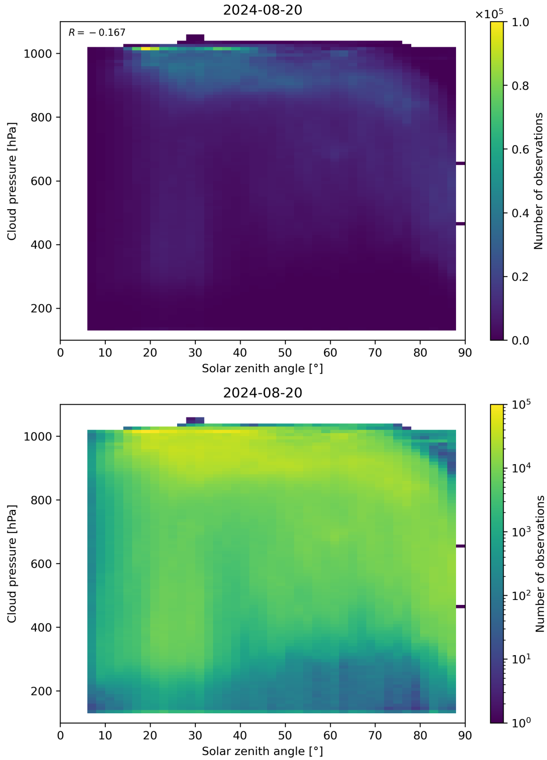
Figure 111: Scatter density plot of “Solar zenith angle” against “Cloud pressure” for 2024-08-19 to 2024-08-21.
