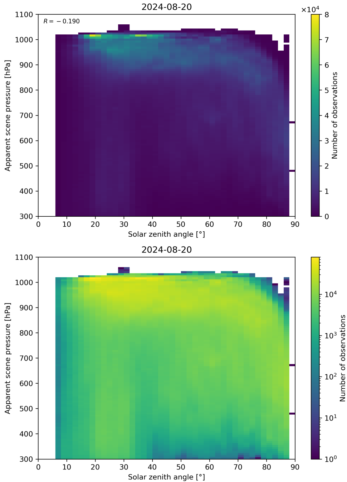
Figure 108: Scatter density plot of “Solar zenith angle” against “Apparent scene pressure” for 2024-08-19 to 2024-08-21.
