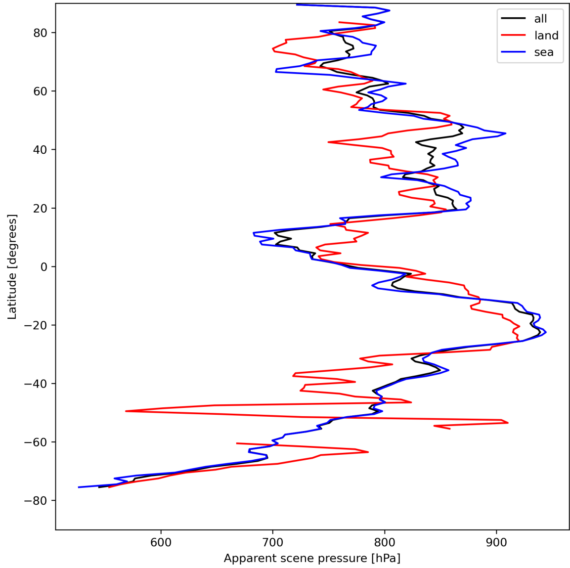
Figure 19: Zonal average of “Apparent scene pressure” for 2024-08-19 to 2024-08-21.
