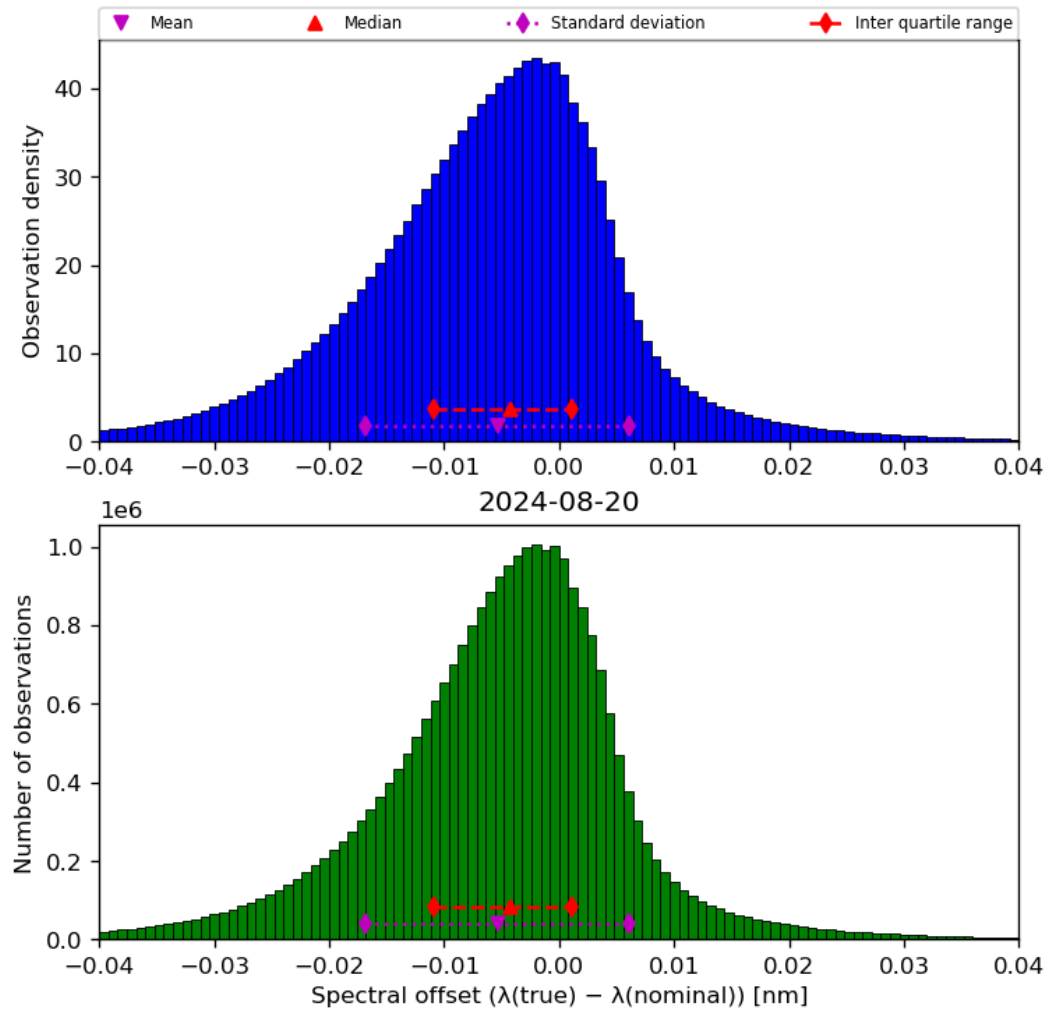
Figure 45: Histogram of “Spectral offset ( \lambda(\text{true}) - \lambda(\text{nominal}) )” for 2024-08-19 to 2024-08-21
