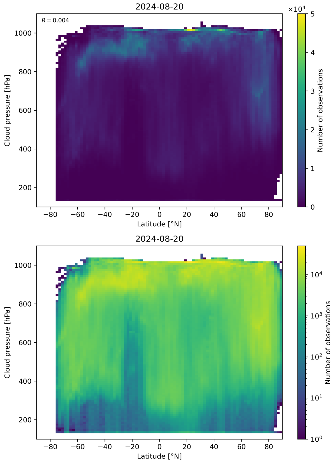
Figure 91: Scatter density plot of “Latitude” against “Cloud pressure” for 2024-08-19 to 2024-08-21.
