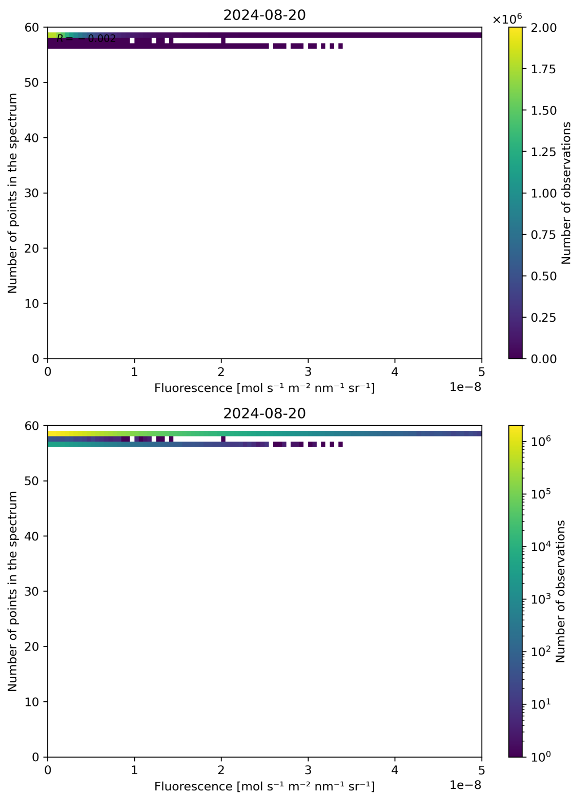
Figure 86: Scatter density plot of “Fluorescence” against “Number of points in the spectrum” for 2024-08-19 to 2024-08-21.
