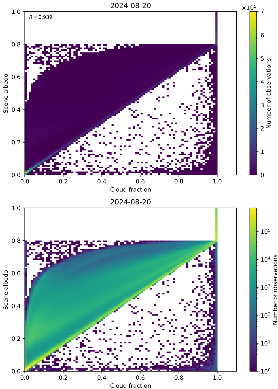
Figure 75: Scatter density plot of “Cloud fraction” against “Scene albedo” for 2024-08-19 to 2024-08-21.
