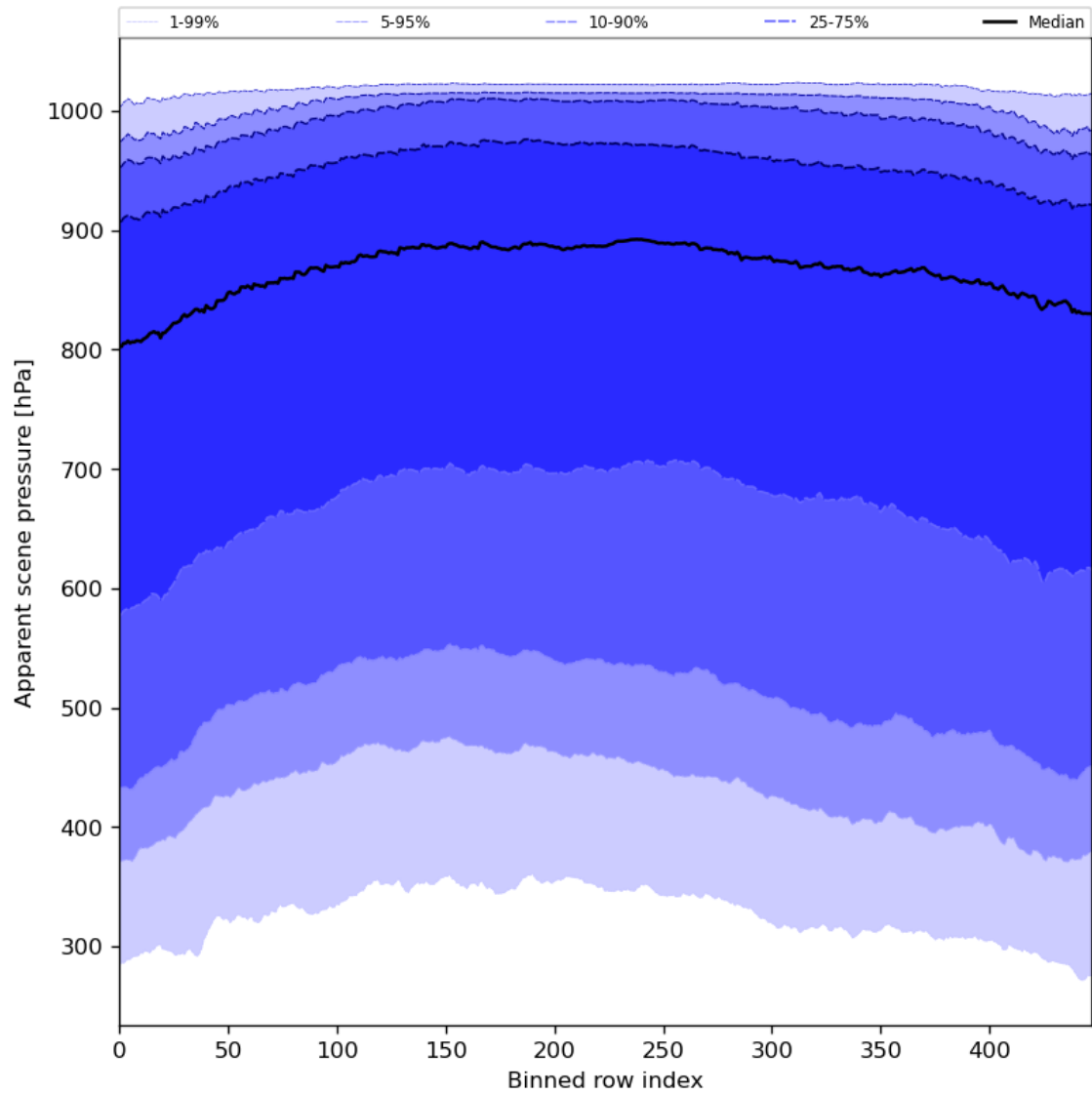
Figure 53: Along track statistics of “Apparent scene pressure” for 2024-08-19 to 2024-08-21
