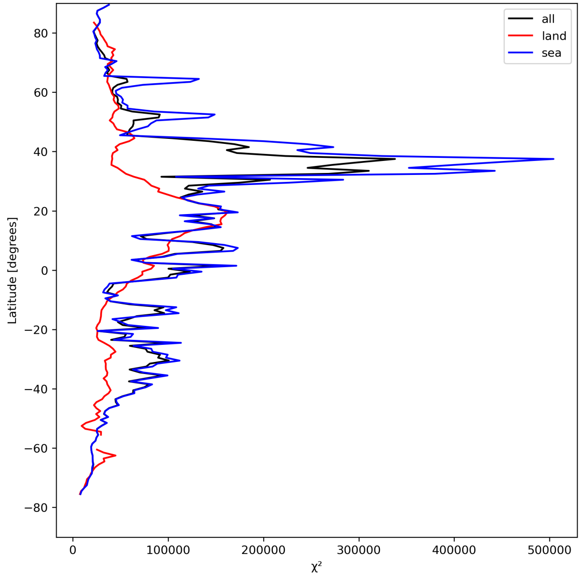
Figure 21: Zonal average of “ \chi^2 ” for 2024-08-19 to 2024-08-21.
