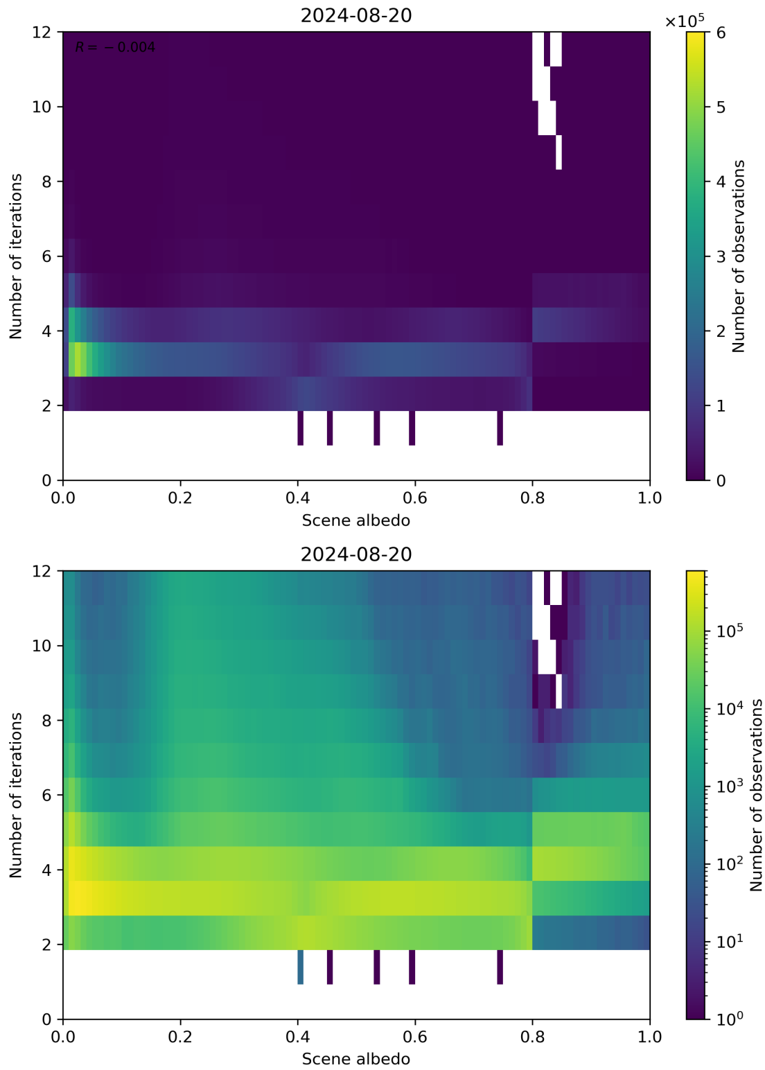
Figure 105: Scatter density plot of “Scene albedo” against “Number of iterations” for 2024-08-19 to 2024-08-21.
