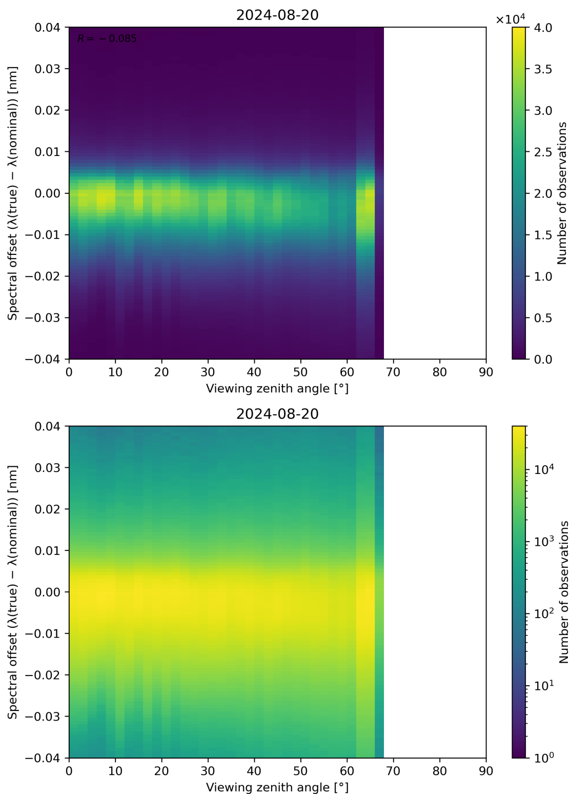
Figure 128: Scatter density plot of “Viewing zenith angle” against “Spectral offset ( \lambda(\text{true}) - \lambda(\text{nominal}) )” for 2024-08-19 to 2024-08-21.
