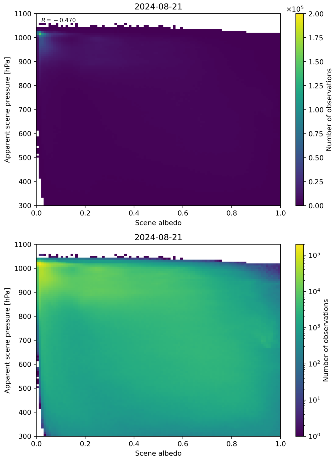
Figure 102: Scatter density plot of “Scene albedo” against “Apparent scene pressure” for 2024-08-21 to 2024-08-22.
