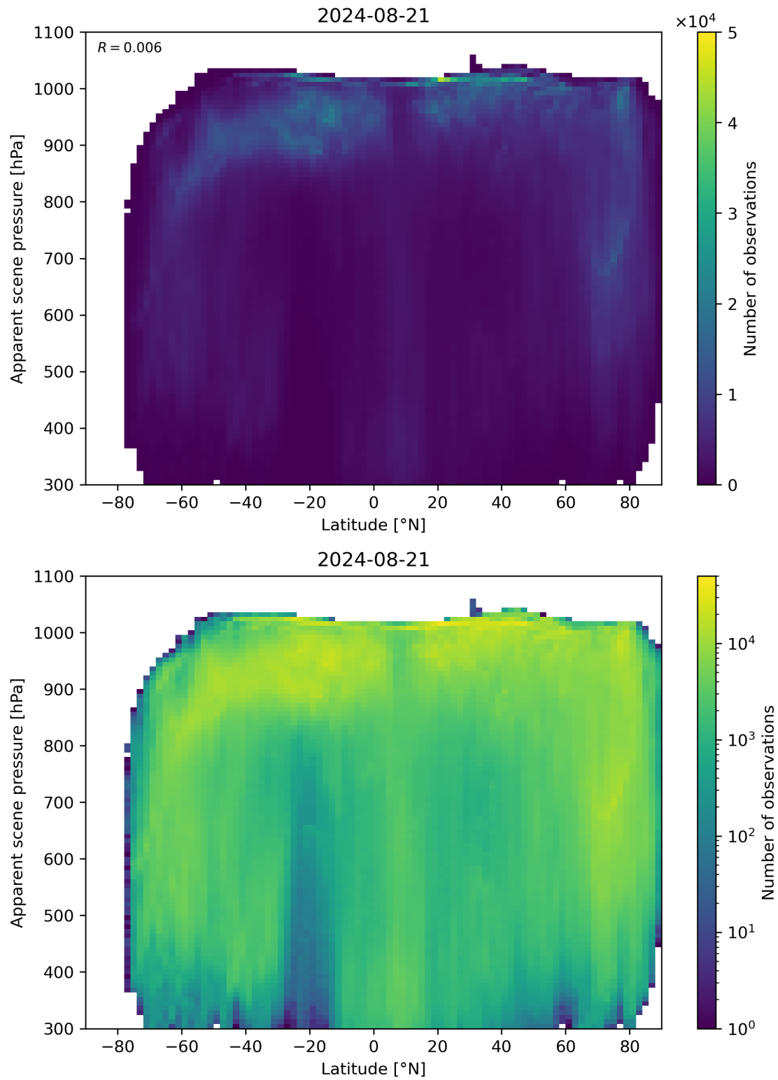
Figure 88: Scatter density plot of “Latitude” against “Apparent scene pressure” for 2024-08-21 to 2024-08-22.
