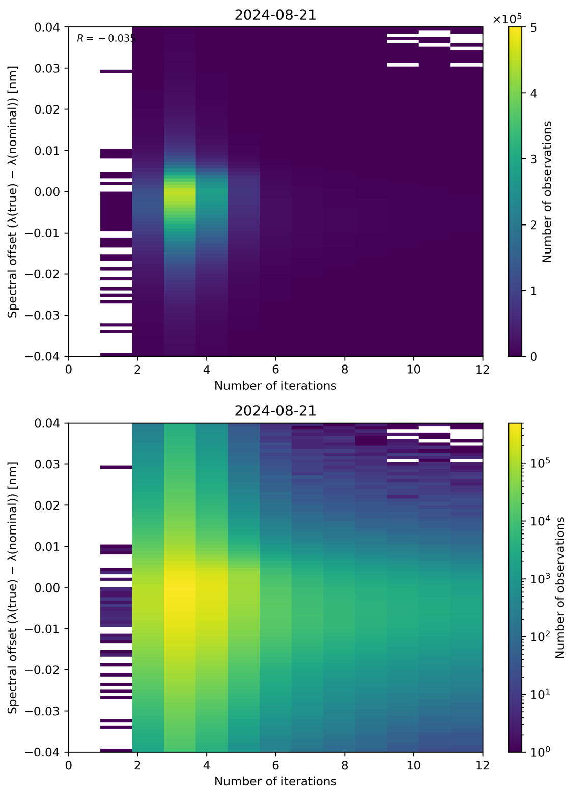
Figure 100: Scatter density plot of “Number of iterations” against “Spectral offset ( \lambda(\text{true}) - \lambda(\text{nominal}) )” for 2024-08-21 to 2024-08-22.
