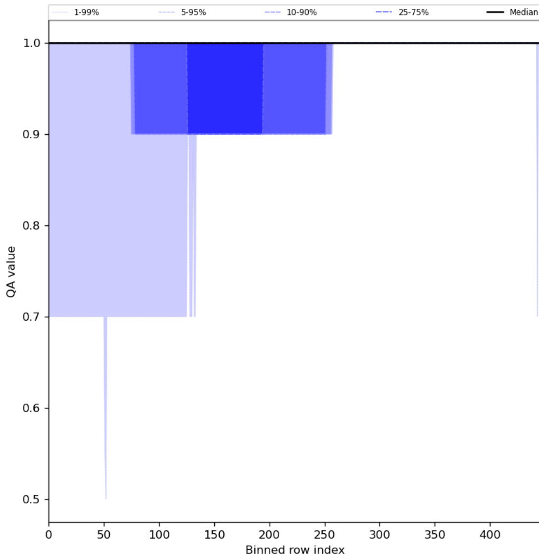
Figure 46: Along track statistics of “QA value” for 2024-08-21 to 2024-08-22
