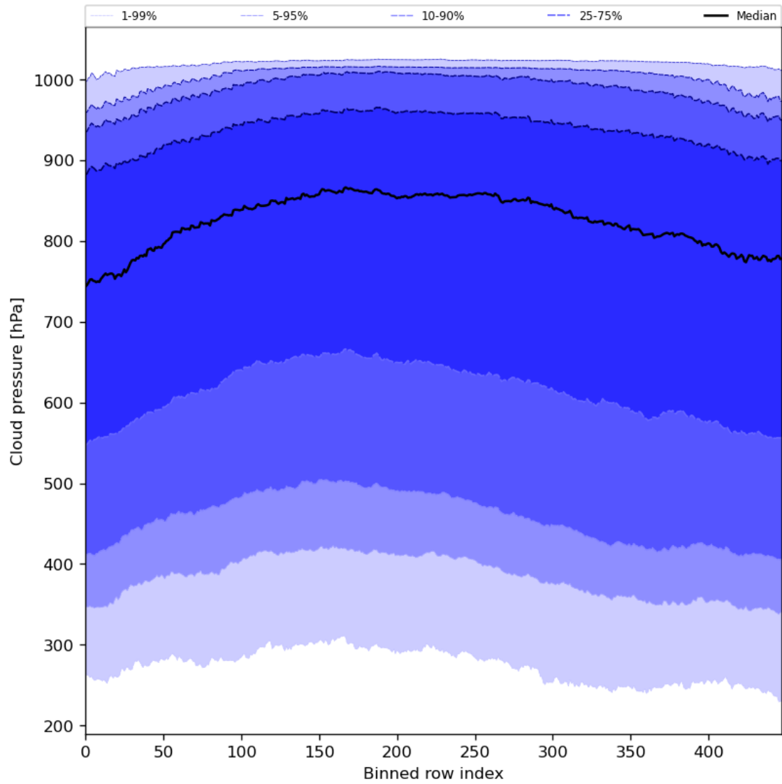
Figure 47: Along track statistics of “Cloud pressure” for 2024-08-21 to 2024-08-22
