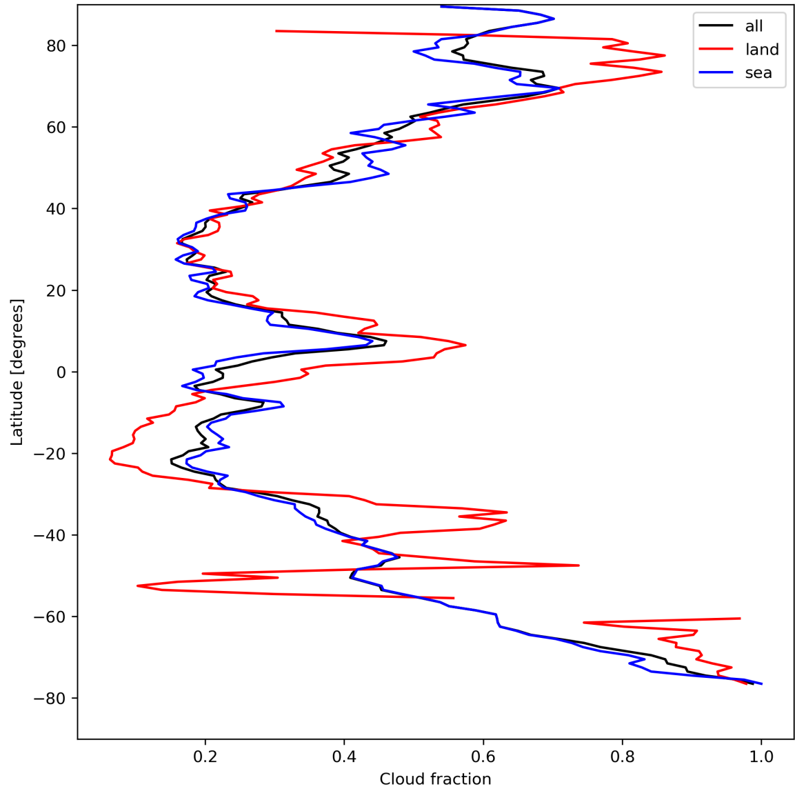
Figure 15: Zonal average of “Cloud fraction” for 2024-08-21 to 2024-08-22.
