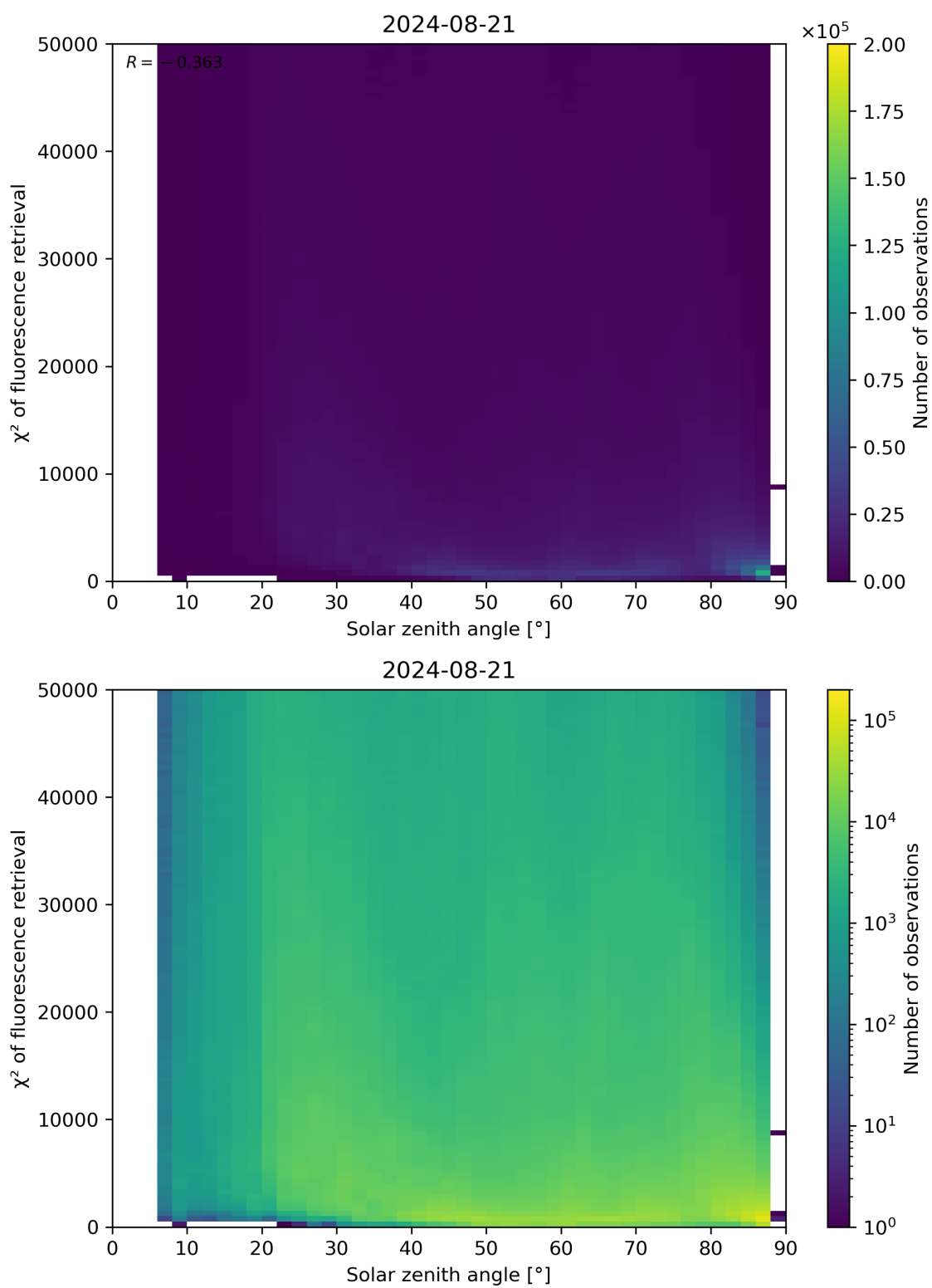
Figure 109: Scatter density plot of “Solar zenith angle” against “ \chi^2 of fluorescence retrieval” for 2024-08-21 to 2024-08-22.
