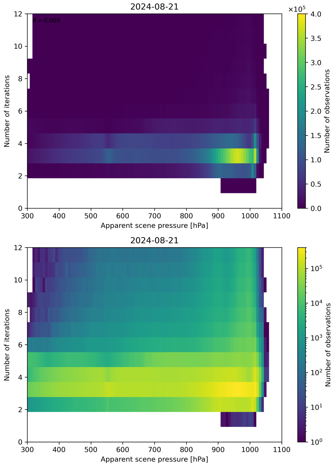
Figure 65: Scatter density plot of “Apparent scene pressure” against “Number of iterations” for 2024-08-21 to 2024-08-22.
