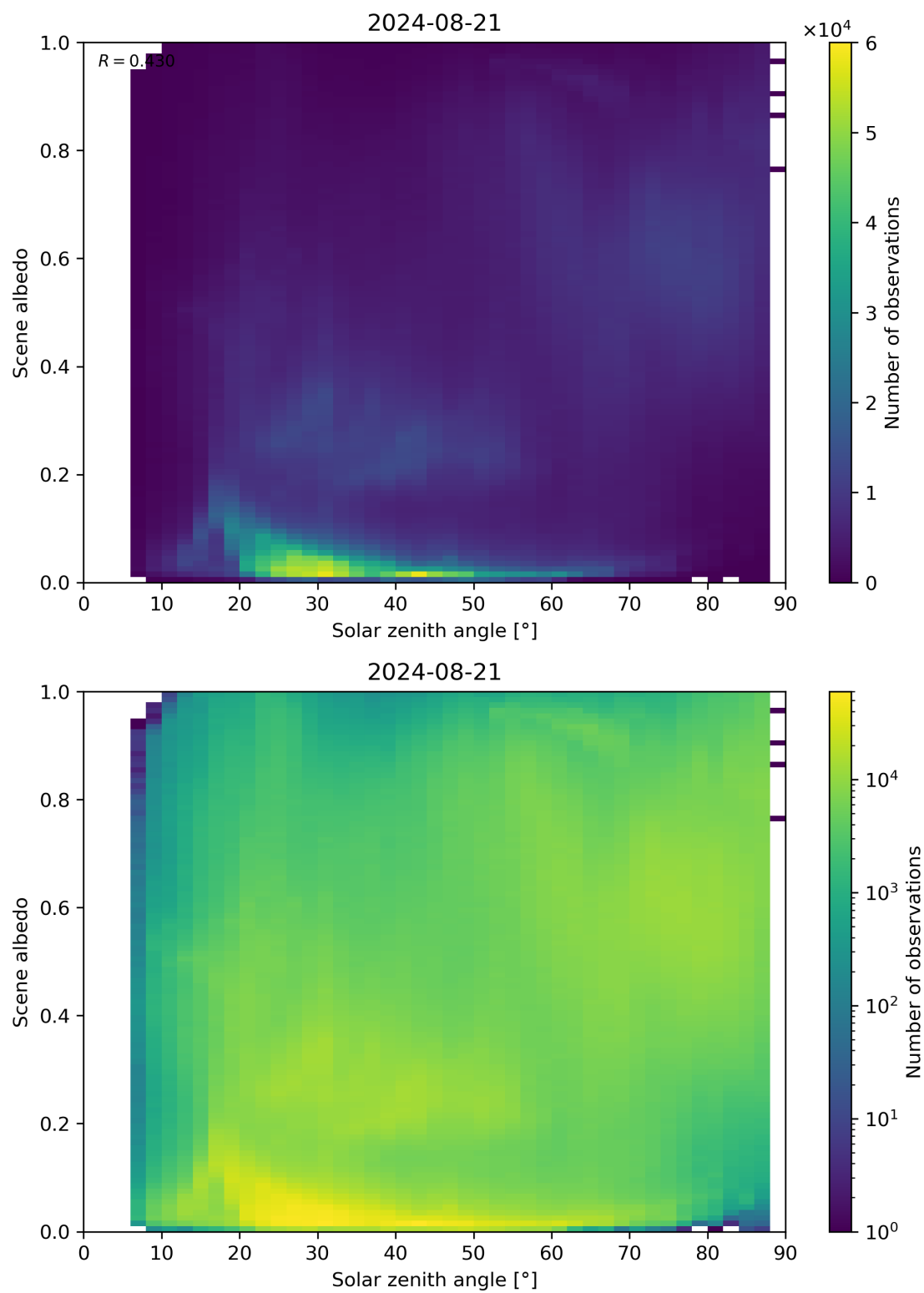
Figure 116: Scatter density plot of “Solar zenith angle” against “Scene albedo” for 2024-08-21 to 2024-08-22.
