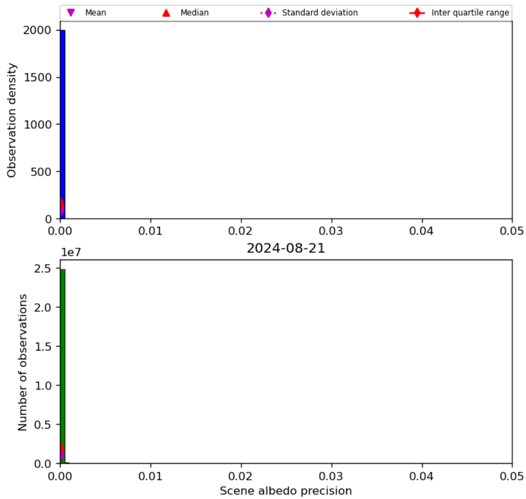
Figure 35: Histogram of “Scene albedo precision” for 2024-08-21 to 2024-08-22
