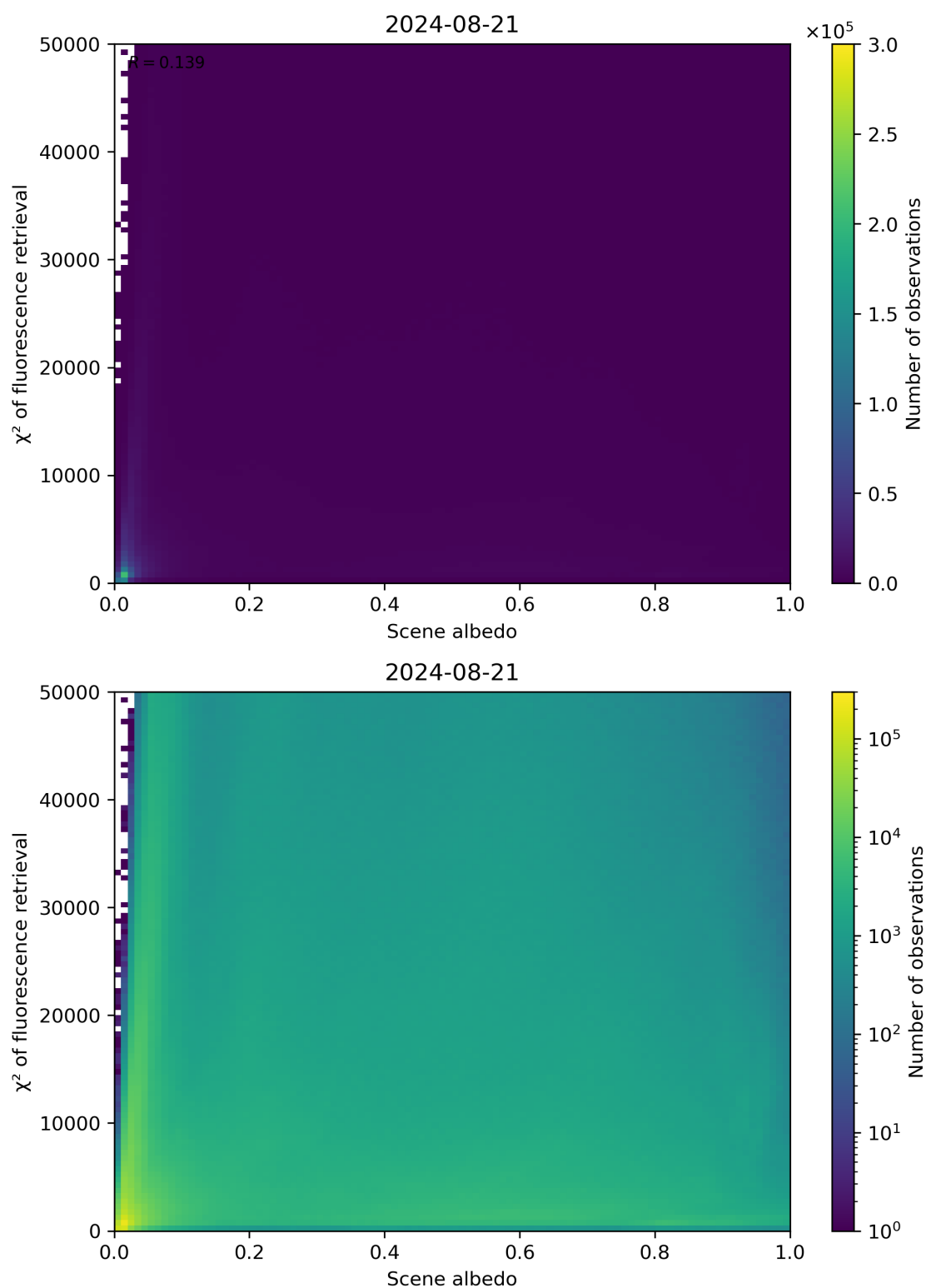
Figure 103: Scatter density plot of “Scene albedo” against “ \chi^2 of fluorescence retrieval” for 2024-08-21 to 2024-08-22.
