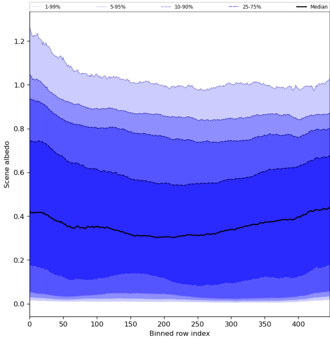
Figure 51: Along track statistics of “Scene albedo” for 2024-08-21 to 2024-08-22
