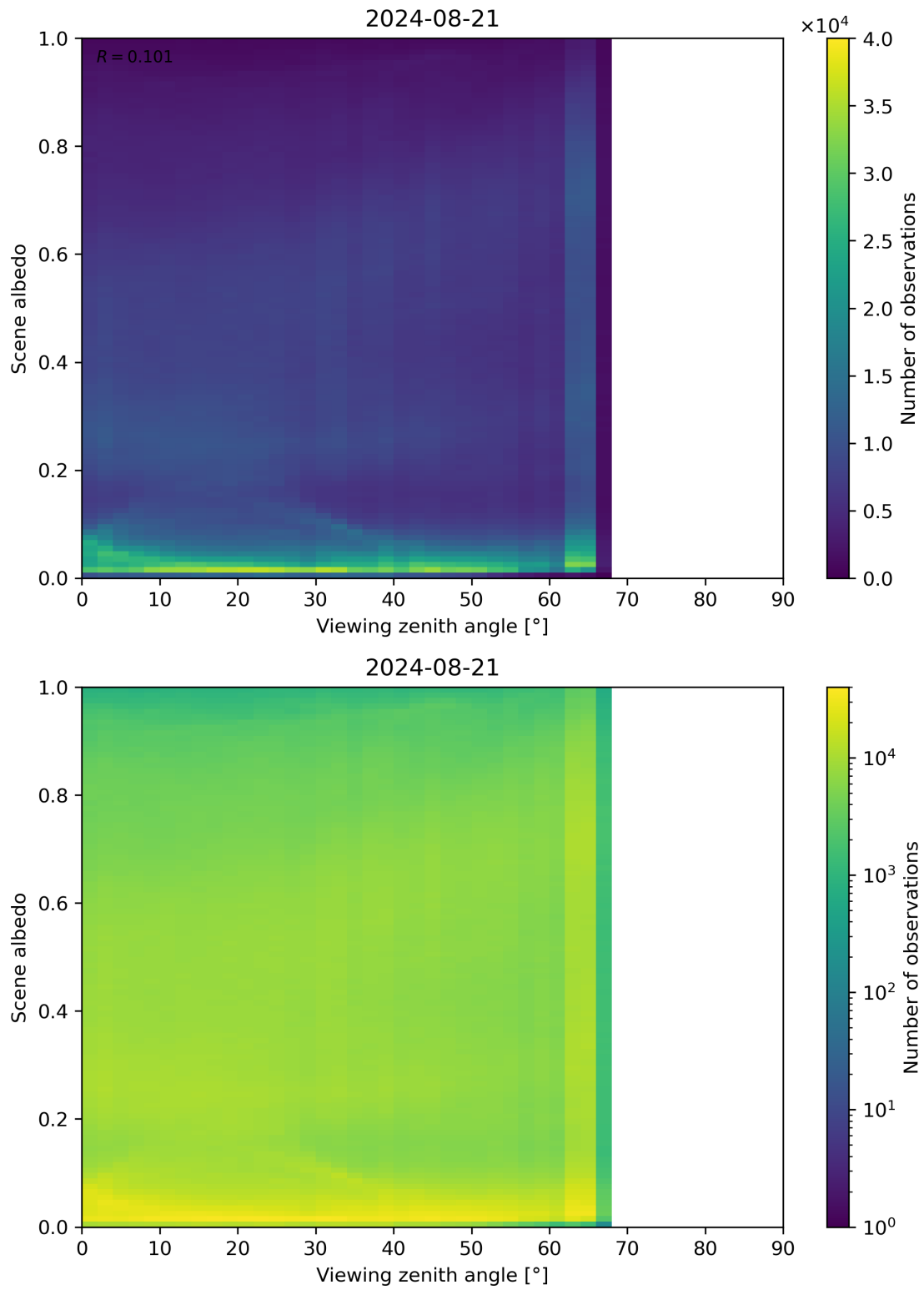
Figure 126: Scatter density plot of “Viewing zenith angle” against “Scene albedo” for 2024-08-21 to 2024-08-22.
