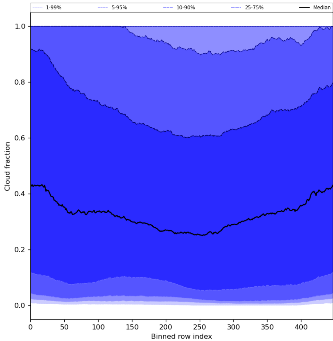
Figure 49: Along track statistics of “Cloud fraction” for 2024-08-21 to 2024-08-22
