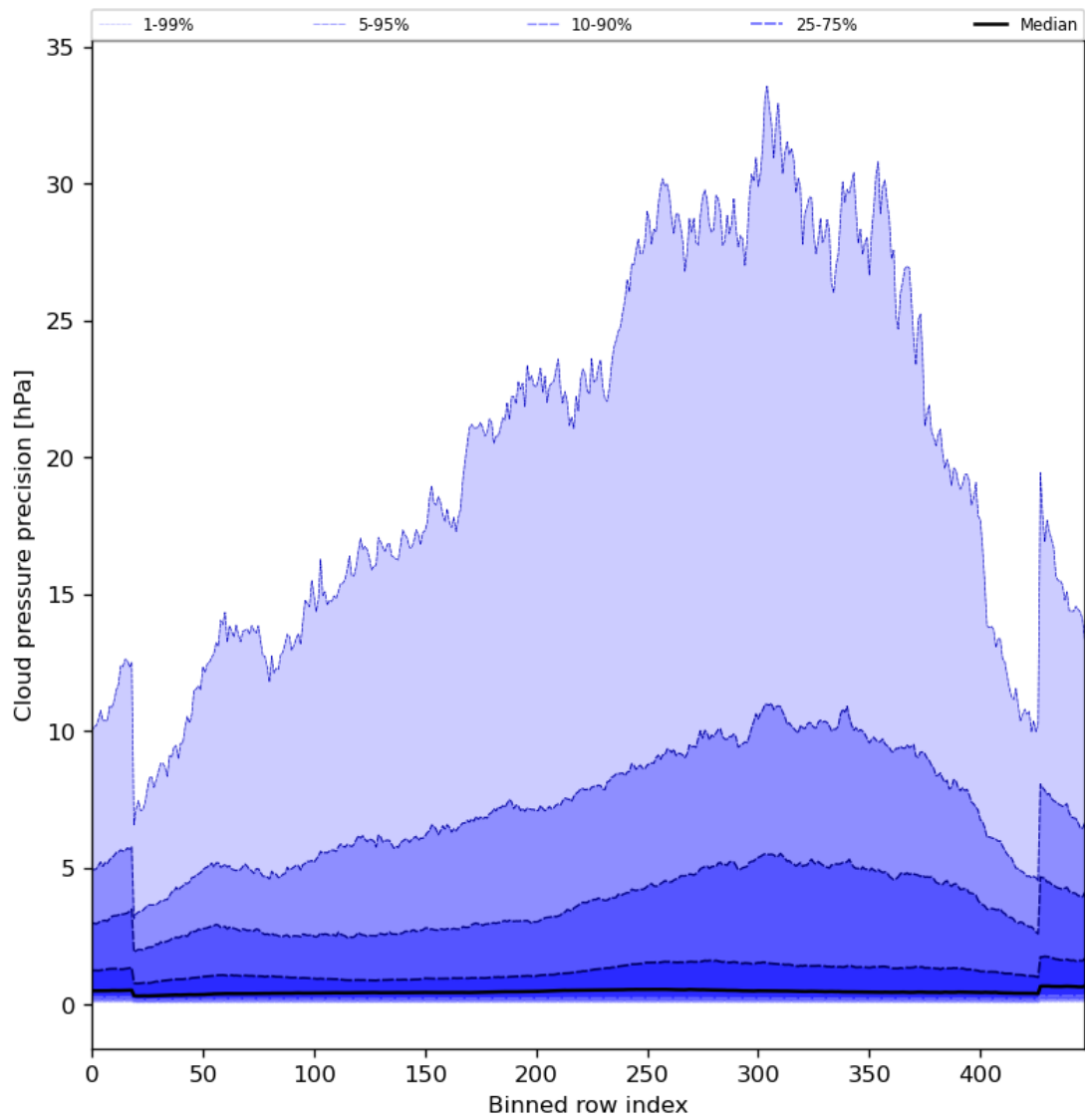
Figure 48: Along track statistics of “Cloud pressure precision” for 2024-08-21 to 2024-08-22
