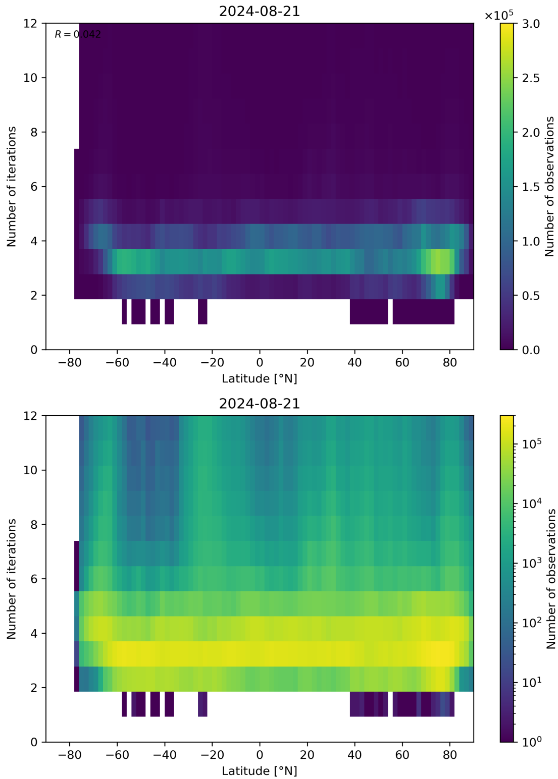
Figure 93: Scatter density plot of “Latitude” against “Number of iterations” for 2024-08-21 to 2024-08-22.
