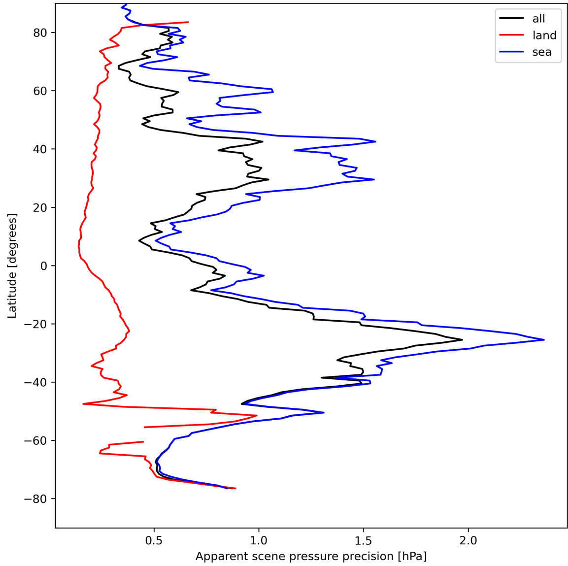
Figure 20: Zonal average of “Apparent scene pressure precision” for 2024-08-21 to 2024-08-22.
