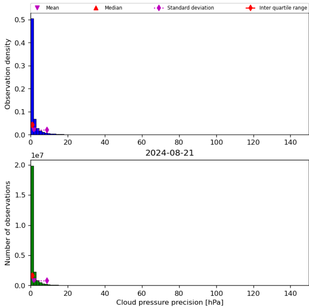
Figure 31: Histogram of “Cloud pressure precision” for 2024-08-21 to 2024-08-22
