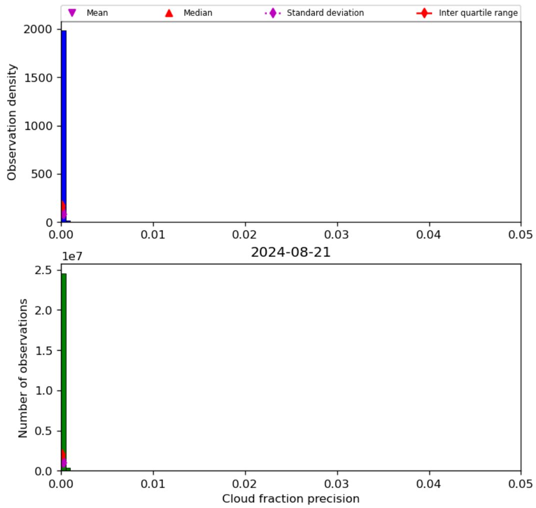
Figure 33: Histogram of “Cloud fraction precision” for 2024-08-21 to 2024-08-22
