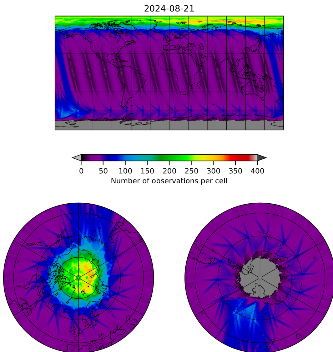
Figure 11: Map of the number of observations for 2024-08-21 to 2024-08-22
