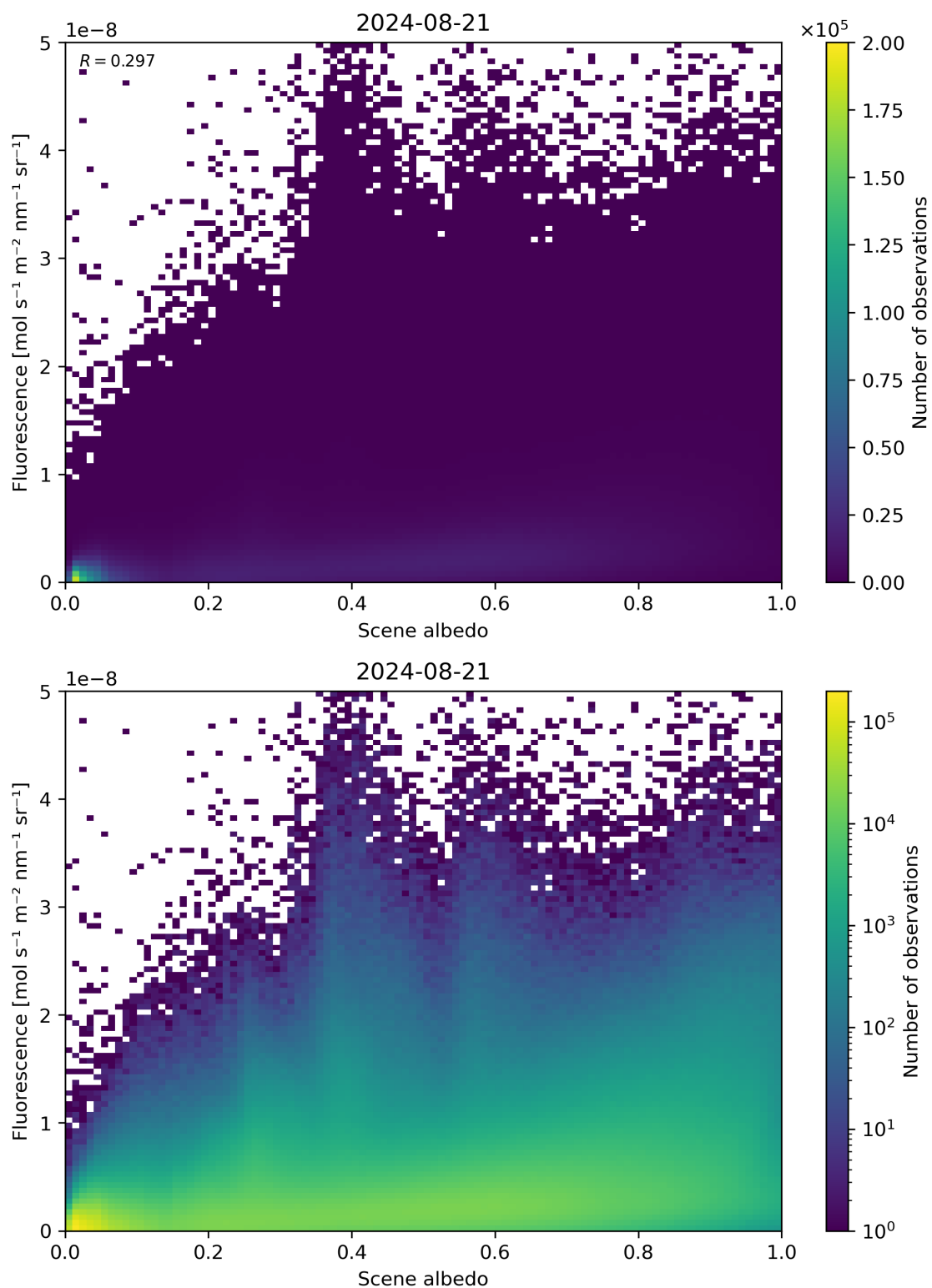
Figure 104: Scatter density plot of “Scene albedo” against “Fluorescence” for 2024-08-21 to 2024-08-22.
