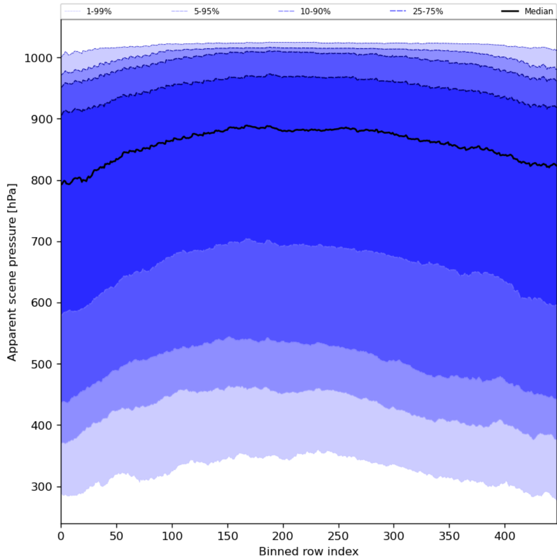
Figure 53: Along track statistics of “Apparent scene pressure” for 2024-08-21 to 2024-08-22
