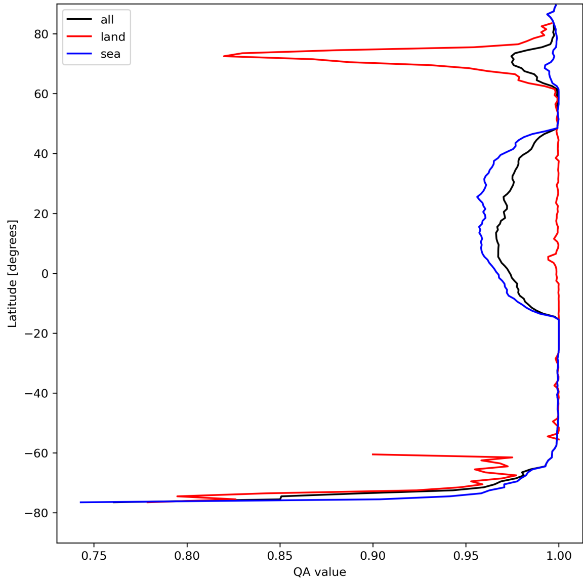
Figure 12: Zonal average of “QA value” for 2024-08-21 to 2024-08-22.
