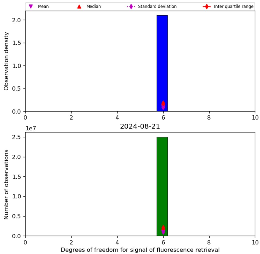
Figure 43: Histogram of “Degrees of freedom for signal of fluorescence retrieval” for 2024-08-21 to 2024-08-22
