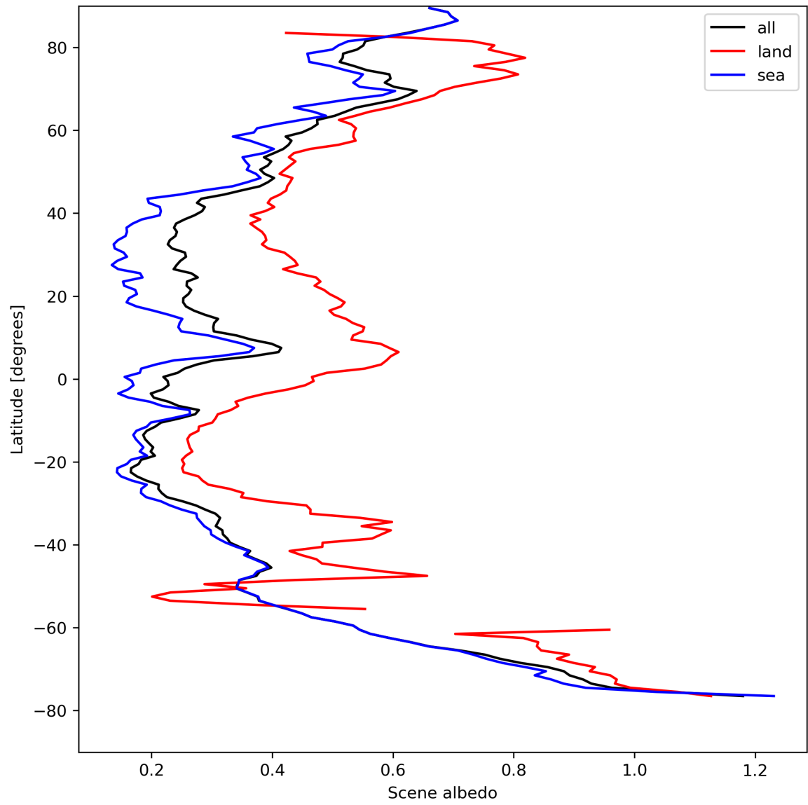
Figure 17: Zonal average of “Scene albedo” for 2024-08-21 to 2024-08-22.
