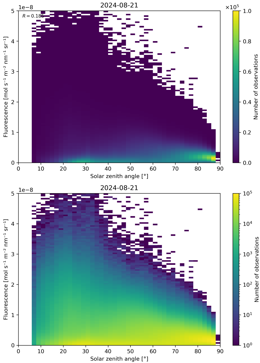
Figure 112: Scatter density plot of “Solar zenith angle” against “Fluorescence” for 2024-08-21 to 2024-08-22.
