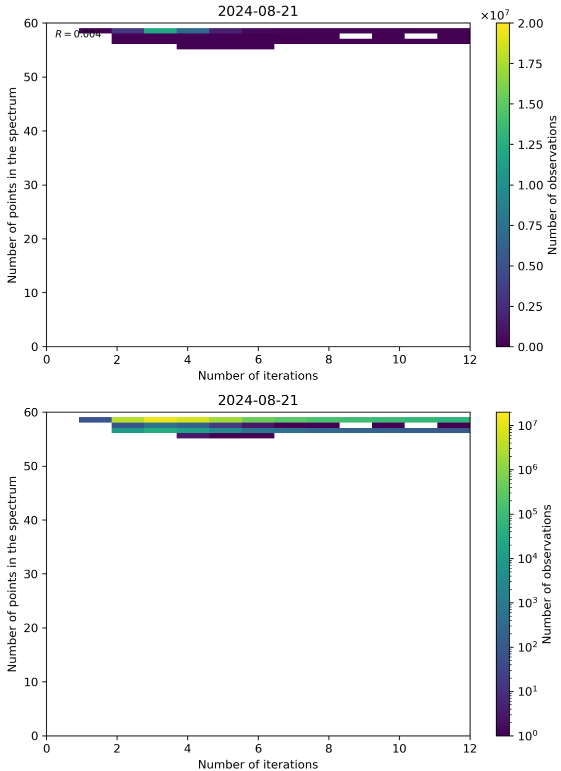
Figure 99: Scatter density plot of “Number of iterations” against “Number of points in the spectrum” for 2024-08-21 to 2024-08-22.
