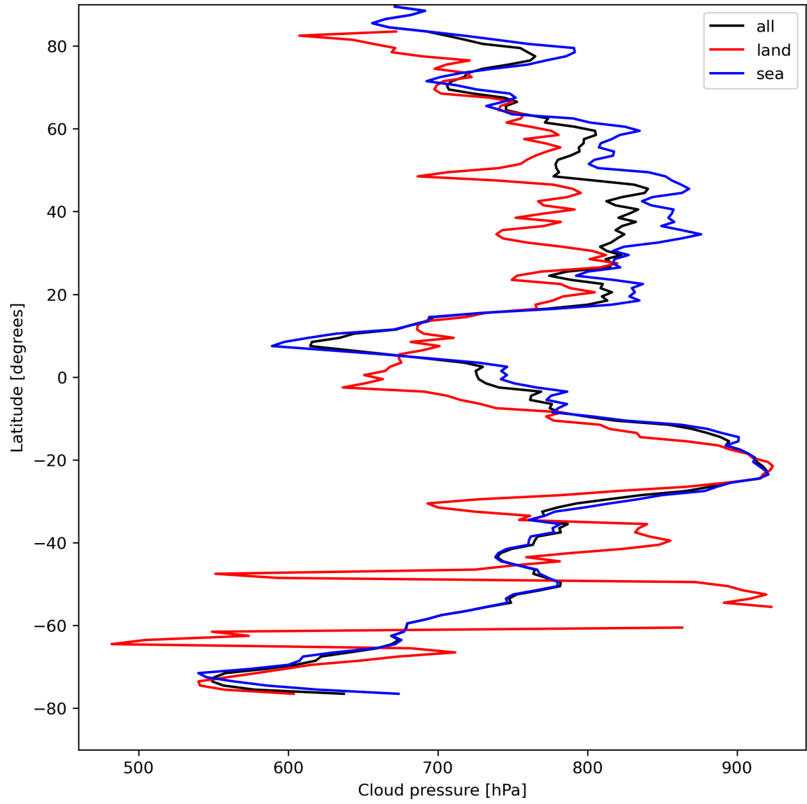
Figure 13: Zonal average of “Cloud pressure” for 2024-08-21 to 2024-08-22.
