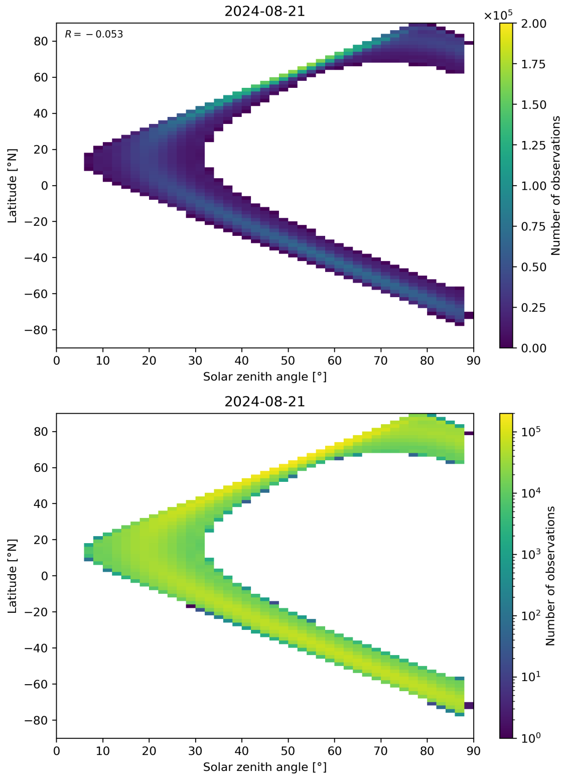
Figure 113: Scatter density plot of “Solar zenith angle” against “Latitude” for 2024-08-21 to 2024-08-22.
