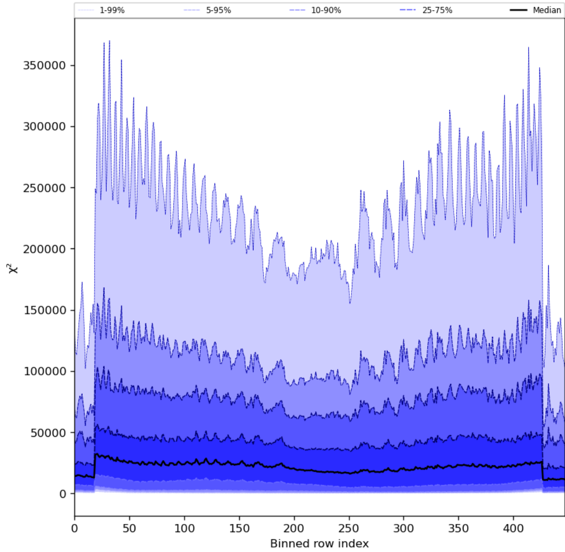
Figure 55: Along track statistics of “ \chi^2 ” for 2024-08-21 to 2024-08-22
