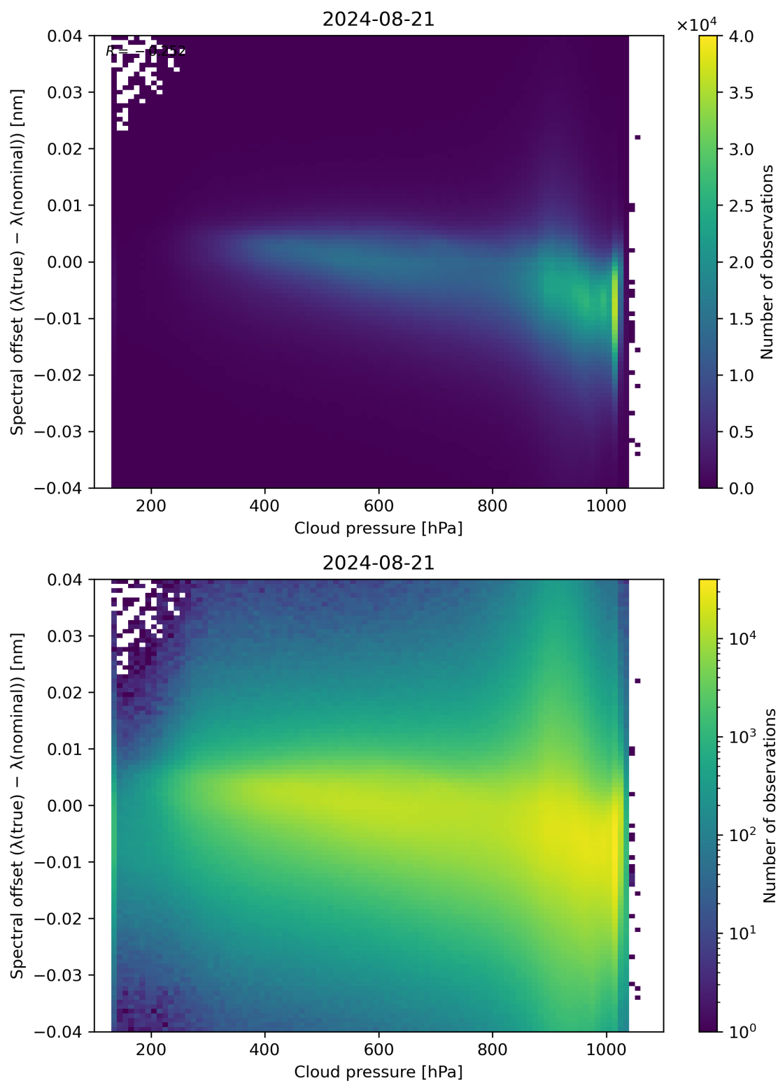
Figure 84: Scatter density plot of “Cloud pressure” against “Spectral offset ( \lambda(\text{true}) - \lambda(\text{nominal}) )” for 2024-08-21 to 2024-08-22.
