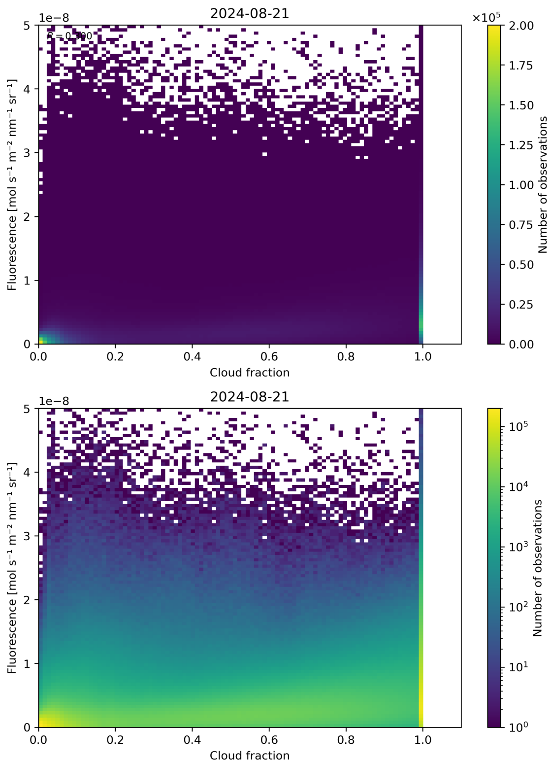
Figure 72: Scatter density plot of “Cloud fraction” against “Fluorescence” for 2024-08-21 to 2024-08-22.
