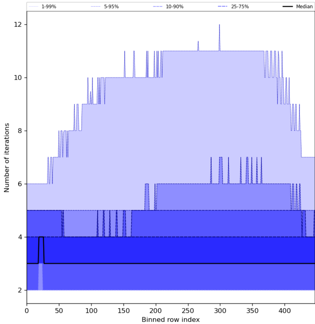
Figure 56: Along track statistics of “Number of iterations” for 2024-08-21 to 2024-08-22
