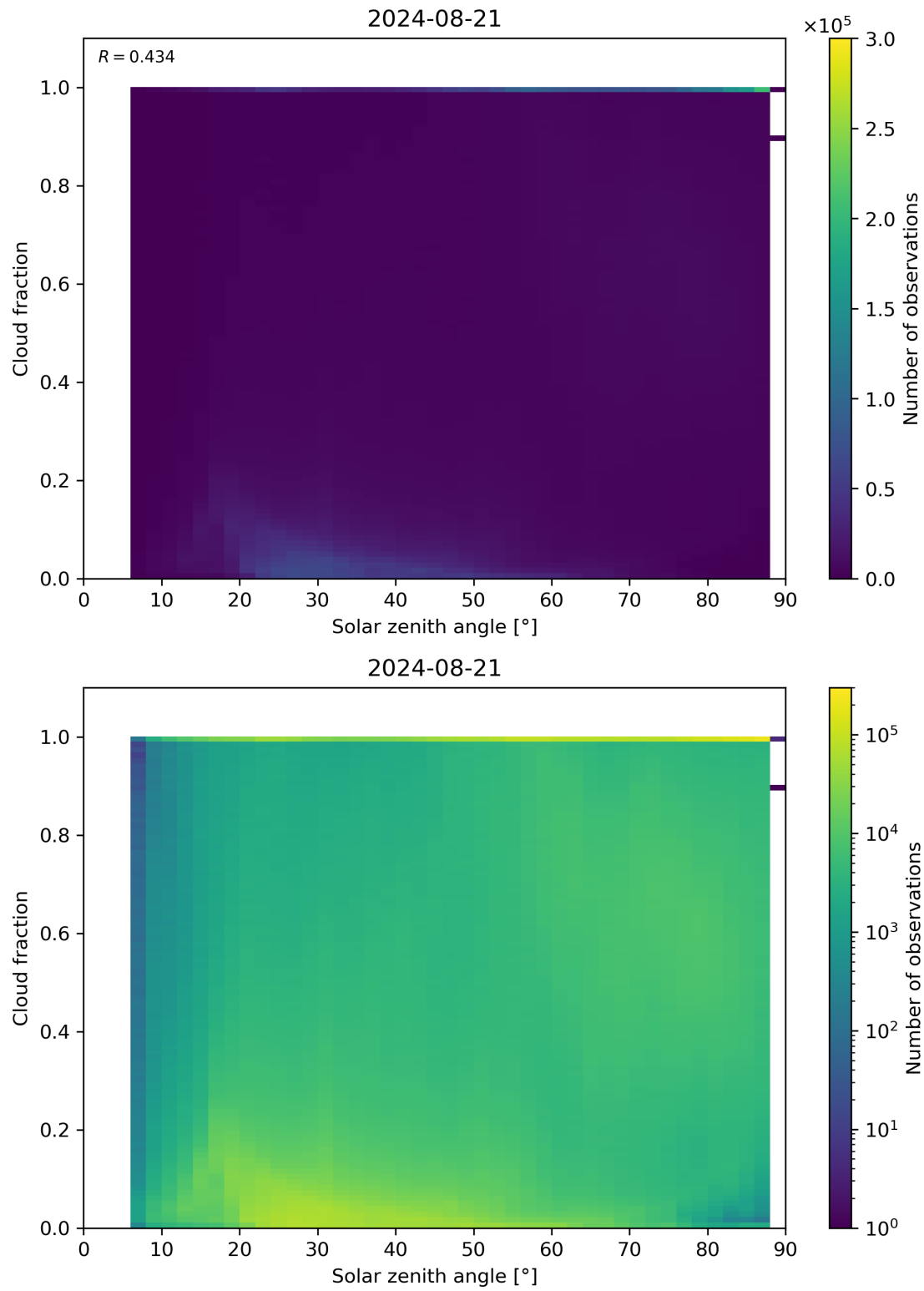
Figure 110: Scatter density plot of “Solar zenith angle” against “Cloud fraction” for 2024-08-21 to 2024-08-22.
