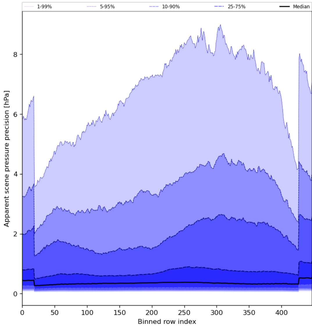
Figure 54: Along track statistics of “Apparent scene pressure precision” for 2024-08-21 to 2024-08-22
