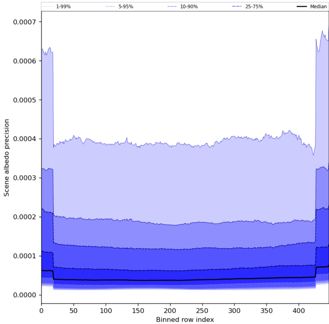
Figure 52: Along track statistics of “Scene albedo precision” for 2024-08-21 to 2024-08-22
