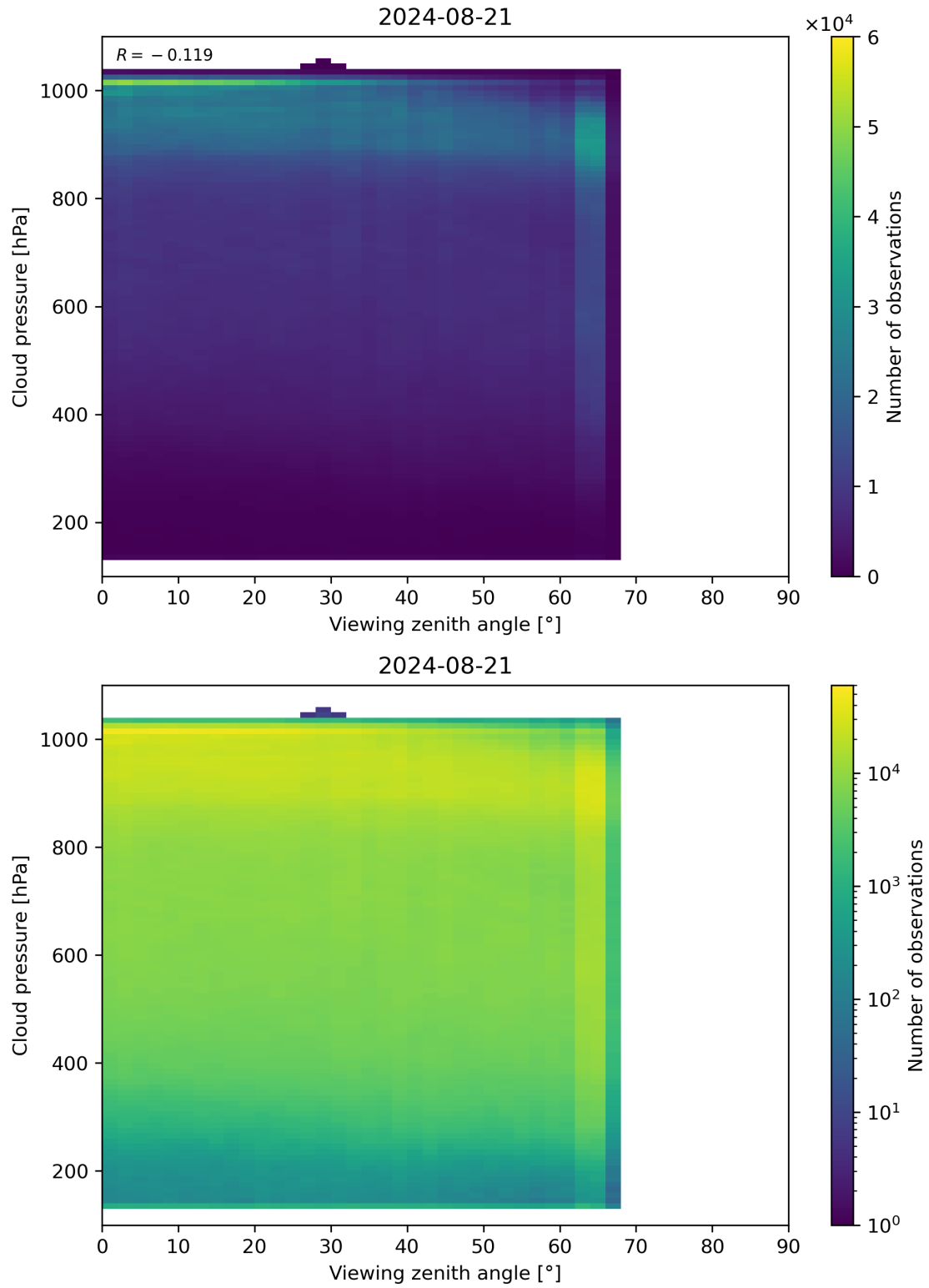
Figure 121: Scatter density plot of “Viewing zenith angle” against “Cloud pressure” for 2024-08-21 to 2024-08-22.
