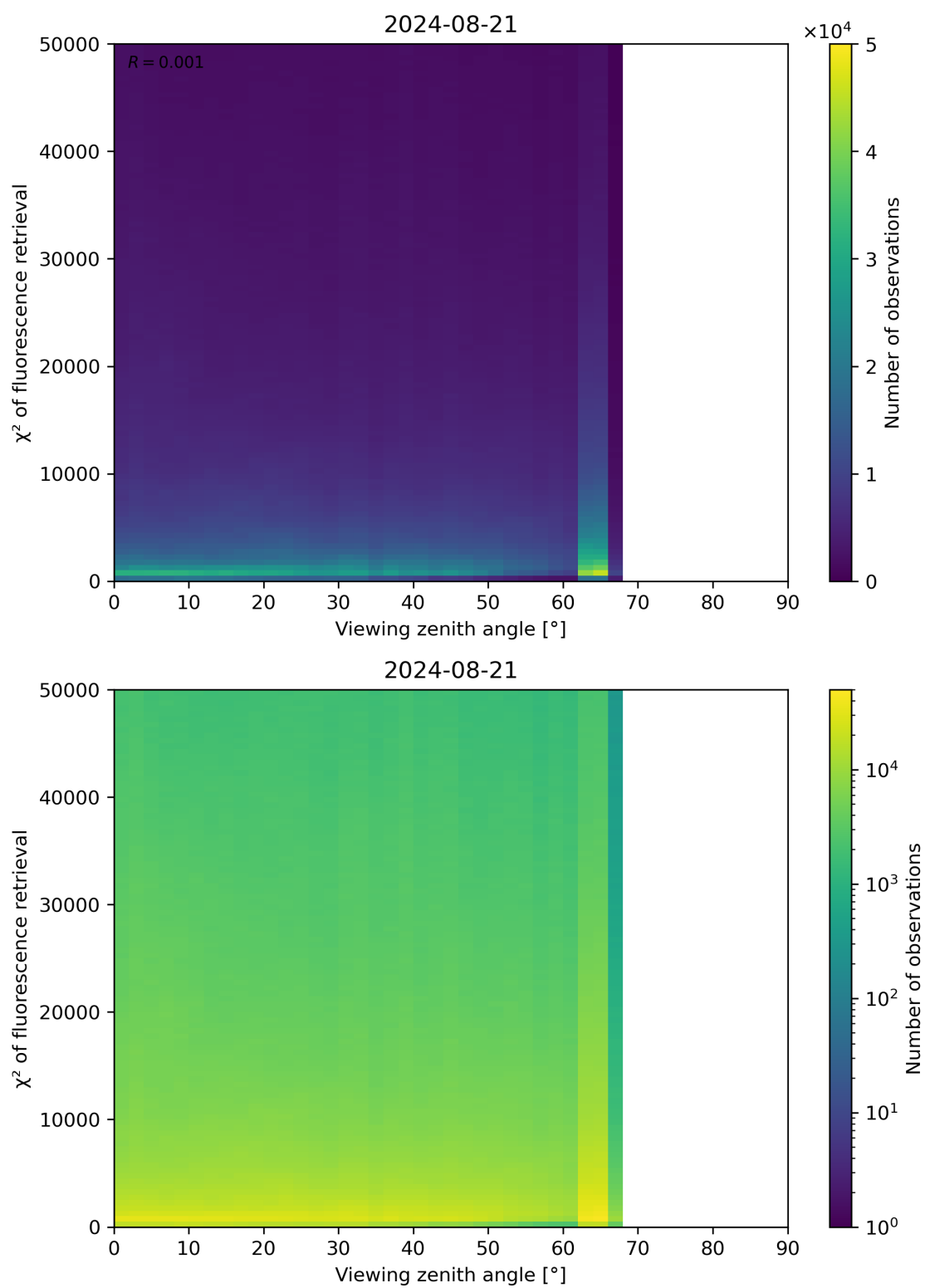
Figure 119: Scatter density plot of “Viewing zenith angle” against “ \chi^2 of fluorescence retrieval” for 2024-08-21 to 2024-08-22.
