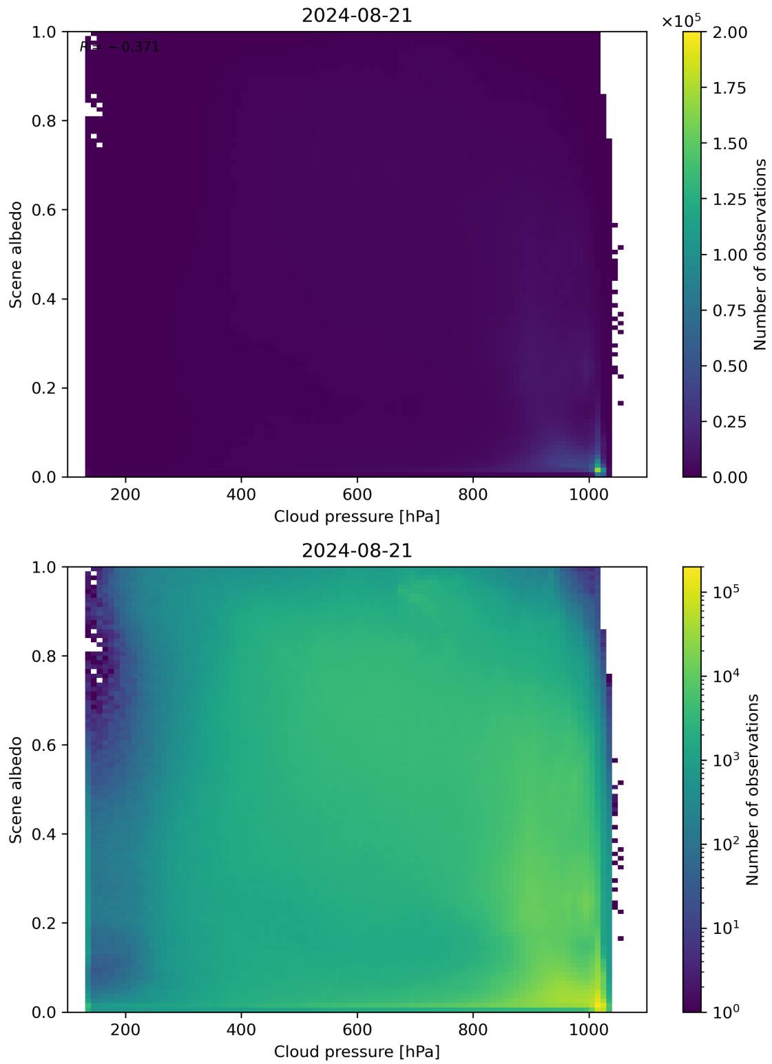
Figure 83: Scatter density plot of “Cloud pressure” against “Scene albedo” for 2024-08-21 to 2024-08-22.
