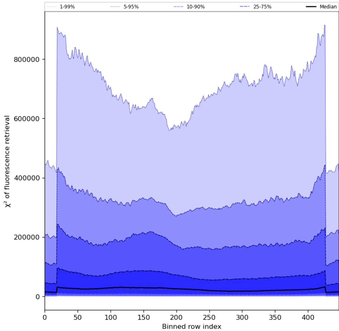
Figure 59: Along track statistics of “ \chi^2 of fluorescence retrieval” for 2024-08-21 to 2024-08-22
