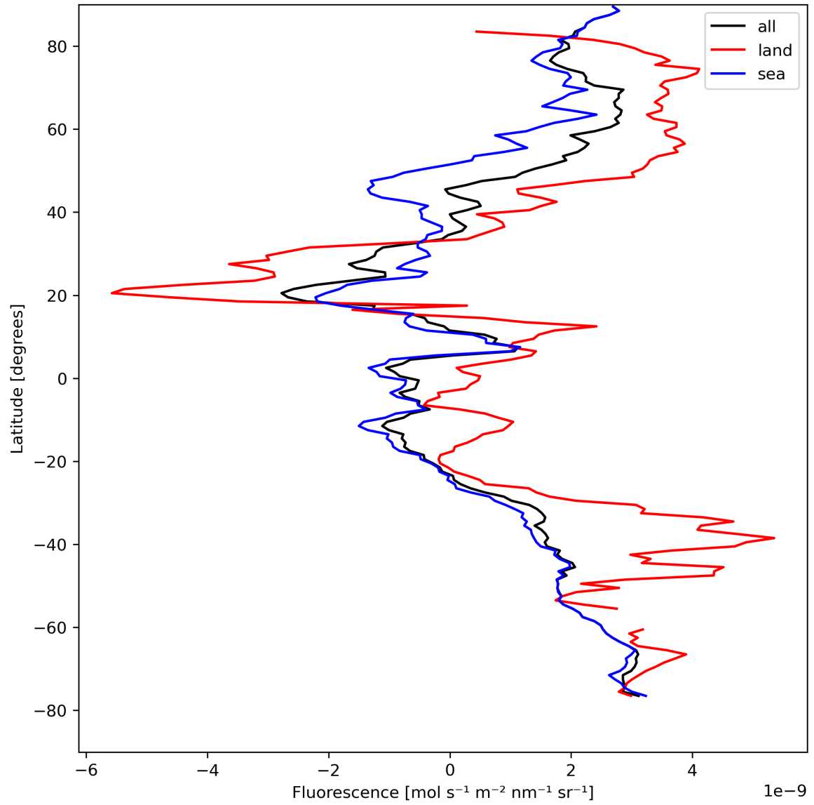
Figure 23: Zonal average of “Fluorescence” for 2024-08-21 to 2024-08-22.
