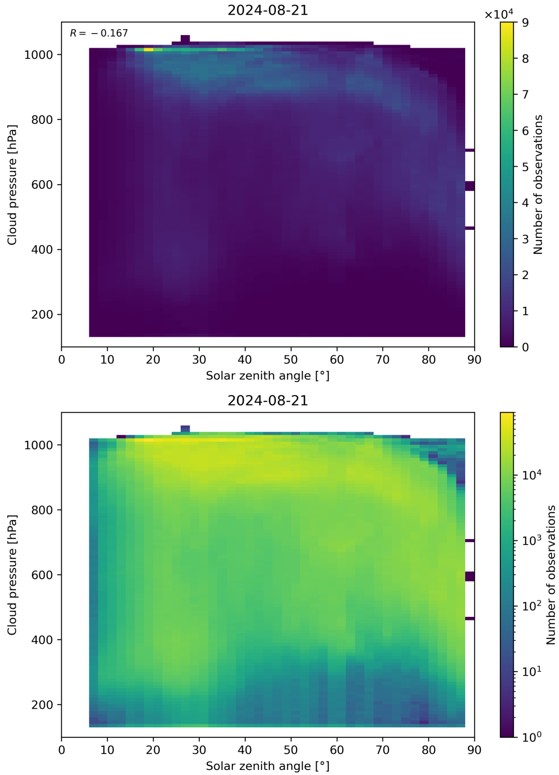
Figure 111: Scatter density plot of “Solar zenith angle” against “Cloud pressure” for 2024-08-21 to 2024-08-22.
