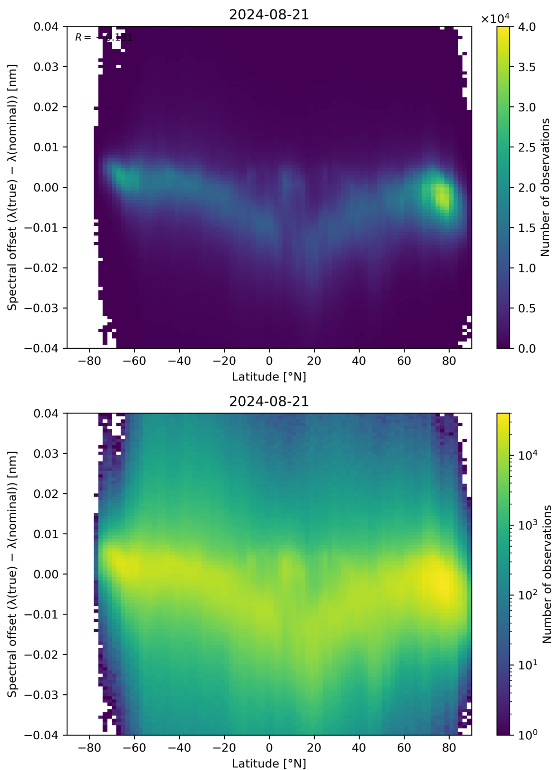
Figure 96: Scatter density plot of “Latitude” against “Spectral offset ( \lambda(\text{true}) - \lambda(\text{nominal}) )” for 2024-08-21 to 2024-08-22.
