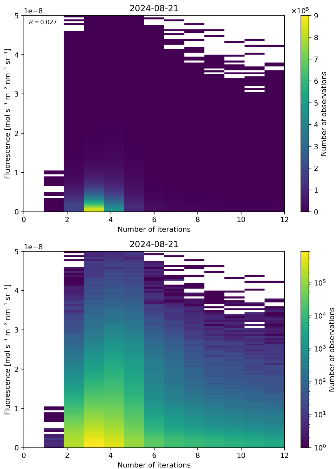
Figure 98: Scatter density plot of “Number of iterations” against “Fluorescence” for 2024-08-21 to 2024-08-22.
