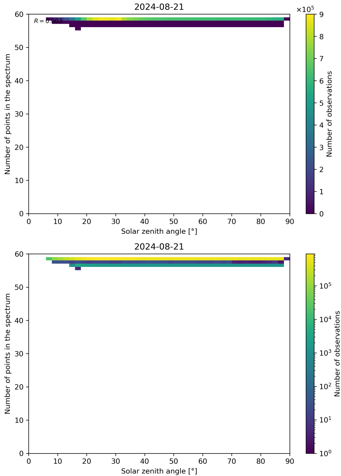
Figure 115: Scatter density plot of “Solar zenith angle” against “Number of points in the spectrum” for 2024-08-21 to 2024-08-22.
