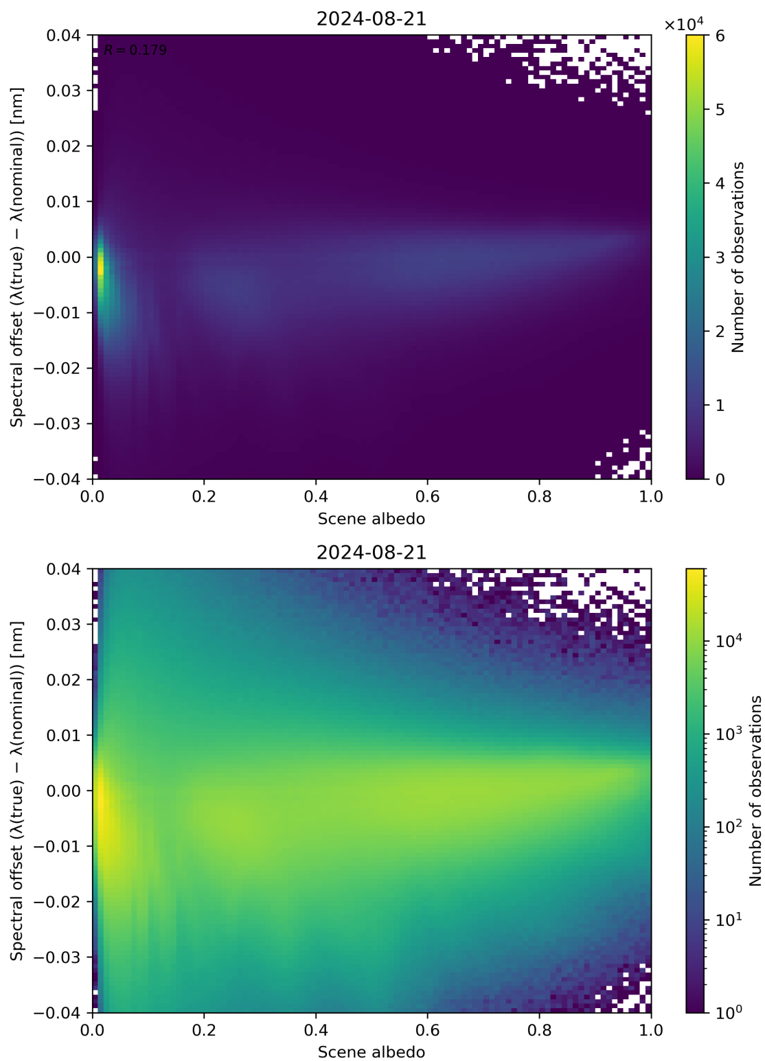
Figure 107: Scatter density plot of “Scene albedo” against “Spectral offset ( \lambda(\text{true}) - \lambda(\text{nominal}) )” for 2024-08-21 to 2024-08-22.
