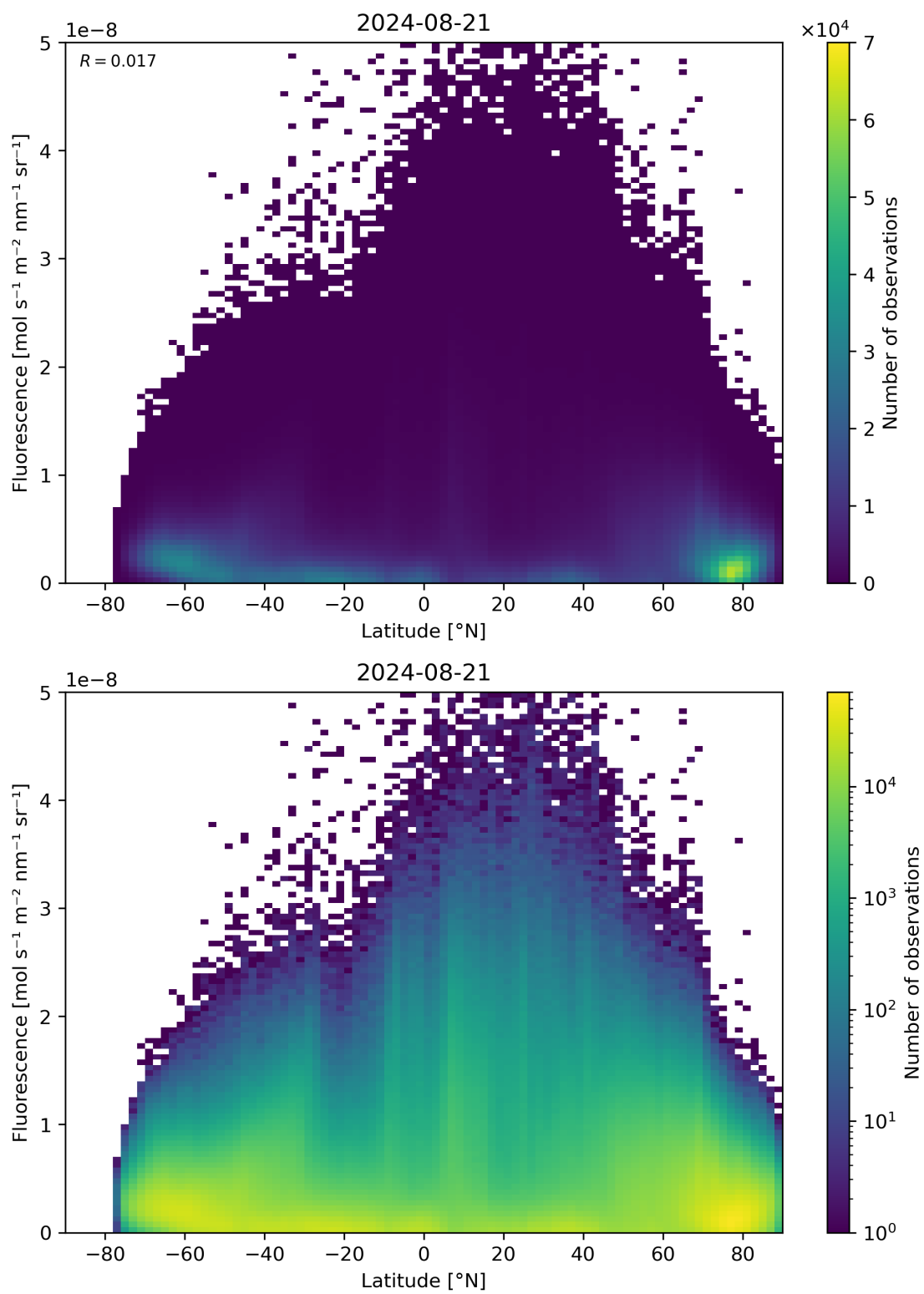
Figure 92: Scatter density plot of “Latitude” against “Fluorescence” for 2024-08-21 to 2024-08-22.
