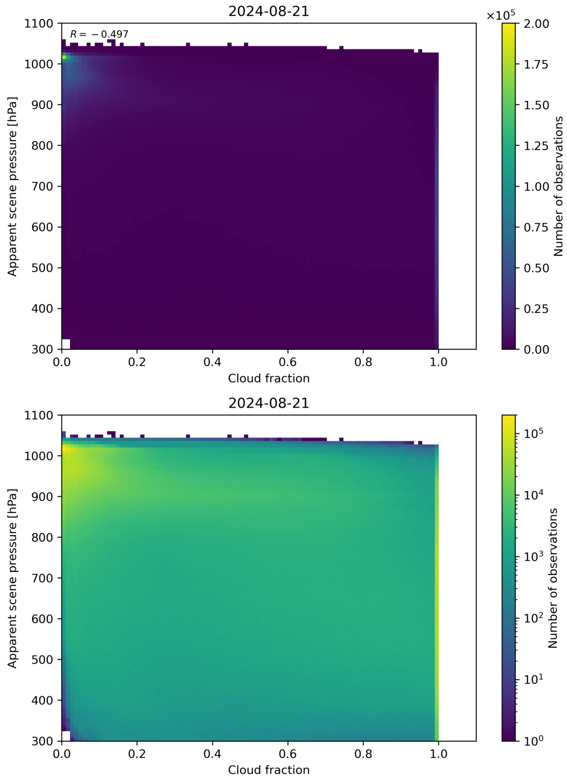
Figure 70: Scatter density plot of “Cloud fraction” against “Apparent scene pressure” for 2024-08-21 to 2024-08-22.
