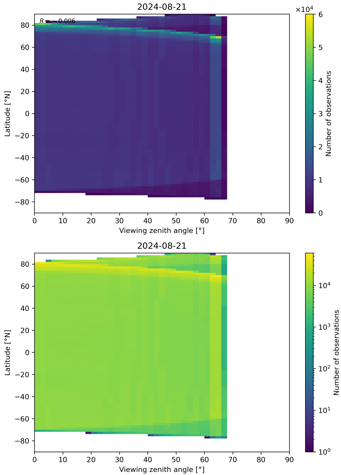
Figure 123: Scatter density plot of “Viewing zenith angle” against “Latitude” for 2024-08-21 to 2024-08-22.
