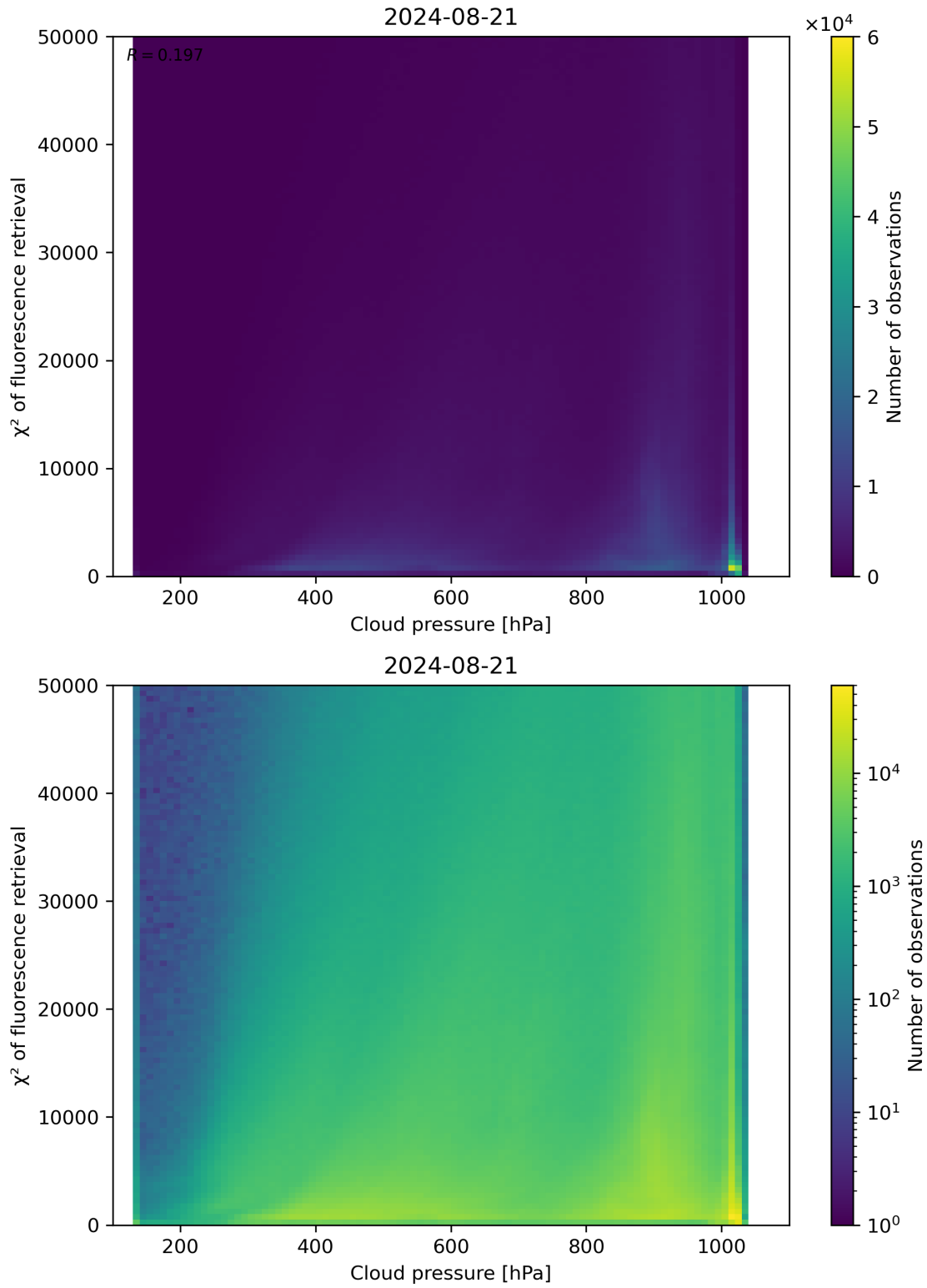
Figure 78: Scatter density plot of “Cloud pressure” against “ \chi^2 of fluorescence retrieval” for 2024-08-21 to 2024-08-22.
