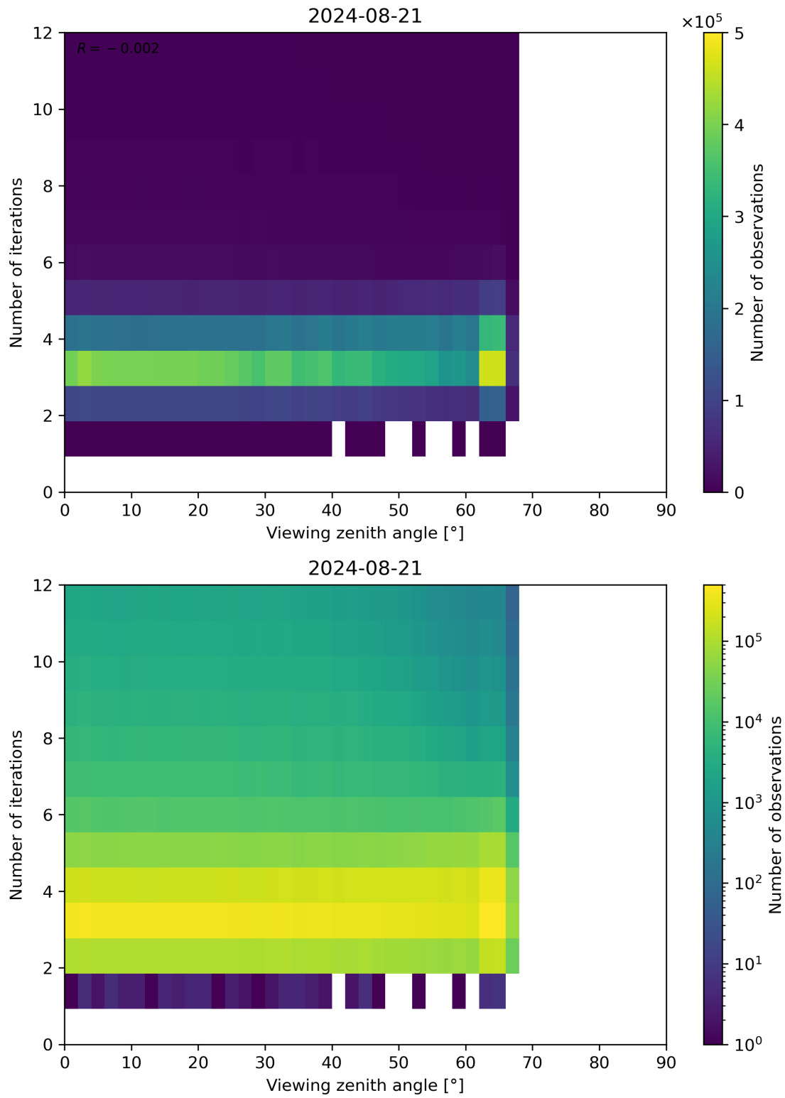
Figure 124: Scatter density plot of “Viewing zenith angle” against “Number of iterations” for 2024-08-21 to 2024-08-22.
