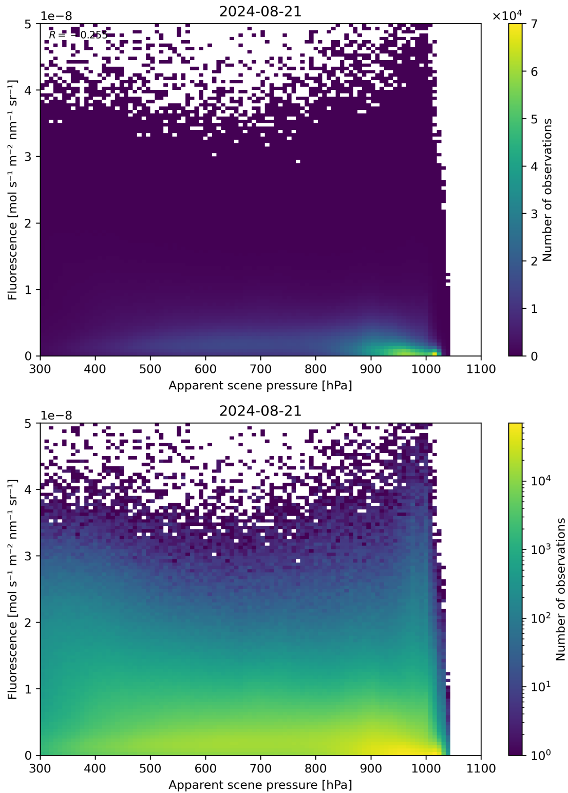
Figure 64: Scatter density plot of “Apparent scene pressure” against “Fluorescence” for 2024-08-21 to 2024-08-22.
