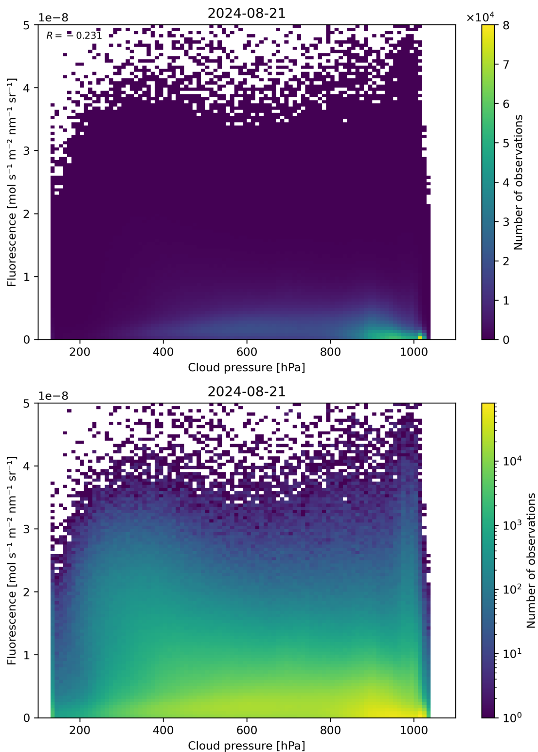
Figure 80: Scatter density plot of “Cloud pressure” against “Fluorescence” for 2024-08-21 to 2024-08-22.
