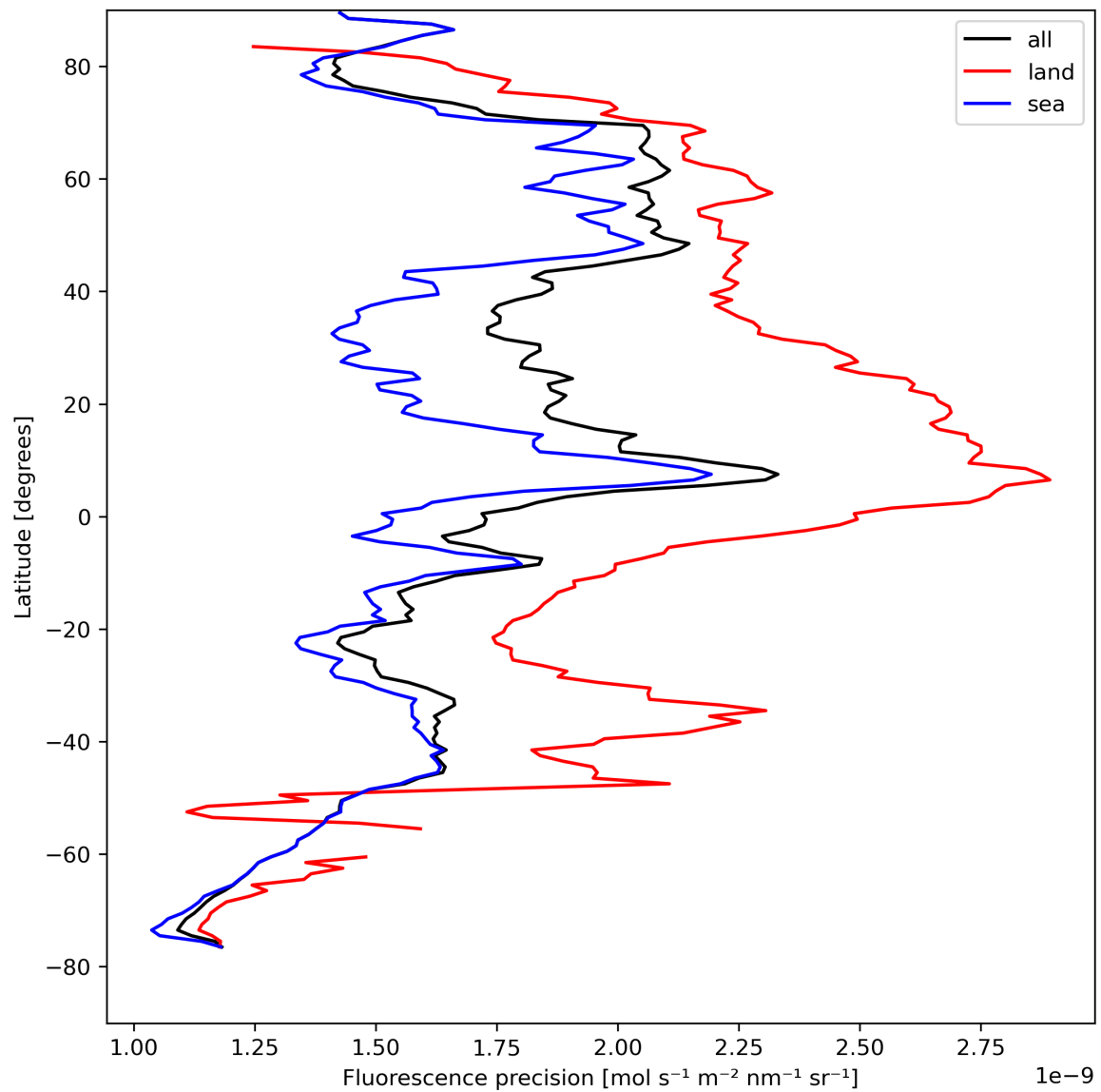
Figure 24: Zonal average of “Fluorescence precision” for 2024-08-21 to 2024-08-22.
