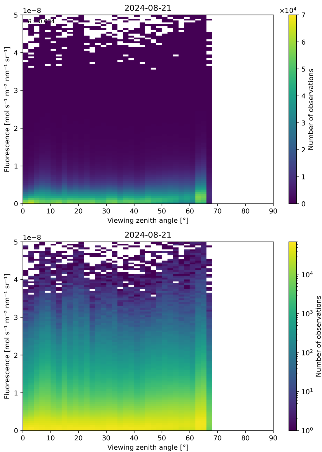
Figure 122: Scatter density plot of “Viewing zenith angle” against “Fluorescence” for 2024-08-21 to 2024-08-22.
