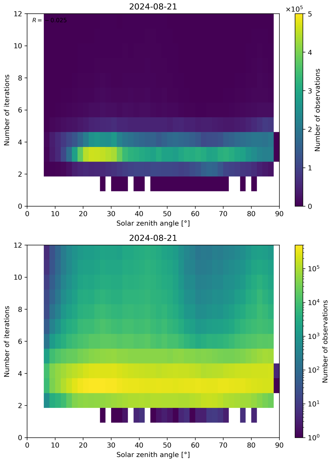
Figure 114: Scatter density plot of “Solar zenith angle” against “Number of iterations” for 2024-08-21 to 2024-08-22.
