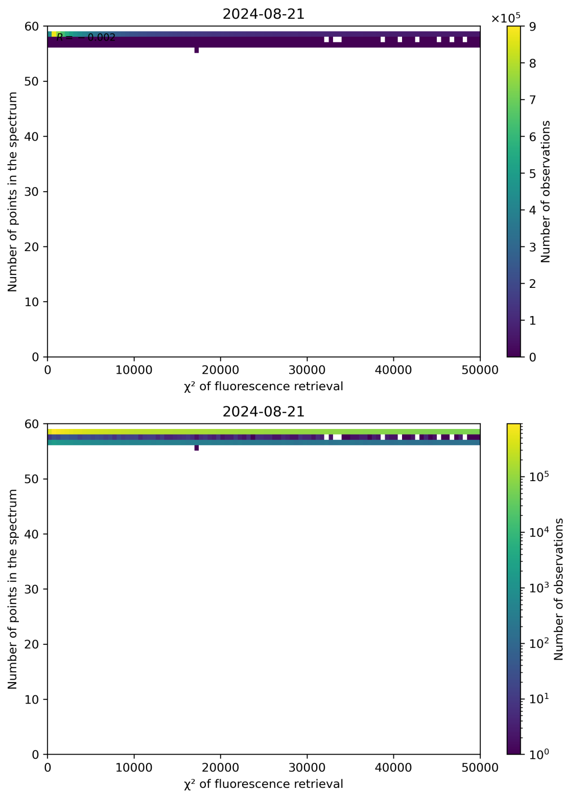
Figure 68: Scatter density plot of “ \chi^2 of fluorescence retrieval” against “Number of points in the spectrum” for 2024-08-21 to 2024-08-22.
