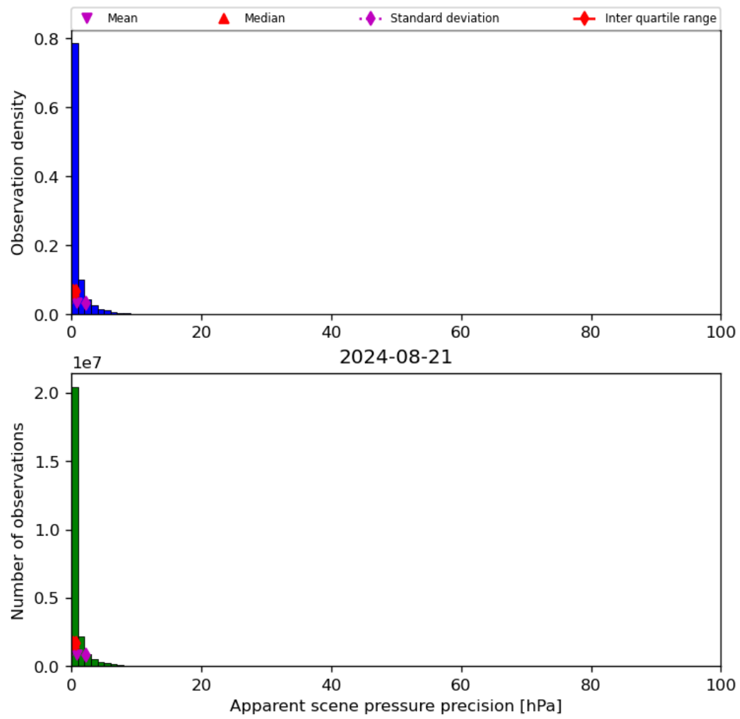
Figure 37: Histogram of “Apparent scene pressure precision” for 2024-08-21 to 2024-08-22
