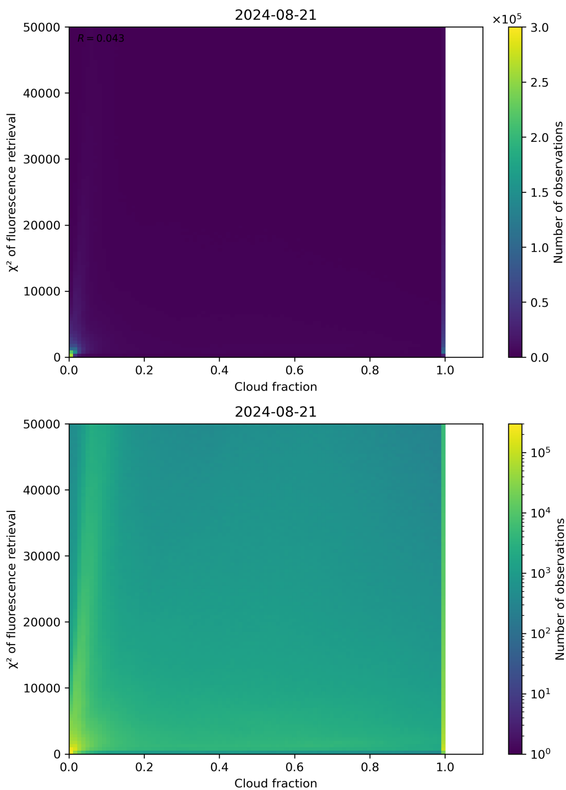
Figure 71: Scatter density plot of “Cloud fraction” against “ \chi^2 of fluorescence retrieval” for 2024-08-21 to 2024-08-22.
