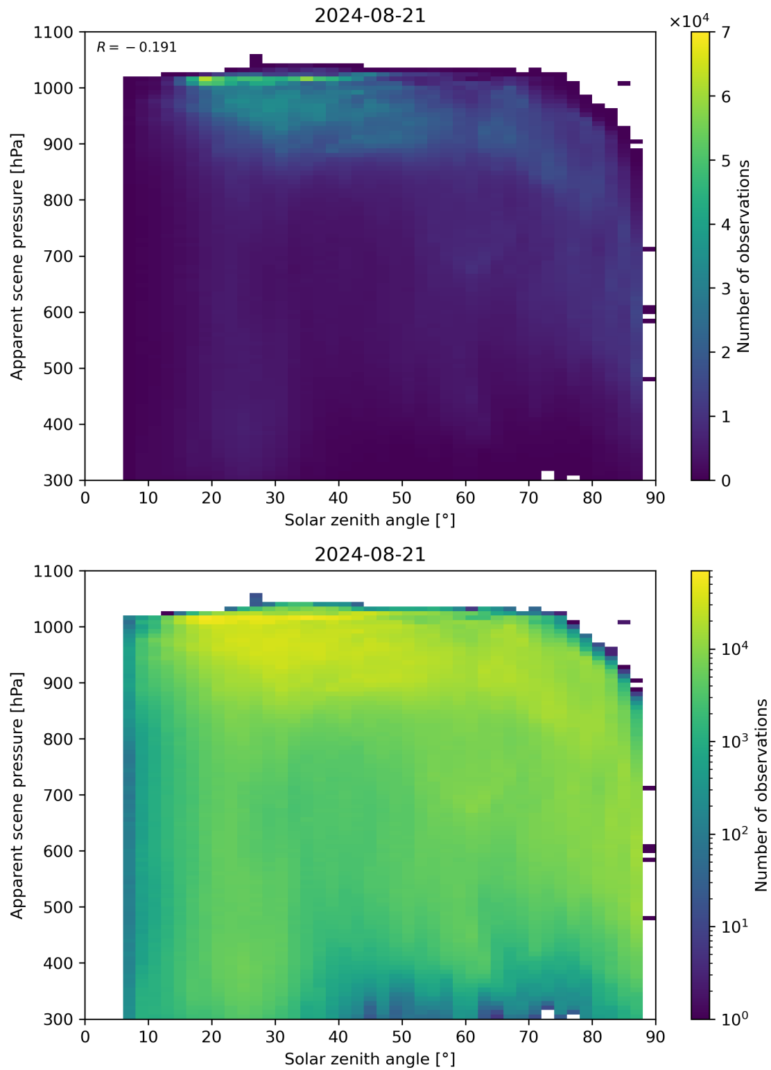
Figure 108: Scatter density plot of “Solar zenith angle” against “Apparent scene pressure” for 2024-08-21 to 2024-08-22.
