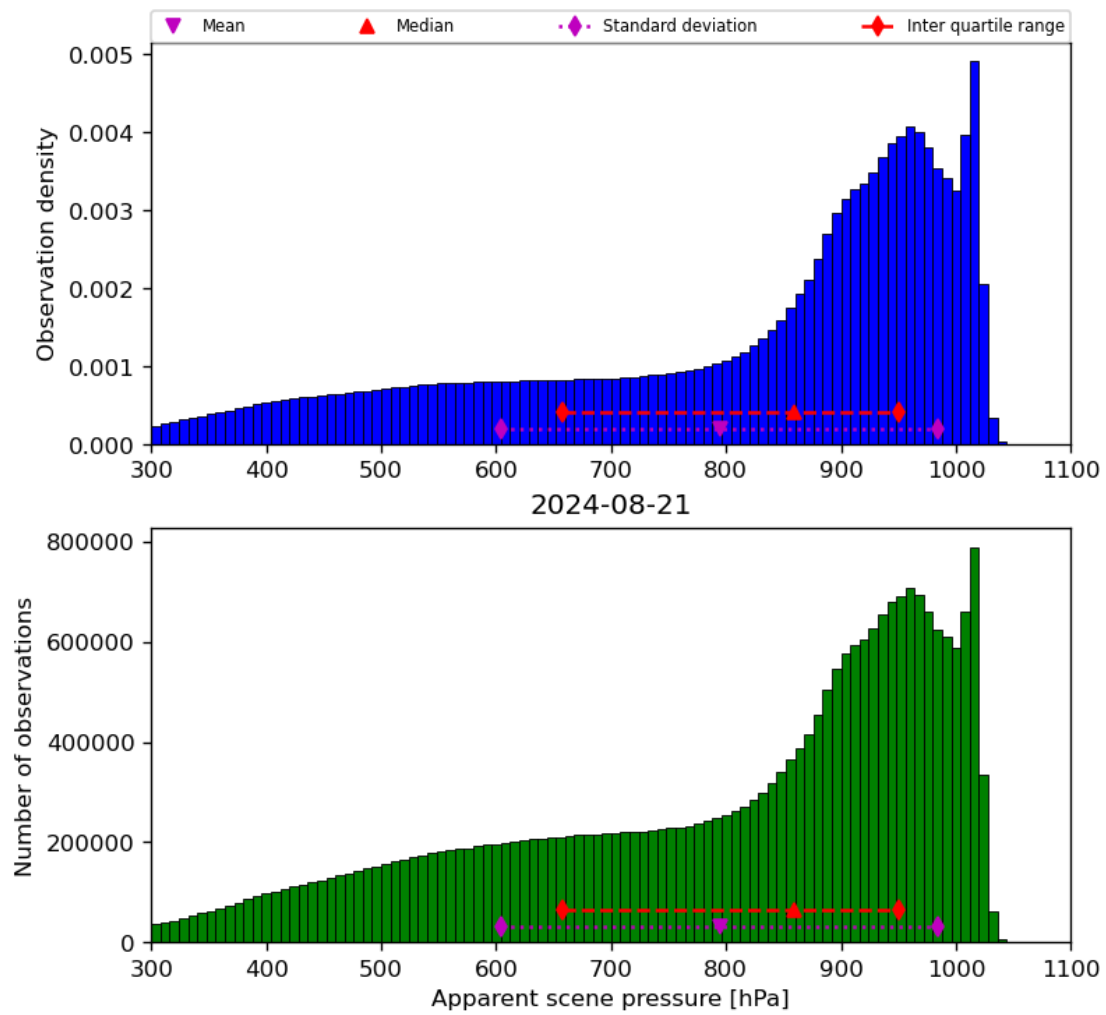
Figure 36: Histogram of “Apparent scene pressure” for 2024-08-21 to 2024-08-22
