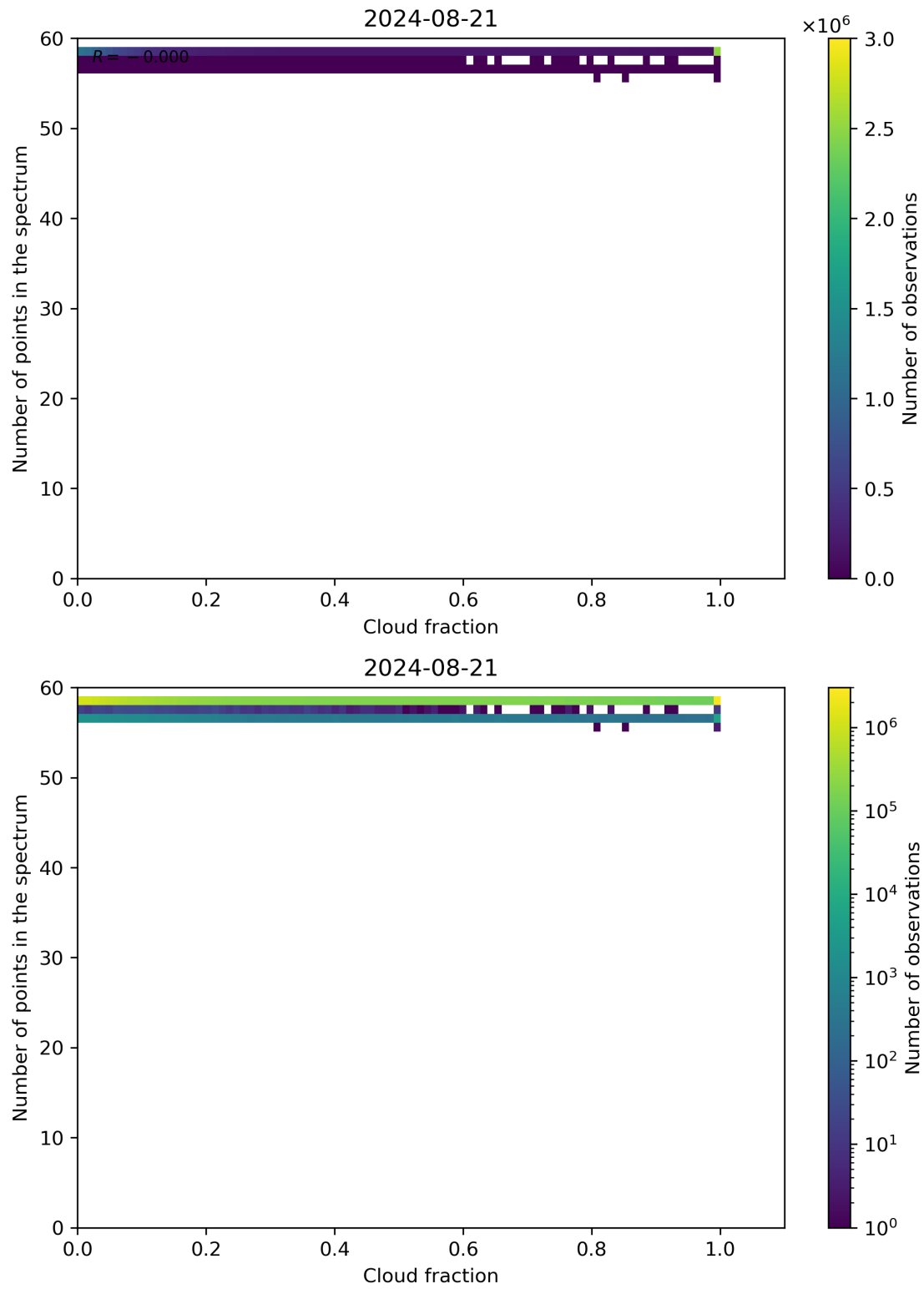
Figure 74: Scatter density plot of “Cloud fraction” against “Number of points in the spectrum” for 2024-08-21 to 2024-08-22.
