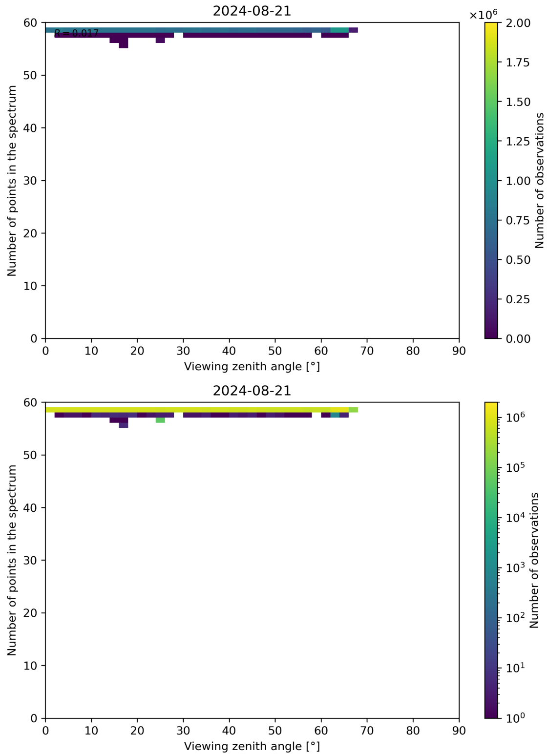
Figure 125: Scatter density plot of “Viewing zenith angle” against “Number of points in the spectrum” for 2024-08-21 to 2024-08-22.
