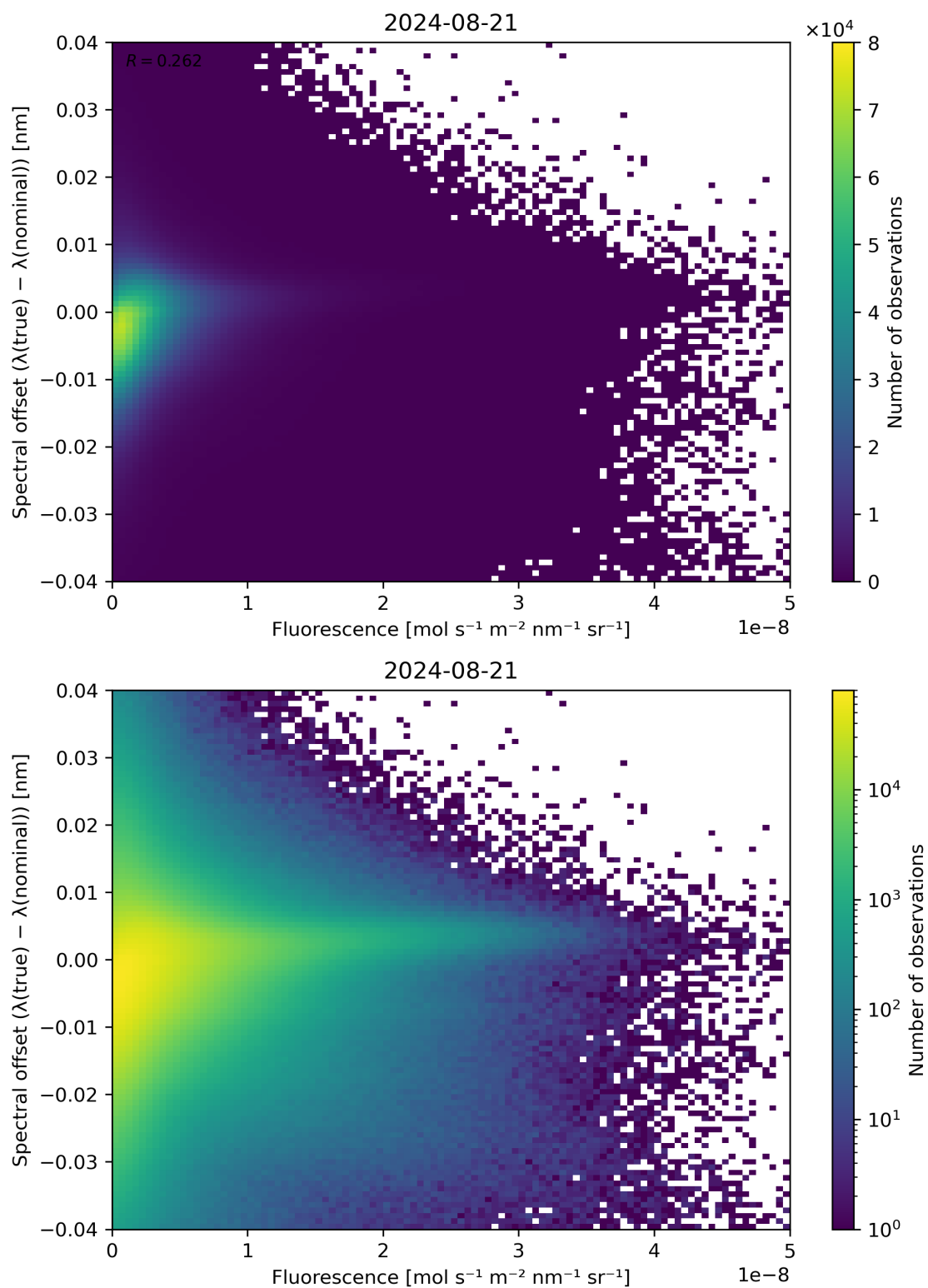
Figure 87: Scatter density plot of “Fluorescence” against “Spectral offset ( \lambda(\text{true}) - \lambda(\text{nominal}) )” for 2024-08-21 to 2024-08-22.
