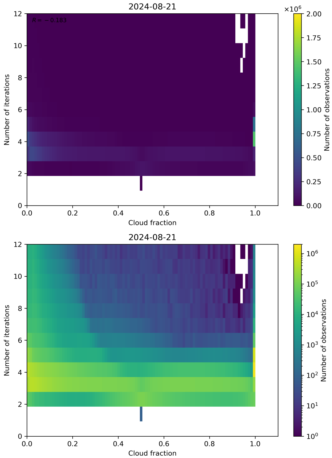
Figure 73: Scatter density plot of “Cloud fraction” against “Number of iterations” for 2024-08-21 to 2024-08-22.
