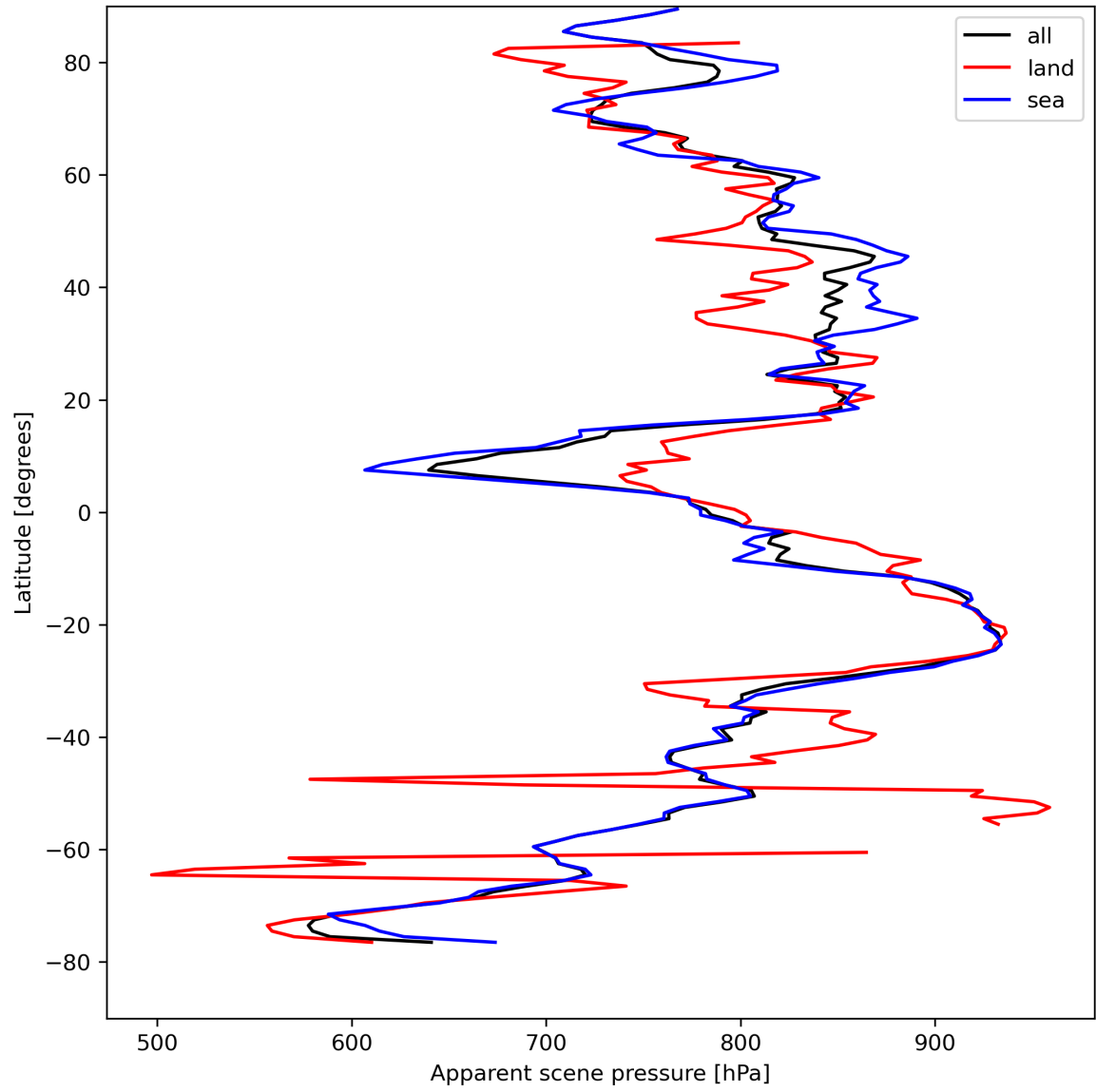
Figure 19: Zonal average of “Apparent scene pressure” for 2024-08-21 to 2024-08-22.
