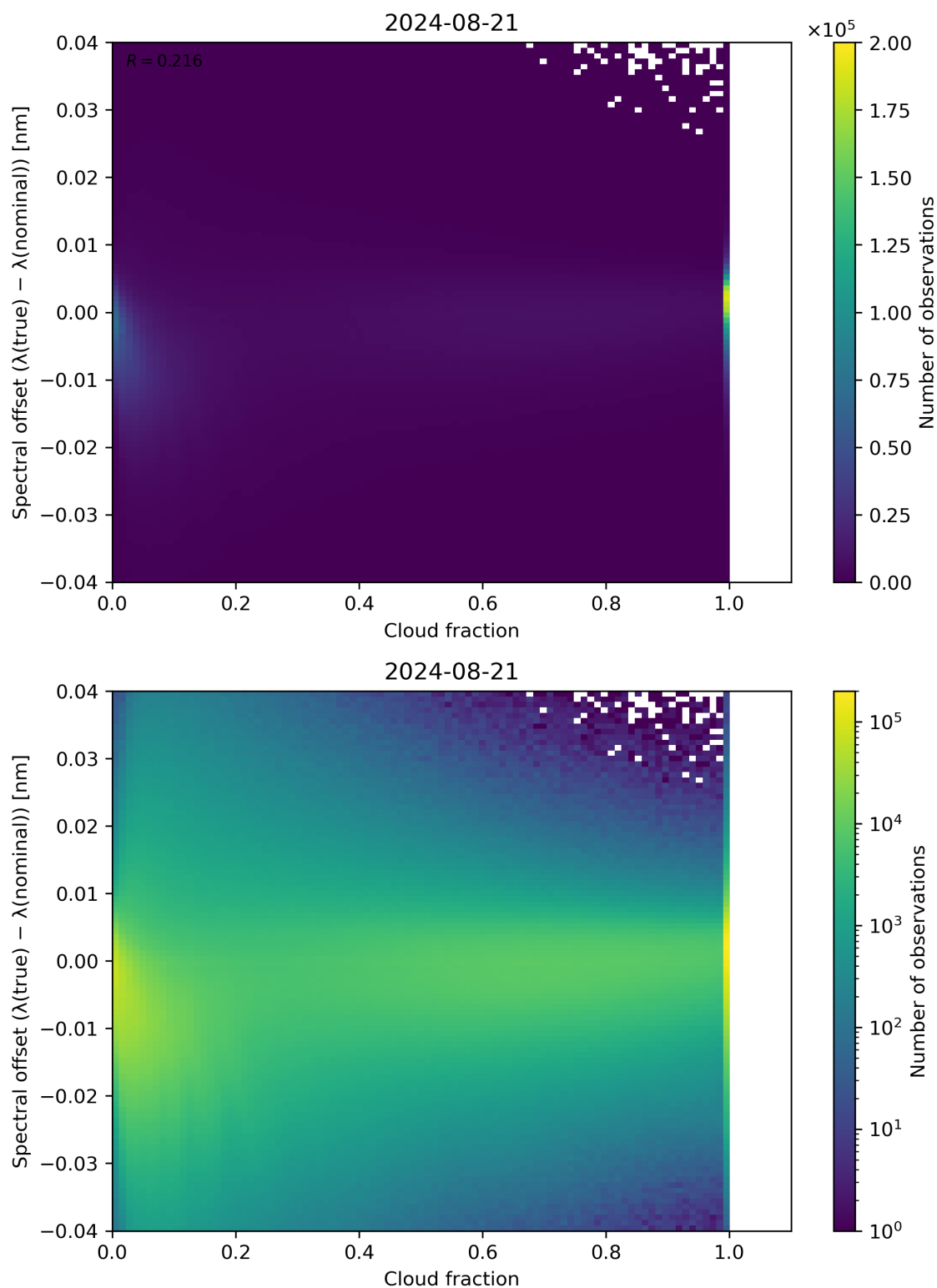
Figure 76: Scatter density plot of “Cloud fraction” against “Spectral offset ( \lambda(\text{true}) - \lambda(\text{nominal}) )” for 2024-08-21 to 2024-08-22.
