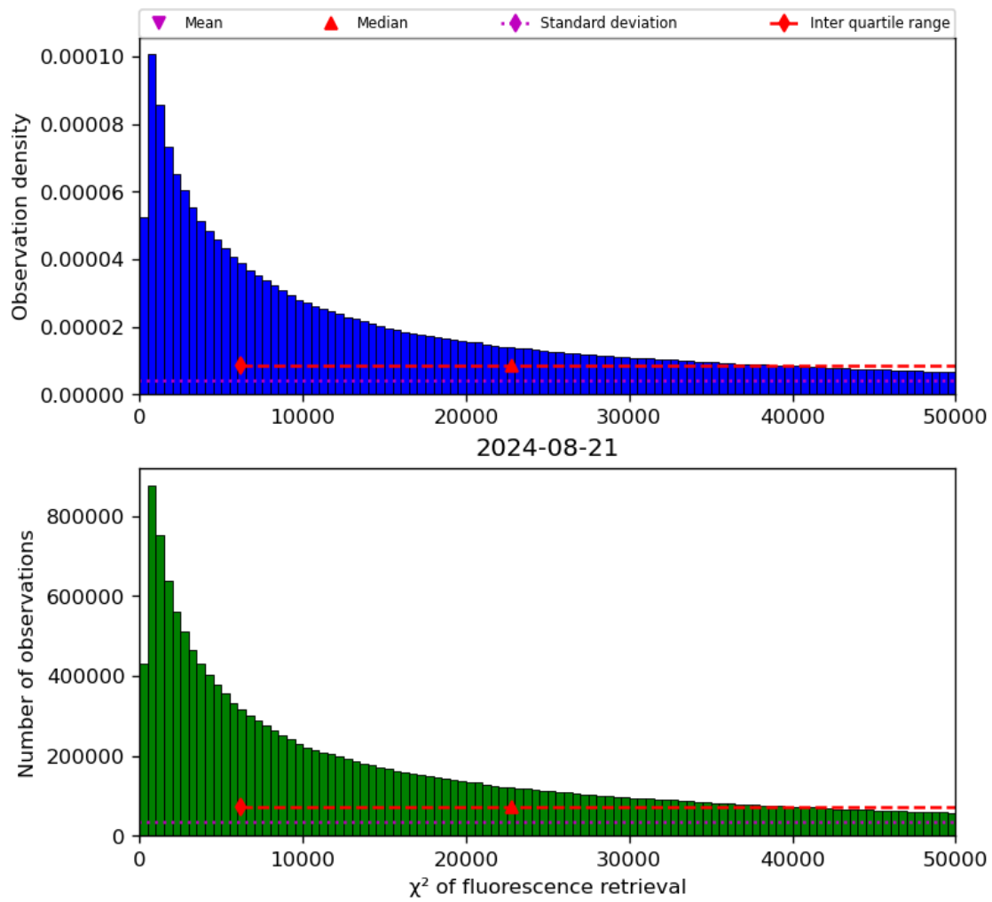
Figure 42: Histogram of “ \chi^2 of fluorescence retrieval” for 2024-08-21 to 2024-08-22
