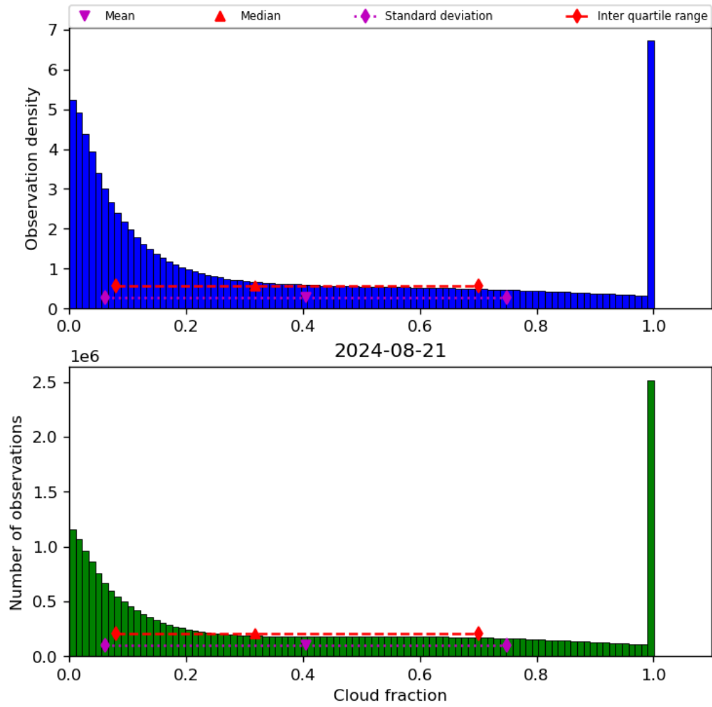
Figure 32: Histogram of “Cloud fraction” for 2024-08-21 to 2024-08-22
