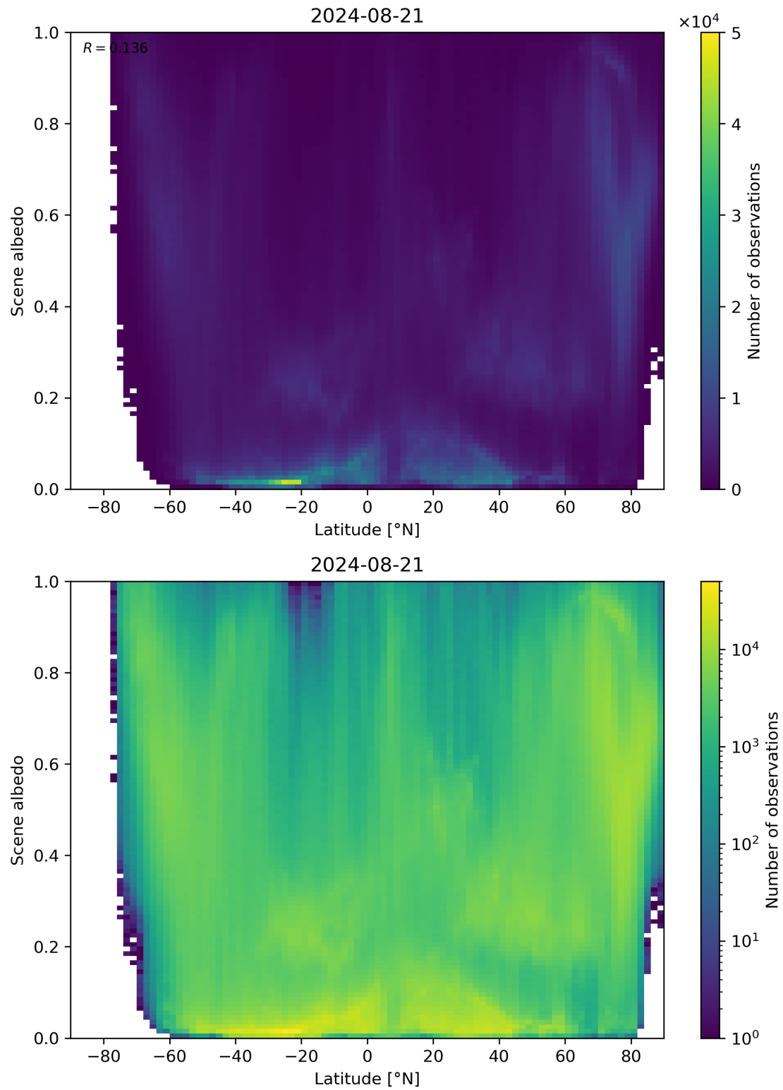
Figure 95: Scatter density plot of “Latitude” against “Scene albedo” for 2024-08-21 to 2024-08-22.
