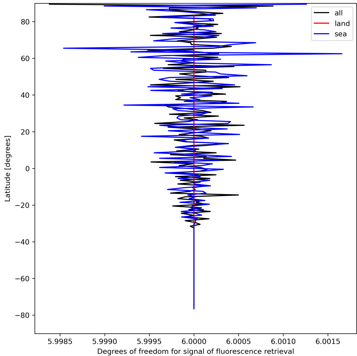
Figure 26: Zonal average of “Degrees of freedom for signal of fluorescence retrieval” for 2024-08-21 to 2024-08-22.
