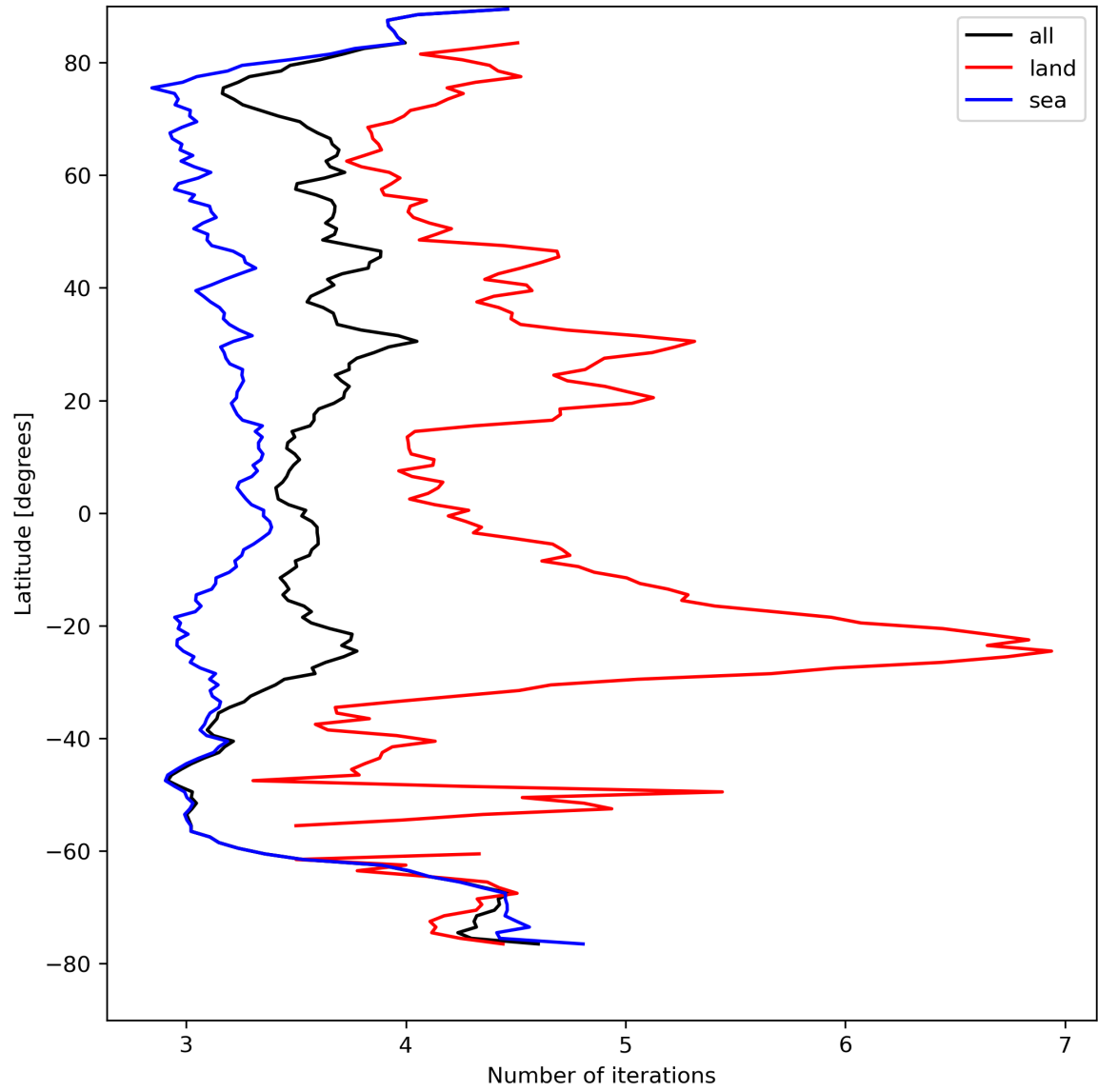
Figure 22: Zonal average of “Number of iterations” for 2024-08-21 to 2024-08-22.
