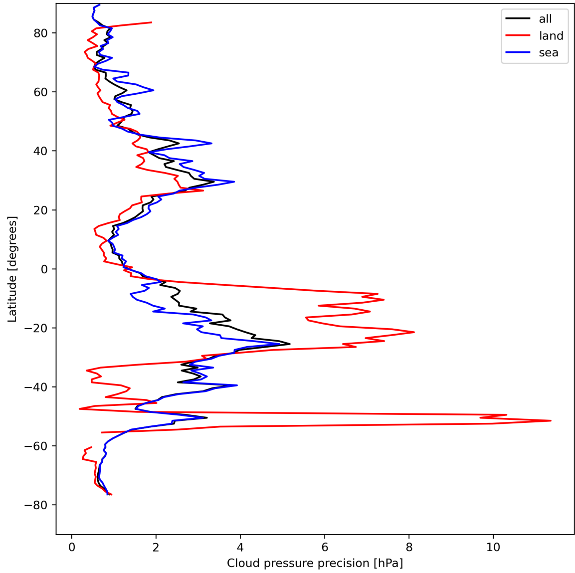
Figure 14: Zonal average of “Cloud pressure precision” for 2024-08-21 to 2024-08-22.
