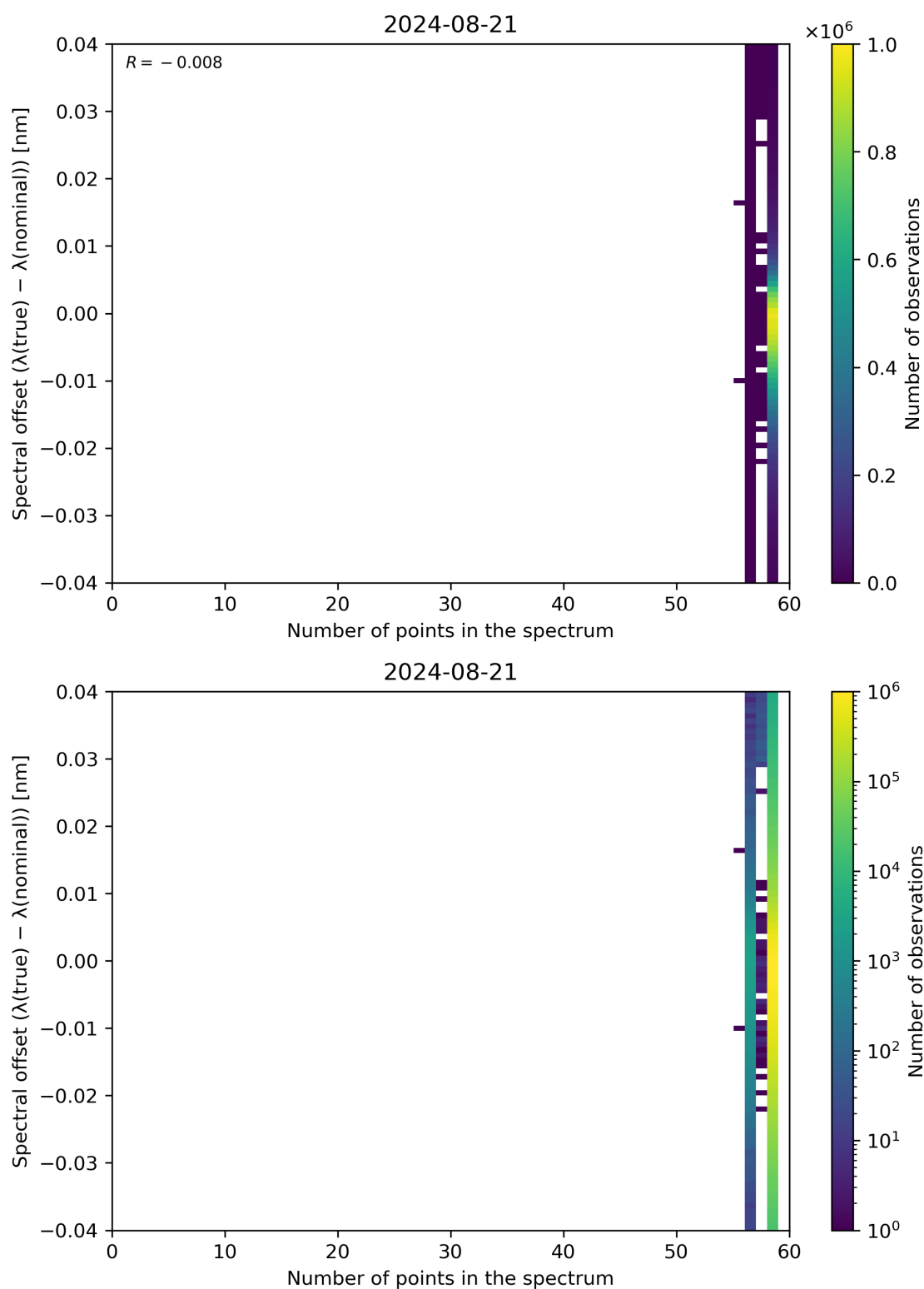
Figure 101: Scatter density plot of “Number of points in the spectrum” against “Spectral offset ( \lambda(\text{true}) - \lambda(\text{nominal}) )” for 2024-08-21 to 2024-08-22.
