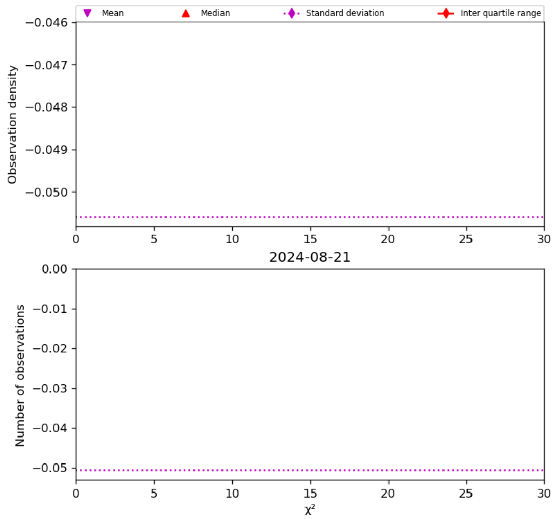
Figure 38: Histogram of " \chi^2 " for 2024-08-21 to 2024-08-22
