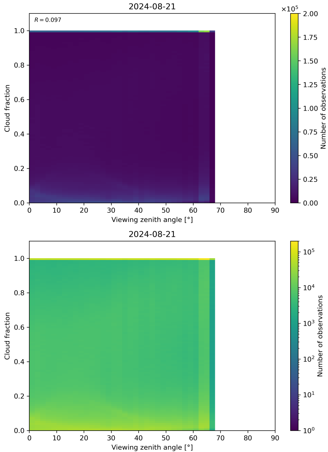
Figure 120: Scatter density plot of “Viewing zenith angle” against “Cloud fraction” for 2024-08-21 to 2024-08-22.
