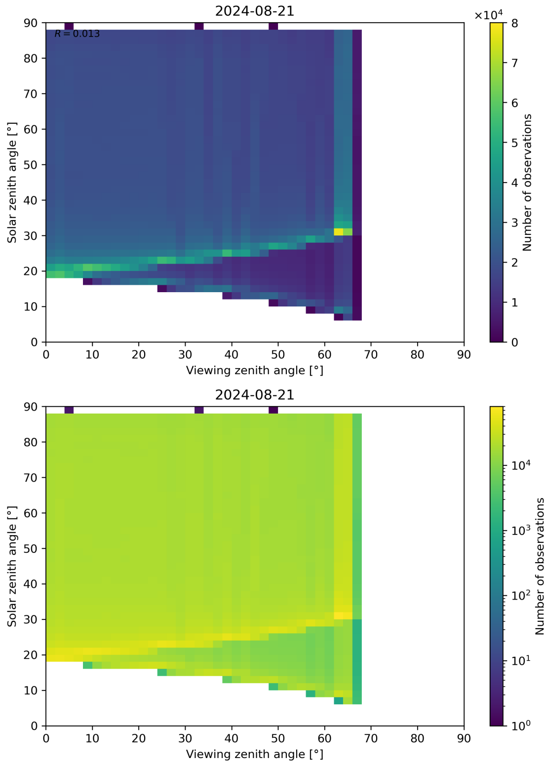
Figure 127: Scatter density plot of “Viewing zenith angle” against “Solar zenith angle” for 2024-08-21 to 2024-08-22.
