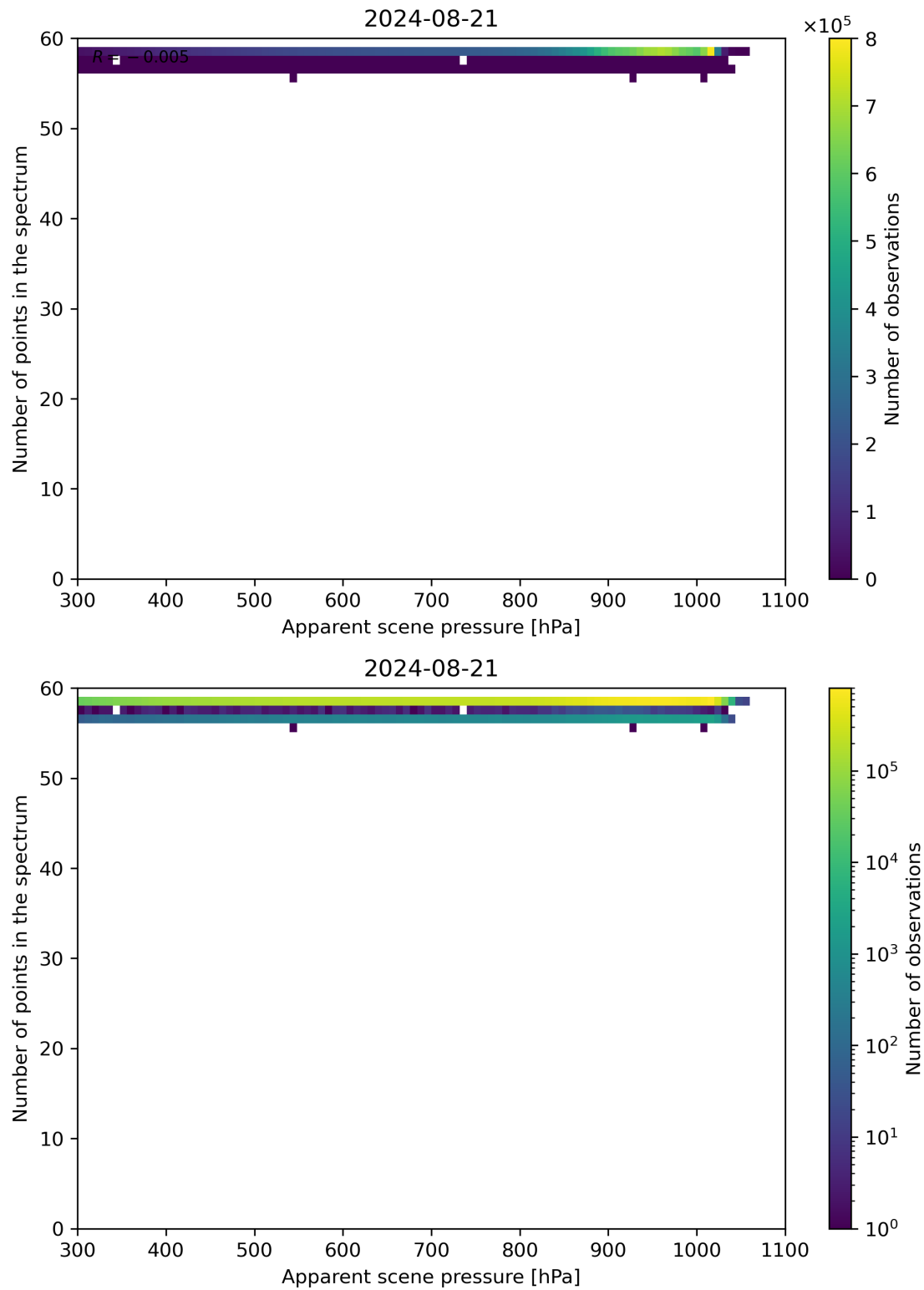
Figure 66: Scatter density plot of “Apparent scene pressure” against “Number of points in the spectrum” for 2024-08-21 to 2024-08-22.
