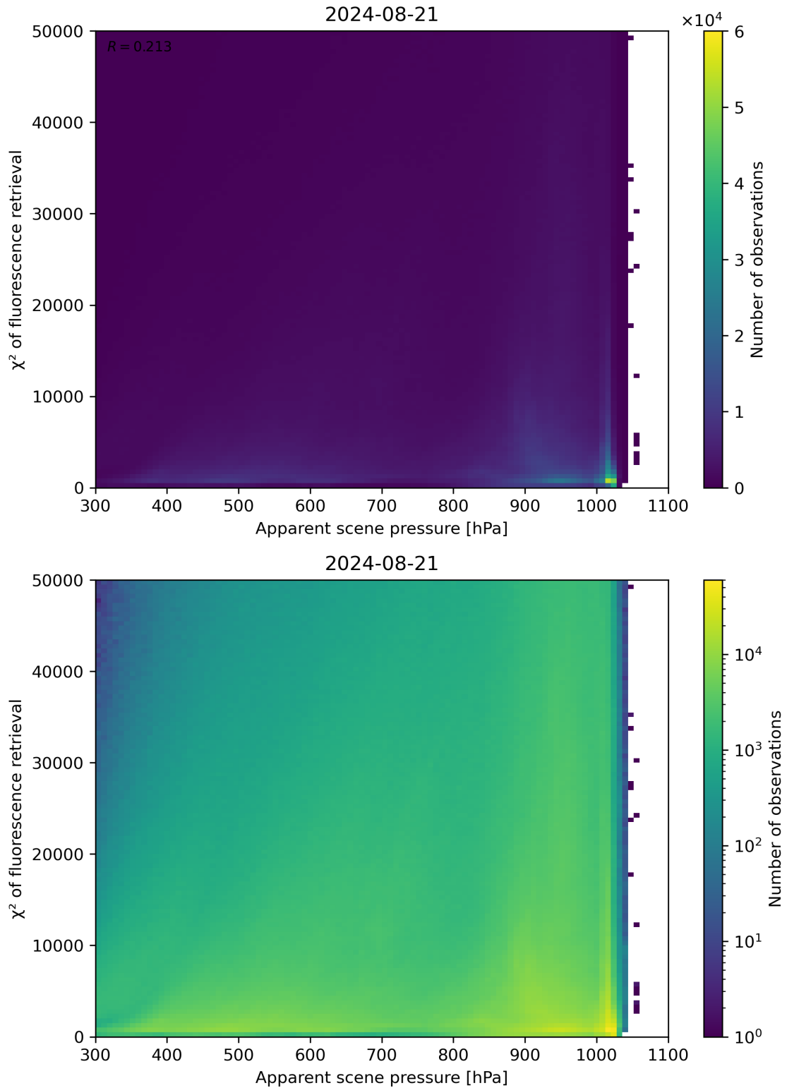
Figure 63: Scatter density plot of “Apparent scene pressure” against “ \chi^2 of fluorescence retrieval” for 2024-08-21 to 2024-08-22.
