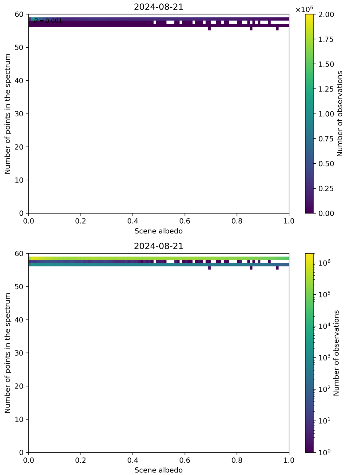
Figure 106: Scatter density plot of “Scene albedo” against “Number of points in the spectrum” for 2024-08-21 to 2024-08-22.
