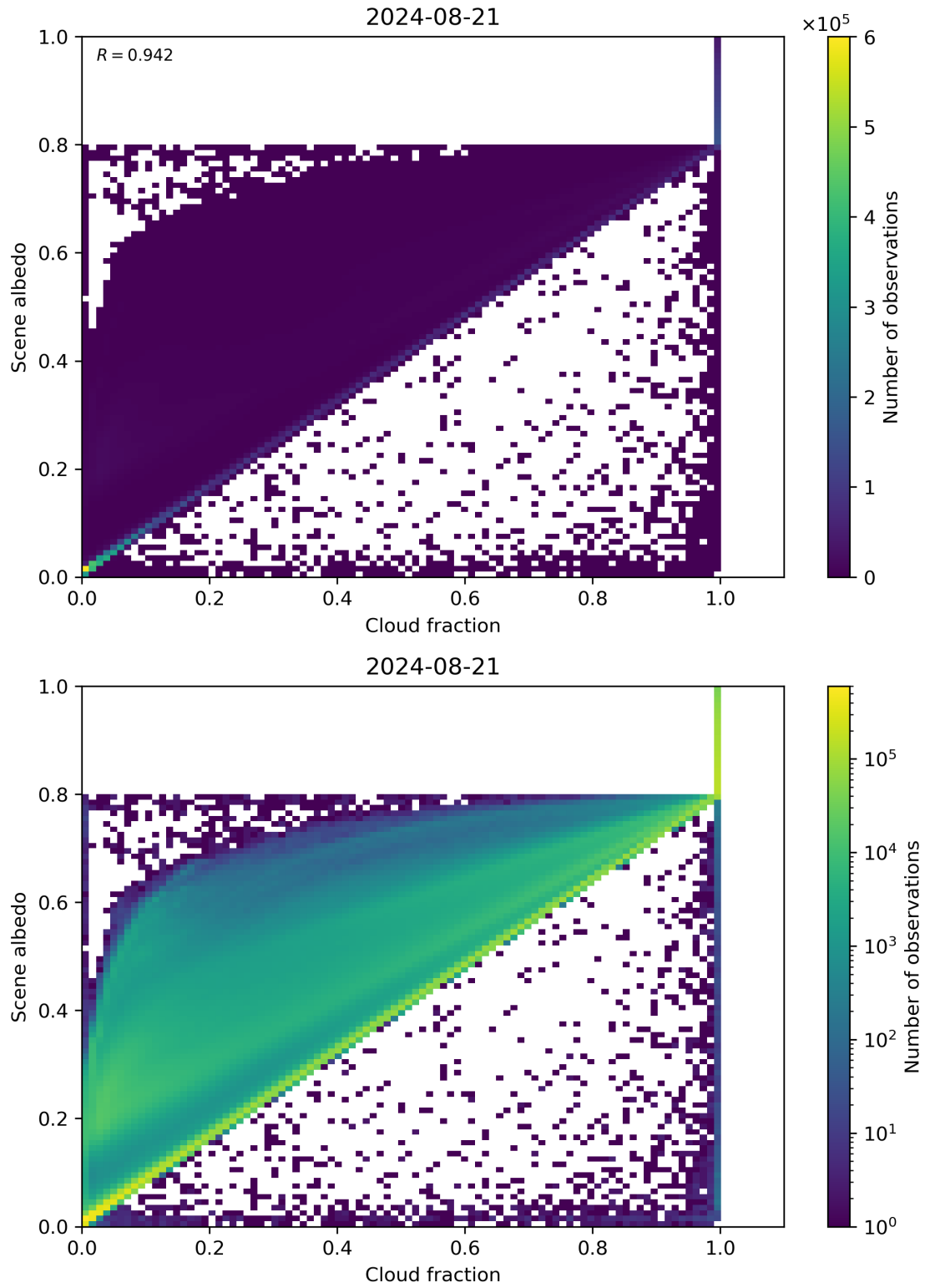
Figure 75: Scatter density plot of “Cloud fraction” against “Scene albedo” for 2024-08-21 to 2024-08-22.
