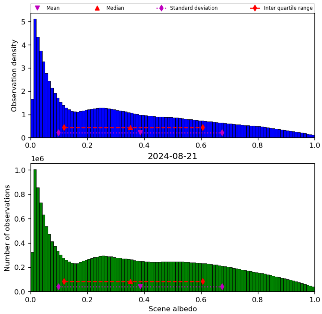
Figure 34: Histogram of “Scene albedo” for 2024-08-21 to 2024-08-22
