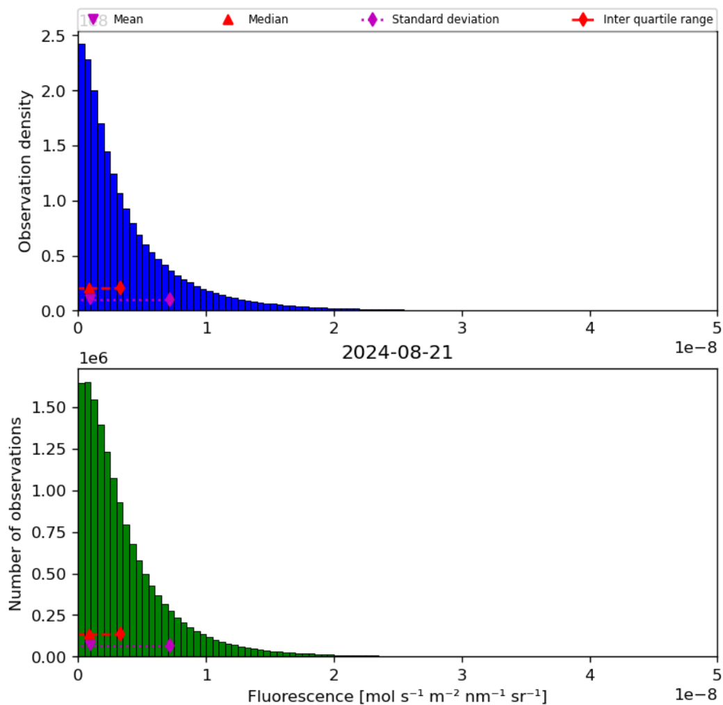
Figure 40: Histogram of “Fluorescence” for 2024-08-21 to 2024-08-22
