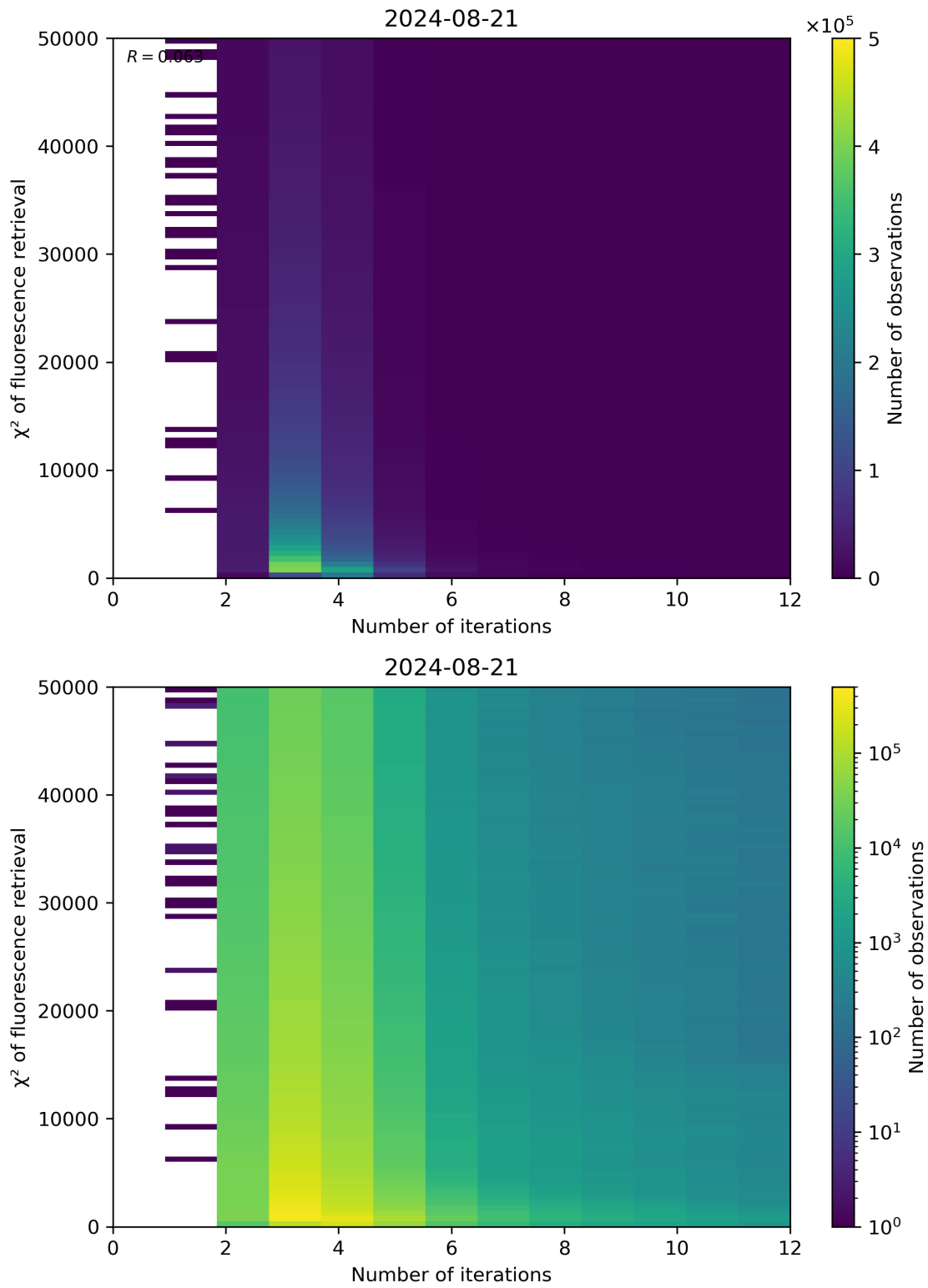
Figure 97: Scatter density plot of “Number of iterations” against “ \chi^2 of fluorescence retrieval” for 2024-08-21 to 2024-08-22.
