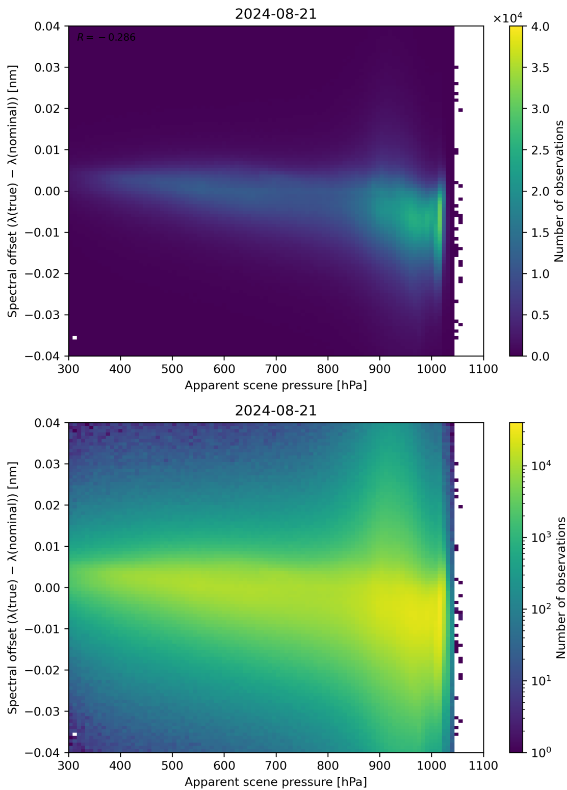
Figure 67: Scatter density plot of “Apparent scene pressure” against “Spectral offset ( \lambda(\text{true}) - \lambda(\text{nominal}) )” for 2024-08-21 to 2024-08-22.
