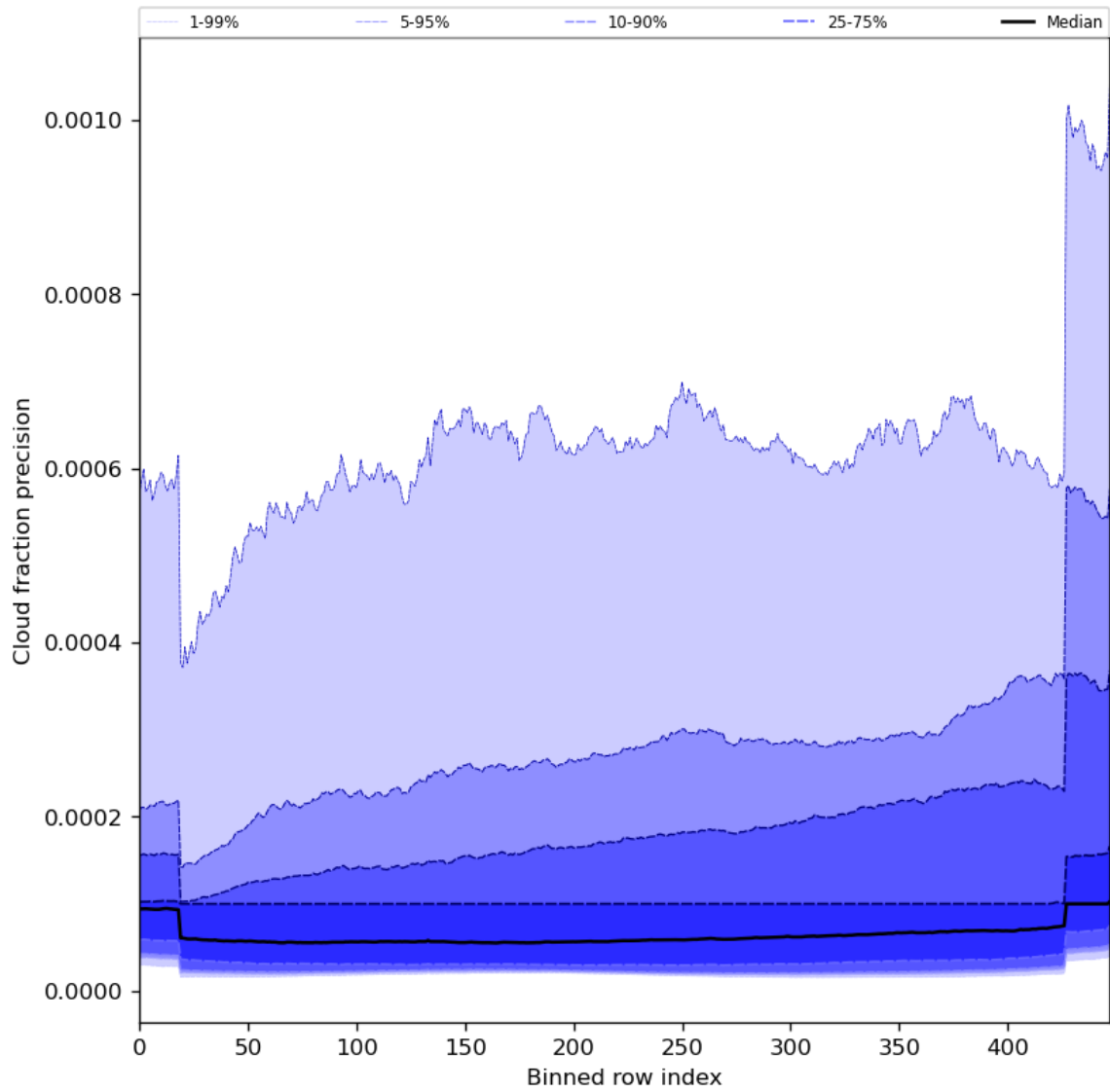
Figure 50: Along track statistics of “Cloud fraction precision” for 2024-08-21 to 2024-08-22
