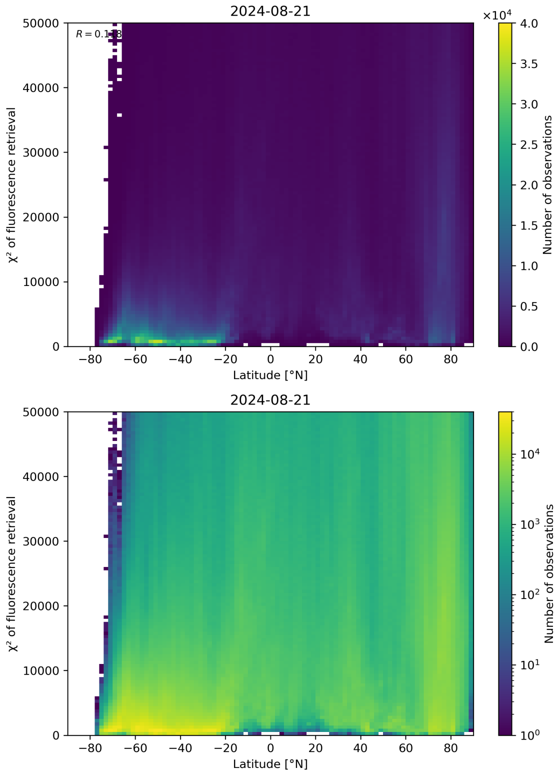
Figure 89: Scatter density plot of “Latitude” against “ \chi^2 of fluorescence retrieval” for 2024-08-21 to 2024-08-22.
