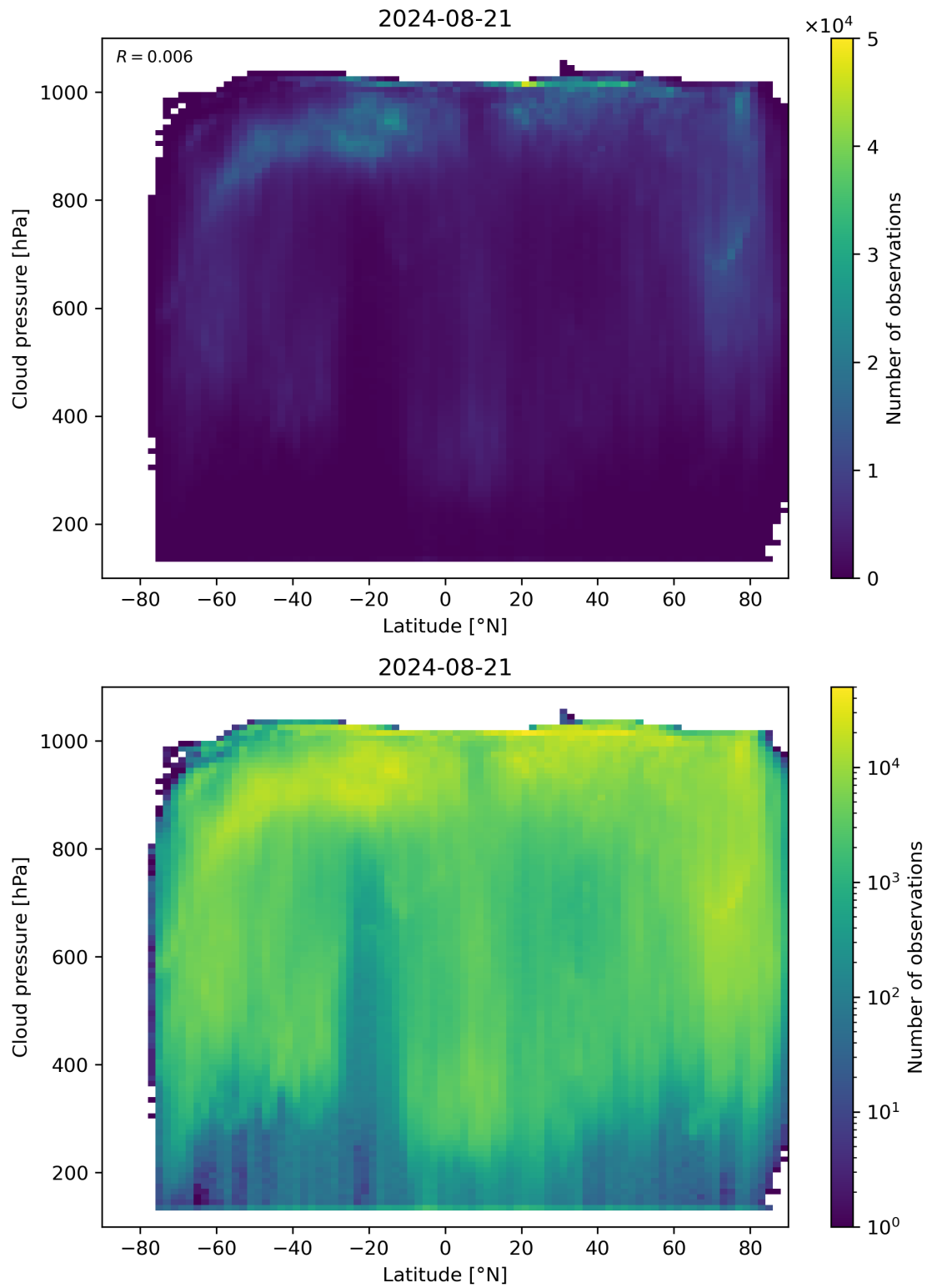
Figure 91: Scatter density plot of “Latitude” against “Cloud pressure” for 2024-08-21 to 2024-08-22.
