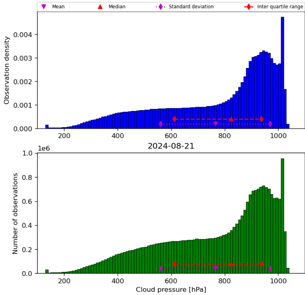
Figure 30: Histogram of “Cloud pressure” for 2024-08-21 to 2024-08-22
