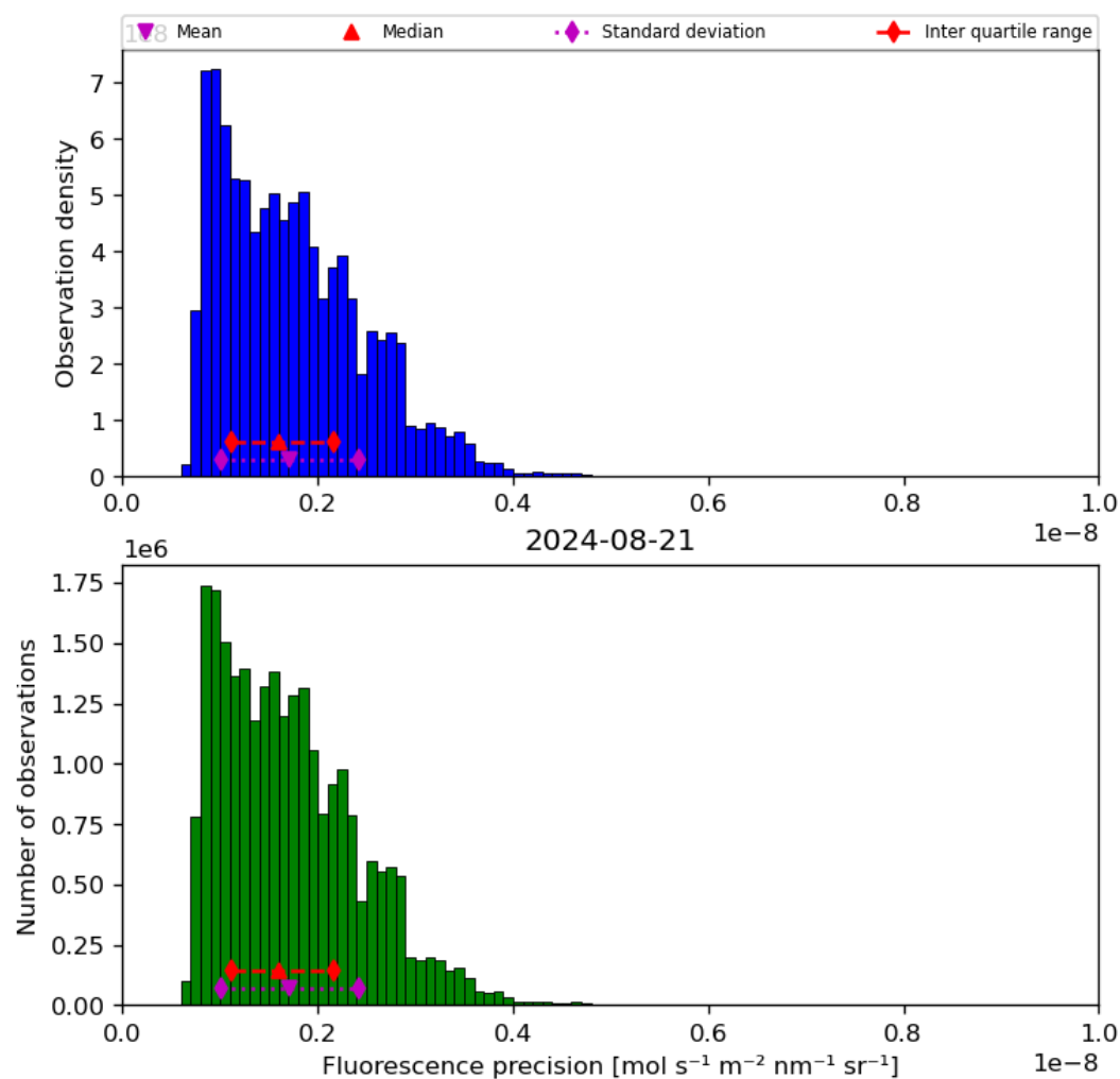
Figure 41: Histogram of “Fluorescence precision” for 2024-08-21 to 2024-08-22
