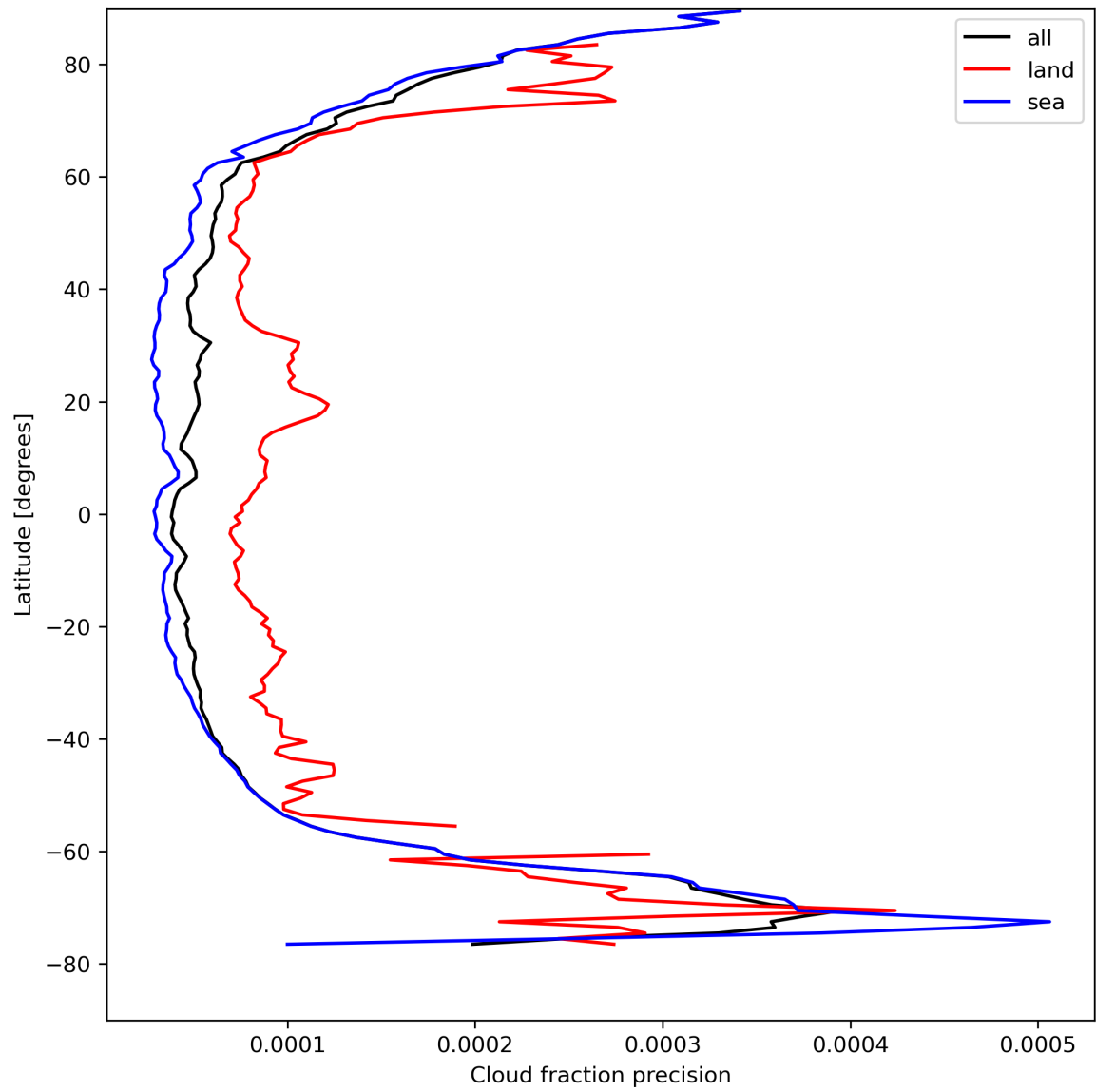
Figure 16: Zonal average of “Cloud fraction precision” for 2024-08-21 to 2024-08-22.
