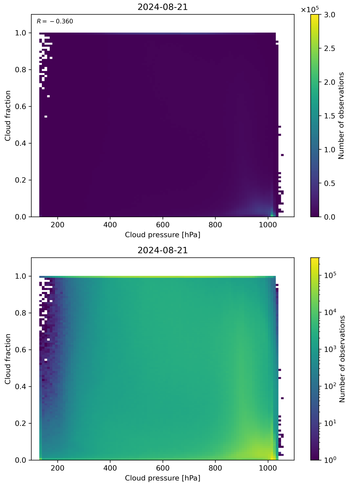
Figure 79: Scatter density plot of “Cloud pressure” against “Cloud fraction” for 2024-08-21 to 2024-08-22.
