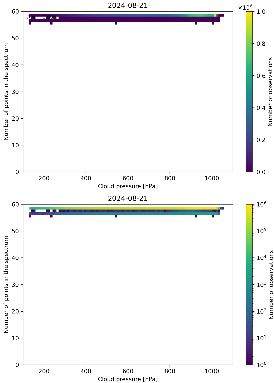
Figure 82: Scatter density plot of “Cloud pressure” against “Number of points in the spectrum” for 2024-08-21 to 2024-08-22.
