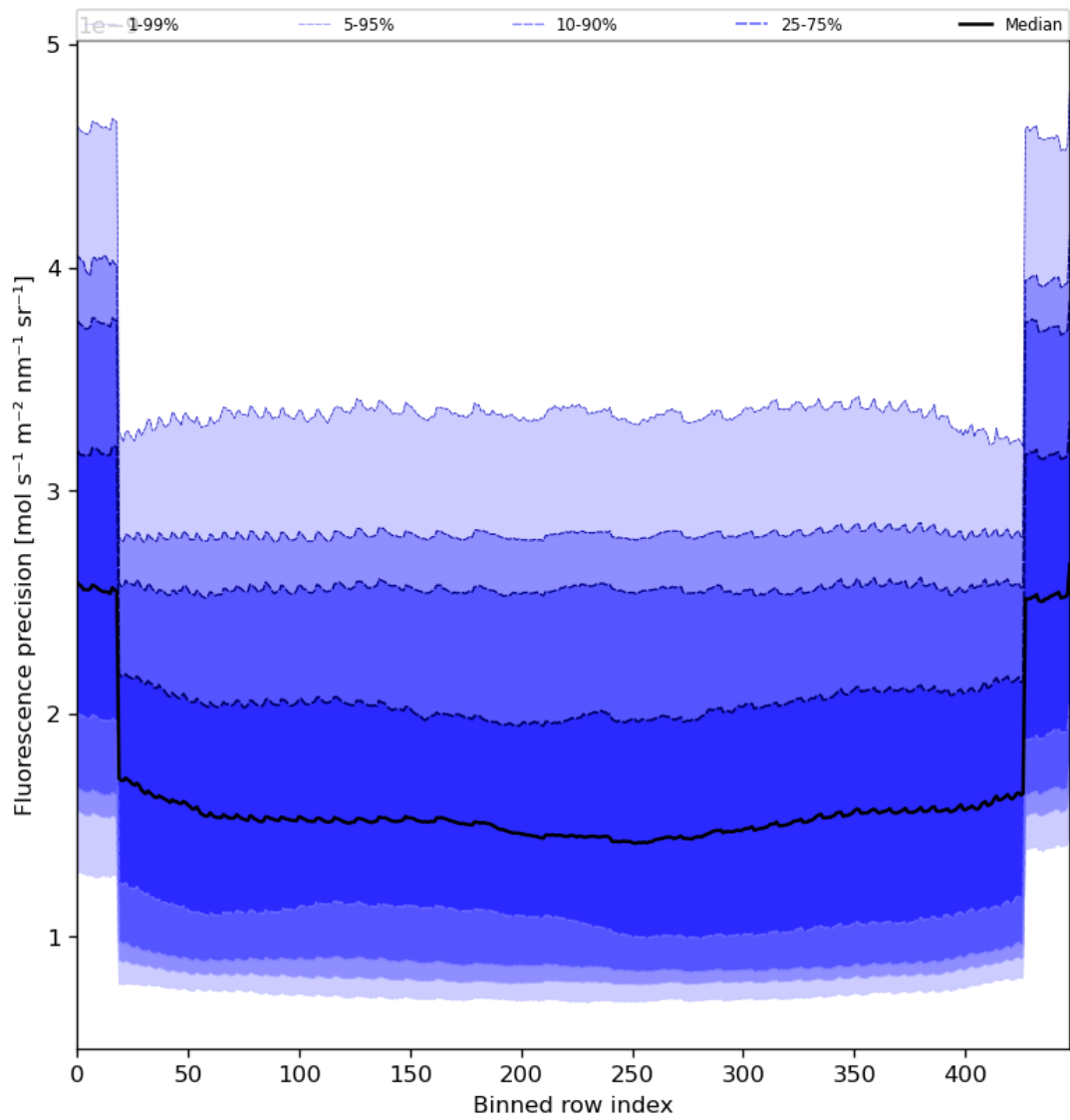
Figure 58: Along track statistics of “Fluorescence precision” for 2024-08-21 to 2024-08-22
