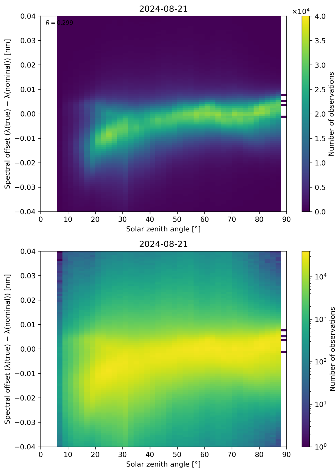
Figure 117: Scatter density plot of “Solar zenith angle” against “Spectral offset ( \lambda(\text{true}) - \lambda(\text{nominal}) )” for 2024-08-21 to 2024-08-22.
