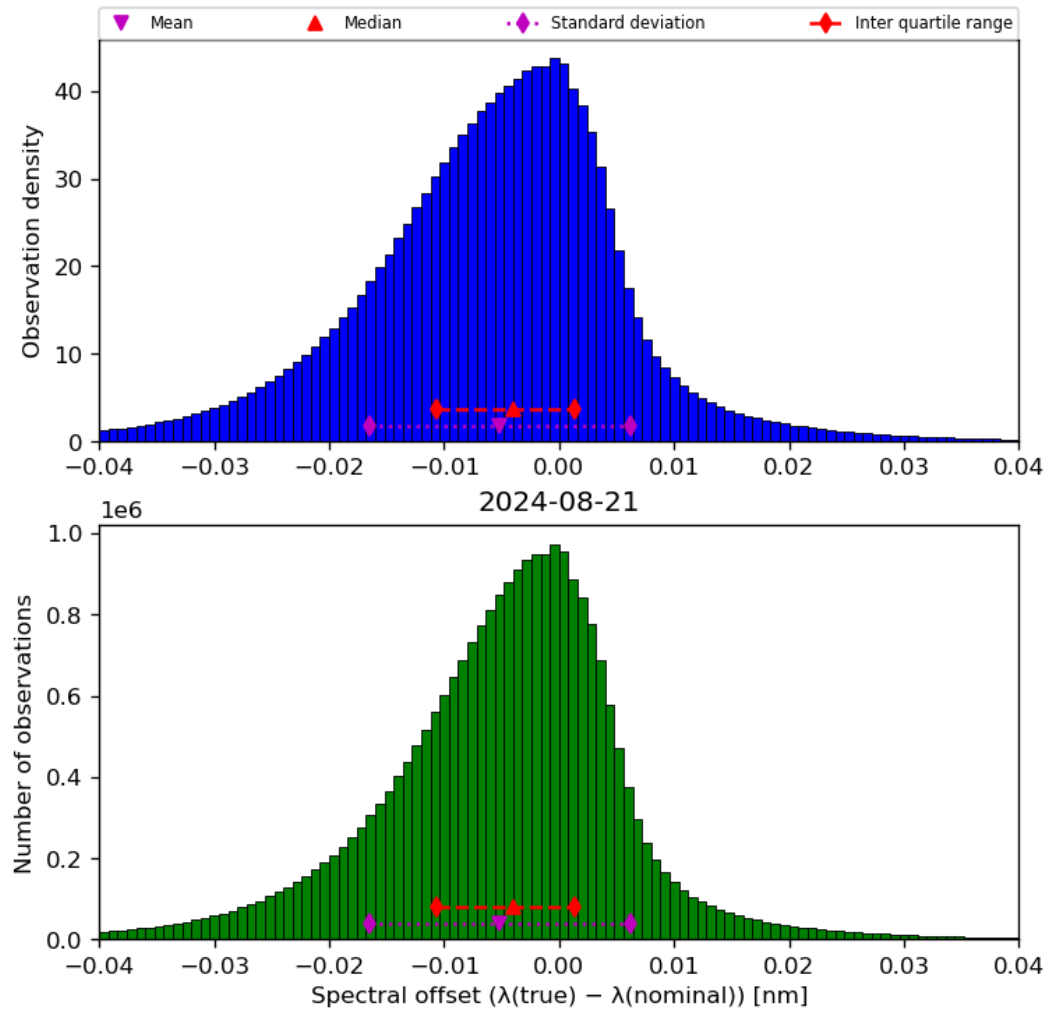
Figure 45: Histogram of “Spectral offset ( \lambda(\text{true}) - \lambda(\text{nominal}) )” for 2024-08-21 to 2024-08-22
