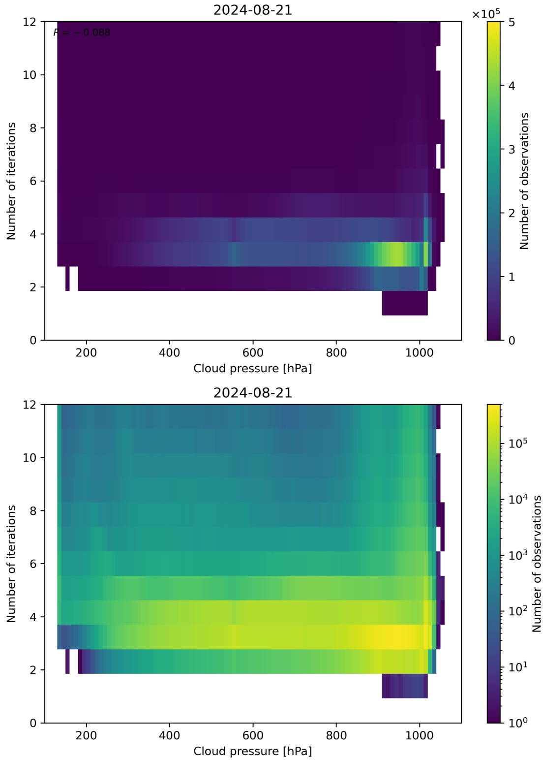
Figure 81: Scatter density plot of “Cloud pressure” against “Number of iterations” for 2024-08-21 to 2024-08-22.
