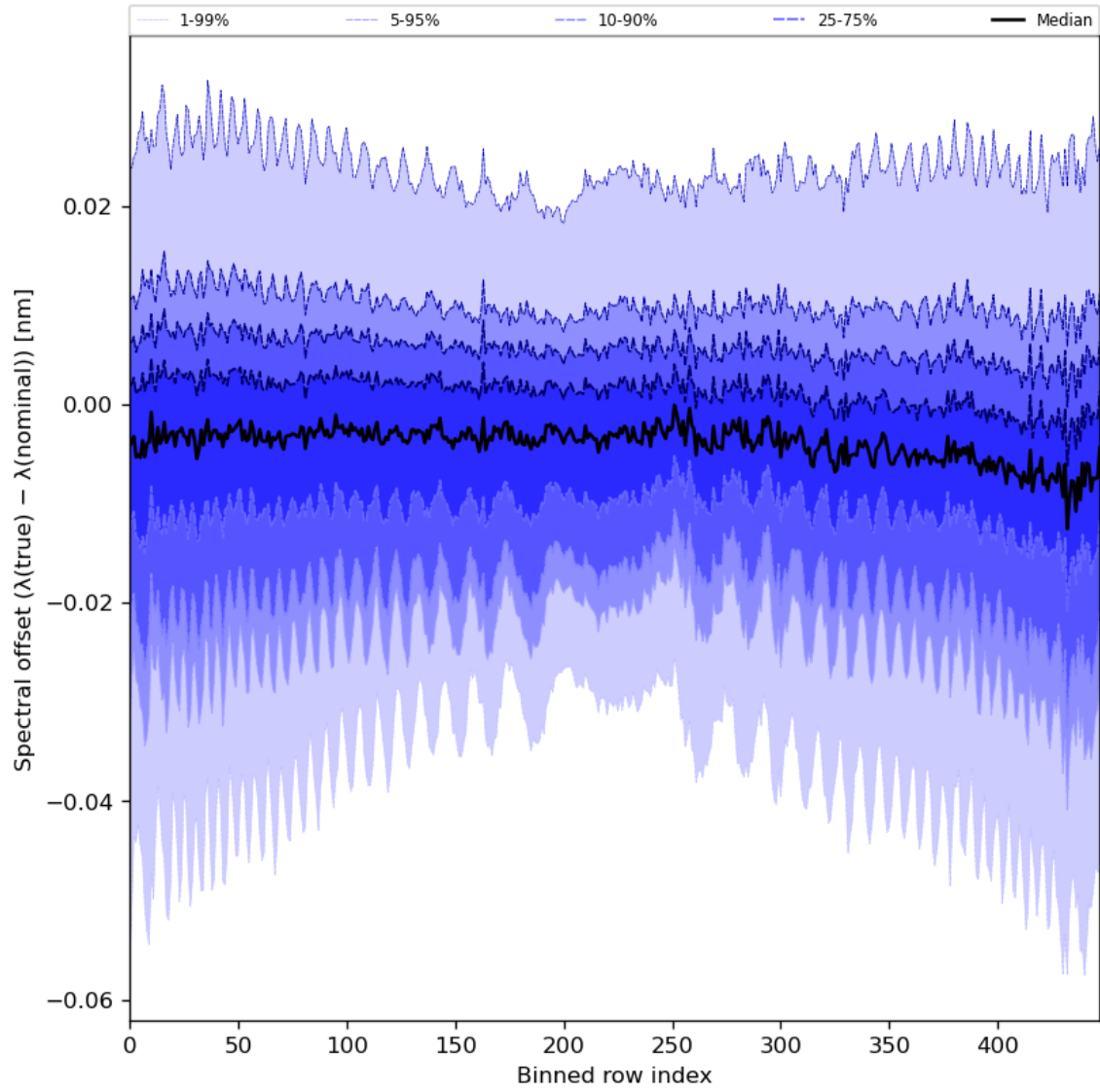
Figure 62: Along track statistics of “Spectral offset ( \lambda(\text{true}) - \lambda(\text{nominal}) )” for 2024-08-21 to 2024-08-22
