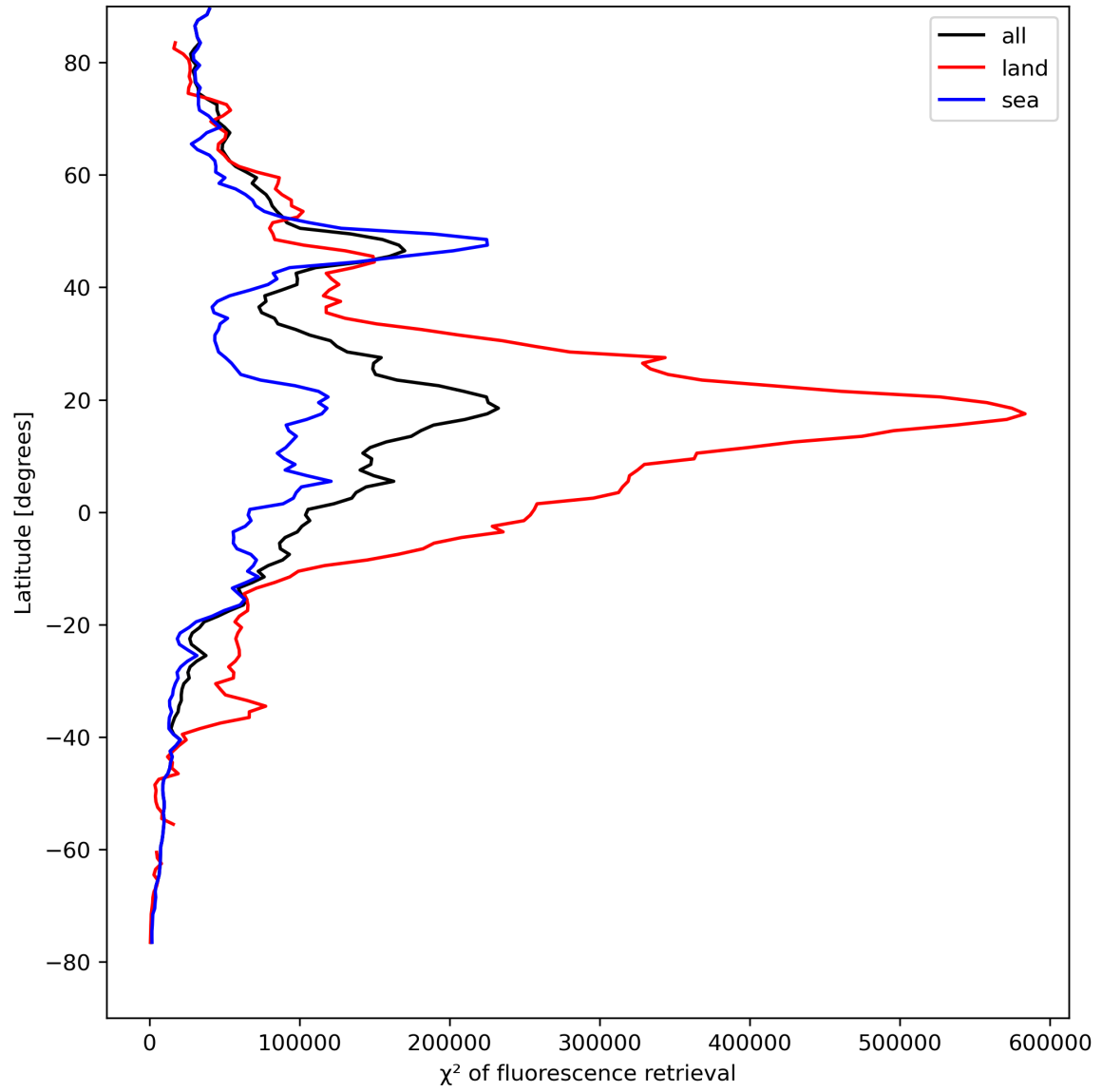
Figure 25: Zonal average of “ \chi^2 of fluorescence retrieval” for 2024-08-21 to 2024-08-22.
