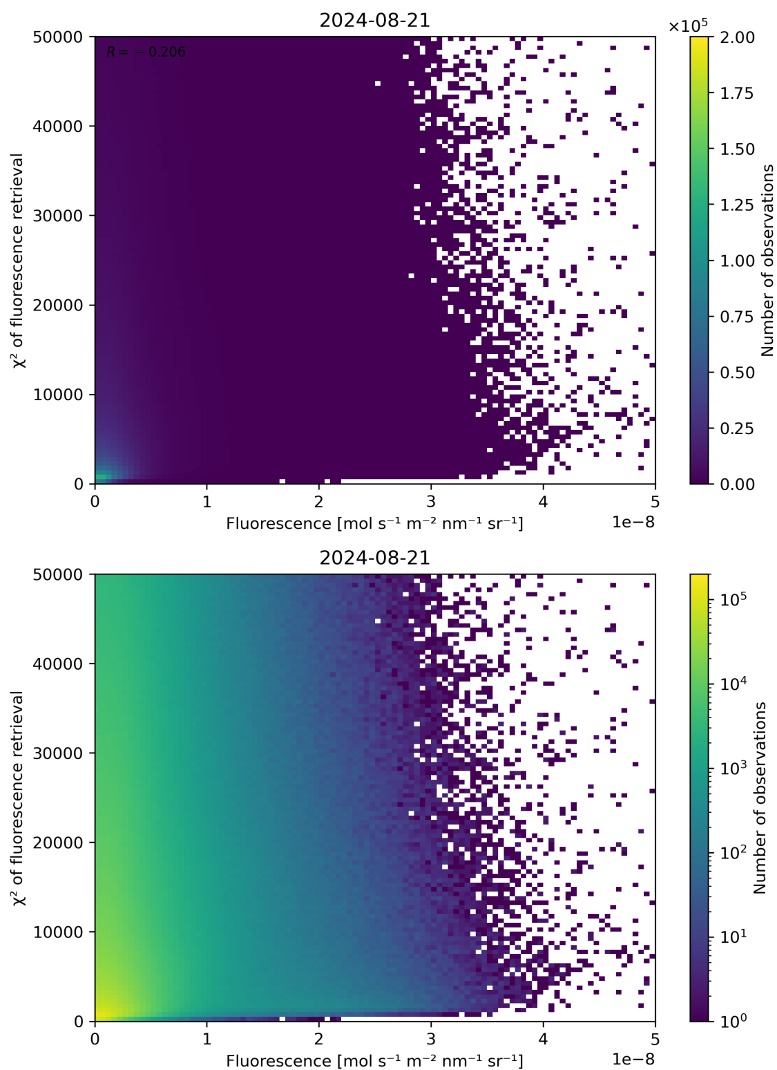
Figure 85: Scatter density plot of “Fluorescence” against “ \chi^2 of fluorescence retrieval” for 2024-08-21 to 2024-08-22.
