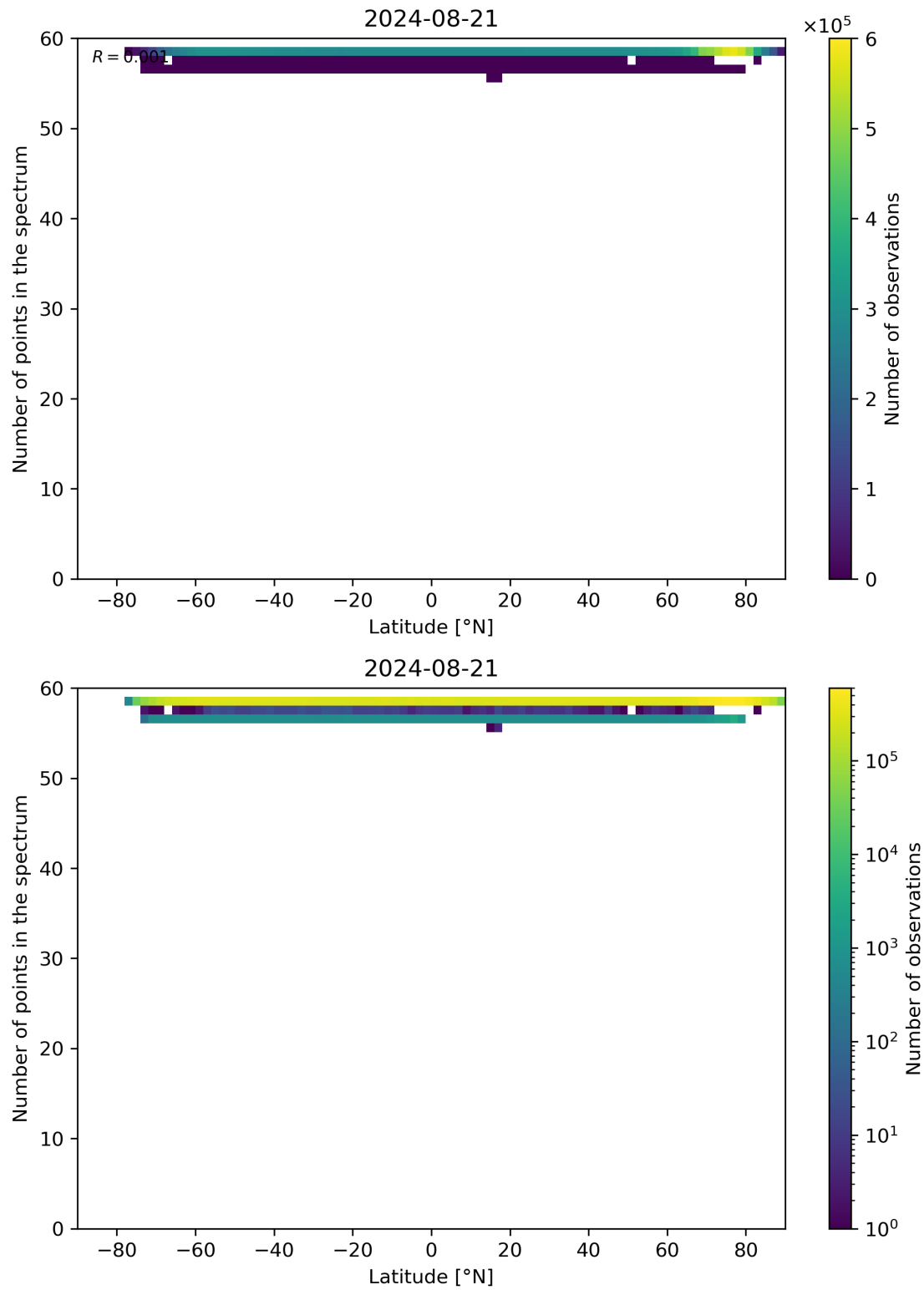
Figure 94: Scatter density plot of “Latitude” against “Number of points in the spectrum” for 2024-08-21 to 2024-08-22.
