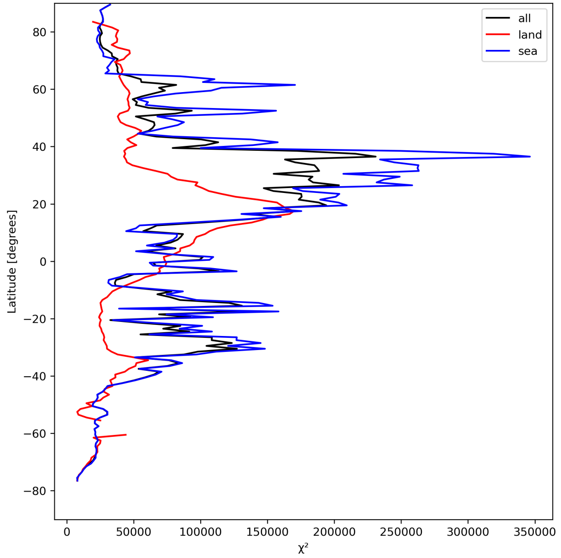
Figure 21: Zonal average of “ \chi^2 ” for 2024-08-21 to 2024-08-22.
