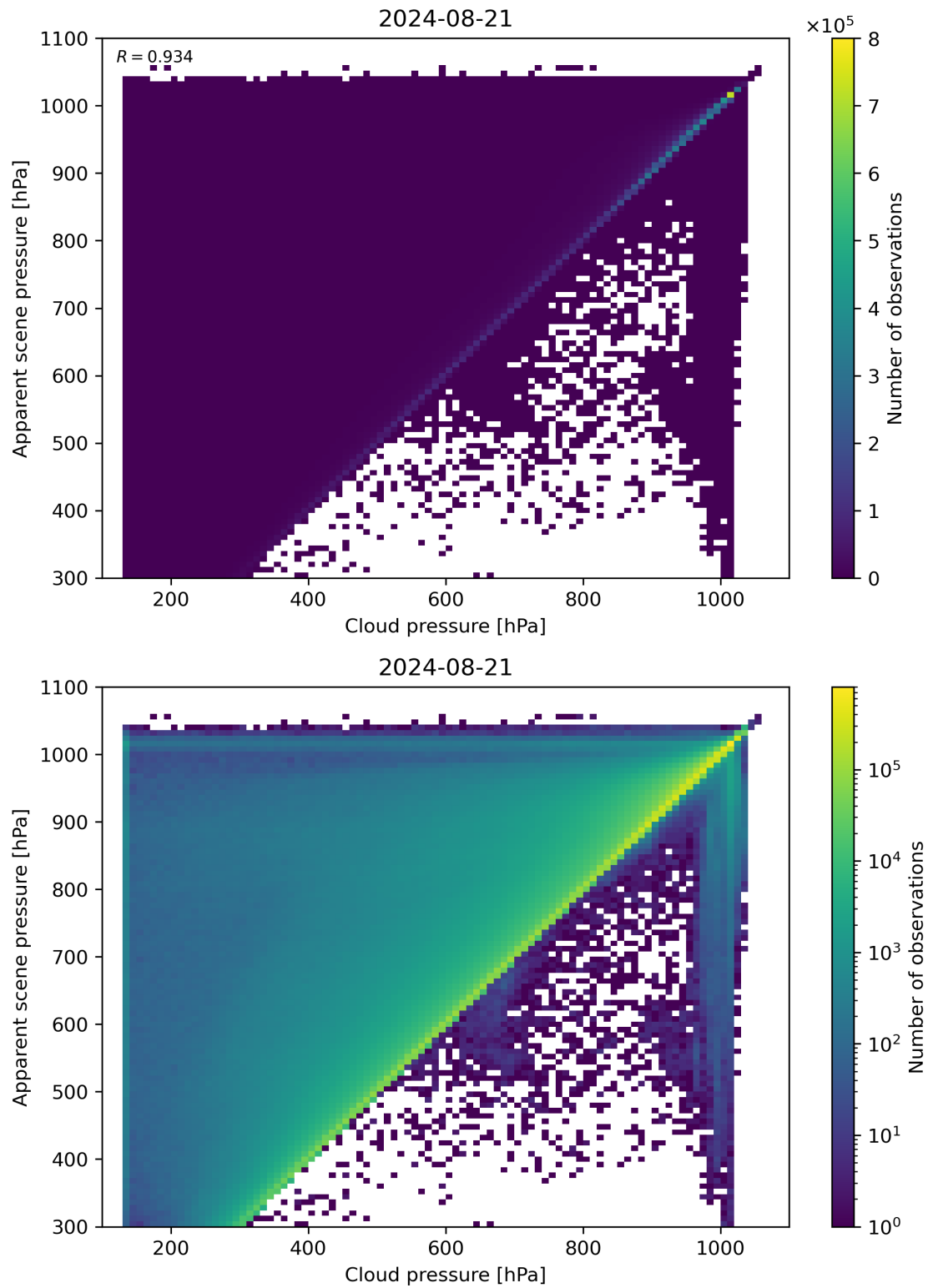
Figure 77: Scatter density plot of “Cloud pressure” against “Apparent scene pressure” for 2024-08-21 to 2024-08-22.
