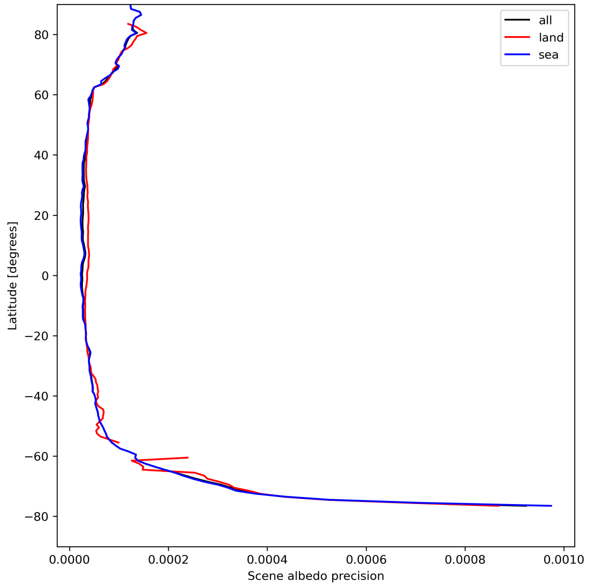
Figure 18: Zonal average of “Scene albedo precision” for 2024-08-21 to 2024-08-22.
