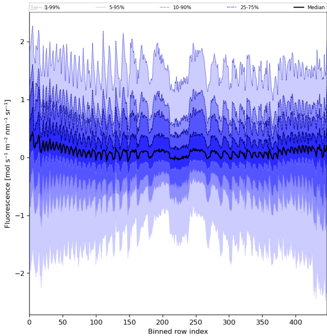
Figure 57: Along track statistics of “Fluorescence” for 2024-08-21 to 2024-08-22
