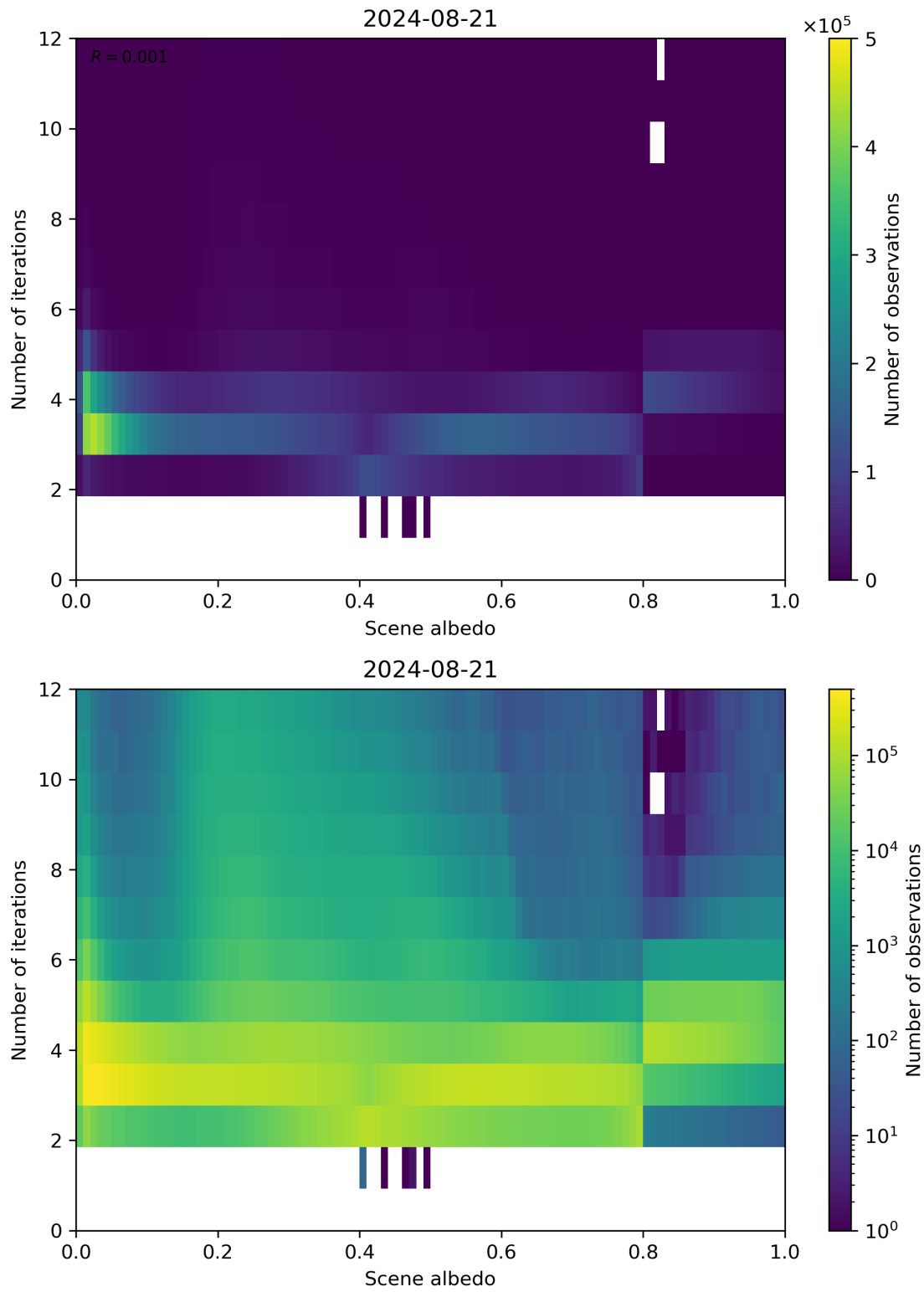
Figure 105: Scatter density plot of “Scene albedo” against “Number of iterations” for 2024-08-21 to 2024-08-22.
