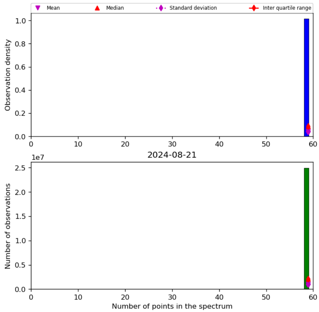
Figure 44: Histogram of “Number of points in the spectrum” for 2024-08-21 to 2024-08-22
