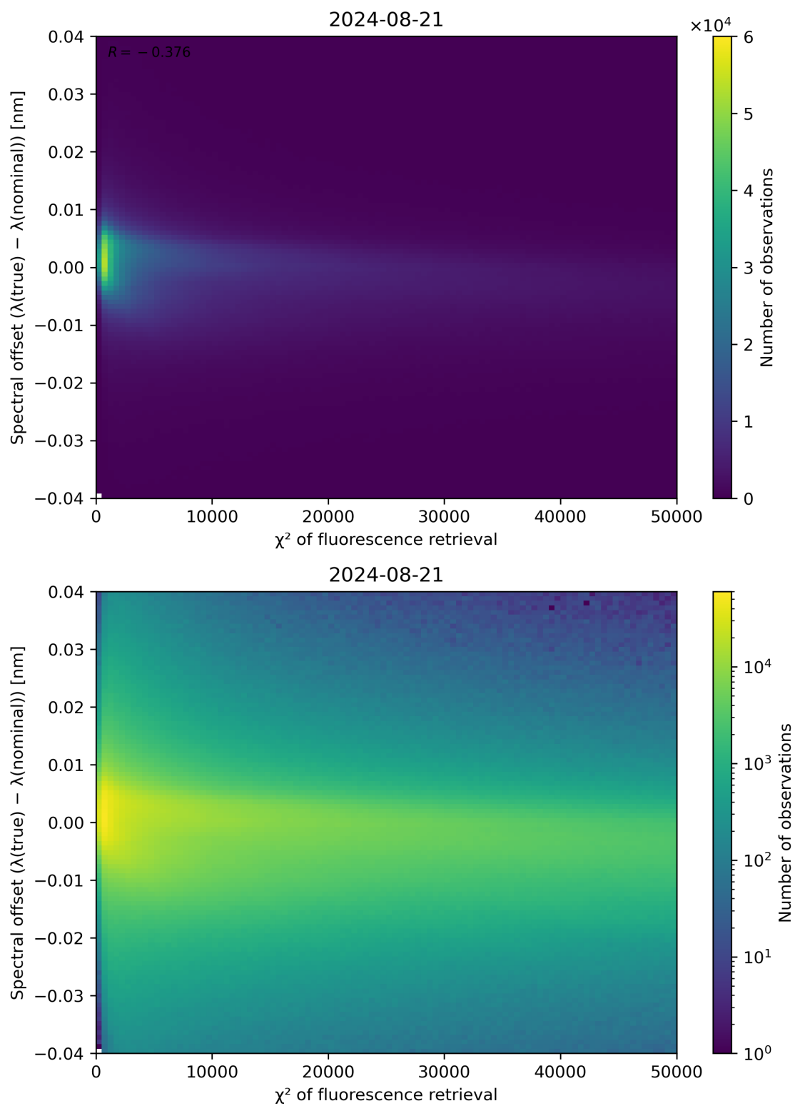
Figure 69: Scatter density plot of " \chi^2 of fluorescence retrieval" against "Spectral offset ( \lambda(\text{true}) - \lambda(\text{nominal}) )" for 2024-08-21 to 2024-08-22.
