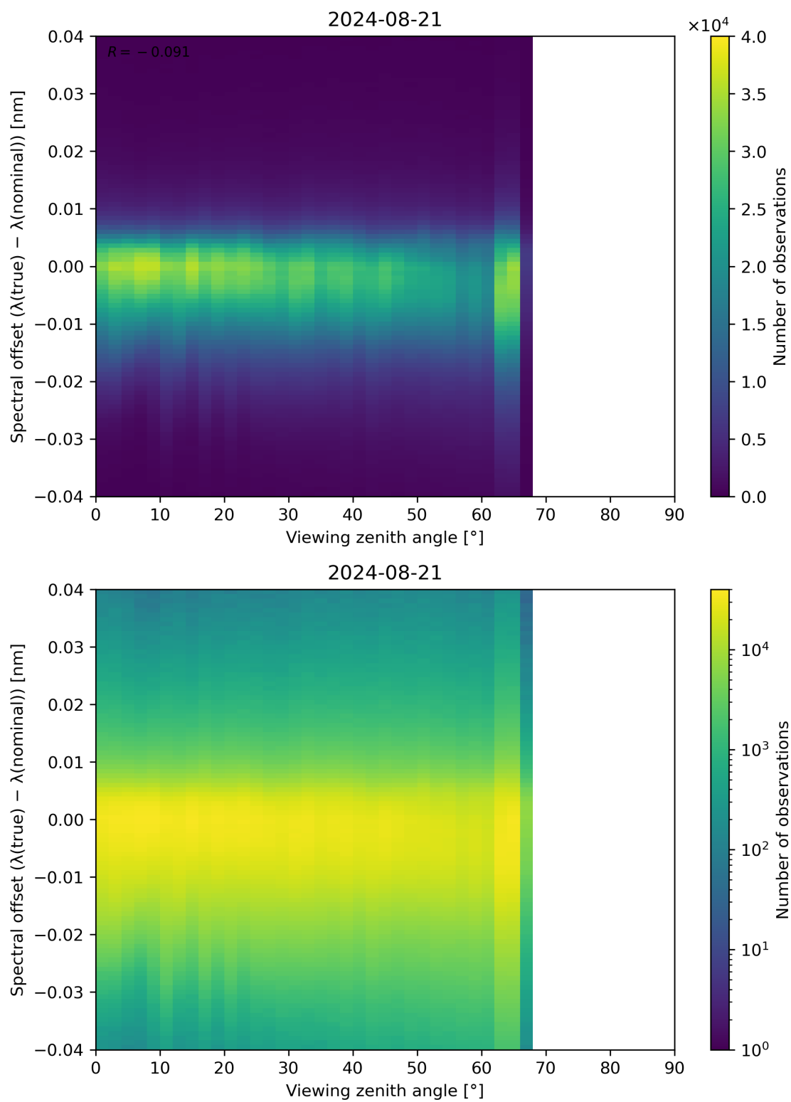
Figure 128: Scatter density plot of “Viewing zenith angle” against “Spectral offset ( \lambda(\text{true}) - \lambda(\text{nominal}) )” for 2024-08-21 to 2024-08-22.
