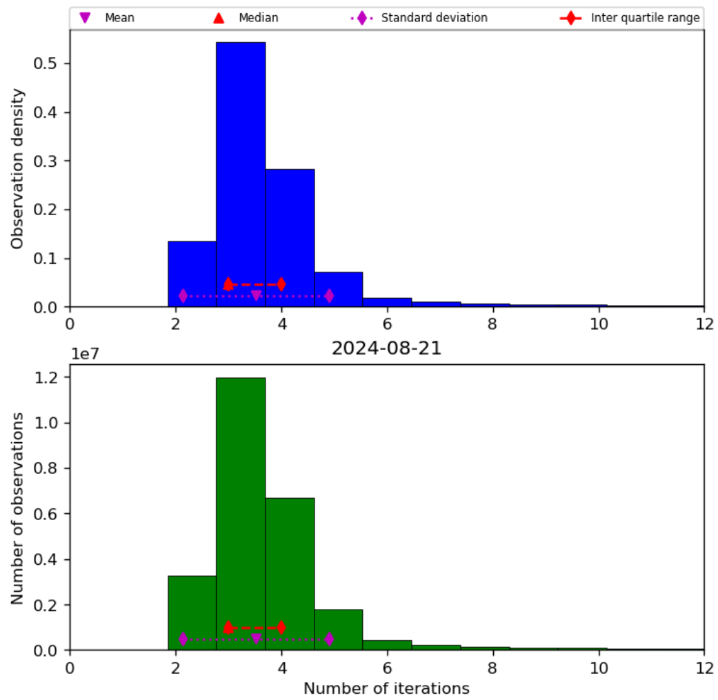
Figure 39: Histogram of “Number of iterations” for 2024-08-21 to 2024-08-22
