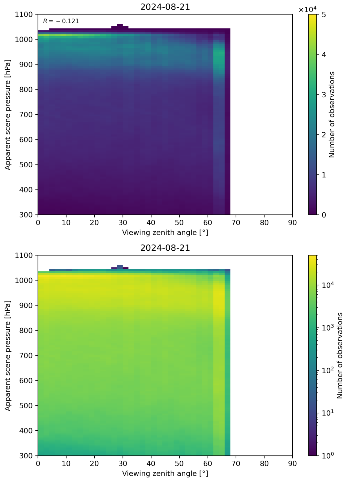
Figure 118: Scatter density plot of “Viewing zenith angle” against “Apparent scene pressure” for 2024-08-21 to 2024-08-22.
