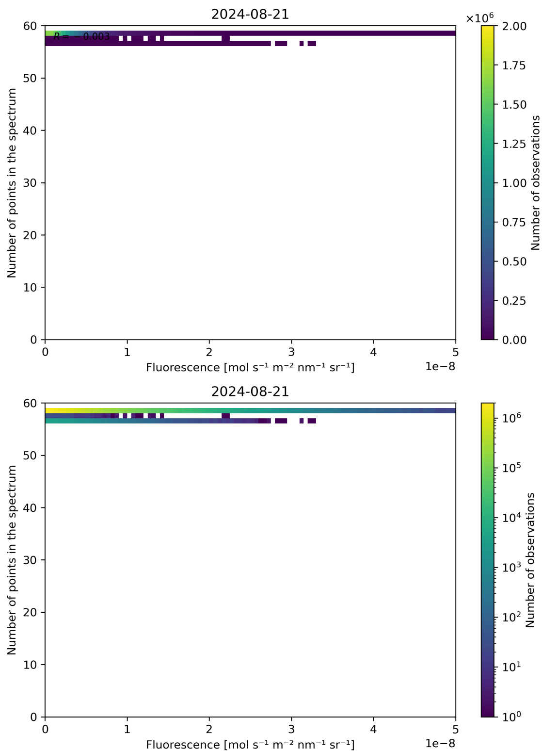
Figure 86: Scatter density plot of “Fluorescence” against “Number of points in the spectrum” for 2024-08-21 to 2024-08-22.
