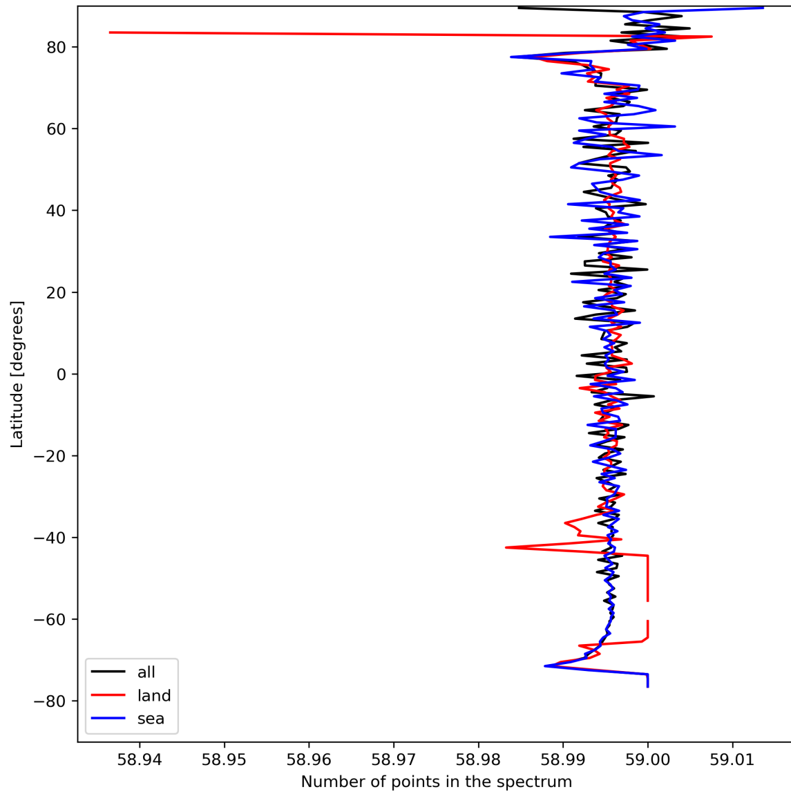
Figure 27: Zonal average of “Number of points in the spectrum” for 2024-08-21 to 2024-08-22.
