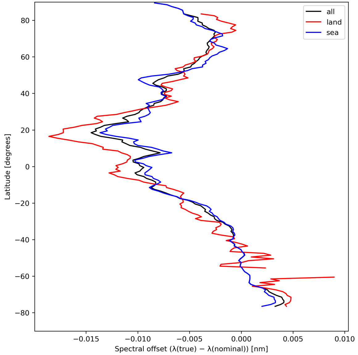
Figure 28: Zonal average of “Spectral offset ( \lambda(\text{true}) - \lambda(\text{nominal}) )” for 2024-08-21 to 2024-08-22.
