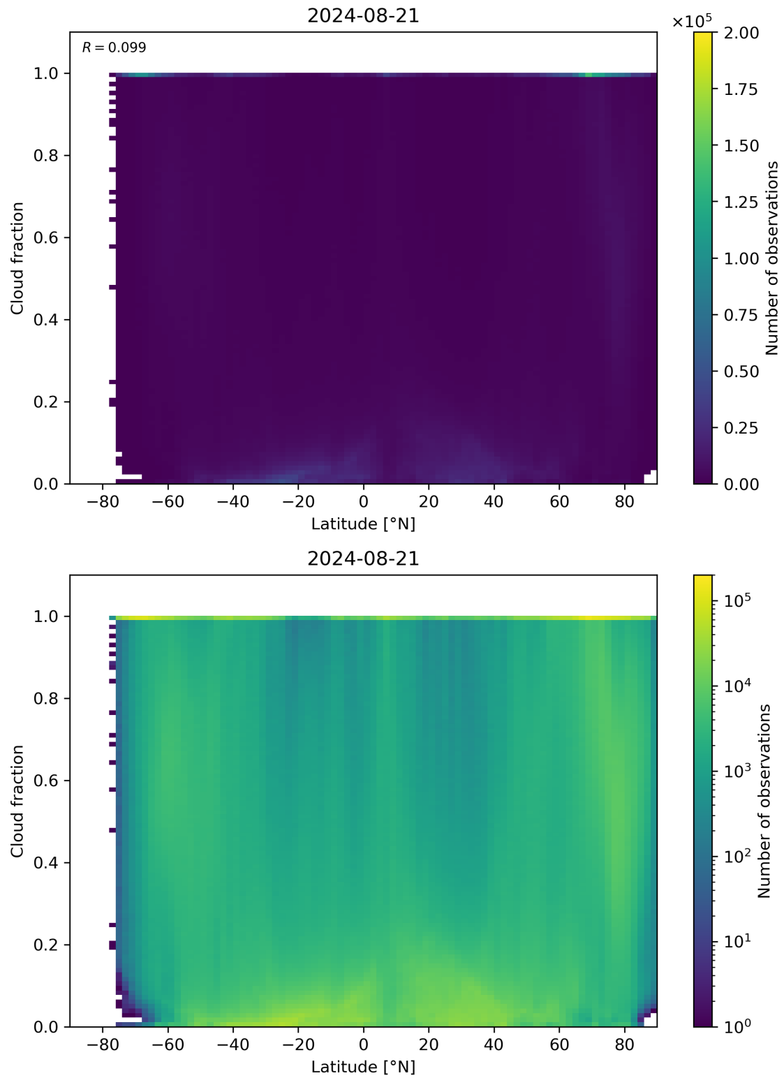
Figure 90: Scatter density plot of “Latitude” against “Cloud fraction” for 2024-08-21 to 2024-08-22.
