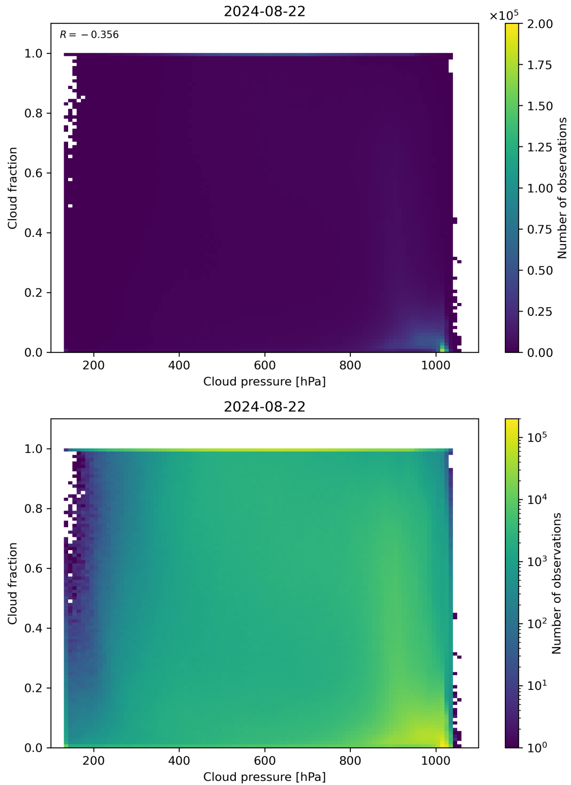
Figure 79: Scatter density plot of “Cloud pressure” against “Cloud fraction” for 2024-08-22 to 2024-08-23.
