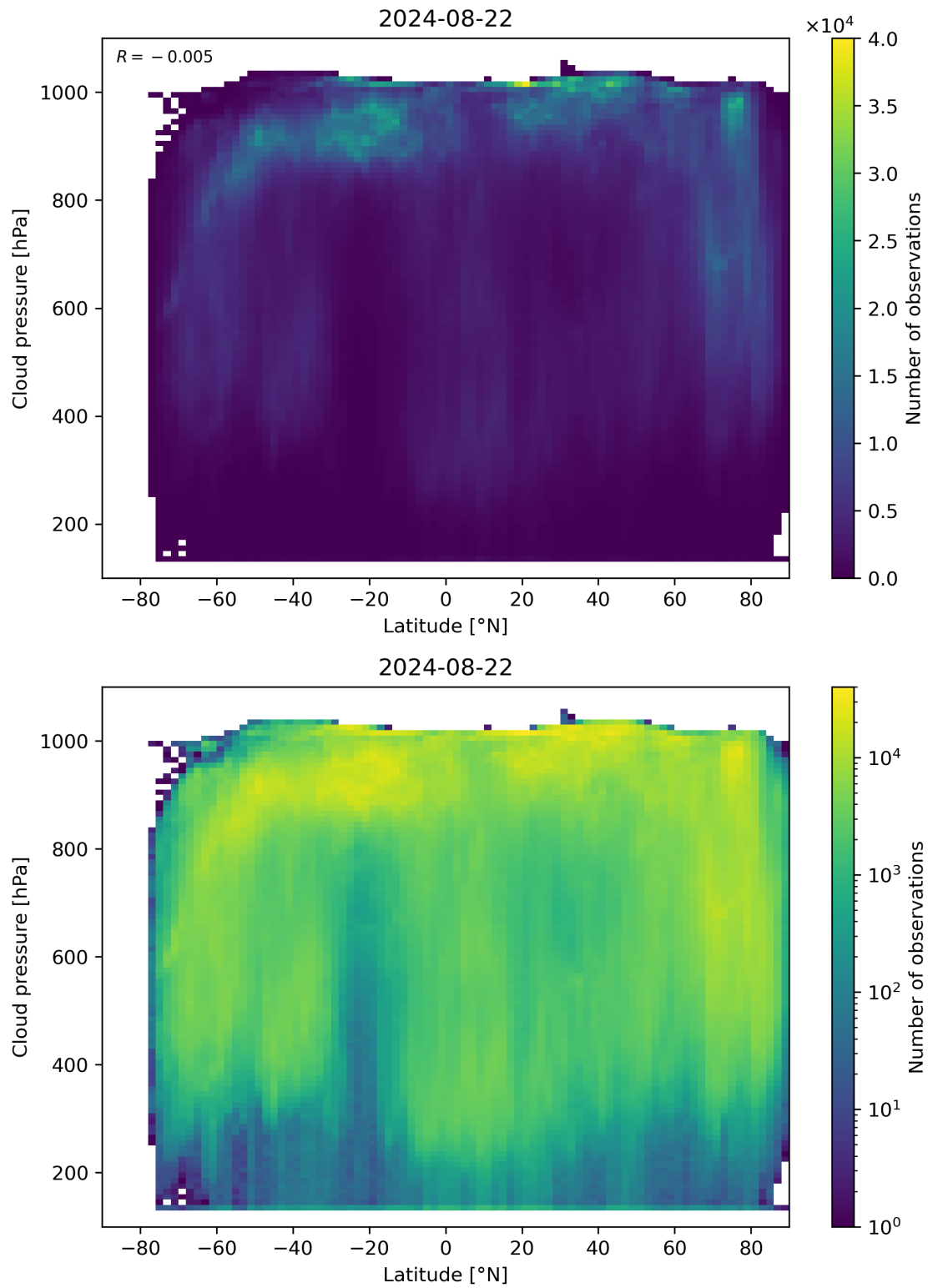
Figure 91: Scatter density plot of “Latitude” against “Cloud pressure” for 2024-08-22 to 2024-08-23.
