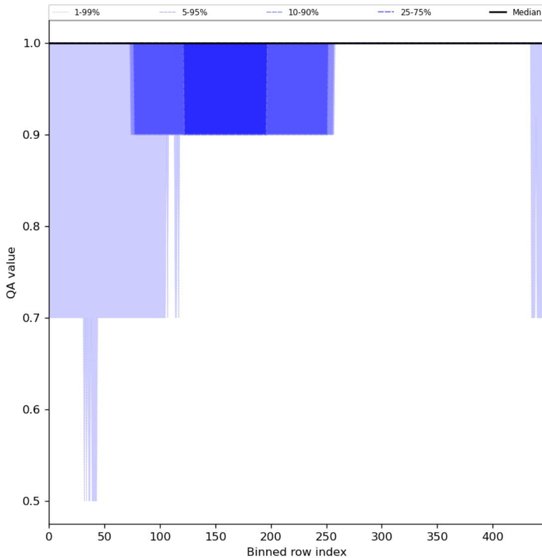
Figure 46: Along track statistics of “QA value” for 2024-08-22 to 2024-08-23
