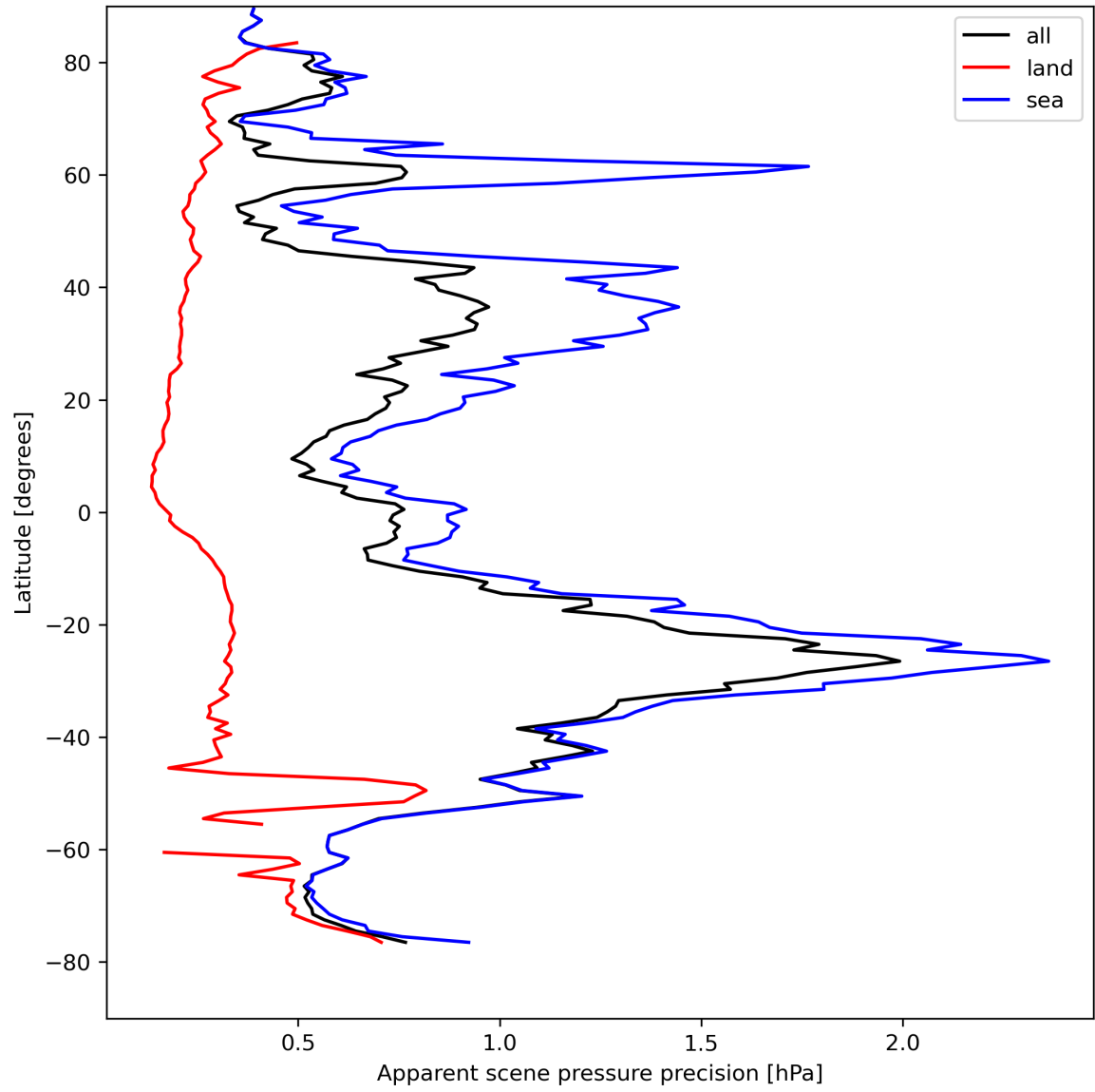
Figure 20: Zonal average of “Apparent scene pressure precision” for 2024-08-22 to 2024-08-23.
