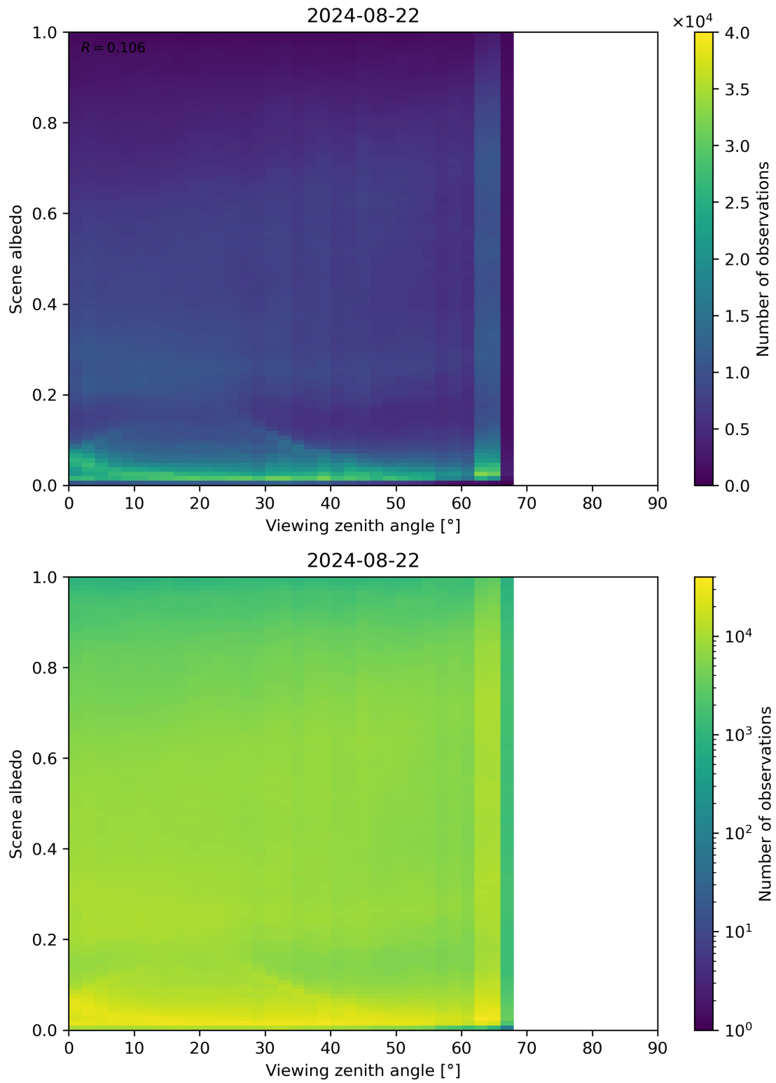
Figure 126: Scatter density plot of “Viewing zenith angle” against “Scene albedo” for 2024-08-22 to 2024-08-23.
