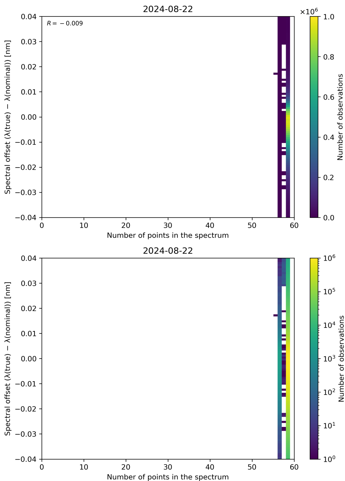
Figure 101: Scatter density plot of “Number of points in the spectrum” against “Spectral offset ( \lambda(\text{true}) - \lambda(\text{nominal}) )” for 2024-08-22 to 2024-08-23.
