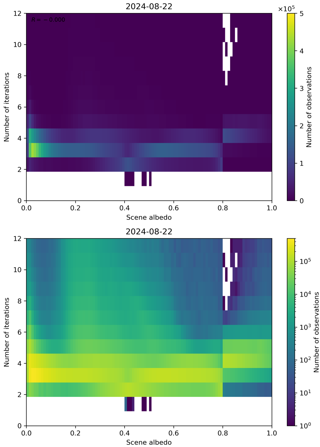
Figure 105: Scatter density plot of “Scene albedo” against “Number of iterations” for 2024-08-22 to 2024-08-23.
