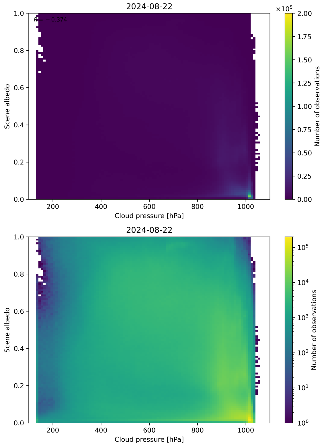
Figure 83: Scatter density plot of “Cloud pressure” against “Scene albedo” for 2024-08-22 to 2024-08-23.
