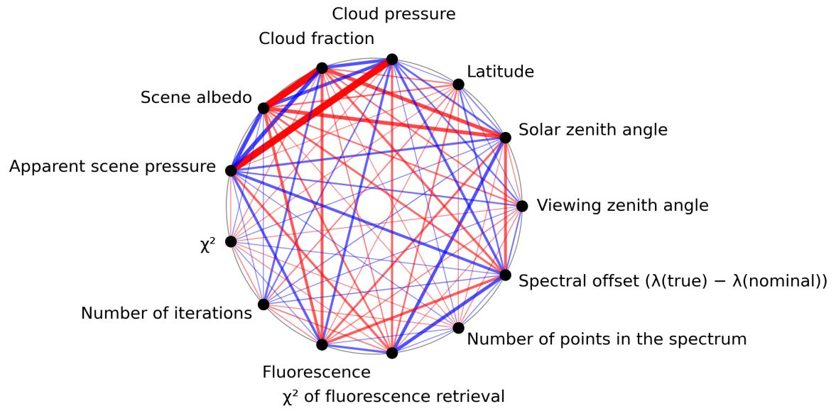
Figure 1: Map of correlation graph for 2024-08-22 to 2024-08-23.
