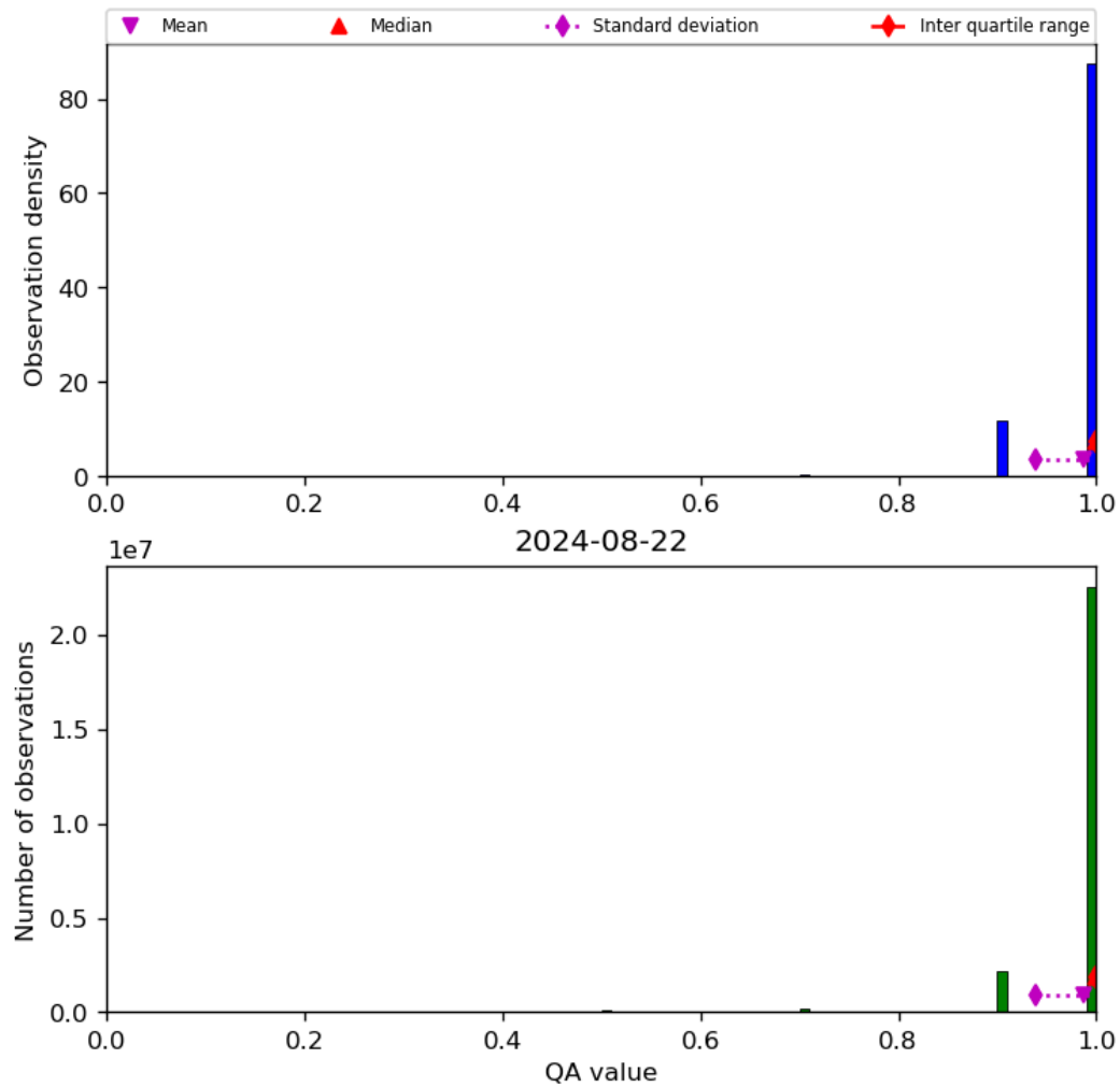
Figure 29: Histogram of “QA value” for 2024-08-22 to 2024-08-23
