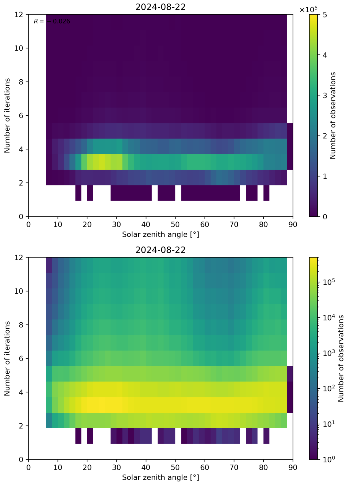
Figure 114: Scatter density plot of “Solar zenith angle” against “Number of iterations” for 2024-08-22 to 2024-08-23.
