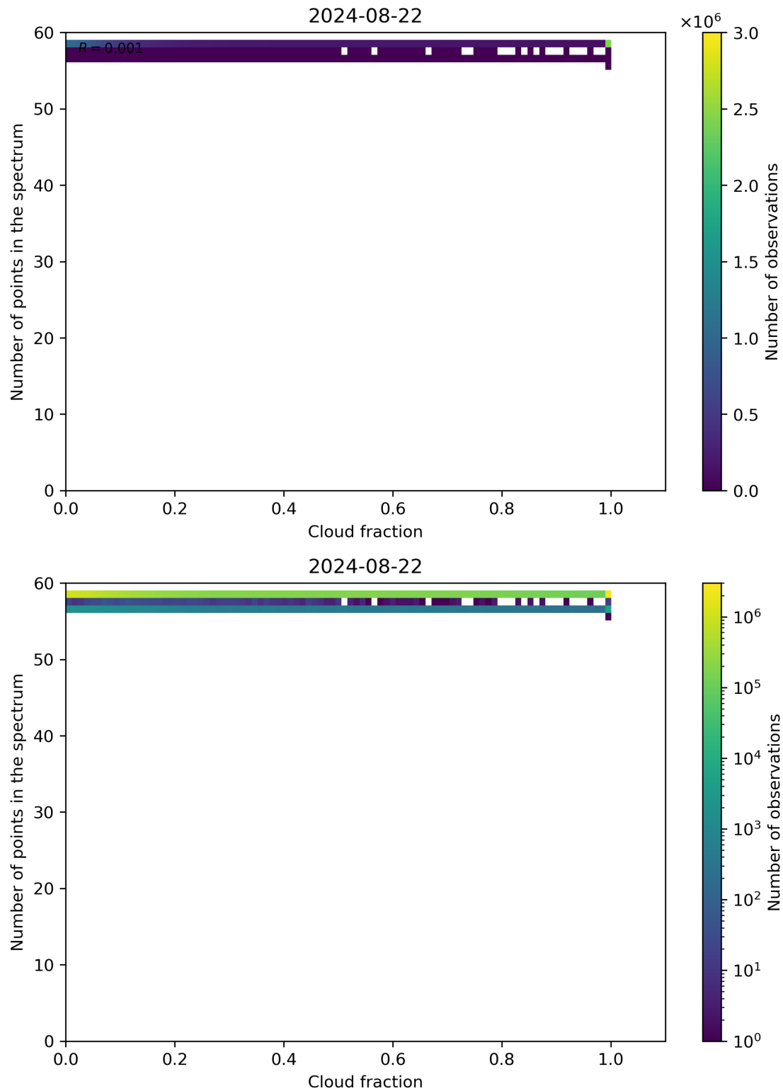
Figure 74: Scatter density plot of “Cloud fraction” against “Number of points in the spectrum” for 2024-08-22 to 2024-08-23.
