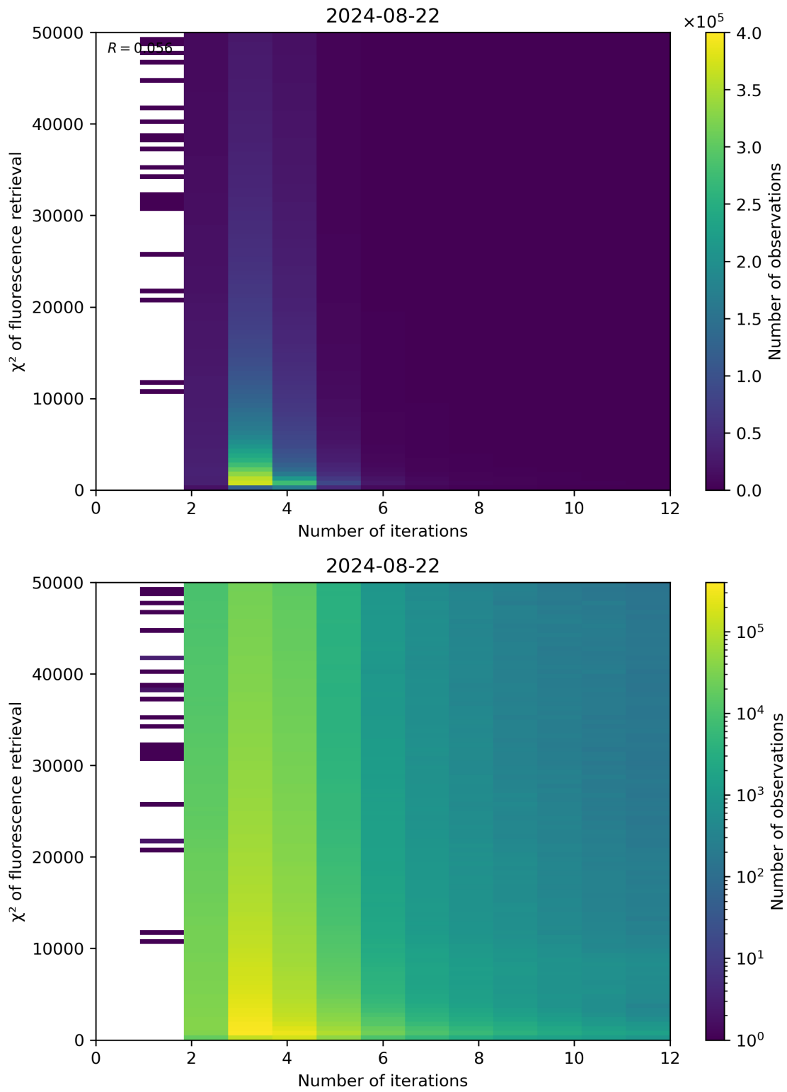
Figure 97: Scatter density plot of “Number of iterations” against “ \chi^2 of fluorescence retrieval” for 2024-08-22 to 2024-08-23.
