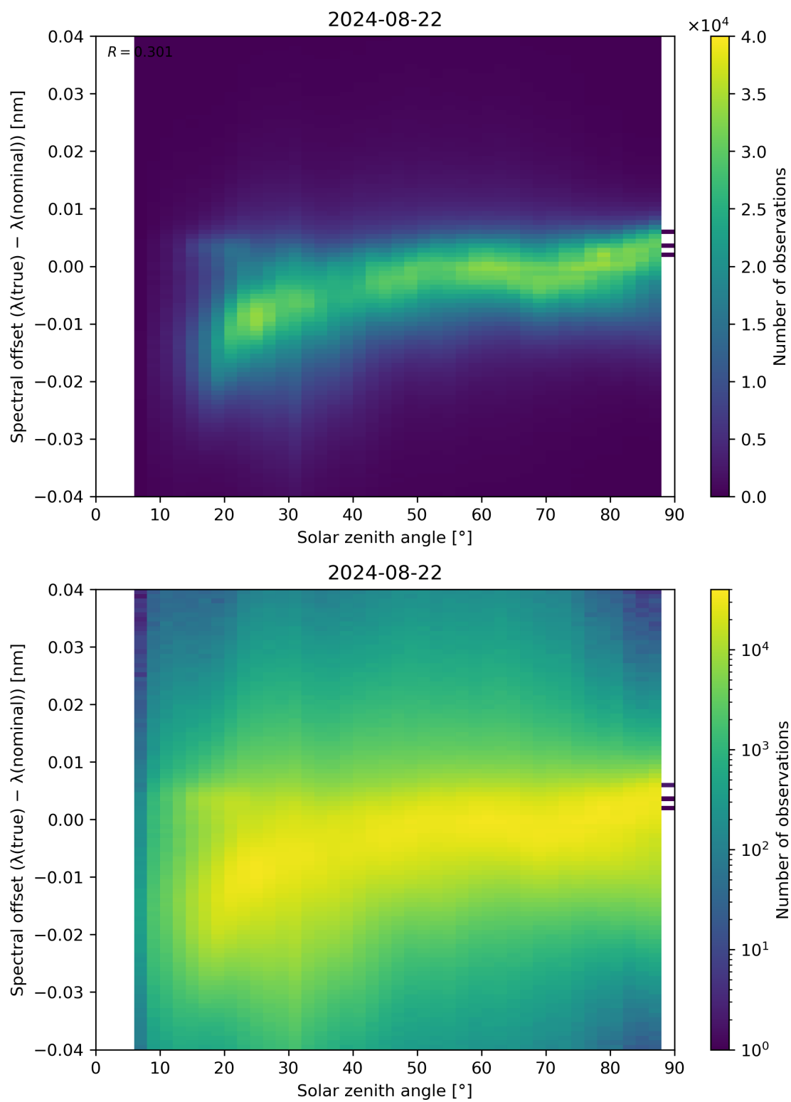
Figure 117: Scatter density plot of “Solar zenith angle” against “Spectral offset ( \lambda(\text{true}) - \lambda(\text{nominal}) )” for 2024-08-22 to 2024-08-23.
