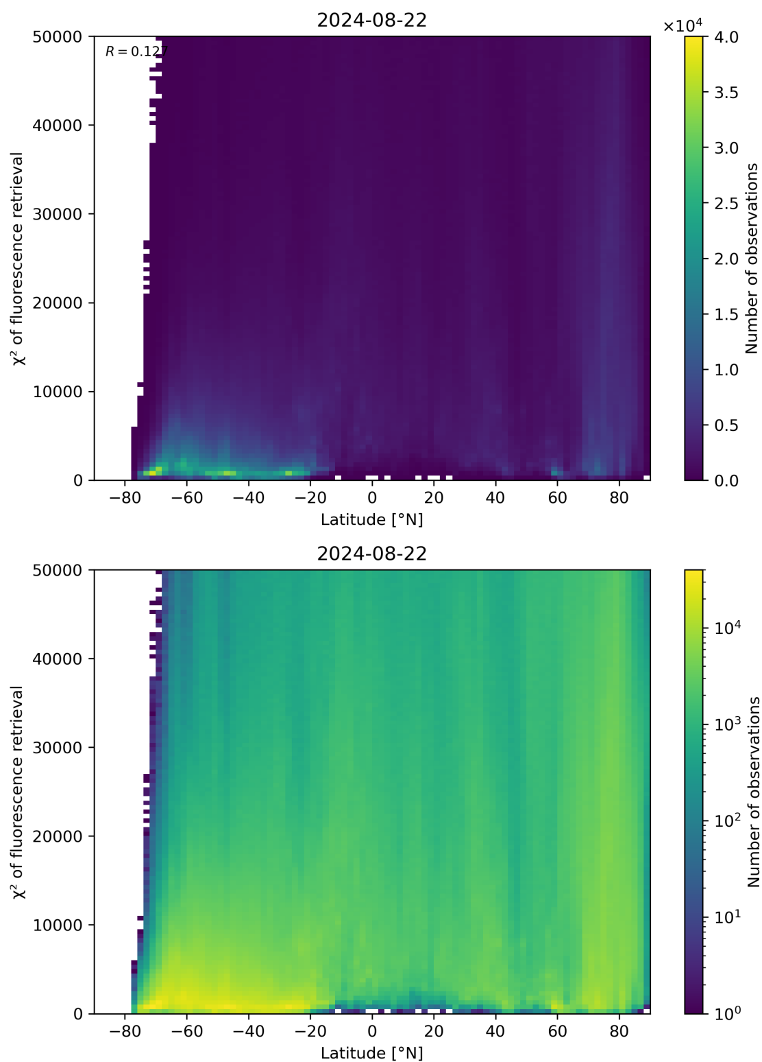
Figure 89: Scatter density plot of “Latitude” against “ \chi^2 of fluorescence retrieval” for 2024-08-22 to 2024-08-23.
