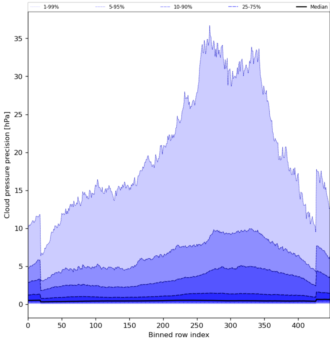
Figure 48: Along track statistics of “Cloud pressure precision” for 2024-08-22 to 2024-08-23
