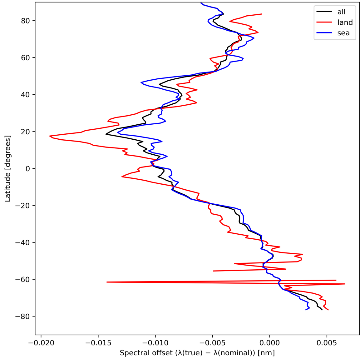
Figure 28: Zonal average of “Spectral offset ( \lambda(\text{true}) - \lambda(\text{nominal}) )” for 2024-08-22 to 2024-08-23.
