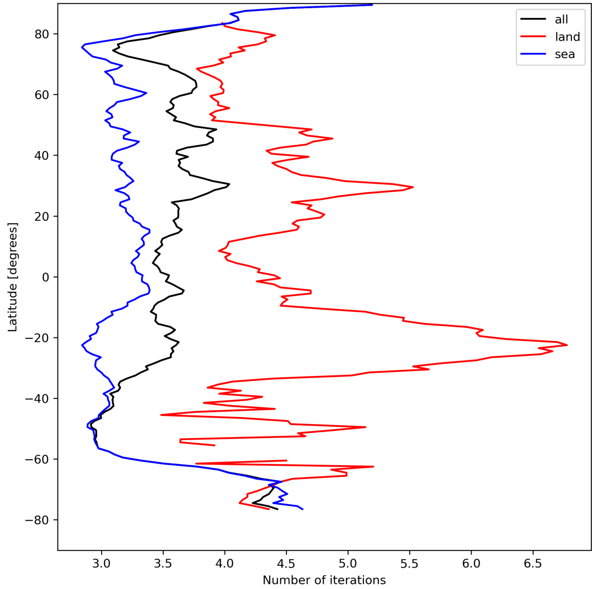
Figure 22: Zonal average of “Number of iterations” for 2024-08-22 to 2024-08-23.
