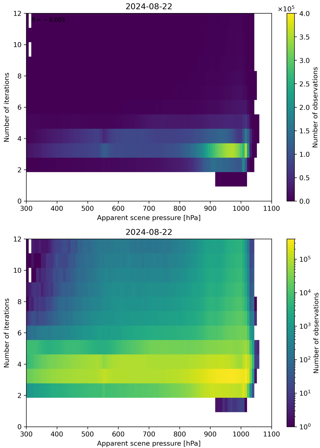
Figure 65: Scatter density plot of “Apparent scene pressure” against “Number of iterations” for 2024-08-22 to 2024-08-23.
