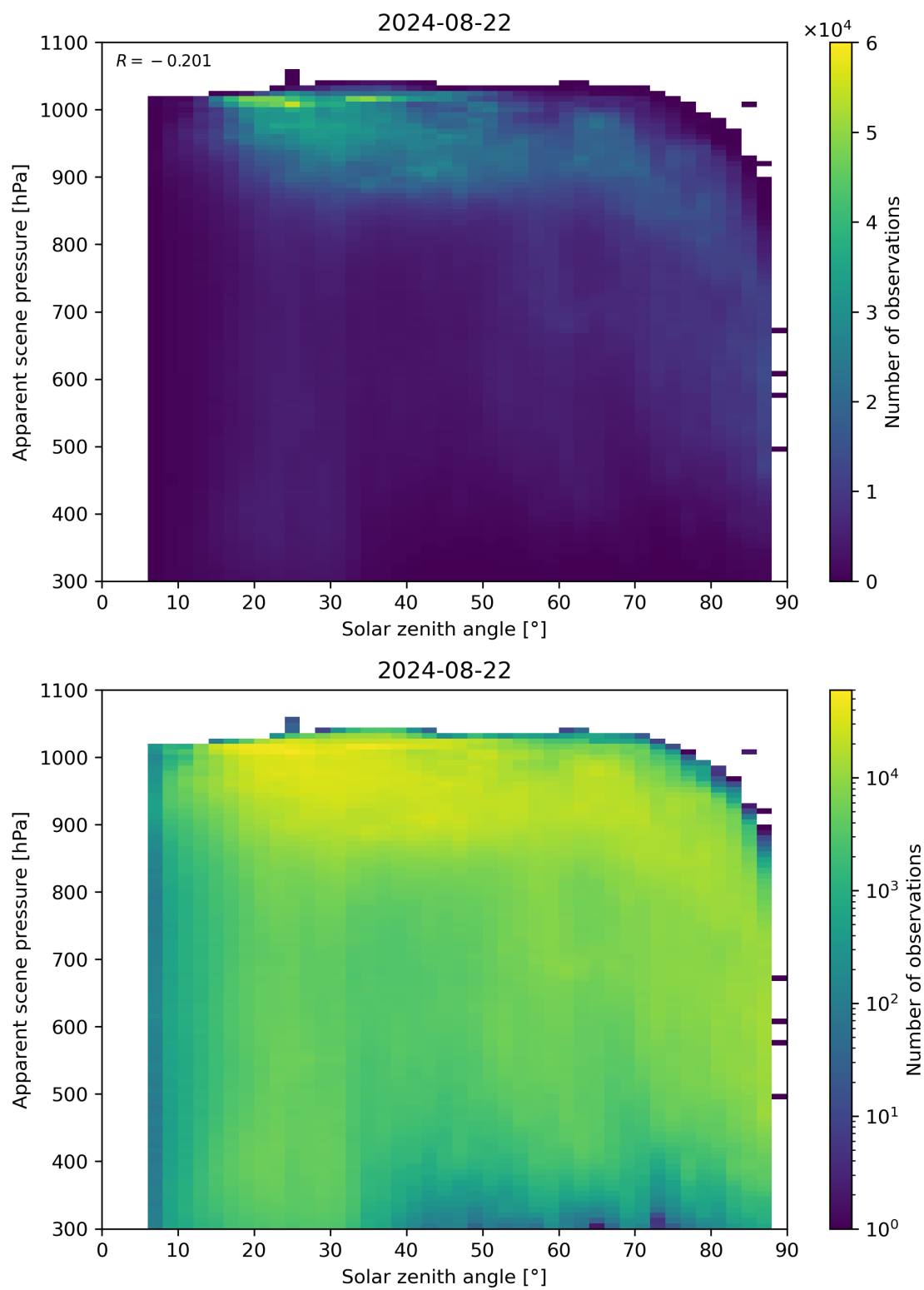
Figure 108: Scatter density plot of “Solar zenith angle” against “Apparent scene pressure” for 2024-08-22 to 2024-08-23.
