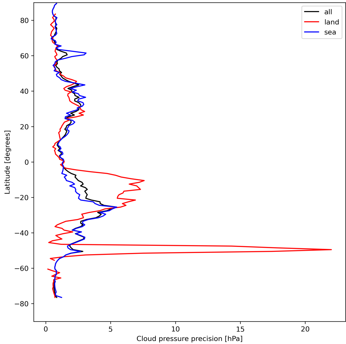
Figure 14: Zonal average of “Cloud pressure precision” for 2024-08-22 to 2024-08-23.
