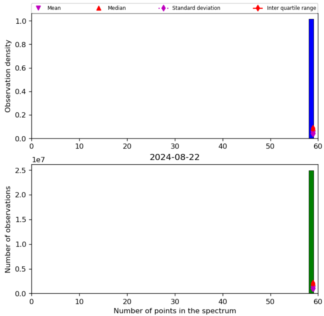
Figure 44: Histogram of “Number of points in the spectrum” for 2024-08-22 to 2024-08-23
