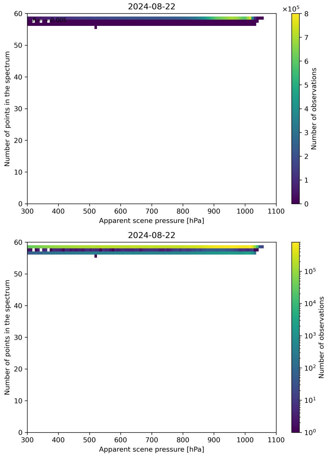
Figure 66: Scatter density plot of “Apparent scene pressure” against “Number of points in the spectrum” for 2024-08-22 to 2024-08-23.
