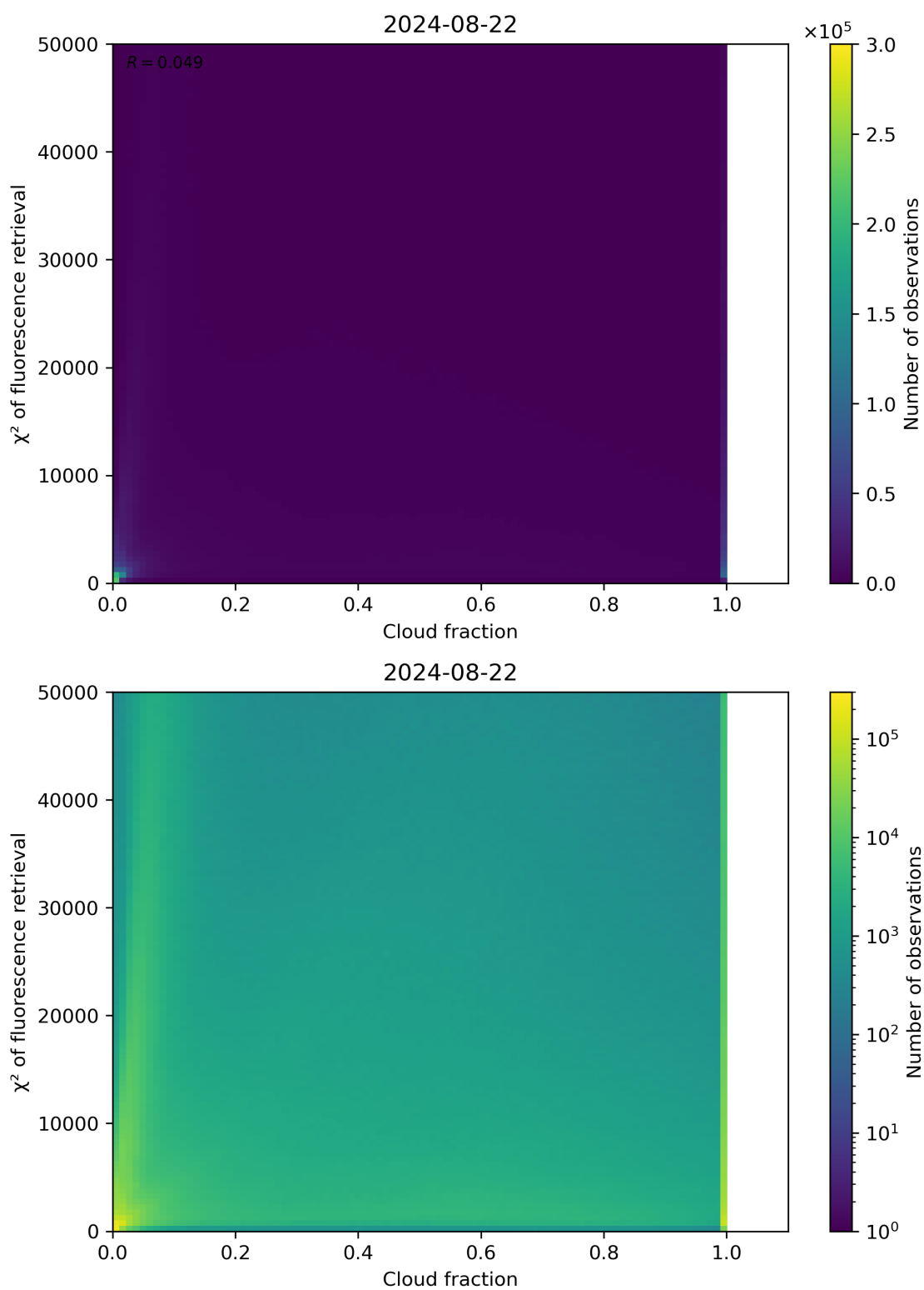
Figure 71: Scatter density plot of “Cloud fraction” against “ \chi^2 of fluorescence retrieval” for 2024-08-22 to 2024-08-23.
