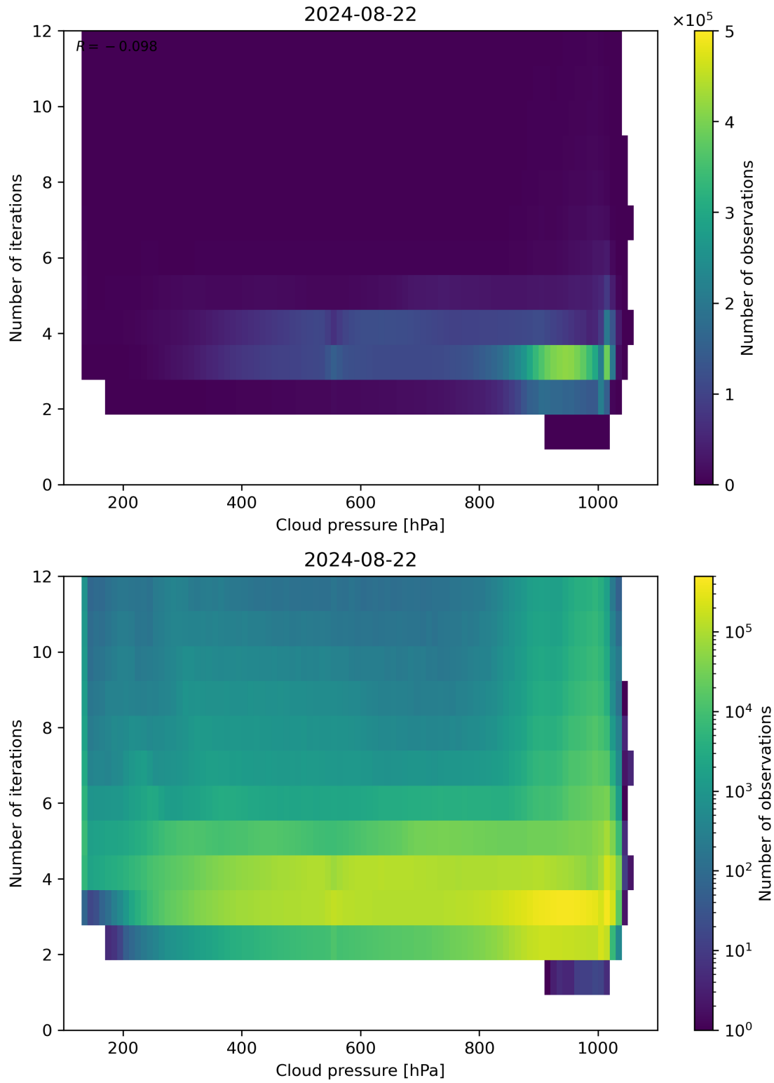
Figure 81: Scatter density plot of “Cloud pressure” against “Number of iterations” for 2024-08-22 to 2024-08-23.
