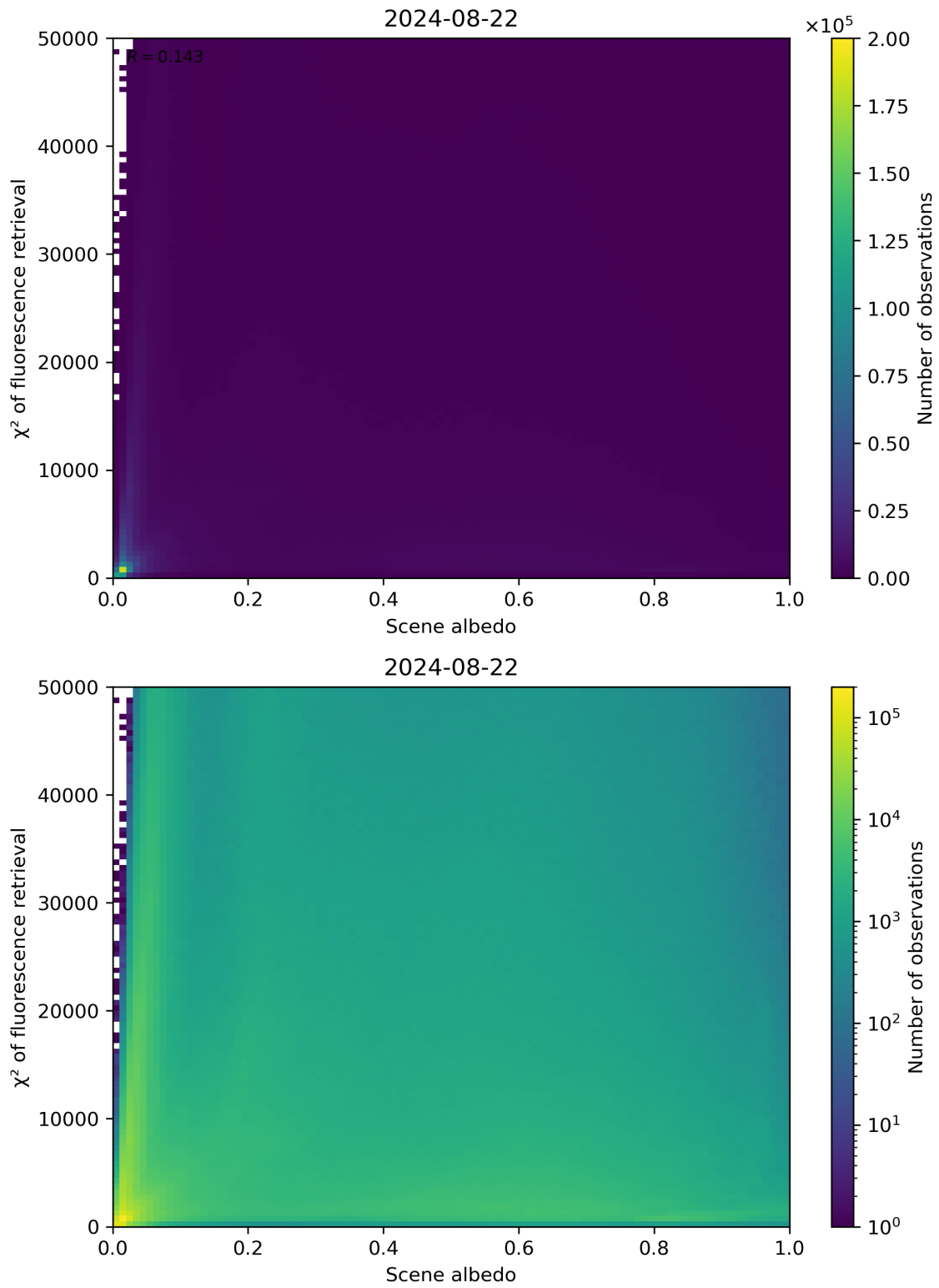
Figure 103: Scatter density plot of “Scene albedo” against “ \chi^2 of fluorescence retrieval” for 2024-08-22 to 2024-08-23.
