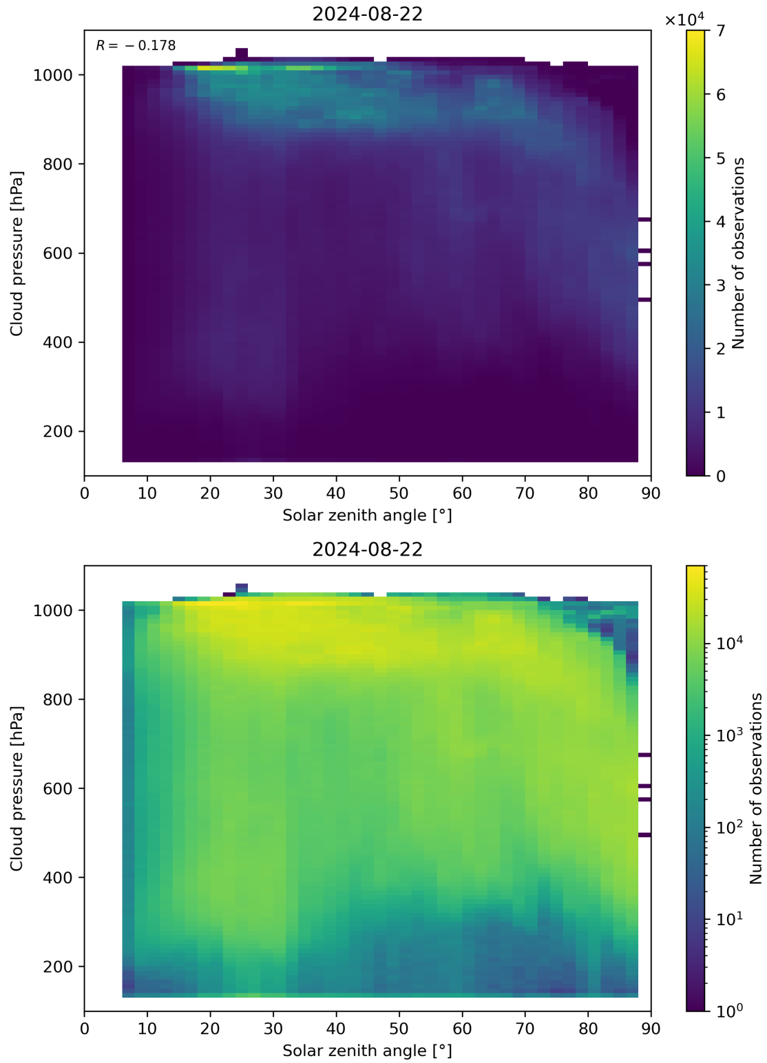
Figure 111: Scatter density plot of “Solar zenith angle” against “Cloud pressure” for 2024-08-22 to 2024-08-23.
