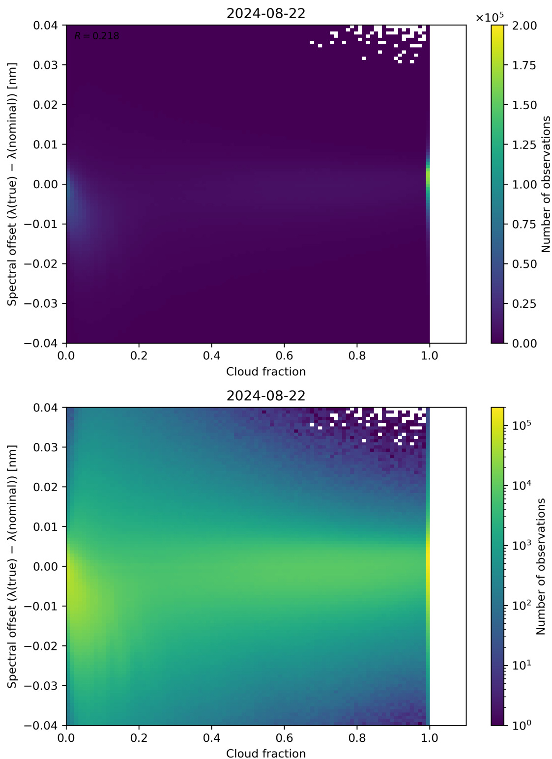
Figure 76: Scatter density plot of “Cloud fraction” against “Spectral offset ( \lambda(\text{true}) - \lambda(\text{nominal}) )” for 2024-08-22 to 2024-08-23.
