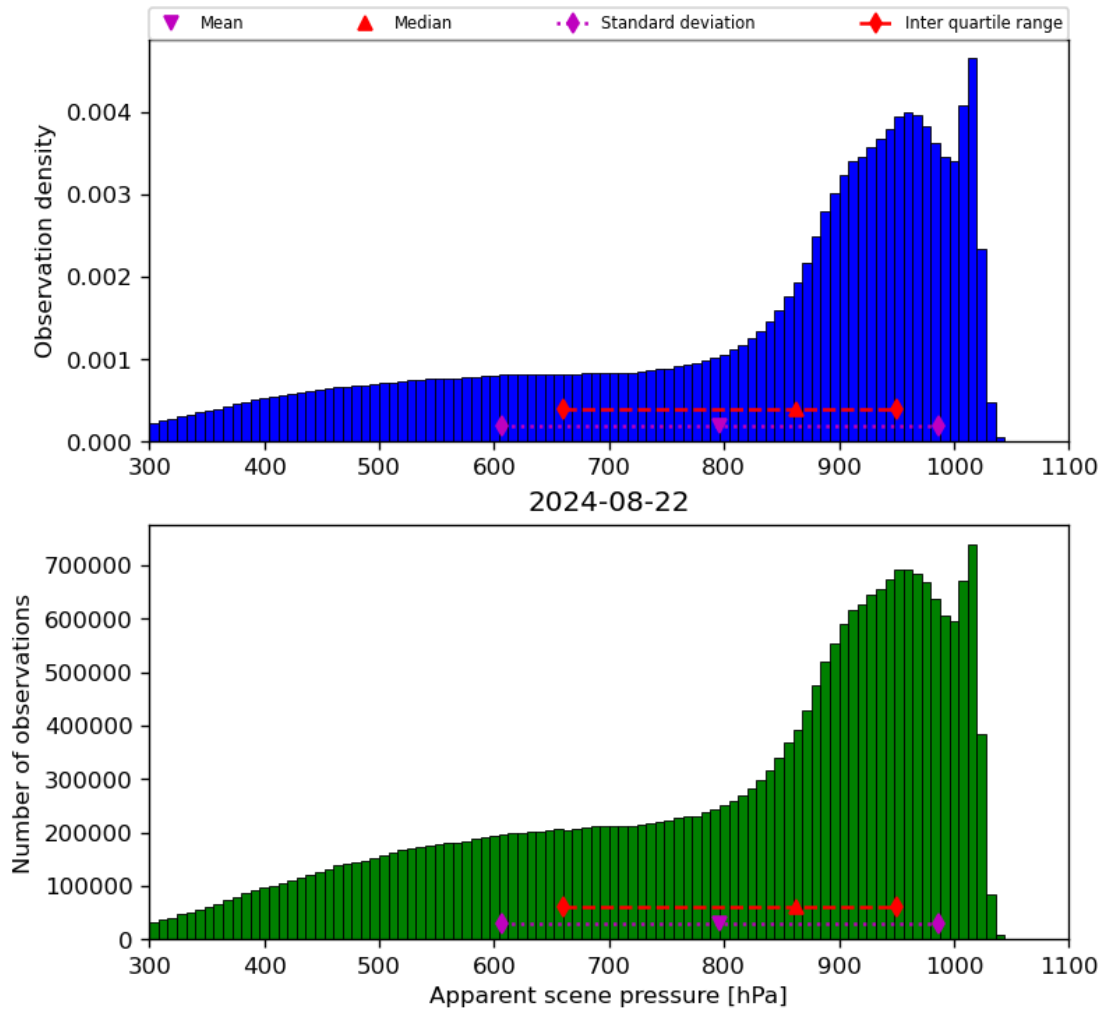
Figure 36: Histogram of “Apparent scene pressure” for 2024-08-22 to 2024-08-23
