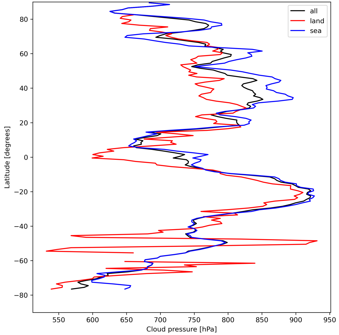
Figure 13: Zonal average of “Cloud pressure” for 2024-08-22 to 2024-08-23.
