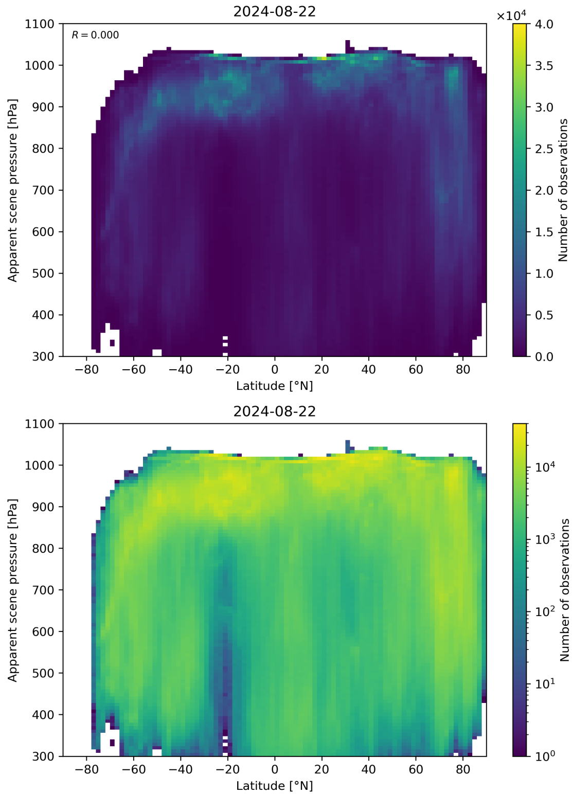
Figure 88: Scatter density plot of “Latitude” against “Apparent scene pressure” for 2024-08-22 to 2024-08-23.
