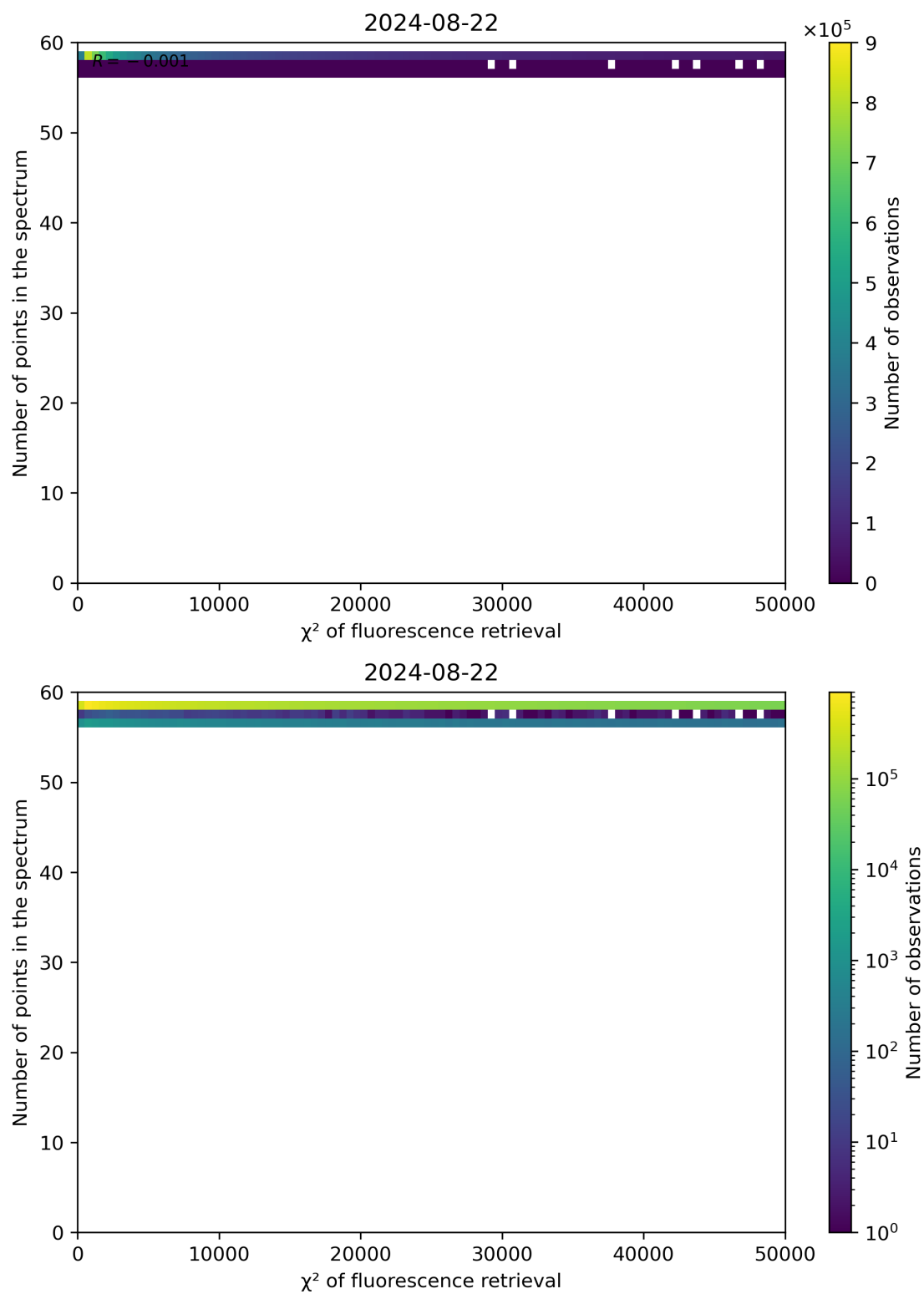
Figure 68: Scatter density plot of " \chi^2 of fluorescence retrieval" against "Number of points in the spectrum" for 2024-08-22 to 2024-08-23.
