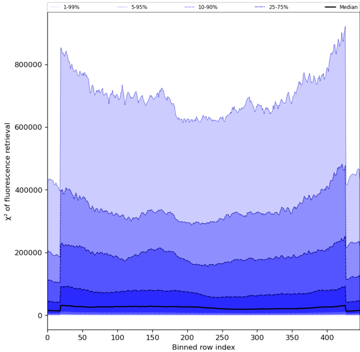
Figure 59: Along track statistics of “ \chi^2 of fluorescence retrieval” for 2024-08-22 to 2024-08-23
