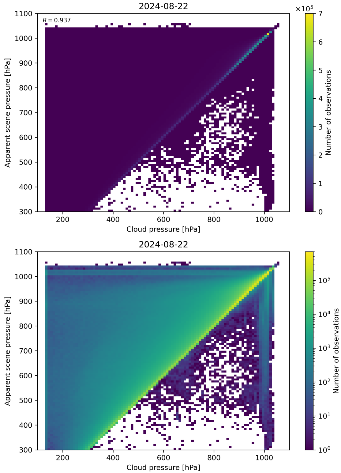
Figure 77: Scatter density plot of “Cloud pressure” against “Apparent scene pressure” for 2024-08-22 to 2024-08-23.
