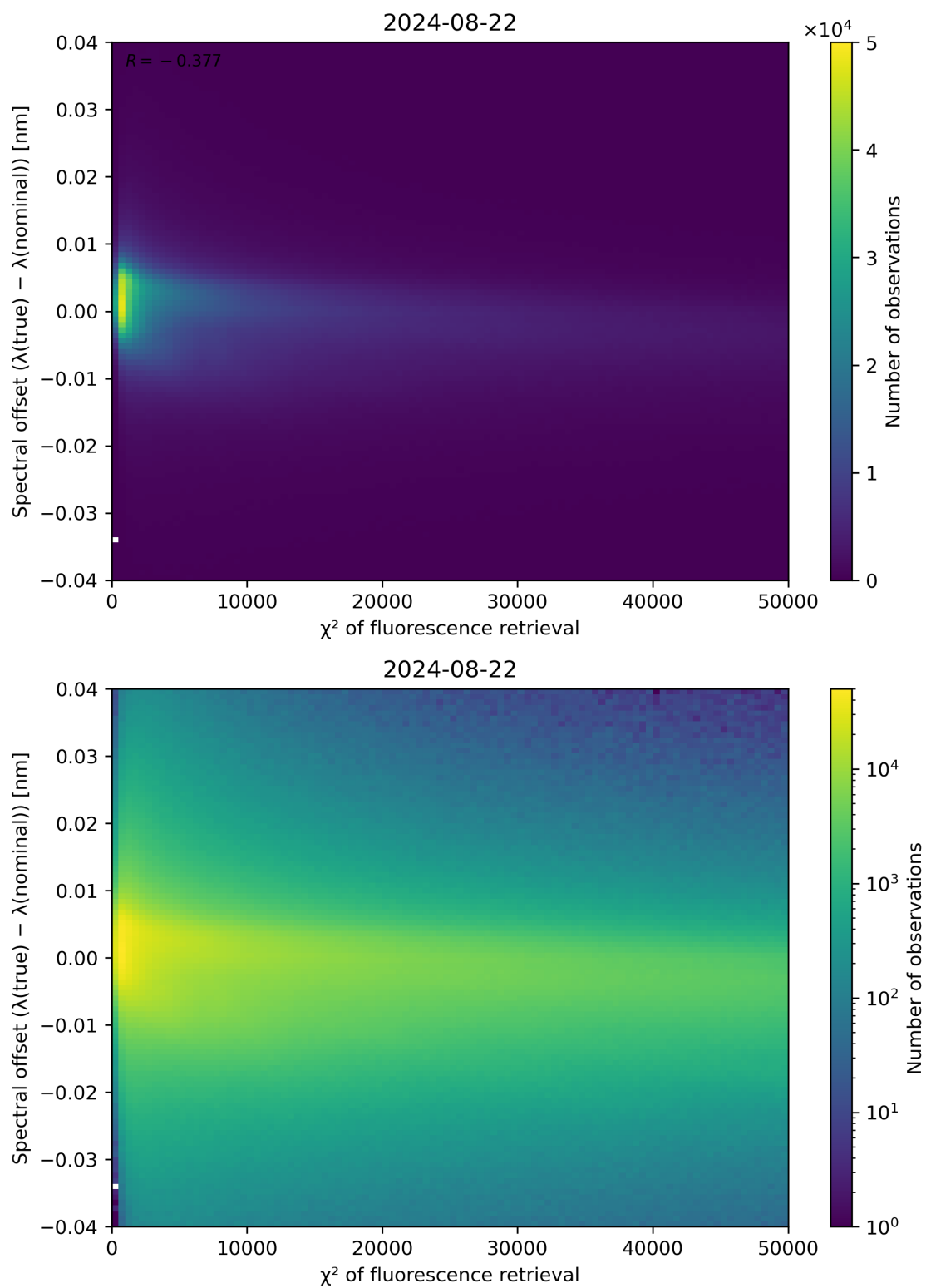
Figure 69: Scatter density plot of “ \chi^2 of fluorescence retrieval” against “Spectral offset ( \lambda(\text{true}) - \lambda(\text{nominal}) )” for 2024-08-22 to 2024-08-23.
