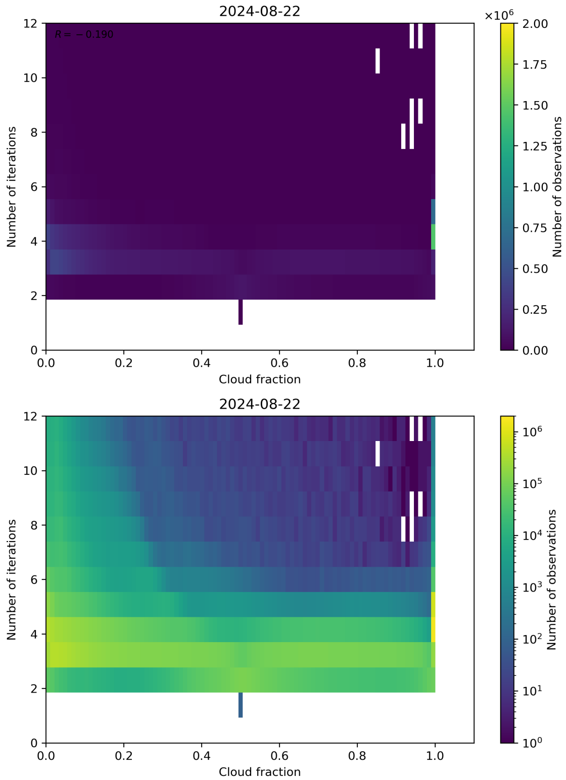
Figure 73: Scatter density plot of “Cloud fraction” against “Number of iterations” for 2024-08-22 to 2024-08-23.
