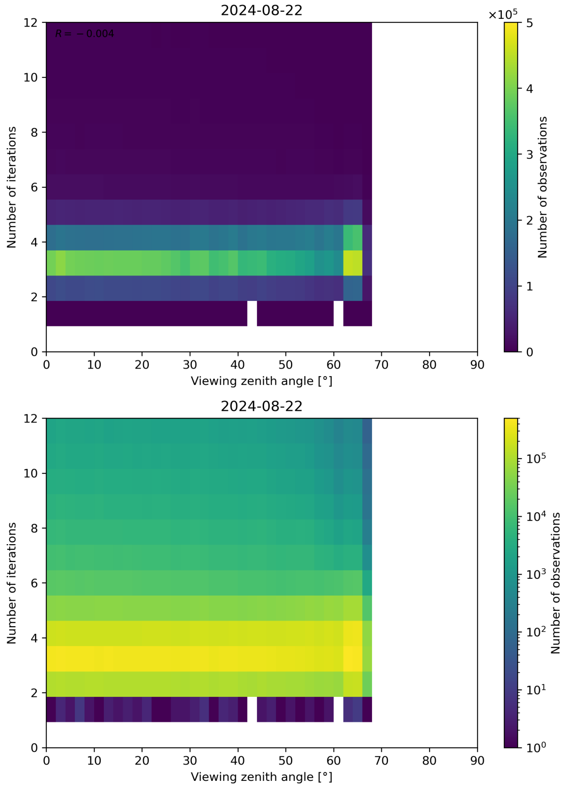
Figure 124: Scatter density plot of “Viewing zenith angle” against “Number of iterations” for 2024-08-22 to 2024-08-23.
