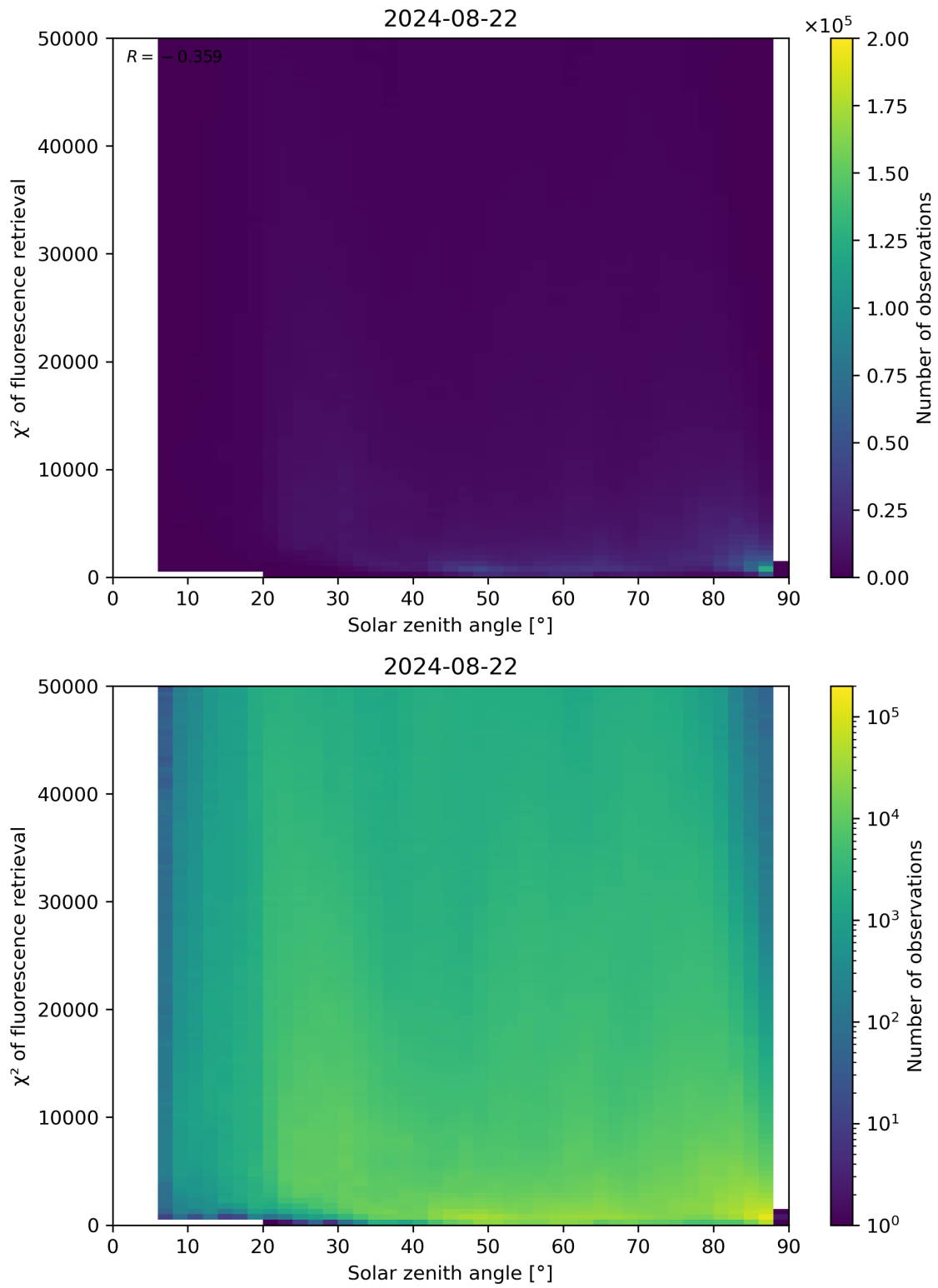
Figure 109: Scatter density plot of “Solar zenith angle” against “ \chi^2 of fluorescence retrieval” for 2024-08-22 to 2024-08-23.
