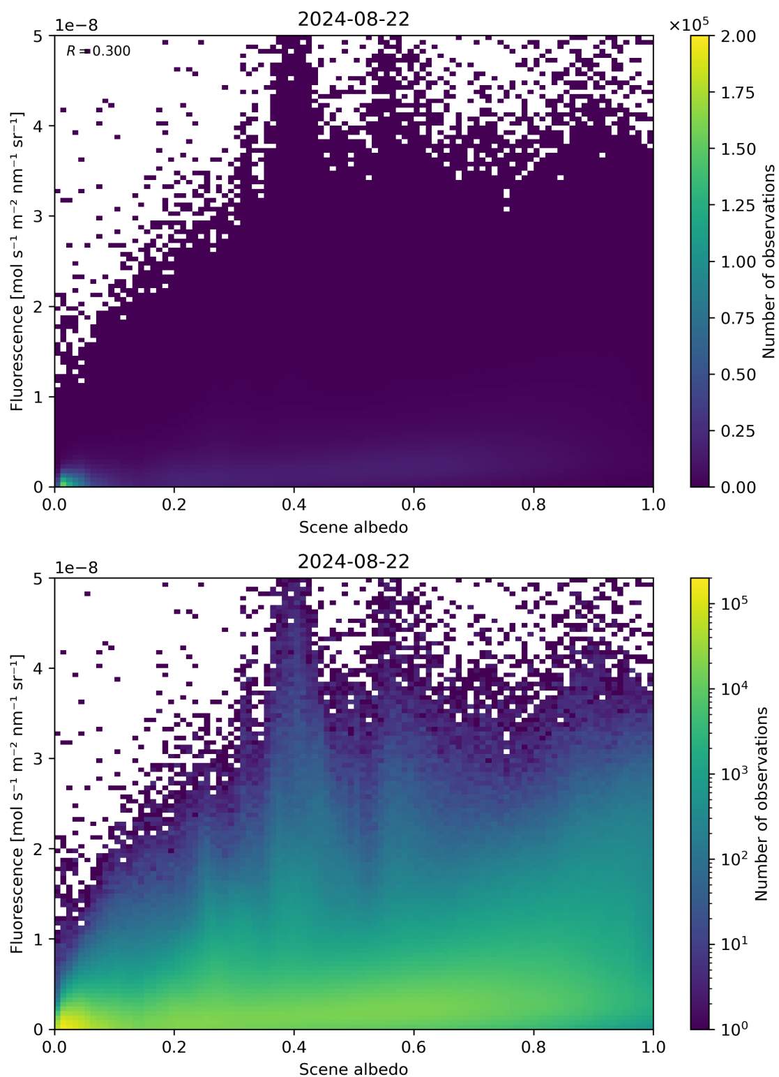
Figure 104: Scatter density plot of “Scene albedo” against “Fluorescence” for 2024-08-22 to 2024-08-23.
