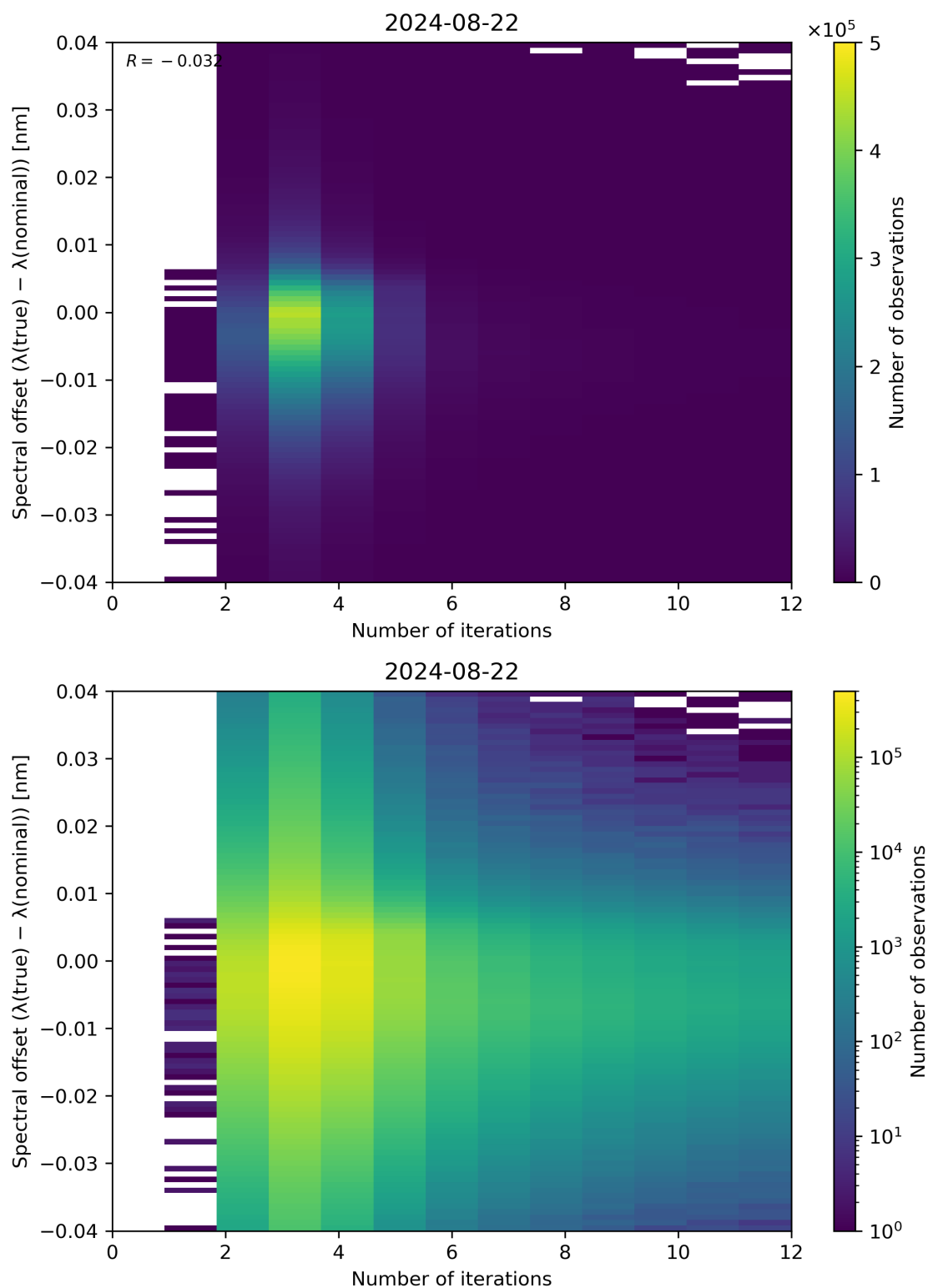
Figure 100: Scatter density plot of “Number of iterations” against “Spectral offset ( \lambda(\text{true}) - \lambda(\text{nominal}) )” for 2024-08-22 to 2024-08-23.
