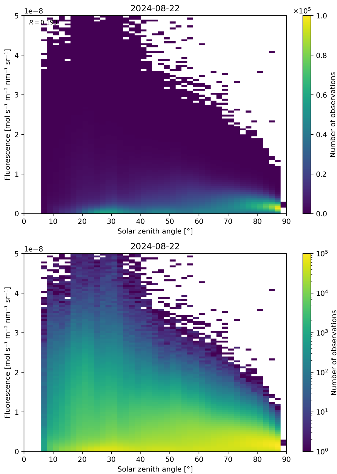
Figure 112: Scatter density plot of “Solar zenith angle” against “Fluorescence” for 2024-08-22 to 2024-08-23.
