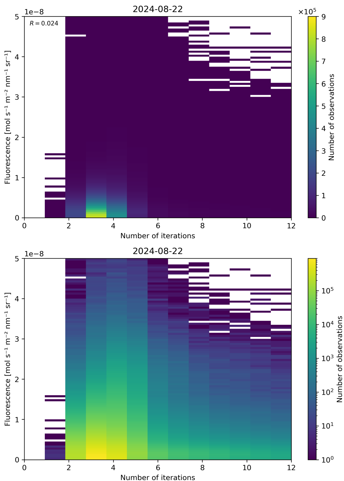
Figure 98: Scatter density plot of “Number of iterations” against “Fluorescence” for 2024-08-22 to 2024-08-23.
