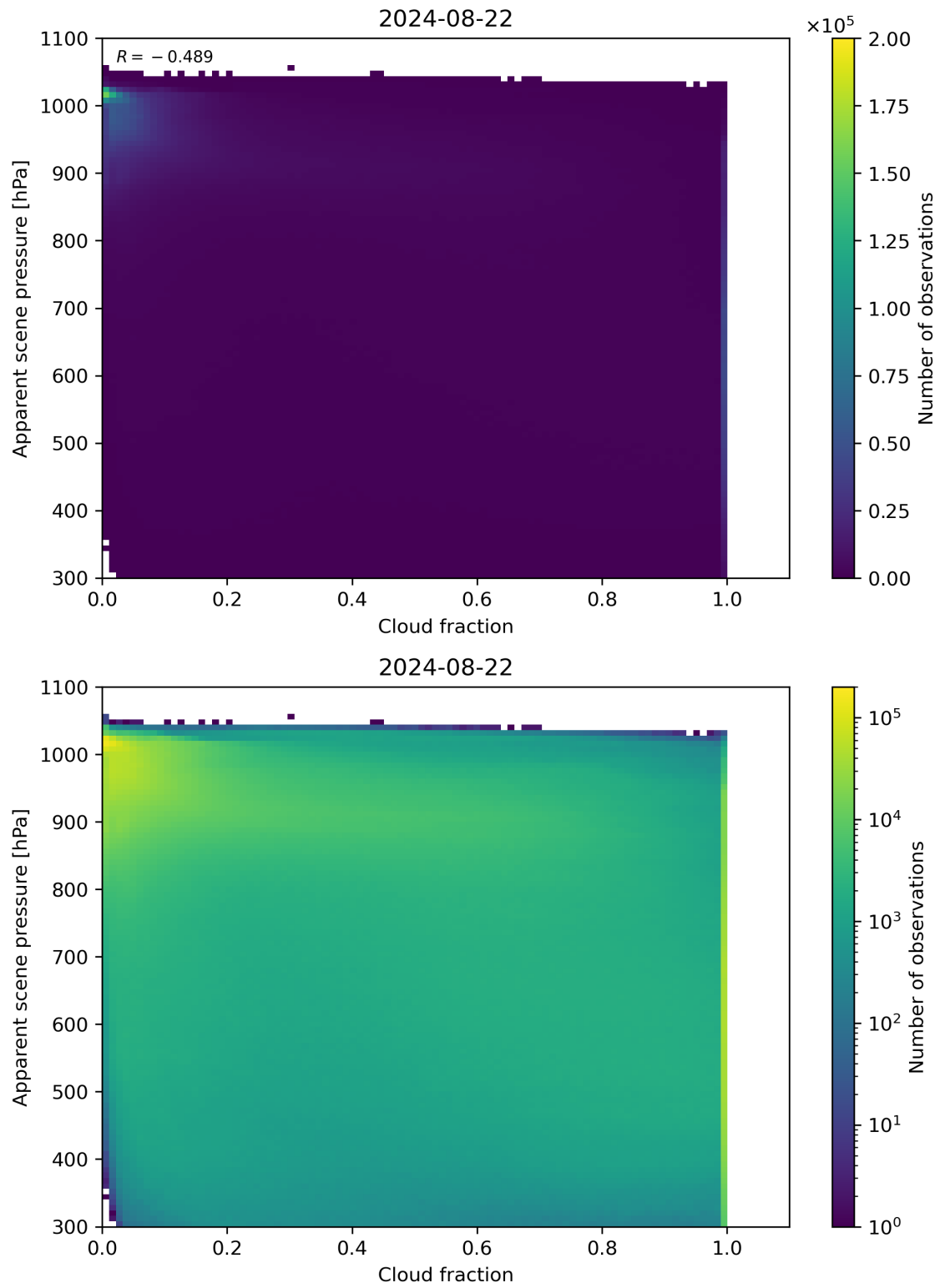
Figure 70: Scatter density plot of “Cloud fraction” against “Apparent scene pressure” for 2024-08-22 to 2024-08-23.
