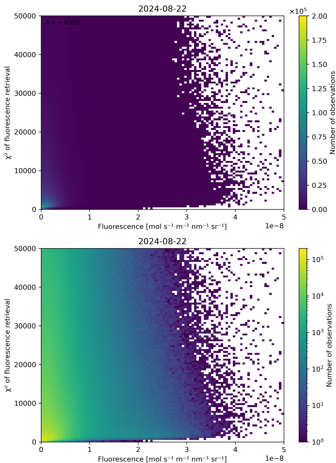
Figure 85: Scatter density plot of “Fluorescence” against “ \chi^2 of fluorescence retrieval” for 2024-08-22 to 2024-08-23.
