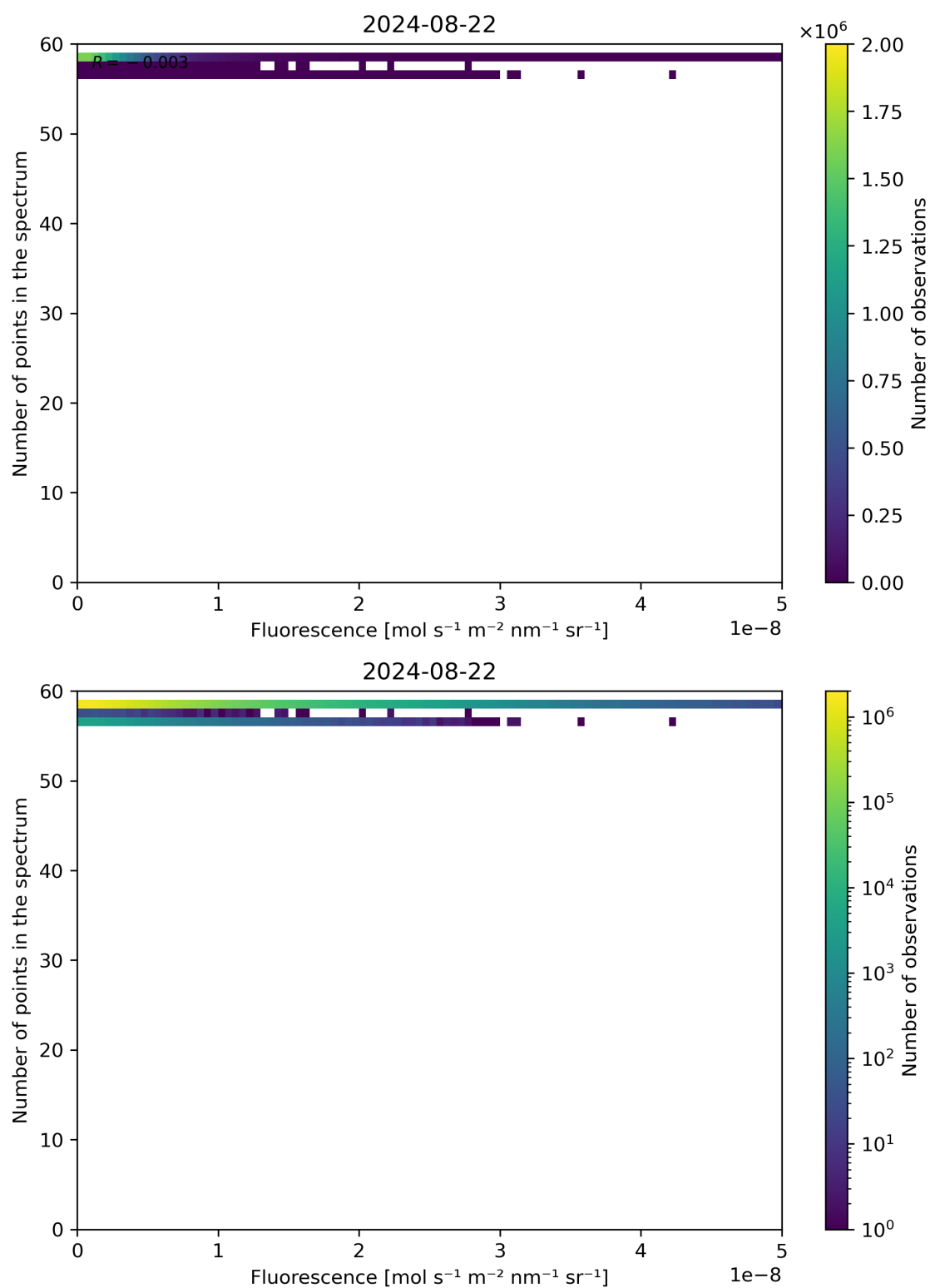
Figure 86: Scatter density plot of “Fluorescence” against “Number of points in the spectrum” for 2024-08-22 to 2024-08-23.
