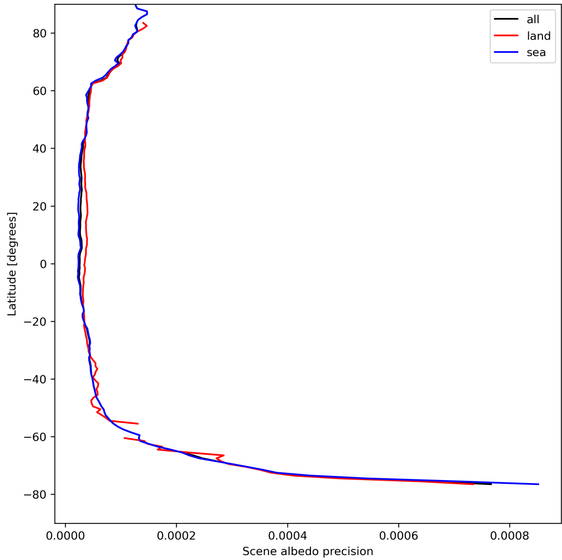
Figure 18: Zonal average of “Scene albedo precision” for 2024-08-22 to 2024-08-23.
