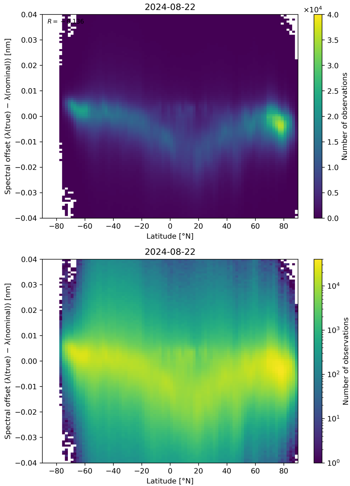
Figure 96: Scatter density plot of “Latitude” against “Spectral offset ( \lambda(\text{true}) - \lambda(\text{nominal}) )” for 2024-08-22 to 2024-08-23.
