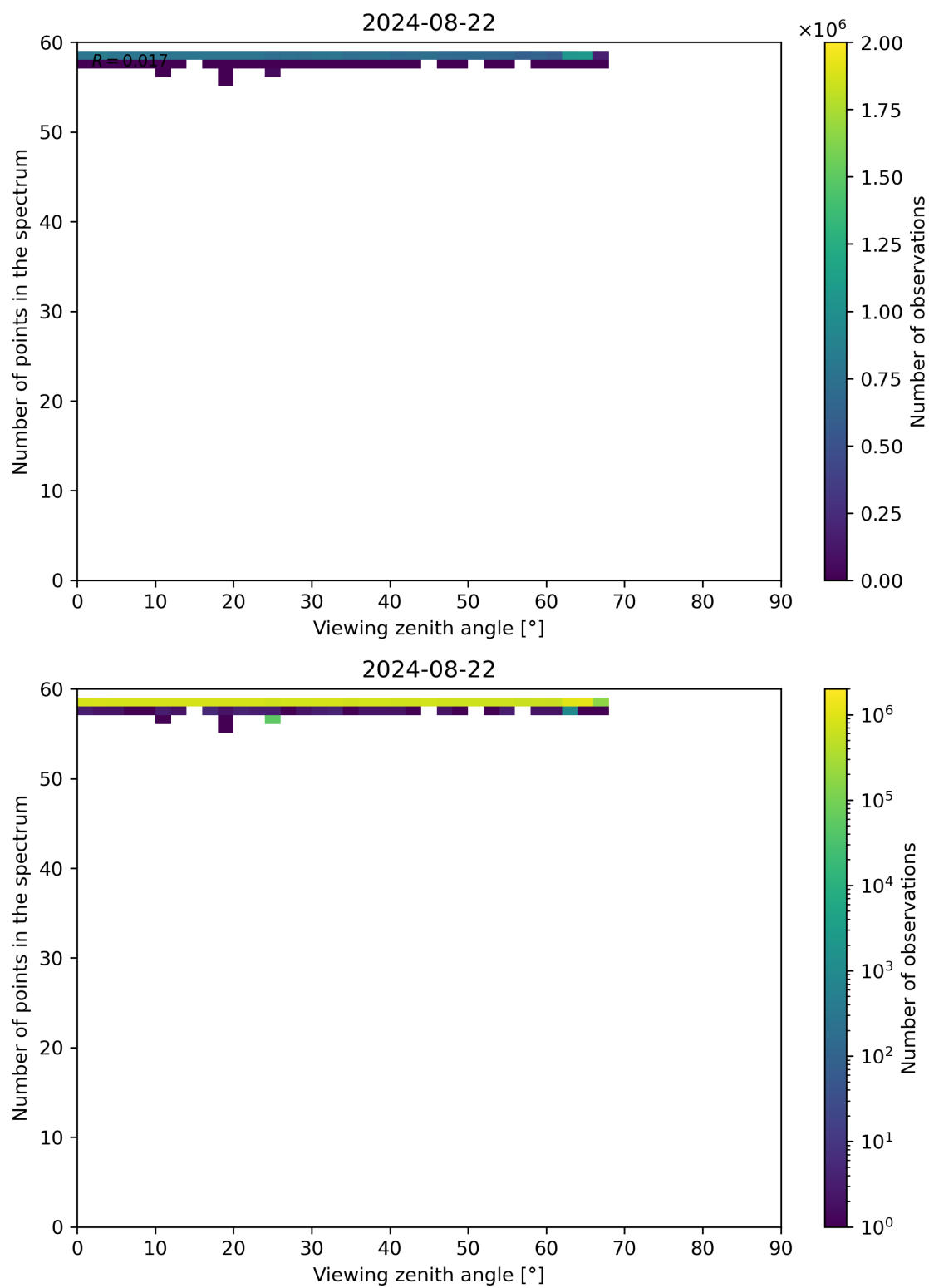
Figure 125: Scatter density plot of “Viewing zenith angle” against “Number of points in the spectrum” for 2024-08-22 to 2024-08-23.
