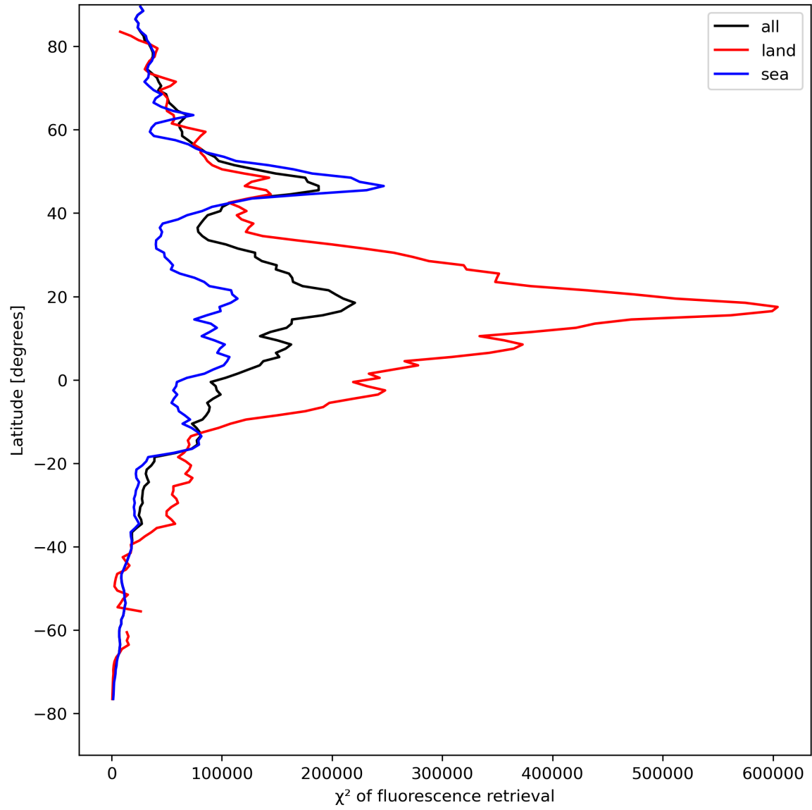
Figure 25: Zonal average of “ \chi^2 of fluorescence retrieval” for 2024-08-22 to 2024-08-23.
