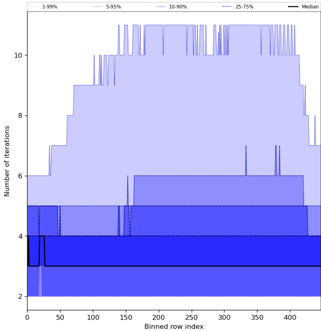
Figure 56: Along track statistics of “Number of iterations” for 2024-08-22 to 2024-08-23
