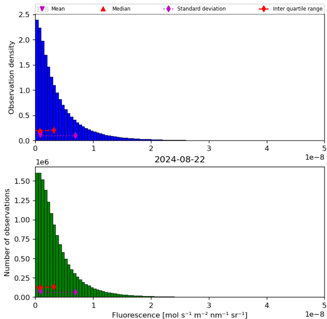
Figure 40: Histogram of “Fluorescence” for 2024-08-22 to 2024-08-23
