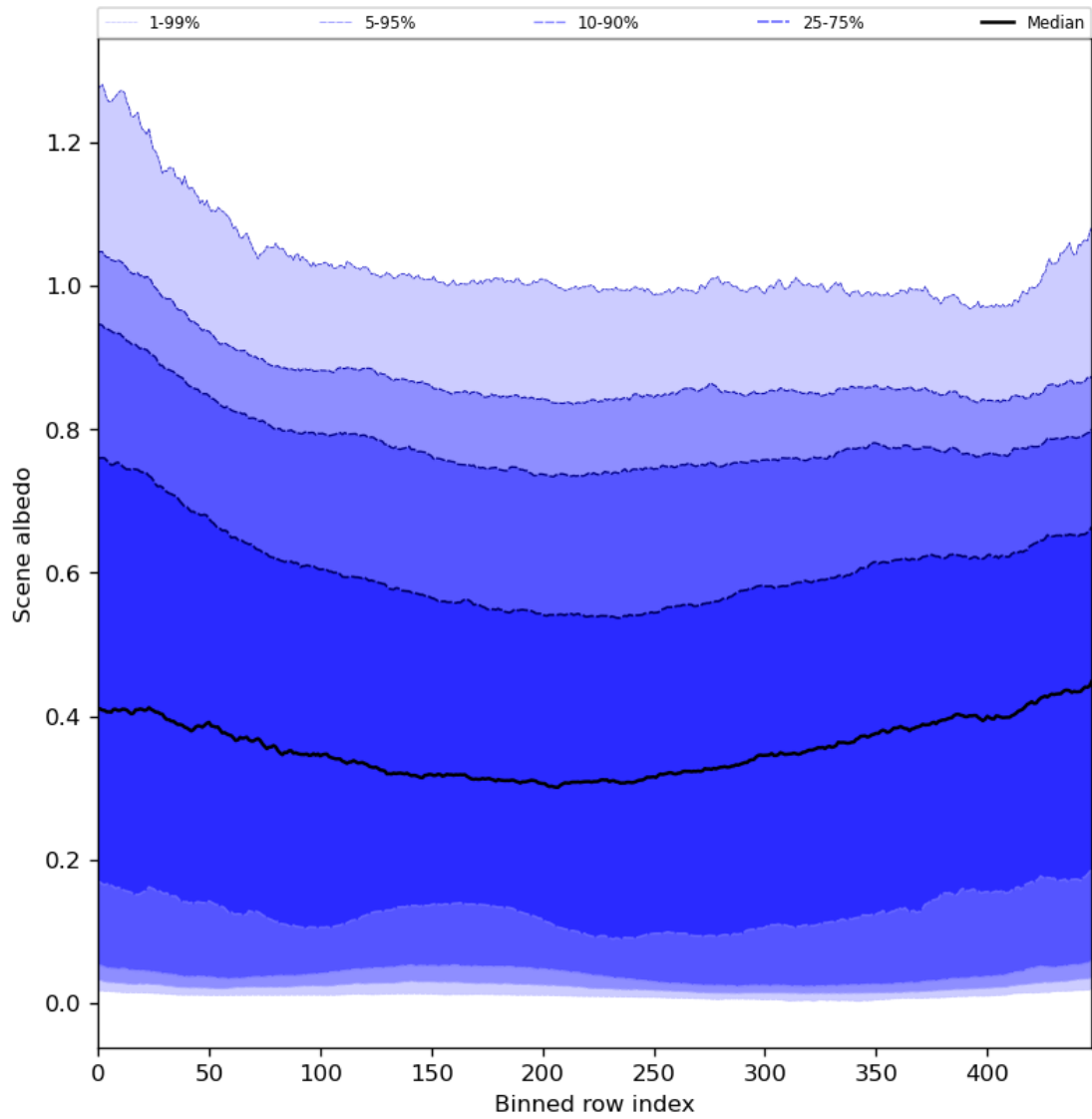
Figure 51: Along track statistics of “Scene albedo” for 2024-08-22 to 2024-08-23
