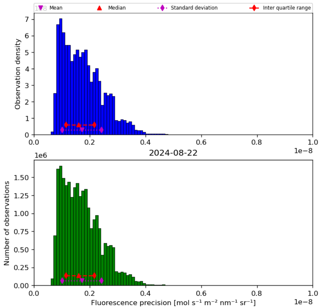
Figure 41: Histogram of “Fluorescence precision” for 2024-08-22 to 2024-08-23
