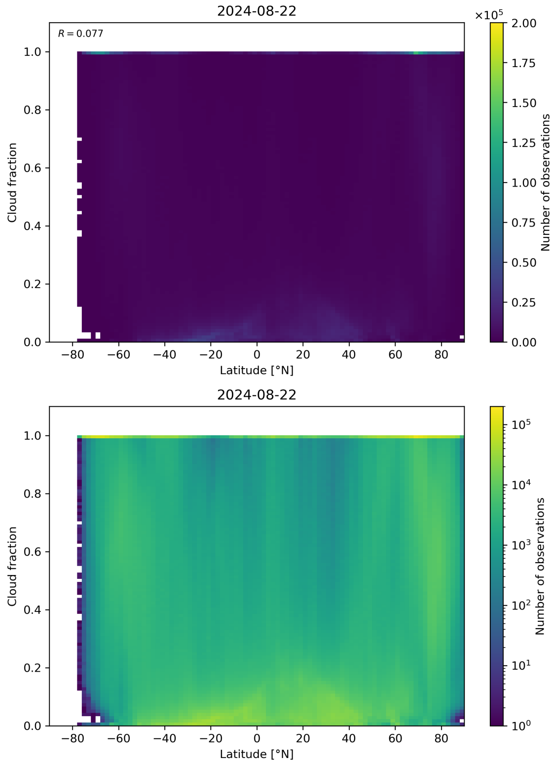
Figure 90: Scatter density plot of “Latitude” against “Cloud fraction” for 2024-08-22 to 2024-08-23.
