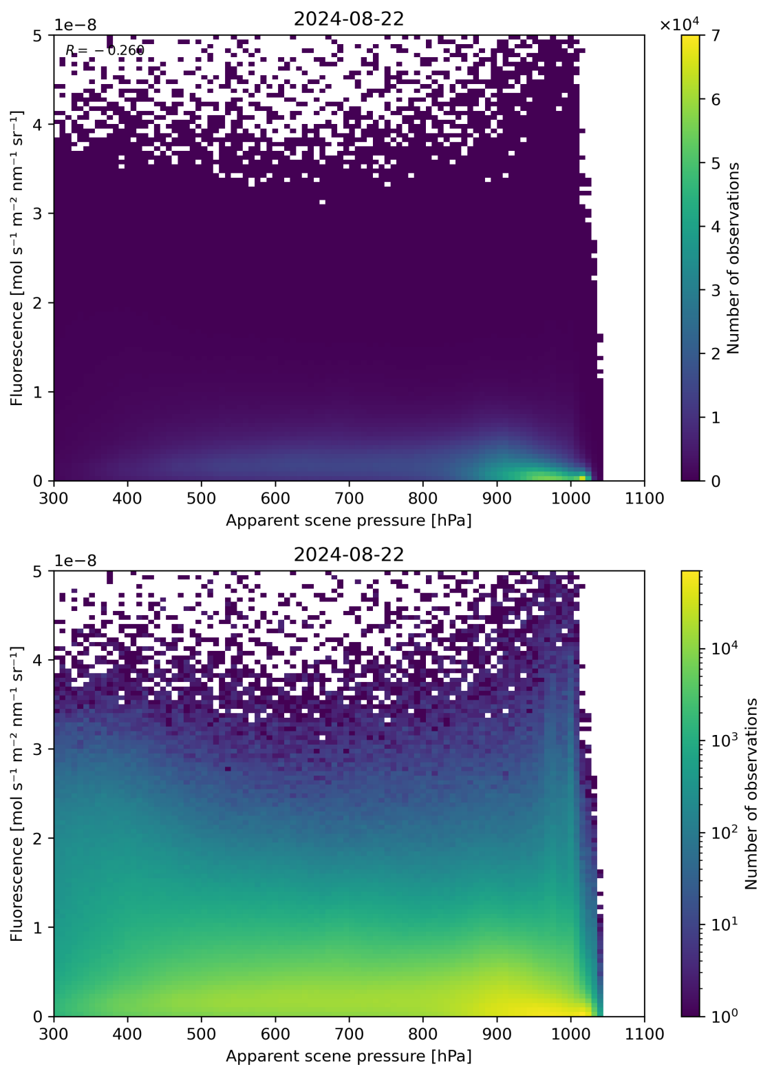
Figure 64: Scatter density plot of “Apparent scene pressure” against “Fluorescence” for 2024-08-22 to 2024-08-23.
