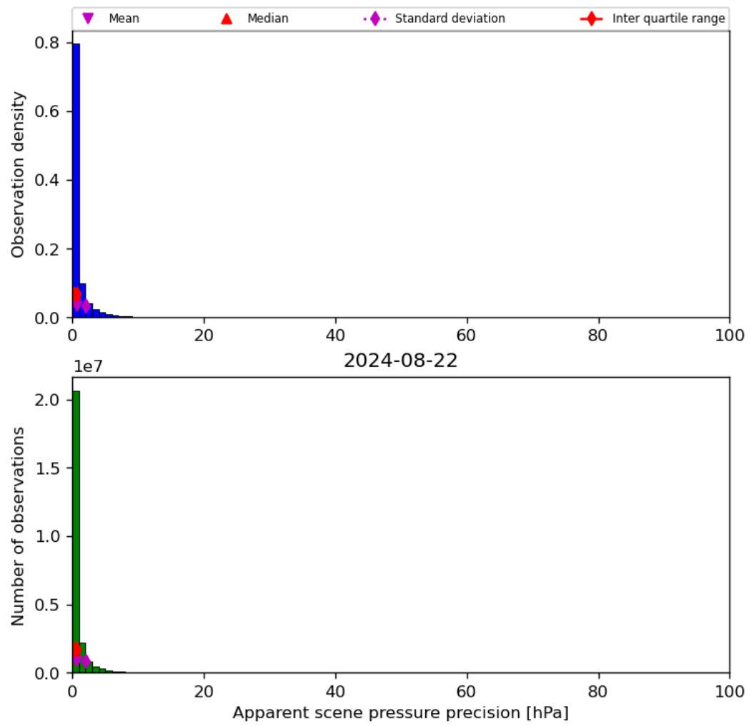
Figure 37: Histogram of “Apparent scene pressure precision” for 2024-08-22 to 2024-08-23
