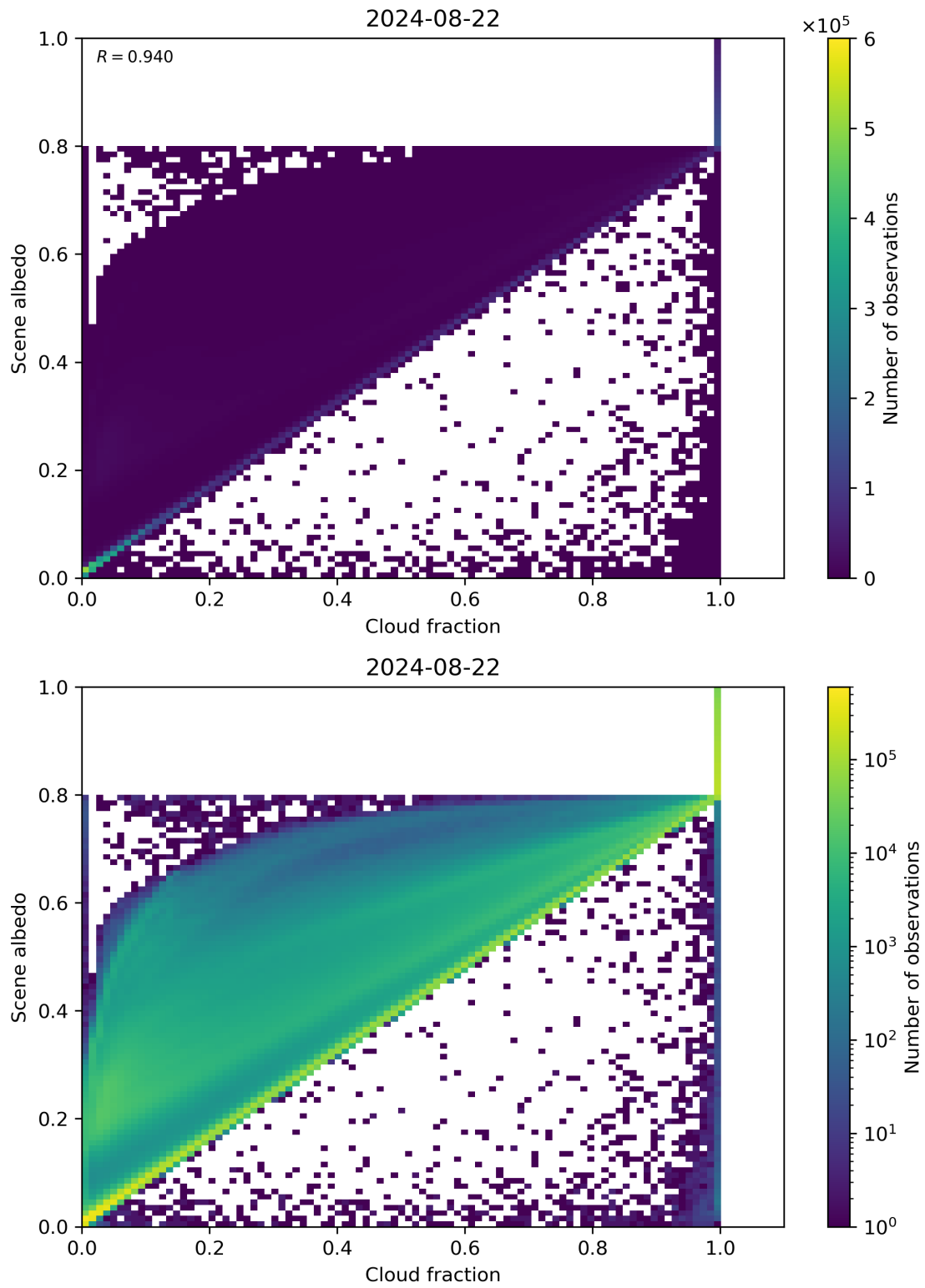
Figure 75: Scatter density plot of “Cloud fraction” against “Scene albedo” for 2024-08-22 to 2024-08-23.
