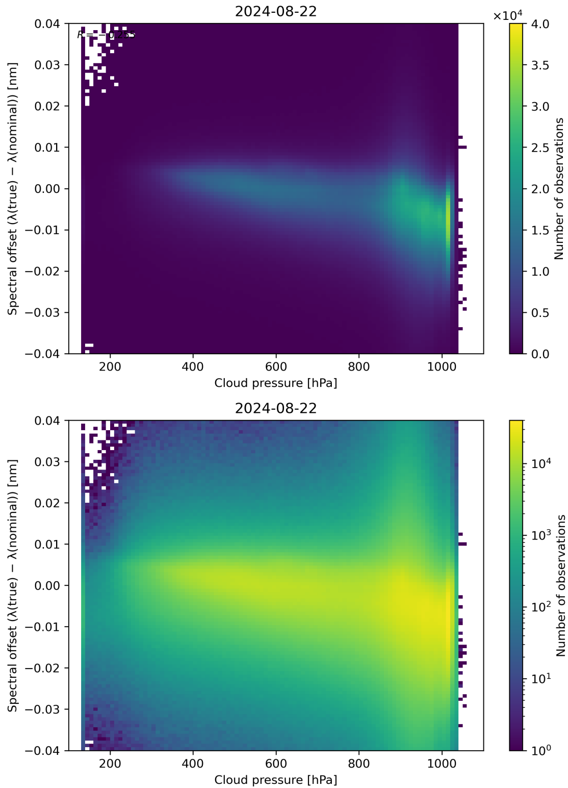
Figure 84: Scatter density plot of “Cloud pressure” against “Spectral offset ( \lambda(\text{true}) - \lambda(\text{nominal}) )” for 2024-08-22 to 2024-08-23.
