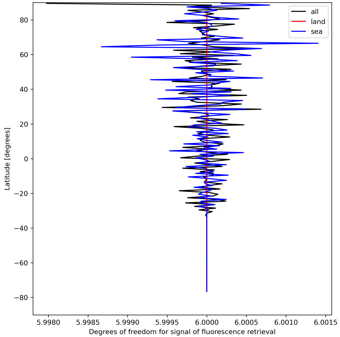
Figure 26: Zonal average of “Degrees of freedom for signal of fluorescence retrieval” for 2024-08-22 to 2024-08-23.
