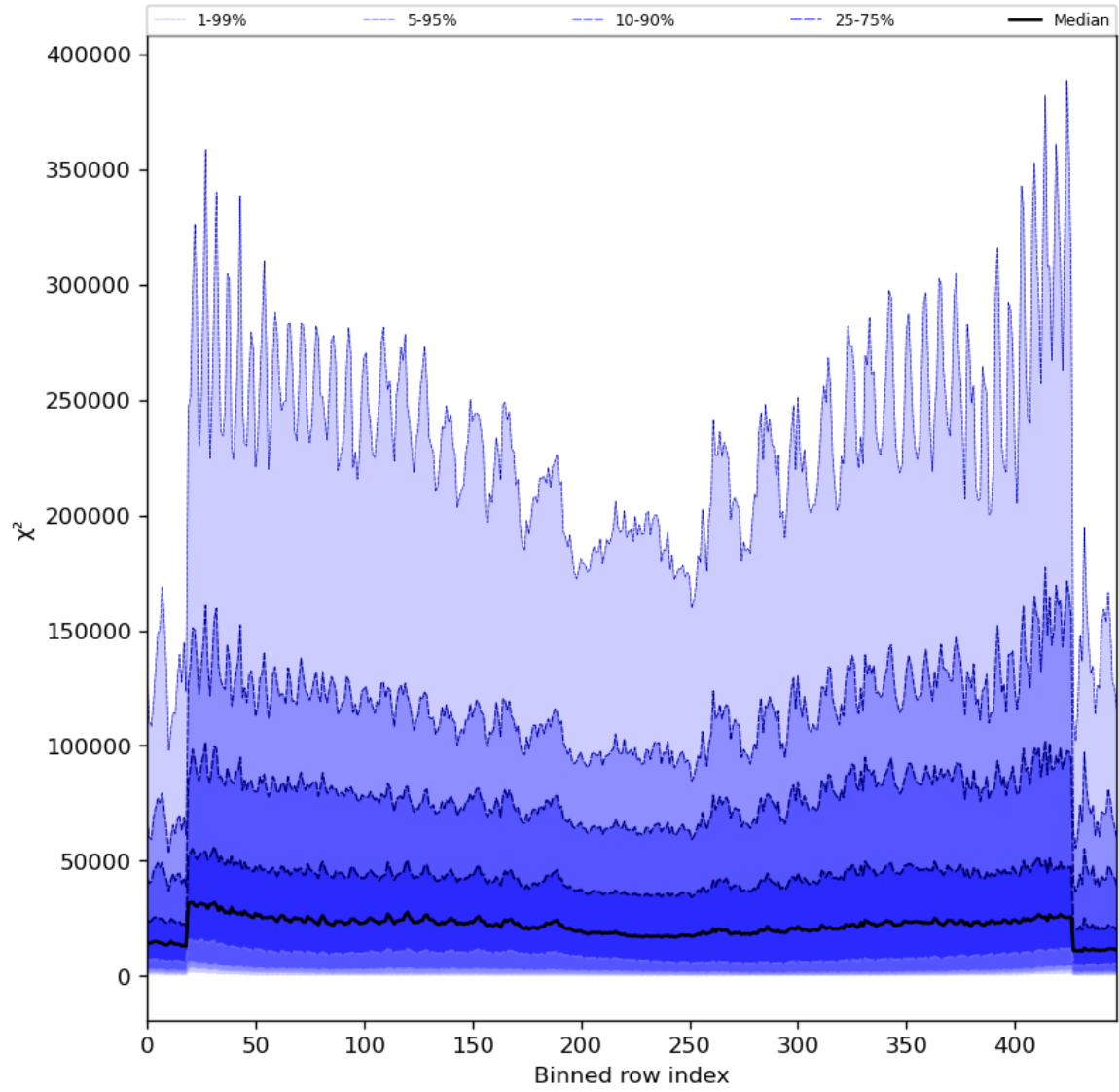
Figure 55: Along track statistics of “ \chi^2 ” for 2024-08-22 to 2024-08-23
