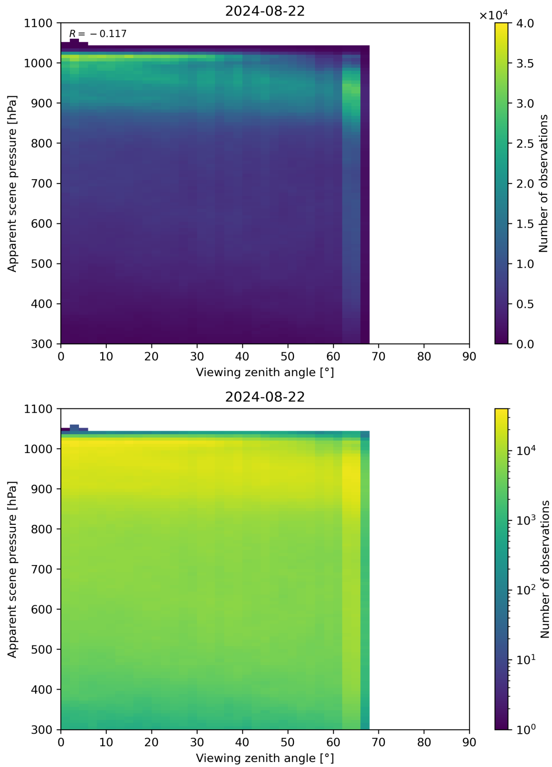
Figure 118: Scatter density plot of “Viewing zenith angle” against “Apparent scene pressure” for 2024-08-22 to 2024-08-23.
