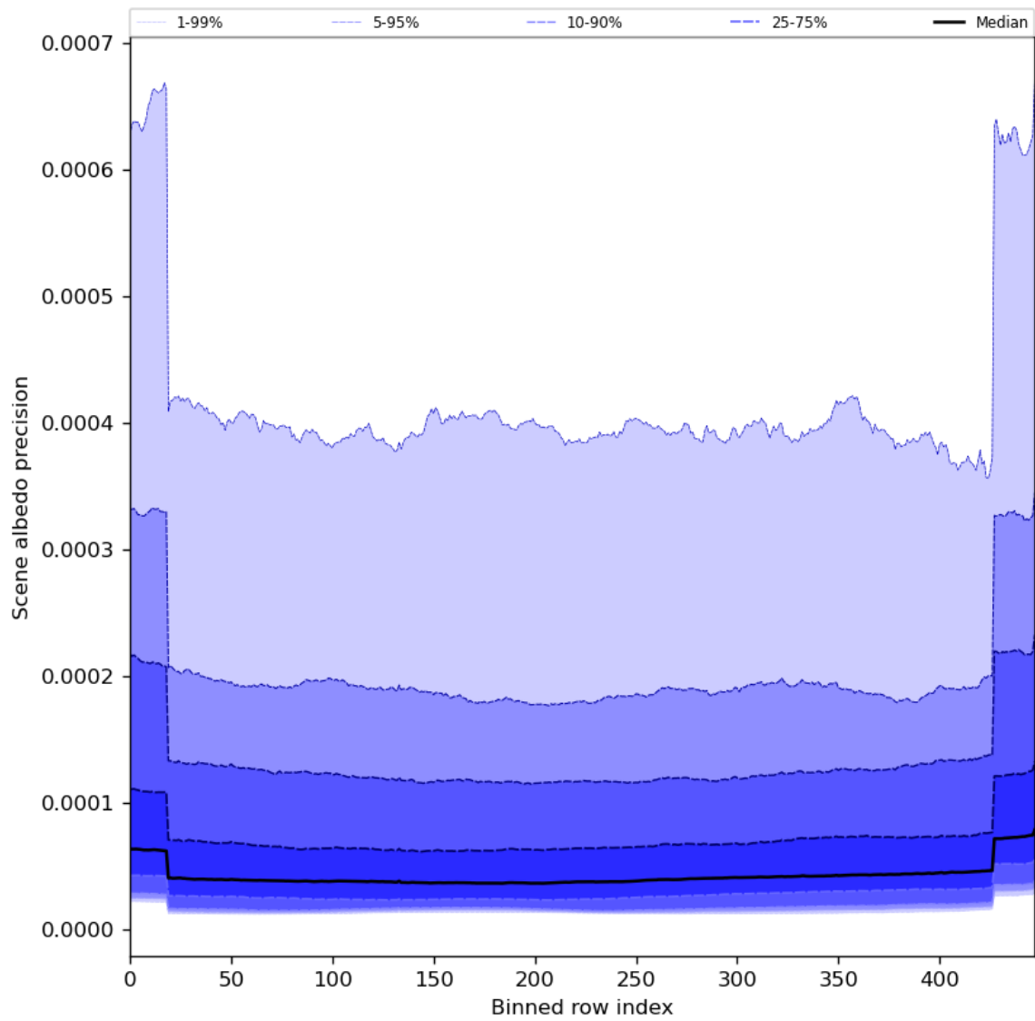
Figure 52: Along track statistics of “Scene albedo precision” for 2024-08-22 to 2024-08-23
