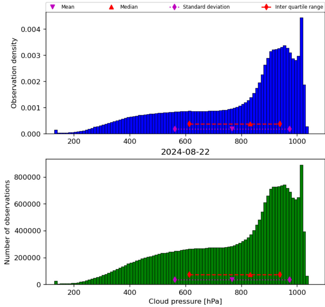
Figure 30: Histogram of “Cloud pressure” for 2024-08-22 to 2024-08-23
