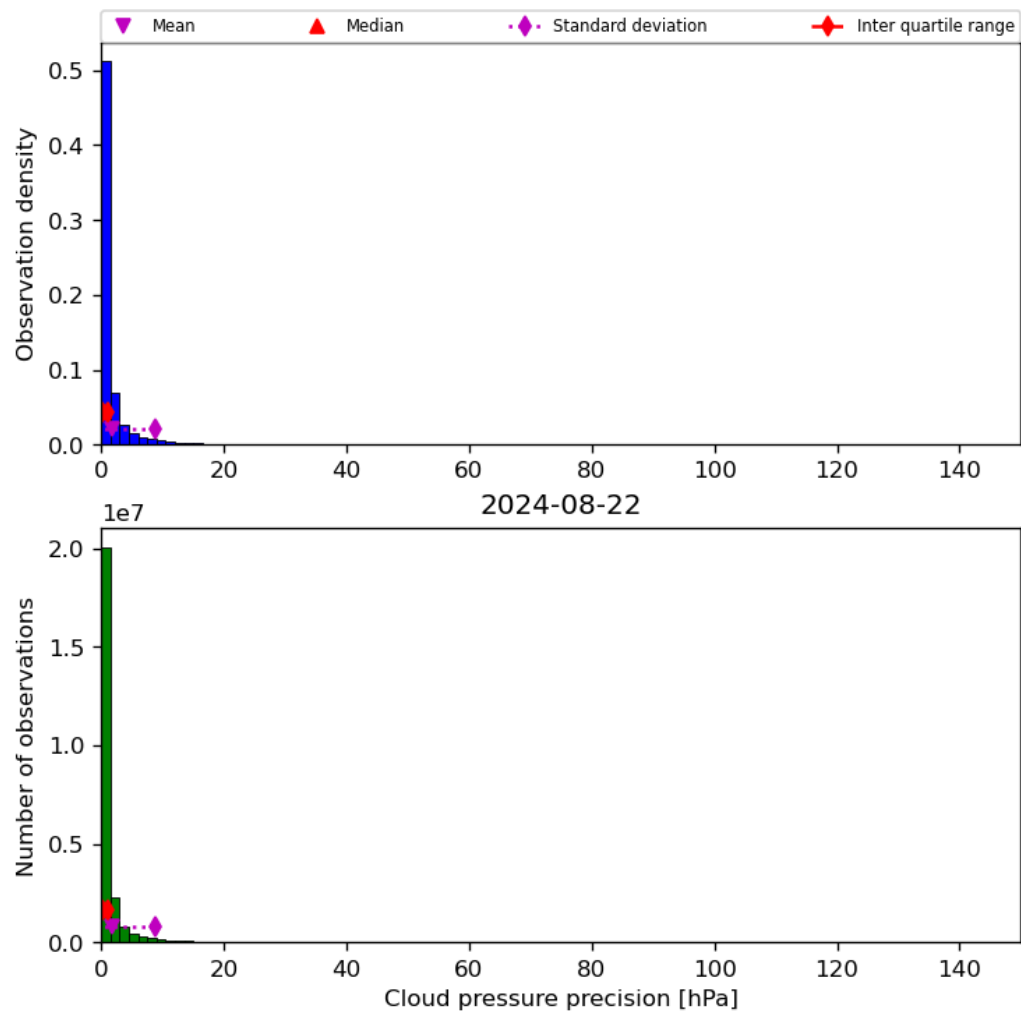
Figure 31: Histogram of “Cloud pressure precision” for 2024-08-22 to 2024-08-23
