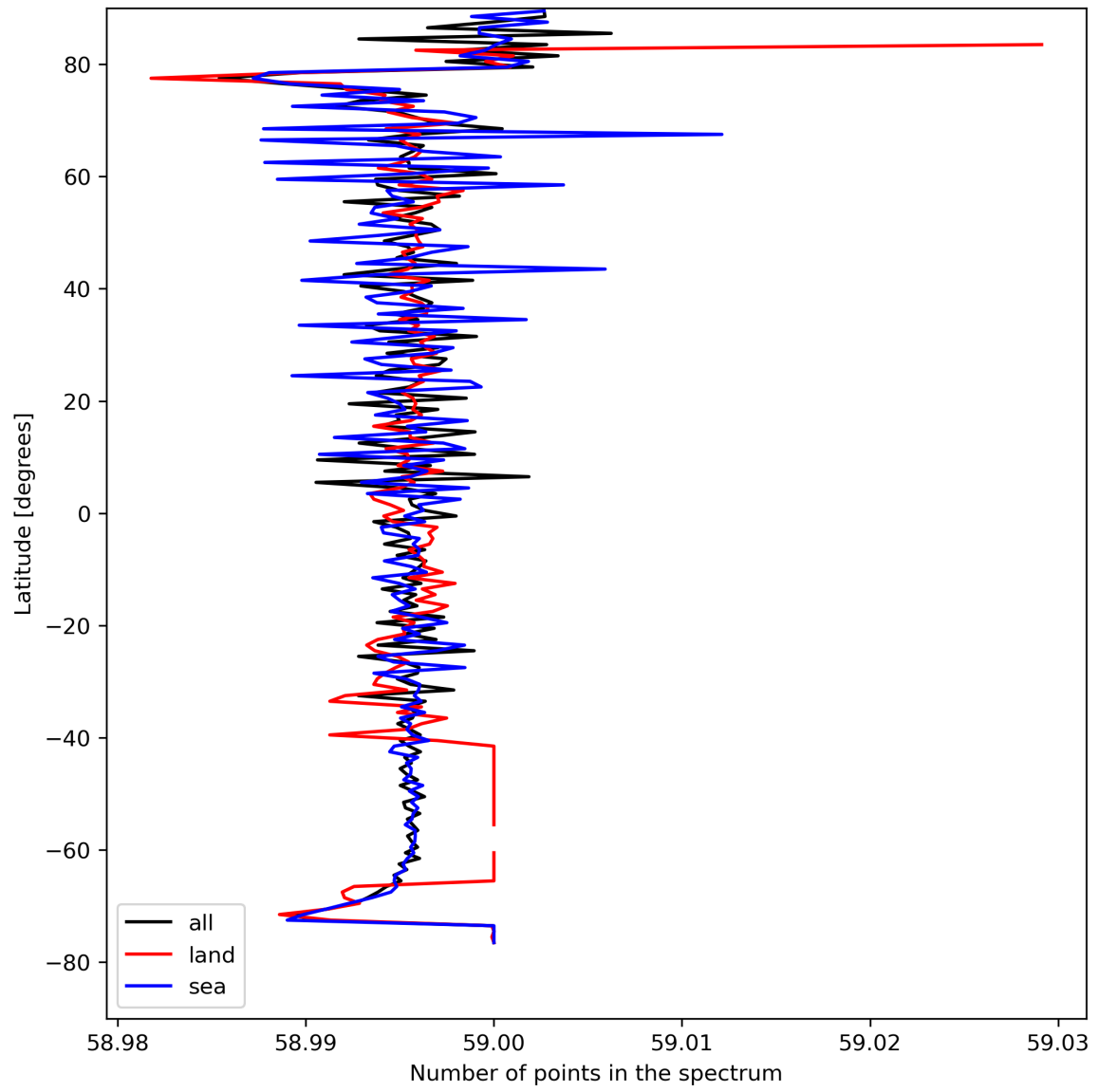
Figure 27: Zonal average of “Number of points in the spectrum” for 2024-08-22 to 2024-08-23.
