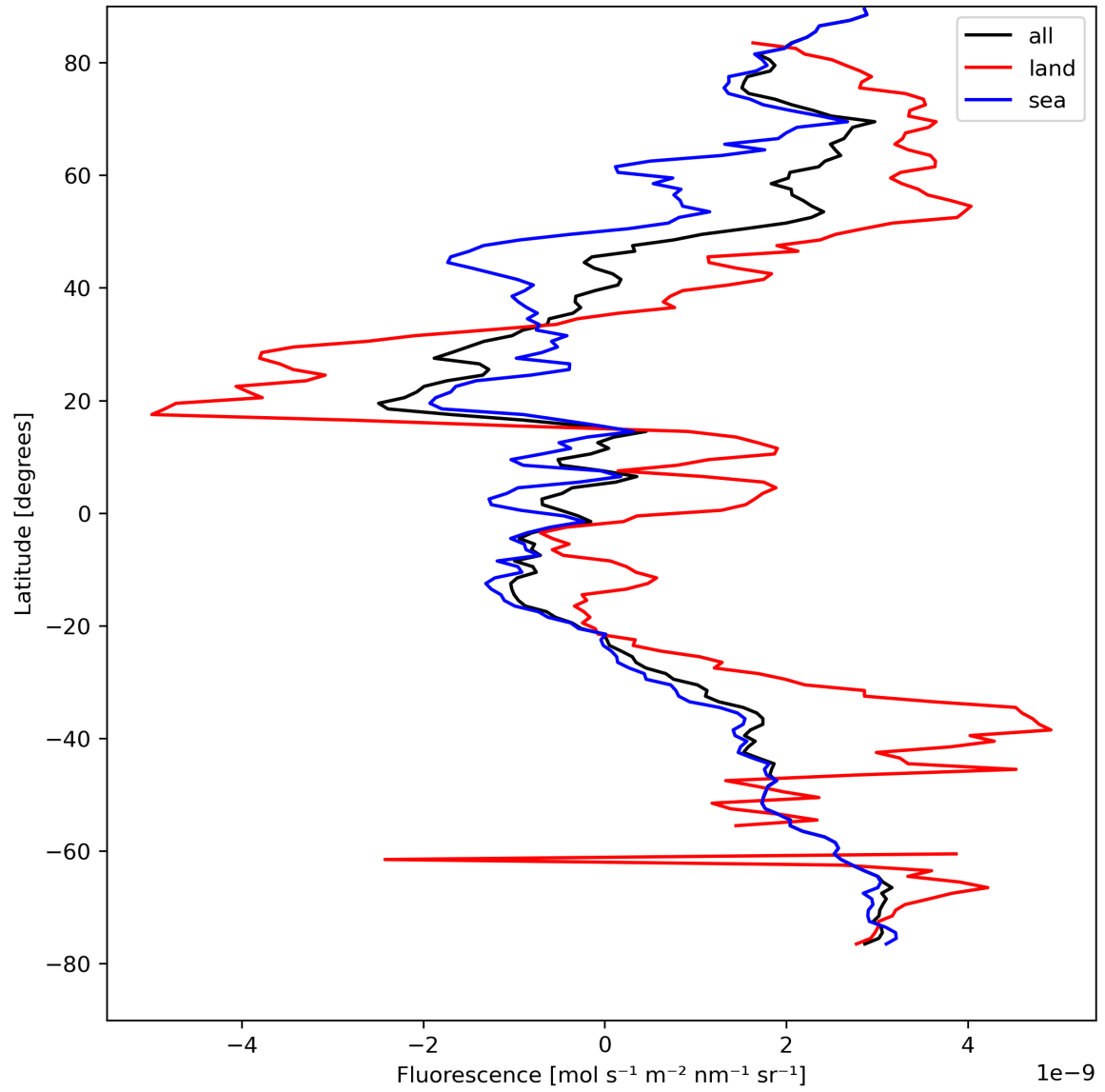
Figure 23: Zonal average of “Fluorescence” for 2024-08-22 to 2024-08-23.
