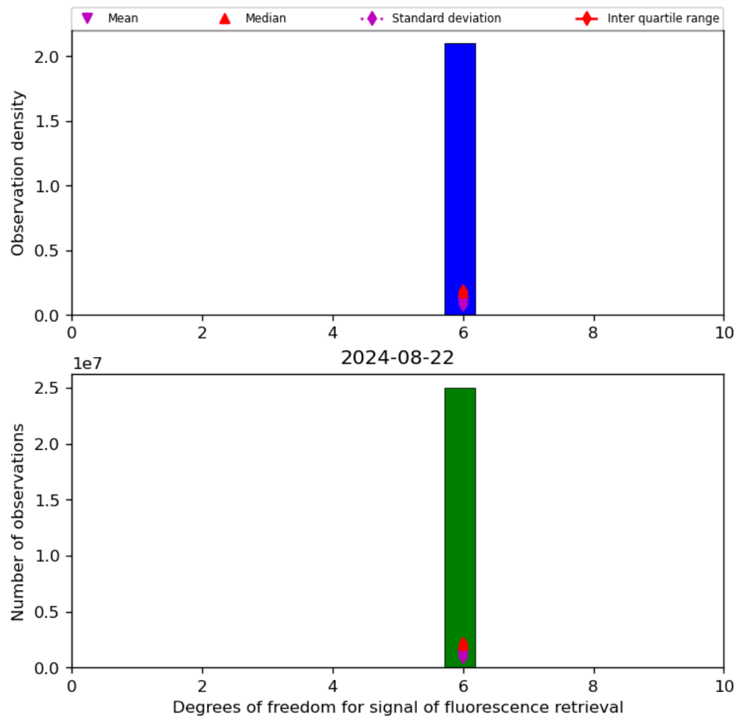
Figure 43: Histogram of “Degrees of freedom for signal of fluorescence retrieval” for 2024-08-22 to 2024-08-23
