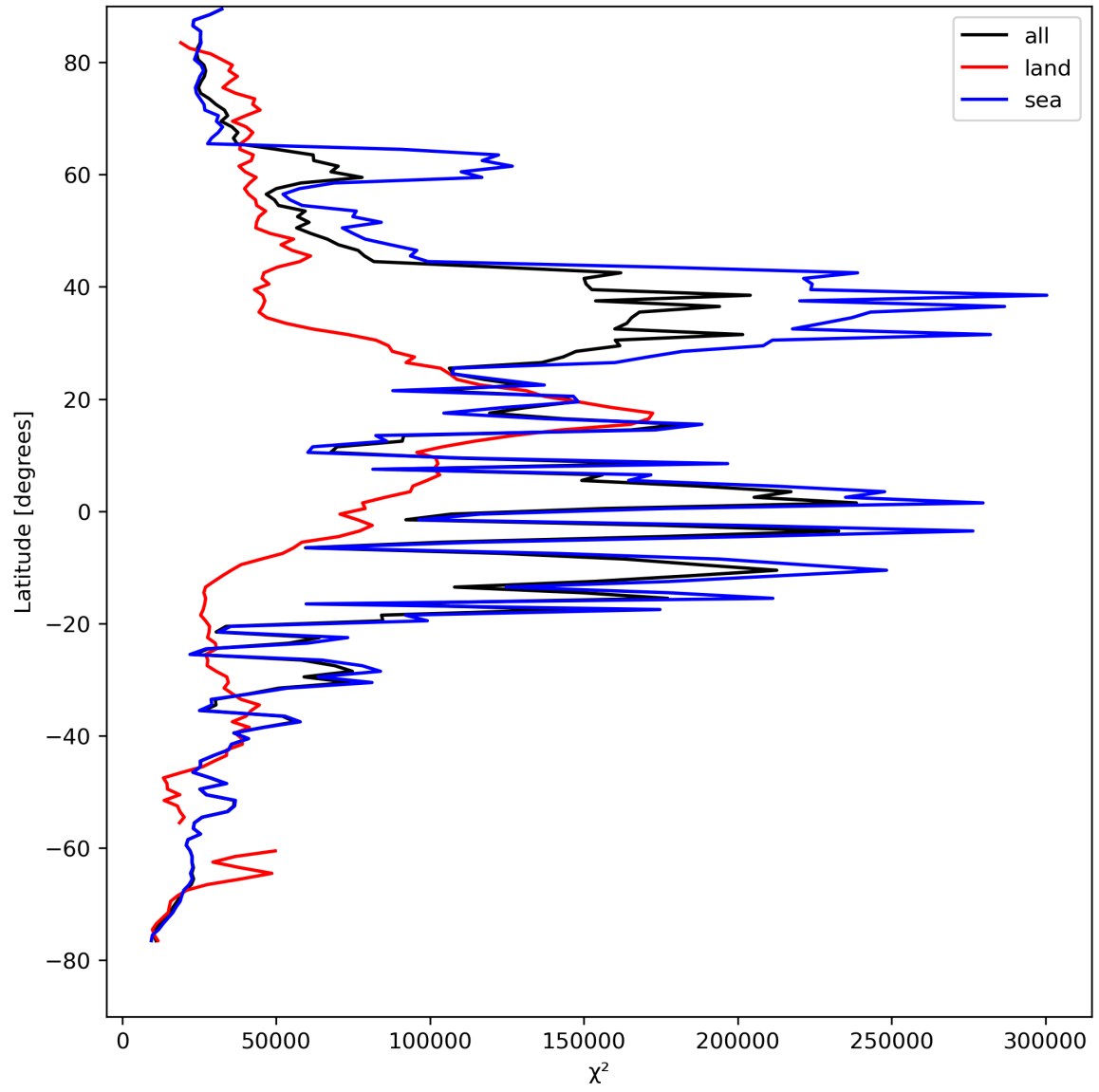
Figure 21: Zonal average of “ \chi^2 ” for 2024-08-22 to 2024-08-23.
