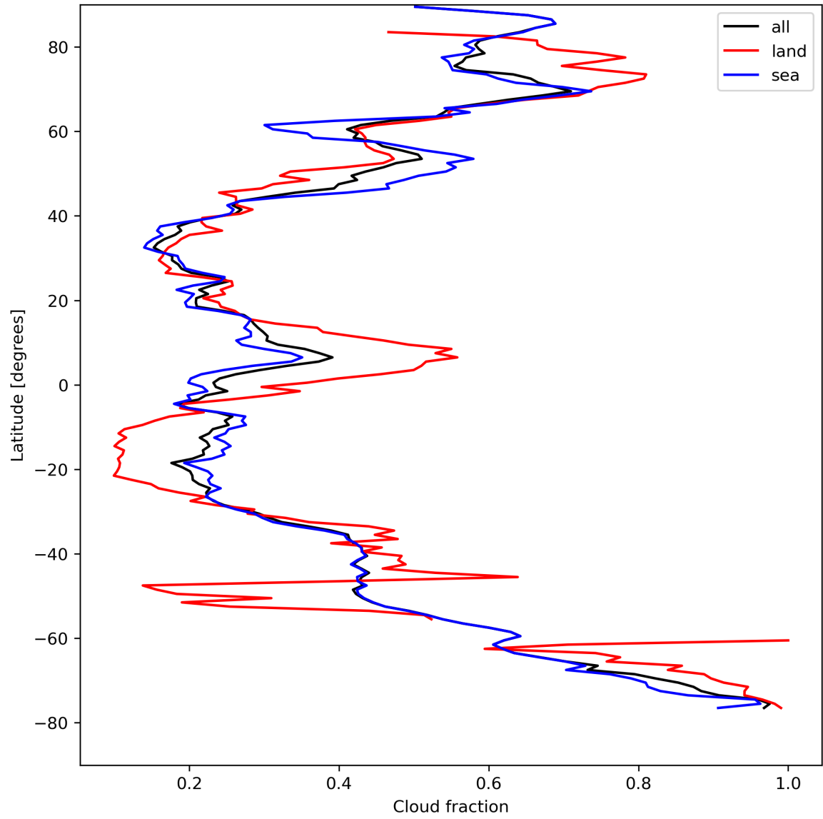
Figure 15: Zonal average of “Cloud fraction” for 2024-08-22 to 2024-08-23.
