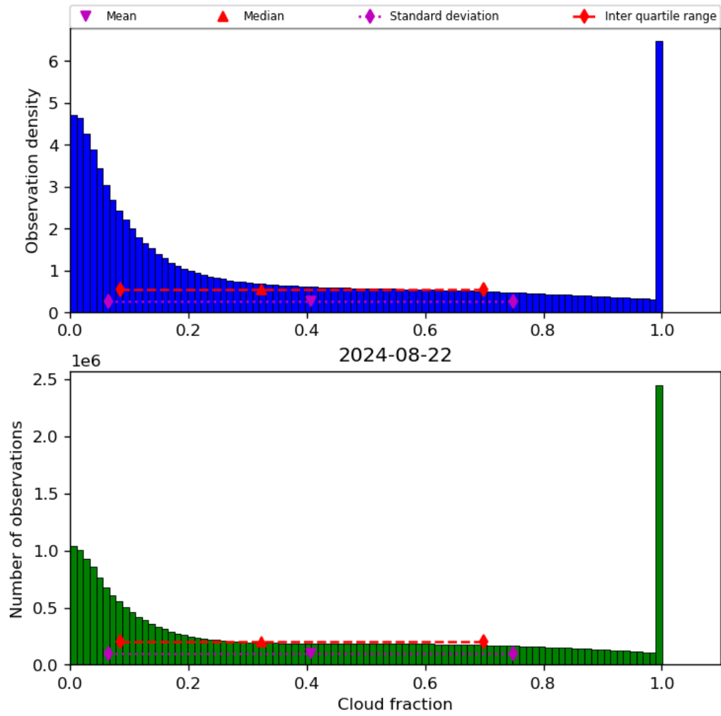
Figure 32: Histogram of “Cloud fraction” for 2024-08-22 to 2024-08-23
