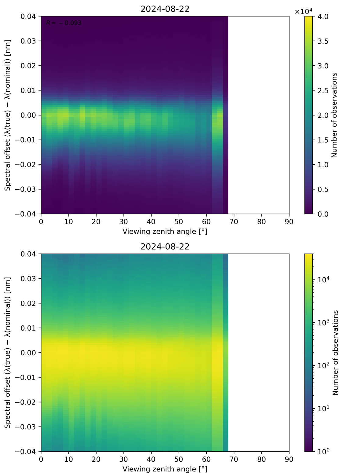
Figure 128: Scatter density plot of “Viewing zenith angle” against “Spectral offset ( \lambda(\text{true}) - \lambda(\text{nominal}) )” for 2024-08-22 to 2024-08-23.
