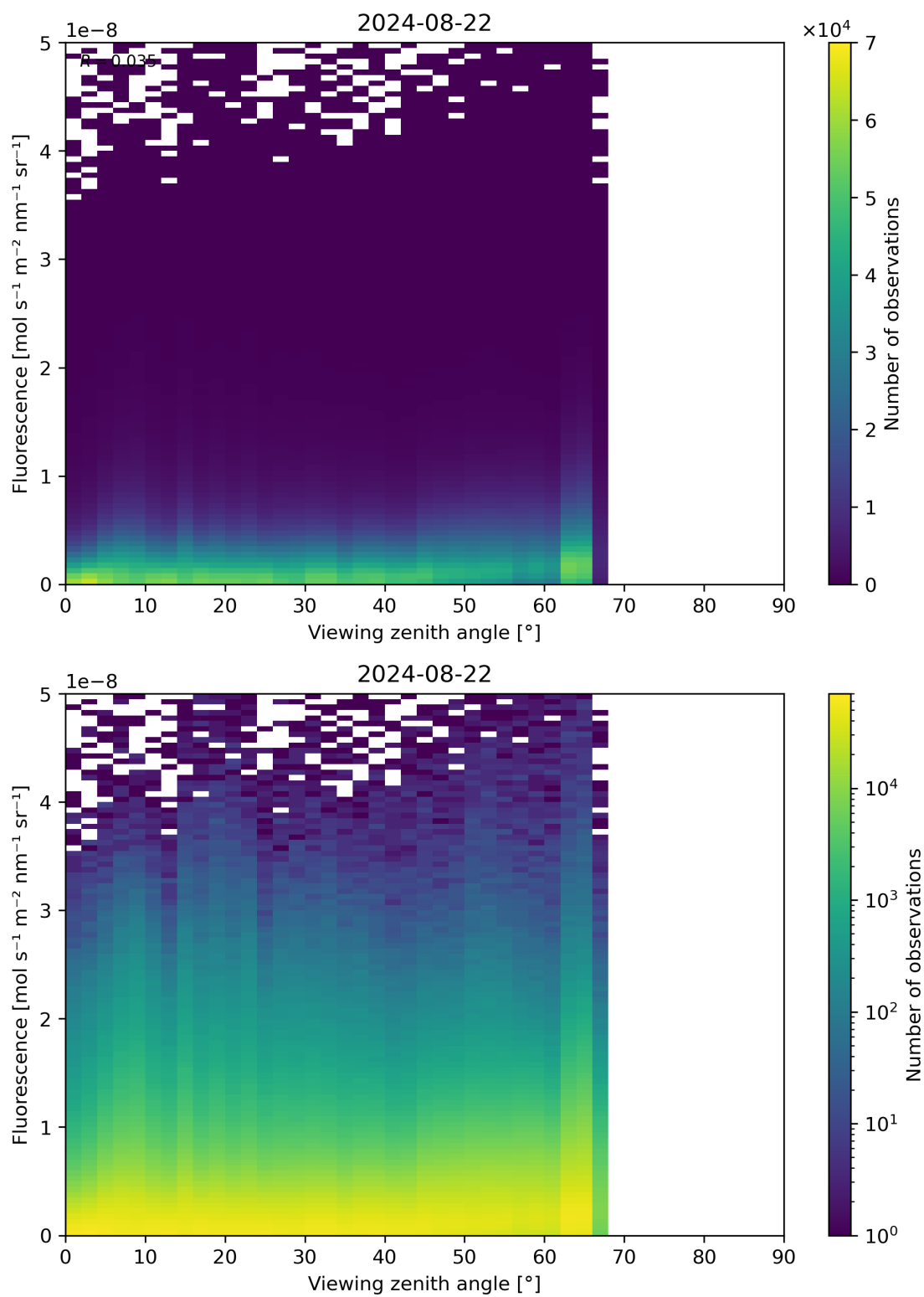
Figure 122: Scatter density plot of “Viewing zenith angle” against “Fluorescence” for 2024-08-22 to 2024-08-23.
