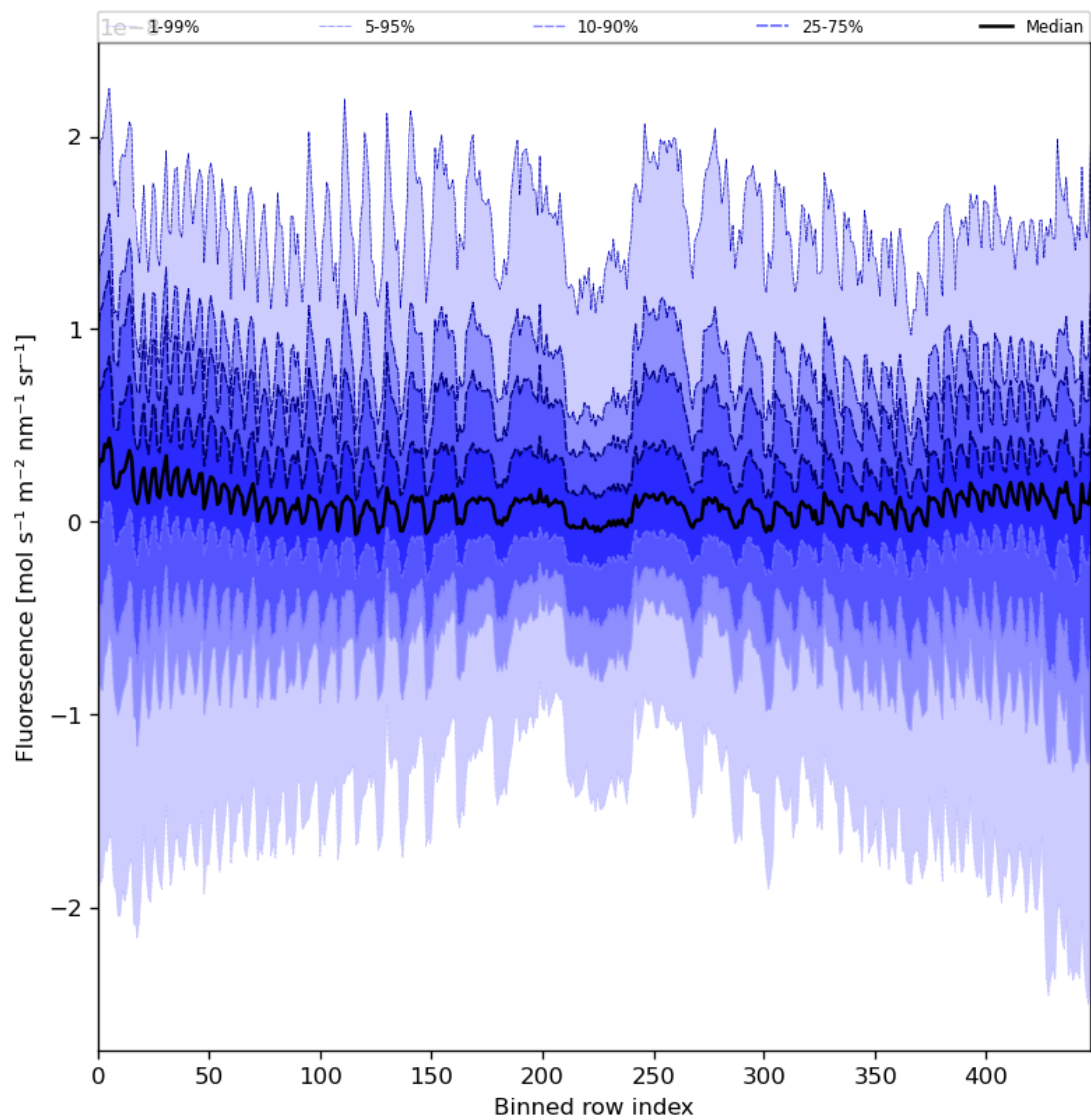
Figure 57: Along track statistics of “Fluorescence” for 2024-08-22 to 2024-08-23
