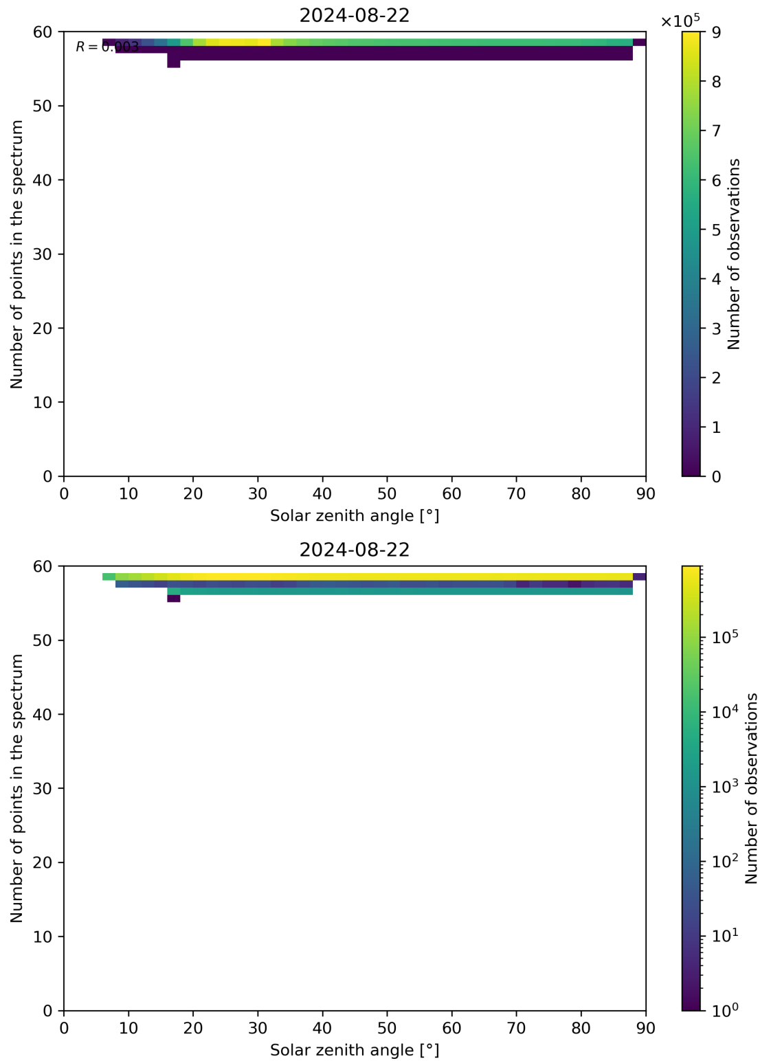
Figure 115: Scatter density plot of “Solar zenith angle” against “Number of points in the spectrum” for 2024-08-22 to 2024-08-23.
