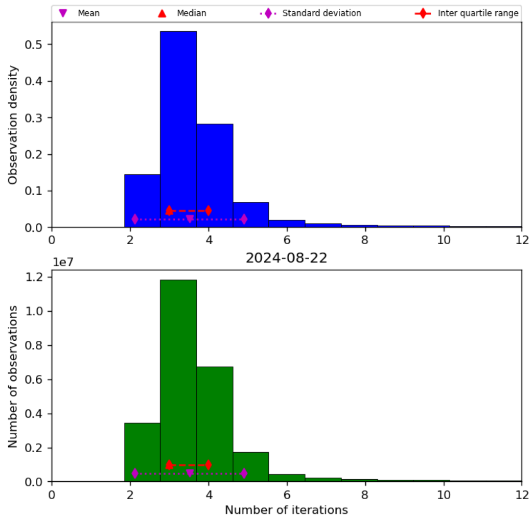
Figure 39: Histogram of “Number of iterations” for 2024-08-22 to 2024-08-23
