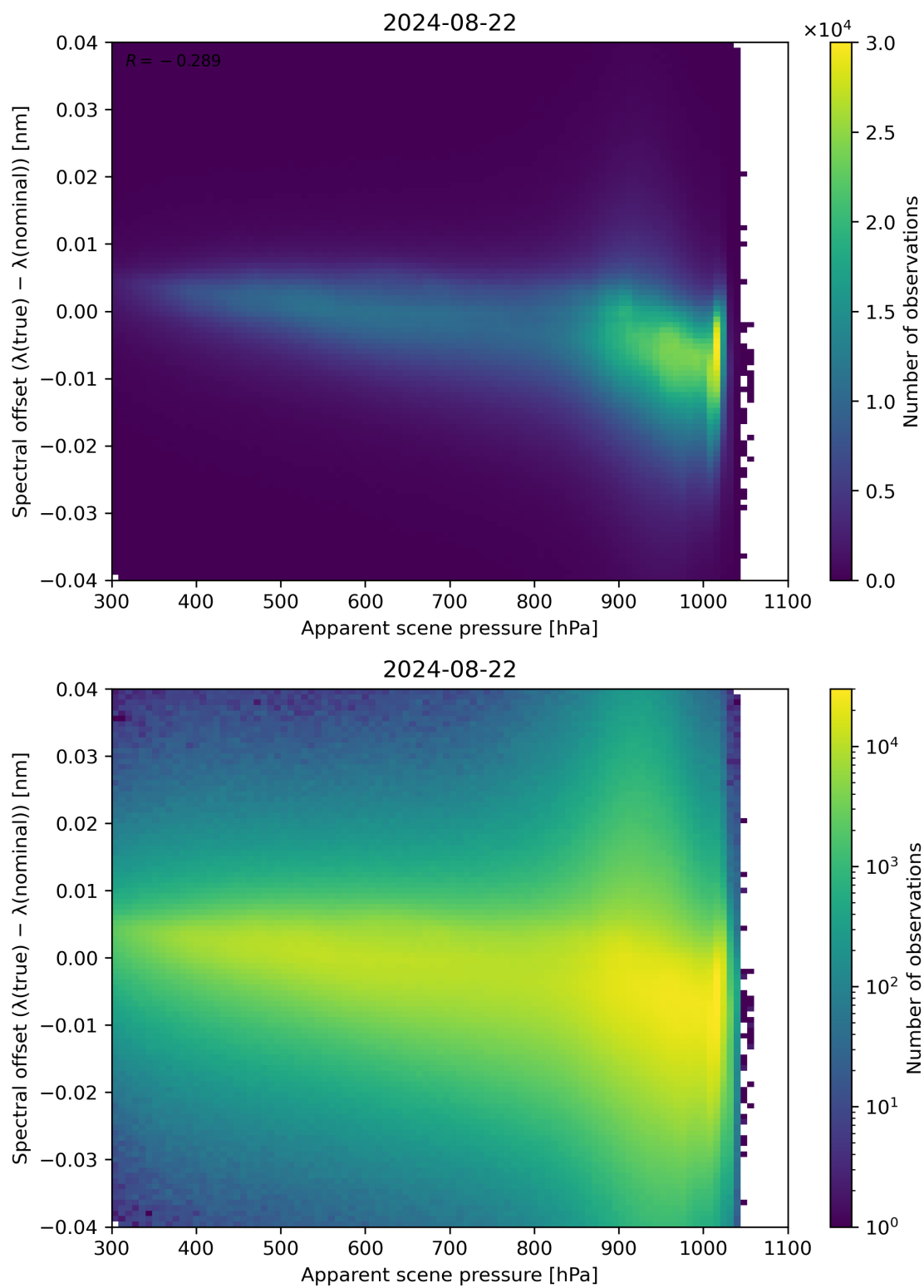
Figure 67: Scatter density plot of “Apparent scene pressure” against “Spectral offset ( \lambda(\text{true}) - \lambda(\text{nominal}) )” for 2024-08-22 to 2024-08-23.
