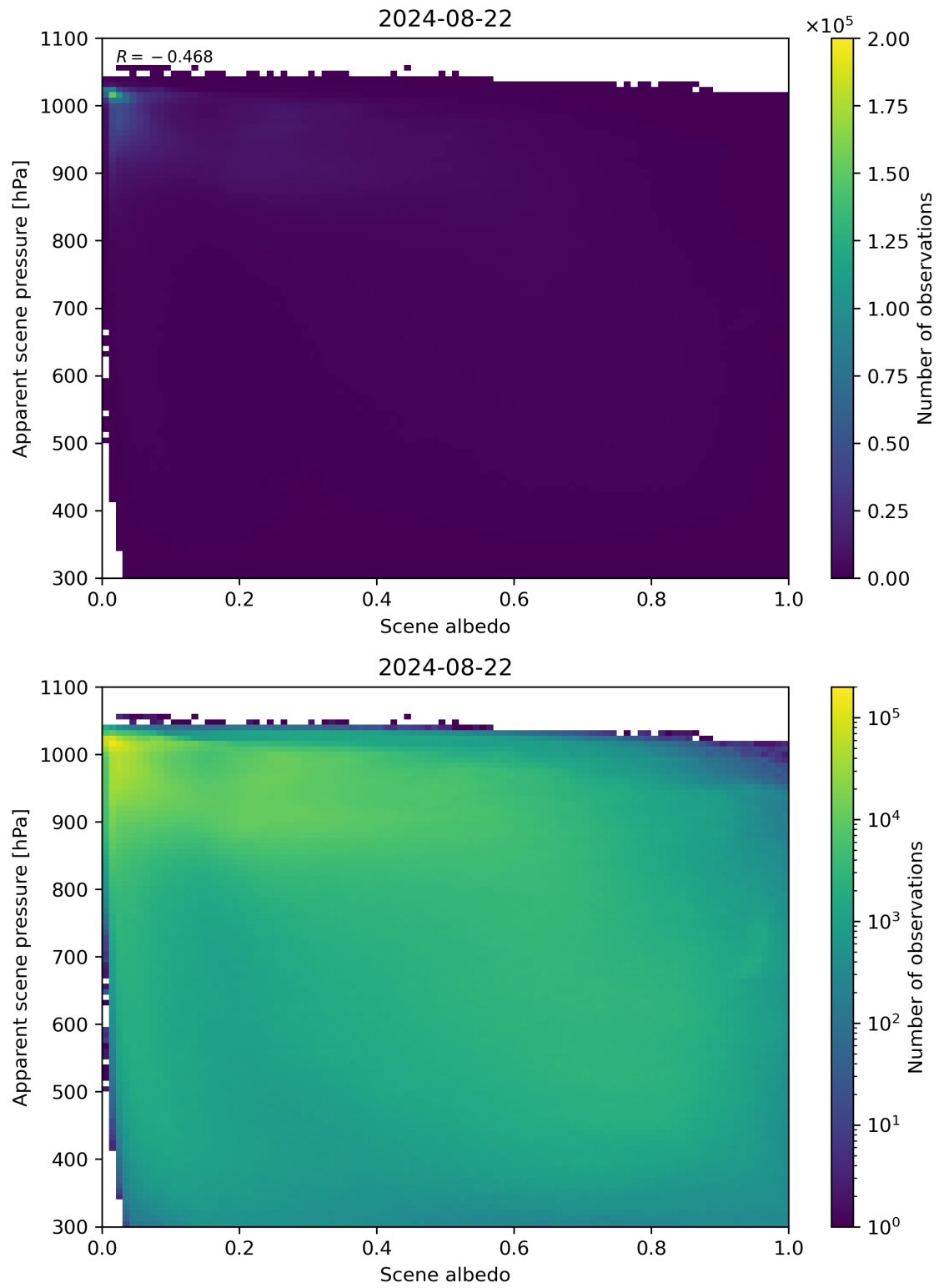
Figure 102: Scatter density plot of “Scene albedo” against “Apparent scene pressure” for 2024-08-22 to 2024-08-23.
