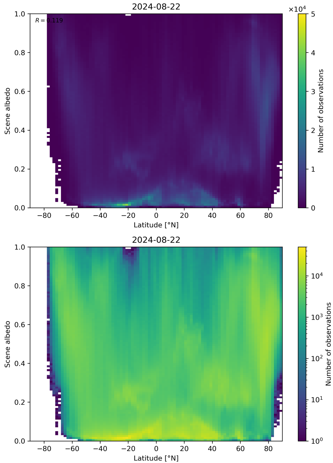
Figure 95: Scatter density plot of “Latitude” against “Scene albedo” for 2024-08-22 to 2024-08-23.
