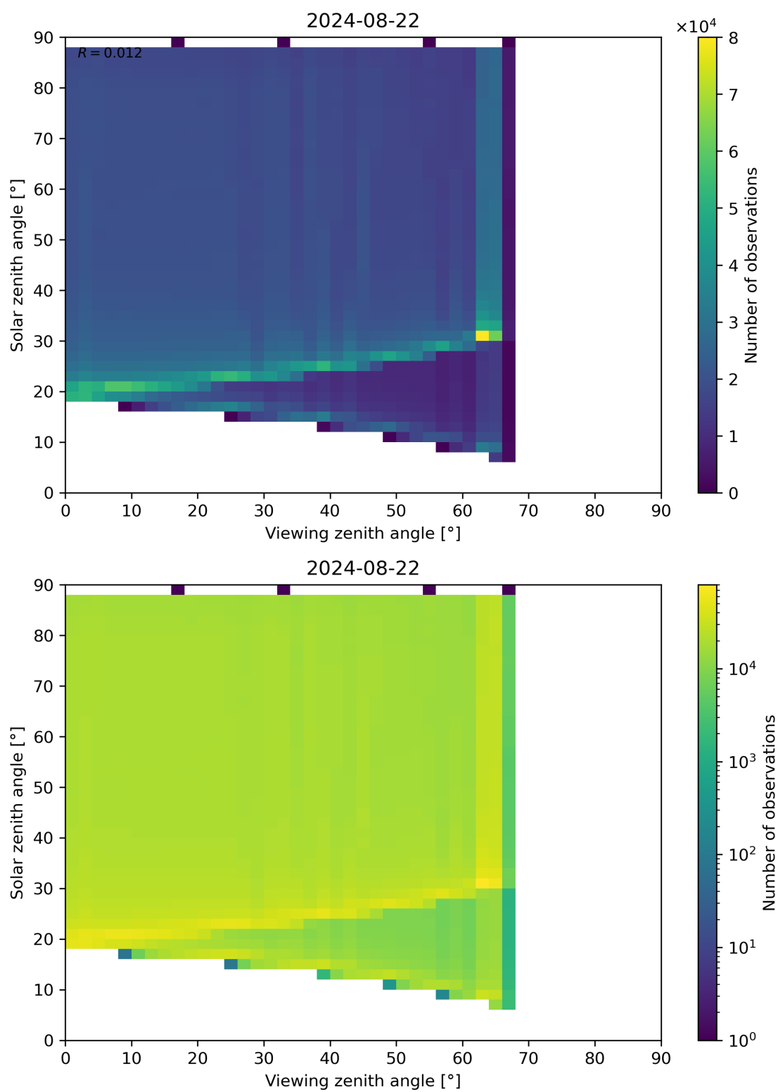
Figure 127: Scatter density plot of “Viewing zenith angle” against “Solar zenith angle” for 2024-08-22 to 2024-08-23.
