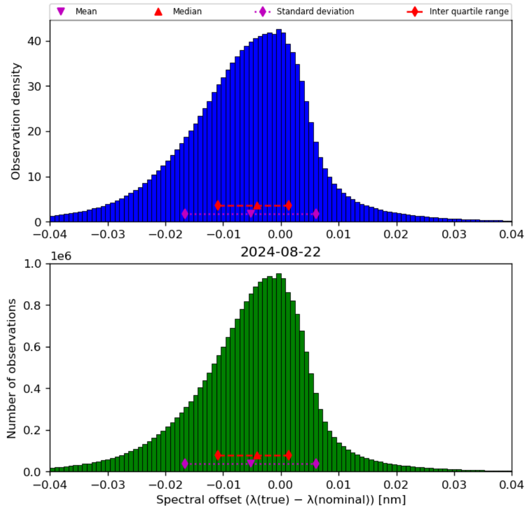
Figure 45: Histogram of “Spectral offset ( \lambda(\text{true}) - \lambda(\text{nominal}) )” for 2024-08-22 to 2024-08-23
