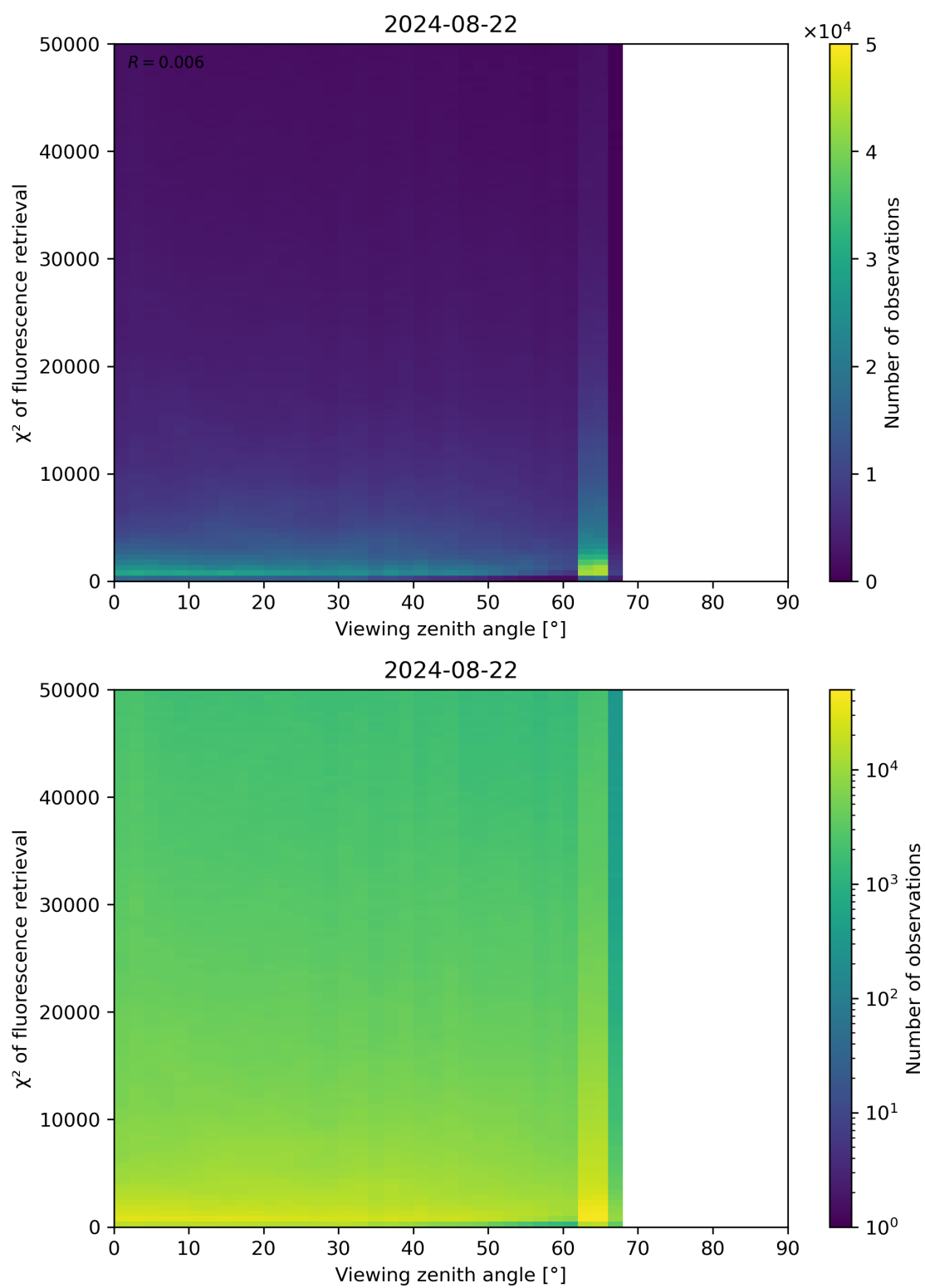
Figure 119: Scatter density plot of “Viewing zenith angle” against “ \chi^2 of fluorescence retrieval” for 2024-08-22 to 2024-08-23.
