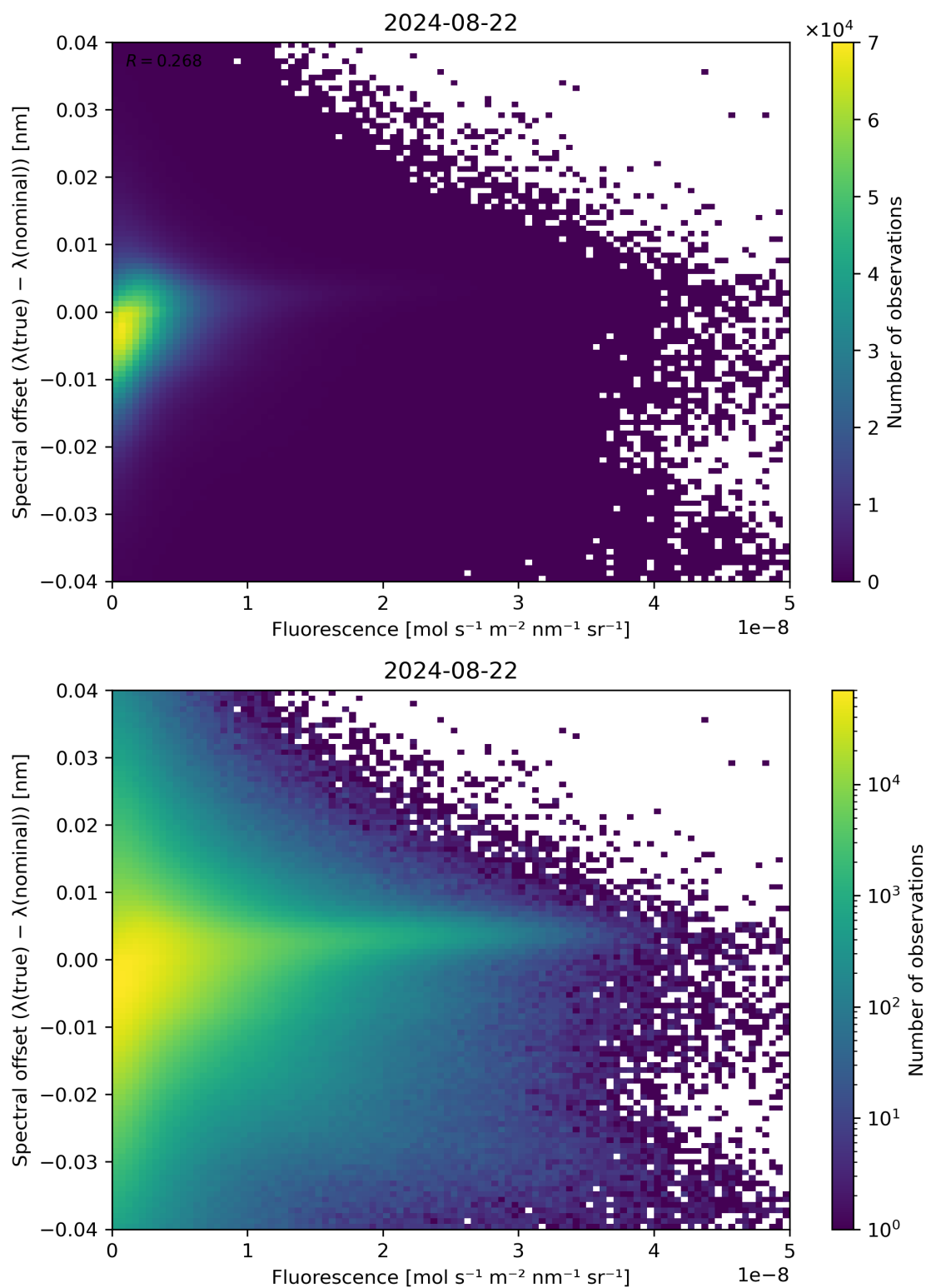
Figure 87: Scatter density plot of “Fluorescence” against “Spectral offset ( \lambda(\text{true}) - \lambda(\text{nominal}) )” for 2024-08-22 to 2024-08-23.
