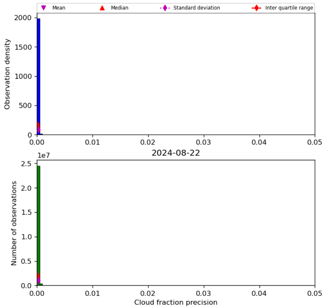
Figure 33: Histogram of “Cloud fraction precision” for 2024-08-22 to 2024-08-23
