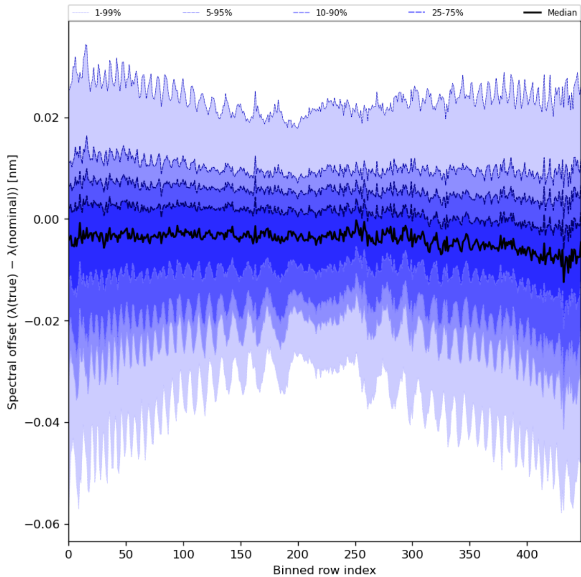
Figure 62: Along track statistics of “Spectral offset ( \lambda(\text{true}) - \lambda(\text{nominal}) )” for 2024-08-22 to 2024-08-23
