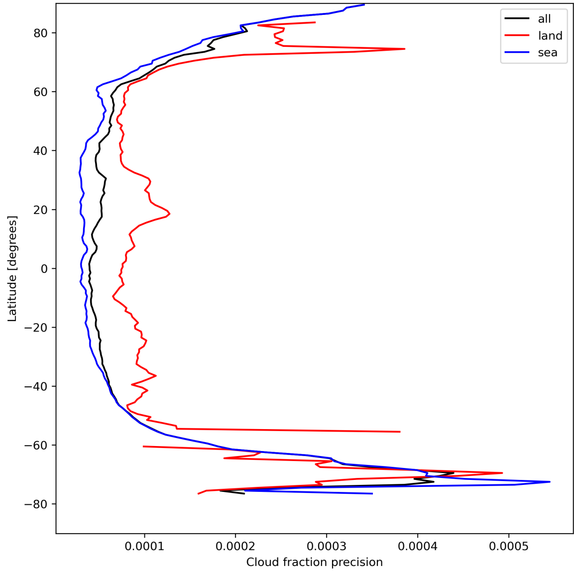
Figure 16: Zonal average of “Cloud fraction precision” for 2024-08-22 to 2024-08-23.
