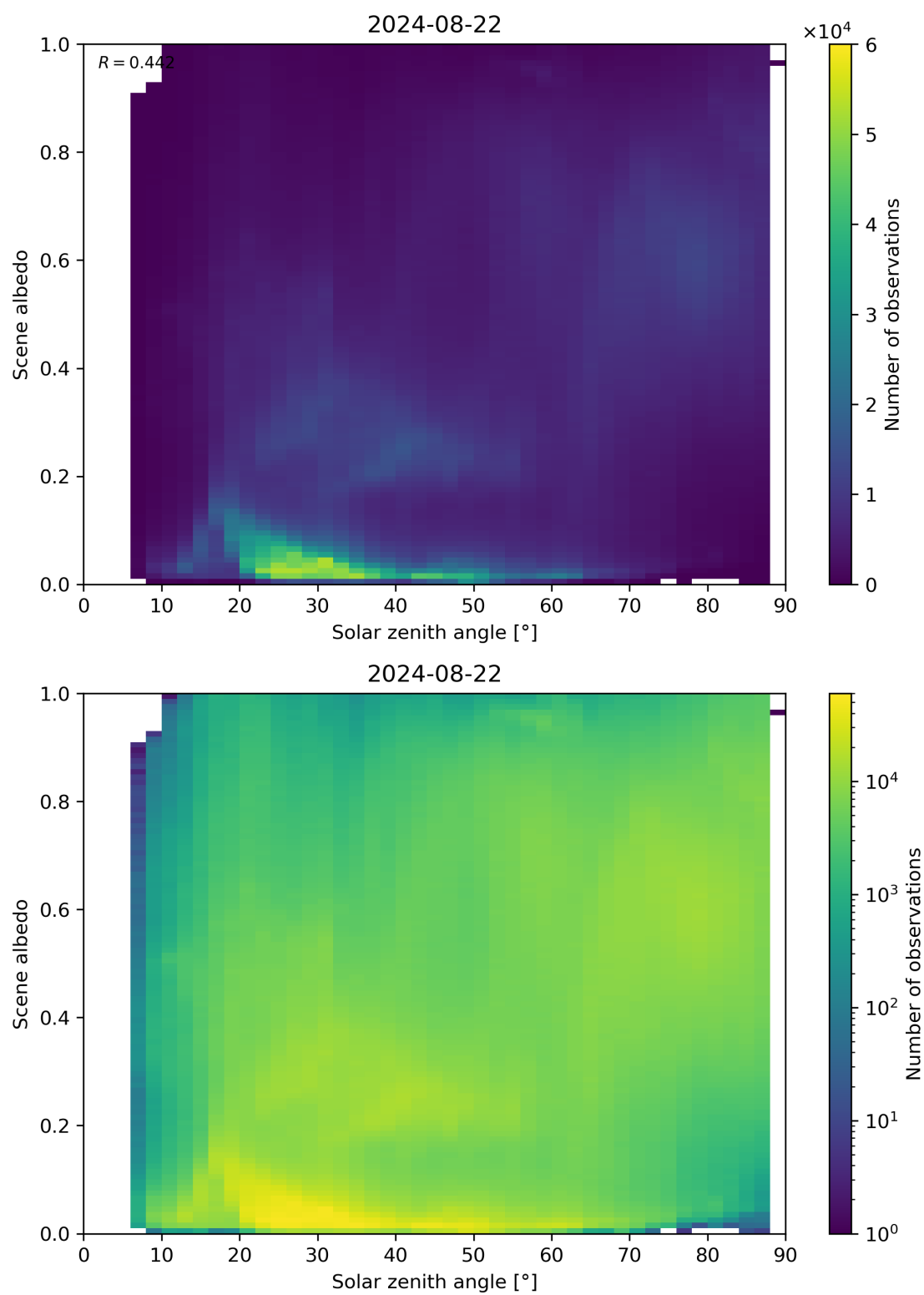
Figure 116: Scatter density plot of “Solar zenith angle” against “Scene albedo” for 2024-08-22 to 2024-08-23.
