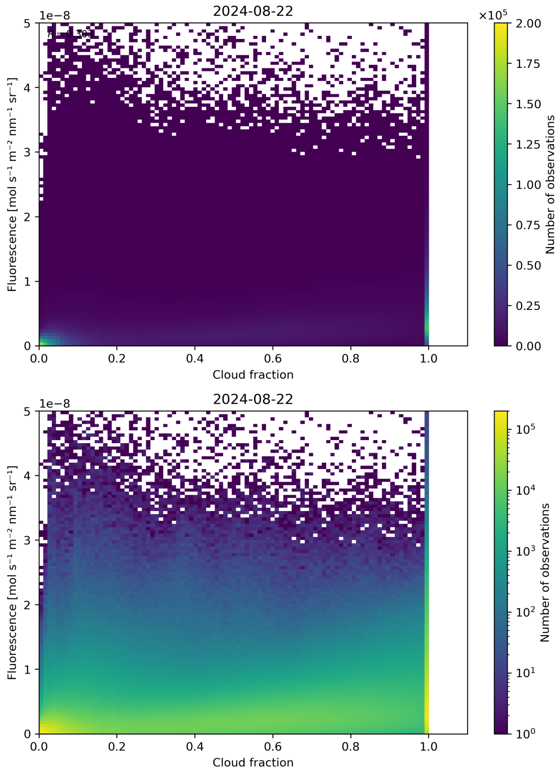
Figure 72: Scatter density plot of “Cloud fraction” against “Fluorescence” for 2024-08-22 to 2024-08-23.
