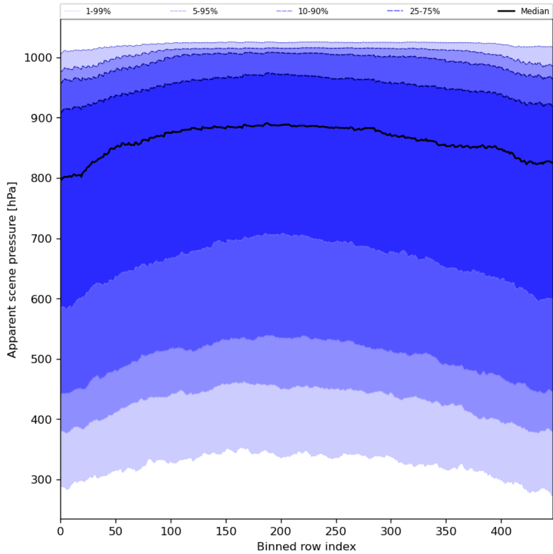
Figure 53: Along track statistics of “Apparent scene pressure” for 2024-08-22 to 2024-08-23
