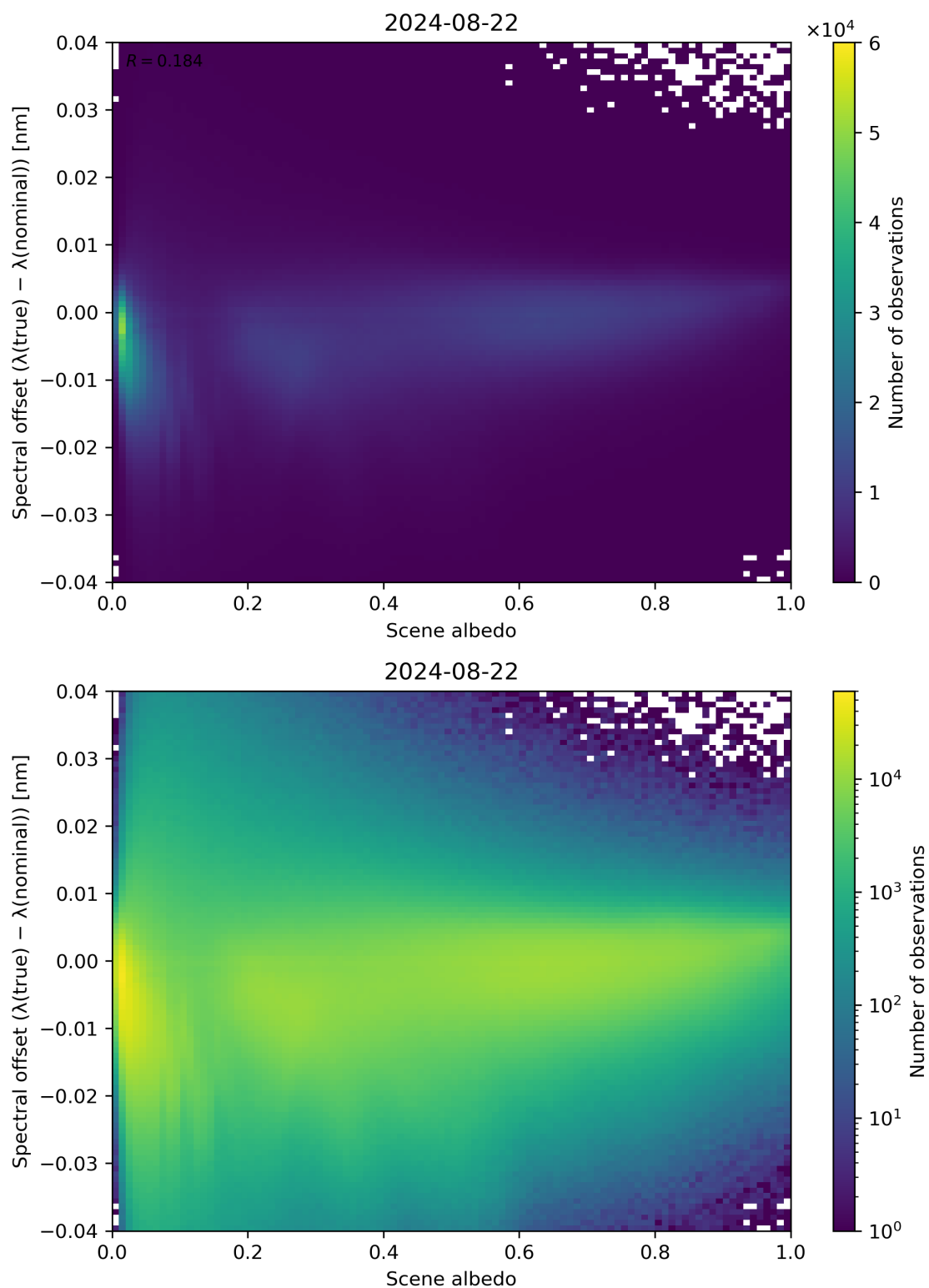
Figure 107: Scatter density plot of “Scene albedo” against “Spectral offset ( \lambda(\text{true}) - \lambda(\text{nominal}) )” for 2024-08-22 to 2024-08-23.
