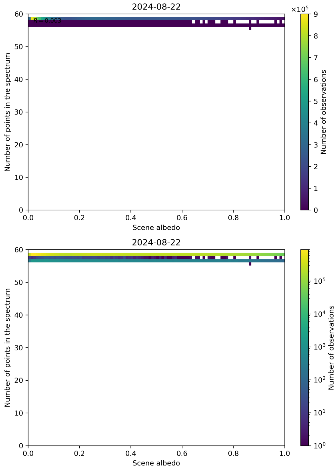
Figure 106: Scatter density plot of “Scene albedo” against “Number of points in the spectrum” for 2024-08-22 to 2024-08-23.
