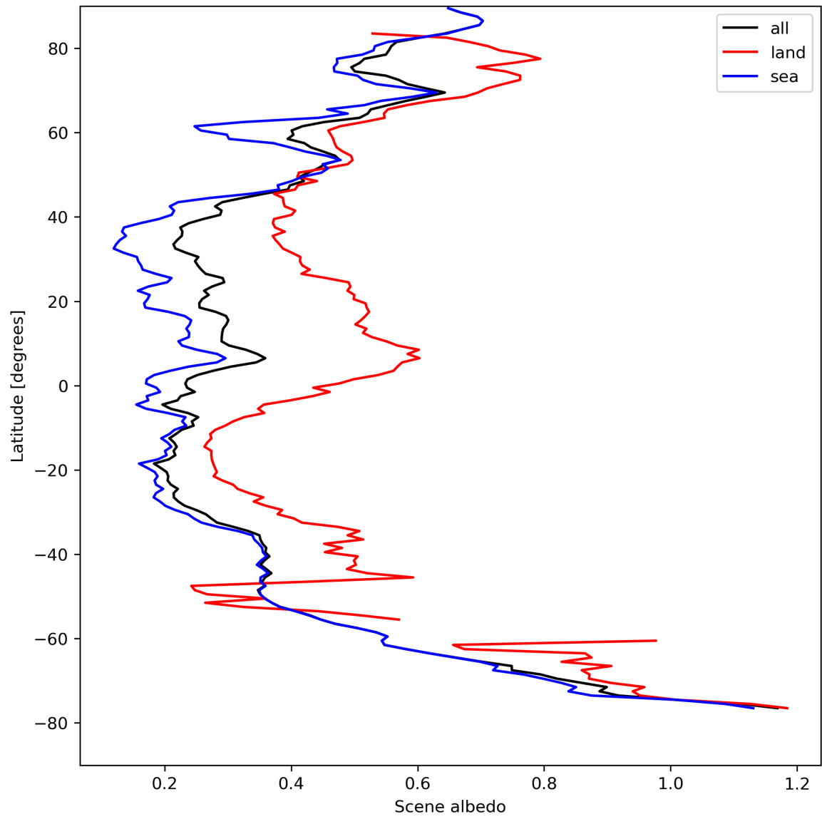
Figure 17: Zonal average of “Scene albedo” for 2024-08-22 to 2024-08-23.
