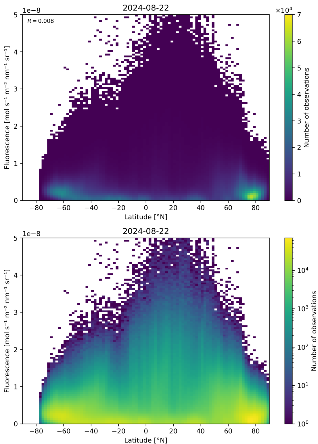
Figure 92: Scatter density plot of “Latitude” against “Fluorescence” for 2024-08-22 to 2024-08-23.
