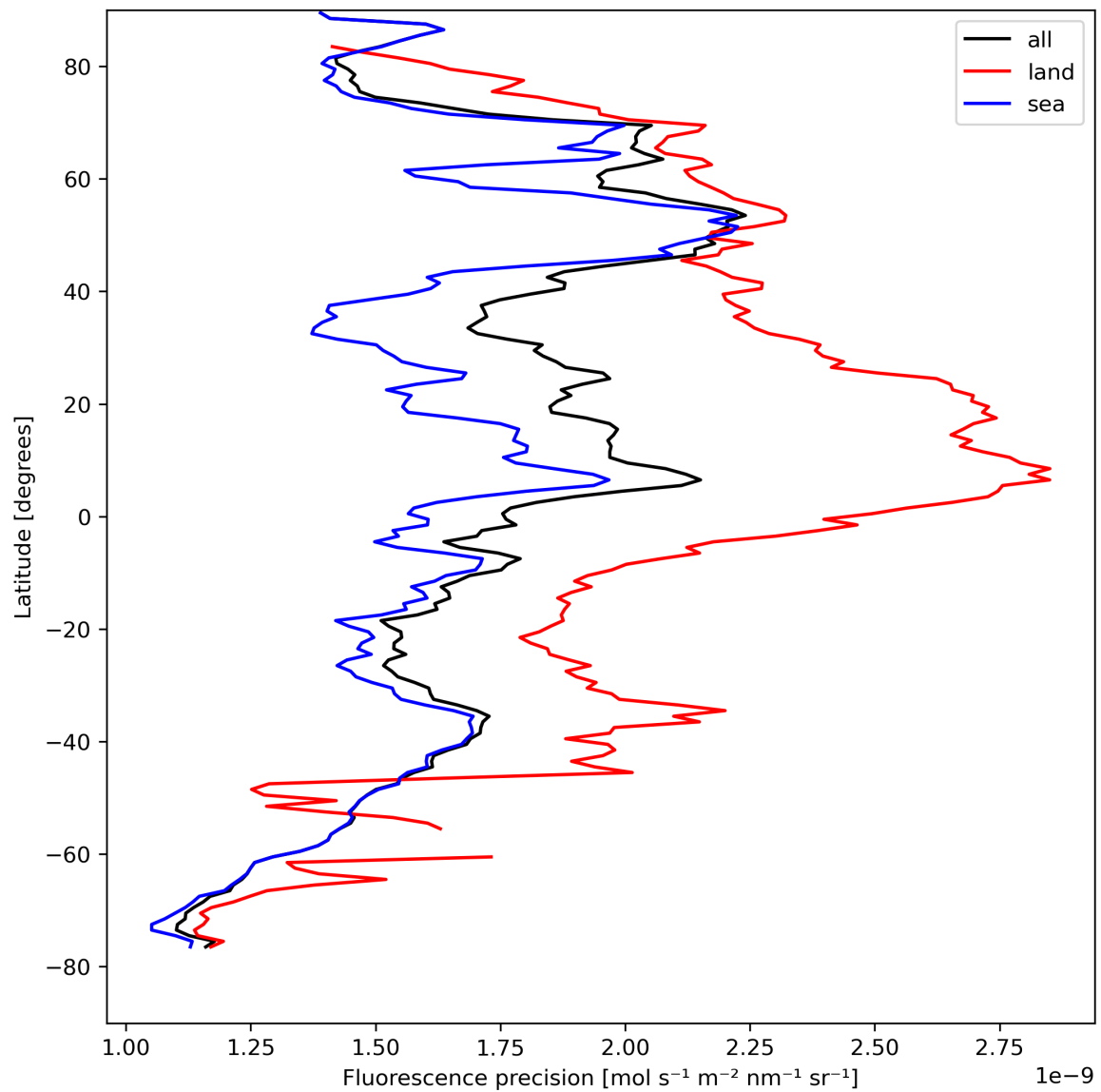
Figure 24: Zonal average of “Fluorescence precision” for 2024-08-22 to 2024-08-23.
