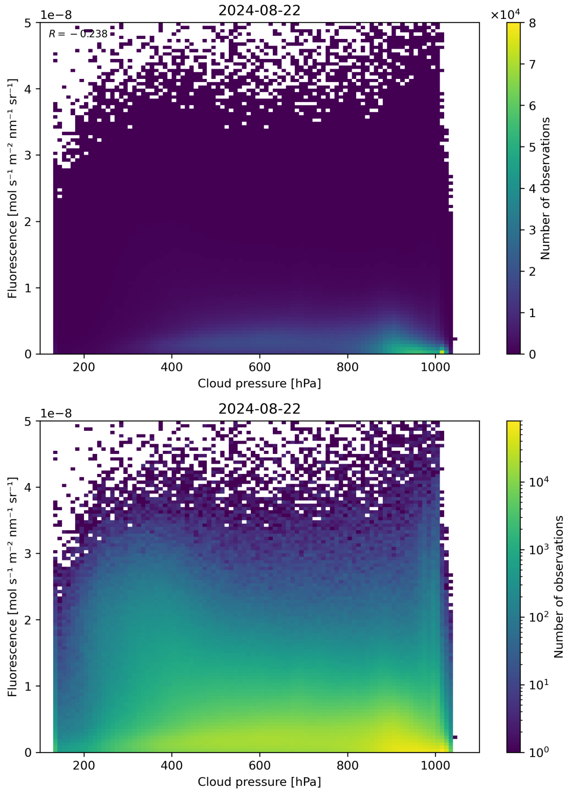
Figure 80: Scatter density plot of “Cloud pressure” against “Fluorescence” for 2024-08-22 to 2024-08-23.
