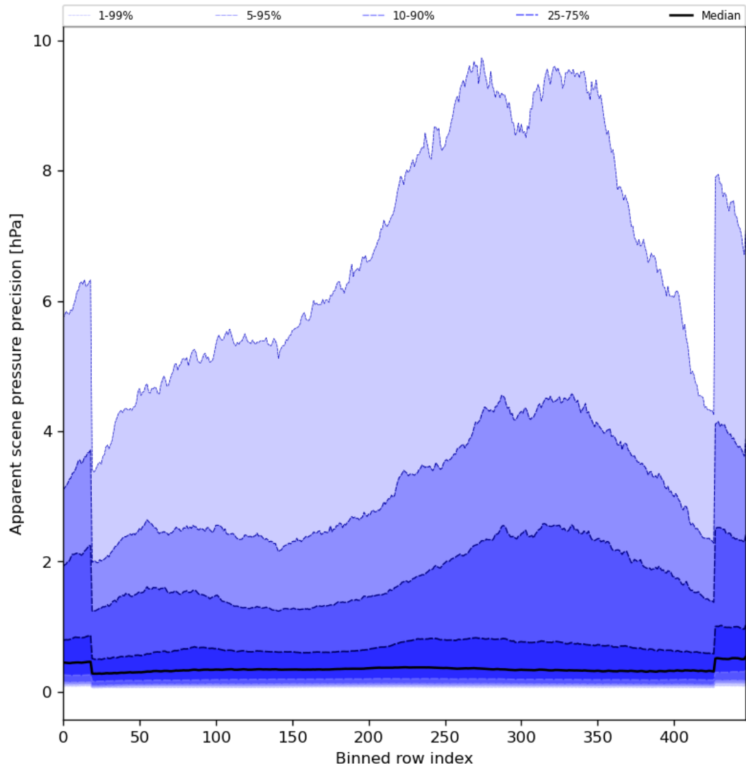
Figure 54: Along track statistics of “Apparent scene pressure precision” for 2024-08-22 to 2024-08-23
