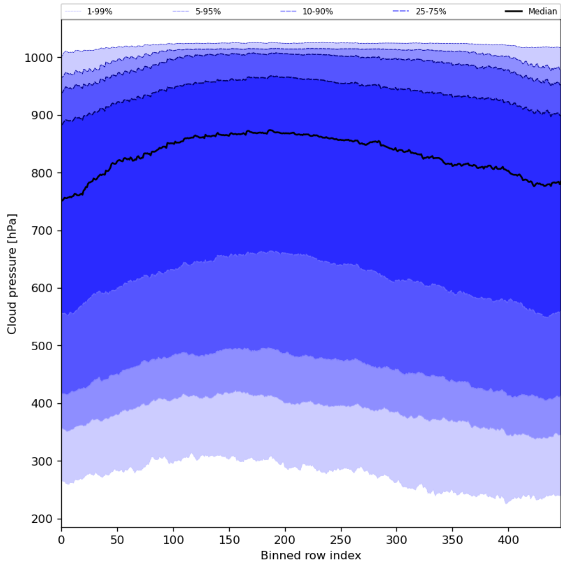
Figure 47: Along track statistics of “Cloud pressure” for 2024-08-22 to 2024-08-23
