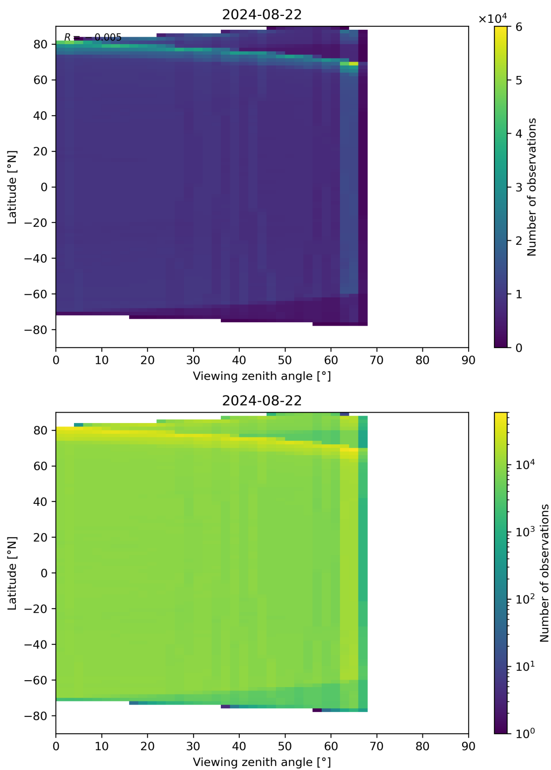
Figure 123: Scatter density plot of “Viewing zenith angle” against “Latitude” for 2024-08-22 to 2024-08-23.
