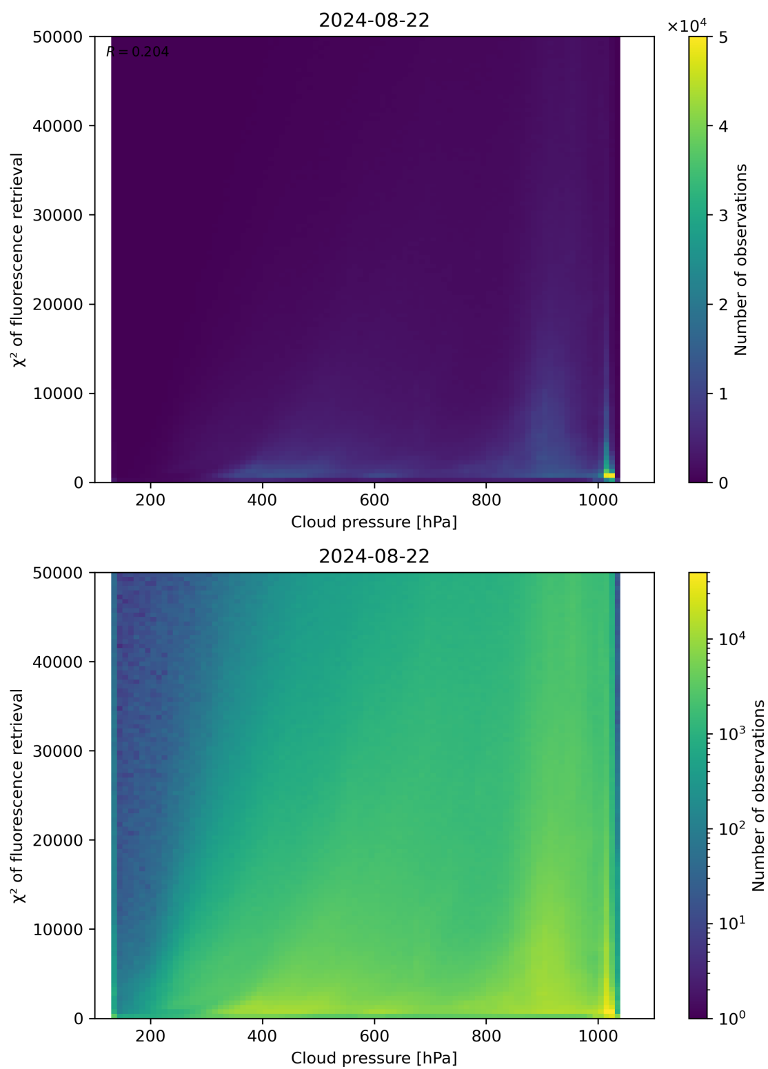
Figure 78: Scatter density plot of “Cloud pressure” against “ \chi^2 of fluorescence retrieval” for 2024-08-22 to 2024-08-23.
