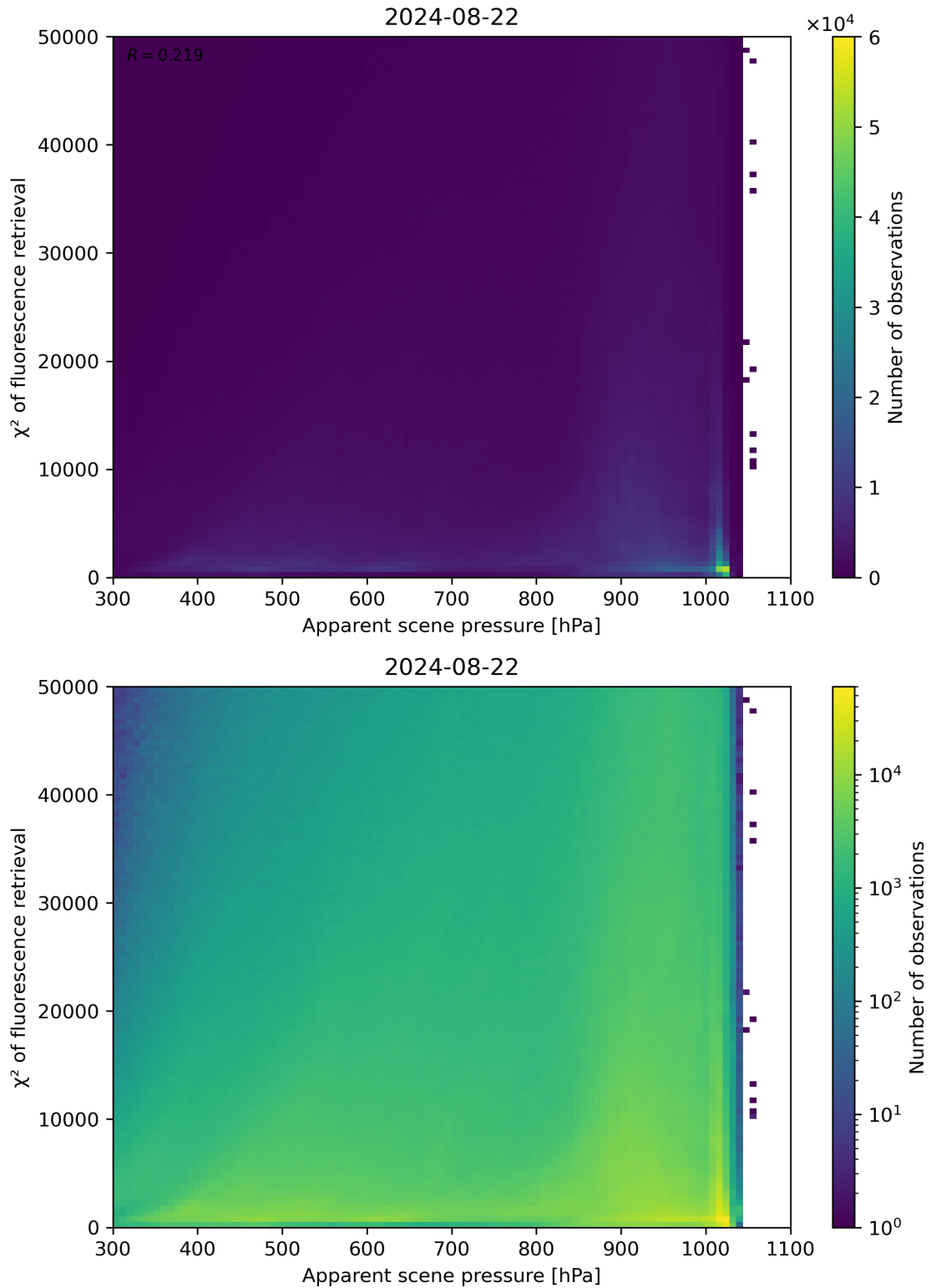
Figure 63: Scatter density plot of “Apparent scene pressure” against “ \chi^2 of fluorescence retrieval” for 2024-08-22 to 2024-08-23.
