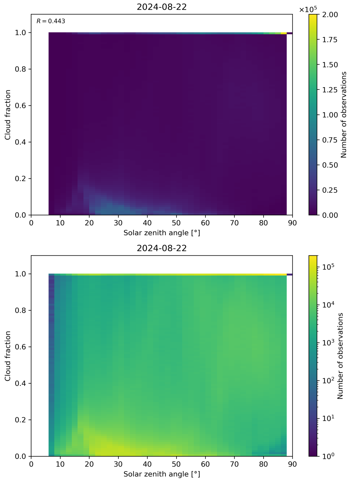
Figure 110: Scatter density plot of “Solar zenith angle” against “Cloud fraction” for 2024-08-22 to 2024-08-23.
