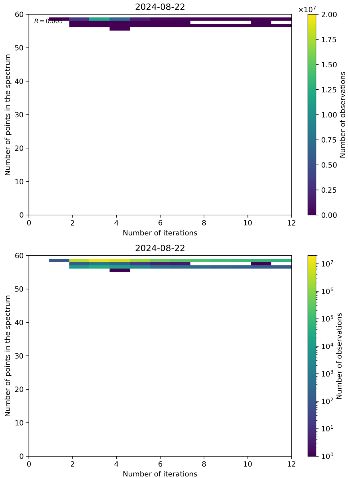
Figure 99: Scatter density plot of “Number of iterations” against “Number of points in the spectrum” for 2024-08-22 to 2024-08-23.
