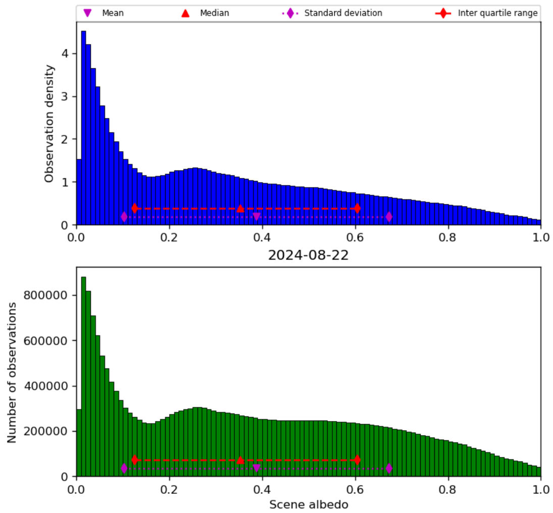
Figure 34: Histogram of “Scene albedo” for 2024-08-22 to 2024-08-23
