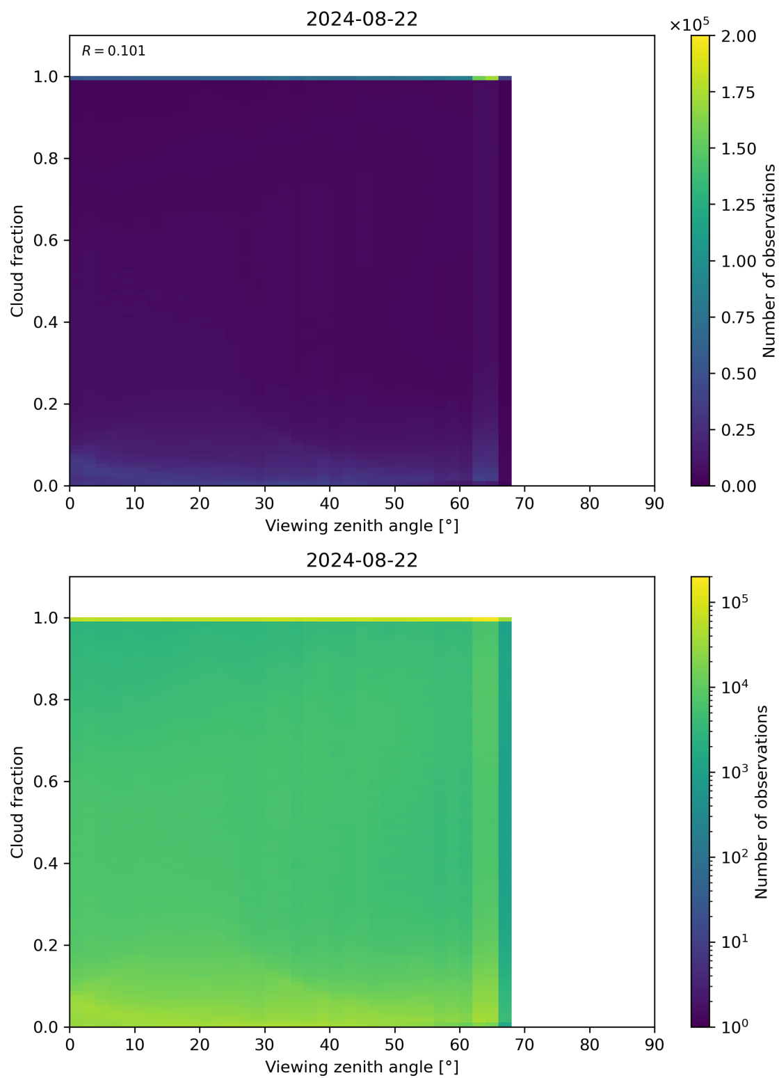
Figure 120: Scatter density plot of “Viewing zenith angle” against “Cloud fraction” for 2024-08-22 to 2024-08-23.
