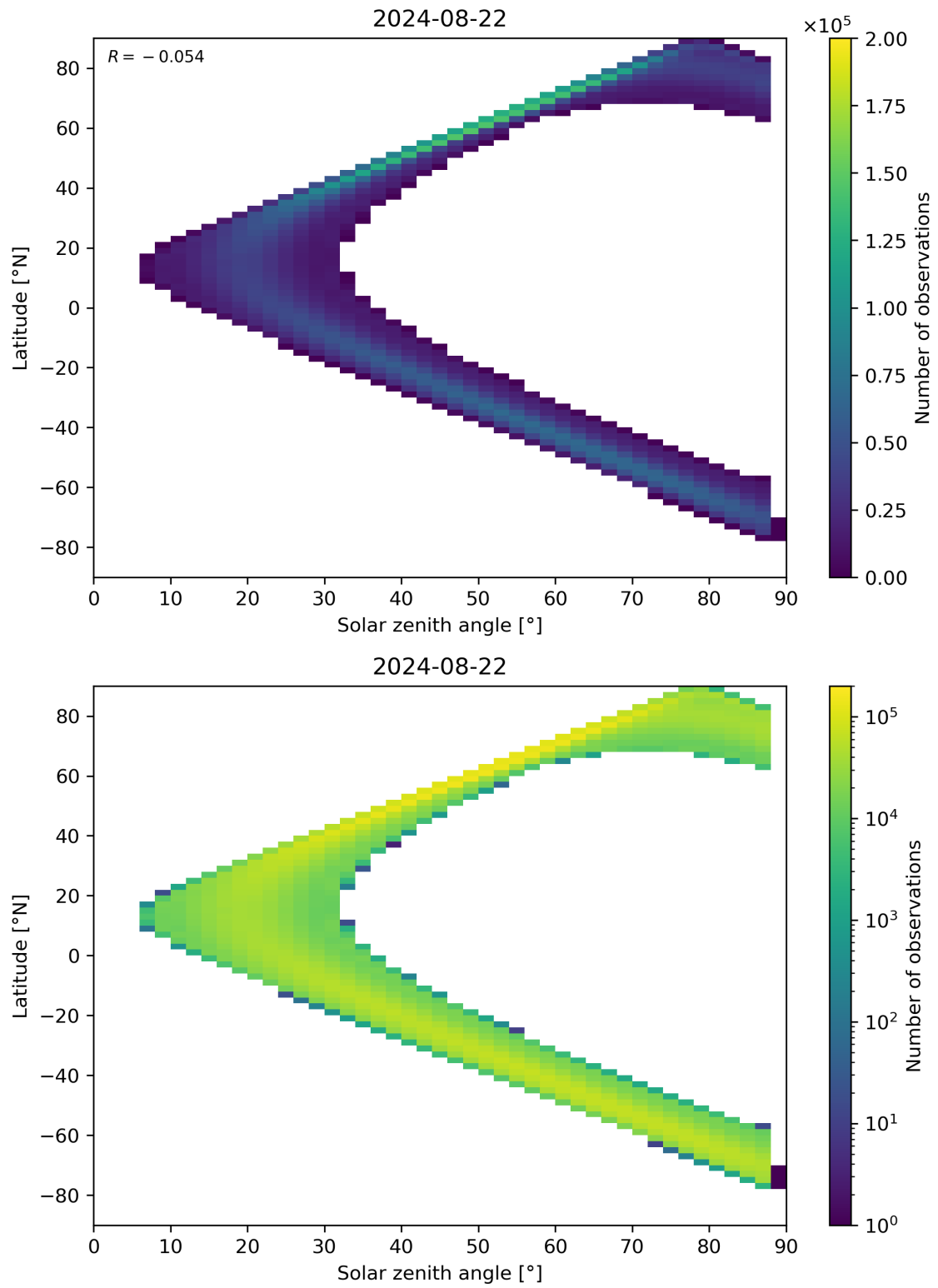
Figure 113: Scatter density plot of “Solar zenith angle” against “Latitude” for 2024-08-22 to 2024-08-23.
