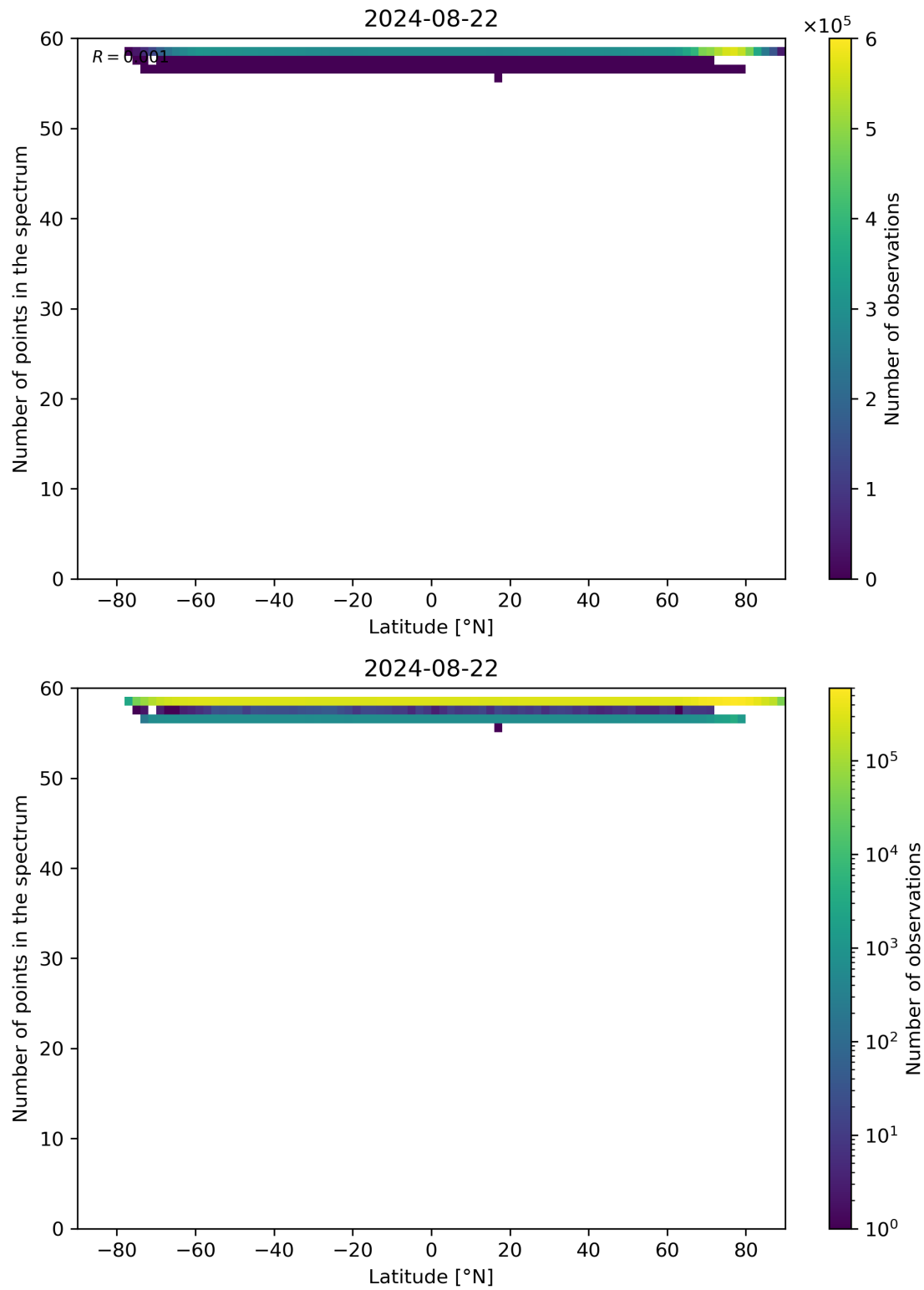
Figure 94: Scatter density plot of “Latitude” against “Number of points in the spectrum” for 2024-08-22 to 2024-08-23.
