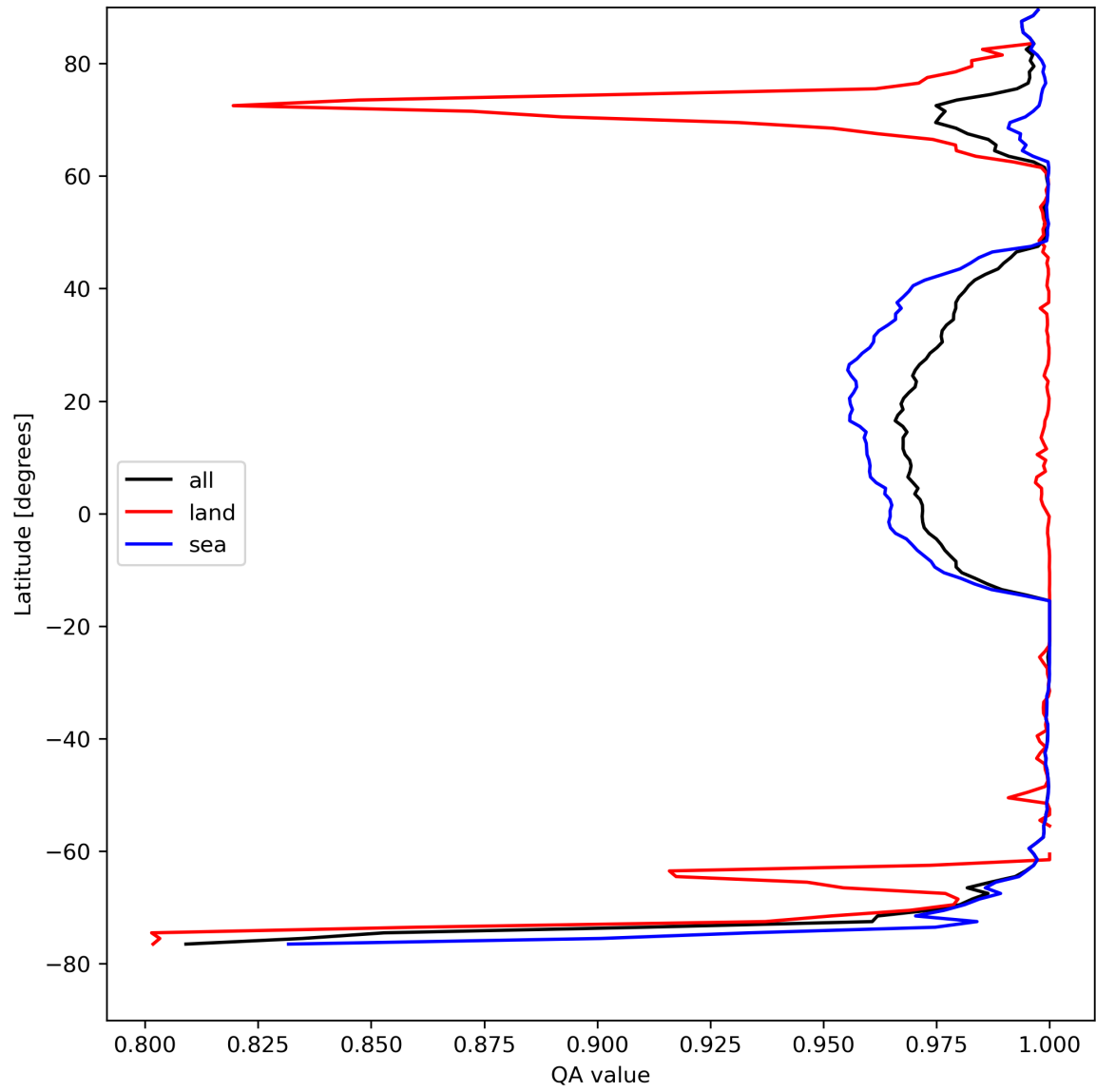
Figure 12: Zonal average of “QA value” for 2024-08-22 to 2024-08-23.
