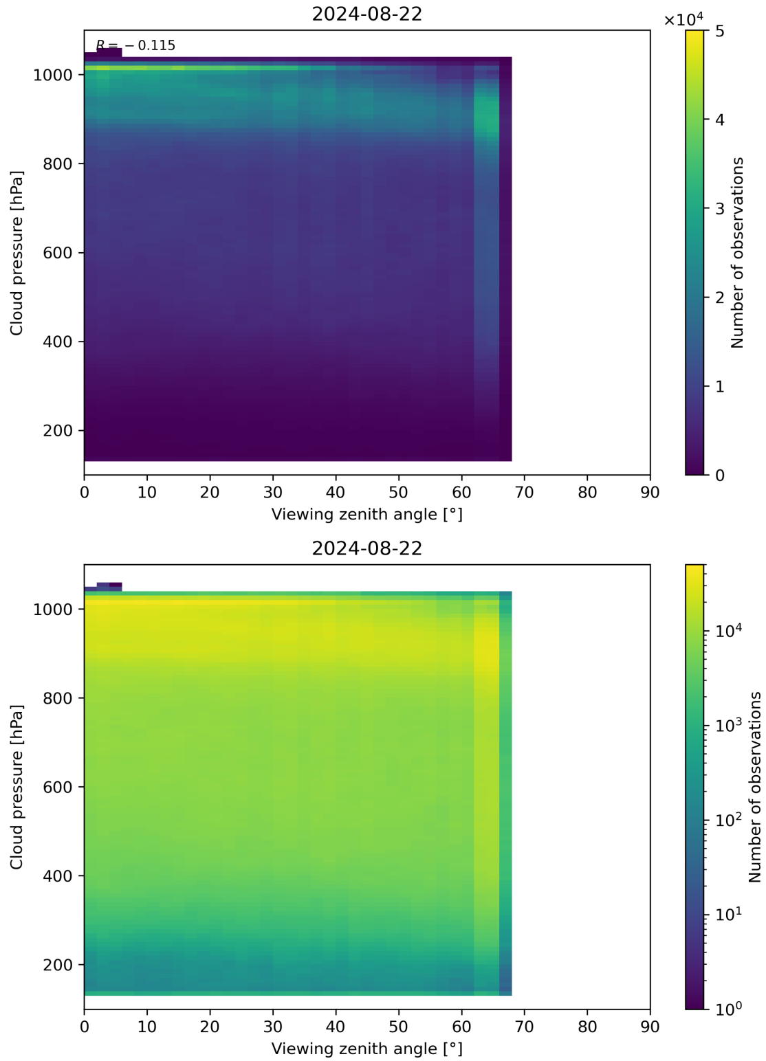
Figure 121: Scatter density plot of “Viewing zenith angle” against “Cloud pressure” for 2024-08-22 to 2024-08-23.
