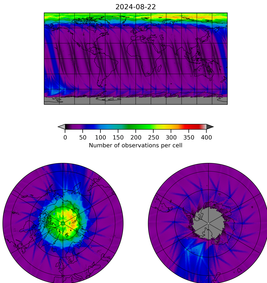
Figure 11: Map of the number of observations for 2024-08-22 to 2024-08-23
