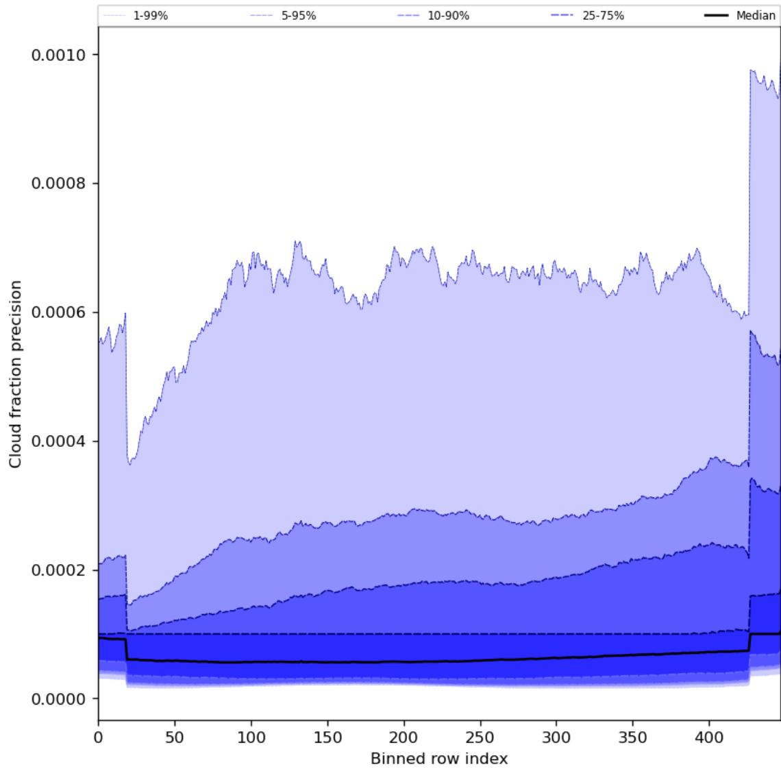
Figure 50: Along track statistics of “Cloud fraction precision” for 2024-08-22 to 2024-08-23
