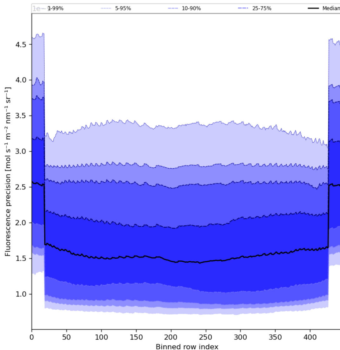
Figure 58: Along track statistics of “Fluorescence precision” for 2024-08-22 to 2024-08-23
