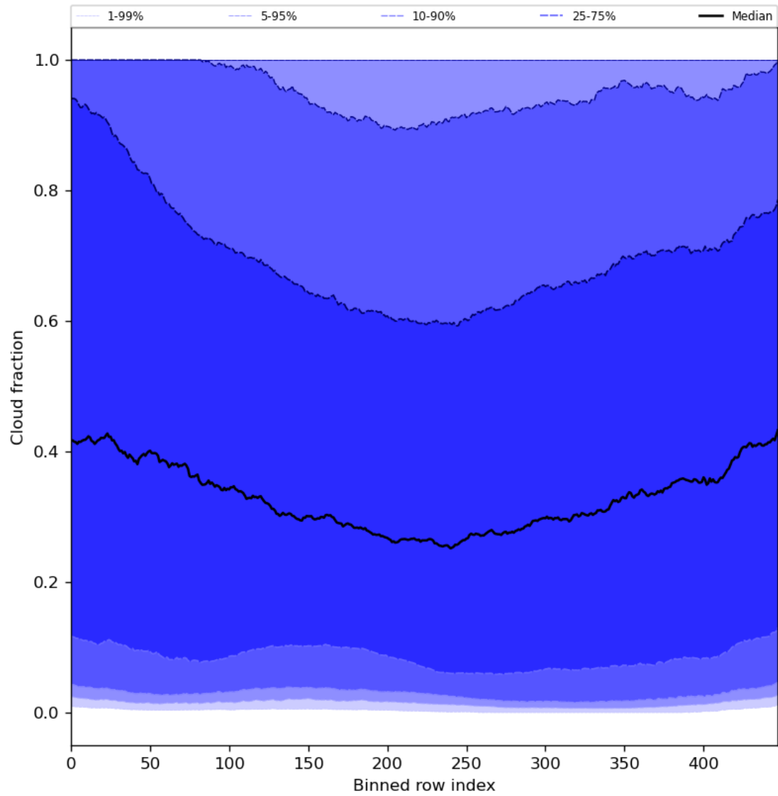
Figure 49: Along track statistics of “Cloud fraction” for 2024-08-22 to 2024-08-23
