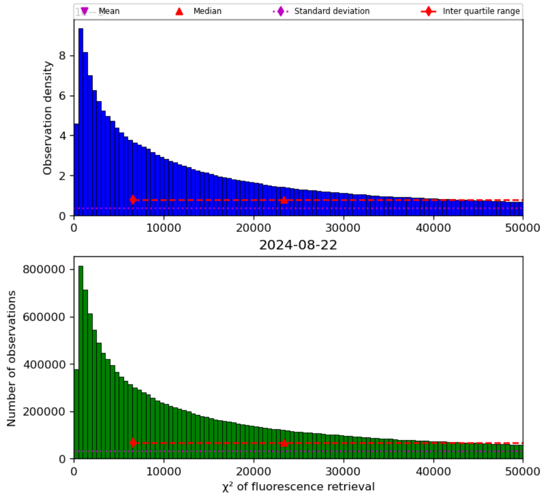
Figure 42: Histogram of “ \chi^2 of fluorescence retrieval” for 2024-08-22 to 2024-08-23
