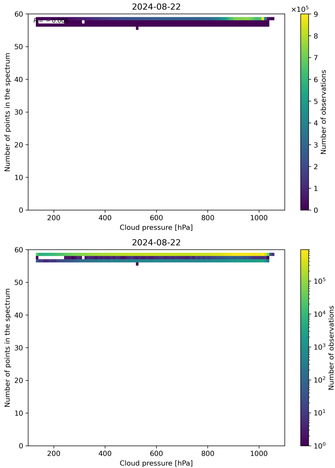
Figure 82: Scatter density plot of “Cloud pressure” against “Number of points in the spectrum” for 2024-08-22 to 2024-08-23.
