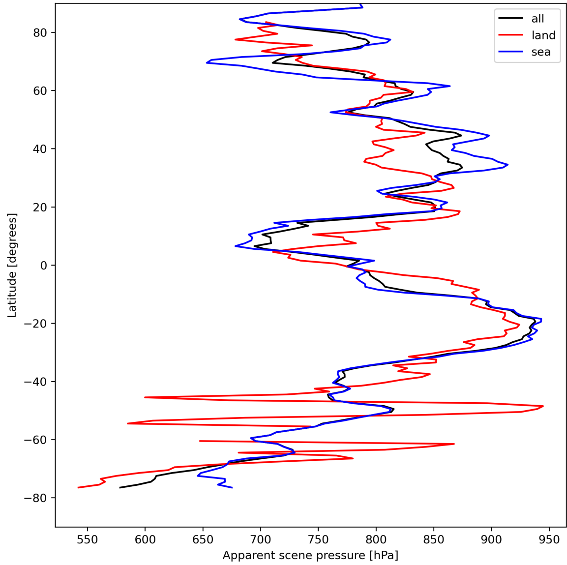
Figure 19: Zonal average of “Apparent scene pressure” for 2024-08-22 to 2024-08-23.
