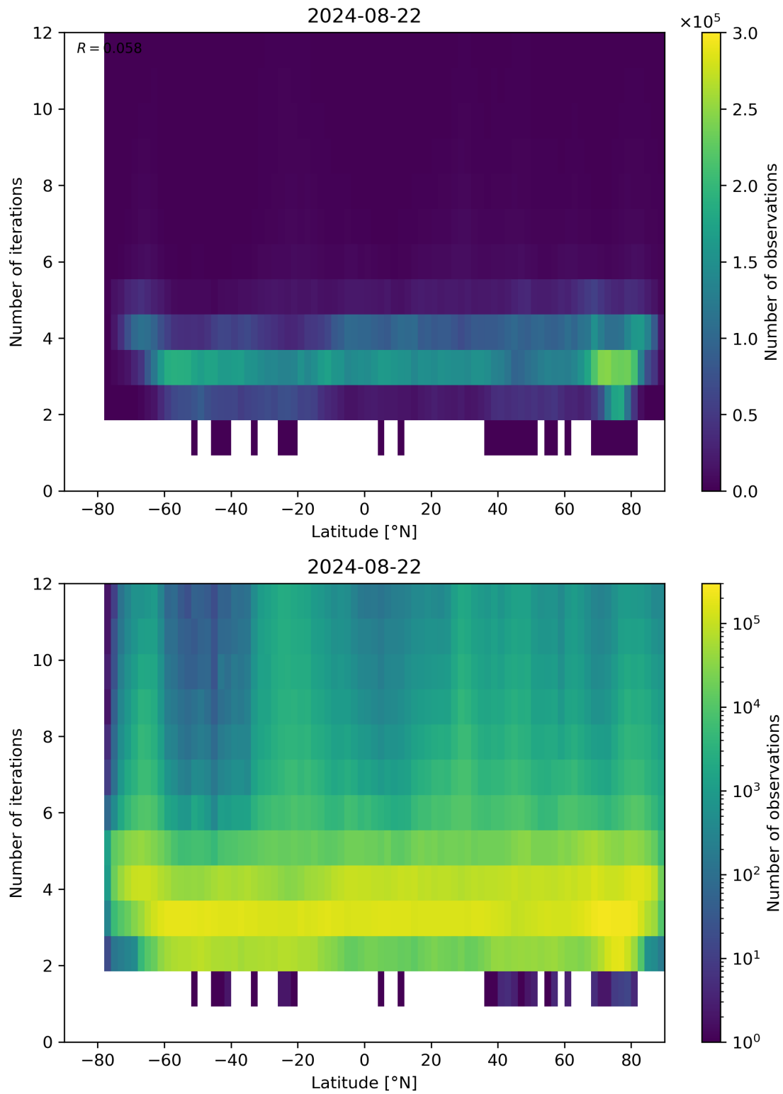
Figure 93: Scatter density plot of “Latitude” against “Number of iterations” for 2024-08-22 to 2024-08-23.
