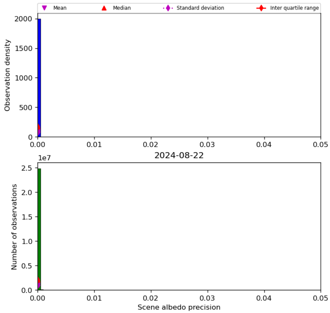
Figure 35: Histogram of “Scene albedo precision” for 2024-08-22 to 2024-08-23
