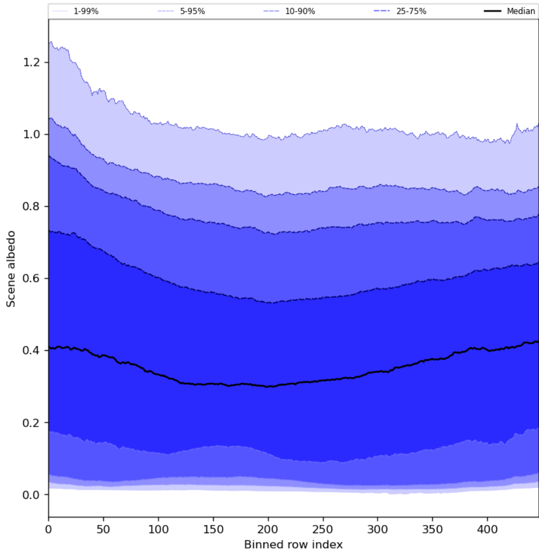
Figure 51: Along track statistics of “Scene albedo” for 2024-08-22 to 2024-08-24
