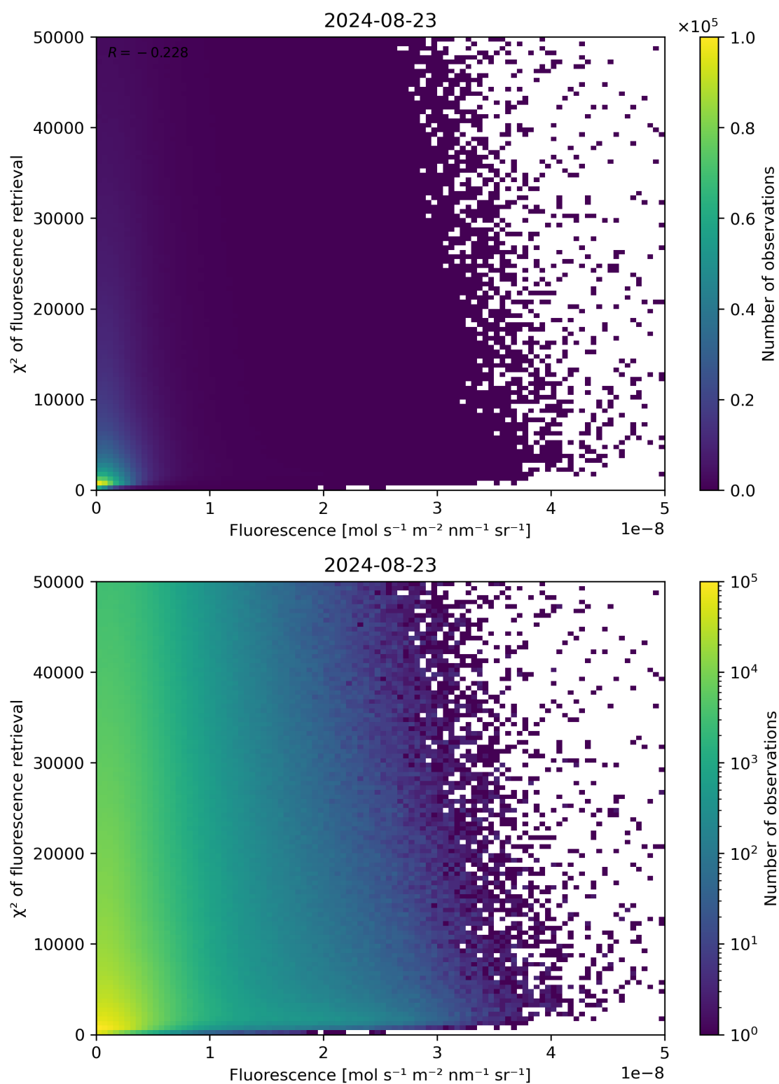
Figure 85: Scatter density plot of “Fluorescence” against “ \chi^2 of fluorescence retrieval” for 2024-08-22 to 2024-08-24.
