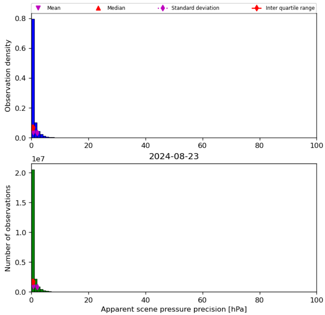
Figure 37: Histogram of “Apparent scene pressure precision” for 2024-08-22 to 2024-08-24
