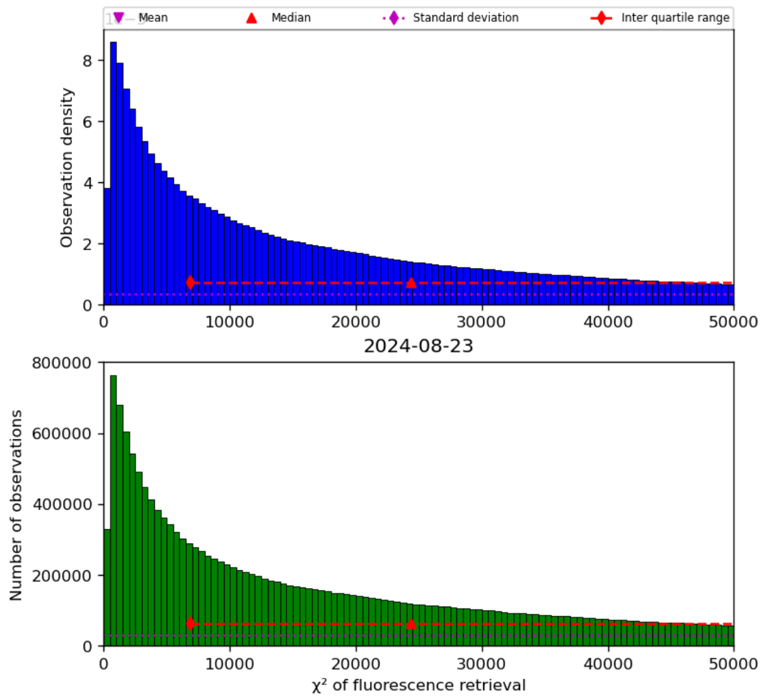
Figure 42: Histogram of “ \chi^2 of fluorescence retrieval” for 2024-08-22 to 2024-08-24
