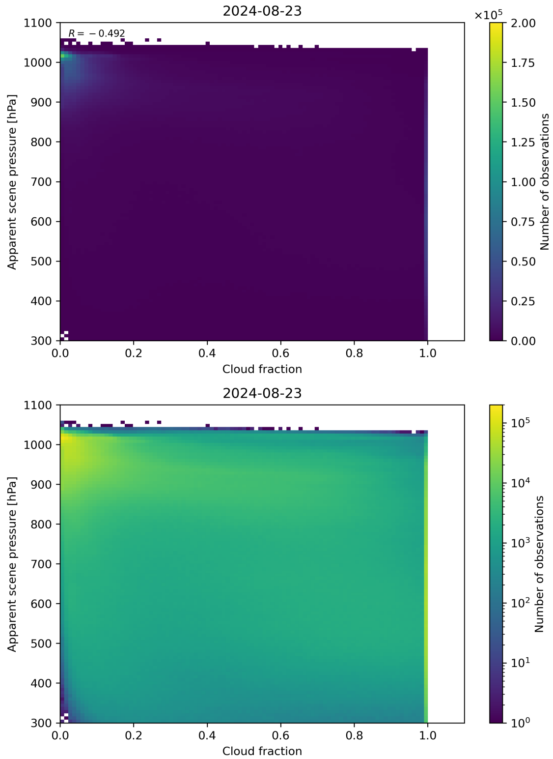
Figure 70: Scatter density plot of “Cloud fraction” against “Apparent scene pressure” for 2024-08-22 to 2024-08-24.
