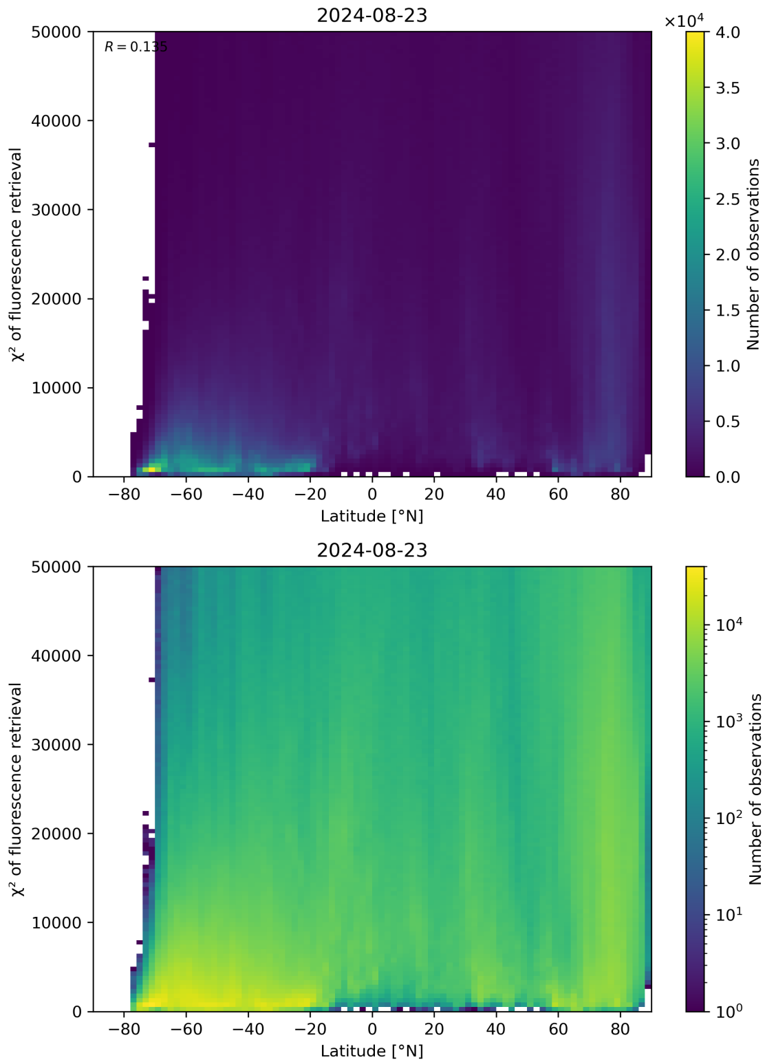
Figure 89: Scatter density plot of “Latitude” against “ \chi^2 of fluorescence retrieval” for 2024-08-22 to 2024-08-24.
