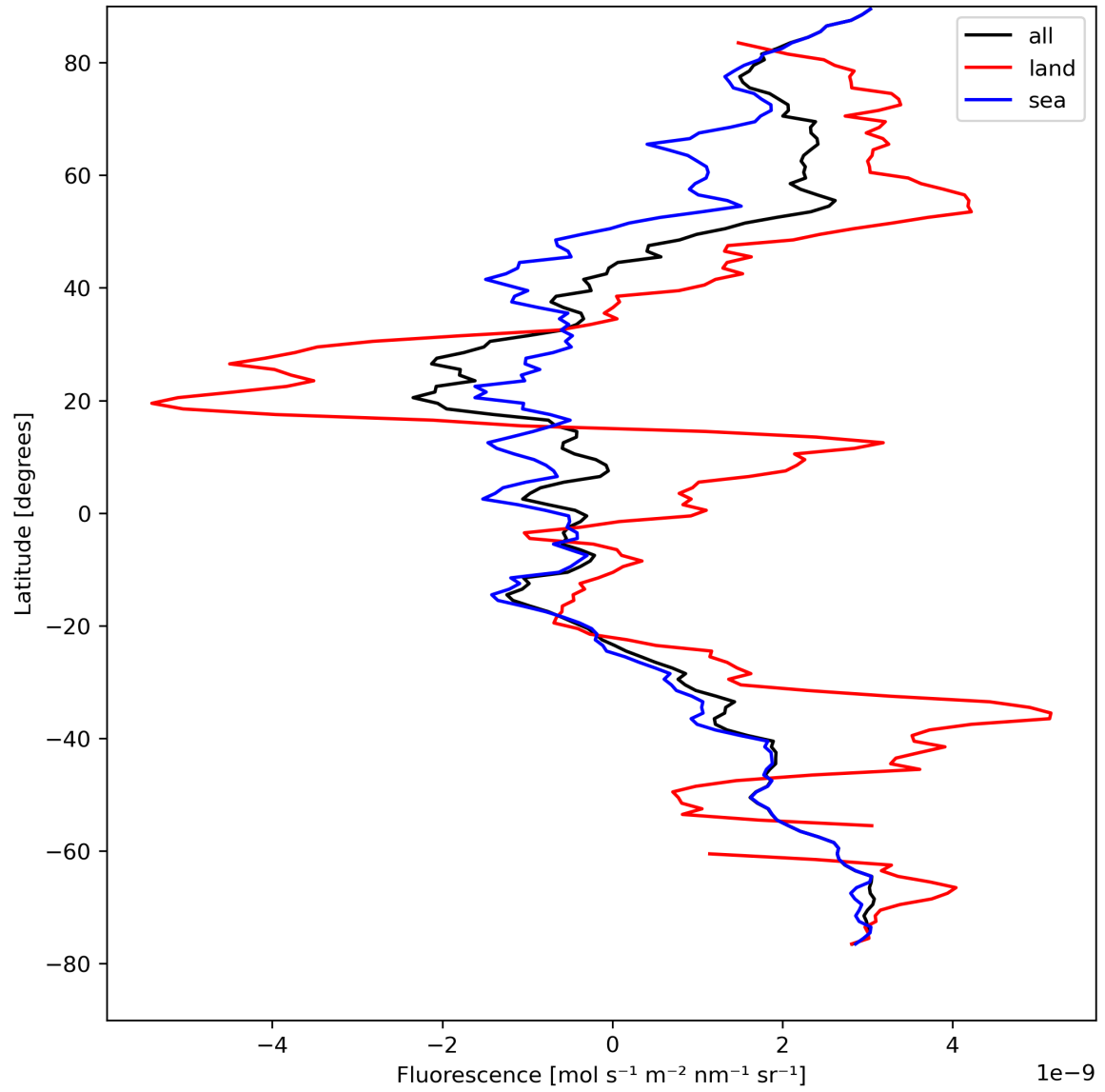
Figure 23: Zonal average of “Fluorescence” for 2024-08-22 to 2024-08-24.
