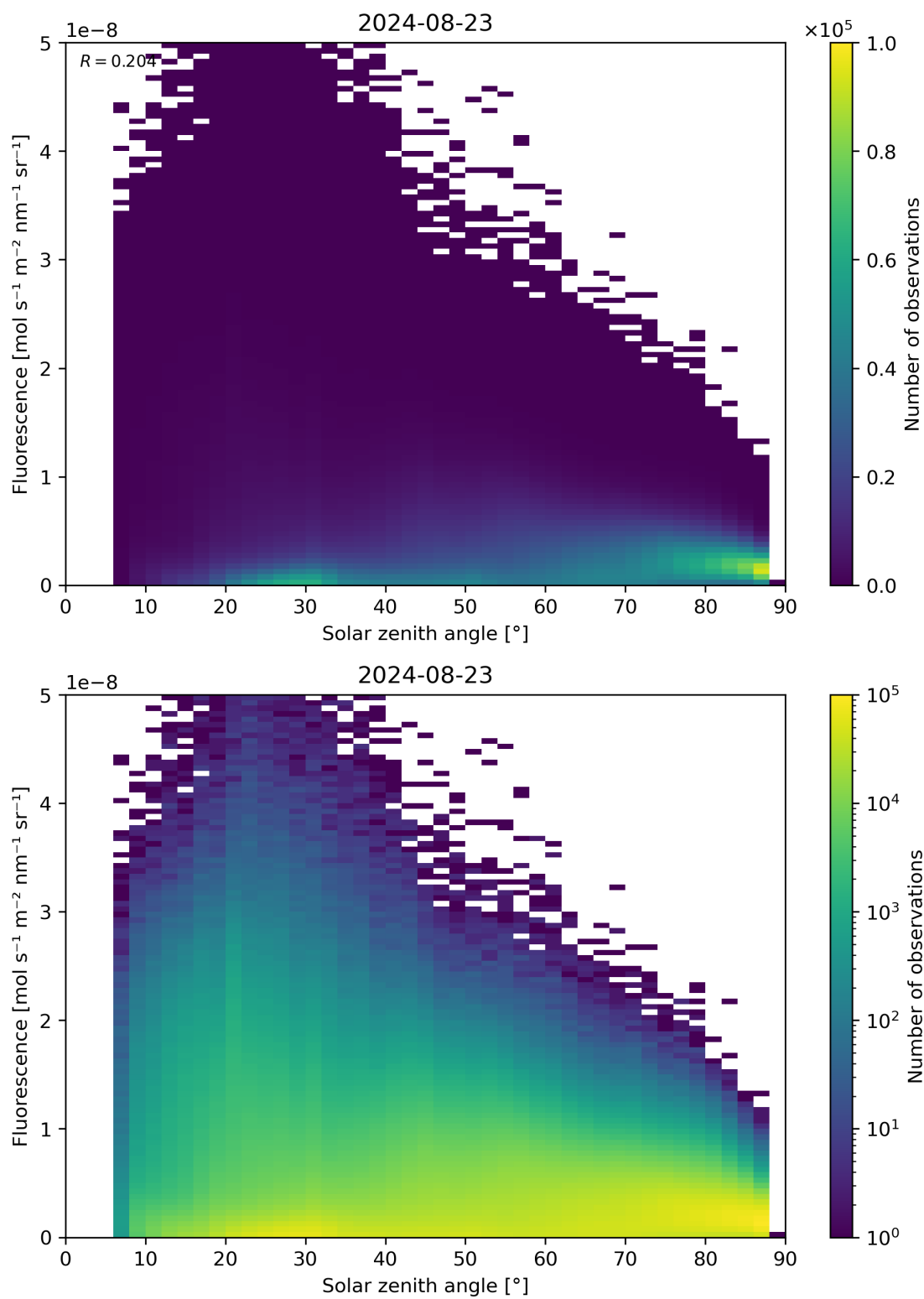
Figure 112: Scatter density plot of “Solar zenith angle” against “Fluorescence” for 2024-08-22 to 2024-08-24.
