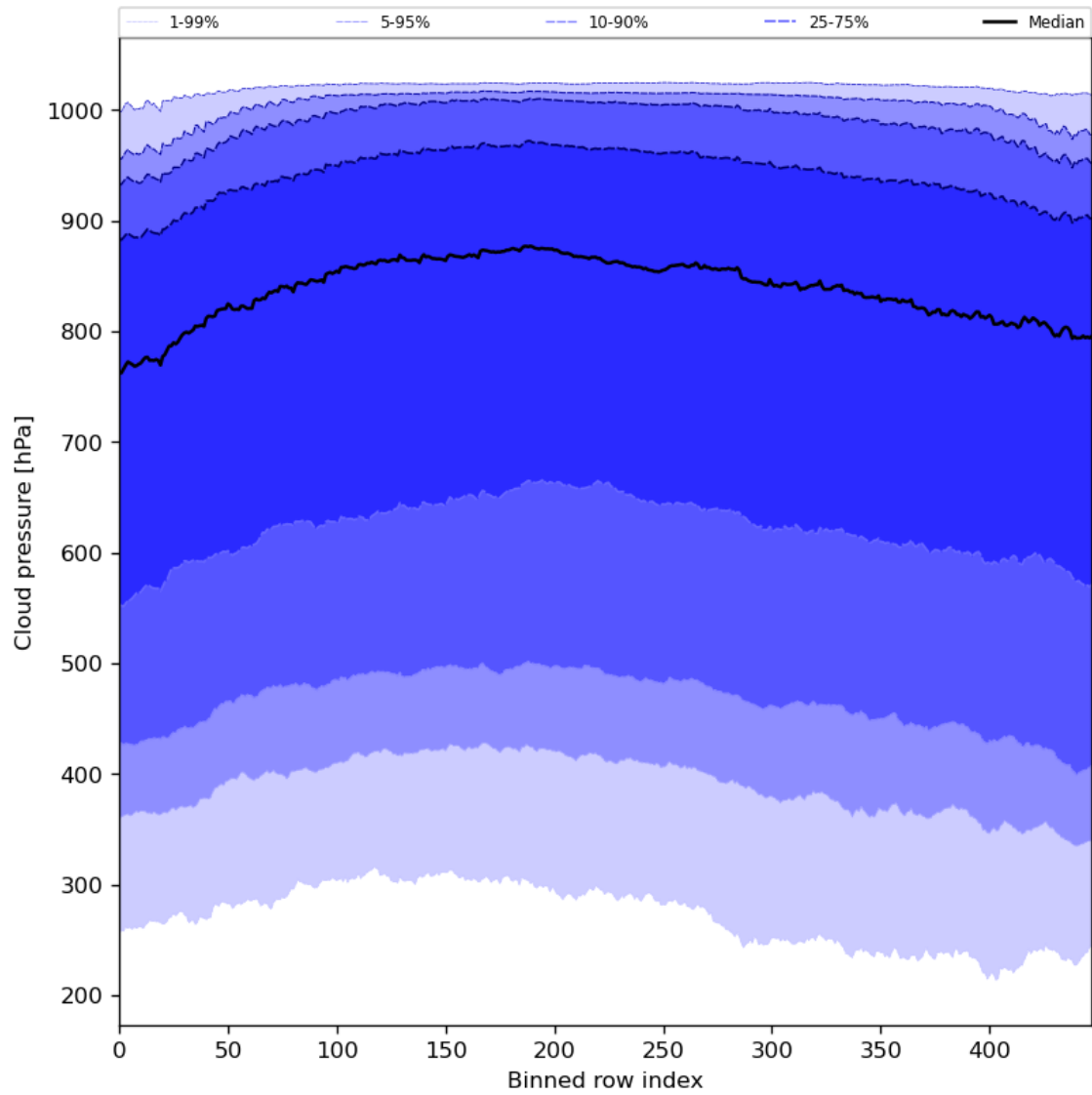
Figure 47: Along track statistics of “Cloud pressure” for 2024-08-22 to 2024-08-24
