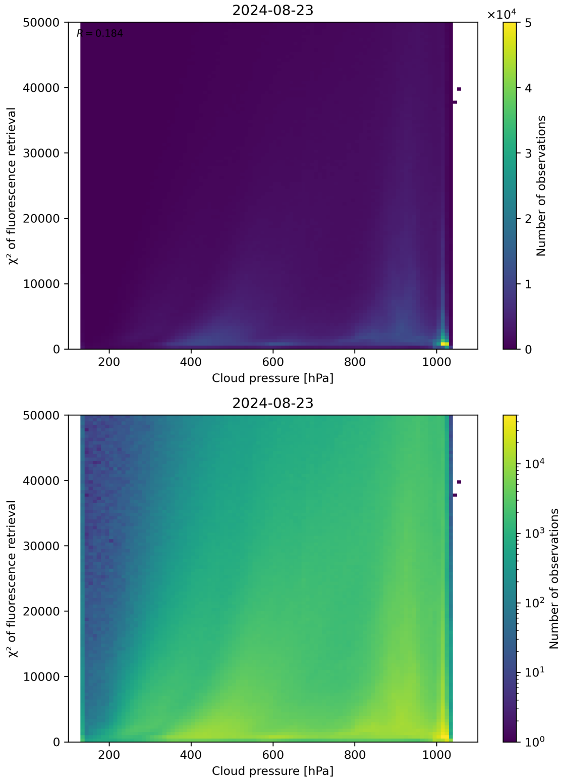
Figure 78: Scatter density plot of “Cloud pressure” against “ \chi^2 of fluorescence retrieval” for 2024-08-22 to 2024-08-24.
