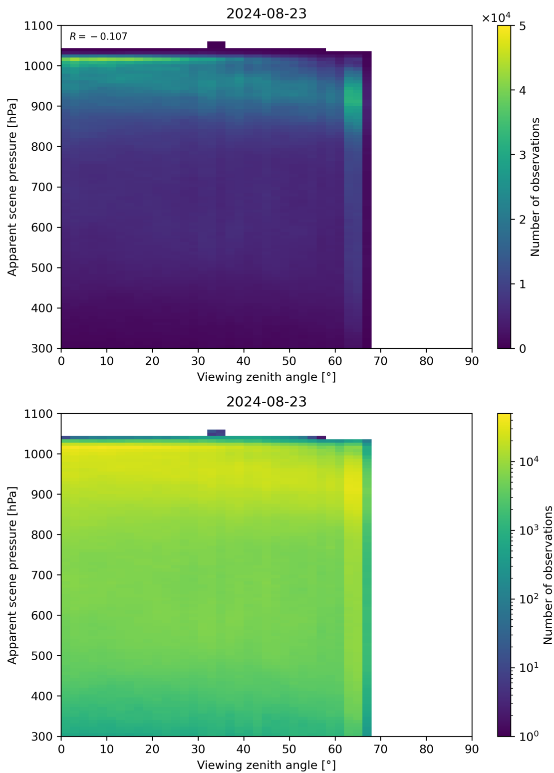
Figure 118: Scatter density plot of “Viewing zenith angle” against “Apparent scene pressure” for 2024-08-22 to 2024-08-24.
