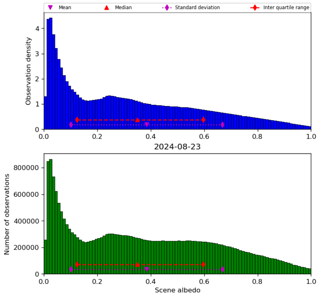
Figure 34: Histogram of “Scene albedo” for 2024-08-22 to 2024-08-24
