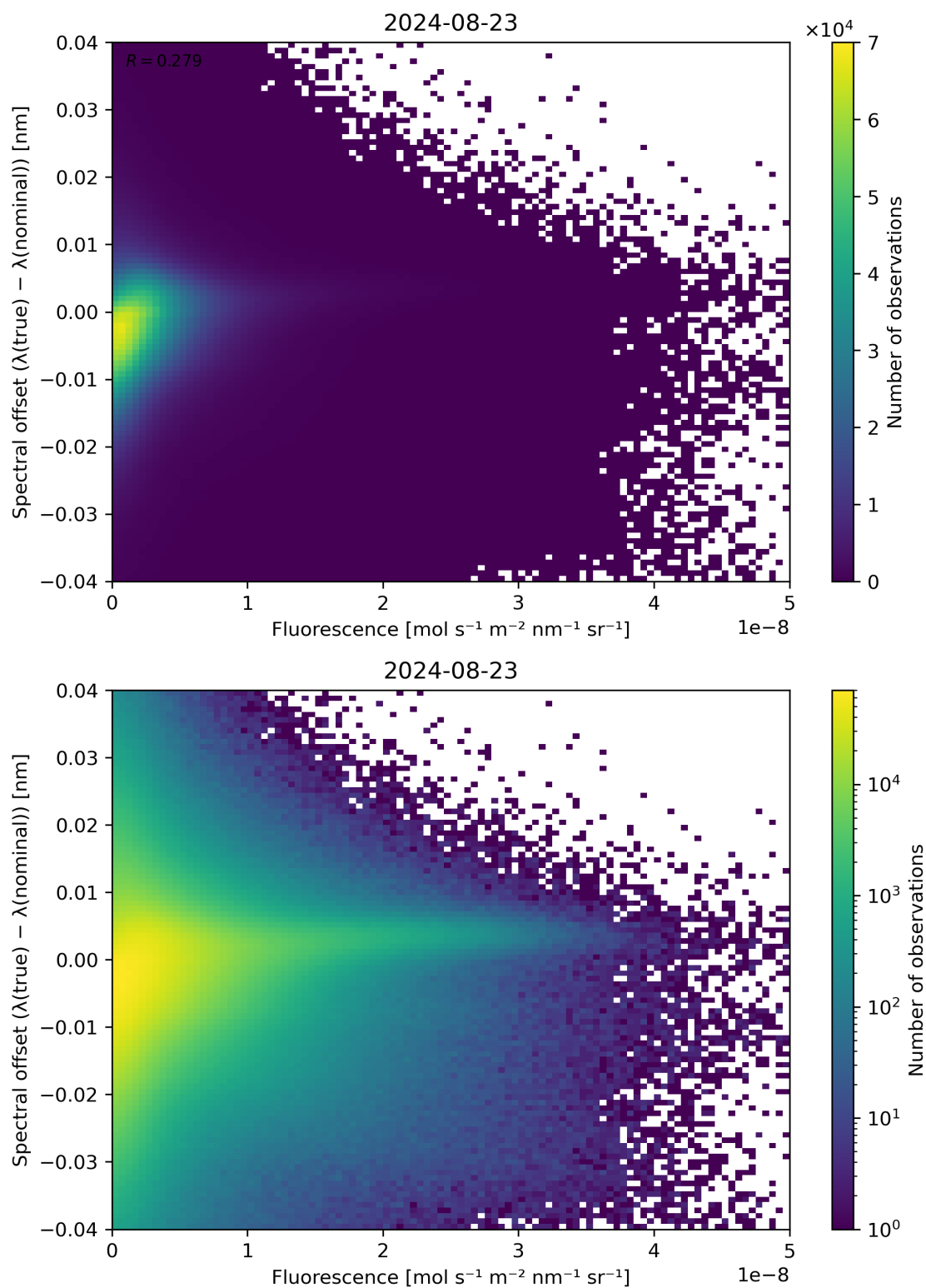
Figure 87: Scatter density plot of “Fluorescence” against “Spectral offset ( \lambda(\text{true}) - \lambda(\text{nominal}) )” for 2024-08-22 to 2024-08-24.
