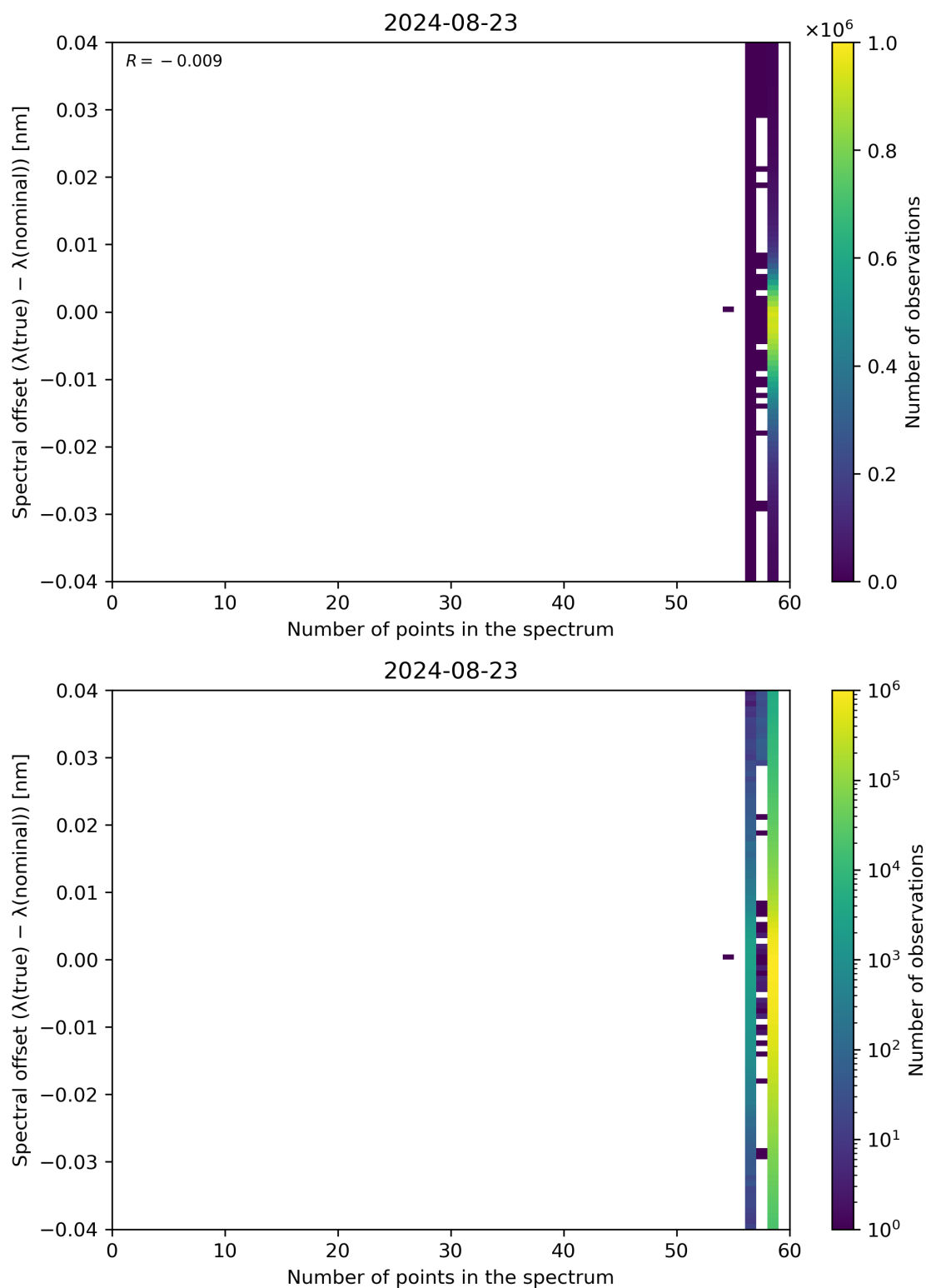
Figure 101: Scatter density plot of “Number of points in the spectrum” against “Spectral offset ( \lambda(\text{true}) - \lambda(\text{nominal}) )” for 2024-08-22 to 2024-08-24.
