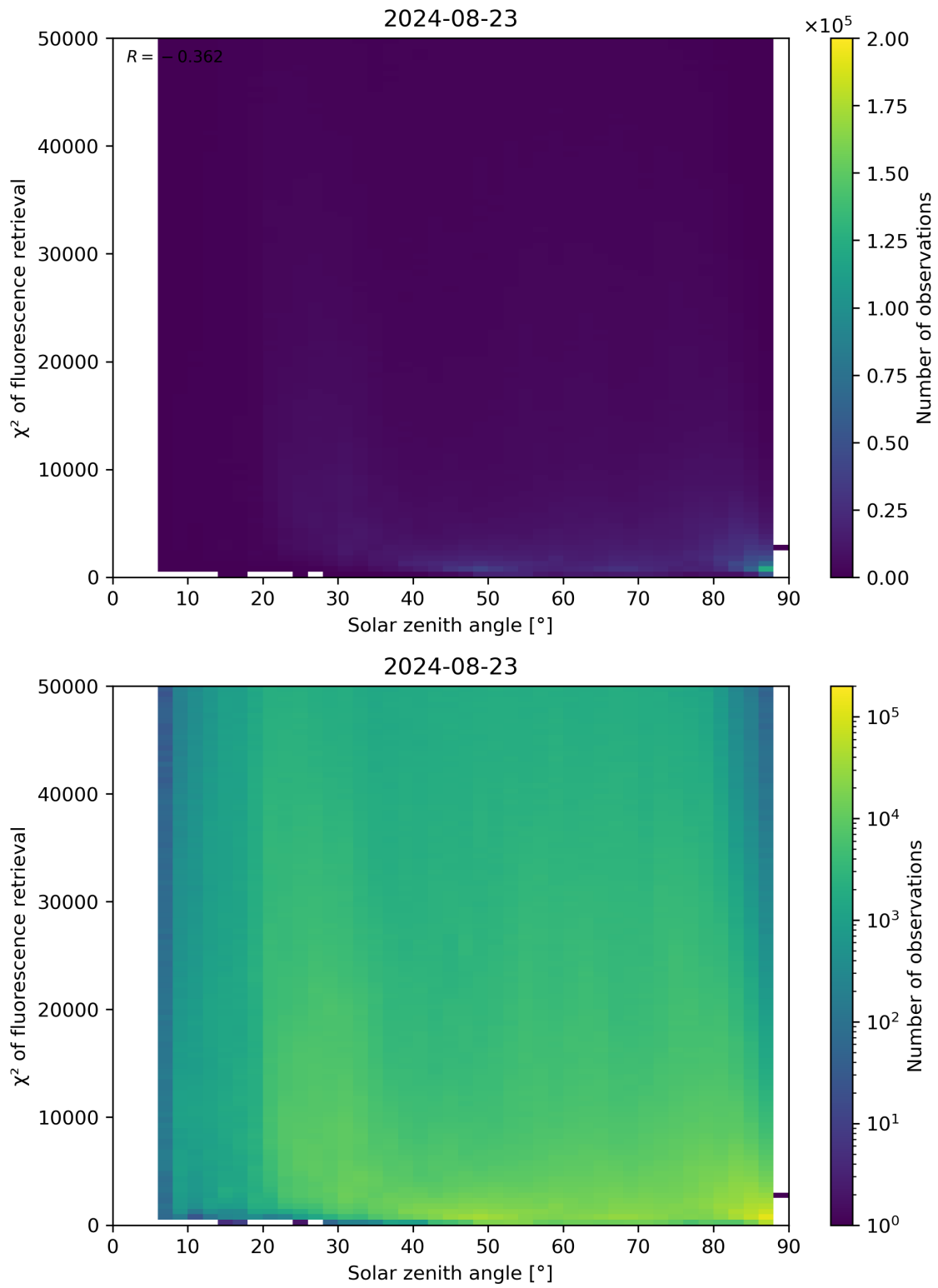
Figure 109: Scatter density plot of “Solar zenith angle” against “ \chi^2 of fluorescence retrieval” for 2024-08-22 to 2024-08-24.
