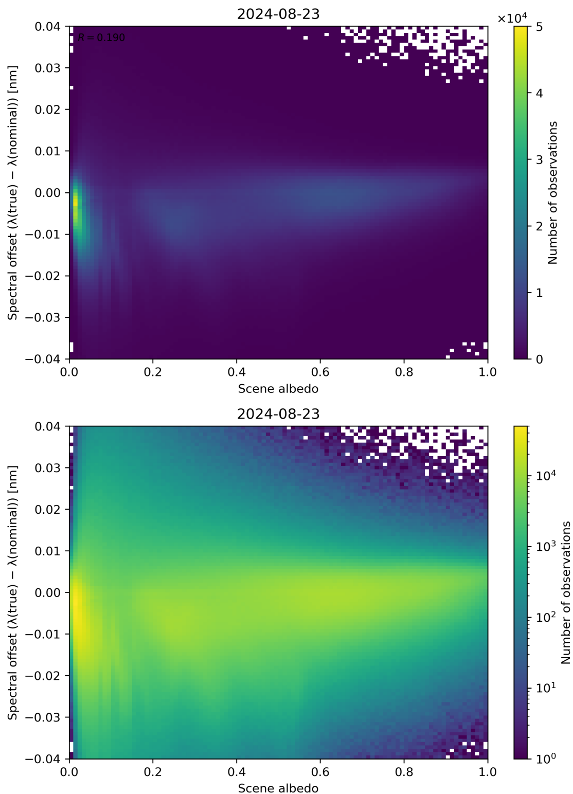
Figure 107: Scatter density plot of “Scene albedo” against “Spectral offset ( \lambda(\text{true}) - \lambda(\text{nominal}) )” for 2024-08-22 to 2024-08-24.
