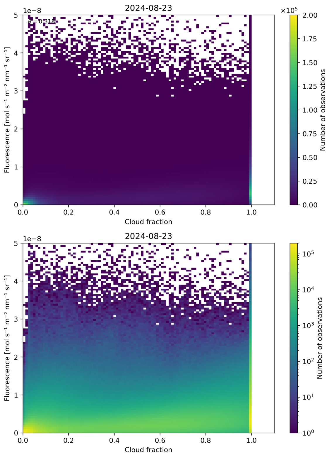
Figure 72: Scatter density plot of “Cloud fraction” against “Fluorescence” for 2024-08-22 to 2024-08-24.
