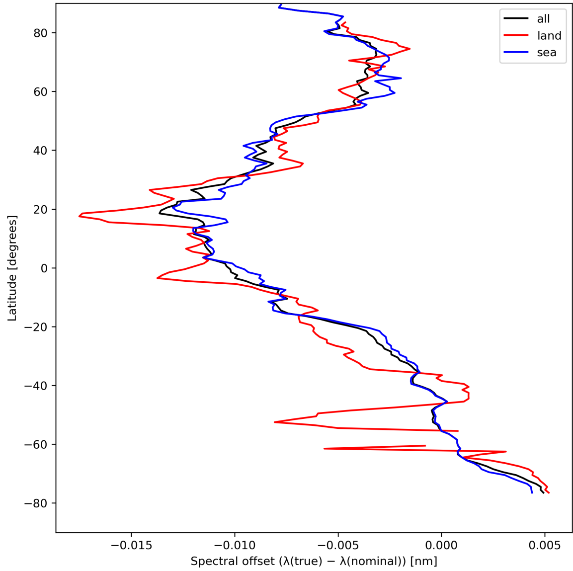
Figure 28: Zonal average of “Spectral offset ( \lambda(\text{true}) - \lambda(\text{nominal}) )” for 2024-08-22 to 2024-08-24.
