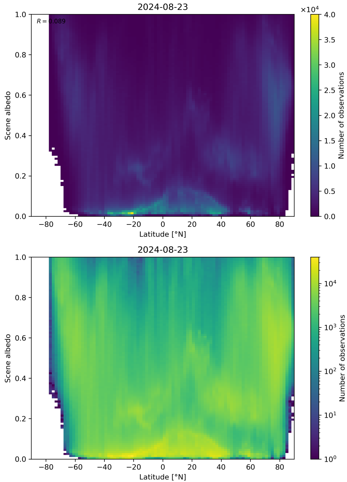
Figure 95: Scatter density plot of “Latitude” against “Scene albedo” for 2024-08-22 to 2024-08-24.
