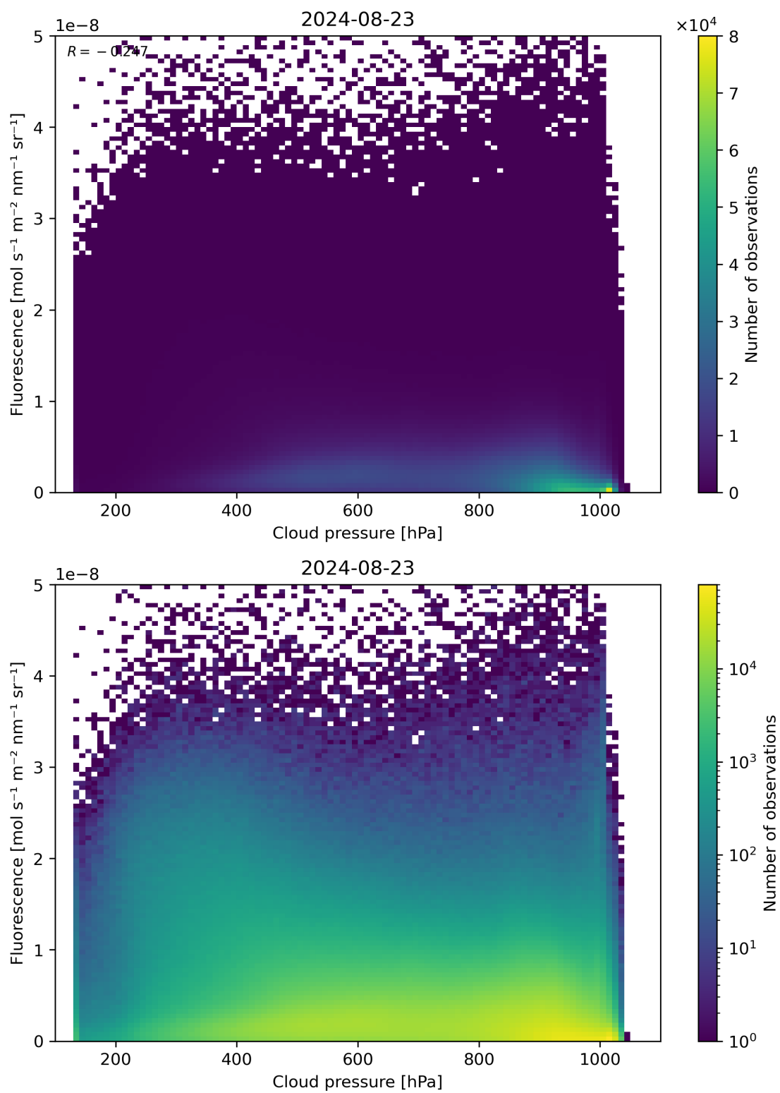
Figure 80: Scatter density plot of “Cloud pressure” against “Fluorescence” for 2024-08-22 to 2024-08-24.
