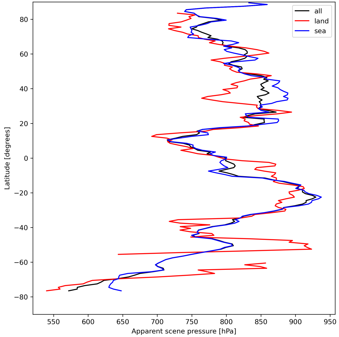
Figure 19: Zonal average of “Apparent scene pressure” for 2024-08-22 to 2024-08-24.
