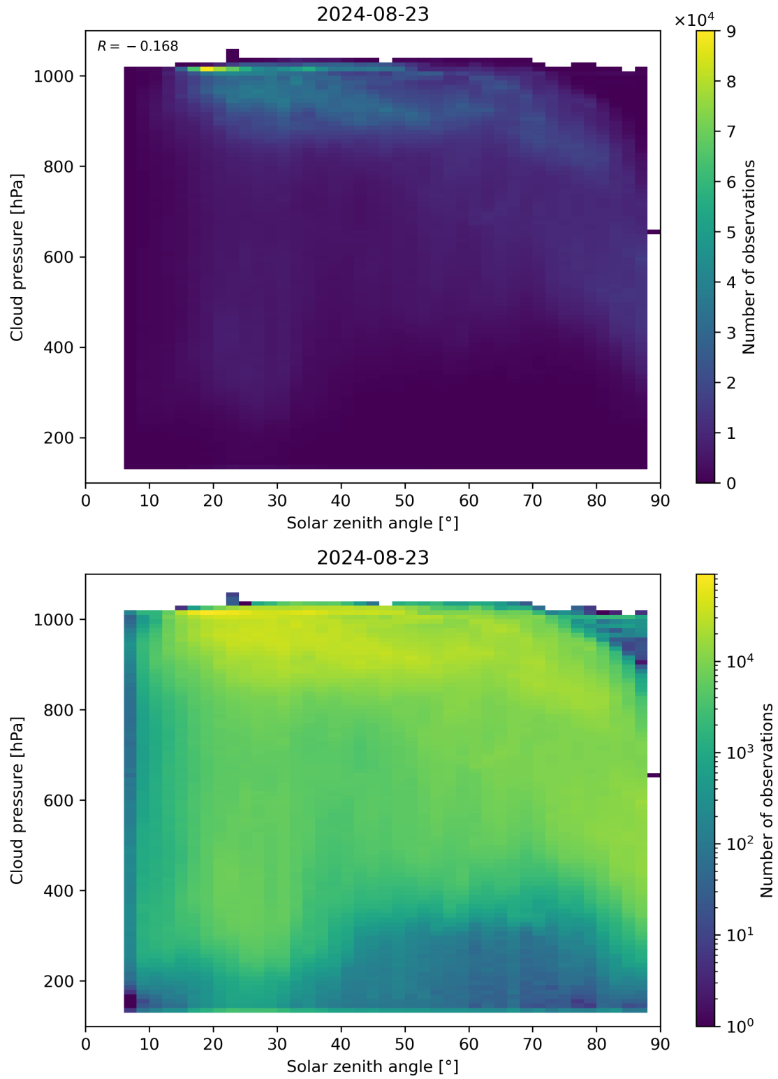
Figure 111: Scatter density plot of “Solar zenith angle” against “Cloud pressure” for 2024-08-22 to 2024-08-24.
