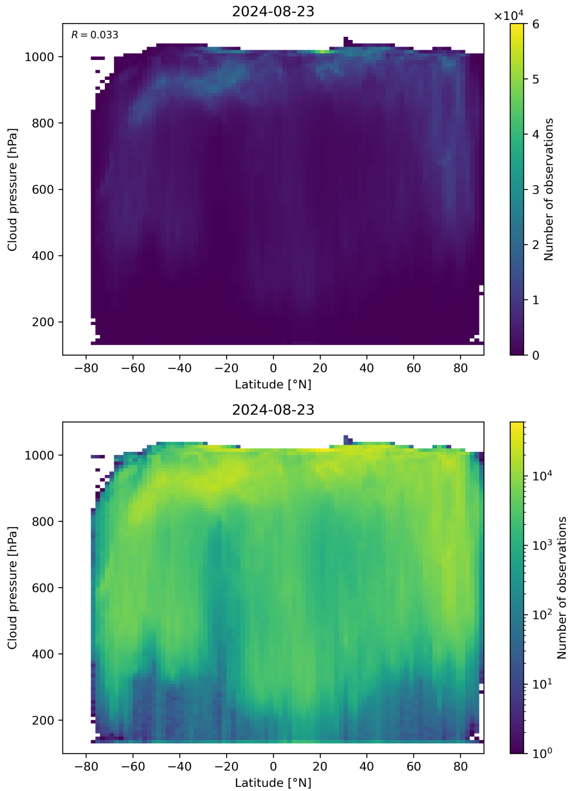
Figure 91: Scatter density plot of “Latitude” against “Cloud pressure” for 2024-08-22 to 2024-08-24.
