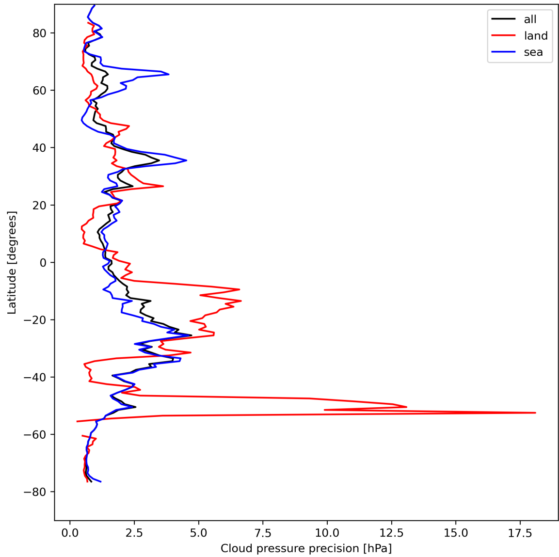
Figure 14: Zonal average of “Cloud pressure precision” for 2024-08-22 to 2024-08-24.
