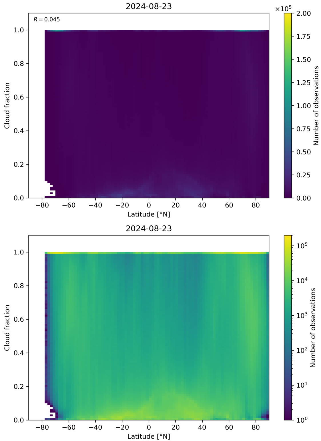
Figure 90: Scatter density plot of “Latitude” against “Cloud fraction” for 2024-08-22 to 2024-08-24.
