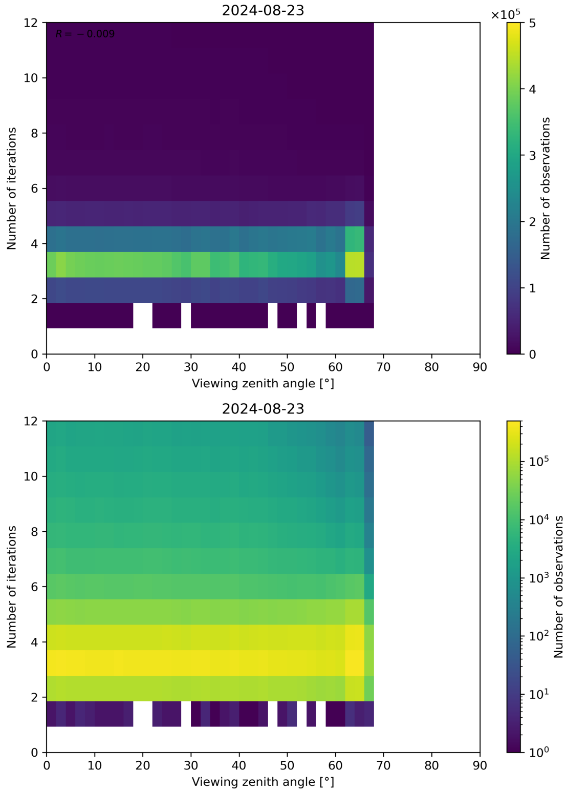
Figure 124: Scatter density plot of “Viewing zenith angle” against “Number of iterations” for 2024-08-22 to 2024-08-24.
