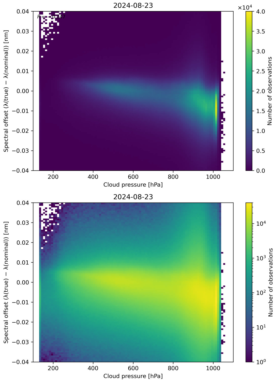
Figure 84: Scatter density plot of “Cloud pressure” against “Spectral offset ( \lambda(\text{true}) - \lambda(\text{nominal}) )” for 2024-08-22 to 2024-08-24.
