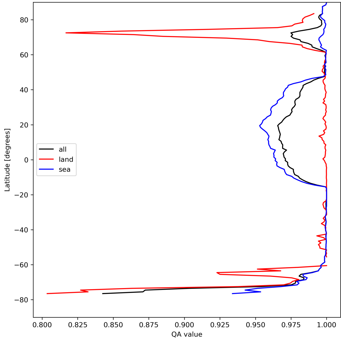
Figure 12: Zonal average of “QA value” for 2024-08-22 to 2024-08-24.
