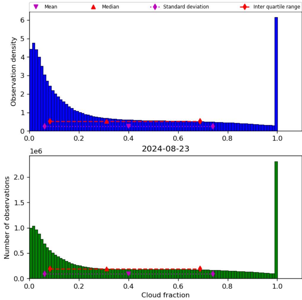
Figure 32: Histogram of “Cloud fraction” for 2024-08-22 to 2024-08-24
