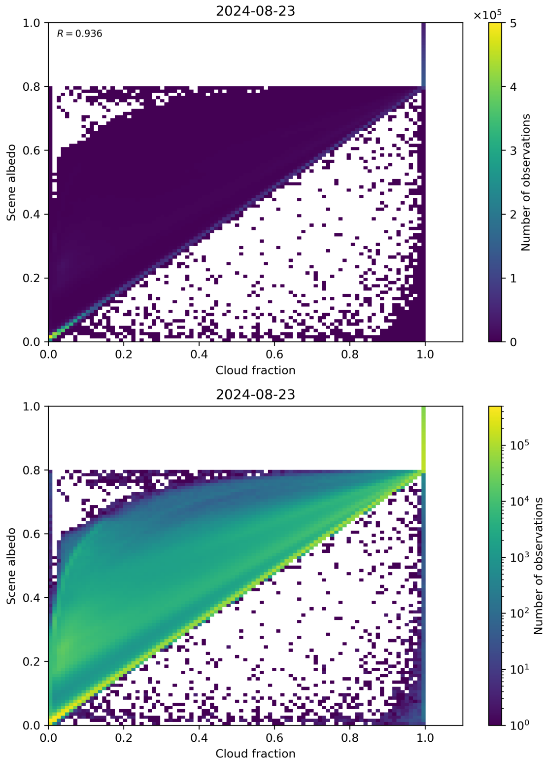
Figure 75: Scatter density plot of “Cloud fraction” against “Scene albedo” for 2024-08-22 to 2024-08-24.
