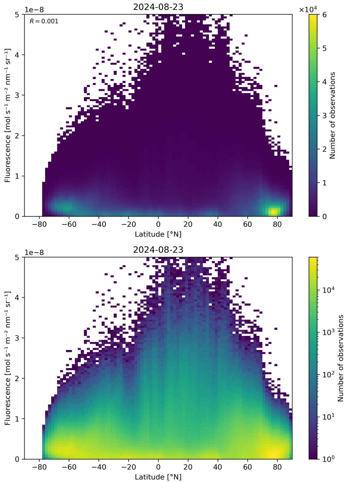
Figure 92: Scatter density plot of “Latitude” against “Fluorescence” for 2024-08-22 to 2024-08-24.
