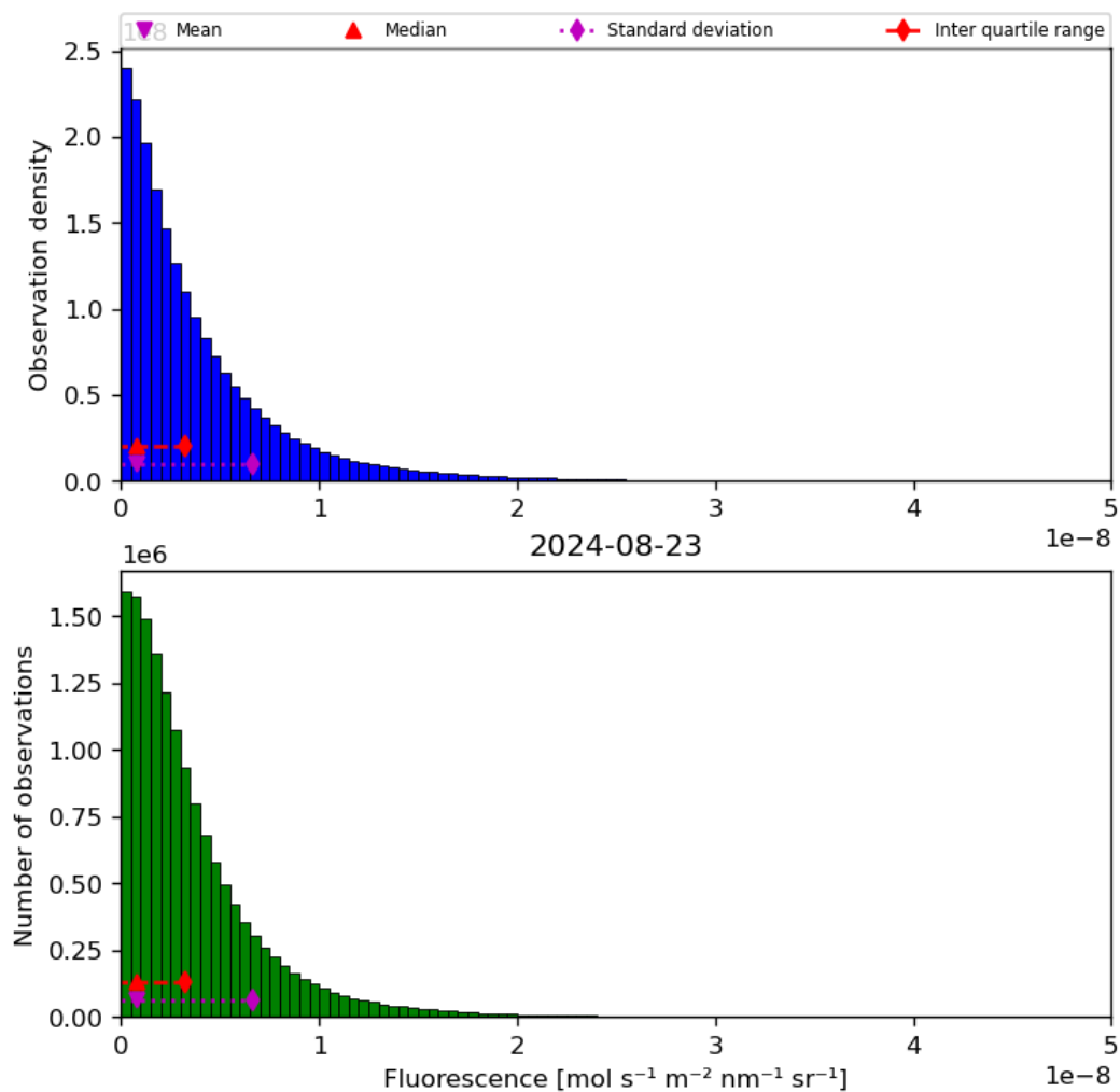
Figure 40: Histogram of “Fluorescence” for 2024-08-22 to 2024-08-24
