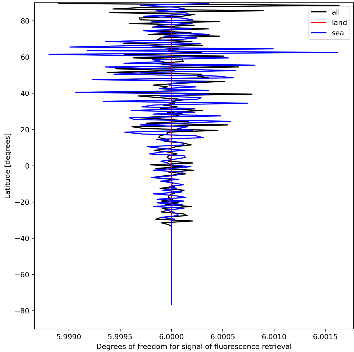
Figure 26: Zonal average of “Degrees of freedom for signal of fluorescence retrieval” for 2024-08-22 to 2024-08-24.
