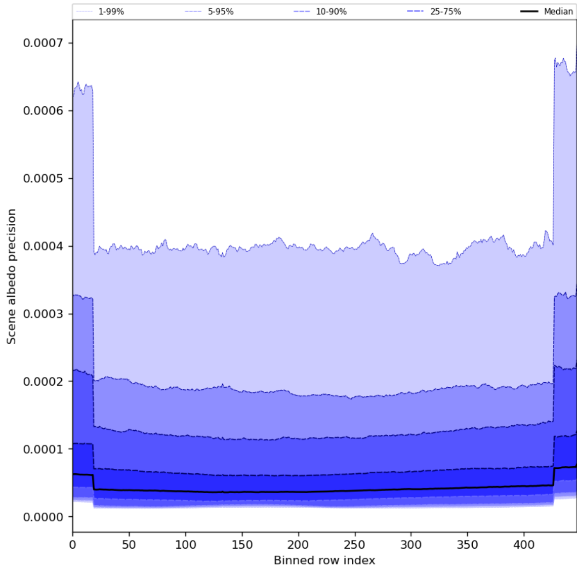
Figure 52: Along track statistics of “Scene albedo precision” for 2024-08-22 to 2024-08-24
