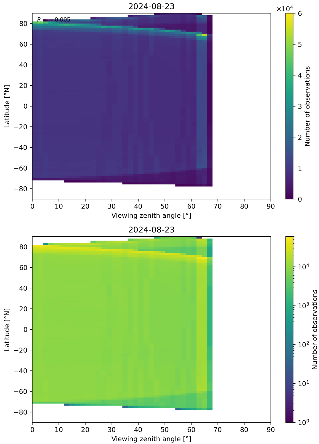
Figure 123: Scatter density plot of “Viewing zenith angle” against “Latitude” for 2024-08-22 to 2024-08-24.
