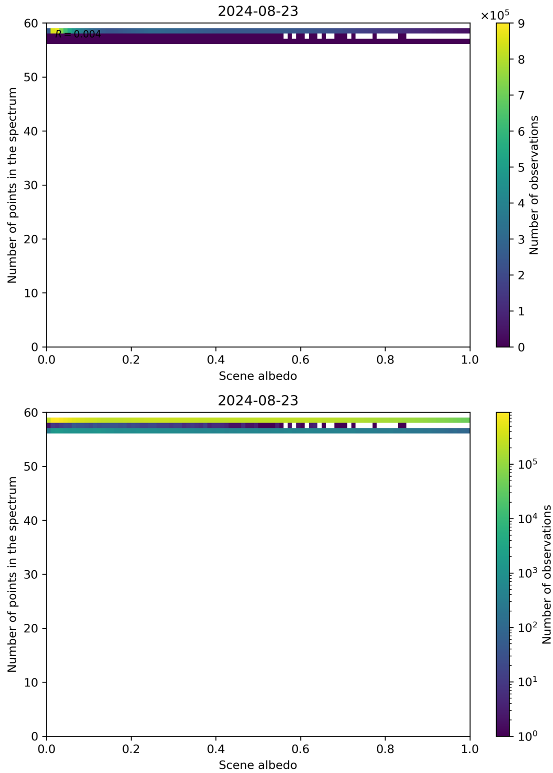
Figure 106: Scatter density plot of “Scene albedo” against “Number of points in the spectrum” for 2024-08-22 to 2024-08-24.
