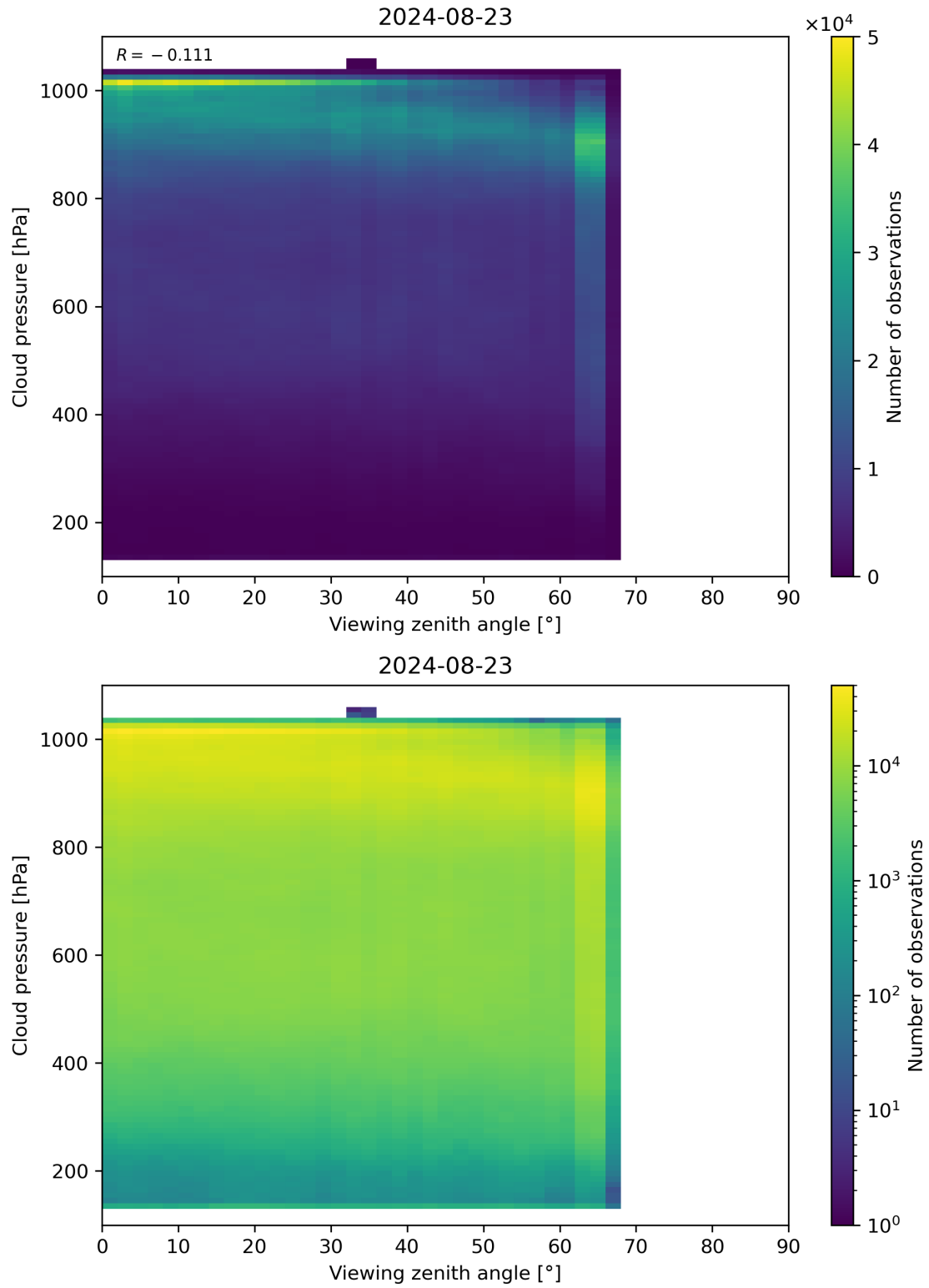
Figure 121: Scatter density plot of “Viewing zenith angle” against “Cloud pressure” for 2024-08-22 to 2024-08-24.
