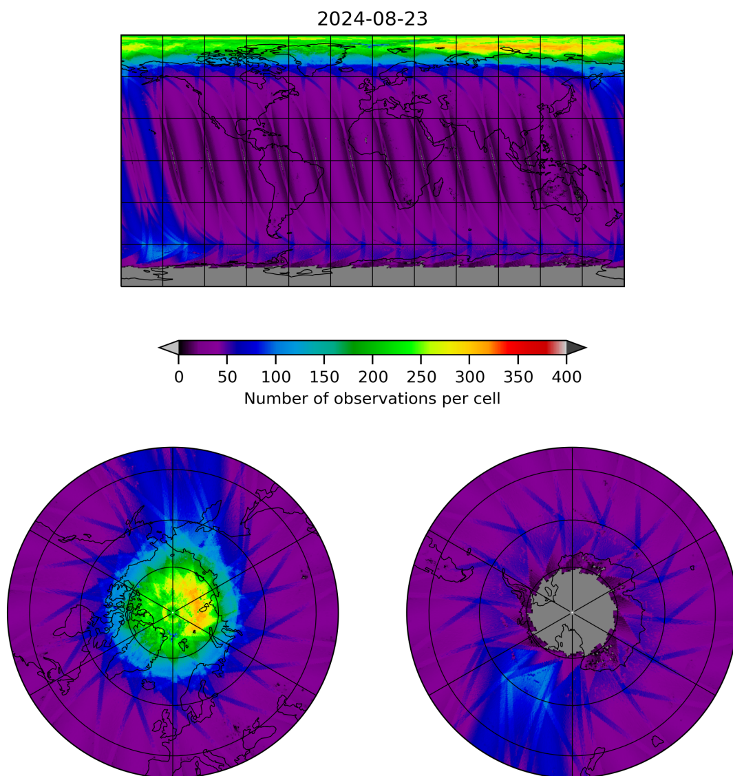
Figure 11: Map of the number of observations for 2024-08-22 to 2024-08-24
