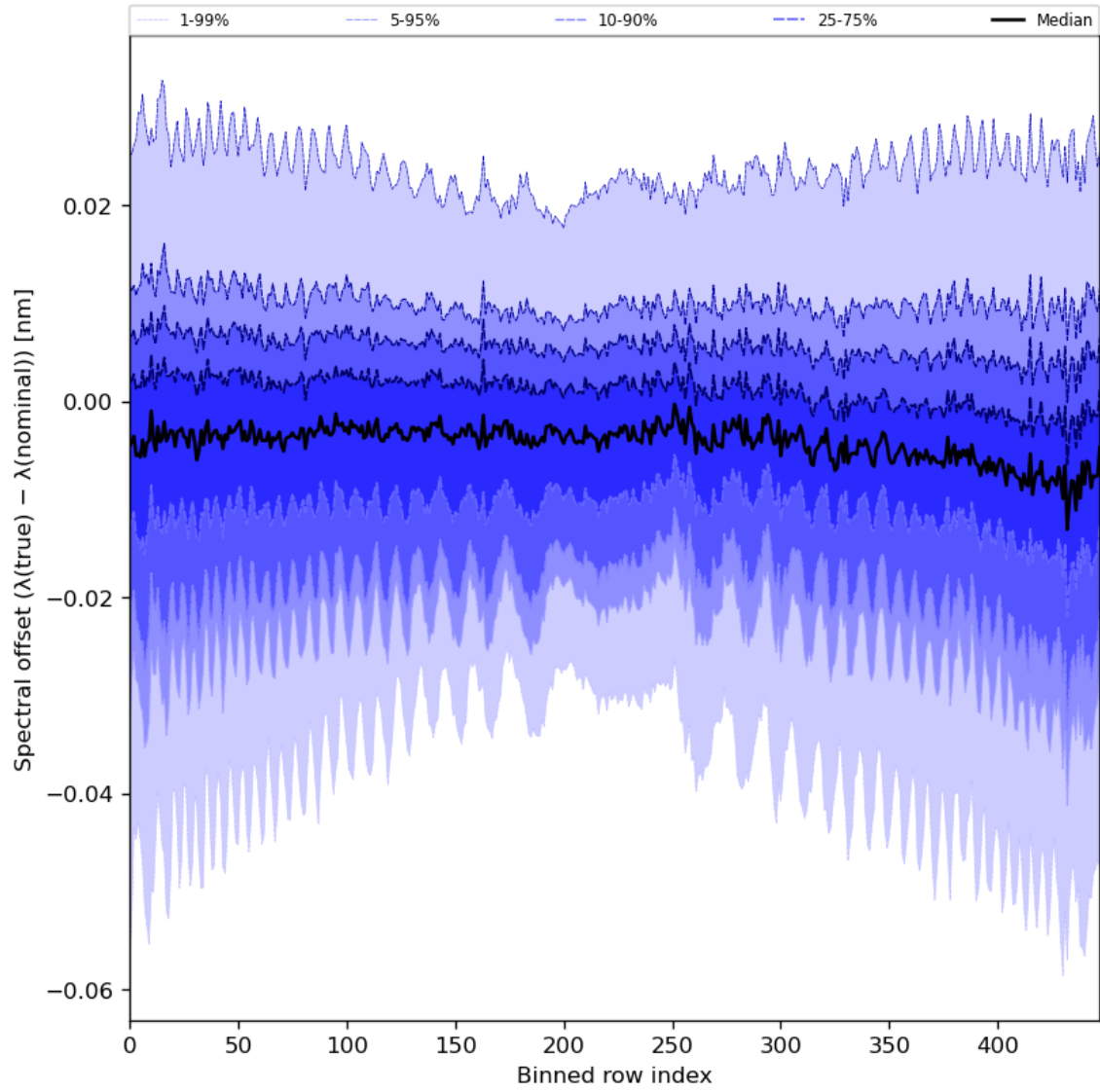
Figure 62: Along track statistics of “Spectral offset ( \lambda(\text{true}) - \lambda(\text{nominal}) )” for 2024-08-22 to 2024-08-24
