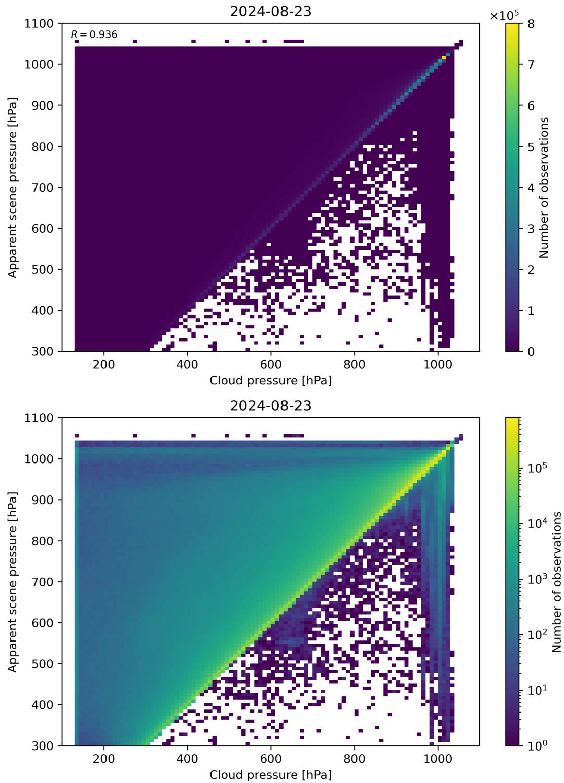
Figure 77: Scatter density plot of “Cloud pressure” against “Apparent scene pressure” for 2024-08-22 to 2024-08-24.
