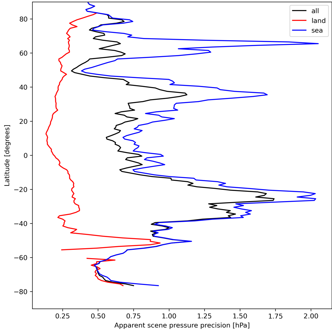
Figure 20: Zonal average of “Apparent scene pressure precision” for 2024-08-22 to 2024-08-24.
