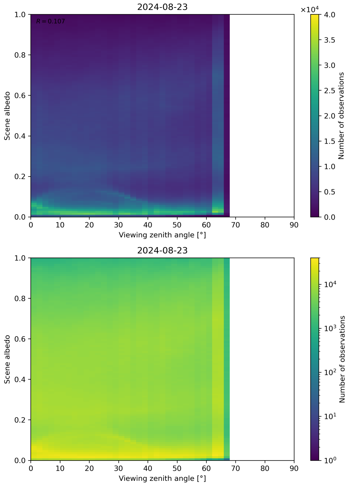
Figure 126: Scatter density plot of “Viewing zenith angle” against “Scene albedo” for 2024-08-22 to 2024-08-24.
