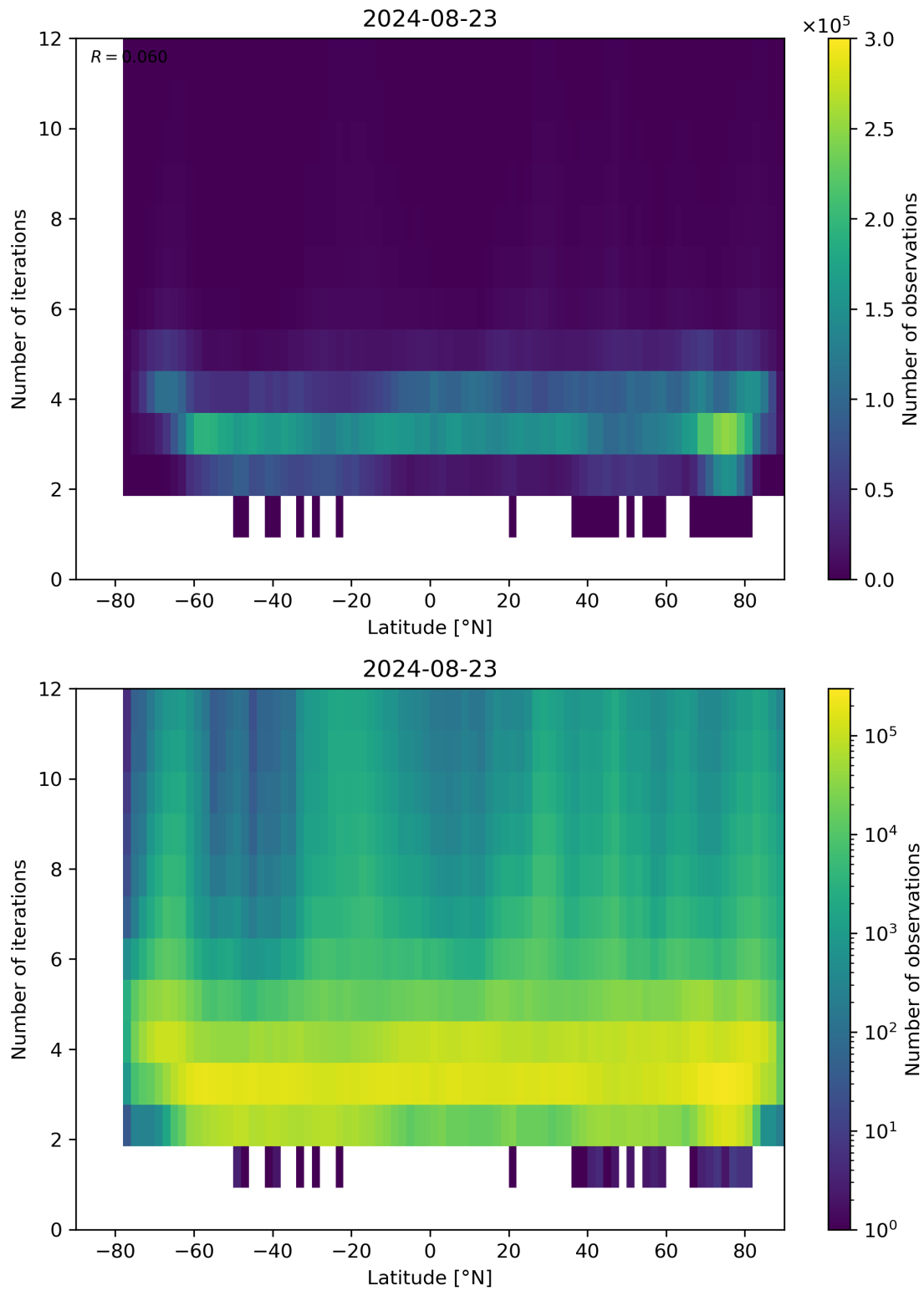
Figure 93: Scatter density plot of “Latitude” against “Number of iterations” for 2024-08-22 to 2024-08-24.
