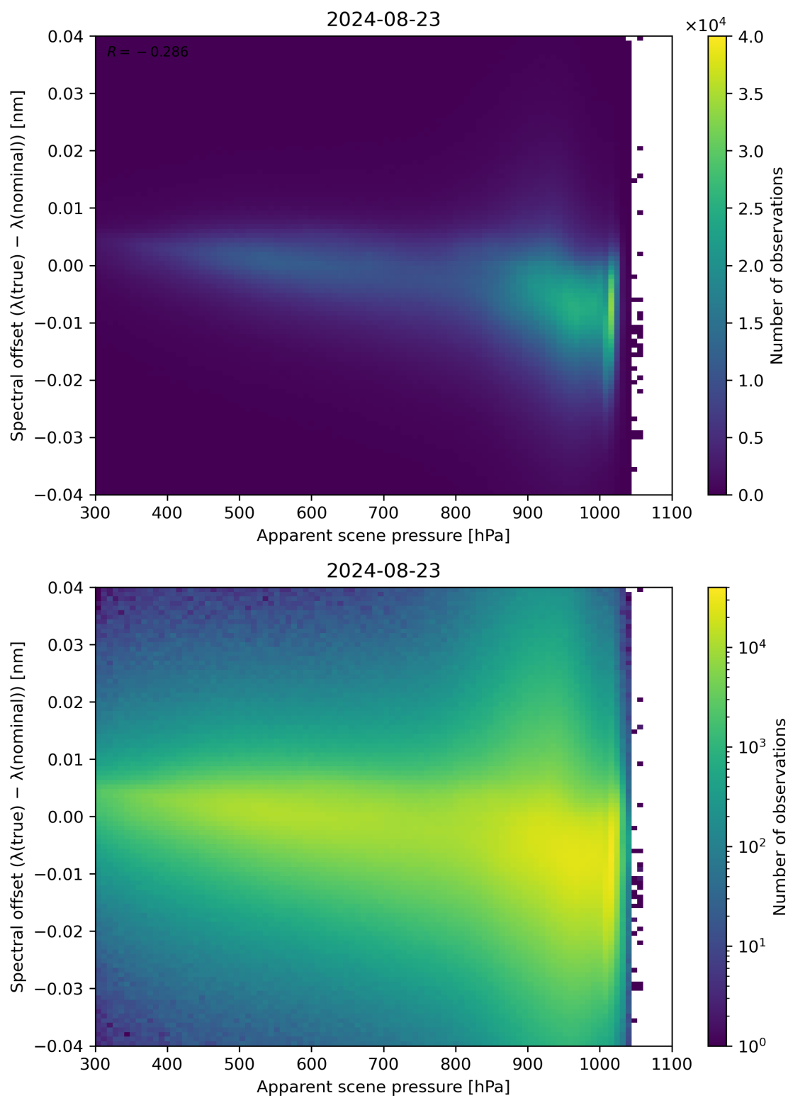
Figure 67: Scatter density plot of “Apparent scene pressure” against “Spectral offset ( \lambda(\text{true}) - \lambda(\text{nominal}) )” for 2024-08-22 to 2024-08-24.
