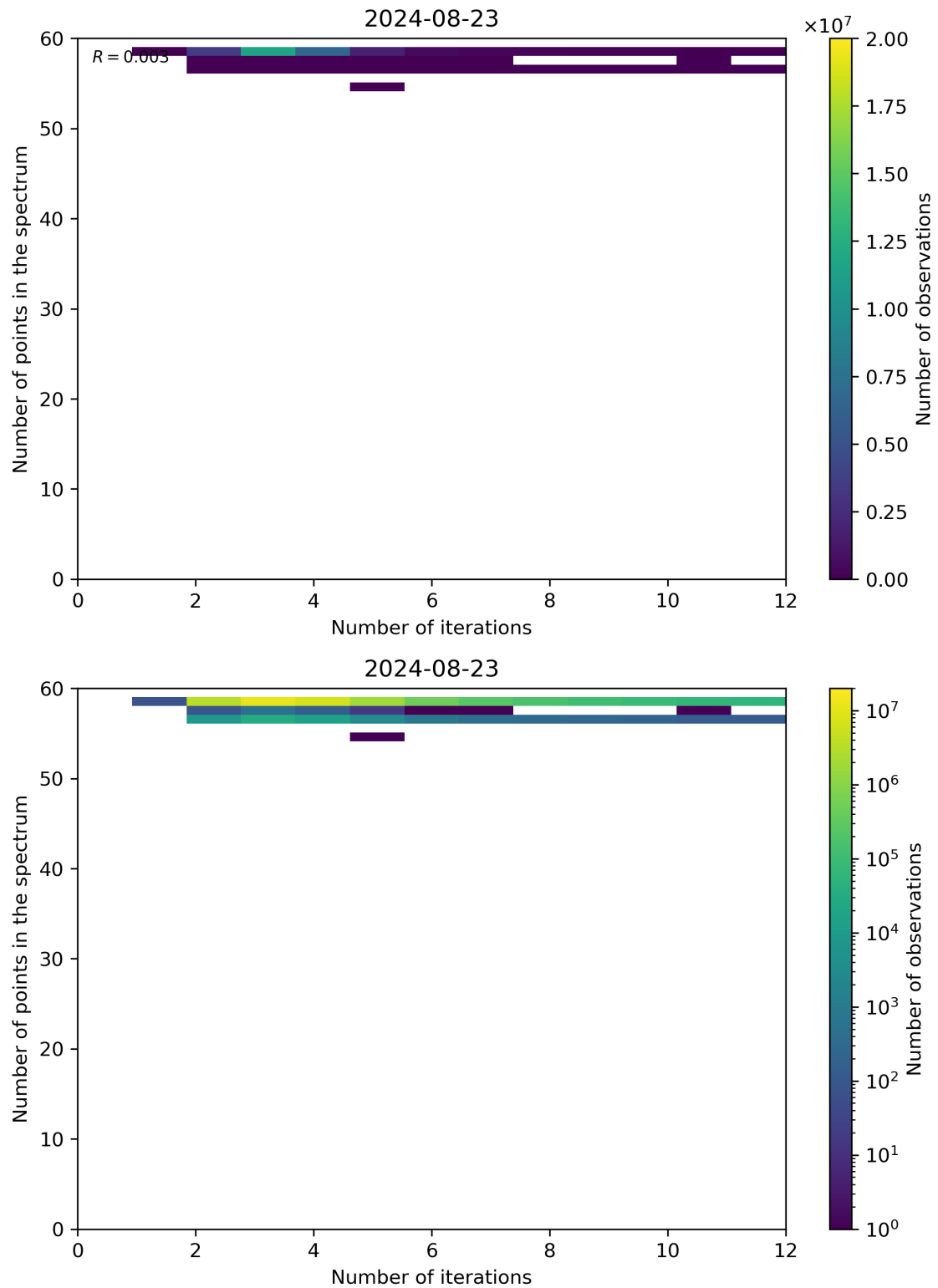
Figure 99: Scatter density plot of “Number of iterations” against “Number of points in the spectrum” for 2024-08-22 to 2024-08-24.
