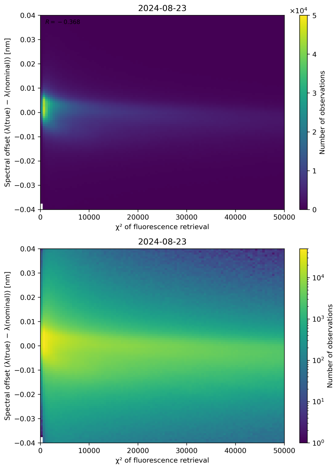
Figure 69: Scatter density plot of “ \chi^2 of fluorescence retrieval” against “Spectral offset ( \lambda(\text{true}) - \lambda(\text{nominal}) )” for 2024-08-22 to 2024-08-24.
