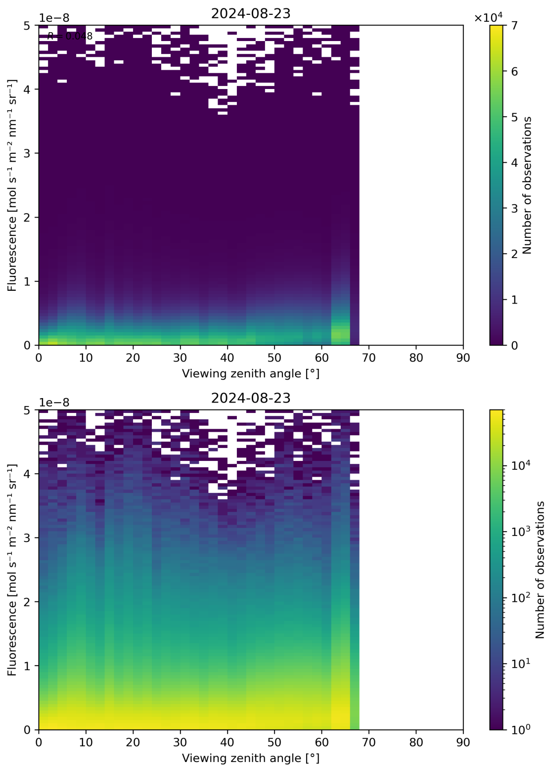
Figure 122: Scatter density plot of “Viewing zenith angle” against “Fluorescence” for 2024-08-22 to 2024-08-24.
