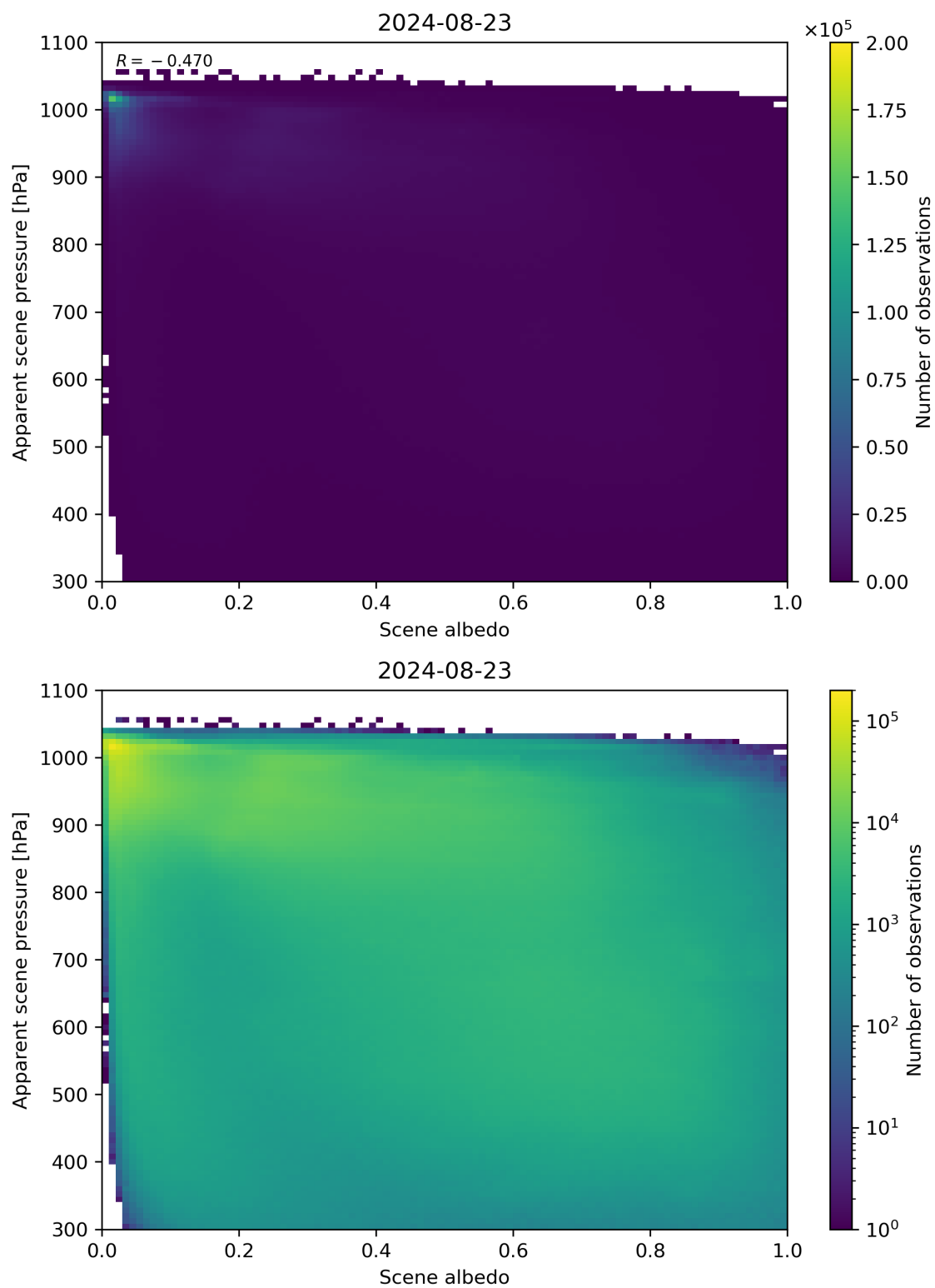
Figure 102: Scatter density plot of “Scene albedo” against “Apparent scene pressure” for 2024-08-22 to 2024-08-24.
