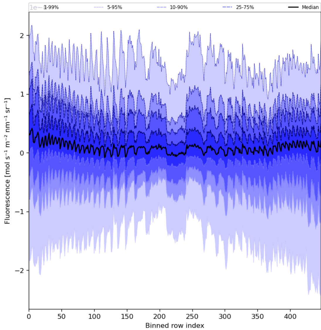
Figure 57: Along track statistics of “Fluorescence” for 2024-08-22 to 2024-08-24
