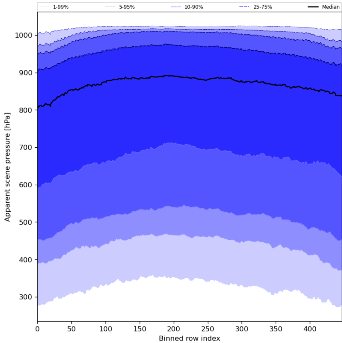
Figure 53: Along track statistics of “Apparent scene pressure” for 2024-08-22 to 2024-08-24
