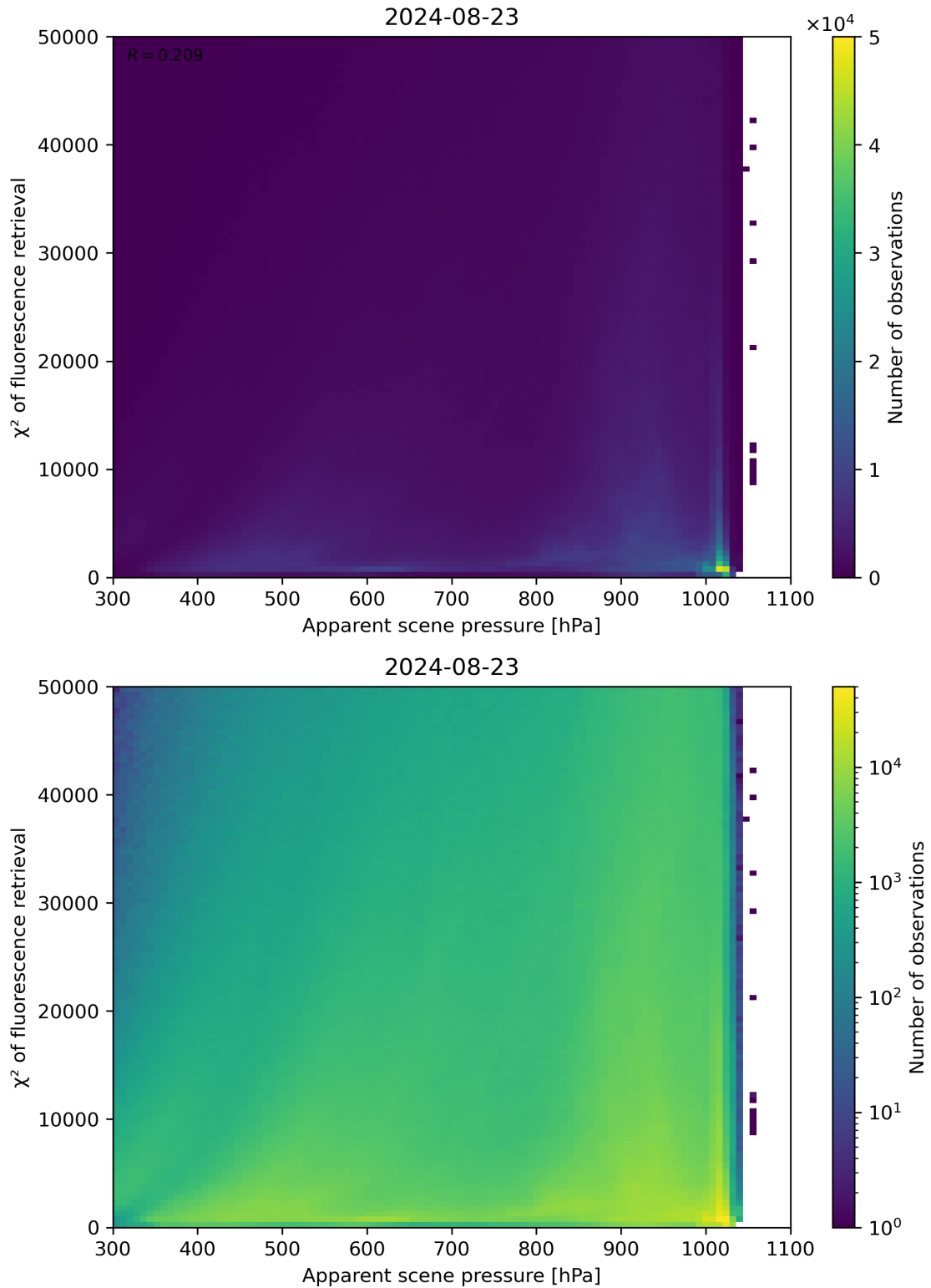
Figure 63: Scatter density plot of “Apparent scene pressure” against “ \chi^2 of fluorescence retrieval” for 2024-08-22 to 2024-08-24.
