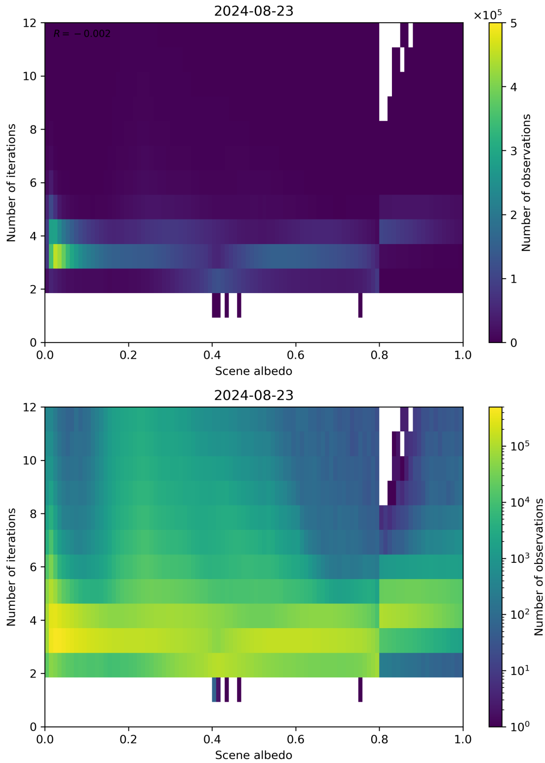
Figure 105: Scatter density plot of “Scene albedo” against “Number of iterations” for 2024-08-22 to 2024-08-24.
