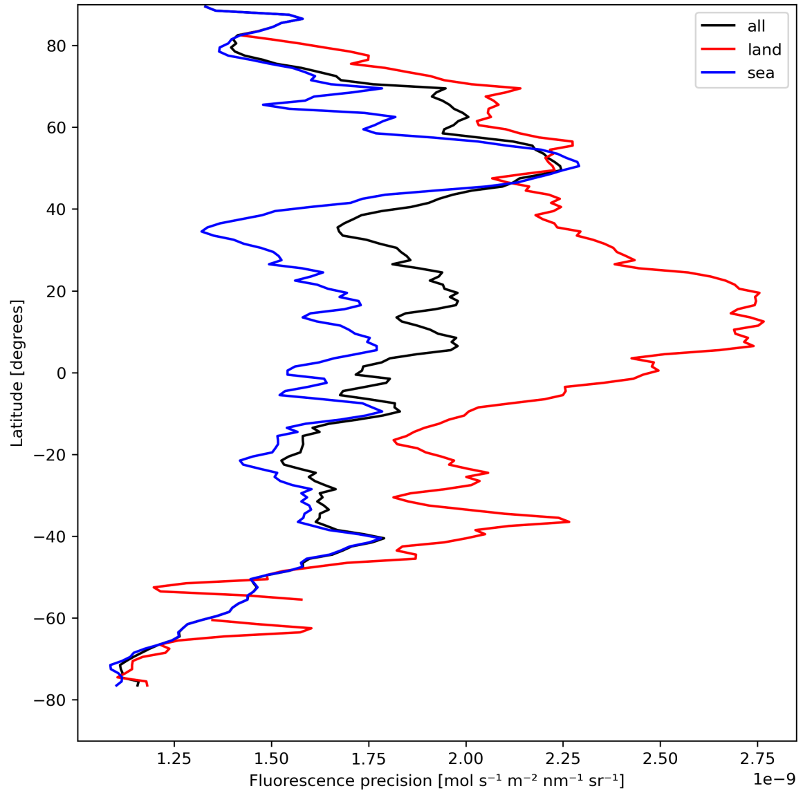
Figure 24: Zonal average of “Fluorescence precision” for 2024-08-22 to 2024-08-24.
