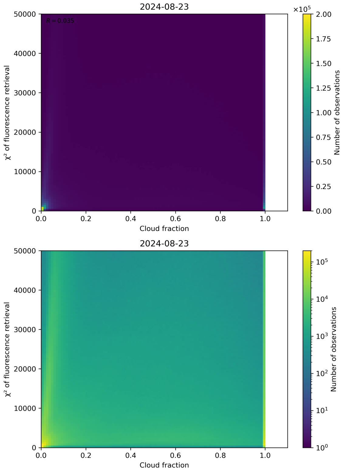
Figure 71: Scatter density plot of “Cloud fraction” against “ \chi^2 of fluorescence retrieval” for 2024-08-22 to 2024-08-24.
