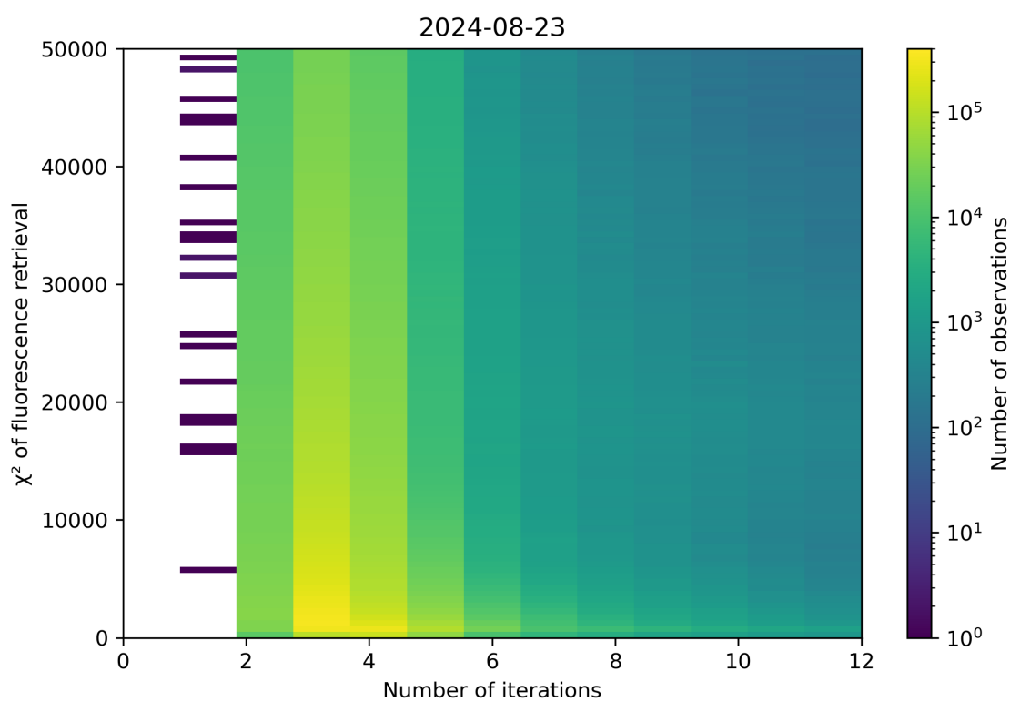
Figure 97: Scatter density plot of “Number of iterations” against “ \chi^2 of fluorescence retrieval” for 2024-08-22 to 2024-08-24.
