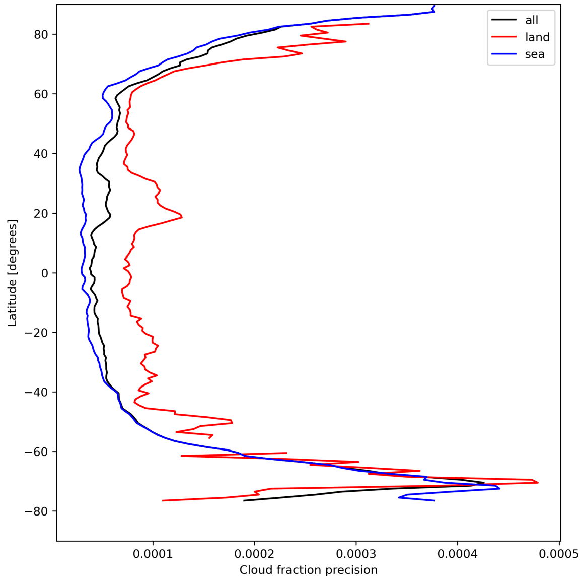
Figure 16: Zonal average of “Cloud fraction precision” for 2024-08-22 to 2024-08-24.
