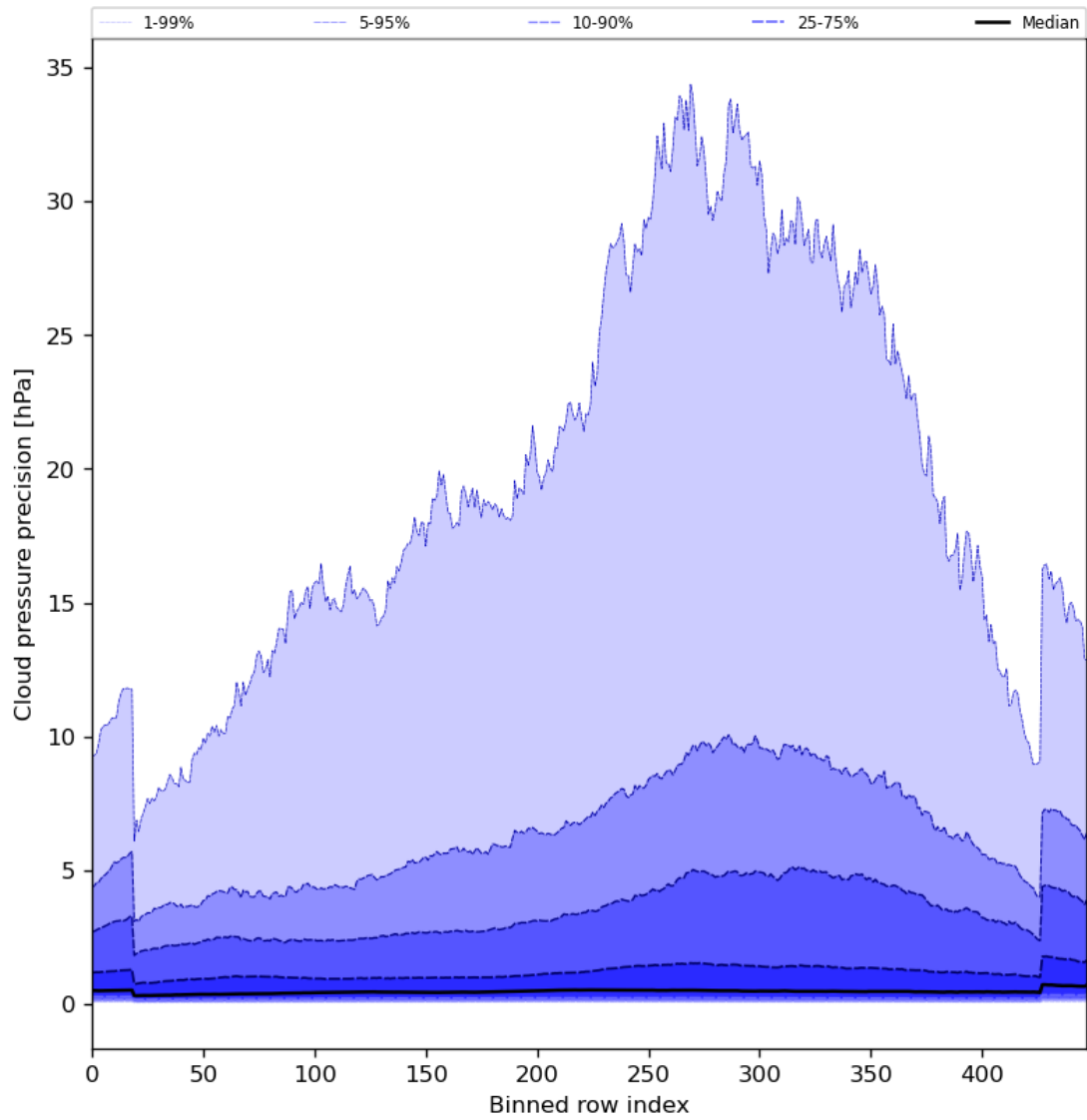
Figure 48: Along track statistics of “Cloud pressure precision” for 2024-08-22 to 2024-08-24
