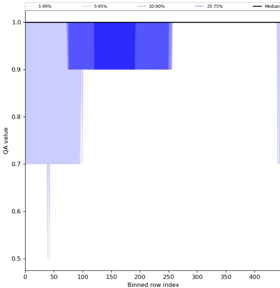
Figure 46: Along track statistics of “QA value” for 2024-08-22 to 2024-08-24
