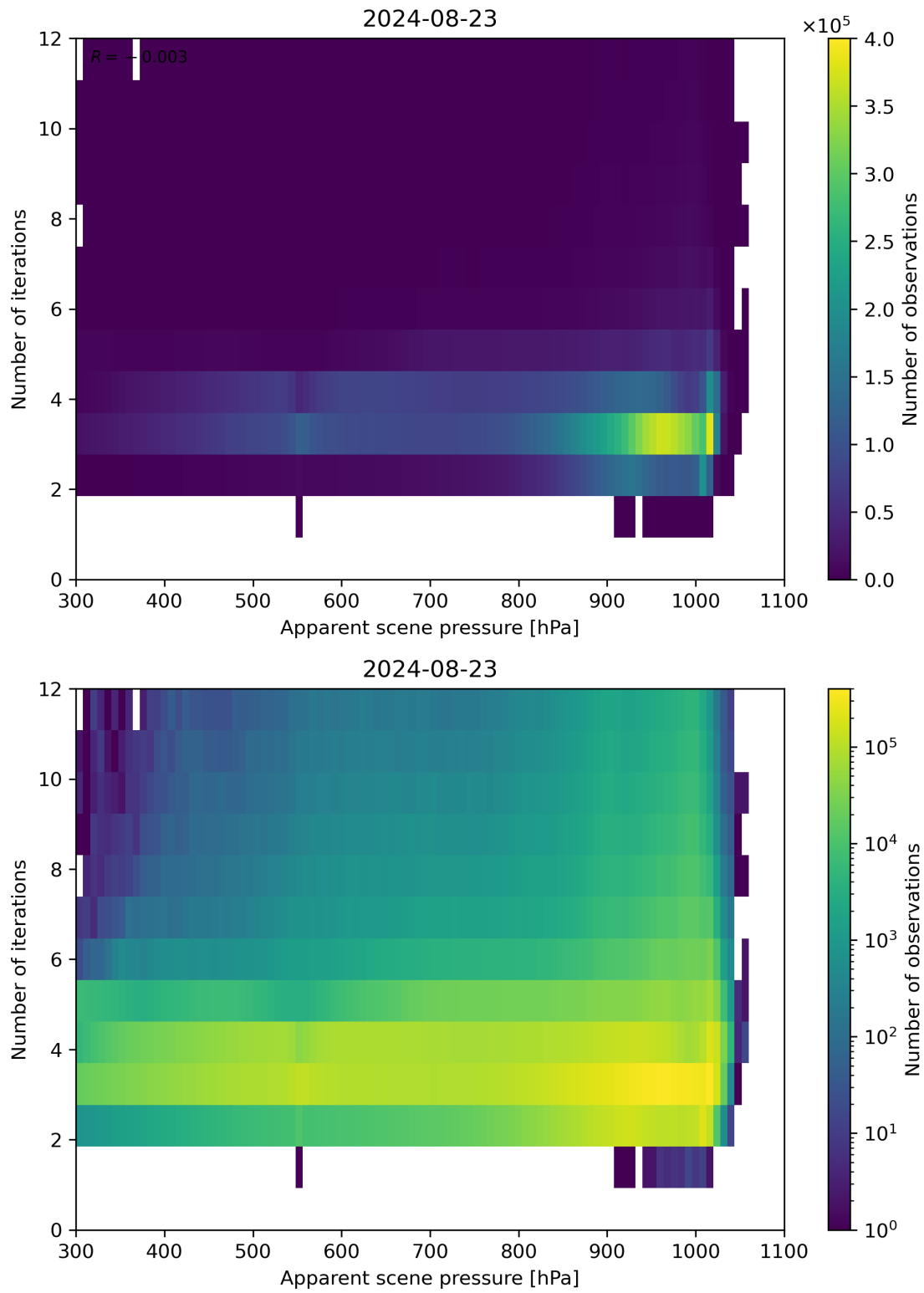
Figure 65: Scatter density plot of “Apparent scene pressure” against “Number of iterations” for 2024-08-22 to 2024-08-24.
