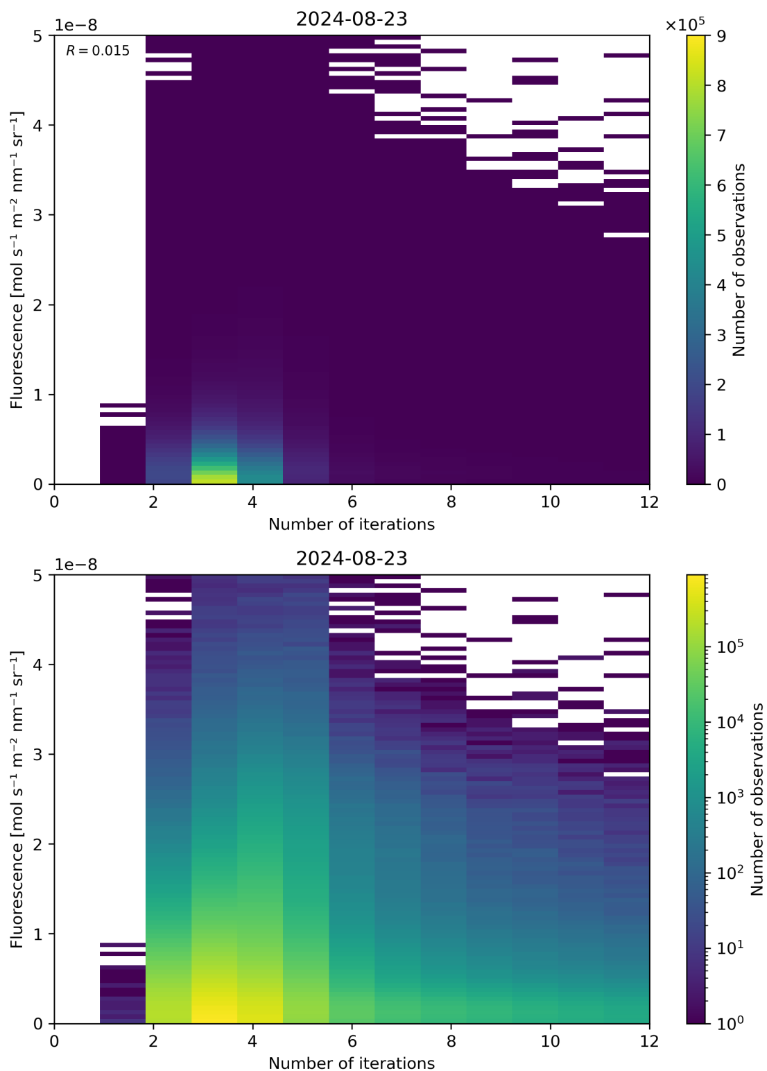
Figure 98: Scatter density plot of “Number of iterations” against “Fluorescence” for 2024-08-22 to 2024-08-24.
