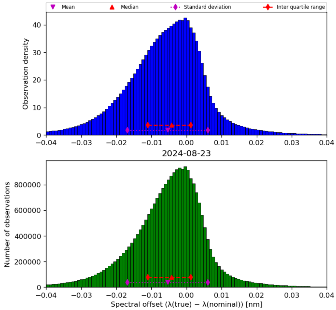
Figure 45: Histogram of “Spectral offset ( \lambda(\text{true}) - \lambda(\text{nominal}) )” for 2024-08-22 to 2024-08-24
