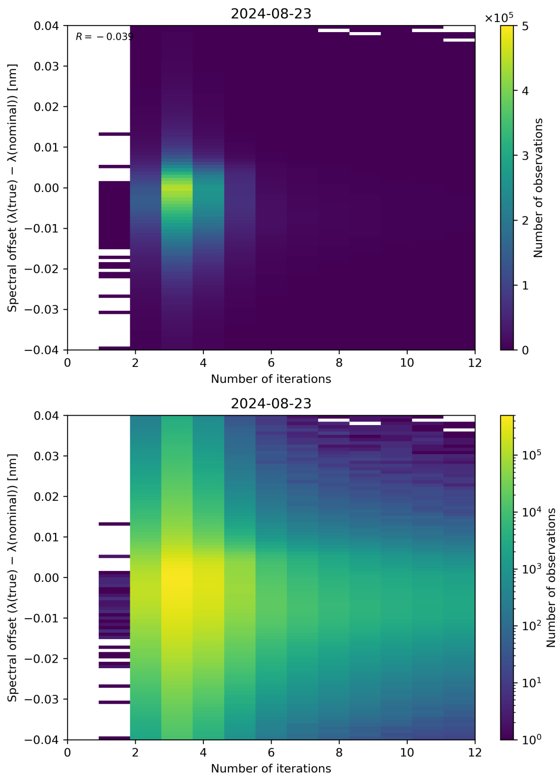
Figure 100: Scatter density plot of “Number of iterations” against “Spectral offset ( \lambda(\text{true}) - \lambda(\text{nominal}) )” for 2024-08-22 to 2024-08-24.
