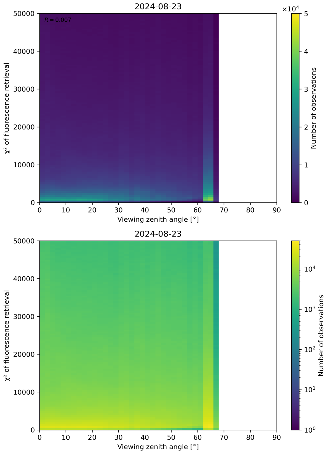
Figure 119: Scatter density plot of “Viewing zenith angle” against “ \chi^2 of fluorescence retrieval” for 2024-08-22 to 2024-08-24.
