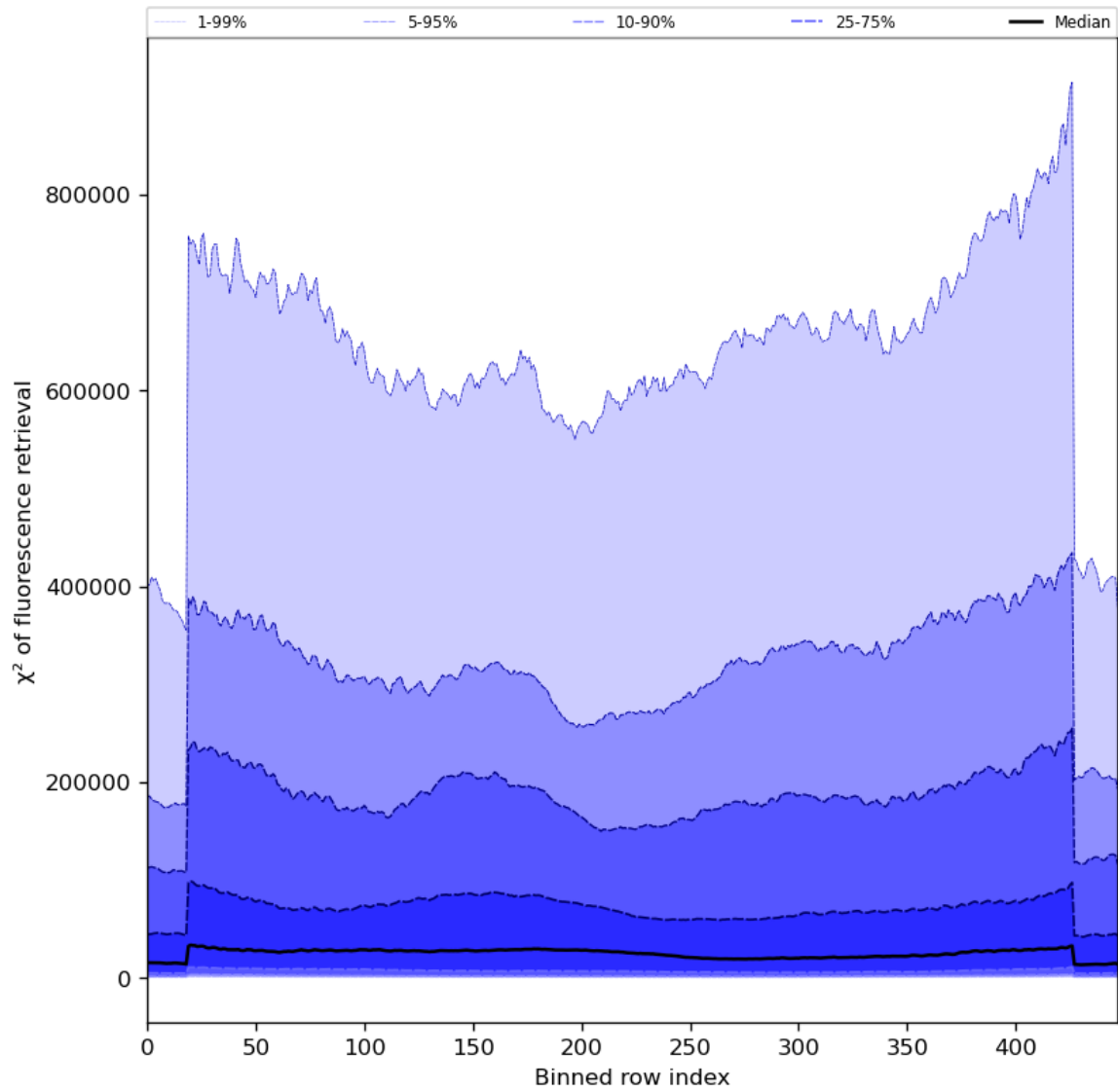
Figure 59: Along track statistics of “ \chi^2 of fluorescence retrieval” for 2024-08-22 to 2024-08-24
