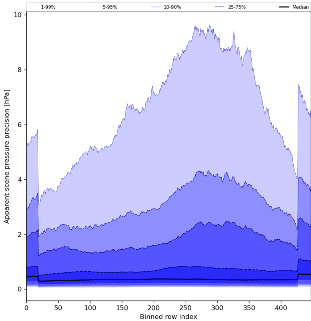
Figure 54: Along track statistics of “Apparent scene pressure precision” for 2024-08-22 to 2024-08-24
