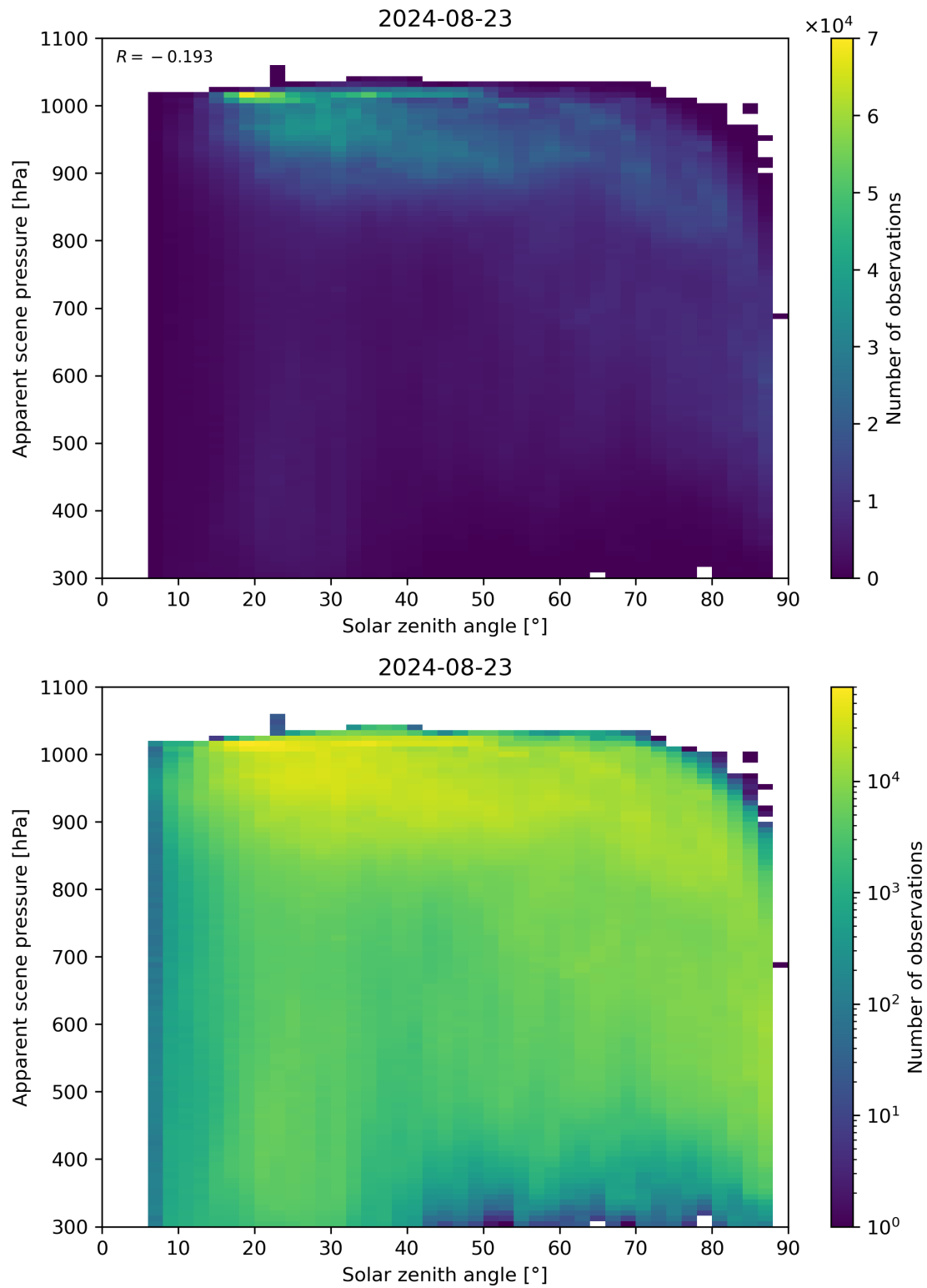
Figure 108: Scatter density plot of “Solar zenith angle” against “Apparent scene pressure” for 2024-08-22 to 2024-08-24.
