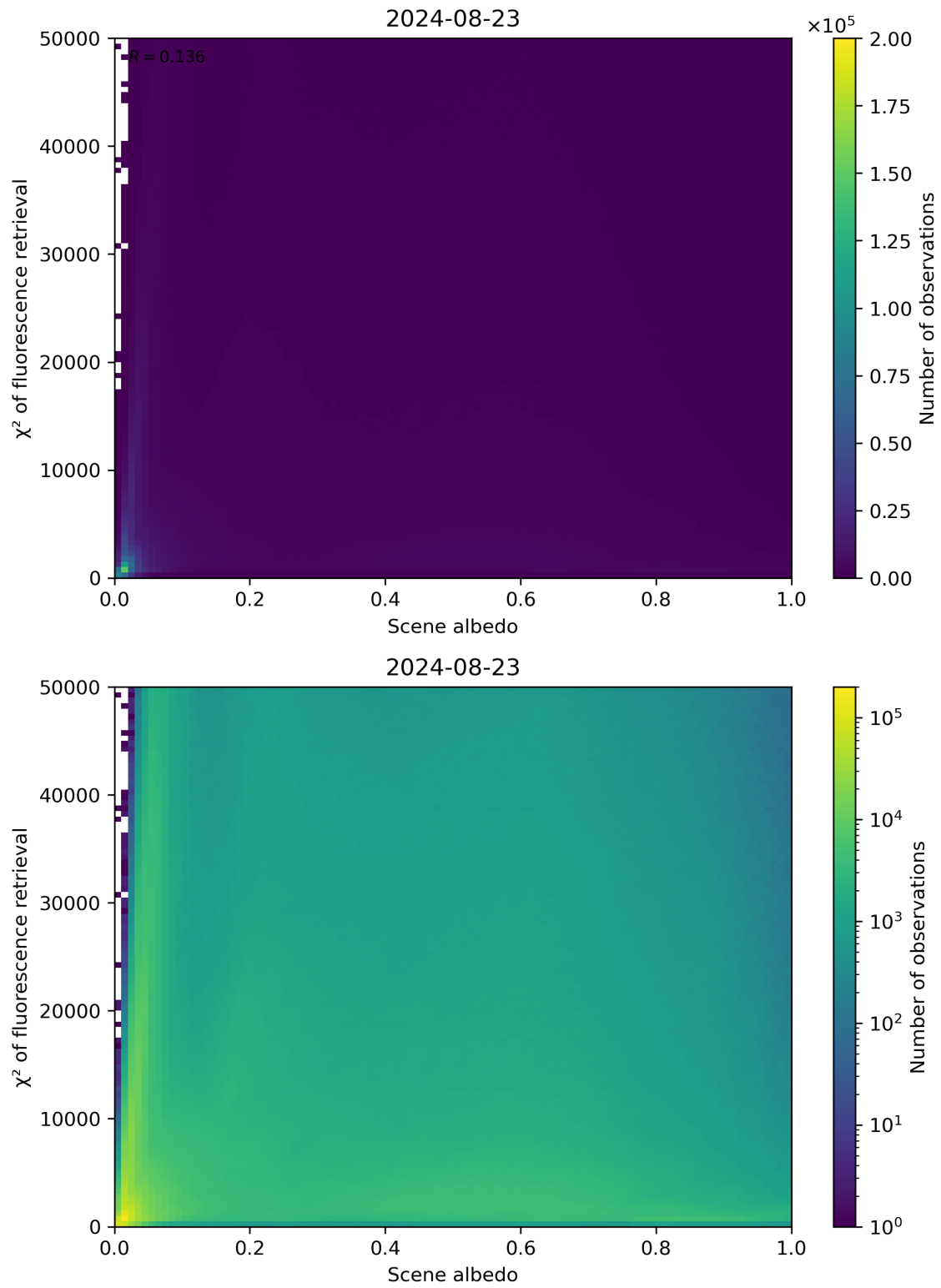
Figure 103: Scatter density plot of “Scene albedo” against “ \chi^2 of fluorescence retrieval” for 2024-08-22 to 2024-08-24.
