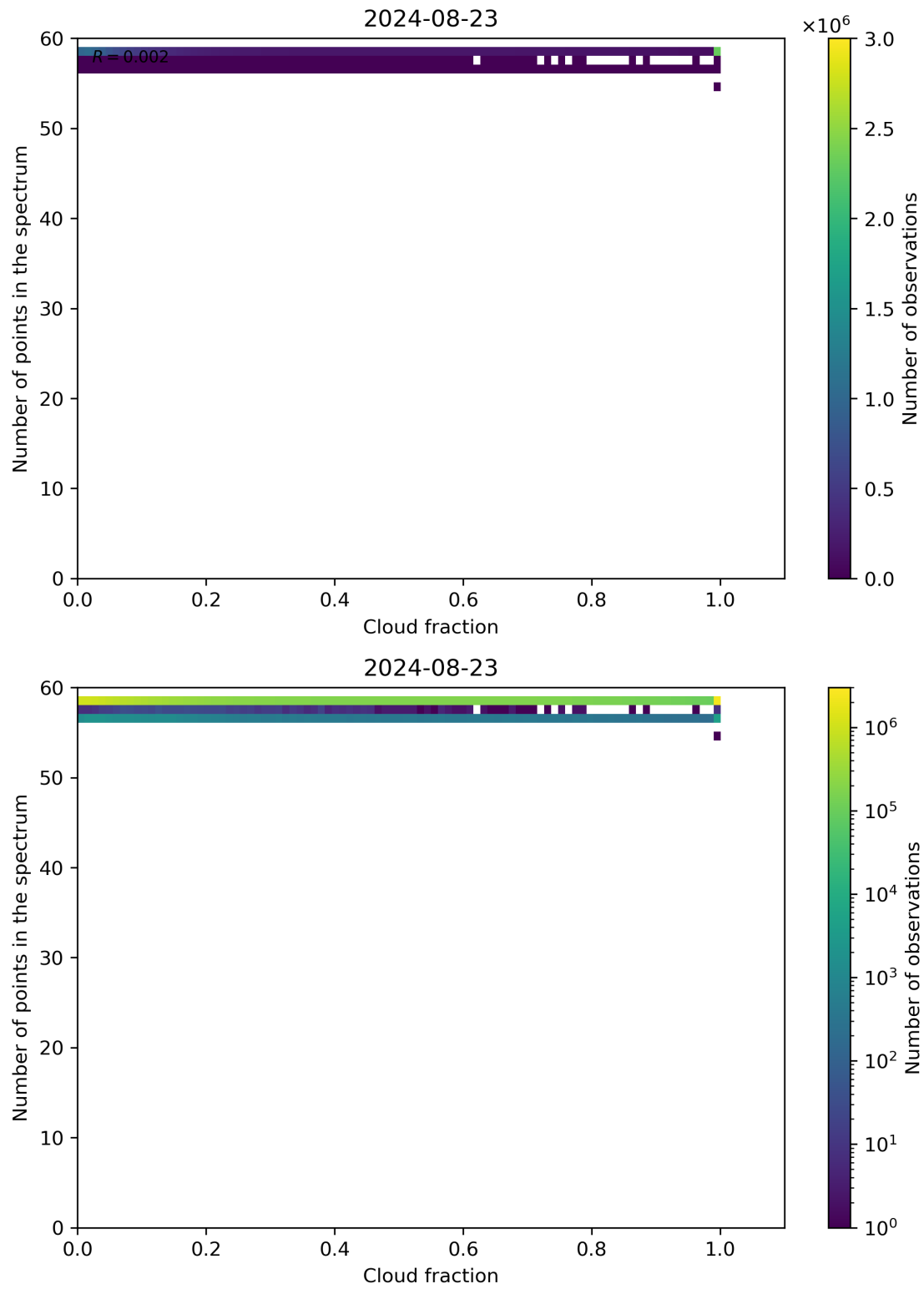
Figure 74: Scatter density plot of “Cloud fraction” against “Number of points in the spectrum” for 2024-08-22 to 2024-08-24.
