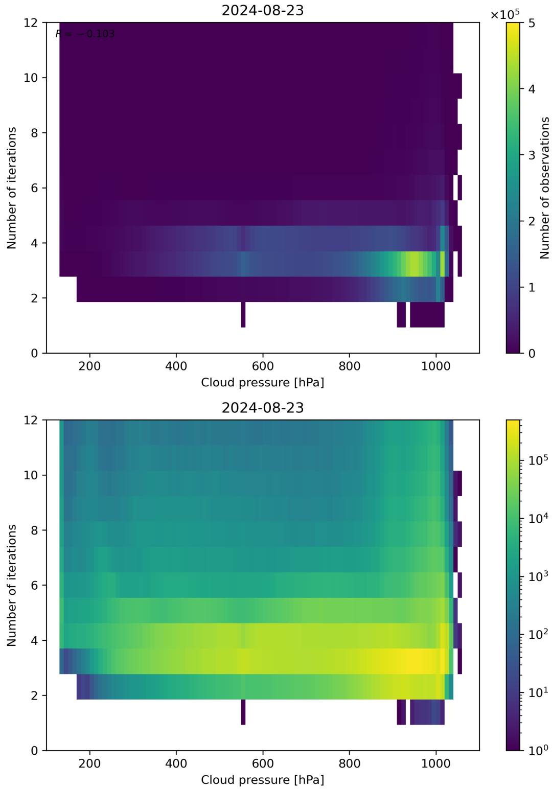
Figure 81: Scatter density plot of “Cloud pressure” against “Number of iterations” for 2024-08-22 to 2024-08-24.
