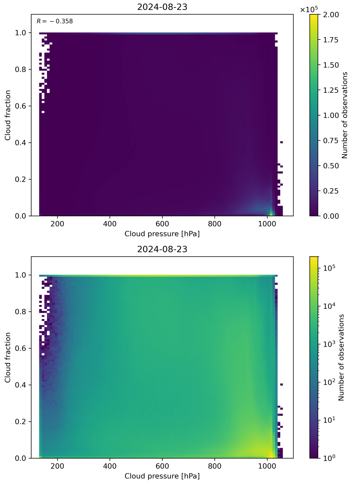
Figure 79: Scatter density plot of “Cloud pressure” against “Cloud fraction” for 2024-08-22 to 2024-08-24.
