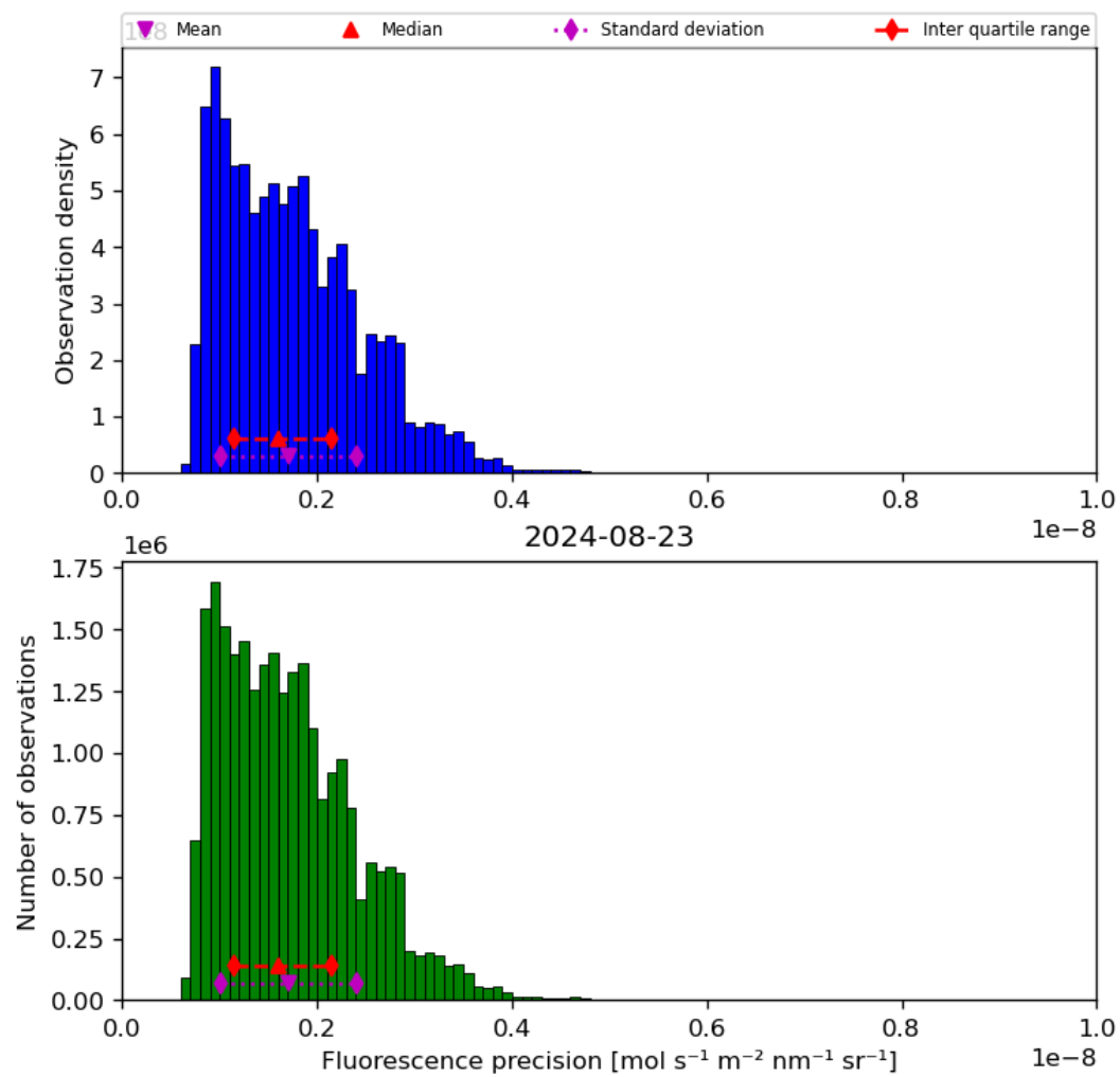
Figure 41: Histogram of “Fluorescence precision” for 2024-08-22 to 2024-08-24
