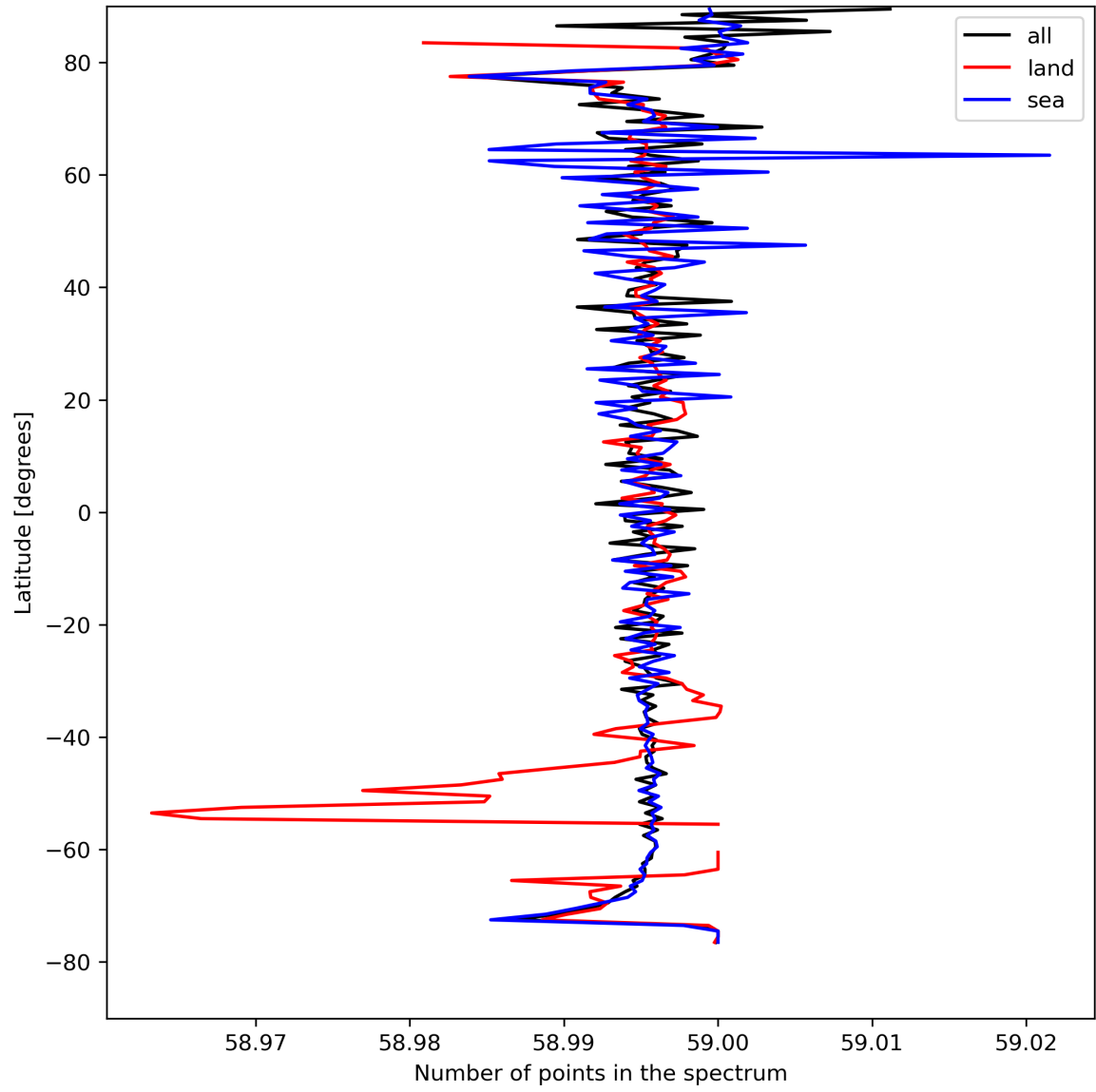
Figure 27: Zonal average of “Number of points in the spectrum” for 2024-08-22 to 2024-08-24.
