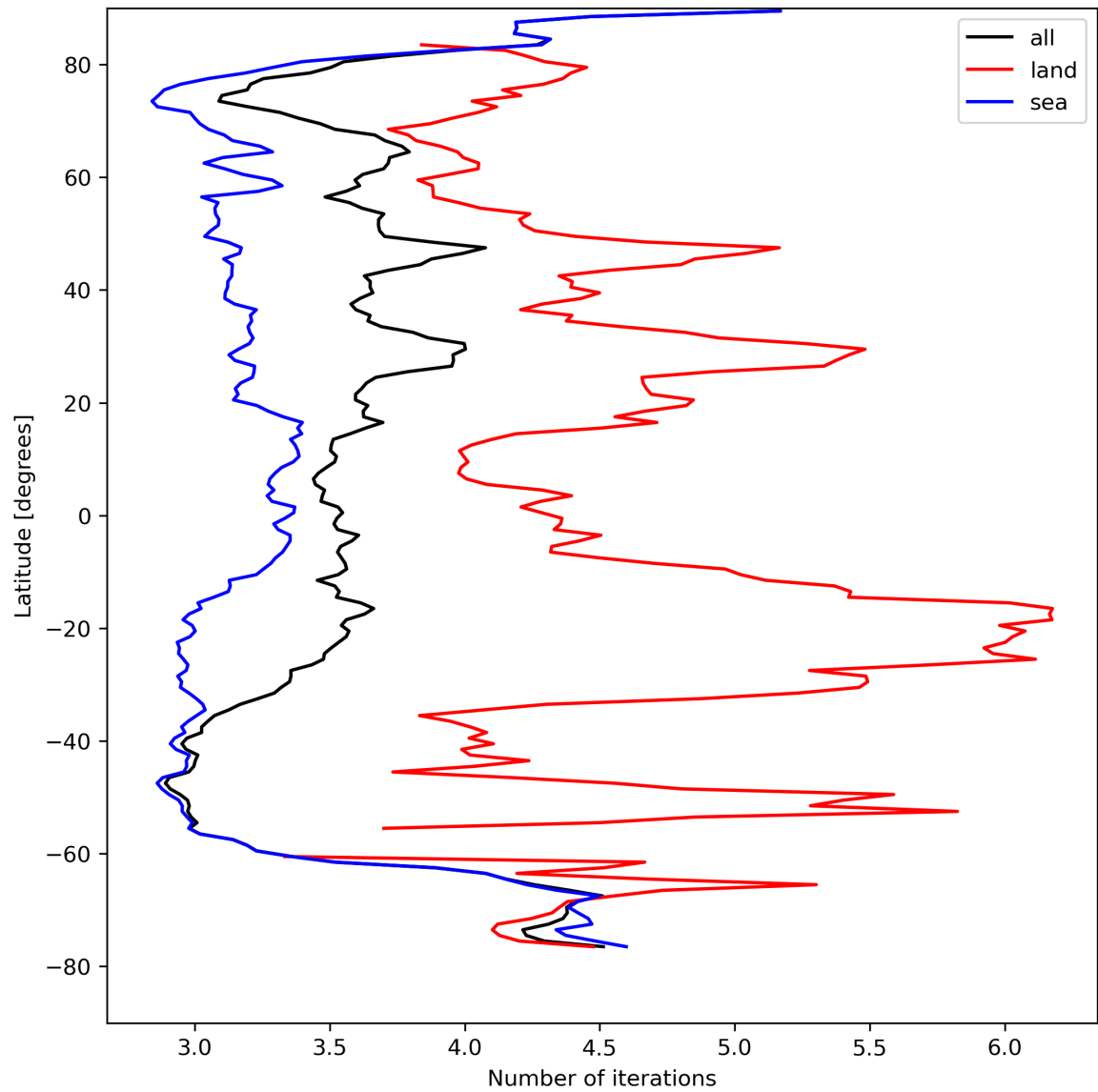
Figure 22: Zonal average of “Number of iterations” for 2024-08-22 to 2024-08-24.
