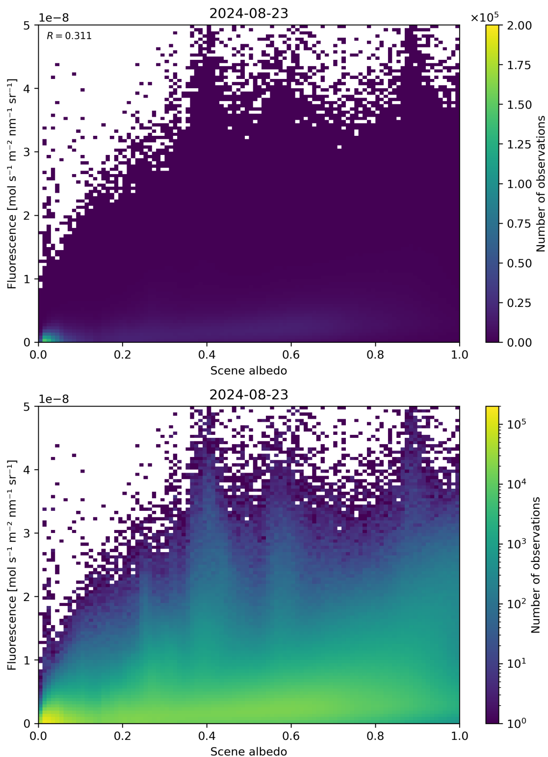
Figure 104: Scatter density plot of “Scene albedo” against “Fluorescence” for 2024-08-22 to 2024-08-24.
