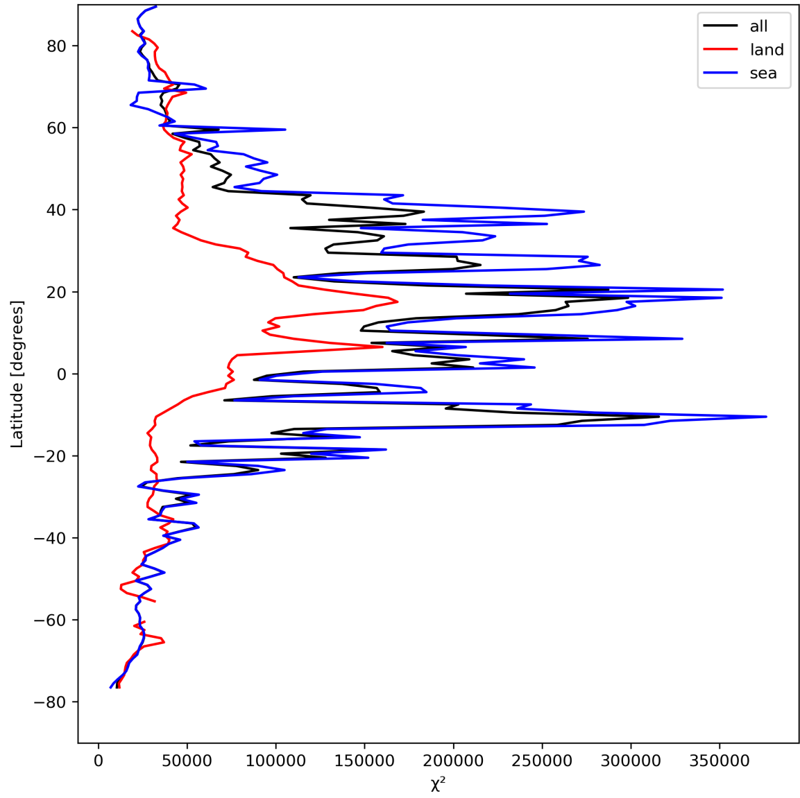
Figure 21: Zonal average of “ \chi^2 ” for 2024-08-22 to 2024-08-24.
