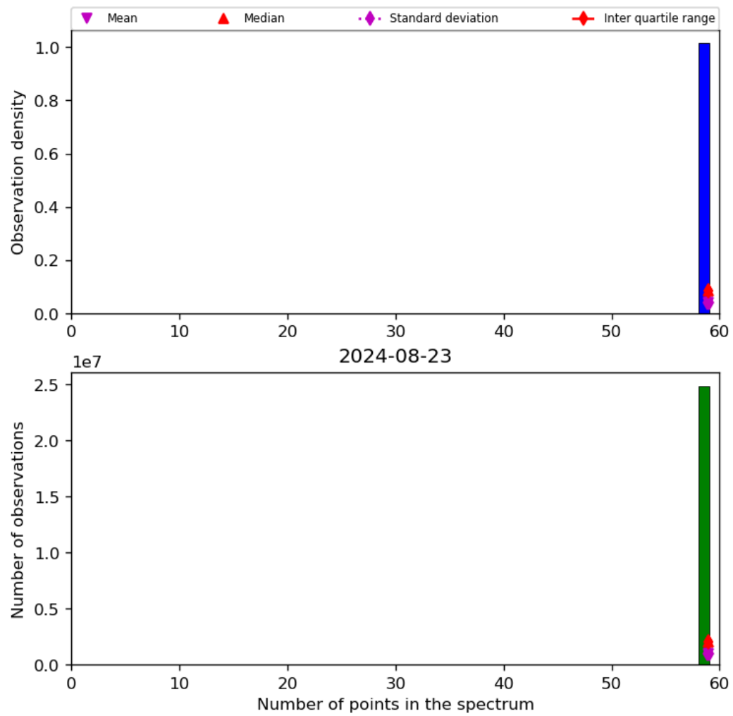
Figure 44: Histogram of “Number of points in the spectrum” for 2024-08-22 to 2024-08-24
