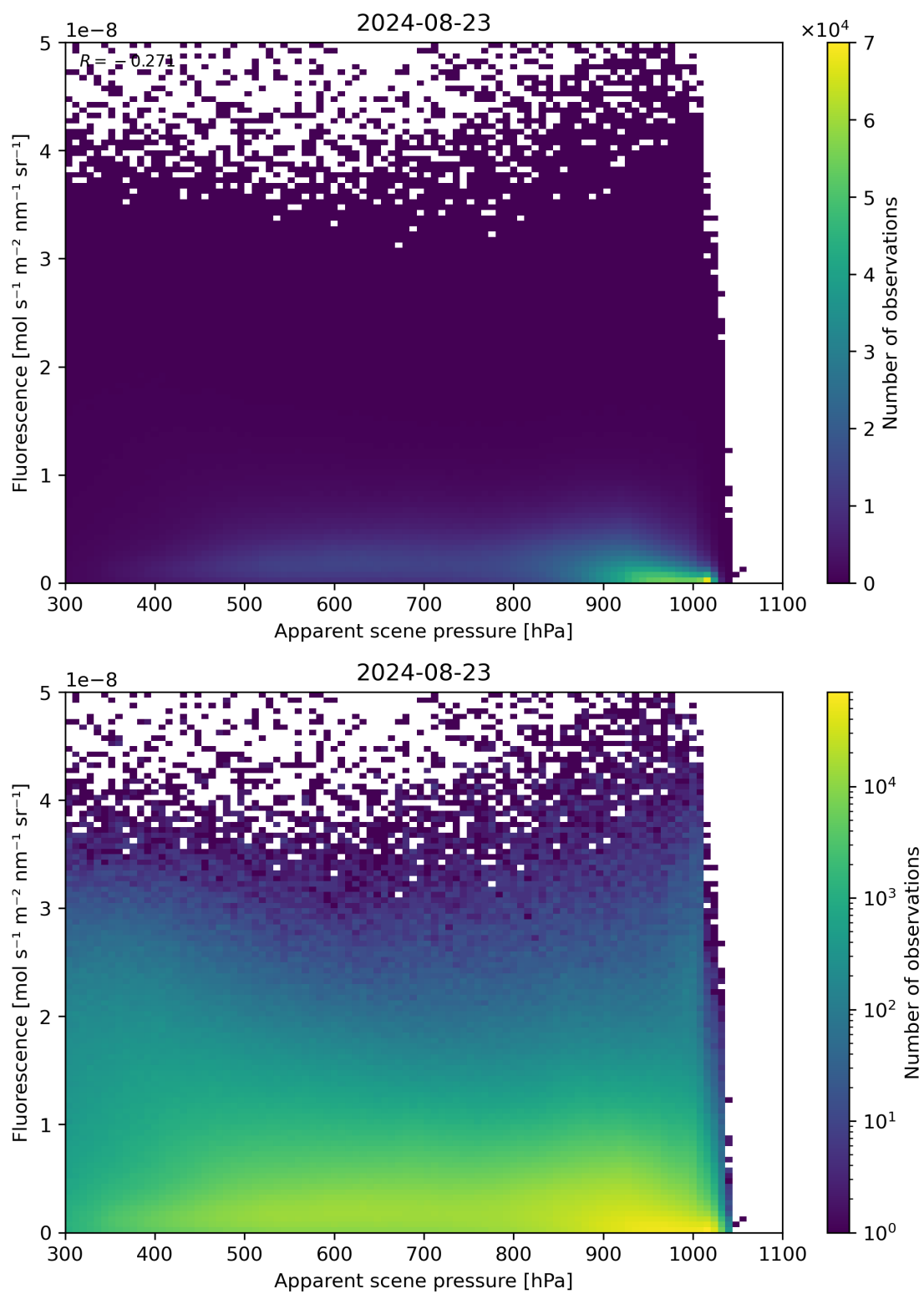
Figure 64: Scatter density plot of “Apparent scene pressure” against “Fluorescence” for 2024-08-22 to 2024-08-24.
