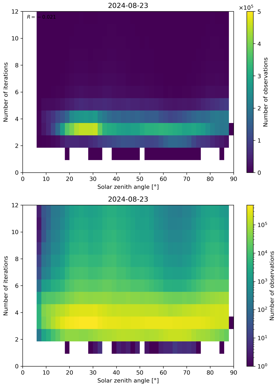
Figure 114: Scatter density plot of “Solar zenith angle” against “Number of iterations” for 2024-08-22 to 2024-08-24.
