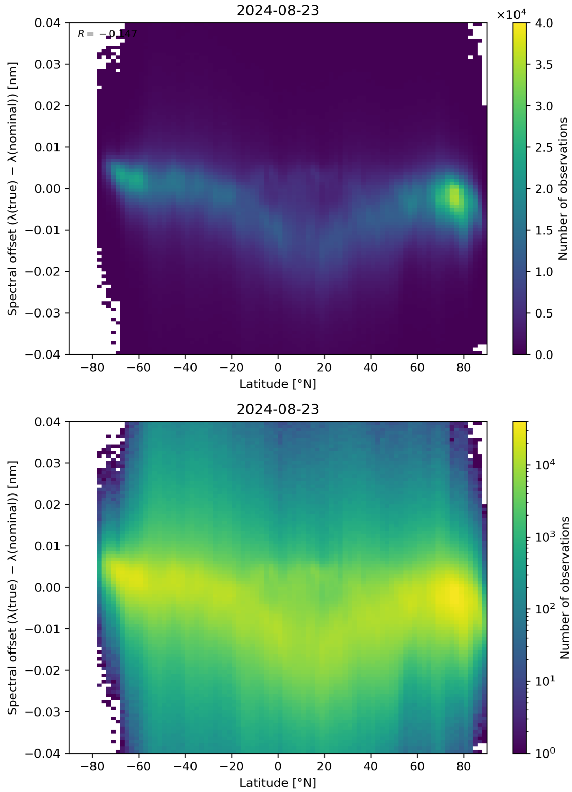
Figure 96: Scatter density plot of “Latitude” against “Spectral offset ( \lambda(\text{true}) - \lambda(\text{nominal}) )” for 2024-08-22 to 2024-08-24.
