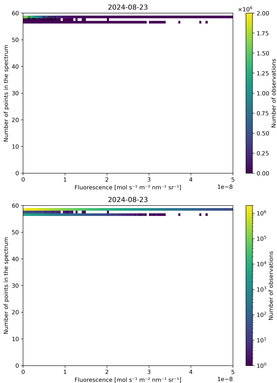
Figure 86: Scatter density plot of “Fluorescence” against “Number of points in the spectrum” for 2024-08-22 to 2024-08-24.
