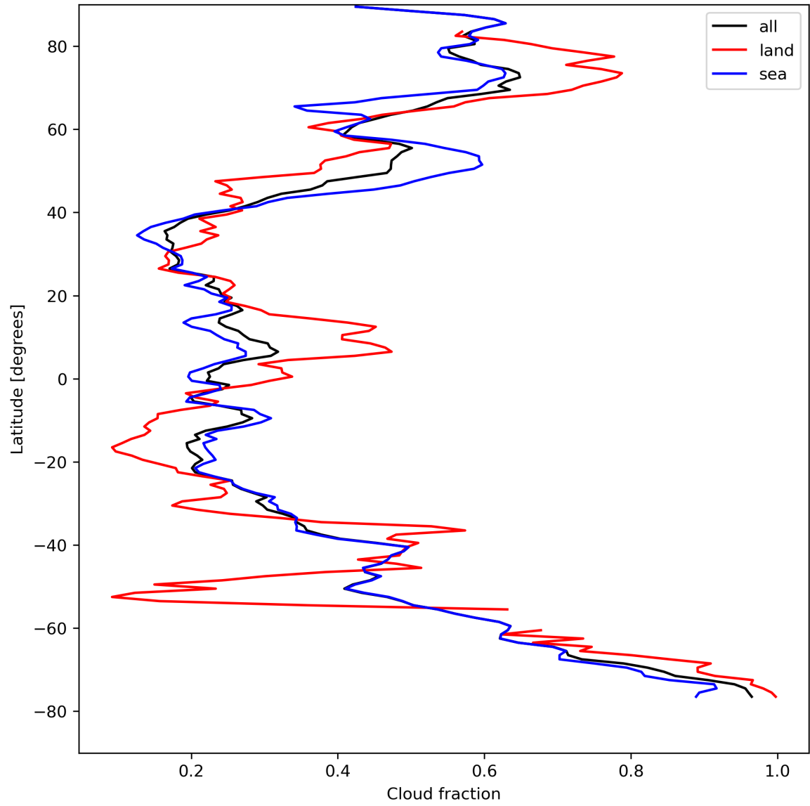
Figure 15: Zonal average of “Cloud fraction” for 2024-08-22 to 2024-08-24.
