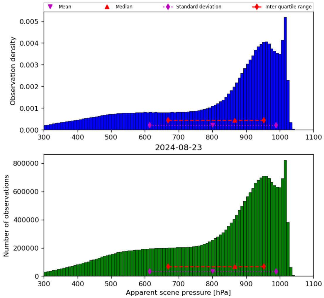
Figure 36: Histogram of “Apparent scene pressure” for 2024-08-22 to 2024-08-24
