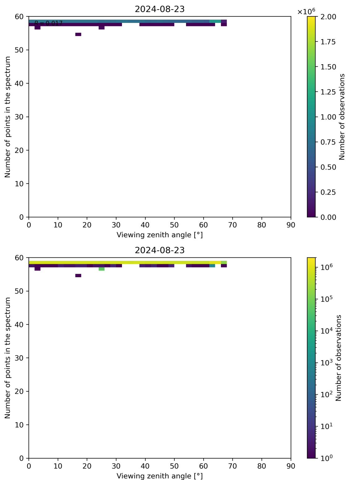
Figure 125: Scatter density plot of “Viewing zenith angle” against “Number of points in the spectrum” for 2024-08-22 to 2024-08-24.
