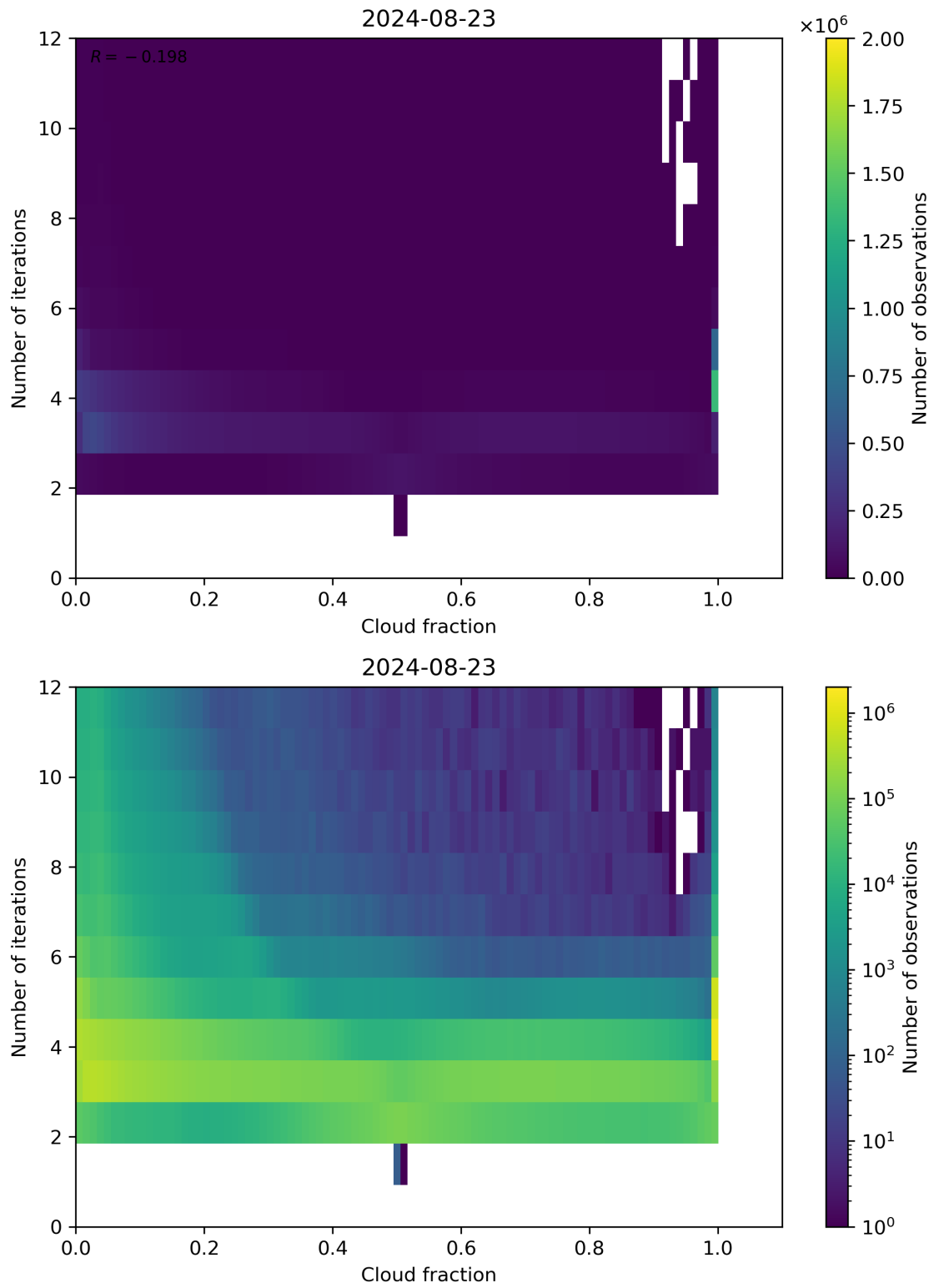
Figure 73: Scatter density plot of “Cloud fraction” against “Number of iterations” for 2024-08-22 to 2024-08-24.
