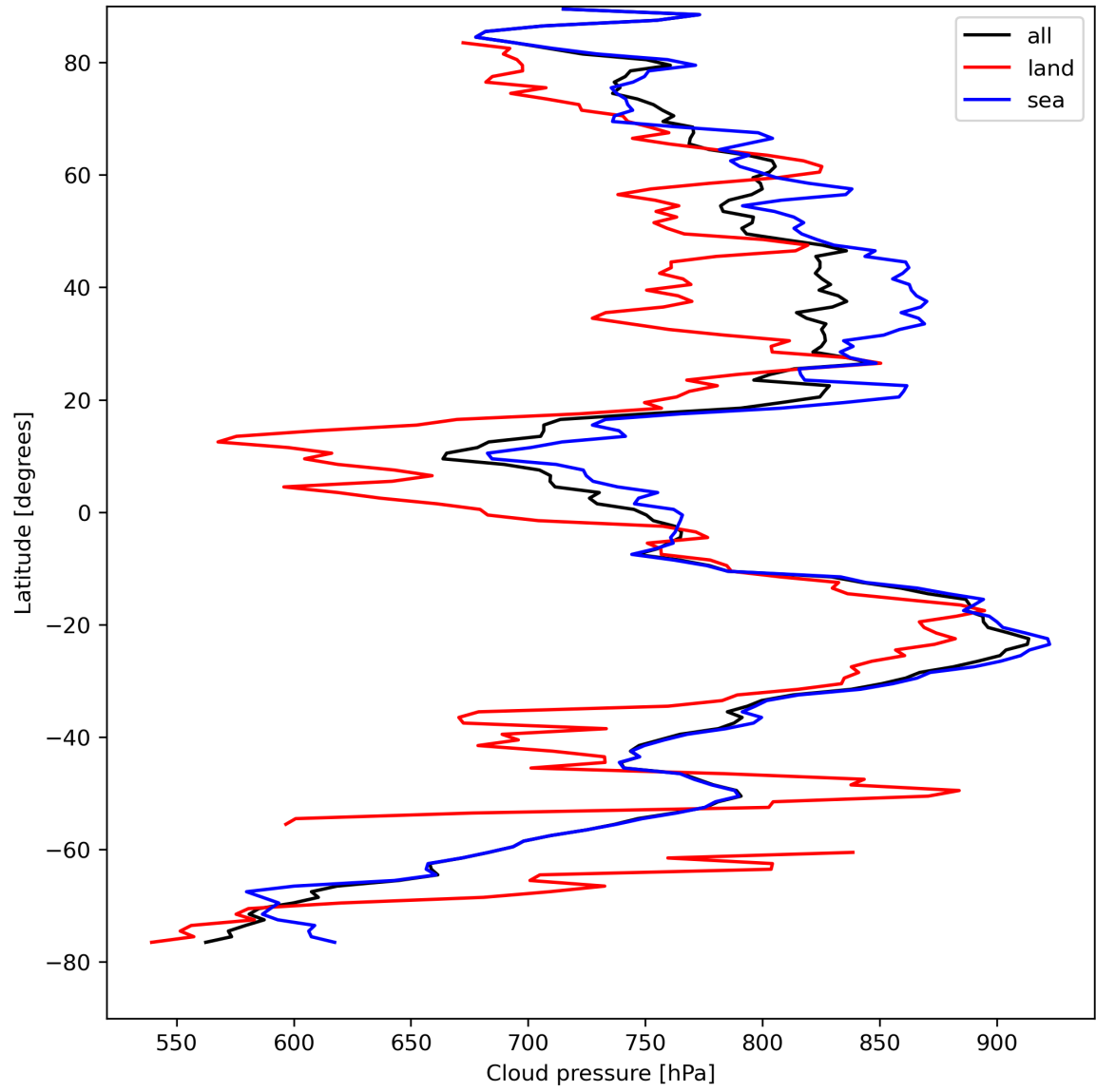
Figure 13: Zonal average of “Cloud pressure” for 2024-08-22 to 2024-08-24.
