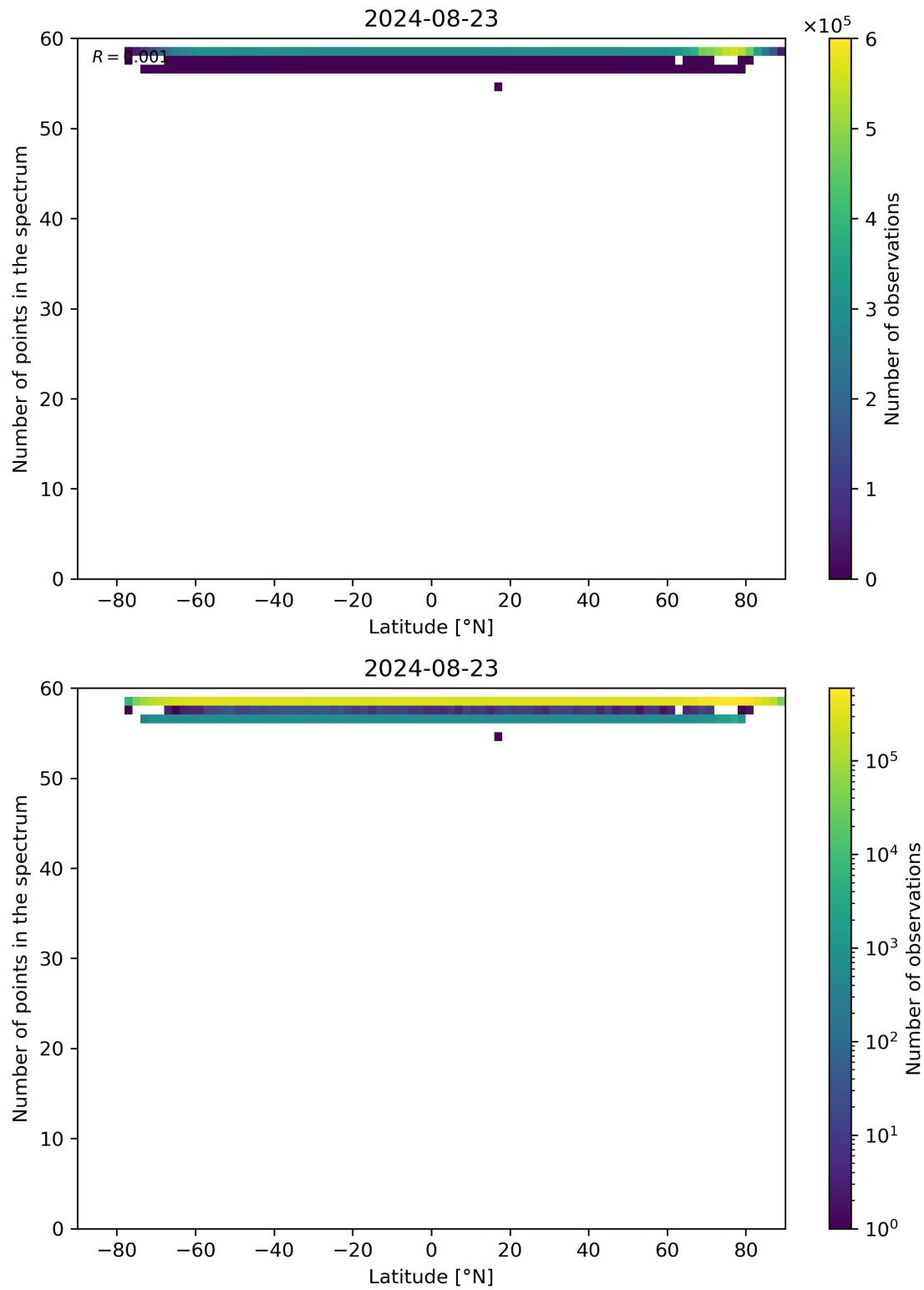
Figure 94: Scatter density plot of “Latitude” against “Number of points in the spectrum” for 2024-08-22 to 2024-08-24.
