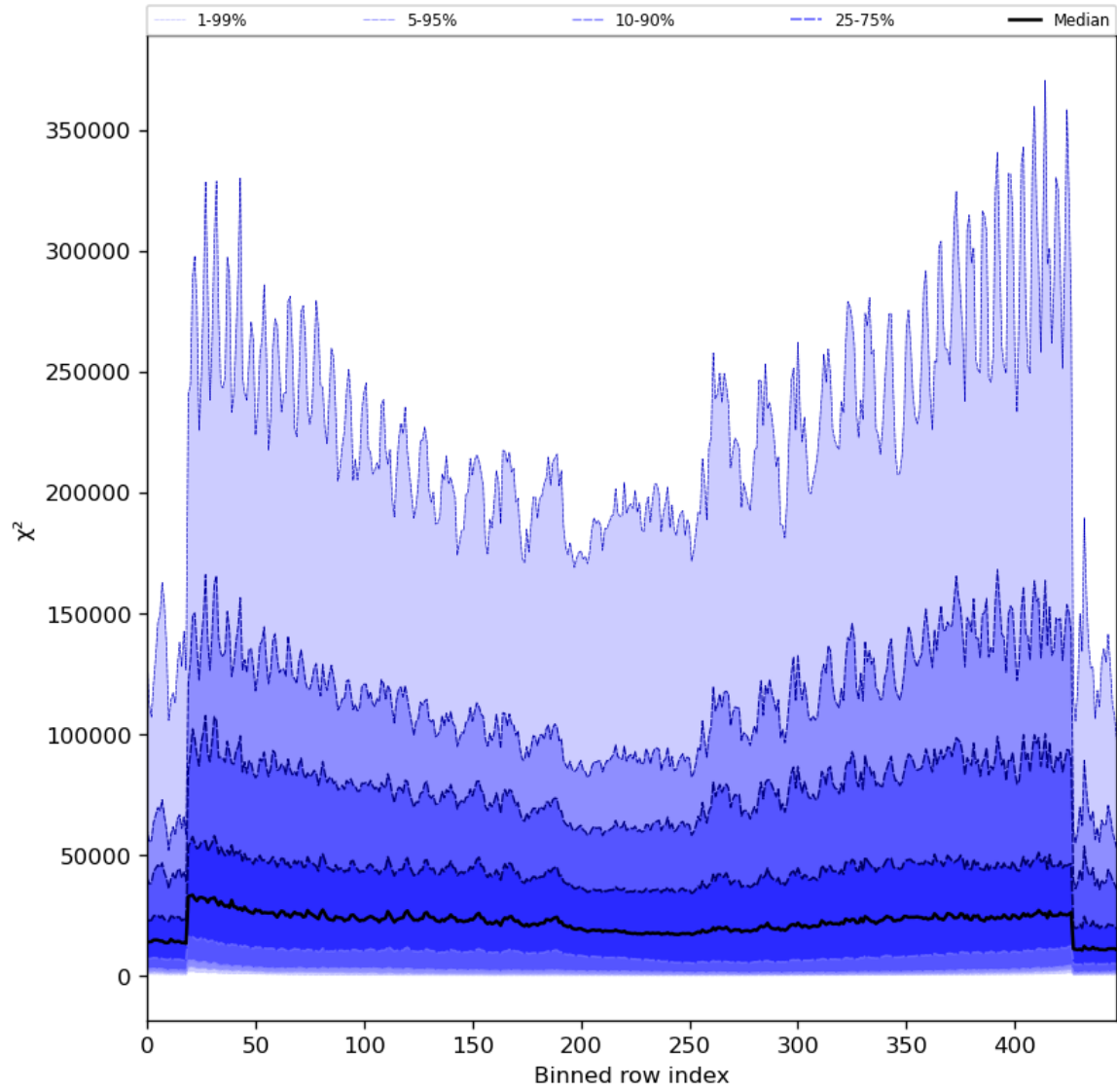
Figure 55: Along track statistics of “ \chi^2 ” for 2024-08-22 to 2024-08-24
