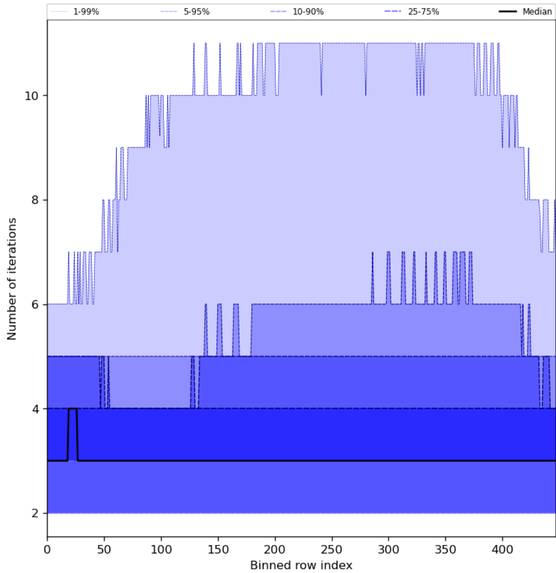
Figure 56: Along track statistics of “Number of iterations” for 2024-08-22 to 2024-08-24
