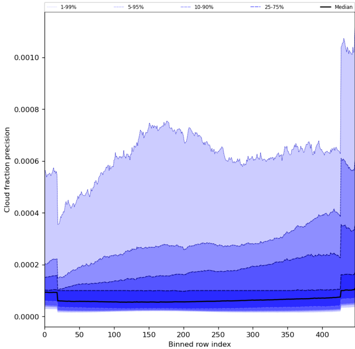
Figure 50: Along track statistics of “Cloud fraction precision” for 2024-08-22 to 2024-08-24
