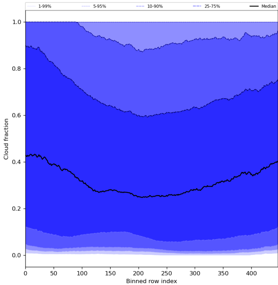
Figure 49: Along track statistics of “Cloud fraction” for 2024-08-22 to 2024-08-24
