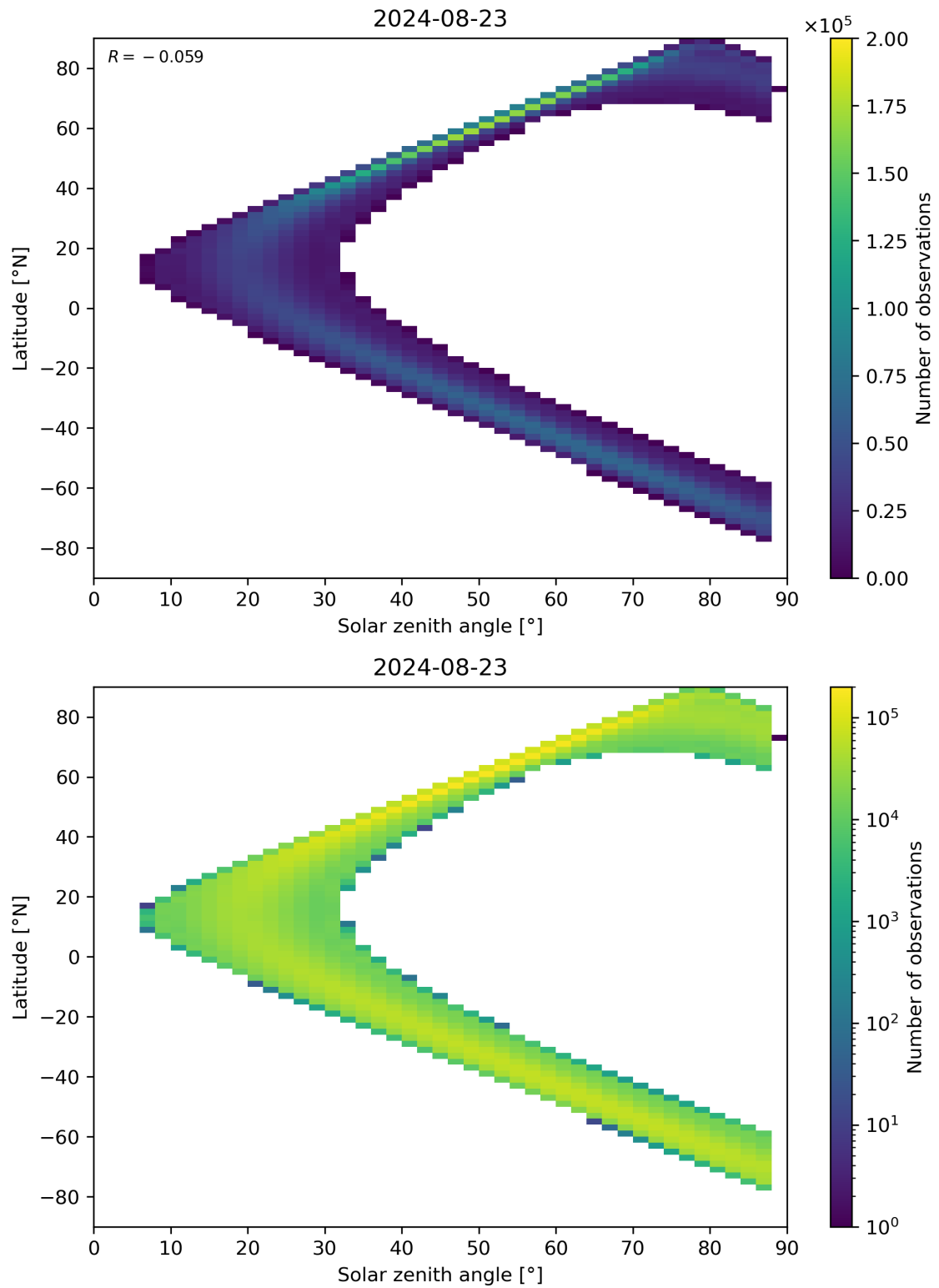
Figure 113: Scatter density plot of “Solar zenith angle” against “Latitude” for 2024-08-22 to 2024-08-24.
