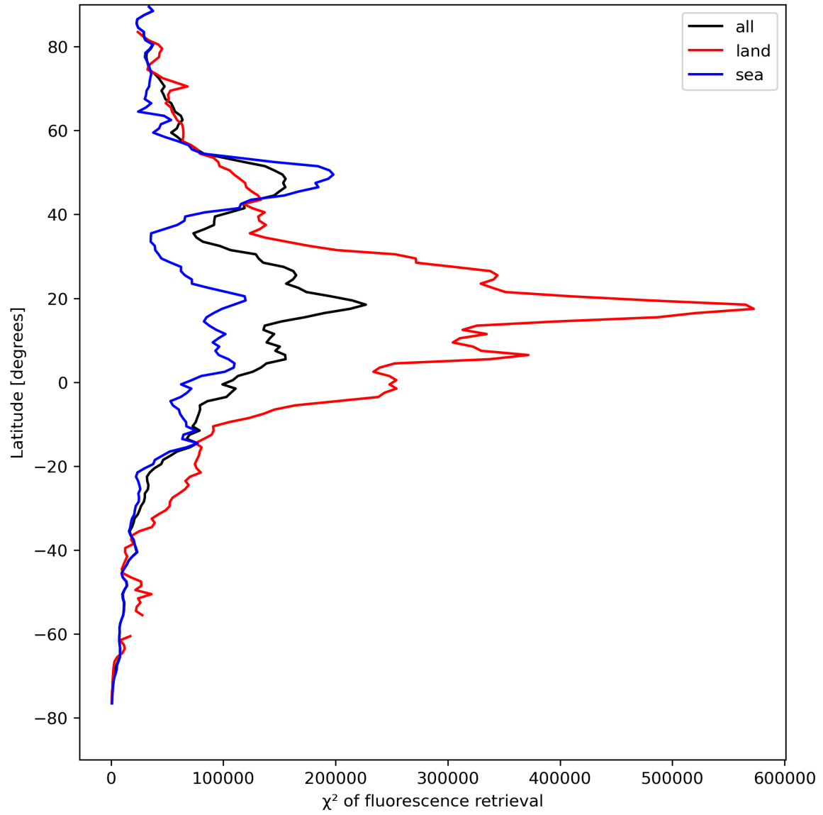
Figure 25: Zonal average of “ \chi^2 of fluorescence retrieval” for 2024-08-22 to 2024-08-24.
