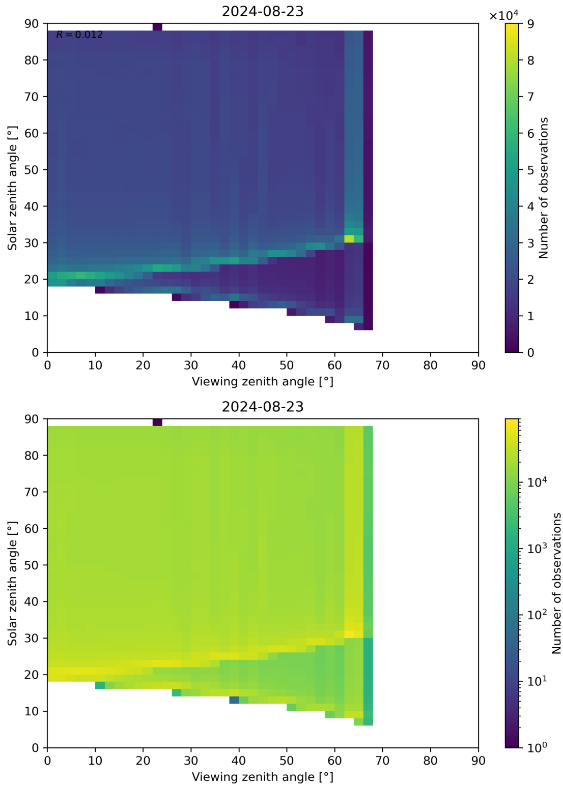
Figure 127: Scatter density plot of “Viewing zenith angle” against “Solar zenith angle” for 2024-08-22 to 2024-08-24.
