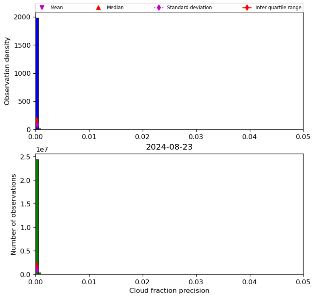
Figure 33: Histogram of “Cloud fraction precision” for 2024-08-22 to 2024-08-24
