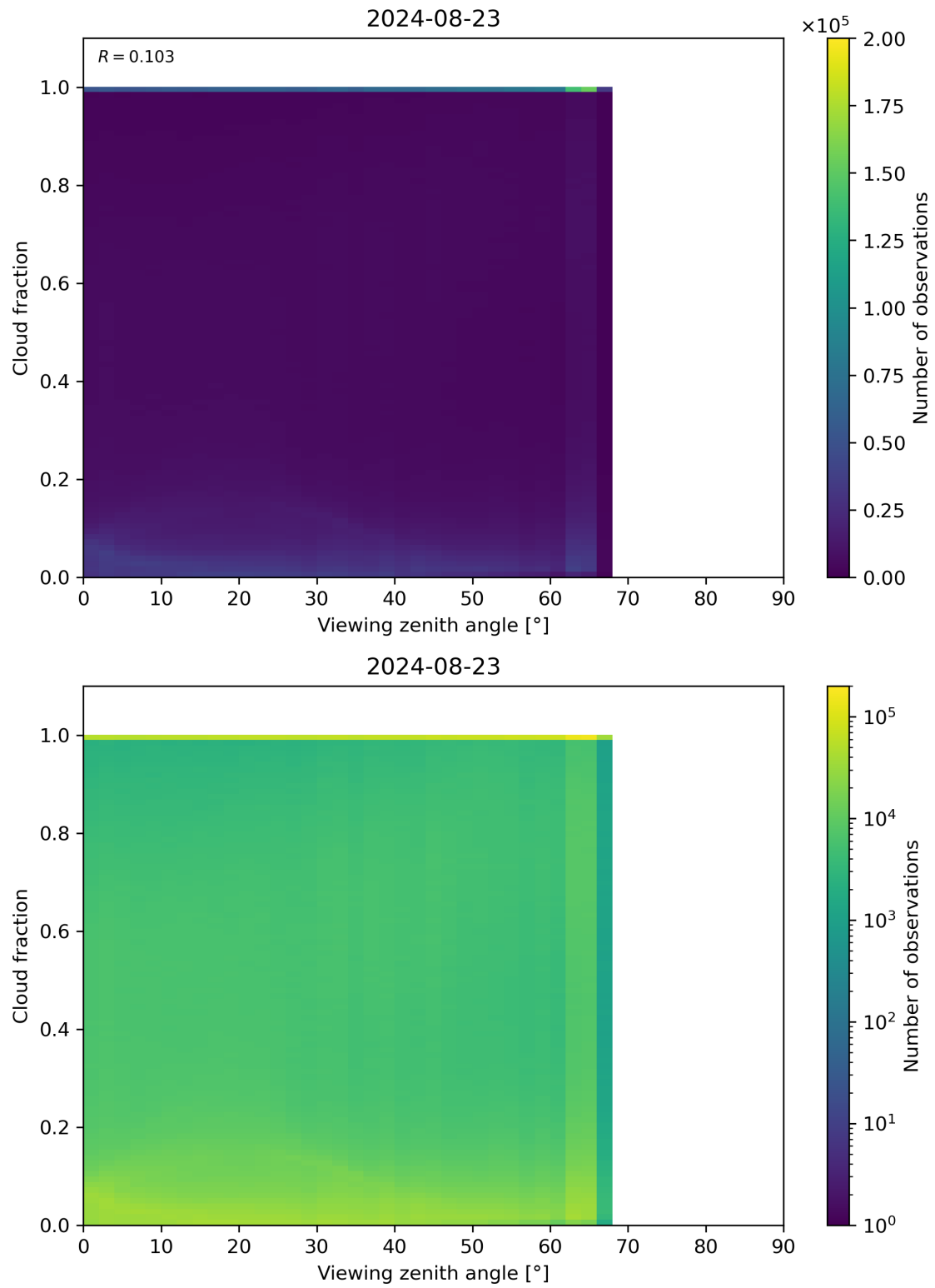
Figure 120: Scatter density plot of “Viewing zenith angle” against “Cloud fraction” for 2024-08-22 to 2024-08-24.
