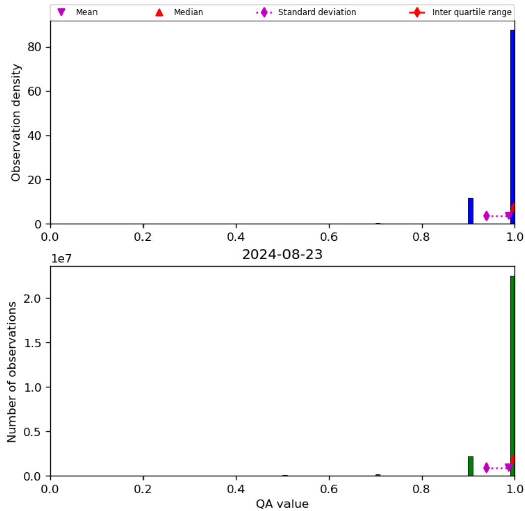
Figure 29: Histogram of “QA value” for 2024-08-22 to 2024-08-24
