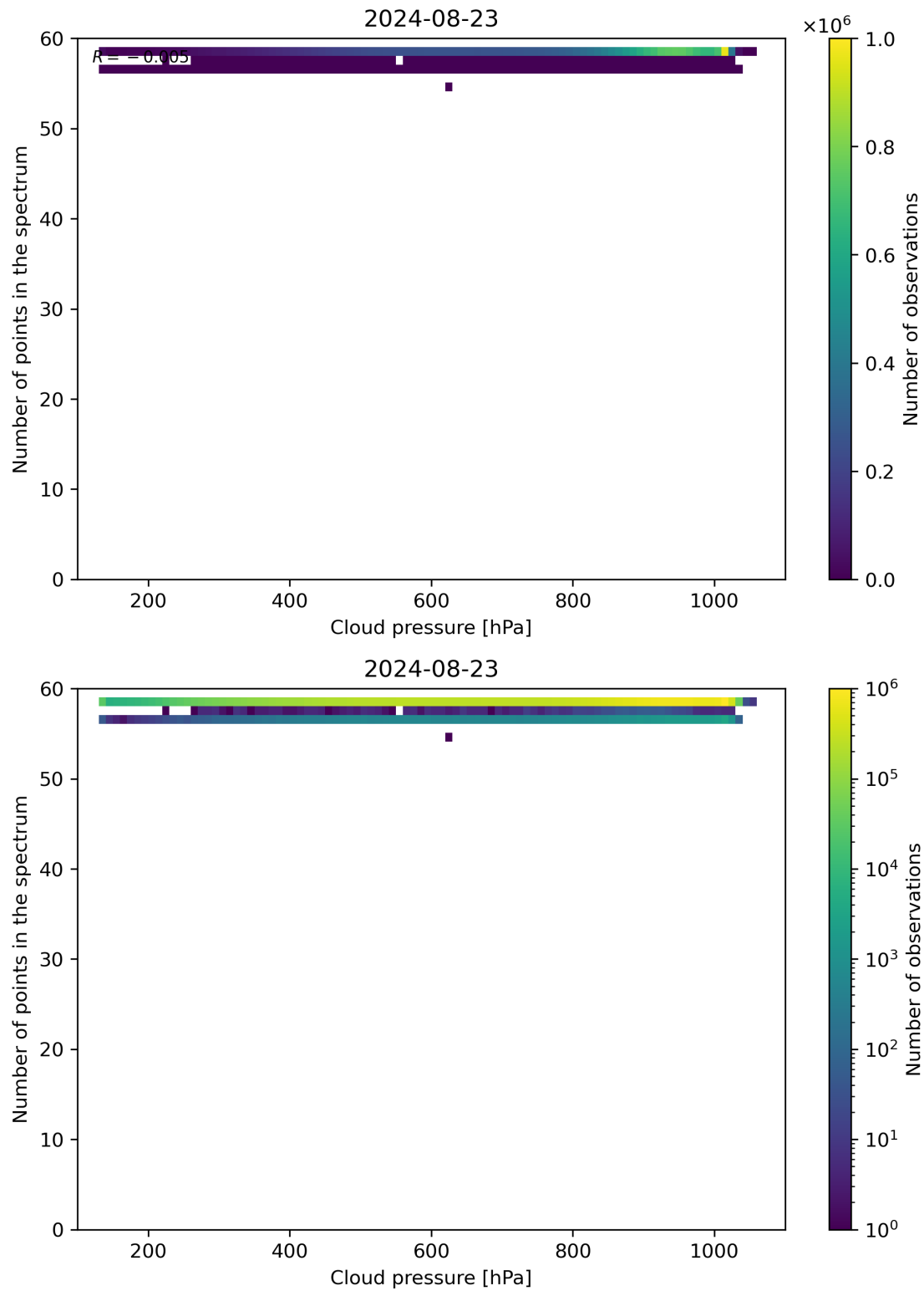
Figure 82: Scatter density plot of “Cloud pressure” against “Number of points in the spectrum” for 2024-08-22 to 2024-08-24.
