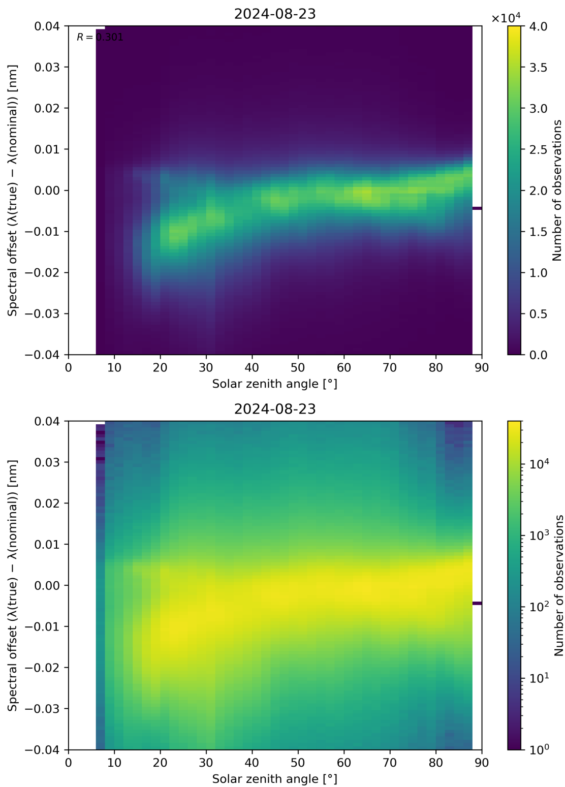
Figure 117: Scatter density plot of “Solar zenith angle” against “Spectral offset ( \lambda(\text{true}) - \lambda(\text{nominal}) )” for 2024-08-22 to 2024-08-24.
