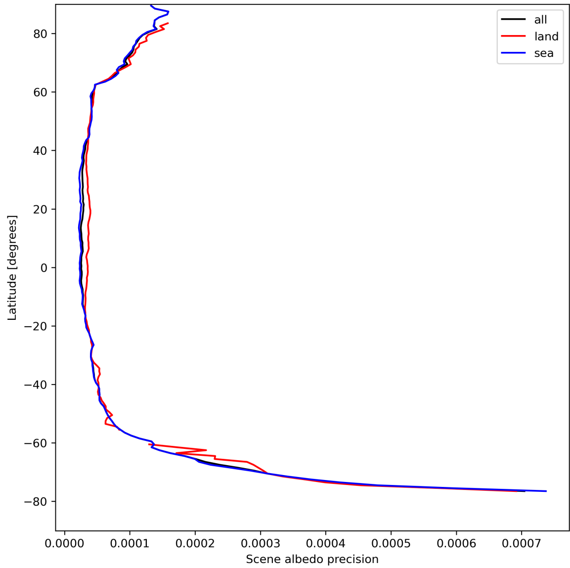
Figure 18: Zonal average of “Scene albedo precision” for 2024-08-22 to 2024-08-24.
