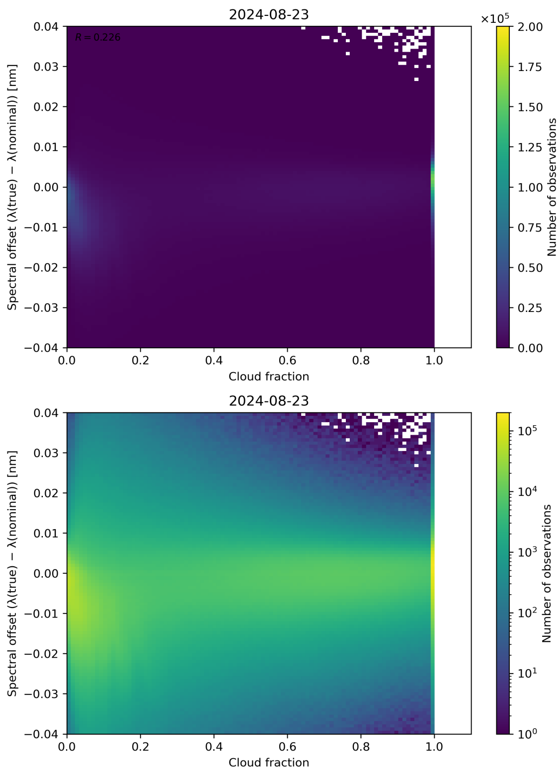
Figure 76: Scatter density plot of “Cloud fraction” against “Spectral offset ( \lambda(\text{true}) - \lambda(\text{nominal}) )” for 2024-08-22 to 2024-08-24.
