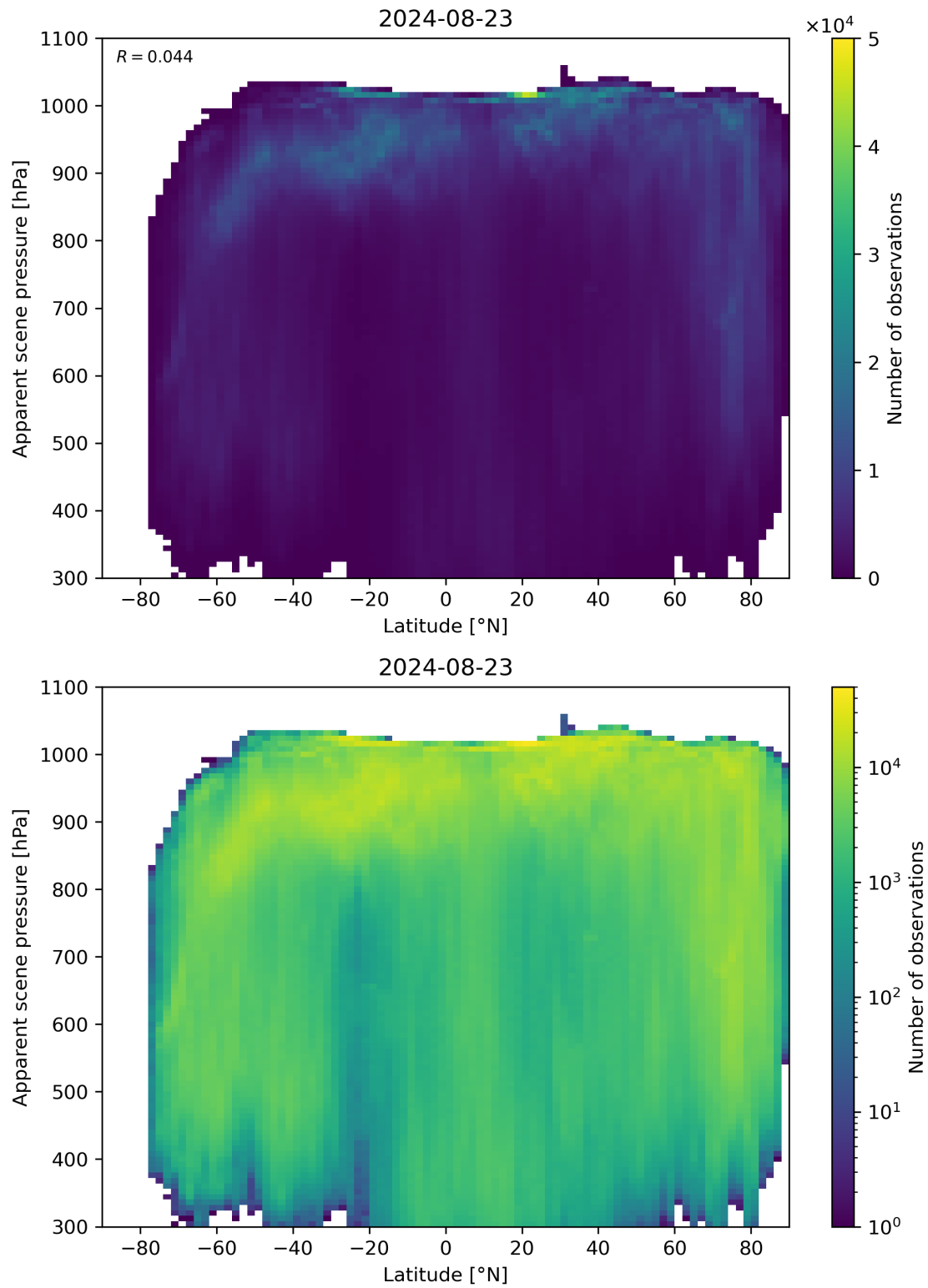
Figure 88: Scatter density plot of “Latitude” against “Apparent scene pressure” for 2024-08-22 to 2024-08-24.
