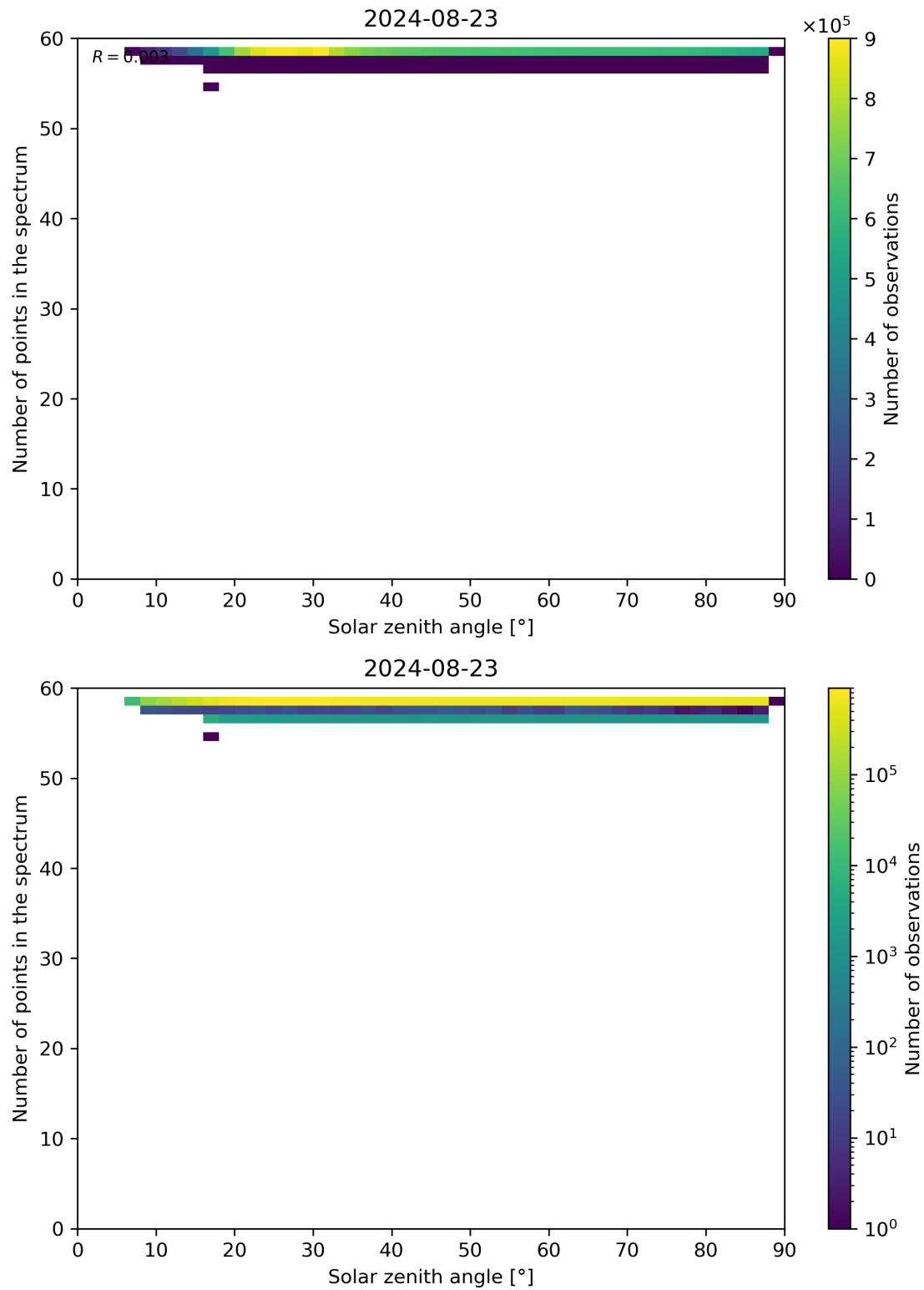
Figure 115: Scatter density plot of “Solar zenith angle” against “Number of points in the spectrum” for 2024-08-22 to 2024-08-24.
