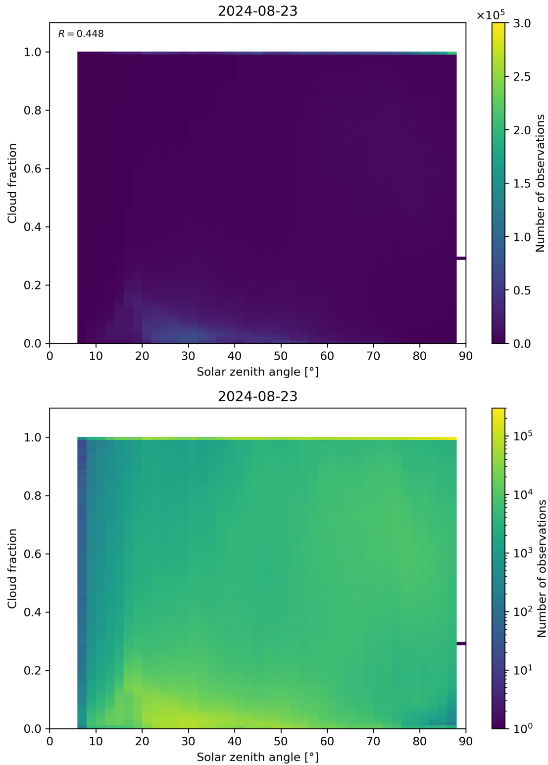
Figure 110: Scatter density plot of “Solar zenith angle” against “Cloud fraction” for 2024-08-22 to 2024-08-24.
