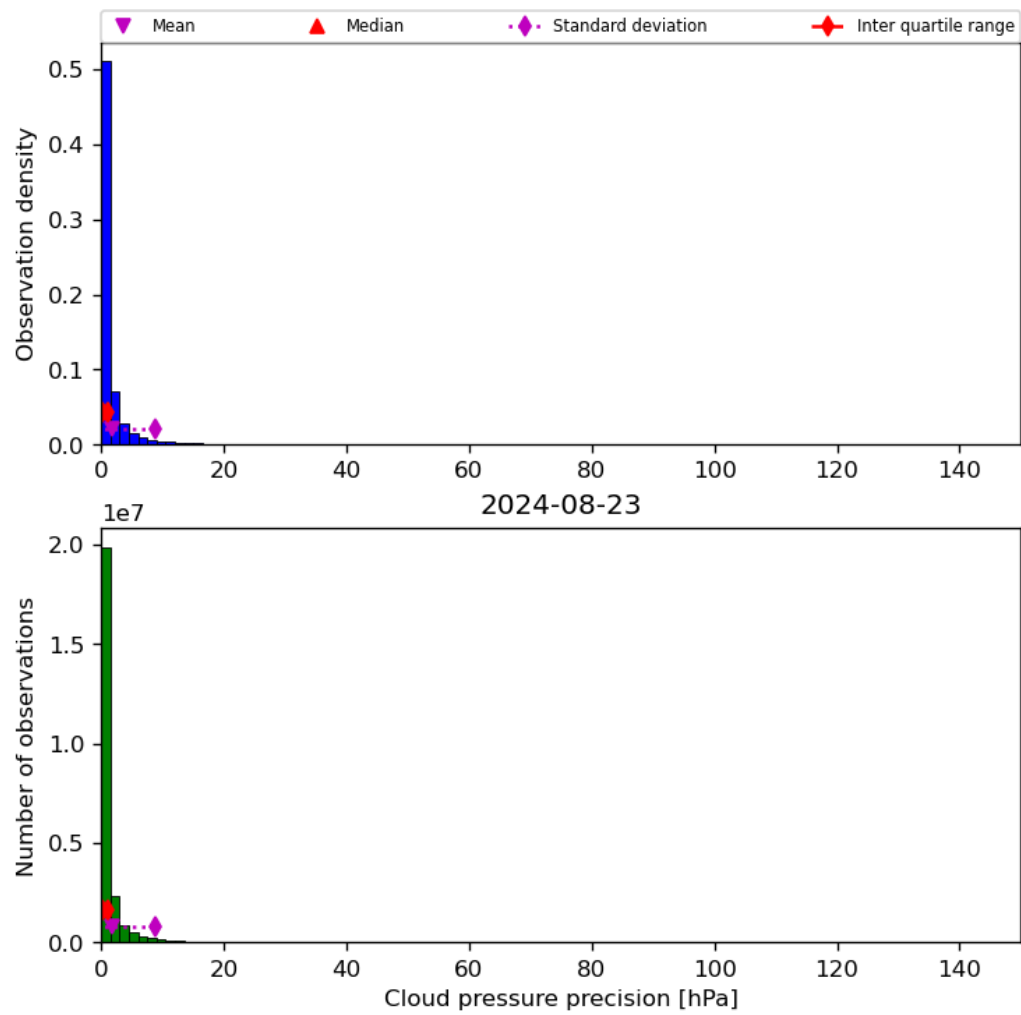
Figure 31: Histogram of “Cloud pressure precision” for 2024-08-22 to 2024-08-24
