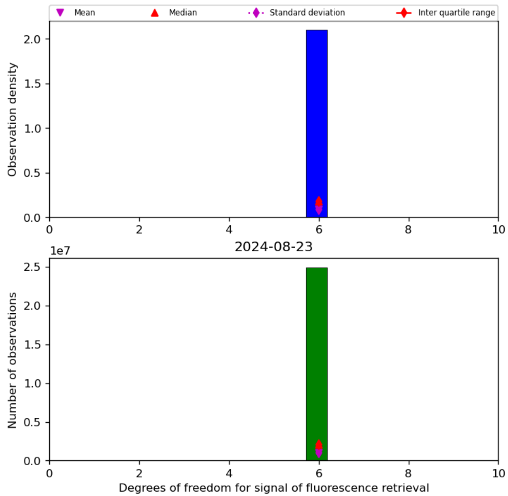
Figure 43: Histogram of “Degrees of freedom for signal of fluorescence retrieval” for 2024-08-22 to 2024-08-24
