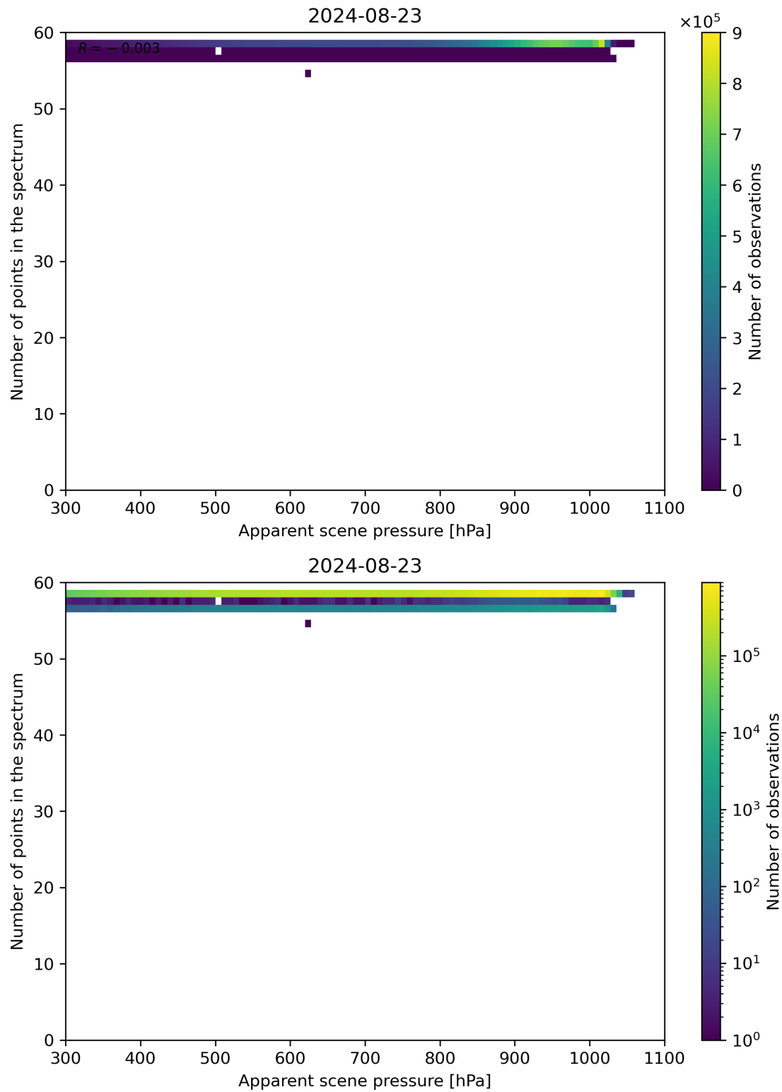
Figure 66: Scatter density plot of “Apparent scene pressure” against “Number of points in the spectrum” for 2024-08-22 to 2024-08-24.
