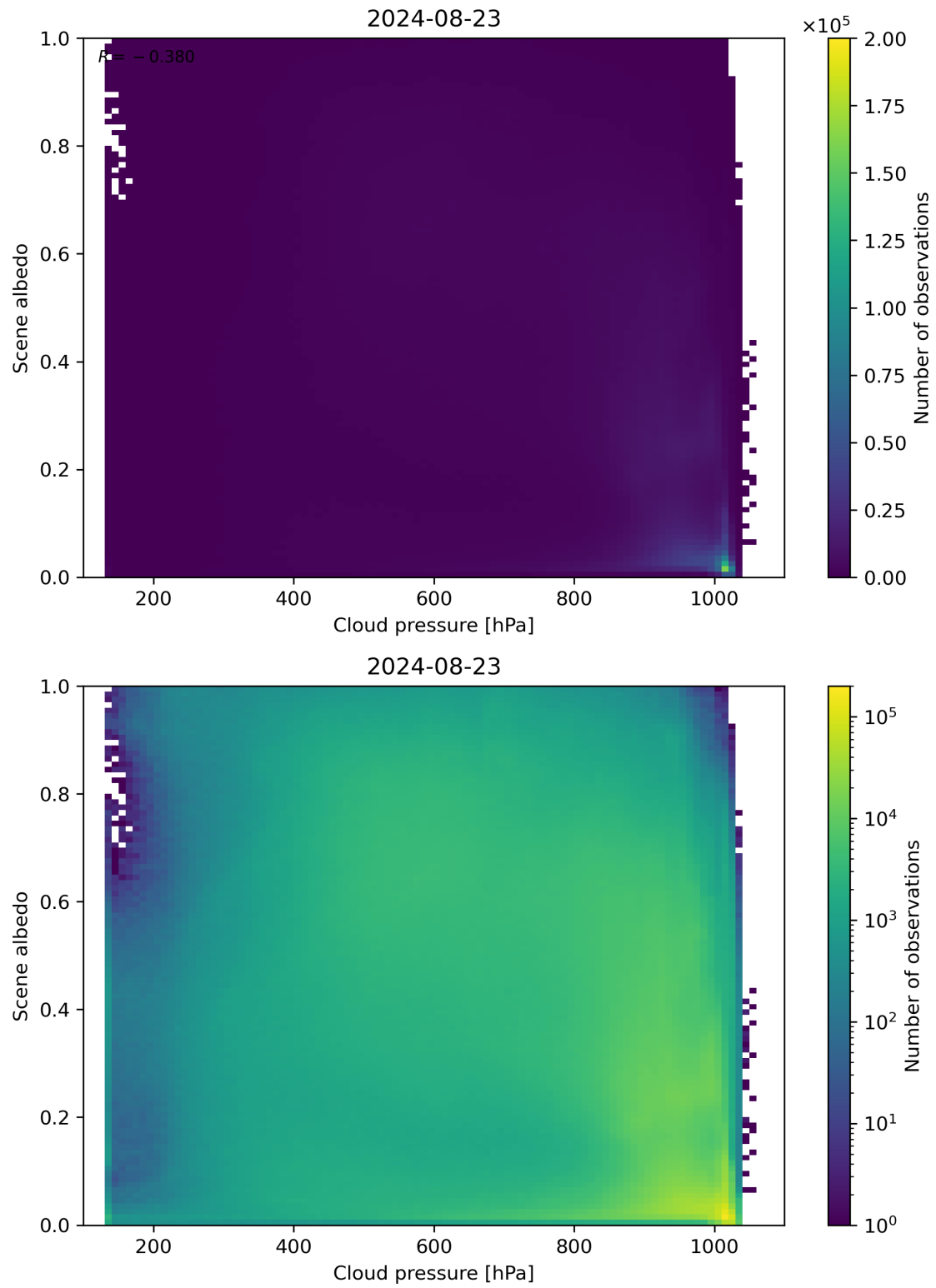
Figure 83: Scatter density plot of “Cloud pressure” against “Scene albedo” for 2024-08-22 to 2024-08-24.
