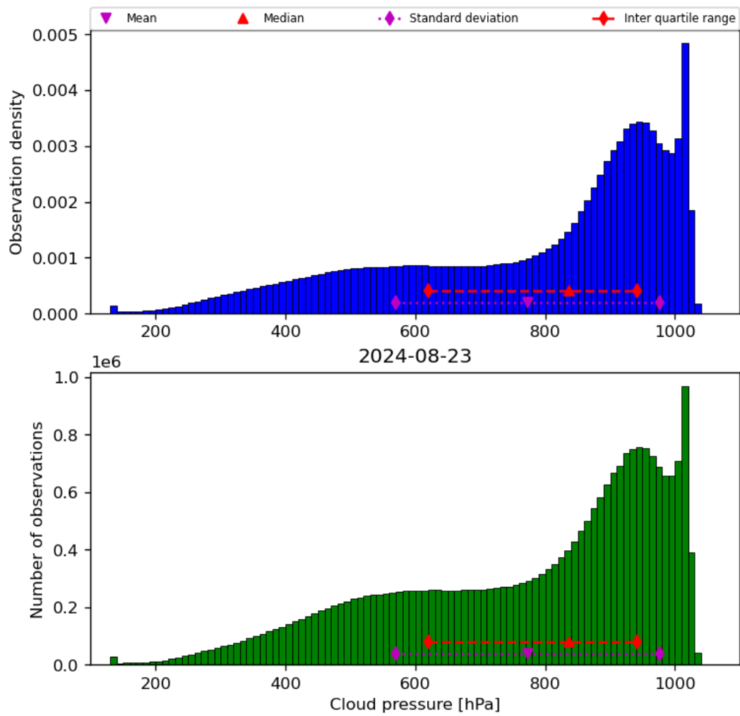
Figure 30: Histogram of “Cloud pressure” for 2024-08-22 to 2024-08-24
