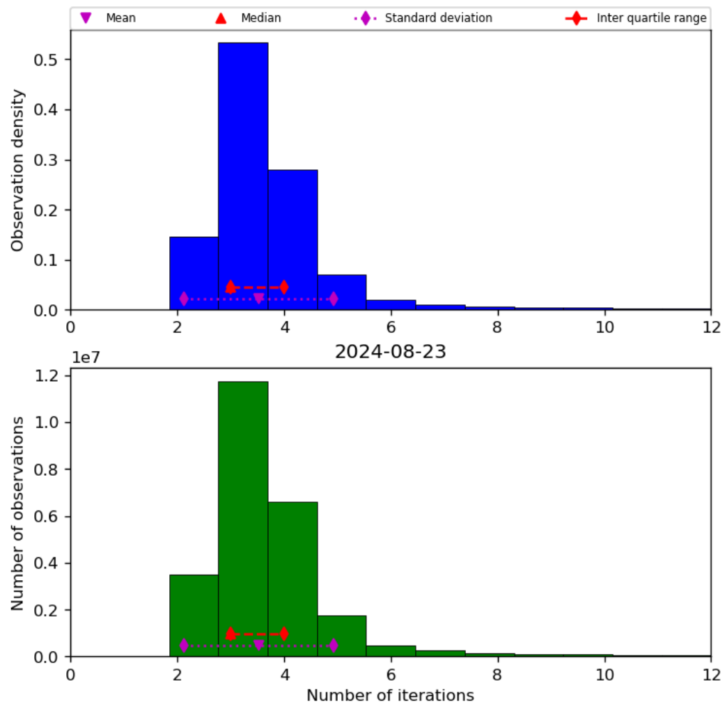
Figure 39: Histogram of “Number of iterations” for 2024-08-22 to 2024-08-24
