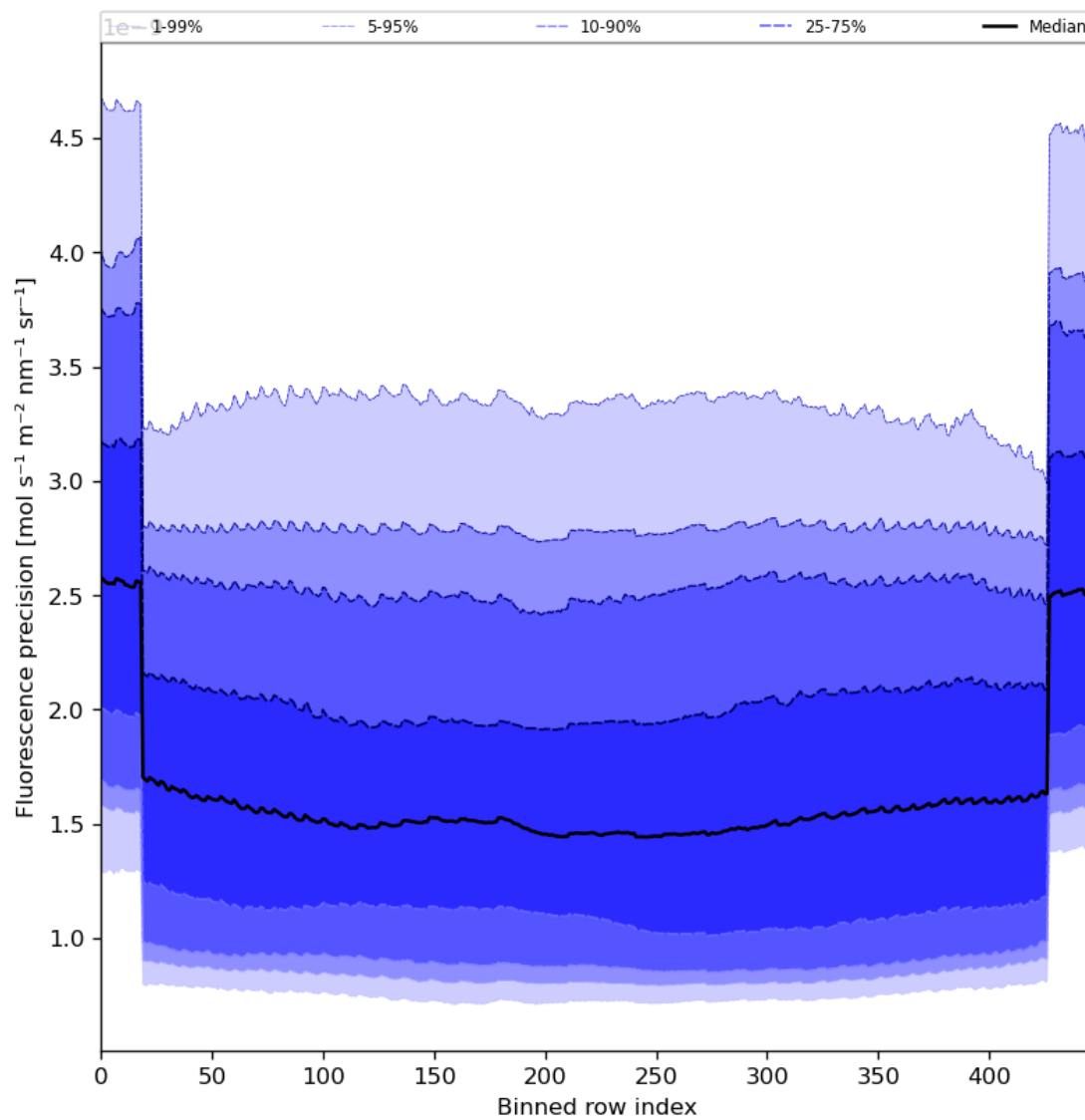
Figure 58: Along track statistics of “Fluorescence precision” for 2024-08-22 to 2024-08-24
