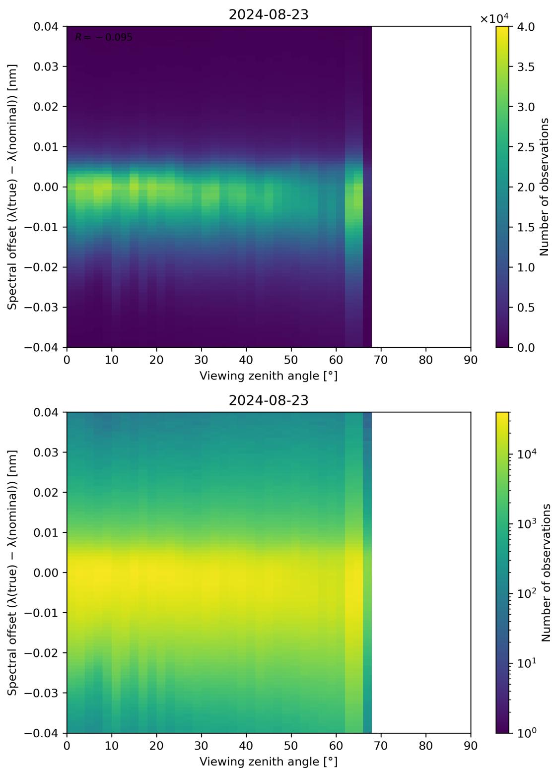
Figure 128: Scatter density plot of “Viewing zenith angle” against “Spectral offset ( \lambda(\text{true}) - \lambda(\text{nominal}) )” for 2024-08-22 to 2024-08-24.
