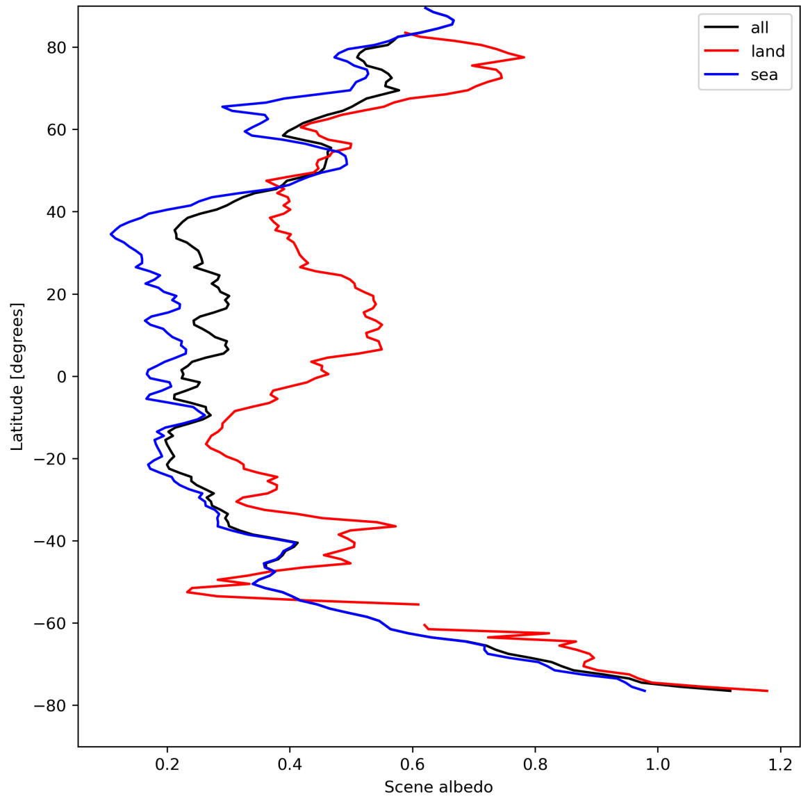
Figure 17: Zonal average of “Scene albedo” for 2024-08-22 to 2024-08-24.
