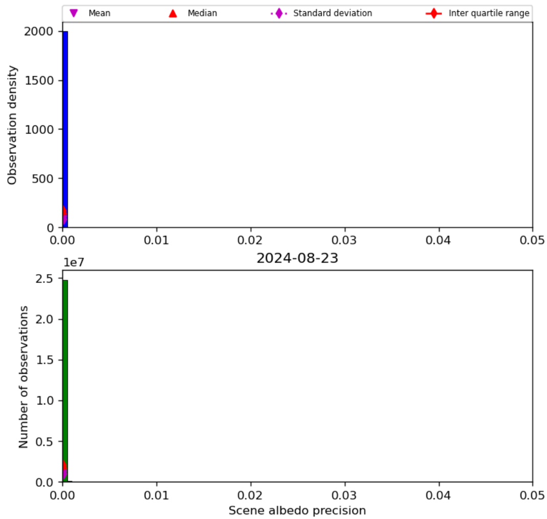
Figure 35: Histogram of “Scene albedo precision” for 2024-08-22 to 2024-08-24
