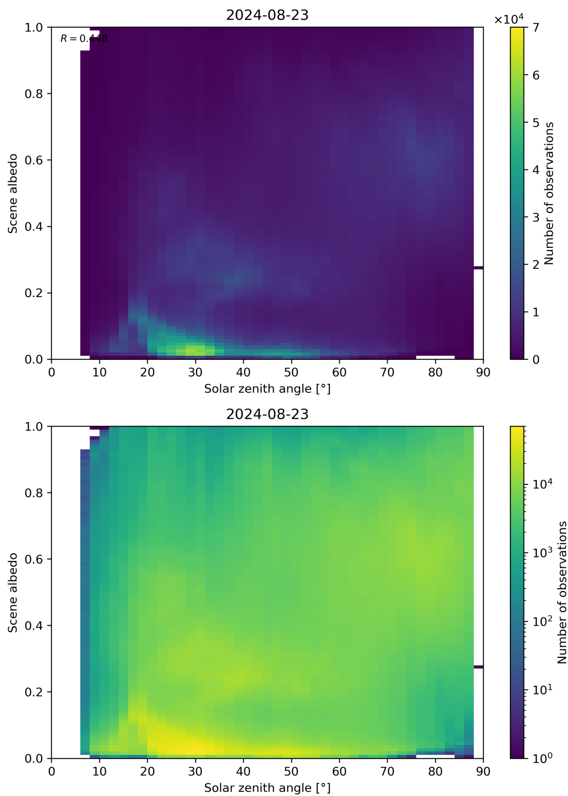
Figure 116: Scatter density plot of “Solar zenith angle” against “Scene albedo” for 2024-08-22 to 2024-08-24.
