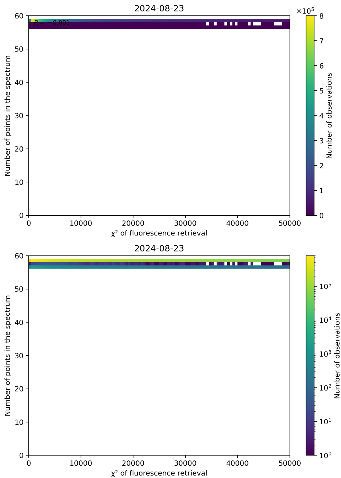
Figure 68: Scatter density plot of " \chi^2 of fluorescence retrieval" against "Number of points in the spectrum" for 2024-08-22 to 2024-08-24.
