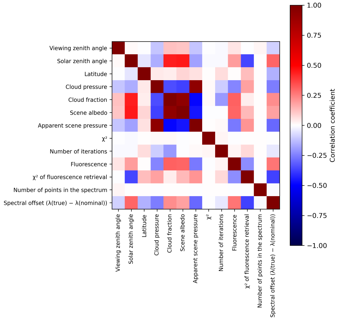
Figure 2: Map of correlation matrix for 2024-08-23 to 2024-08-25.
