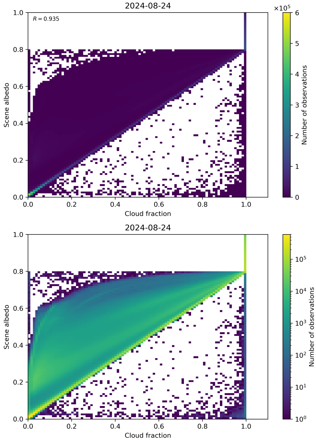
Figure 75: Scatter density plot of “Cloud fraction” against “Scene albedo” for 2024-08-23 to 2024-08-25.
