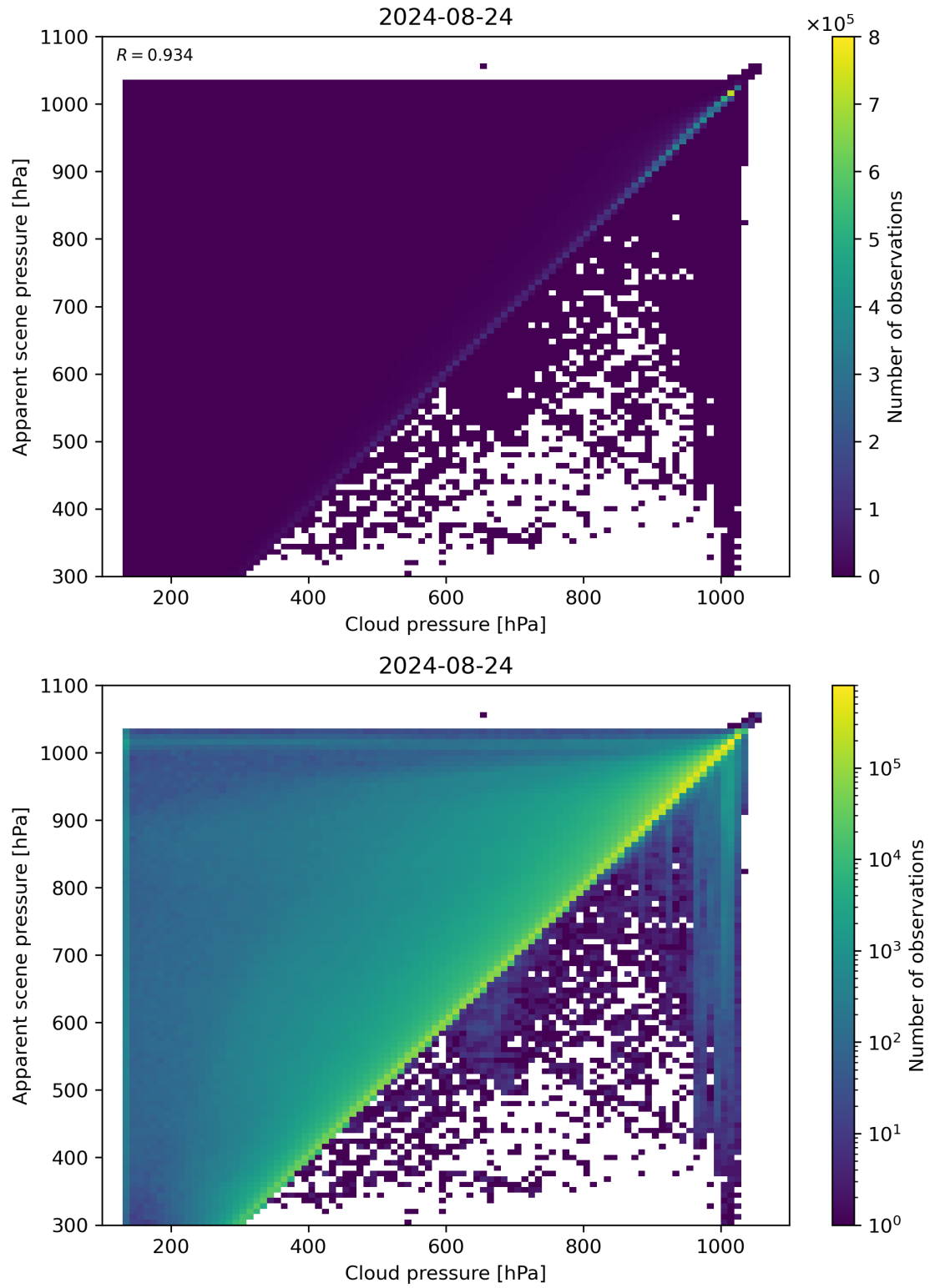
Figure 77: Scatter density plot of “Cloud pressure” against “Apparent scene pressure” for 2024-08-23 to 2024-08-25.
