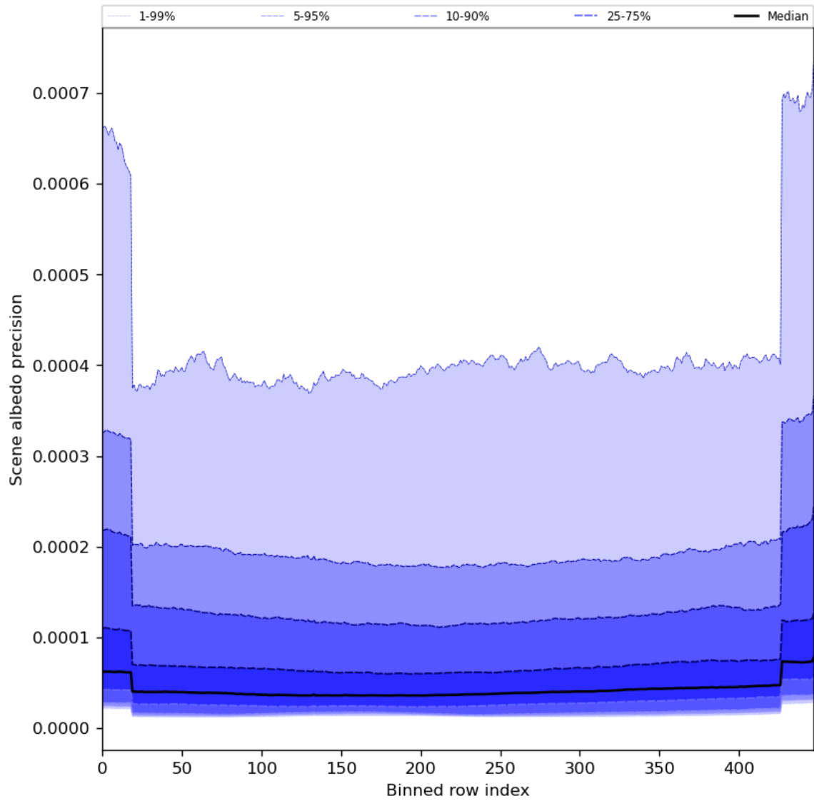
Figure 52: Along track statistics of “Scene albedo precision” for 2024-08-23 to 2024-08-25
