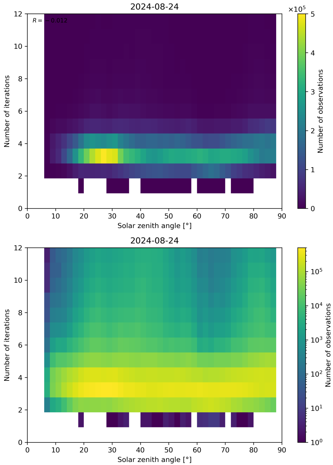
Figure 114: Scatter density plot of “Solar zenith angle” against “Number of iterations” for 2024-08-23 to 2024-08-25.
