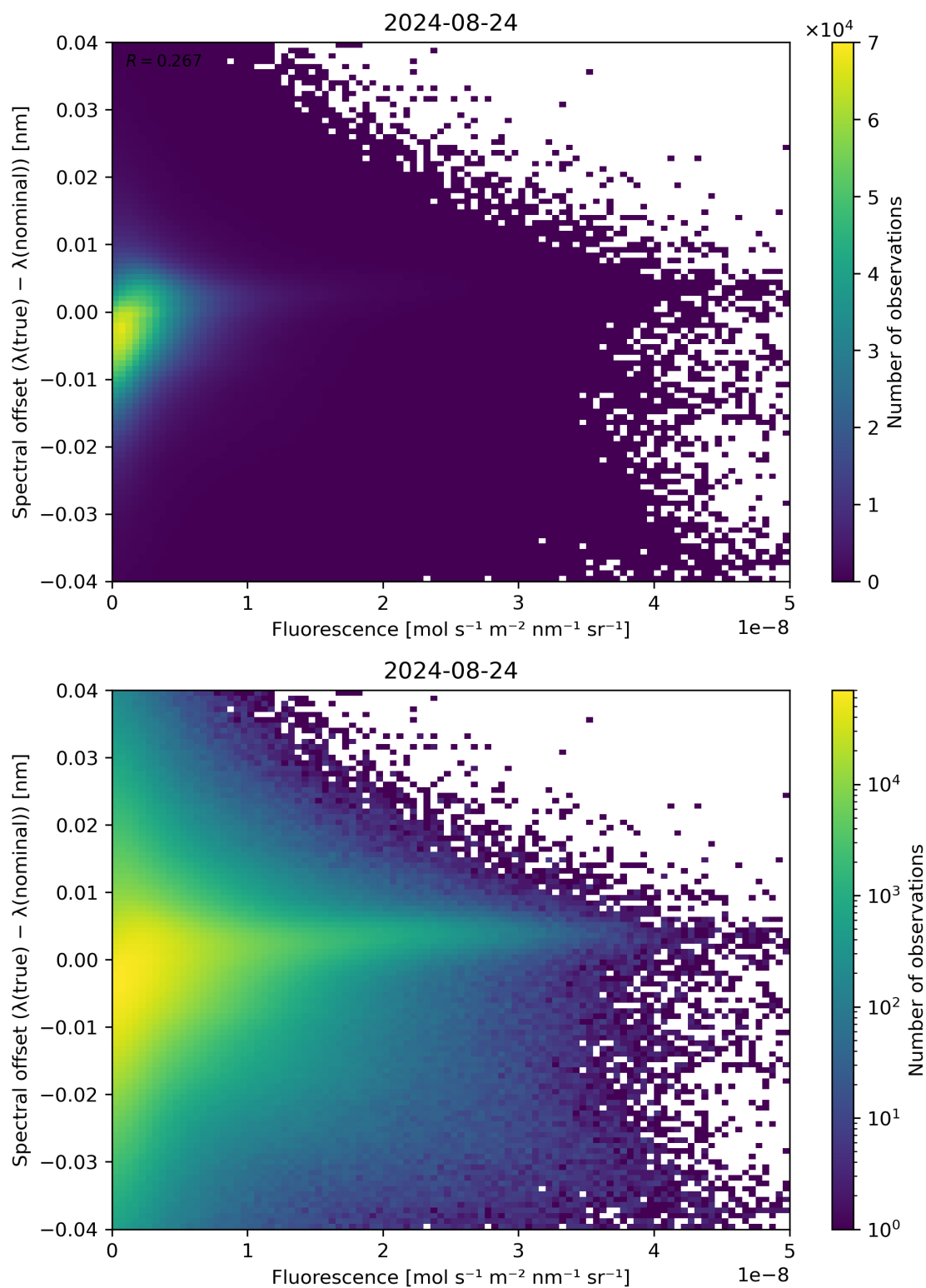
Figure 87: Scatter density plot of “Fluorescence” against “Spectral offset ( \lambda(\text{true}) - \lambda(\text{nominal}) )” for 2024-08-23 to 2024-08-25.
