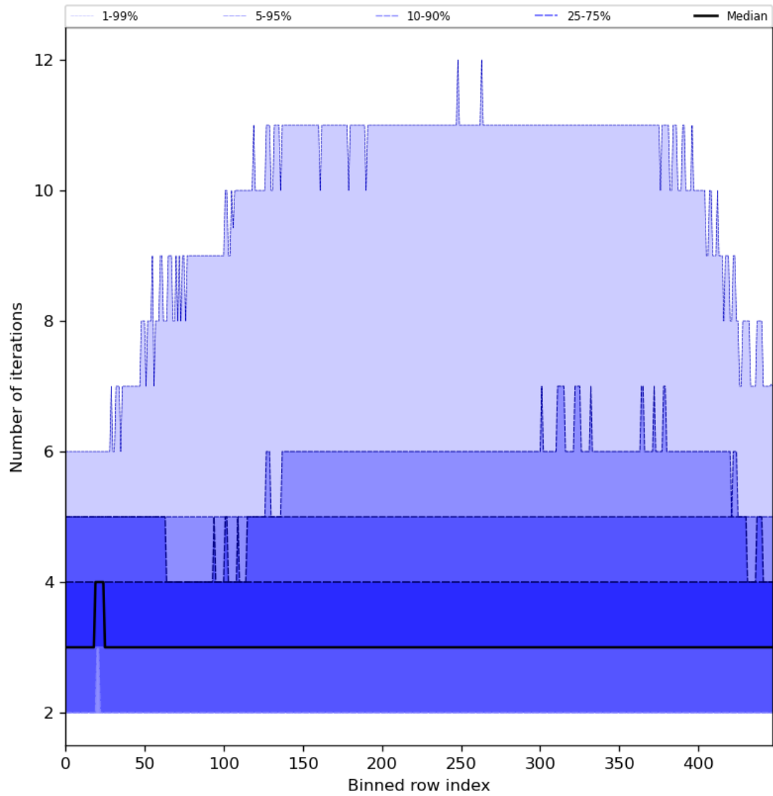
Figure 56: Along track statistics of “Number of iterations” for 2024-08-23 to 2024-08-25
