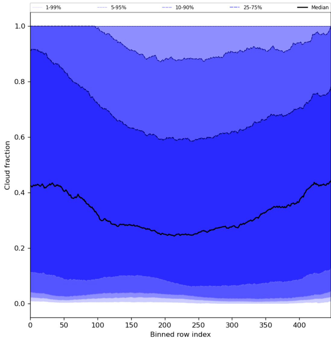
Figure 49: Along track statistics of “Cloud fraction” for 2024-08-23 to 2024-08-25
