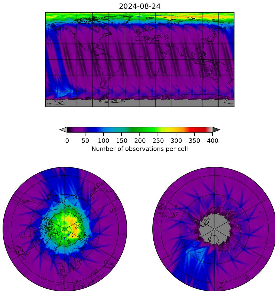
Figure 11: Map of the number of observations for 2024-08-23 to 2024-08-25
