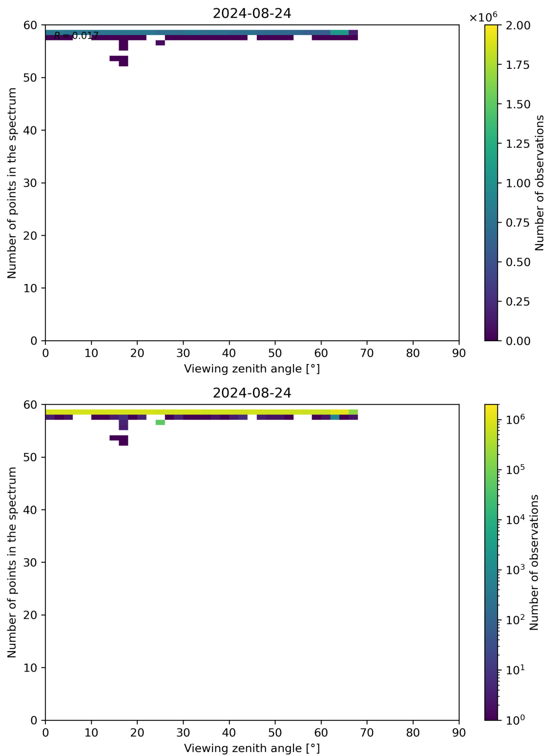
Figure 125: Scatter density plot of “Viewing zenith angle” against “Number of points in the spectrum” for 2024-08-23 to 2024-08-25.
