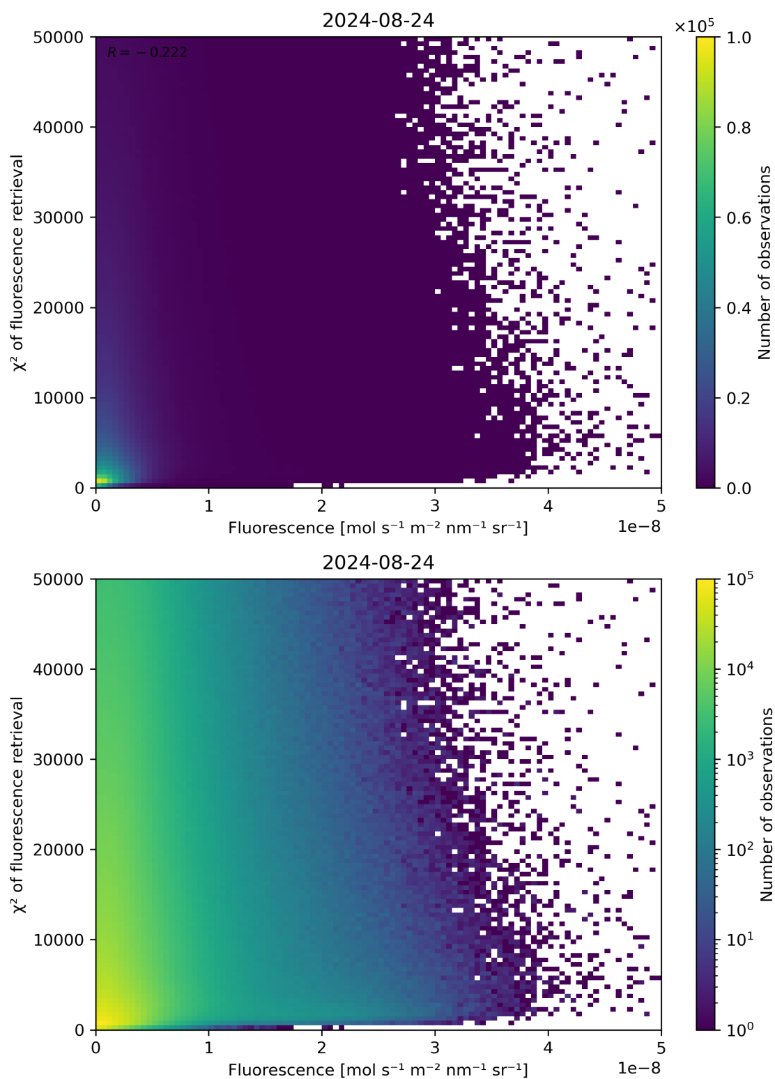
Figure 85: Scatter density plot of “Fluorescence” against “ \chi^2 of fluorescence retrieval” for 2024-08-23 to 2024-08-25.
