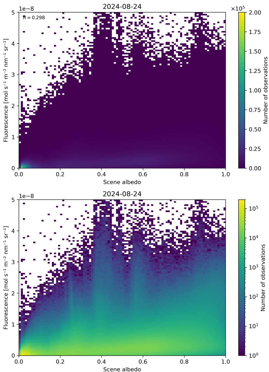
Figure 104: Scatter density plot of “Scene albedo” against “Fluorescence” for 2024-08-23 to 2024-08-25.
