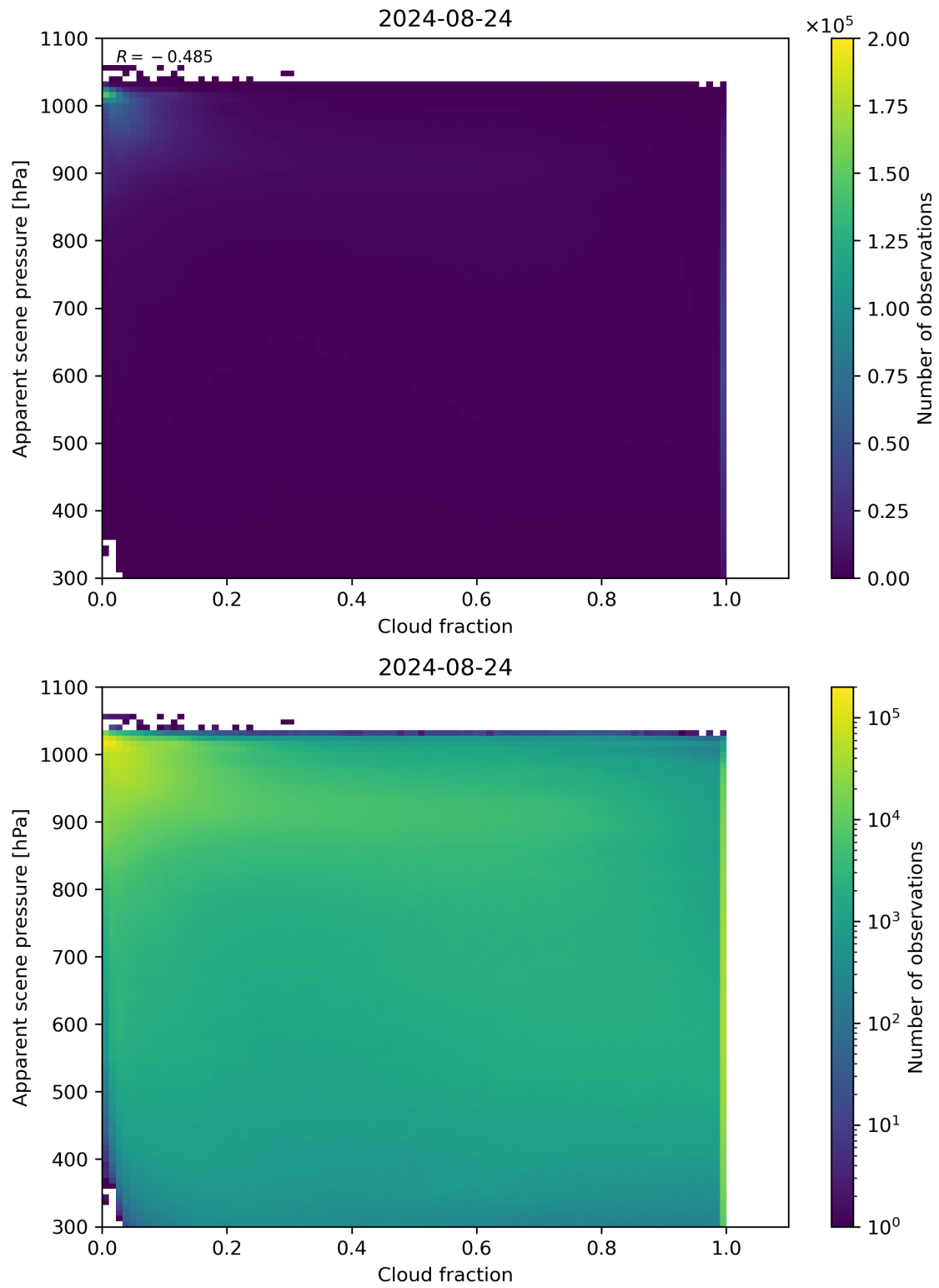
Figure 70: Scatter density plot of “Cloud fraction” against “Apparent scene pressure” for 2024-08-23 to 2024-08-25.
