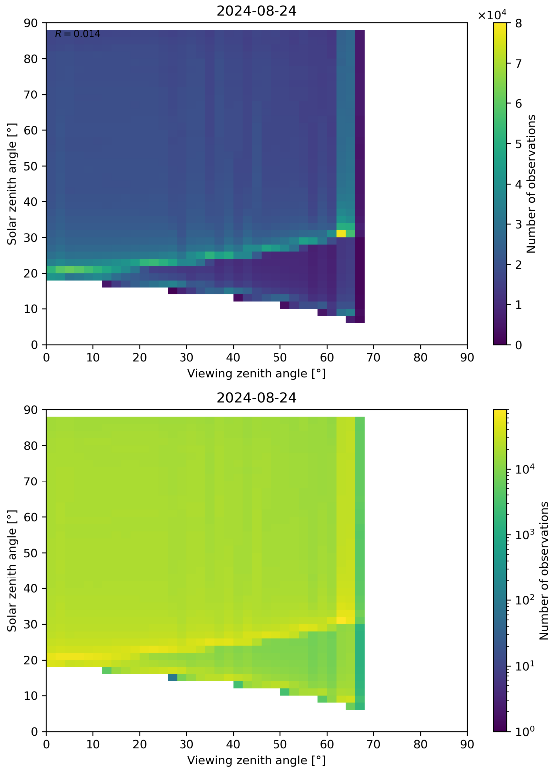
Figure 127: Scatter density plot of “Viewing zenith angle” against “Solar zenith angle” for 2024-08-23 to 2024-08-25.
