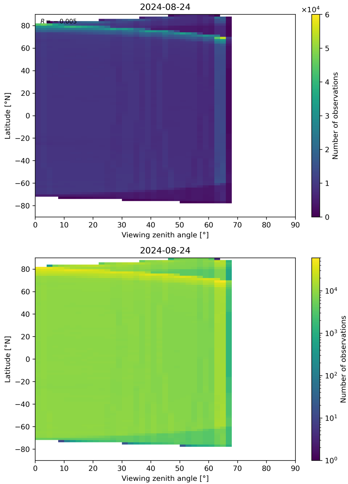
Figure 123: Scatter density plot of “Viewing zenith angle” against “Latitude” for 2024-08-23 to 2024-08-25.
