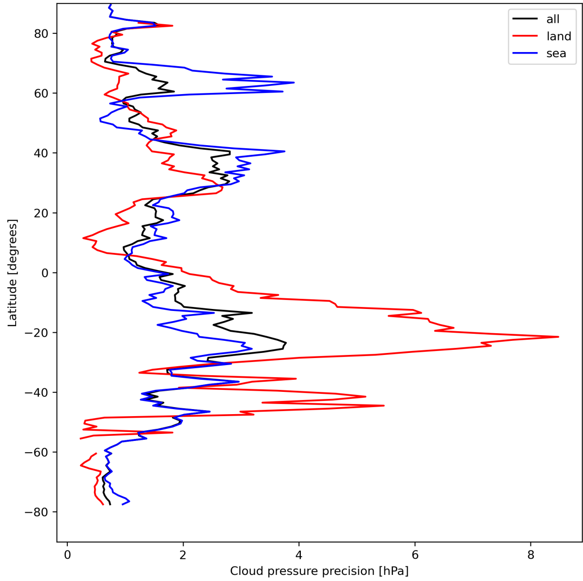
Figure 14: Zonal average of “Cloud pressure precision” for 2024-08-23 to 2024-08-25.
