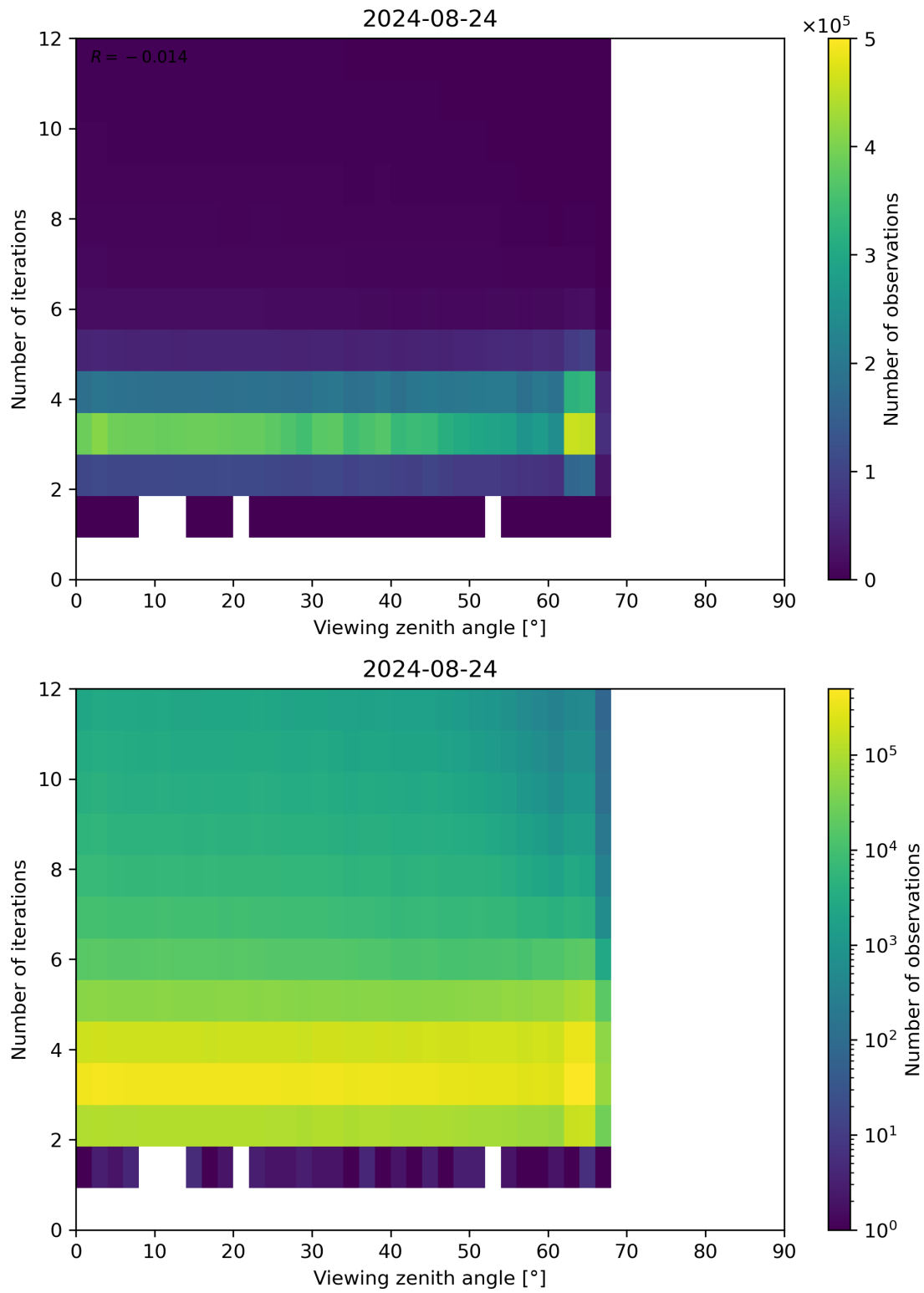
Figure 124: Scatter density plot of “Viewing zenith angle” against “Number of iterations” for 2024-08-23 to 2024-08-25.
