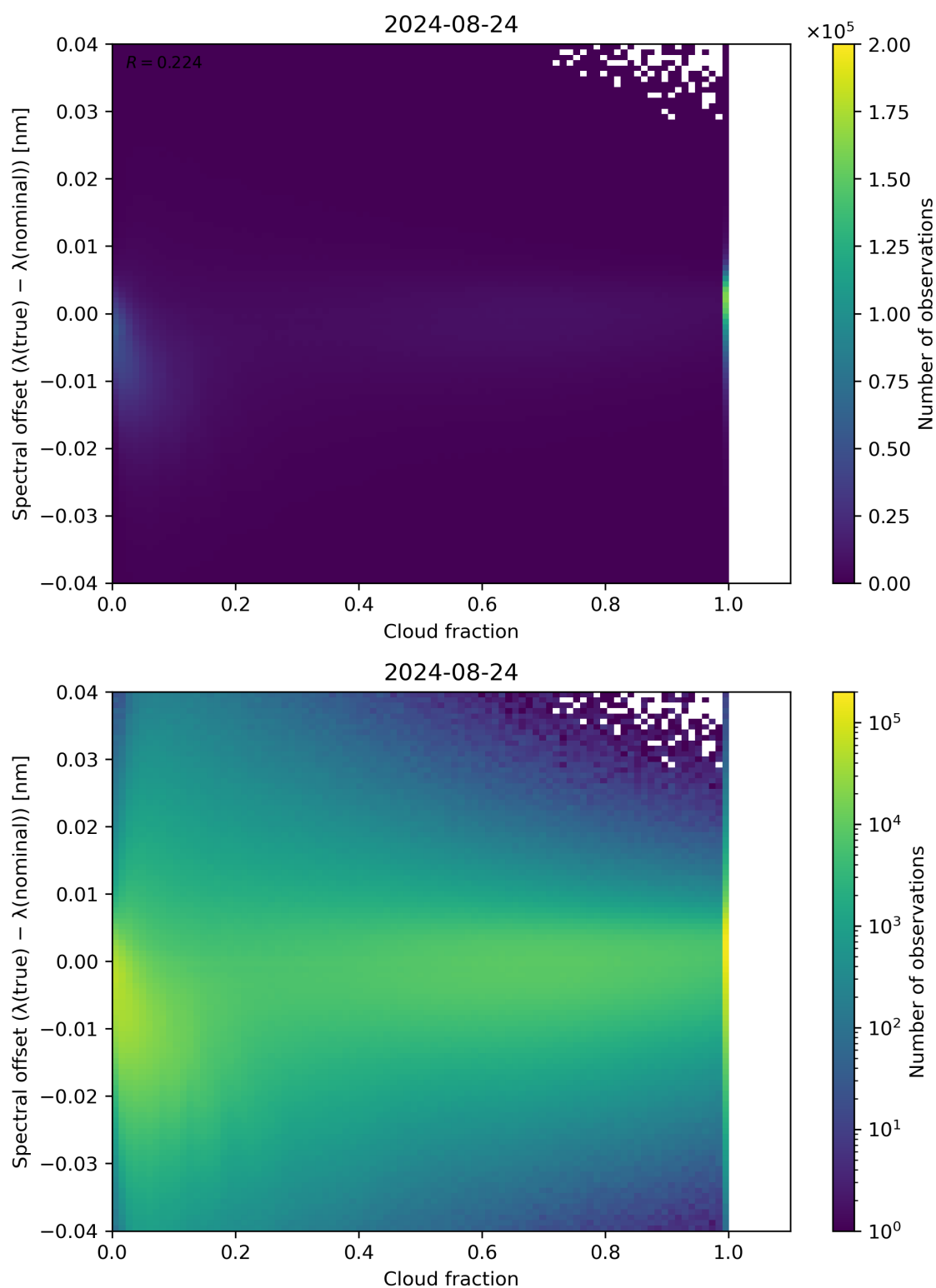
Figure 76: Scatter density plot of “Cloud fraction” against “Spectral offset ( \lambda(\text{true}) - \lambda(\text{nominal}) )” for 2024-08-23 to 2024-08-25.
