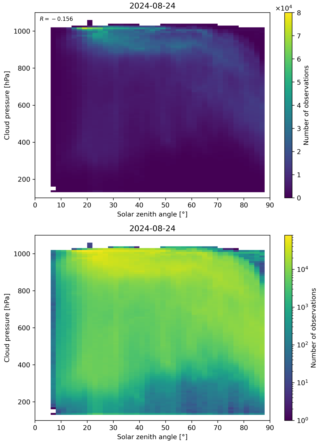
Figure 111: Scatter density plot of “Solar zenith angle” against “Cloud pressure” for 2024-08-23 to 2024-08-25.
