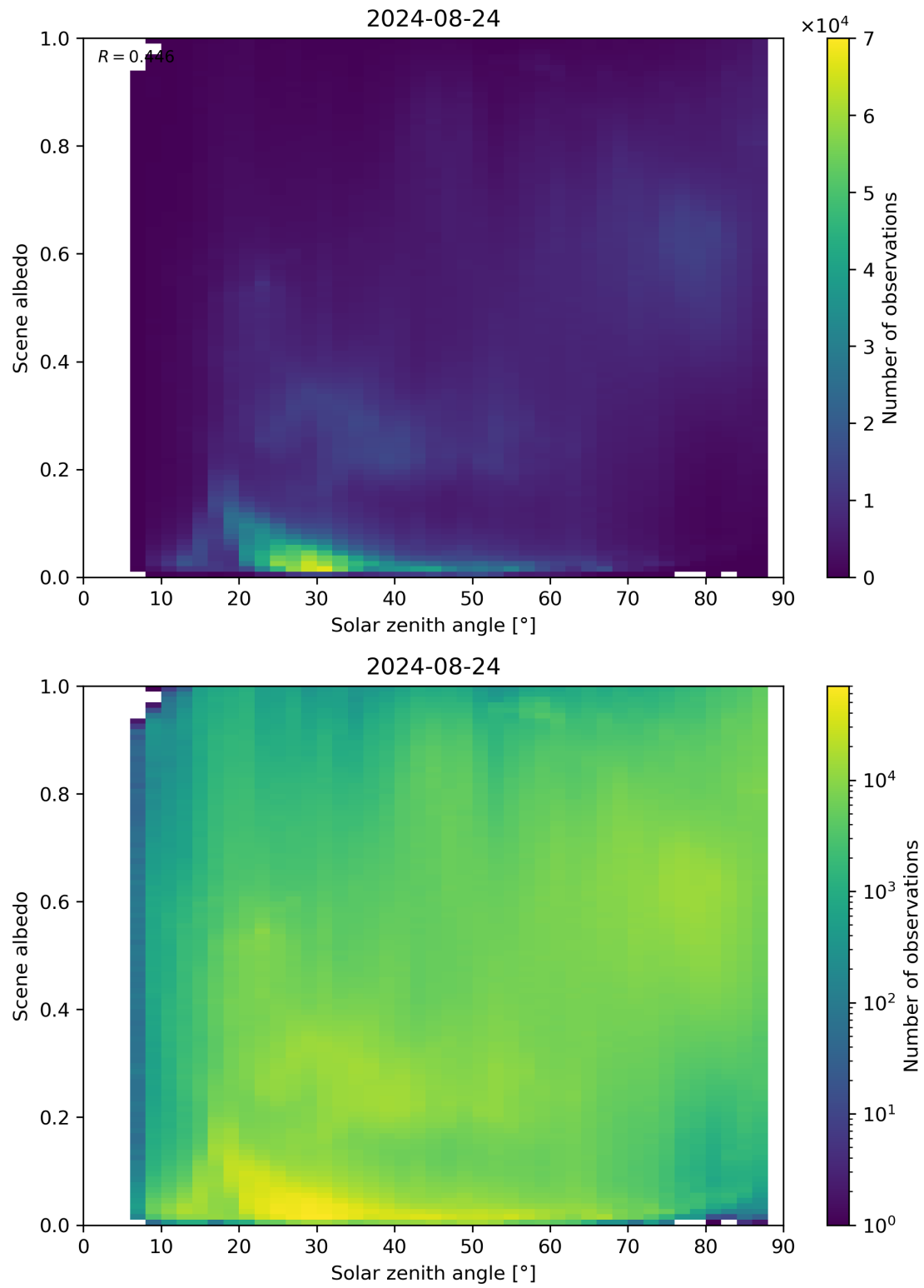
Figure 116: Scatter density plot of “Solar zenith angle” against “Scene albedo” for 2024-08-23 to 2024-08-25.
