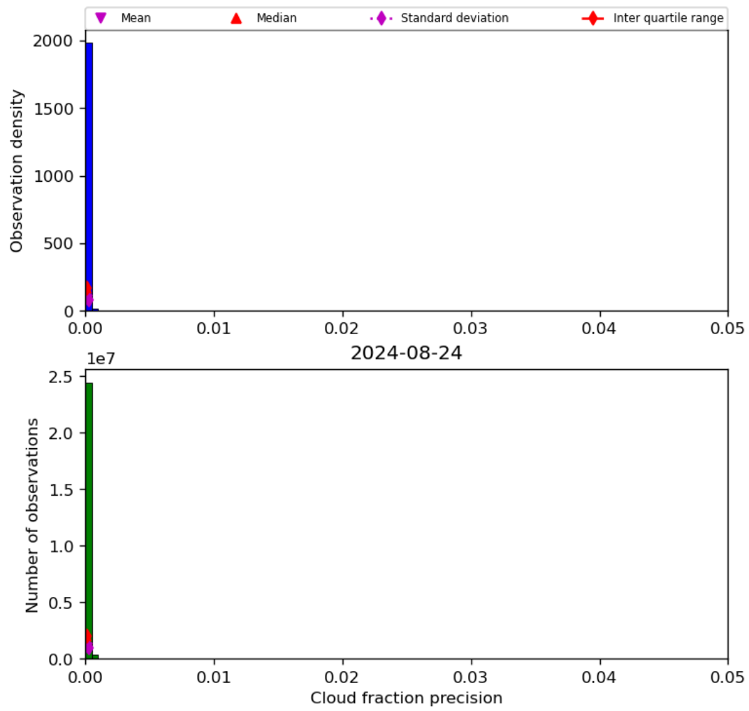
Figure 33: Histogram of “Cloud fraction precision” for 2024-08-23 to 2024-08-25
