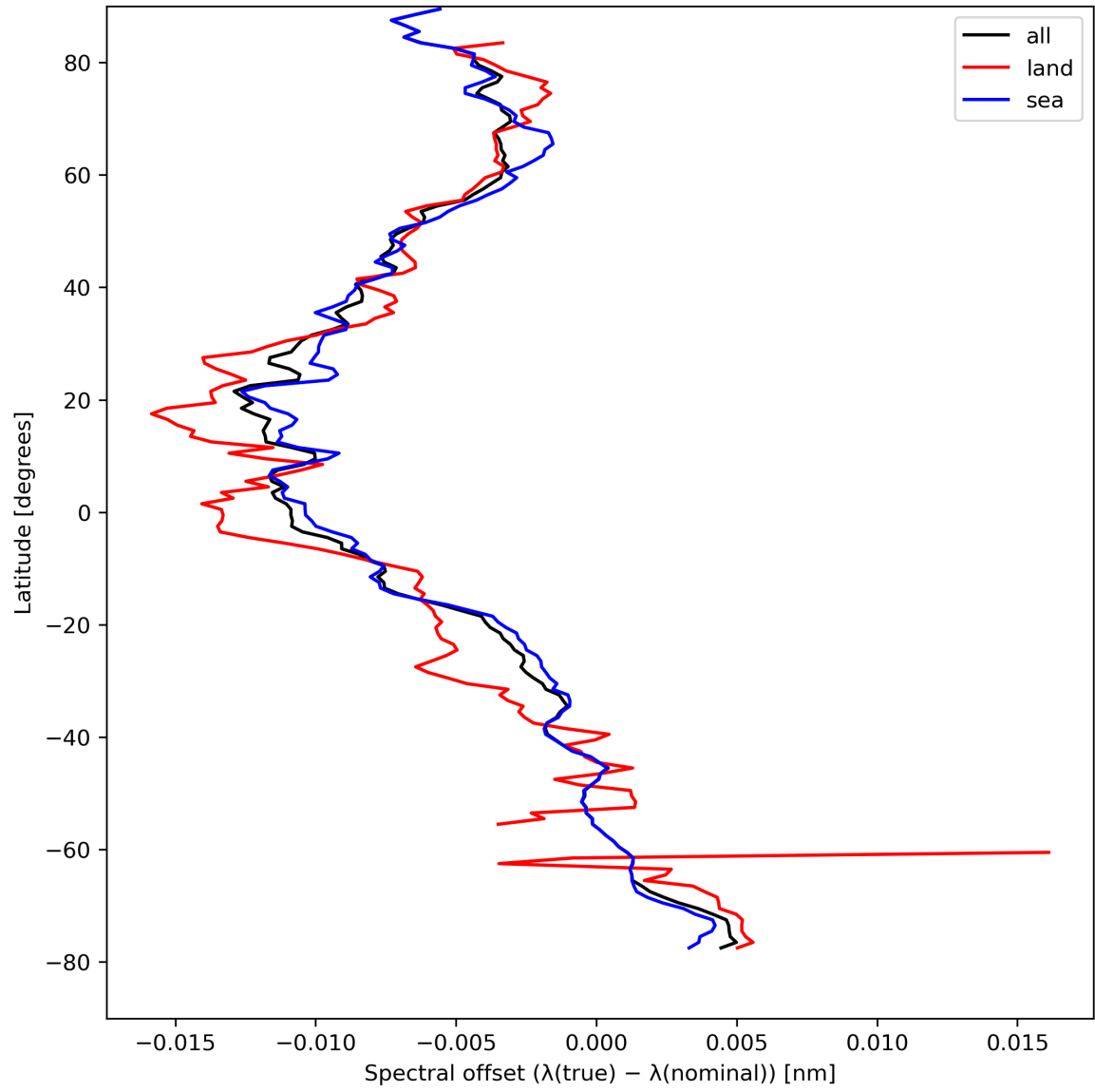
Figure 28: Zonal average of “Spectral offset ( \lambda(\text{true}) - \lambda(\text{nominal}) )” for 2024-08-23 to 2024-08-25.
