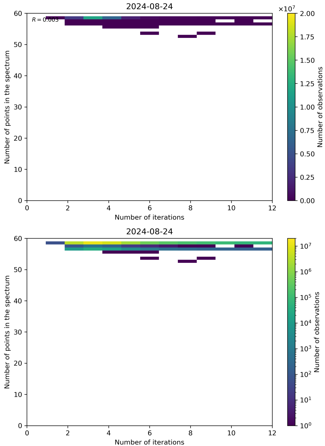
Figure 99: Scatter density plot of “Number of iterations” against “Number of points in the spectrum” for 2024-08-23 to 2024-08-25.
