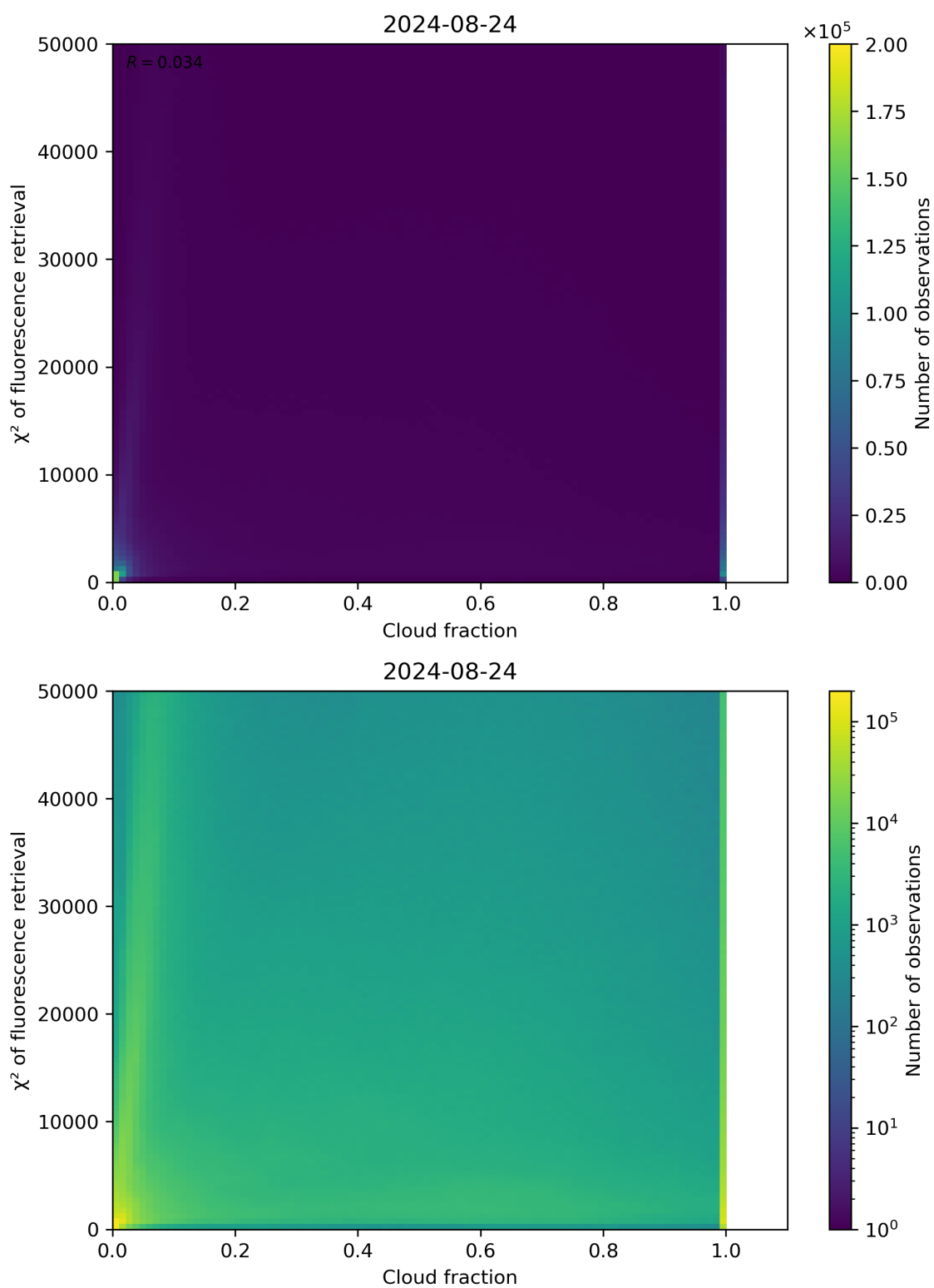
Figure 71: Scatter density plot of “Cloud fraction” against “ \chi^2 of fluorescence retrieval” for 2024-08-23 to 2024-08-25.
