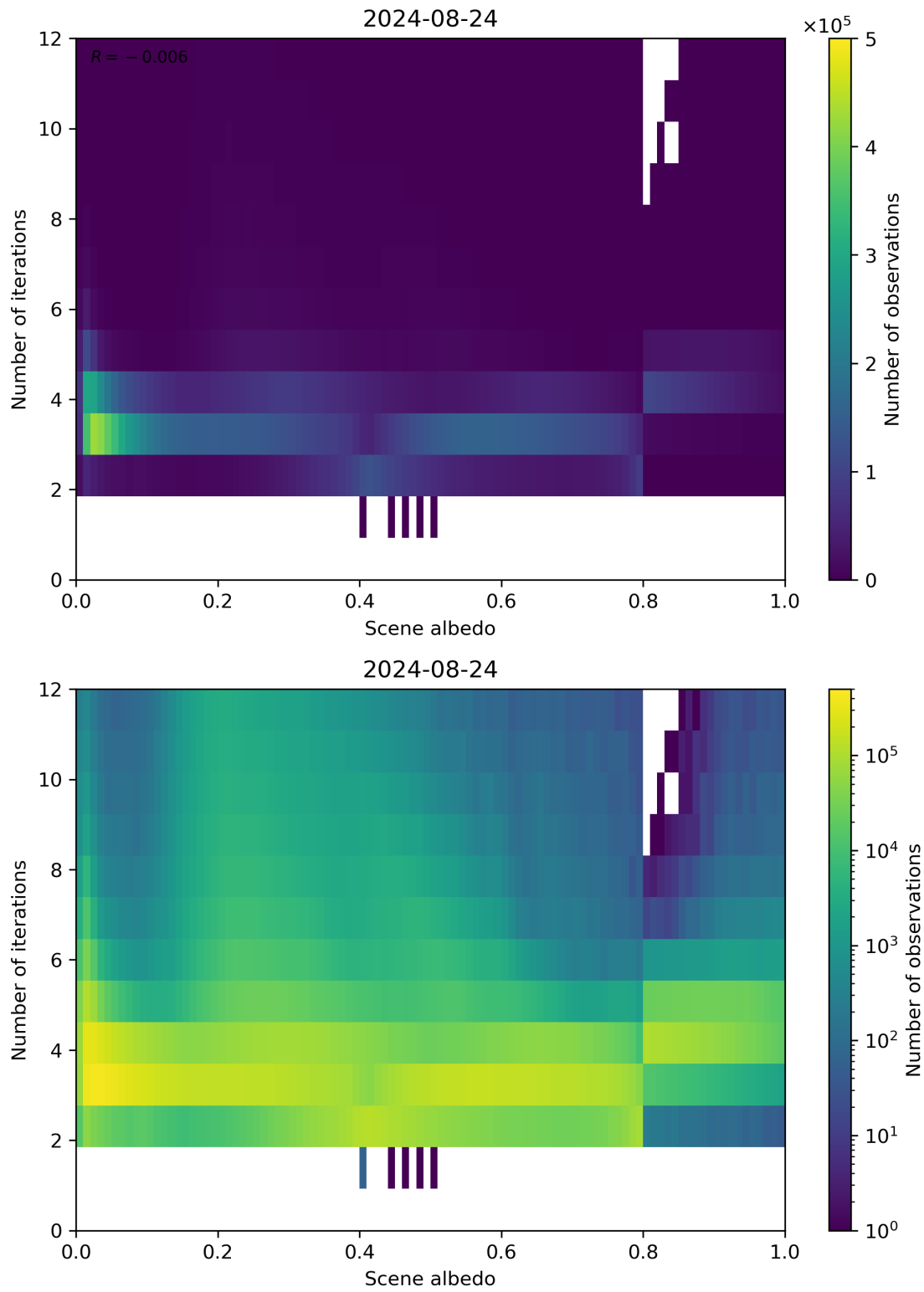
Figure 105: Scatter density plot of “Scene albedo” against “Number of iterations” for 2024-08-23 to 2024-08-25.
