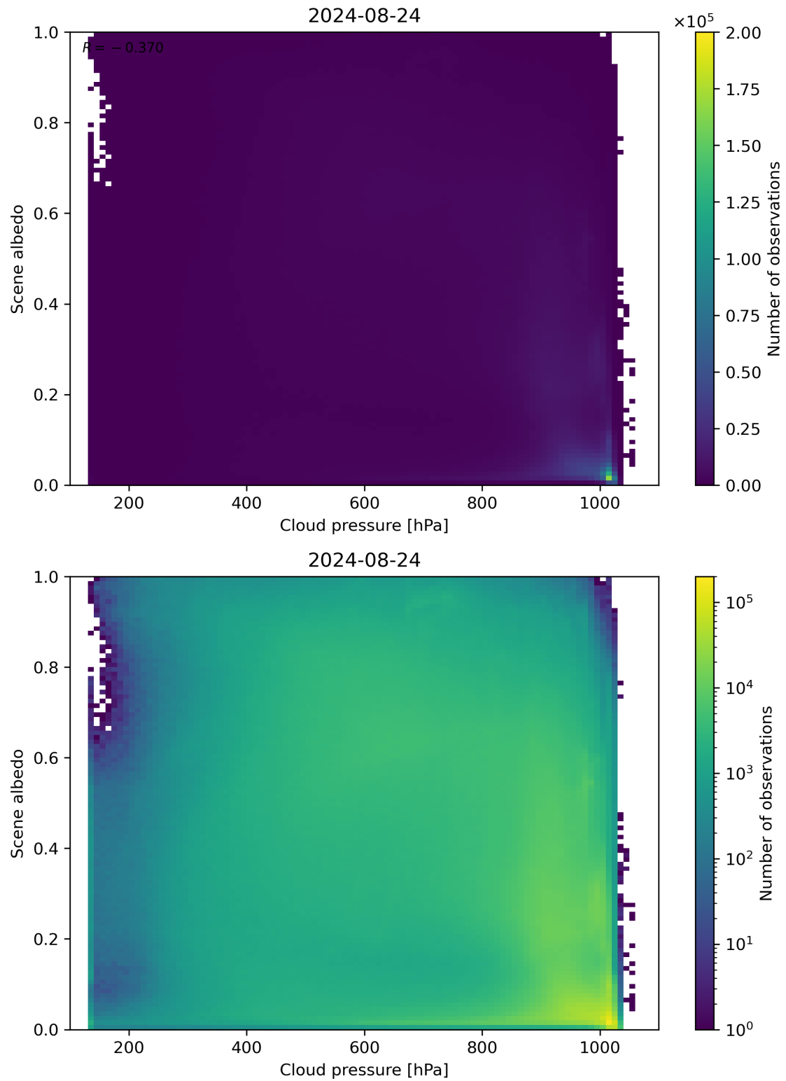
Figure 83: Scatter density plot of “Cloud pressure” against “Scene albedo” for 2024-08-23 to 2024-08-25.
