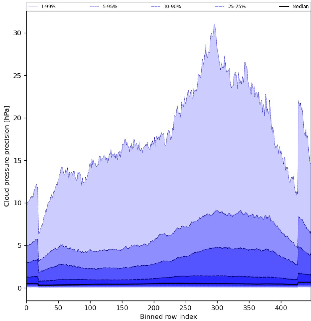
Figure 48: Along track statistics of “Cloud pressure precision” for 2024-08-23 to 2024-08-25
