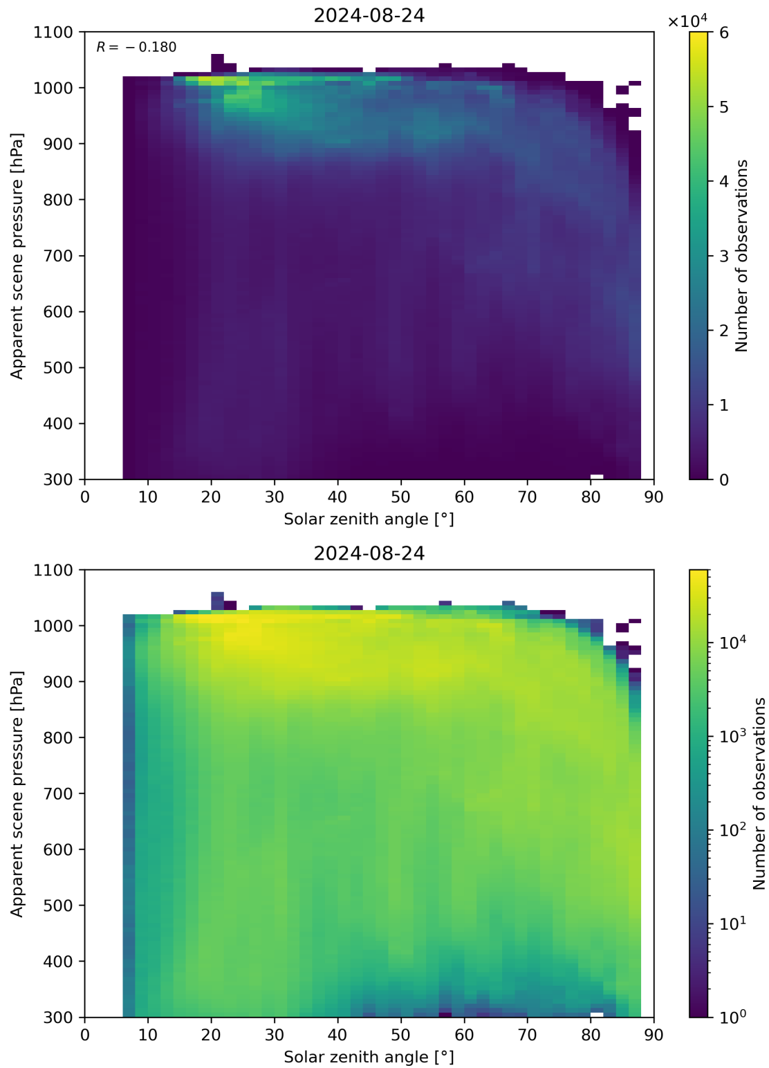
Figure 108: Scatter density plot of “Solar zenith angle” against “Apparent scene pressure” for 2024-08-23 to 2024-08-25.
