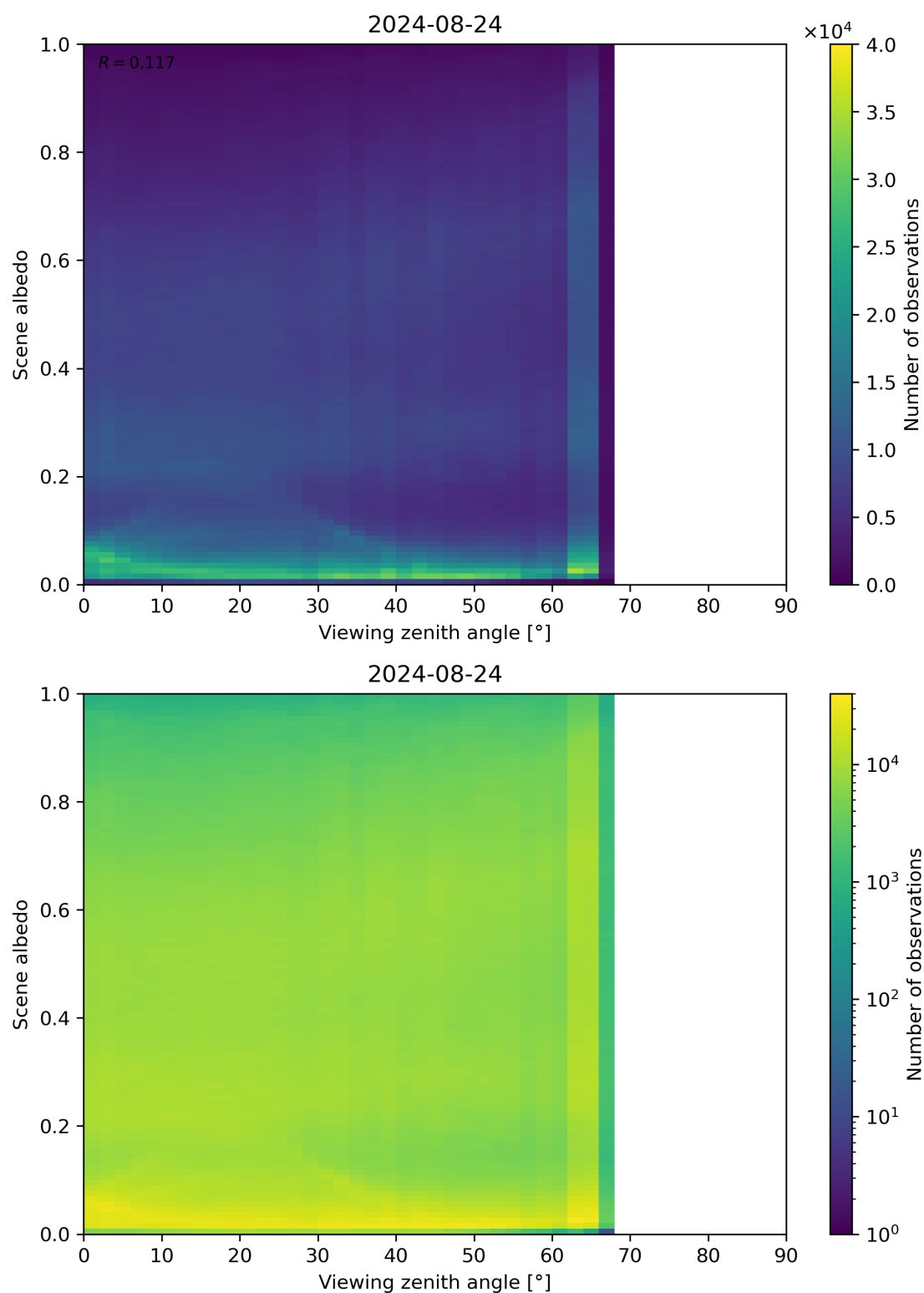
Figure 126: Scatter density plot of “Viewing zenith angle” against “Scene albedo” for 2024-08-23 to 2024-08-25.
