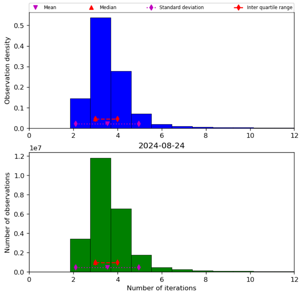
Figure 39: Histogram of “Number of iterations” for 2024-08-23 to 2024-08-25
