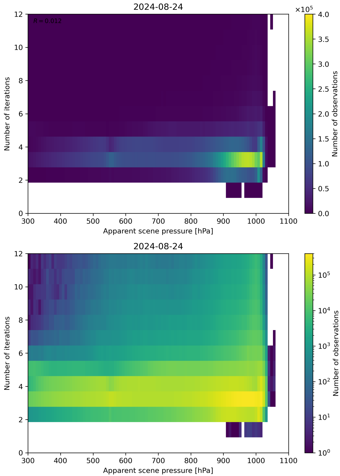
Figure 65: Scatter density plot of “Apparent scene pressure” against “Number of iterations” for 2024-08-23 to 2024-08-25.
