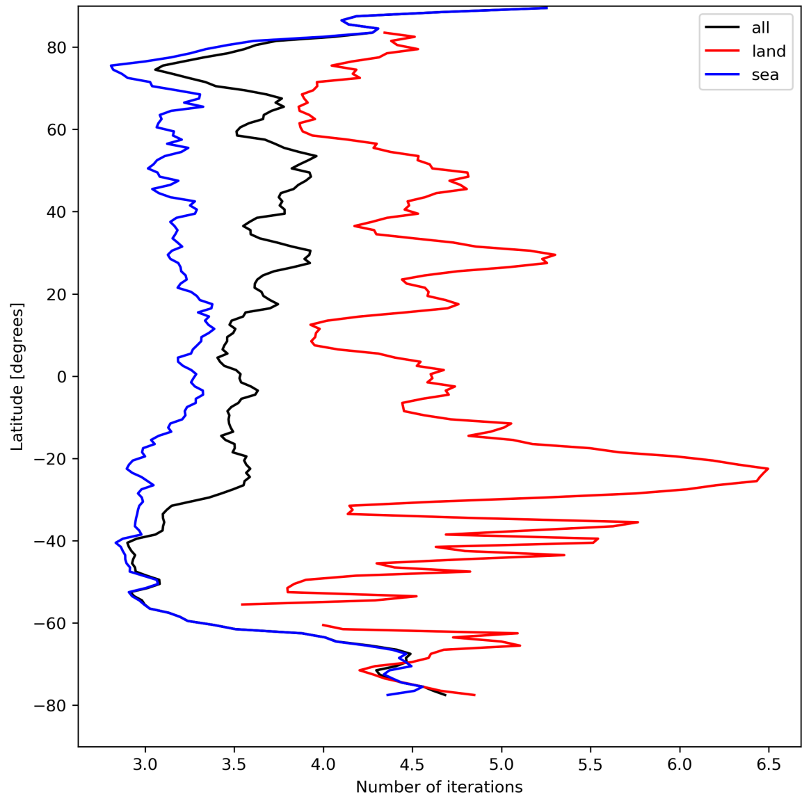
Figure 22: Zonal average of “Number of iterations” for 2024-08-23 to 2024-08-25.
