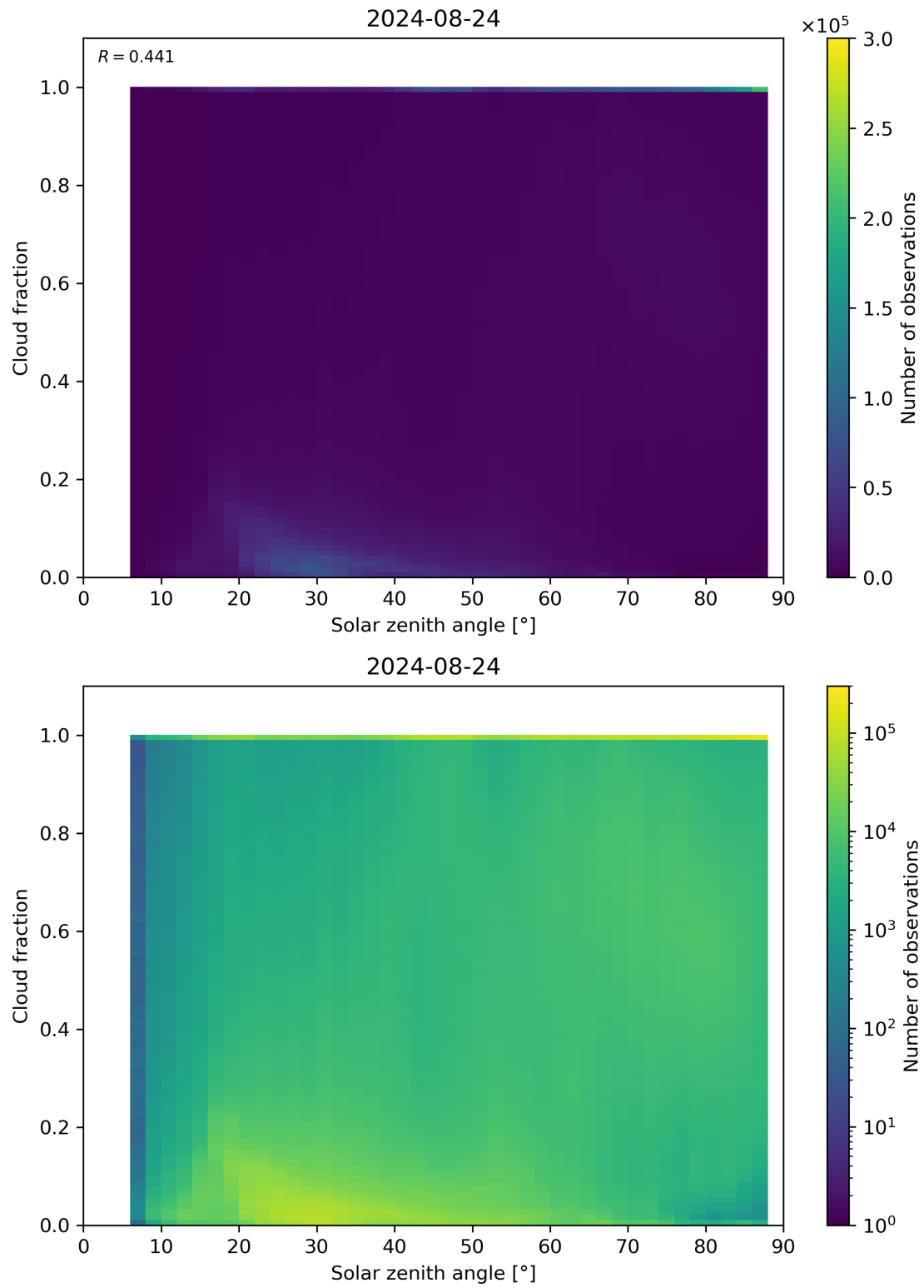
Figure 110: Scatter density plot of “Solar zenith angle” against “Cloud fraction” for 2024-08-23 to 2024-08-25.
