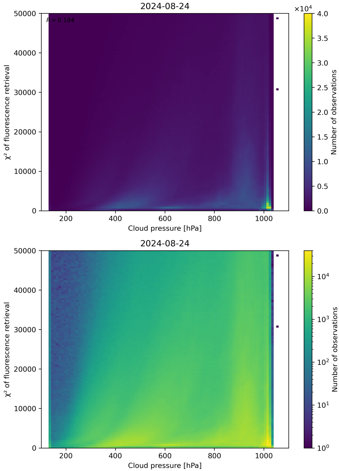
Figure 78: Scatter density plot of “Cloud pressure” against “ \chi^2 of fluorescence retrieval” for 2024-08-23 to 2024-08-25.
