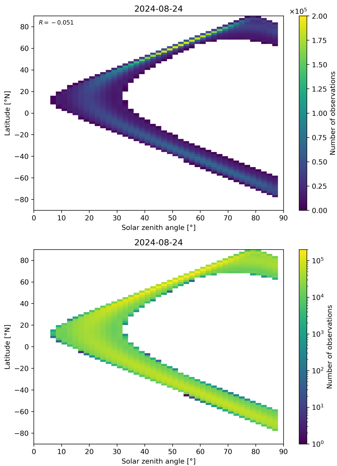
Figure 113: Scatter density plot of “Solar zenith angle” against “Latitude” for 2024-08-23 to 2024-08-25.
