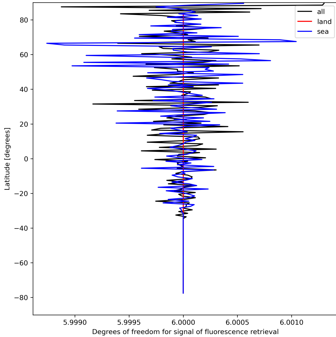
Figure 26: Zonal average of “Degrees of freedom for signal of fluorescence retrieval” for 2024-08-23 to 2024-08-25.
