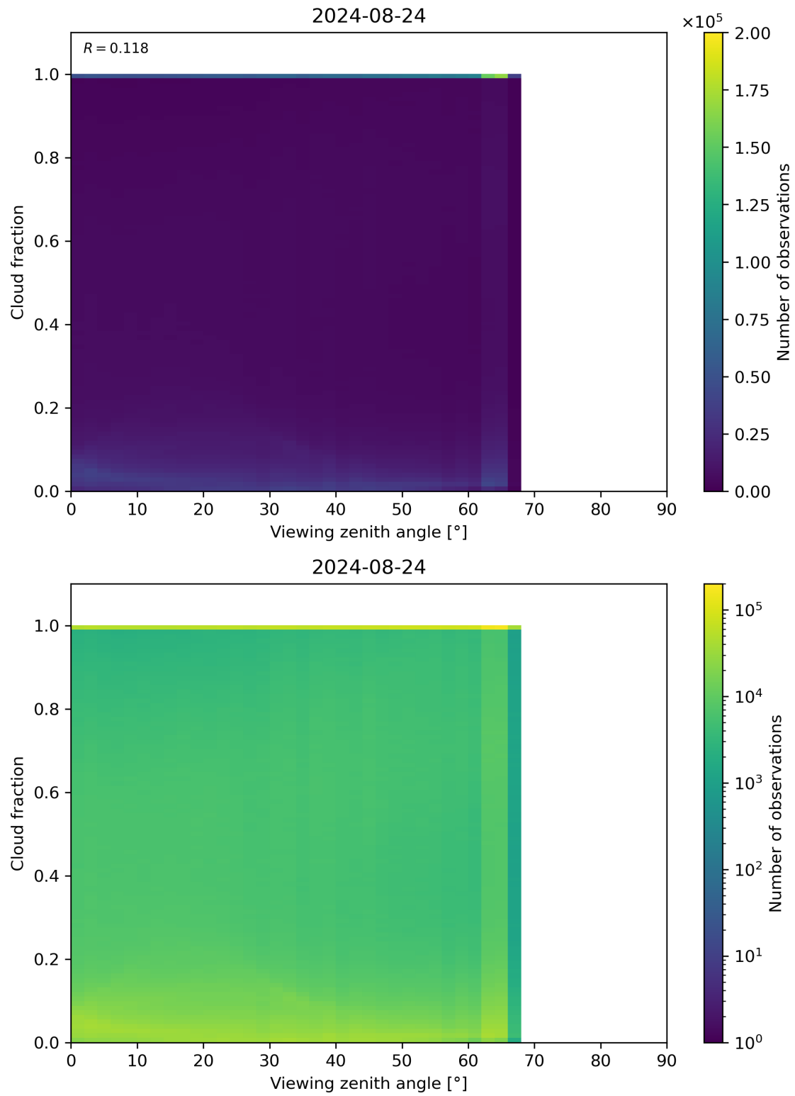
Figure 120: Scatter density plot of “Viewing zenith angle” against “Cloud fraction” for 2024-08-23 to 2024-08-25.
