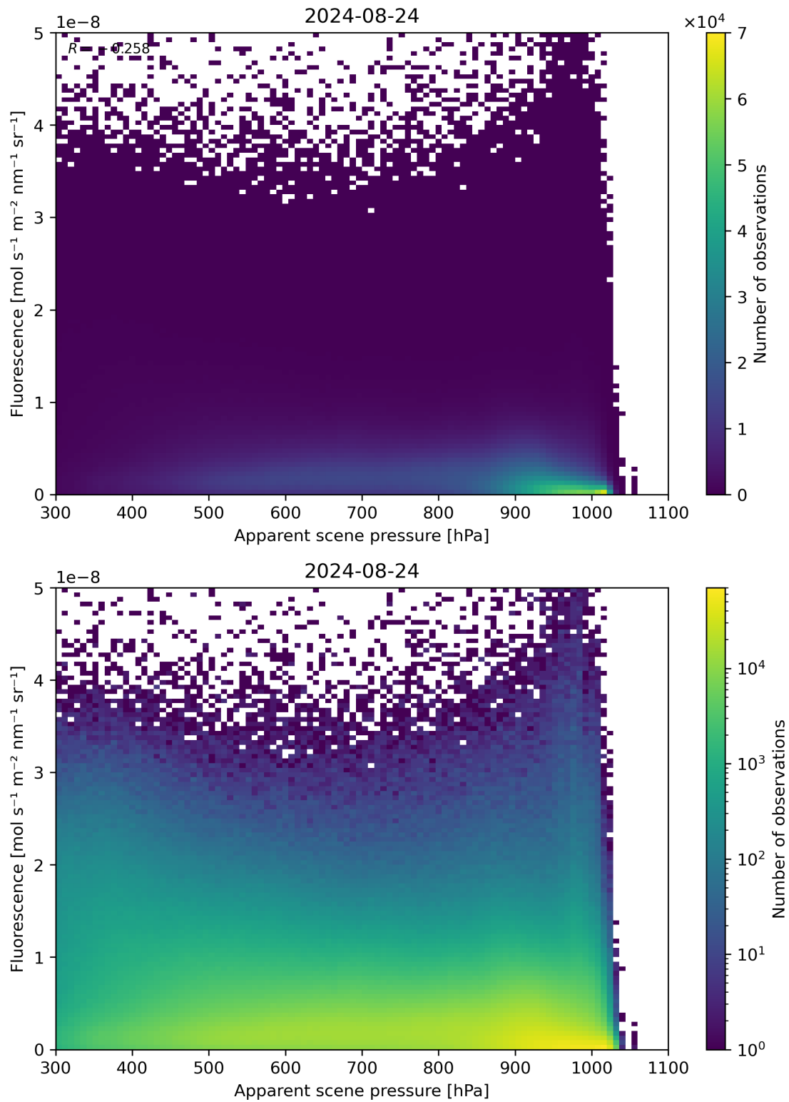
Figure 64: Scatter density plot of “Apparent scene pressure” against “Fluorescence” for 2024-08-23 to 2024-08-25.
