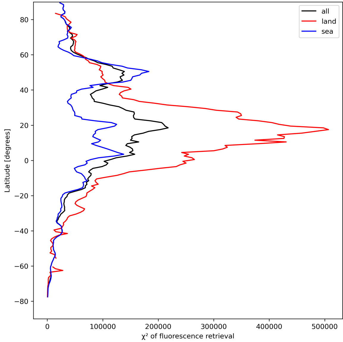
Figure 25: Zonal average of “ \chi^2 of fluorescence retrieval” for 2024-08-23 to 2024-08-25.
