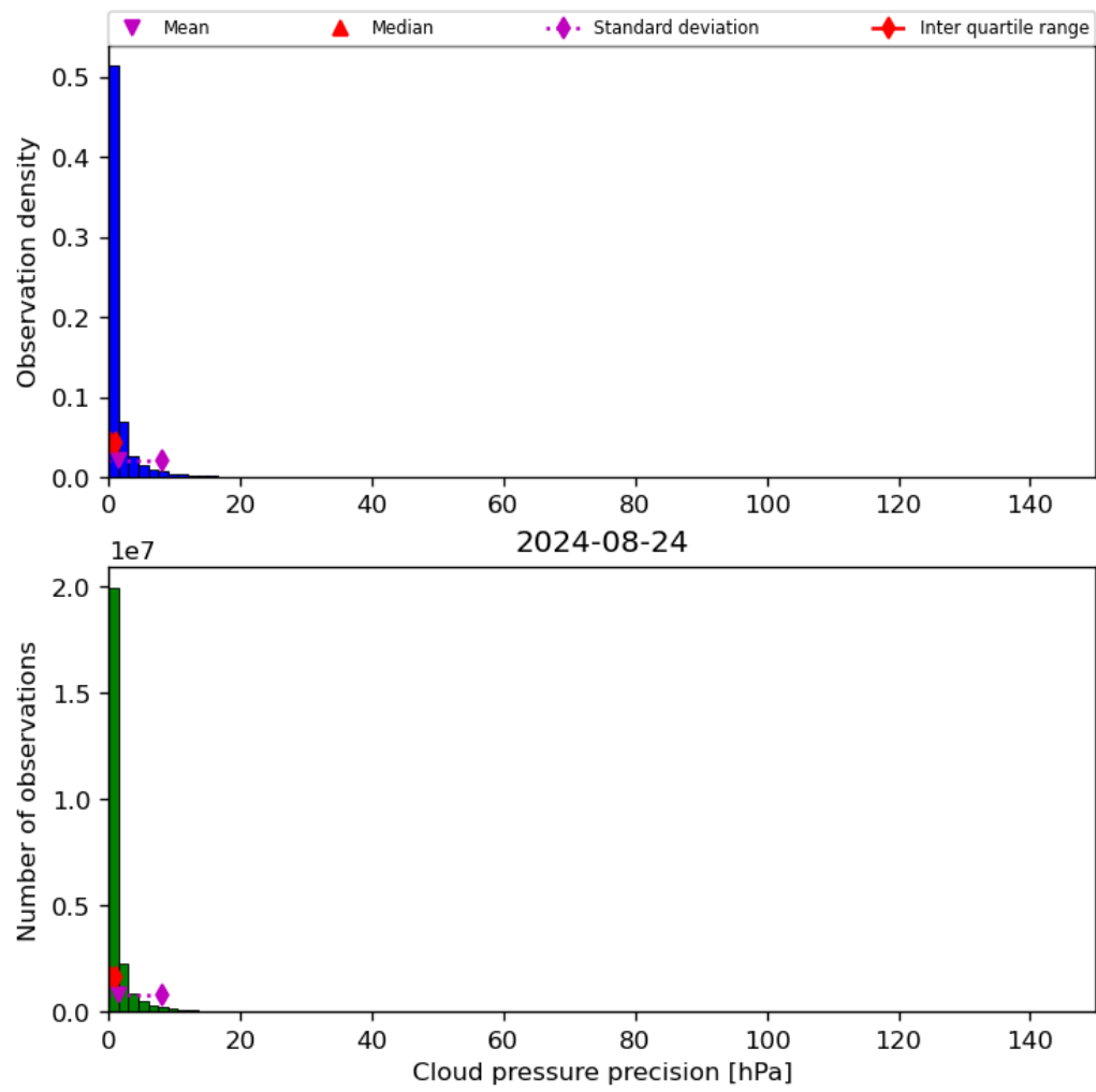
Figure 31: Histogram of “Cloud pressure precision” for 2024-08-23 to 2024-08-25
