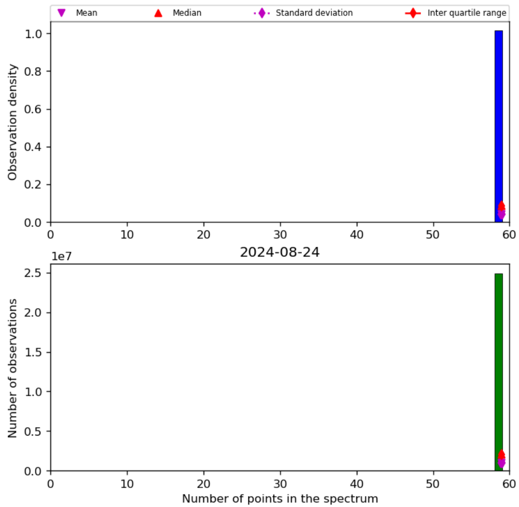
Figure 44: Histogram of “Number of points in the spectrum” for 2024-08-23 to 2024-08-25
