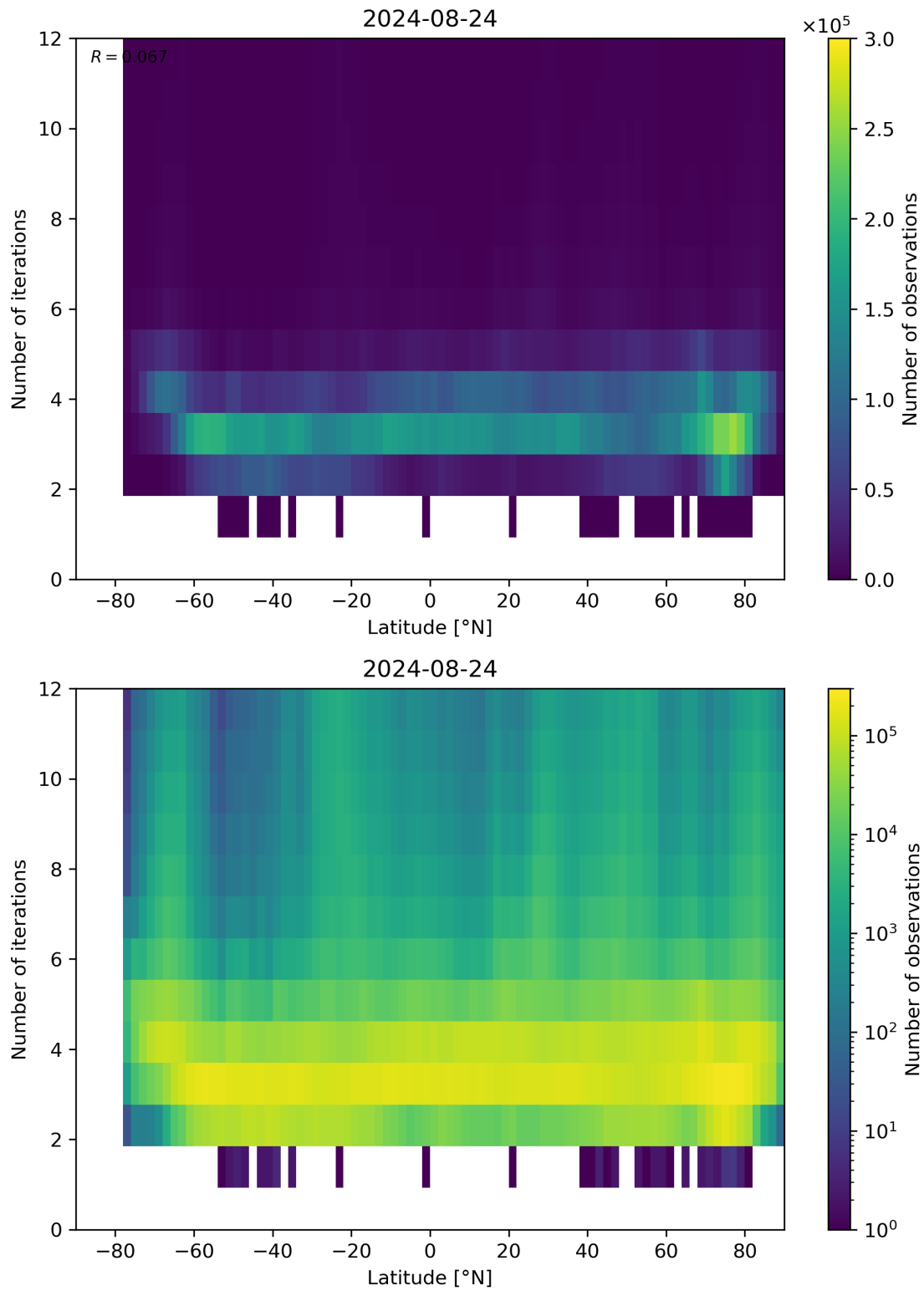
Figure 93: Scatter density plot of “Latitude” against “Number of iterations” for 2024-08-23 to 2024-08-25.
