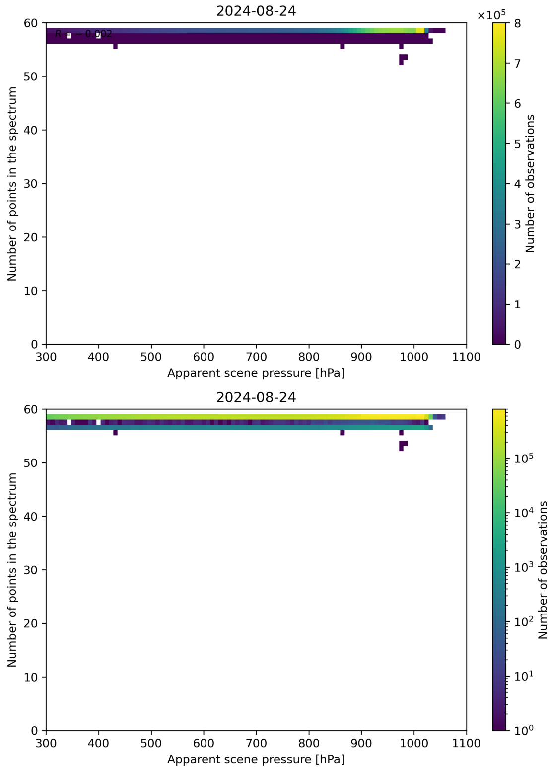
Figure 66: Scatter density plot of “Apparent scene pressure” against “Number of points in the spectrum” for 2024-08-23 to 2024-08-25.
