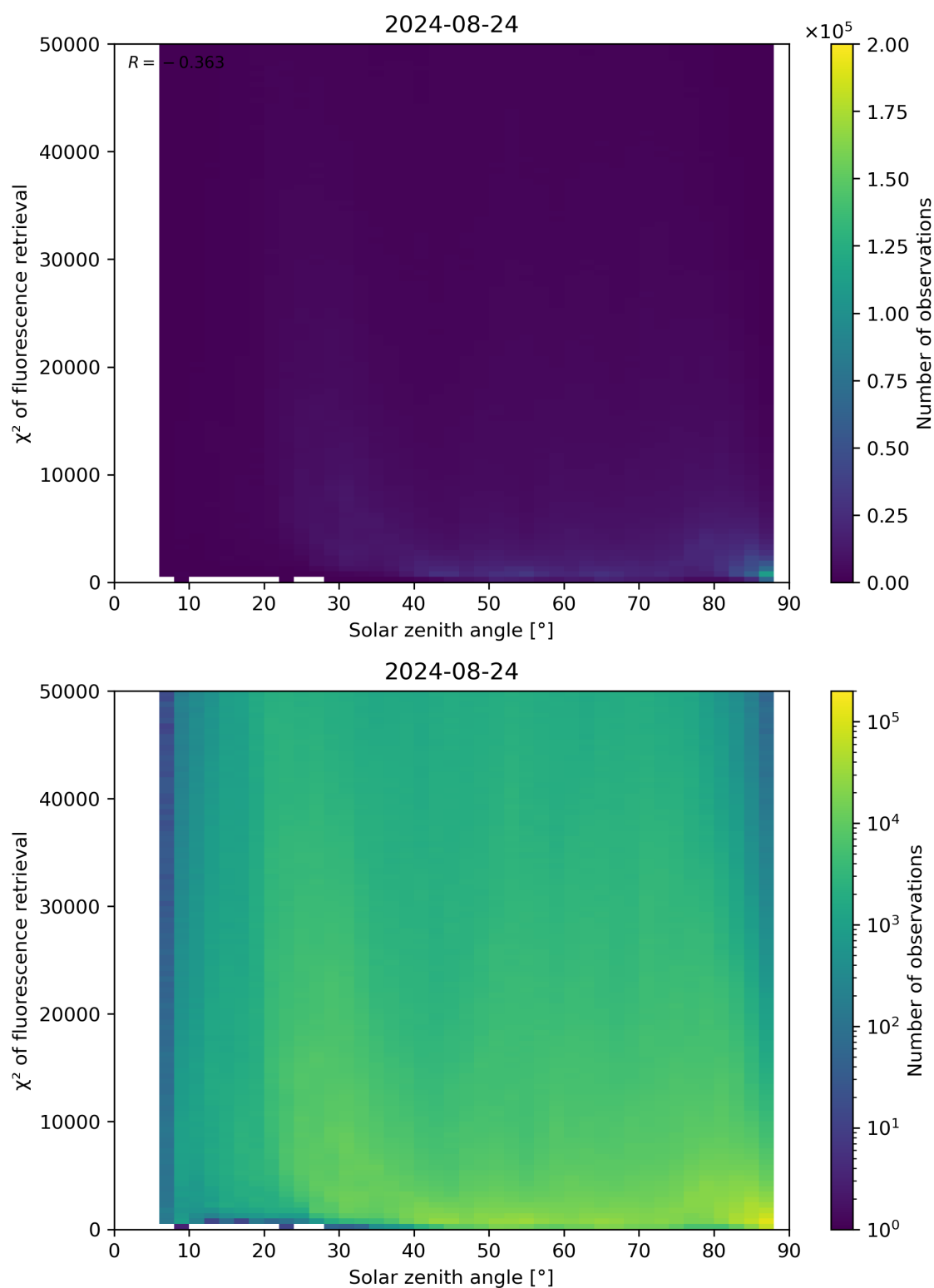
Figure 109: Scatter density plot of “Solar zenith angle” against “ \chi^2 of fluorescence retrieval” for 2024-08-23 to 2024-08-25.
