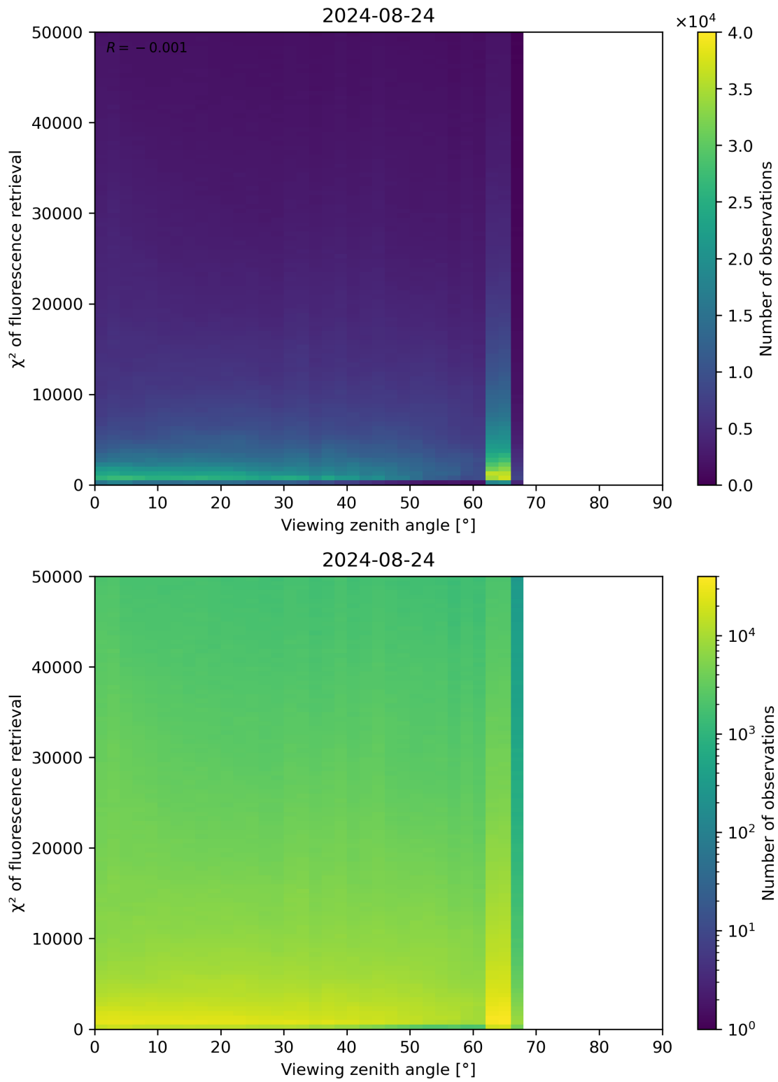
Figure 119: Scatter density plot of “Viewing zenith angle” against “ \chi^2 of fluorescence retrieval” for 2024-08-23 to 2024-08-25.
