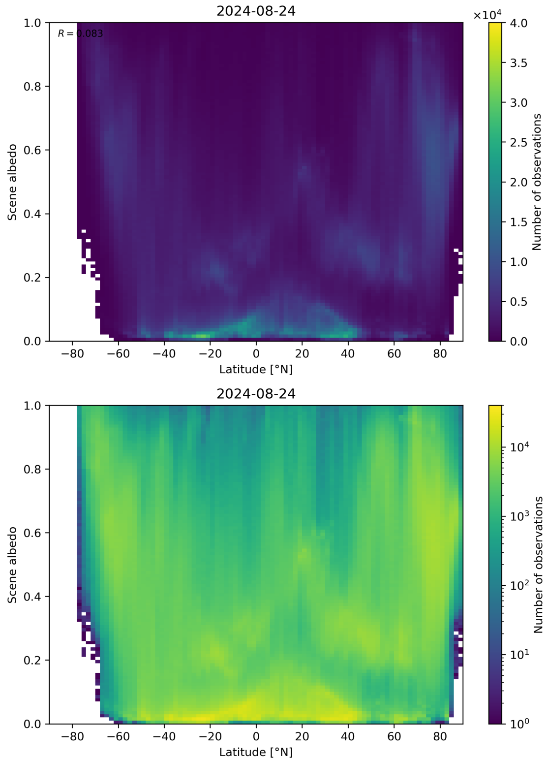
Figure 95: Scatter density plot of “Latitude” against “Scene albedo” for 2024-08-23 to 2024-08-25.
