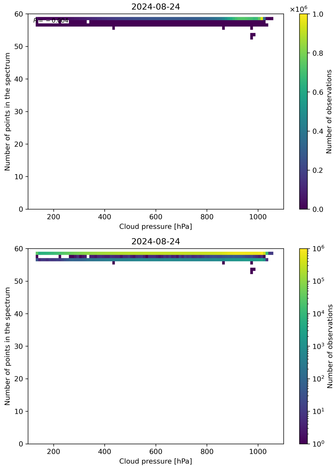
Figure 82: Scatter density plot of “Cloud pressure” against “Number of points in the spectrum” for 2024-08-23 to 2024-08-25.
