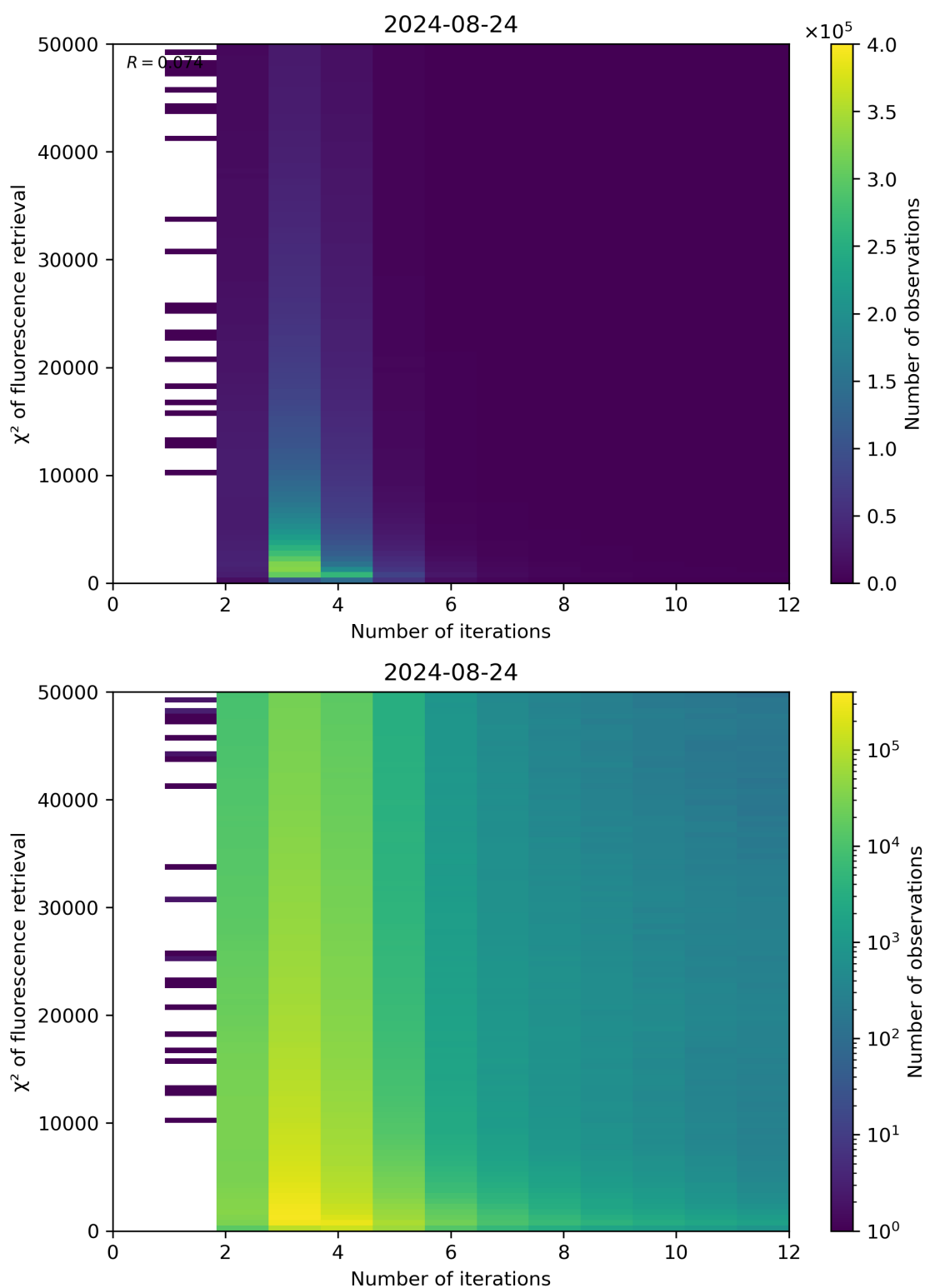
Figure 97: Scatter density plot of “Number of iterations” against “ \chi^2 of fluorescence retrieval” for 2024-08-23 to 2024-08-25.
