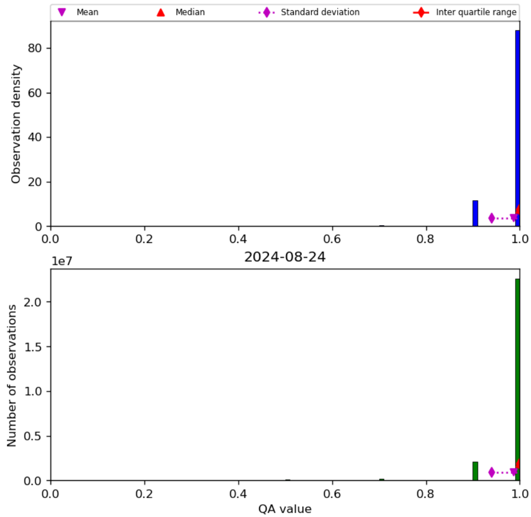
Figure 29: Histogram of “QA value” for 2024-08-23 to 2024-08-25
