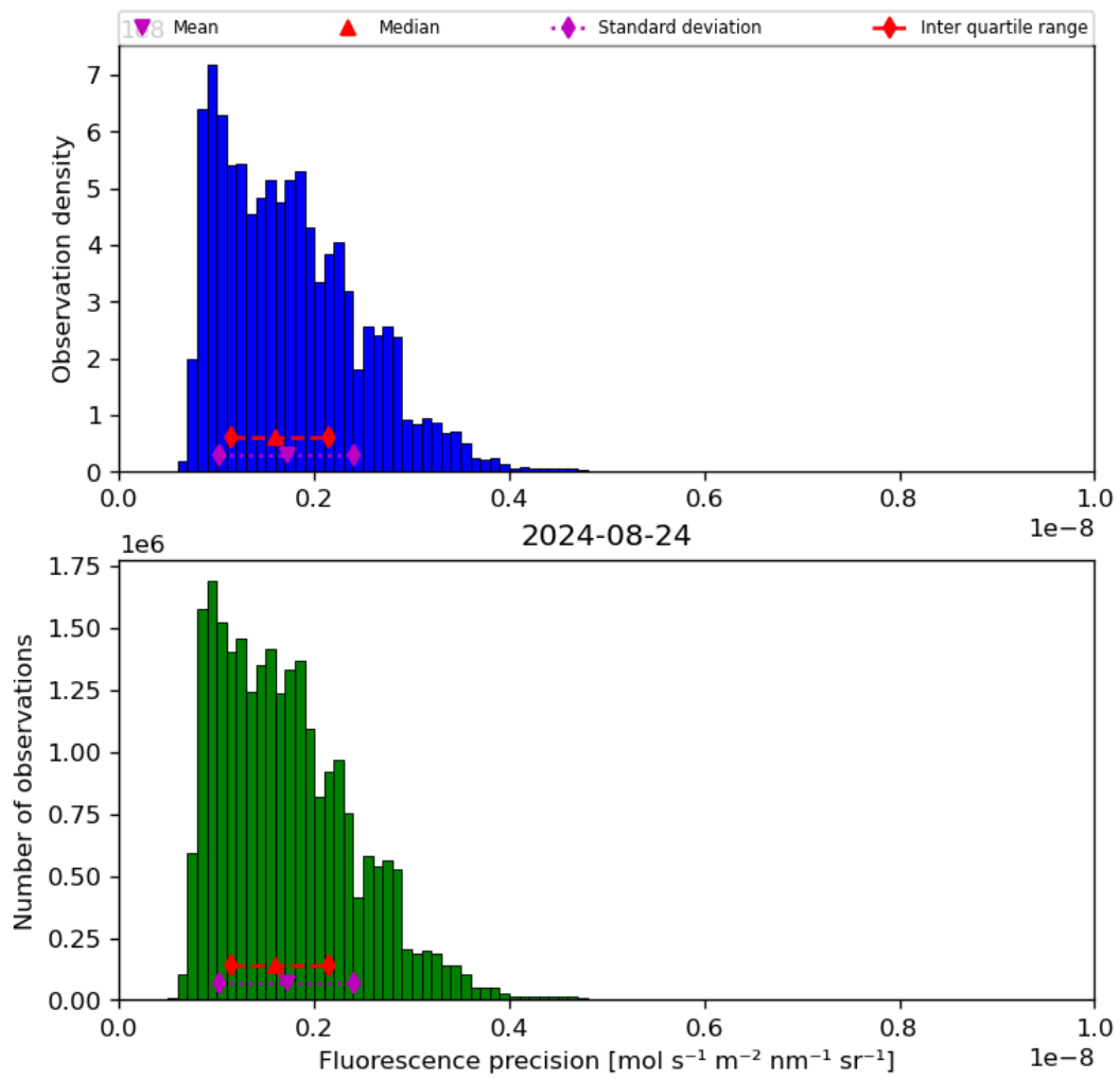
Figure 41: Histogram of “Fluorescence precision” for 2024-08-23 to 2024-08-25
