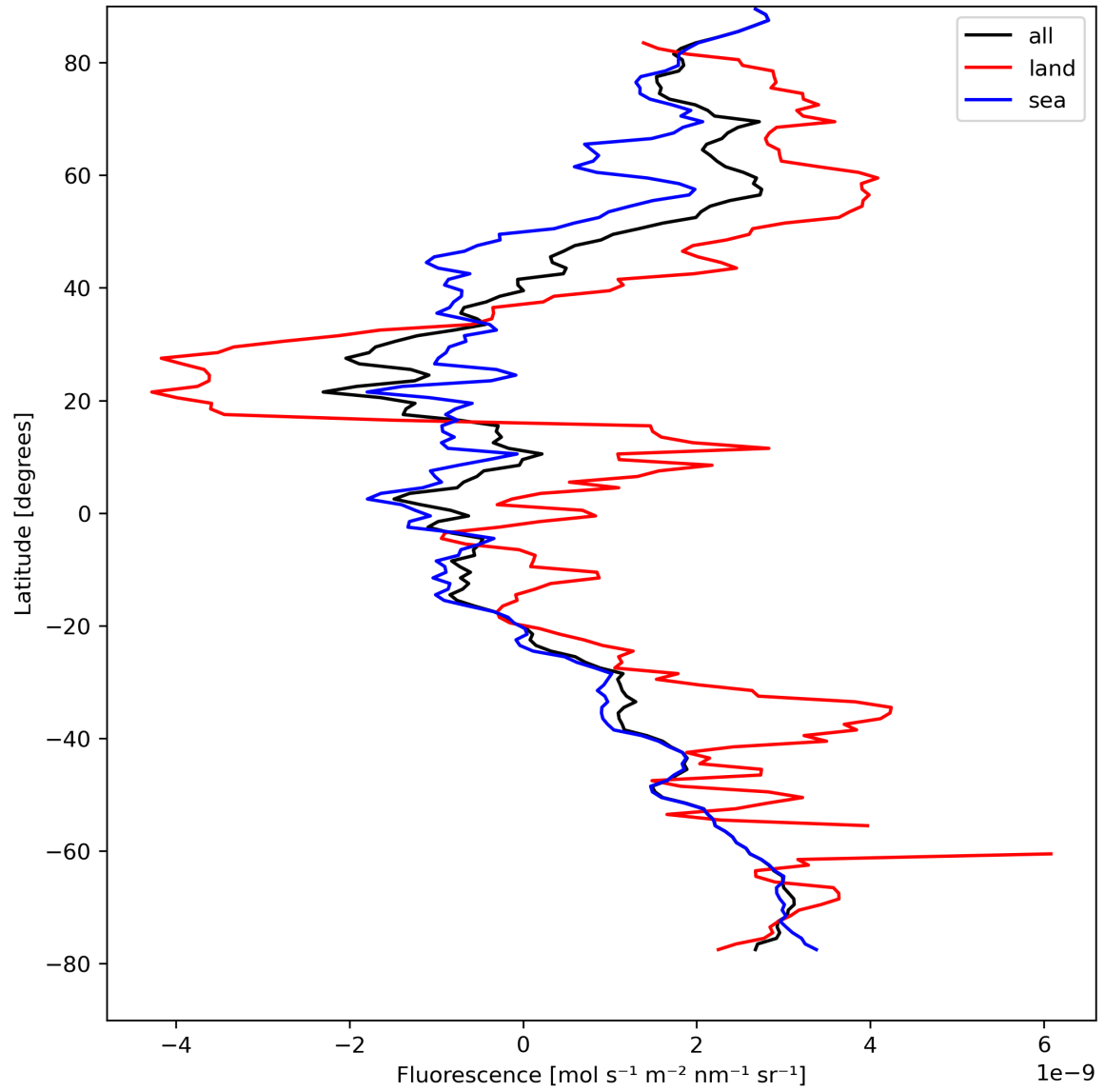
Figure 23: Zonal average of “Fluorescence” for 2024-08-23 to 2024-08-25.
