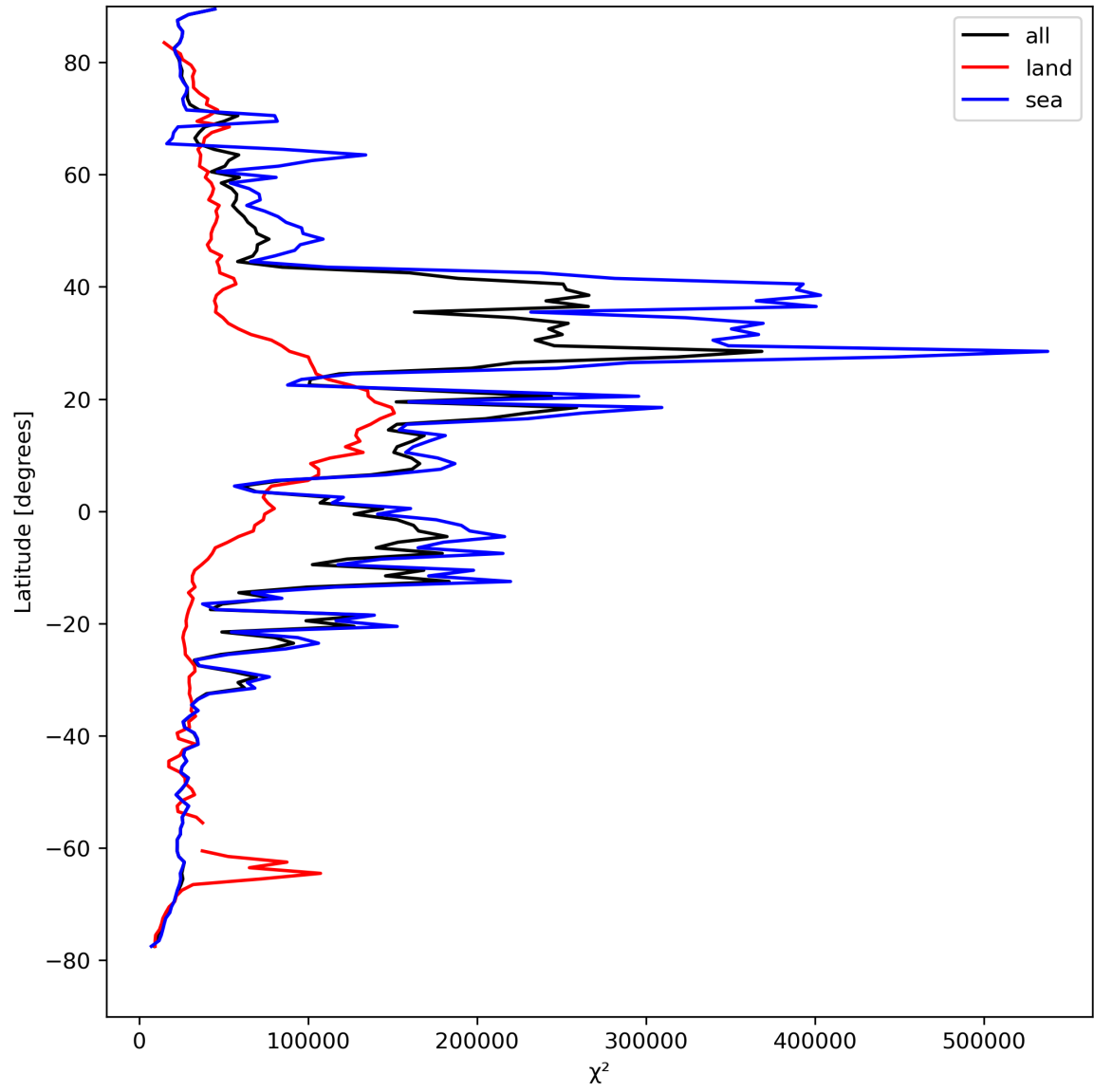
Figure 21: Zonal average of “ \chi^2 ” for 2024-08-23 to 2024-08-25.
