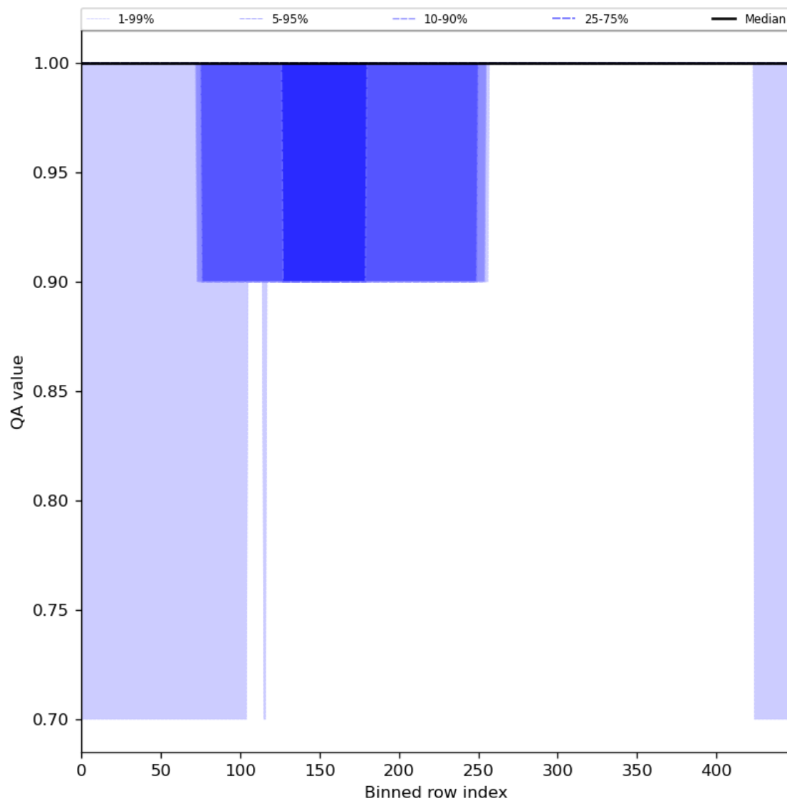
Figure 46: Along track statistics of “QA value” for 2024-08-23 to 2024-08-25
