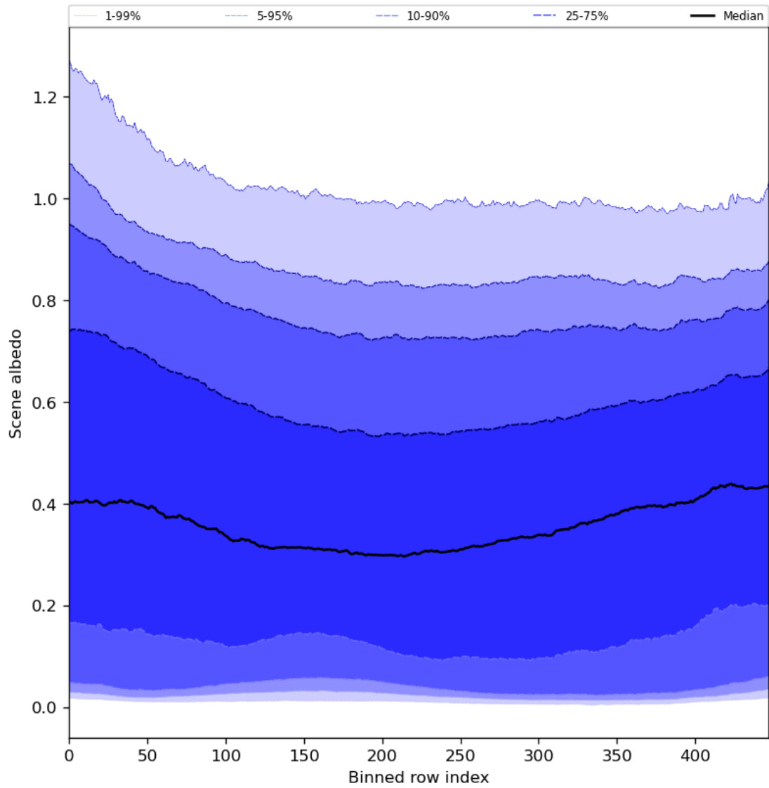
Figure 51: Along track statistics of “Scene albedo” for 2024-08-23 to 2024-08-25
