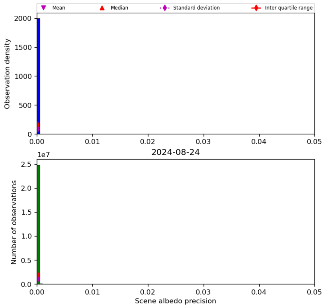
Figure 35: Histogram of “Scene albedo precision” for 2024-08-23 to 2024-08-25
