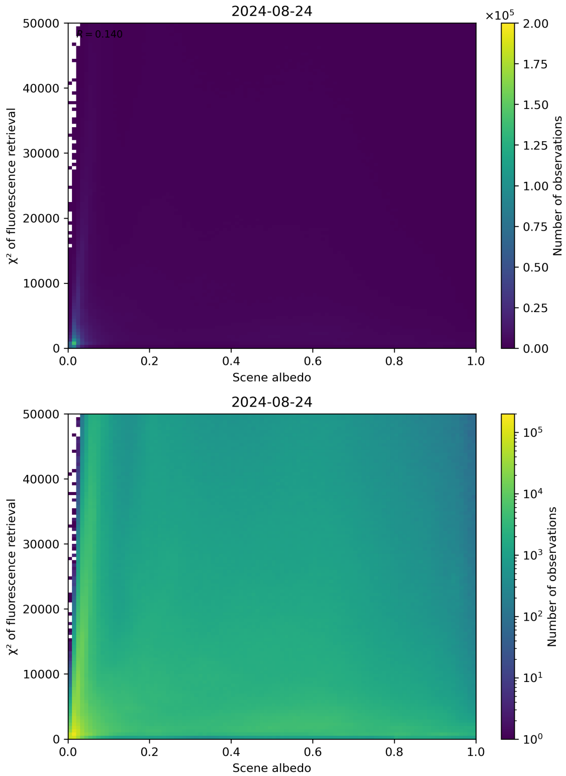
Figure 103: Scatter density plot of “Scene albedo” against “ \chi^2 of fluorescence retrieval” for 2024-08-23 to 2024-08-25.
