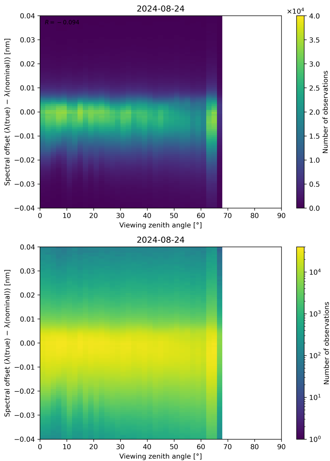
Figure 128: Scatter density plot of “Viewing zenith angle” against “Spectral offset ( \lambda(\text{true}) - \lambda(\text{nominal}) )” for 2024-08-23 to 2024-08-25.
