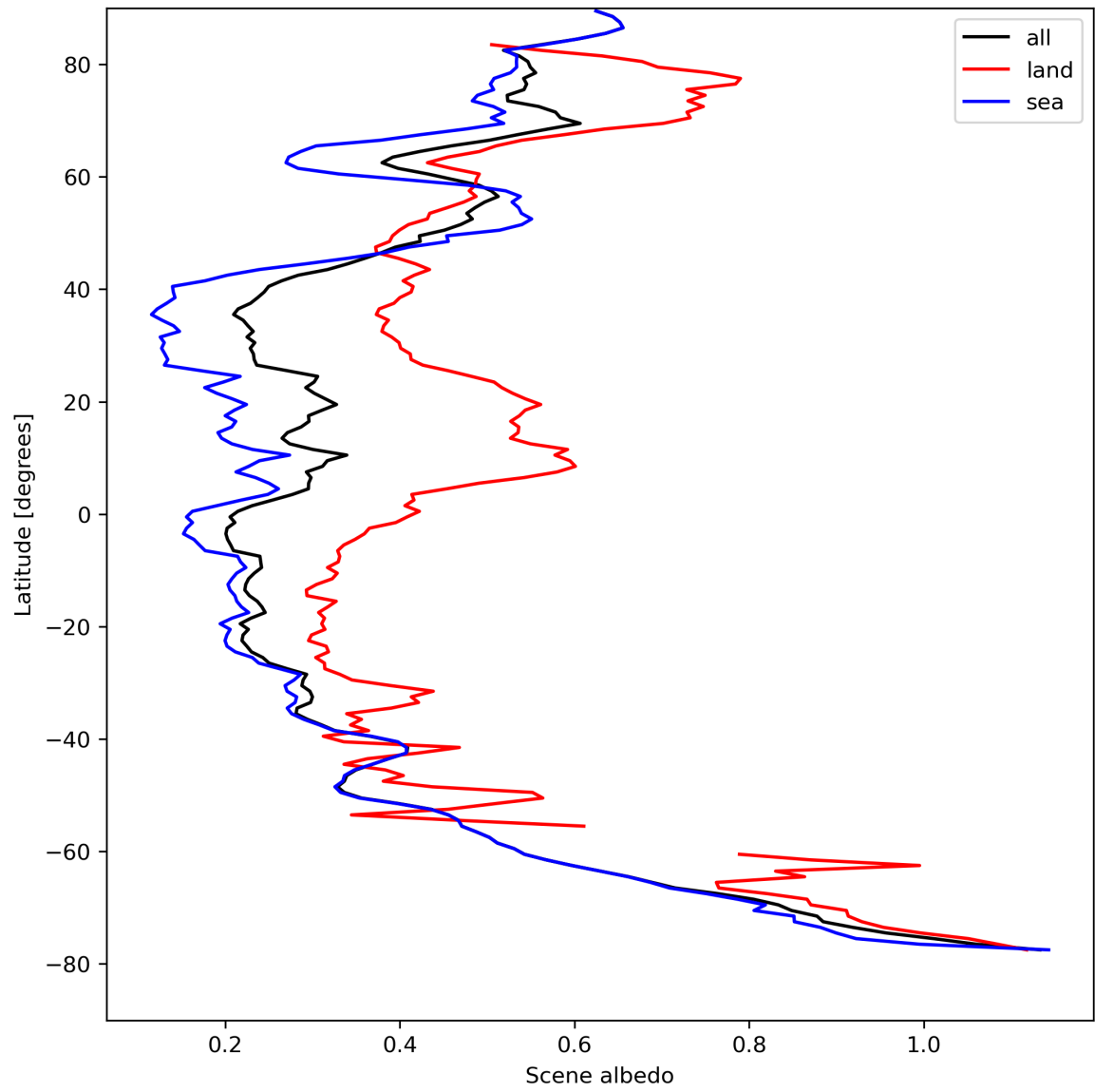
Figure 17: Zonal average of “Scene albedo” for 2024-08-23 to 2024-08-25.
