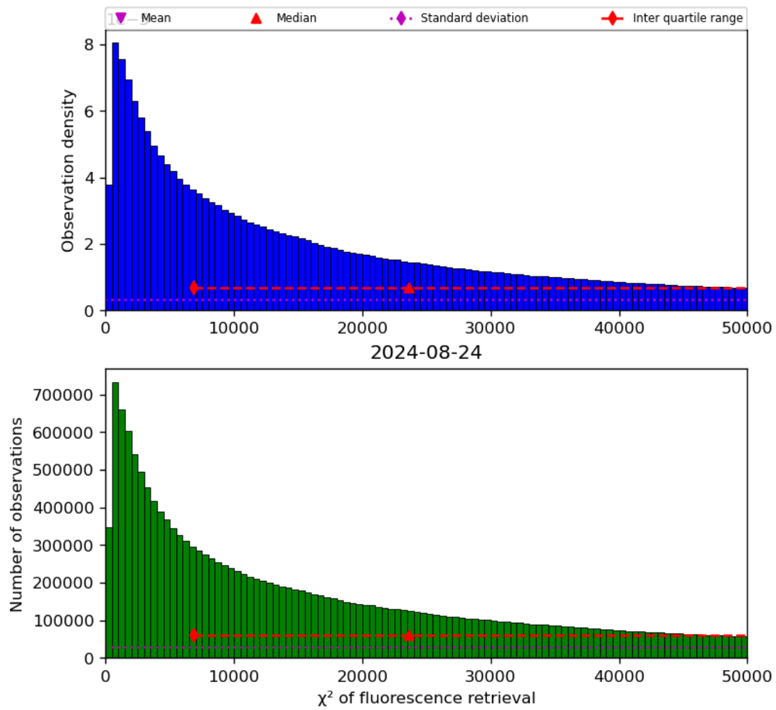
Figure 42: Histogram of “ \chi^2 of fluorescence retrieval” for 2024-08-23 to 2024-08-25
