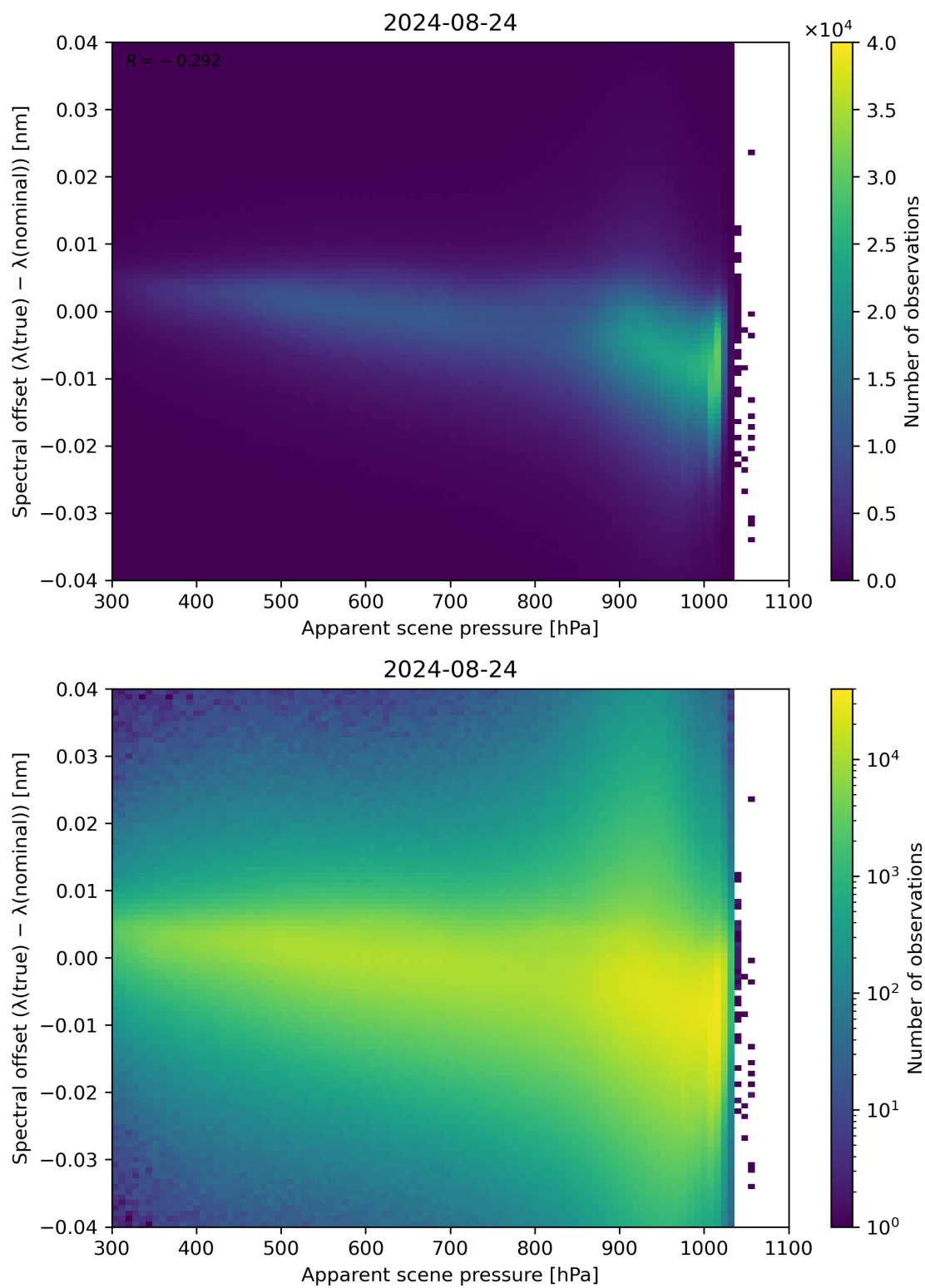
Figure 67: Scatter density plot of “Apparent scene pressure” against “Spectral offset ( \lambda(\text{true}) - \lambda(\text{nominal}) )” for 2024-08-23 to 2024-08-25.
