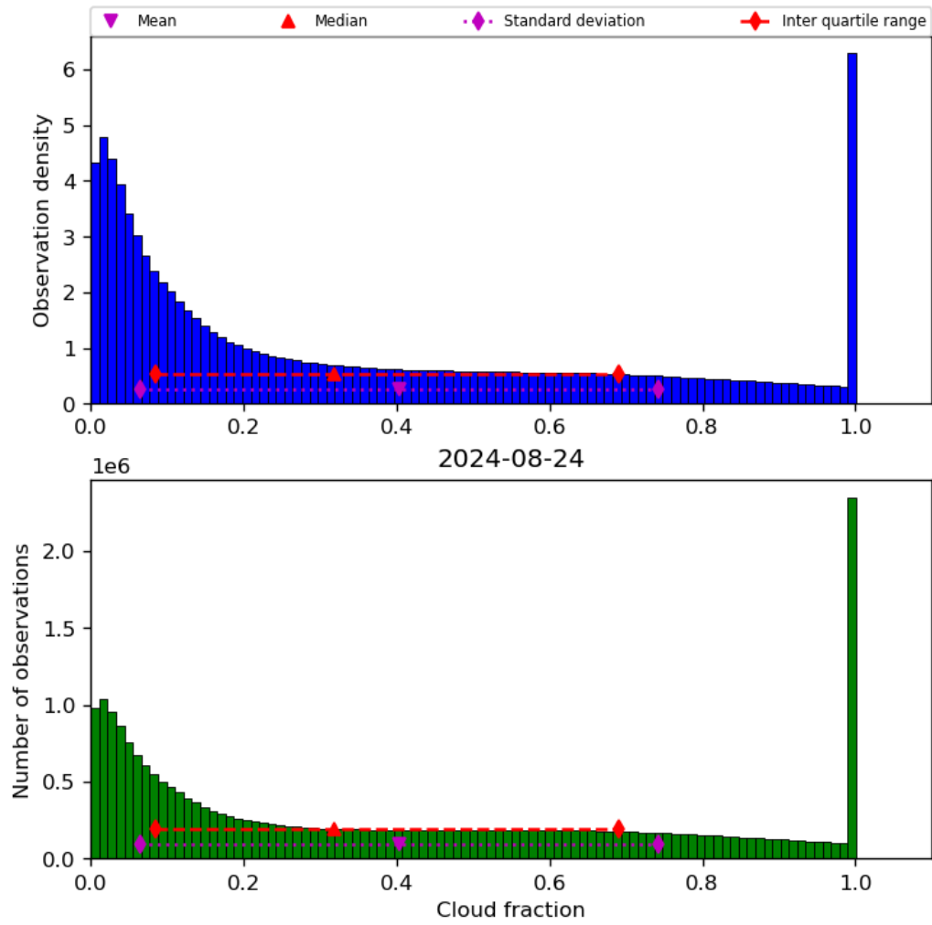
Figure 32: Histogram of “Cloud fraction” for 2024-08-23 to 2024-08-25
