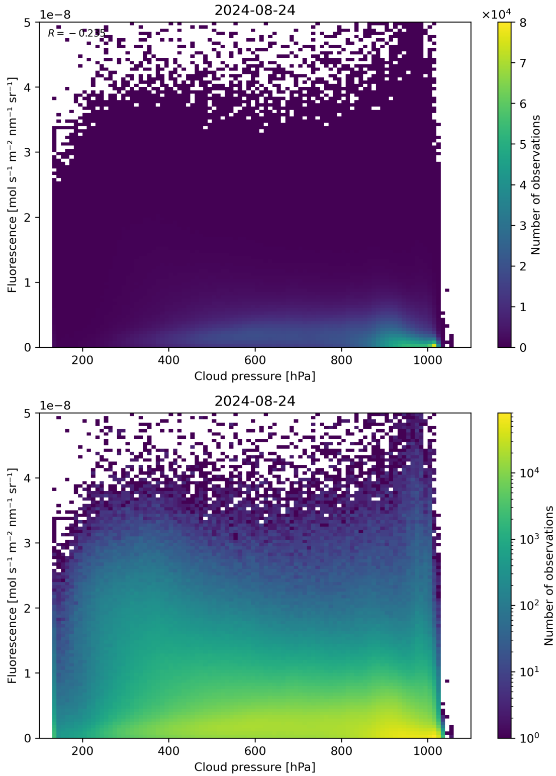
Figure 80: Scatter density plot of “Cloud pressure” against “Fluorescence” for 2024-08-23 to 2024-08-25.
