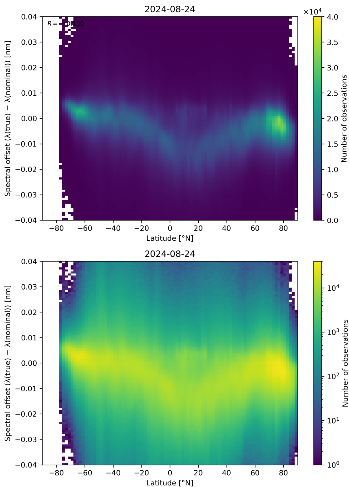
Figure 96: Scatter density plot of “Latitude” against “Spectral offset ( \lambda(\text{true}) - \lambda(\text{nominal}) )” for 2024-08-23 to 2024-08-25.
