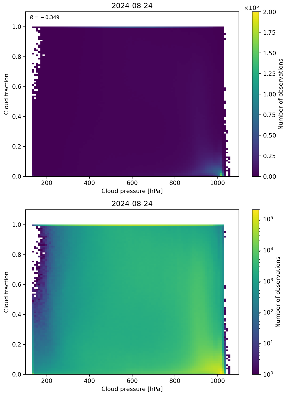
Figure 79: Scatter density plot of “Cloud pressure” against “Cloud fraction” for 2024-08-23 to 2024-08-25.
