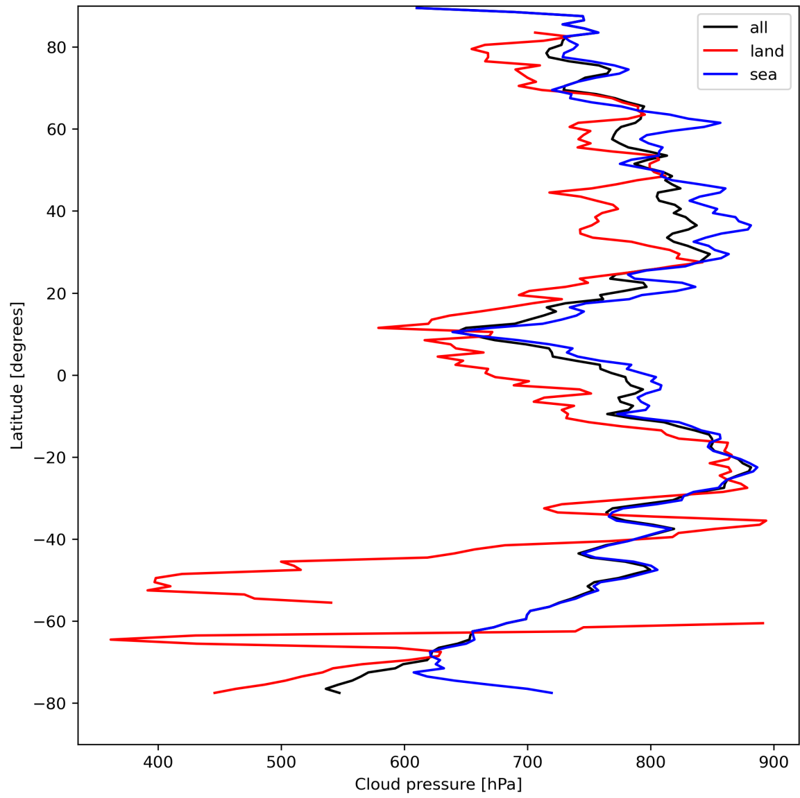
Figure 13: Zonal average of “Cloud pressure” for 2024-08-23 to 2024-08-25.
