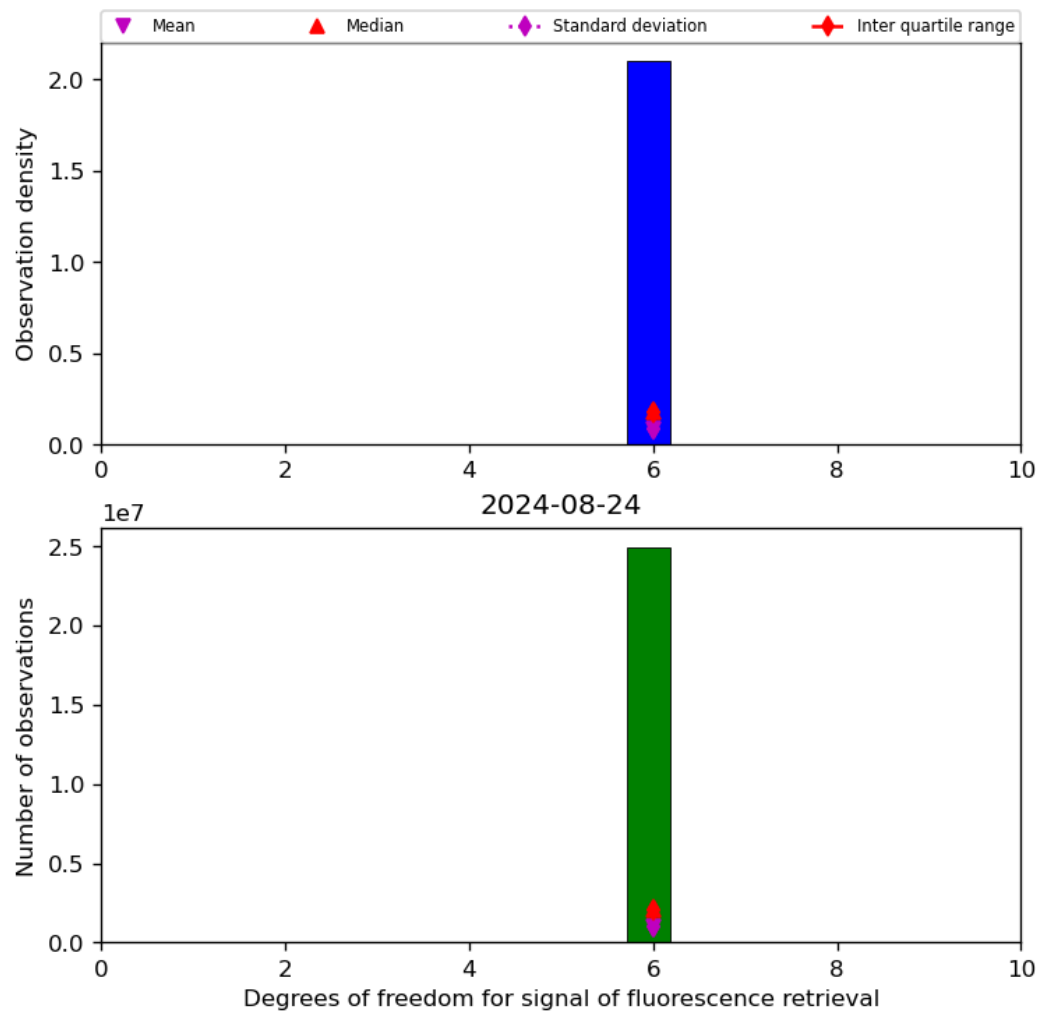
Figure 43: Histogram of “Degrees of freedom for signal of fluorescence retrieval” for 2024-08-23 to 2024-08-25
