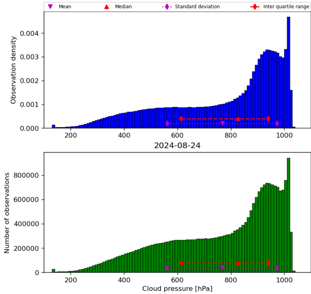
Figure 30: Histogram of “Cloud pressure” for 2024-08-23 to 2024-08-25
