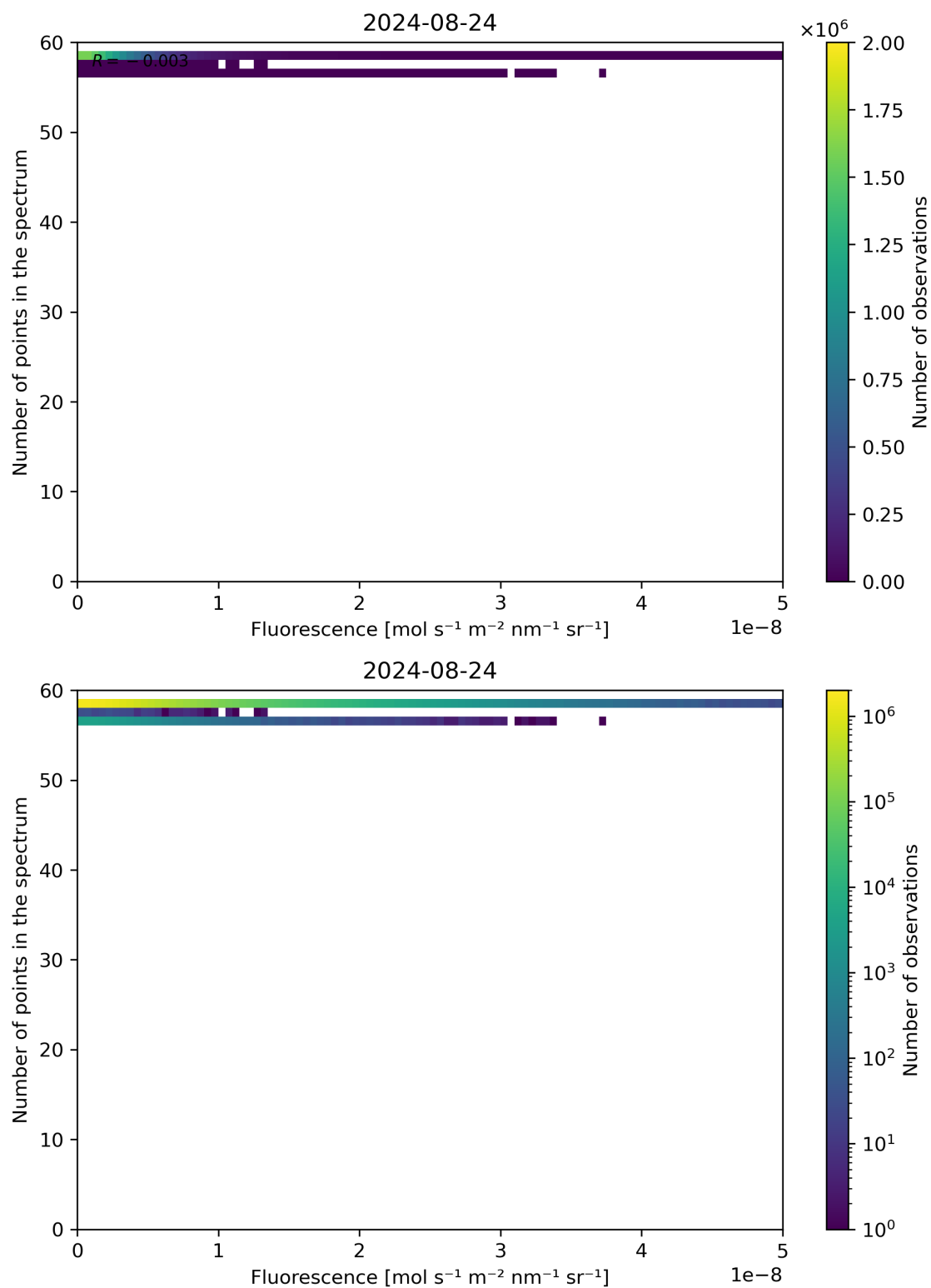
Figure 86: Scatter density plot of “Fluorescence” against “Number of points in the spectrum” for 2024-08-23 to 2024-08-25.
