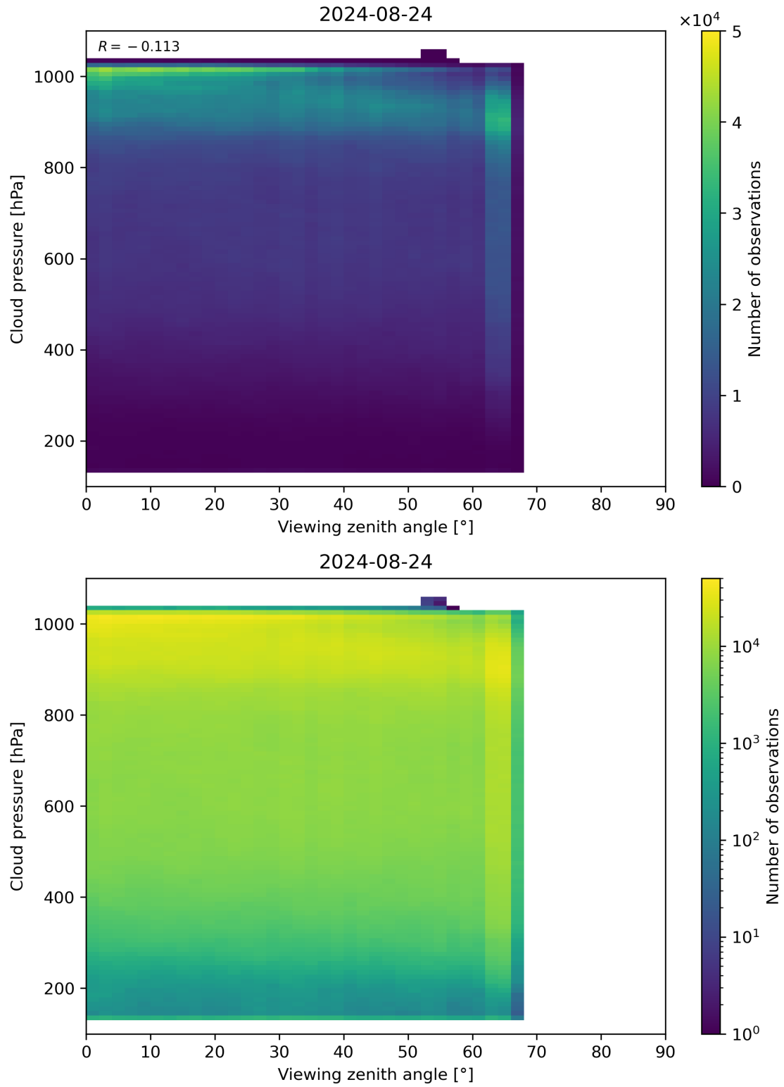
Figure 121: Scatter density plot of “Viewing zenith angle” against “Cloud pressure” for 2024-08-23 to 2024-08-25.
