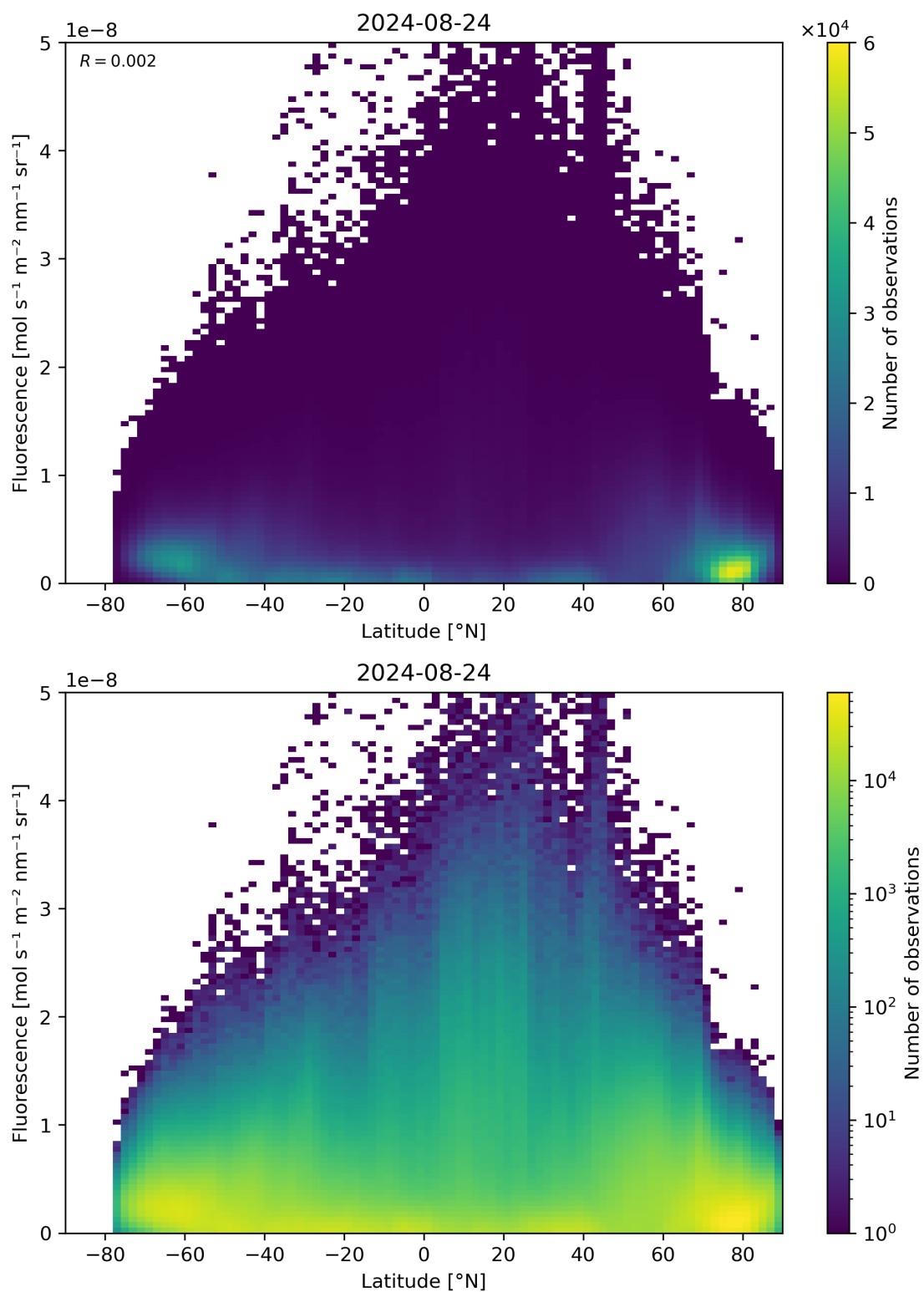
Figure 92: Scatter density plot of “Latitude” against “Fluorescence” for 2024-08-23 to 2024-08-25.
