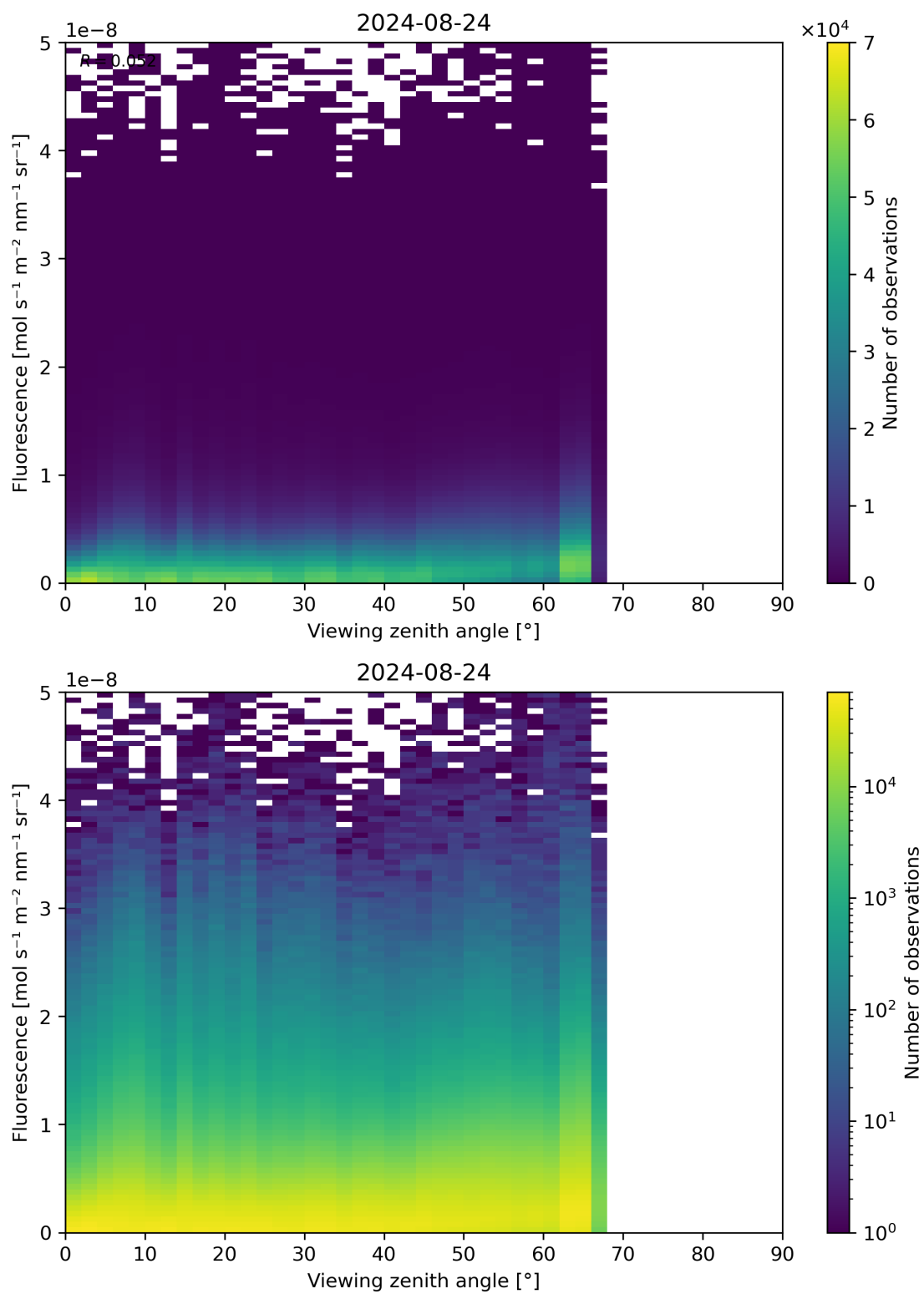
Figure 122: Scatter density plot of “Viewing zenith angle” against “Fluorescence” for 2024-08-23 to 2024-08-25.
