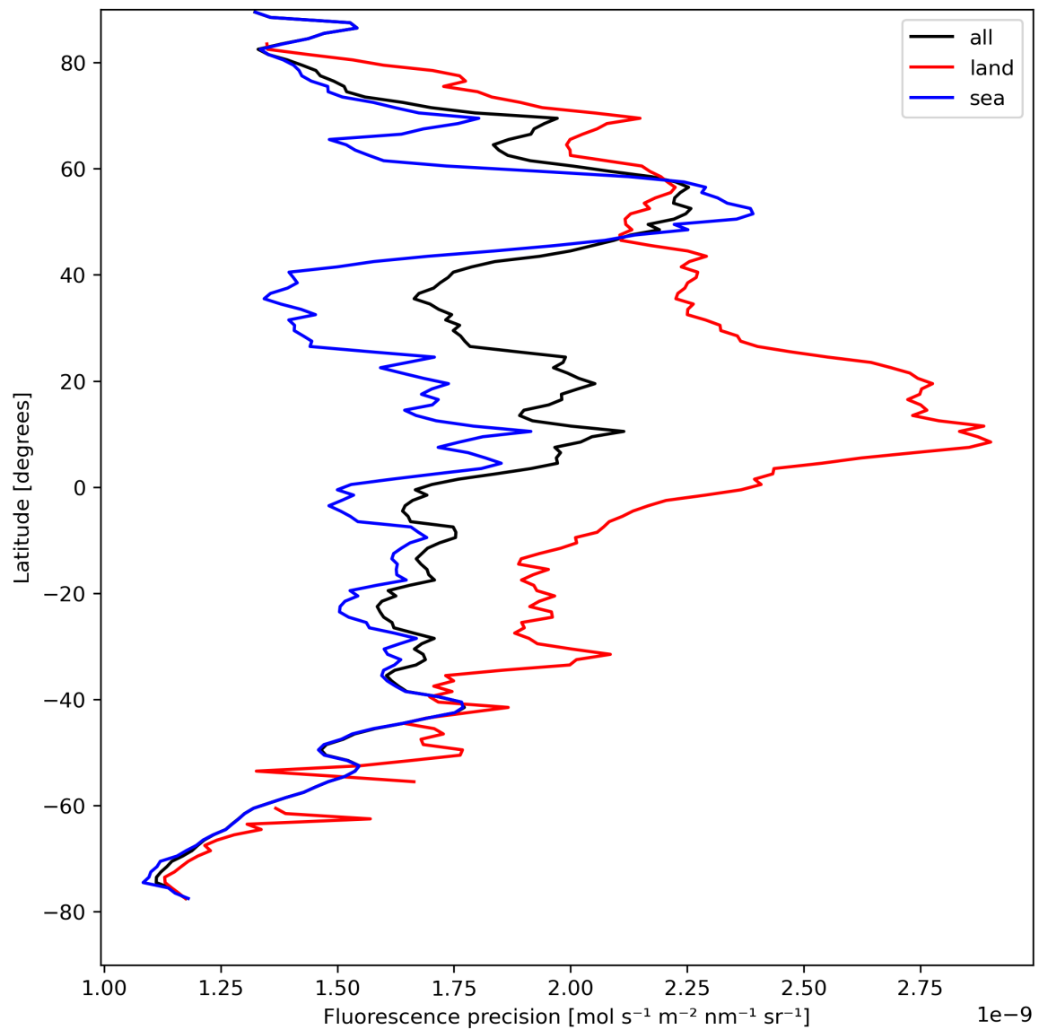
Figure 24: Zonal average of “Fluorescence precision” for 2024-08-23 to 2024-08-25.
