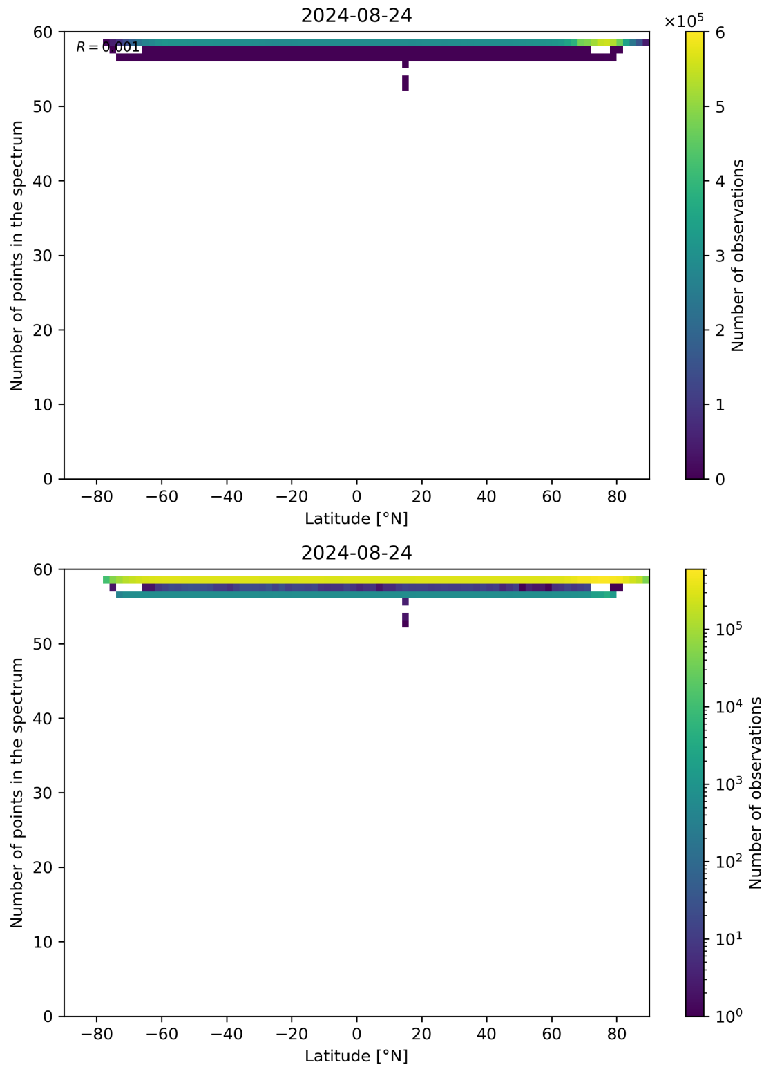
Figure 94: Scatter density plot of “Latitude” against “Number of points in the spectrum” for 2024-08-23 to 2024-08-25.
