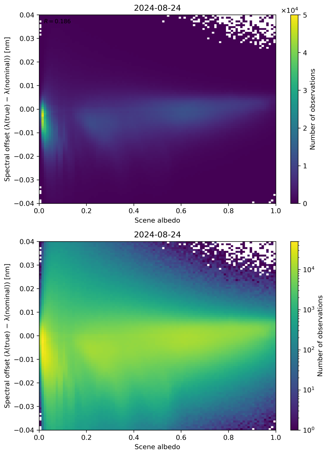
Figure 107: Scatter density plot of “Scene albedo” against “Spectral offset ( \lambda(\text{true}) - \lambda(\text{nominal}) )” for 2024-08-23 to 2024-08-25.
