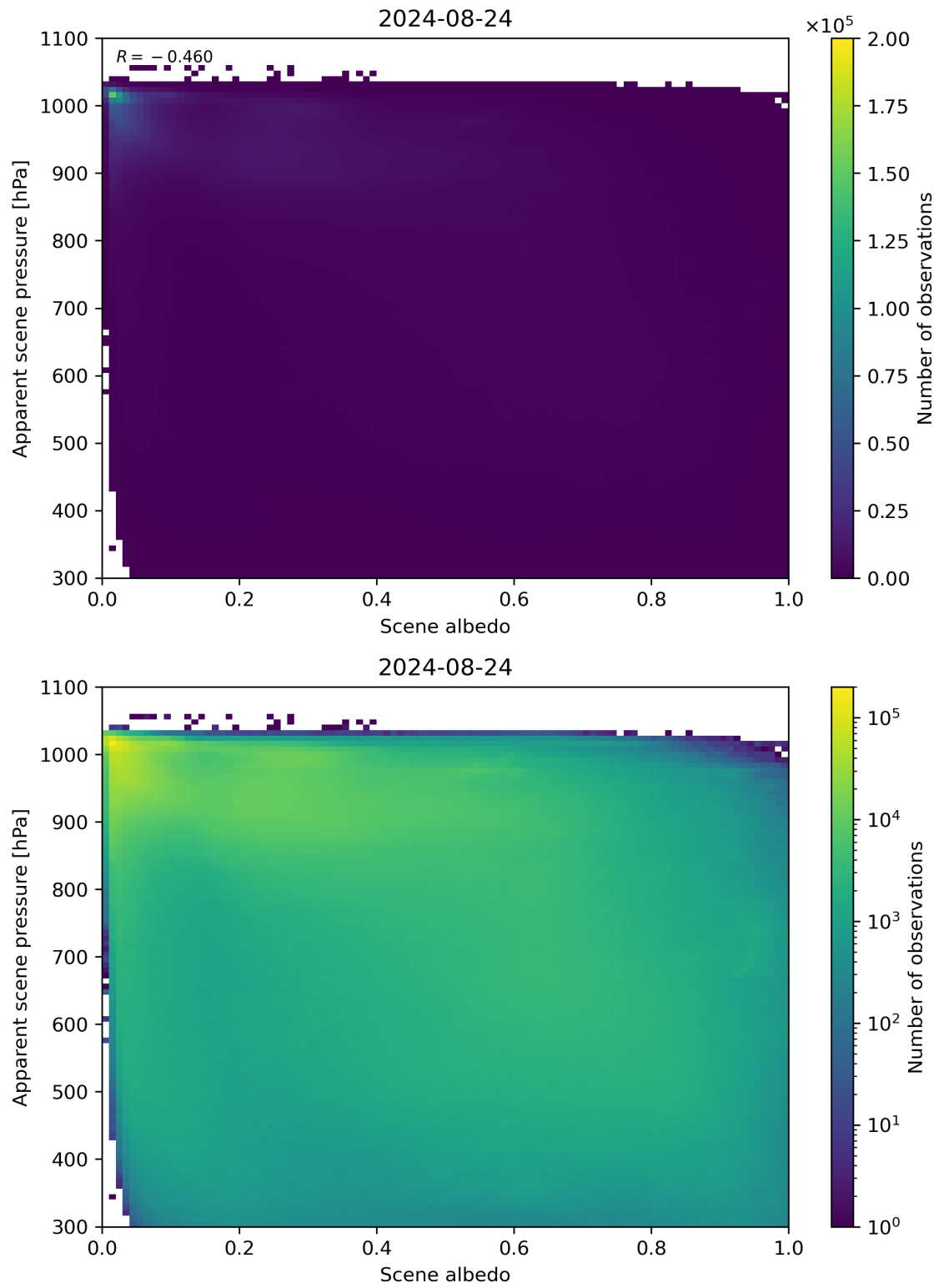
Figure 102: Scatter density plot of “Scene albedo” against “Apparent scene pressure” for 2024-08-23 to 2024-08-25.
