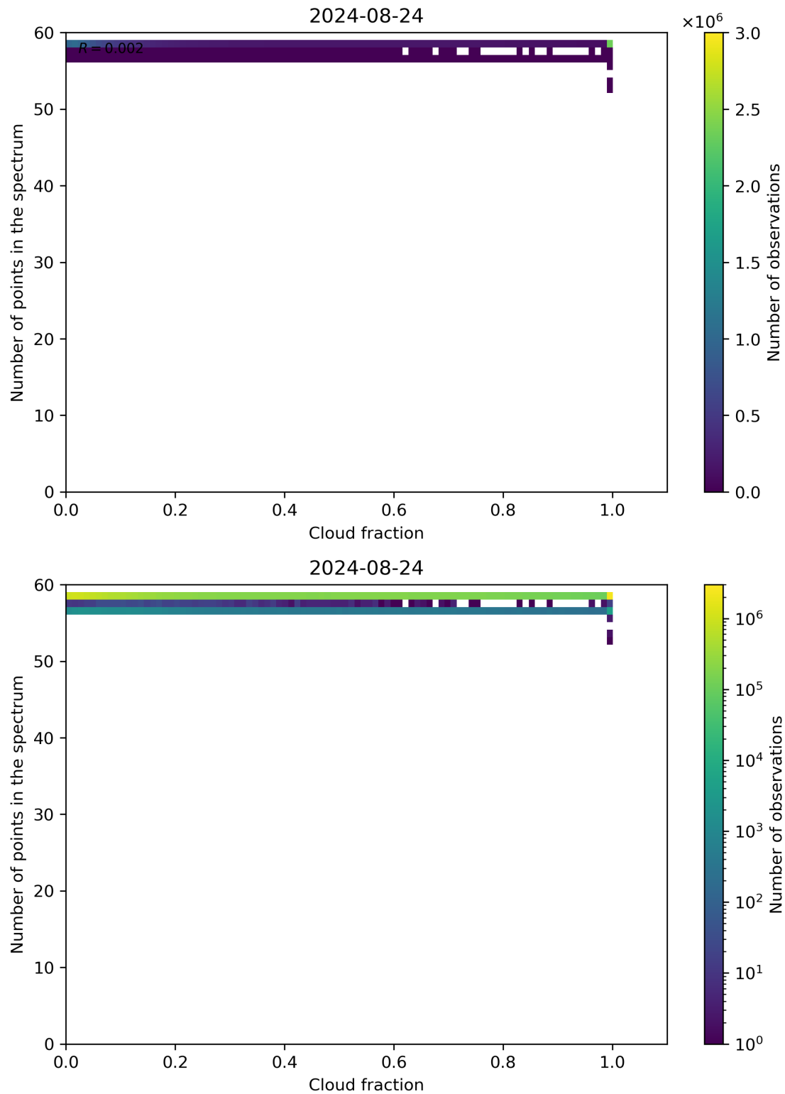
Figure 74: Scatter density plot of “Cloud fraction” against “Number of points in the spectrum” for 2024-08-23 to 2024-08-25.
