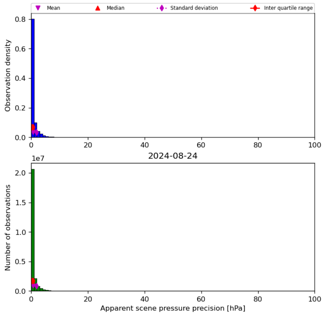
Figure 37: Histogram of “Apparent scene pressure precision” for 2024-08-23 to 2024-08-25
