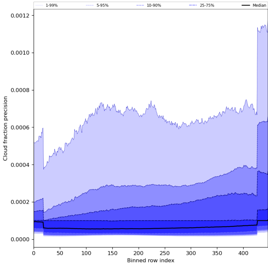
Figure 50: Along track statistics of “Cloud fraction precision” for 2024-08-23 to 2024-08-25
