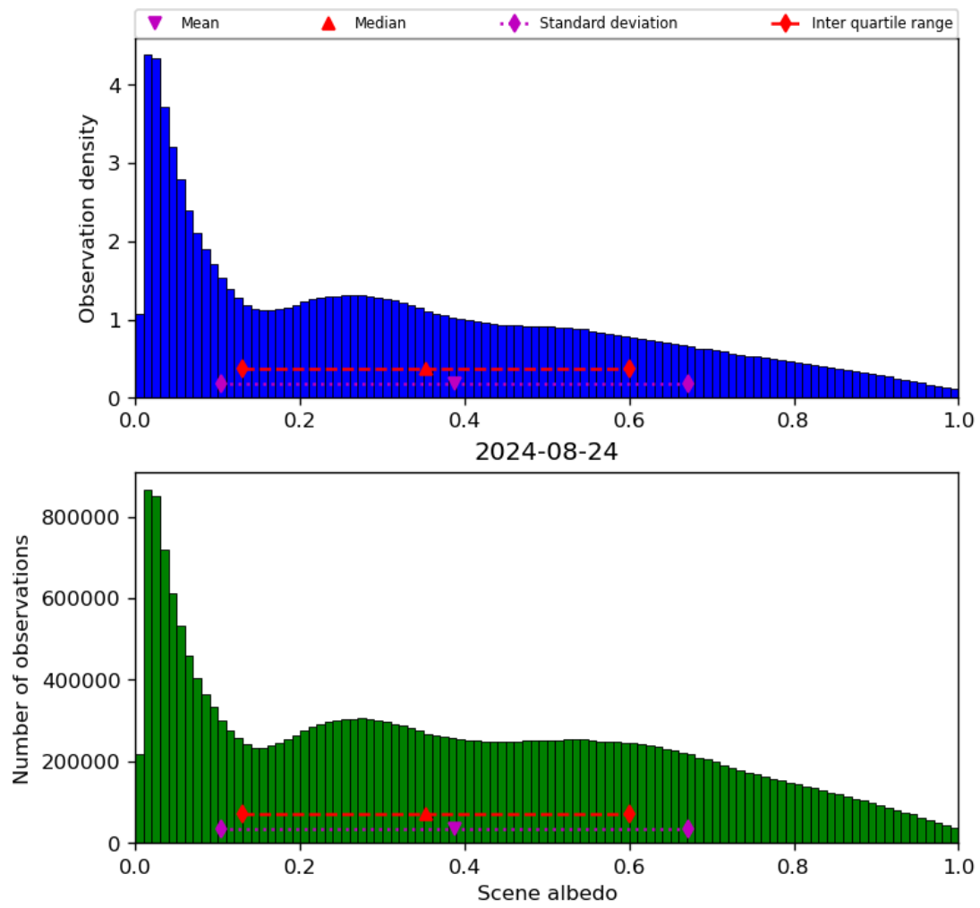
Figure 34: Histogram of “Scene albedo” for 2024-08-23 to 2024-08-25
