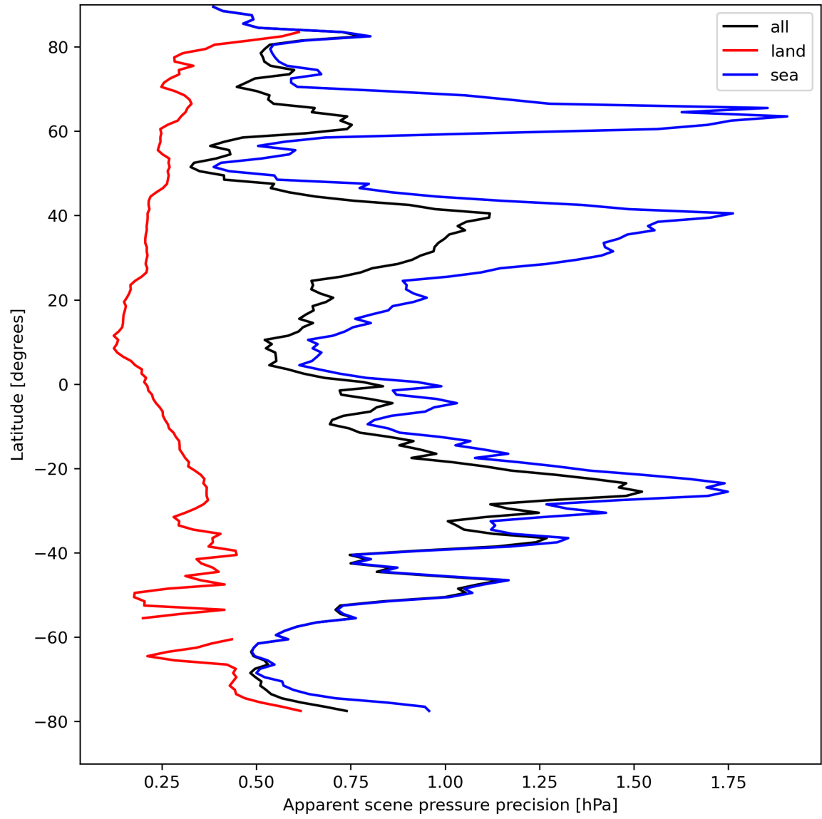
Figure 20: Zonal average of “Apparent scene pressure precision” for 2024-08-23 to 2024-08-25.
