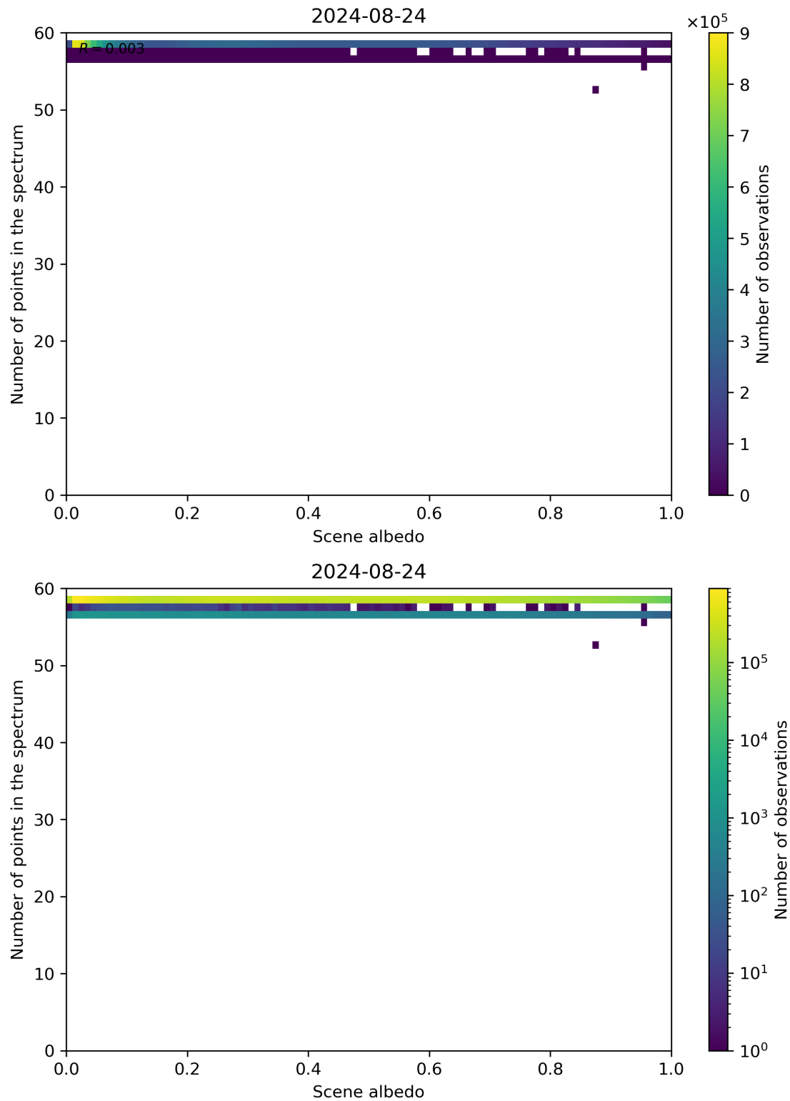
Figure 106: Scatter density plot of “Scene albedo” against “Number of points in the spectrum” for 2024-08-23 to 2024-08-25.
