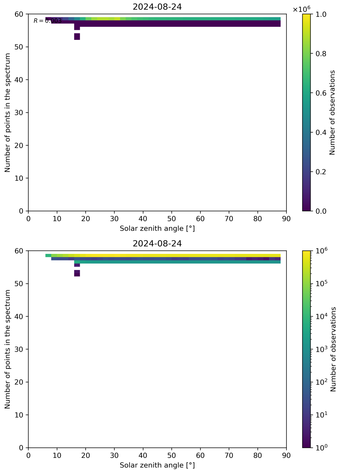
Figure 115: Scatter density plot of “Solar zenith angle” against “Number of points in the spectrum” for 2024-08-23 to 2024-08-25.
