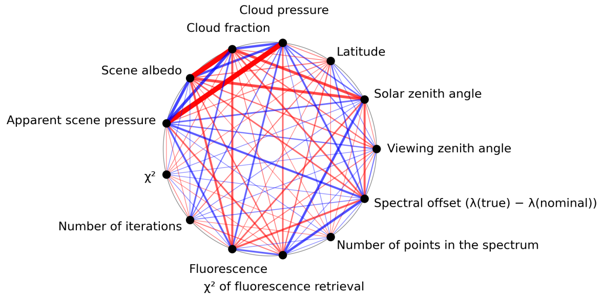
Figure 1: Map of correlation graph for 2024-08-23 to 2024-08-25.
