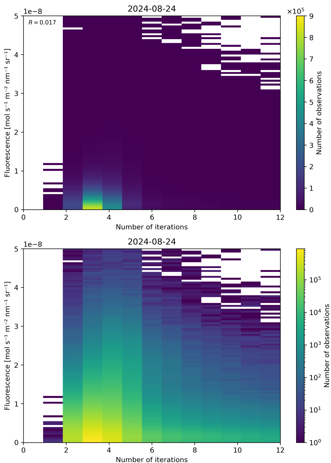
Figure 98: Scatter density plot of “Number of iterations” against “Fluorescence” for 2024-08-23 to 2024-08-25.
