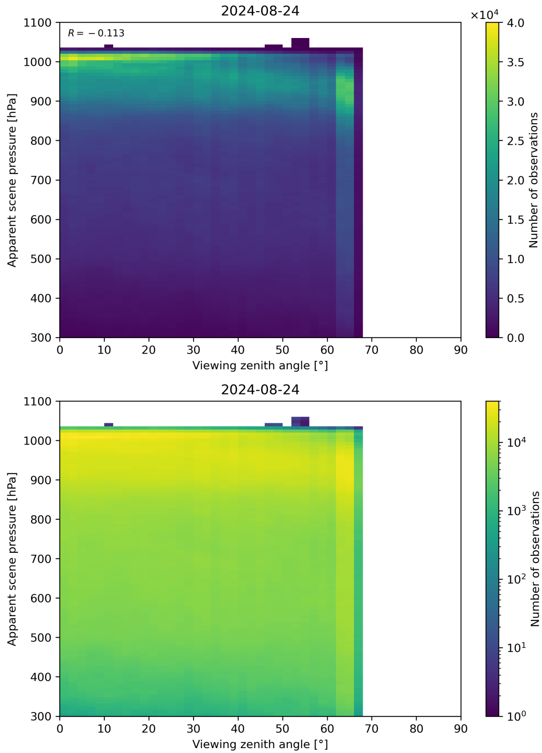
Figure 118: Scatter density plot of “Viewing zenith angle” against “Apparent scene pressure” for 2024-08-23 to 2024-08-25.
