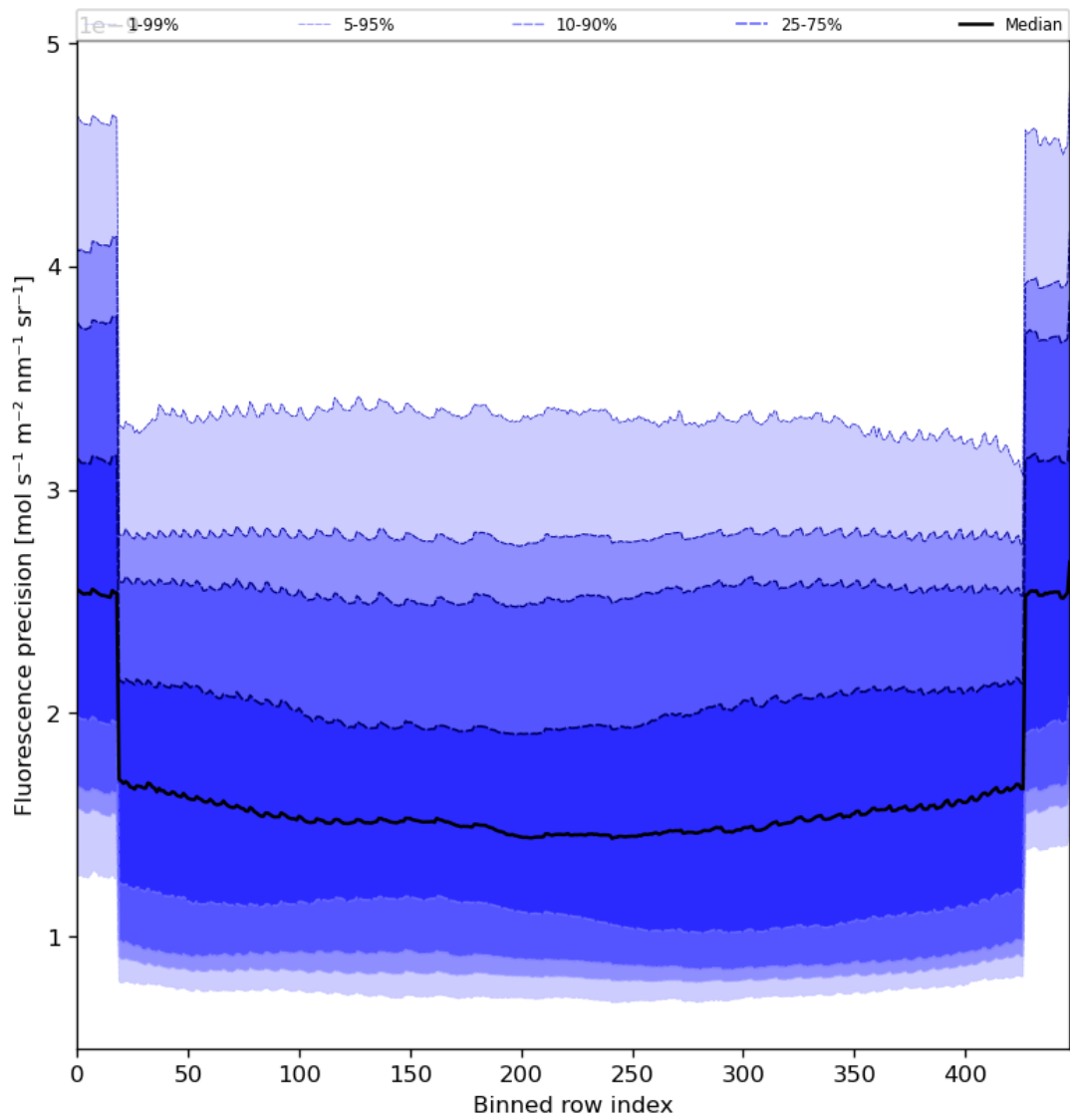
Figure 58: Along track statistics of “Fluorescence precision” for 2024-08-23 to 2024-08-25
