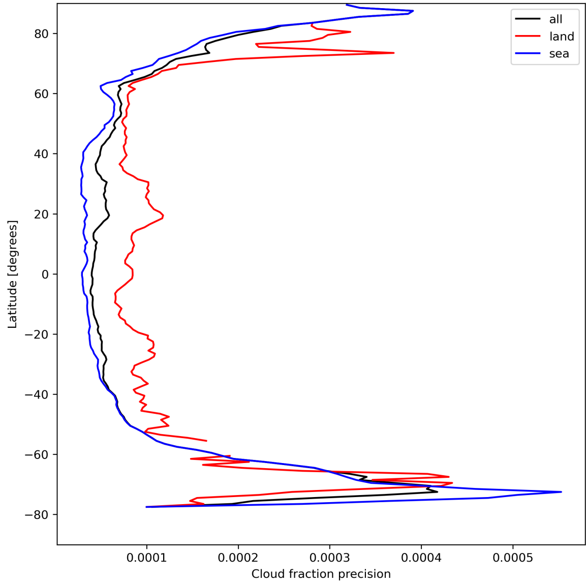
Figure 16: Zonal average of “Cloud fraction precision” for 2024-08-23 to 2024-08-25.
