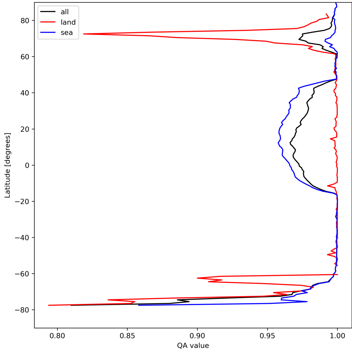
Figure 12: Zonal average of “QA value” for 2024-08-23 to 2024-08-25.
