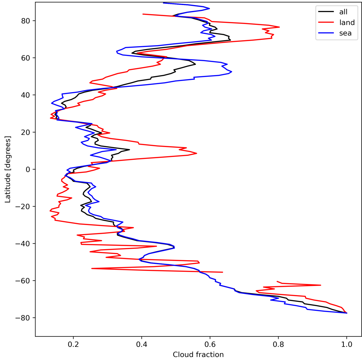
Figure 15: Zonal average of “Cloud fraction” for 2024-08-23 to 2024-08-25.
