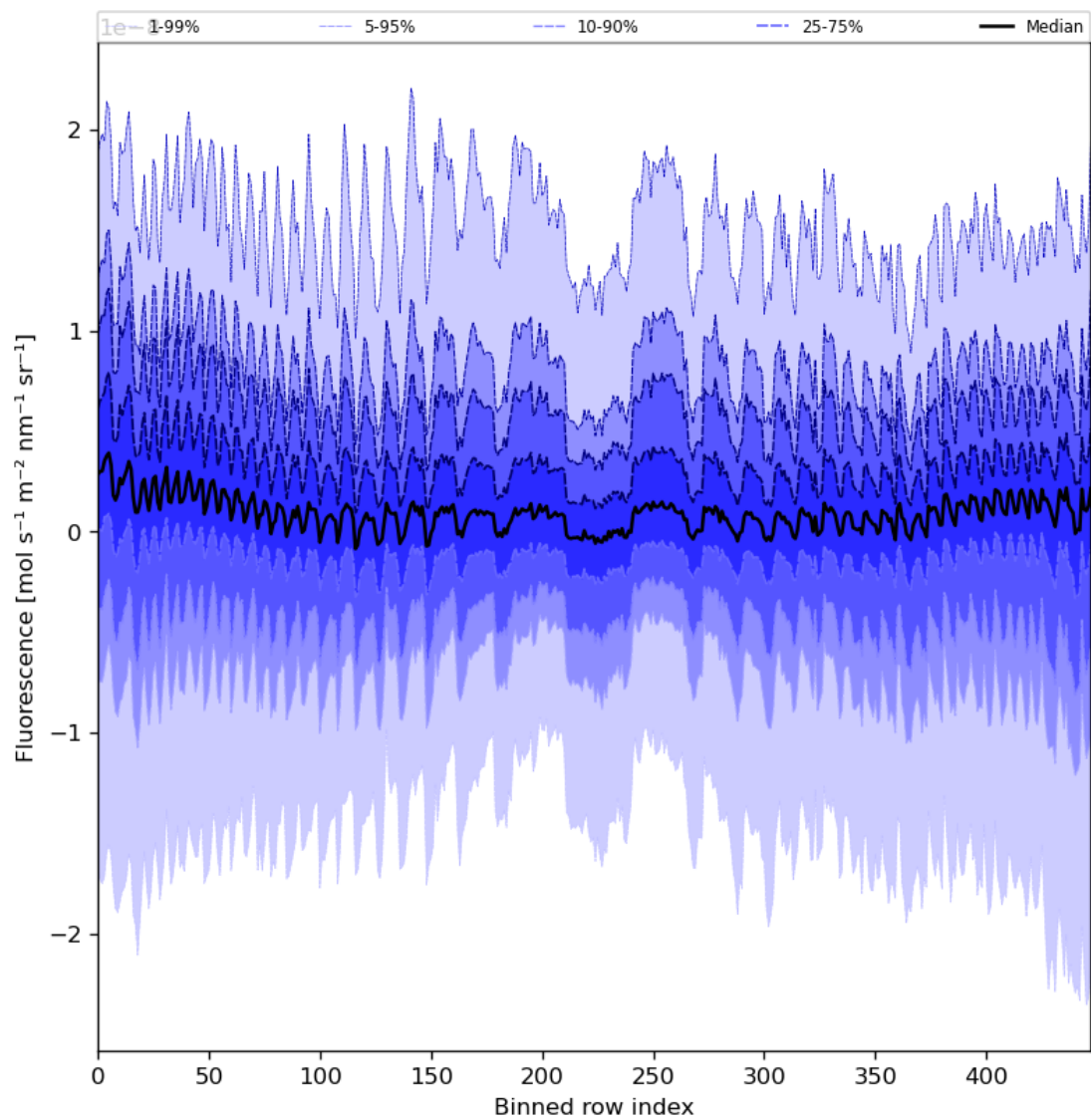
Figure 57: Along track statistics of “Fluorescence” for 2024-08-23 to 2024-08-25
