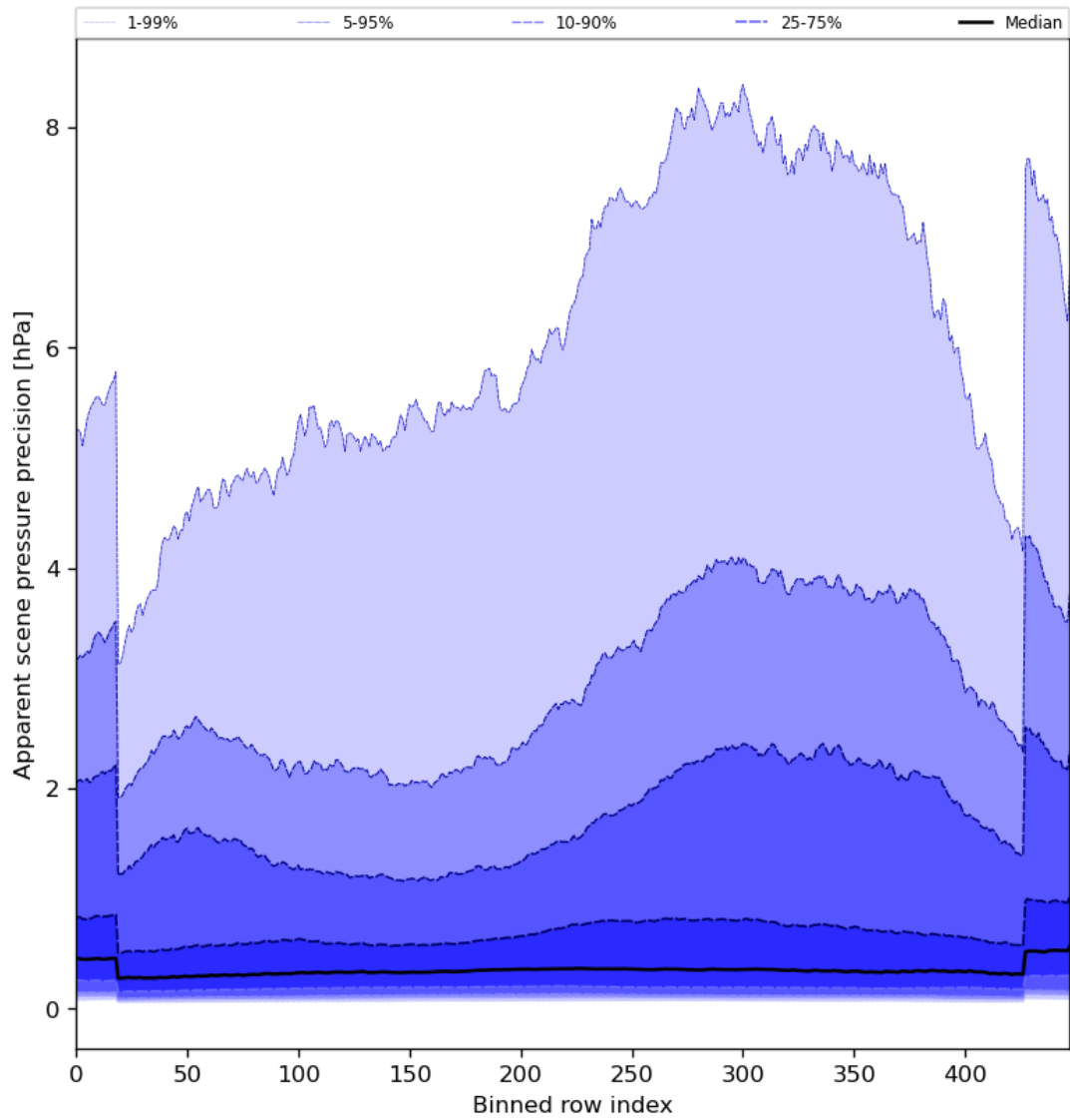
Figure 54: Along track statistics of “Apparent scene pressure precision” for 2024-08-23 to 2024-08-25
