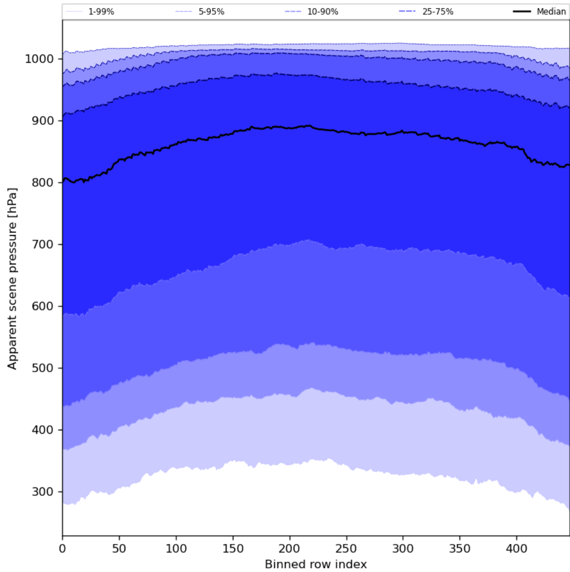
Figure 53: Along track statistics of “Apparent scene pressure” for 2024-08-23 to 2024-08-25
