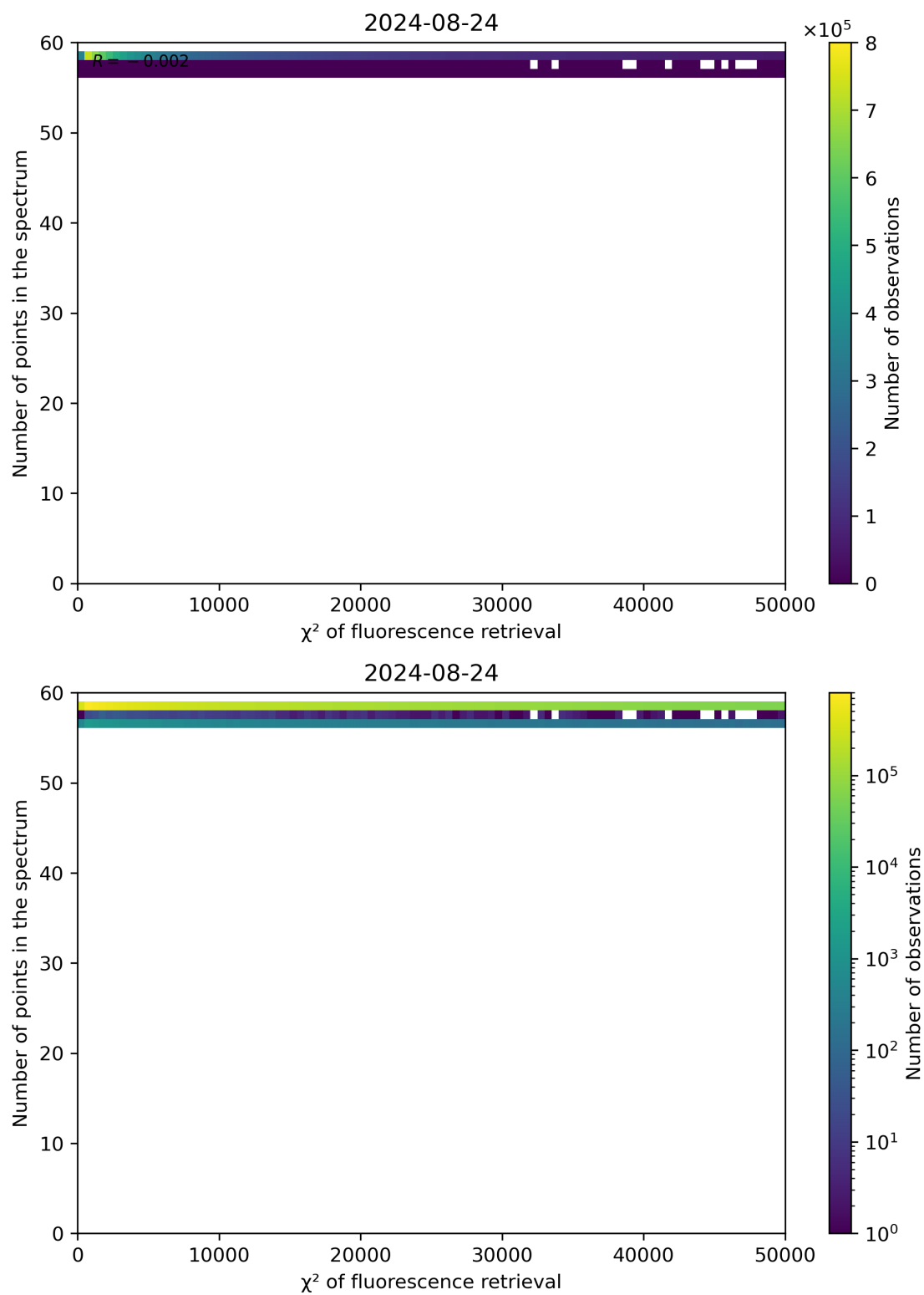
Figure 68: Scatter density plot of " \chi^2 of fluorescence retrieval" against "Number of points in the spectrum" for 2024-08-23 to 2024-08-25.
