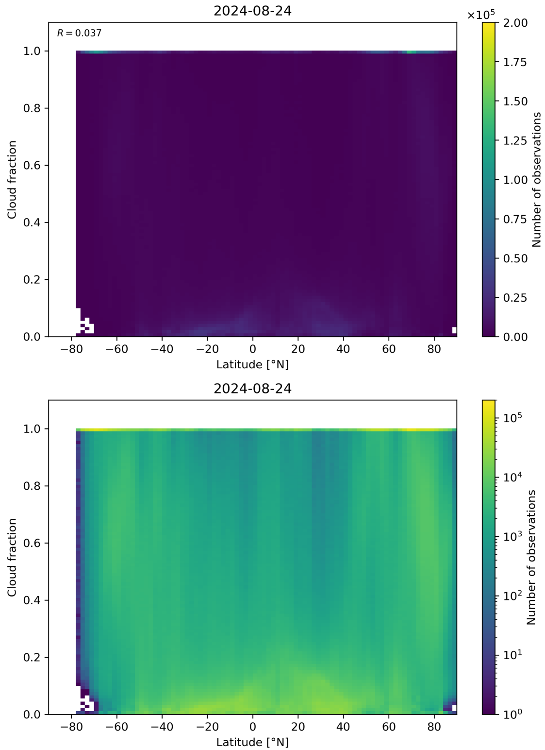
Figure 90: Scatter density plot of “Latitude” against “Cloud fraction” for 2024-08-23 to 2024-08-25.
