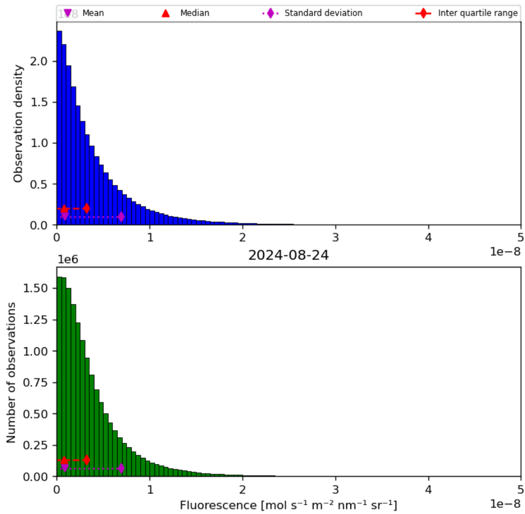
Figure 40: Histogram of “Fluorescence” for 2024-08-23 to 2024-08-25
