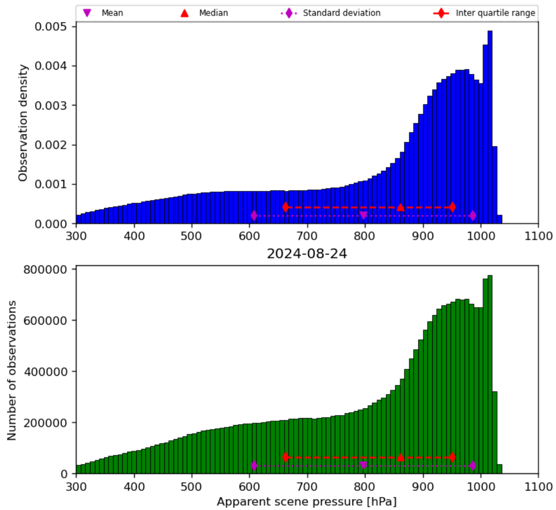
Figure 36: Histogram of “Apparent scene pressure” for 2024-08-23 to 2024-08-25
