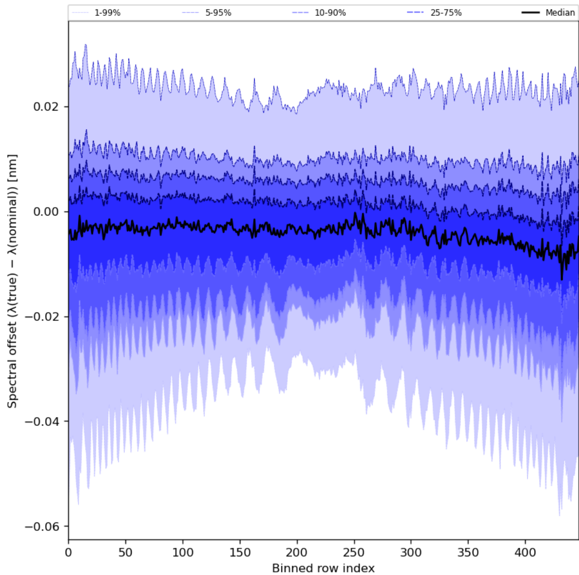
Figure 62: Along track statistics of “Spectral offset ( \lambda(\text{true}) - \lambda(\text{nominal}) )” for 2024-08-23 to 2024-08-25
