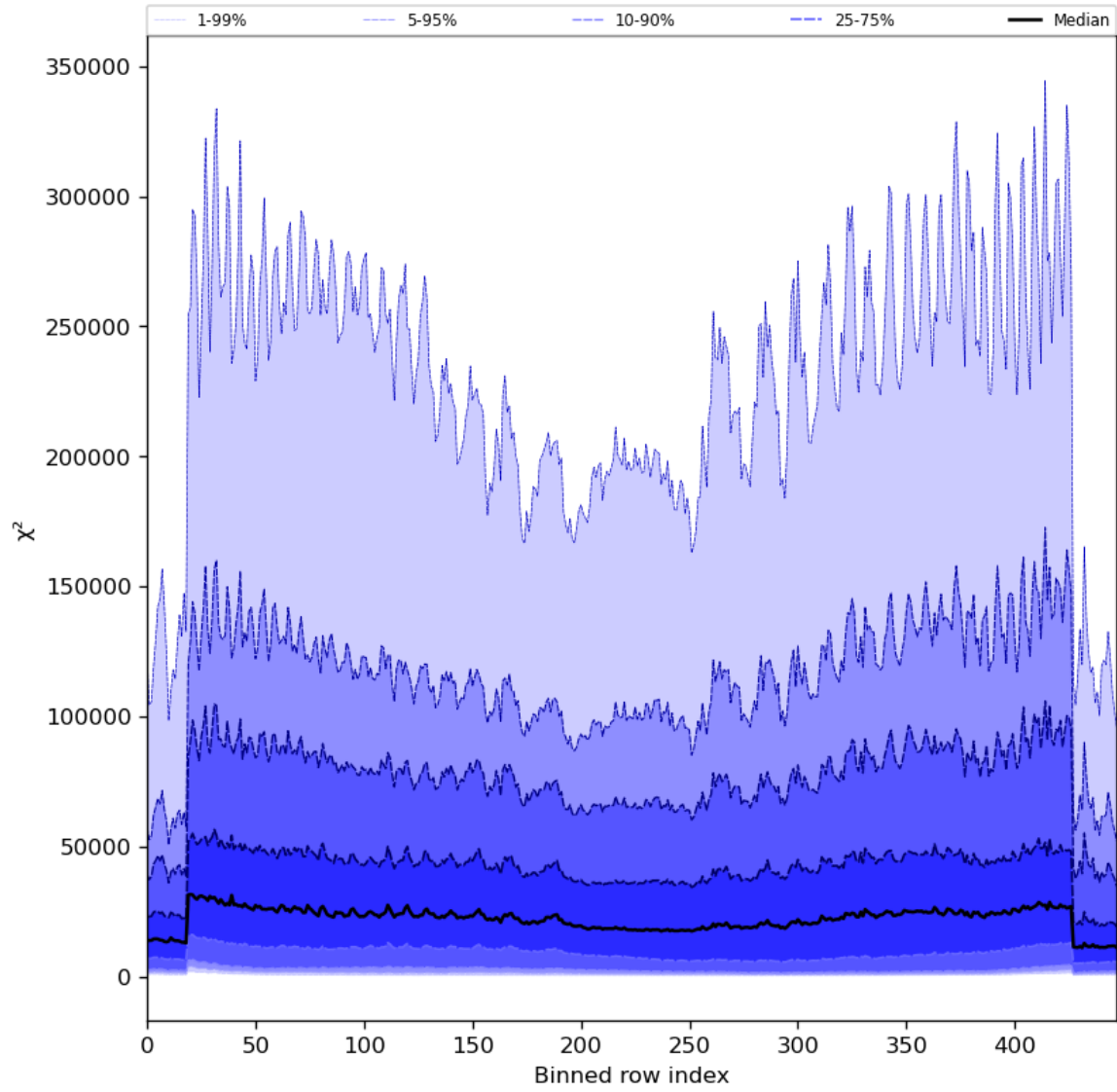
Figure 55: Along track statistics of “ \chi^2 ” for 2024-08-23 to 2024-08-25
