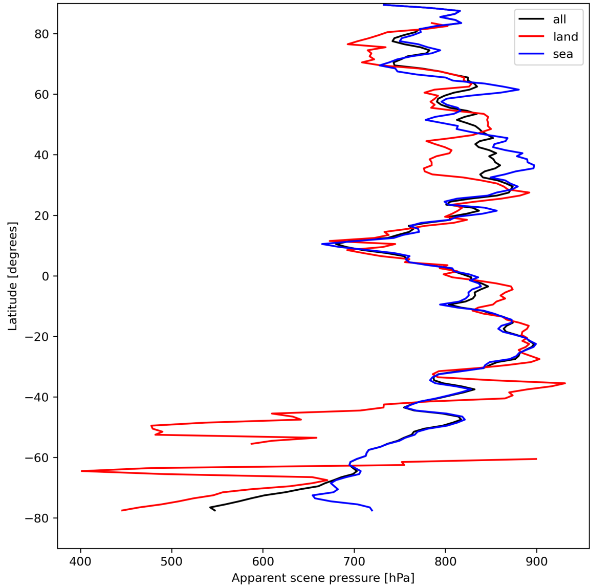
Figure 19: Zonal average of “Apparent scene pressure” for 2024-08-23 to 2024-08-25.
