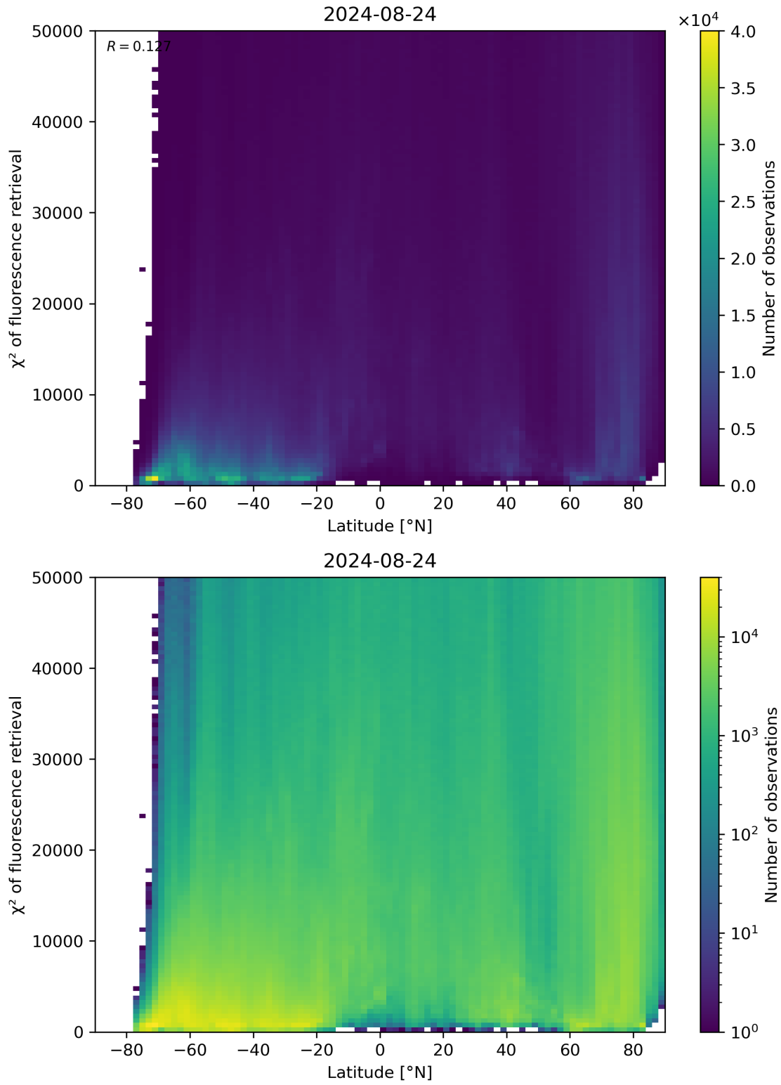
Figure 89: Scatter density plot of “Latitude” against “ \chi^2 of fluorescence retrieval” for 2024-08-23 to 2024-08-25.
