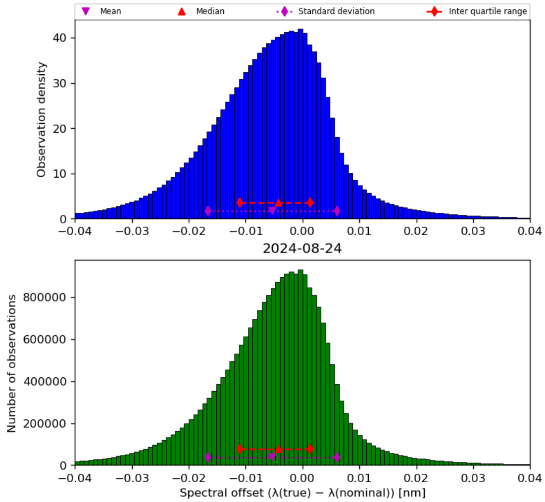
Figure 45: Histogram of “Spectral offset ( \lambda(\text{true}) - \lambda(\text{nominal}) )” for 2024-08-23 to 2024-08-25
