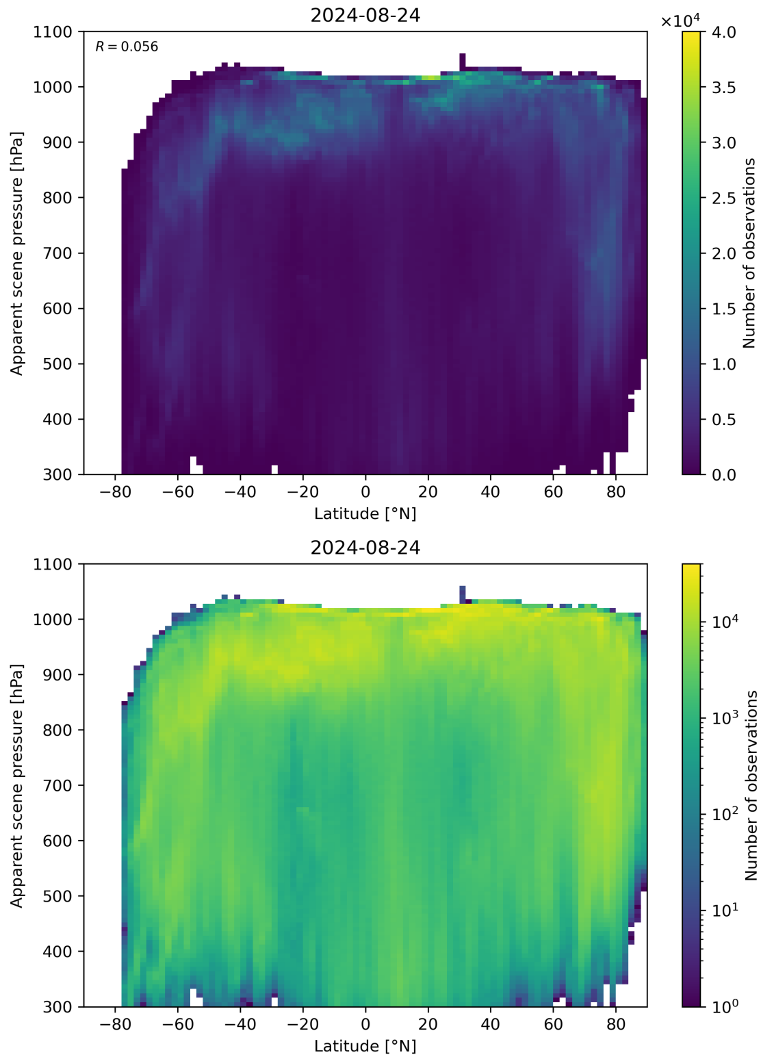
Figure 88: Scatter density plot of “Latitude” against “Apparent scene pressure” for 2024-08-23 to 2024-08-25.
