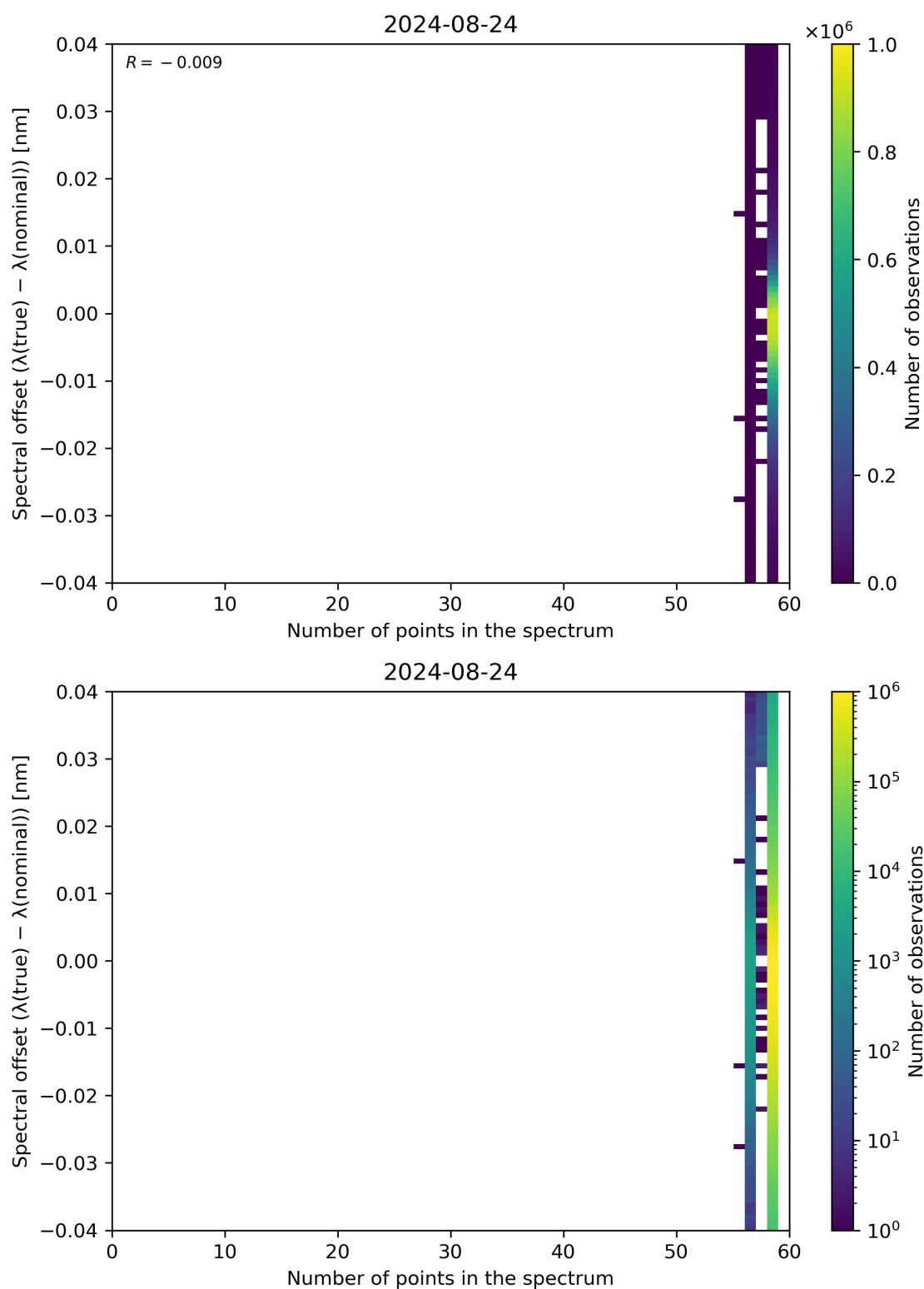
Figure 101: Scatter density plot of “Number of points in the spectrum” against “Spectral offset ( \lambda(\text{true}) - \lambda(\text{nominal}) )” for 2024-08-23 to 2024-08-25.
