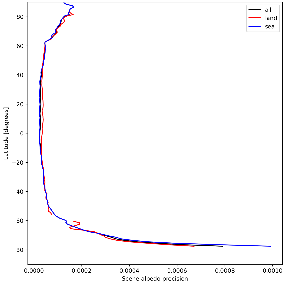
Figure 18: Zonal average of “Scene albedo precision” for 2024-08-23 to 2024-08-25.
