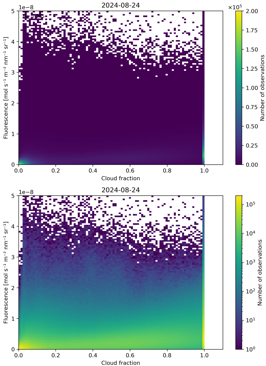
Figure 72: Scatter density plot of “Cloud fraction” against “Fluorescence” for 2024-08-23 to 2024-08-25.
