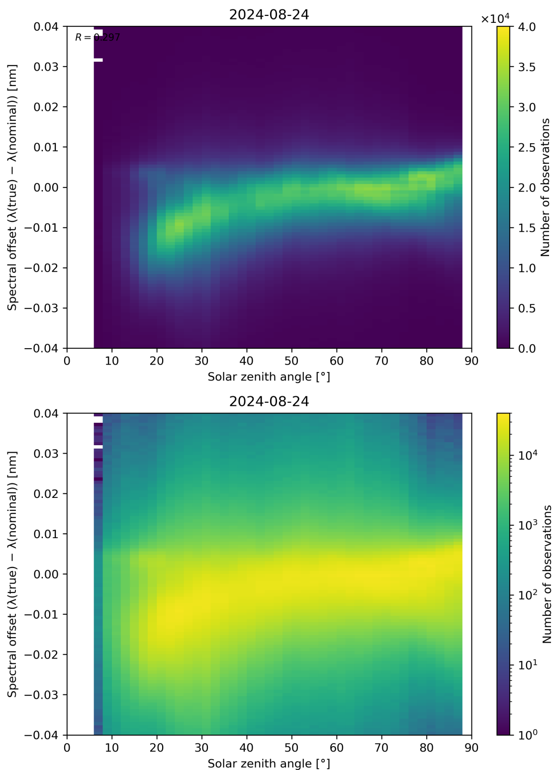
Figure 117: Scatter density plot of “Solar zenith angle” against “Spectral offset ( \lambda(\text{true}) - \lambda(\text{nominal}) )” for 2024-08-23 to 2024-08-25.
