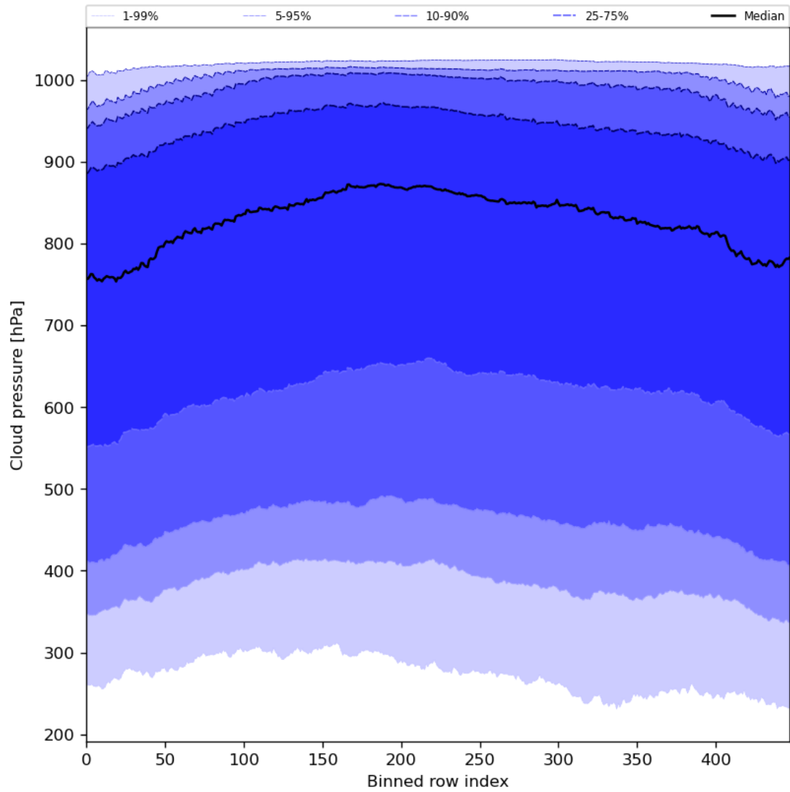
Figure 47: Along track statistics of “Cloud pressure” for 2024-08-23 to 2024-08-25
