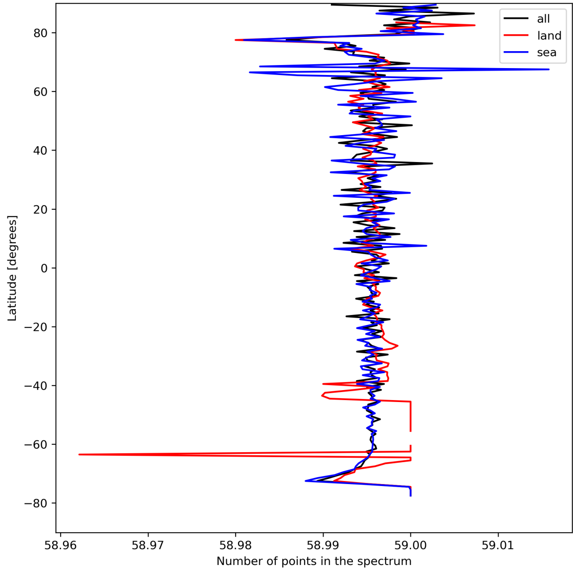
Figure 27: Zonal average of “Number of points in the spectrum” for 2024-08-23 to 2024-08-25.
