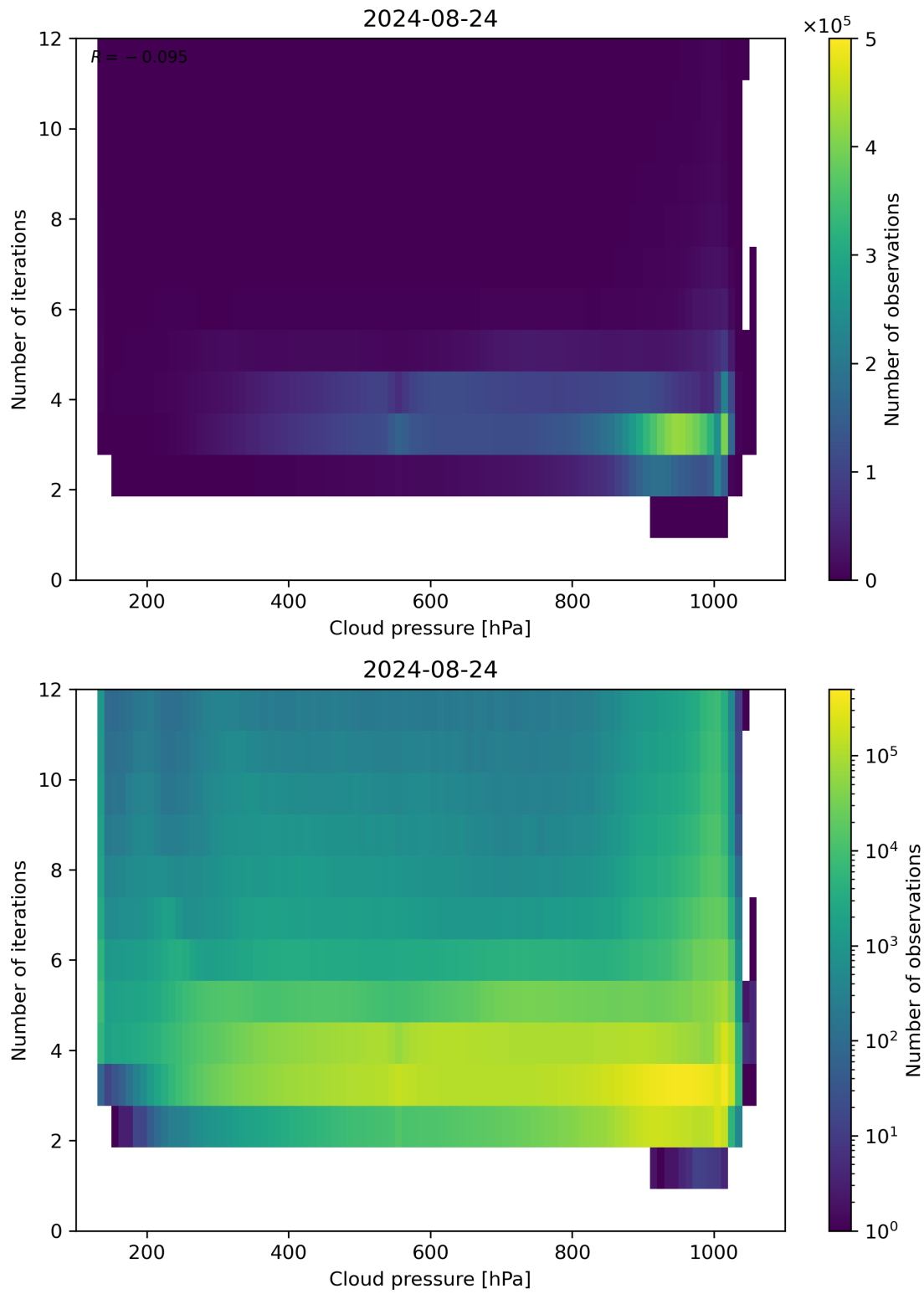
Figure 81: Scatter density plot of “Cloud pressure” against “Number of iterations” for 2024-08-23 to 2024-08-25.
