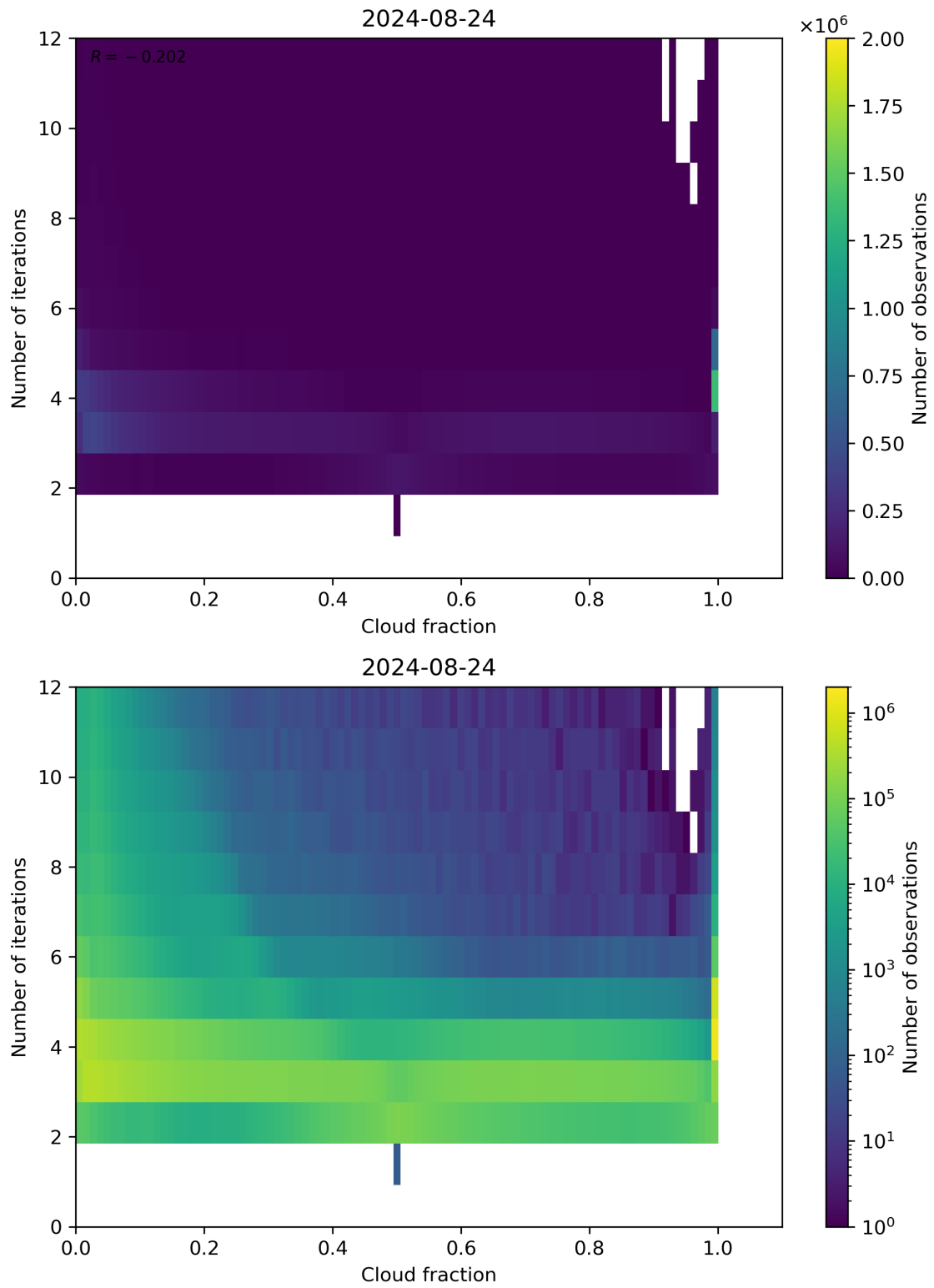
Figure 73: Scatter density plot of “Cloud fraction” against “Number of iterations” for 2024-08-23 to 2024-08-25.
