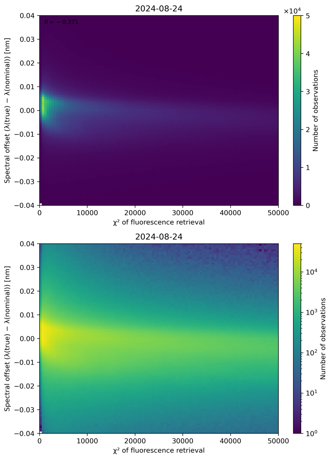
Figure 69: Scatter density plot of “ \chi^2 of fluorescence retrieval” against “Spectral offset ( \lambda(\text{true}) - \lambda(\text{nominal}) )” for 2024-08-23 to 2024-08-25.
