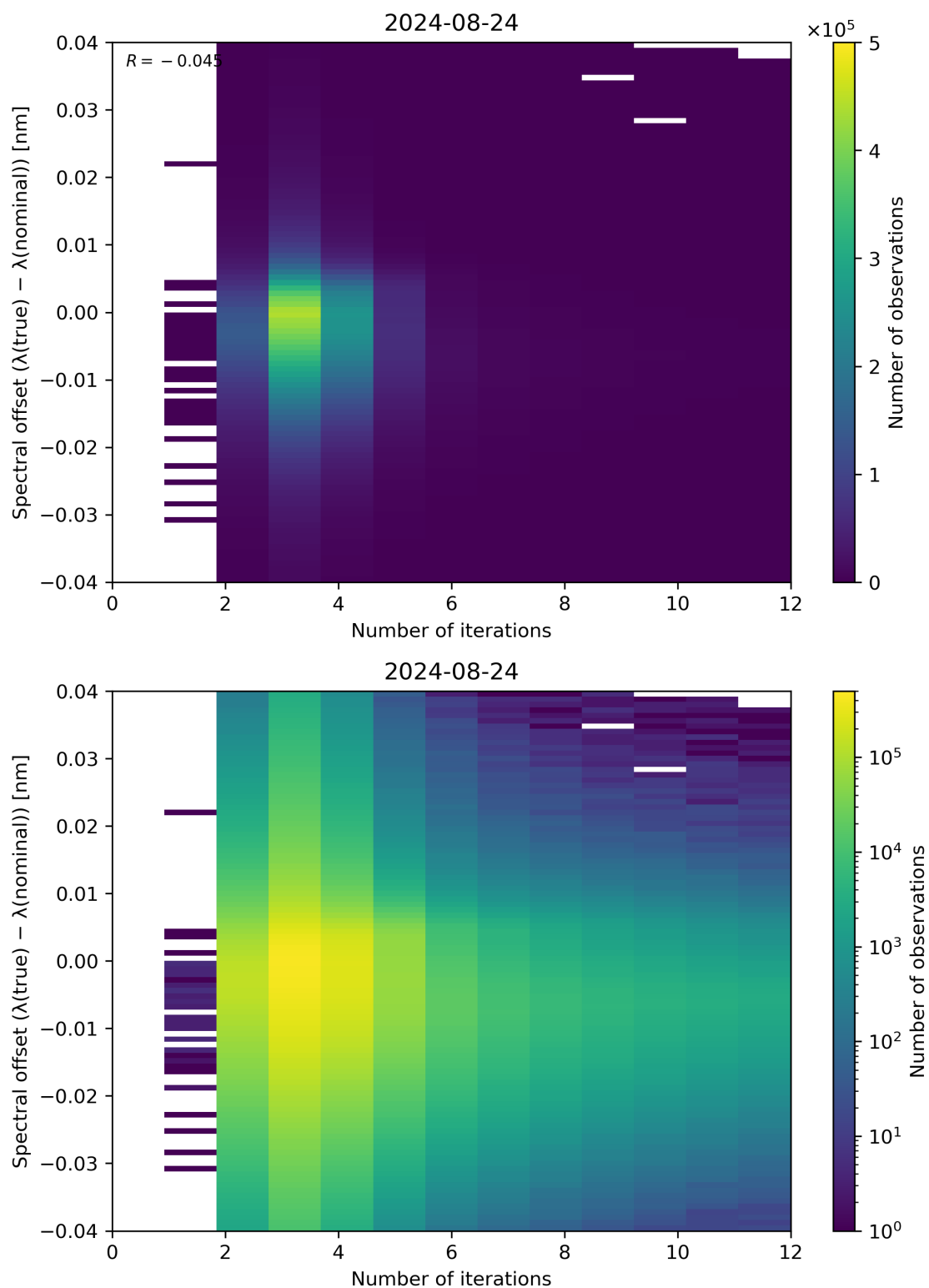
Figure 100: Scatter density plot of “Number of iterations” against “Spectral offset ( \lambda(\text{true}) - \lambda(\text{nominal}) )” for 2024-08-23 to 2024-08-25.
