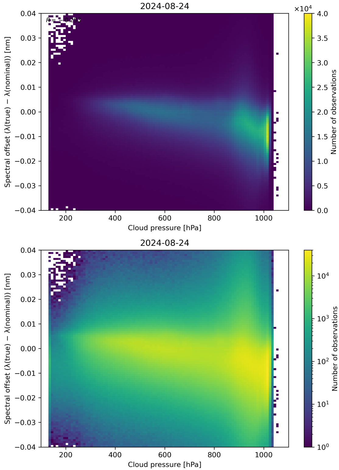
Figure 84: Scatter density plot of “Cloud pressure” against “Spectral offset ( \lambda(\text{true}) - \lambda(\text{nominal}) )” for 2024-08-23 to 2024-08-25.
