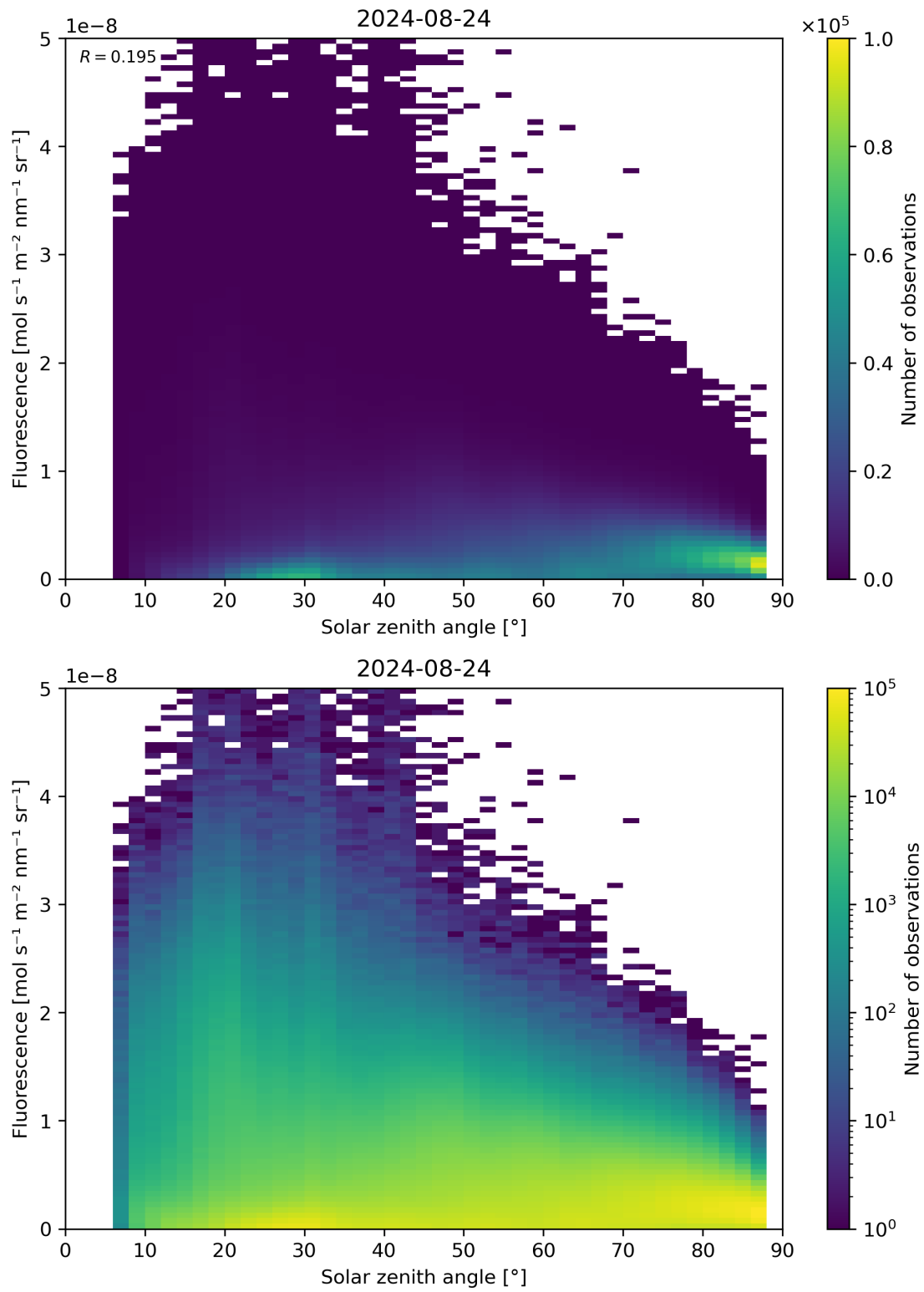
Figure 112: Scatter density plot of “Solar zenith angle” against “Fluorescence” for 2024-08-23 to 2024-08-25.
