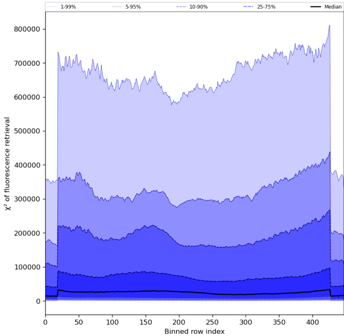
Figure 59: Along track statistics of “ \chi^2 of fluorescence retrieval” for 2024-08-23 to 2024-08-25
