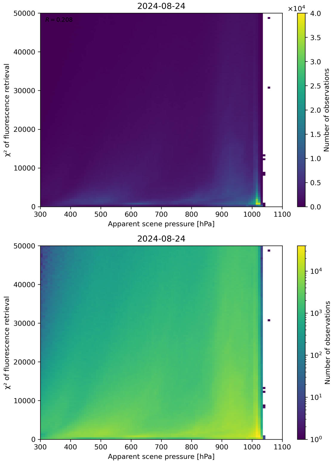
Figure 63: Scatter density plot of “Apparent scene pressure” against “ \chi^2 of fluorescence retrieval” for 2024-08-23 to 2024-08-25.
