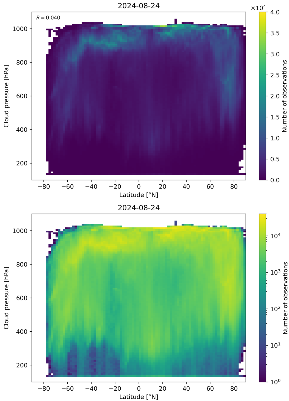
Figure 91: Scatter density plot of “Latitude” against “Cloud pressure” for 2024-08-23 to 2024-08-25.
