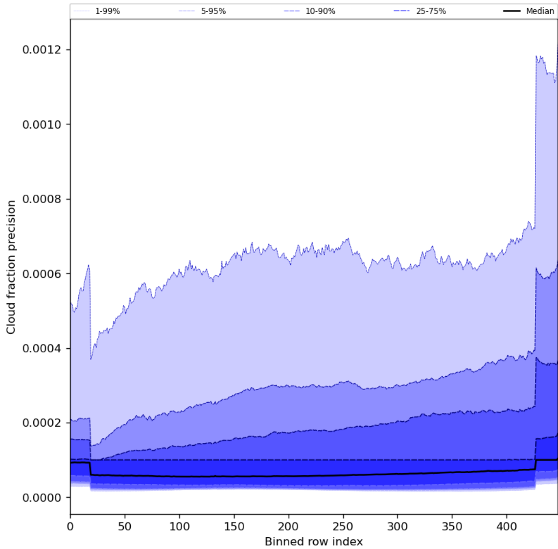
Figure 50: Along track statistics of “Cloud fraction precision” for 2024-08-24 to 2024-08-26
