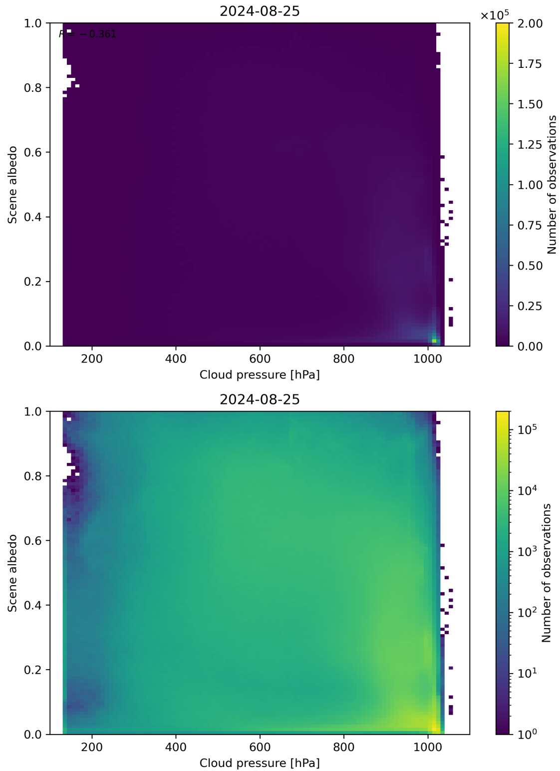
Figure 83: Scatter density plot of “Cloud pressure” against “Scene albedo” for 2024-08-24 to 2024-08-26.
