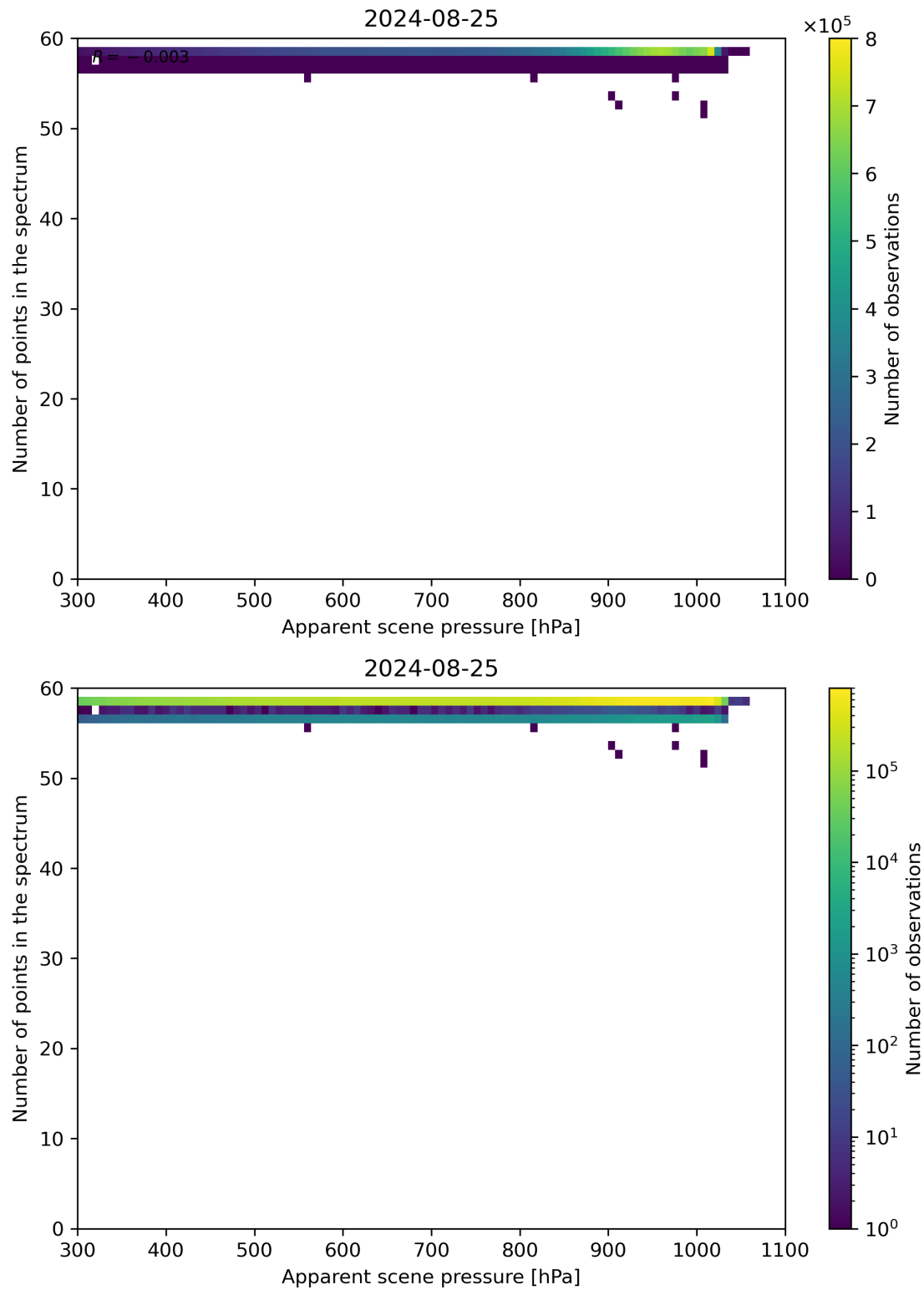
Figure 66: Scatter density plot of “Apparent scene pressure” against “Number of points in the spectrum” for 2024-08-24 to 2024-08-26.
