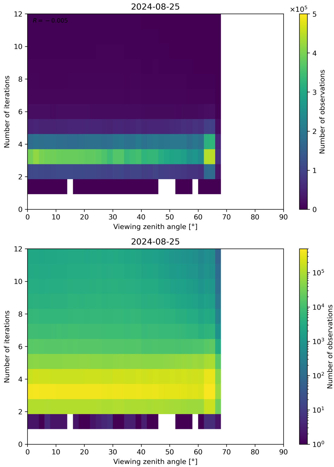
Figure 124: Scatter density plot of “Viewing zenith angle” against “Number of iterations” for 2024-08-24 to 2024-08-26.
