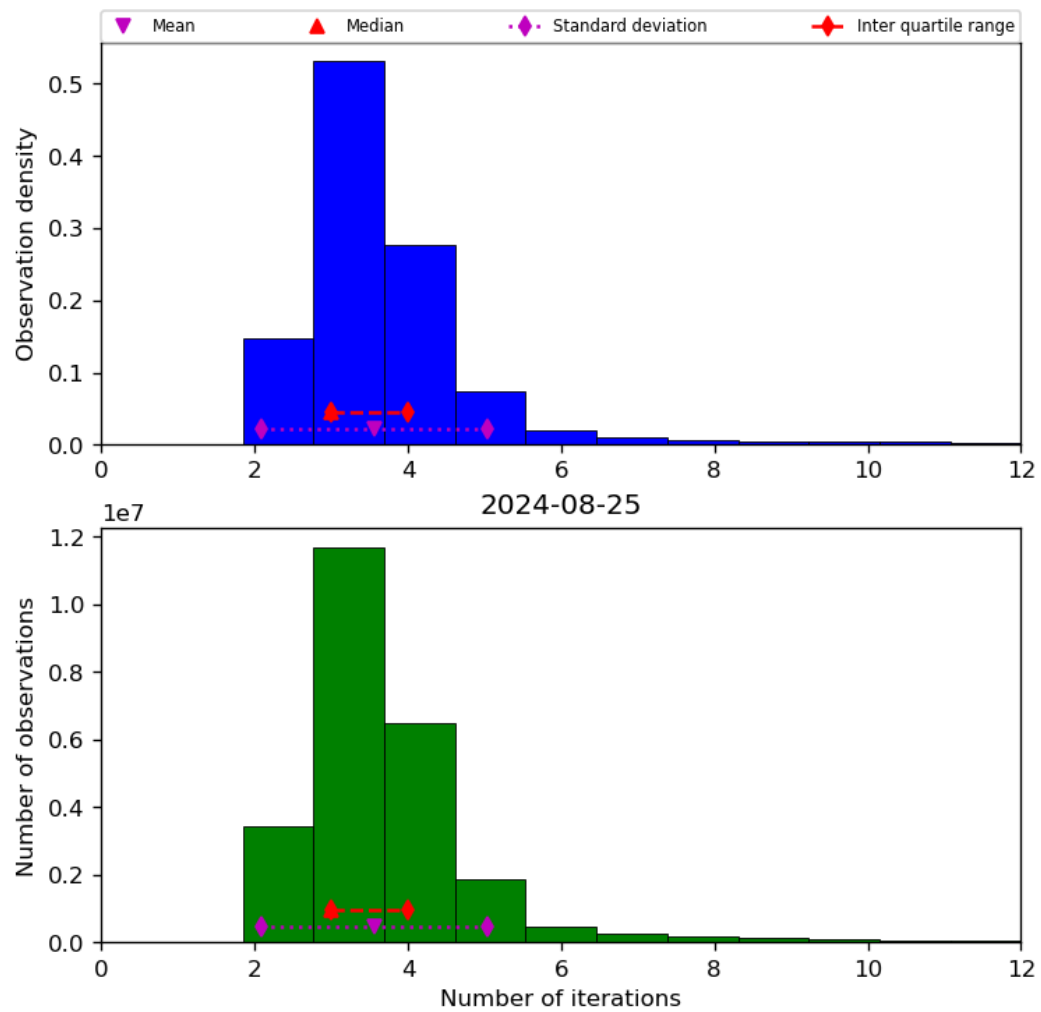
Figure 39: Histogram of “Number of iterations” for 2024-08-24 to 2024-08-26
