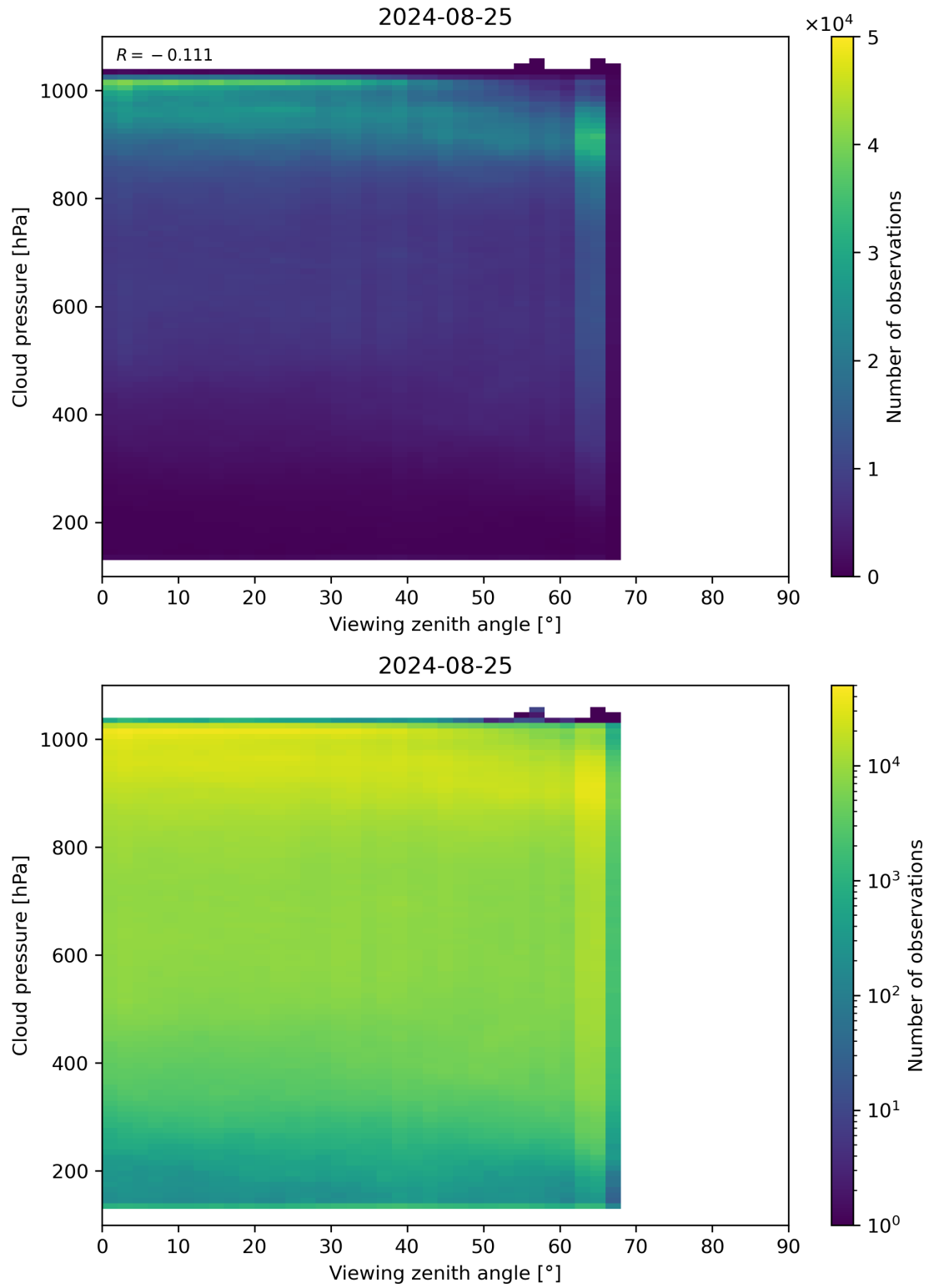
Figure 121: Scatter density plot of “Viewing zenith angle” against “Cloud pressure” for 2024-08-24 to 2024-08-26.
