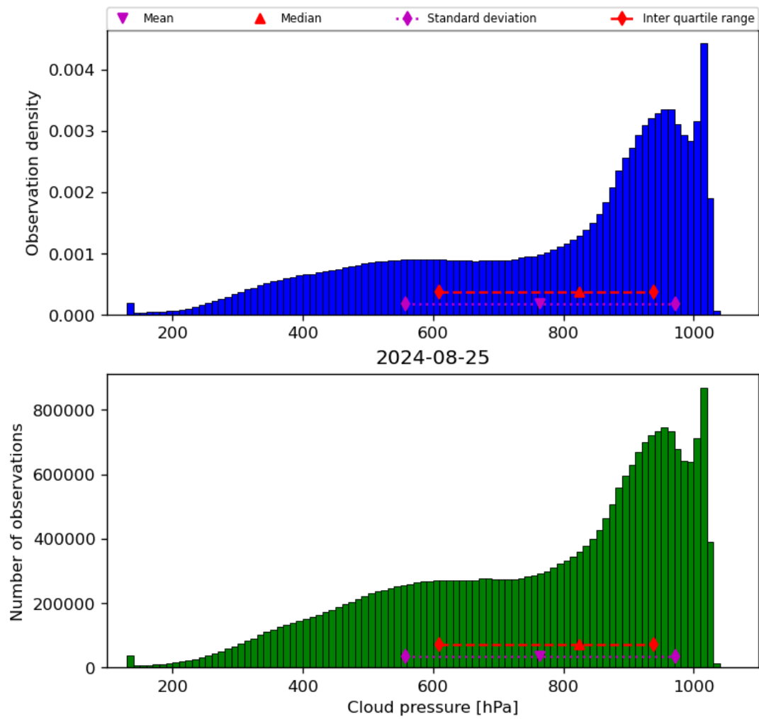
Figure 30: Histogram of “Cloud pressure” for 2024-08-24 to 2024-08-26
