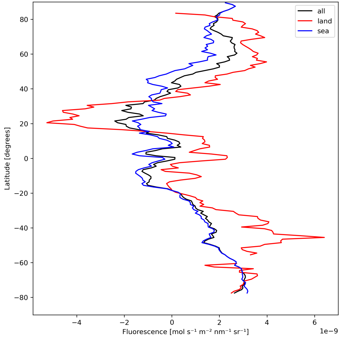
Figure 23: Zonal average of “Fluorescence” for 2024-08-24 to 2024-08-26.
