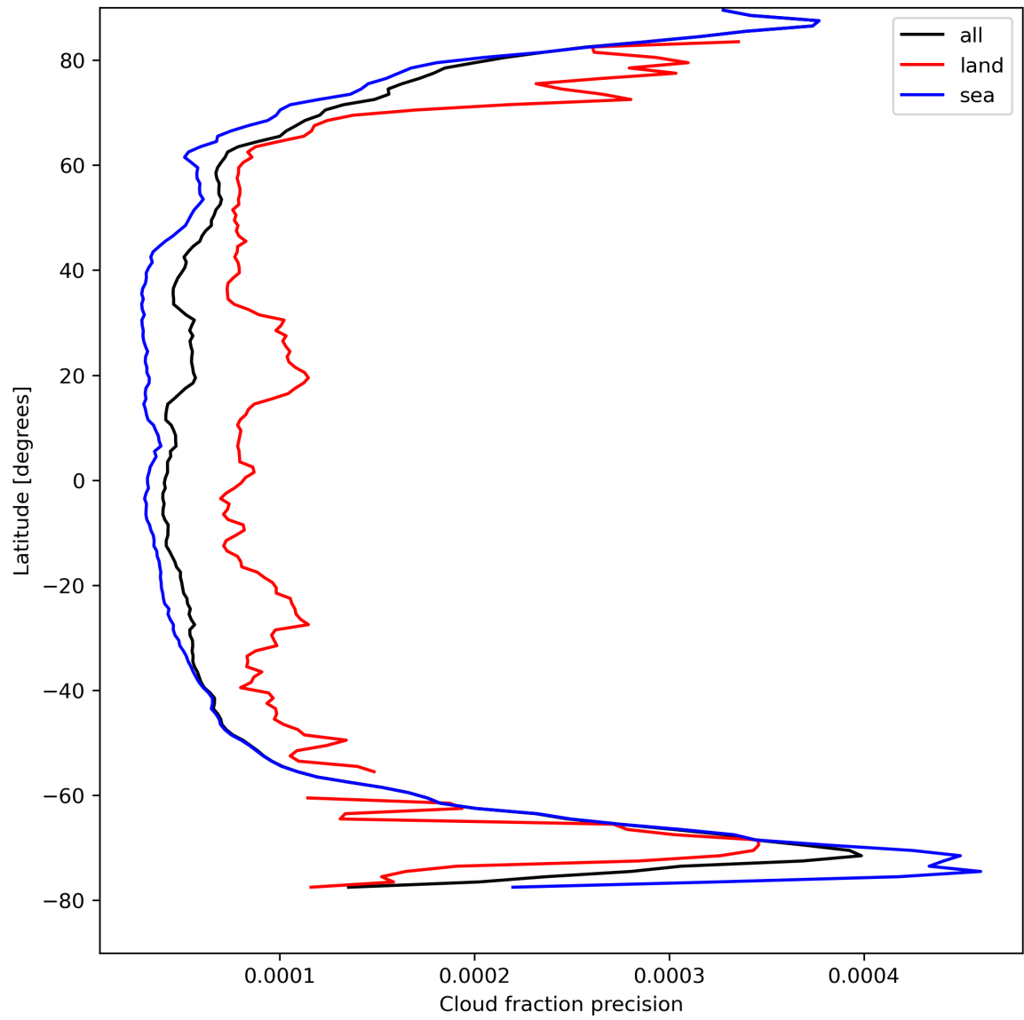
Figure 16: Zonal average of “Cloud fraction precision” for 2024-08-24 to 2024-08-26.
