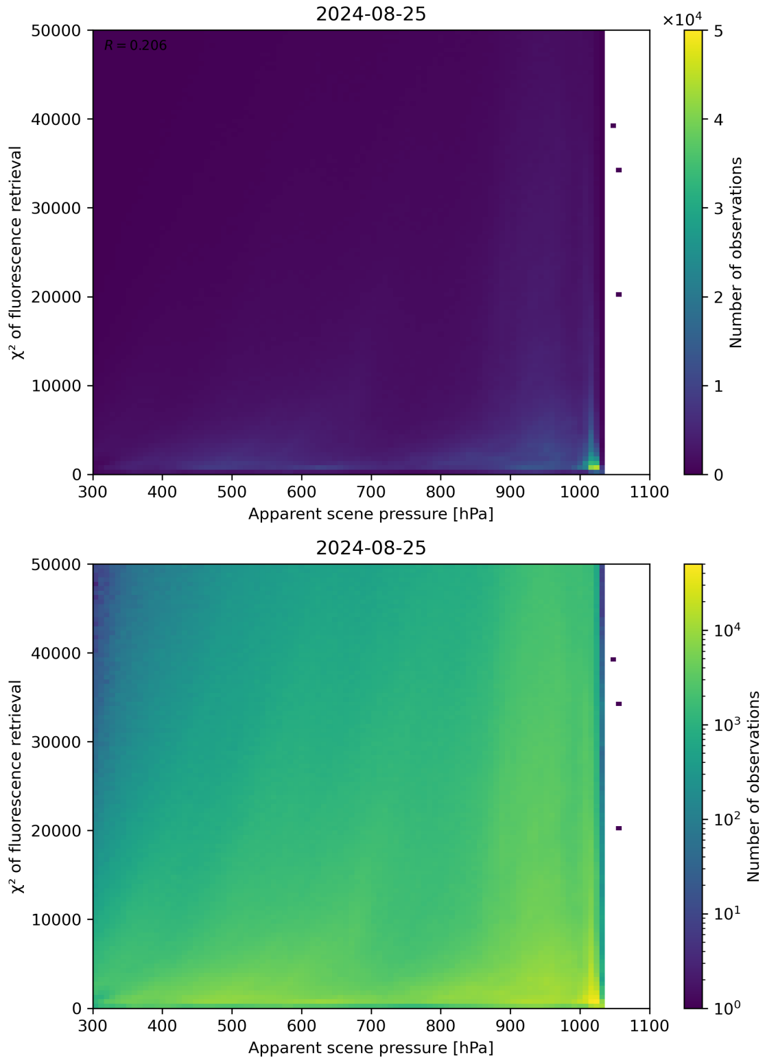
Figure 63: Scatter density plot of “Apparent scene pressure” against “ \chi^2 of fluorescence retrieval” for 2024-08-24 to 2024-08-26.
