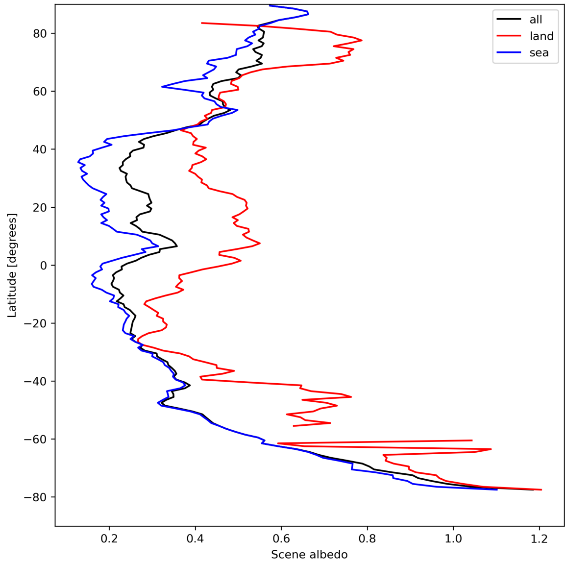
Figure 17: Zonal average of “Scene albedo” for 2024-08-24 to 2024-08-26.
