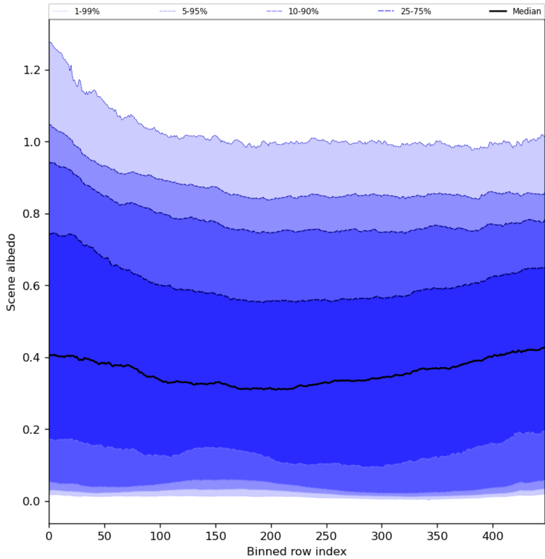
Figure 51: Along track statistics of “Scene albedo” for 2024-08-24 to 2024-08-26
