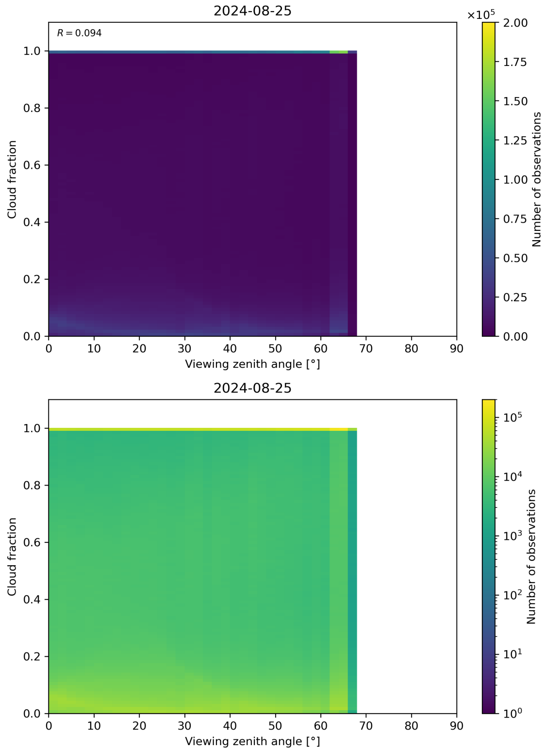
Figure 120: Scatter density plot of “Viewing zenith angle” against “Cloud fraction” for 2024-08-24 to 2024-08-26.
