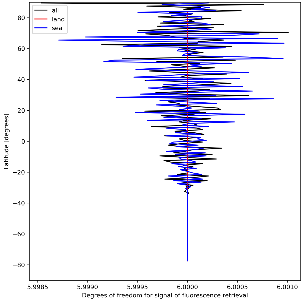
Figure 26: Zonal average of “Degrees of freedom for signal of fluorescence retrieval” for 2024-08-24 to 2024-08-26.
