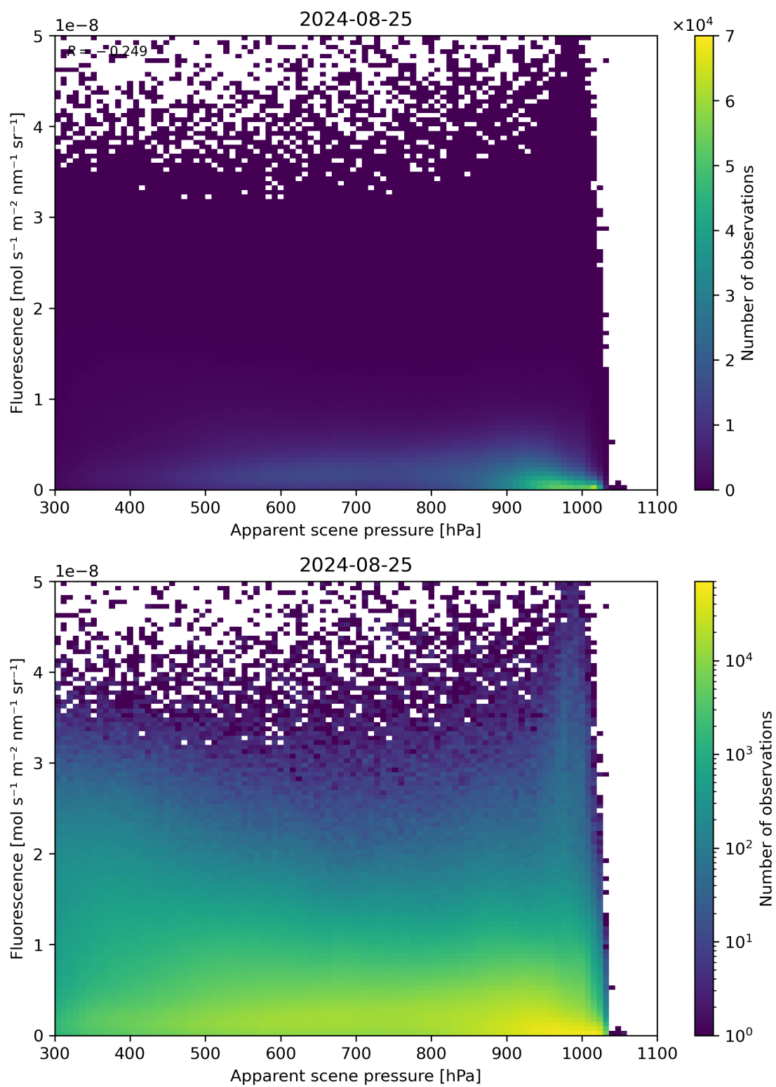
Figure 64: Scatter density plot of “Apparent scene pressure” against “Fluorescence” for 2024-08-24 to 2024-08-26.
