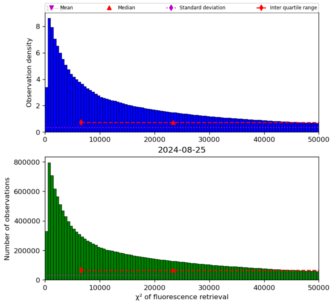
Figure 42: Histogram of “ \chi^2 of fluorescence retrieval” for 2024-08-24 to 2024-08-26
