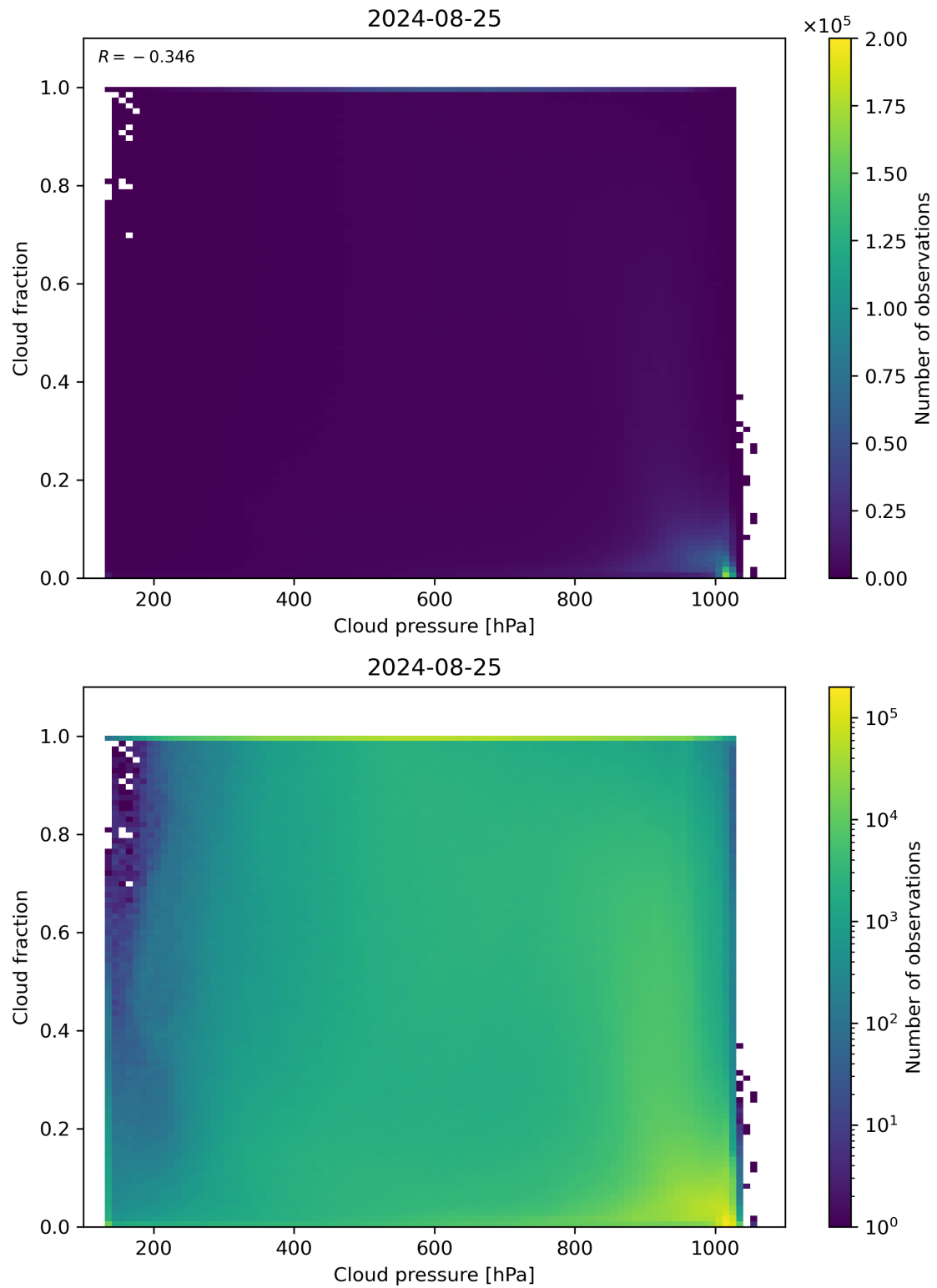
Figure 79: Scatter density plot of “Cloud pressure” against “Cloud fraction” for 2024-08-24 to 2024-08-26.
