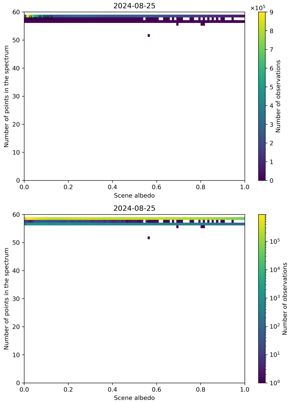
Figure 106: Scatter density plot of “Scene albedo” against “Number of points in the spectrum” for 2024-08-24 to 2024-08-26.
