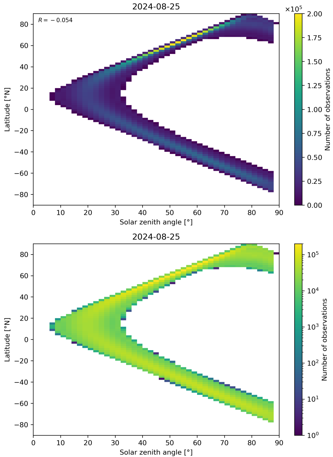
Figure 113: Scatter density plot of “Solar zenith angle” against “Latitude” for 2024-08-24 to 2024-08-26.
