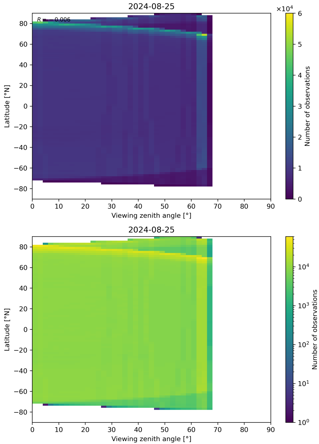
Figure 123: Scatter density plot of “Viewing zenith angle” against “Latitude” for 2024-08-24 to 2024-08-26.
