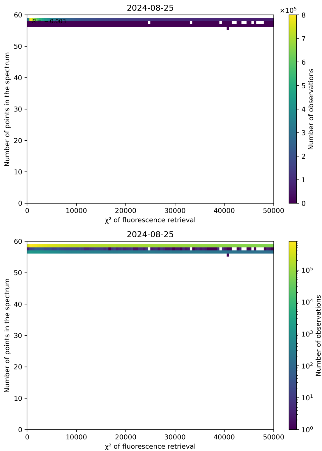
Figure 68: Scatter density plot of " \chi^2 of fluorescence retrieval" against "Number of points in the spectrum" for 2024-08-24 to 2024-08-26.
