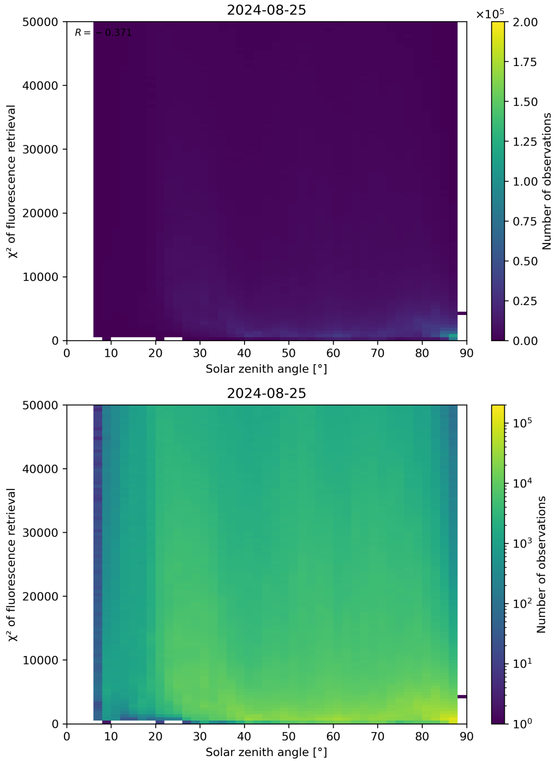
Figure 109: Scatter density plot of “Solar zenith angle” against “ \chi^2 of fluorescence retrieval” for 2024-08-24 to 2024-08-26.
