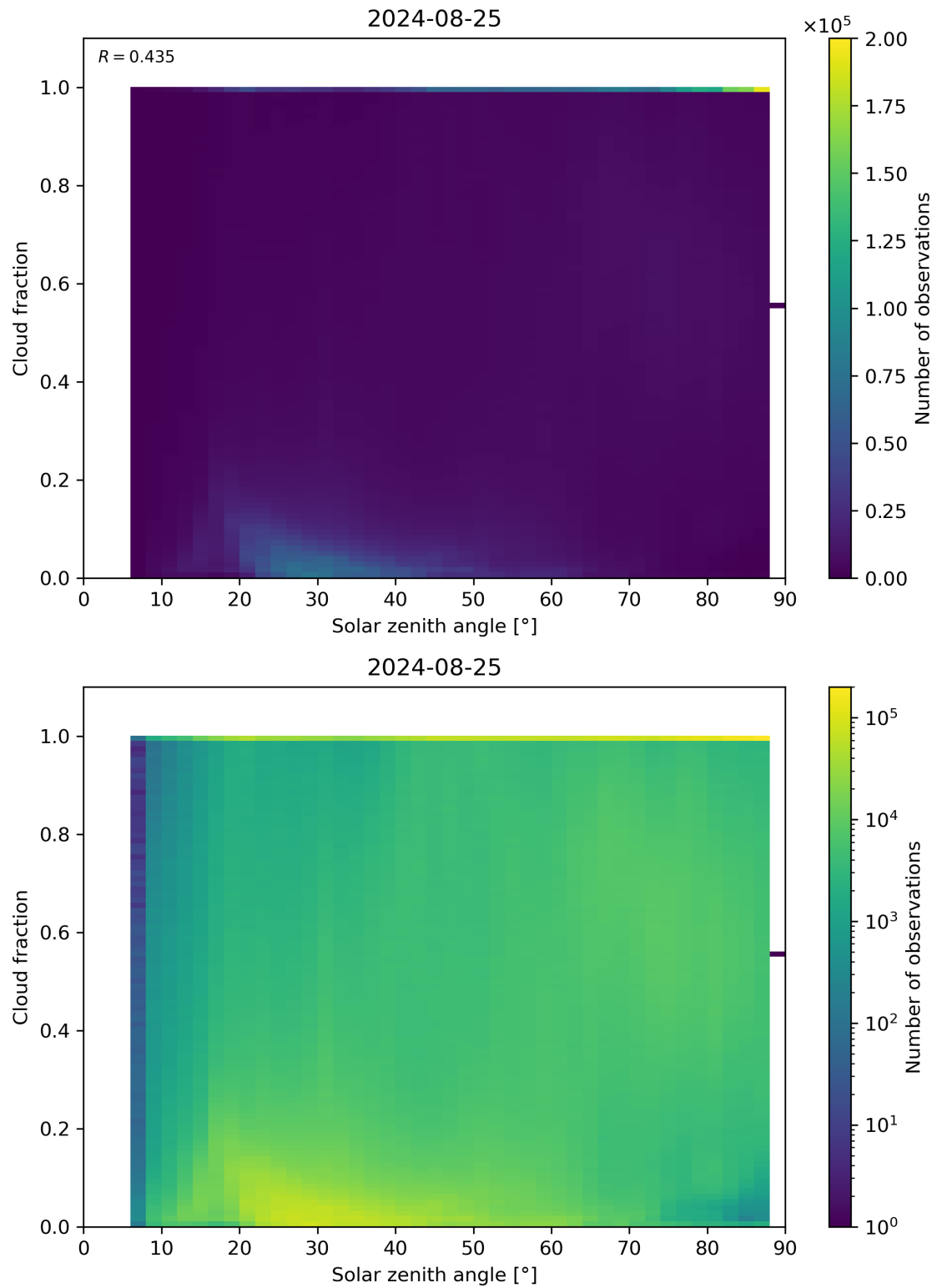
Figure 110: Scatter density plot of “Solar zenith angle” against “Cloud fraction” for 2024-08-24 to 2024-08-26.
