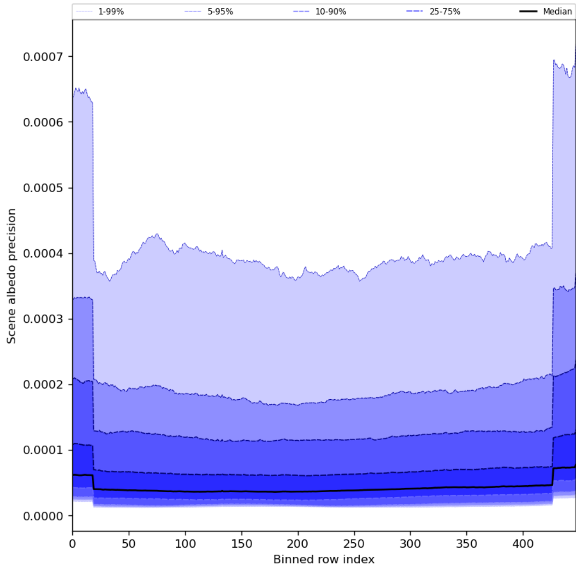
Figure 52: Along track statistics of “Scene albedo precision” for 2024-08-24 to 2024-08-26
