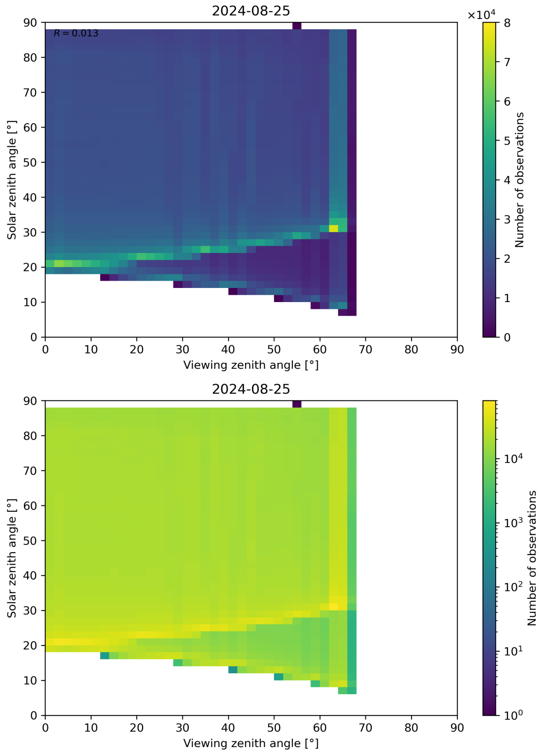
Figure 127: Scatter density plot of “Viewing zenith angle” against “Solar zenith angle” for 2024-08-24 to 2024-08-26.
