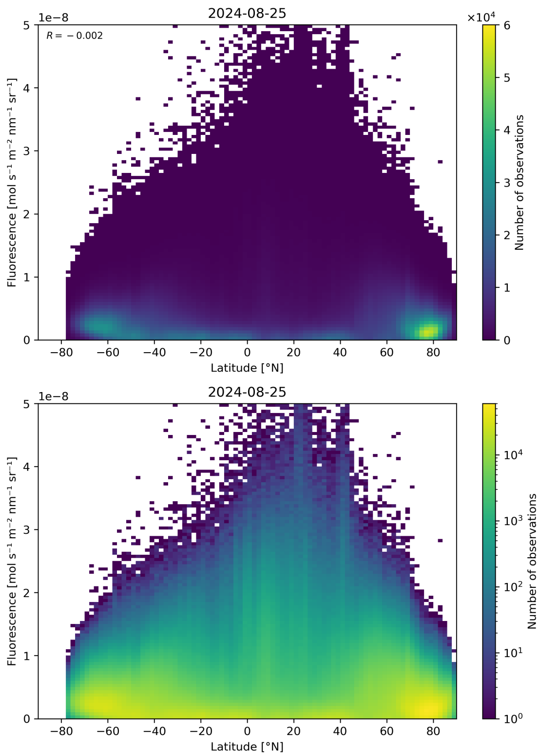
Figure 92: Scatter density plot of “Latitude” against “Fluorescence” for 2024-08-24 to 2024-08-26.
