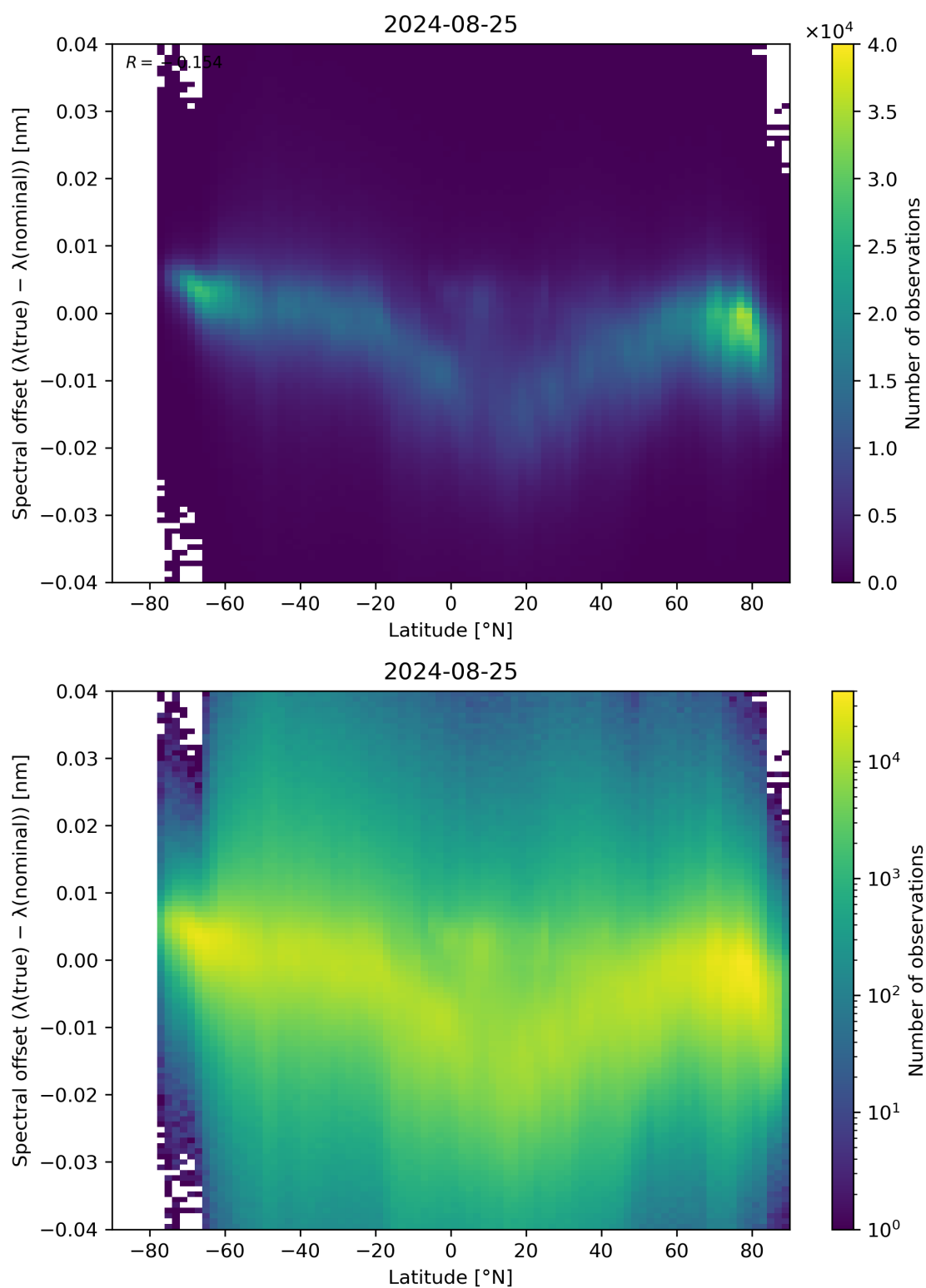
Figure 96: Scatter density plot of “Latitude” against “Spectral offset ( \lambda(\text{true}) - \lambda(\text{nominal}) )” for 2024-08-24 to 2024-08-26.
