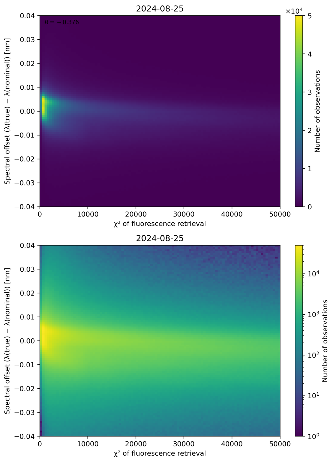
Figure 69: Scatter density plot of “ \chi^2 of fluorescence retrieval” against “Spectral offset ( \lambda(\text{true}) - \lambda(\text{nominal}) )” for 2024-08-24 to 2024-08-26.
