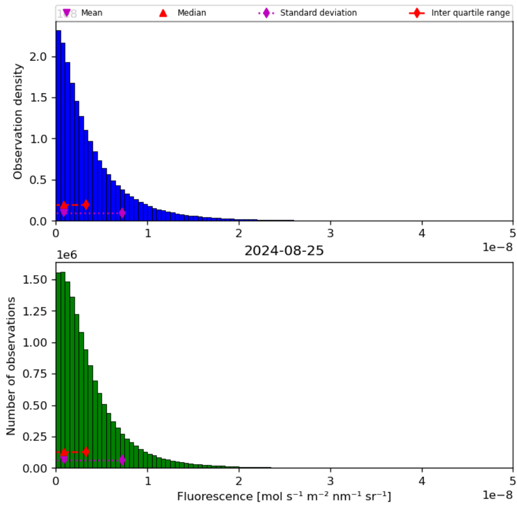
Figure 40: Histogram of “Fluorescence” for 2024-08-24 to 2024-08-26
