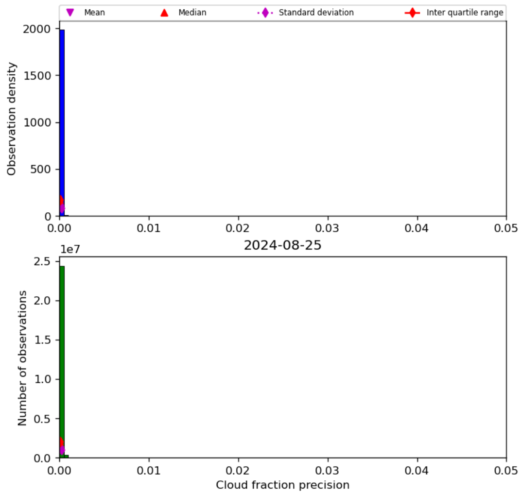
Figure 33: Histogram of “Cloud fraction precision” for 2024-08-24 to 2024-08-26
