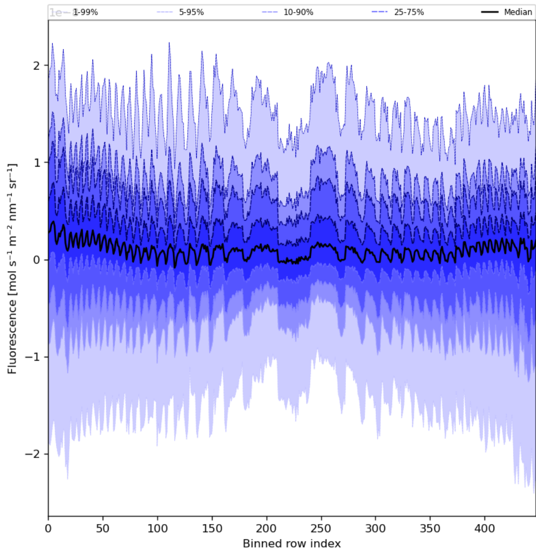
Figure 57: Along track statistics of “Fluorescence” for 2024-08-24 to 2024-08-26
