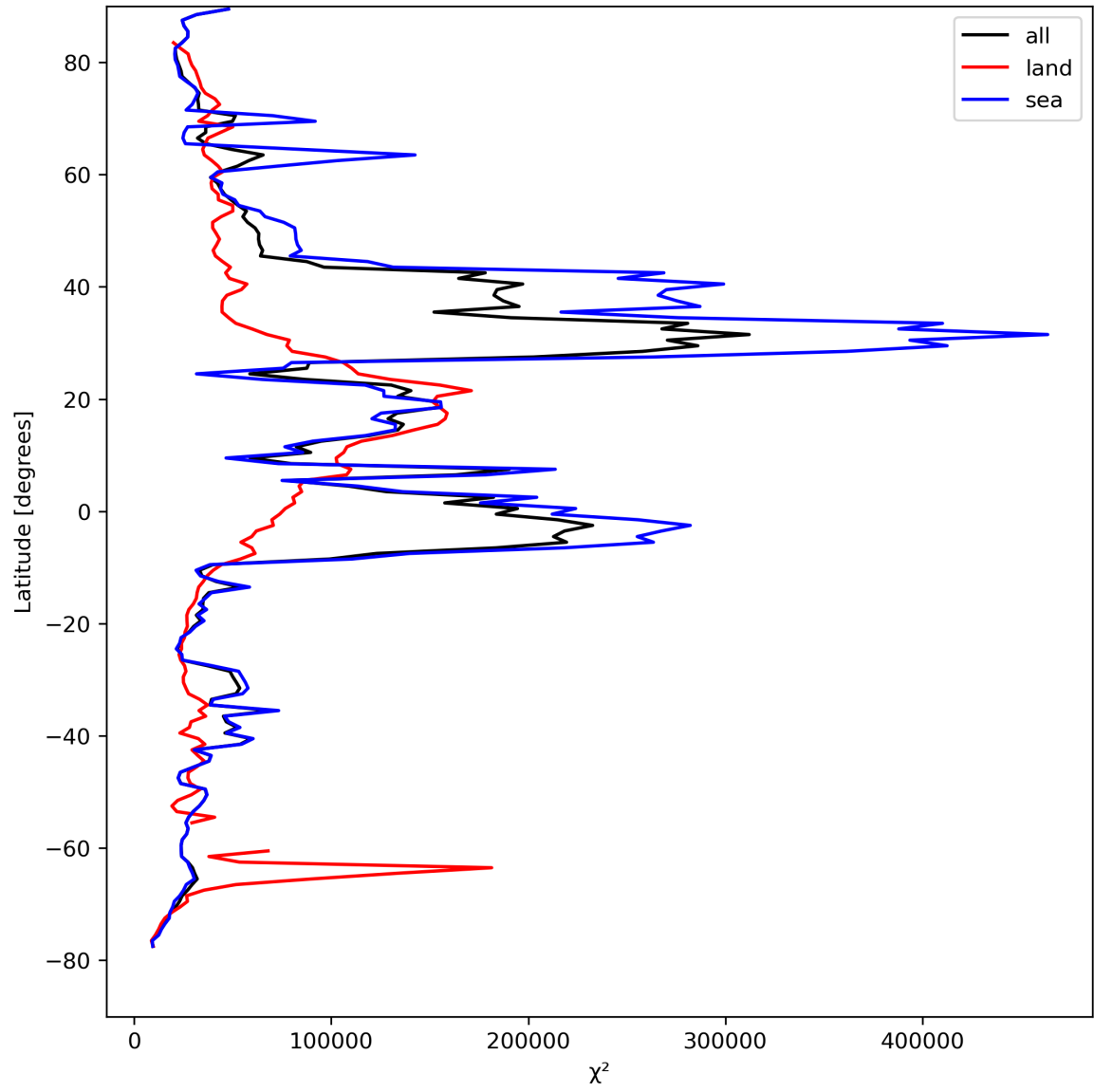
Figure 21: Zonal average of “ \chi^2 ” for 2024-08-24 to 2024-08-26.
