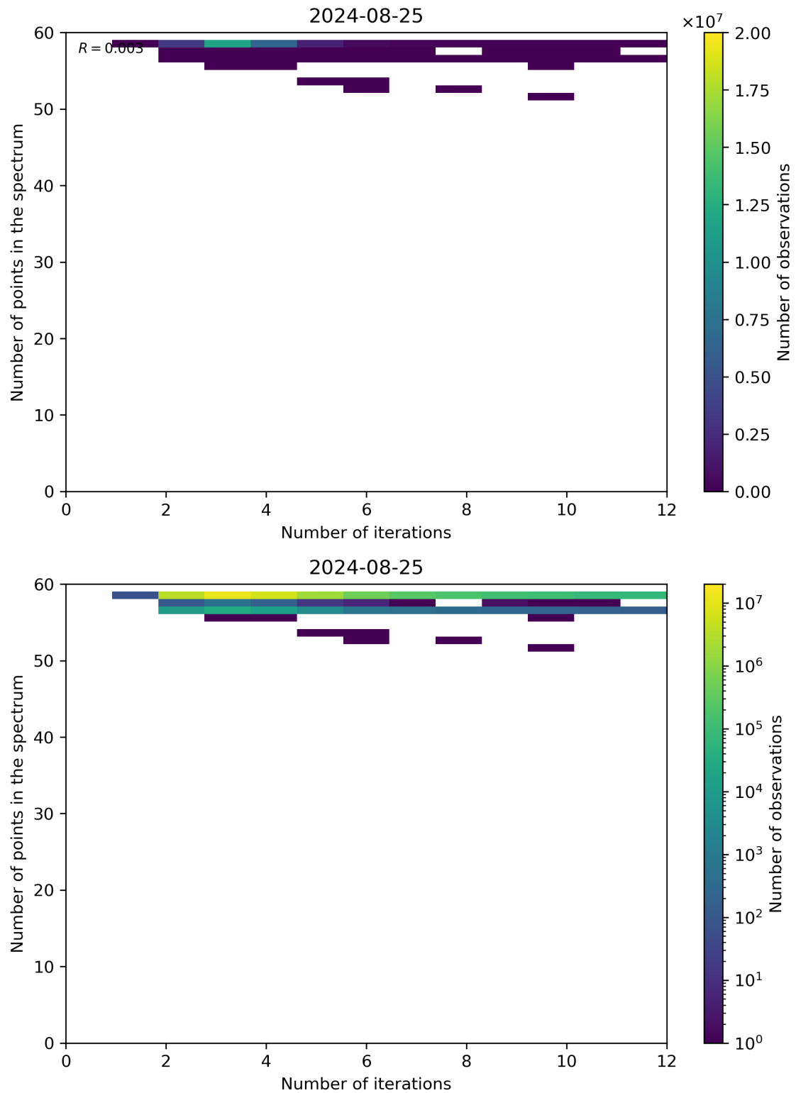
Figure 99: Scatter density plot of “Number of iterations” against “Number of points in the spectrum” for 2024-08-24 to 2024-08-26.
