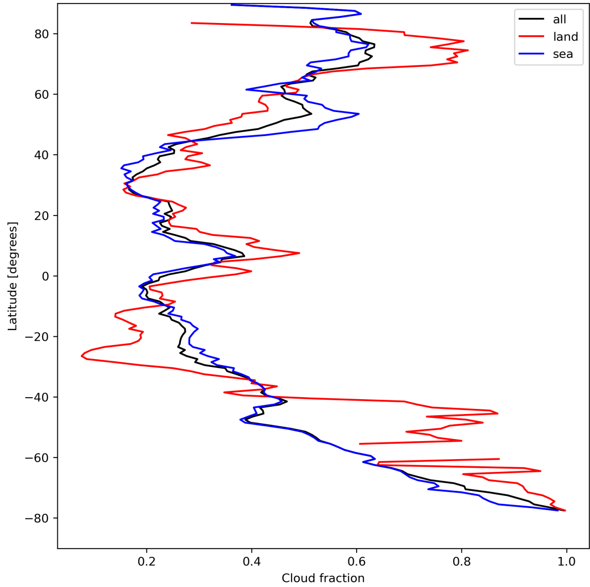
Figure 15: Zonal average of “Cloud fraction” for 2024-08-24 to 2024-08-26.
