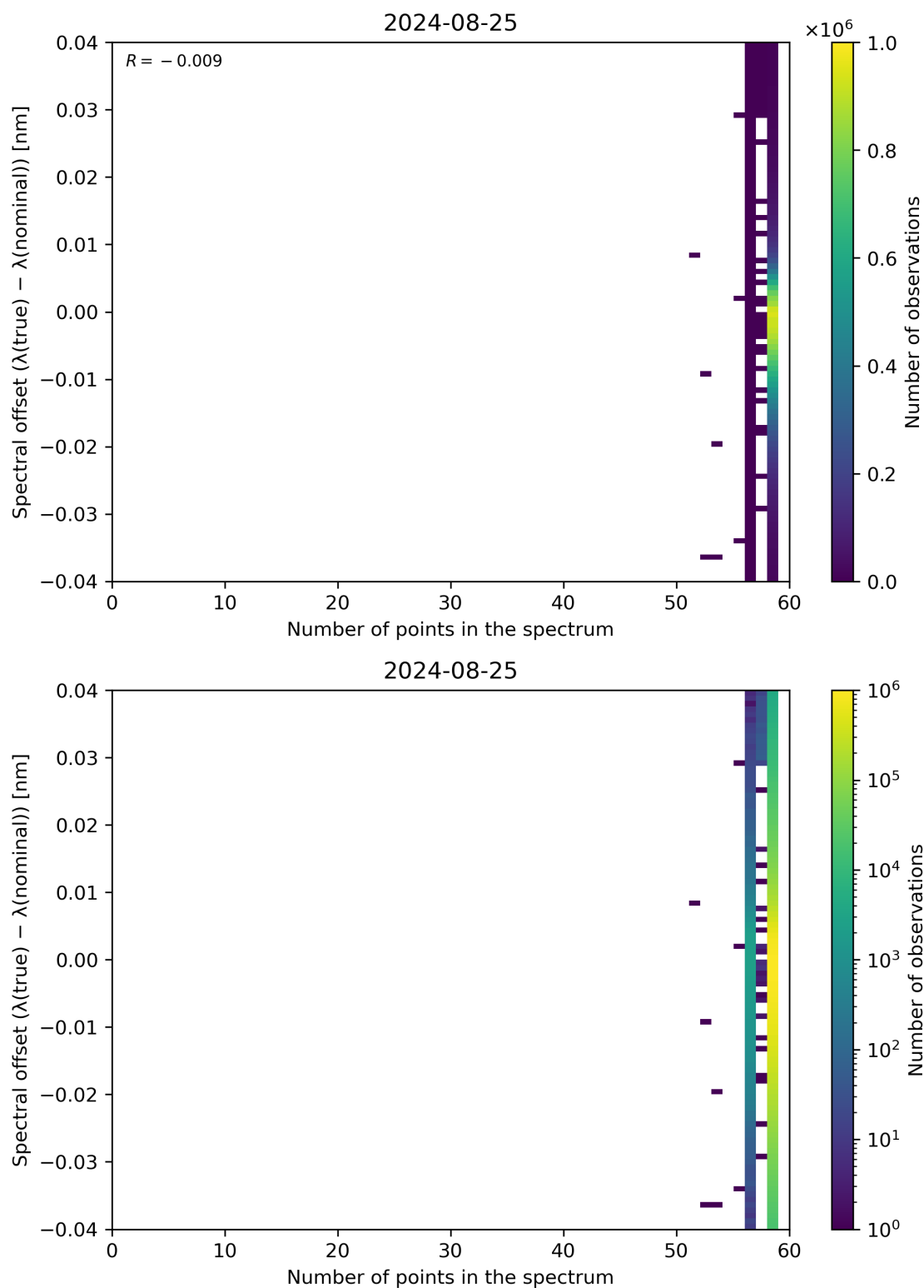
Figure 101: Scatter density plot of “Number of points in the spectrum” against “Spectral offset ( \lambda(\text{true}) - \lambda(\text{nominal}) )” for 2024-08-24 to 2024-08-26.
