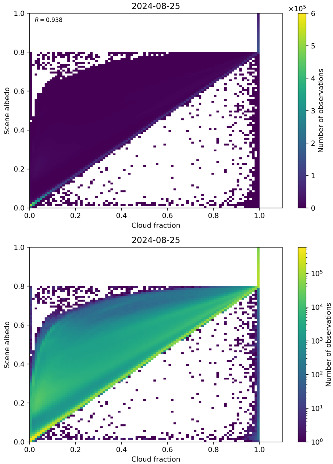
Figure 75: Scatter density plot of “Cloud fraction” against “Scene albedo” for 2024-08-24 to 2024-08-26.
