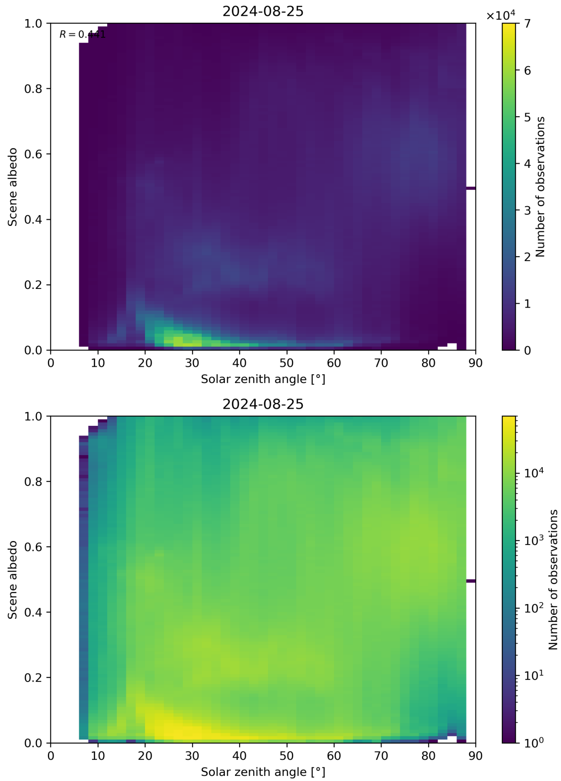
Figure 116: Scatter density plot of “Solar zenith angle” against “Scene albedo” for 2024-08-24 to 2024-08-26.
