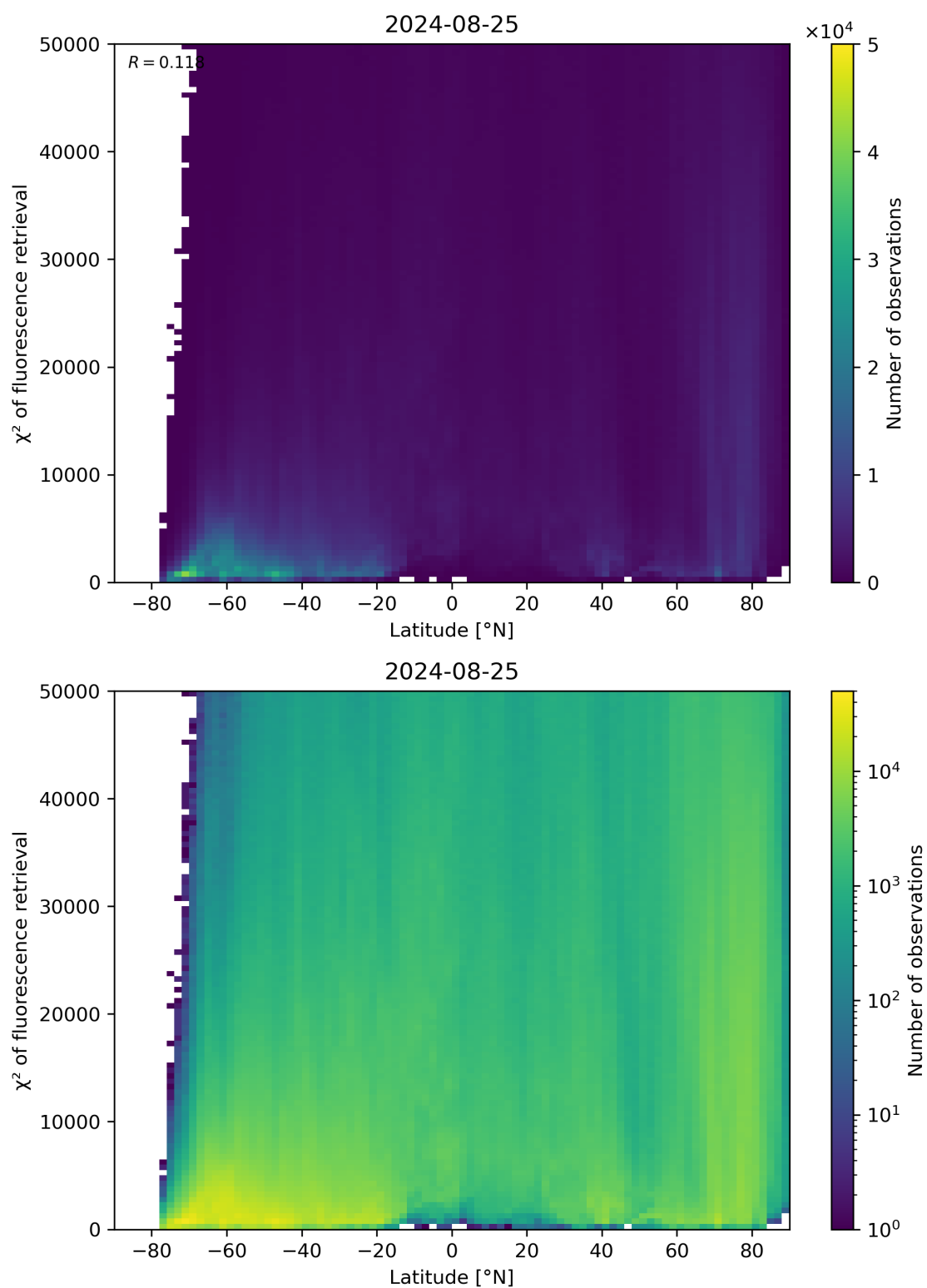
Figure 89: Scatter density plot of “Latitude” against “ \chi^2 of fluorescence retrieval” for 2024-08-24 to 2024-08-26.
