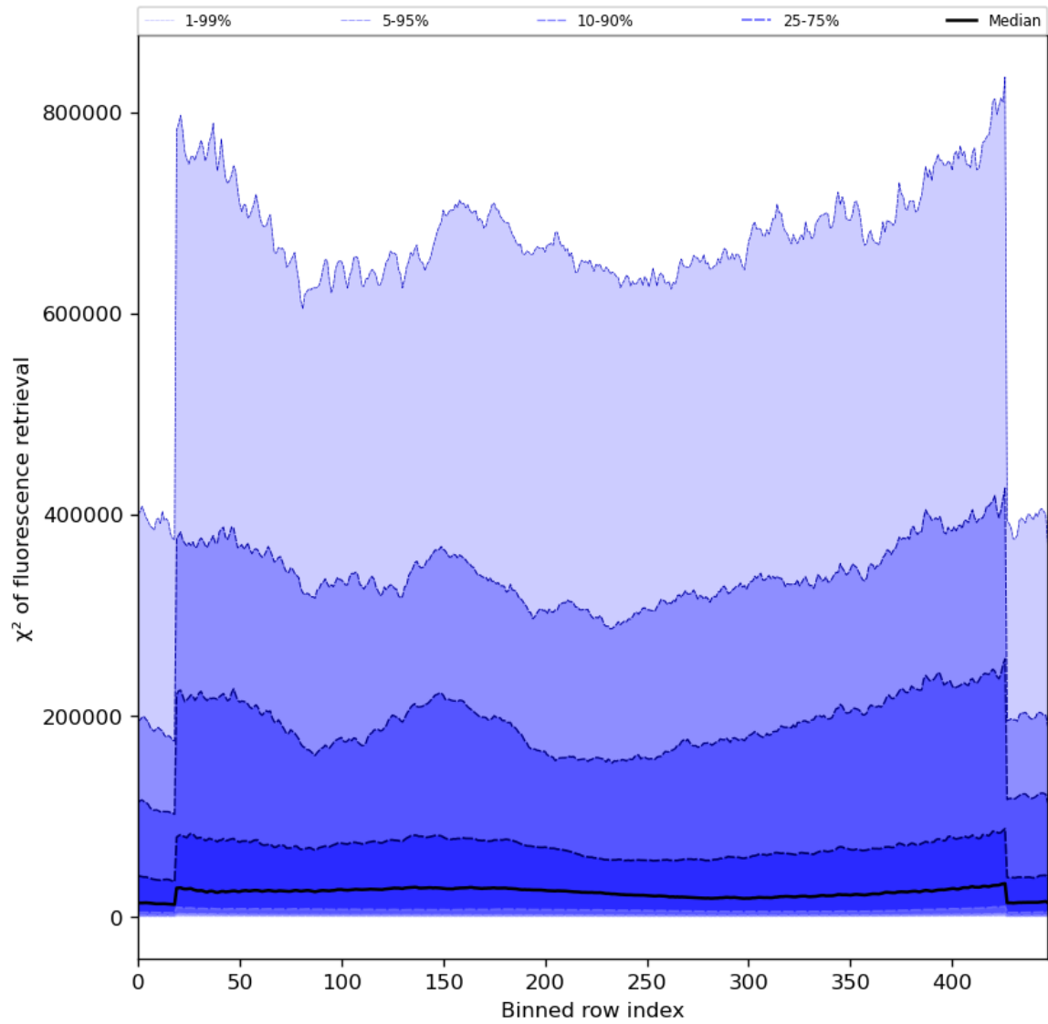
Figure 59: Along track statistics of “ \chi^2 of fluorescence retrieval” for 2024-08-24 to 2024-08-26
