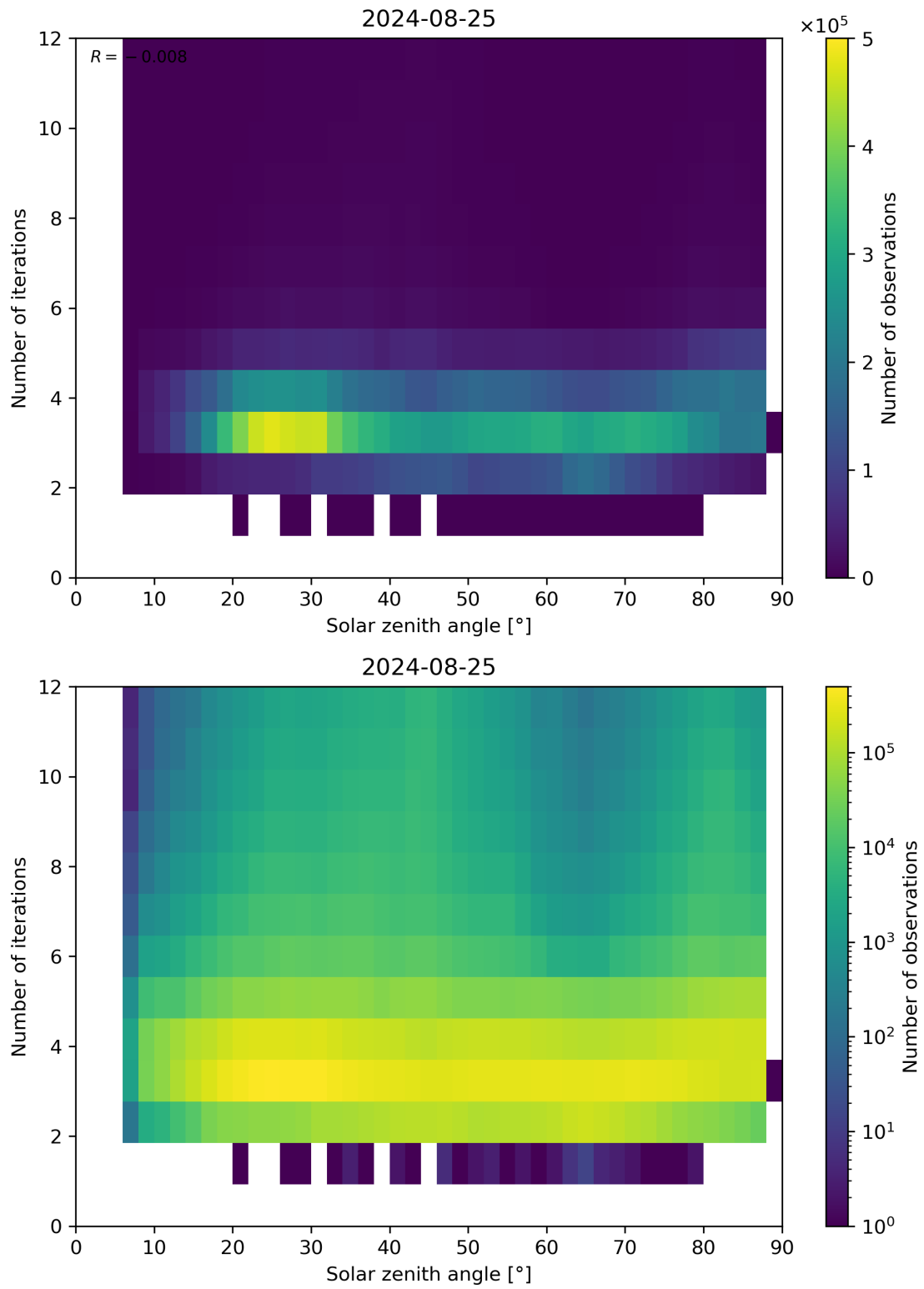
Figure 114: Scatter density plot of “Solar zenith angle” against “Number of iterations” for 2024-08-24 to 2024-08-26.
