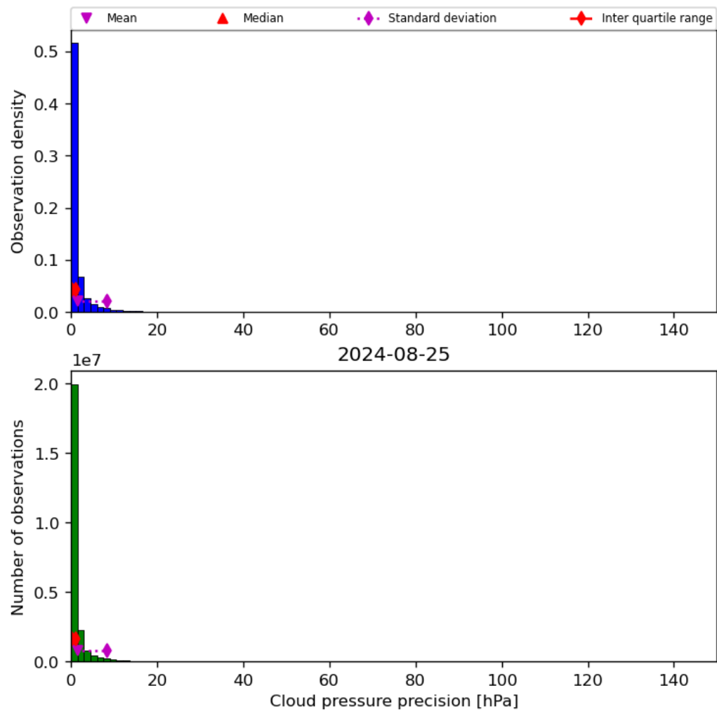
Figure 31: Histogram of “Cloud pressure precision” for 2024-08-24 to 2024-08-26
