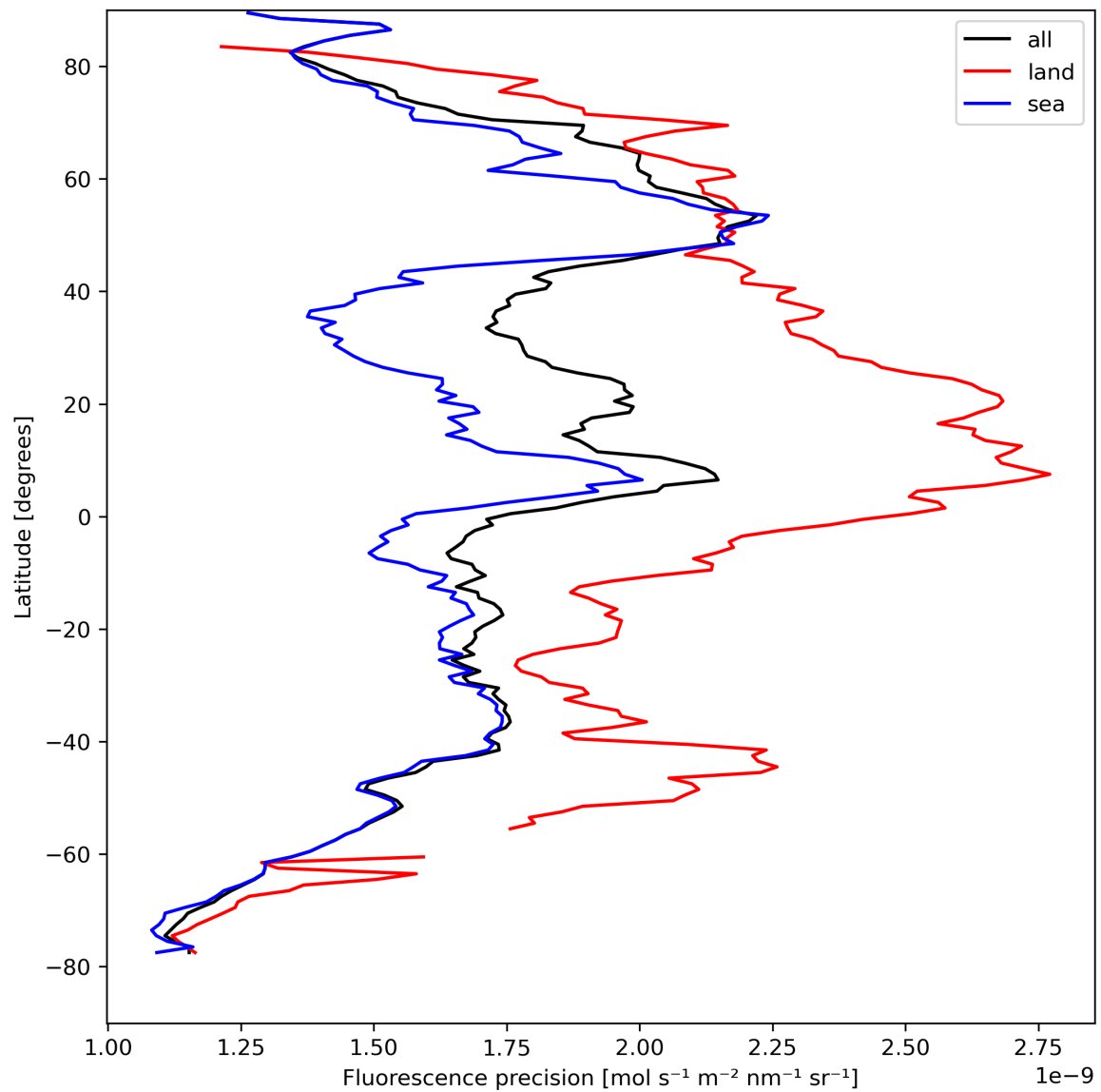
Figure 24: Zonal average of “Fluorescence precision” for 2024-08-24 to 2024-08-26.
