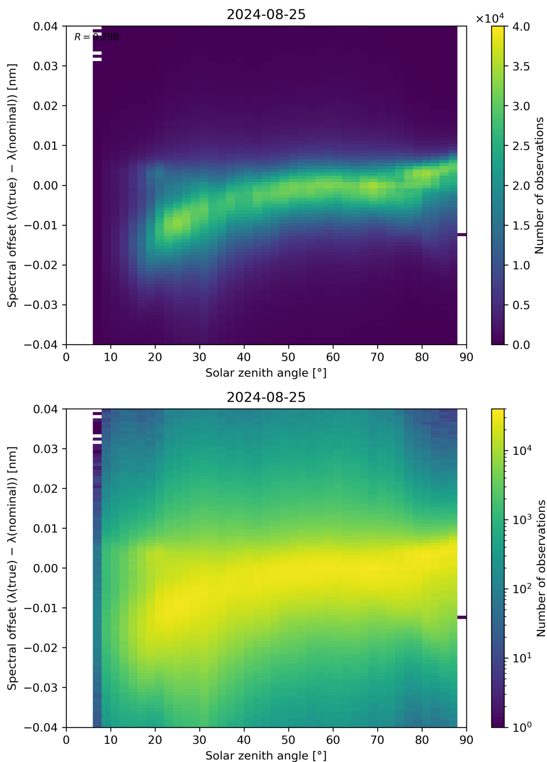
Figure 117: Scatter density plot of “Solar zenith angle” against “Spectral offset ( \lambda(\text{true}) - \lambda(\text{nominal}) )” for 2024-08-24 to 2024-08-26.
