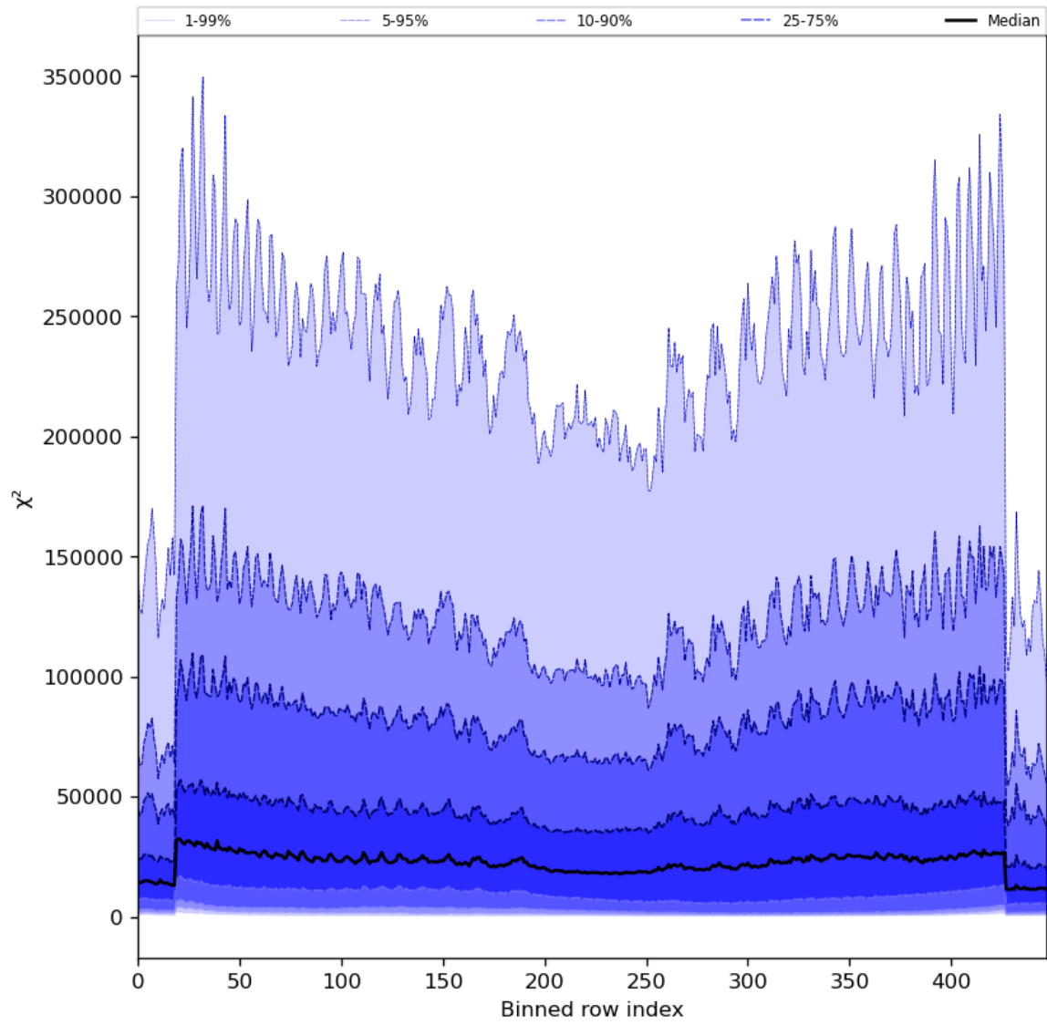
Figure 55: Along track statistics of “ \chi^2 ” for 2024-08-24 to 2024-08-26
