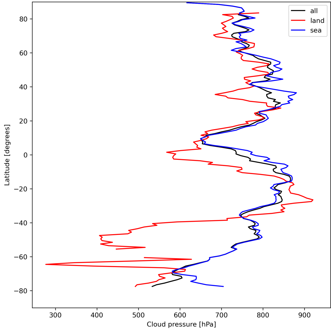
Figure 13: Zonal average of “Cloud pressure” for 2024-08-24 to 2024-08-26.
