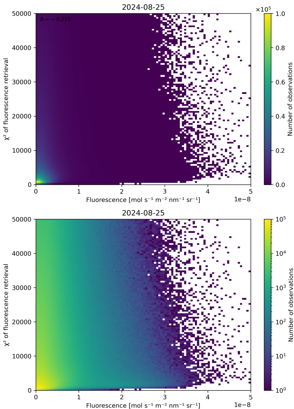
Figure 85: Scatter density plot of “Fluorescence” against “ \chi^2 of fluorescence retrieval” for 2024-08-24 to 2024-08-26.
