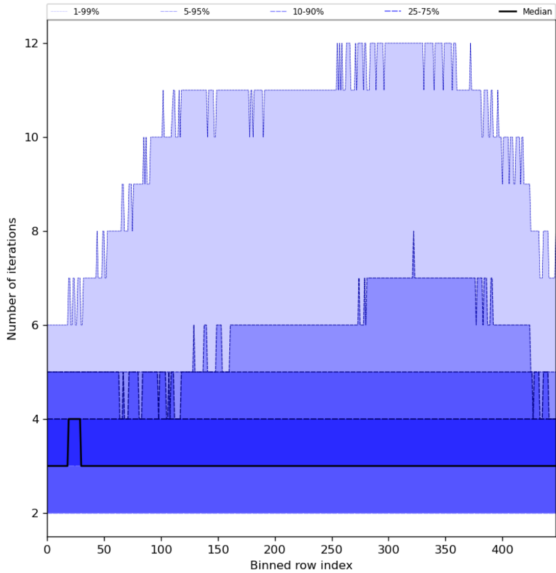
Figure 56: Along track statistics of “Number of iterations” for 2024-08-24 to 2024-08-26
