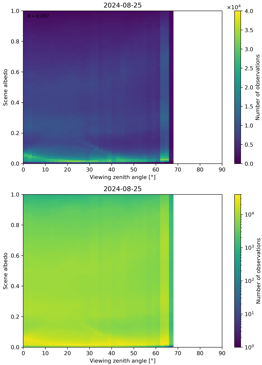
Figure 126: Scatter density plot of “Viewing zenith angle” against “Scene albedo” for 2024-08-24 to 2024-08-26.
