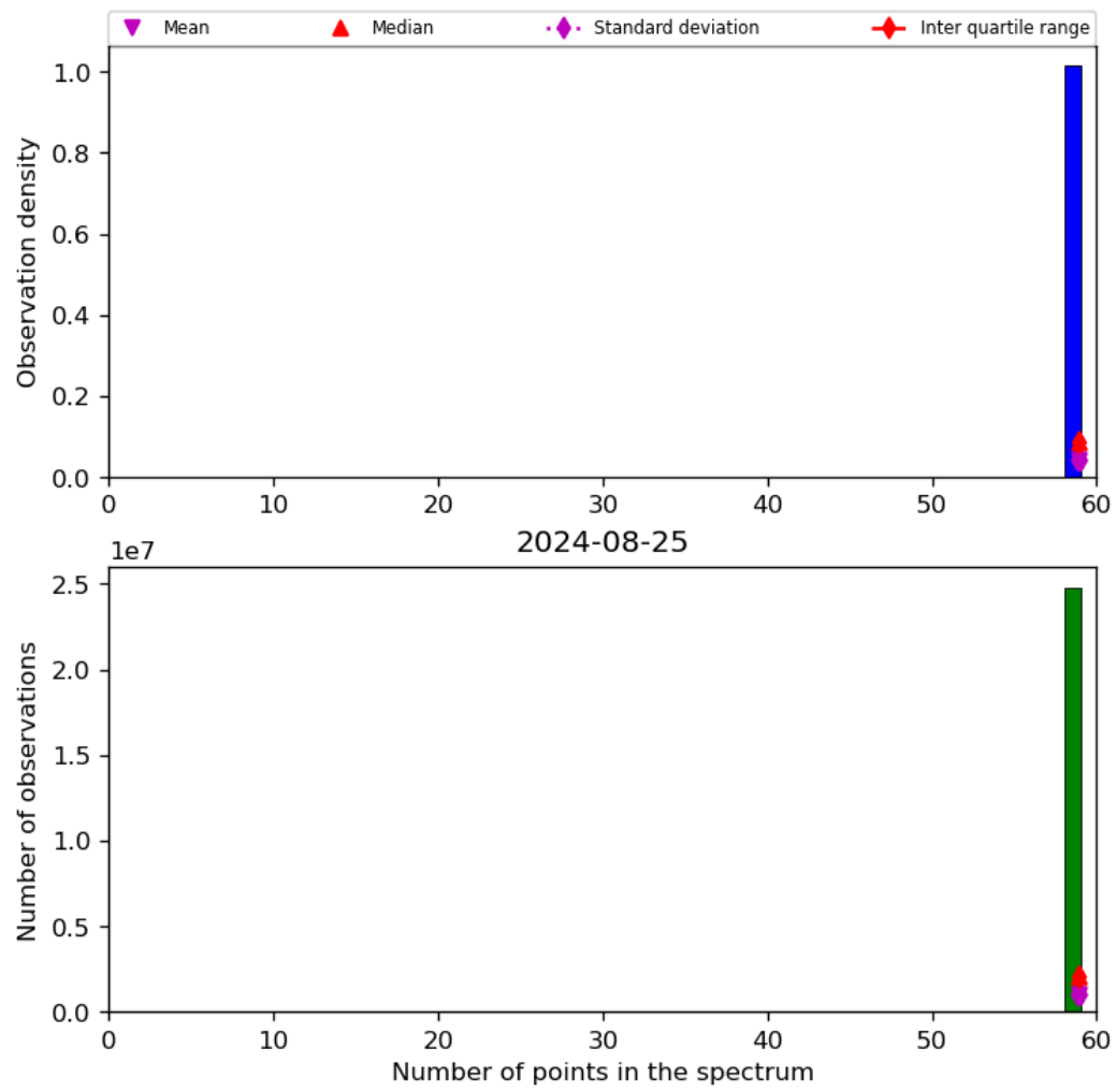
Figure 44: Histogram of “Number of points in the spectrum” for 2024-08-24 to 2024-08-26
