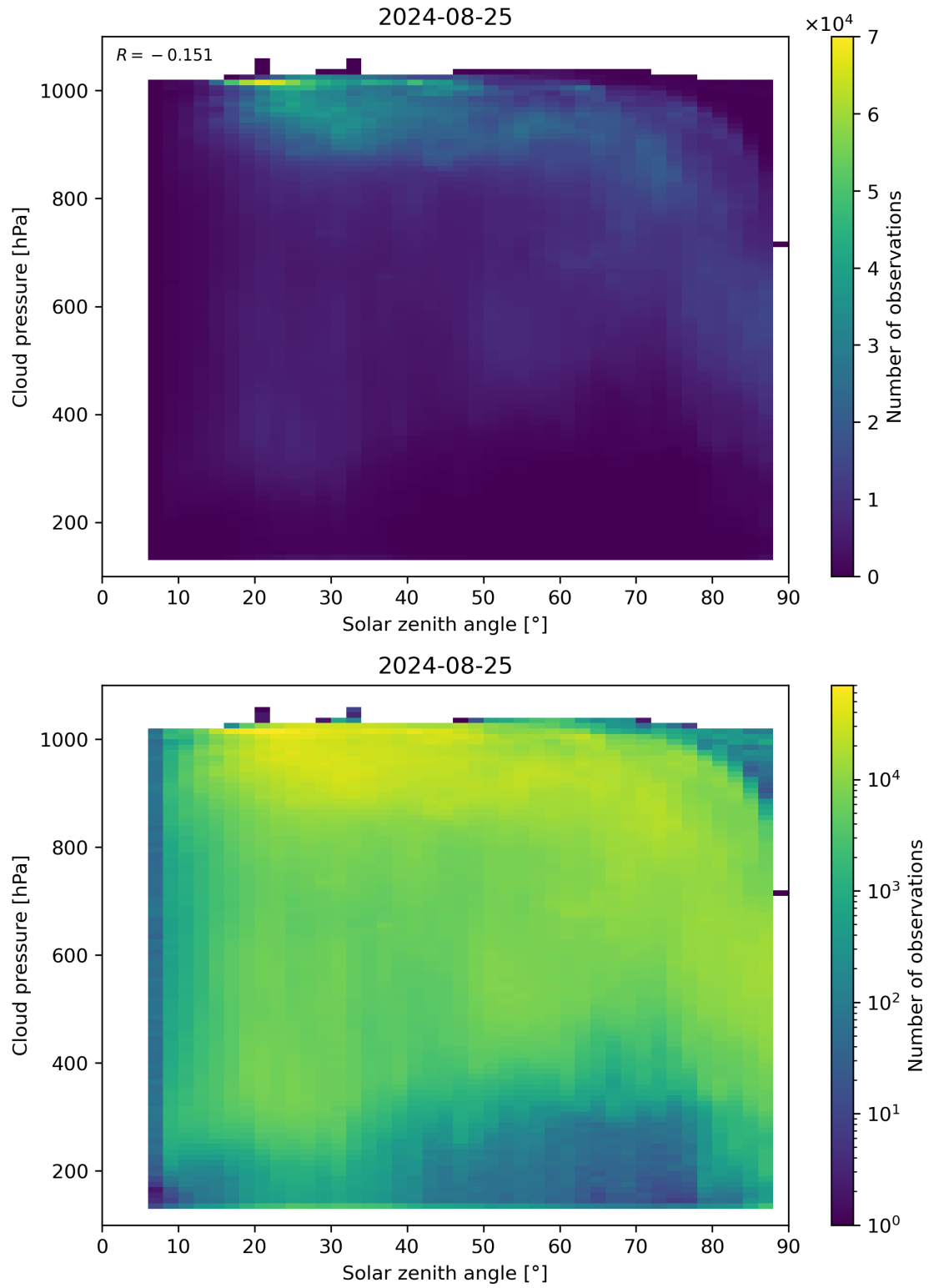
Figure 111: Scatter density plot of “Solar zenith angle” against “Cloud pressure” for 2024-08-24 to 2024-08-26.
