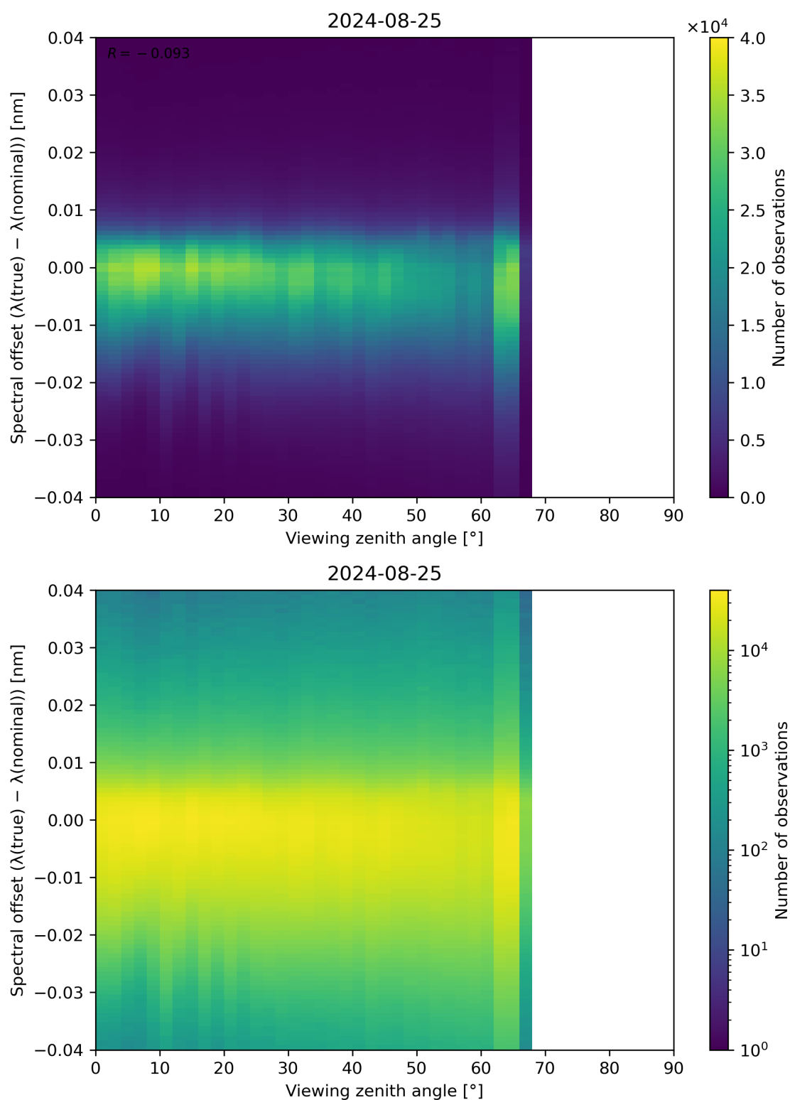
Figure 128: Scatter density plot of “Viewing zenith angle” against “Spectral offset ( \lambda(\text{true}) - \lambda(\text{nominal}) )” for 2024-08-24 to 2024-08-26.
