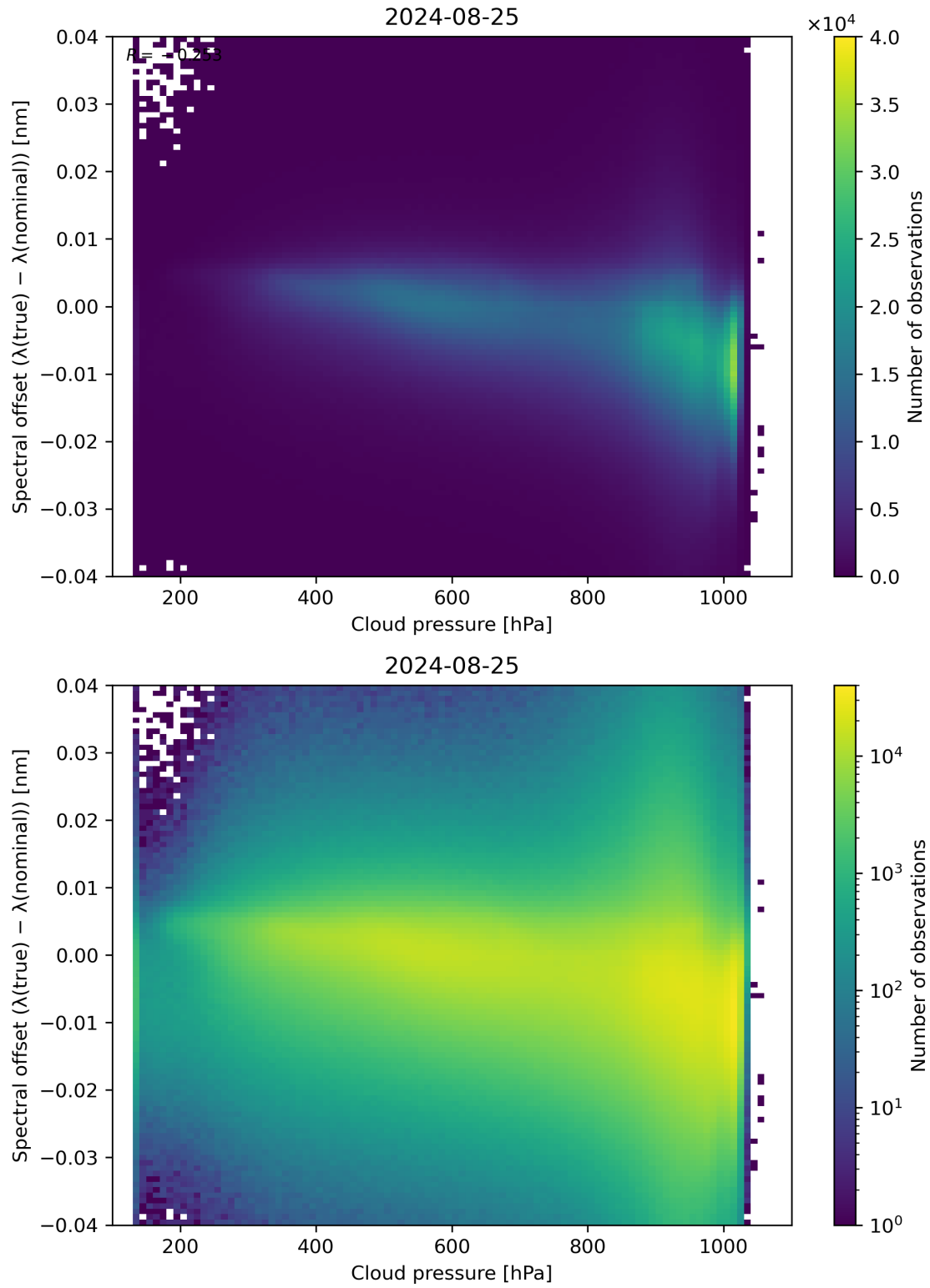
Figure 84: Scatter density plot of “Cloud pressure” against “Spectral offset ( \lambda(\text{true}) - \lambda(\text{nominal}) )” for 2024-08-24 to 2024-08-26.
