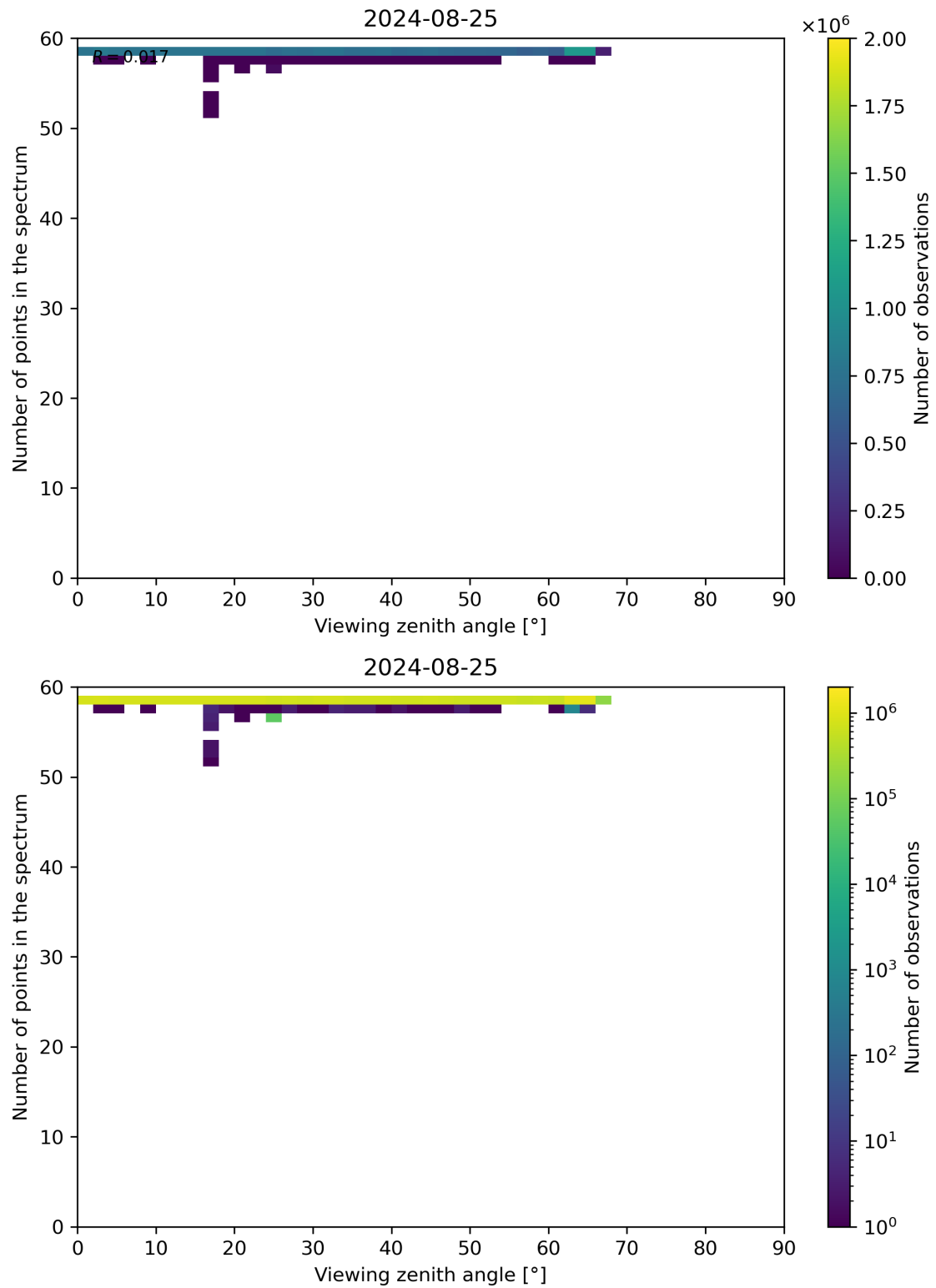
Figure 125: Scatter density plot of “Viewing zenith angle” against “Number of points in the spectrum” for 2024-08-24 to 2024-08-26.
