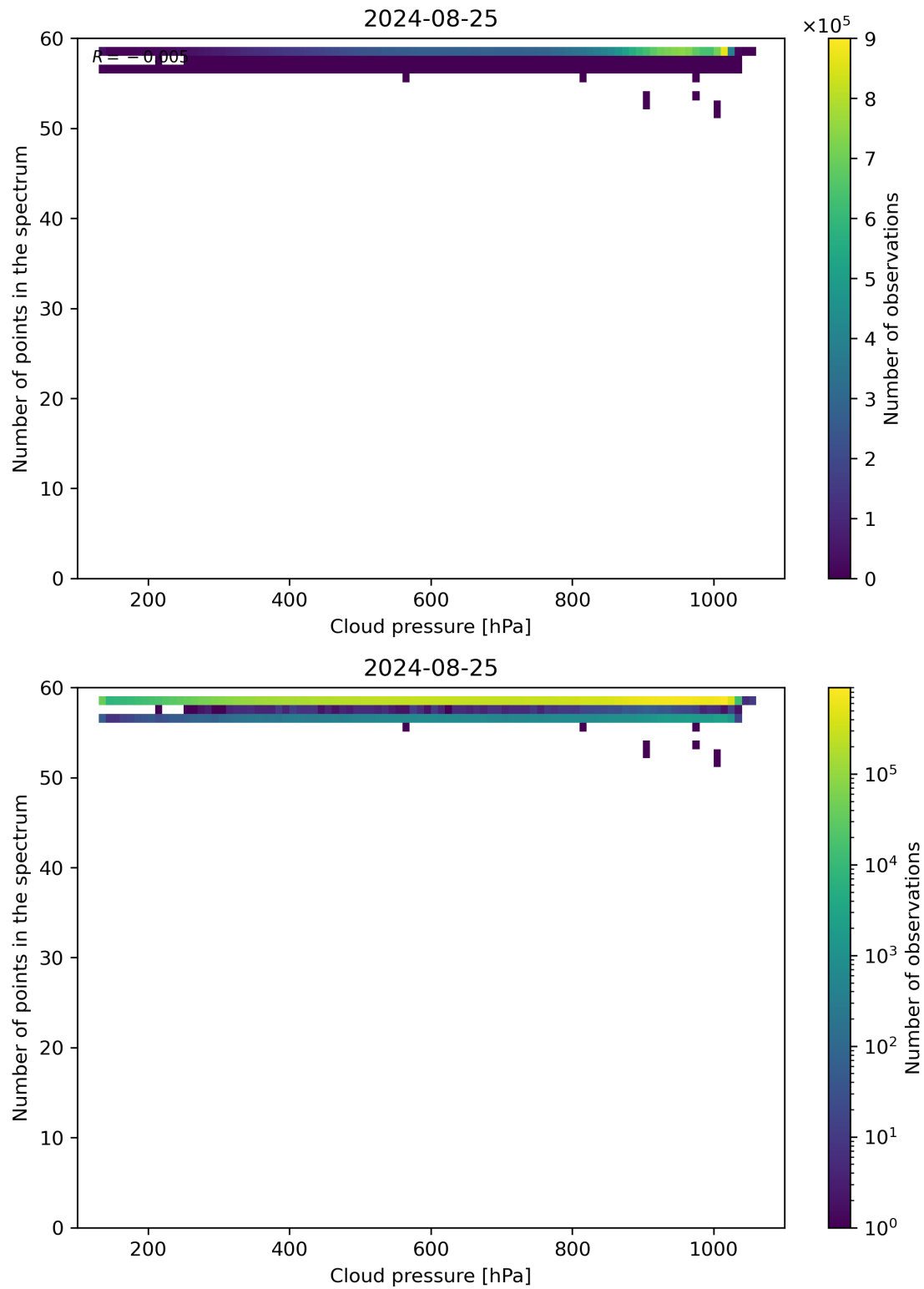
Figure 82: Scatter density plot of “Cloud pressure” against “Number of points in the spectrum” for 2024-08-24 to 2024-08-26.
