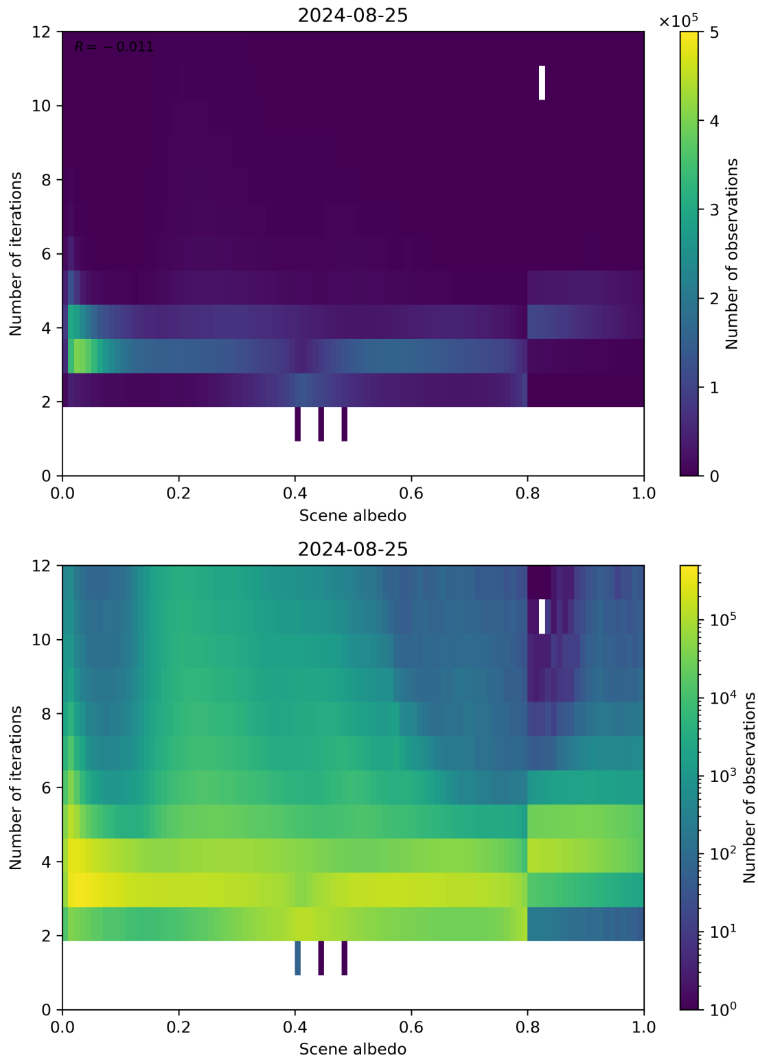
Figure 105: Scatter density plot of “Scene albedo” against “Number of iterations” for 2024-08-24 to 2024-08-26.
