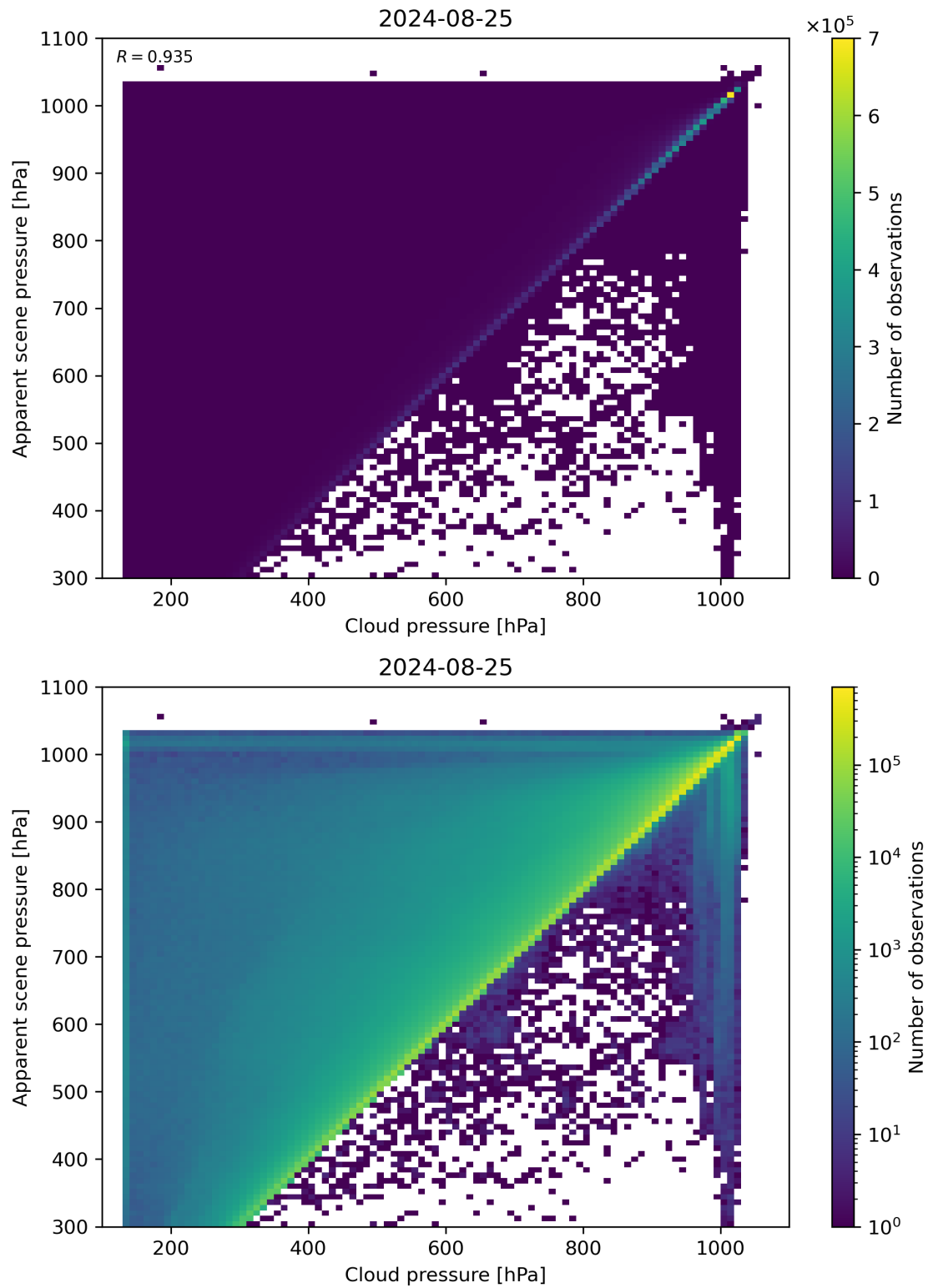
Figure 77: Scatter density plot of “Cloud pressure” against “Apparent scene pressure” for 2024-08-24 to 2024-08-26.
