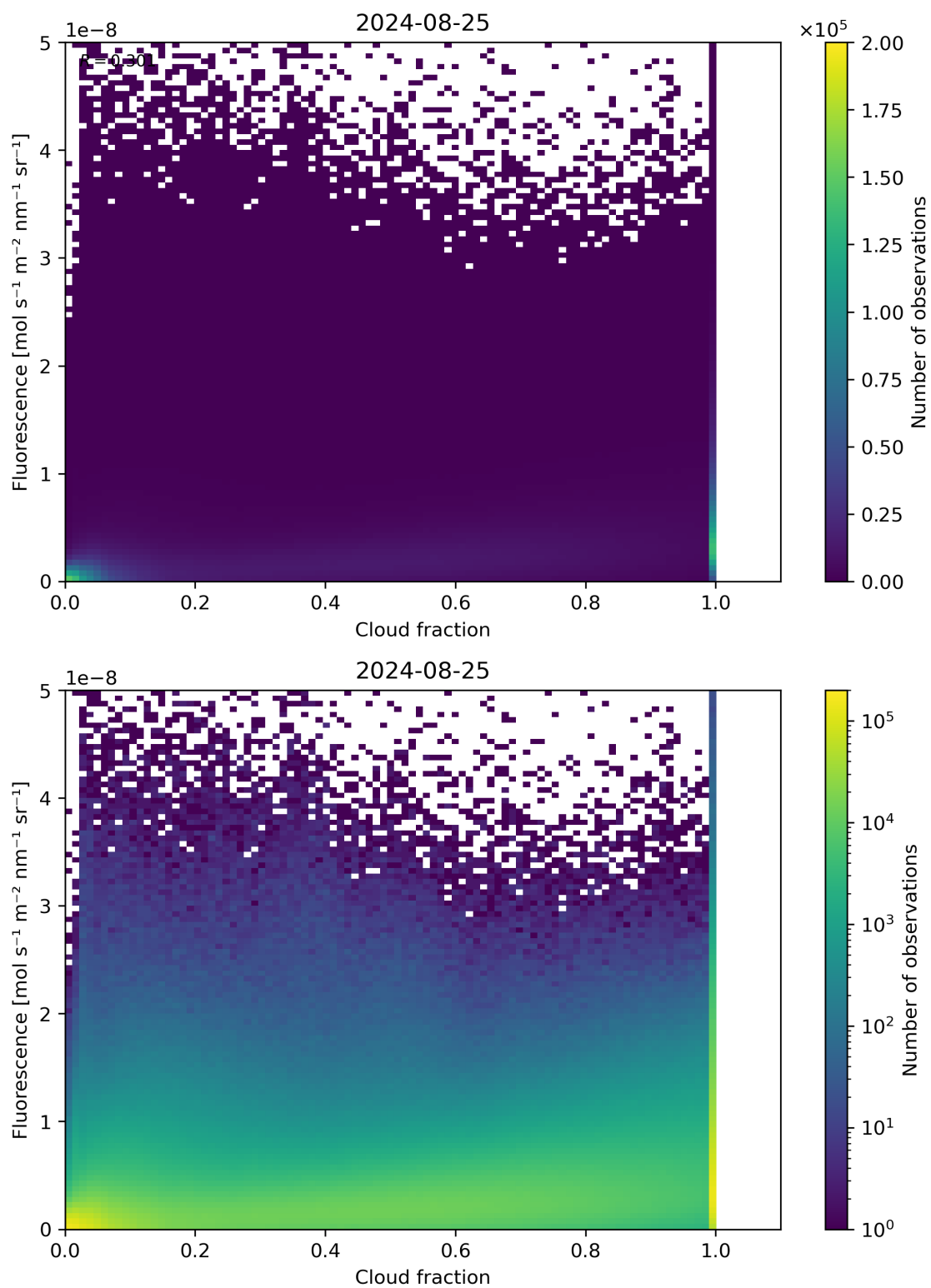
Figure 72: Scatter density plot of "Cloud fraction" against "Fluorescence" for 2024-08-24 to 2024-08-26.
