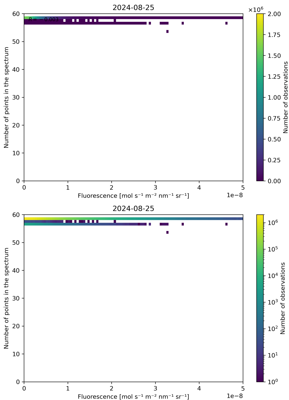
Figure 86: Scatter density plot of “Fluorescence” against “Number of points in the spectrum” for 2024-08-24 to 2024-08-26.
