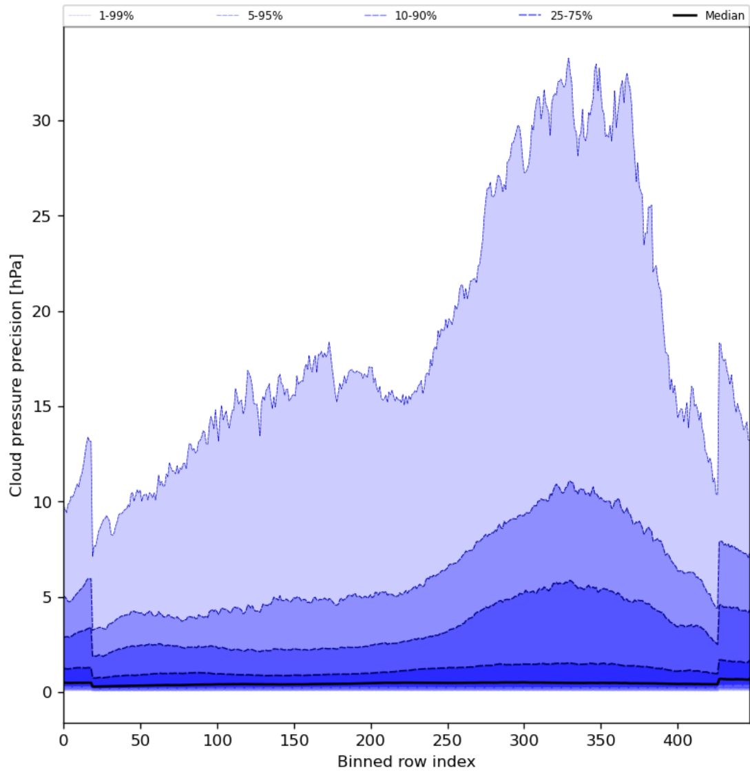
Figure 48: Along track statistics of “Cloud pressure precision” for 2024-08-24 to 2024-08-26
