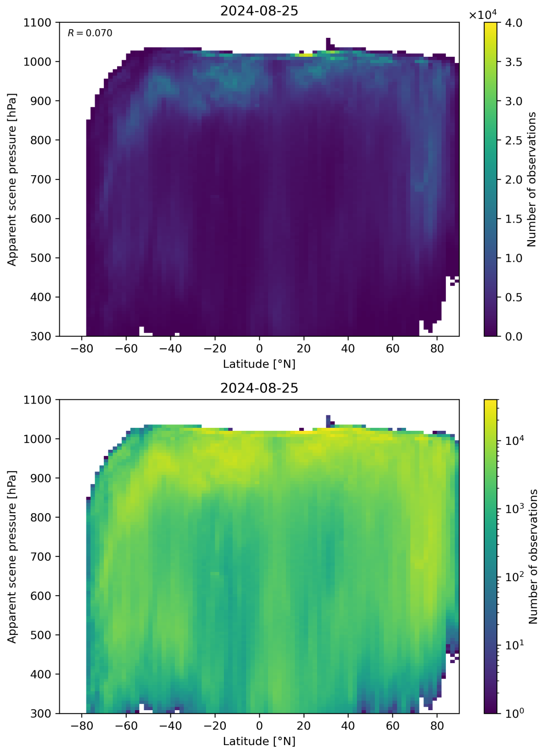
Figure 88: Scatter density plot of “Latitude” against “Apparent scene pressure” for 2024-08-24 to 2024-08-26.
