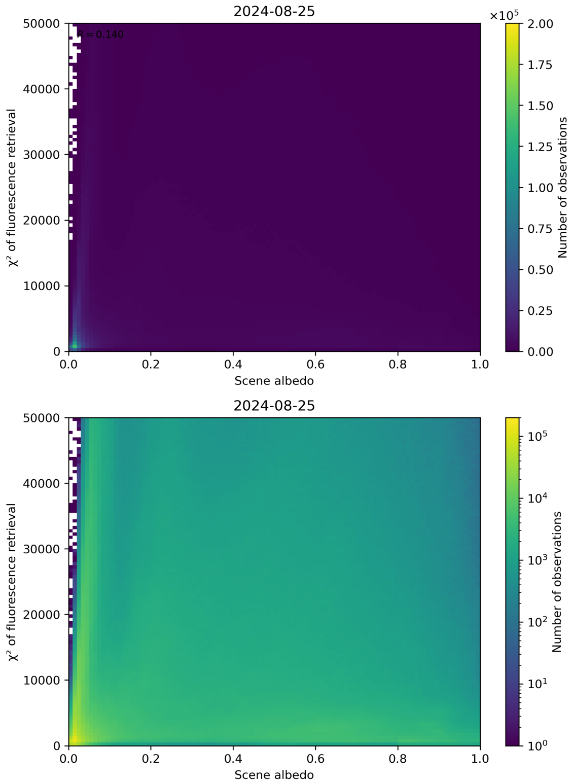
Figure 103: Scatter density plot of “Scene albedo” against “ \chi^2 of fluorescence retrieval” for 2024-08-24 to 2024-08-26.
