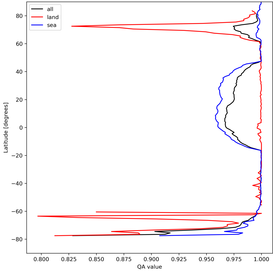
Figure 12: Zonal average of "QA value" for 2024-08-24 to 2024-08-26.
