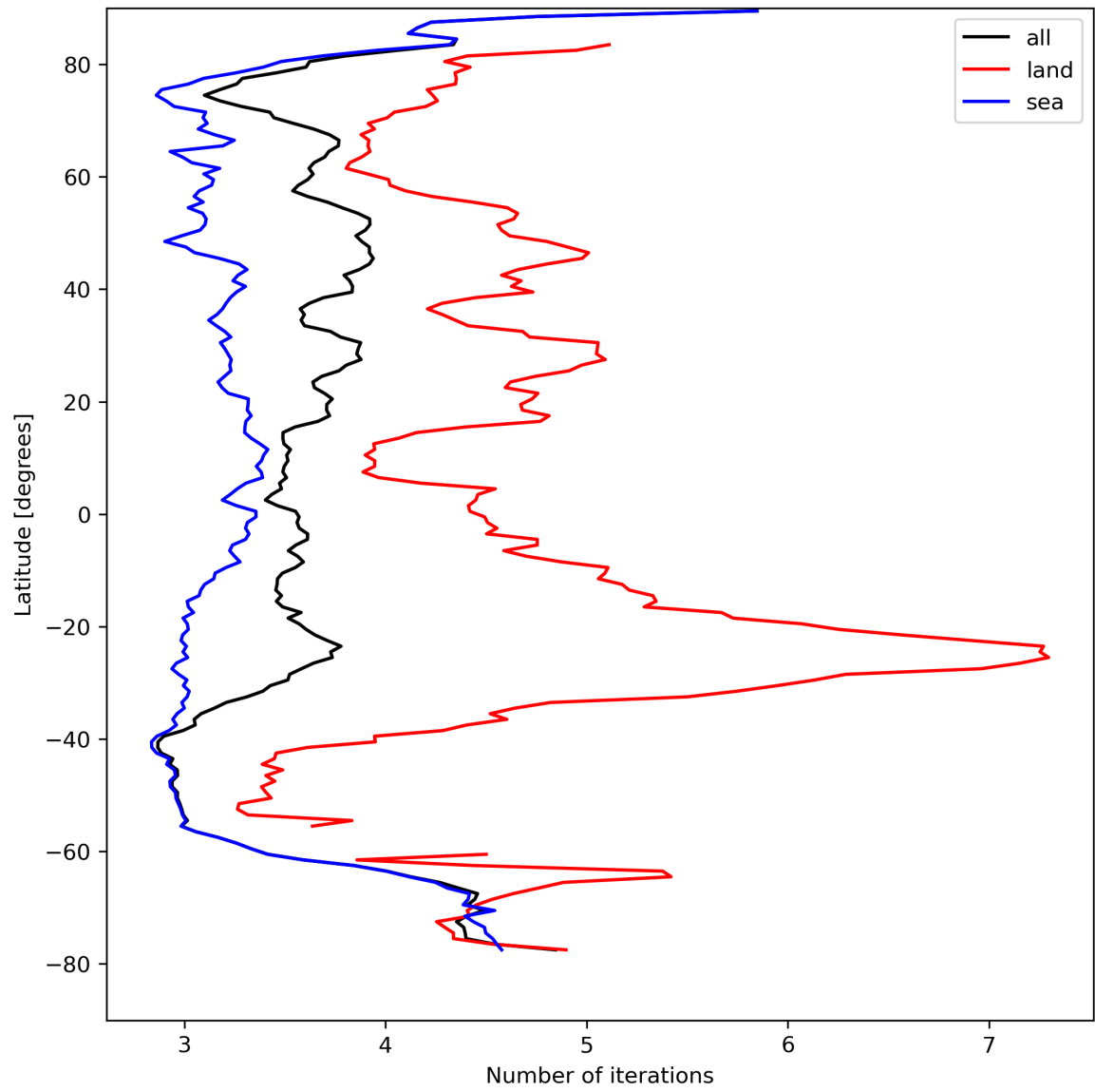
Figure 22: Zonal average of “Number of iterations” for 2024-08-24 to 2024-08-26.
