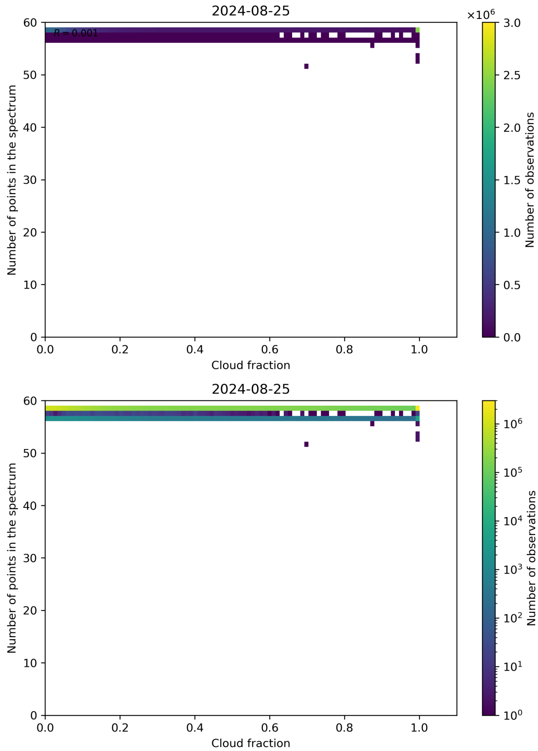
Figure 74: Scatter density plot of “Cloud fraction” against “Number of points in the spectrum” for 2024-08-24 to 2024-08-26.
