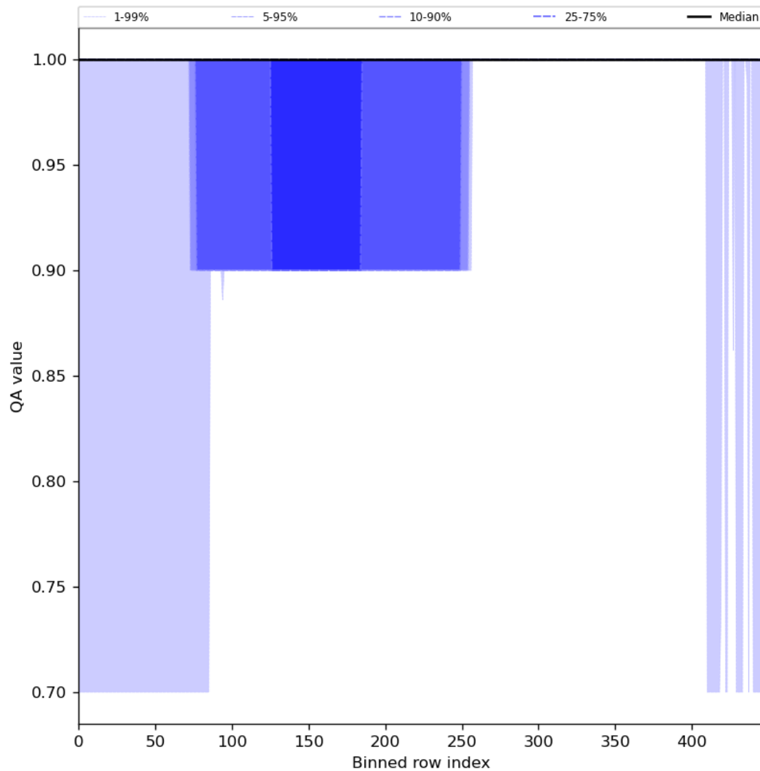
Figure 46: Along track statistics of “QA value” for 2024-08-24 to 2024-08-26
