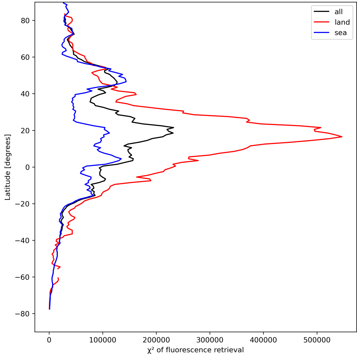
Figure 25: Zonal average of “ \chi^2 of fluorescence retrieval” for 2024-08-24 to 2024-08-26.
