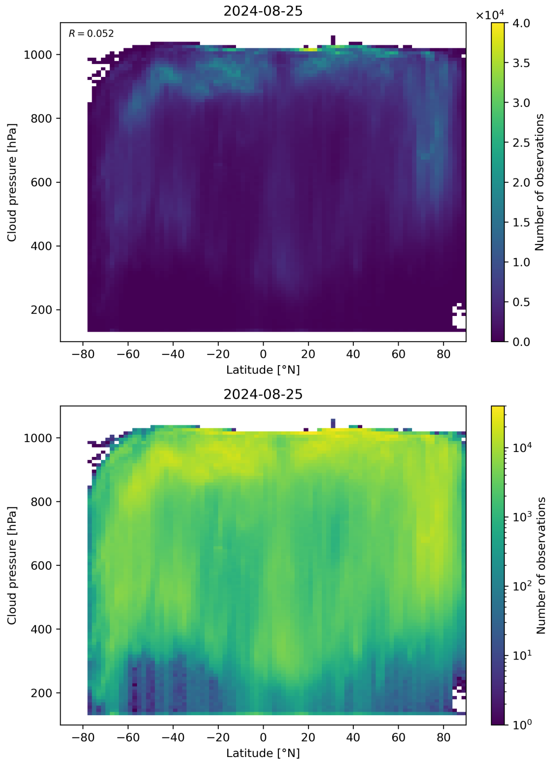
Figure 91: Scatter density plot of “Latitude” against “Cloud pressure” for 2024-08-24 to 2024-08-26.
