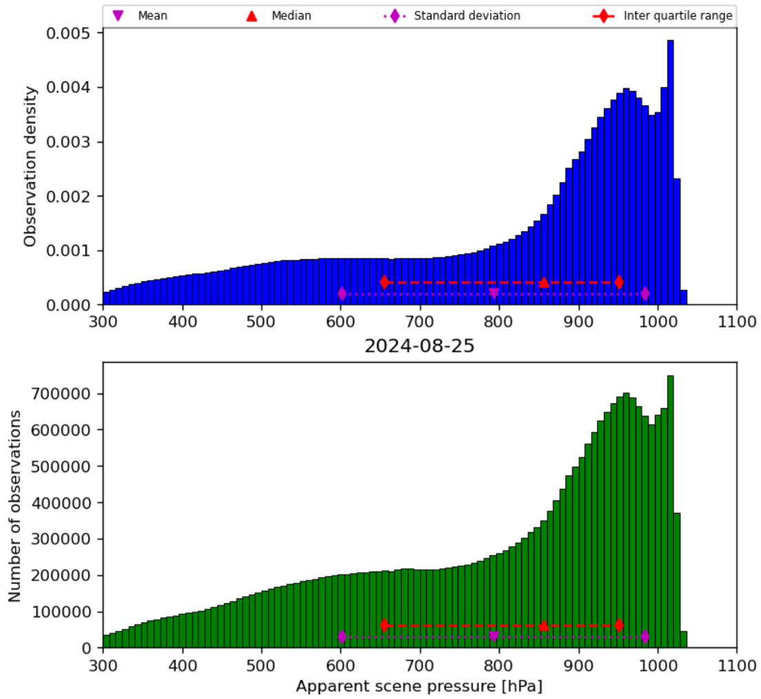
Figure 36: Histogram of “Apparent scene pressure” for 2024-08-24 to 2024-08-26
