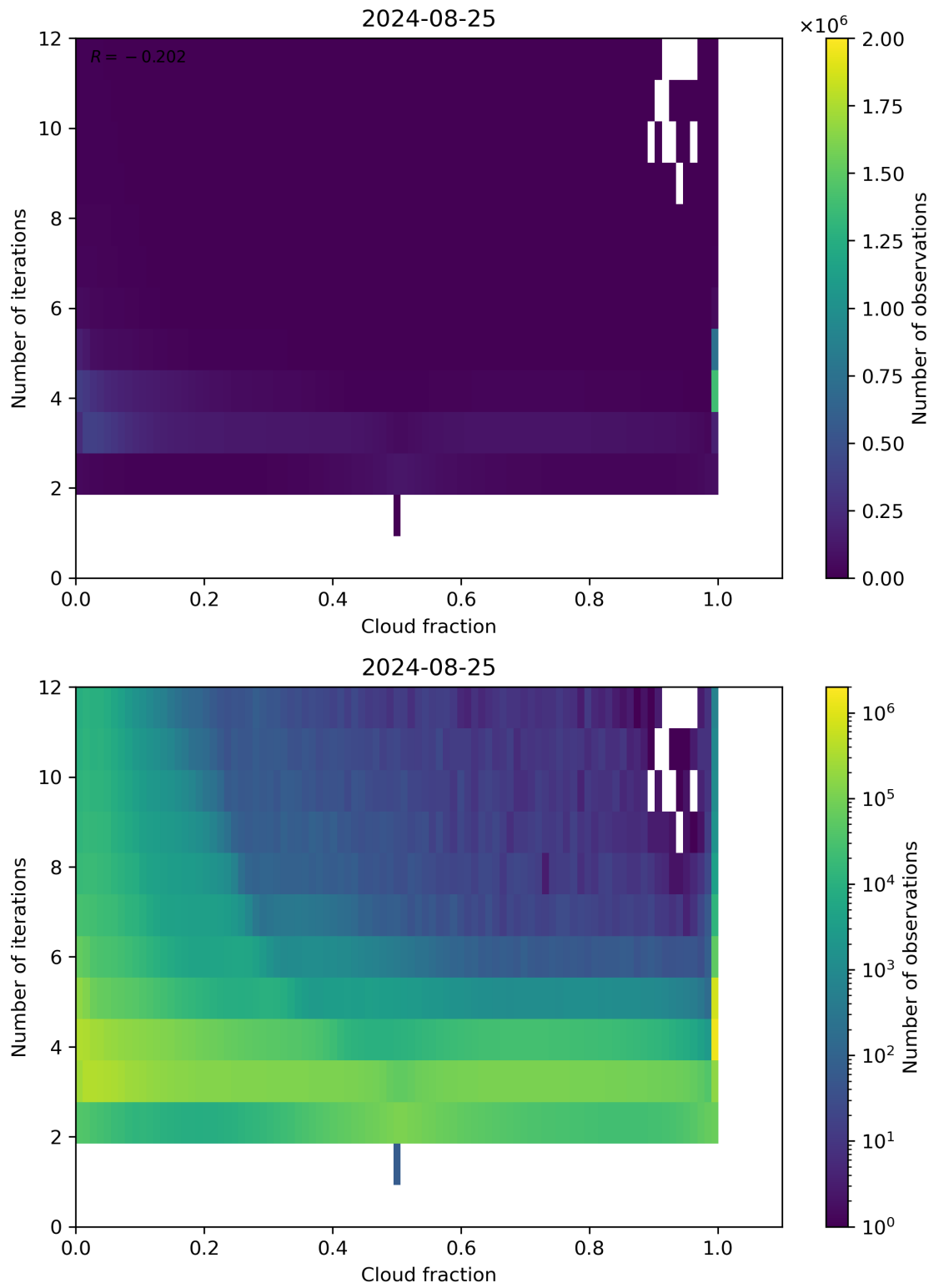
Figure 73: Scatter density plot of “Cloud fraction” against “Number of iterations” for 2024-08-24 to 2024-08-26.
