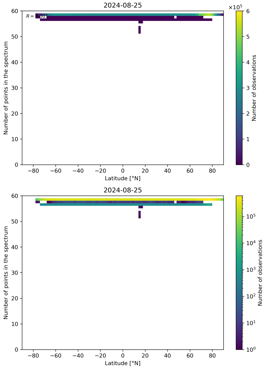
Figure 94: Scatter density plot of “Latitude” against “Number of points in the spectrum” for 2024-08-24 to 2024-08-26.
