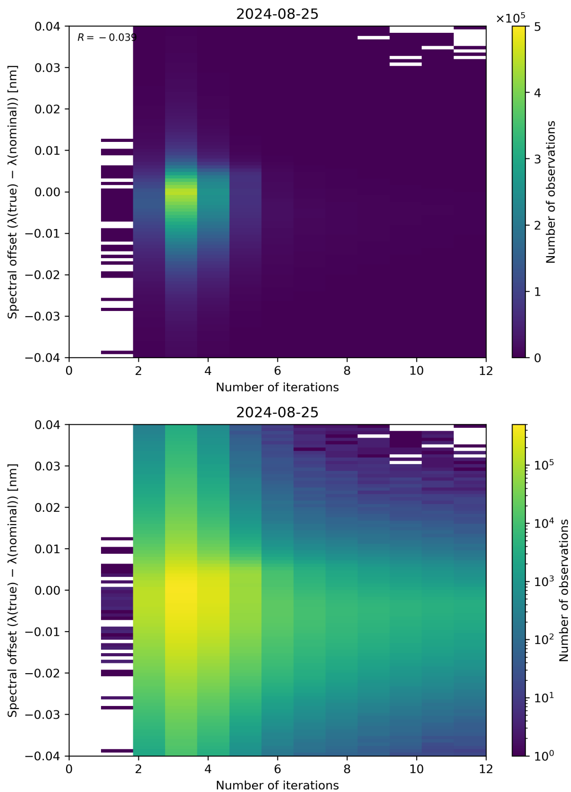
Figure 100: Scatter density plot of “Number of iterations” against “Spectral offset ( \lambda(\text{true}) - \lambda(\text{nominal}) )” for 2024-08-24 to 2024-08-26.
