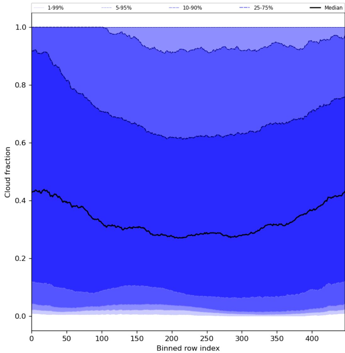
Figure 49: Along track statistics of “Cloud fraction” for 2024-08-24 to 2024-08-26
