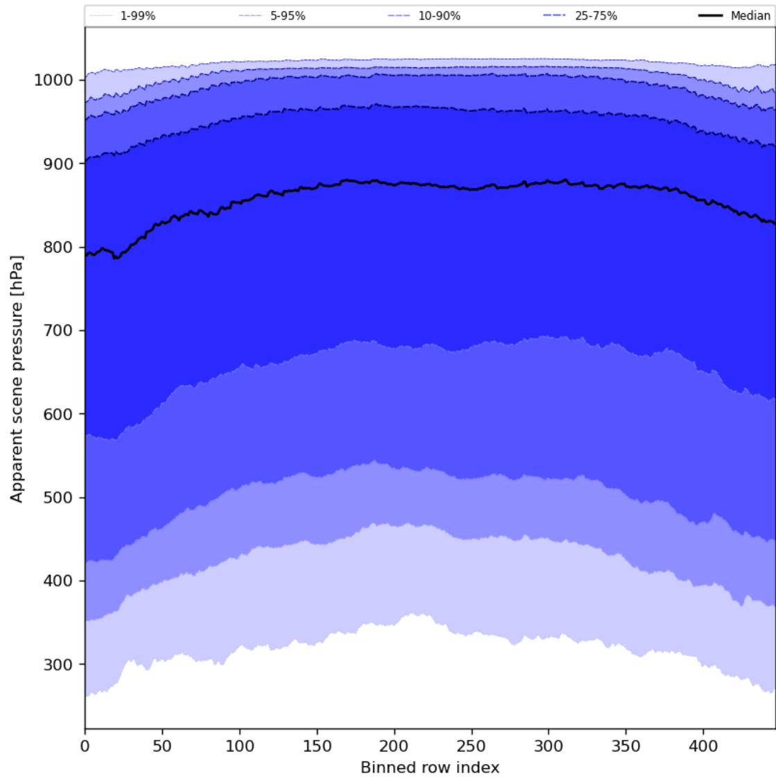
Figure 53: Along track statistics of “Apparent scene pressure” for 2024-08-24 to 2024-08-26
