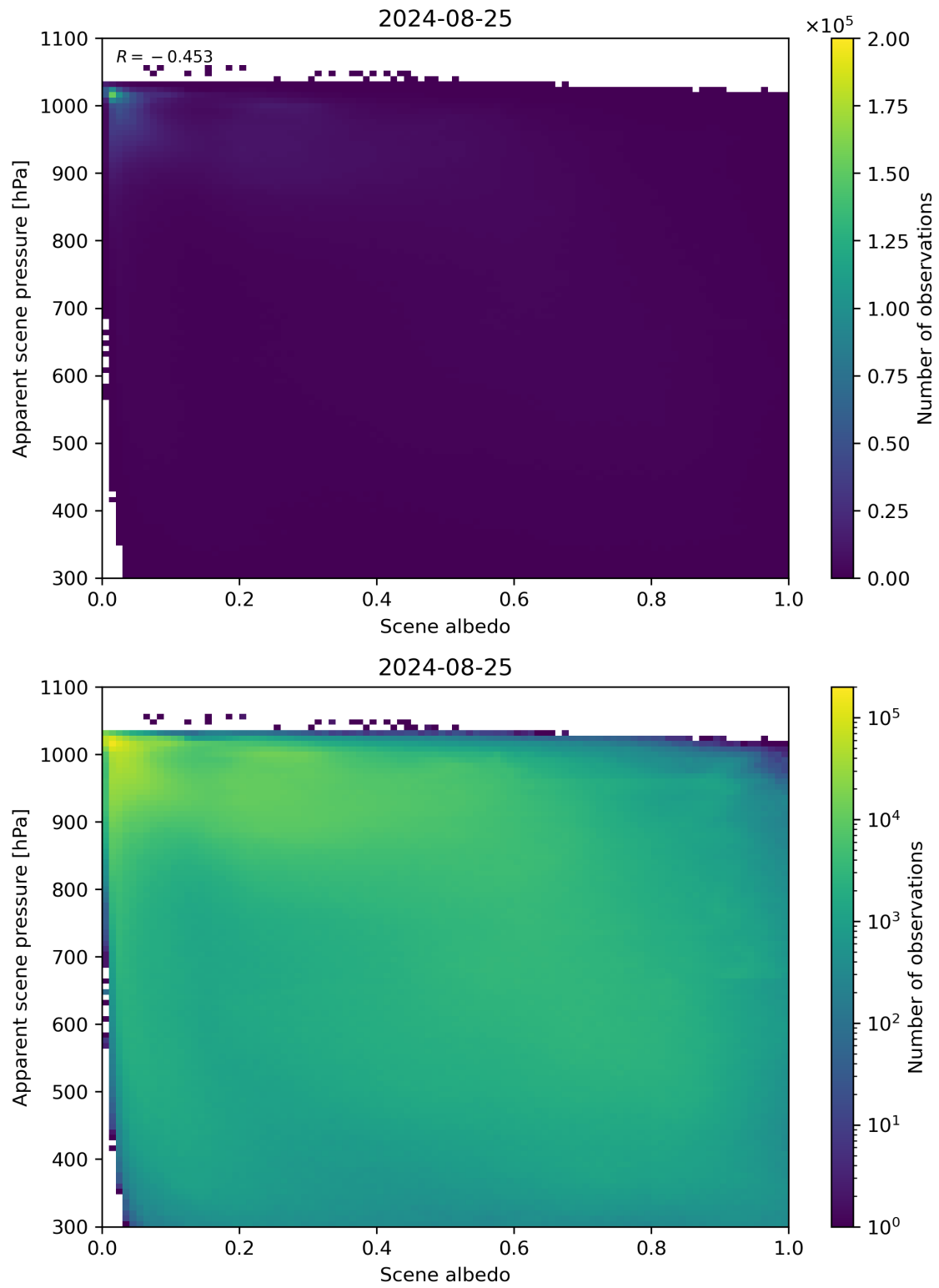
Figure 102: Scatter density plot of “Scene albedo” against “Apparent scene pressure” for 2024-08-24 to 2024-08-26.
