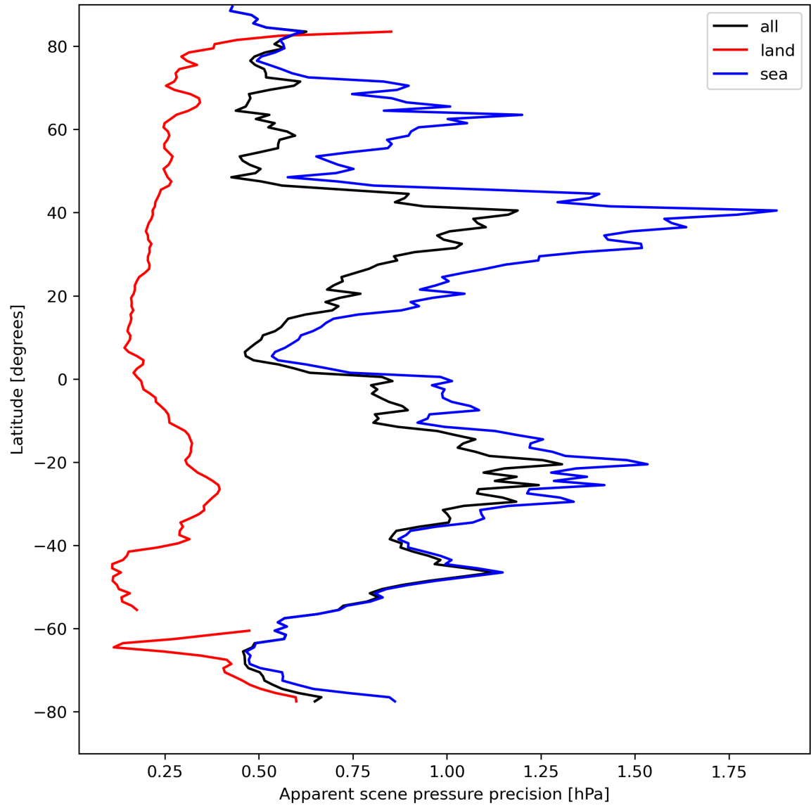
Figure 20: Zonal average of “Apparent scene pressure precision” for 2024-08-24 to 2024-08-26.
