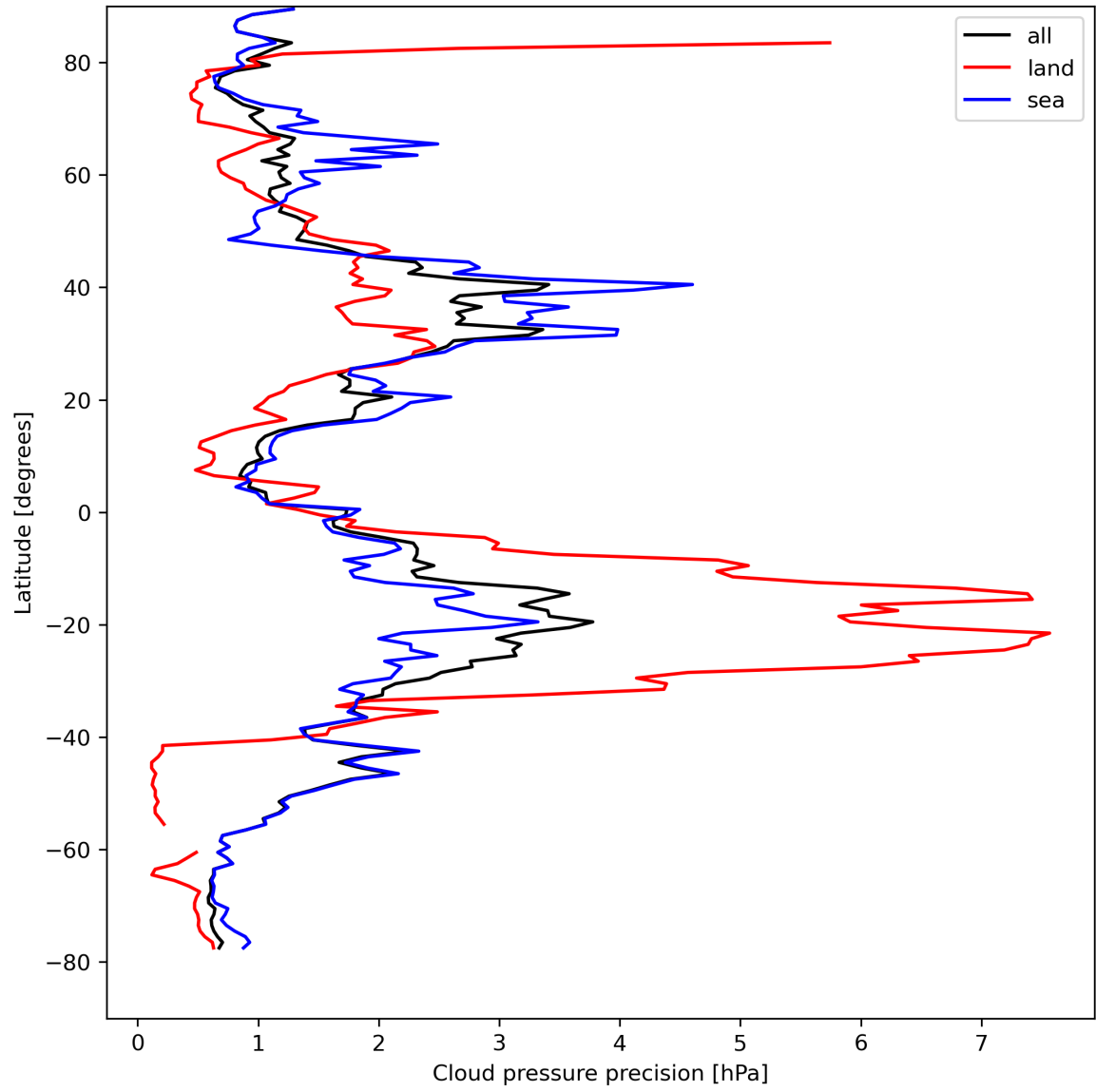
Figure 14: Zonal average of "Cloud pressure precision" for 2024-08-24 to 2024-08-26.
