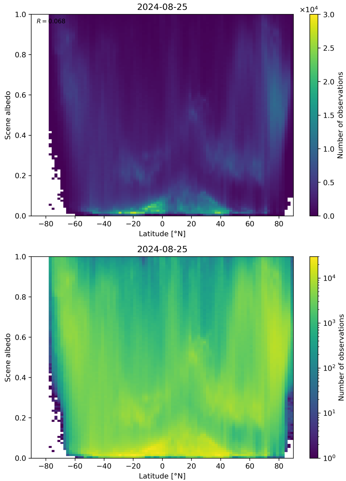
Figure 95: Scatter density plot of “Latitude” against “Scene albedo” for 2024-08-24 to 2024-08-26.
