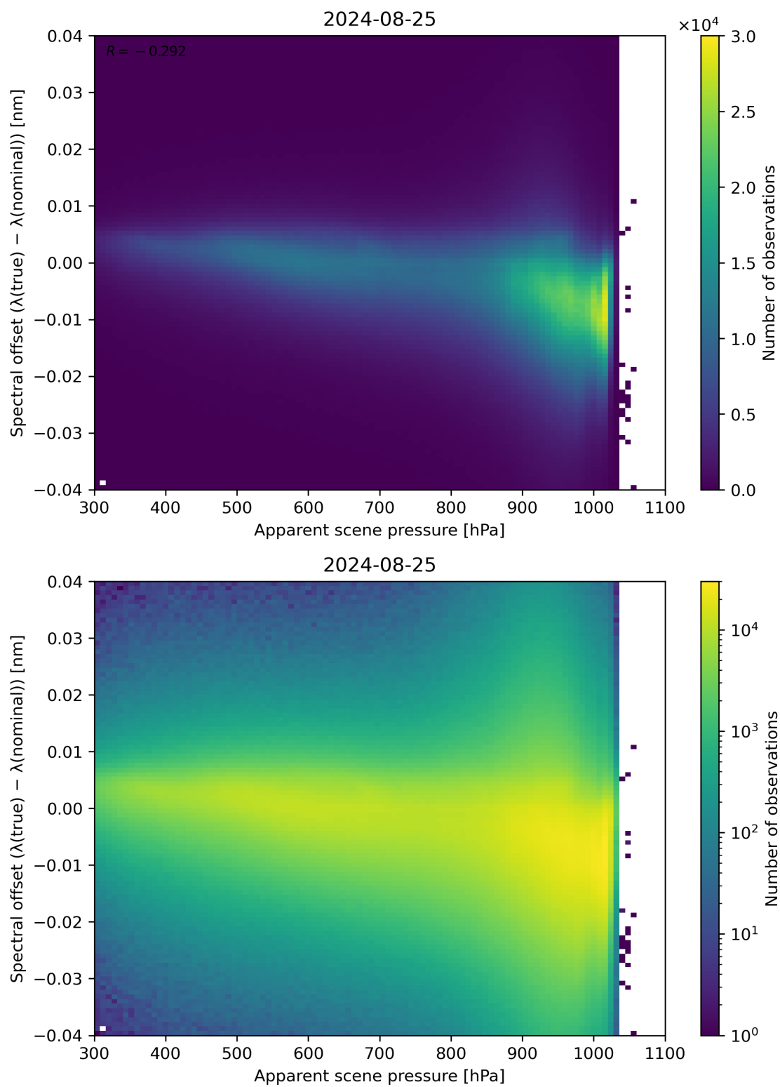
Figure 67: Scatter density plot of “Apparent scene pressure” against “Spectral offset ( \lambda(\text{true}) - \lambda(\text{nominal}) )” for 2024-08-24 to 2024-08-26.
