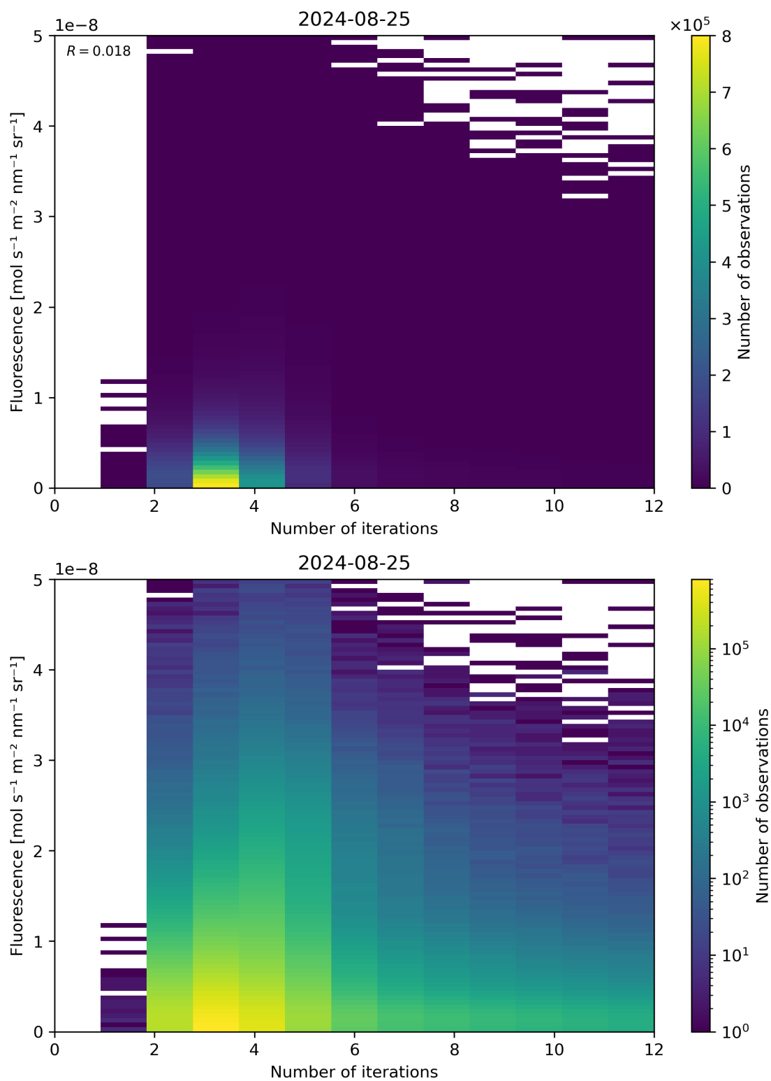
Figure 98: Scatter density plot of “Number of iterations” against “Fluorescence” for 2024-08-24 to 2024-08-26.
