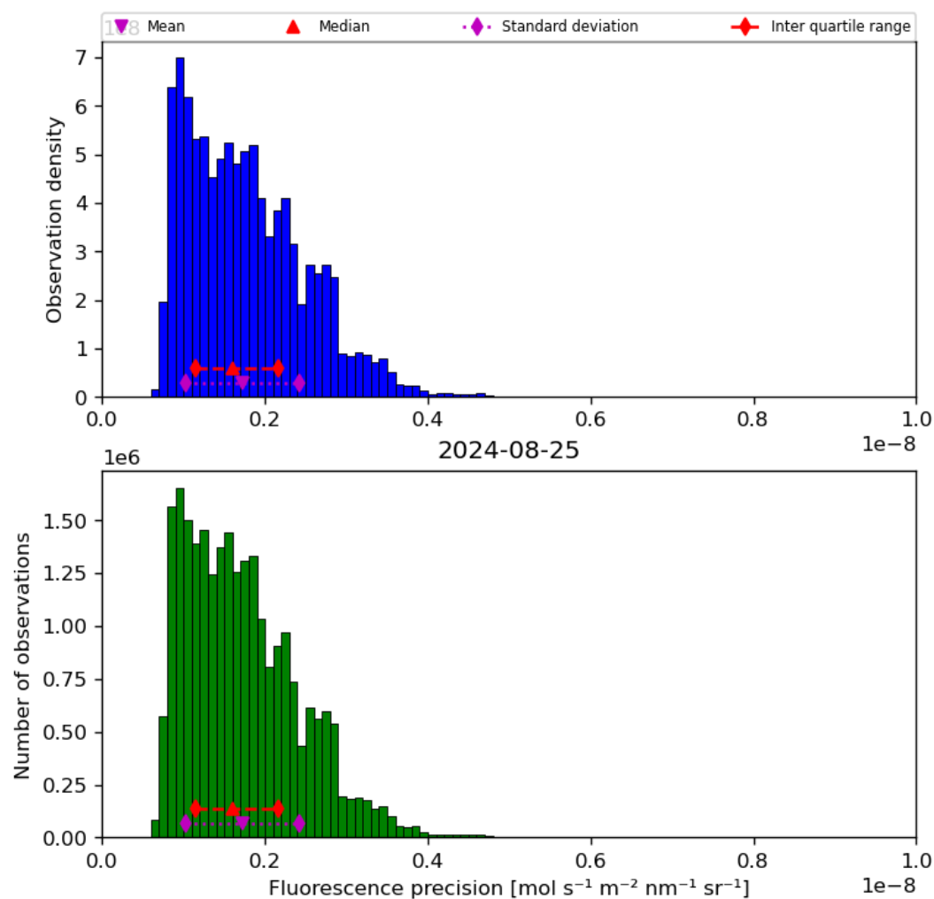
Figure 41: Histogram of “Fluorescence precision” for 2024-08-24 to 2024-08-26
