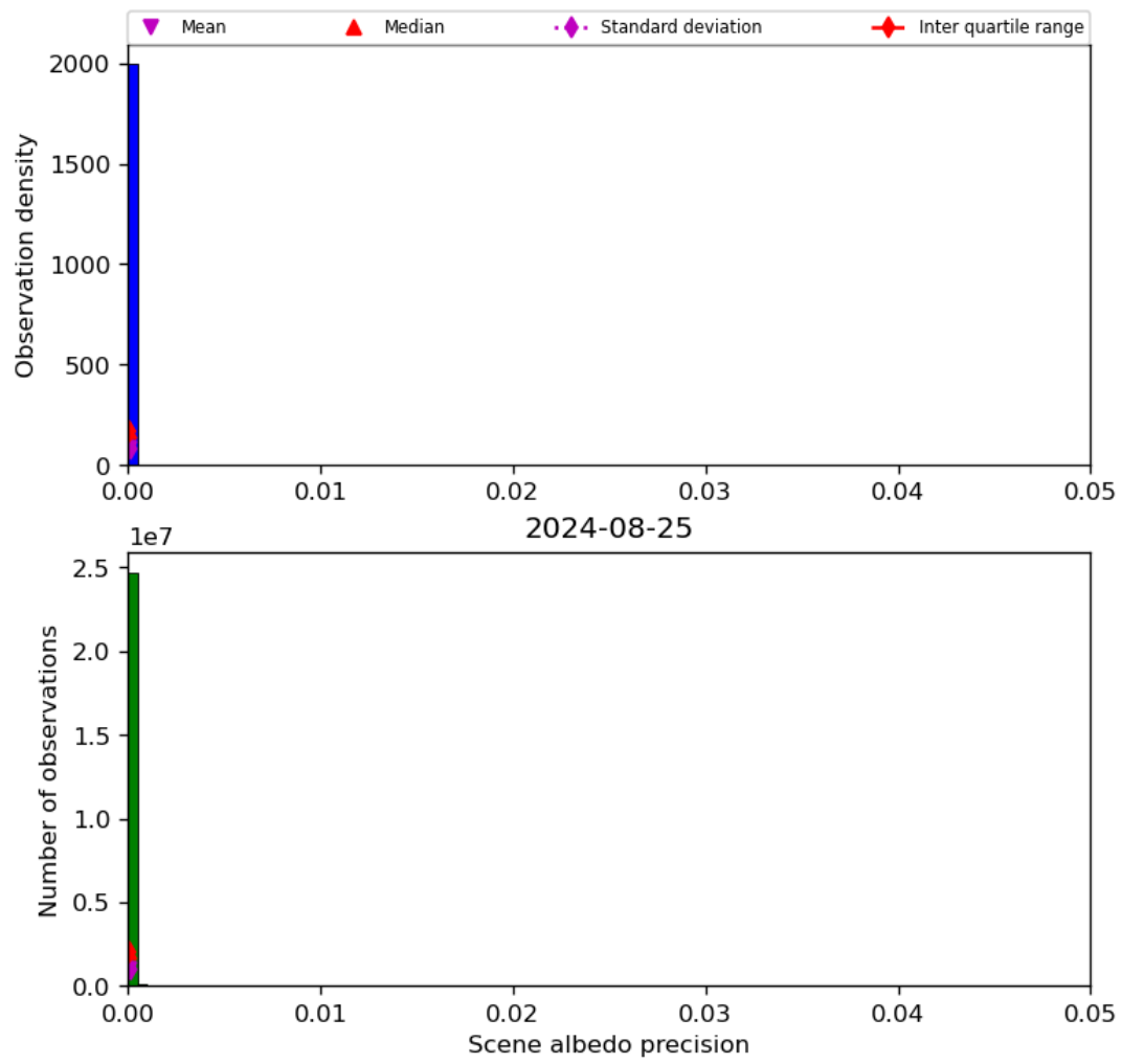
Figure 35: Histogram of “Scene albedo precision” for 2024-08-24 to 2024-08-26
