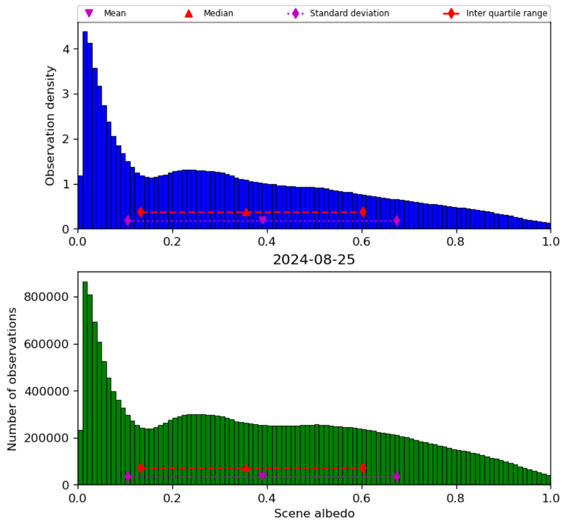
Figure 34: Histogram of “Scene albedo” for 2024-08-24 to 2024-08-26
