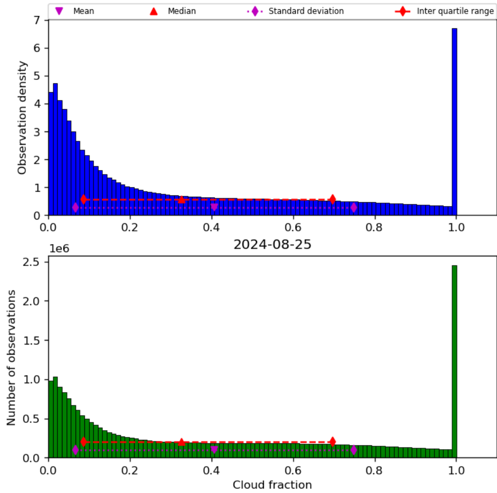
Figure 32: Histogram of “Cloud fraction” for 2024-08-24 to 2024-08-26
