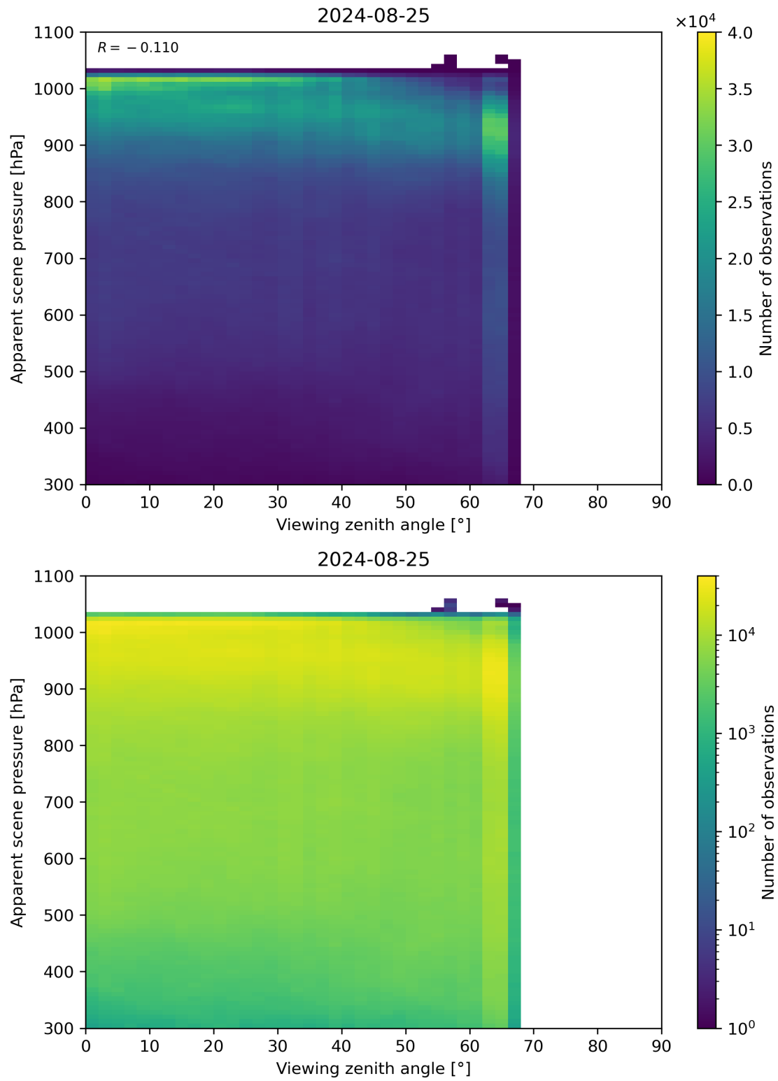
Figure 118: Scatter density plot of “Viewing zenith angle” against “Apparent scene pressure” for 2024-08-24 to 2024-08-26.
