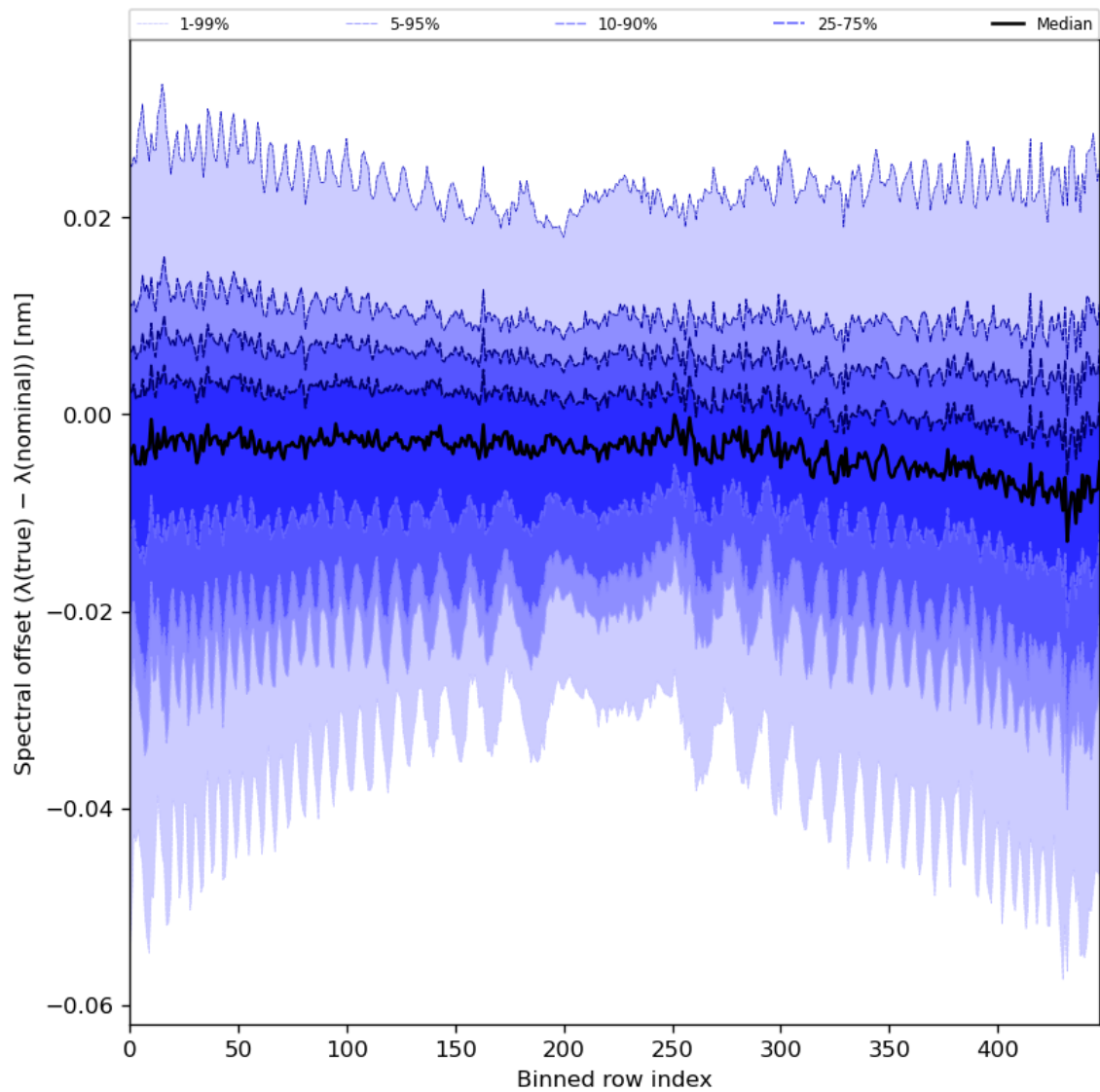
Figure 62: Along track statistics of “Spectral offset ( \lambda(\text{true}) - \lambda(\text{nominal}) )” for 2024-08-24 to 2024-08-26
