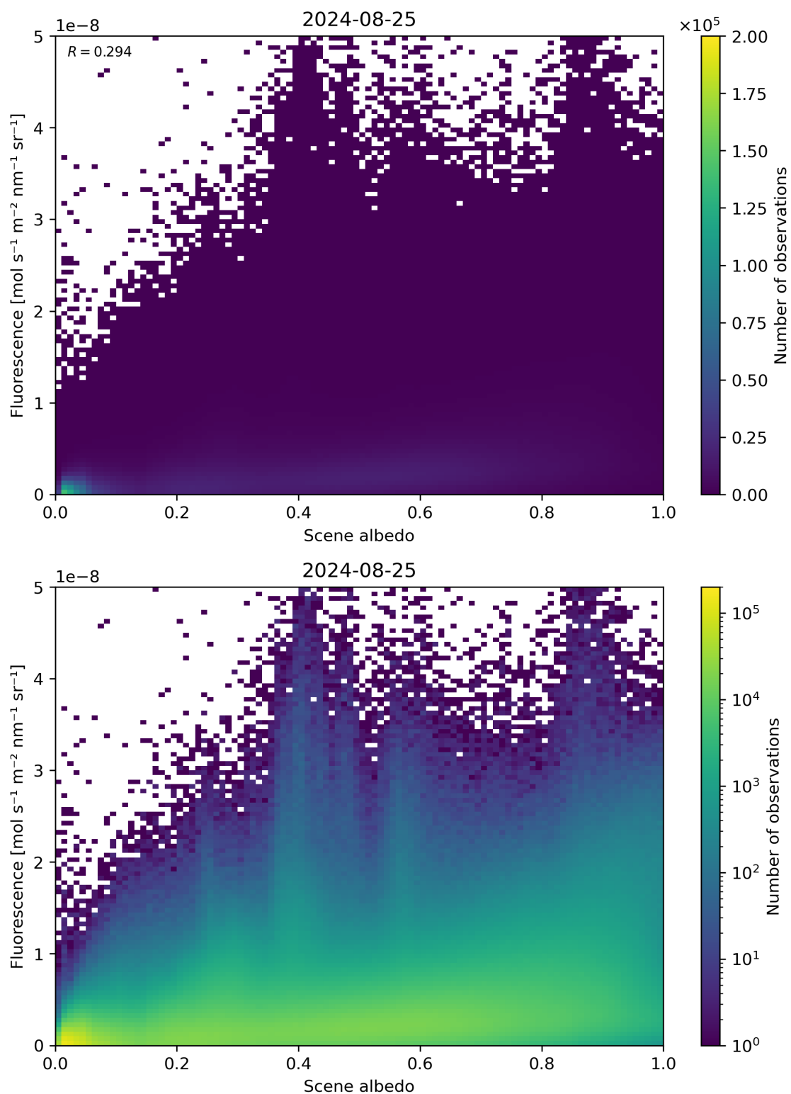
Figure 104: Scatter density plot of “Scene albedo” against “Fluorescence” for 2024-08-24 to 2024-08-26.
