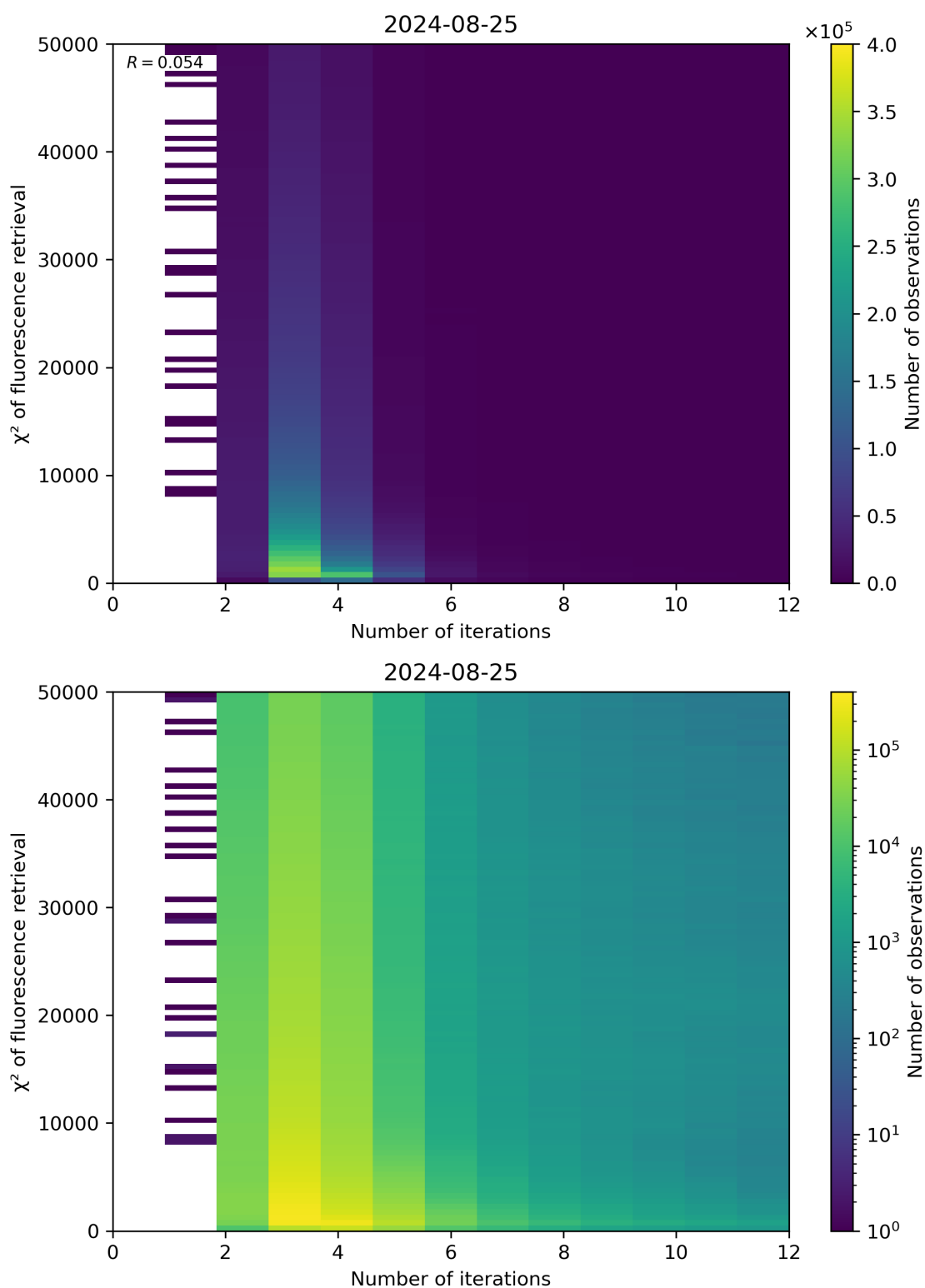
Figure 97: Scatter density plot of “Number of iterations” against “ \chi^2 of fluorescence retrieval” for 2024-08-24 to 2024-08-26.
