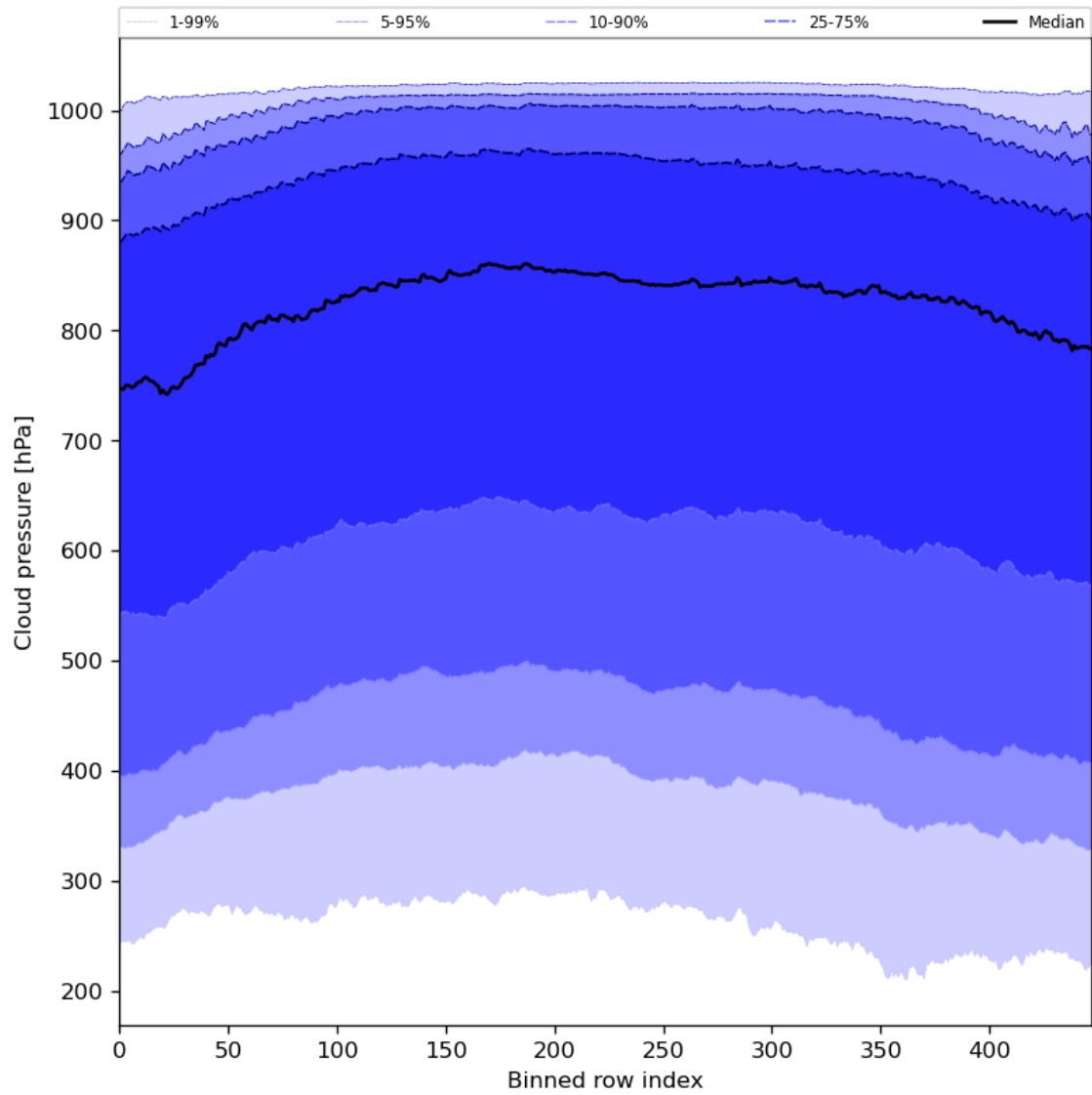
Figure 47: Along track statistics of “Cloud pressure” for 2024-08-24 to 2024-08-26
