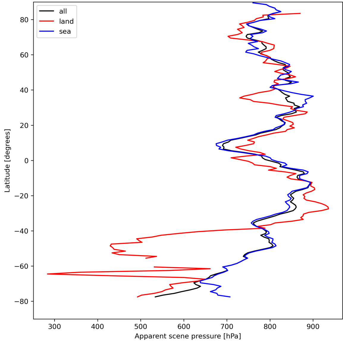
Figure 19: Zonal average of “Apparent scene pressure” for 2024-08-24 to 2024-08-26.
