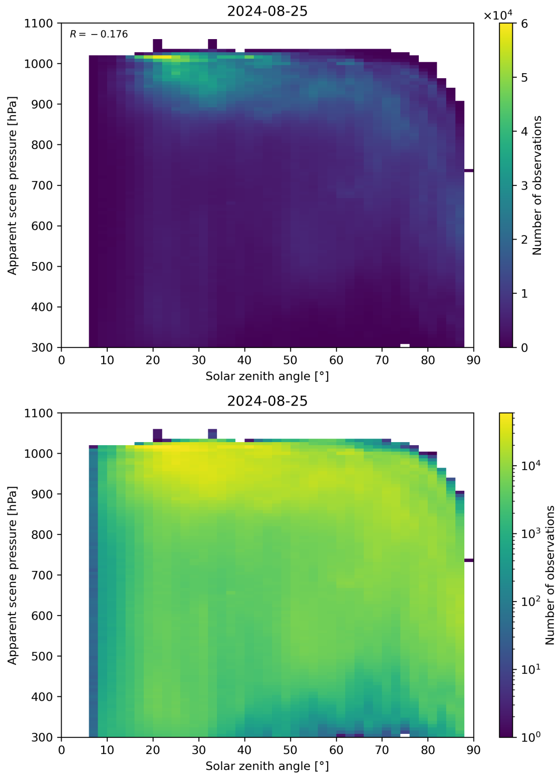
Figure 108: Scatter density plot of “Solar zenith angle” against “Apparent scene pressure” for 2024-08-24 to 2024-08-26.
