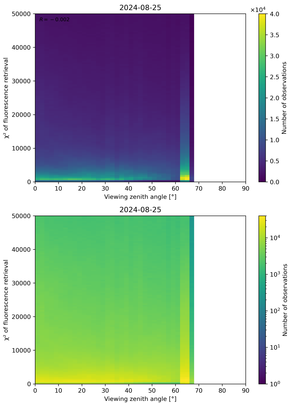
Figure 119: Scatter density plot of “Viewing zenith angle” against “ \chi^2 of fluorescence retrieval” for 2024-08-24 to 2024-08-26.
