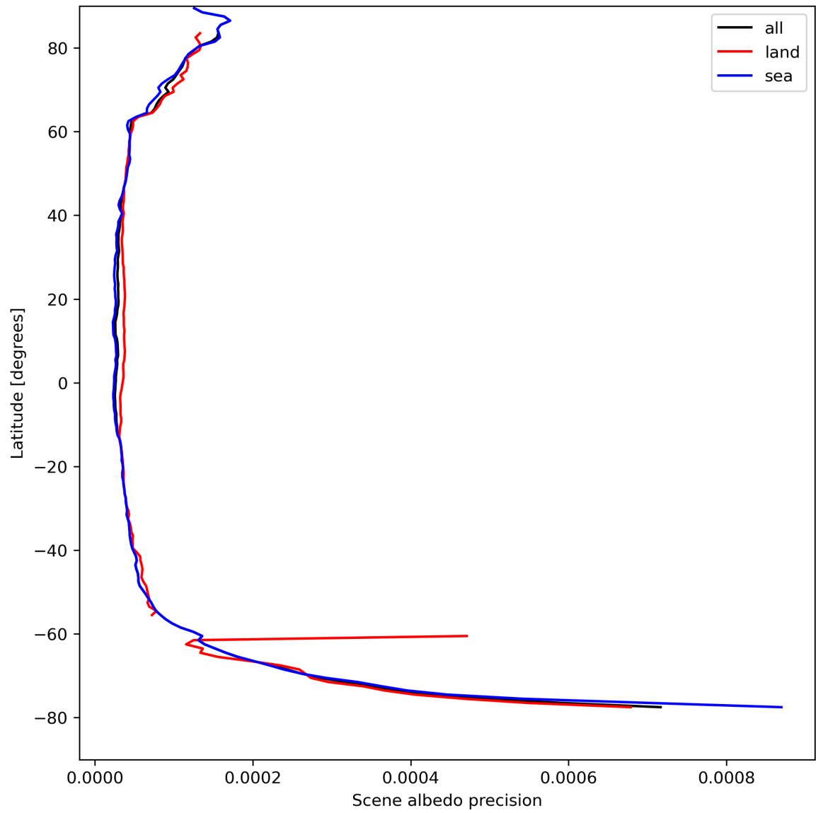
Figure 18: Zonal average of “Scene albedo precision” for 2024-08-24 to 2024-08-26.
