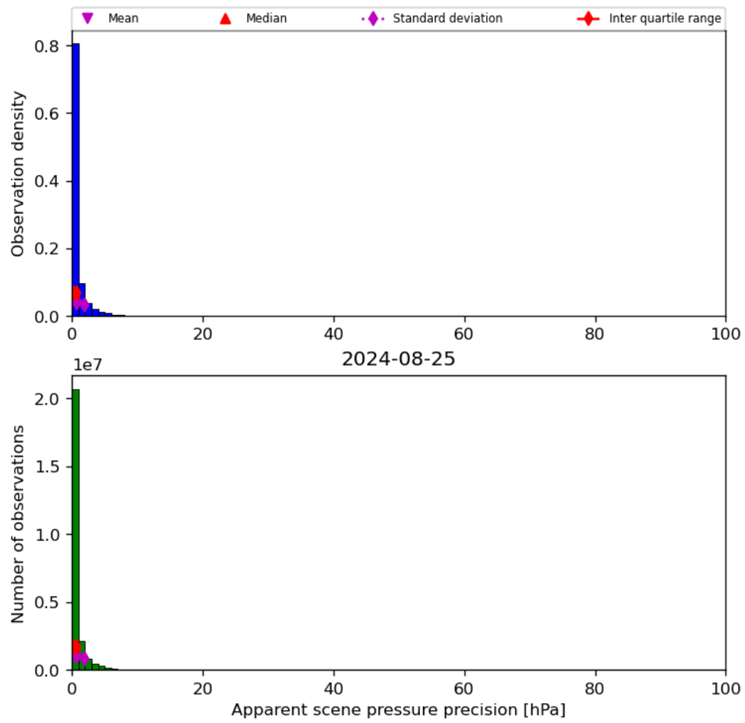
Figure 37: Histogram of “Apparent scene pressure precision” for 2024-08-24 to 2024-08-26
