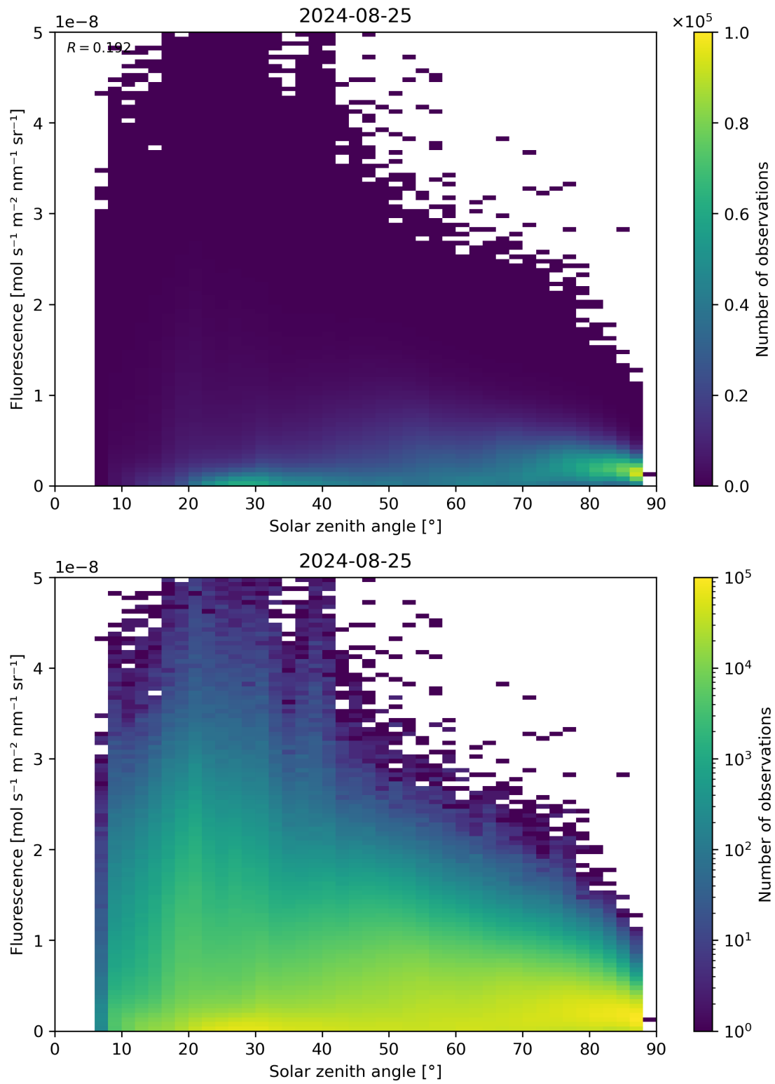
Figure 112: Scatter density plot of “Solar zenith angle” against “Fluorescence” for 2024-08-24 to 2024-08-26.
