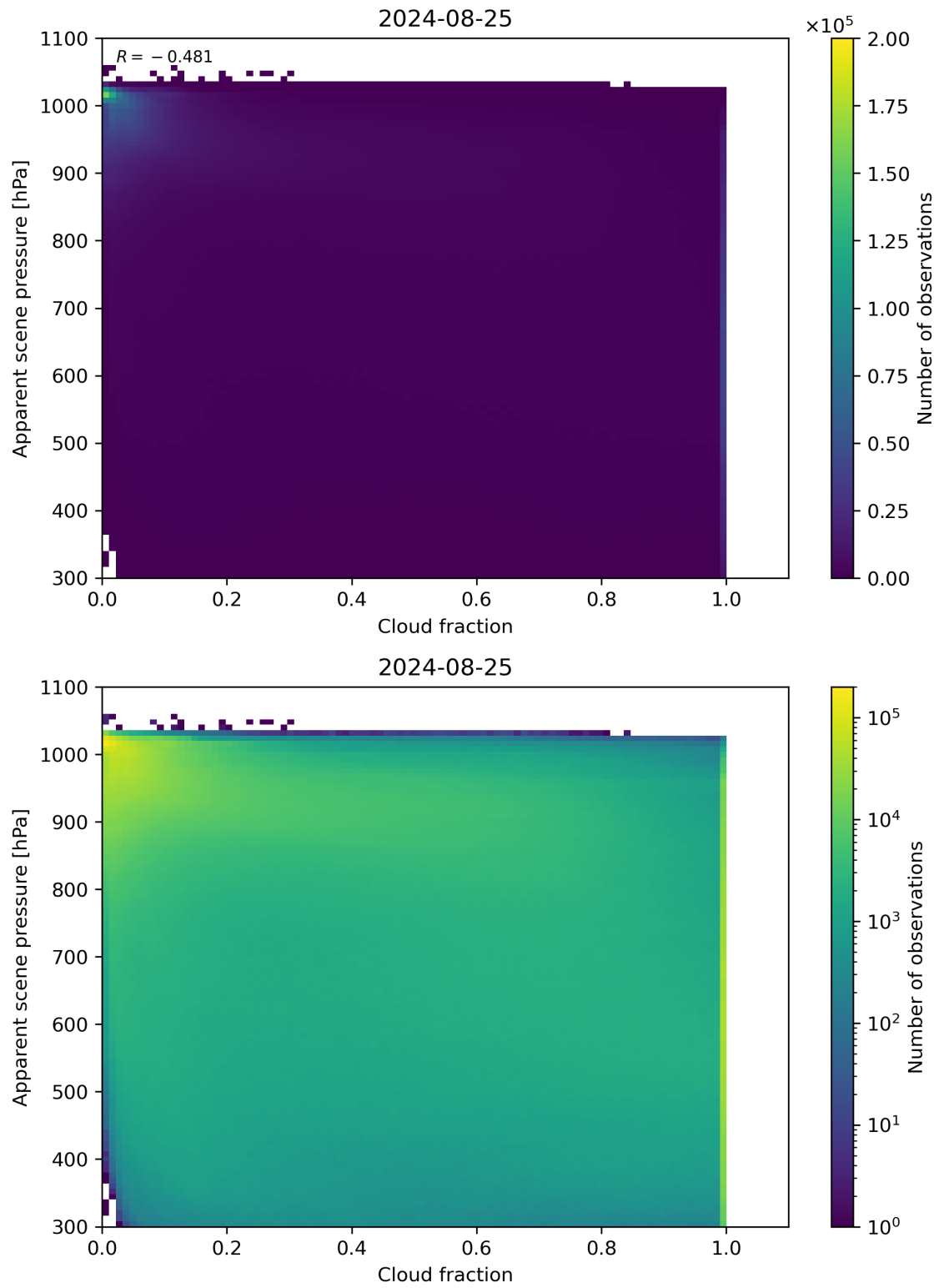
Figure 70: Scatter density plot of “Cloud fraction” against “Apparent scene pressure” for 2024-08-24 to 2024-08-26.
