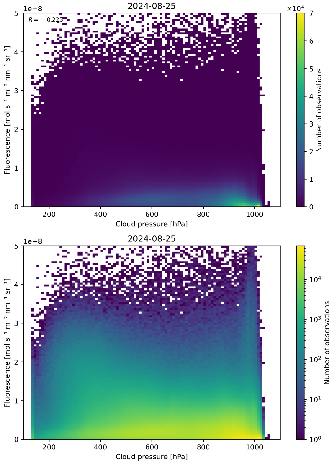
Figure 80: Scatter density plot of “Cloud pressure” against “Fluorescence” for 2024-08-24 to 2024-08-26.
