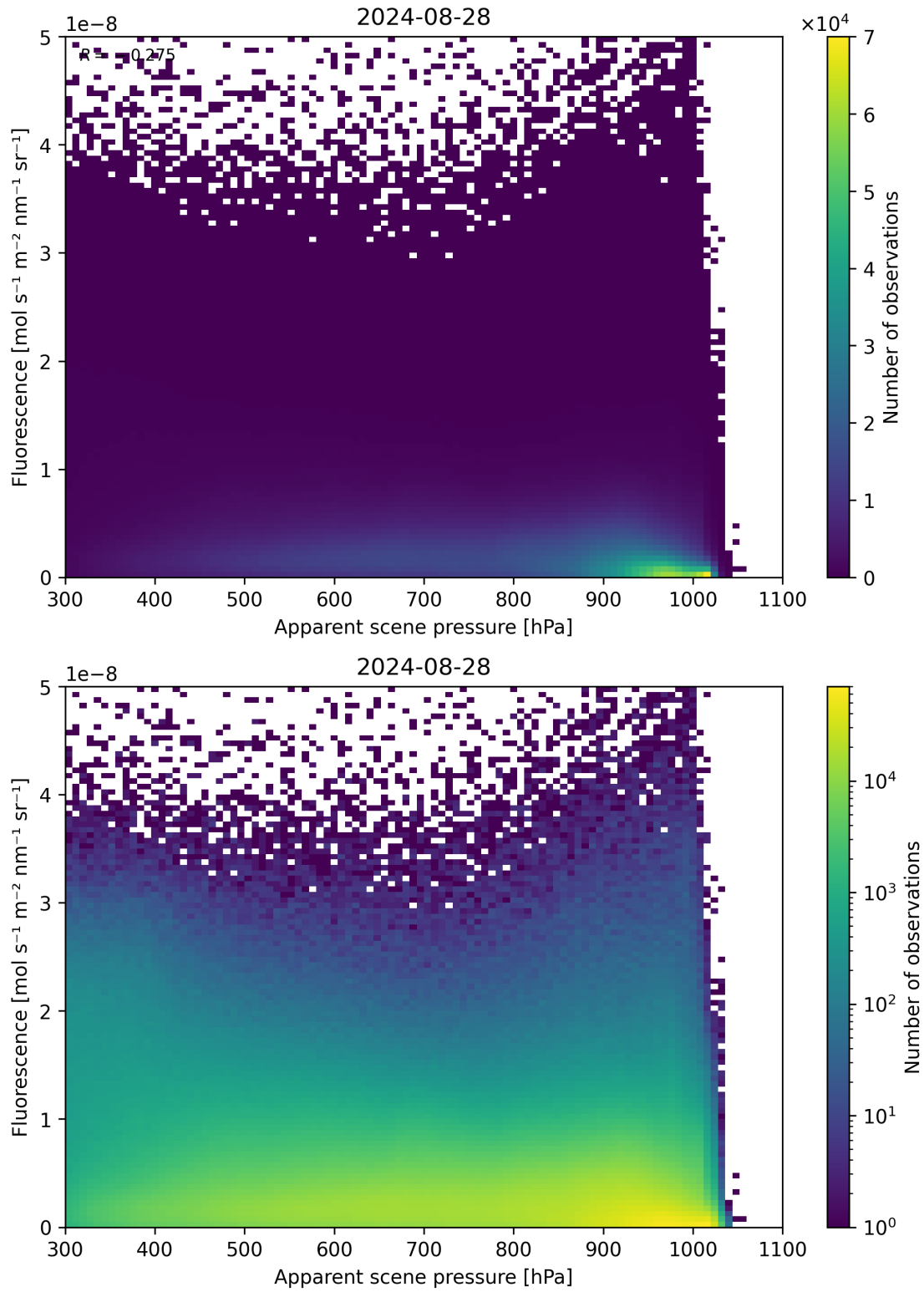
Figure 64: Scatter density plot of “Apparent scene pressure” against “Fluorescence” for 2024-08-27 to 2024-08-29.
