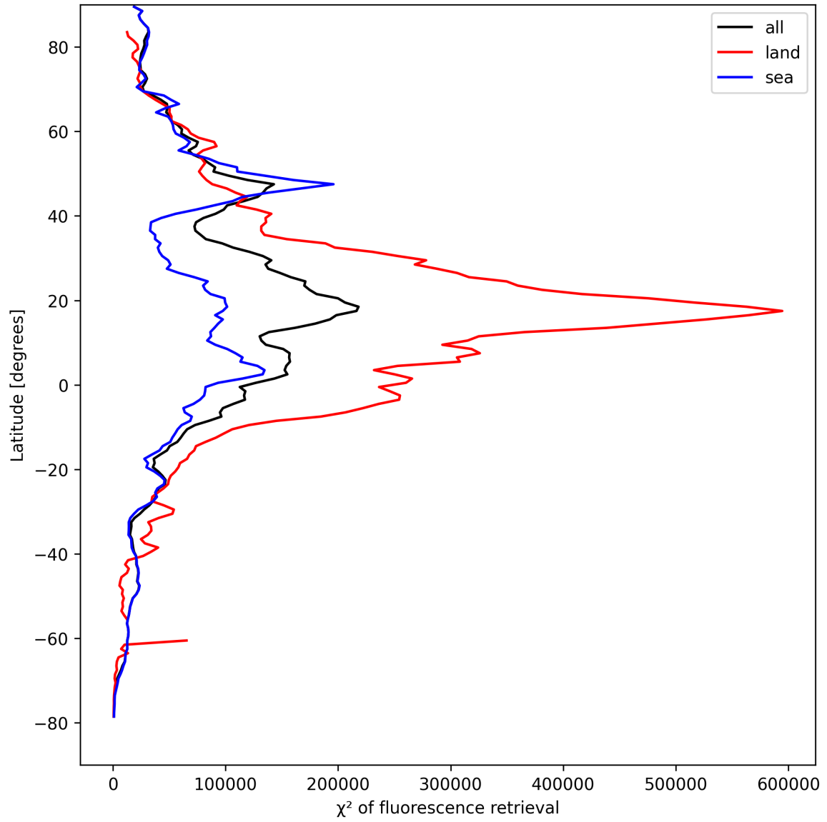
Figure 25: Zonal average of “ \chi^2 of fluorescence retrieval” for 2024-08-27 to 2024-08-29.
