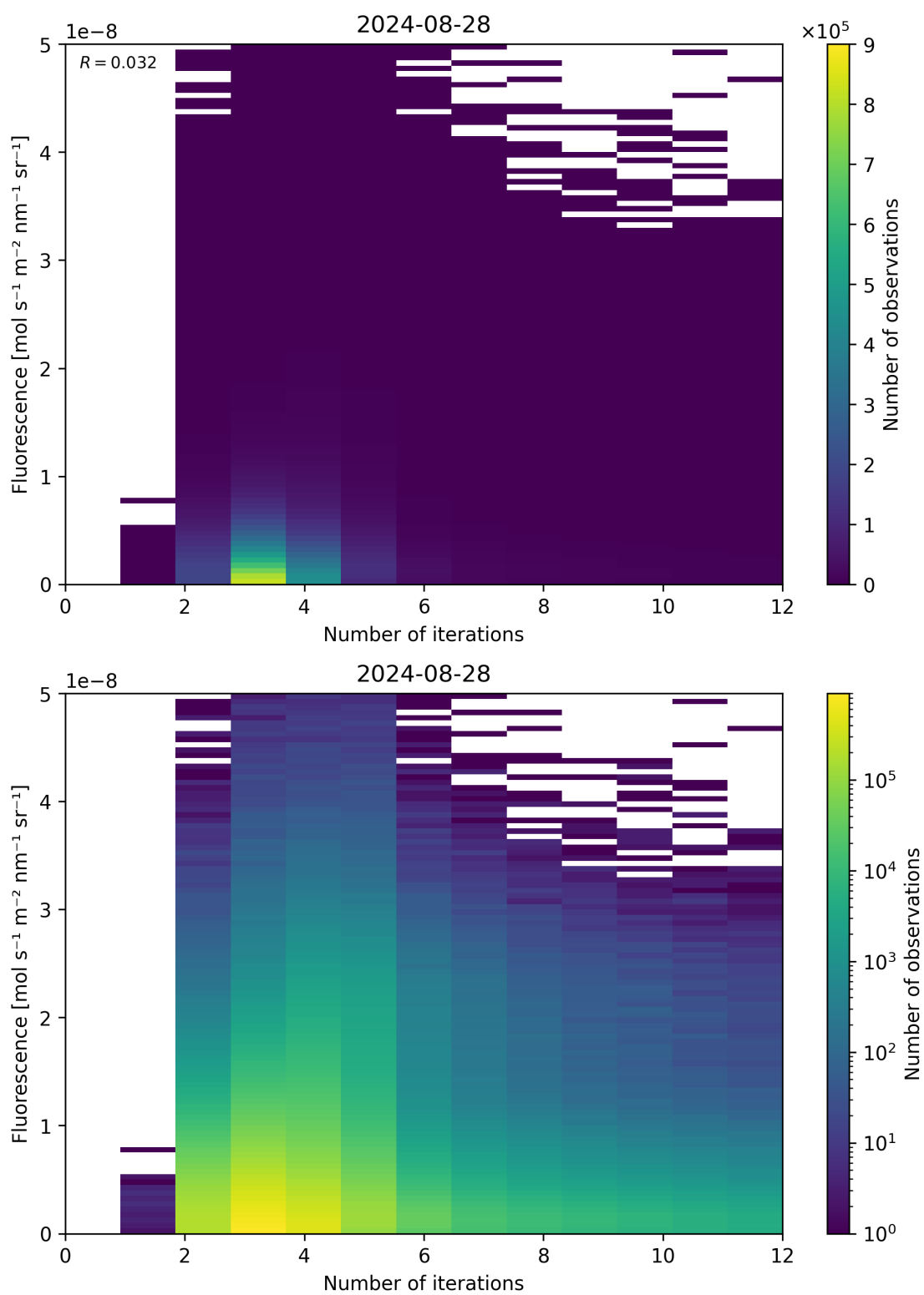
Figure 98: Scatter density plot of “Number of iterations” against “Fluorescence” for 2024-08-27 to 2024-08-29.
