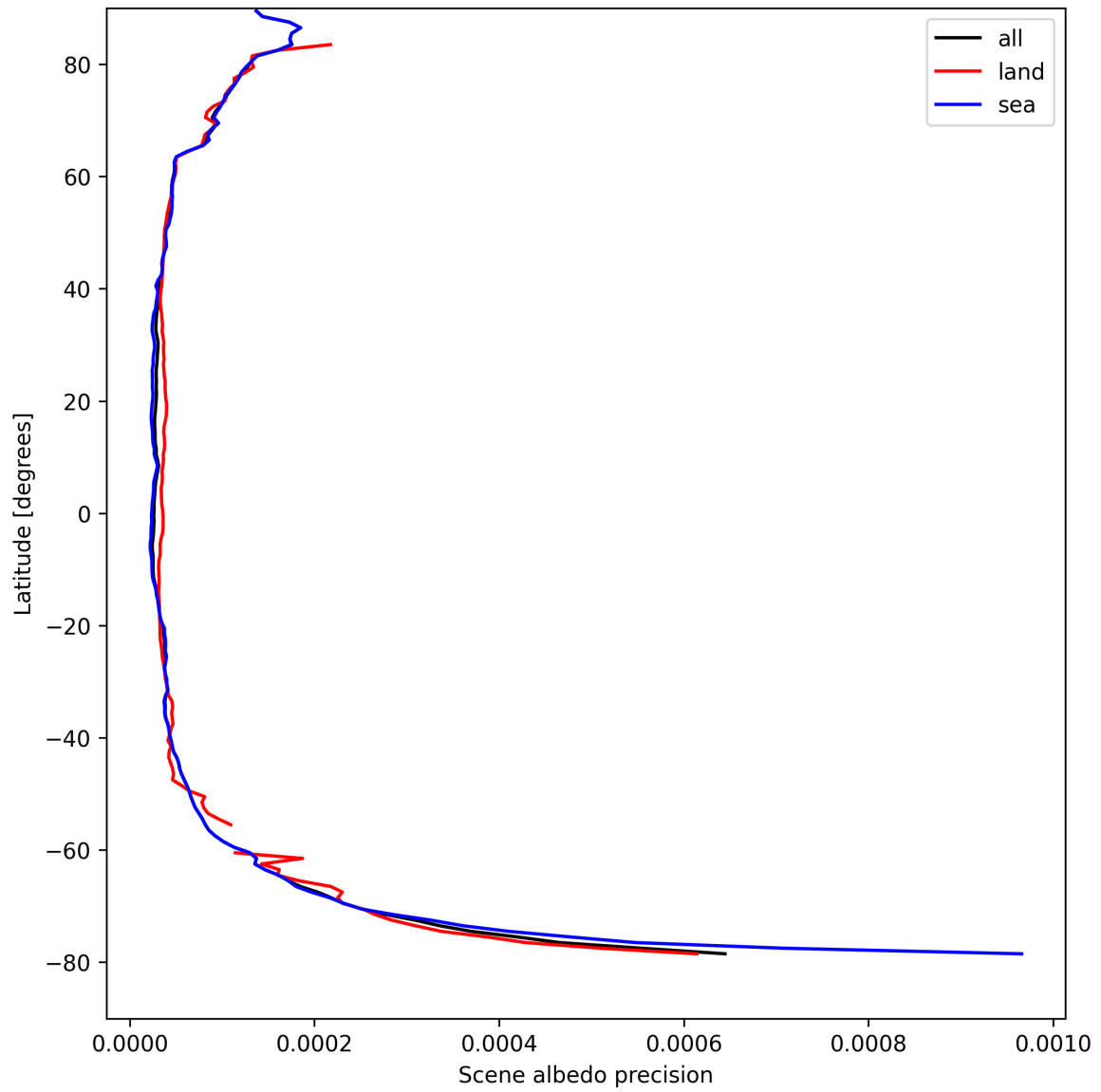
Figure 18: Zonal average of “Scene albedo precision” for 2024-08-27 to 2024-08-29.
