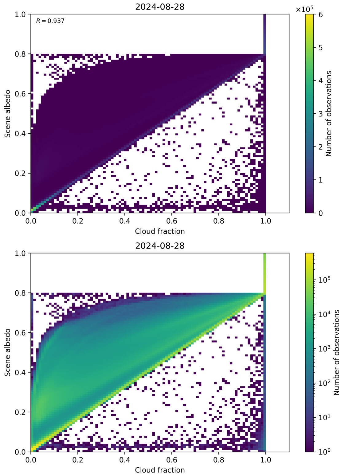
Figure 75: Scatter density plot of “Cloud fraction” against “Scene albedo” for 2024-08-27 to 2024-08-29.
