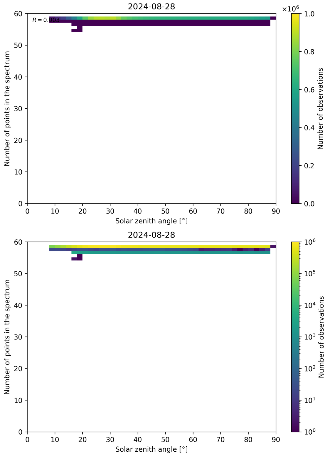
Figure 115: Scatter density plot of “Solar zenith angle” against “Number of points in the spectrum” for 2024-08-27 to 2024-08-29.
