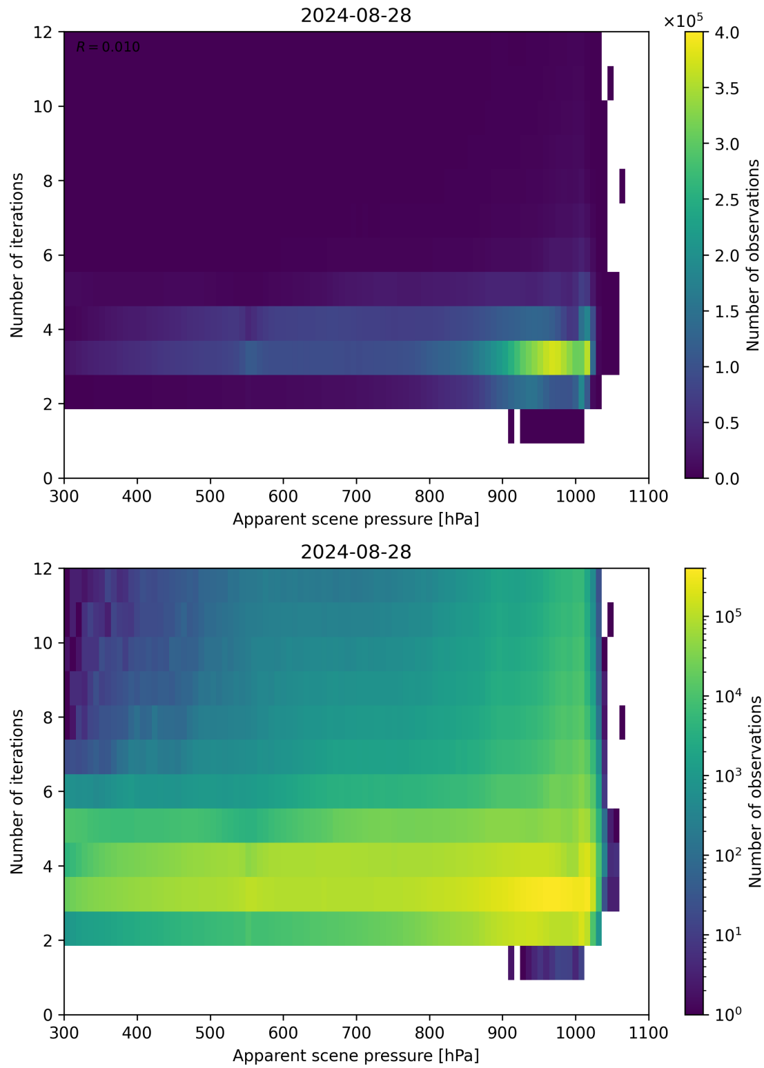
Figure 65: Scatter density plot of “Apparent scene pressure” against “Number of iterations” for 2024-08-27 to 2024-08-29.
