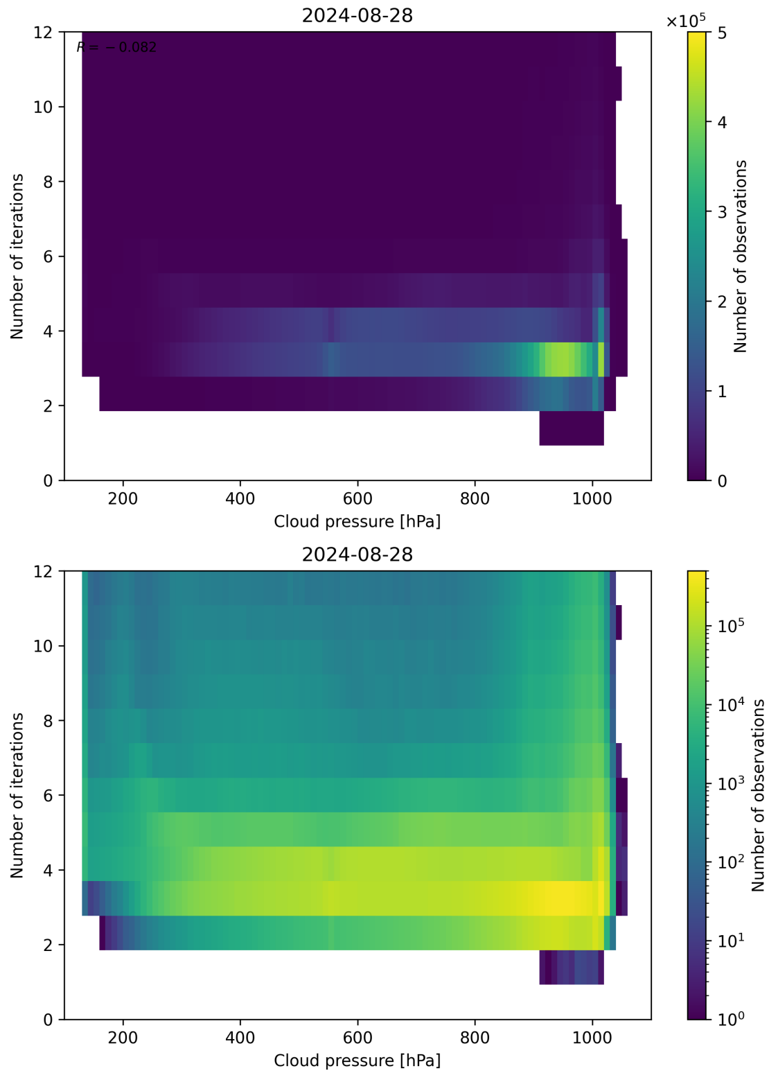
Figure 81: Scatter density plot of “Cloud pressure” against “Number of iterations” for 2024-08-27 to 2024-08-29.
