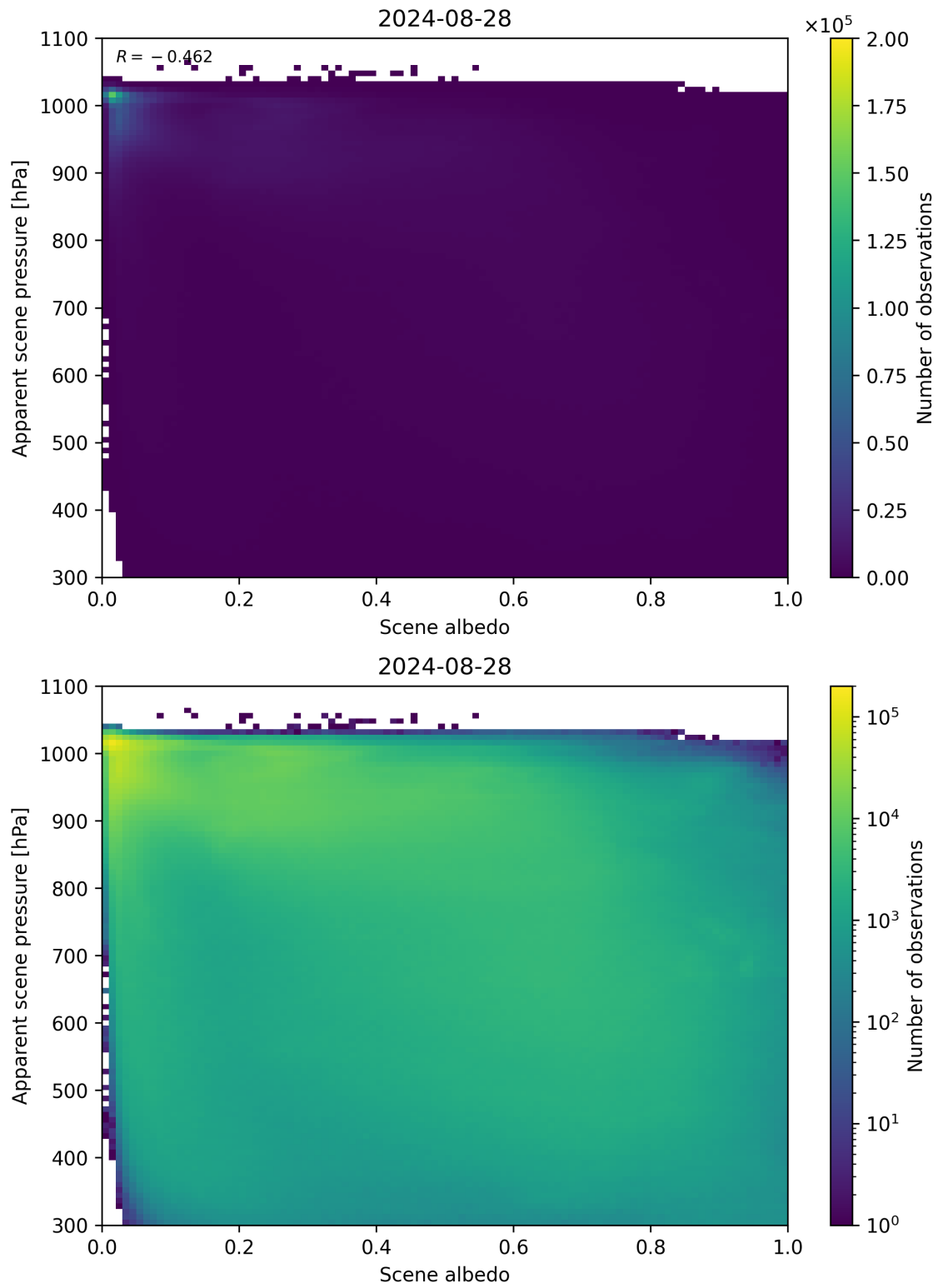
Figure 102: Scatter density plot of “Scene albedo” against “Apparent scene pressure” for 2024-08-27 to 2024-08-29.
