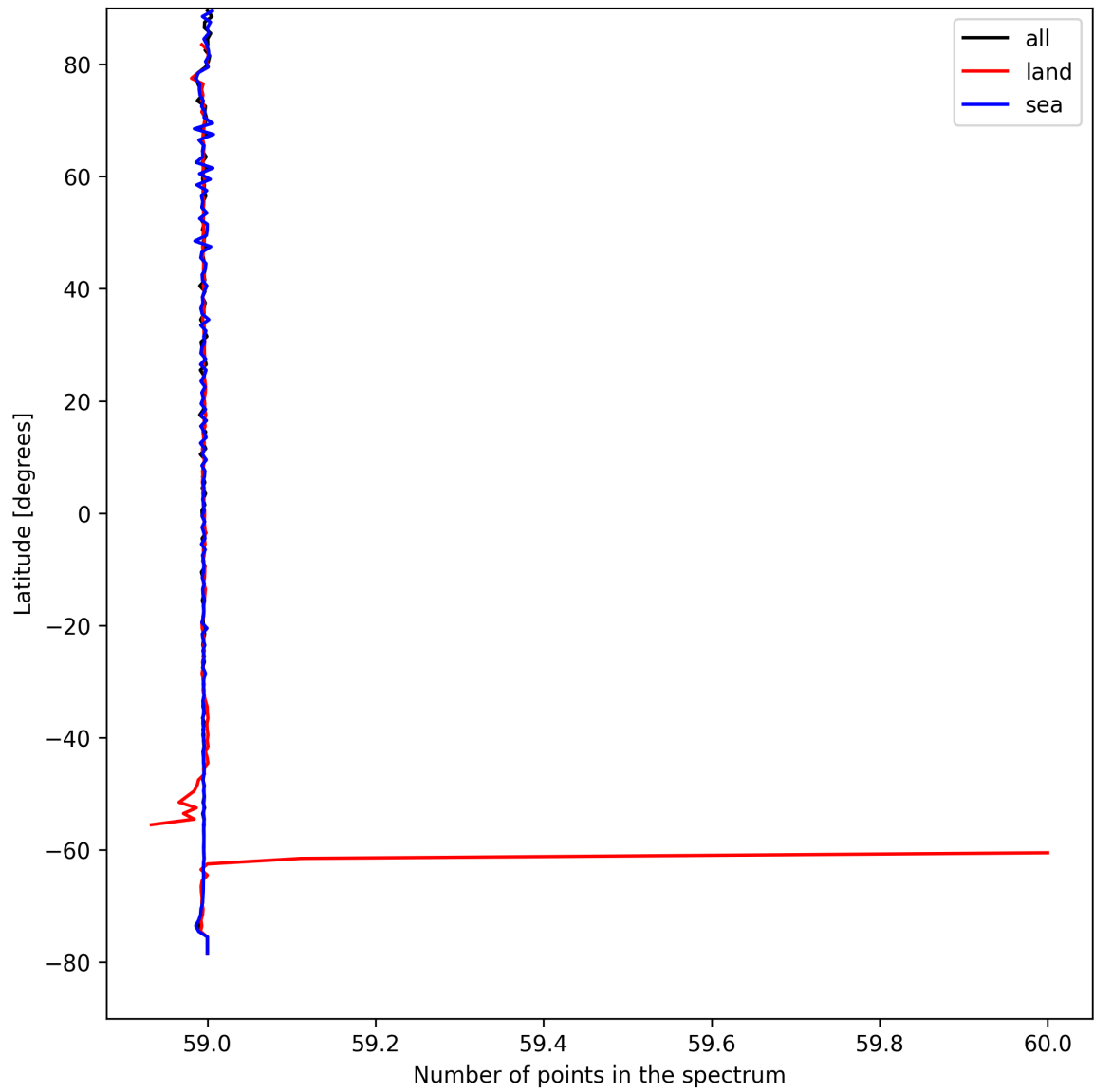
Figure 27: Zonal average of “Number of points in the spectrum” for 2024-08-27 to 2024-08-29.
