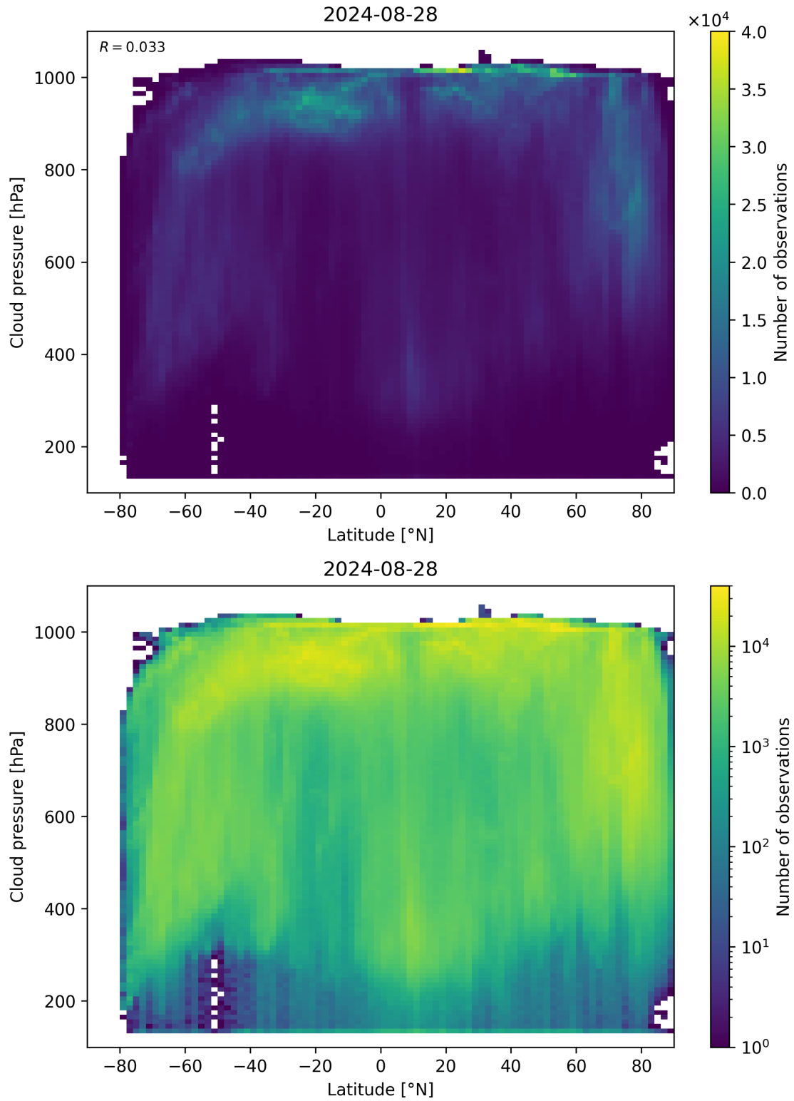
Figure 91: Scatter density plot of “Latitude” against “Cloud pressure” for 2024-08-27 to 2024-08-29.
