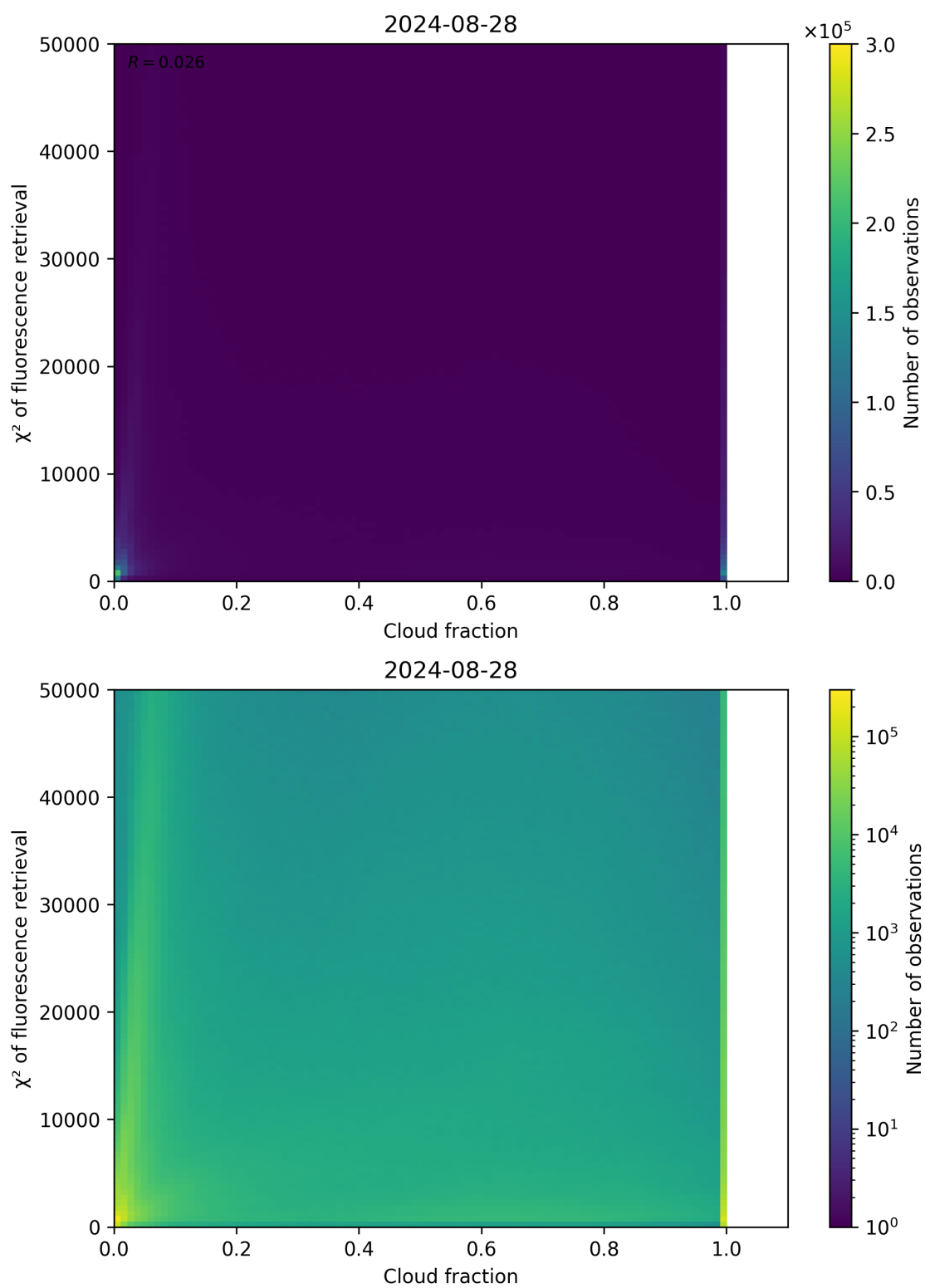
Figure 71: Scatter density plot of “Cloud fraction” against “ \chi^2 of fluorescence retrieval” for 2024-08-27 to 2024-08-29.
