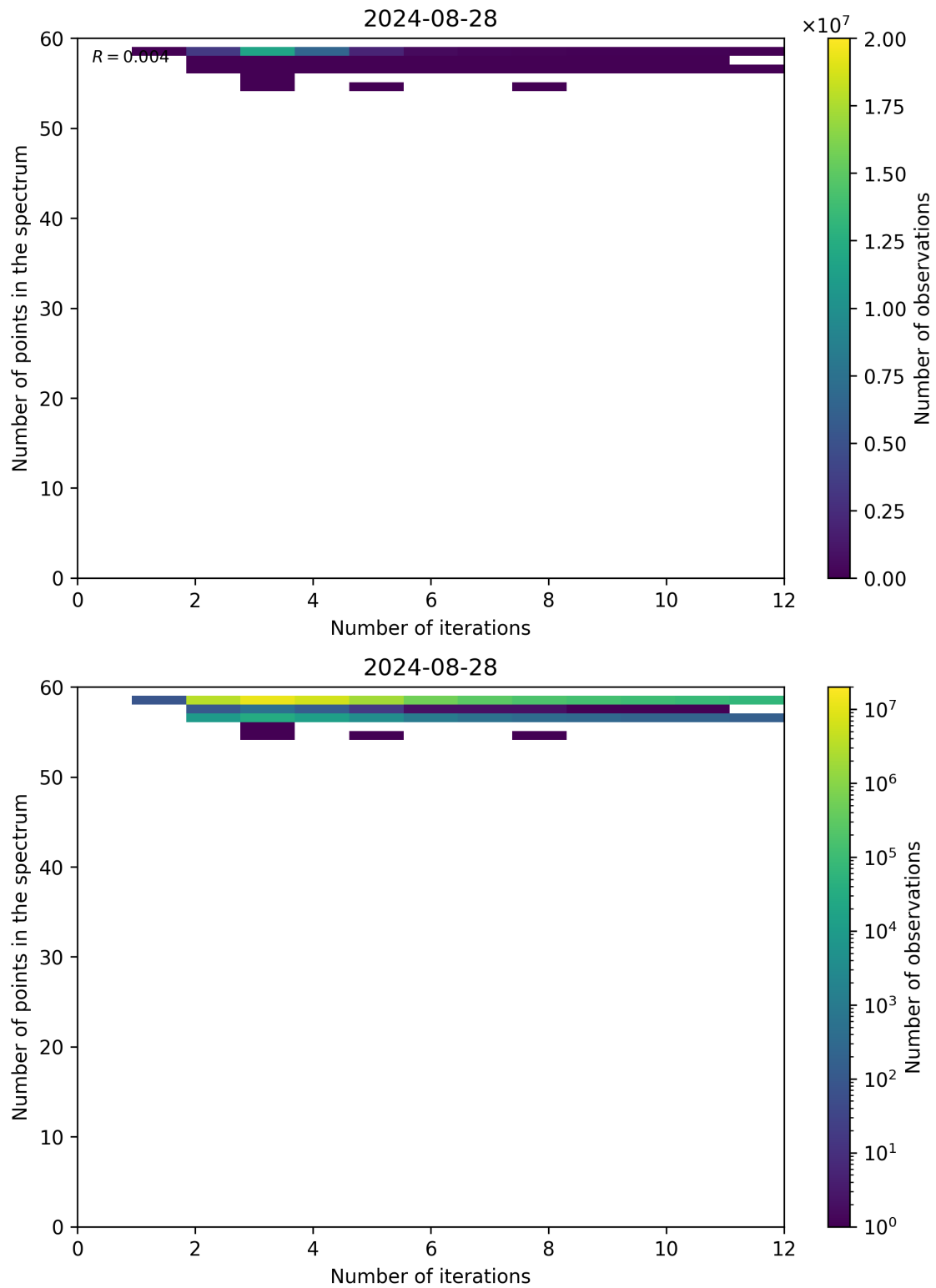
Figure 99: Scatter density plot of “Number of iterations” against “Number of points in the spectrum” for 2024-08-27 to 2024-08-29.
