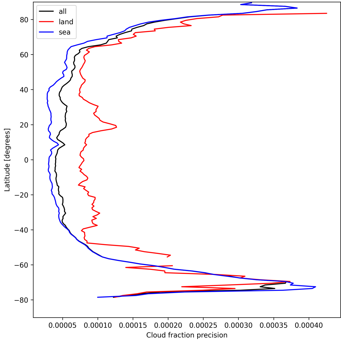
Figure 16: Zonal average of “Cloud fraction precision” for 2024-08-27 to 2024-08-29.
