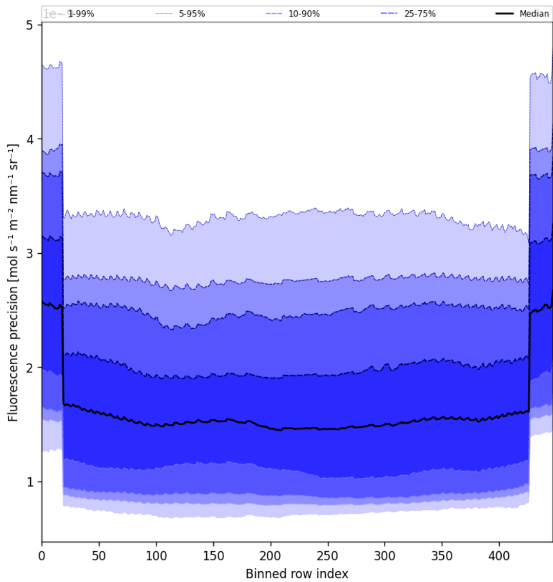
Figure 58: Along track statistics of “Fluorescence precision” for 2024-08-27 to 2024-08-29
