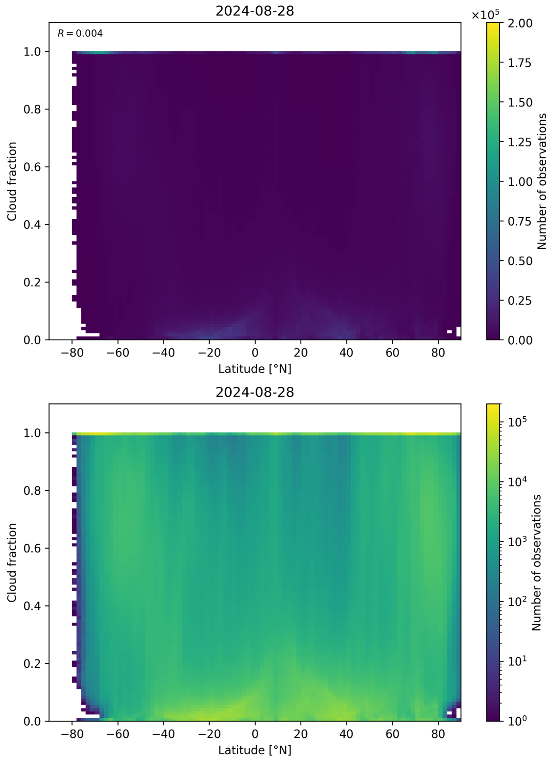
Figure 90: Scatter density plot of “Latitude” against “Cloud fraction” for 2024-08-27 to 2024-08-29.
