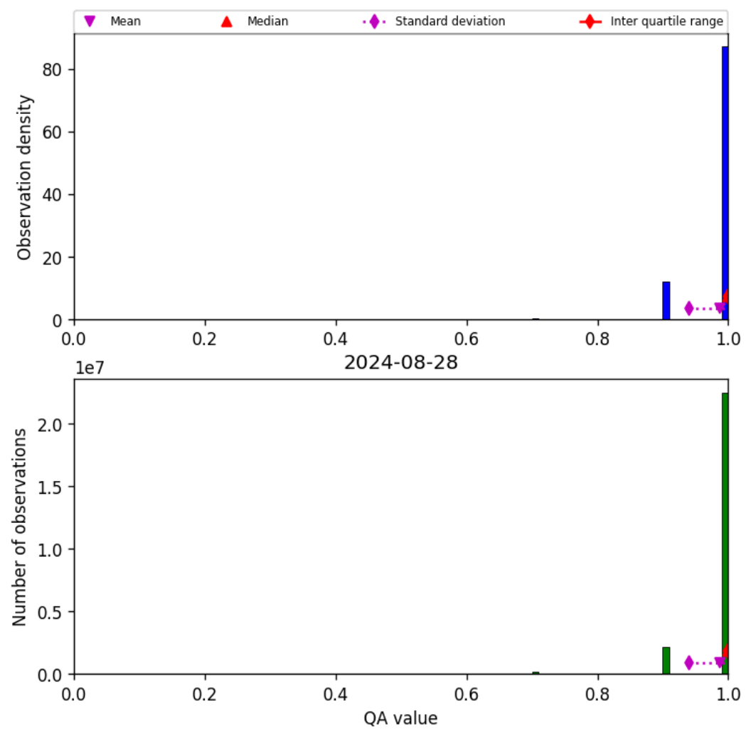
Figure 29: Histogram of “QA value” for 2024-08-27 to 2024-08-29
