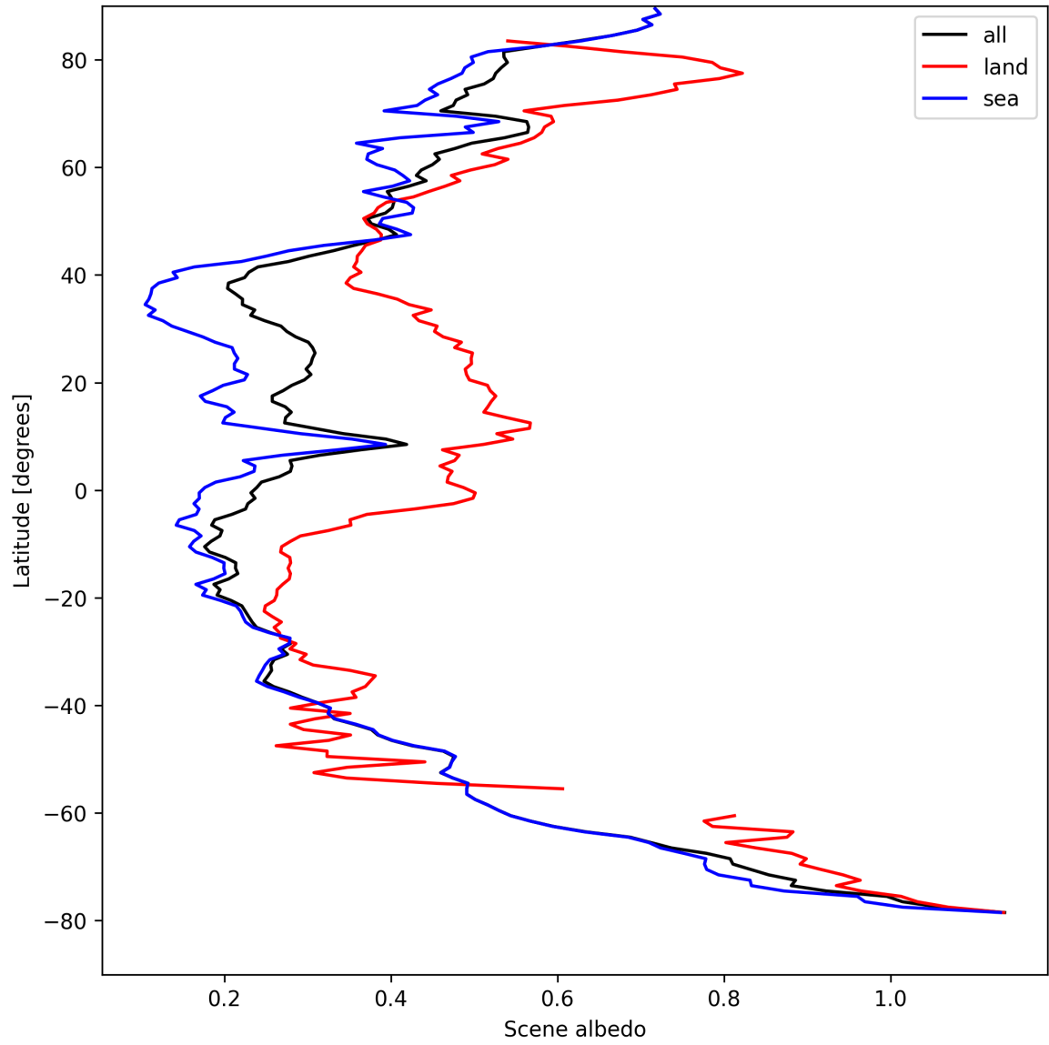
Figure 17: Zonal average of “Scene albedo” for 2024-08-27 to 2024-08-29.
