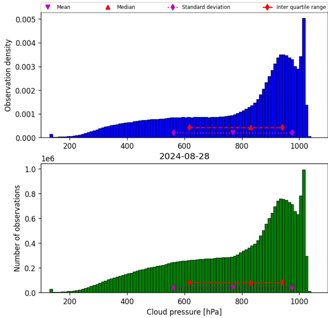
Figure 30: Histogram of “Cloud pressure” for 2024-08-27 to 2024-08-29
