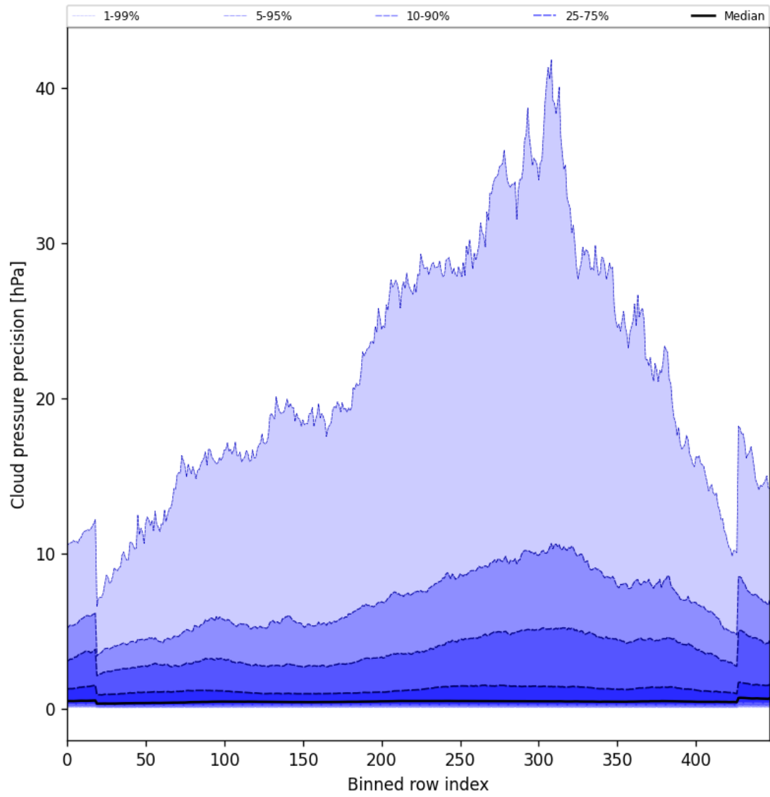
Figure 48: Along track statistics of “Cloud pressure precision” for 2024-08-27 to 2024-08-29
