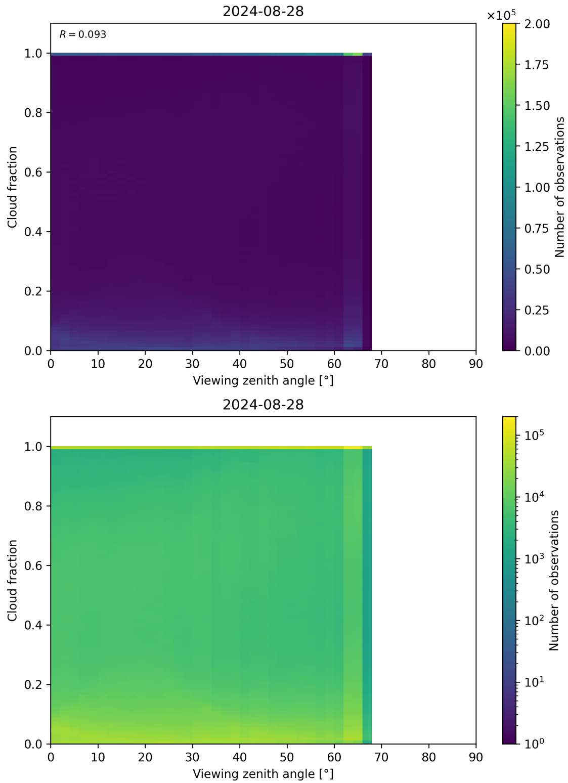
Figure 120: Scatter density plot of “Viewing zenith angle” against “Cloud fraction” for 2024-08-27 to 2024-08-29.
