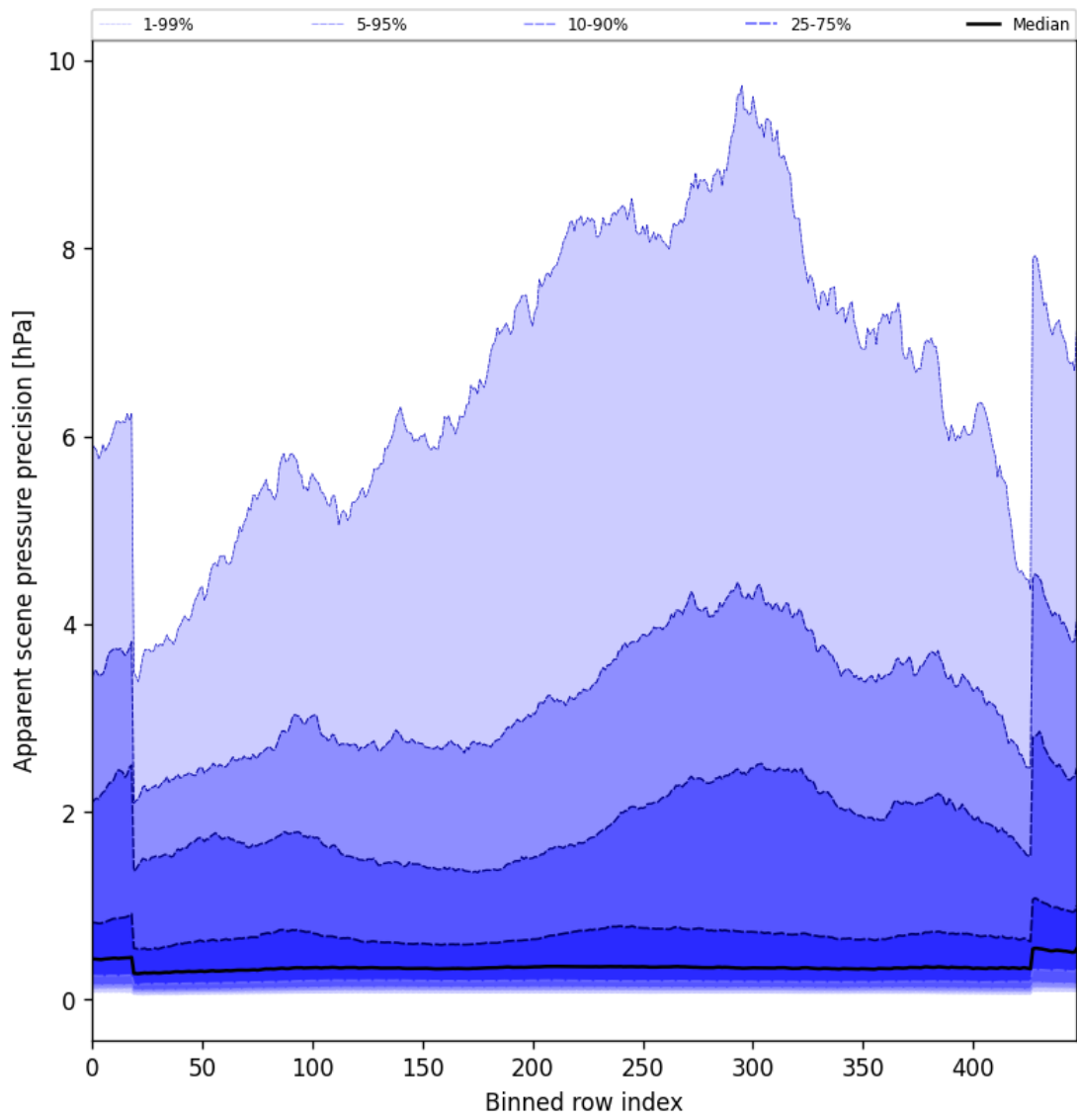
Figure 54: Along track statistics of “Apparent scene pressure precision” for 2024-08-27 to 2024-08-29
