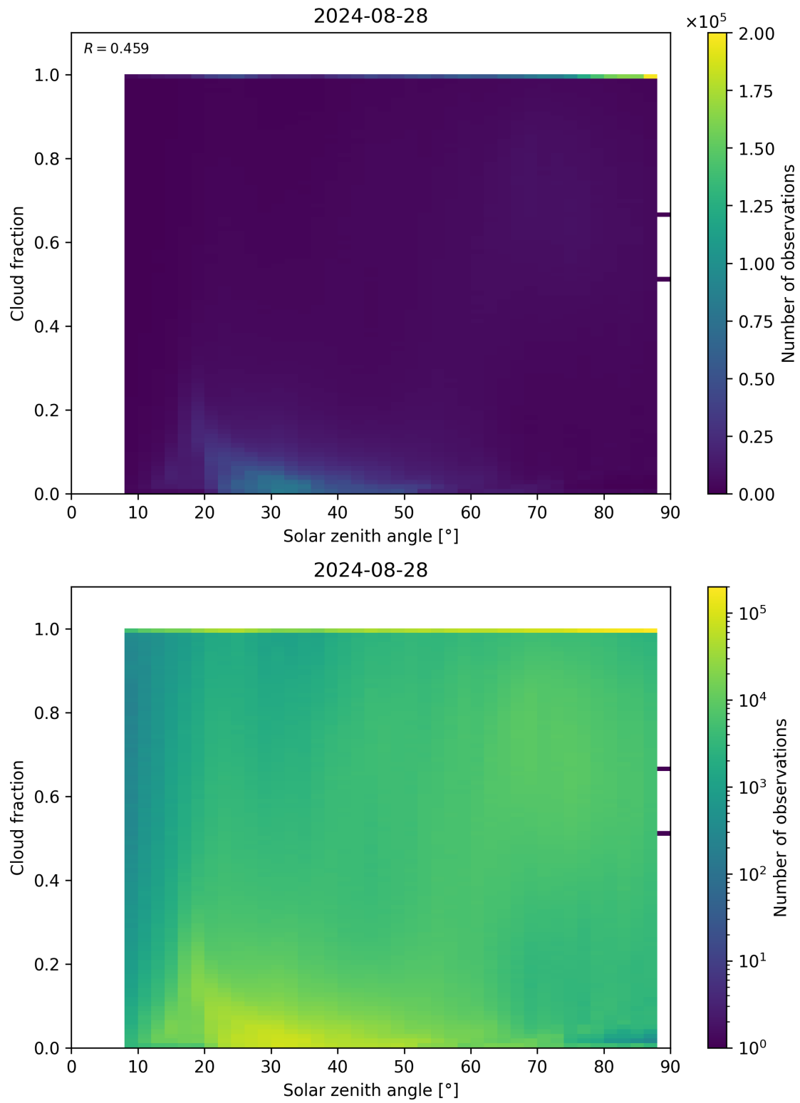
Figure 110: Scatter density plot of “Solar zenith angle” against “Cloud fraction” for 2024-08-27 to 2024-08-29.
