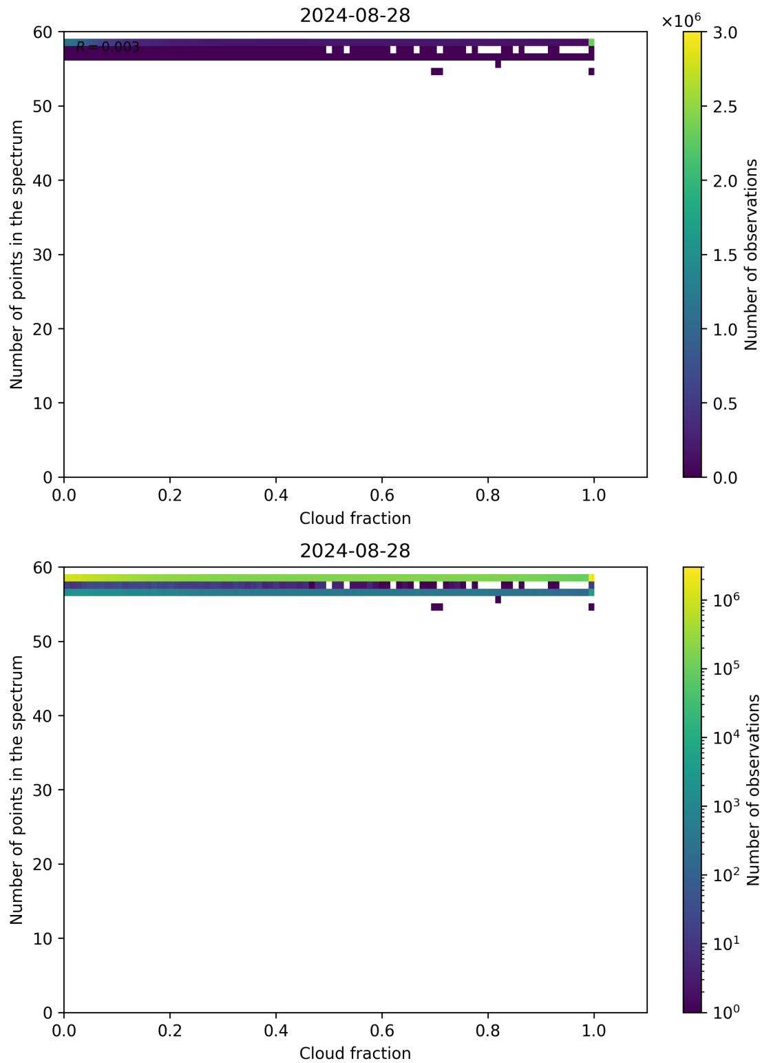
Figure 74: Scatter density plot of “Cloud fraction” against “Number of points in the spectrum” for 2024-08-27 to 2024-08-29.
