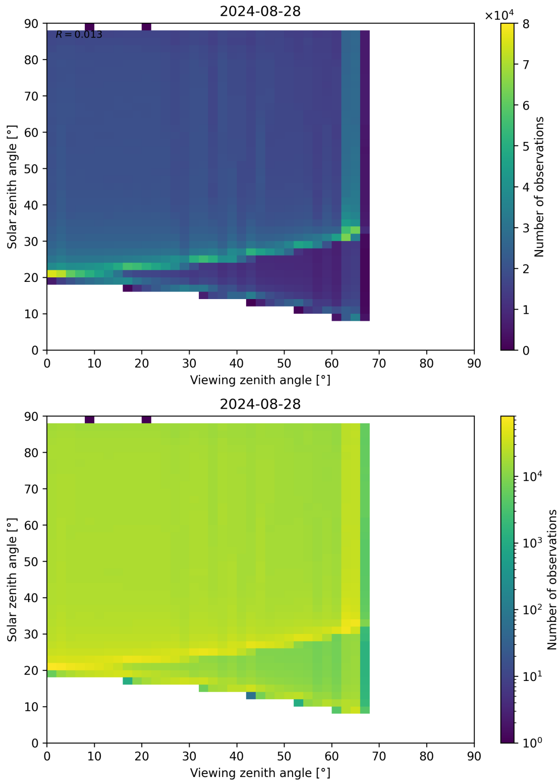
Figure 127: Scatter density plot of “Viewing zenith angle” against “Solar zenith angle” for 2024-08-27 to 2024-08-29.
