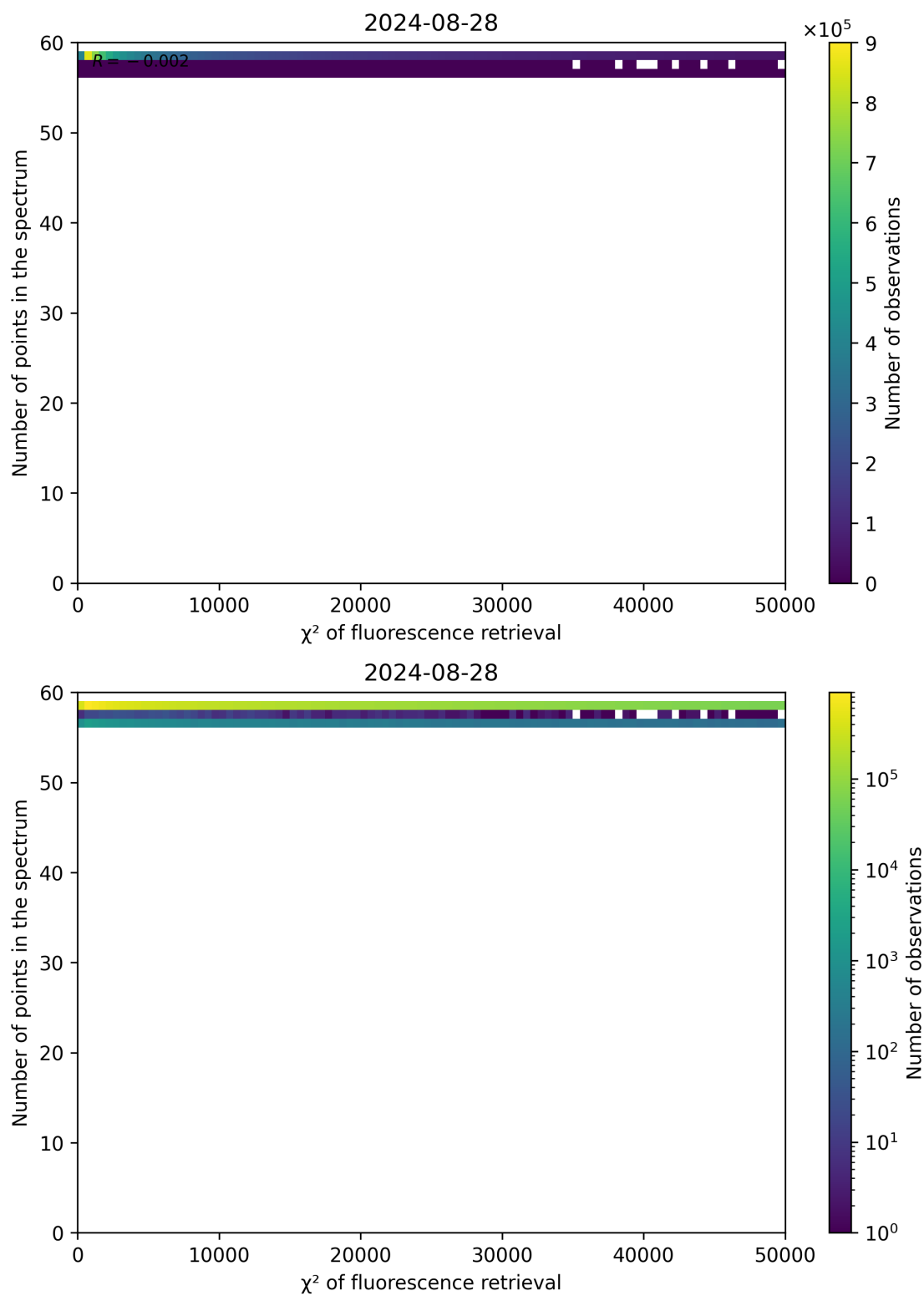
Figure 68: Scatter density plot of " \chi^2 of fluorescence retrieval" against "Number of points in the spectrum" for 2024-08-27 to 2024-08-29.
