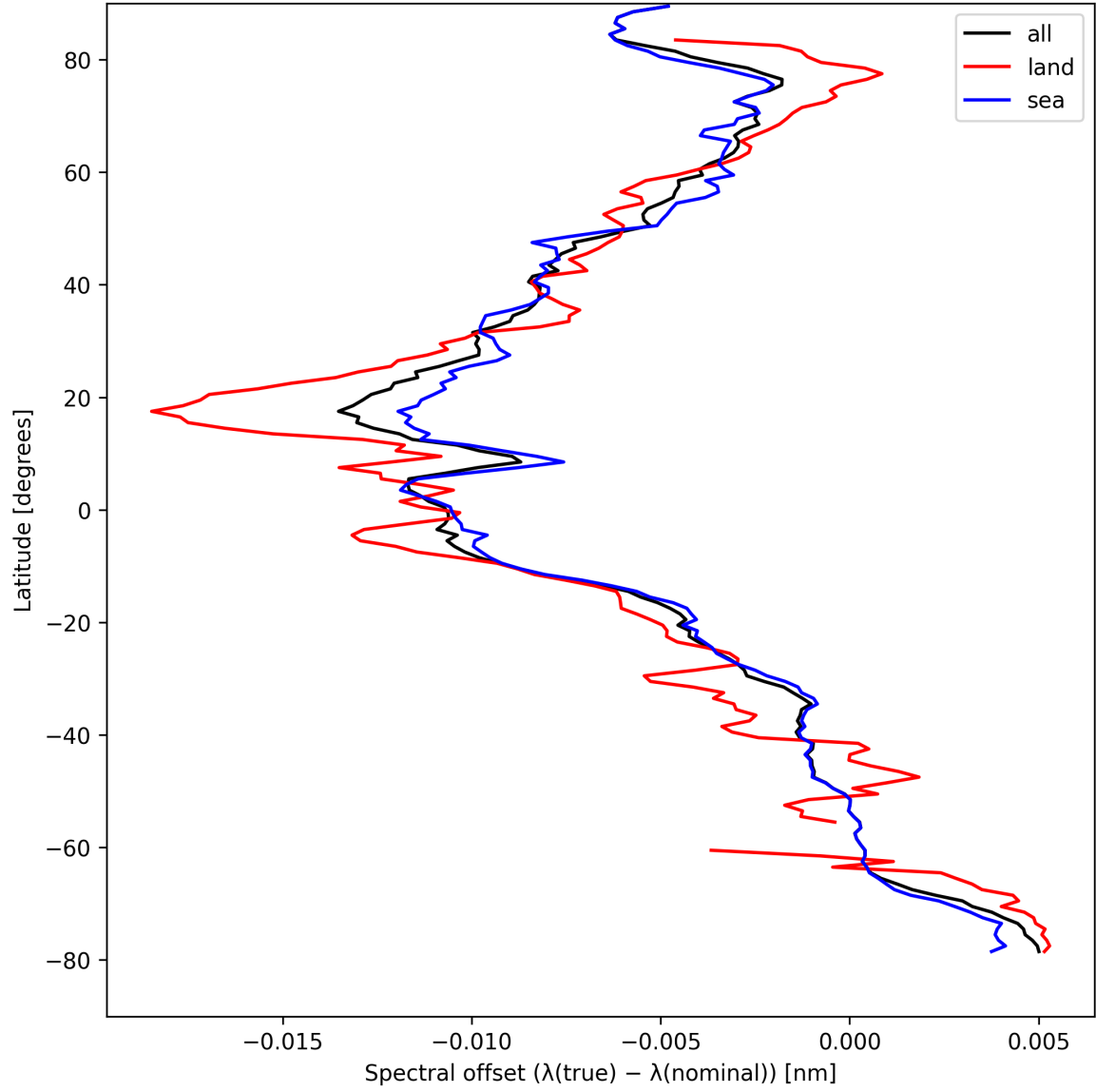
Figure 28: Zonal average of “Spectral offset ( \lambda_{\text{true}} - \lambda_{\text{nominal}} )” for 2024-08-27 to 2024-08-29.
