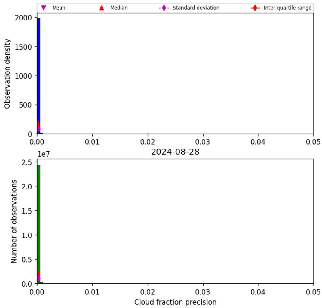
Figure 33: Histogram of “Cloud fraction precision” for 2024-08-27 to 2024-08-29
