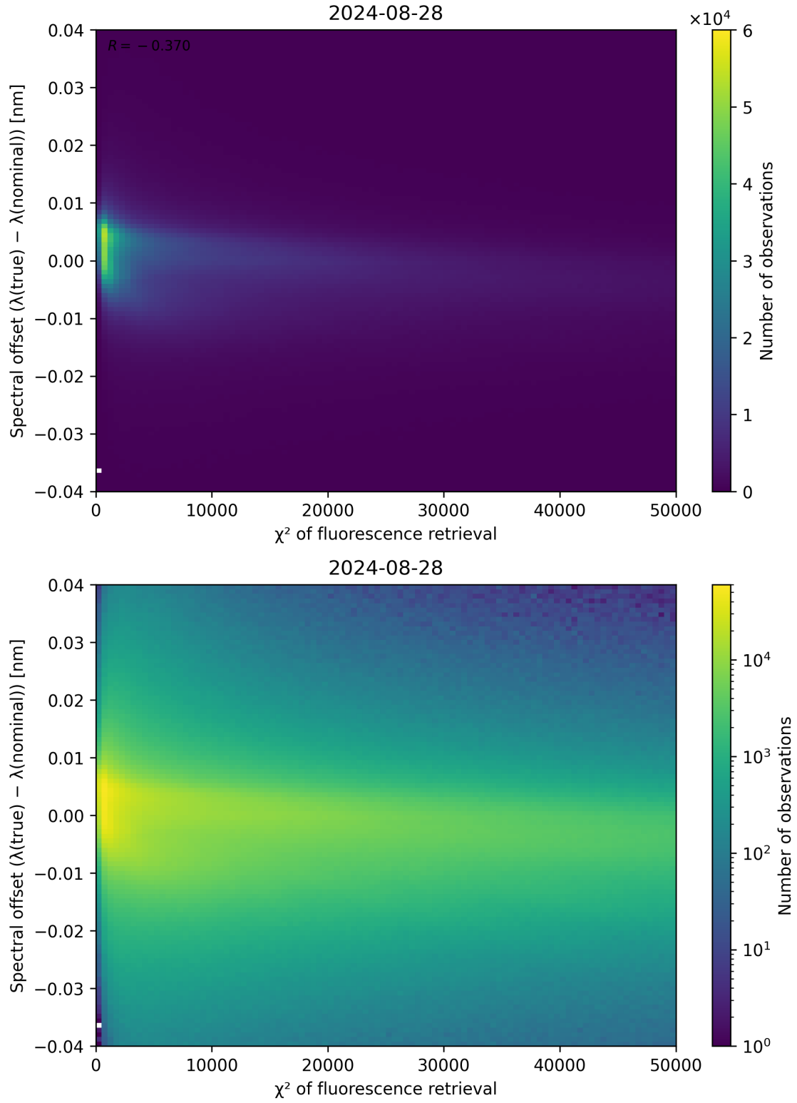
Figure 69: Scatter density plot of “ \chi^2 of fluorescence retrieval” against “Spectral offset ( \lambda_{\text{true}} - \lambda_{\text{nominal}} )” for 2024-08-27 to 2024-08-29.
