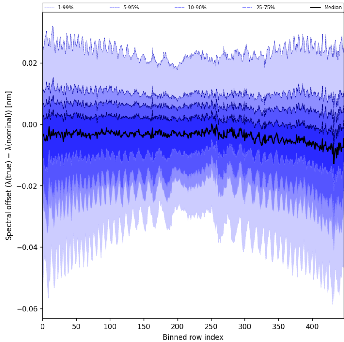
Figure 62: Along track statistics of “Spectral offset ( \lambda_{\text{true}} - \lambda_{\text{nominal}} )” for 2024-08-27 to 2024-08-29
