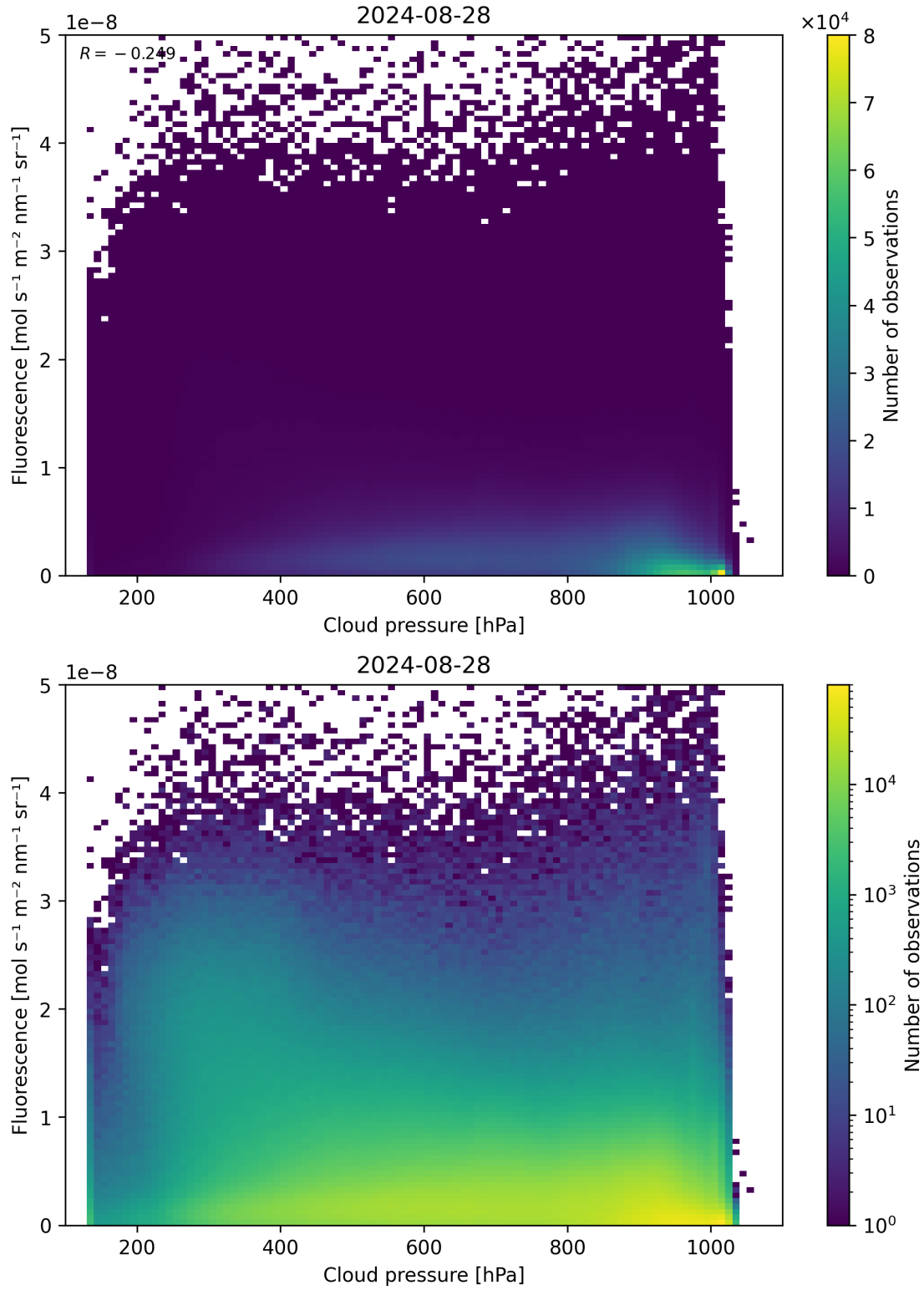
Figure 80: Scatter density plot of “Cloud pressure” against “Fluorescence” for 2024-08-27 to 2024-08-29.
