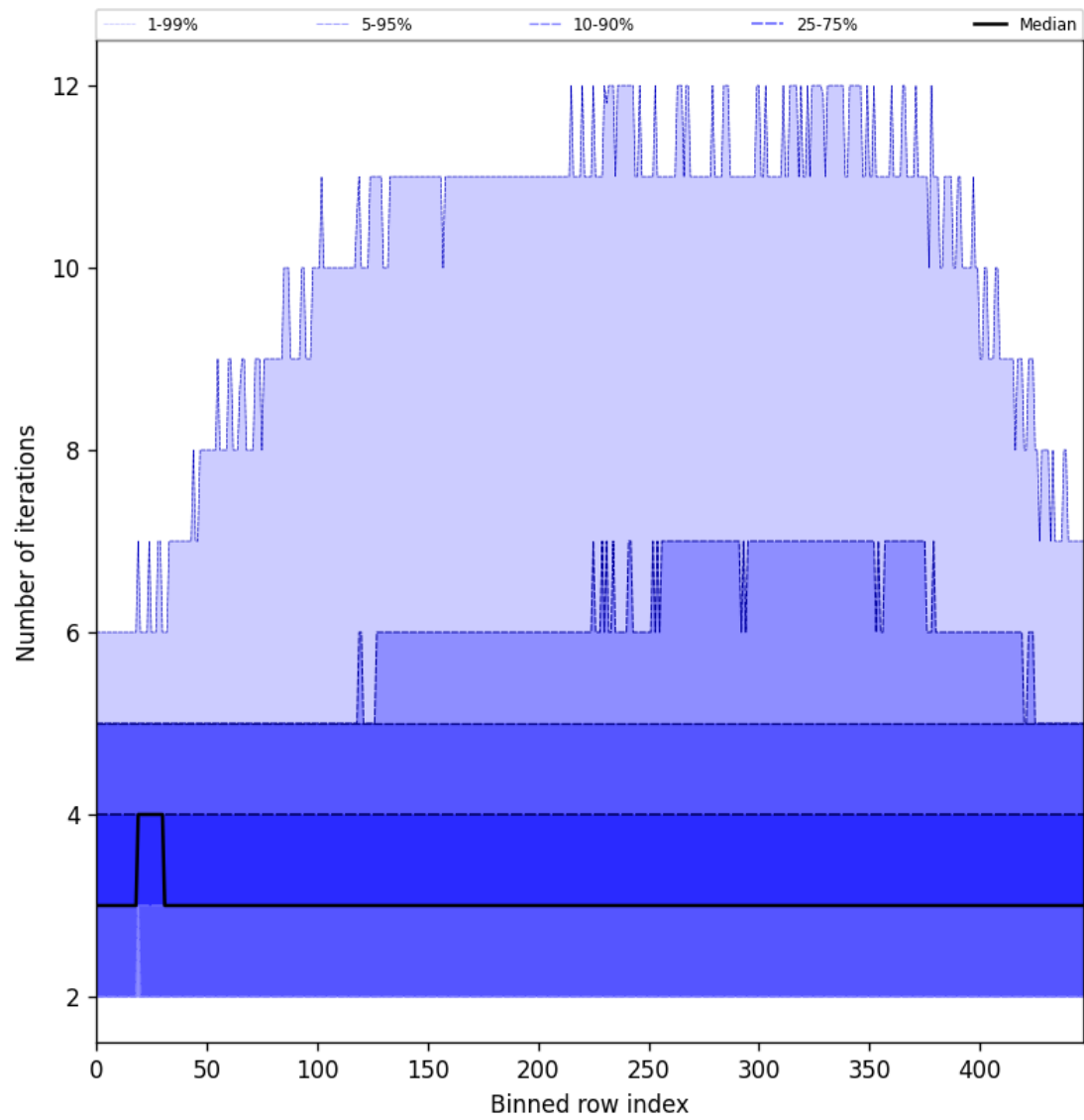
Figure 56: Along track statistics of “Number of iterations” for 2024-08-27 to 2024-08-29
