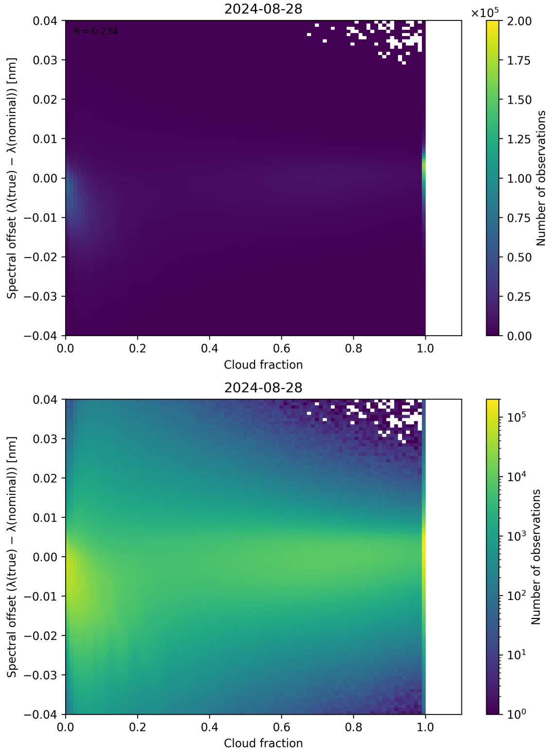
Figure 76: Scatter density plot of “Cloud fraction” against “Spectral offset ( \lambda_{\text{true}} - \lambda_{\text{nominal}} )” for 2024-08-27 to 2024-08-29.
