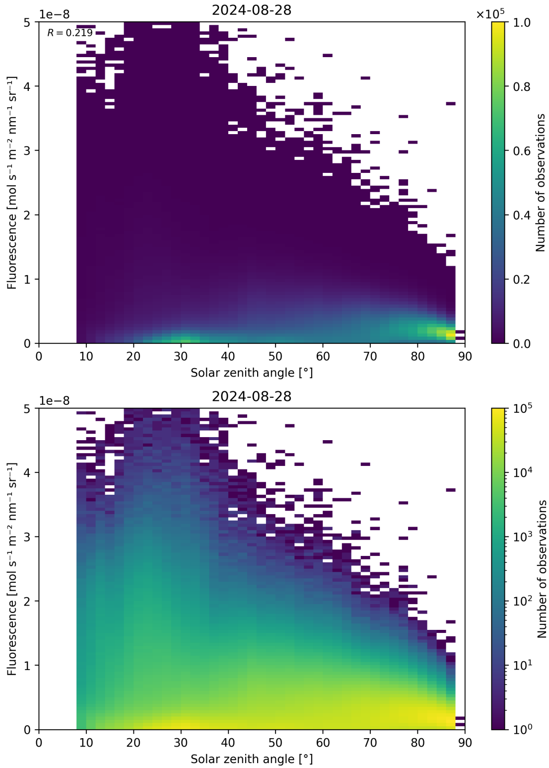
Figure 112: Scatter density plot of “Solar zenith angle” against “Fluorescence” for 2024-08-27 to 2024-08-29.
