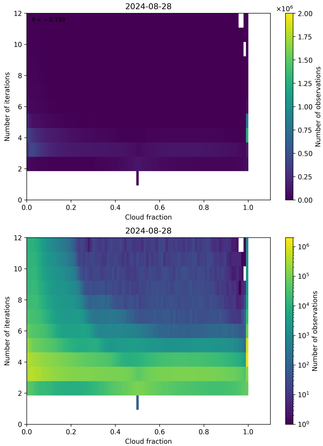
Figure 73: Scatter density plot of “Cloud fraction” against “Number of iterations” for 2024-08-27 to 2024-08-29.
