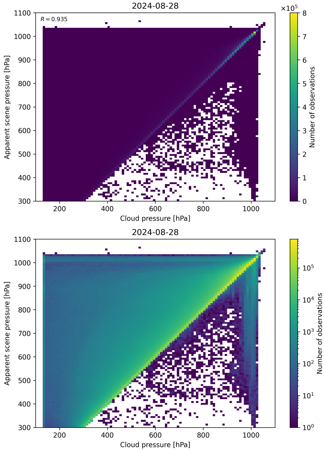
Figure 77: Scatter density plot of “Cloud pressure” against “Apparent scene pressure” for 2024-08-27 to 2024-08-29.
