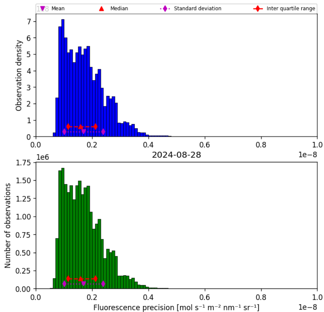
Figure 41: Histogram of “Fluorescence precision” for 2024-08-27 to 2024-08-29
