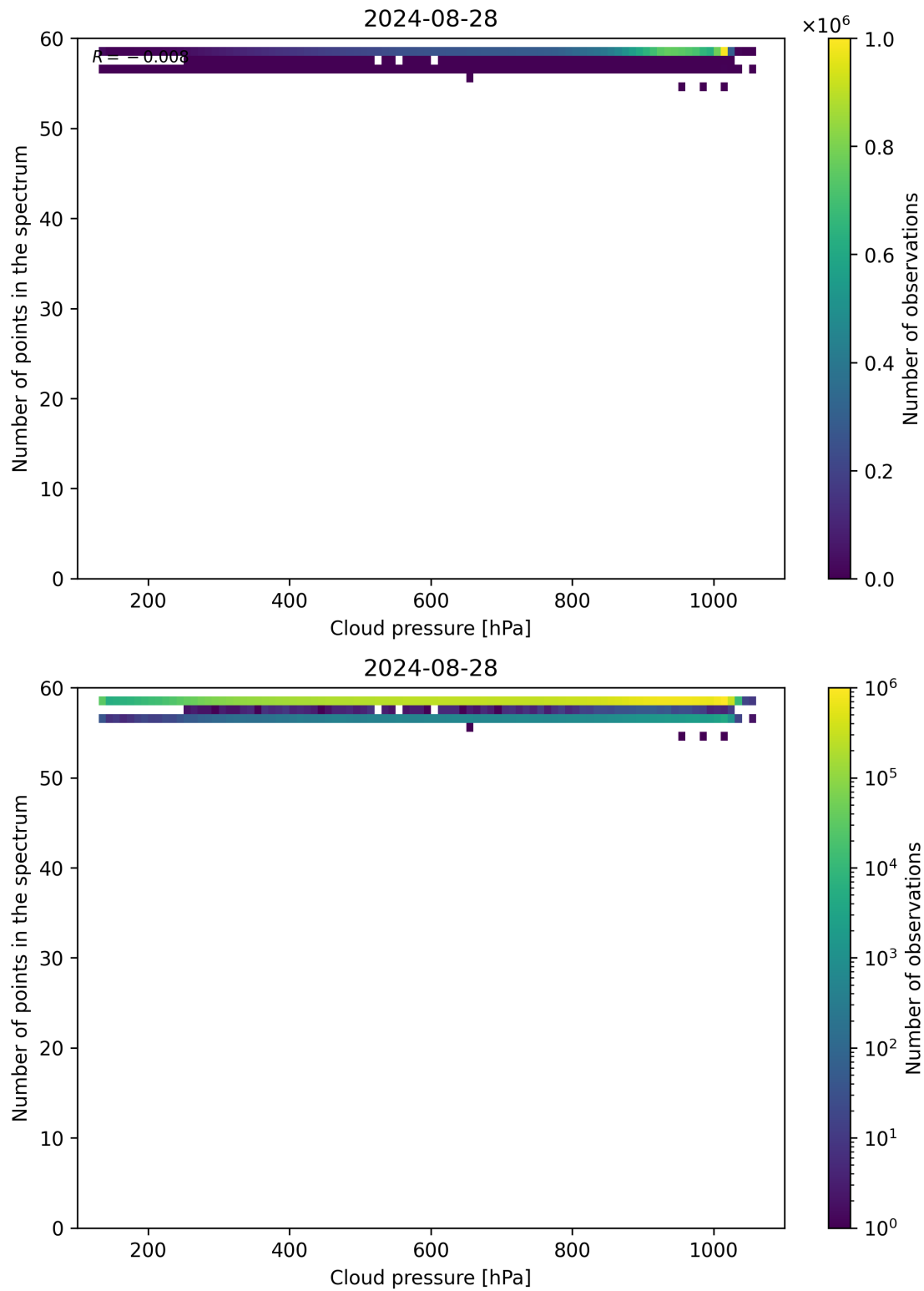
Figure 82: Scatter density plot of “Cloud pressure” against “Number of points in the spectrum” for 2024-08-27 to 2024-08-29.
