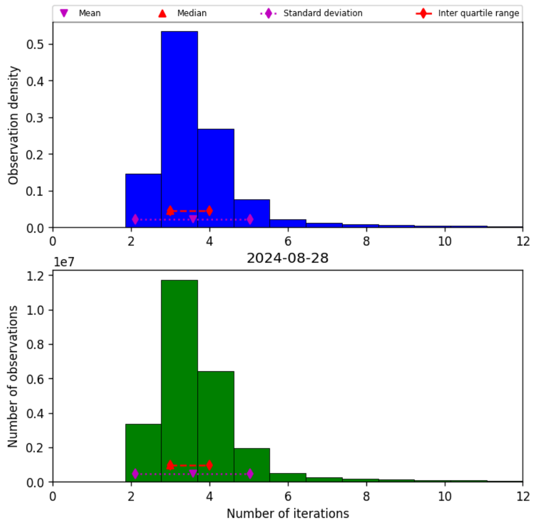
Figure 39: Histogram of “Number of iterations” for 2024-08-27 to 2024-08-29
