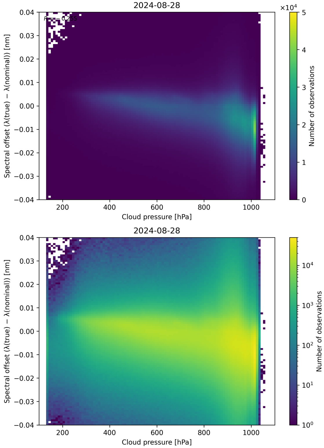
Figure 84: Scatter density plot of “Cloud pressure” against “Spectral offset ( \lambda_{\text{true}} - \lambda_{\text{nominal}} )” for 2024-08-27 to 2024-08-29.
