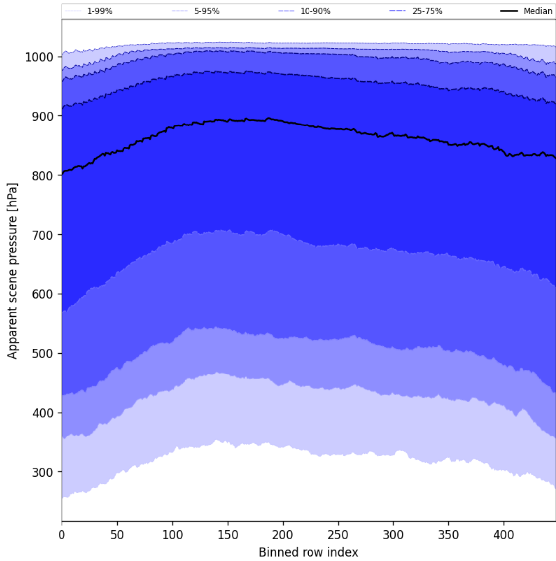
Figure 53: Along track statistics of “Apparent scene pressure” for 2024-08-27 to 2024-08-29
