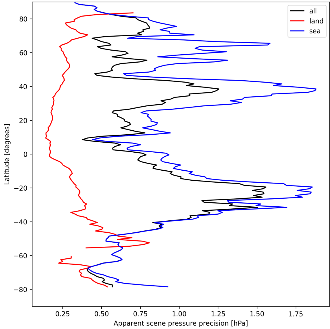
Figure 20: Zonal average of “Apparent scene pressure precision” for 2024-08-27 to 2024-08-29.
