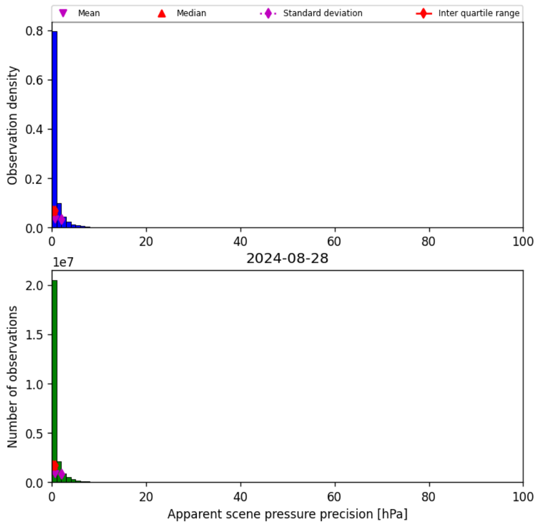
Figure 37: Histogram of “Apparent scene pressure precision” for 2024-08-27 to 2024-08-29
