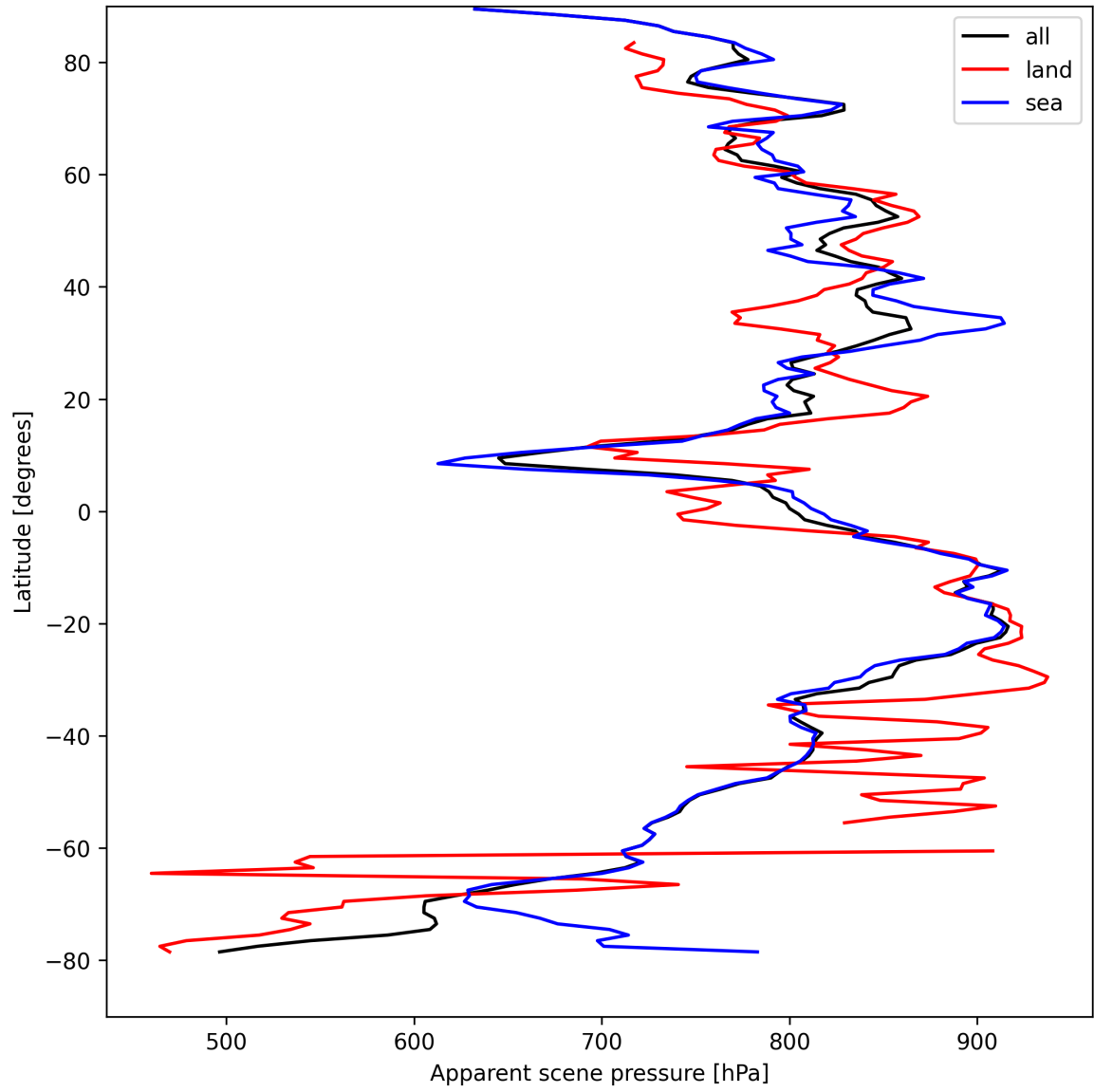
Figure 19: Zonal average of “Apparent scene pressure” for 2024-08-27 to 2024-08-29.
