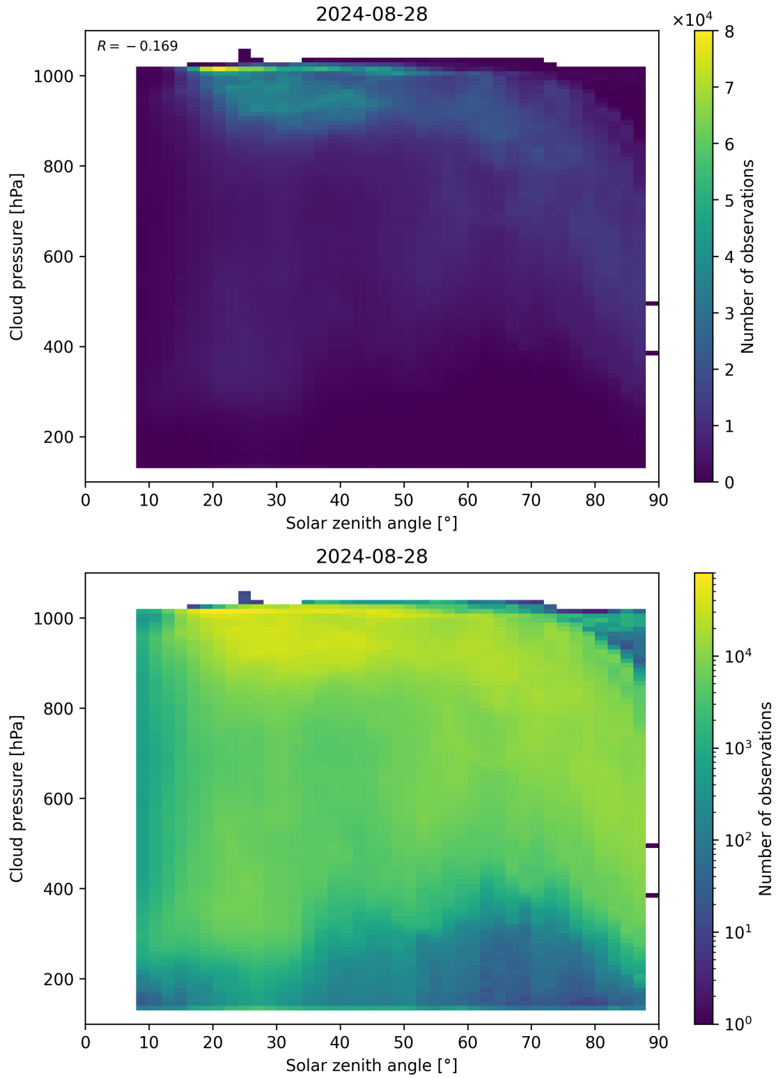
Figure 111: Scatter density plot of “Solar zenith angle” against “Cloud pressure” for 2024-08-27 to 2024-08-29.
