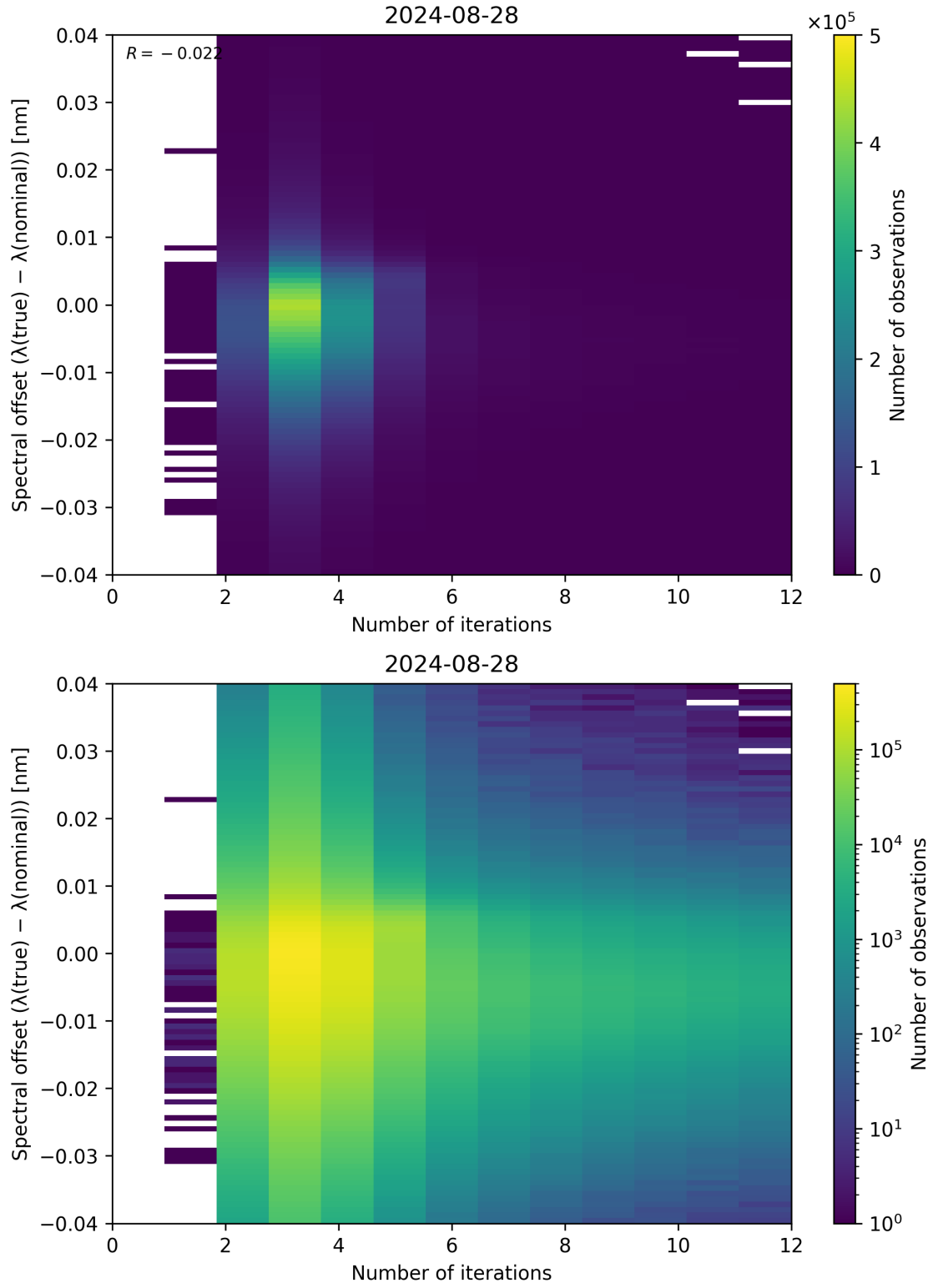
Figure 100: Scatter density plot of “Number of iterations” against “Spectral offset ( \lambda_{\text{true}} - \lambda_{\text{nominal}} )” for 2024-08-27 to 2024-08-29.
