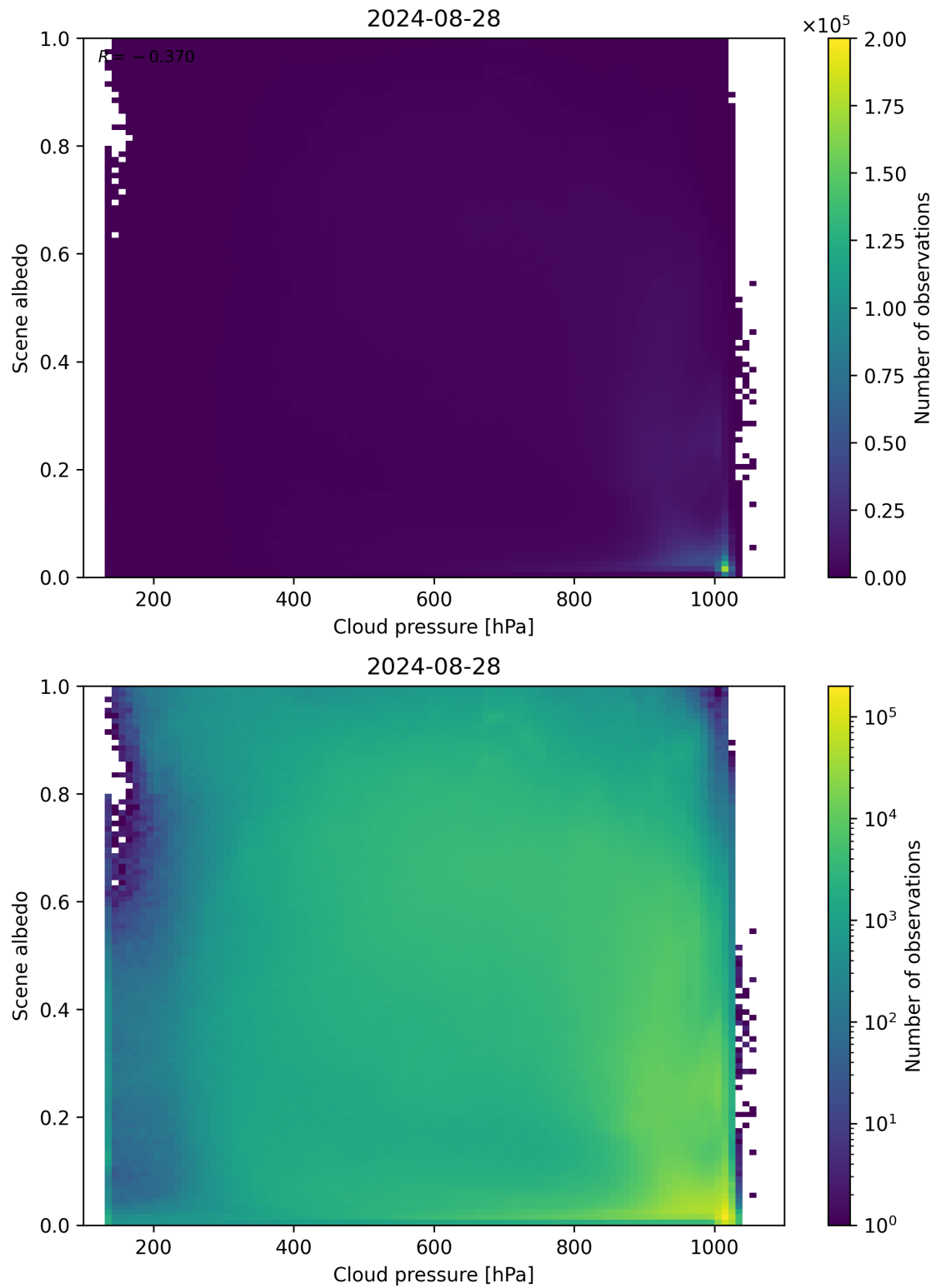
Figure 83: Scatter density plot of “Cloud pressure” against “Scene albedo” for 2024-08-27 to 2024-08-29.
