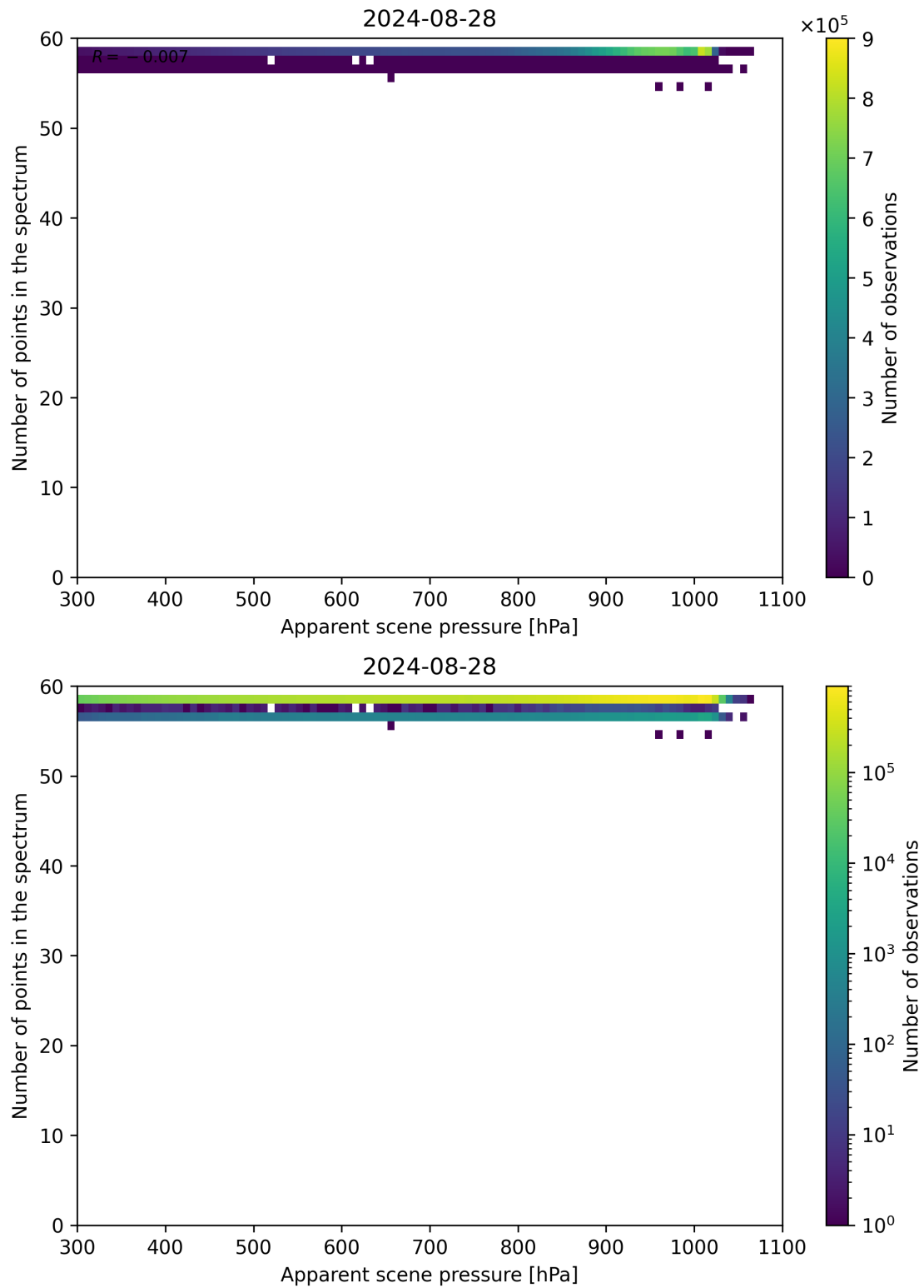
Figure 66: Scatter density plot of “Apparent scene pressure” against “Number of points in the spectrum” for 2024-08-27 to 2024-08-29.
