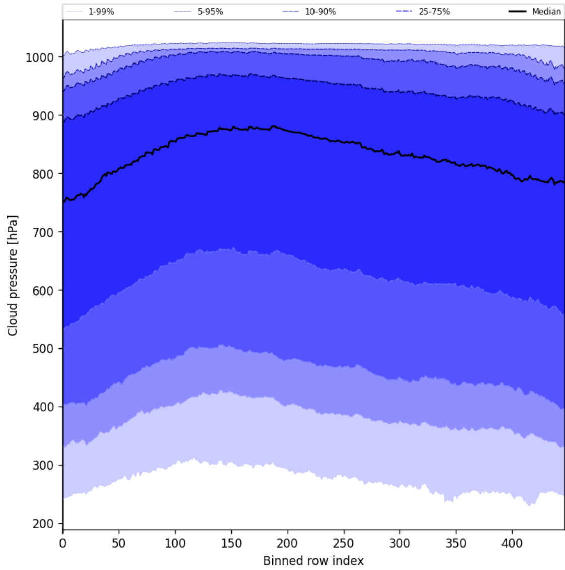
Figure 47: Along track statistics of “Cloud pressure” for 2024-08-27 to 2024-08-29
