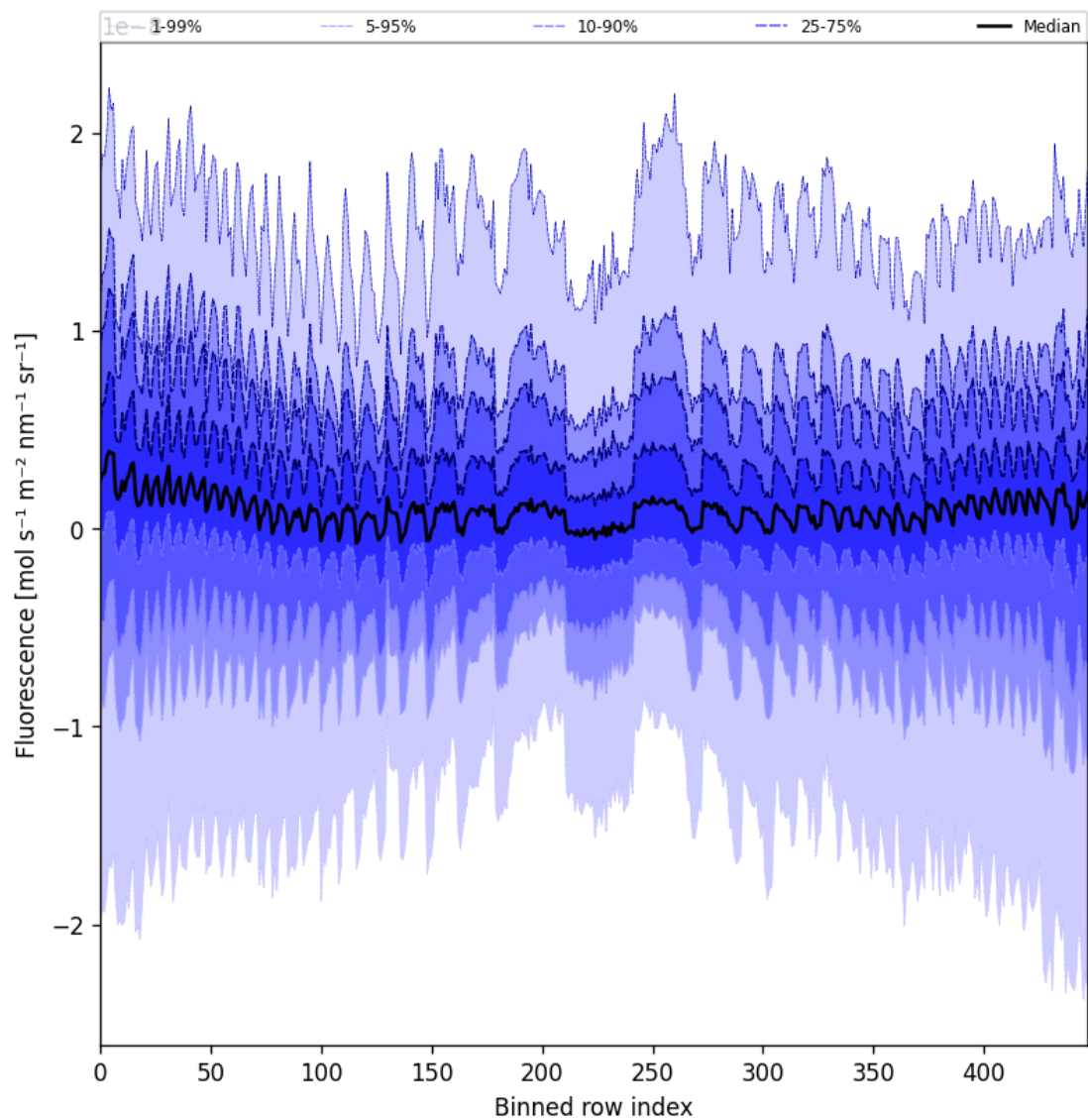
Figure 57: Along track statistics of “Fluorescence” for 2024-08-27 to 2024-08-29
