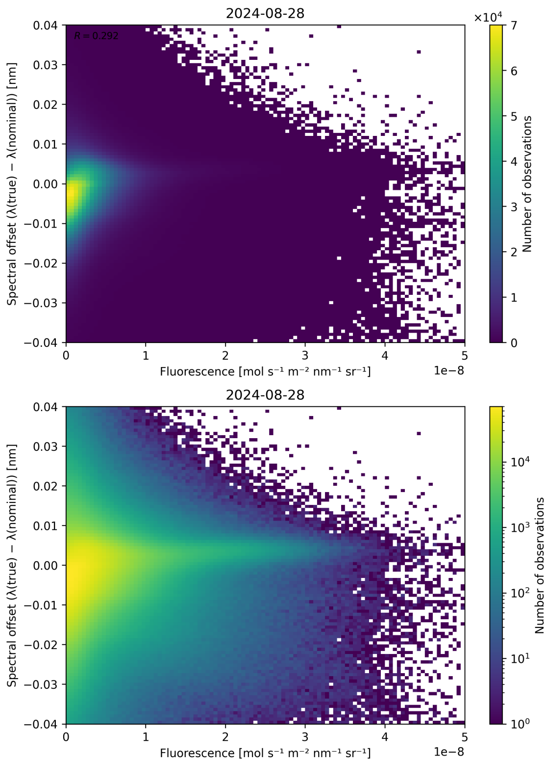
Figure 87: Scatter density plot of “Fluorescence” against “Spectral offset ( \lambda_{\text{true}} - \lambda_{\text{nominal}} )” for 2024-08-27 to 2024-08-29.
