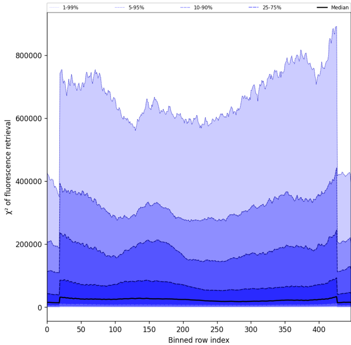
Figure 59: Along track statistics of “ \chi^2 of fluorescence retrieval” for 2024-08-27 to 2024-08-29
