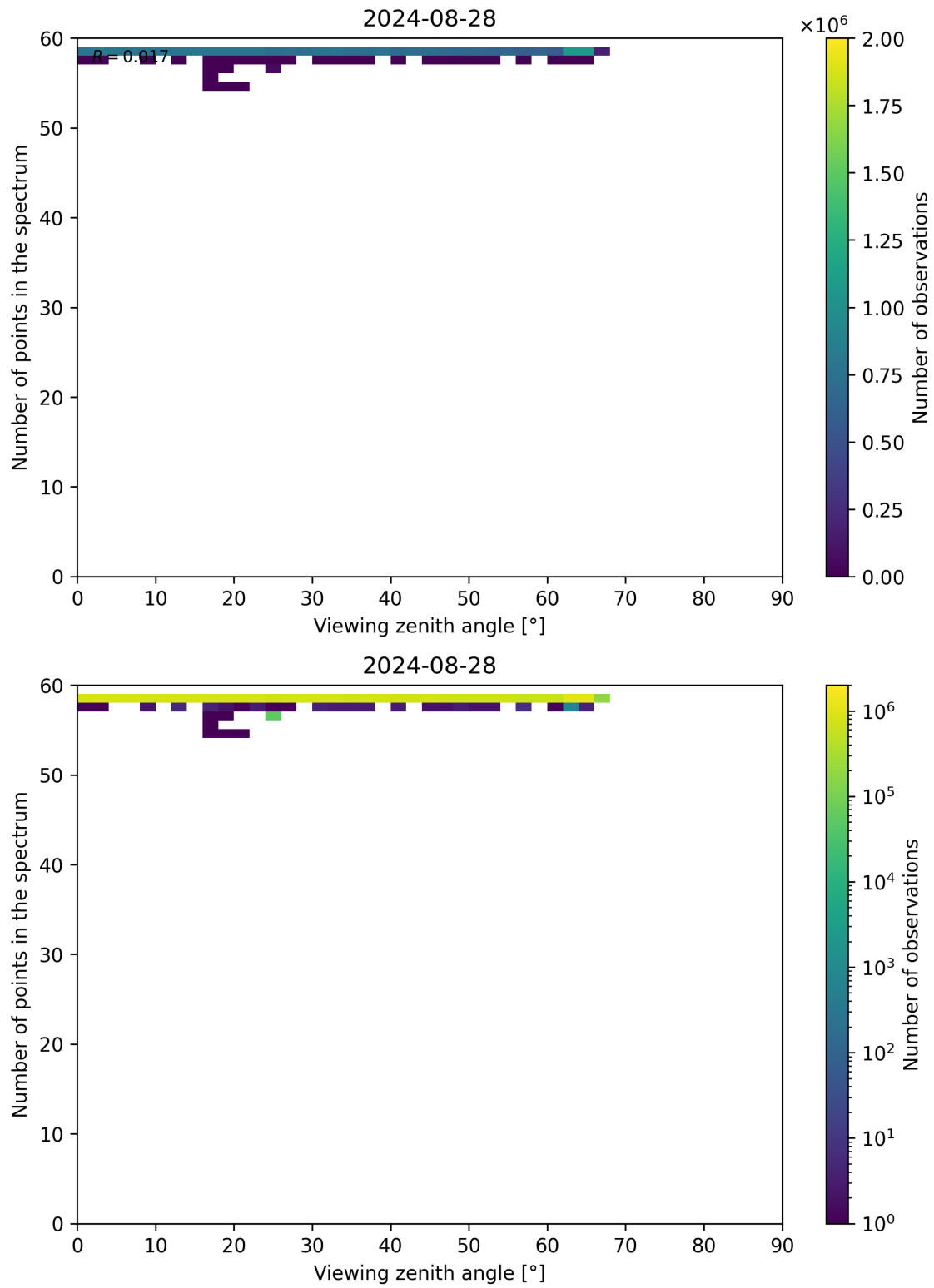
Figure 125: Scatter density plot of “Viewing zenith angle” against “Number of points in the spectrum” for 2024-08-27 to 2024-08-29.
