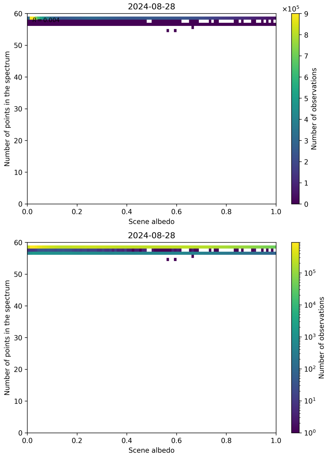
Figure 106: Scatter density plot of “Scene albedo” against “Number of points in the spectrum” for 2024-08-27 to 2024-08-29.
