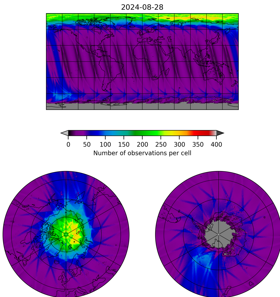
Figure 11: Map of the number of observations for 2024-08-27 to 2024-08-29
