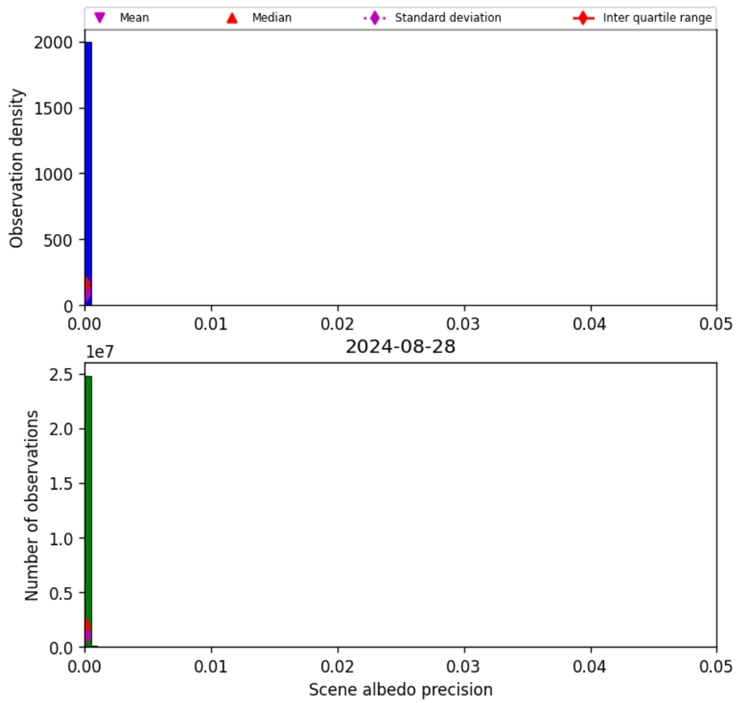
Figure 35: Histogram of “Scene albedo precision” for 2024-08-27 to 2024-08-29
