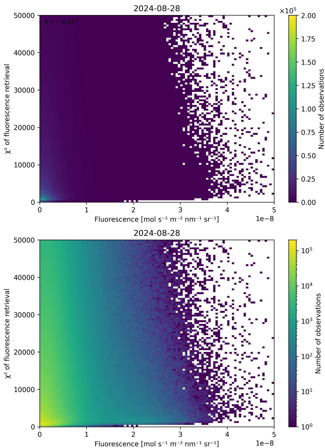
Figure 85: Scatter density plot of “Fluorescence” against “ \chi^2 of fluorescence retrieval” for 2024-08-27 to 2024-08-29.
