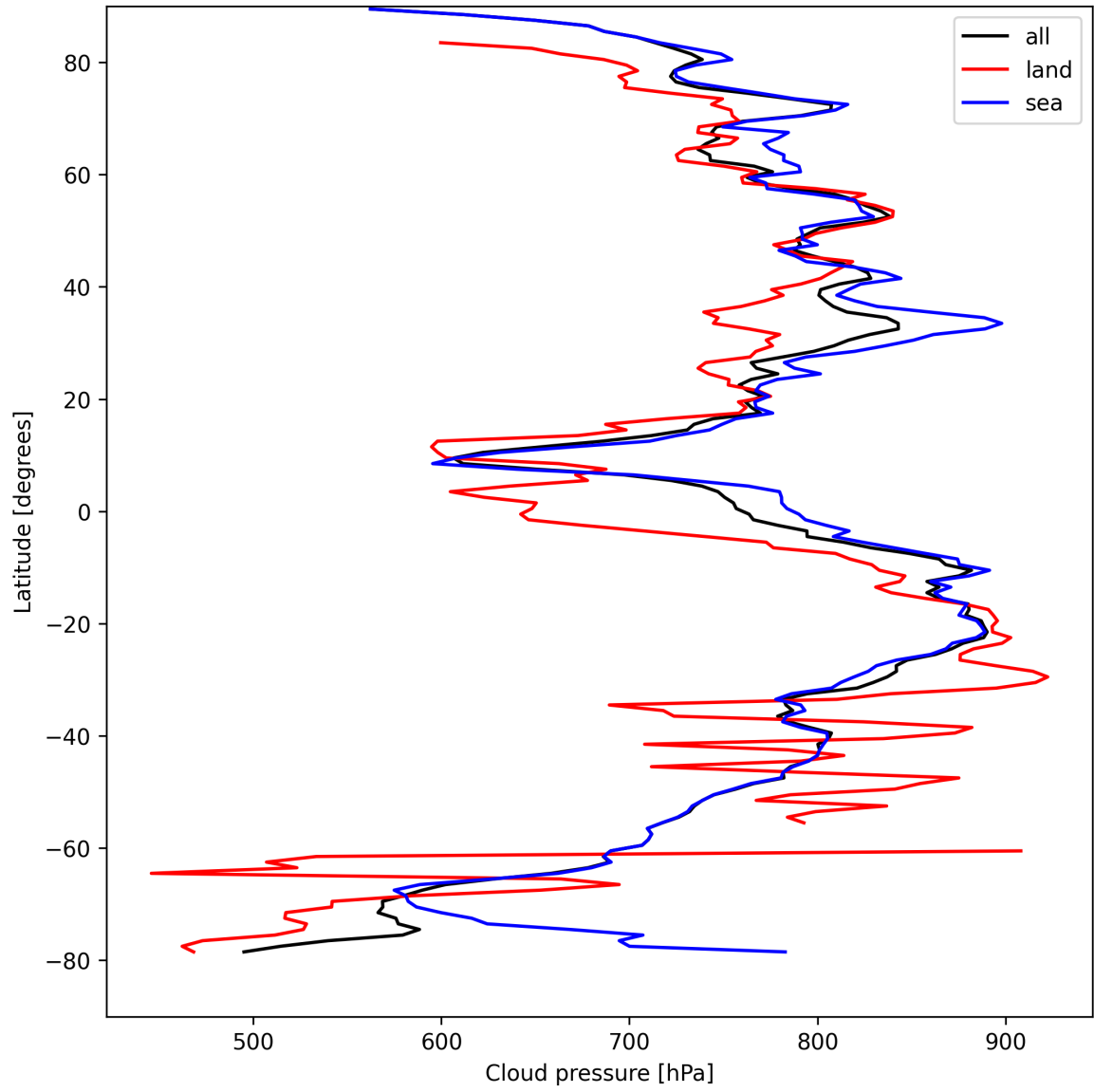
Figure 13: Zonal average of “Cloud pressure” for 2024-08-27 to 2024-08-29.
