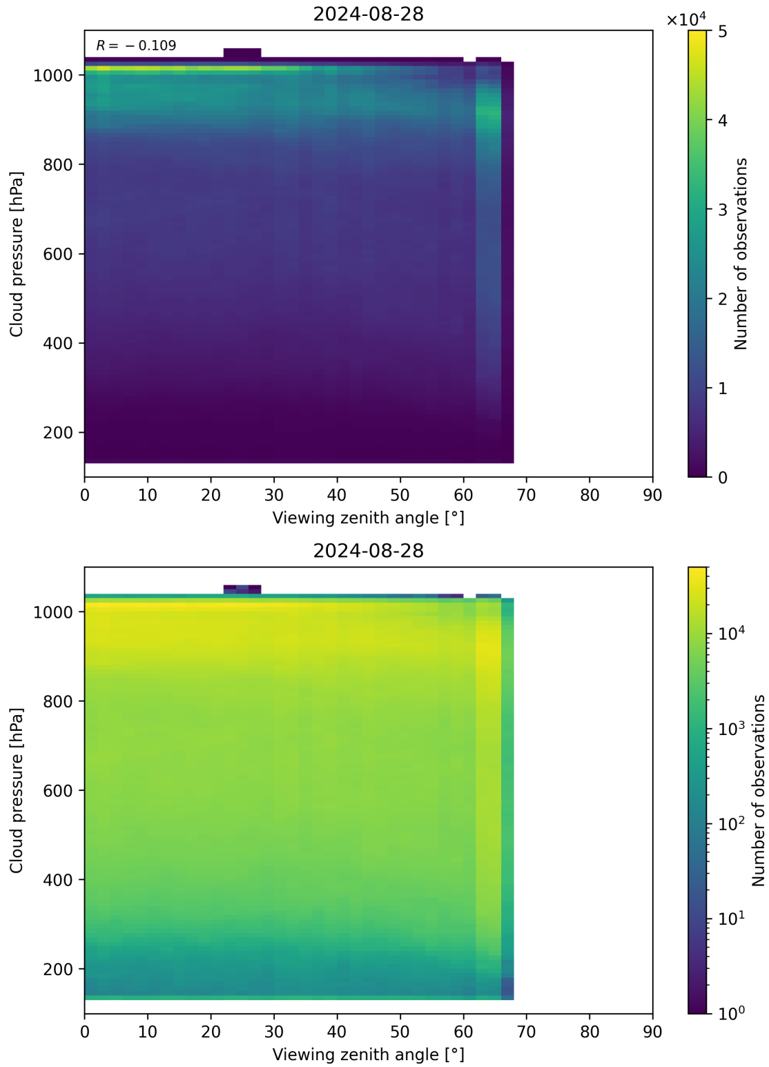
Figure 121: Scatter density plot of “Viewing zenith angle” against “Cloud pressure” for 2024-08-27 to 2024-08-29.
