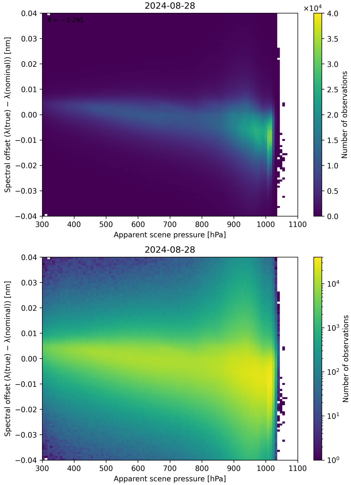
Figure 67: Scatter density plot of “Apparent scene pressure” against “Spectral offset ( \lambda_{\text{true}} - \lambda_{\text{nominal}} )” for 2024-08-27 to 2024-08-29.
