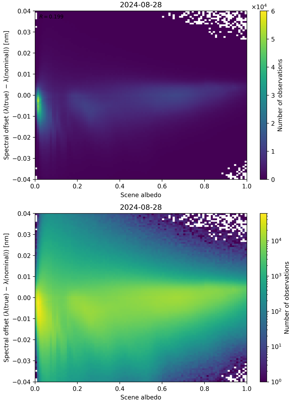
Figure 107: Scatter density plot of “Scene albedo” against “Spectral offset ( \lambda_{\text{true}} - \lambda_{\text{nominal}} )” for 2024-08-27 to 2024-08-29.
