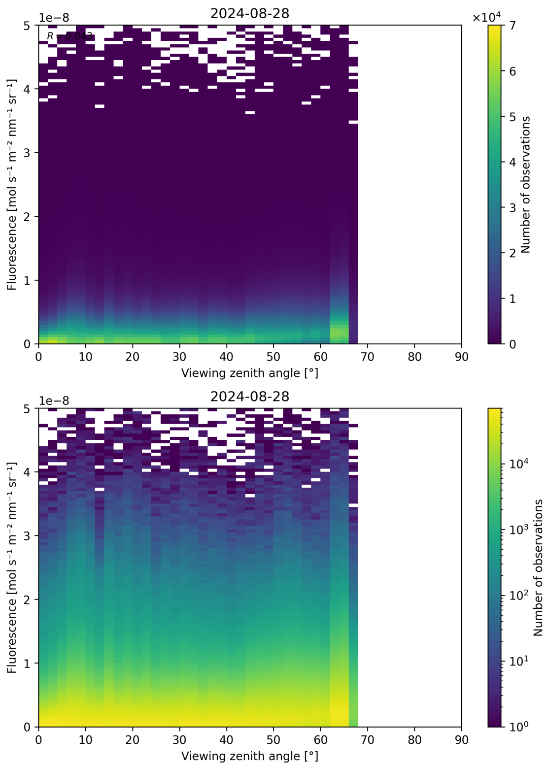
Figure 122: Scatter density plot of “Viewing zenith angle” against “Fluorescence” for 2024-08-27 to 2024-08-29.
