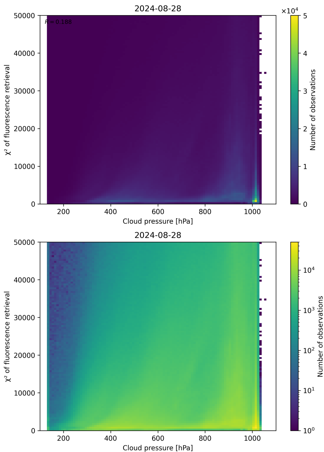
Figure 78: Scatter density plot of “Cloud pressure” against “ \chi^2 of fluorescence retrieval” for 2024-08-27 to 2024-08-29.
