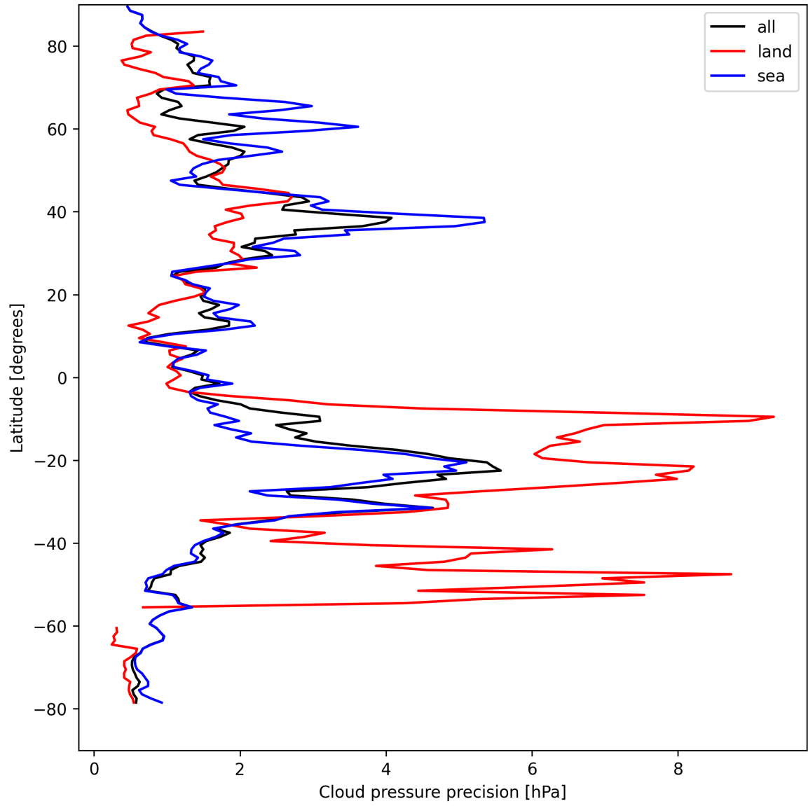
Figure 14: Zonal average of “Cloud pressure precision” for 2024-08-27 to 2024-08-29.
