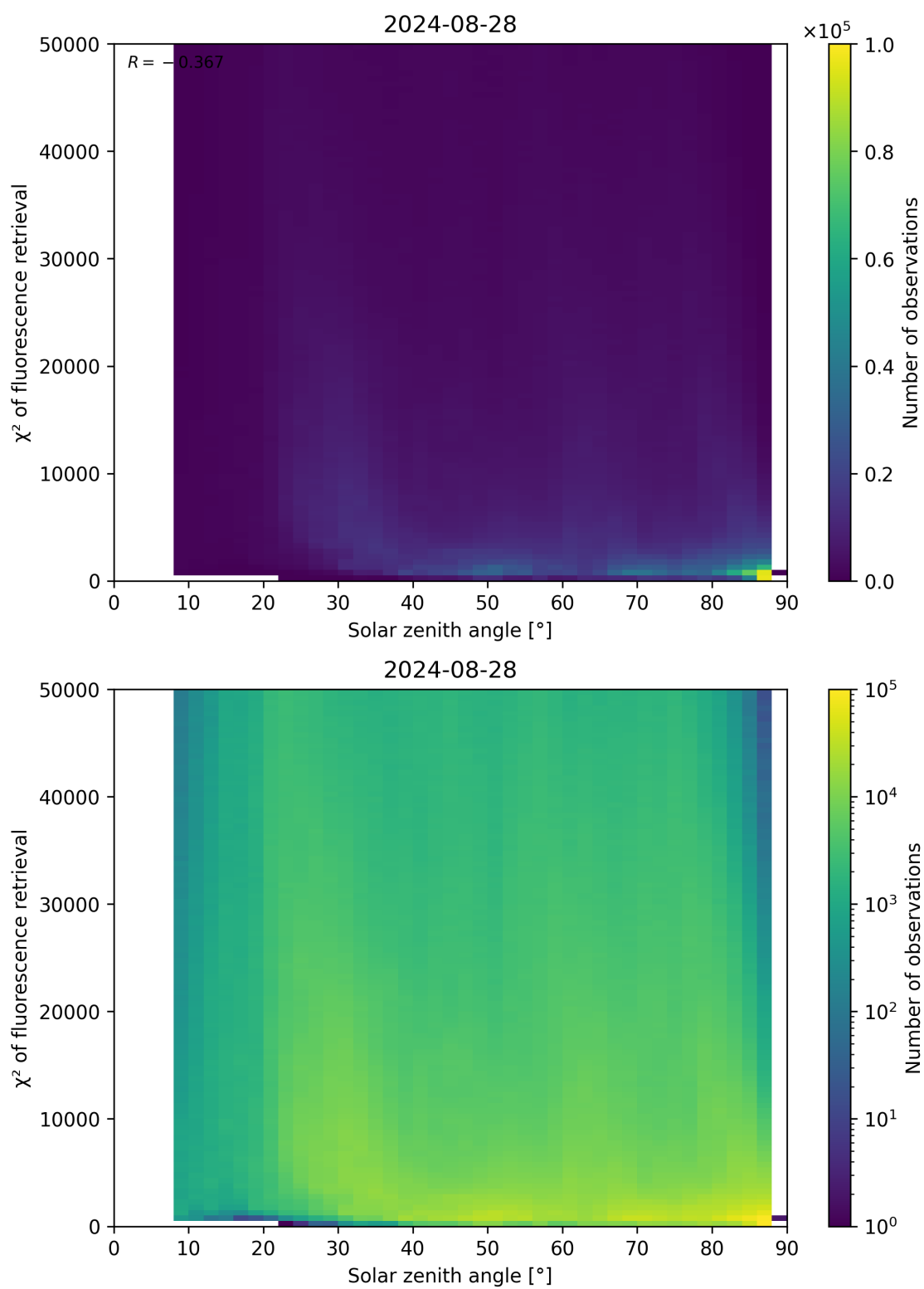
Figure 109: Scatter density plot of “Solar zenith angle” against “ \chi^2 of fluorescence retrieval” for 2024-08-27 to 2024-08-29.
