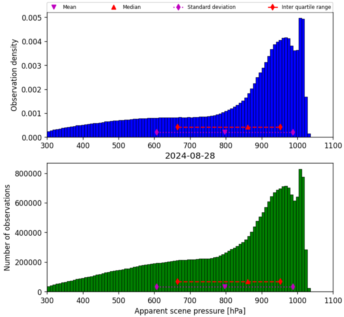
Figure 36: Histogram of “Apparent scene pressure” for 2024-08-27 to 2024-08-29
