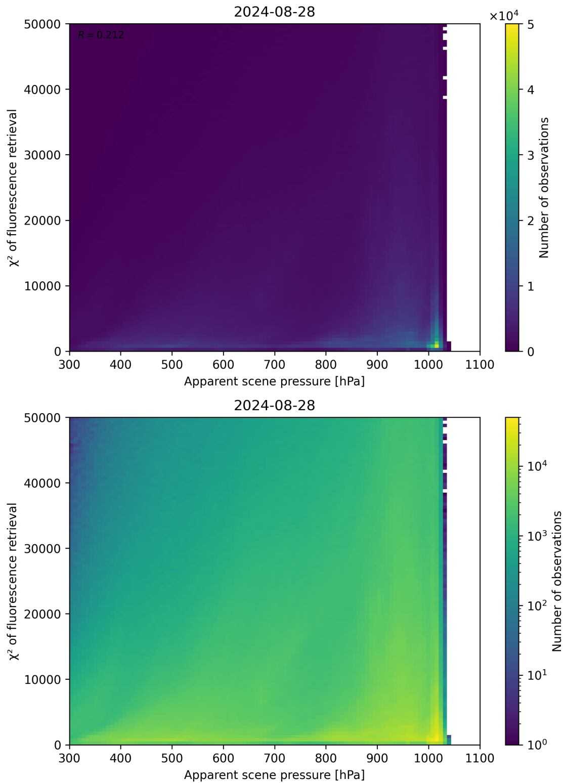
Figure 63: Scatter density plot of “Apparent scene pressure” against “ \chi^2 of fluorescence retrieval” for 2024-08-27 to 2024-08-29.
