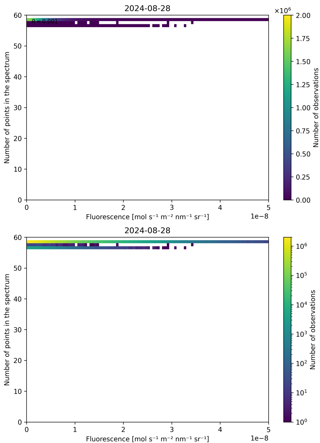
Figure 86: Scatter density plot of “Fluorescence” against “Number of points in the spectrum” for 2024-08-27 to 2024-08-29.
