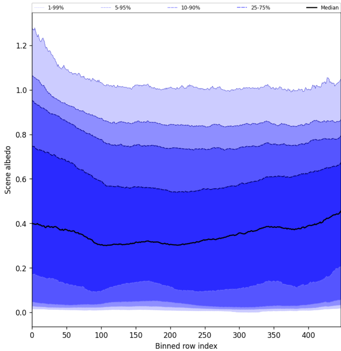
Figure 51: Along track statistics of “Scene albedo” for 2024-08-27 to 2024-08-29
