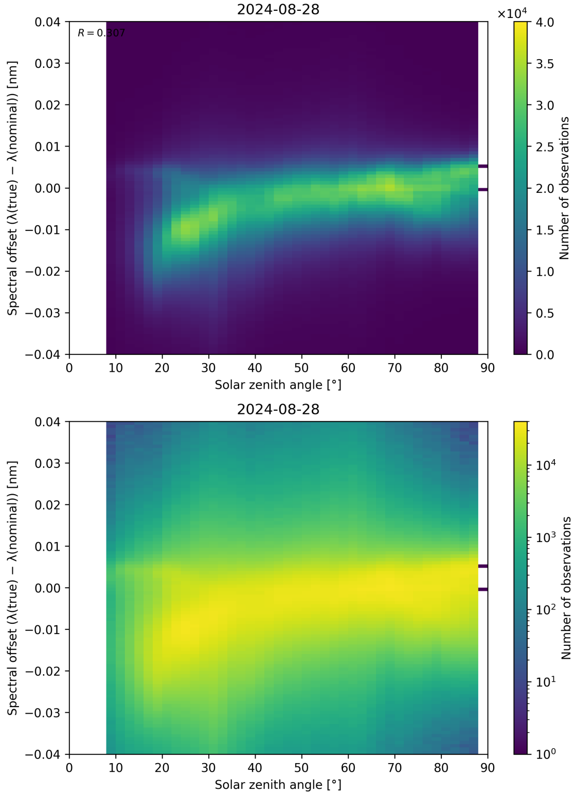
Figure 117: Scatter density plot of “Solar zenith angle” against “Spectral offset ( \lambda_{\text{true}} - \lambda_{\text{nominal}} )” for 2024-08-27 to 2024-08-29.
