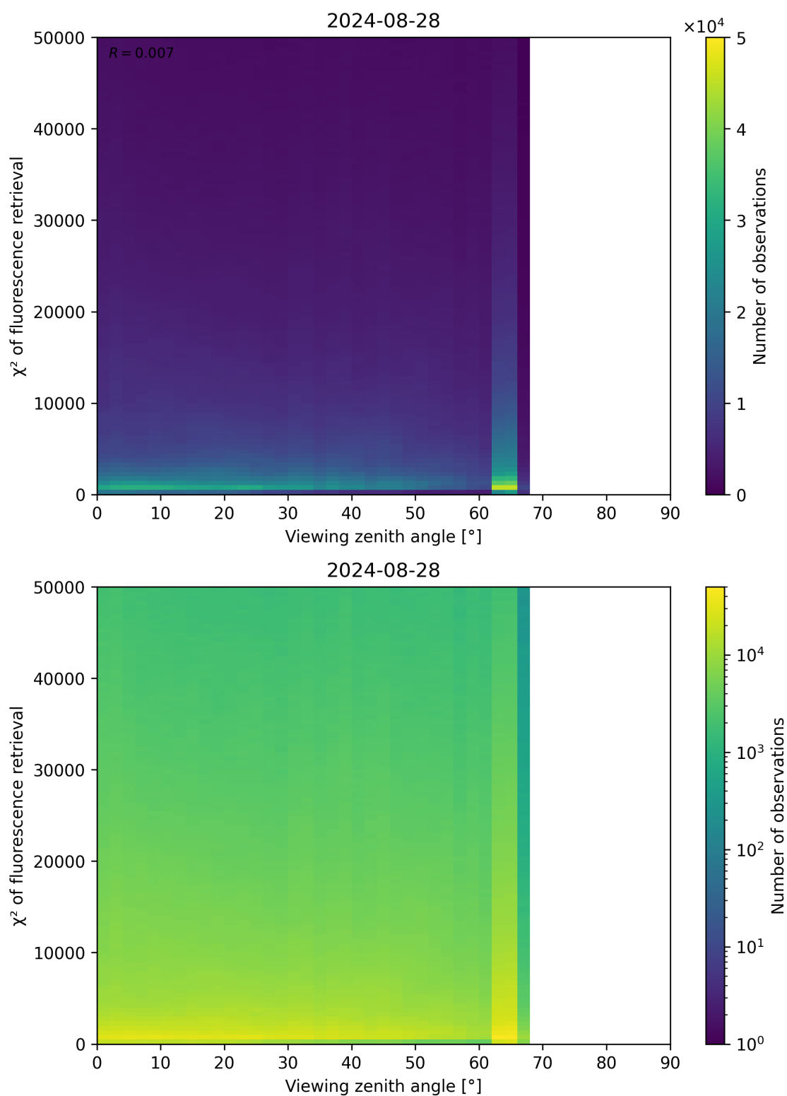
Figure 119: Scatter density plot of “Viewing zenith angle” against “ \chi^2 of fluorescence retrieval” for 2024-08-27 to 2024-08-29.
