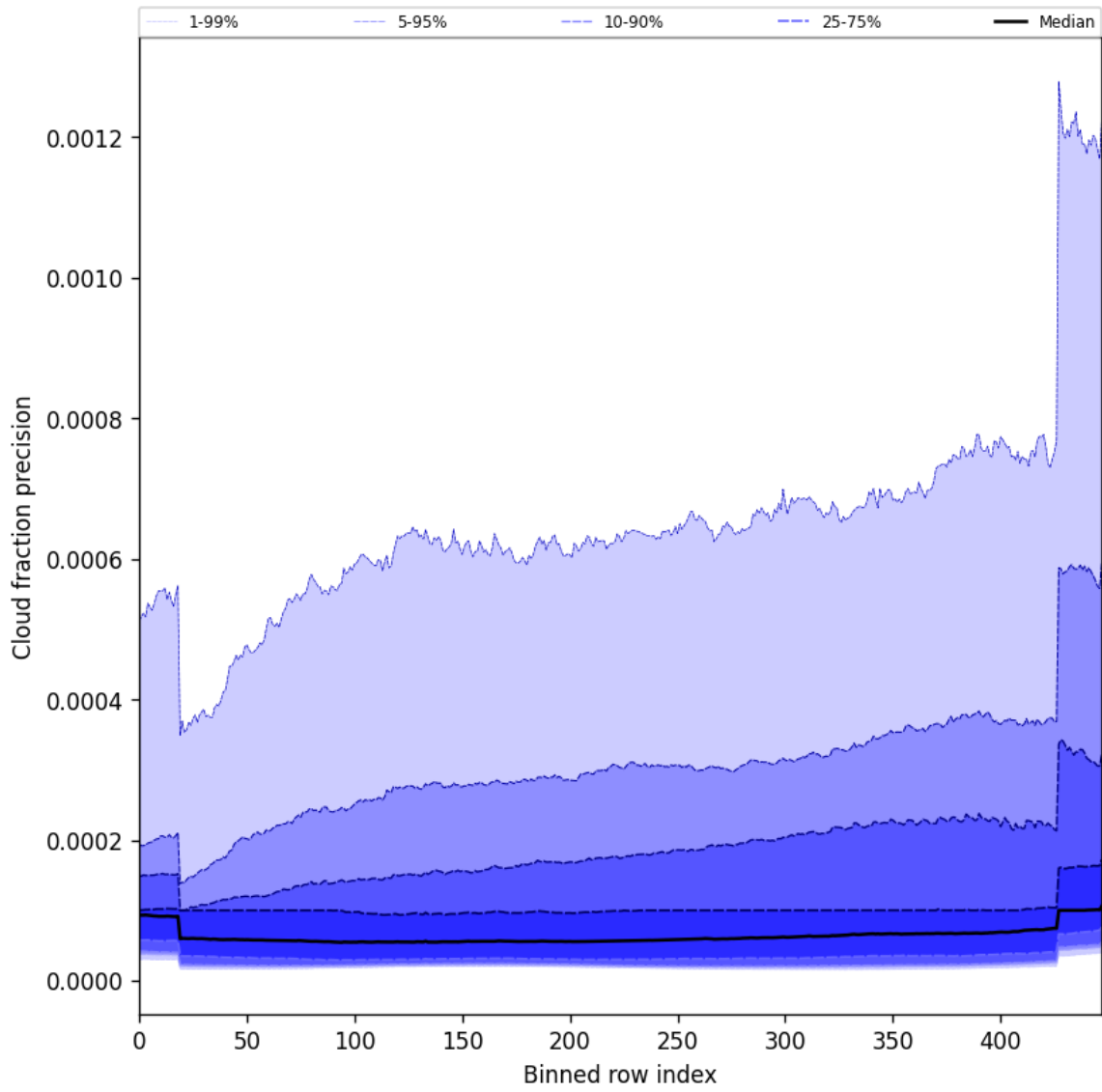
Figure 50: Along track statistics of “Cloud fraction precision” for 2024-08-27 to 2024-08-29
