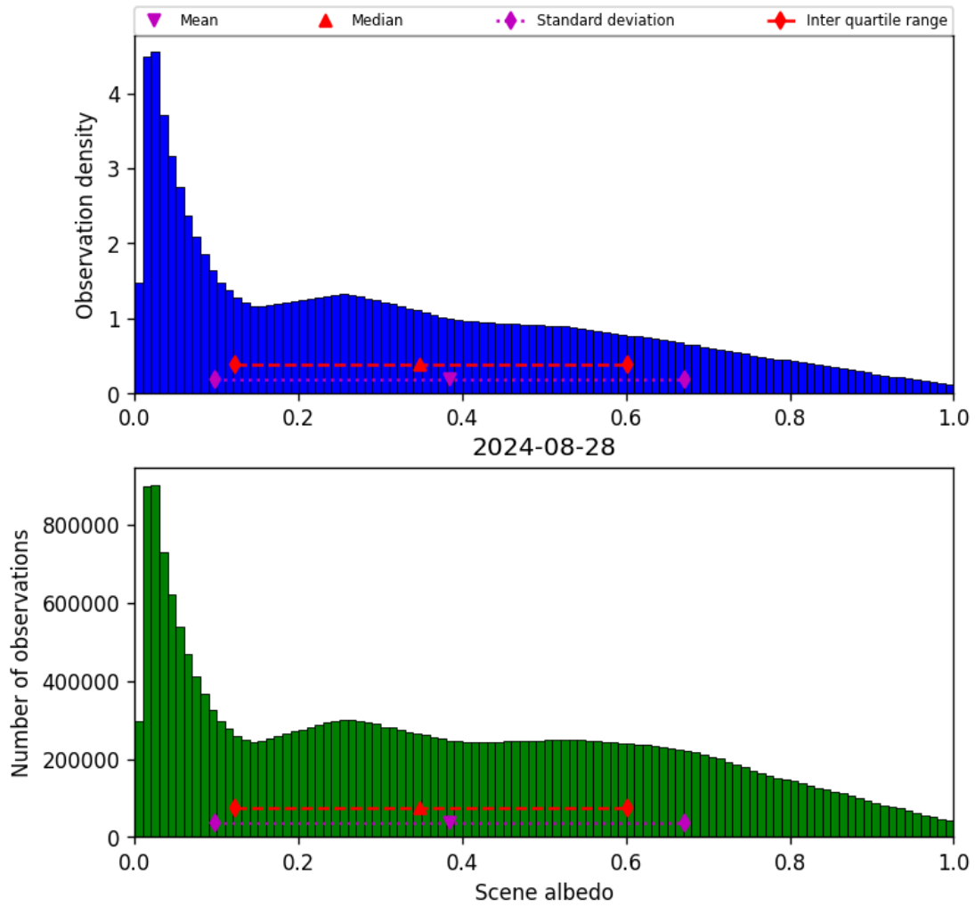
Figure 34: Histogram of “Scene albedo” for 2024-08-27 to 2024-08-29
