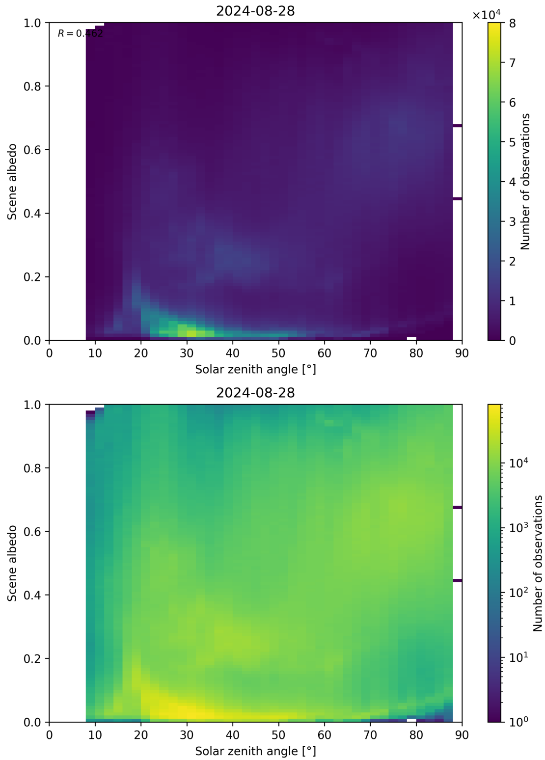
Figure 116: Scatter density plot of “Solar zenith angle” against “Scene albedo” for 2024-08-27 to 2024-08-29.
