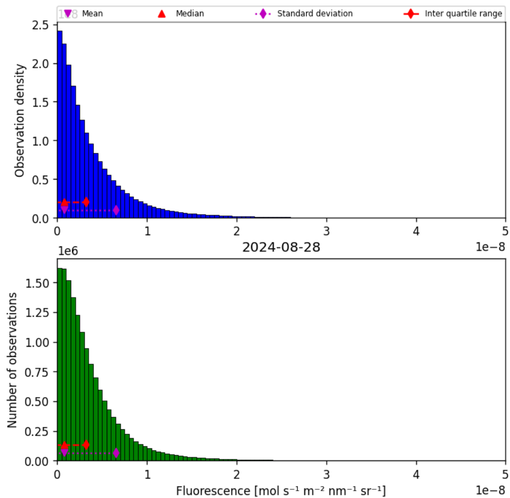
Figure 40: Histogram of “Fluorescence” for 2024-08-27 to 2024-08-29
