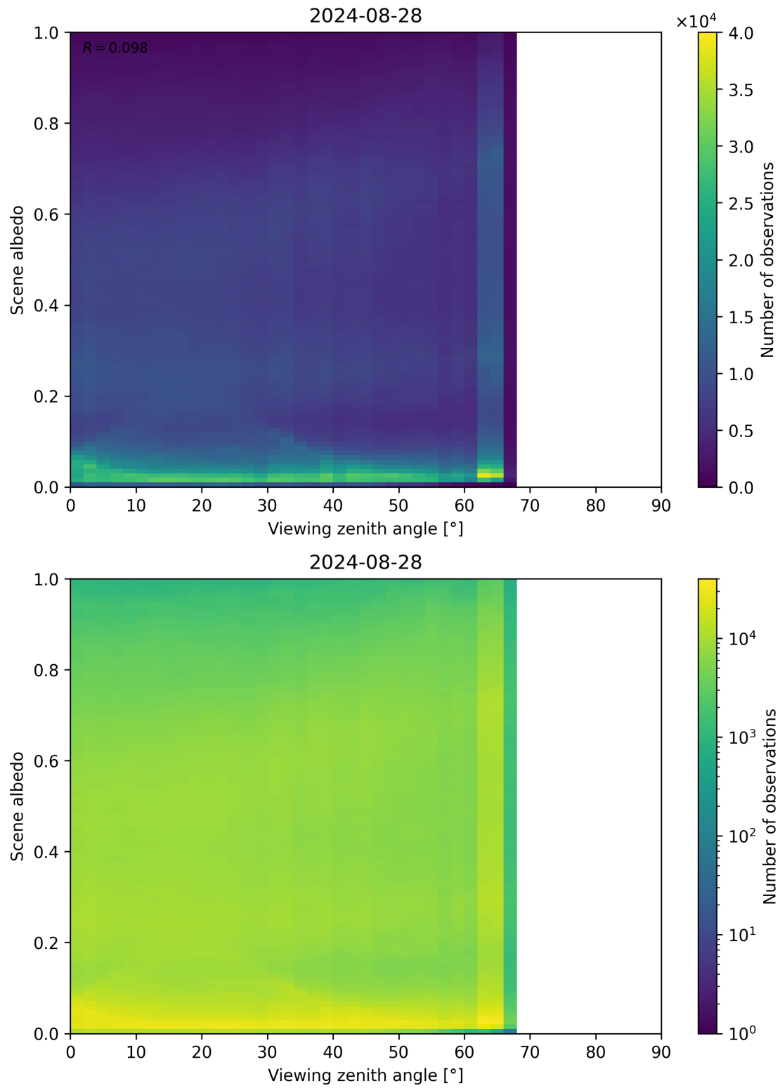
Figure 126: Scatter density plot of “Viewing zenith angle” against “Scene albedo” for 2024-08-27 to 2024-08-29.
