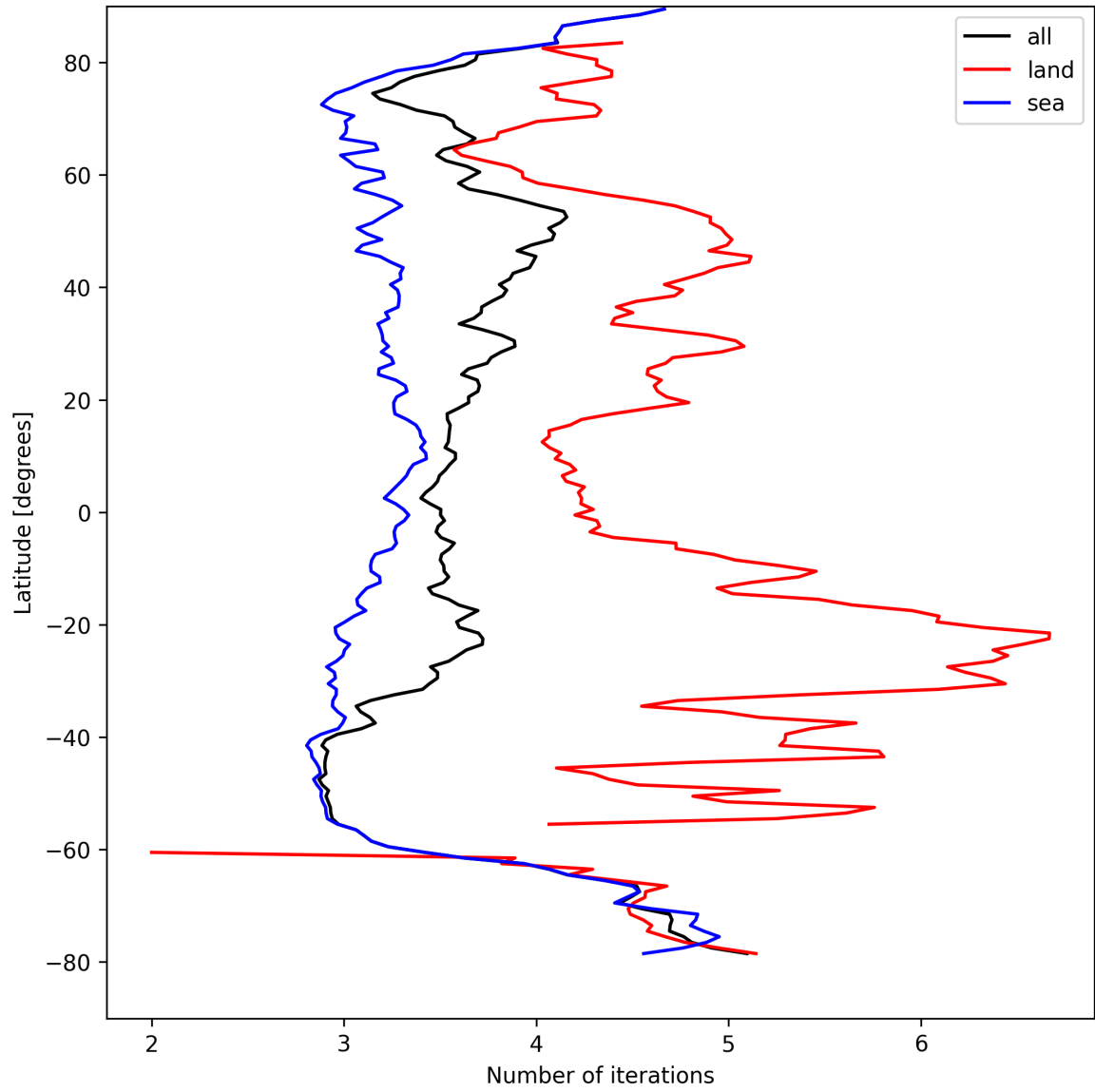
Figure 22: Zonal average of “Number of iterations” for 2024-08-27 to 2024-08-29.
