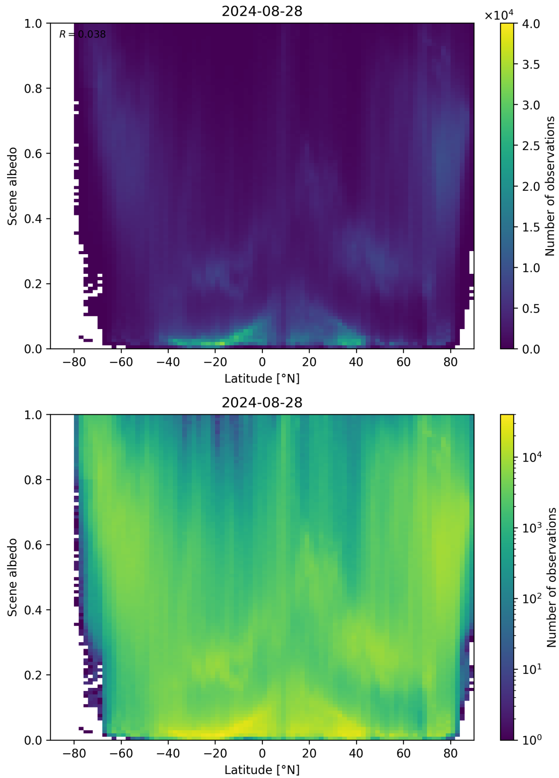
Figure 95: Scatter density plot of “Latitude” against “Scene albedo” for 2024-08-27 to 2024-08-29.
