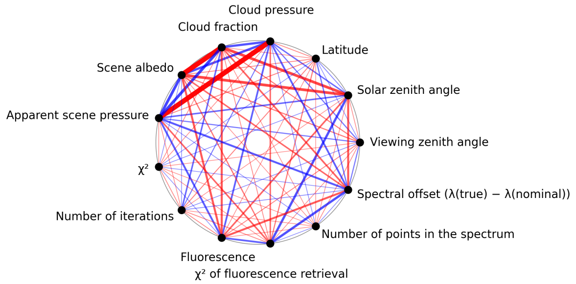
Figure 1: Map of correlation graph for 2024-08-27 to 2024-08-29.
