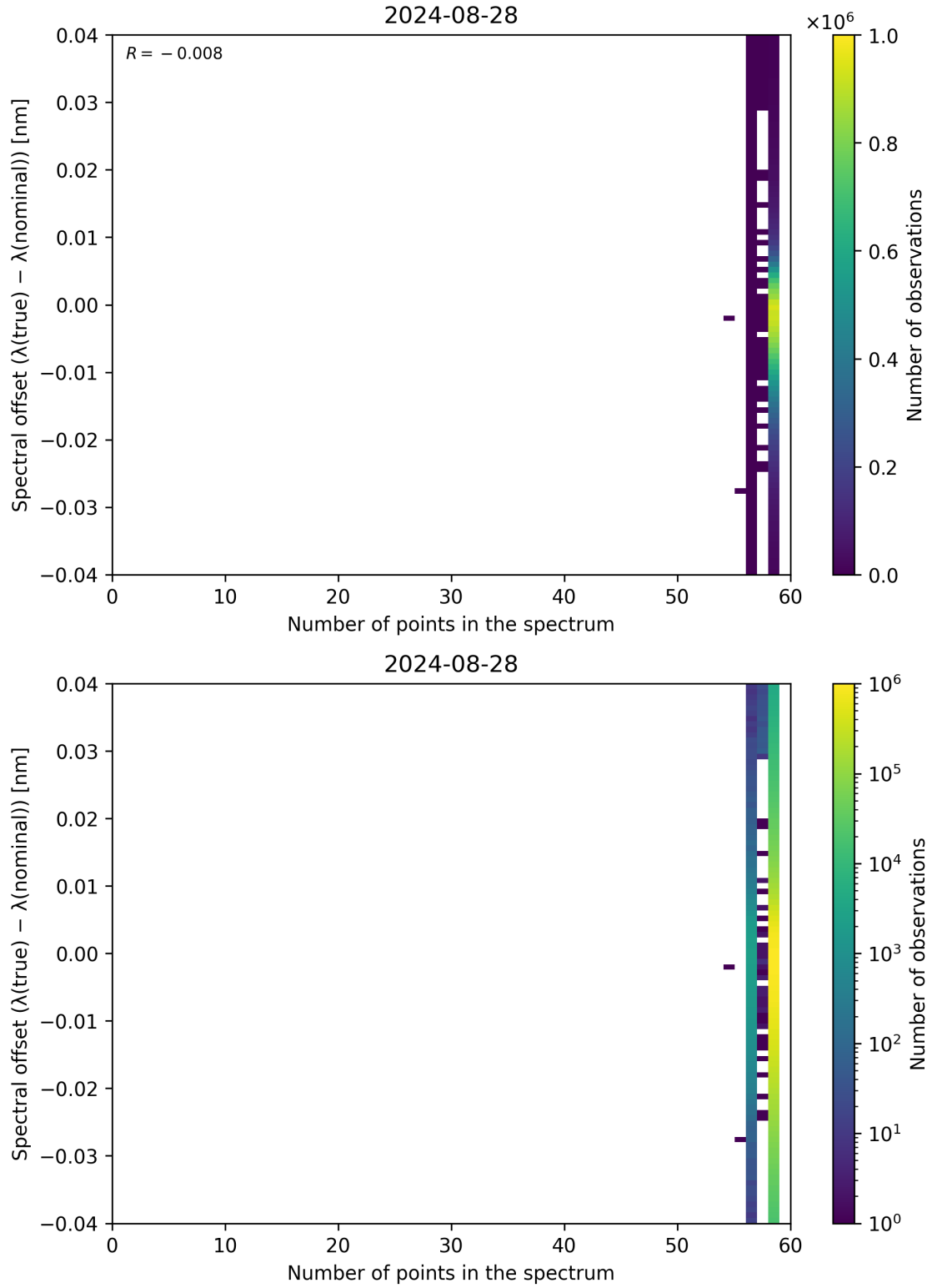
Figure 101: Scatter density plot of “Number of points in the spectrum” against “Spectral offset ( \lambda_{\text{true}} - \lambda_{\text{nominal}} )” for 2024-08-27 to 2024-08-29.
