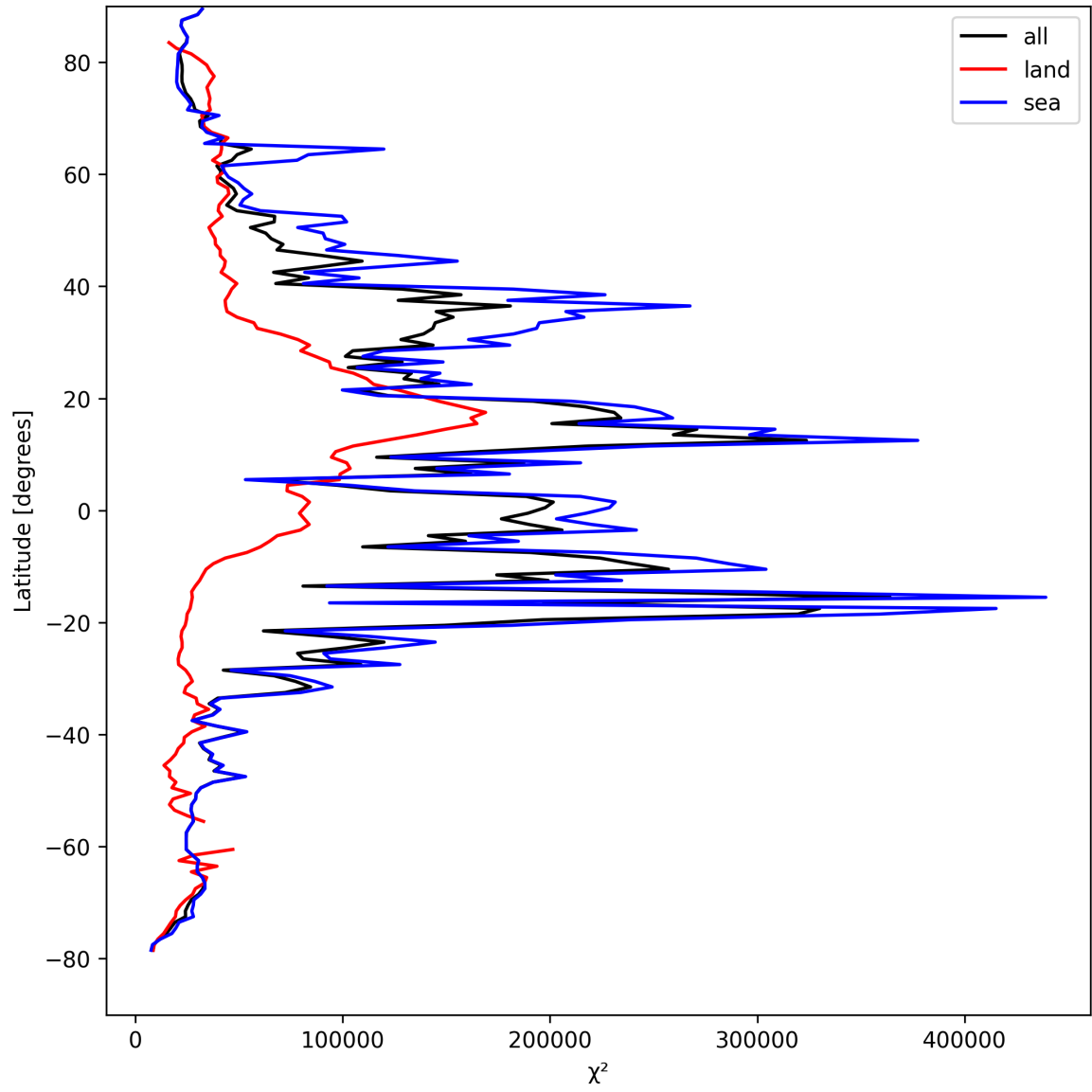
Figure 21: Zonal average of “ \chi^2 ” for 2024-08-27 to 2024-08-29.
