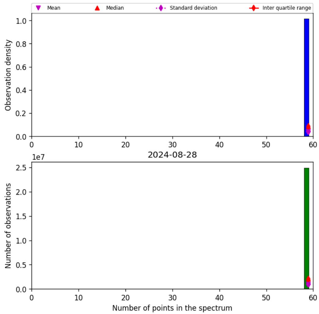
Figure 44: Histogram of “Number of points in the spectrum” for 2024-08-27 to 2024-08-29
