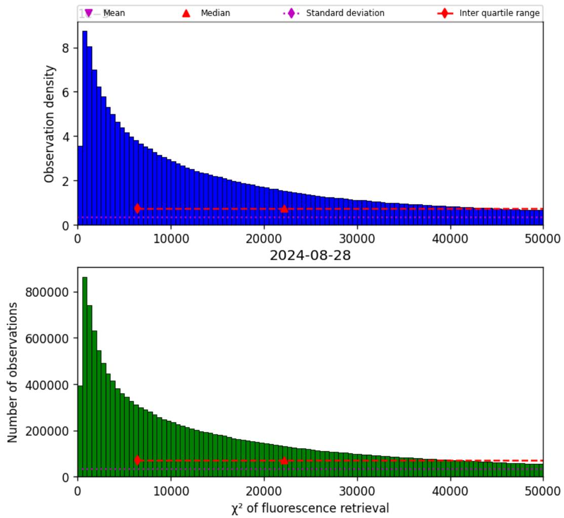
Figure 42: Histogram of “ \chi^2 of fluorescence retrieval” for 2024-08-27 to 2024-08-29
