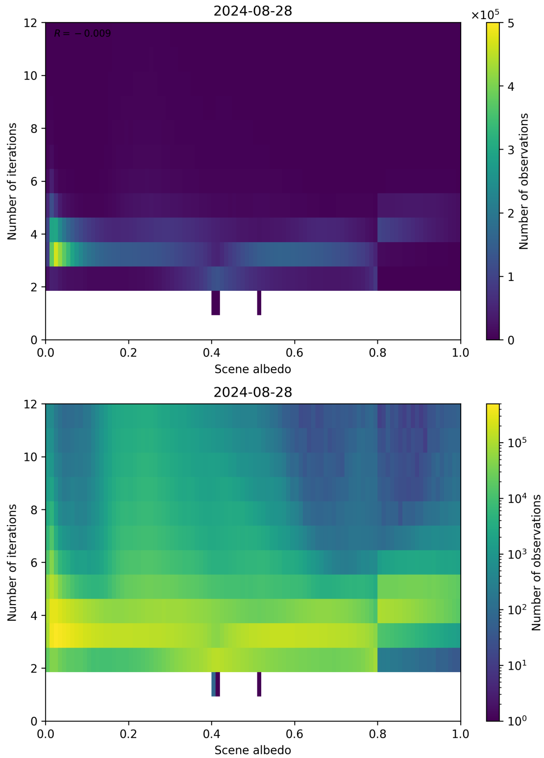
Figure 105: Scatter density plot of “Scene albedo” against “Number of iterations” for 2024-08-27 to 2024-08-29.
