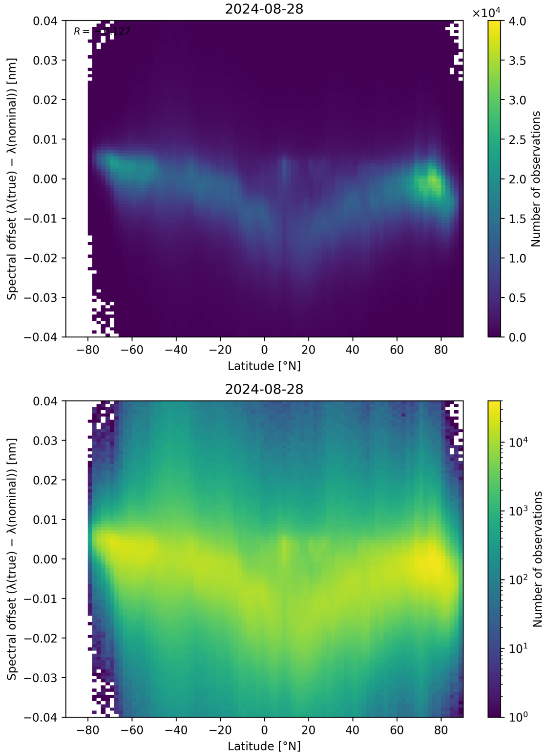
Figure 96: Scatter density plot of “Latitude” against “Spectral offset ( \lambda_{\text{true}} - \lambda_{\text{nominal}} )” for 2024-08-27 to 2024-08-29.
