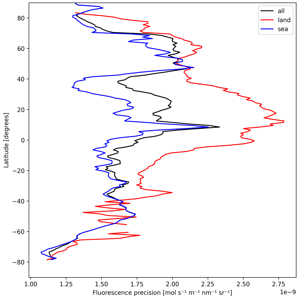
Figure 24: Zonal average of “Fluorescence precision” for 2024-08-27 to 2024-08-29.
