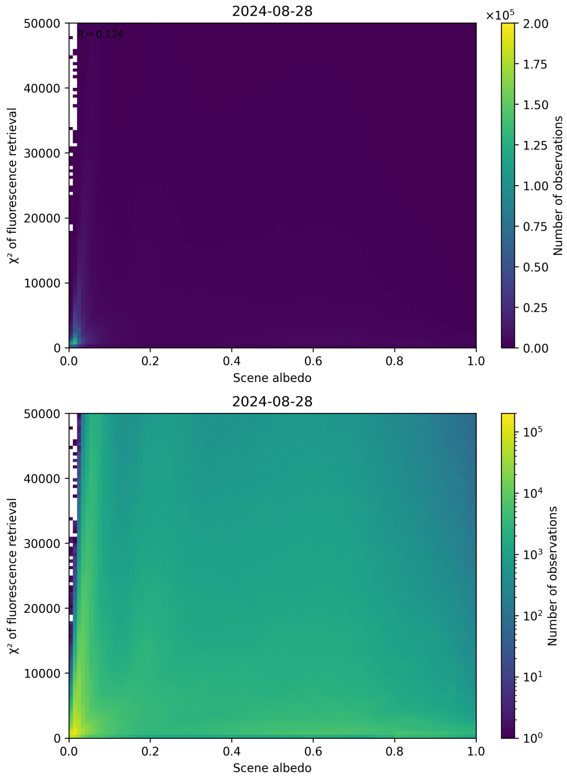
Figure 103: Scatter density plot of “Scene albedo” against “ \chi^2 of fluorescence retrieval” for 2024-08-27 to 2024-08-29.
