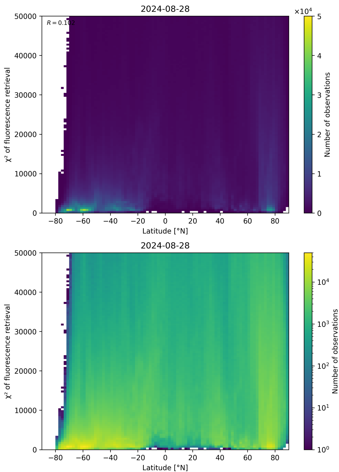
Figure 89: Scatter density plot of “Latitude” against “ \chi^2 of fluorescence retrieval” for 2024-08-27 to 2024-08-29.
