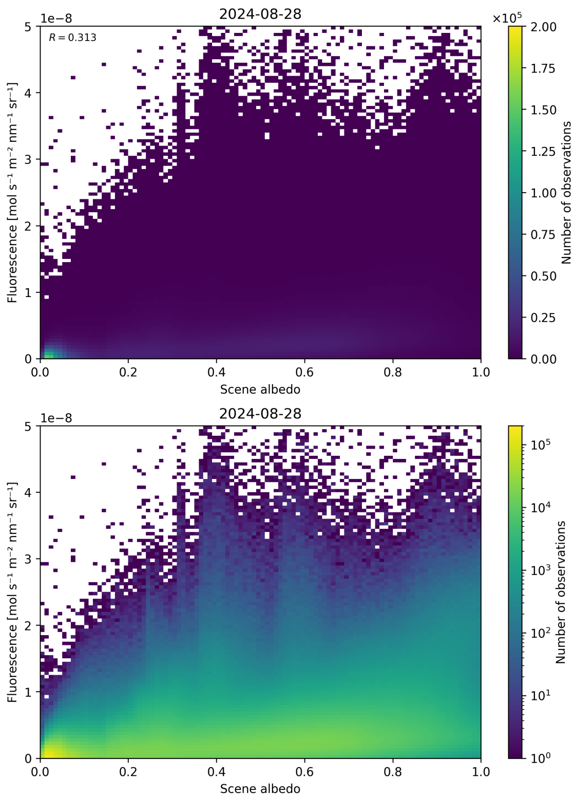
Figure 104: Scatter density plot of “Scene albedo” against “Fluorescence” for 2024-08-27 to 2024-08-29.
