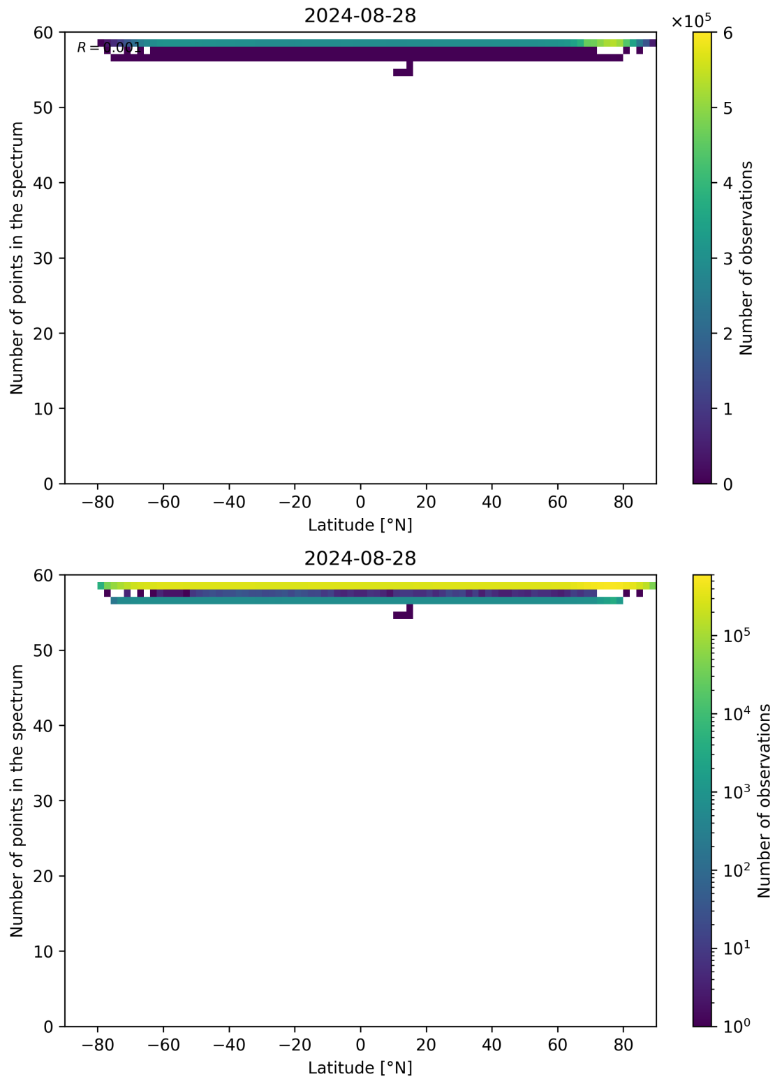
Figure 94: Scatter density plot of “Latitude” against “Number of points in the spectrum” for 2024-08-27 to 2024-08-29.
