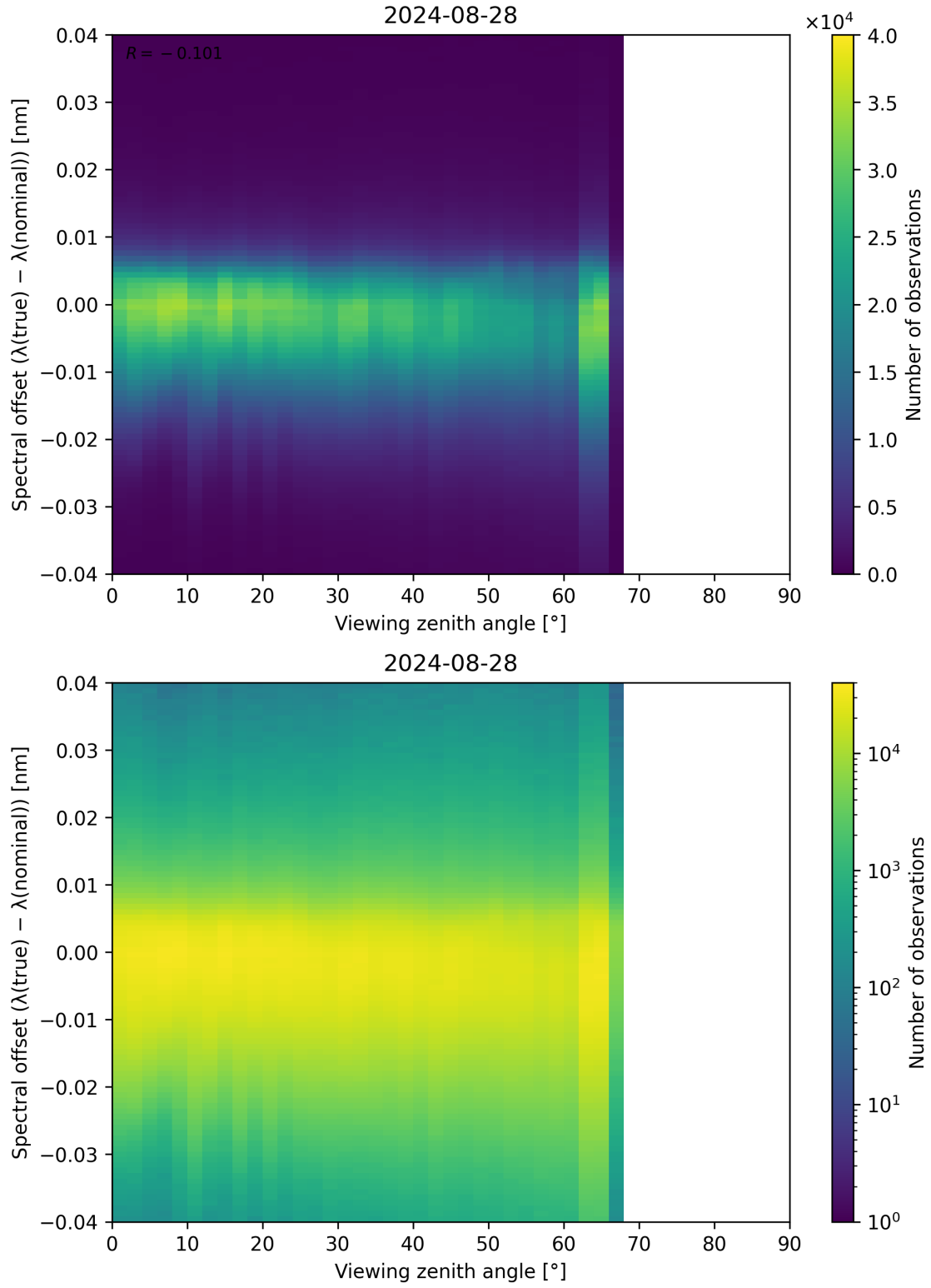
Figure 128: Scatter density plot of “Viewing zenith angle” against “Spectral offset ( \lambda_{\text{true}} - \lambda_{\text{nominal}} )” for 2024-08-27 to 2024-08-29.
