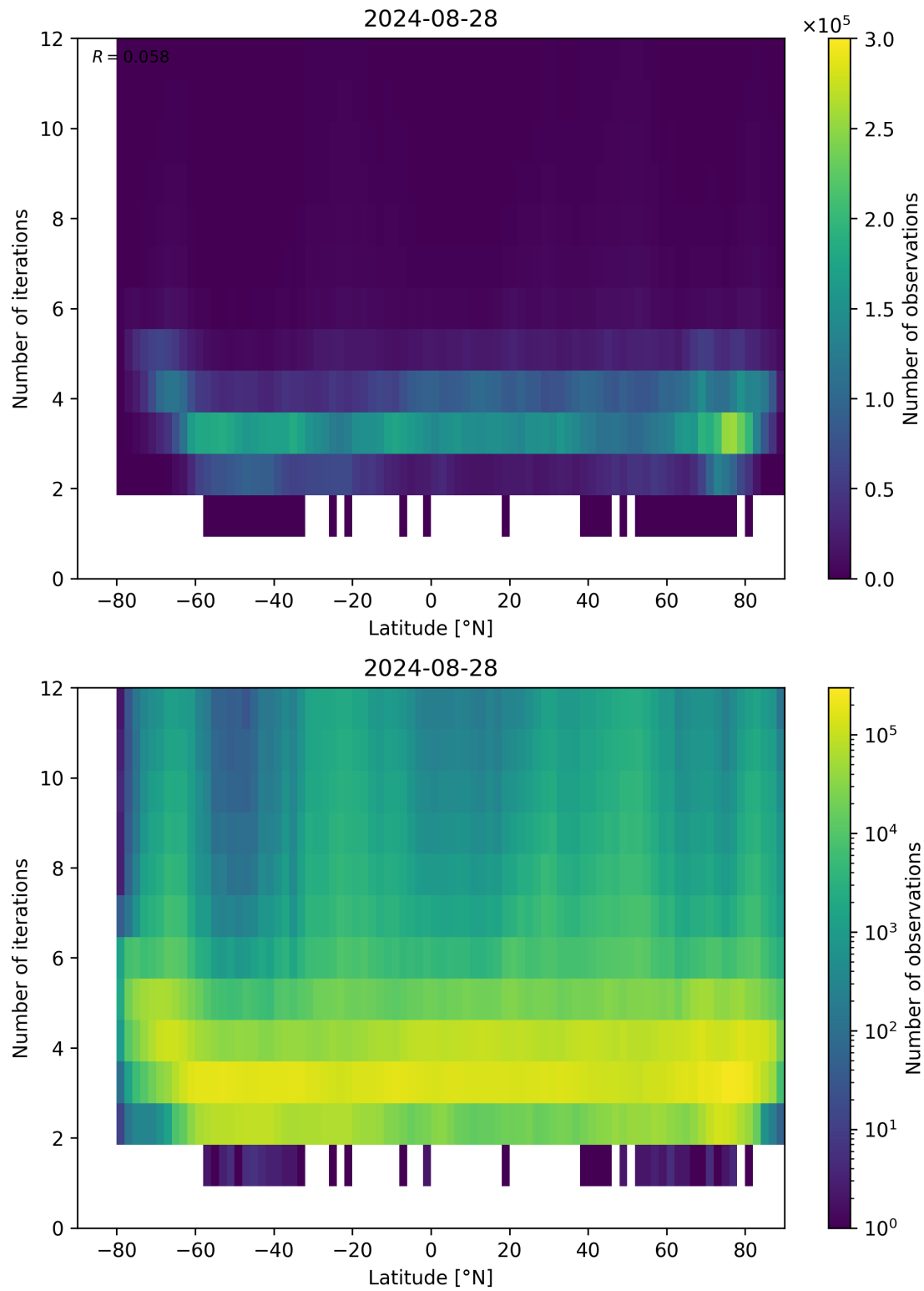
Figure 93: Scatter density plot of “Latitude” against “Number of iterations” for 2024-08-27 to 2024-08-29.
