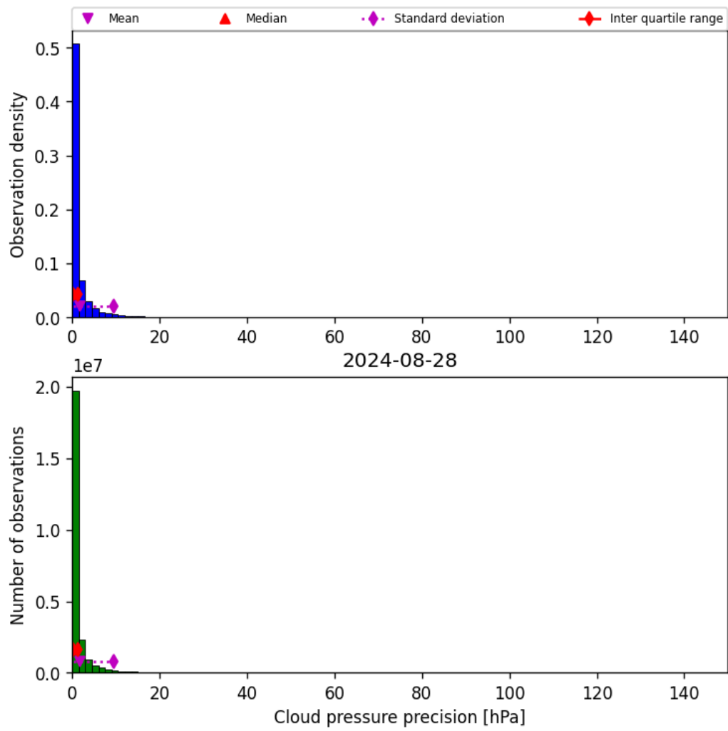
Figure 31: Histogram of “Cloud pressure precision” for 2024-08-27 to 2024-08-29
