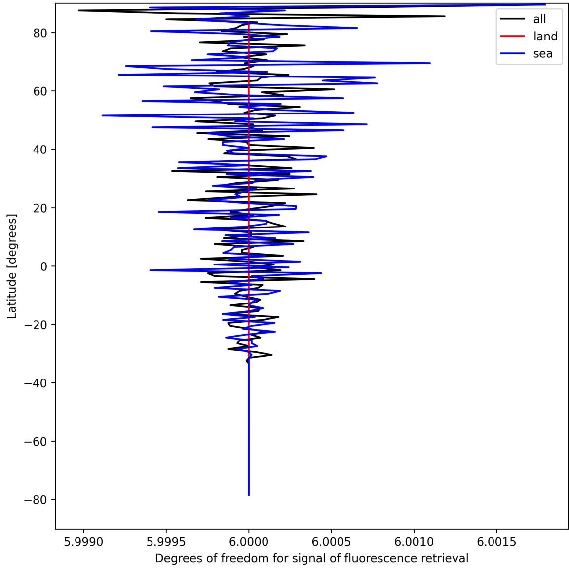
Figure 26: Zonal average of “Degrees of freedom for signal of fluorescence retrieval” for 2024-08-27 to 2024-08-29.
