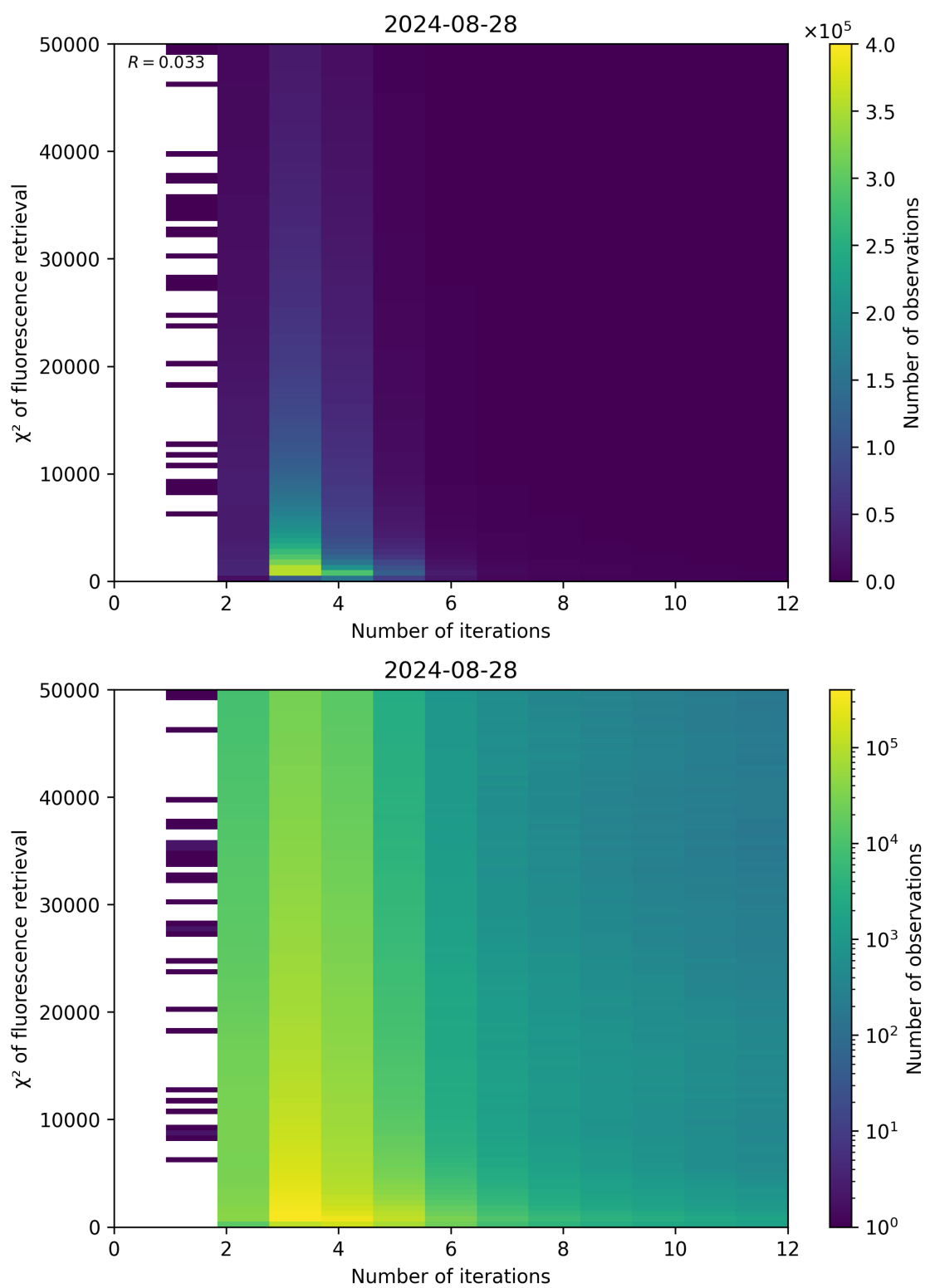
Figure 97: Scatter density plot of “Number of iterations” against “ \chi^2 of fluorescence retrieval” for 2024-08-27 to 2024-08-29.
