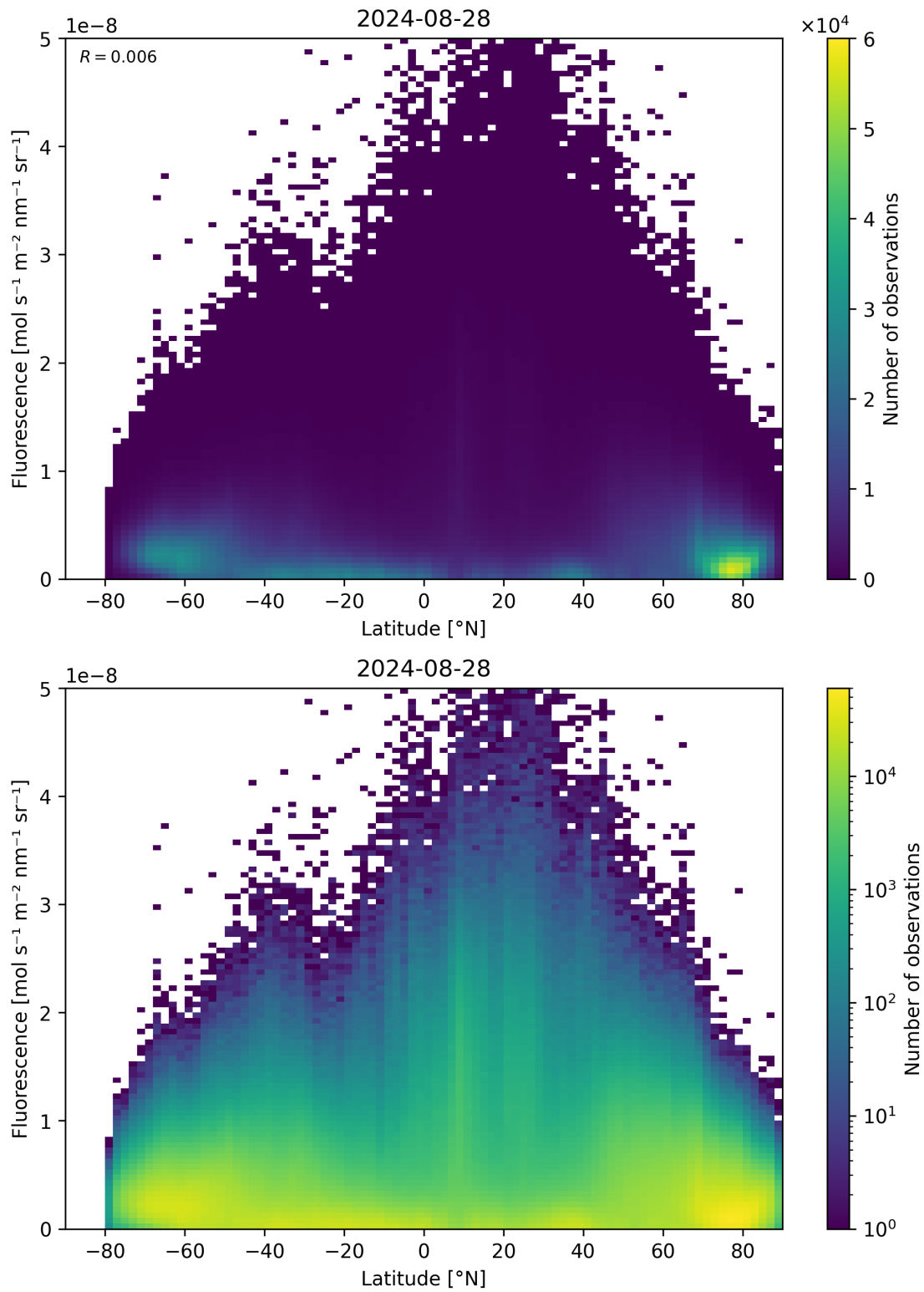
Figure 92: Scatter density plot of “Latitude” against “Fluorescence” for 2024-08-27 to 2024-08-29.
