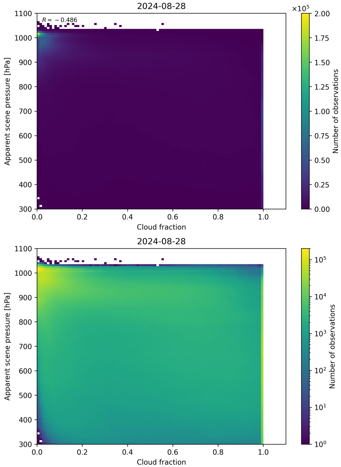
Figure 70: Scatter density plot of “Cloud fraction” against “Apparent scene pressure” for 2024-08-27 to 2024-08-29.
