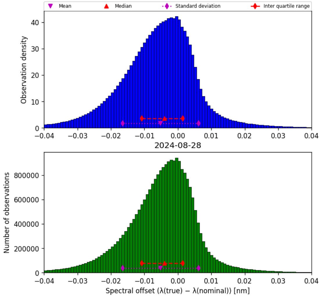
Figure 45: Histogram of “Spectral offset ( \lambda_{\text{true}} - \lambda_{\text{nominal}} )” for 2024-08-27 to 2024-08-29
