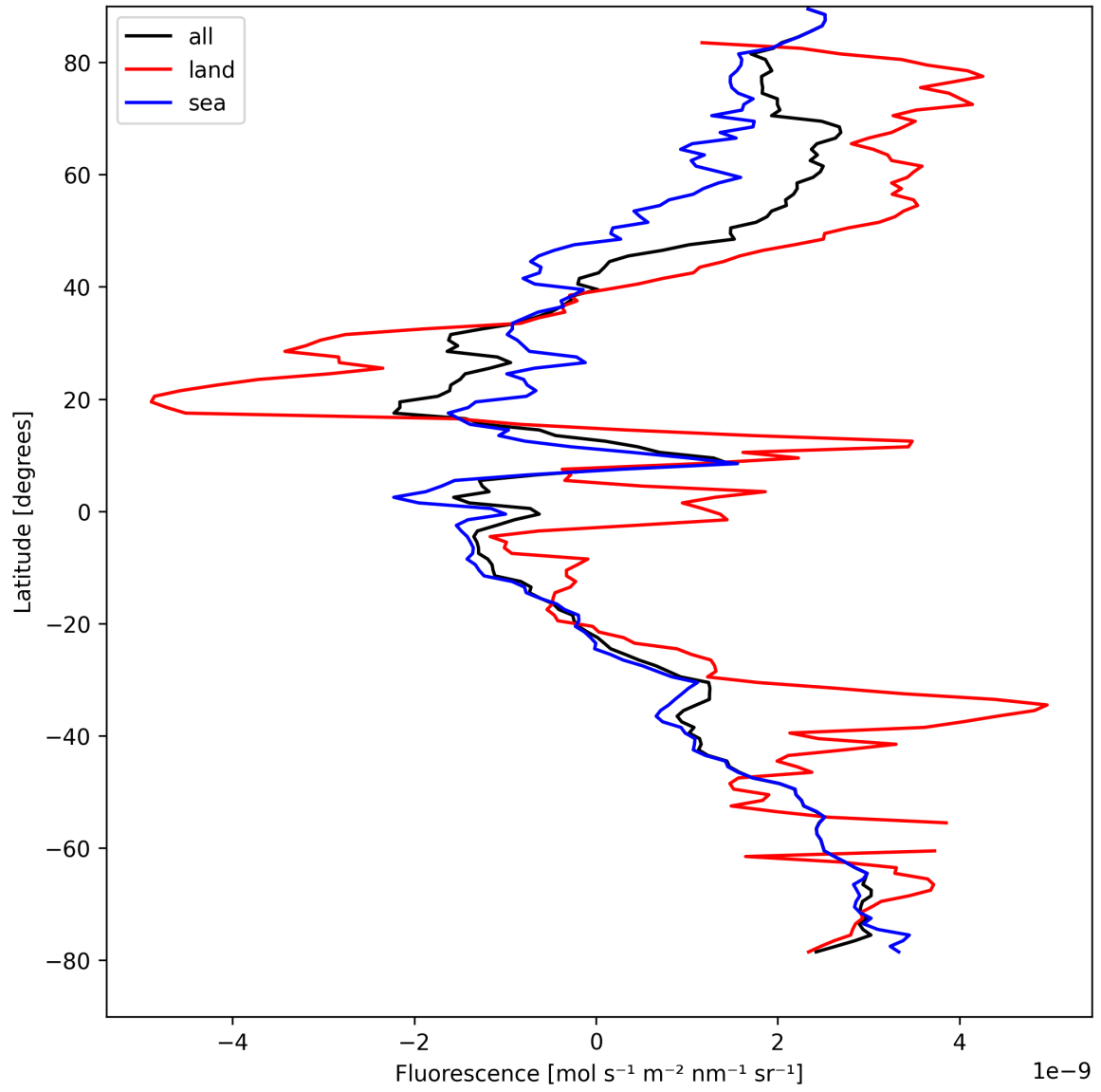
Figure 23: Zonal average of “Fluorescence” for 2024-08-27 to 2024-08-29.
