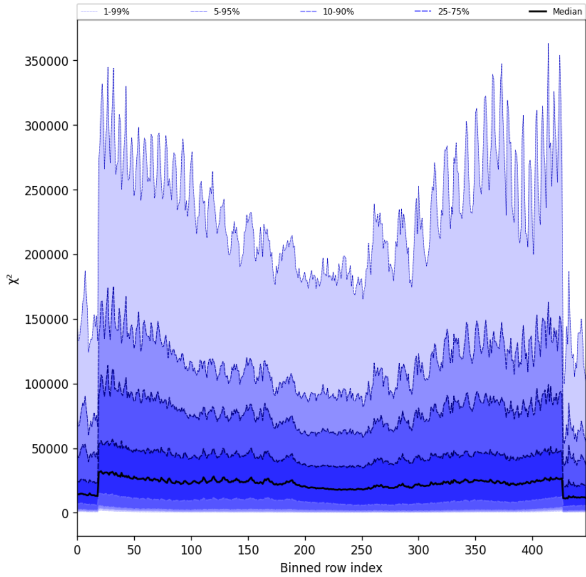
Figure 55: Along track statistics of “ \chi^2 ” for 2024-08-27 to 2024-08-29
