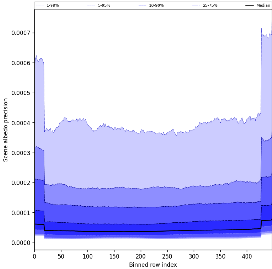
Figure 52: Along track statistics of “Scene albedo precision” for 2024-08-27 to 2024-08-29
