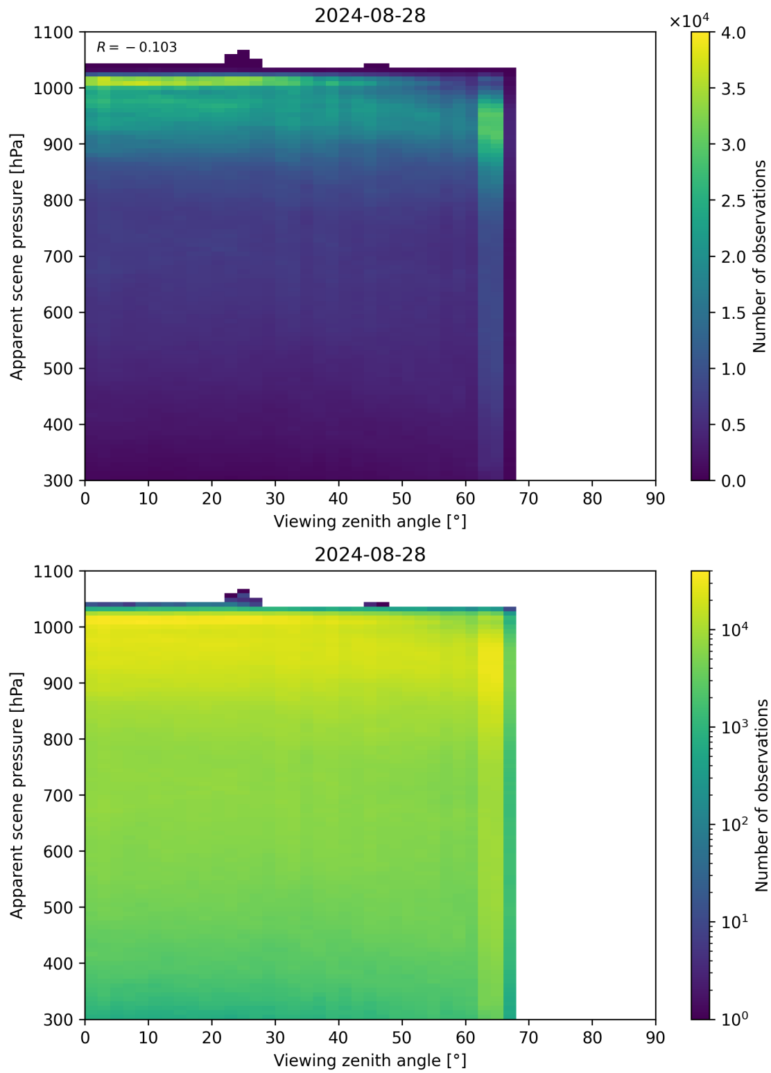
Figure 118: Scatter density plot of “Viewing zenith angle” against “Apparent scene pressure” for 2024-08-27 to 2024-08-29.
