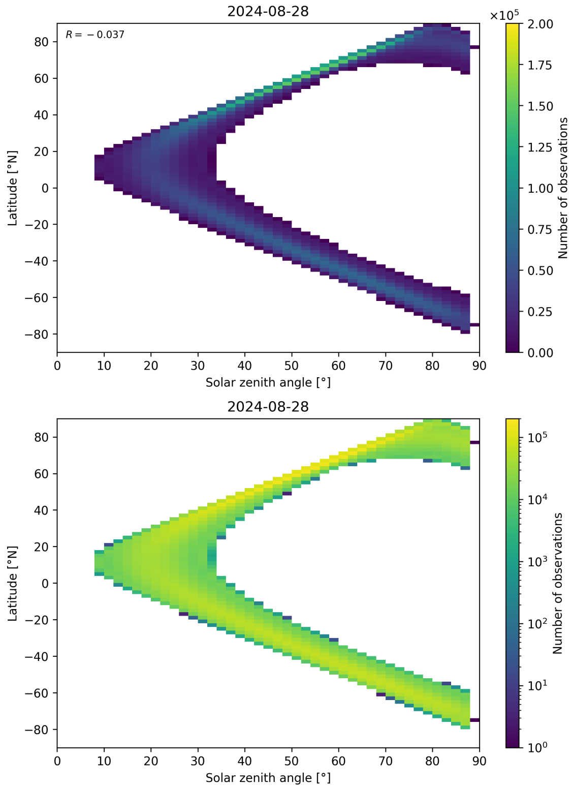
Figure 113: Scatter density plot of “Solar zenith angle” against “Latitude” for 2024-08-27 to 2024-08-29.
