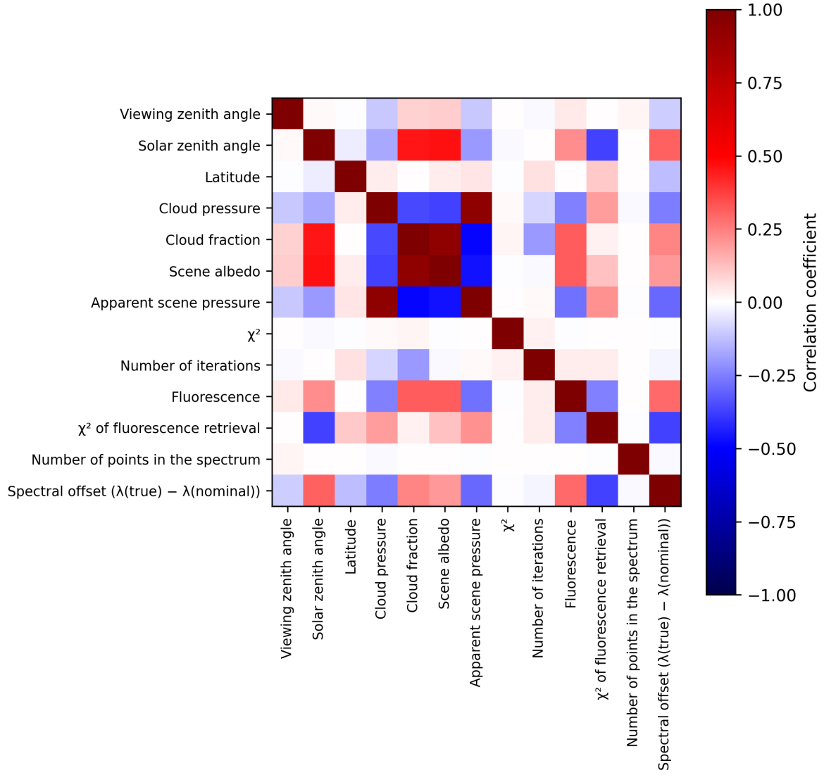
Figure 2: Map of correlation matrix for 2024-08-27 to 2024-08-29.
