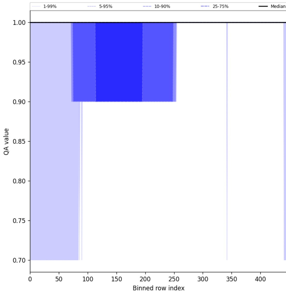
Figure 46: Along track statistics of “QA value” for 2024-08-27 to 2024-08-29
