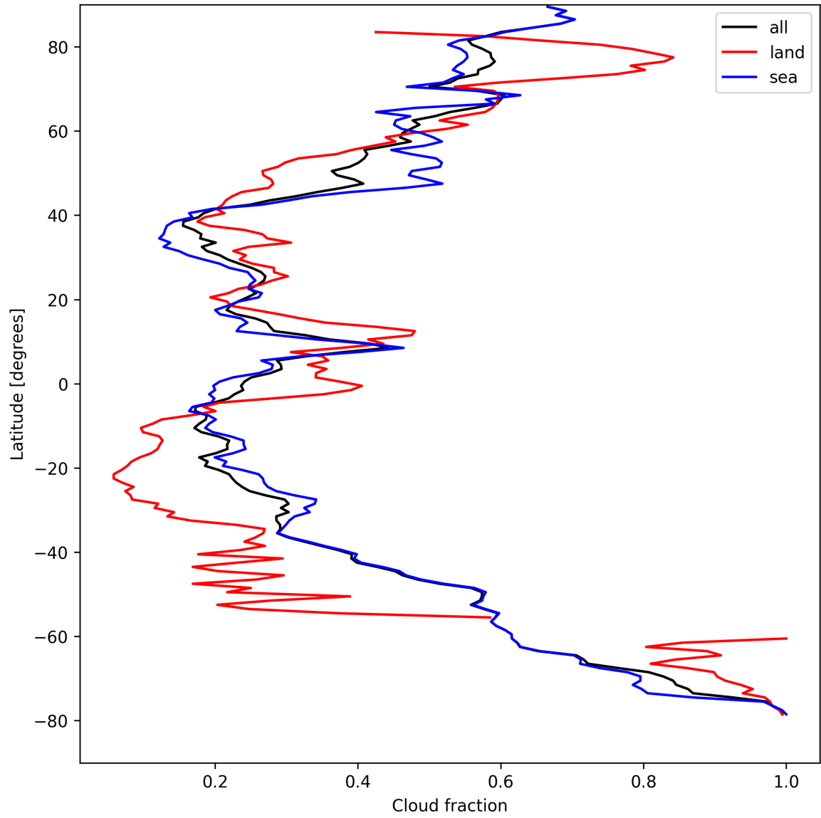
Figure 15: Zonal average of “Cloud fraction” for 2024-08-27 to 2024-08-29.
