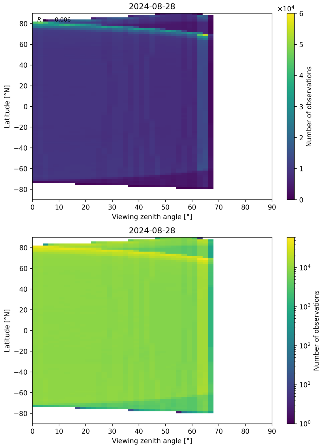
Figure 123: Scatter density plot of “Viewing zenith angle” against “Latitude” for 2024-08-27 to 2024-08-29.
