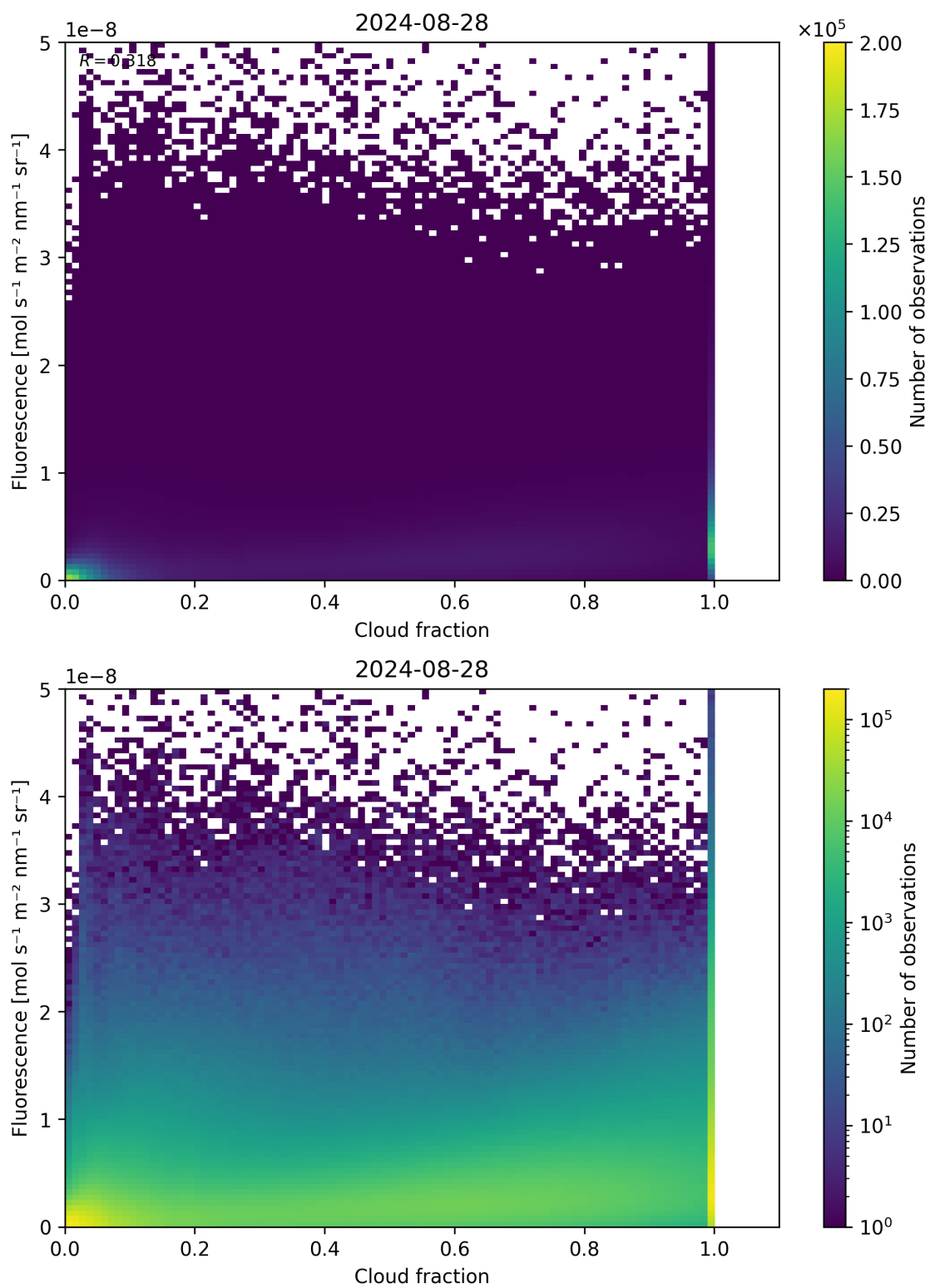
Figure 72: Scatter density plot of “Cloud fraction” against “Fluorescence” for 2024-08-27 to 2024-08-29.
