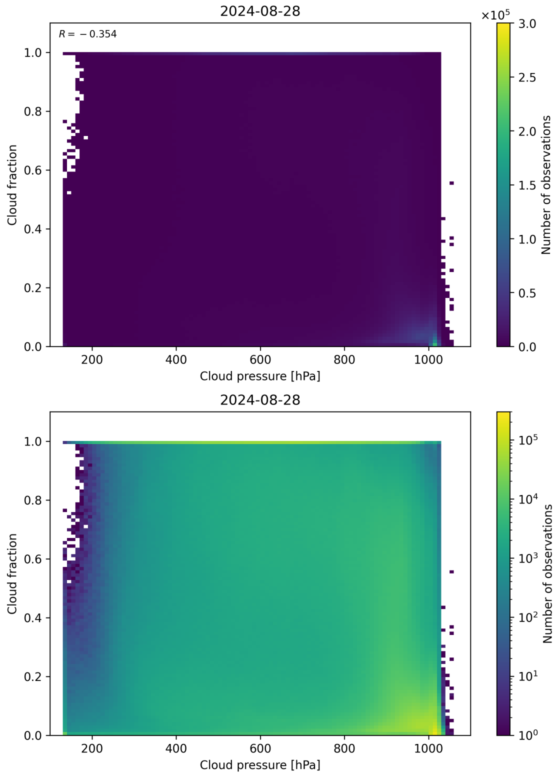
Figure 79: Scatter density plot of “Cloud pressure” against “Cloud fraction” for 2024-08-27 to 2024-08-29.
