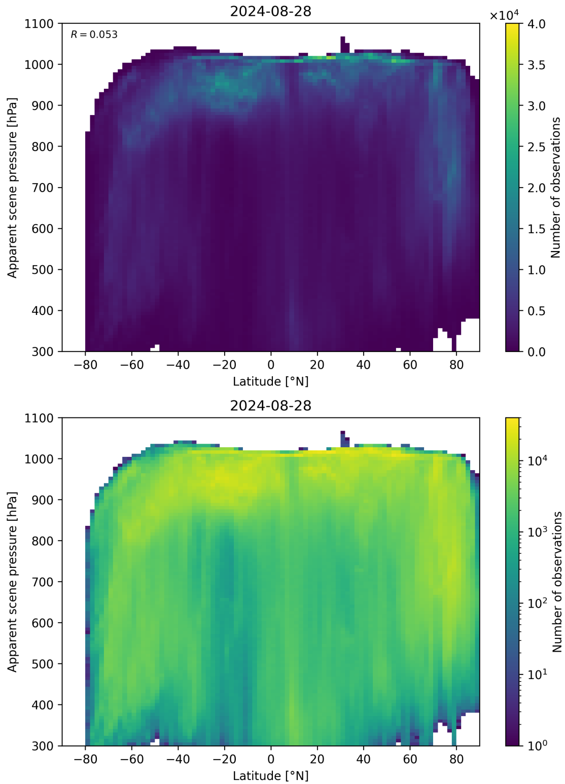
Figure 88: Scatter density plot of “Latitude” against “Apparent scene pressure” for 2024-08-27 to 2024-08-29.
