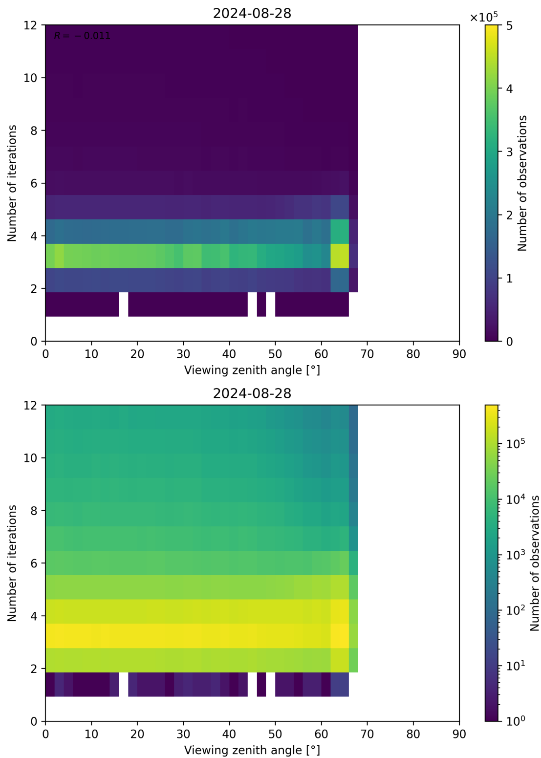
Figure 124: Scatter density plot of “Viewing zenith angle” against “Number of iterations” for 2024-08-27 to 2024-08-29.
