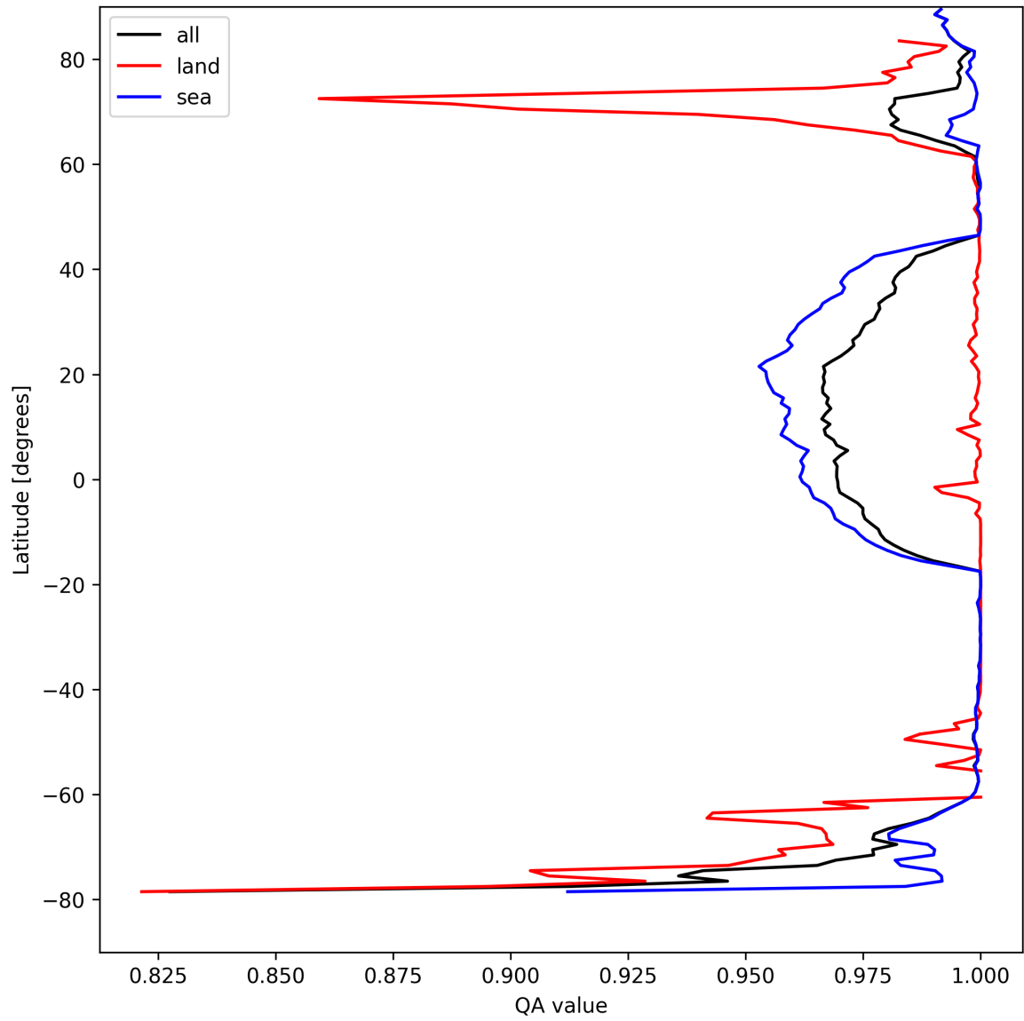
Figure 12: Zonal average of “QA value” for 2024-08-27 to 2024-08-29.
