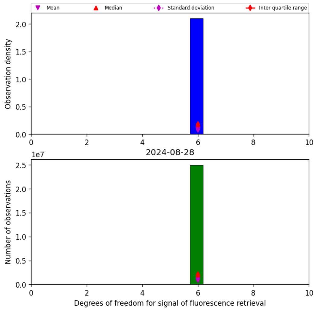
Figure 43: Histogram of "Degrees of freedom for signal of fluorescence retrieval" for 2024-08-27 to 2024-08-29
