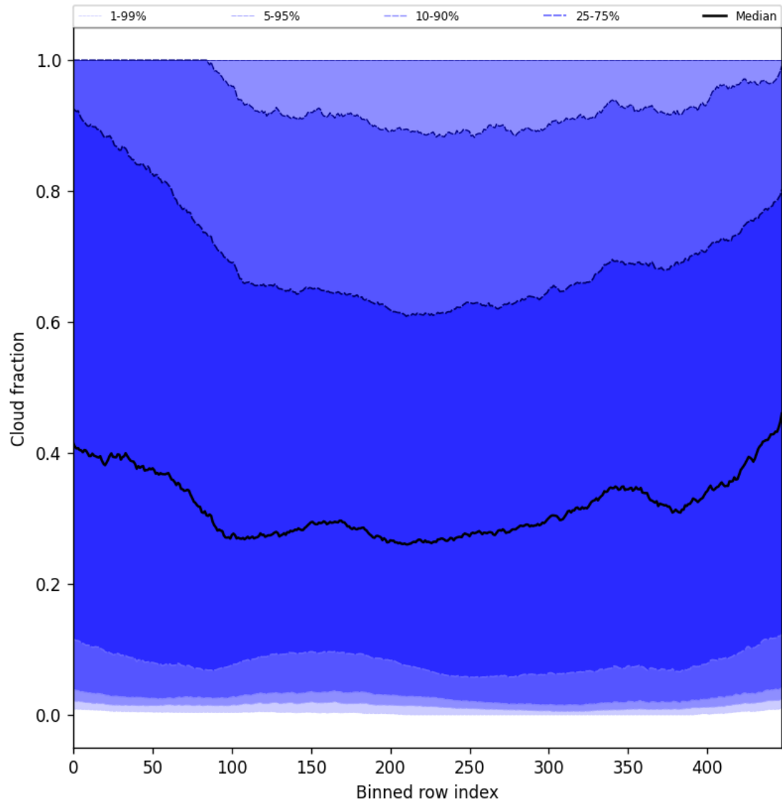
Figure 49: Along track statistics of “Cloud fraction” for 2024-08-27 to 2024-08-29
