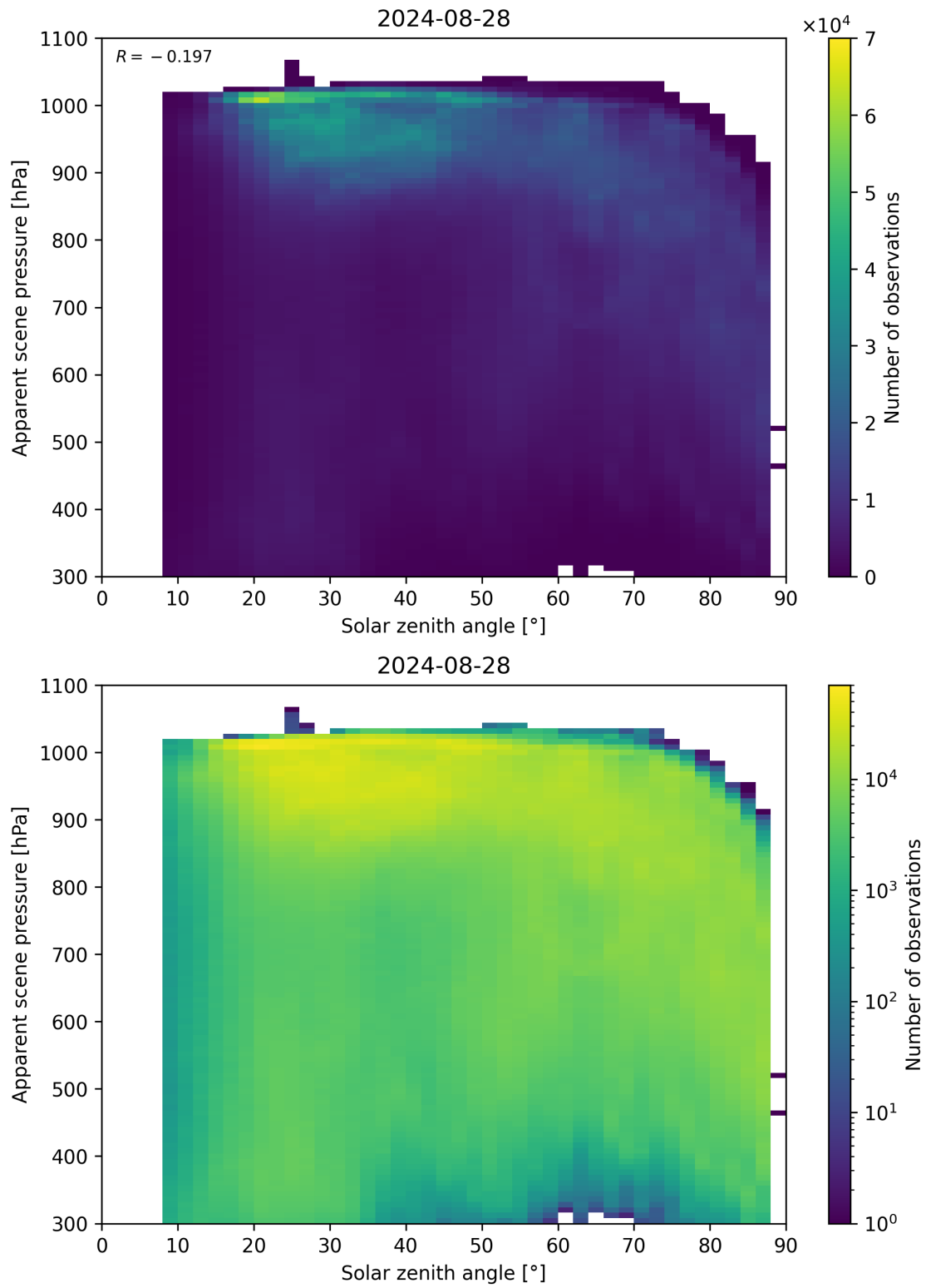
Figure 108: Scatter density plot of “Solar zenith angle” against “Apparent scene pressure” for 2024-08-27 to 2024-08-29.
