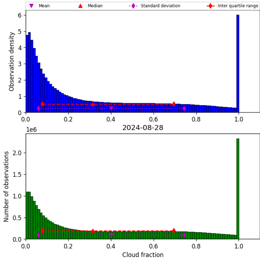
Figure 32: Histogram of “Cloud fraction” for 2024-08-27 to 2024-08-29
