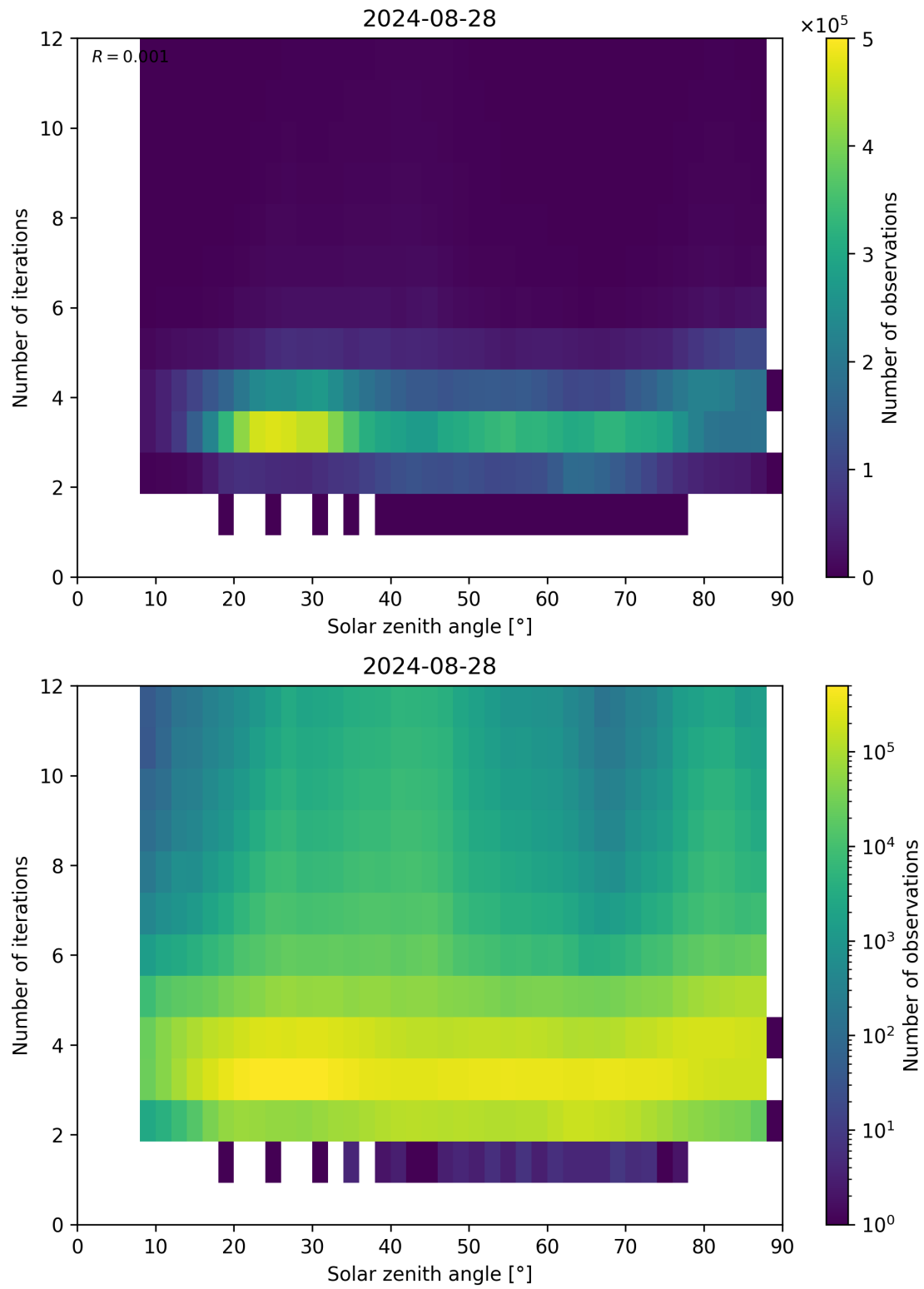
Figure 114: Scatter density plot of “Solar zenith angle” against “Number of iterations” for 2024-08-27 to 2024-08-29.
