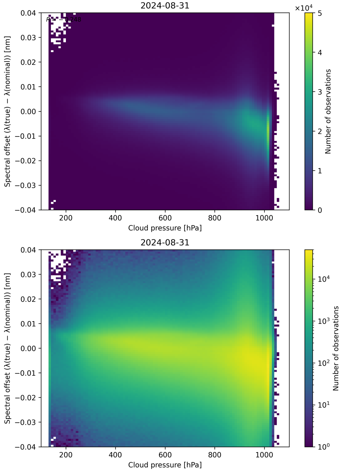
Figure 84: Scatter density plot of “Cloud pressure” against “Spectral offset ( \lambda_{\text{true}} - \lambda_{\text{nominal}} )” for 2024-08-30 to 2024-09-01.
