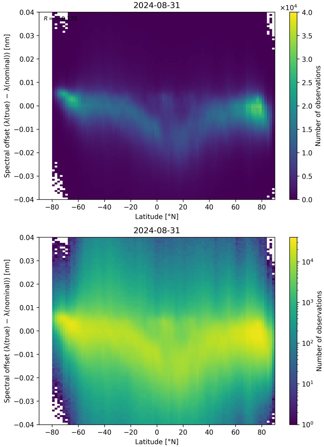
Figure 96: Scatter density plot of “Latitude” against “Spectral offset ( \lambda_{\text{true}} - \lambda_{\text{nominal}} )” for 2024-08-30 to 2024-09-01.
