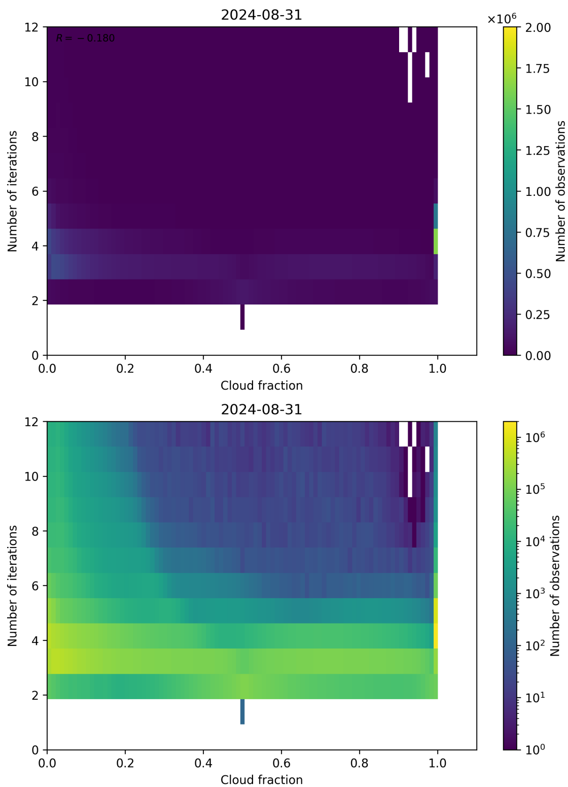
Figure 73: Scatter density plot of “Cloud fraction” against “Number of iterations” for 2024-08-30 to 2024-09-01.
