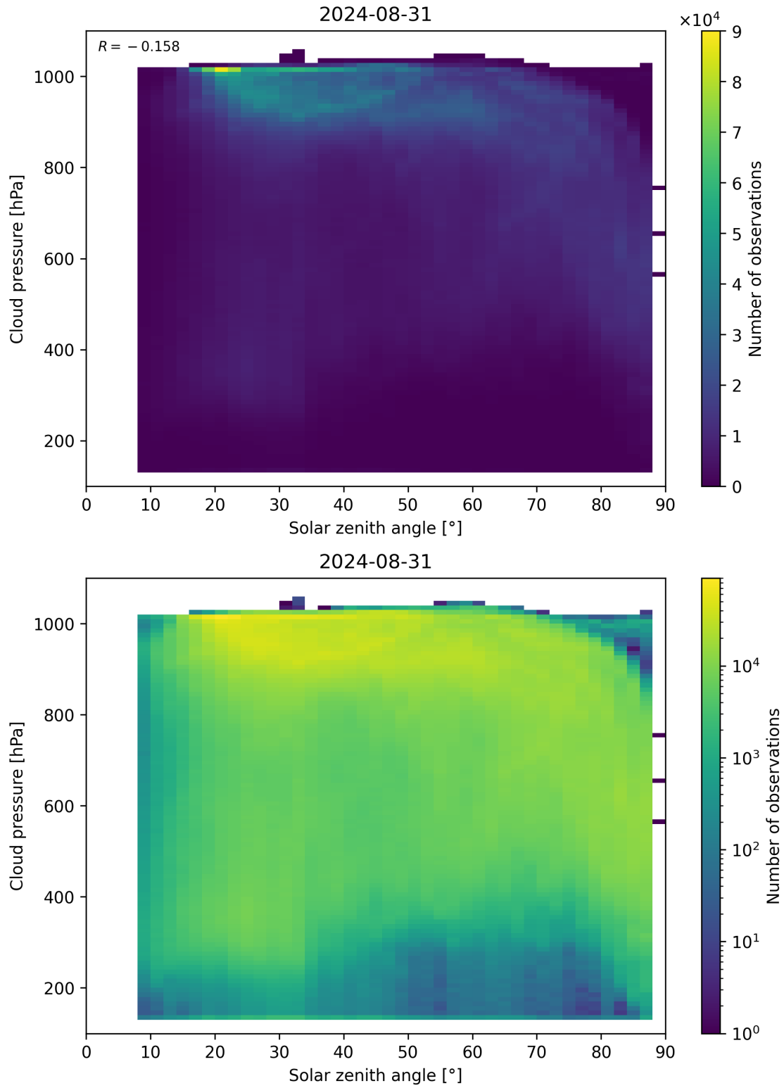
Figure 111: Scatter density plot of “Solar zenith angle” against “Cloud pressure” for 2024-08-30 to 2024-09-01.
