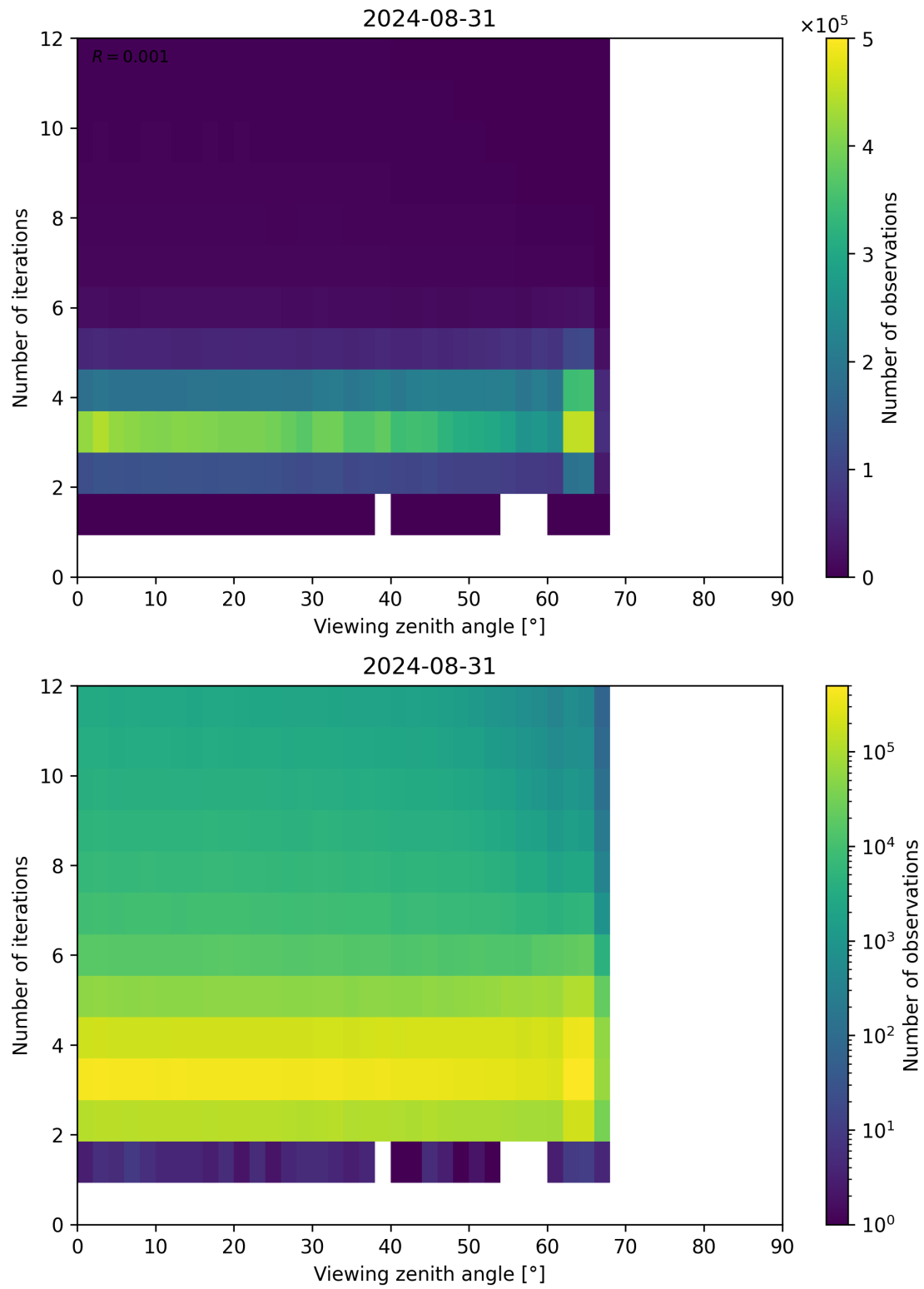
Figure 124: Scatter density plot of “Viewing zenith angle” against “Number of iterations” for 2024-08-30 to 2024-09-01.
