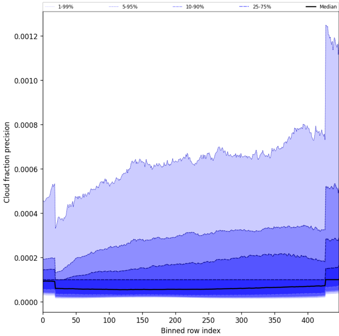
Figure 50: Along track statistics of “Cloud fraction precision” for 2024-08-30 to 2024-09-01
