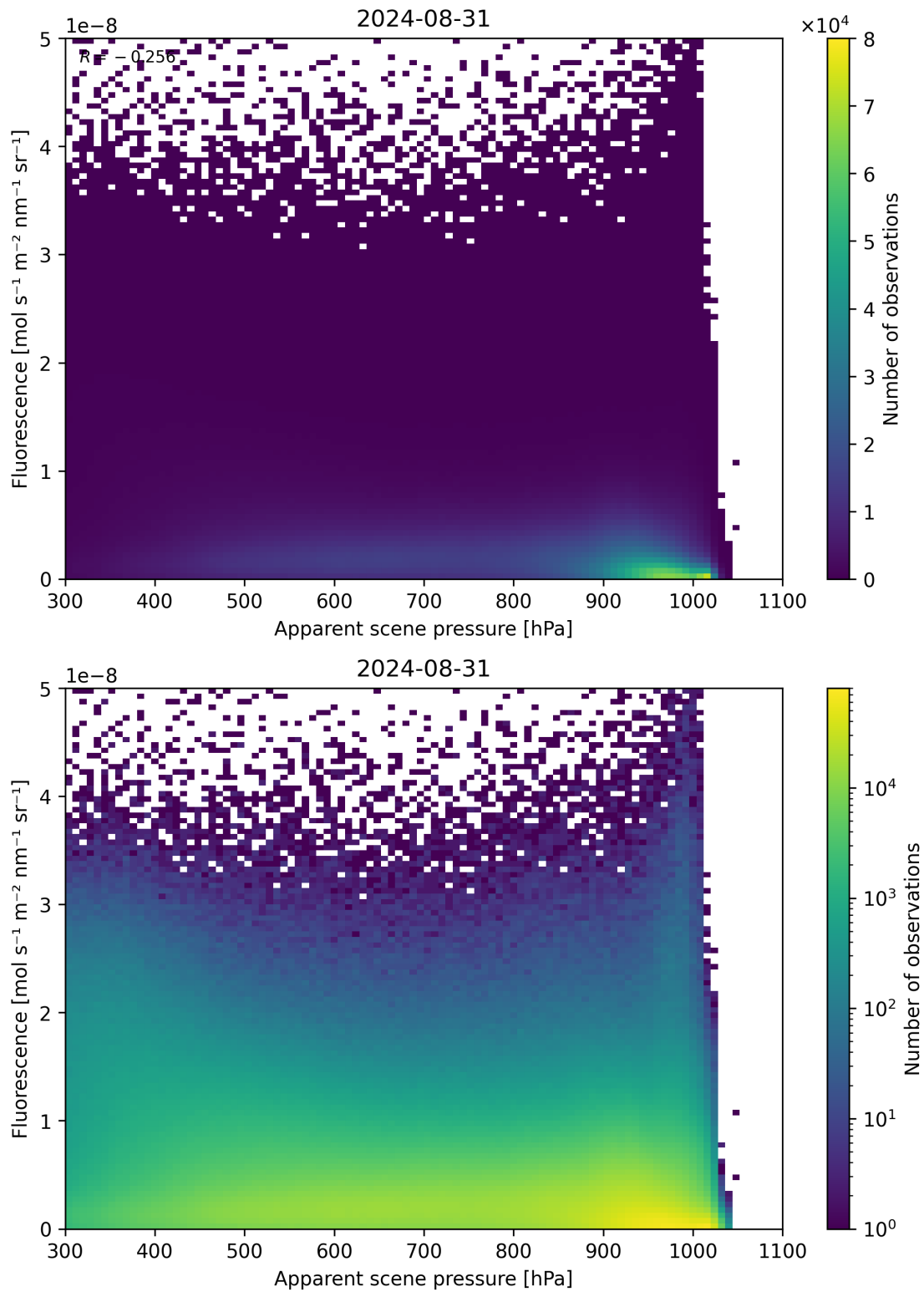
Figure 64: Scatter density plot of “Apparent scene pressure” against “Fluorescence” for 2024-08-30 to 2024-09-01.
