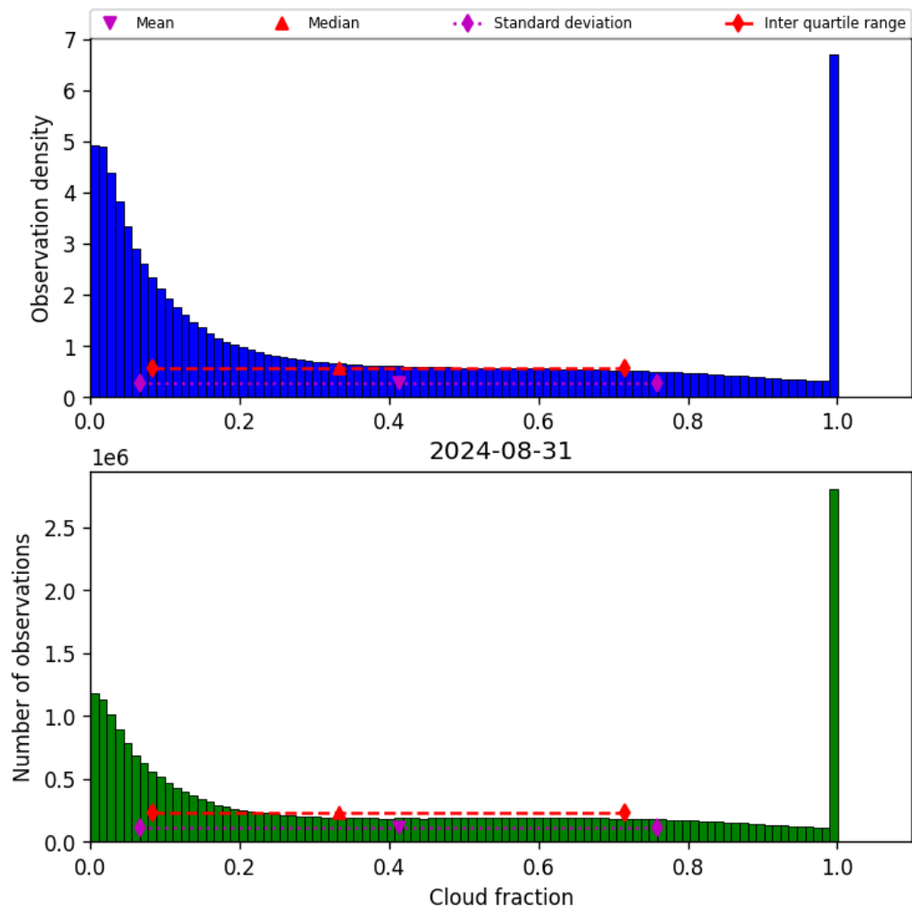
Figure 32: Histogram of “Cloud fraction” for 2024-08-30 to 2024-09-01
