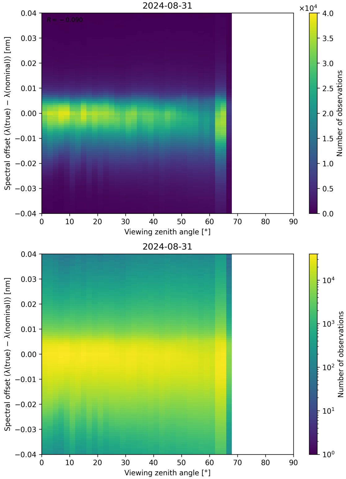
Figure 128: Scatter density plot of “Viewing zenith angle” against “Spectral offset ( \lambda_{\text{true}} - \lambda_{\text{nominal}} )” for 2024-08-30 to 2024-09-01.
