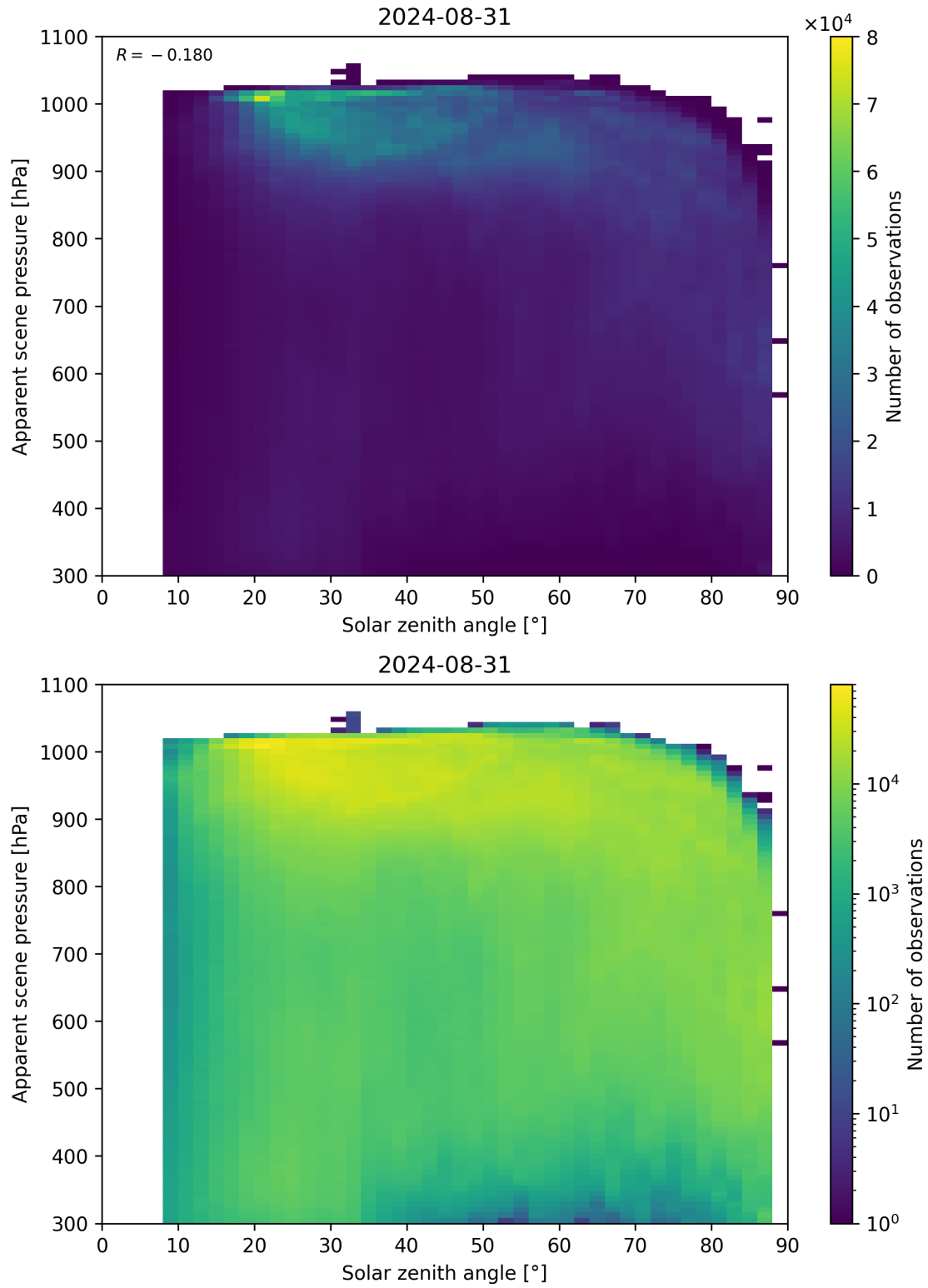
Figure 108: Scatter density plot of “Solar zenith angle” against “Apparent scene pressure” for 2024-08-30 to 2024-09-01.
