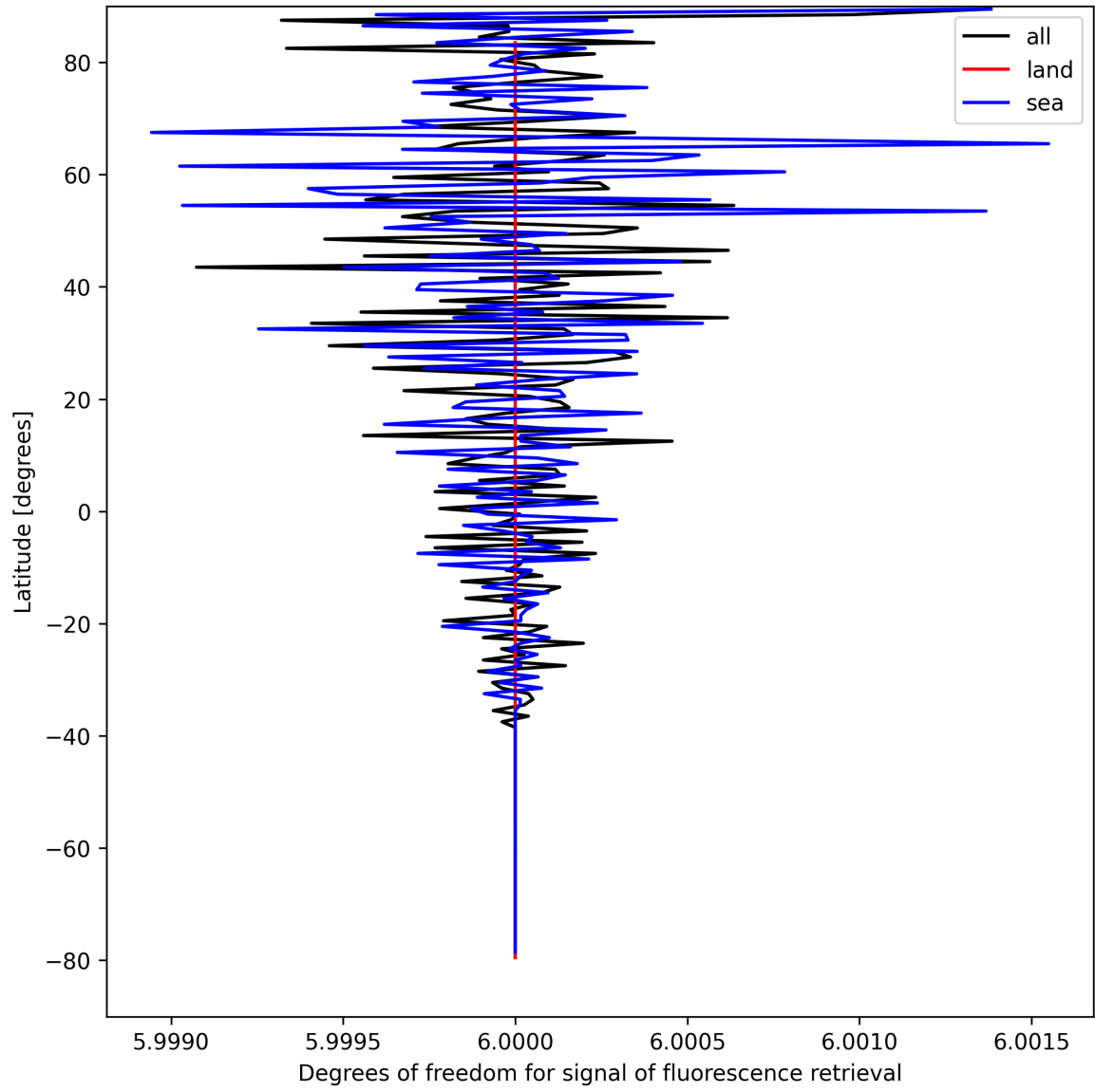
Figure 26: Zonal average of “Degrees of freedom for signal of fluorescence retrieval” for 2024-08-30 to 2024-09-01.
