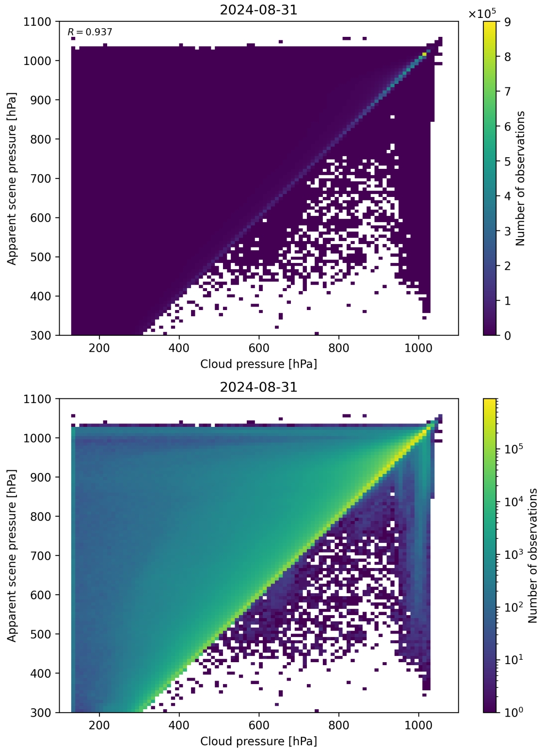
Figure 77: Scatter density plot of “Cloud pressure” against “Apparent scene pressure” for 2024-08-30 to 2024-09-01.
