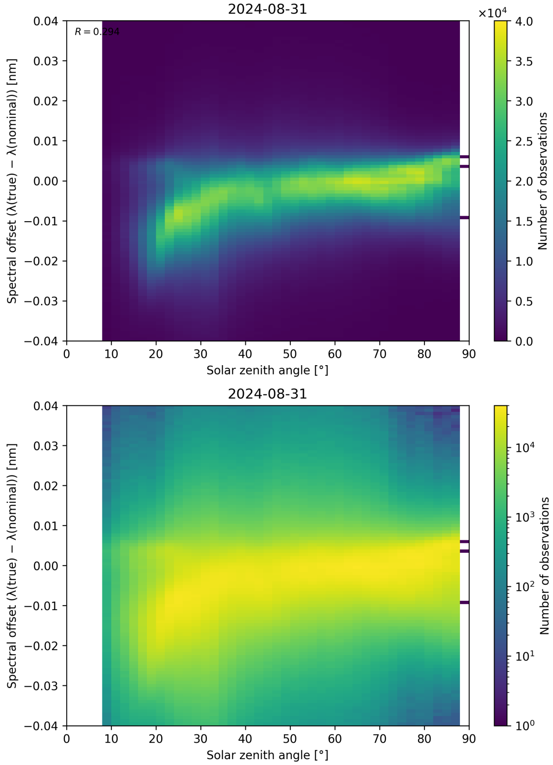
Figure 117: Scatter density plot of “Solar zenith angle” against “Spectral offset ( \lambda_{\text{true}} - \lambda_{\text{nominal}} )” for 2024-08-30 to 2024-09-01.
