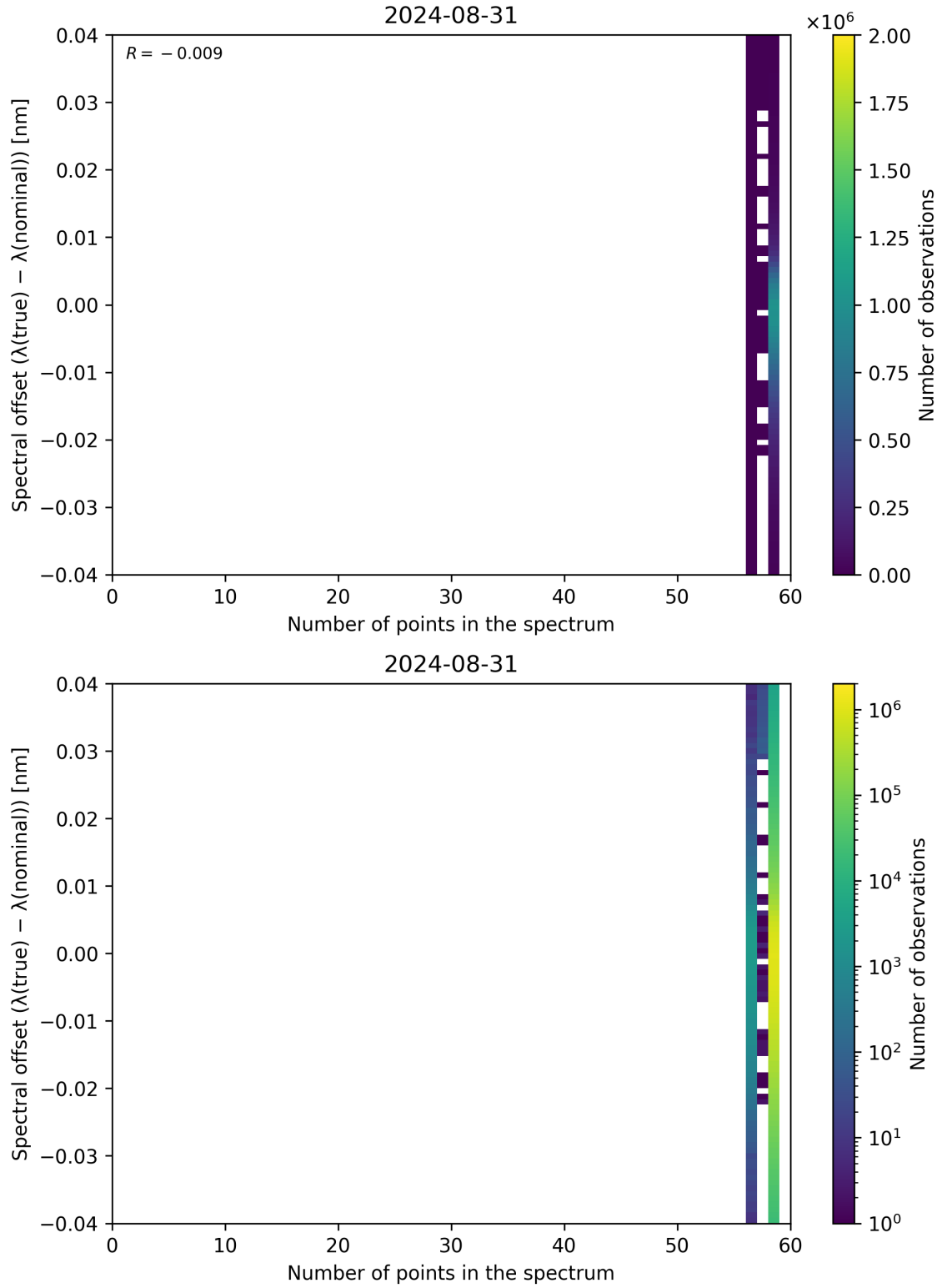
Figure 101: Scatter density plot of “Number of points in the spectrum” against “Spectral offset ( \lambda_{\text{true}} - \lambda_{\text{nominal}} )” for 2024-08-30 to 2024-09-01.
