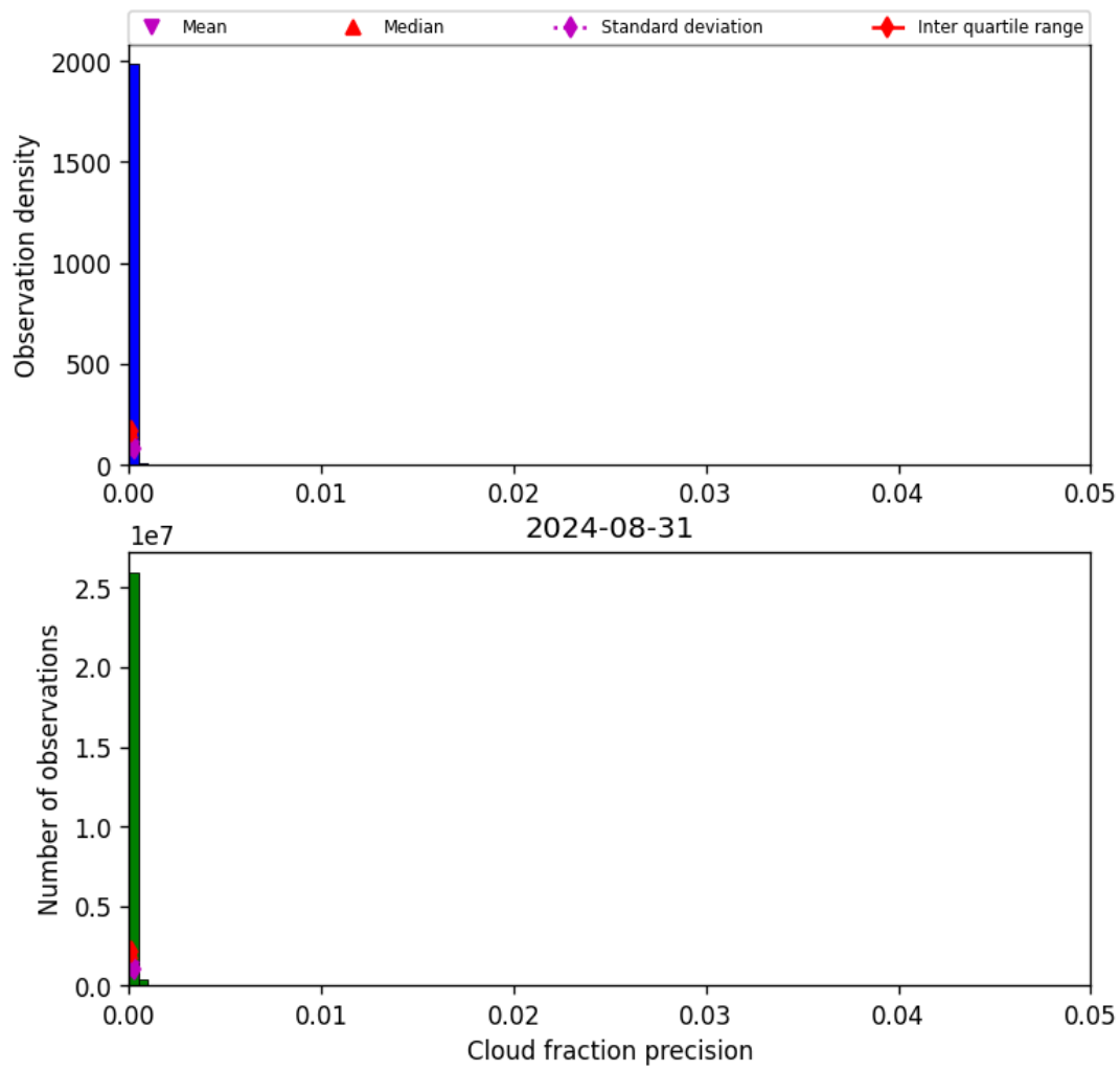
Figure 33: Histogram of “Cloud fraction precision” for 2024-08-30 to 2024-09-01
