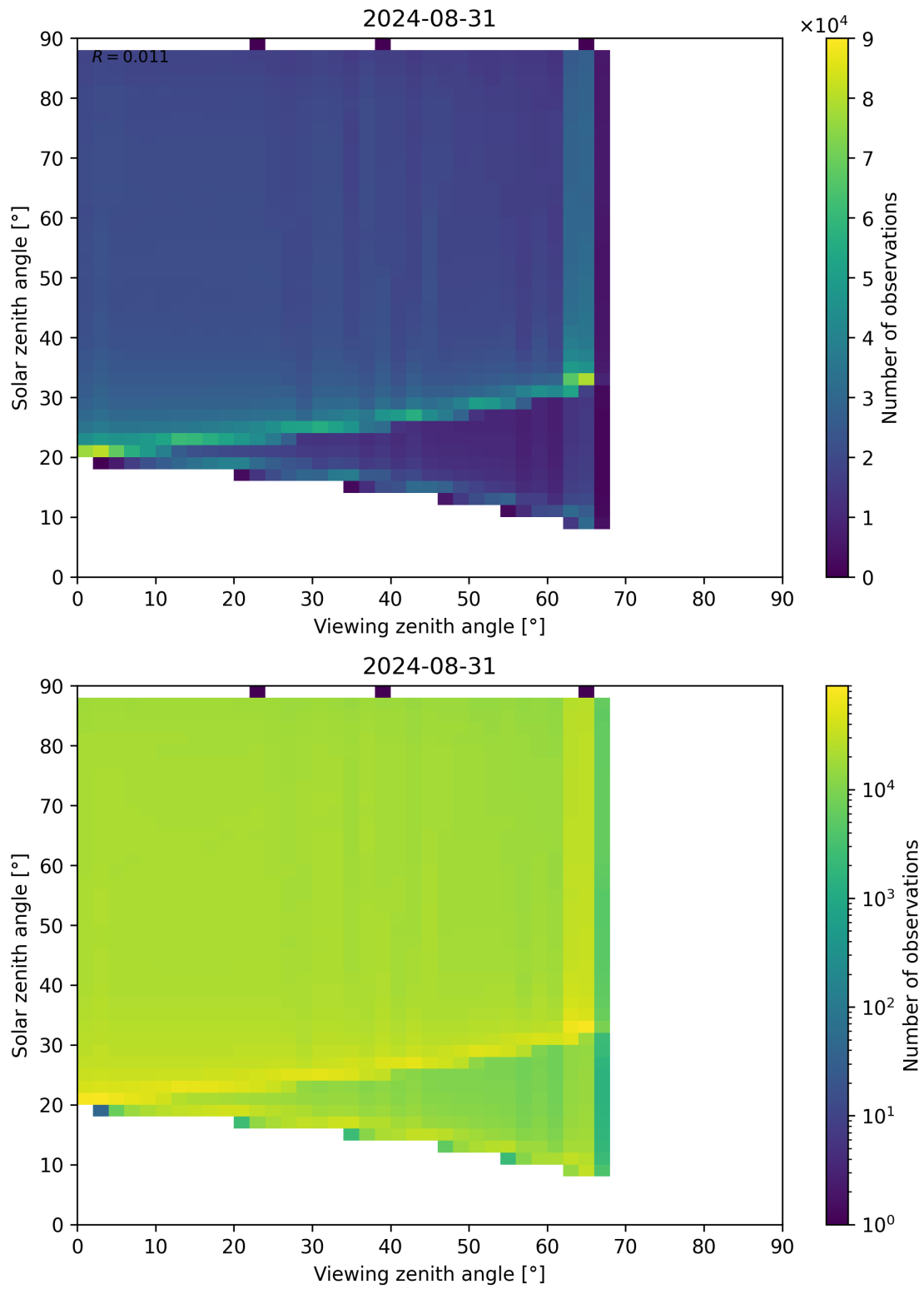
Figure 127: Scatter density plot of “Viewing zenith angle” against “Solar zenith angle” for 2024-08-30 to 2024-09-01.
