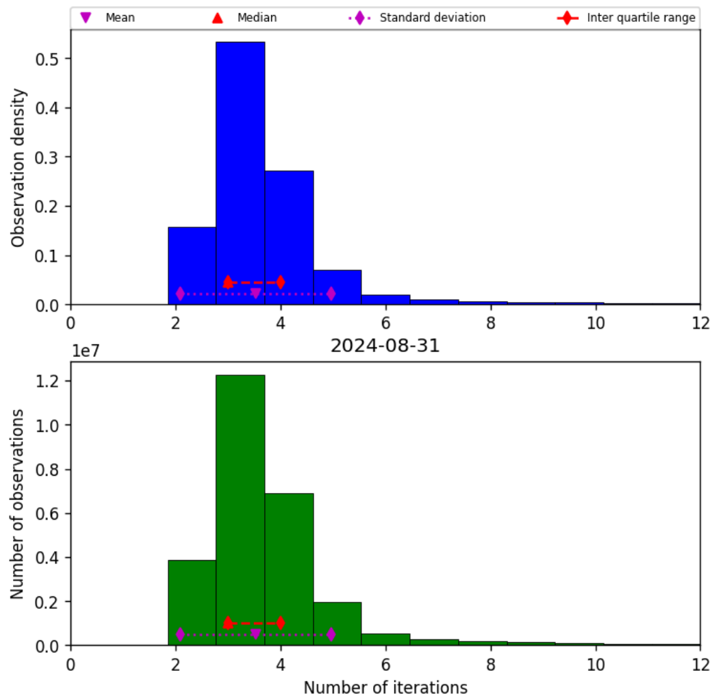
Figure 39: Histogram of “Number of iterations” for 2024-08-30 to 2024-09-01
