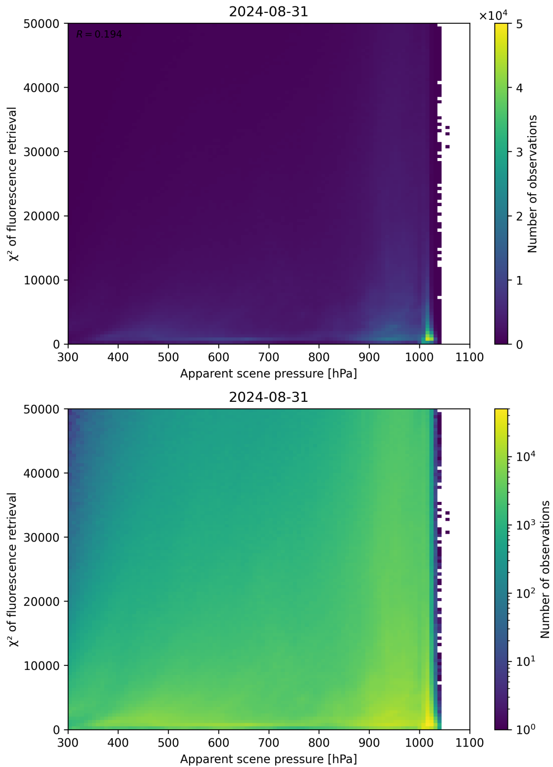
Figure 63: Scatter density plot of “Apparent scene pressure” against “ \chi^2 of fluorescence retrieval” for 2024-08-30 to 2024-09-01.
