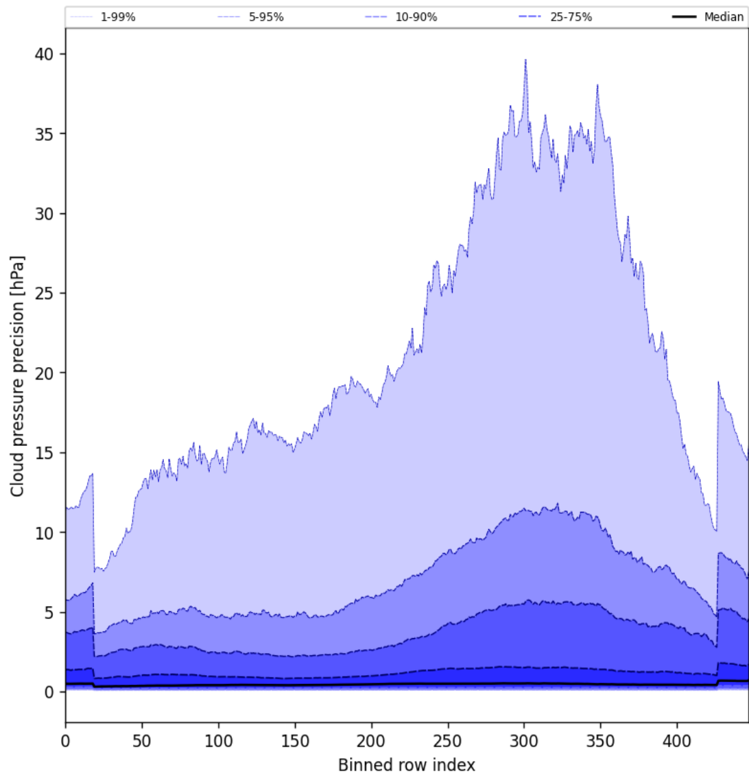
Figure 48: Along track statistics of “Cloud pressure precision” for 2024-08-30 to 2024-09-01
