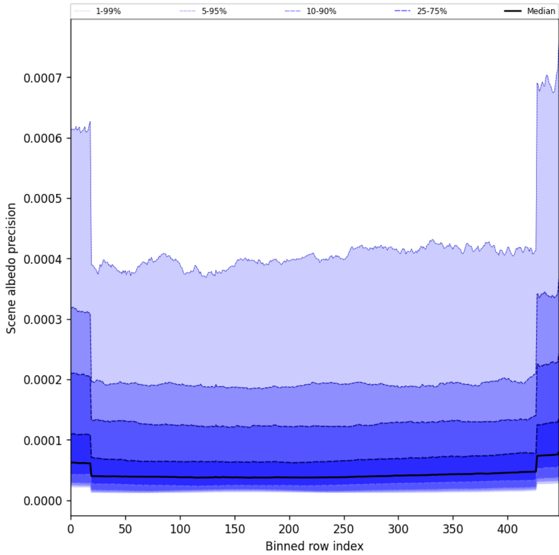
Figure 52: Along track statistics of “Scene albedo precision” for 2024-08-30 to 2024-09-01
