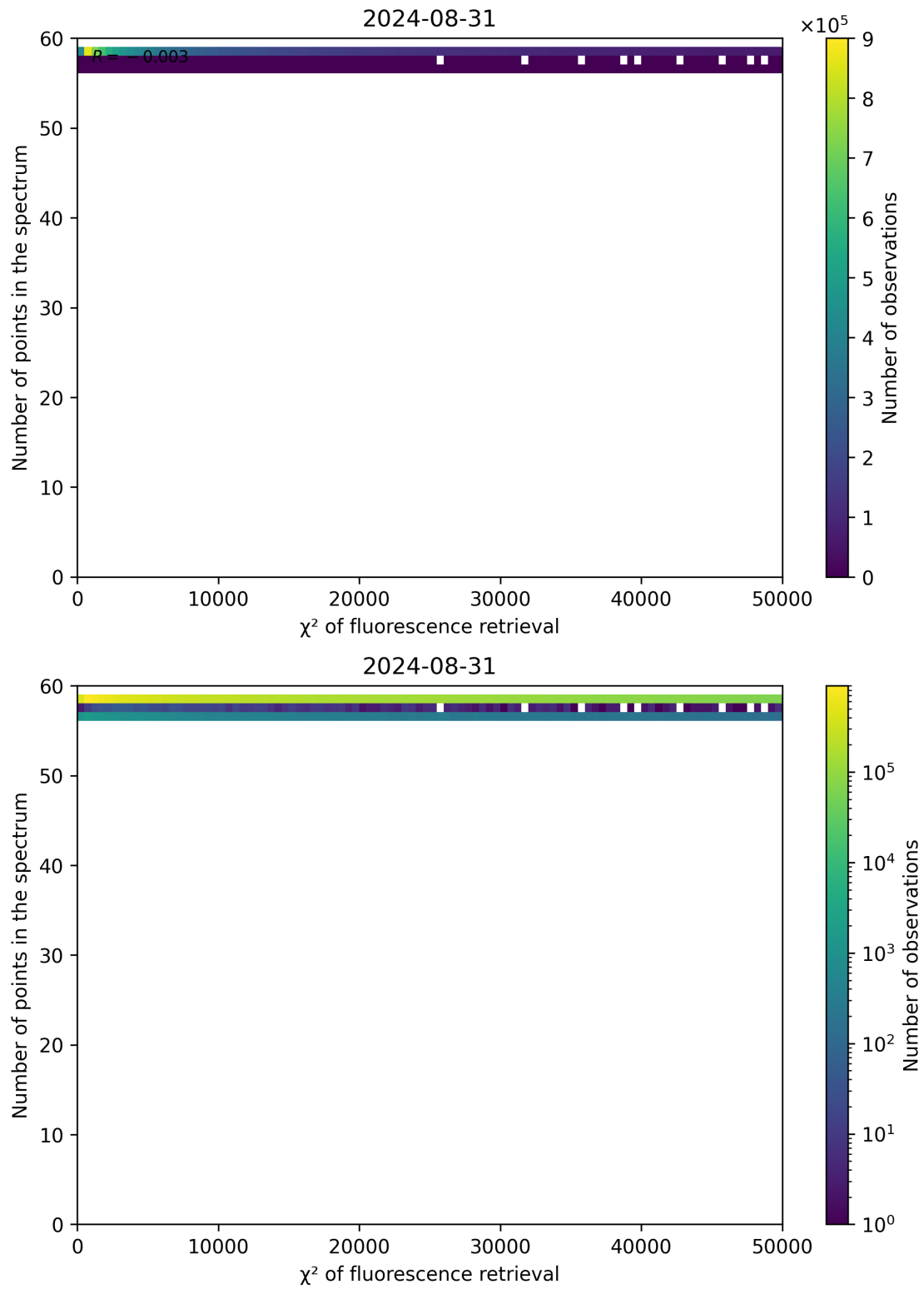
Figure 68: Scatter density plot of “ \chi^2 of fluorescence retrieval” against “Number of points in the spectrum” for 2024-08-30 to 2024-09-01.
