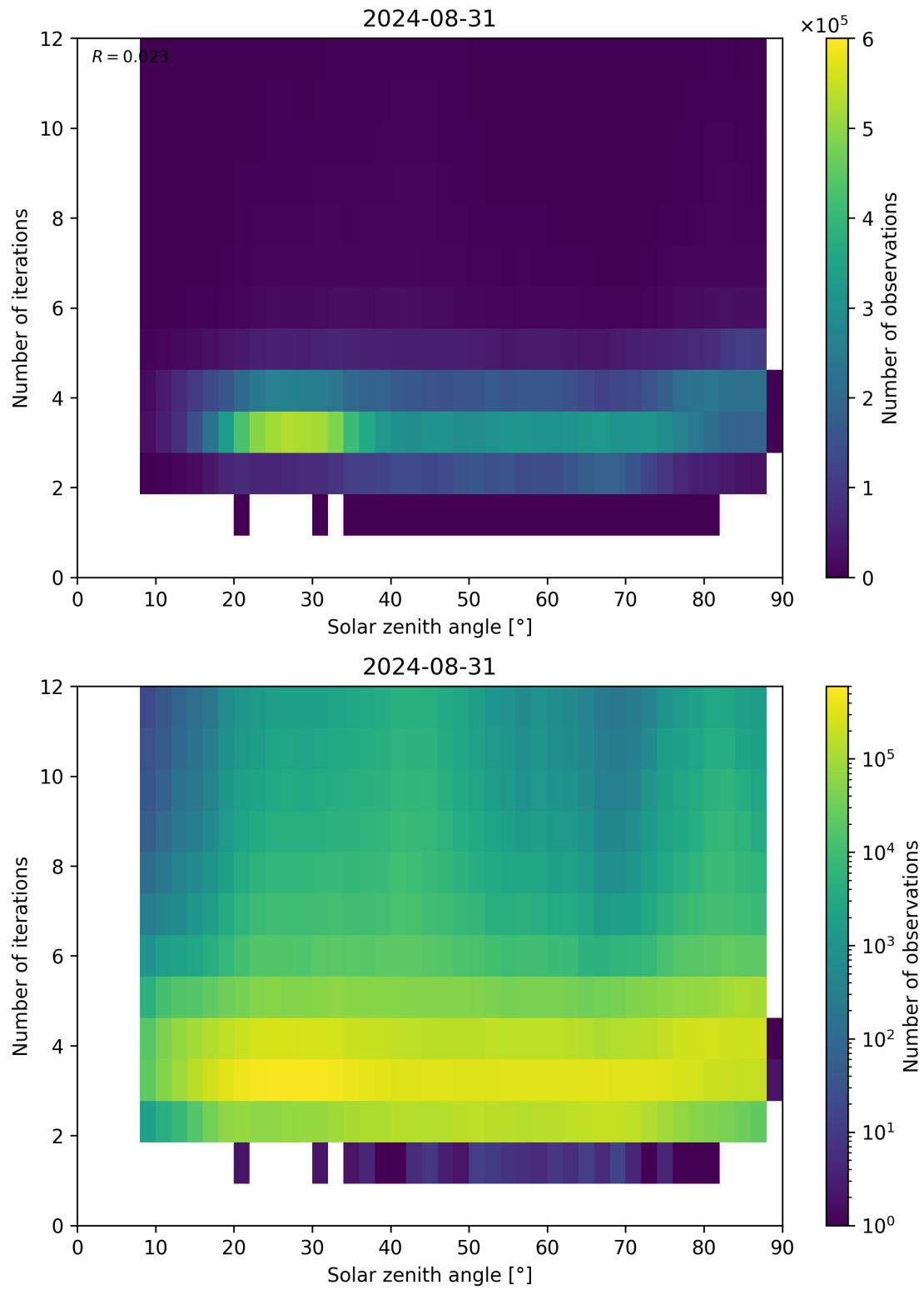
Figure 114: Scatter density plot of “Solar zenith angle” against “Number of iterations” for 2024-08-30 to 2024-09-01.
