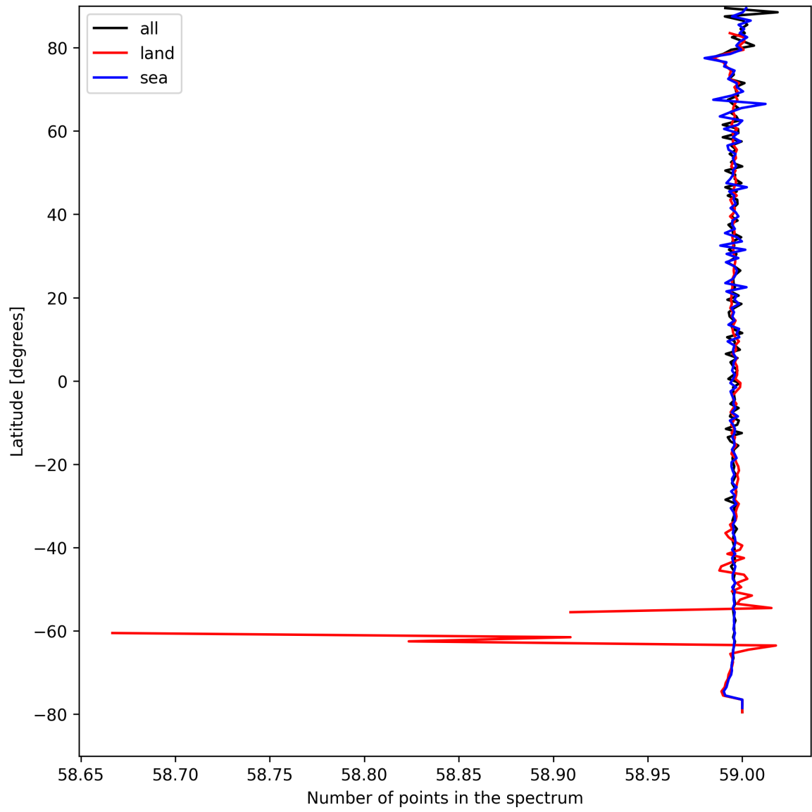
Figure 27: Zonal average of “Number of points in the spectrum” for 2024-08-30 to 2024-09-01.
