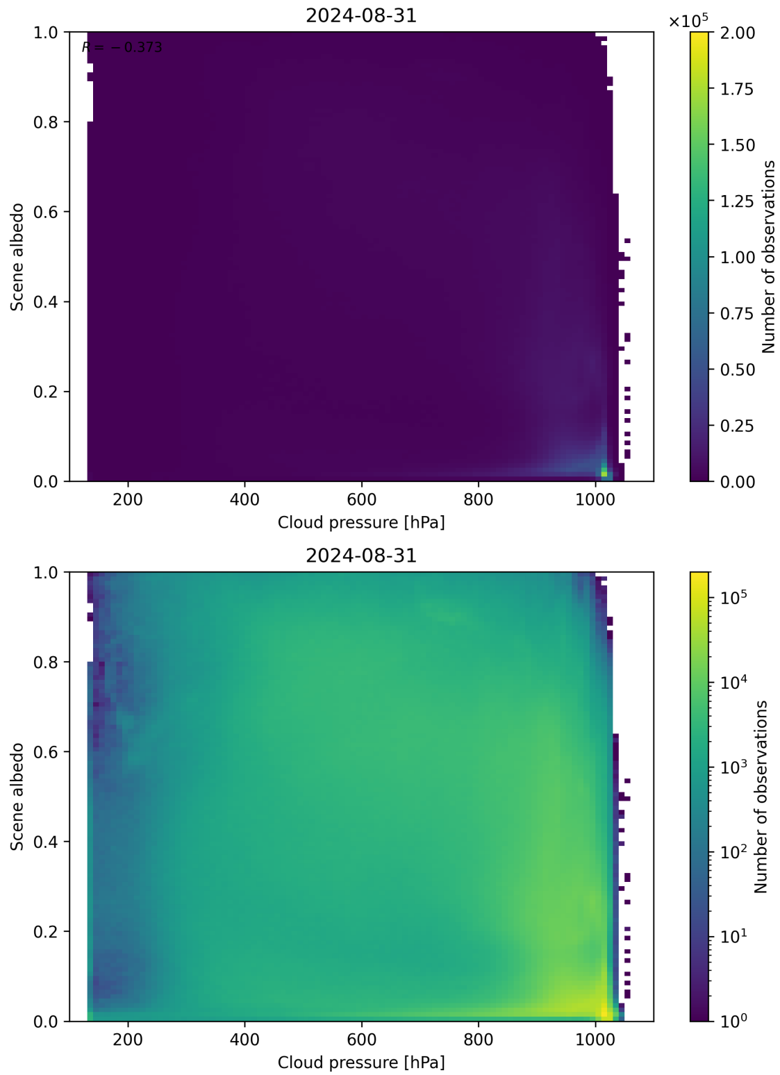
Figure 83: Scatter density plot of “Cloud pressure” against “Scene albedo” for 2024-08-30 to 2024-09-01.
