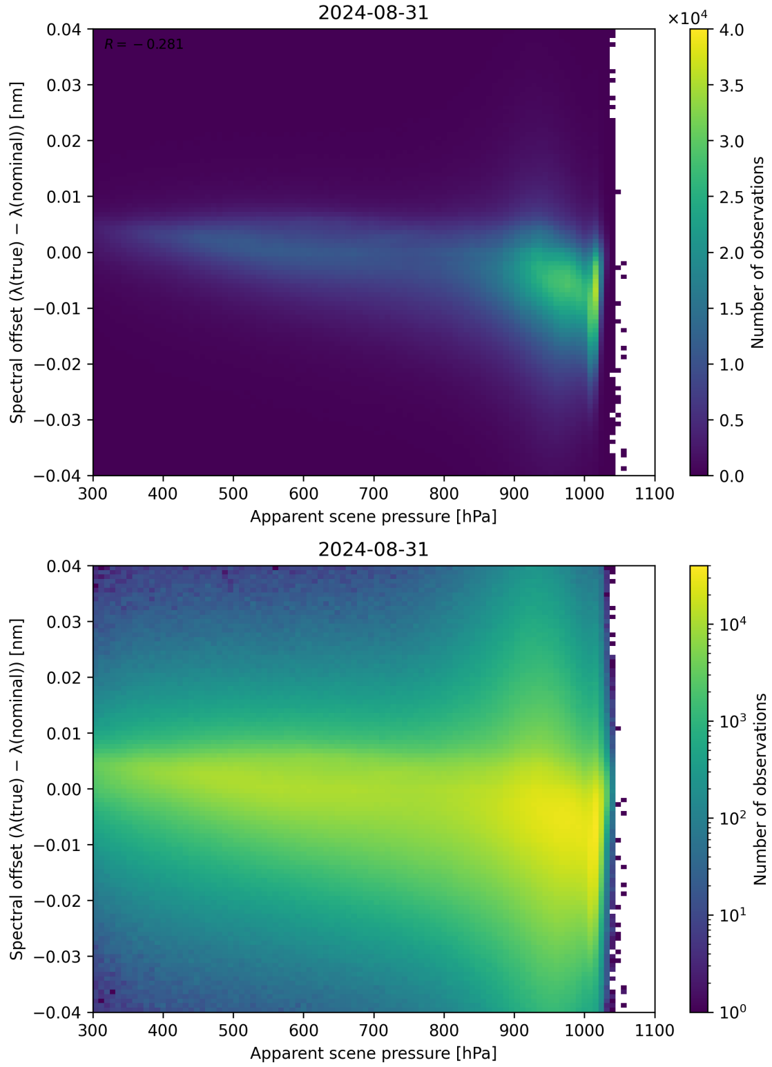
Figure 67: Scatter density plot of “Apparent scene pressure” against “Spectral offset ( \lambda_{\text{true}} - \lambda_{\text{nominal}} )” for 2024-08-30 to 2024-09-01.
