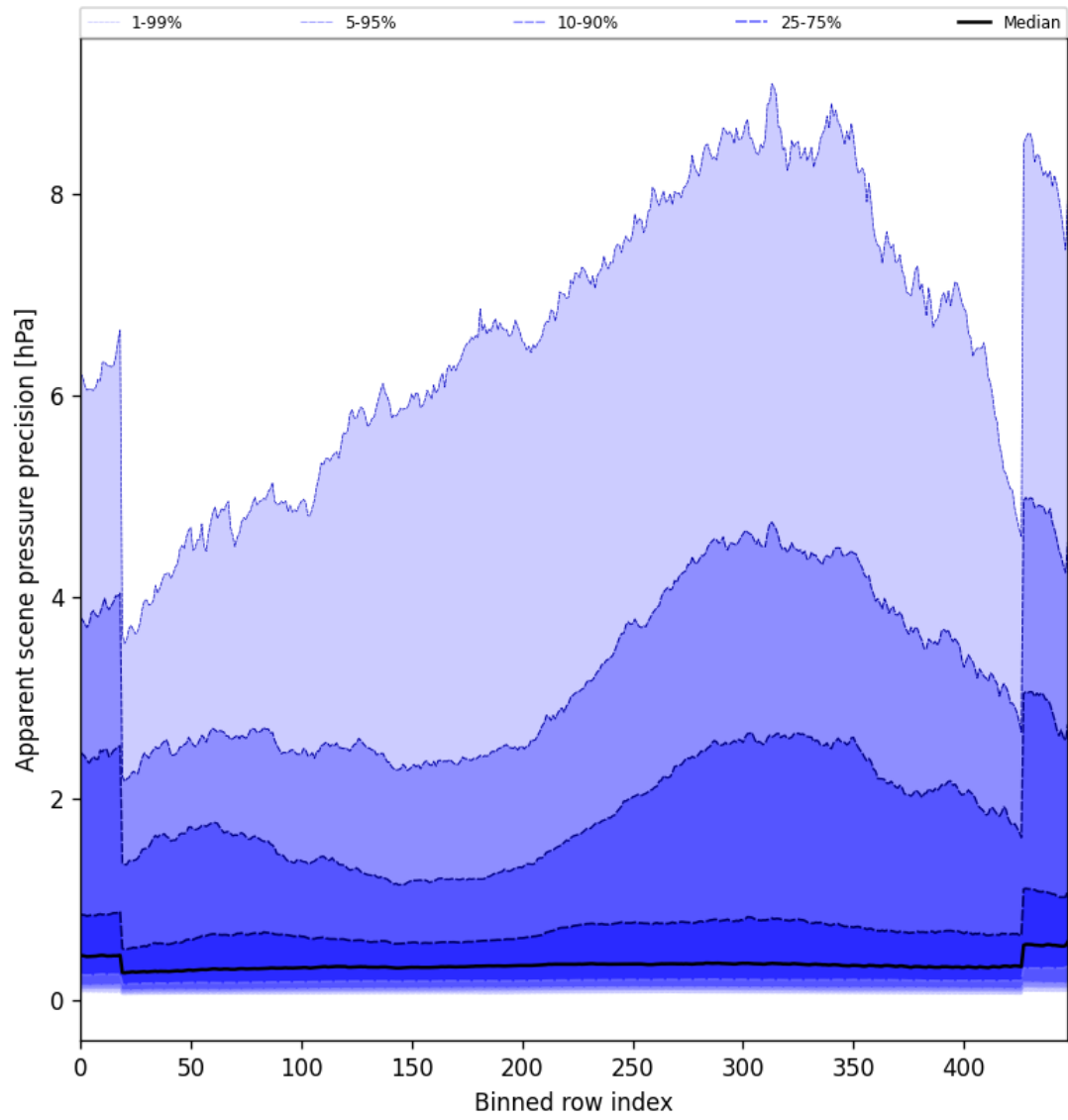
Figure 54: Along track statistics of “Apparent scene pressure precision” for 2024-08-30 to 2024-09-01
