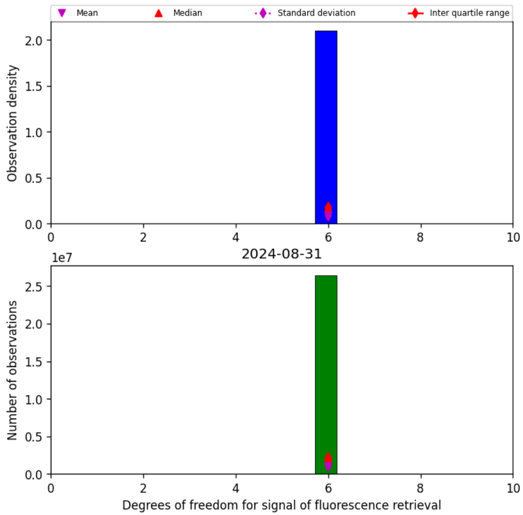
Figure 43: Histogram of "Degrees of freedom for signal of fluorescence retrieval" for 2024-08-30 to 2024-09-01
