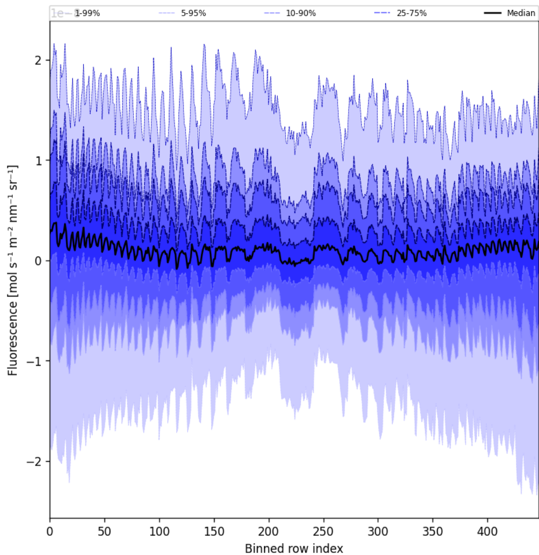
Figure 57: Along track statistics of “Fluorescence” for 2024-08-30 to 2024-09-01
