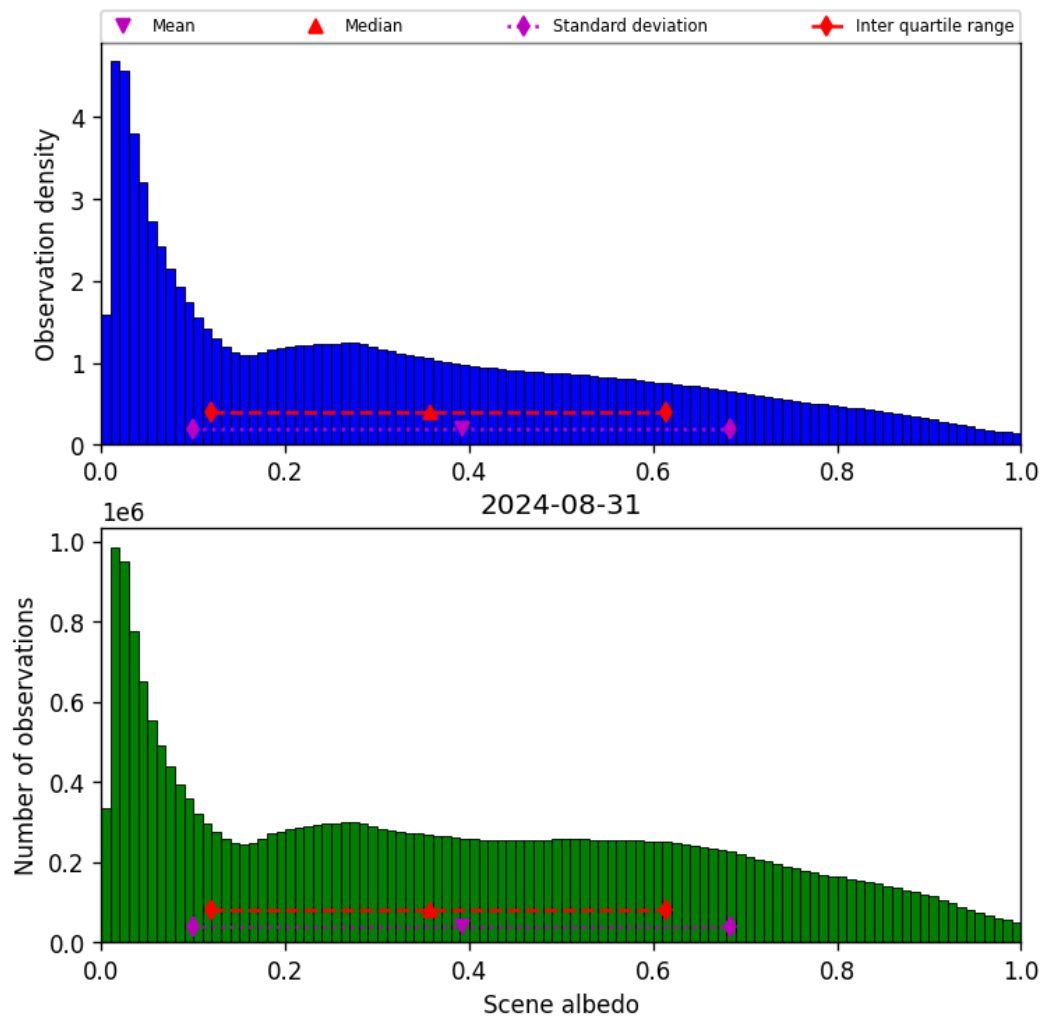
Figure 34: Histogram of “Scene albedo” for 2024-08-30 to 2024-09-01
