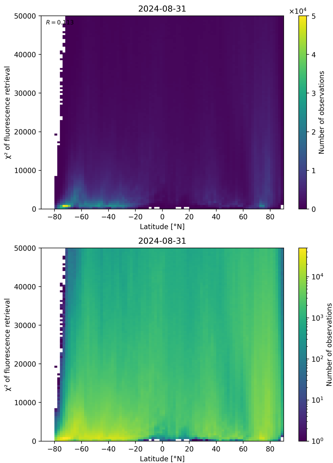
Figure 89: Scatter density plot of “Latitude” against “ \chi^2 of fluorescence retrieval” for 2024-08-30 to 2024-09-01.
