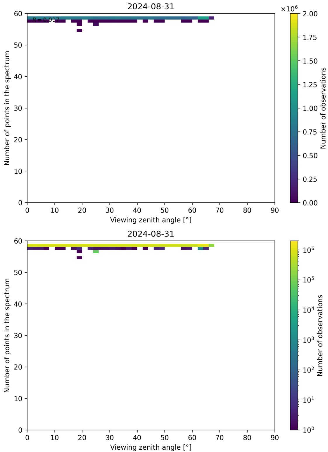
Figure 125: Scatter density plot of “Viewing zenith angle” against “Number of points in the spectrum” for 2024-08-30 to 2024-09-01.
