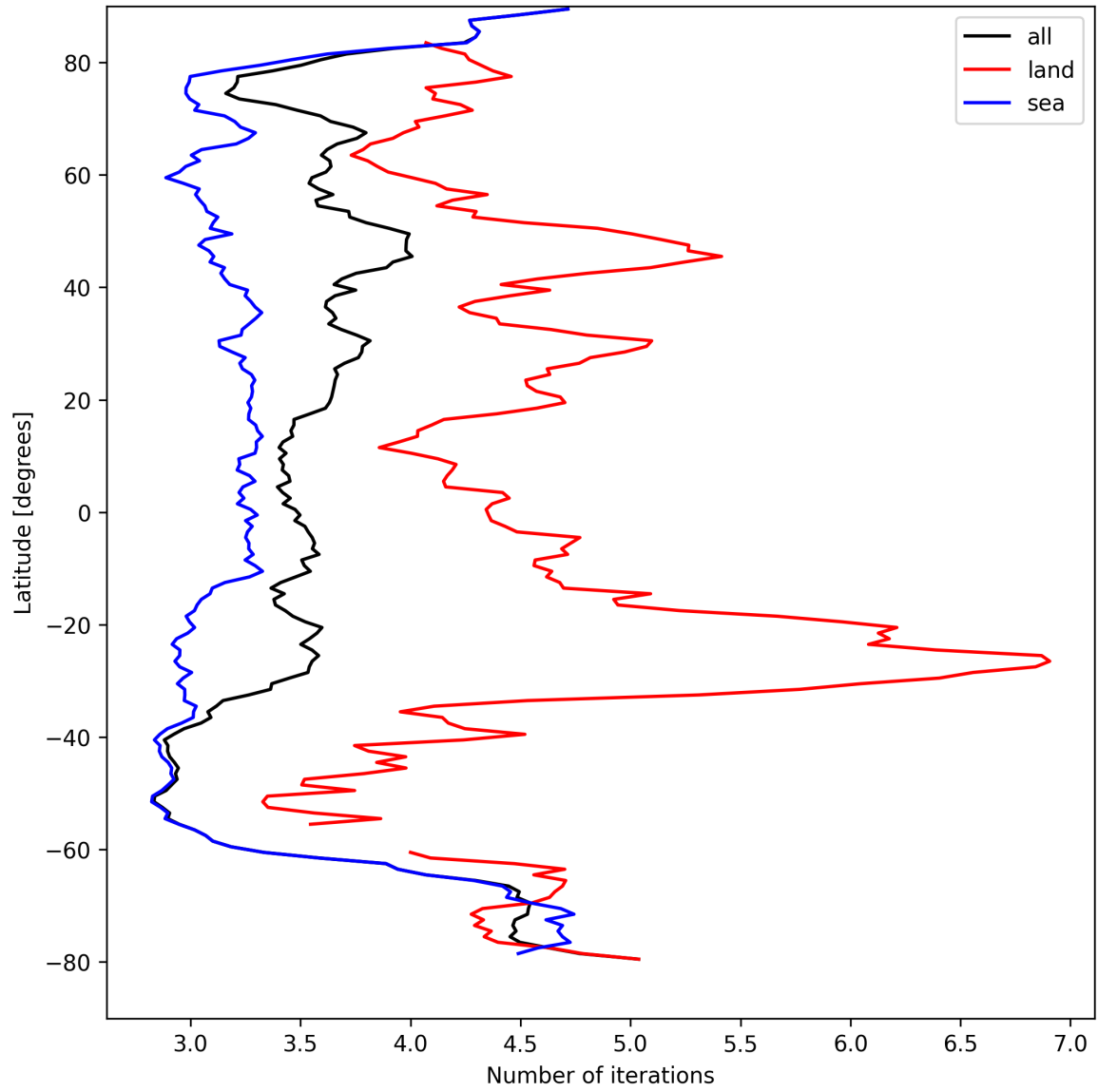
Figure 22: Zonal average of “Number of iterations” for 2024-08-30 to 2024-09-01.
