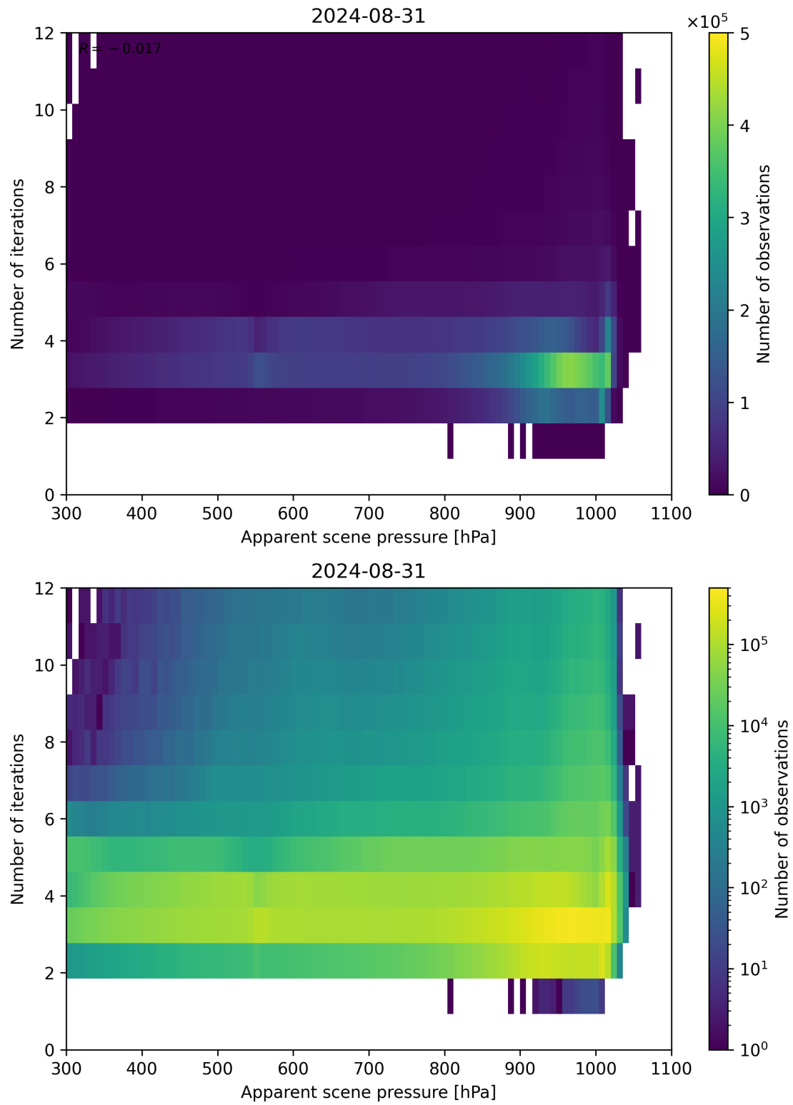
Figure 65: Scatter density plot of “Apparent scene pressure” against “Number of iterations” for 2024-08-30 to 2024-09-01.
