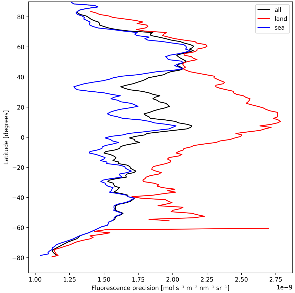
Figure 24: Zonal average of “Fluorescence precision” for 2024-08-30 to 2024-09-01.
