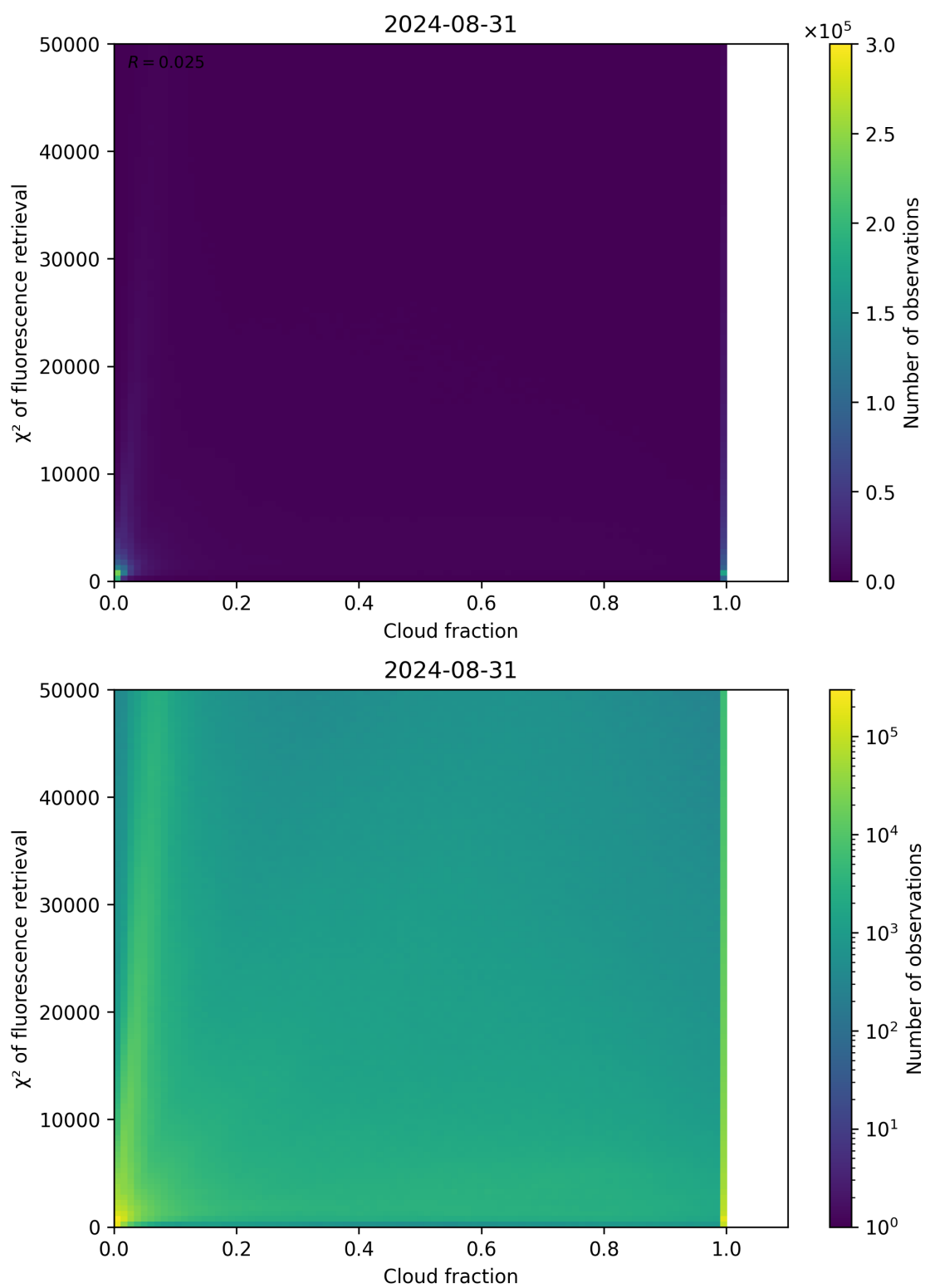
Figure 71: Scatter density plot of “Cloud fraction” against “ \chi^2 of fluorescence retrieval” for 2024-08-30 to 2024-09-01.
