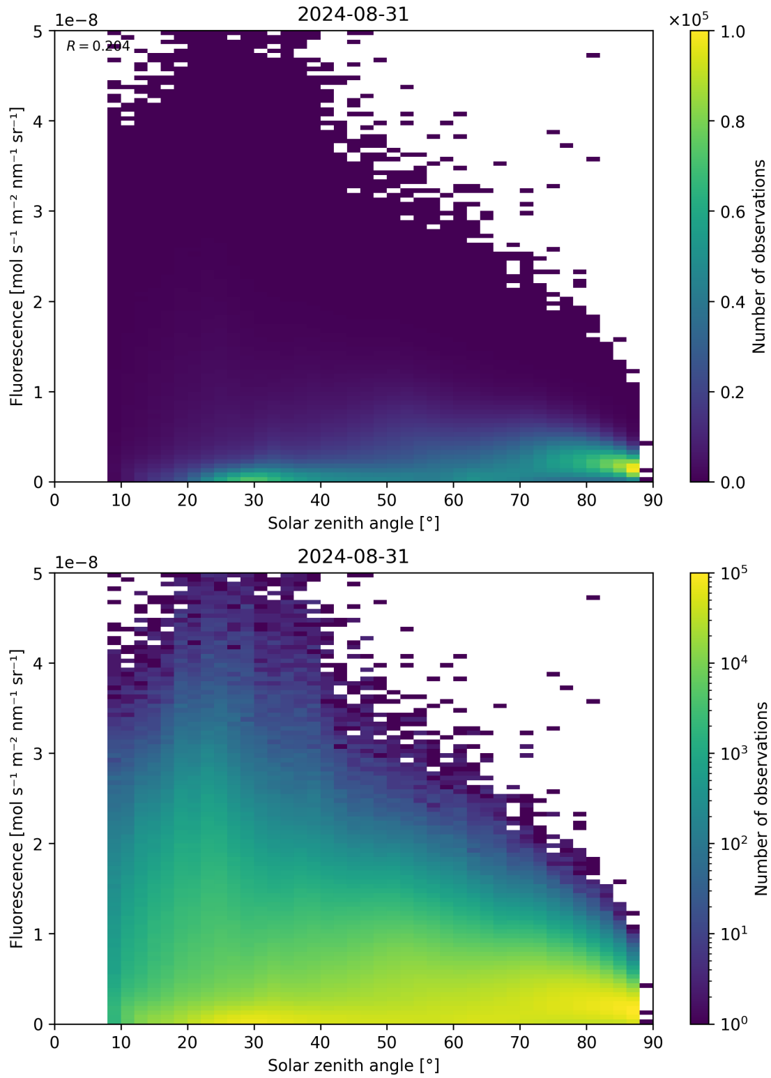
Figure 112: Scatter density plot of “Solar zenith angle” against “Fluorescence” for 2024-08-30 to 2024-09-01.
