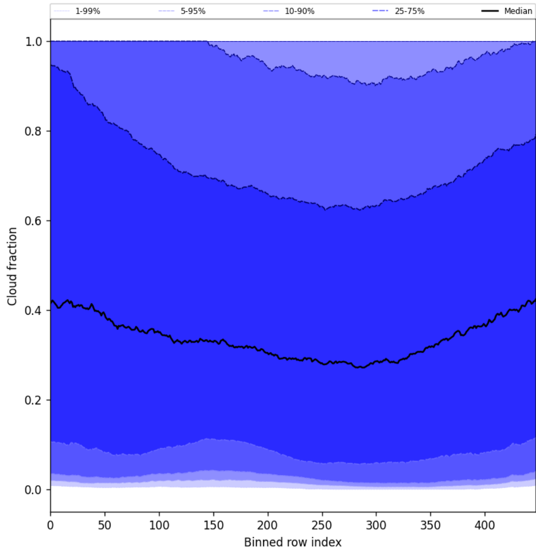
Figure 49: Along track statistics of “Cloud fraction” for 2024-08-30 to 2024-09-01
