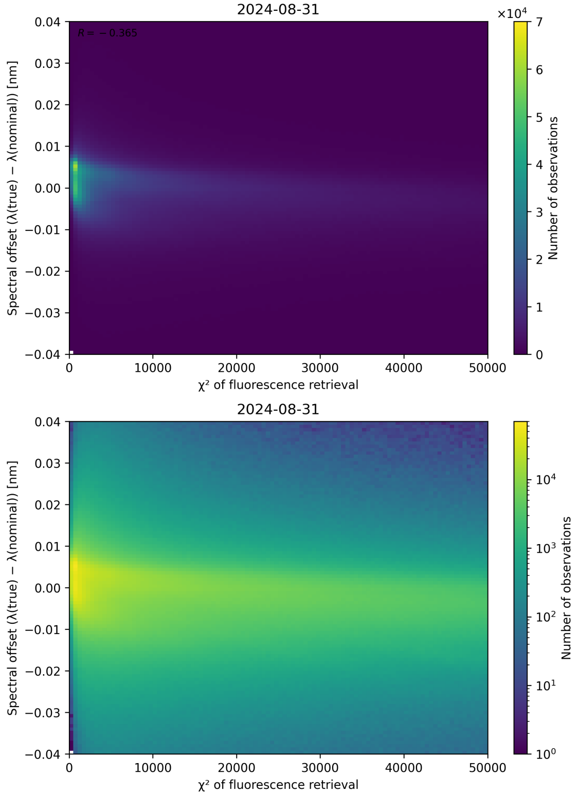
Figure 69: Scatter density plot of “ \chi^2 of fluorescence retrieval” against “Spectral offset ( \lambda_{\text{true}} - \lambda_{\text{nominal}} )” for 2024-08-30 to 2024-09-01.
