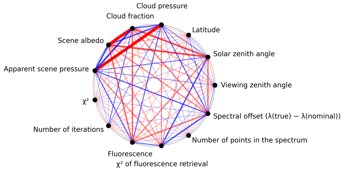
Figure 1: Map of correlation graph for 2024-08-30 to 2024-09-01.
