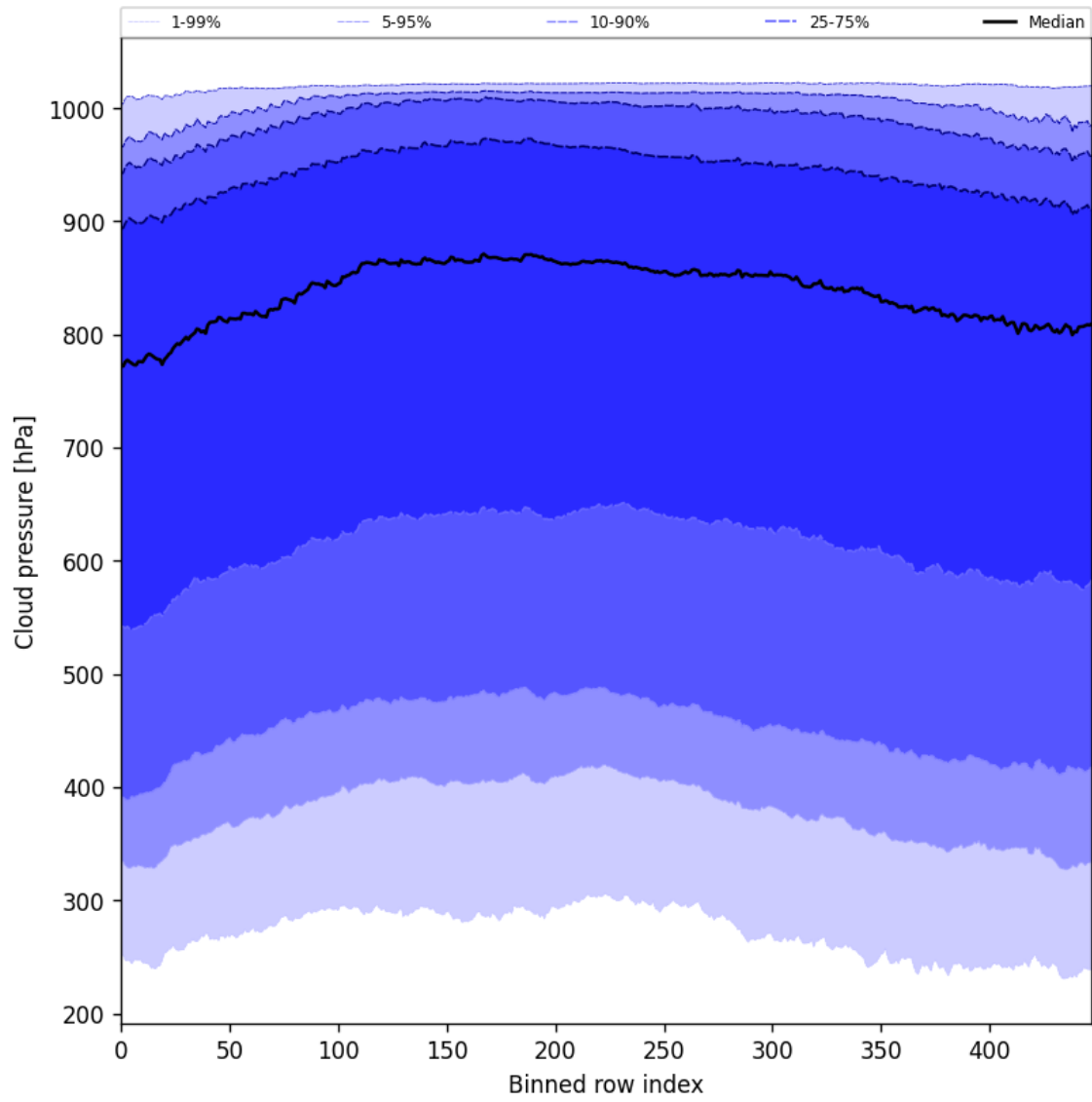
Figure 47: Along track statistics of “Cloud pressure” for 2024-08-30 to 2024-09-01
