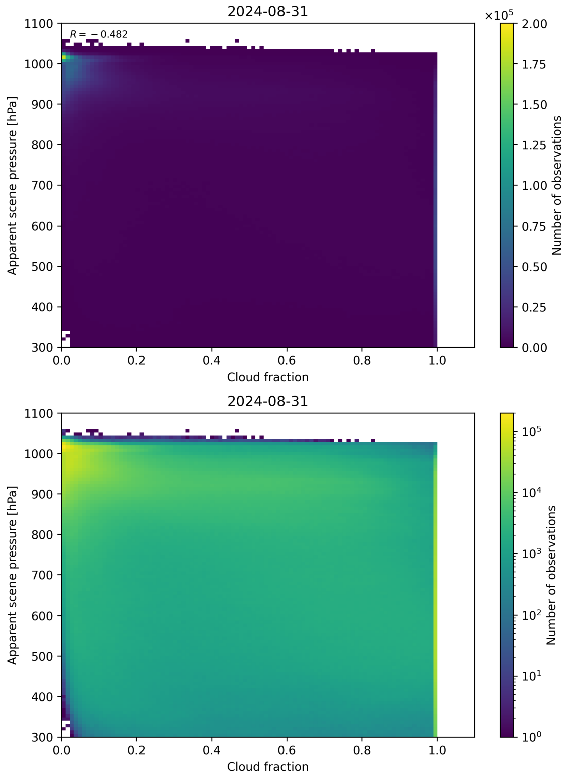
Figure 70: Scatter density plot of “Cloud fraction” against “Apparent scene pressure” for 2024-08-30 to 2024-09-01.
