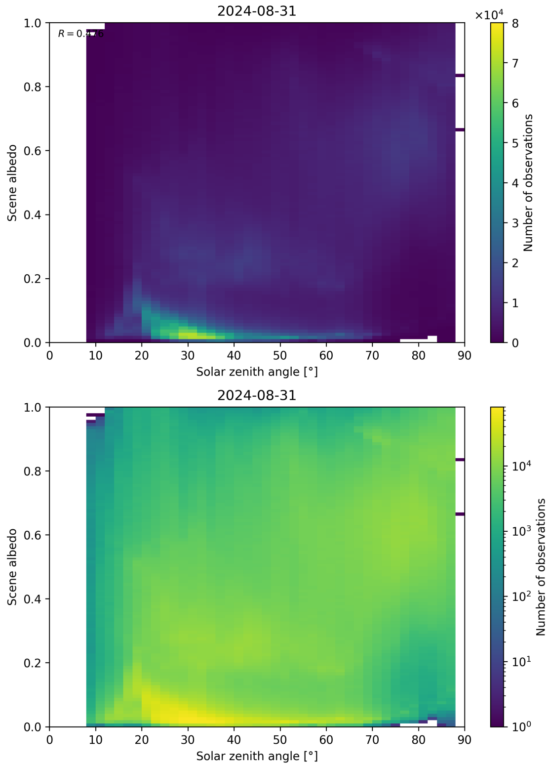
Figure 116: Scatter density plot of “Solar zenith angle” against “Scene albedo” for 2024-08-30 to 2024-09-01.
