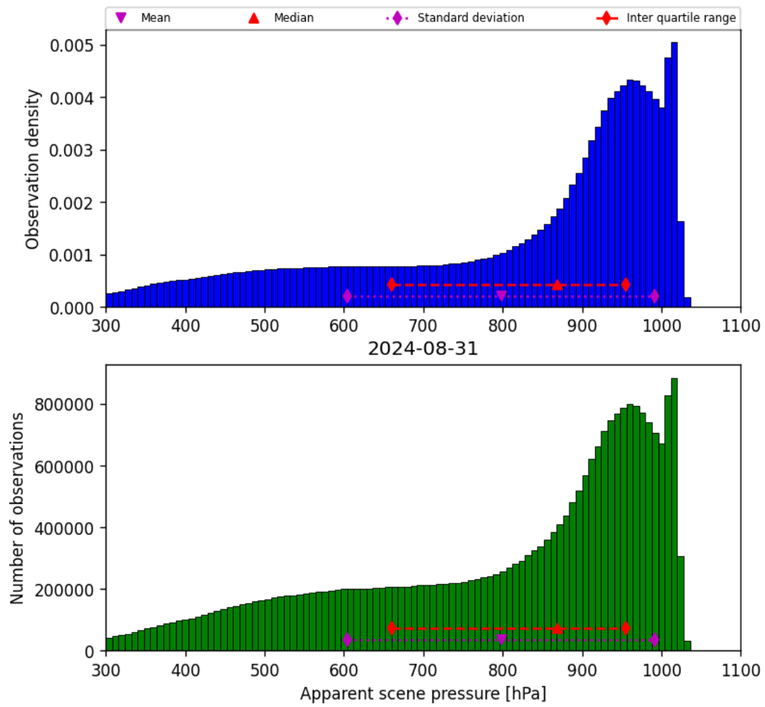
Figure 36: Histogram of “Apparent scene pressure” for 2024-08-30 to 2024-09-01
