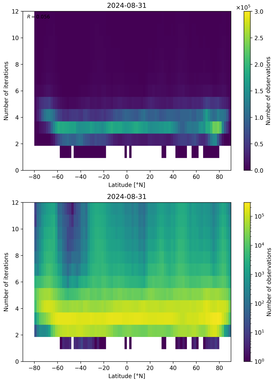
Figure 93: Scatter density plot of “Latitude” against “Number of iterations” for 2024-08-30 to 2024-09-01.
