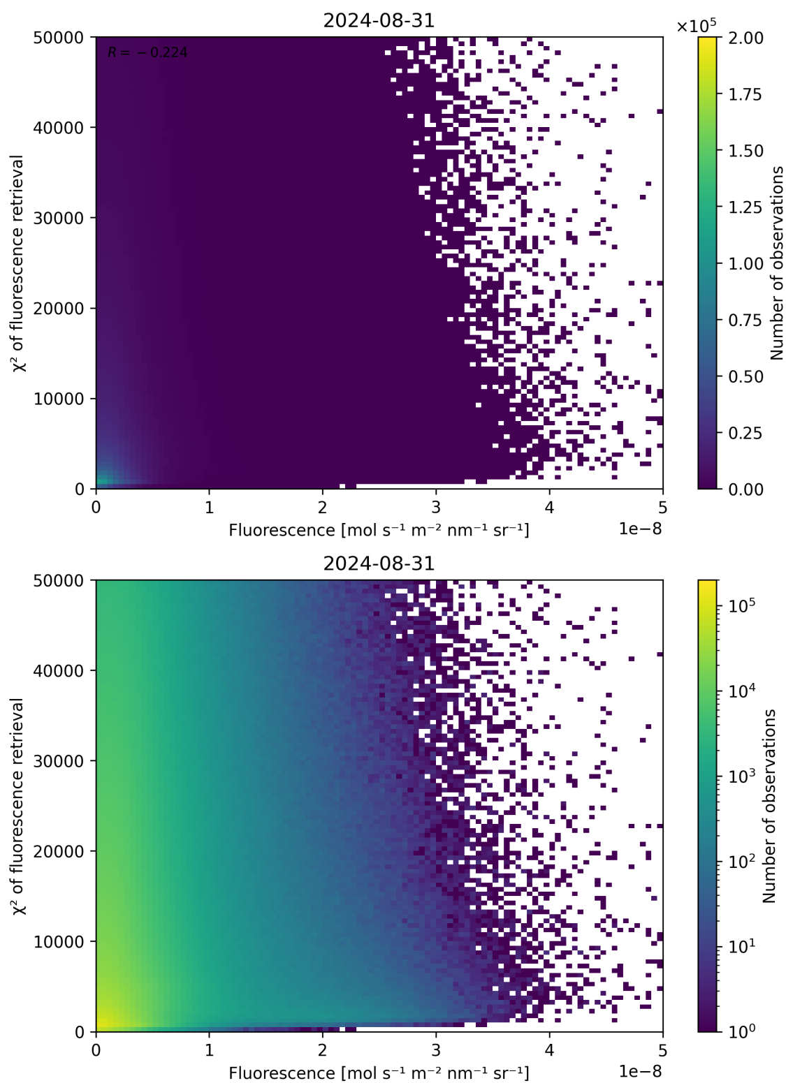
Figure 85: Scatter density plot of “Fluorescence” against “ \chi^2 of fluorescence retrieval” for 2024-08-30 to 2024-09-01.
