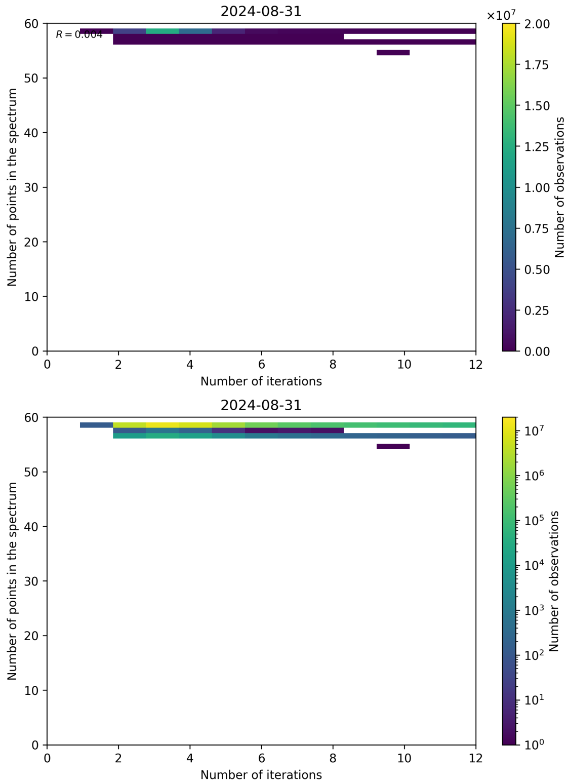
Figure 99: Scatter density plot of “Number of iterations” against “Number of points in the spectrum” for 2024-08-30 to 2024-09-01.
