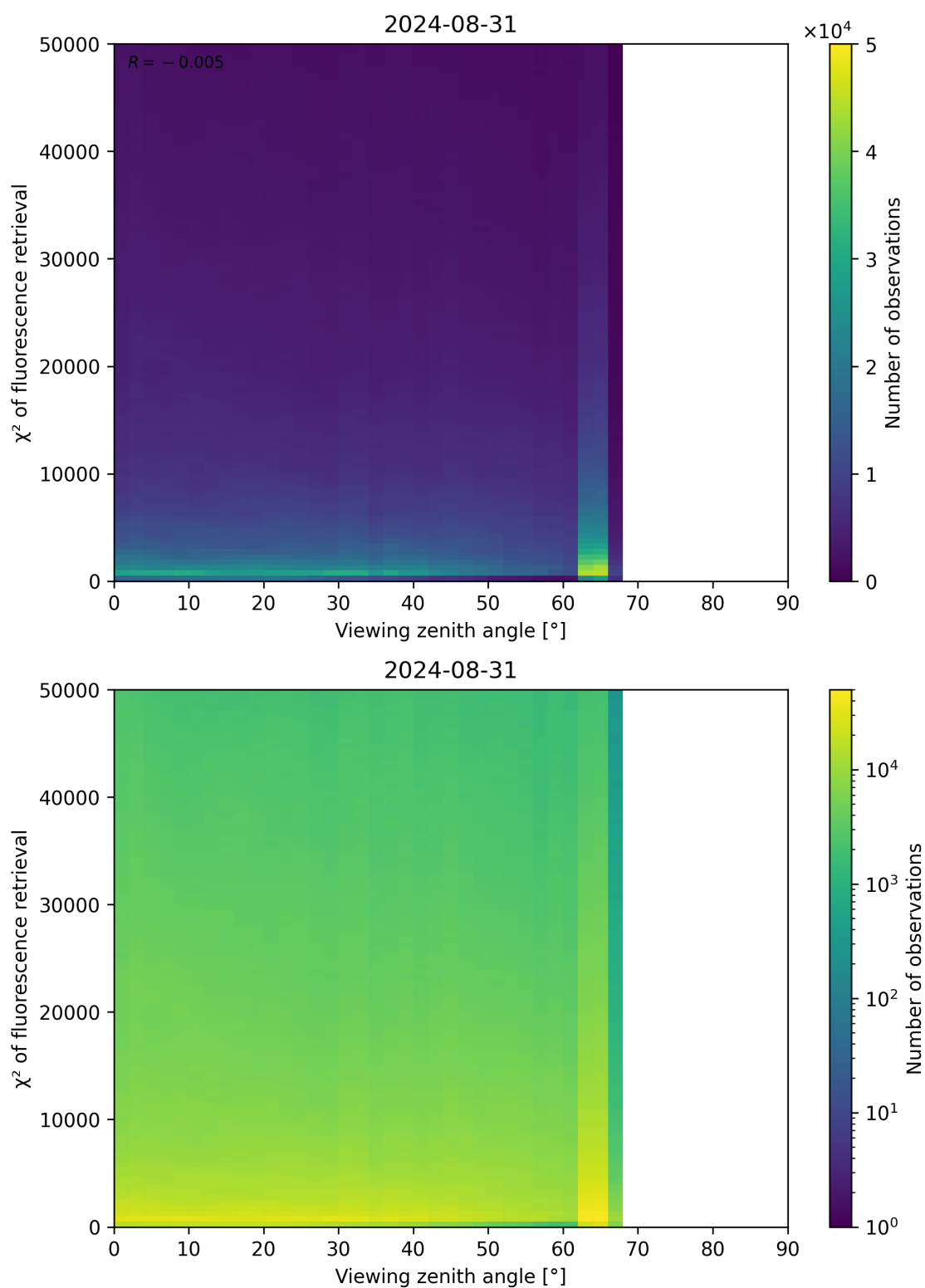
Figure 119: Scatter density plot of “Viewing zenith angle” against “ \chi^2 of fluorescence retrieval” for 2024-08-30 to 2024-09-01.
