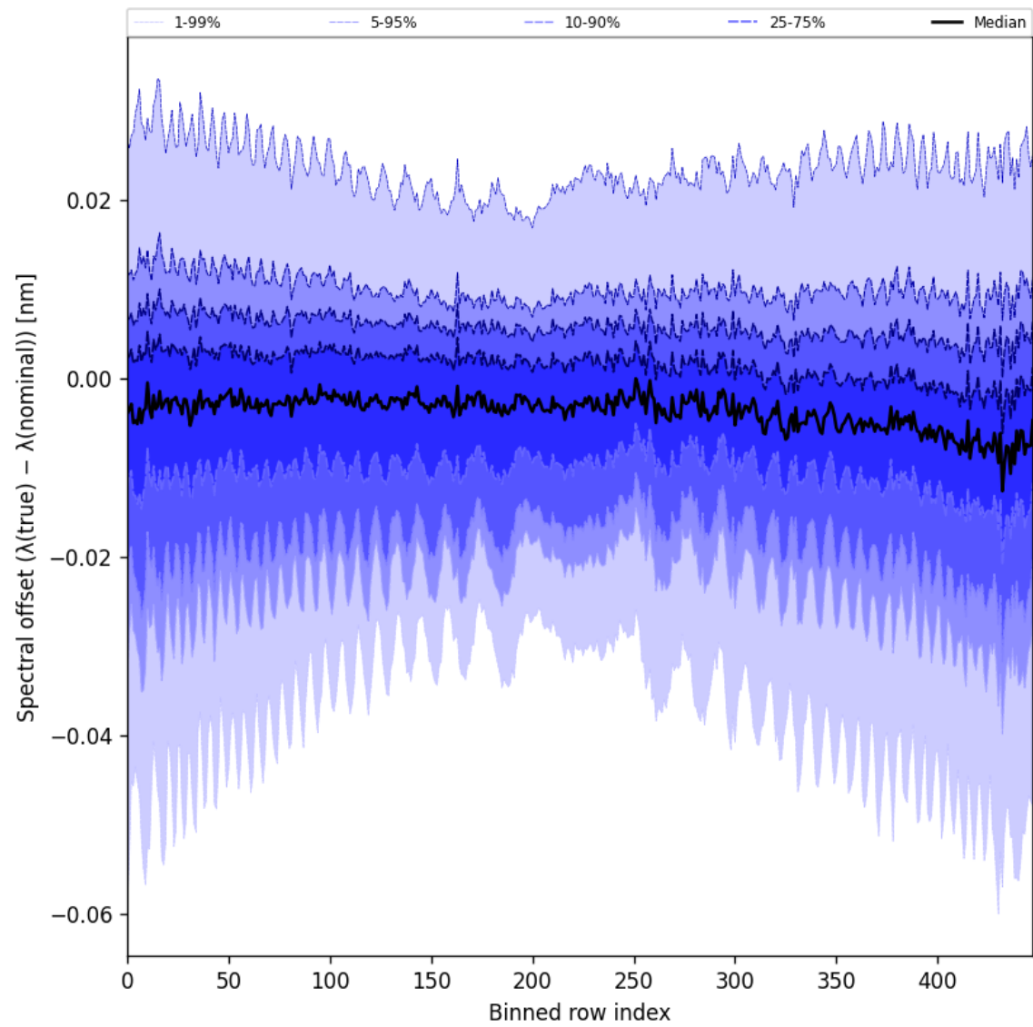
Figure 62: Along track statistics of “Spectral offset ( \lambda_{\text{true}} - \lambda_{\text{nominal}} )” for 2024-08-30 to 2024-09-01
