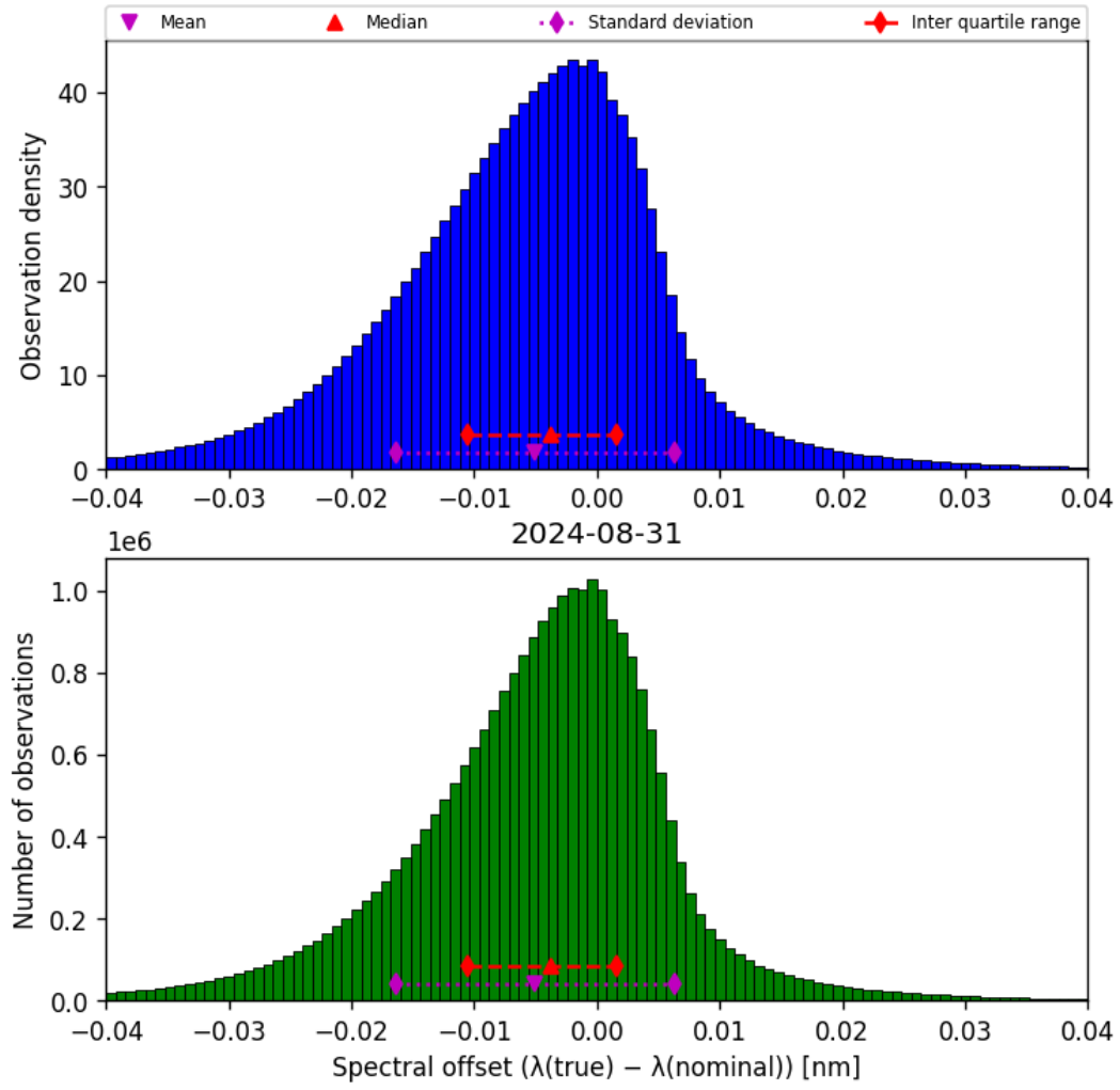
Figure 45: Histogram of “Spectral offset ( \lambda_{\text{true}} - \lambda_{\text{nominal}} )” for 2024-08-30 to 2024-09-01
