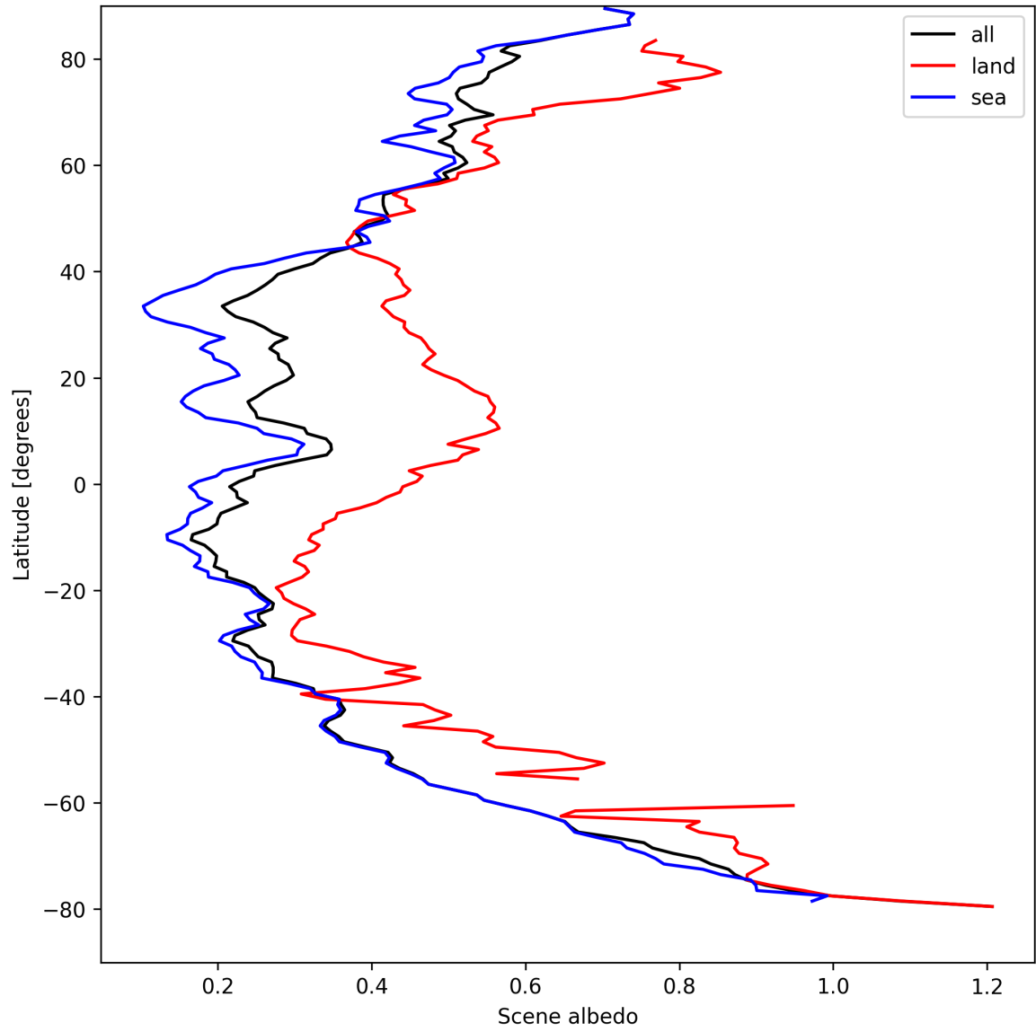
Figure 17: Zonal average of “Scene albedo” for 2024-08-30 to 2024-09-01.
