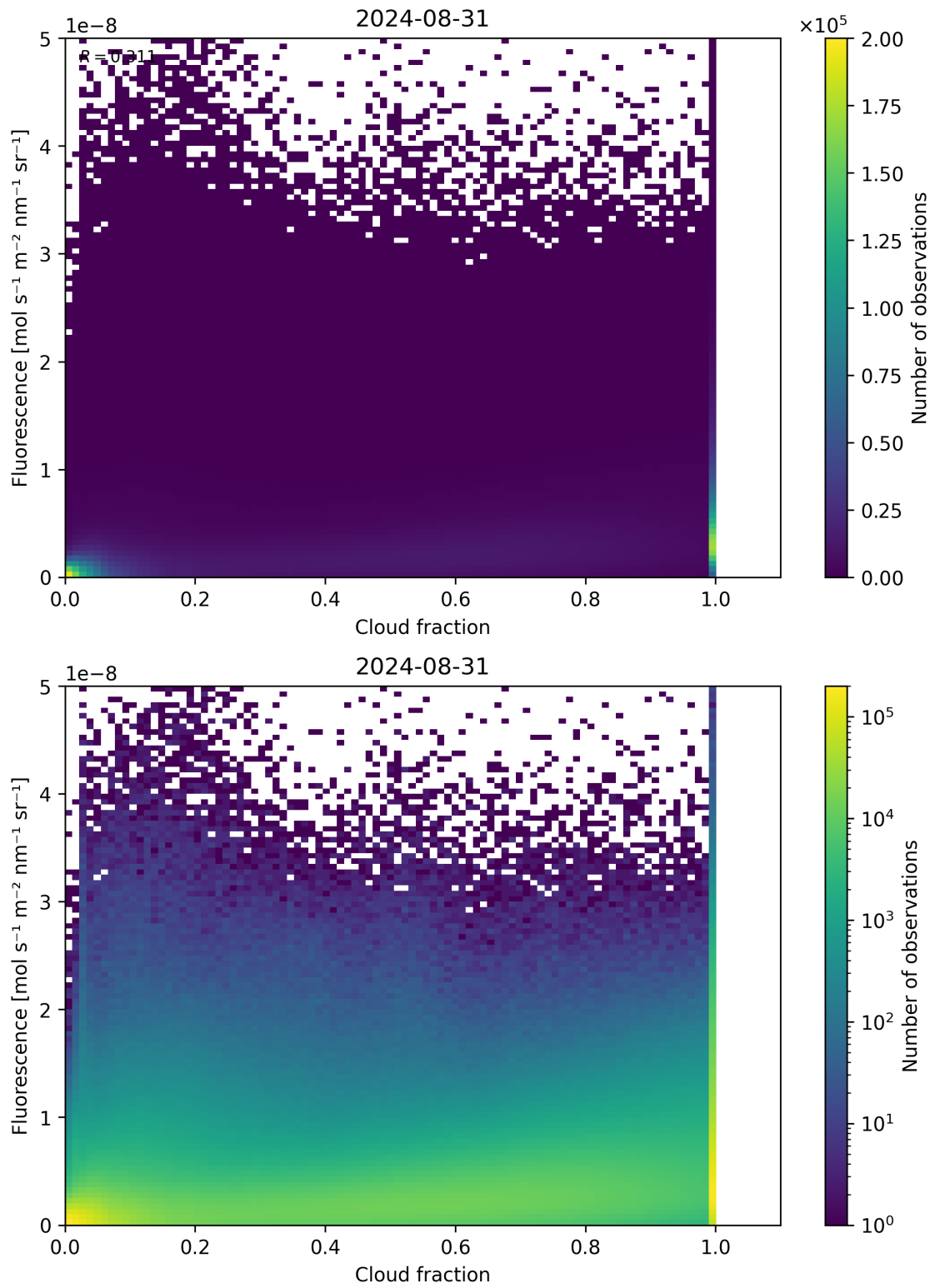
Figure 72: Scatter density plot of “Cloud fraction” against “Fluorescence” for 2024-08-30 to 2024-09-01.
