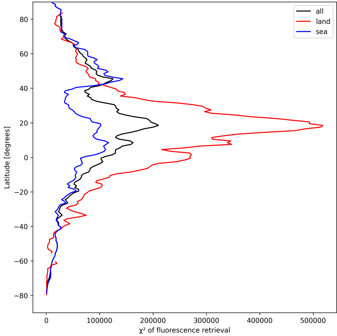
Figure 25: Zonal average of “ \chi^2 of fluorescence retrieval” for 2024-08-30 to 2024-09-01.
