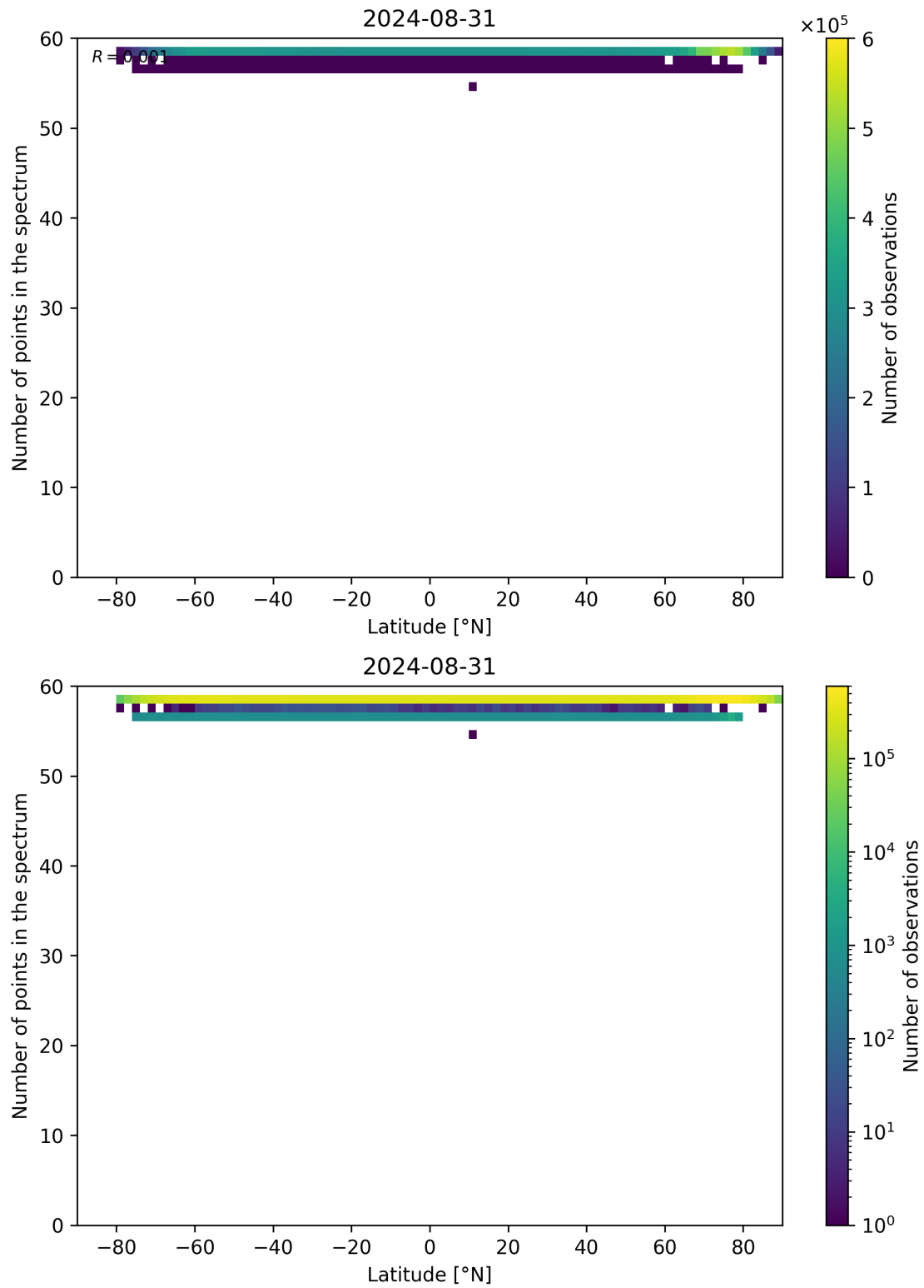
Figure 94: Scatter density plot of “Latitude” against “Number of points in the spectrum” for 2024-08-30 to 2024-09-01.
