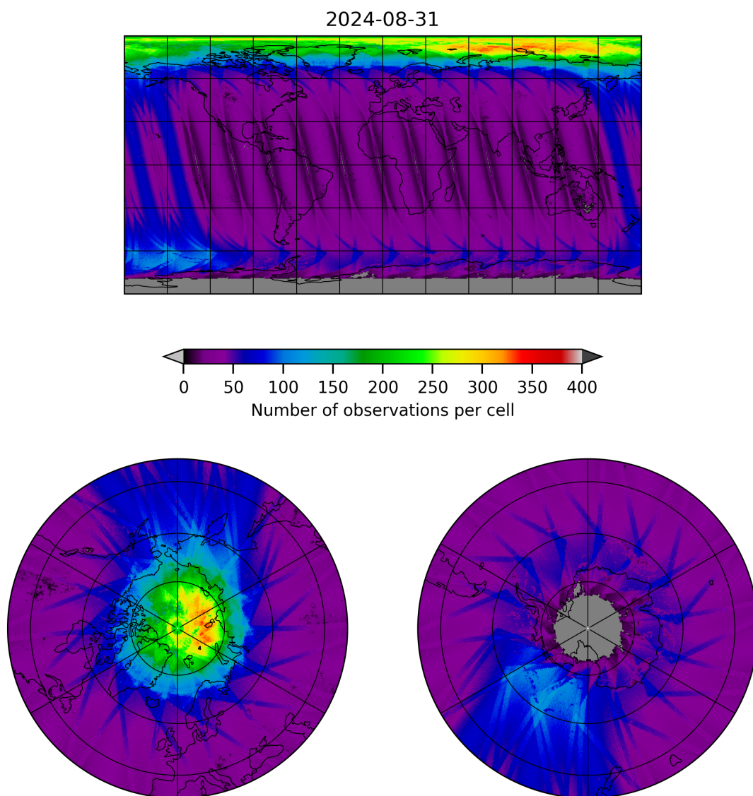
Figure 11: Map of the number of observations for 2024-08-30 to 2024-09-01
