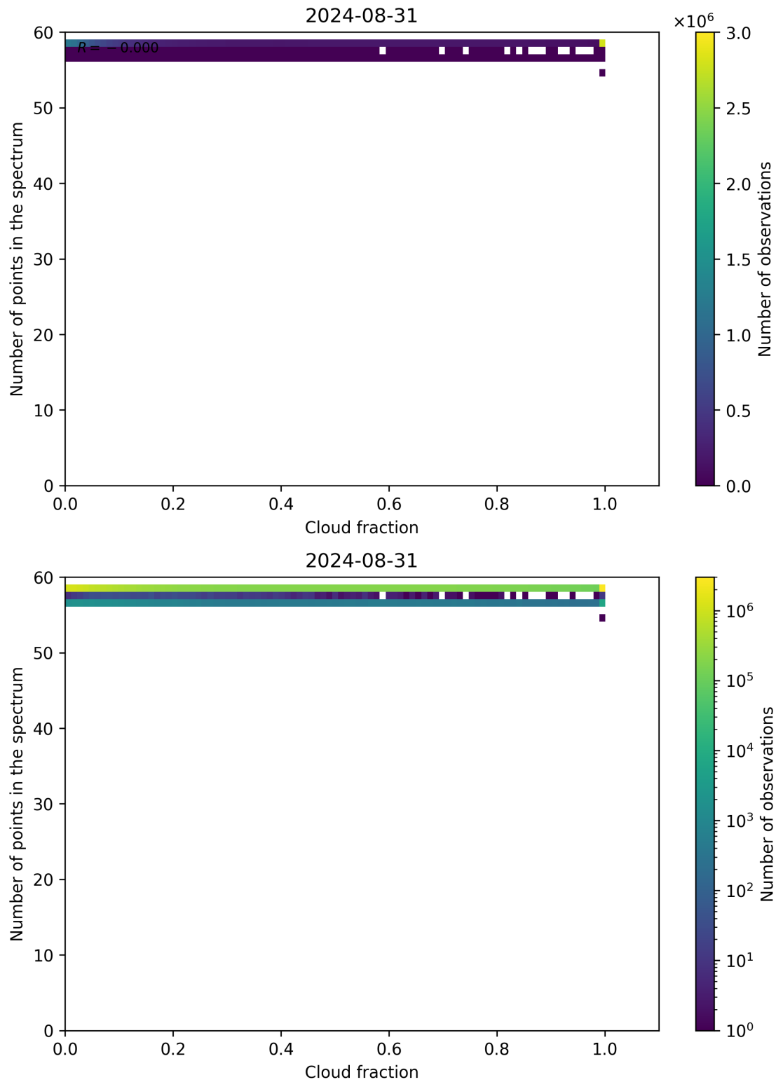
Figure 74: Scatter density plot of “Cloud fraction” against “Number of points in the spectrum” for 2024-08-30 to 2024-09-01.
