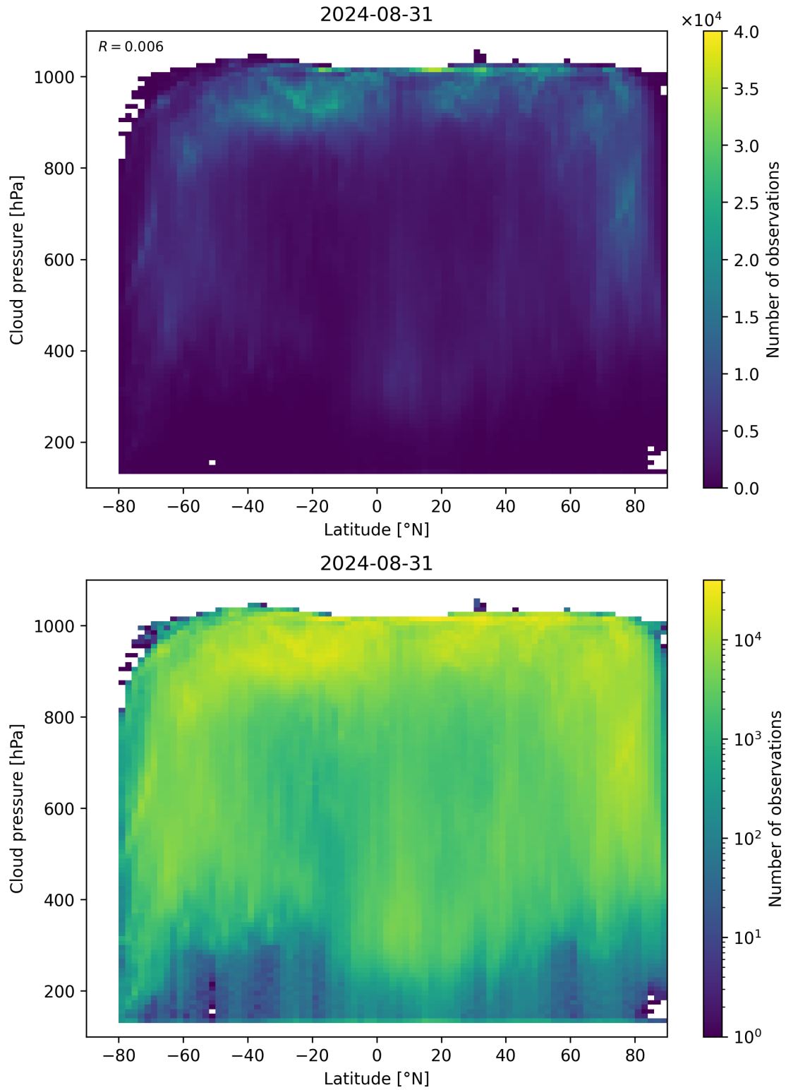
Figure 91: Scatter density plot of “Latitude” against “Cloud pressure” for 2024-08-30 to 2024-09-01.
