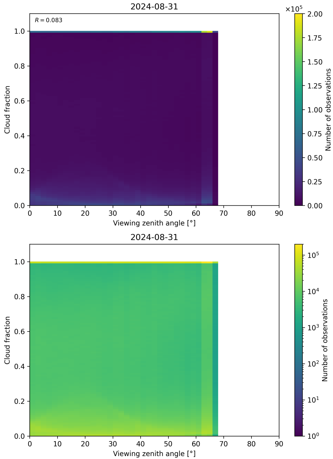
Figure 120: Scatter density plot of “Viewing zenith angle” against “Cloud fraction” for 2024-08-30 to 2024-09-01.
