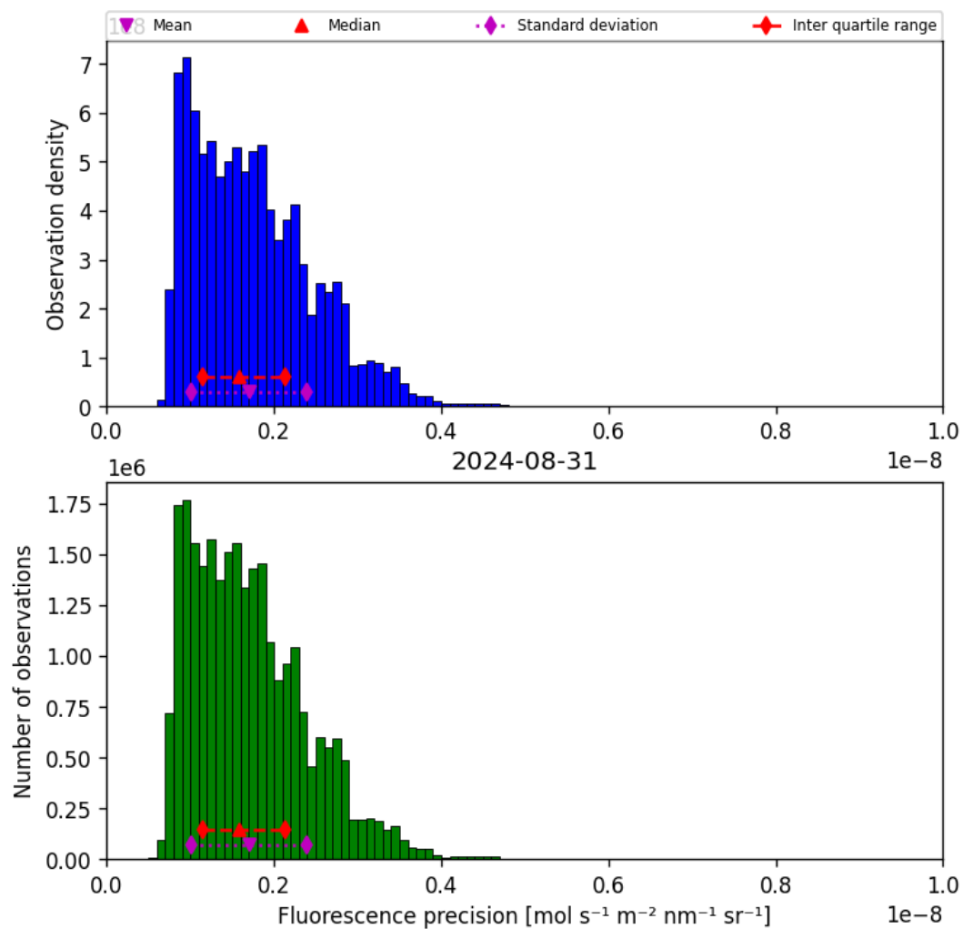
Figure 41: Histogram of “Fluorescence precision” for 2024-08-30 to 2024-09-01
