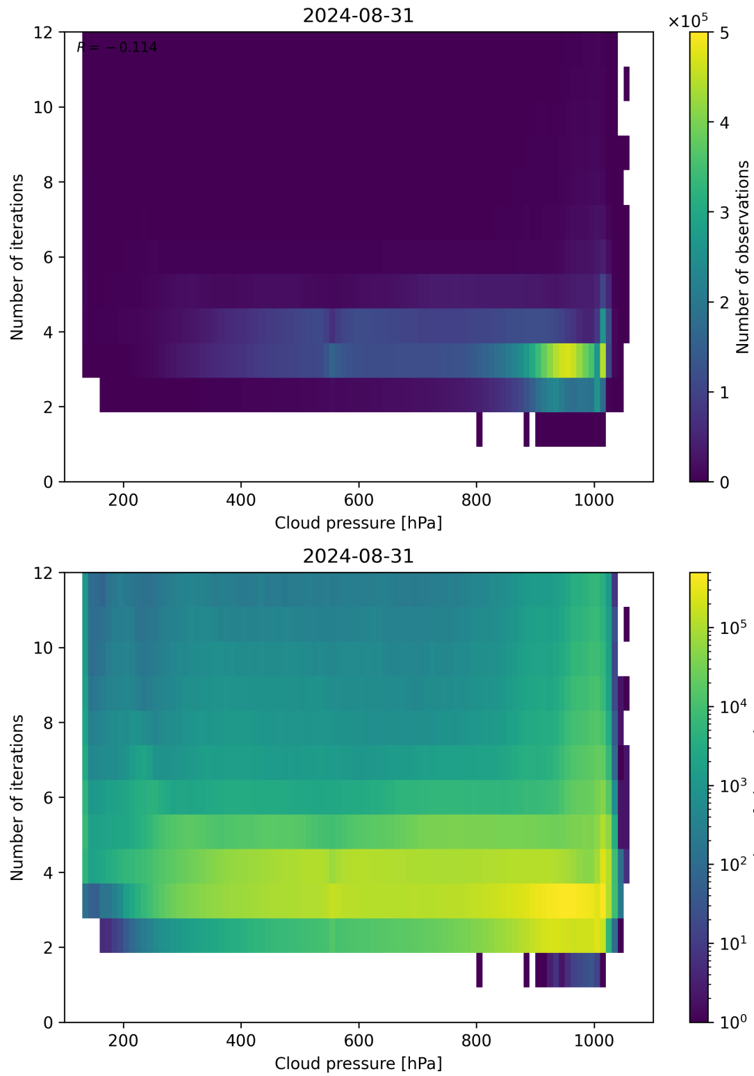
Figure 81: Scatter density plot of “Cloud pressure” against “Number of iterations” for 2024-08-30 to 2024-09-01.
