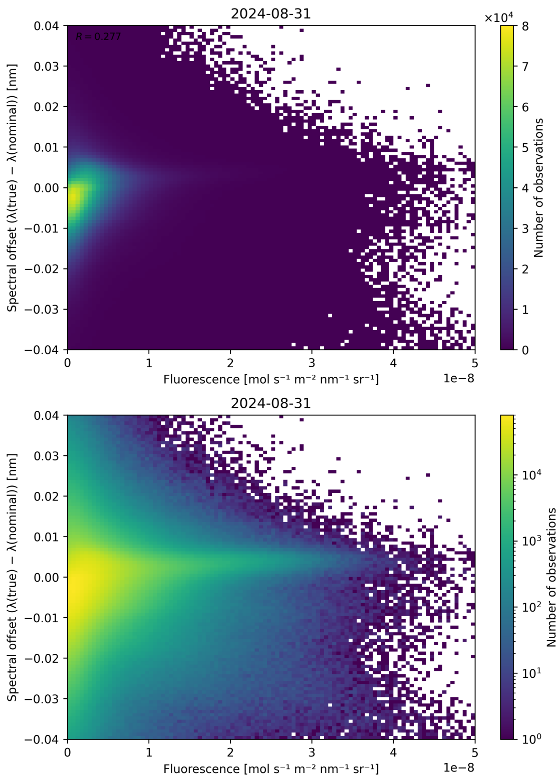
Figure 87: Scatter density plot of “Fluorescence” against “Spectral offset ( \lambda_{\text{true}} - \lambda_{\text{nominal}} )” for 2024-08-30 to 2024-09-01.
