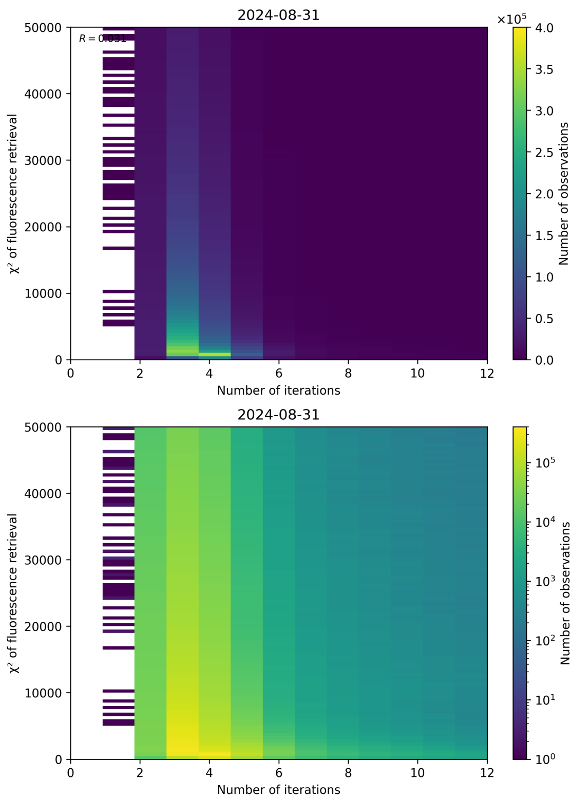
Figure 97: Scatter density plot of “Number of iterations” against “ \chi^2 of fluorescence retrieval” for 2024-08-30 to 2024-09-01.
