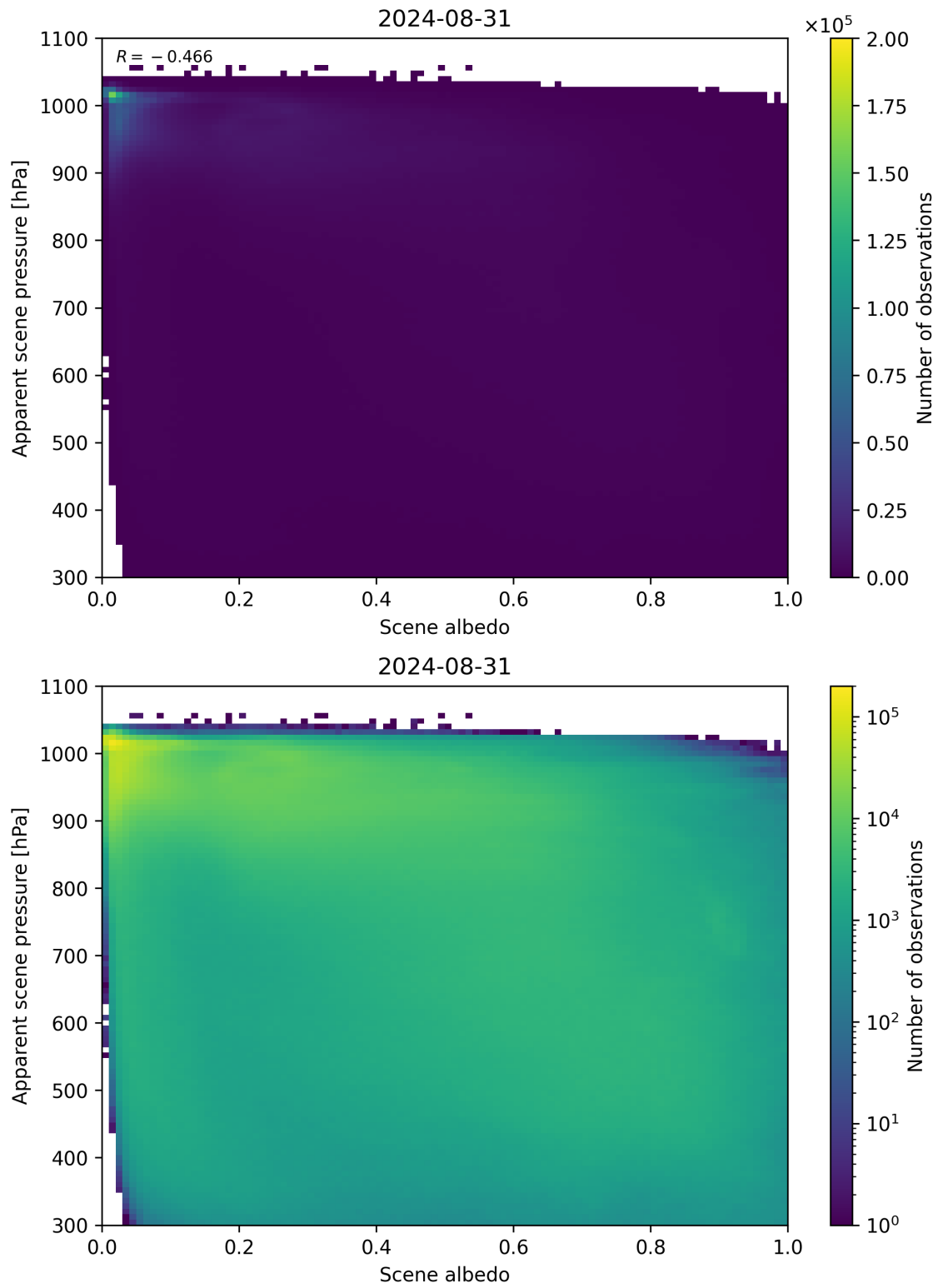
Figure 102: Scatter density plot of “Scene albedo” against “Apparent scene pressure” for 2024-08-30 to 2024-09-01.
