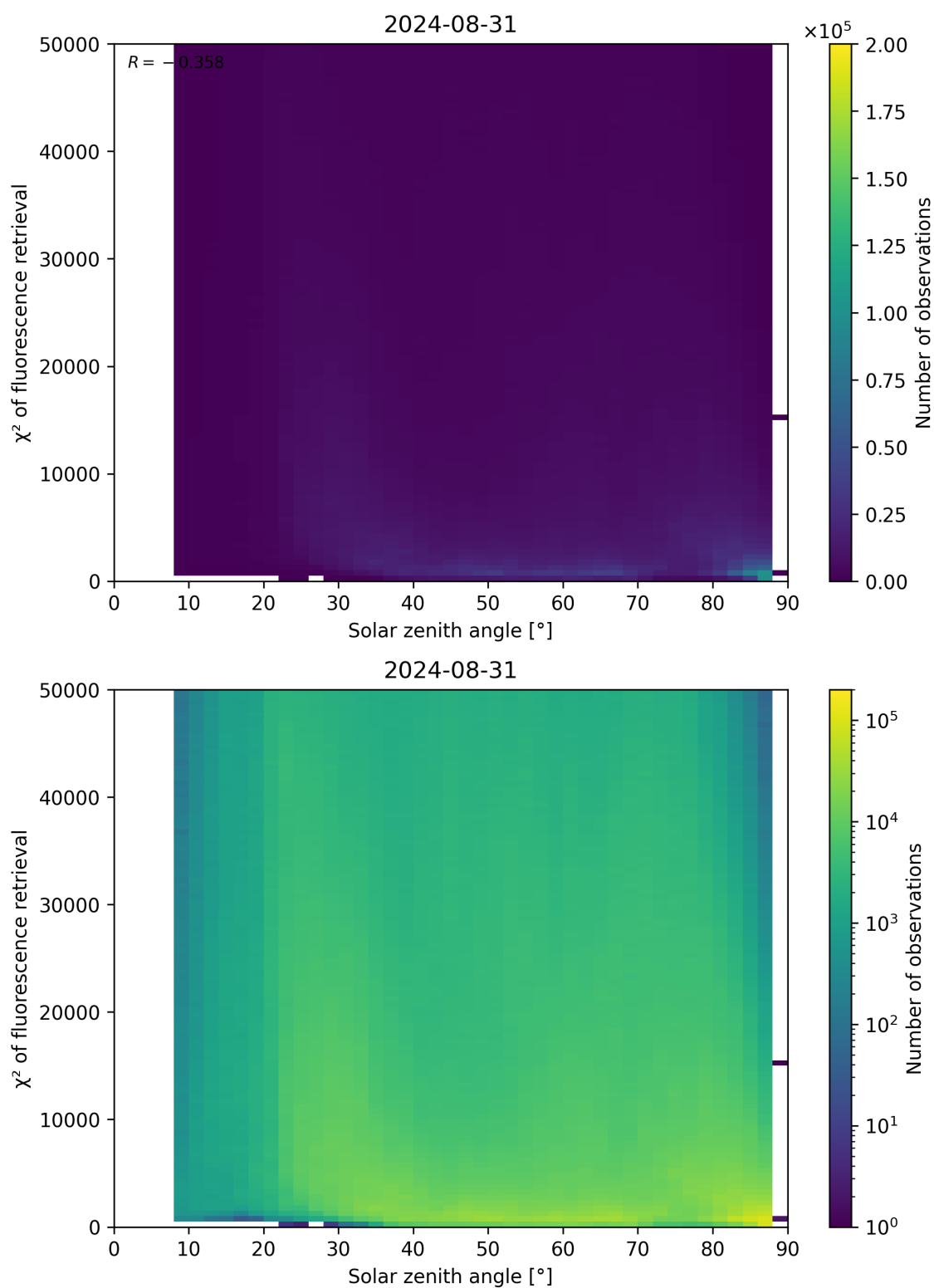
Figure 109: Scatter density plot of “Solar zenith angle” against “ \chi^2 of fluorescence retrieval” for 2024-08-30 to 2024-09-01.
