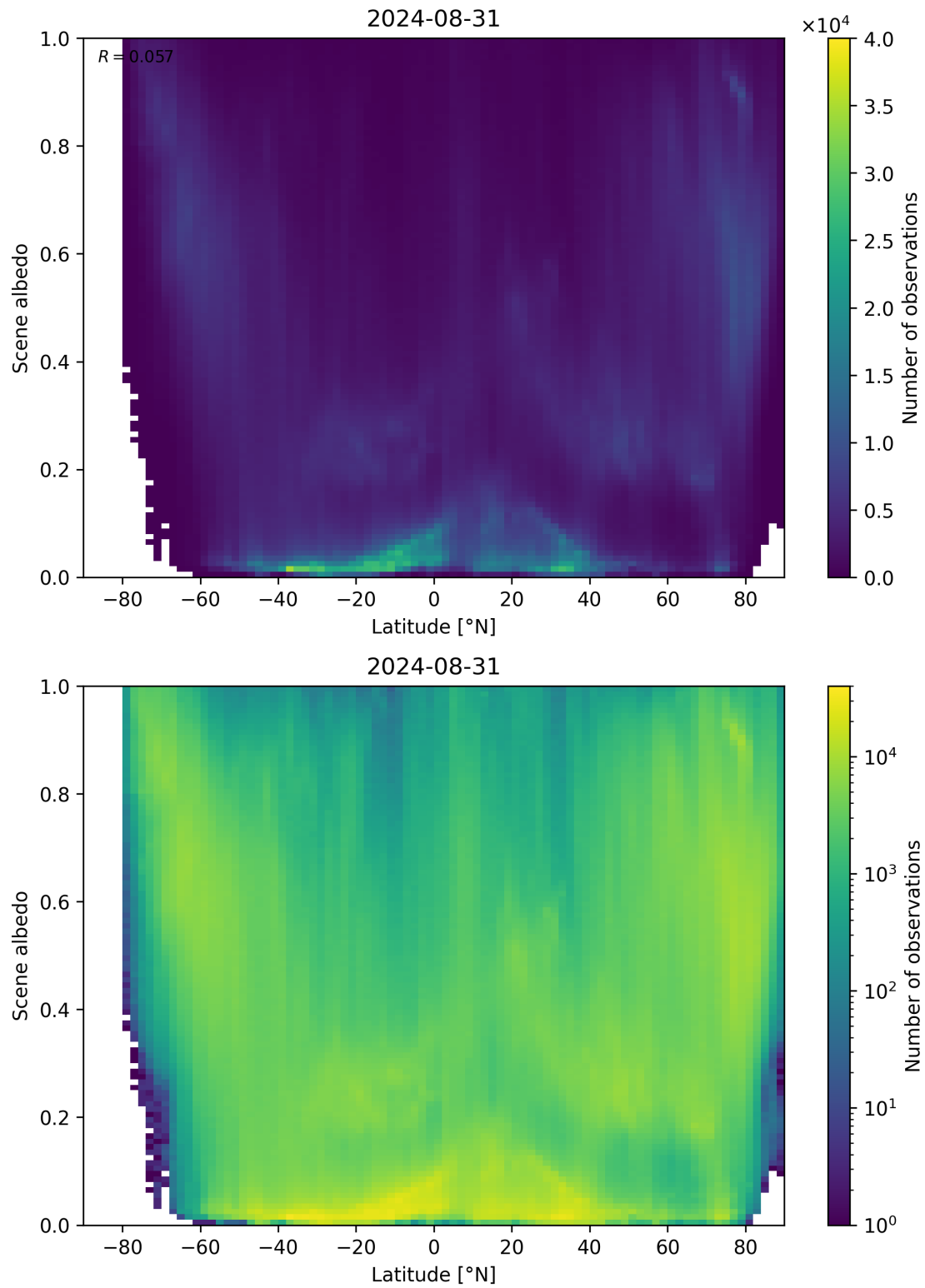
Figure 95: Scatter density plot of “Latitude” against “Scene albedo” for 2024-08-30 to 2024-09-01.
