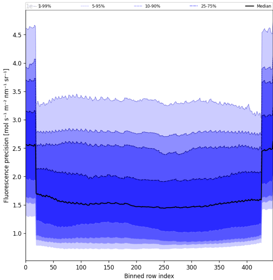
Figure 58: Along track statistics of “Fluorescence precision” for 2024-08-30 to 2024-09-01
