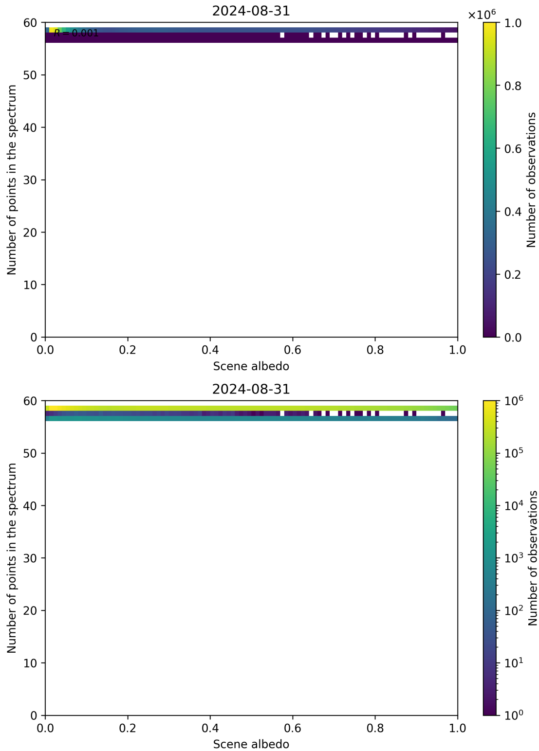
Figure 106: Scatter density plot of “Scene albedo” against “Number of points in the spectrum” for 2024-08-30 to 2024-09-01.
