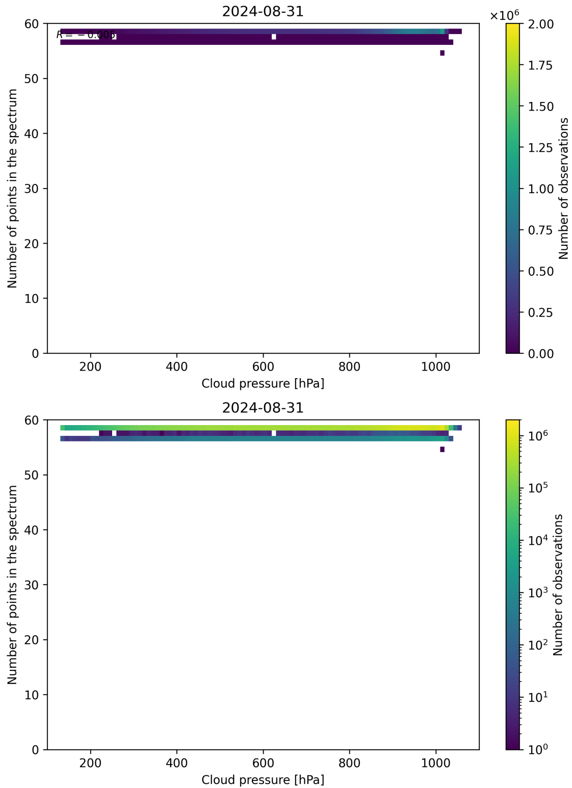
Figure 82: Scatter density plot of “Cloud pressure” against “Number of points in the spectrum” for 2024-08-30 to 2024-09-01.
