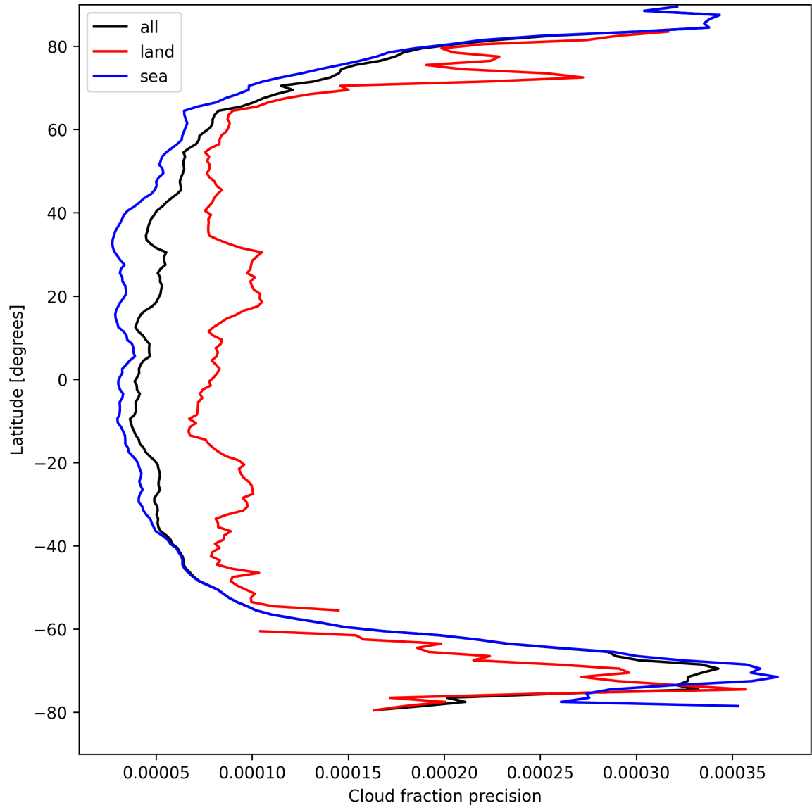
Figure 16: Zonal average of “Cloud fraction precision” for 2024-08-30 to 2024-09-01.
