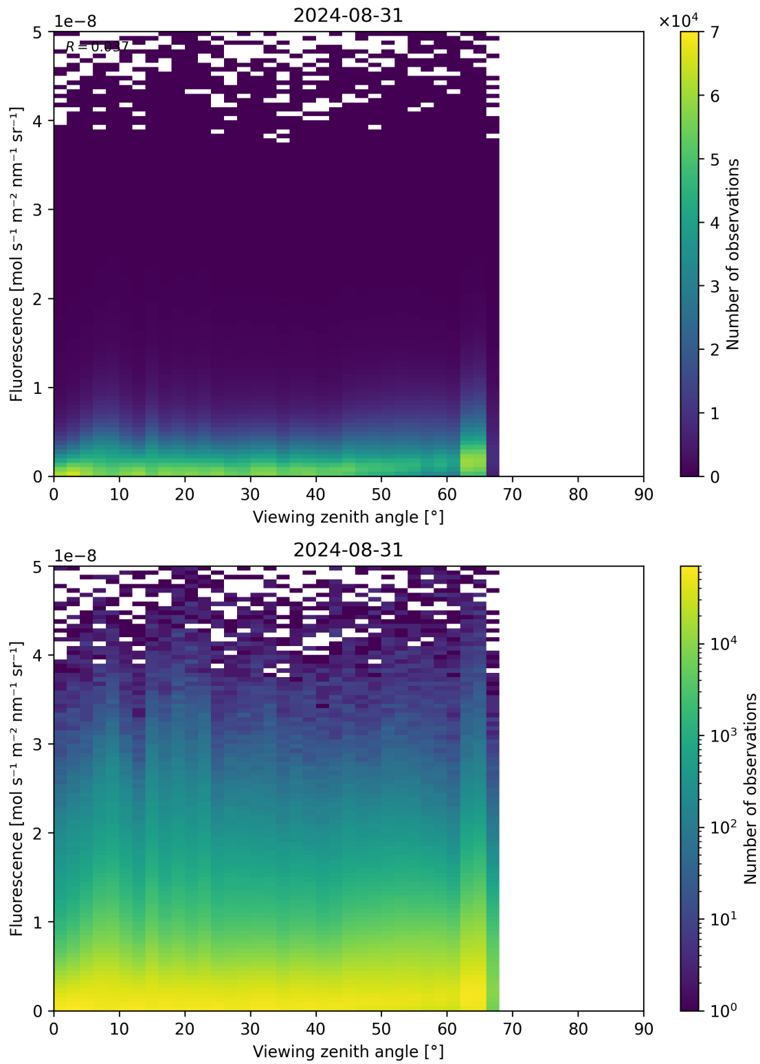
Figure 122: Scatter density plot of “Viewing zenith angle” against “Fluorescence” for 2024-08-30 to 2024-09-01.
