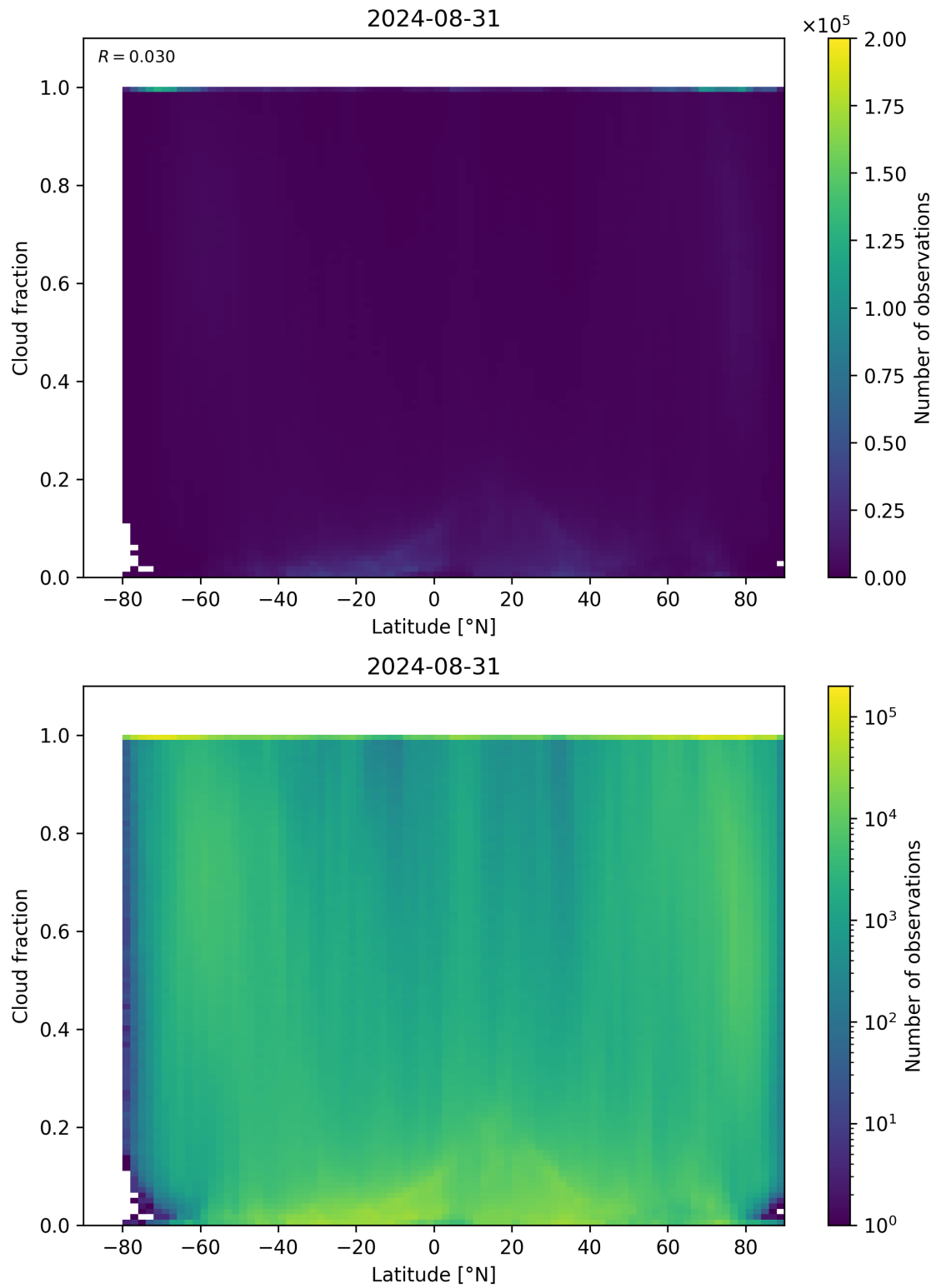
Figure 90: Scatter density plot of “Latitude” against “Cloud fraction” for 2024-08-30 to 2024-09-01.
