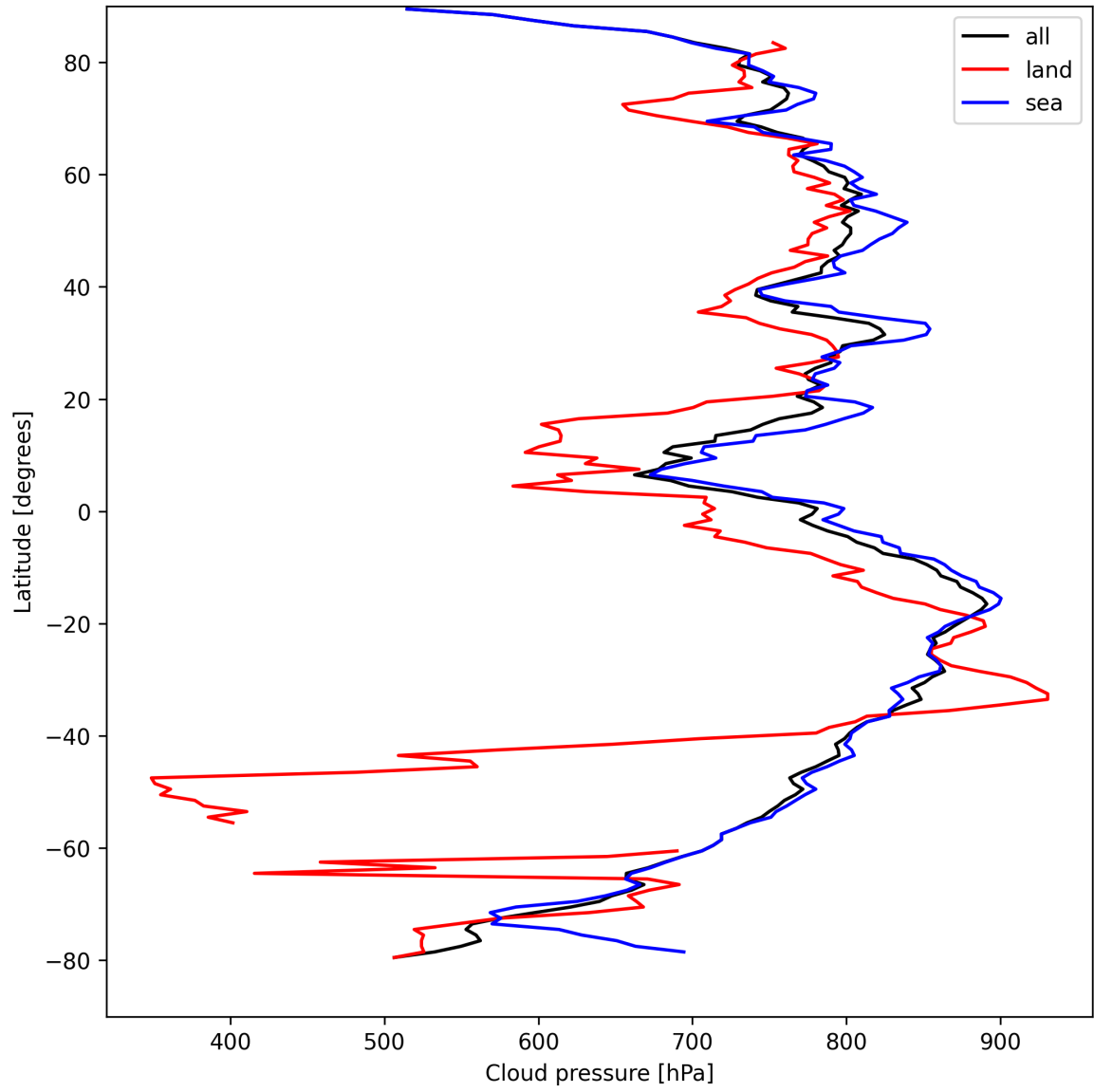
Figure 13: Zonal average of “Cloud pressure” for 2024-08-30 to 2024-09-01.
