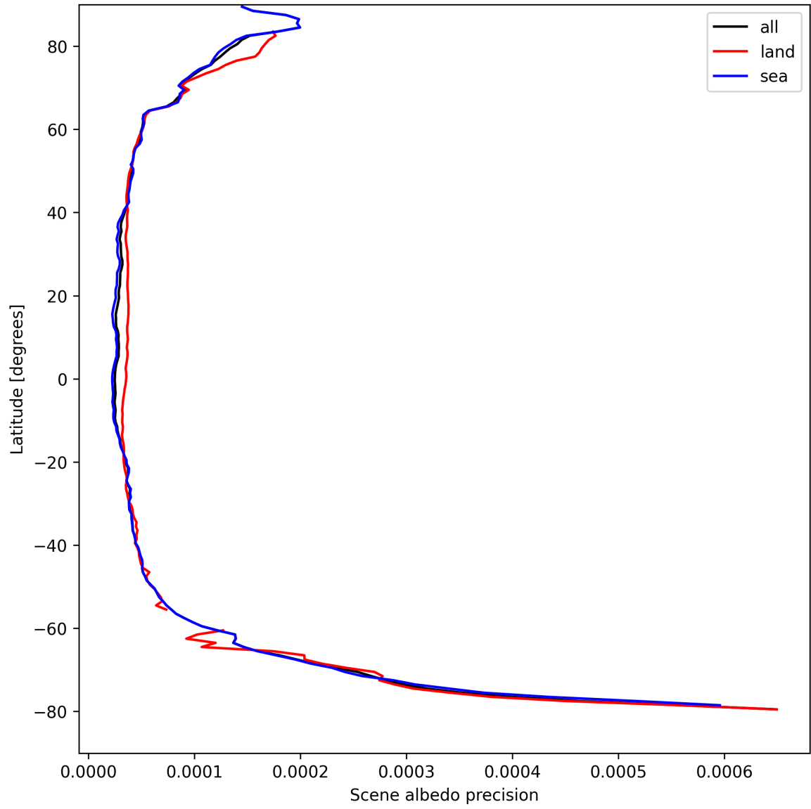
Figure 18: Zonal average of “Scene albedo precision” for 2024-08-30 to 2024-09-01.
