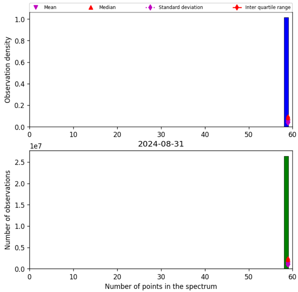
Figure 44: Histogram of “Number of points in the spectrum” for 2024-08-30 to 2024-09-01
