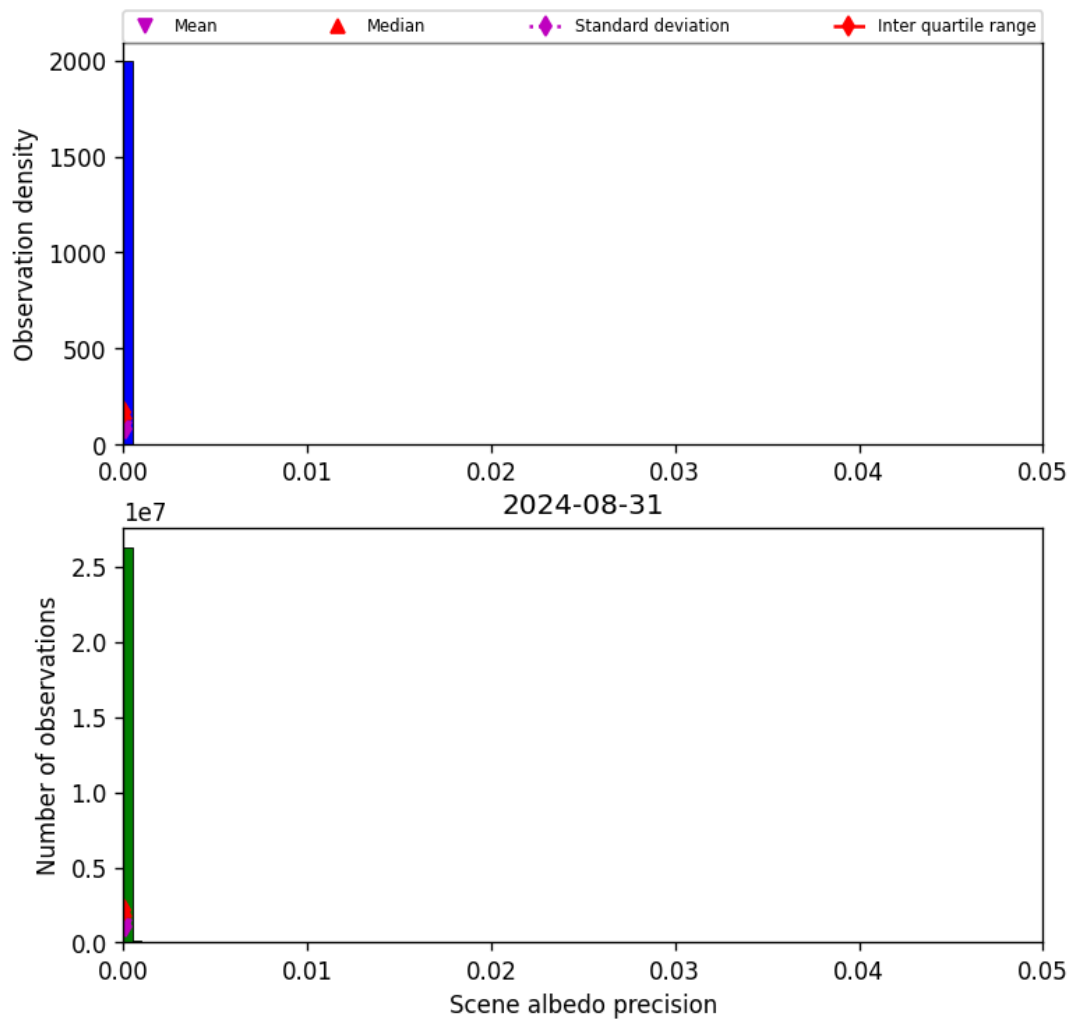
Figure 35: Histogram of “Scene albedo precision” for 2024-08-30 to 2024-09-01
