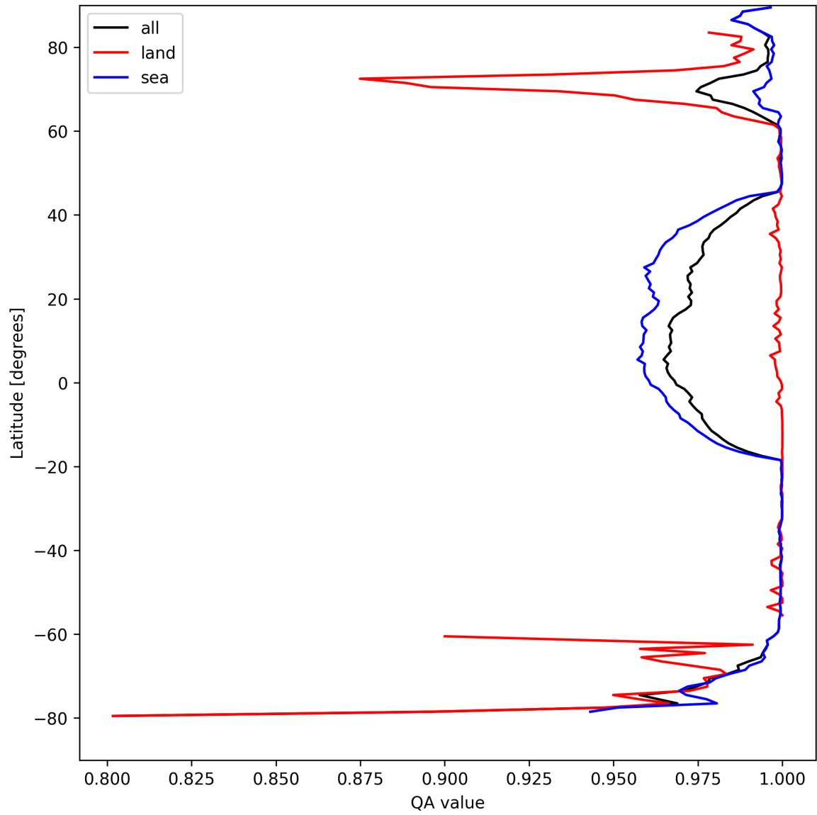
Figure 12: Zonal average of “QA value” for 2024-08-30 to 2024-09-01.
