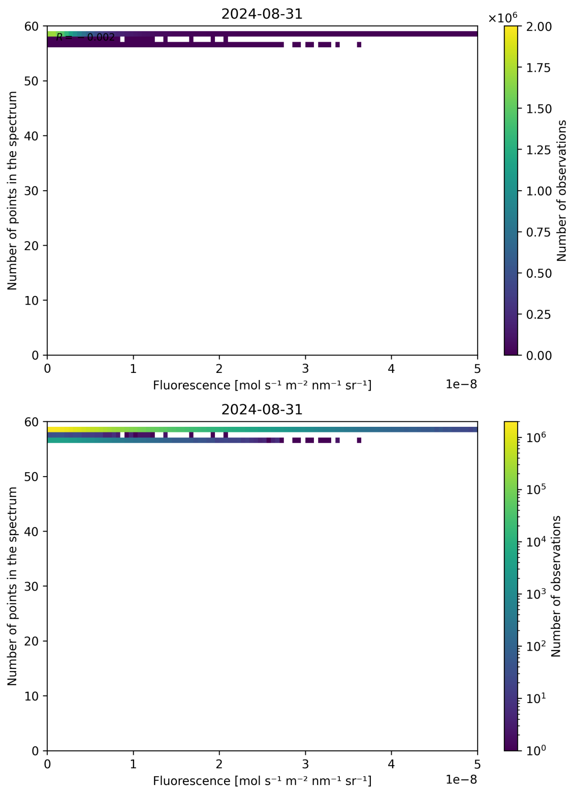
Figure 86: Scatter density plot of “Fluorescence” against “Number of points in the spectrum” for 2024-08-30 to 2024-09-01.
