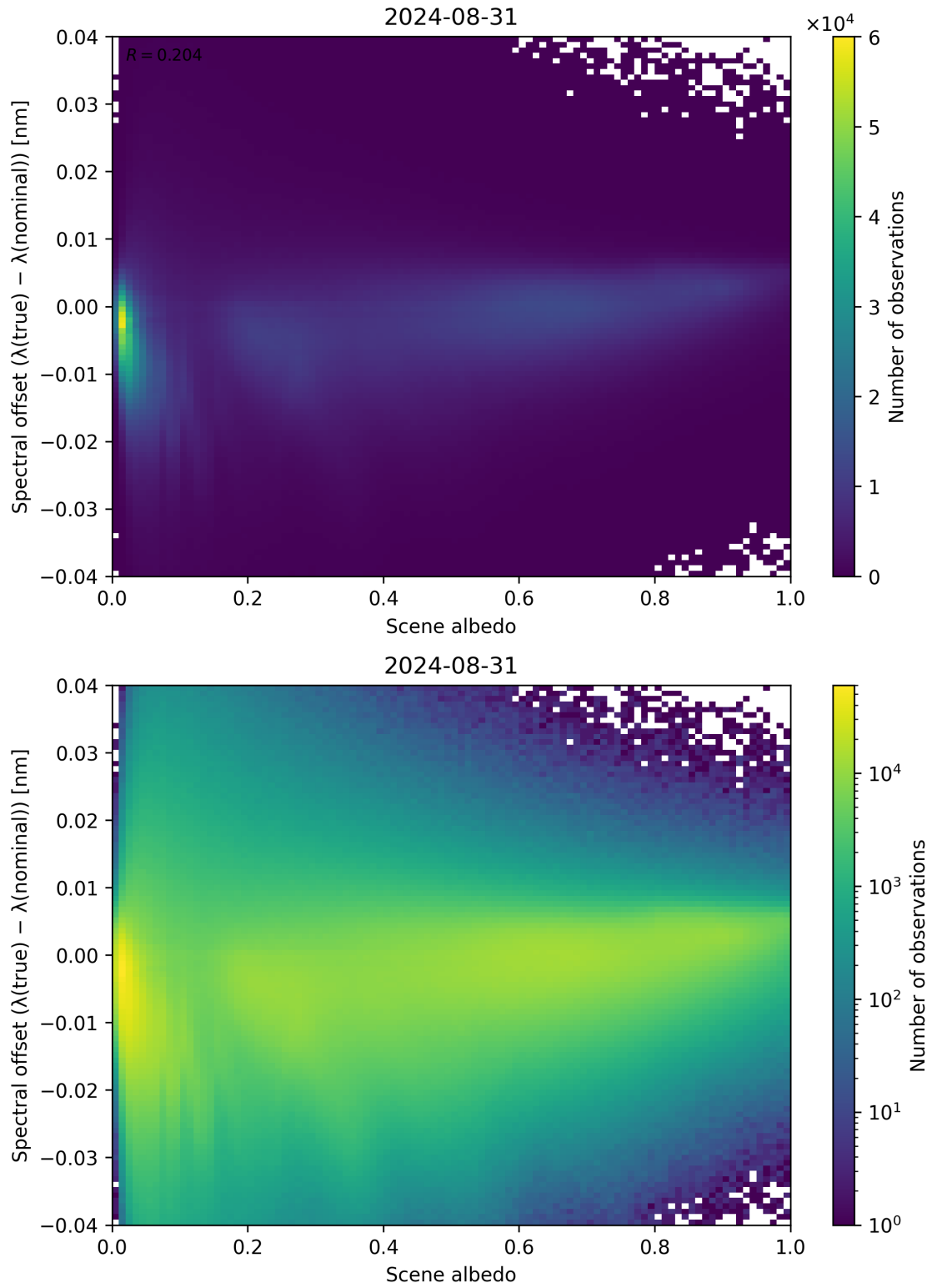
Figure 107: Scatter density plot of “Scene albedo” against “Spectral offset ( \lambda_{\text{true}} - \lambda_{\text{nominal}} )” for 2024-08-30 to 2024-09-01.
