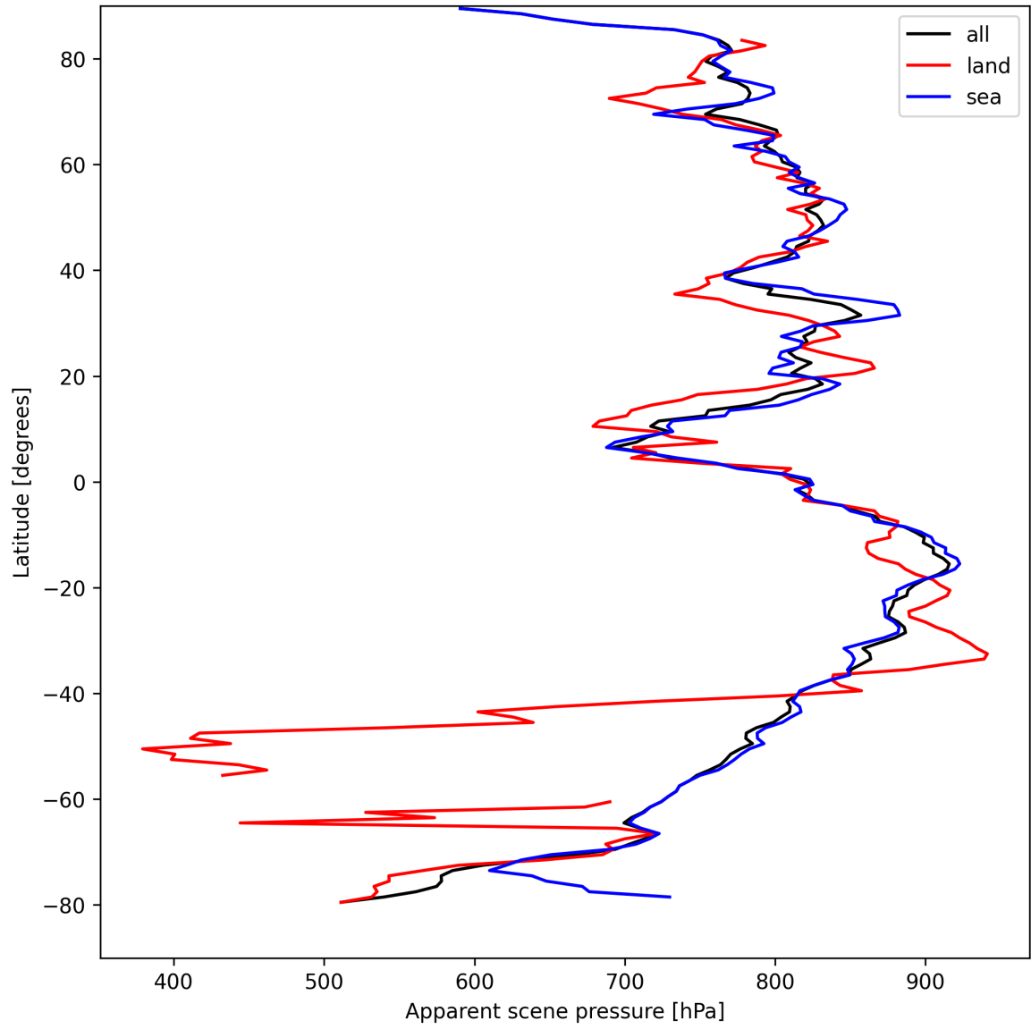
Figure 19: Zonal average of “Apparent scene pressure” for 2024-08-30 to 2024-09-01.
