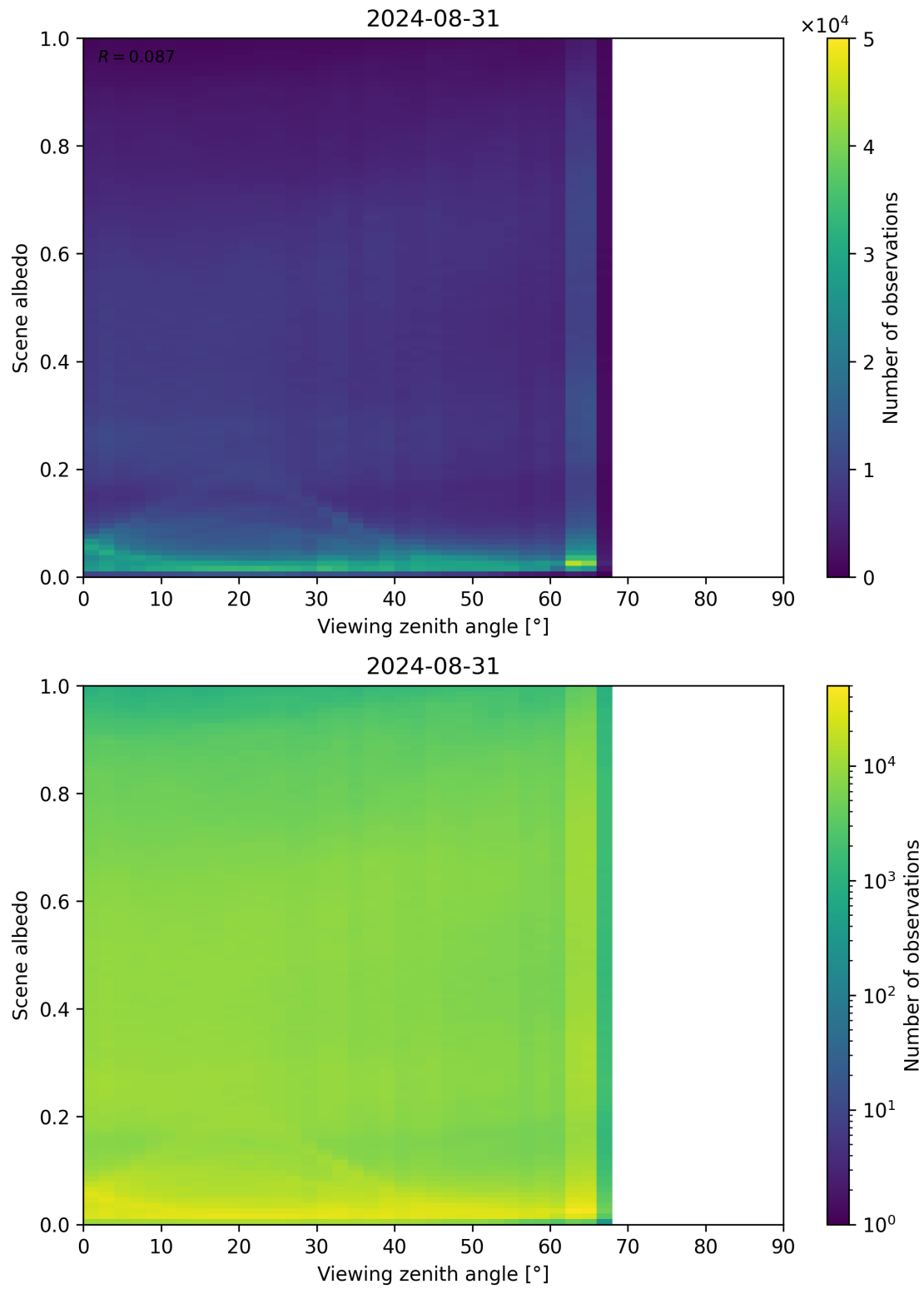
Figure 126: Scatter density plot of “Viewing zenith angle” against “Scene albedo” for 2024-08-30 to 2024-09-01.
