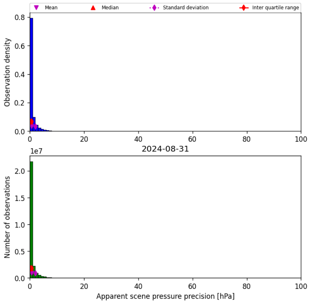
Figure 37: Histogram of “Apparent scene pressure precision” for 2024-08-30 to 2024-09-01
