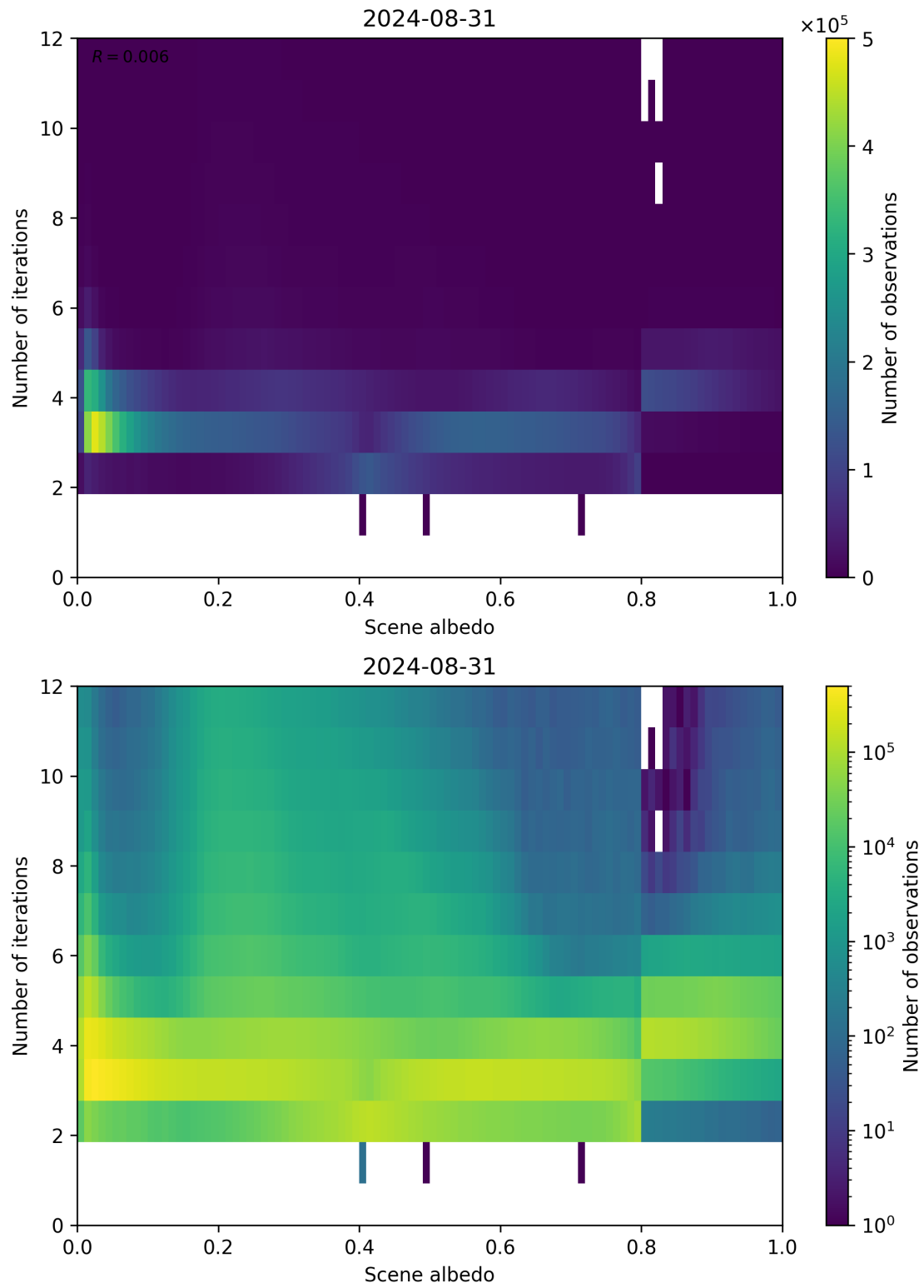
Figure 105: Scatter density plot of “Scene albedo” against “Number of iterations” for 2024-08-30 to 2024-09-01.
