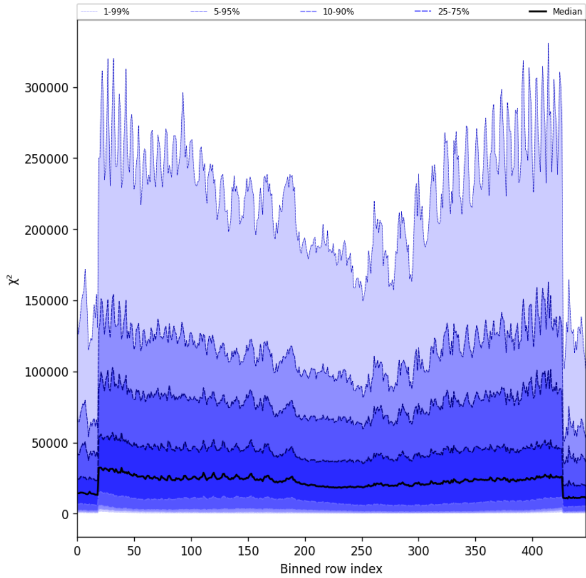
Figure 55: Along track statistics of “ \chi^2 ” for 2024-08-30 to 2024-09-01
