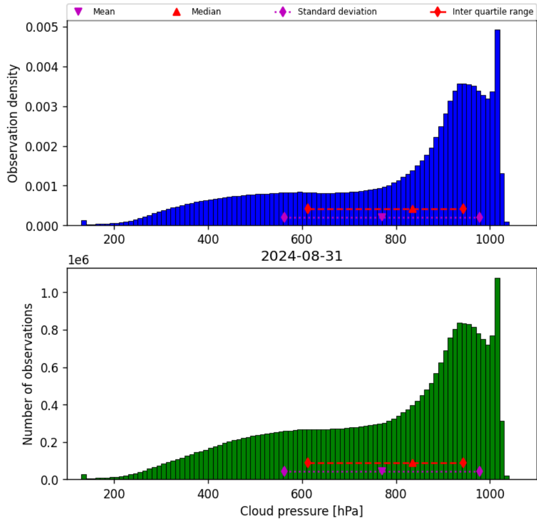
Figure 30: Histogram of “Cloud pressure” for 2024-08-30 to 2024-09-01
