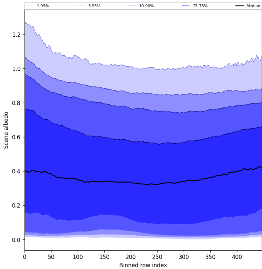
Figure 51: Along track statistics of “Scene albedo” for 2024-08-30 to 2024-09-01
