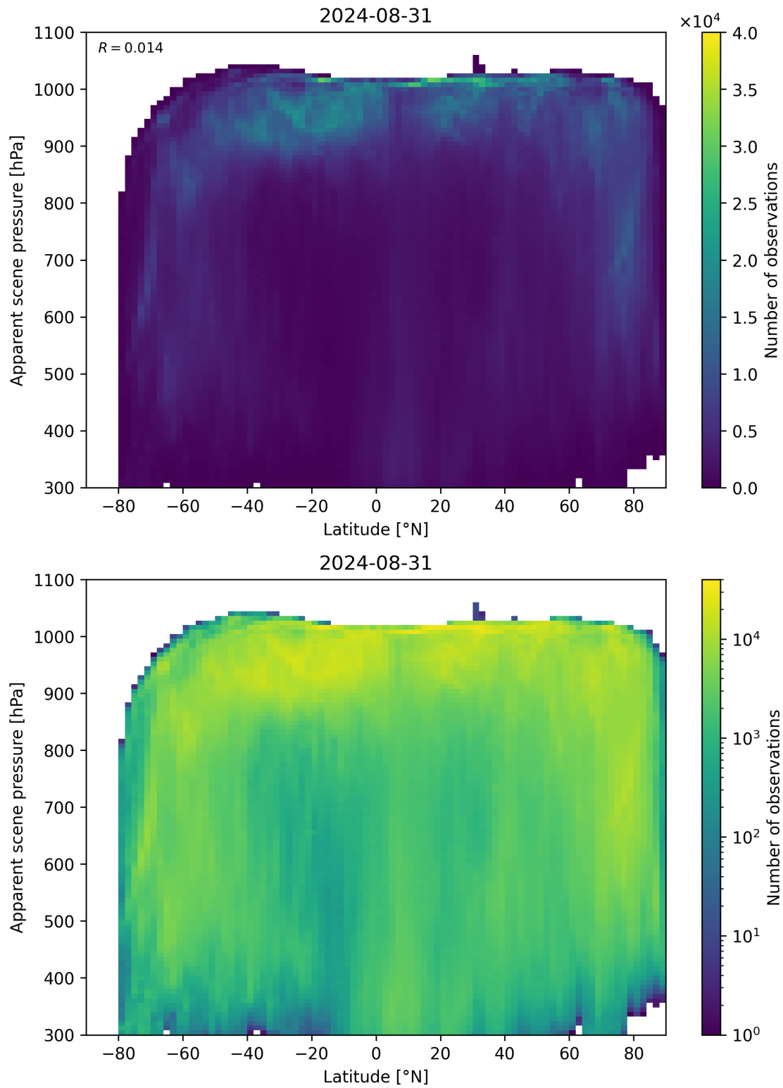
Figure 88: Scatter density plot of “Latitude” against “Apparent scene pressure” for 2024-08-30 to 2024-09-01.
