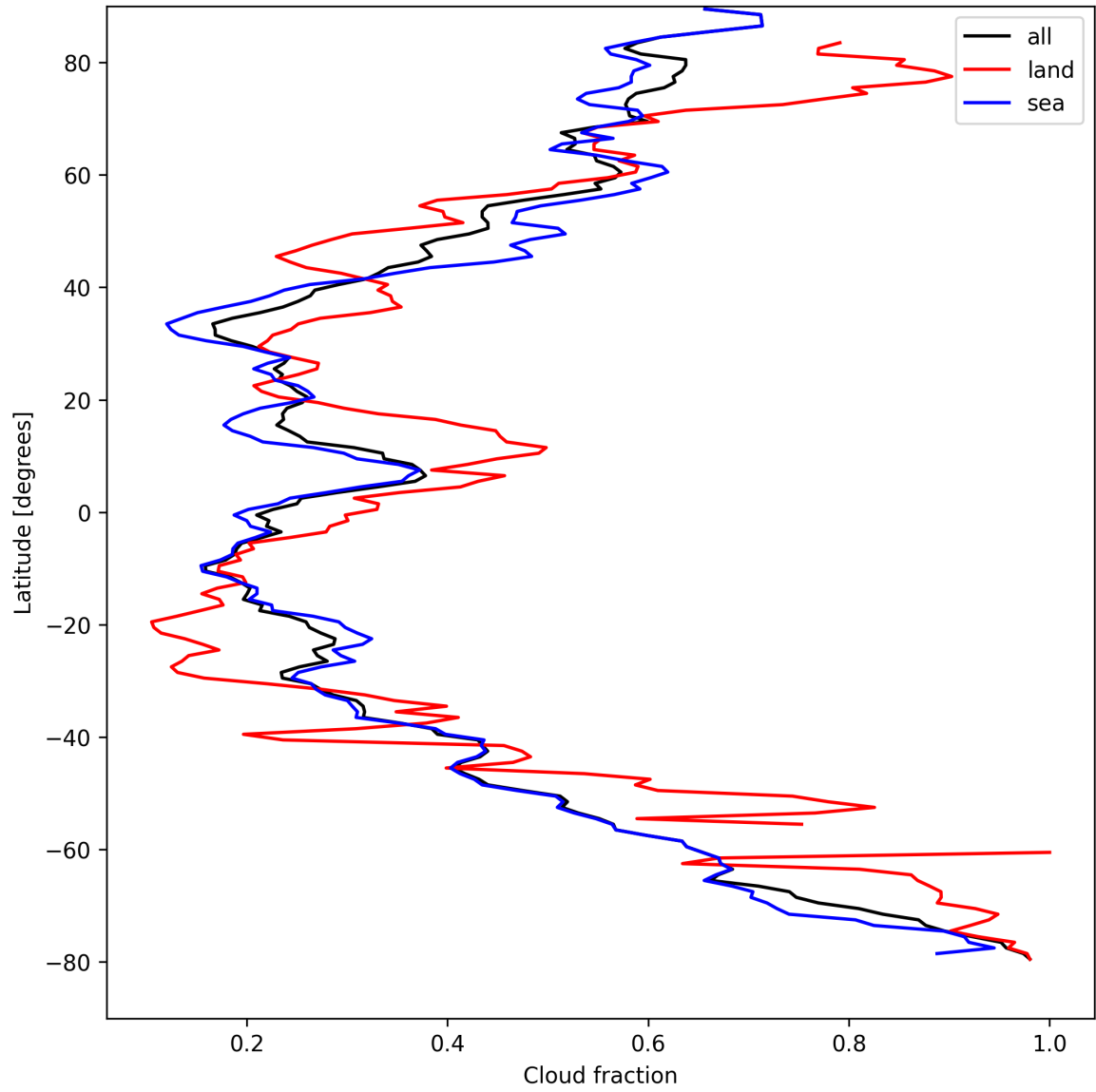
Figure 15: Zonal average of “Cloud fraction” for 2024-08-30 to 2024-09-01.
