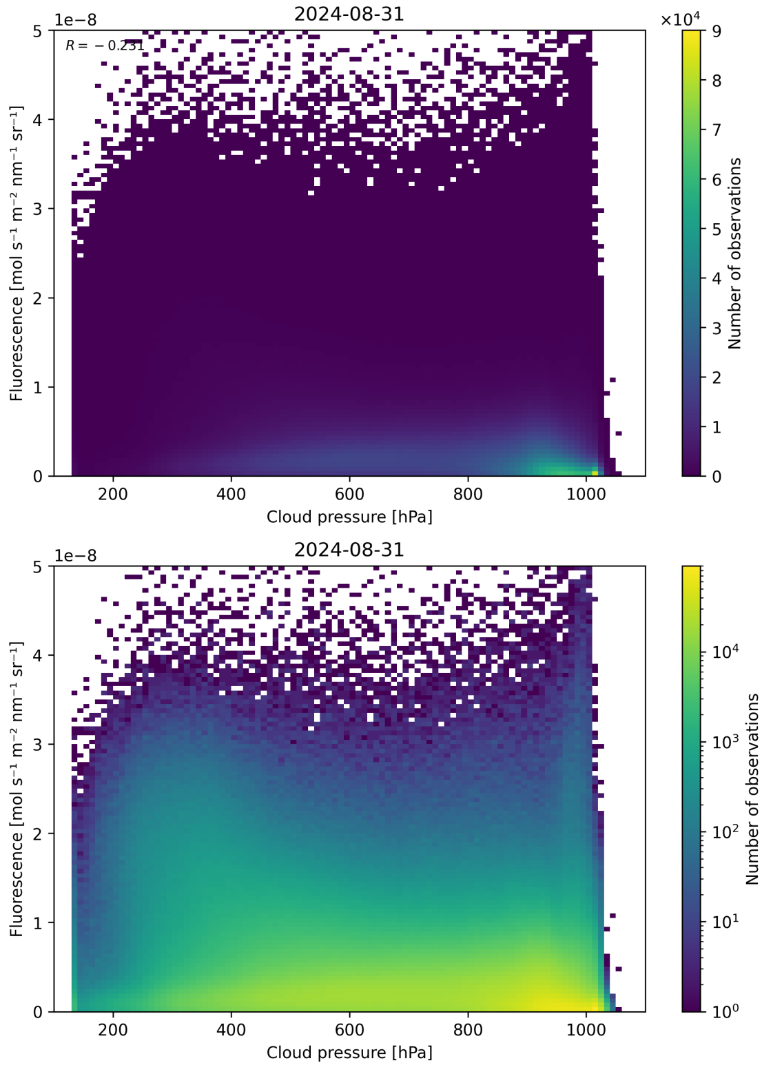
Figure 80: Scatter density plot of “Cloud pressure” against “Fluorescence” for 2024-08-30 to 2024-09-01.
