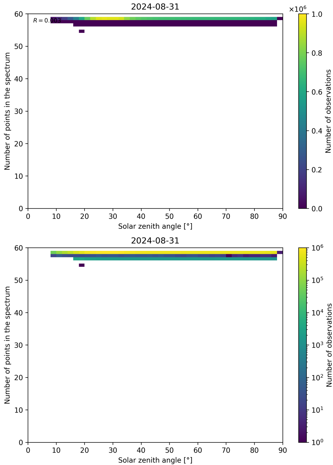
Figure 115: Scatter density plot of “Solar zenith angle” against “Number of points in the spectrum” for 2024-08-30 to 2024-09-01.
