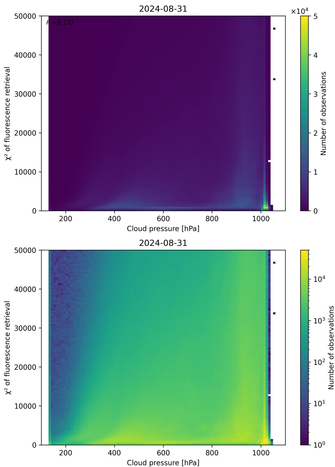
Figure 78: Scatter density plot of “Cloud pressure” against “ \chi^2 of fluorescence retrieval” for 2024-08-30 to 2024-09-01.
