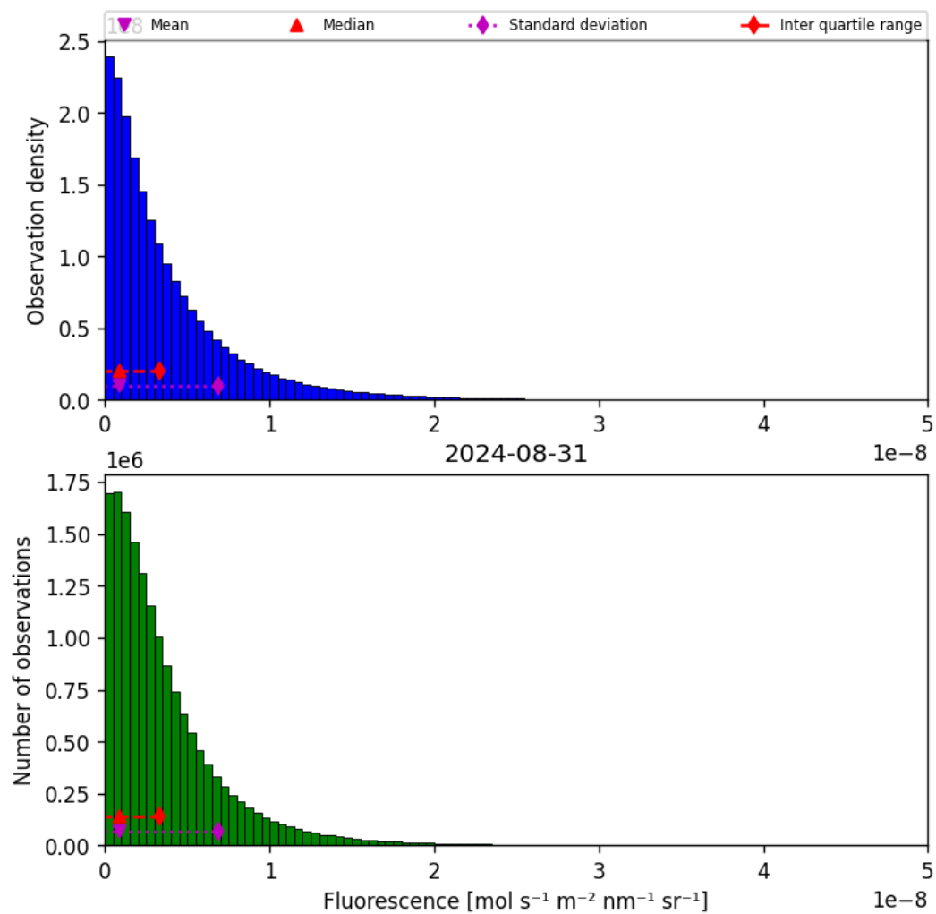
Figure 40: Histogram of “Fluorescence” for 2024-08-30 to 2024-09-01
