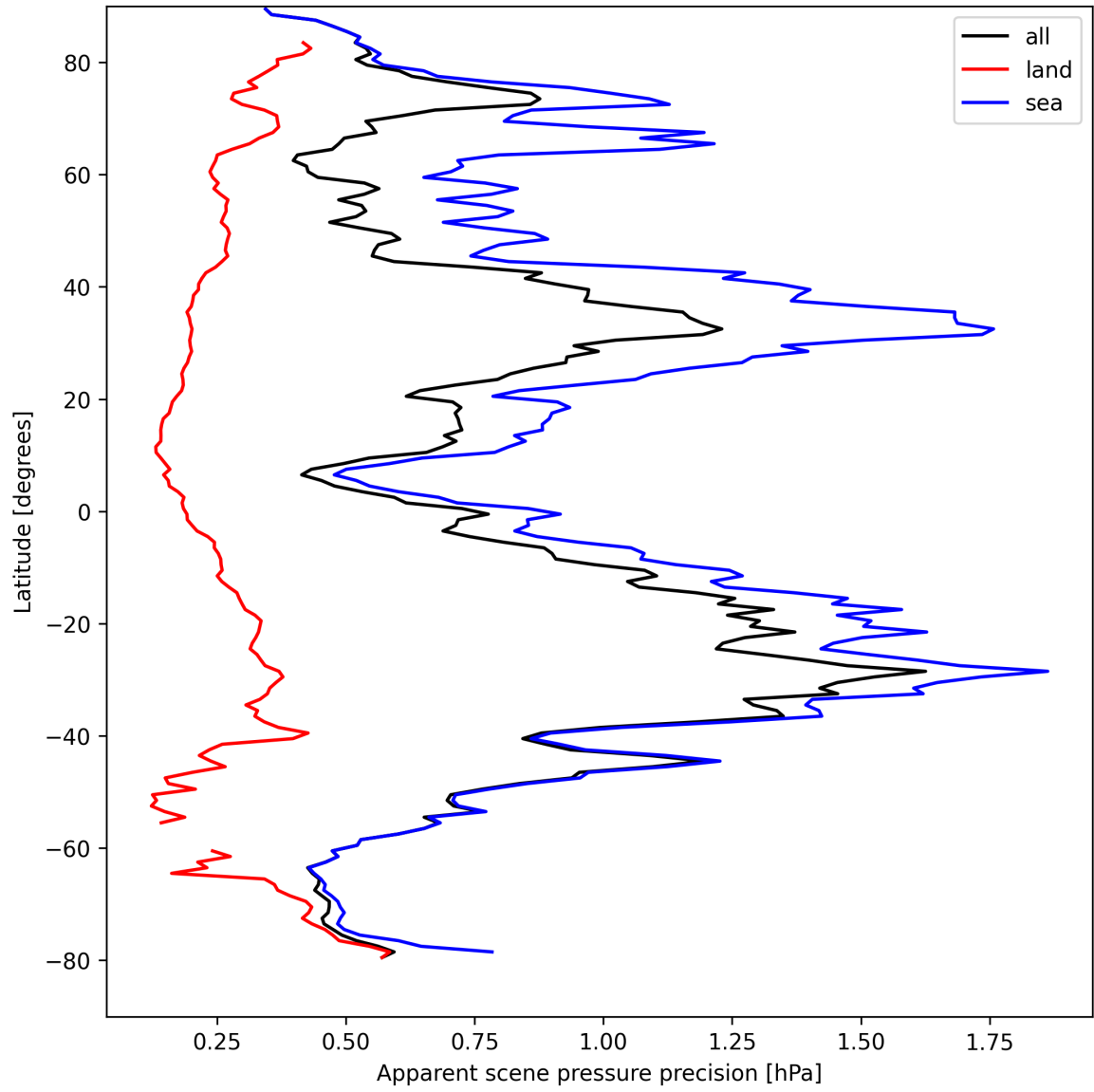
Figure 20: Zonal average of “Apparent scene pressure precision” for 2024-08-30 to 2024-09-01.
