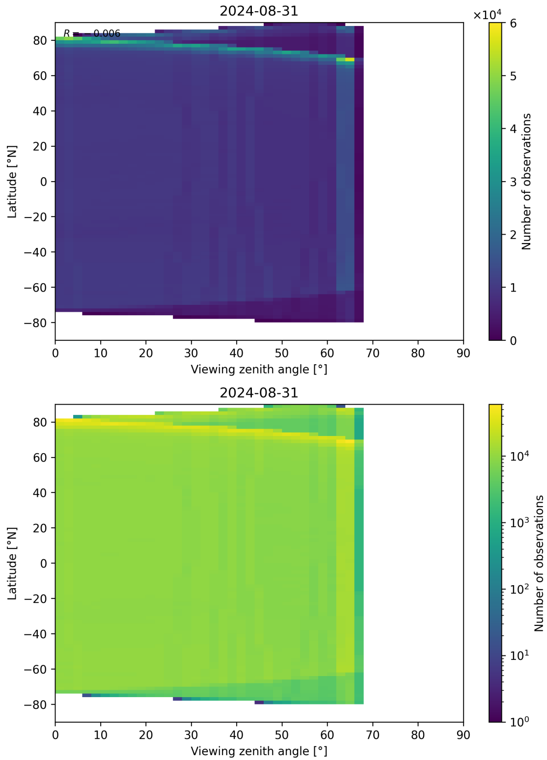
Figure 123: Scatter density plot of “Viewing zenith angle” against “Latitude” for 2024-08-30 to 2024-09-01.
