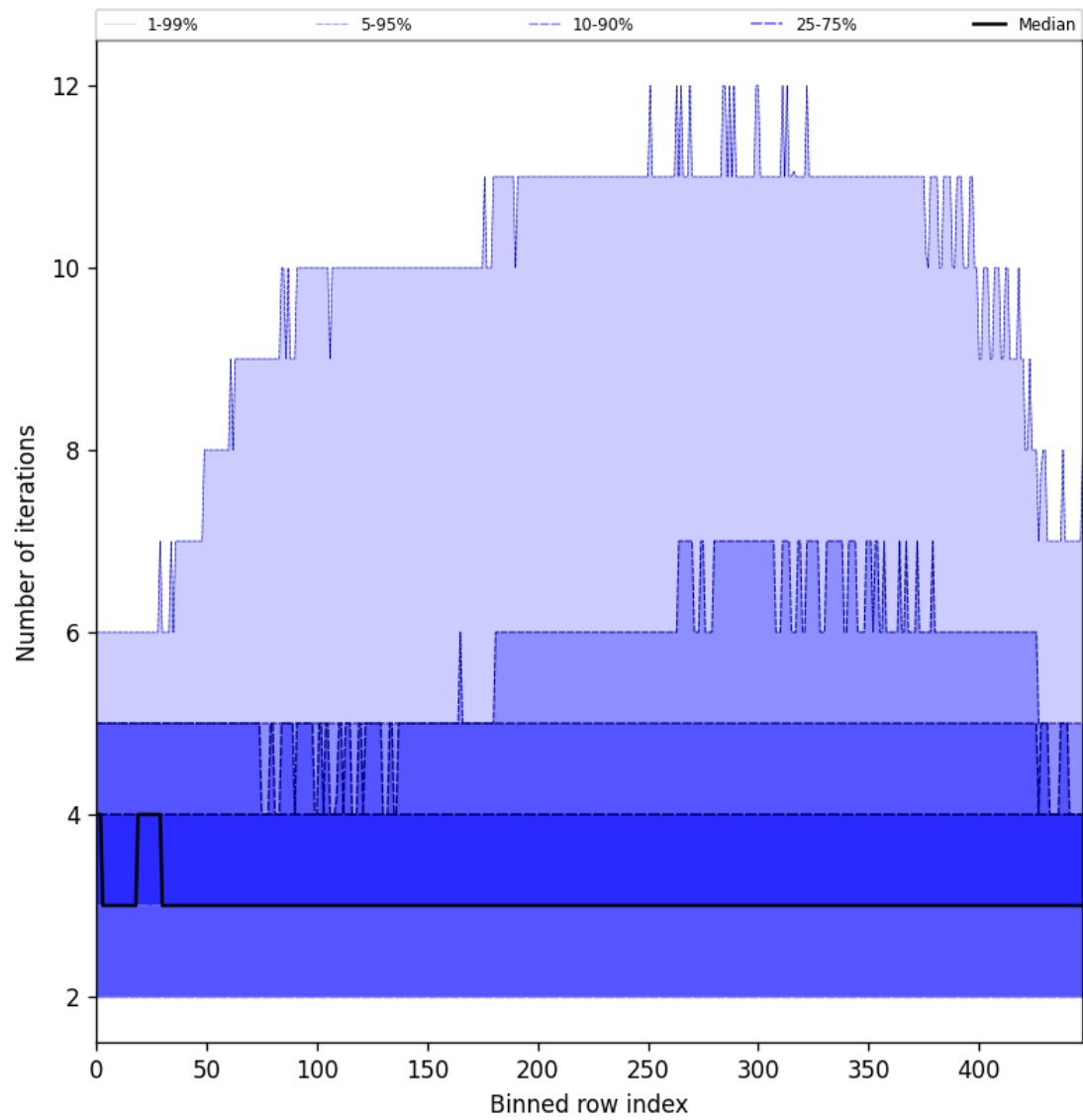
Figure 56: Along track statistics of “Number of iterations” for 2024-08-30 to 2024-09-01
