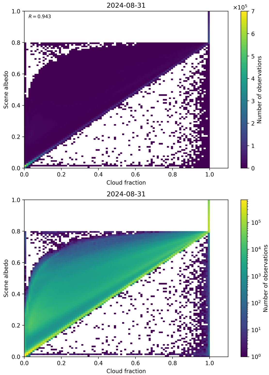
Figure 75: Scatter density plot of “Cloud fraction” against “Scene albedo” for 2024-08-30 to 2024-09-01.
