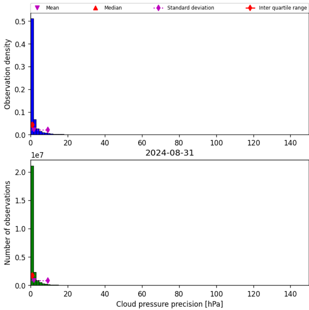
Figure 31: Histogram of “Cloud pressure precision” for 2024-08-30 to 2024-09-01
