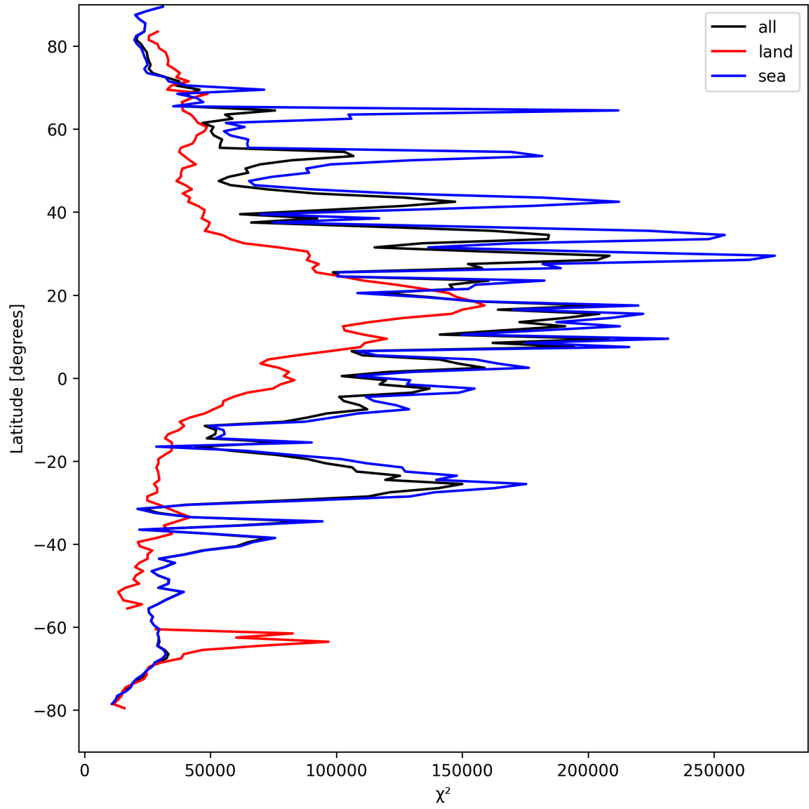
Figure 21: Zonal average of “ \chi^2 ” for 2024-08-30 to 2024-09-01.
