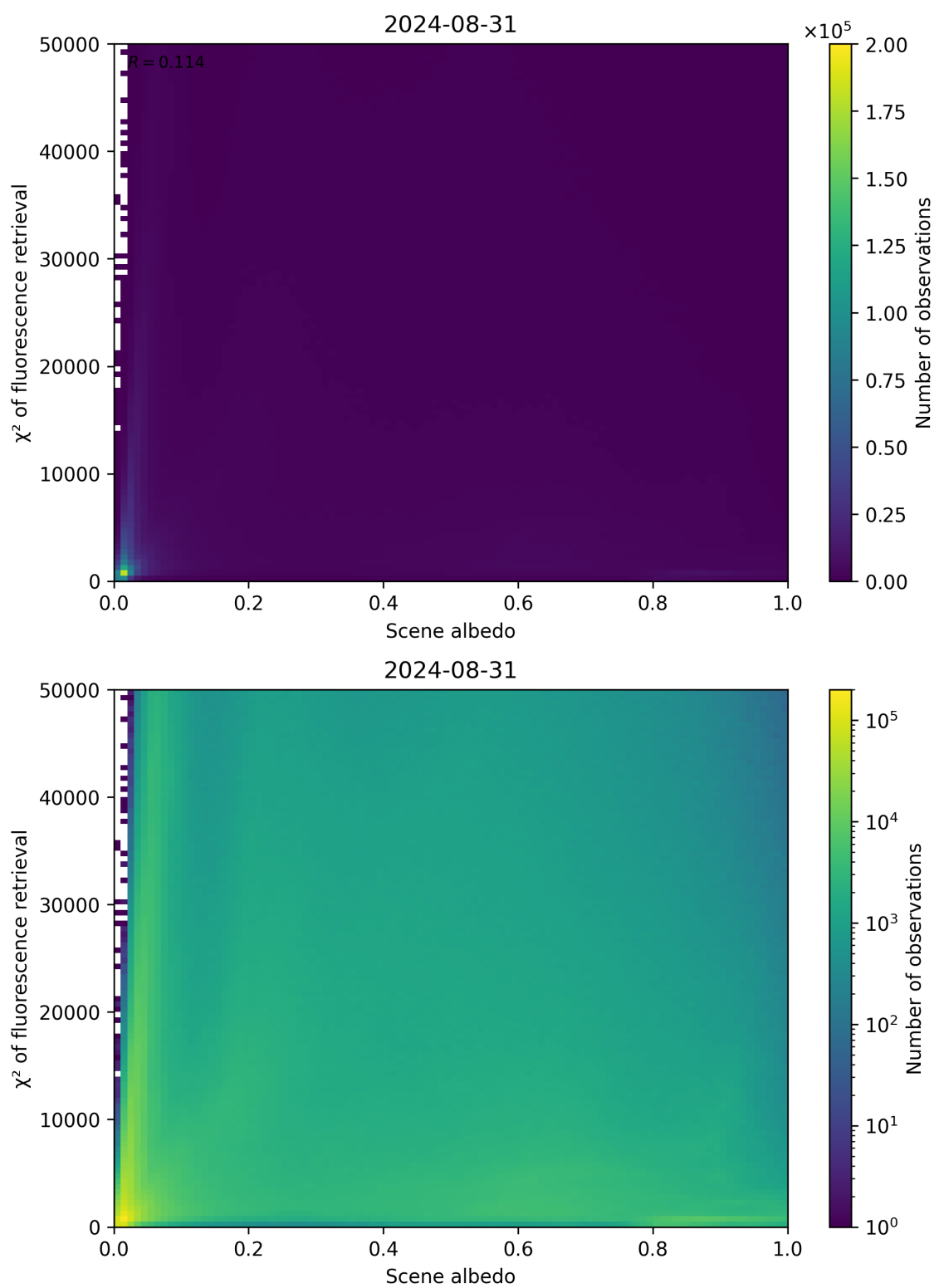
Figure 103: Scatter density plot of “Scene albedo” against “ \chi^2 of fluorescence retrieval” for 2024-08-30 to 2024-09-01.
