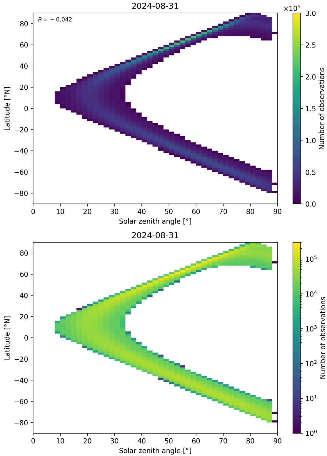
Figure 113: Scatter density plot of “Solar zenith angle” against “Latitude” for 2024-08-30 to 2024-09-01.
