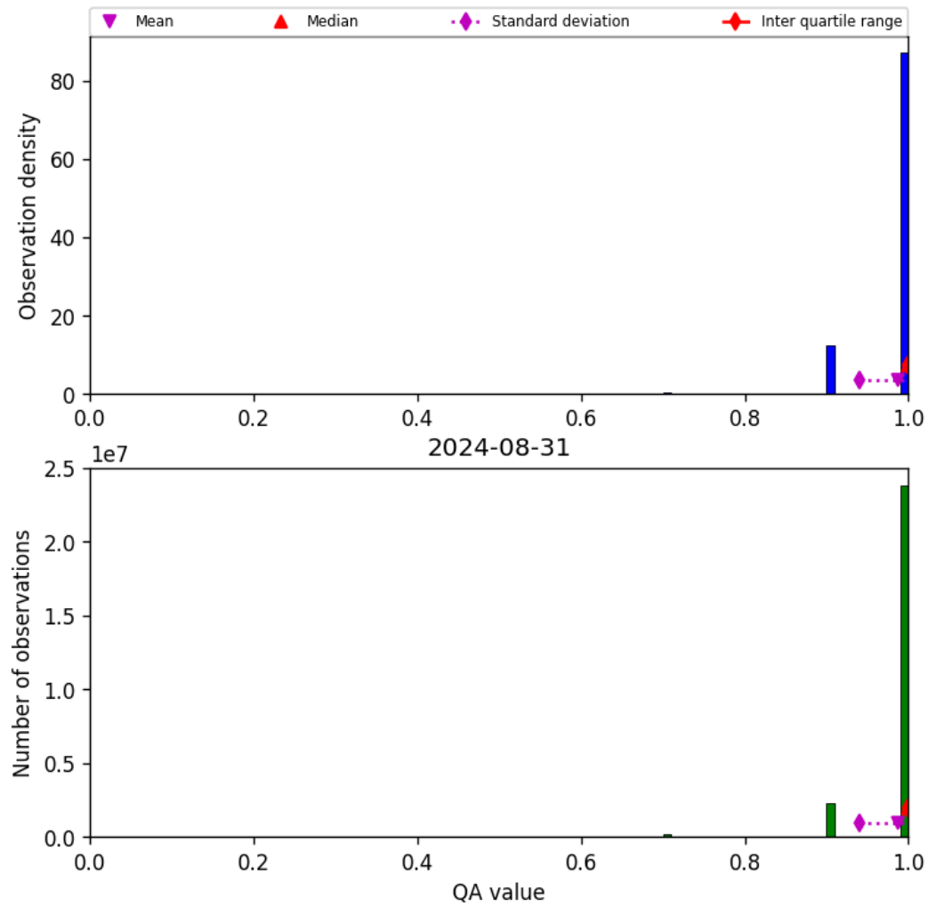
Figure 29: Histogram of “QA value” for 2024-08-30 to 2024-09-01
