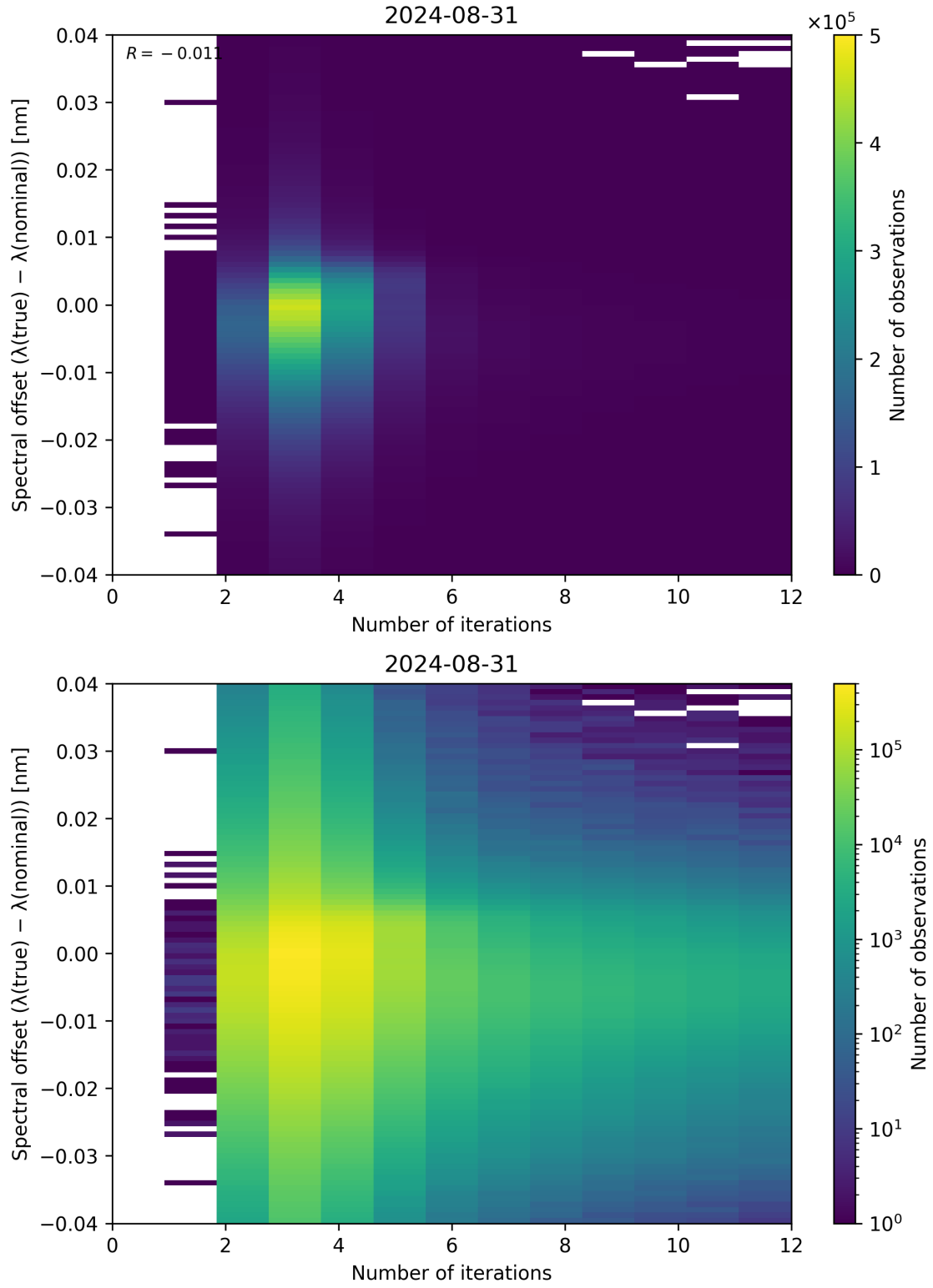
Figure 100: Scatter density plot of “Number of iterations” against “Spectral offset ( \lambda_{\text{true}} - \lambda_{\text{nominal}} )” for 2024-08-30 to 2024-09-01.
