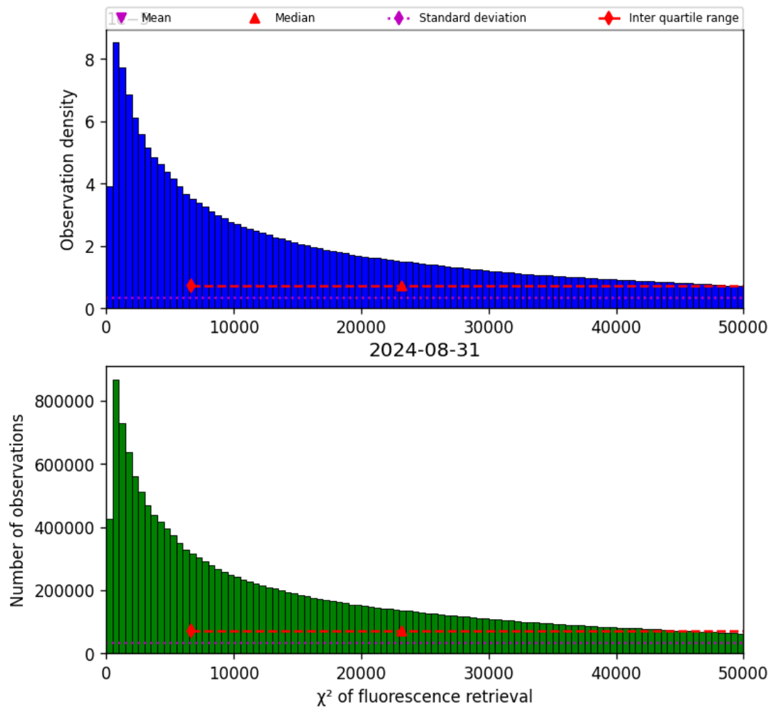
Figure 42: Histogram of “ \chi^2 of fluorescence retrieval” for 2024-08-30 to 2024-09-01
