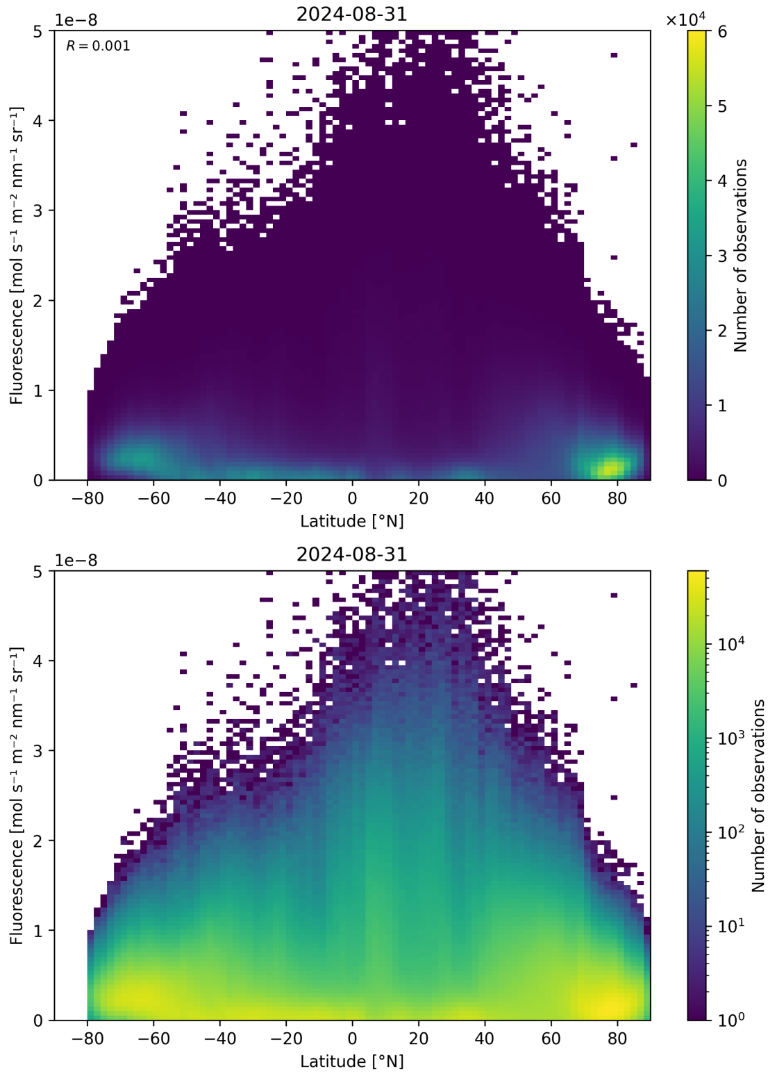
Figure 92: Scatter density plot of “Latitude” against “Fluorescence” for 2024-08-30 to 2024-09-01.
