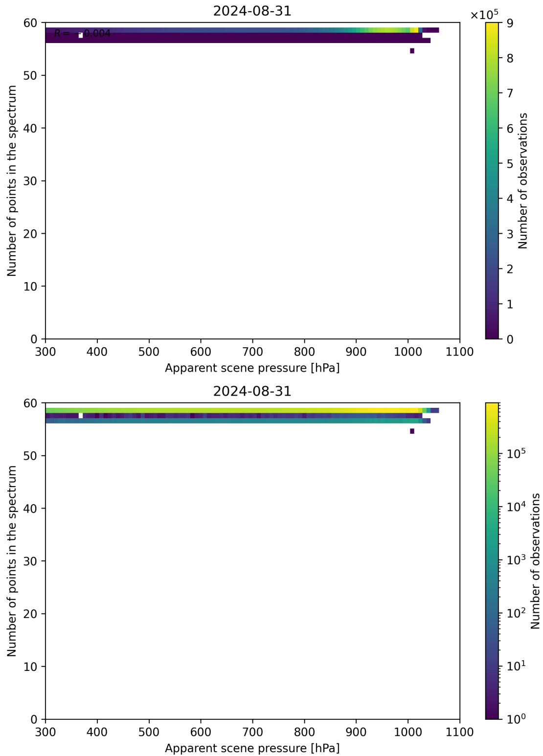
Figure 66: Scatter density plot of “Apparent scene pressure” against “Number of points in the spectrum” for 2024-08-30 to 2024-09-01.
