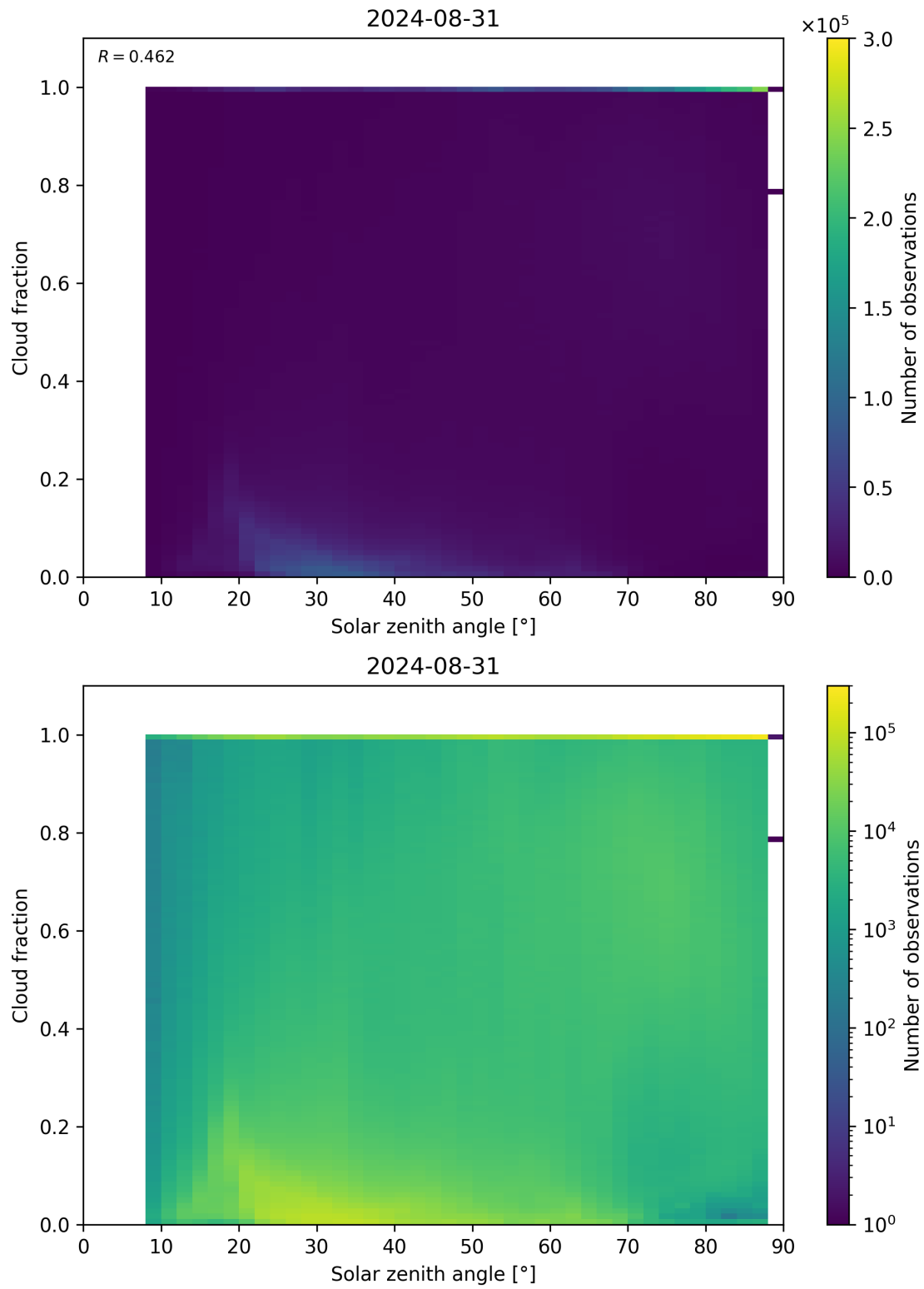
Figure 110: Scatter density plot of “Solar zenith angle” against “Cloud fraction” for 2024-08-30 to 2024-09-01.
