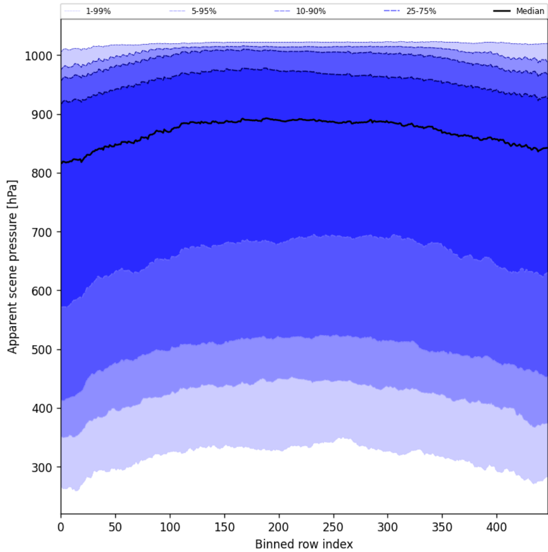
Figure 53: Along track statistics of “Apparent scene pressure” for 2024-08-30 to 2024-09-01
