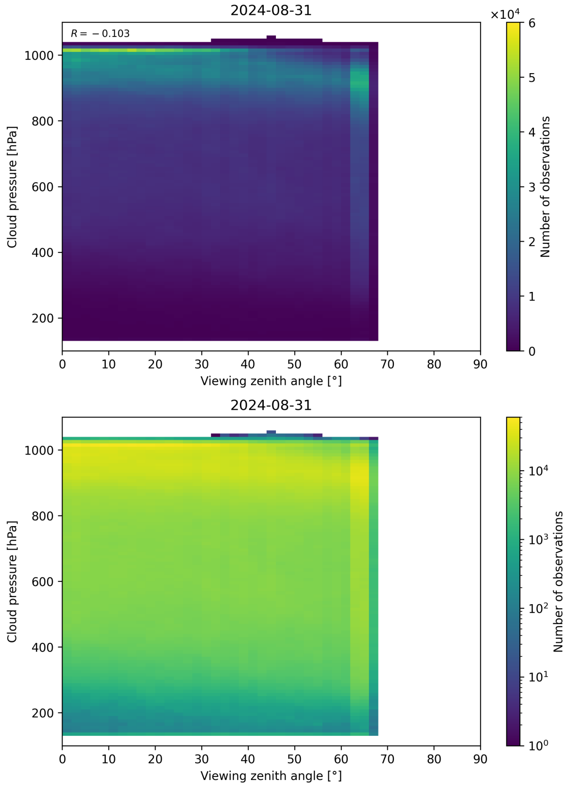
Figure 121: Scatter density plot of “Viewing zenith angle” against “Cloud pressure” for 2024-08-30 to 2024-09-01.
