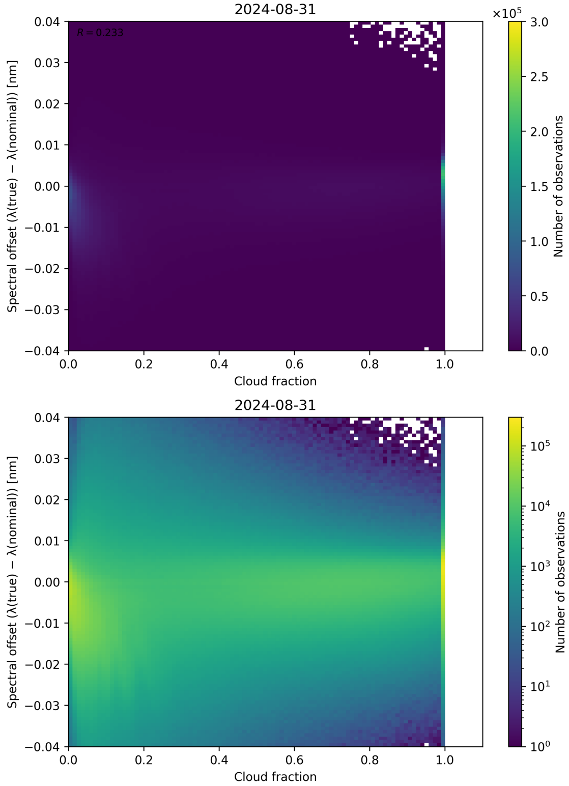
Figure 76: Scatter density plot of “Cloud fraction” against “Spectral offset ( \lambda_{\text{true}} - \lambda_{\text{nominal}} )” for 2024-08-30 to 2024-09-01.
