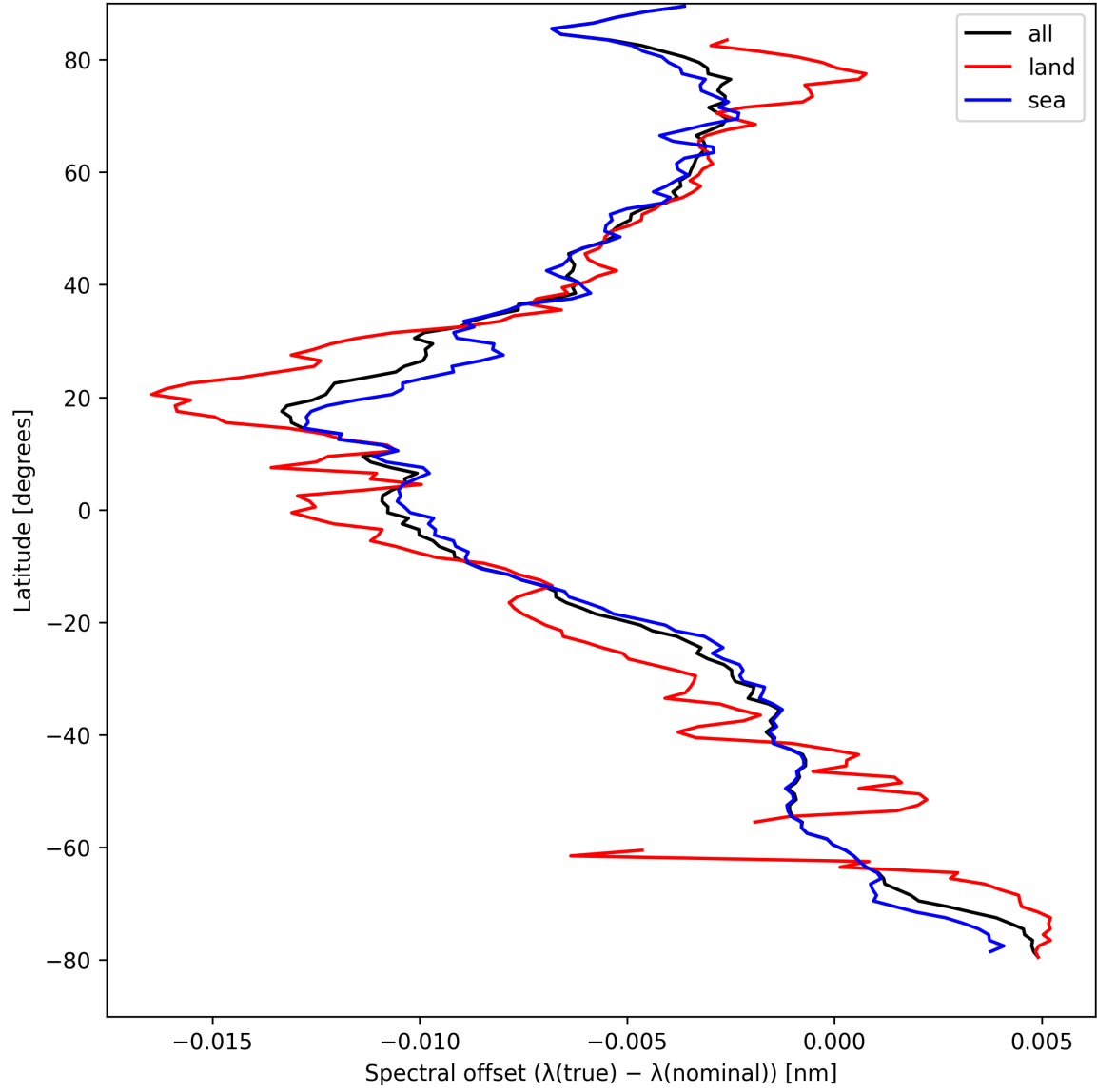
Figure 28: Zonal average of “Spectral offset ( \lambda_{\text{true}} - \lambda_{\text{nominal}} )” for 2024-08-30 to 2024-09-01.
