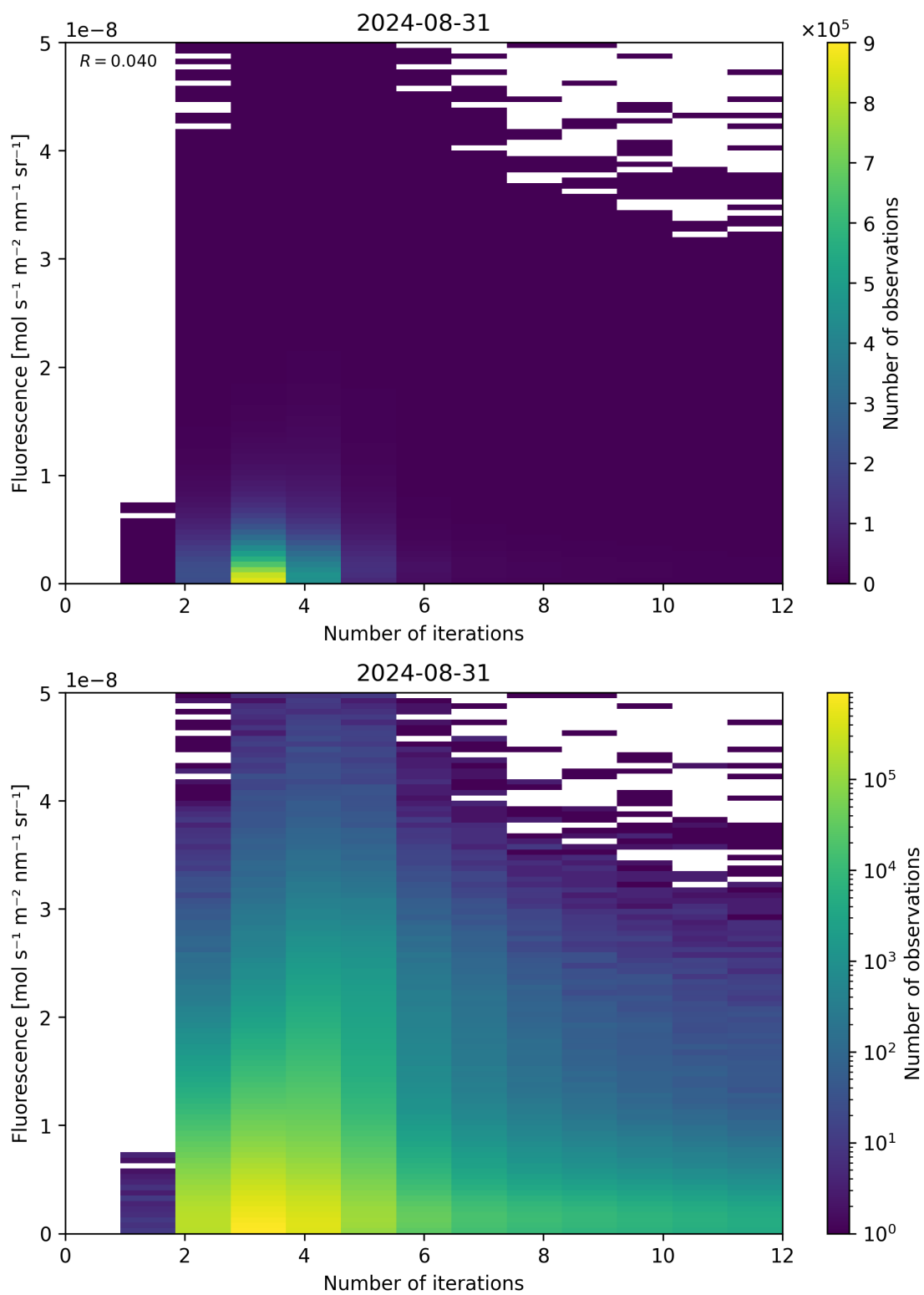
Figure 98: Scatter density plot of “Number of iterations” against “Fluorescence” for 2024-08-30 to 2024-09-01.
