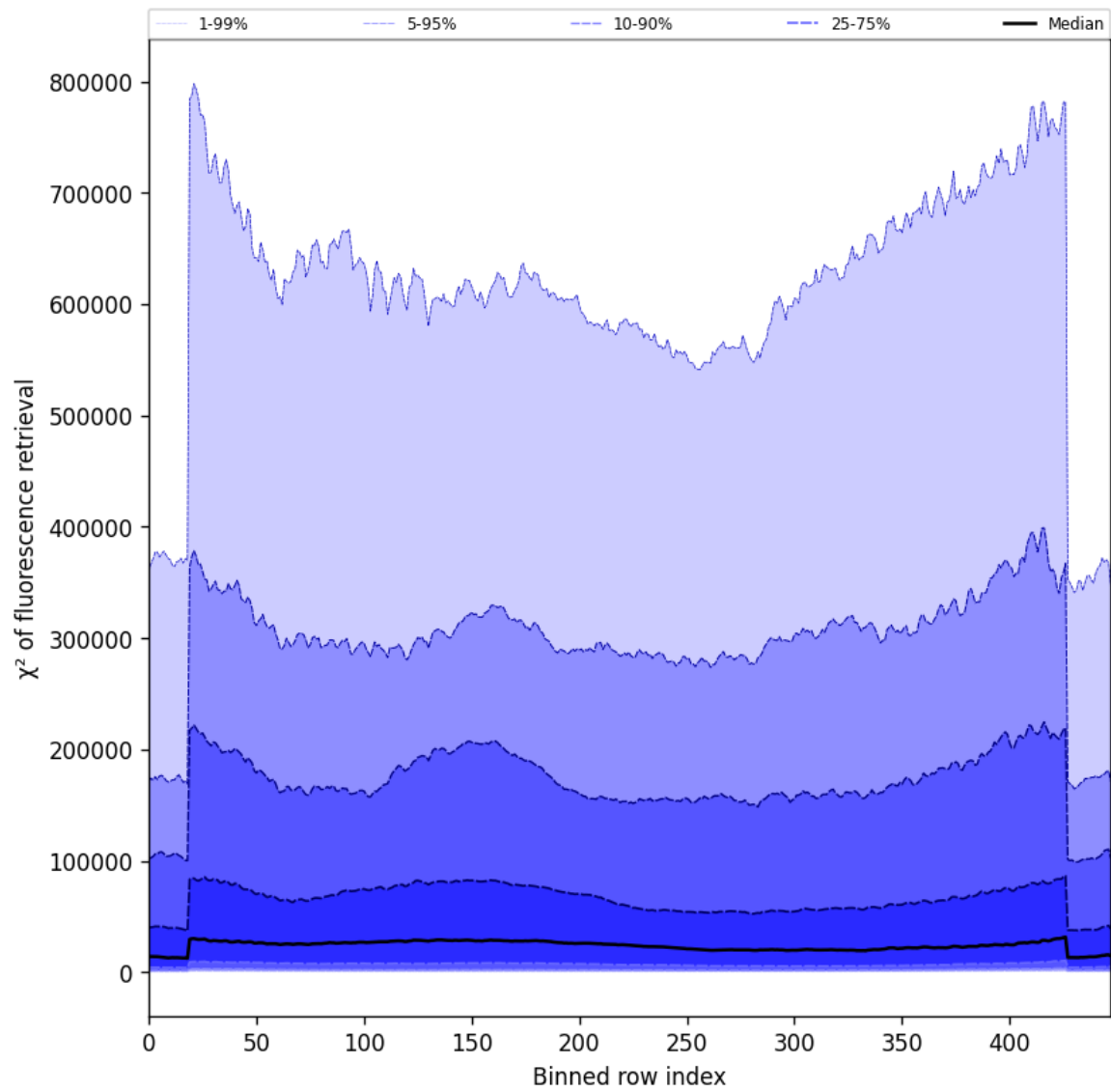
Figure 59: Along track statistics of " \chi^2 of fluorescence retrieval" for 2024-08-30 to 2024-09-01
