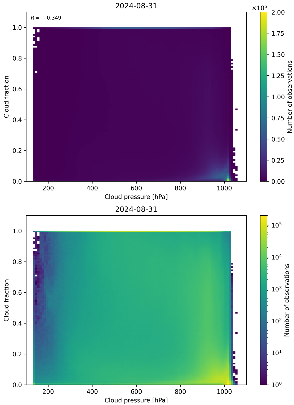
Figure 79: Scatter density plot of “Cloud pressure” against “Cloud fraction” for 2024-08-30 to 2024-09-01.
