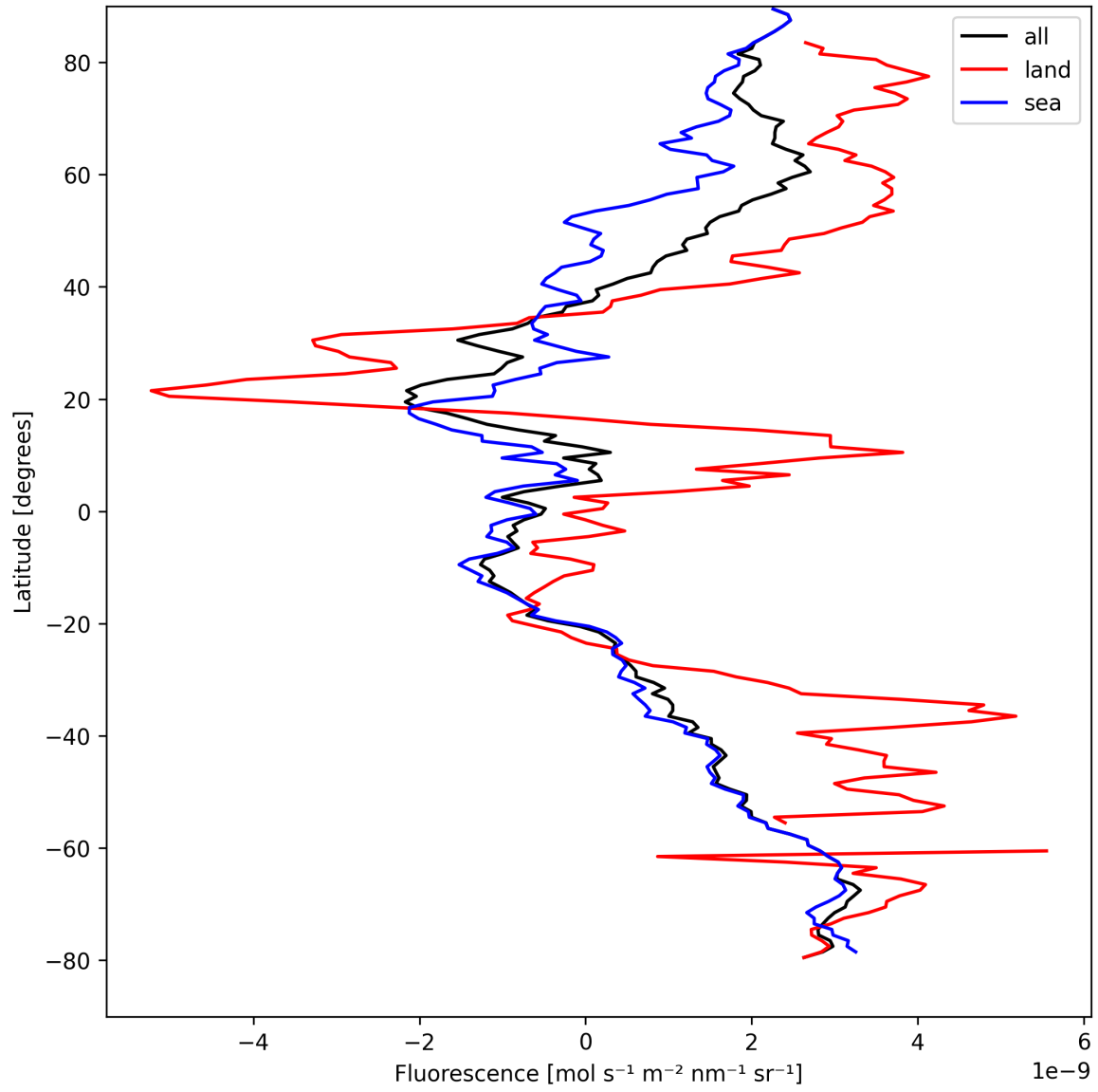
Figure 23: Zonal average of “Fluorescence” for 2024-08-30 to 2024-09-01.
