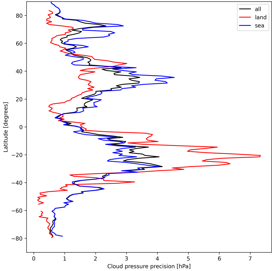
Figure 14: Zonal average of “Cloud pressure precision” for 2024-08-30 to 2024-09-01.
