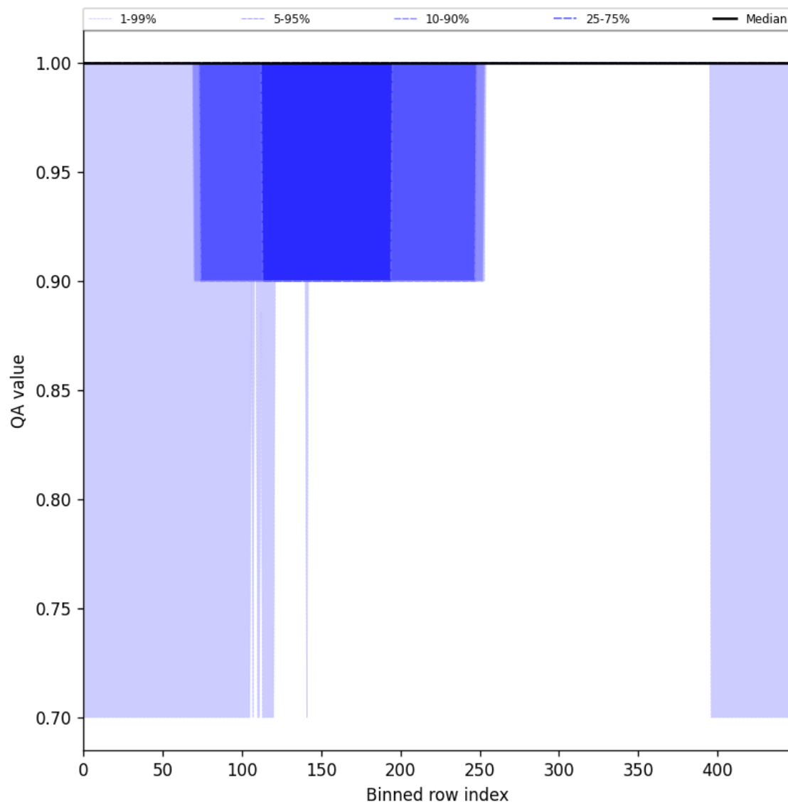
Figure 46: Along track statistics of “QA value” for 2024-08-30 to 2024-09-01
