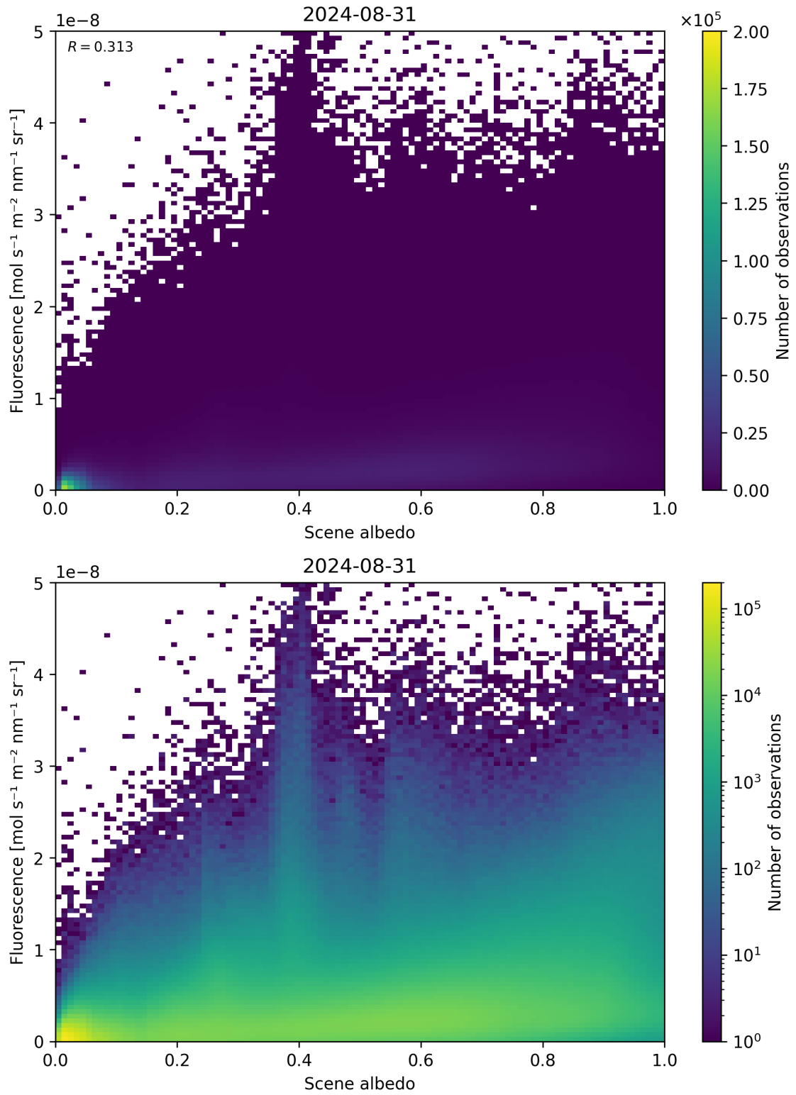
Figure 104: Scatter density plot of “Scene albedo” against “Fluorescence” for 2024-08-30 to 2024-09-01.
