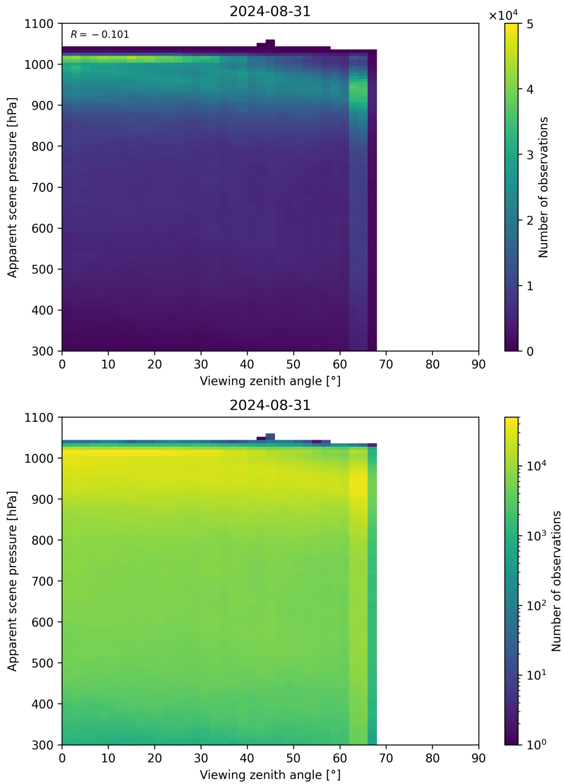
Figure 118: Scatter density plot of “Viewing zenith angle” against “Apparent scene pressure” for 2024-08-30 to 2024-09-01.
