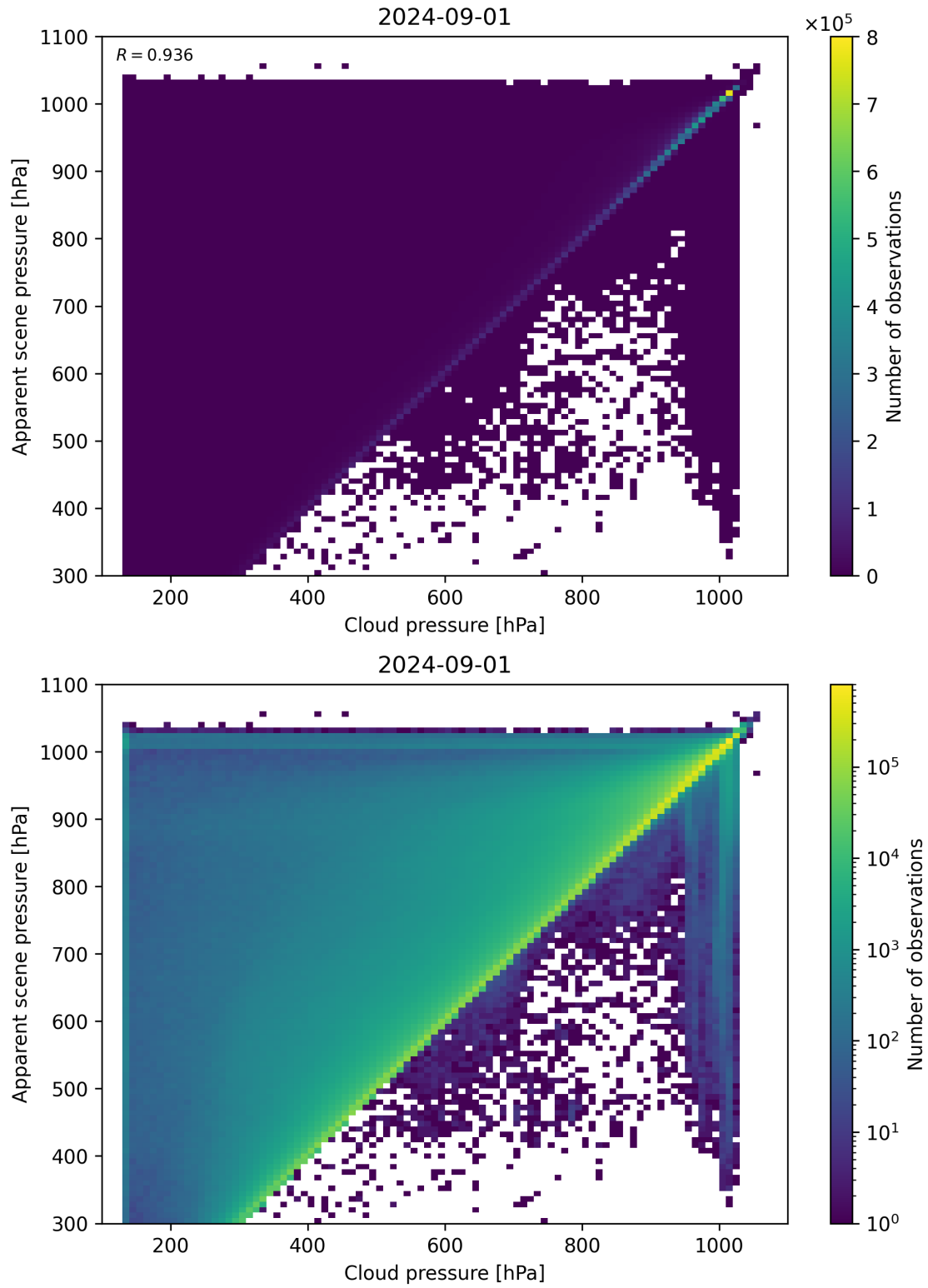
Figure 77: Scatter density plot of “Cloud pressure” against “Apparent scene pressure” for 2024-09-01 to 2024-09-02.
