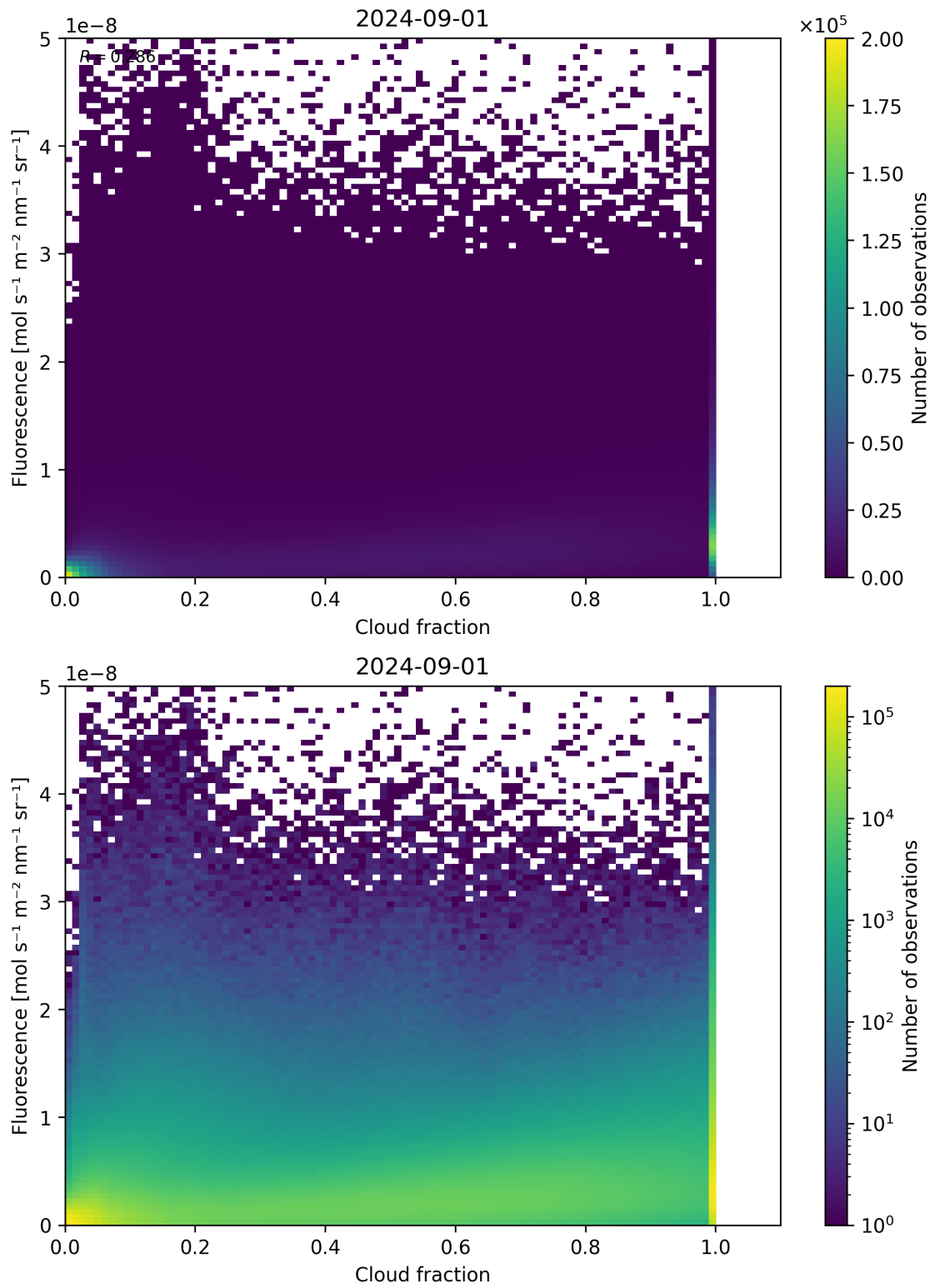
Figure 72: Scatter density plot of “Cloud fraction” against “Fluorescence” for 2024-09-01 to 2024-09-02.
