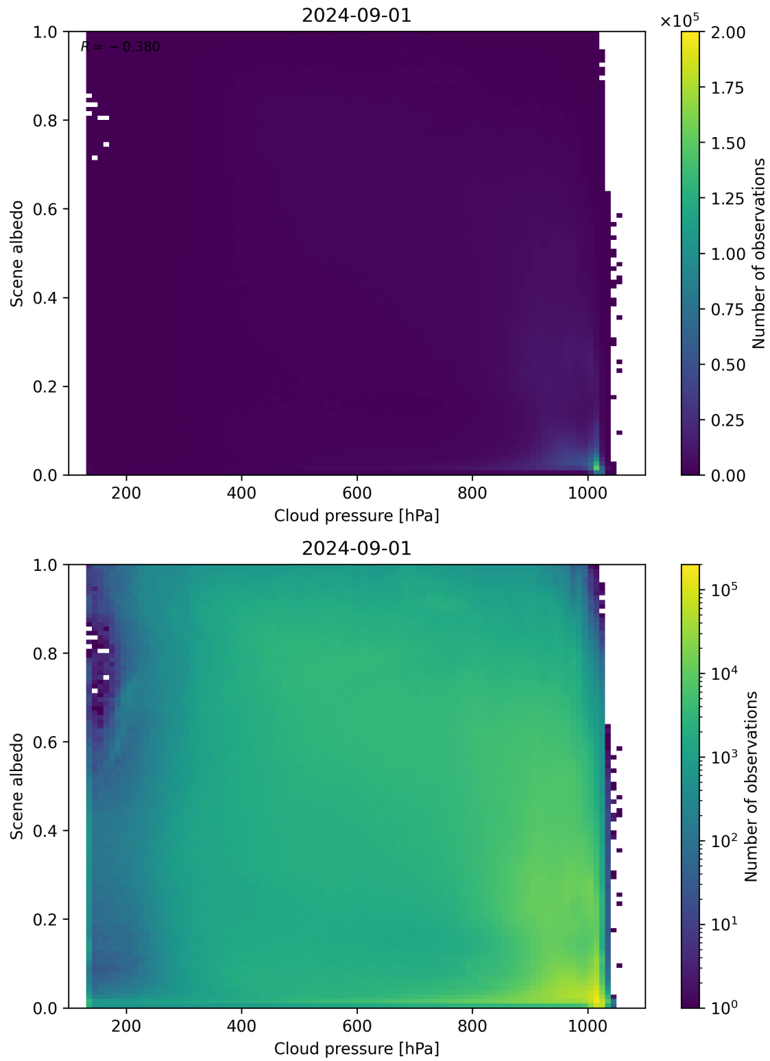
Figure 83: Scatter density plot of “Cloud pressure” against “Scene albedo” for 2024-09-01 to 2024-09-02.
