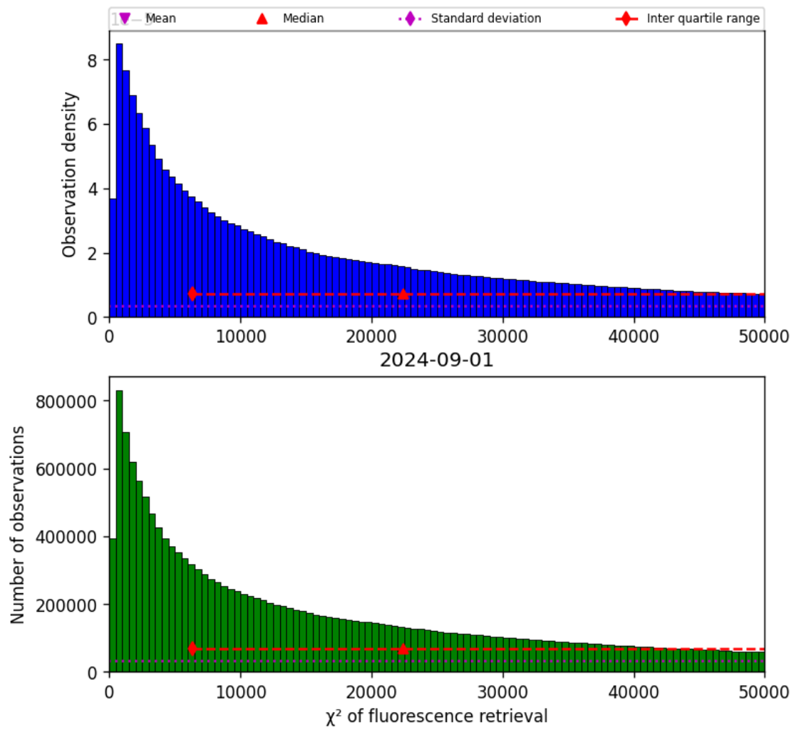
Figure 42: Histogram of “ \chi^2 of fluorescence retrieval” for 2024-09-01 to 2024-09-02
