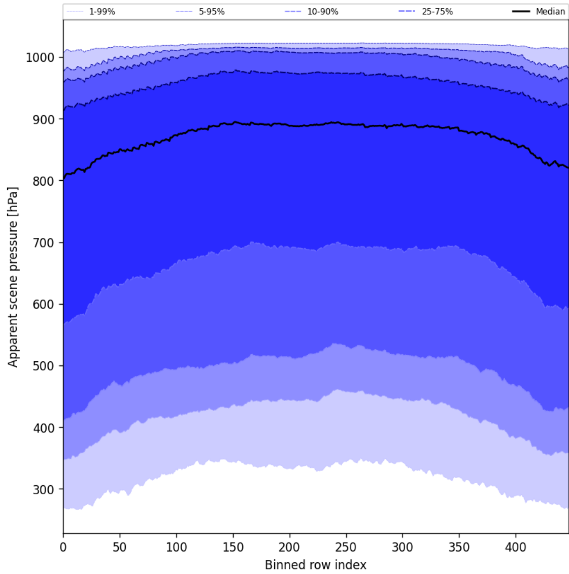
Figure 53: Along track statistics of “Apparent scene pressure” for 2024-09-01 to 2024-09-02
