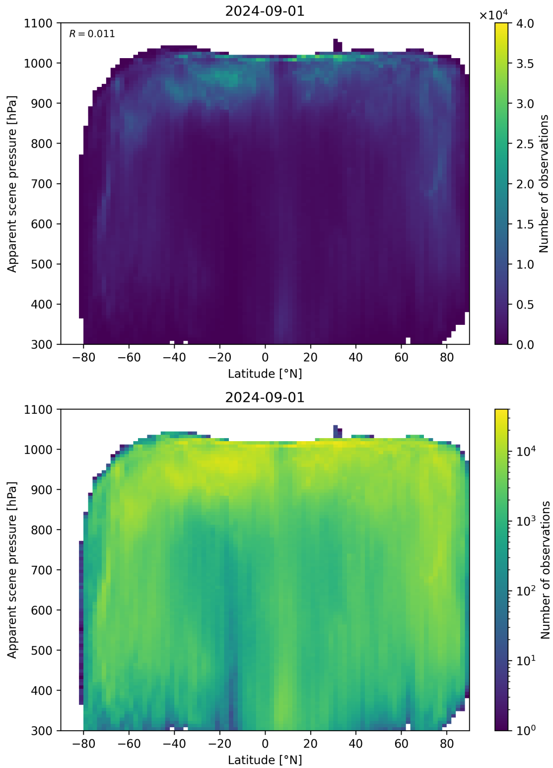
Figure 88: Scatter density plot of “Latitude” against “Apparent scene pressure” for 2024-09-01 to 2024-09-02.
