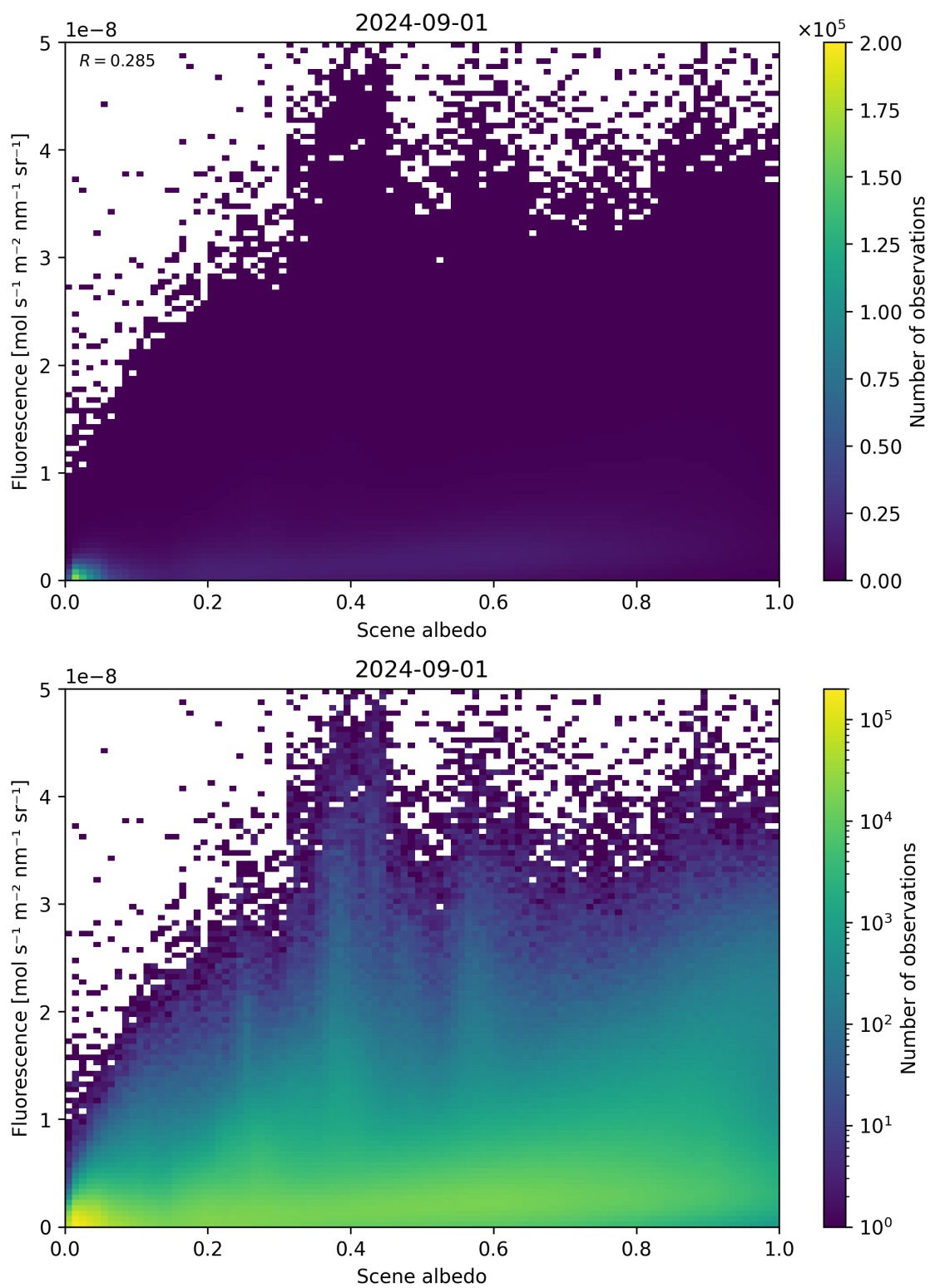
Figure 104: Scatter density plot of “Scene albedo” against “Fluorescence” for 2024-09-01 to 2024-09-02.
