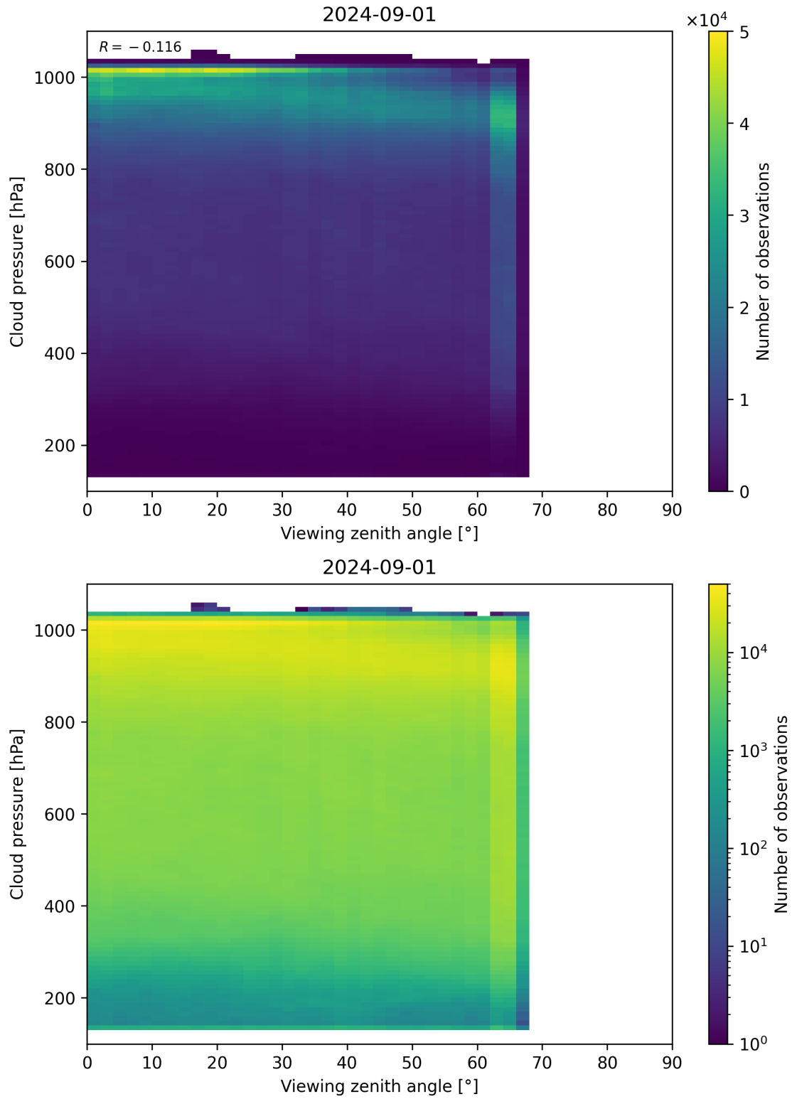
Figure 121: Scatter density plot of “Viewing zenith angle” against “Cloud pressure” for 2024-09-01 to 2024-09-02.
