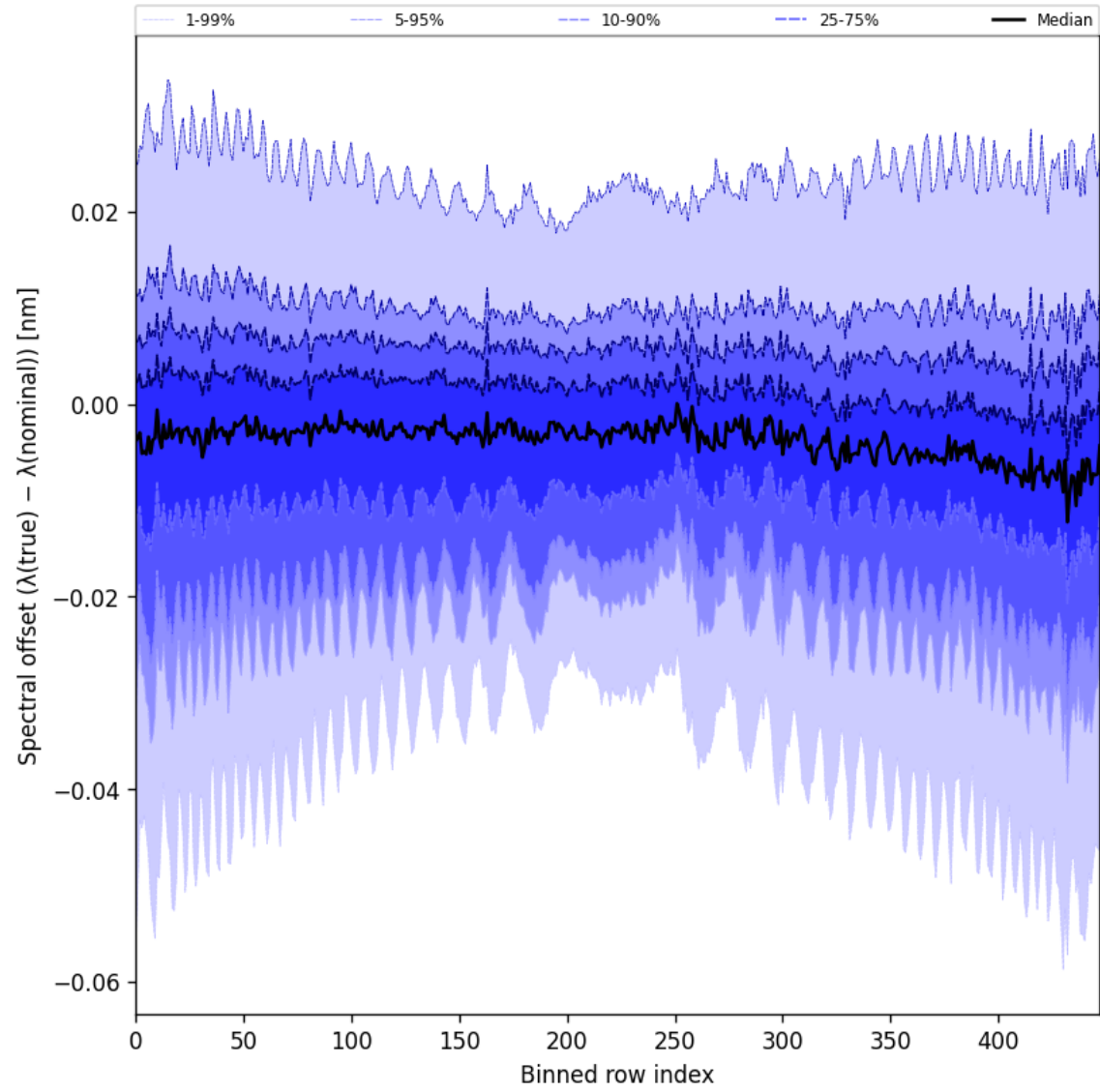
Figure 62: Along track statistics of “Spectral offset ( \lambda_{\text{true}} - \lambda_{\text{nominal}} )” for 2024-09-01 to 2024-09-02
