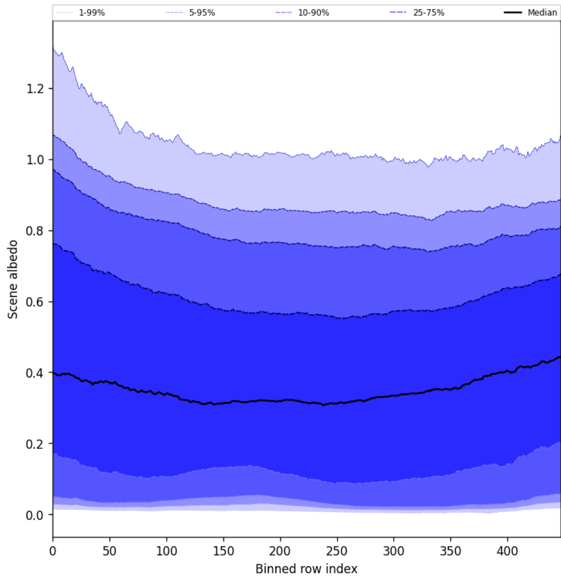
Figure 51: Along track statistics of “Scene albedo” for 2024-09-01 to 2024-09-02
