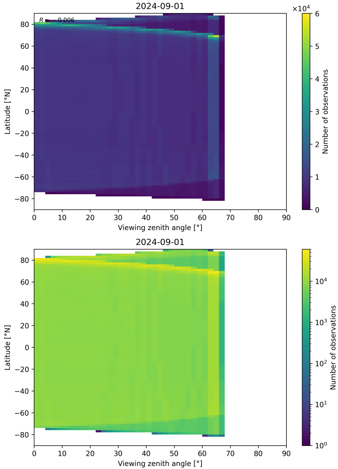
Figure 123: Scatter density plot of “Viewing zenith angle” against “Latitude” for 2024-09-01 to 2024-09-02.
