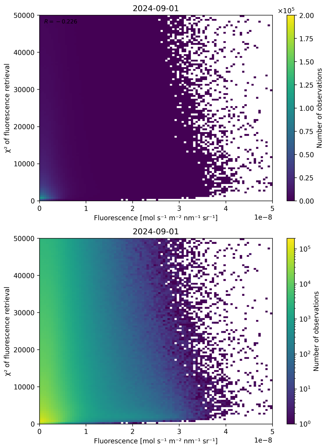
Figure 85: Scatter density plot of “Fluorescence” against “ \chi^2 of fluorescence retrieval” for 2024-09-01 to 2024-09-02.
