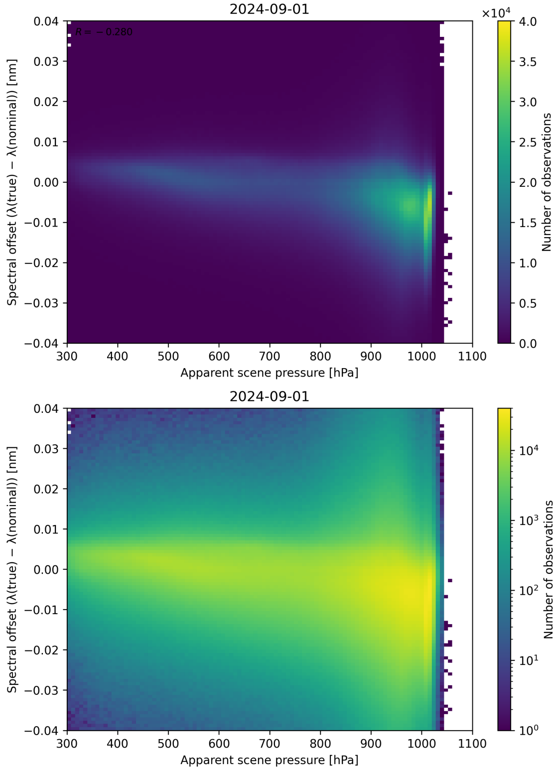
Figure 67: Scatter density plot of “Apparent scene pressure” against “Spectral offset ( \lambda_{\text{true}} - \lambda_{\text{nominal}} )” for 2024-09-01 to 2024-09-02.
