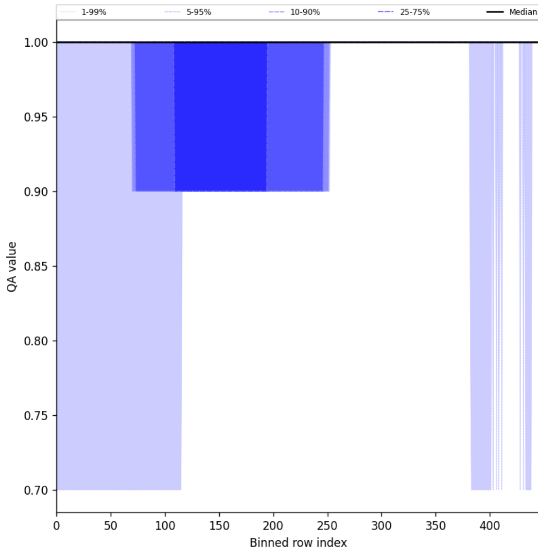
Figure 46: Along track statistics of “QA value” for 2024-09-01 to 2024-09-02
