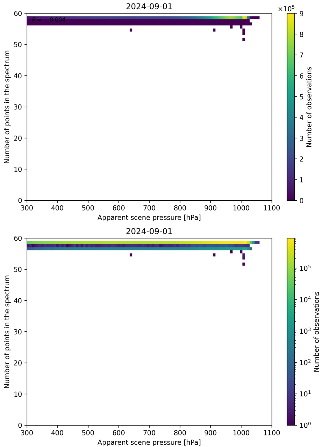
Figure 66: Scatter density plot of “Apparent scene pressure” against “Number of points in the spectrum” for 2024-09-01 to 2024-09-02.
