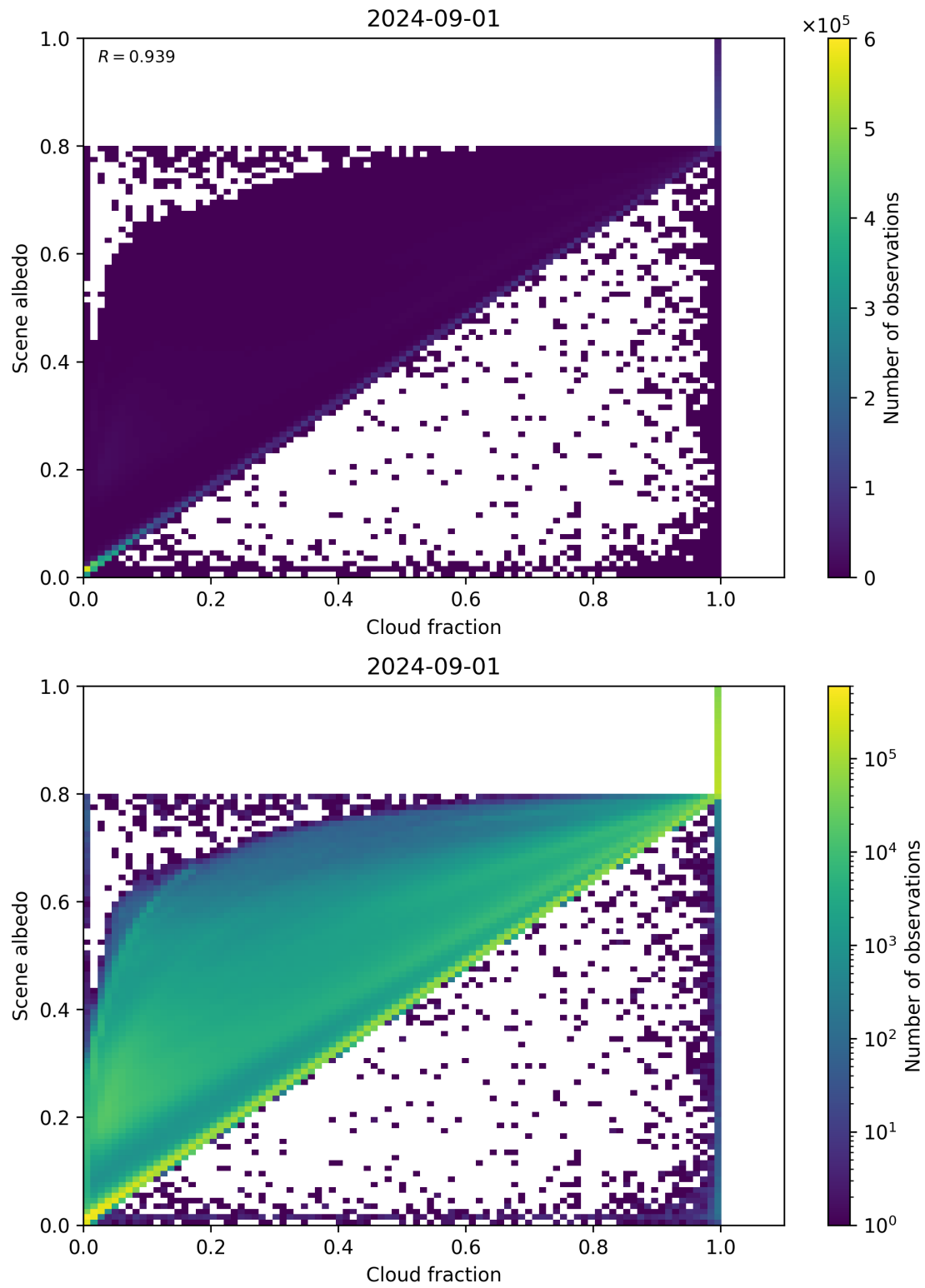
Figure 75: Scatter density plot of “Cloud fraction” against “Scene albedo” for 2024-09-01 to 2024-09-02.
