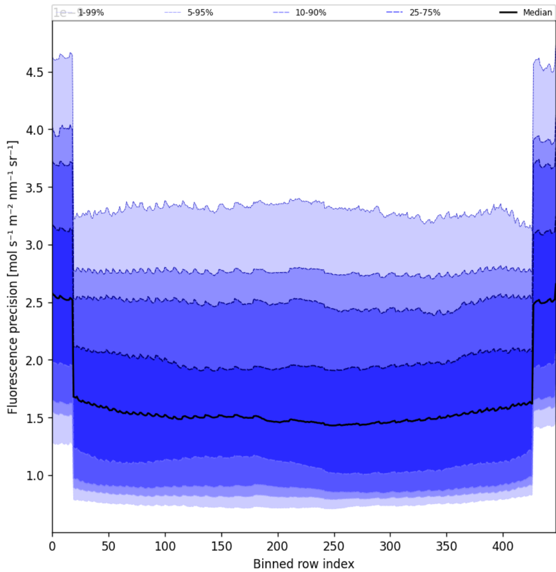
Figure 58: Along track statistics of “Fluorescence precision” for 2024-09-01 to 2024-09-02
