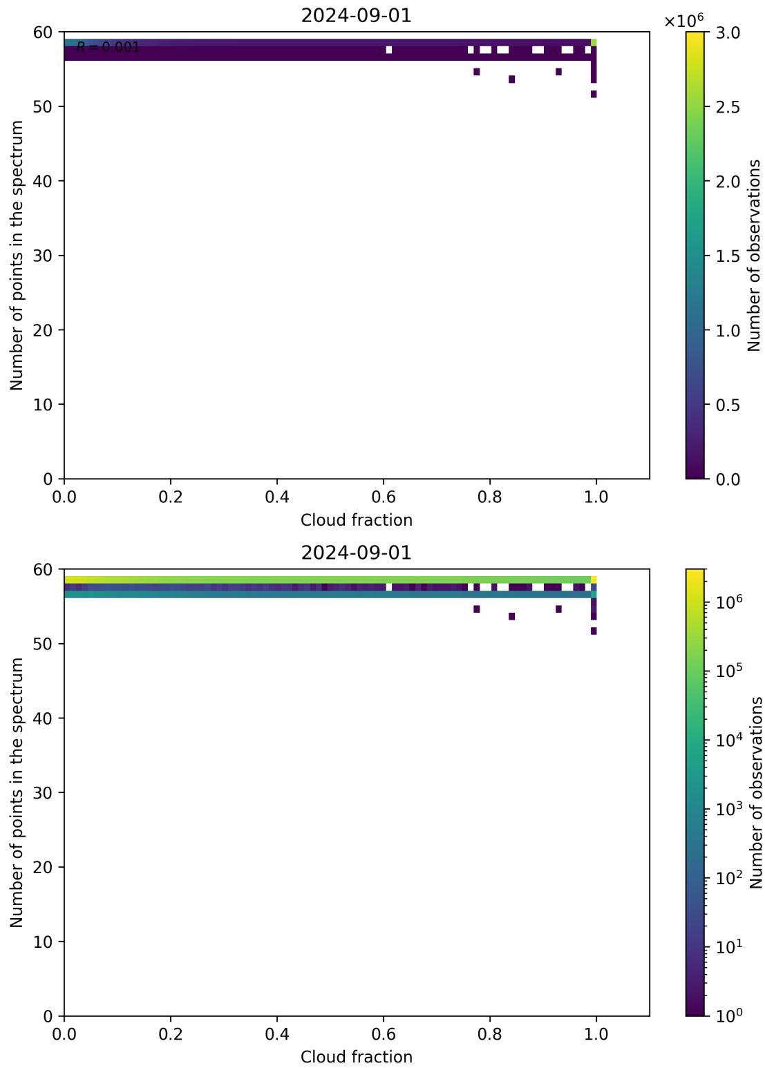
Figure 74: Scatter density plot of “Cloud fraction” against “Number of points in the spectrum” for 2024-09-01 to 2024-09-02.
