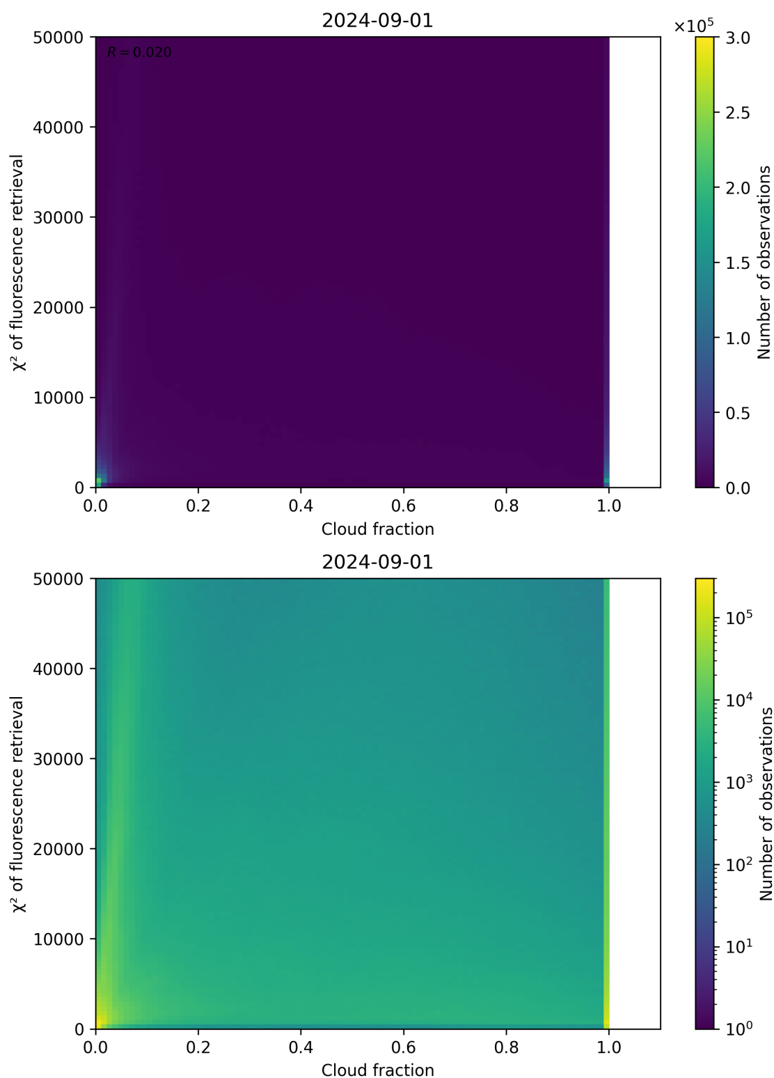
Figure 71: Scatter density plot of “Cloud fraction” against “ \chi^2 of fluorescence retrieval” for 2024-09-01 to 2024-09-02.
