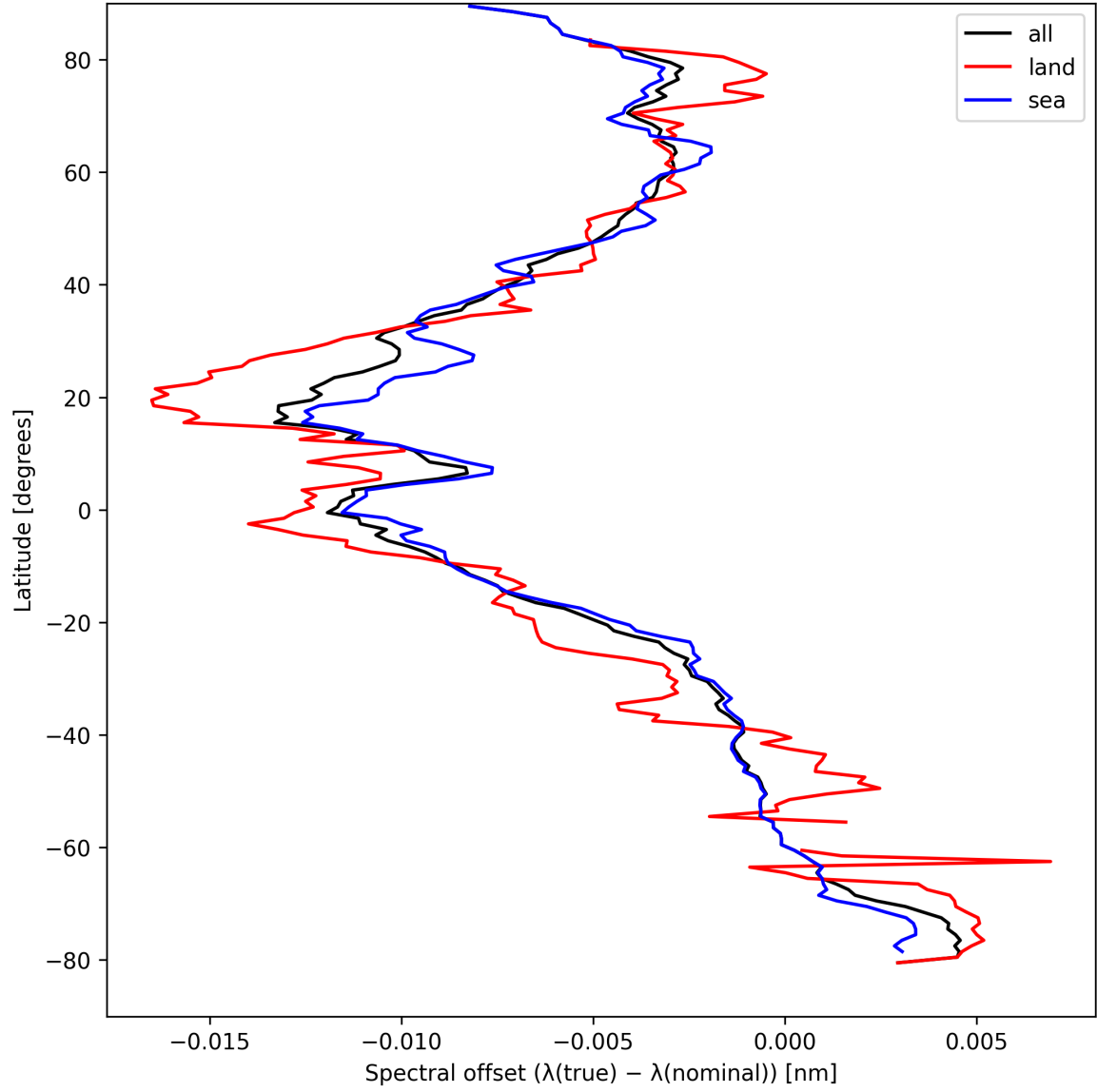
Figure 28: Zonal average of “Spectral offset ( \lambda_{\text{true}} - \lambda_{\text{nominal}} )” for 2024-09-01 to 2024-09-02.
