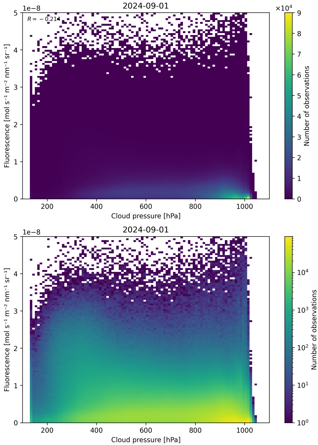
Figure 80: Scatter density plot of “Cloud pressure” against “Fluorescence” for 2024-09-01 to 2024-09-02.
