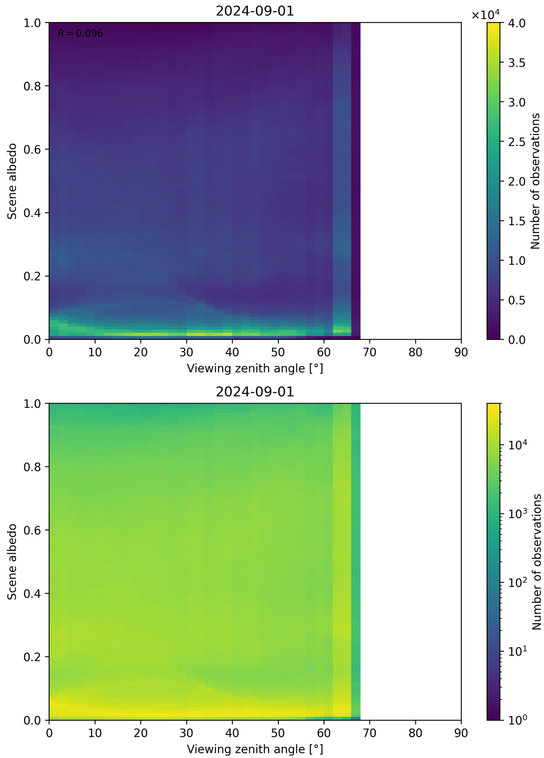
Figure 126: Scatter density plot of “Viewing zenith angle” against “Scene albedo” for 2024-09-01 to 2024-09-02.
