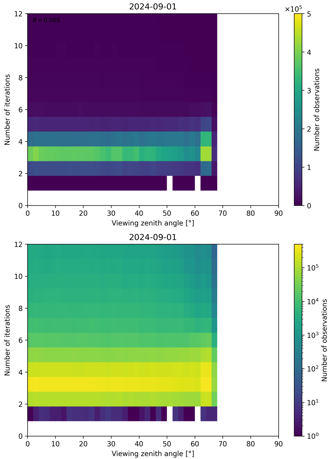
Figure 124: Scatter density plot of “Viewing zenith angle” against “Number of iterations” for 2024-09-01 to 2024-09-02.
