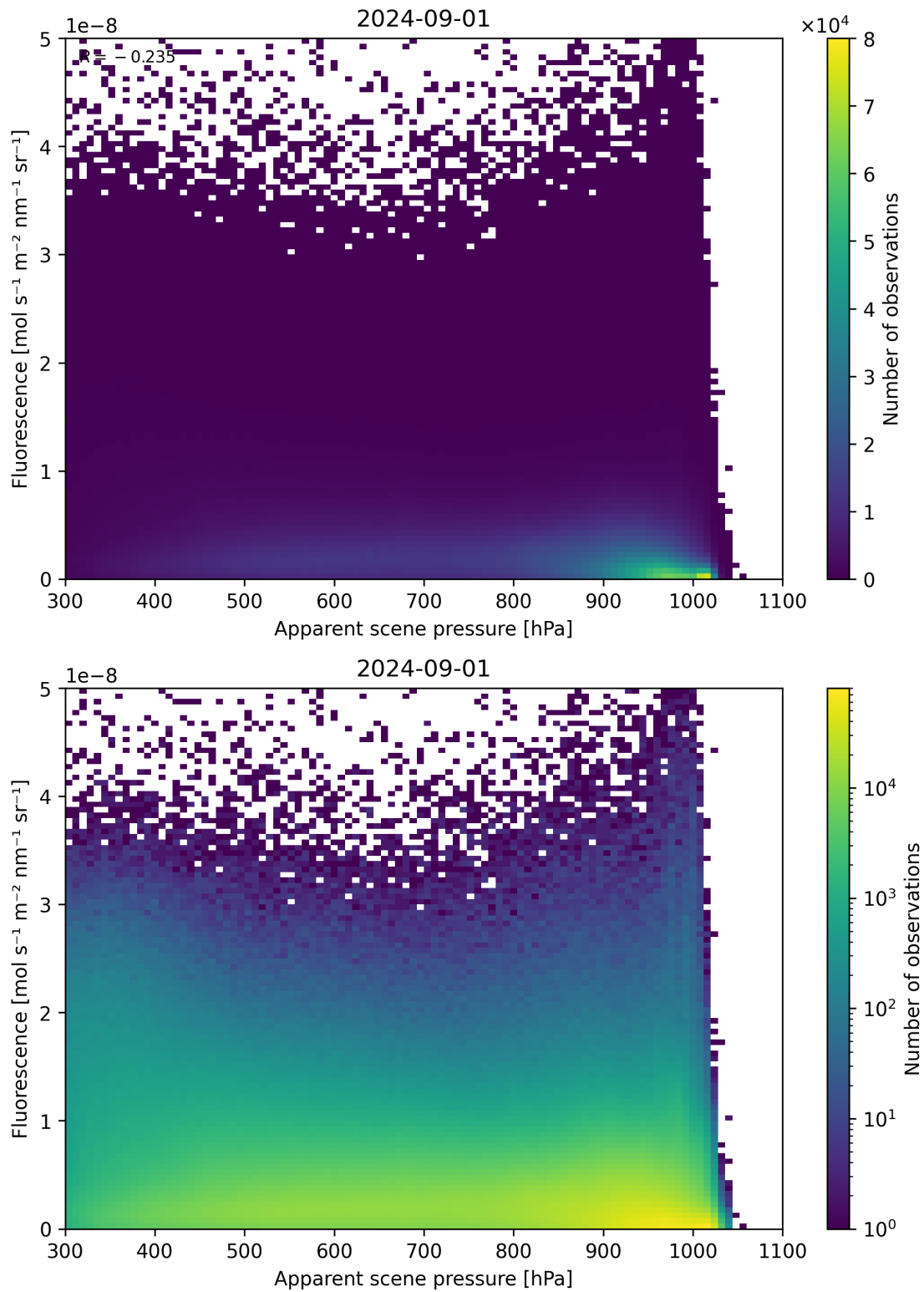
Figure 64: Scatter density plot of “Apparent scene pressure” against “Fluorescence” for 2024-09-01 to 2024-09-02.
