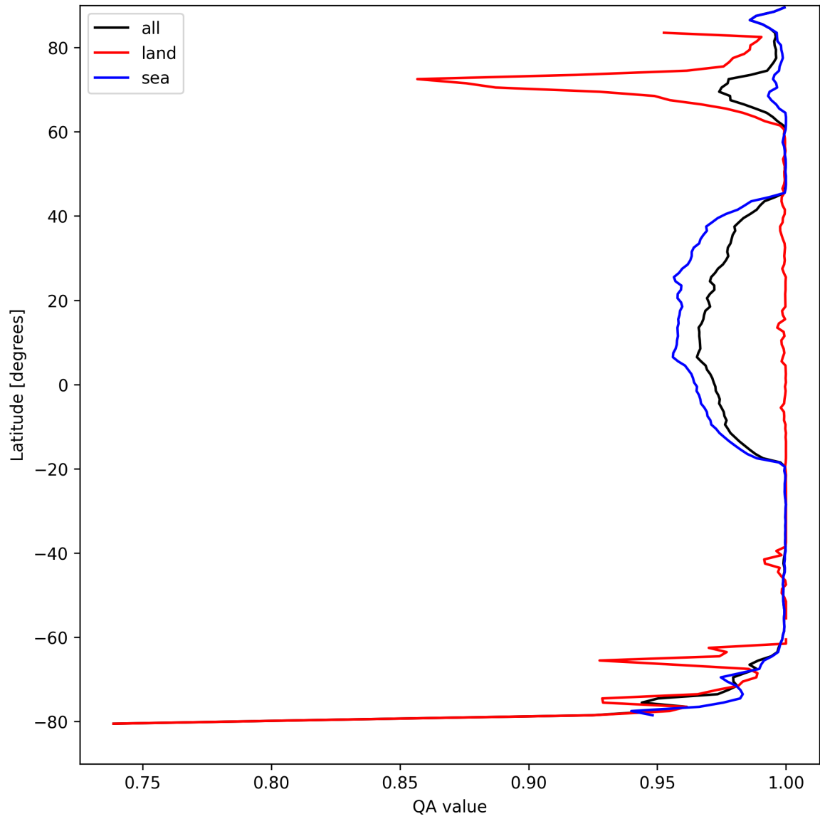
Figure 12: Zonal average of "QA value" for 2024-09-01 to 2024-09-02.
