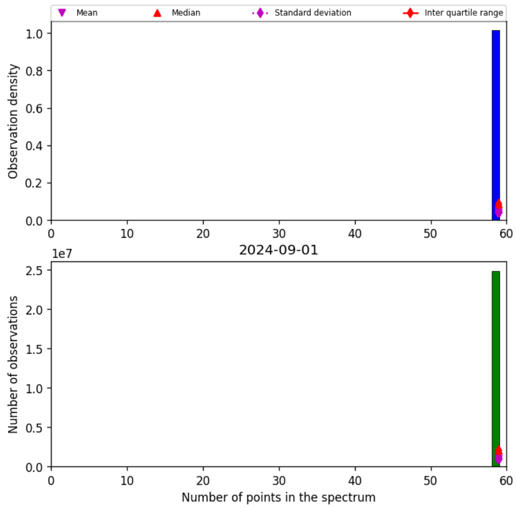
Figure 44: Histogram of “Number of points in the spectrum” for 2024-09-01 to 2024-09-02
