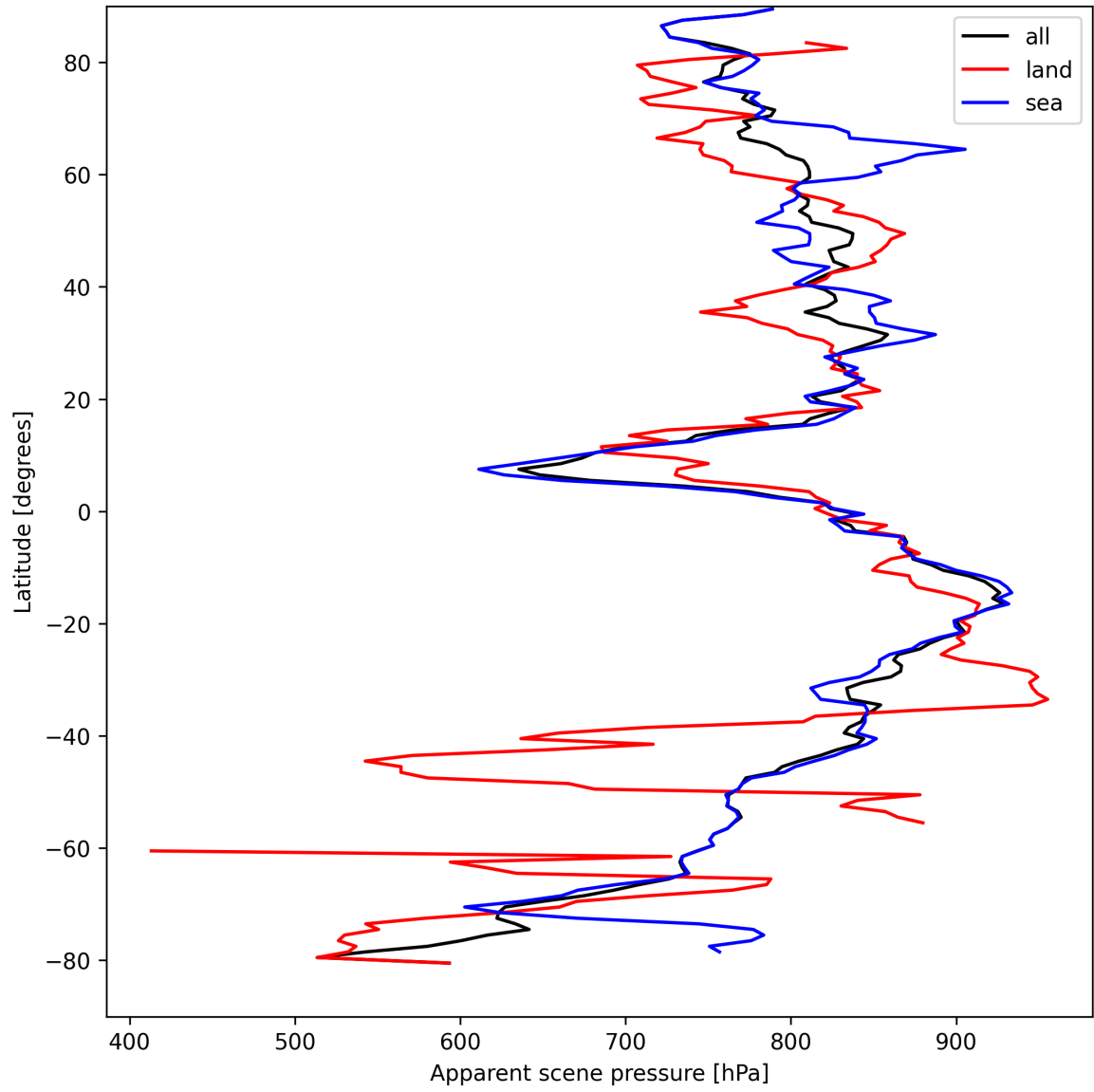
Figure 19: Zonal average of “Apparent scene pressure” for 2024-09-01 to 2024-09-02.
