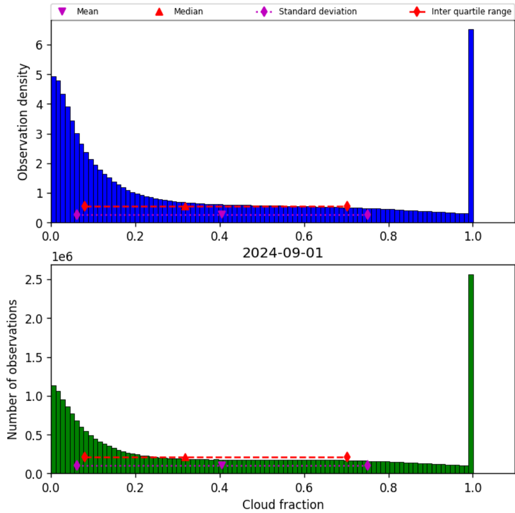
Figure 32: Histogram of “Cloud fraction” for 2024-09-01 to 2024-09-02
