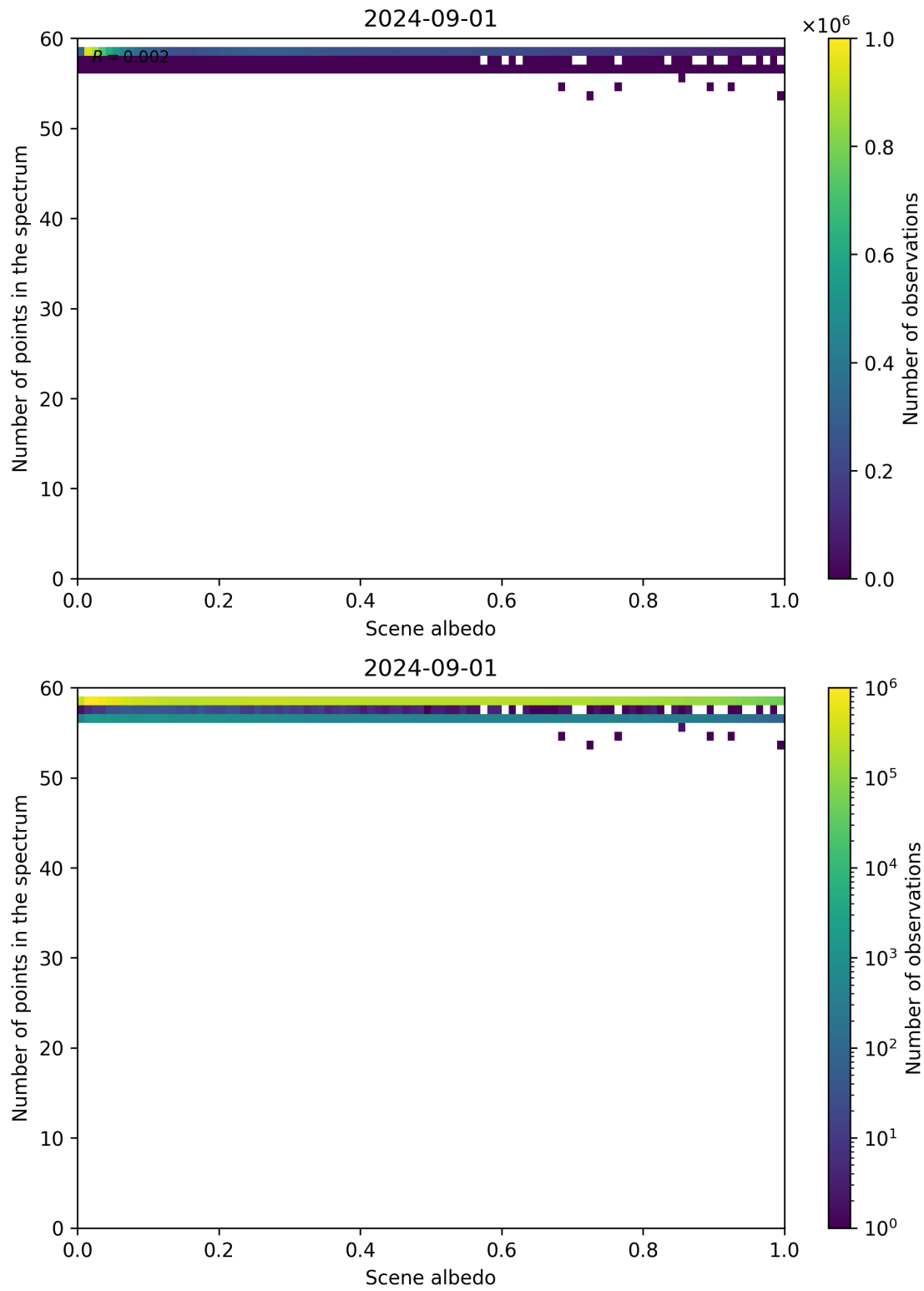
Figure 106: Scatter density plot of “Scene albedo” against “Number of points in the spectrum” for 2024-09-01 to 2024-09-02.
