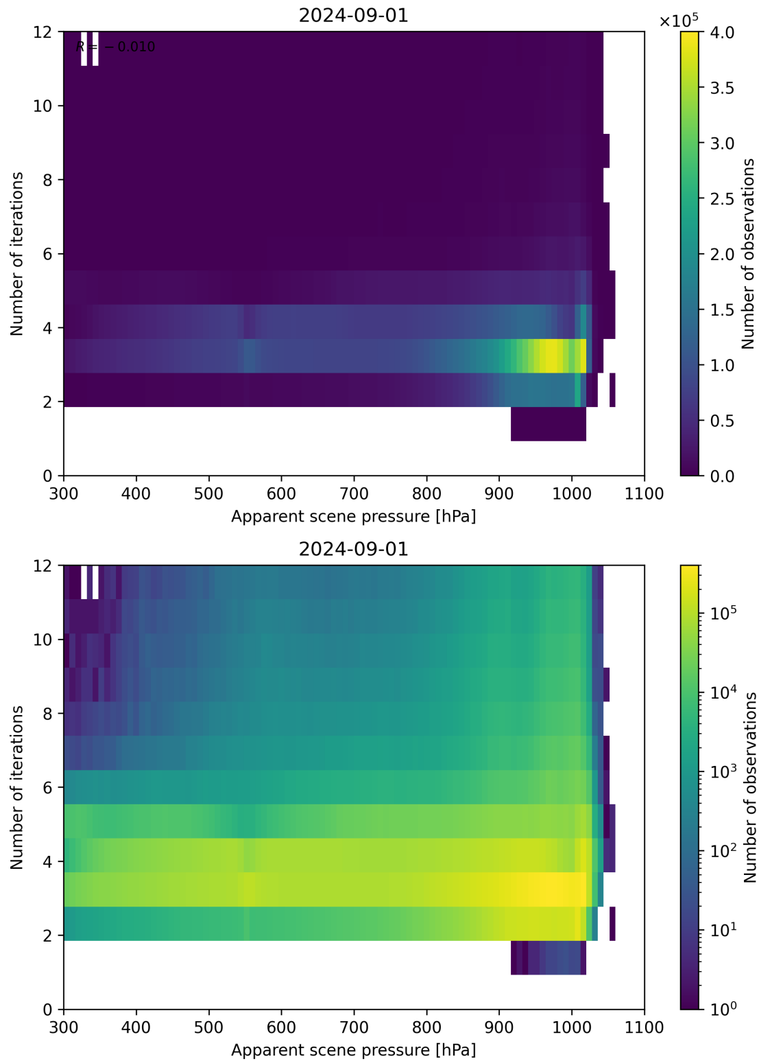
Figure 65: Scatter density plot of “Apparent scene pressure” against “Number of iterations” for 2024-09-01 to 2024-09-02.
