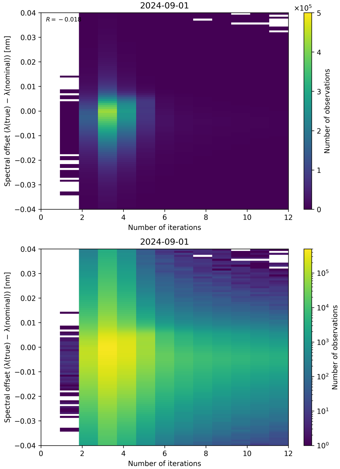
Figure 100: Scatter density plot of “Number of iterations” against “Spectral offset ( \lambda_{\text{true}} - \lambda_{\text{nominal}} )” for 2024-09-01 to 2024-09-02.
