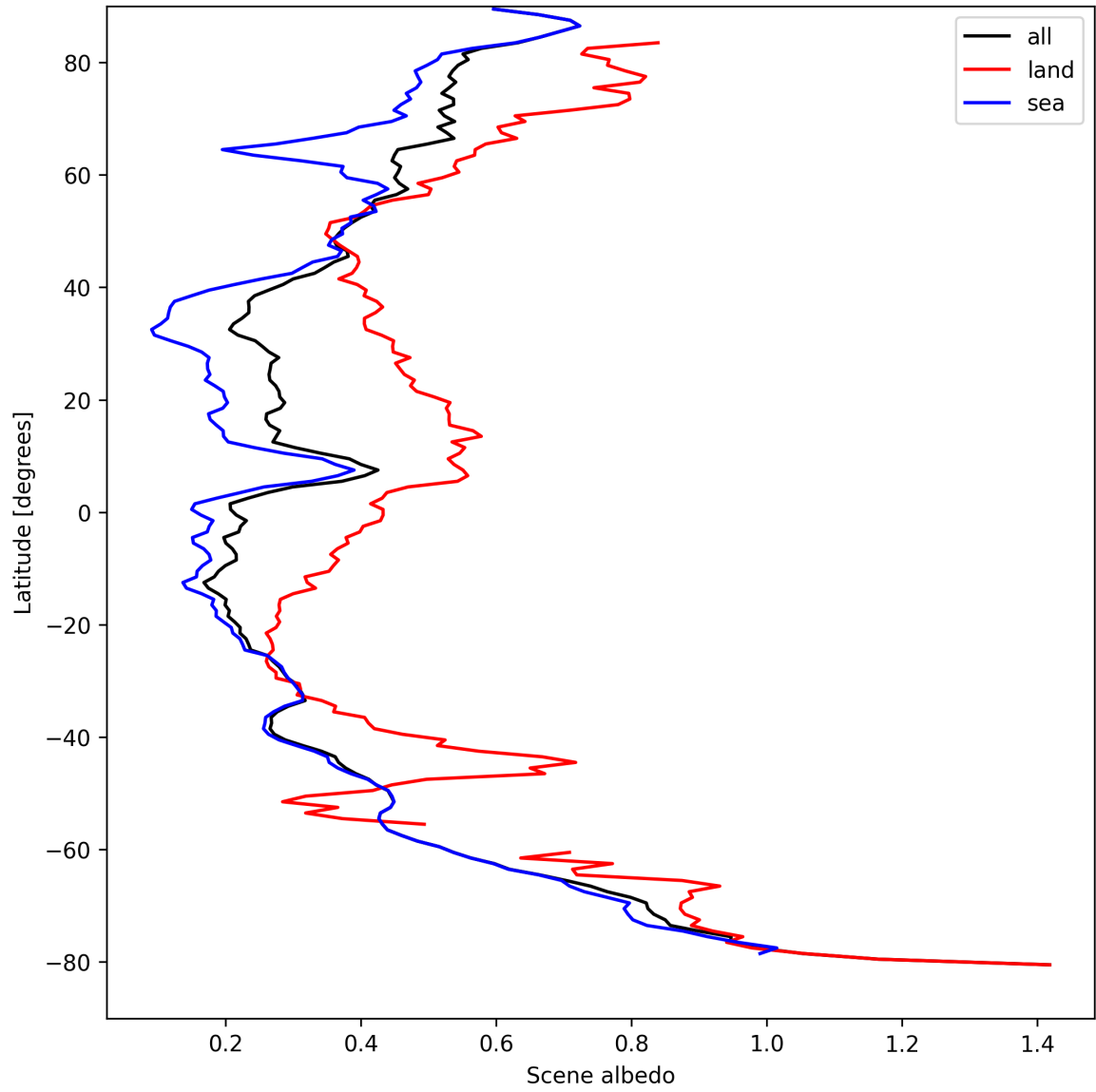
Figure 17: Zonal average of “Scene albedo” for 2024-09-01 to 2024-09-02.
