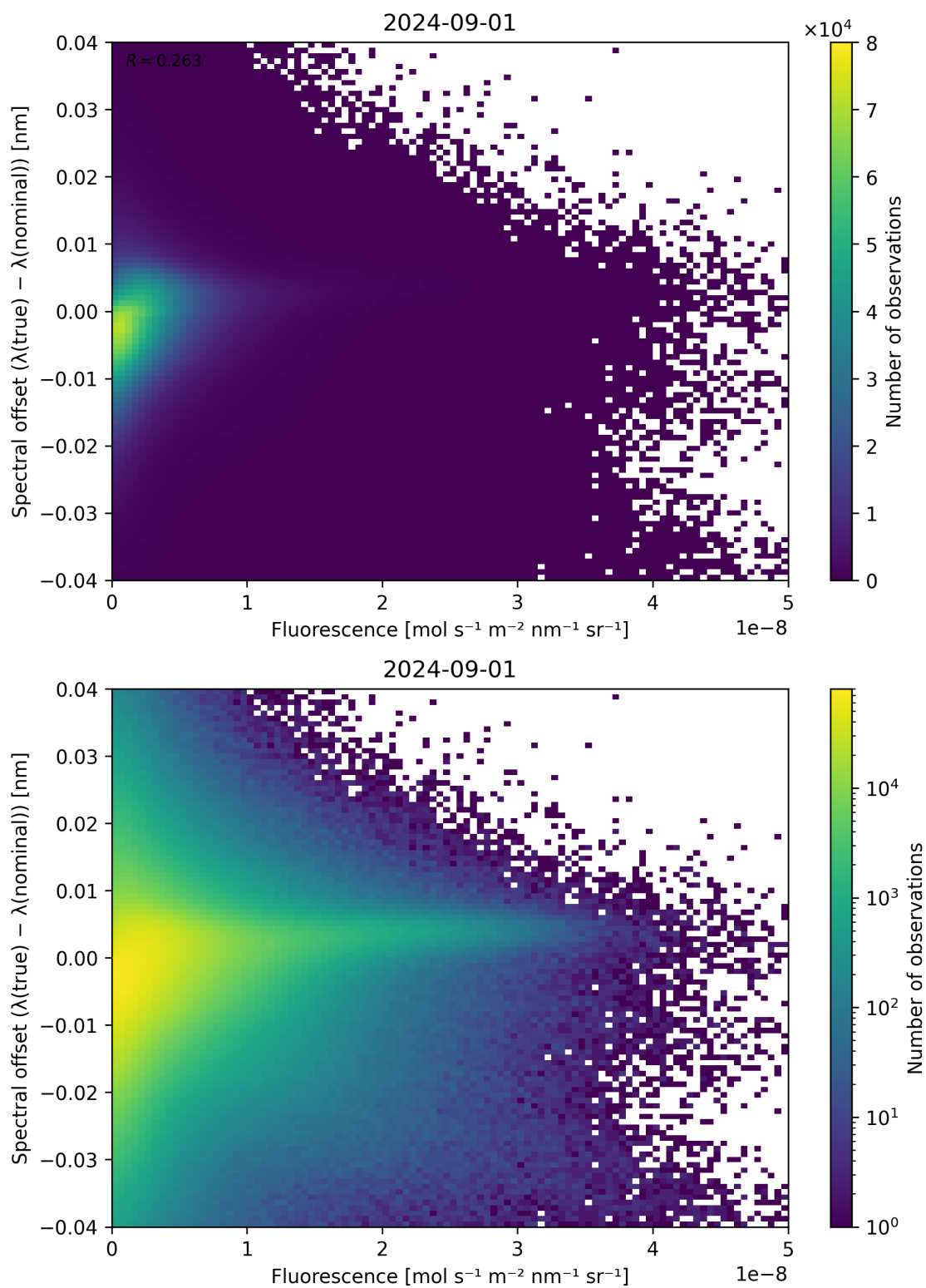
Figure 87: Scatter density plot of “Fluorescence” against “Spectral offset ( \lambda_{\text{true}} - \lambda_{\text{nominal}} )” for 2024-09-01 to 2024-09-02.
