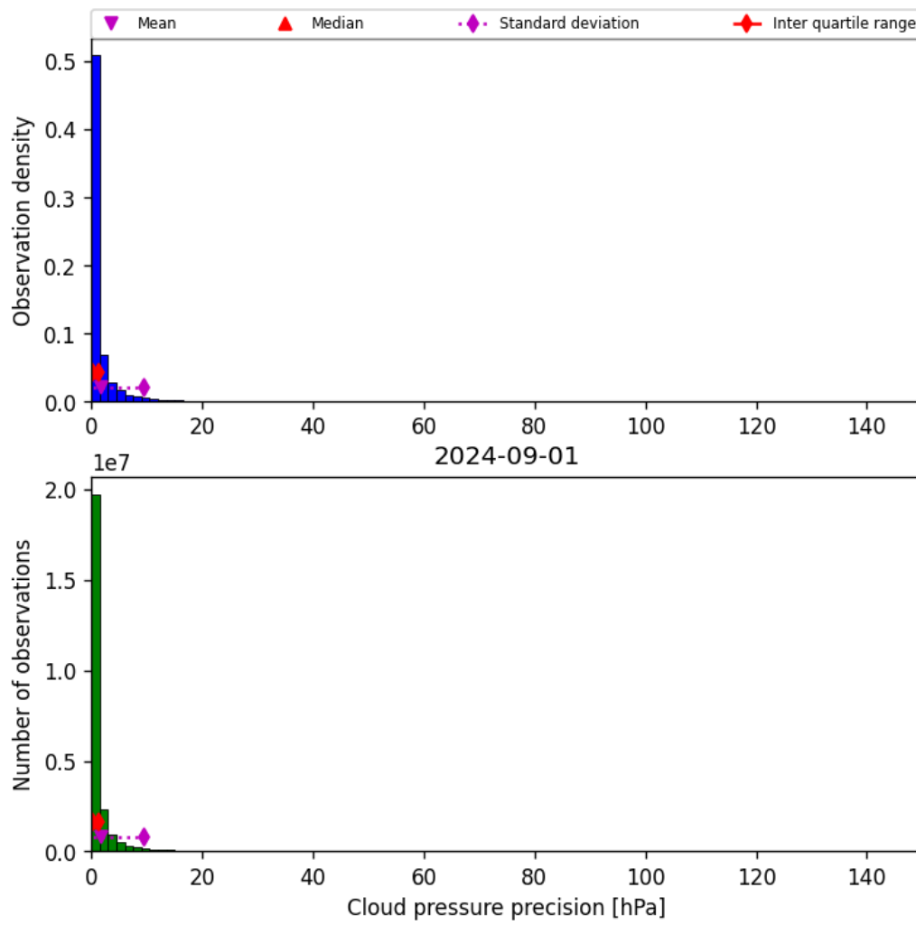
Figure 31: Histogram of “Cloud pressure precision” for 2024-09-01 to 2024-09-02
