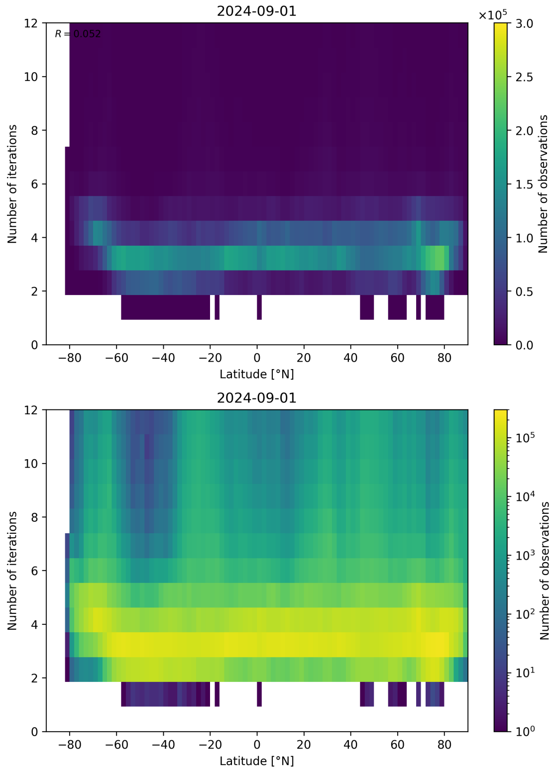
Figure 93: Scatter density plot of “Latitude” against “Number of iterations” for 2024-09-01 to 2024-09-02.
