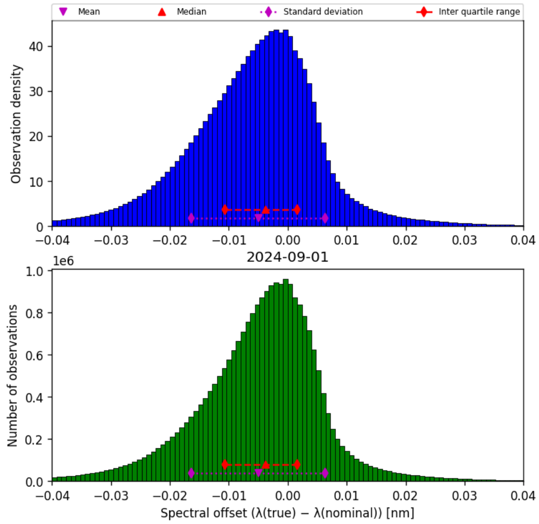
Figure 45: Histogram of “Spectral offset ( \lambda_{\text{true}} - \lambda_{\text{nominal}} )” for 2024-09-01 to 2024-09-02
