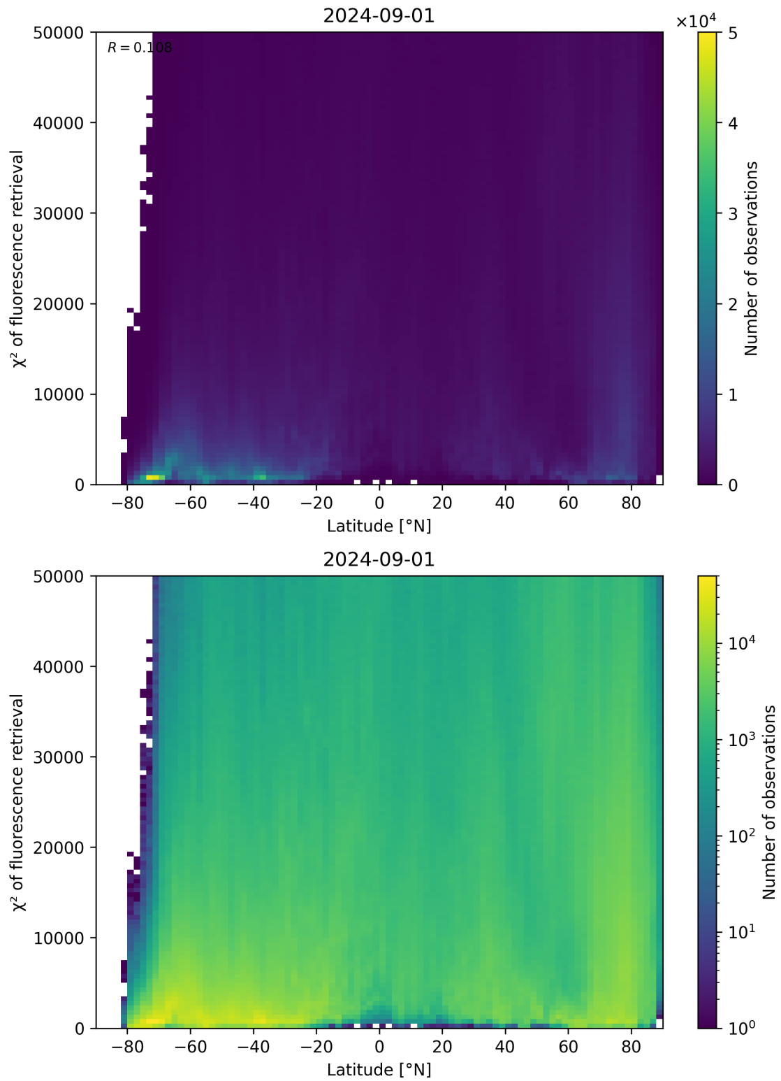
Figure 89: Scatter density plot of “Latitude” against “ \chi^2 of fluorescence retrieval” for 2024-09-01 to 2024-09-02.
