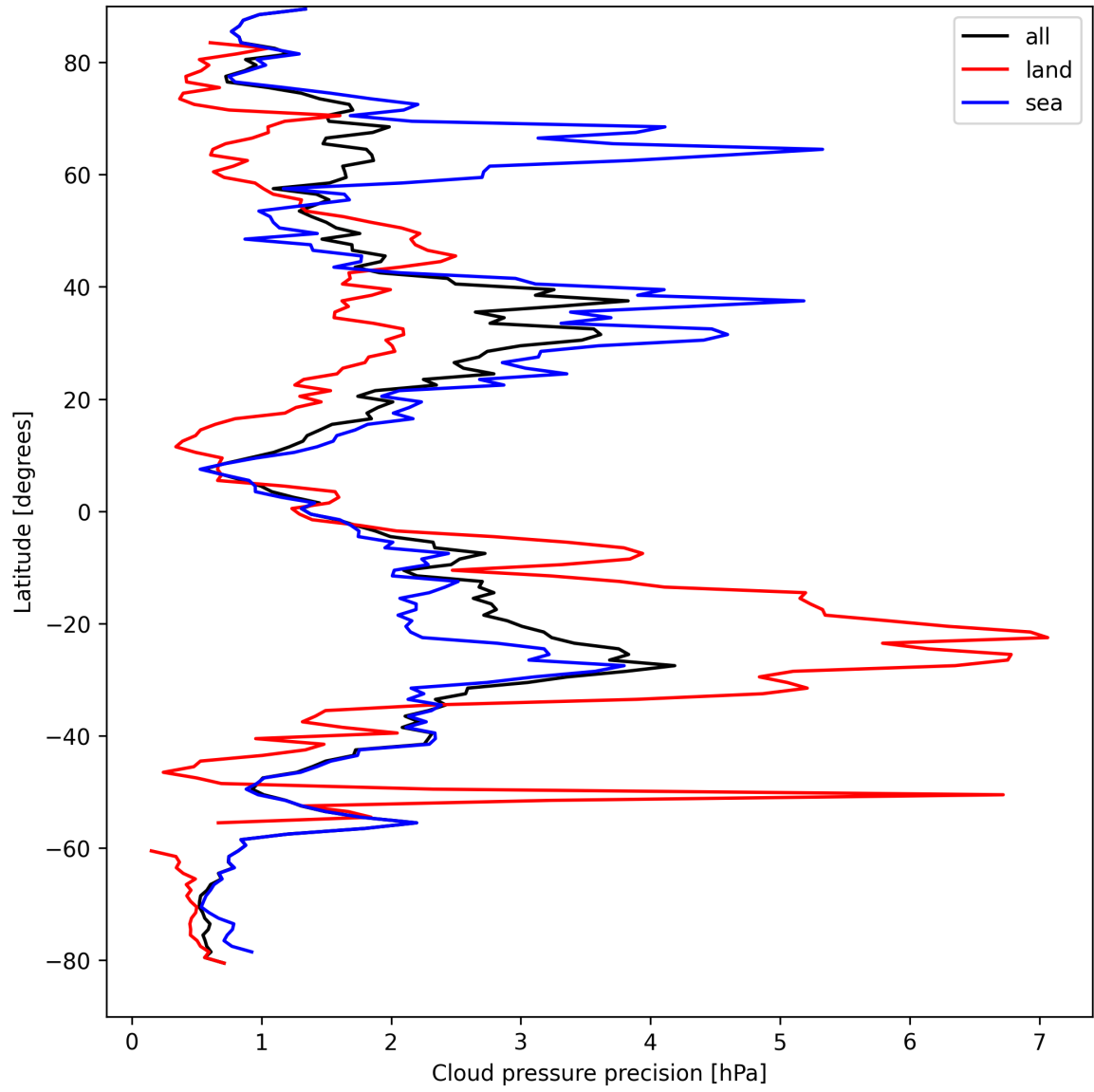
Figure 14: Zonal average of “Cloud pressure precision” for 2024-09-01 to 2024-09-02.
