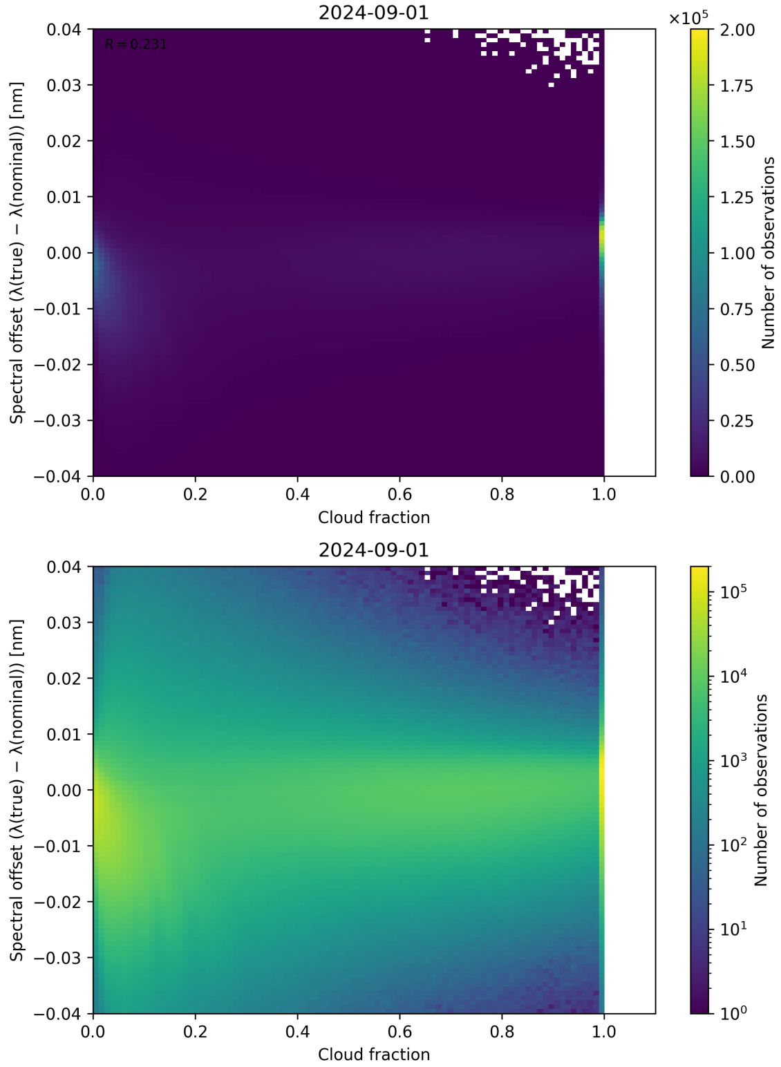
Figure 76: Scatter density plot of “Cloud fraction” against “Spectral offset ( \lambda_{\text{true}} - \lambda_{\text{nominal}} )” for 2024-09-01 to 2024-09-02.
