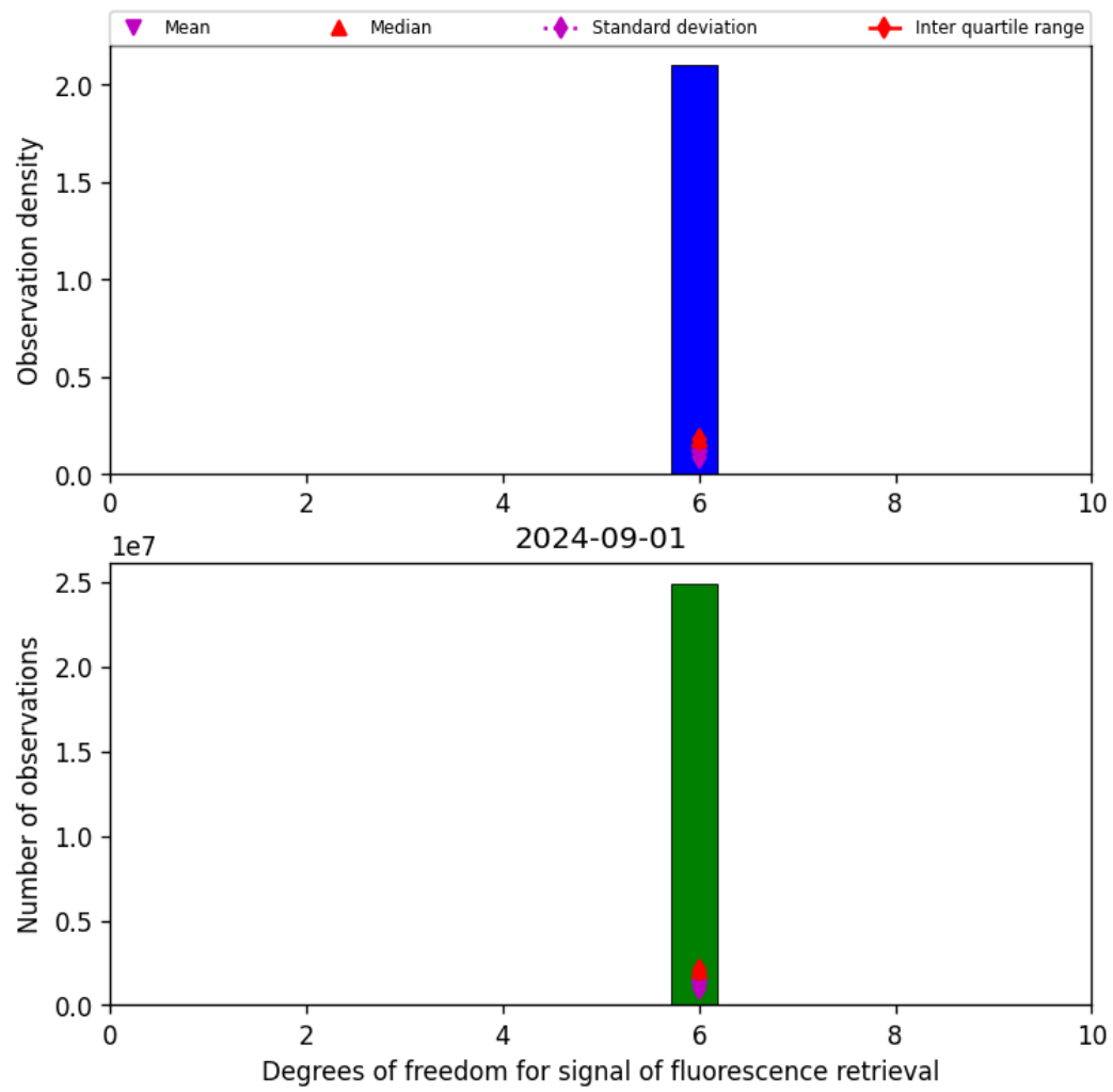
Figure 43: Histogram of “Degrees of freedom for signal of fluorescence retrieval” for 2024-09-01 to 2024-09-02
