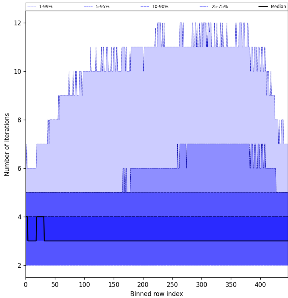
Figure 56: Along track statistics of “Number of iterations” for 2024-09-01 to 2024-09-02
