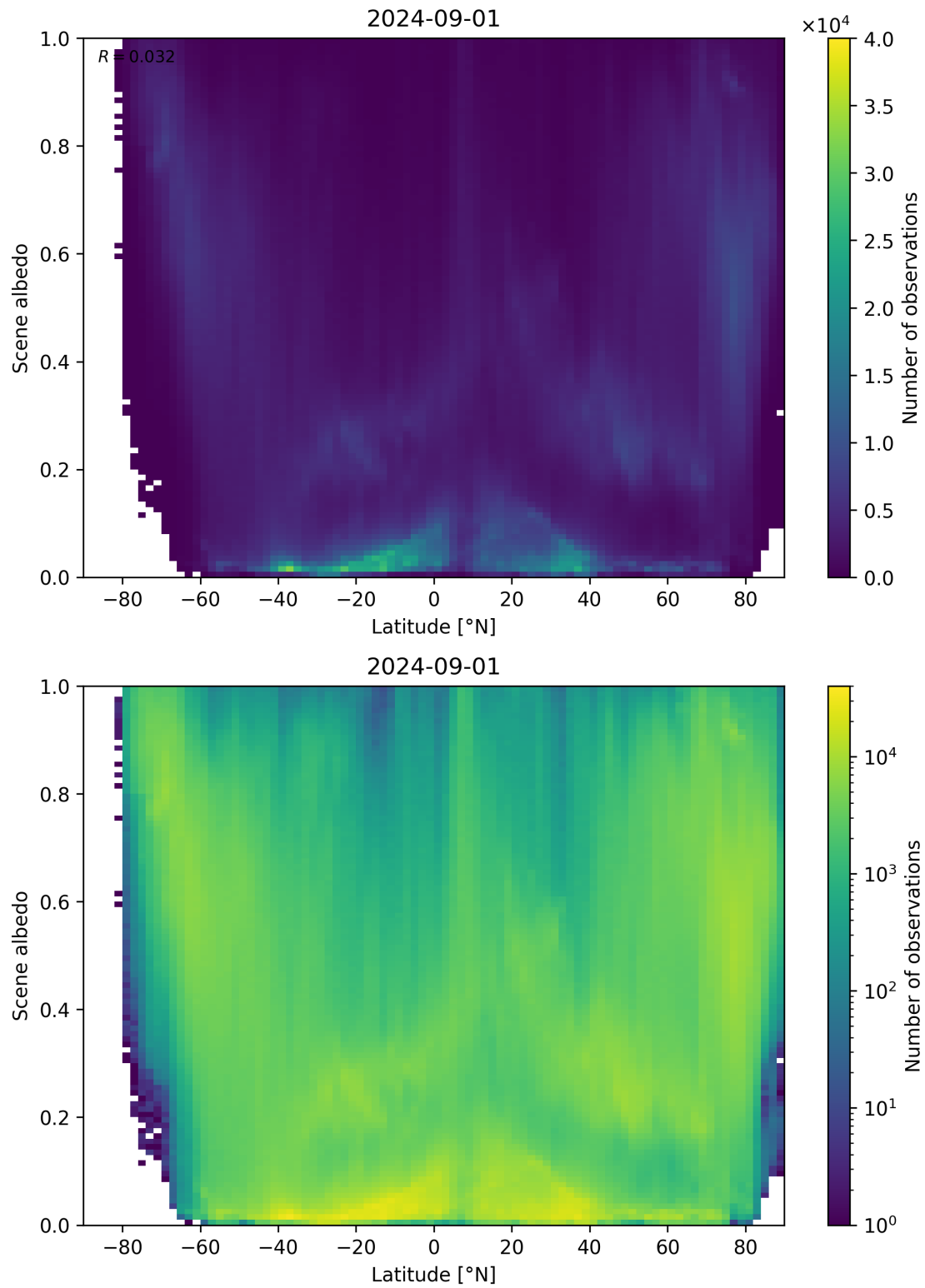
Figure 95: Scatter density plot of “Latitude” against “Scene albedo” for 2024-09-01 to 2024-09-02.
