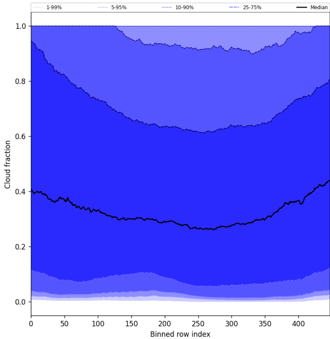
Figure 49: Along track statistics of “Cloud fraction” for 2024-09-01 to 2024-09-02
