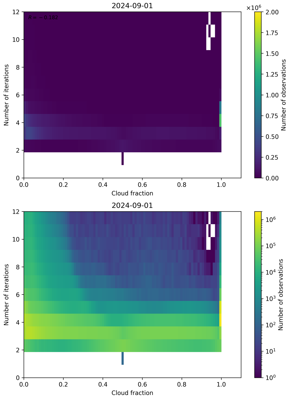
Figure 73: Scatter density plot of “Cloud fraction” against “Number of iterations” for 2024-09-01 to 2024-09-02.
