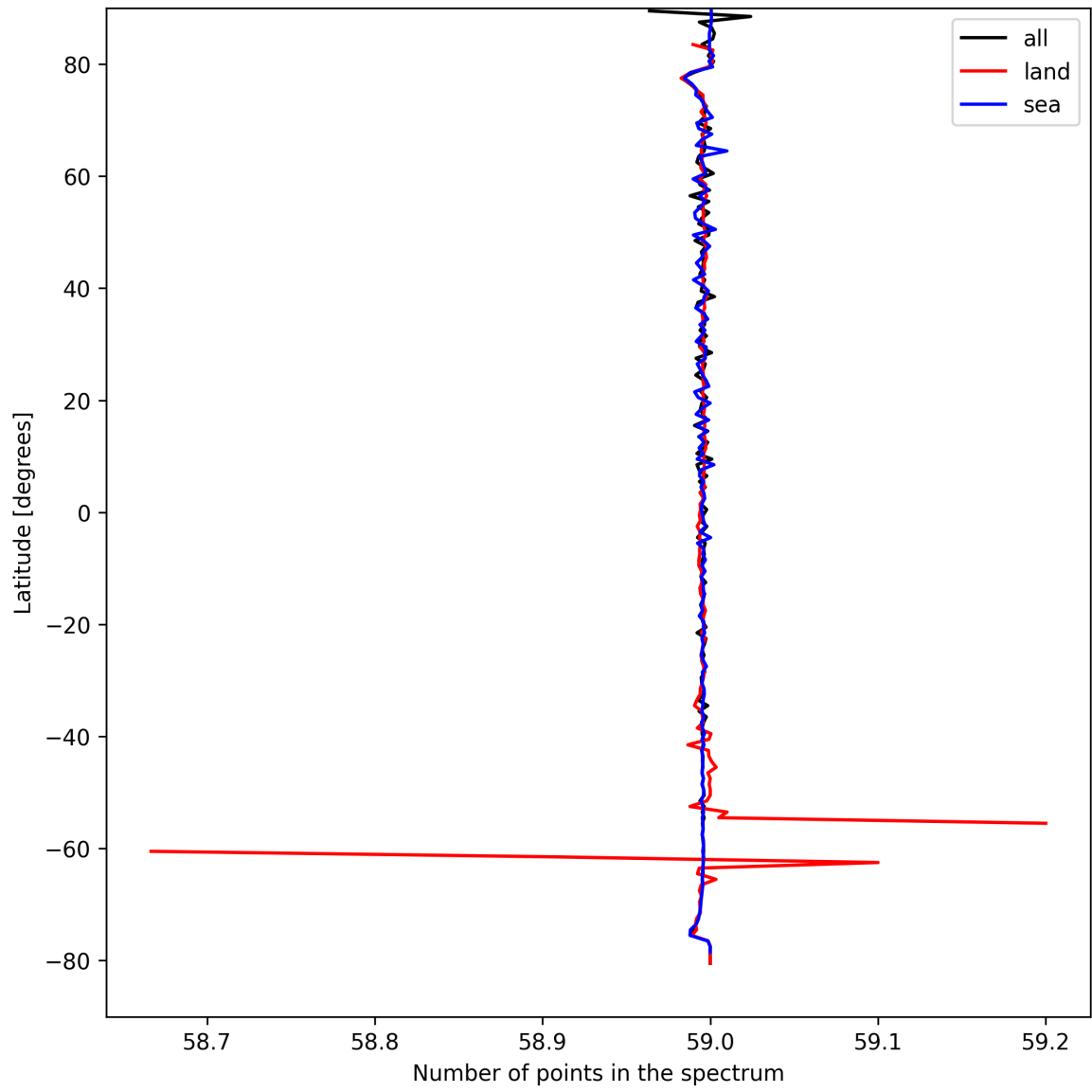
Figure 27: Zonal average of “Number of points in the spectrum” for 2024-09-01 to 2024-09-02.
