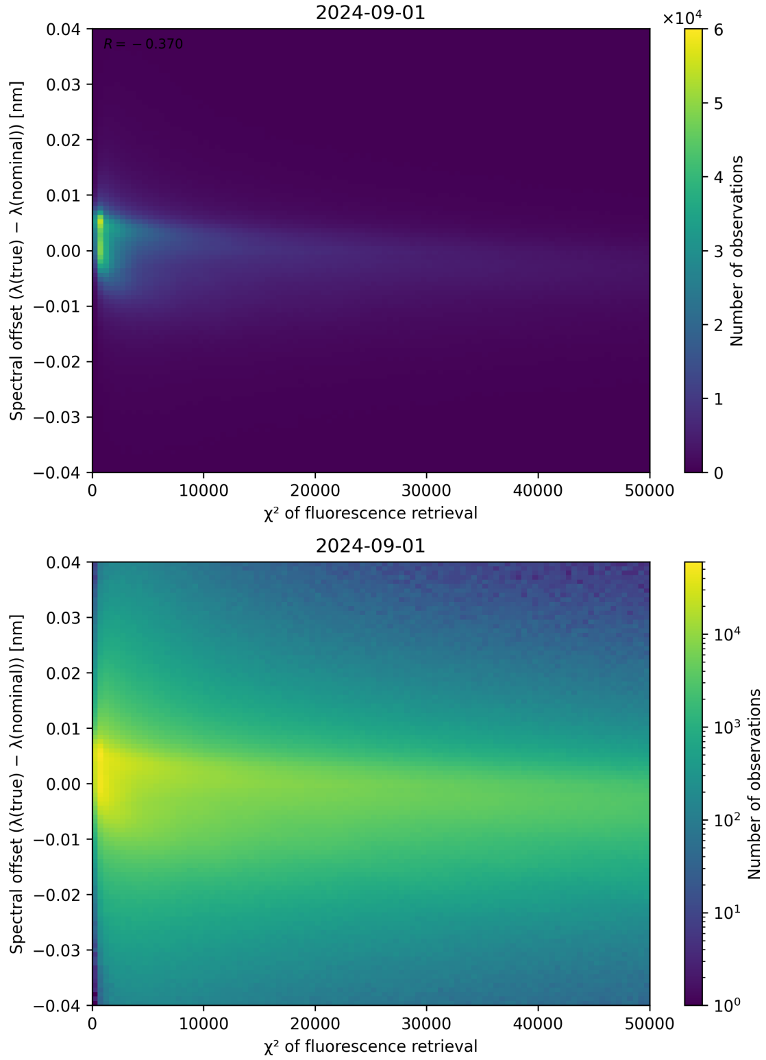
Figure 69: Scatter density plot of “ \chi^2 of fluorescence retrieval” against “Spectral offset ( \lambda_{\text{true}} - \lambda_{\text{nominal}} )” for 2024-09-01 to 2024-09-02.
