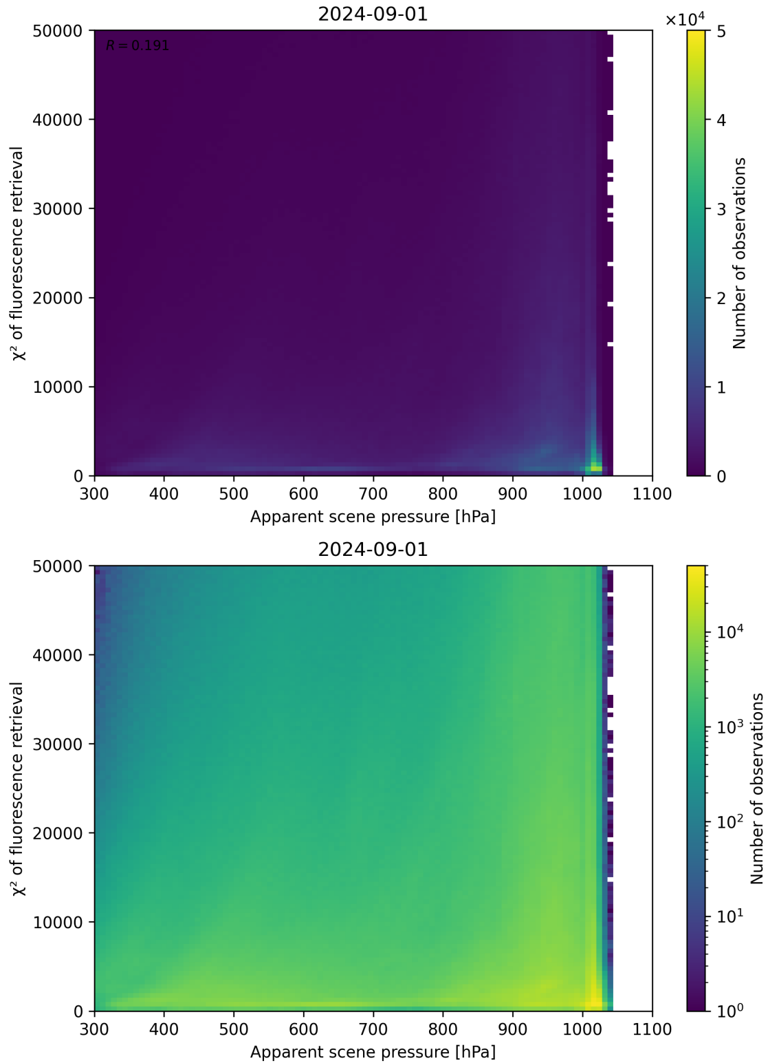
Figure 63: Scatter density plot of “Apparent scene pressure” against “ \chi^2 of fluorescence retrieval” for 2024-09-01 to 2024-09-02.
