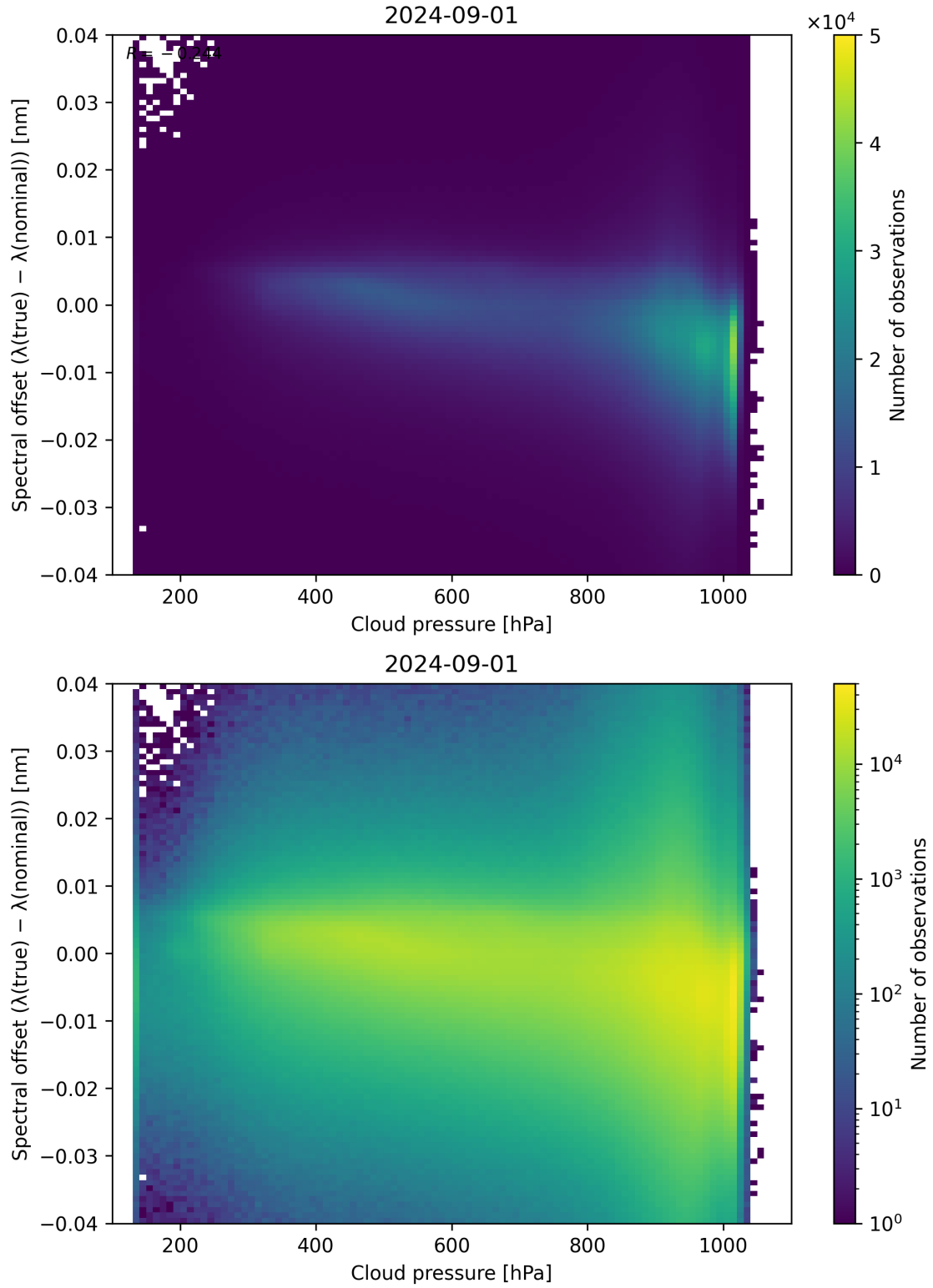
Figure 84: Scatter density plot of “Cloud pressure” against “Spectral offset ( \lambda_{\text{true}} - \lambda_{\text{nominal}} )” for 2024-09-01 to 2024-09-02.
