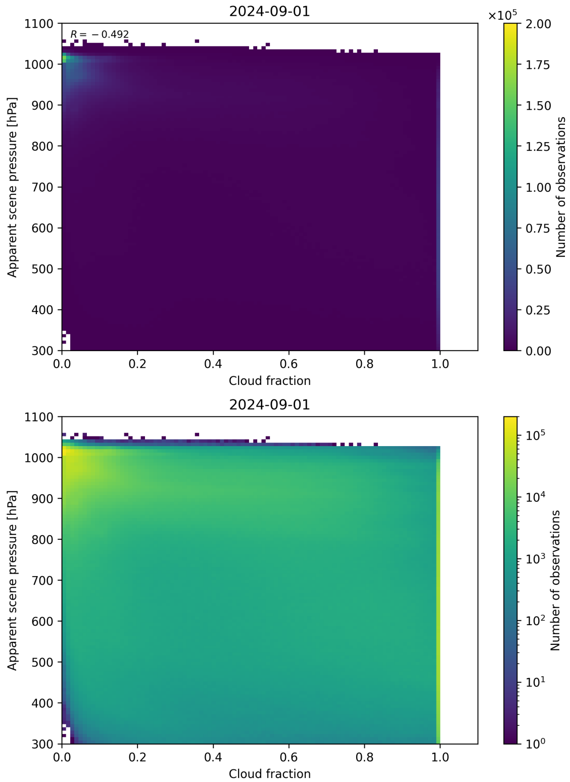
Figure 70: Scatter density plot of “Cloud fraction” against “Apparent scene pressure” for 2024-09-01 to 2024-09-02.
