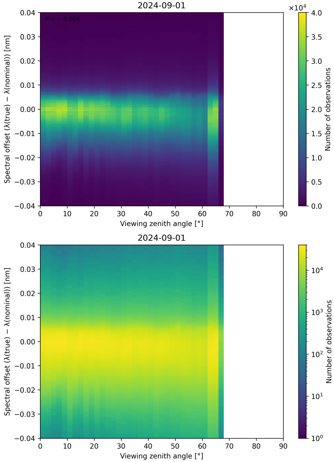
Figure 128: Scatter density plot of “Viewing zenith angle” against “Spectral offset ( \lambda_{\text{true}} - \lambda_{\text{nominal}} )” for 2024-09-01 to 2024-09-02.
