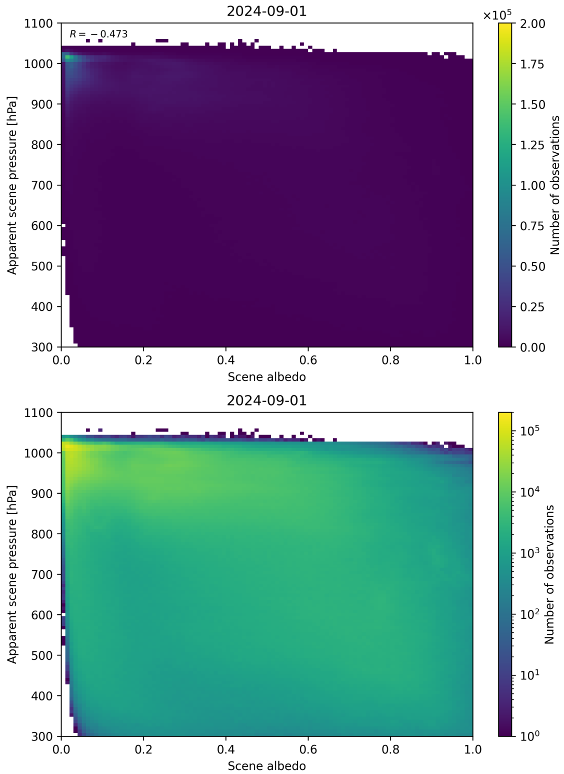
Figure 102: Scatter density plot of “Scene albedo” against “Apparent scene pressure” for 2024-09-01 to 2024-09-02.
