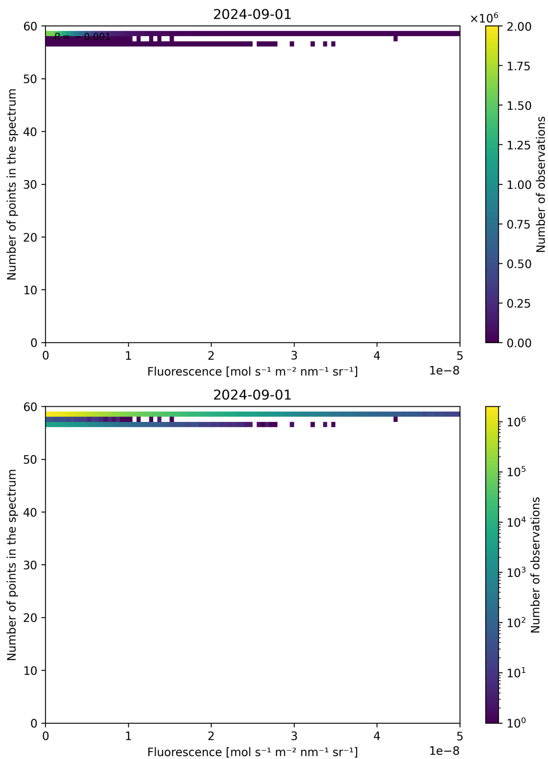
Figure 86: Scatter density plot of “Fluorescence” against “Number of points in the spectrum” for 2024-09-01 to 2024-09-02.
