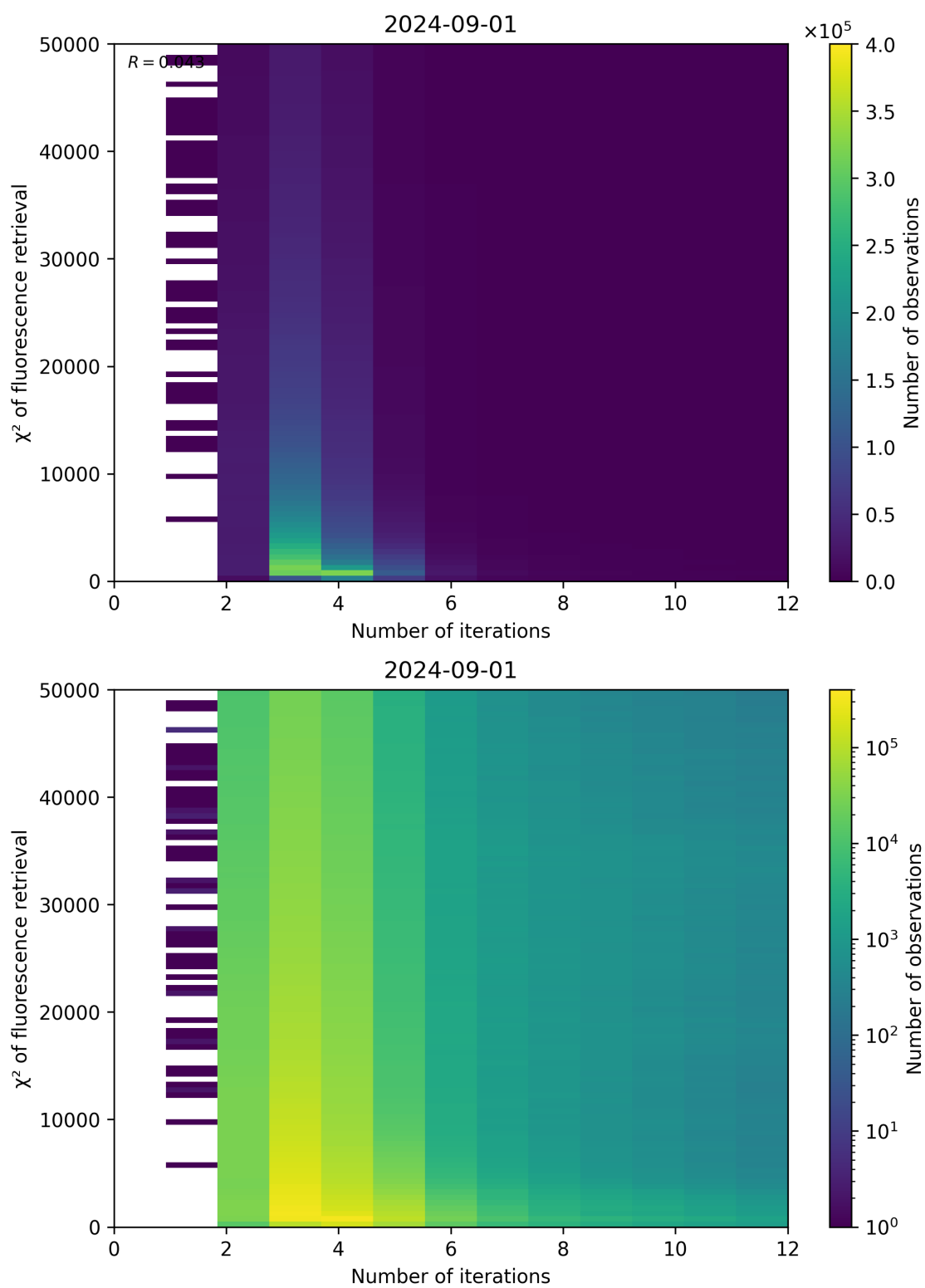
Figure 97: Scatter density plot of “Number of iterations” against “ \chi^2 of fluorescence retrieval” for 2024-09-01 to 2024-09-02.
