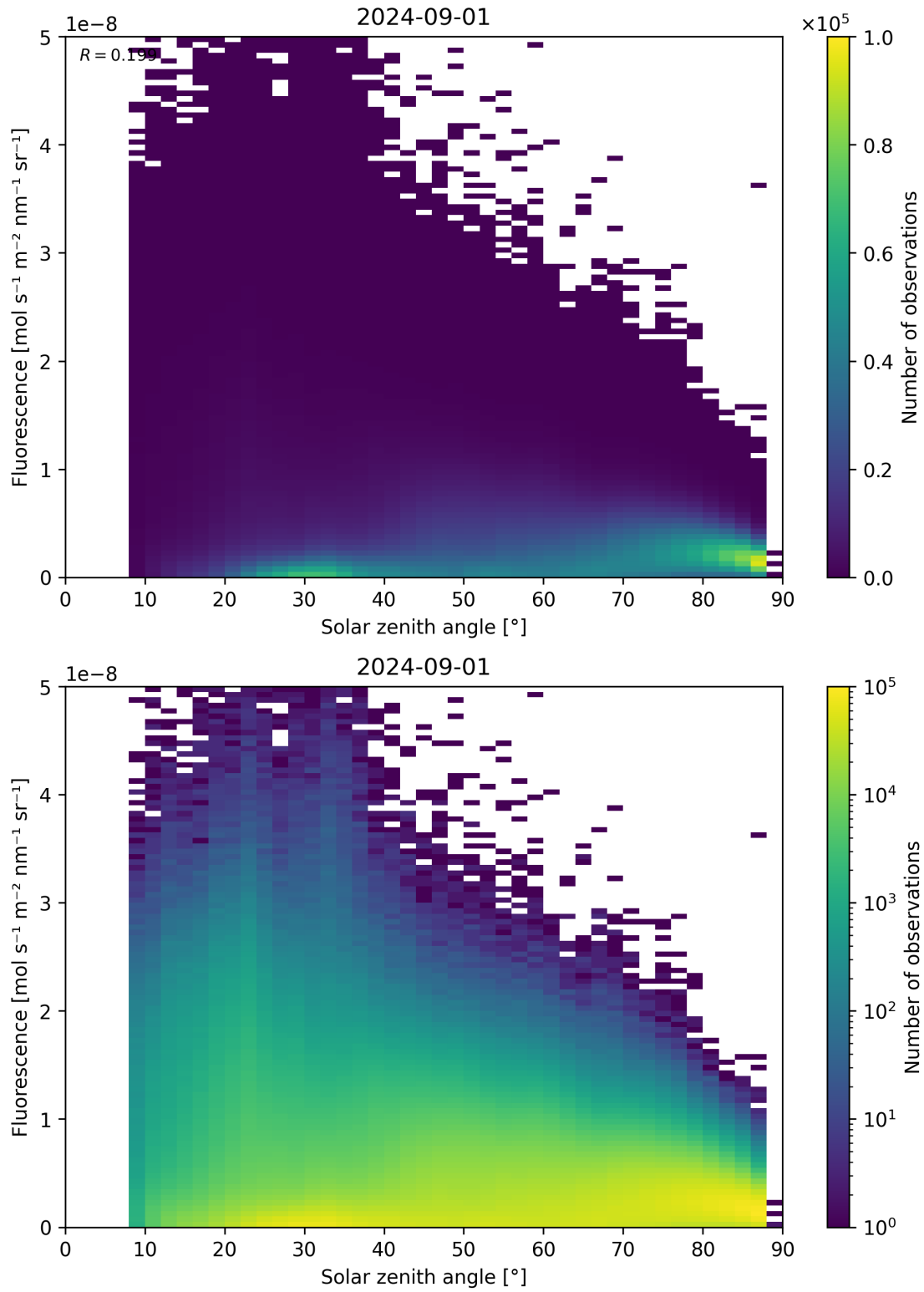
Figure 112: Scatter density plot of “Solar zenith angle” against “Fluorescence” for 2024-09-01 to 2024-09-02.
