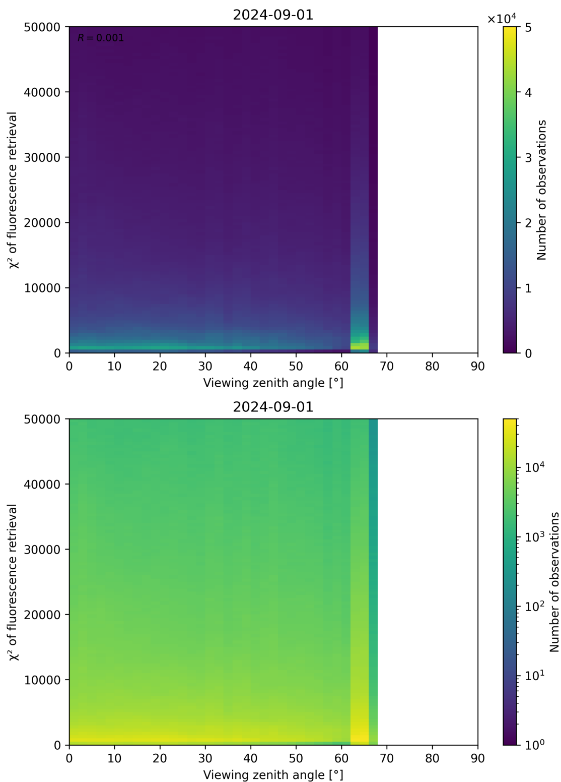
Figure 119: Scatter density plot of “Viewing zenith angle” against “ \chi^2 of fluorescence retrieval” for 2024-09-01 to 2024-09-02.
