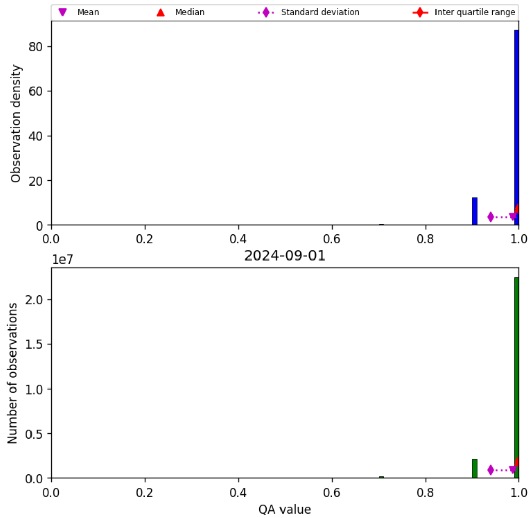
Figure 29: Histogram of “QA value” for 2024-09-01 to 2024-09-02
