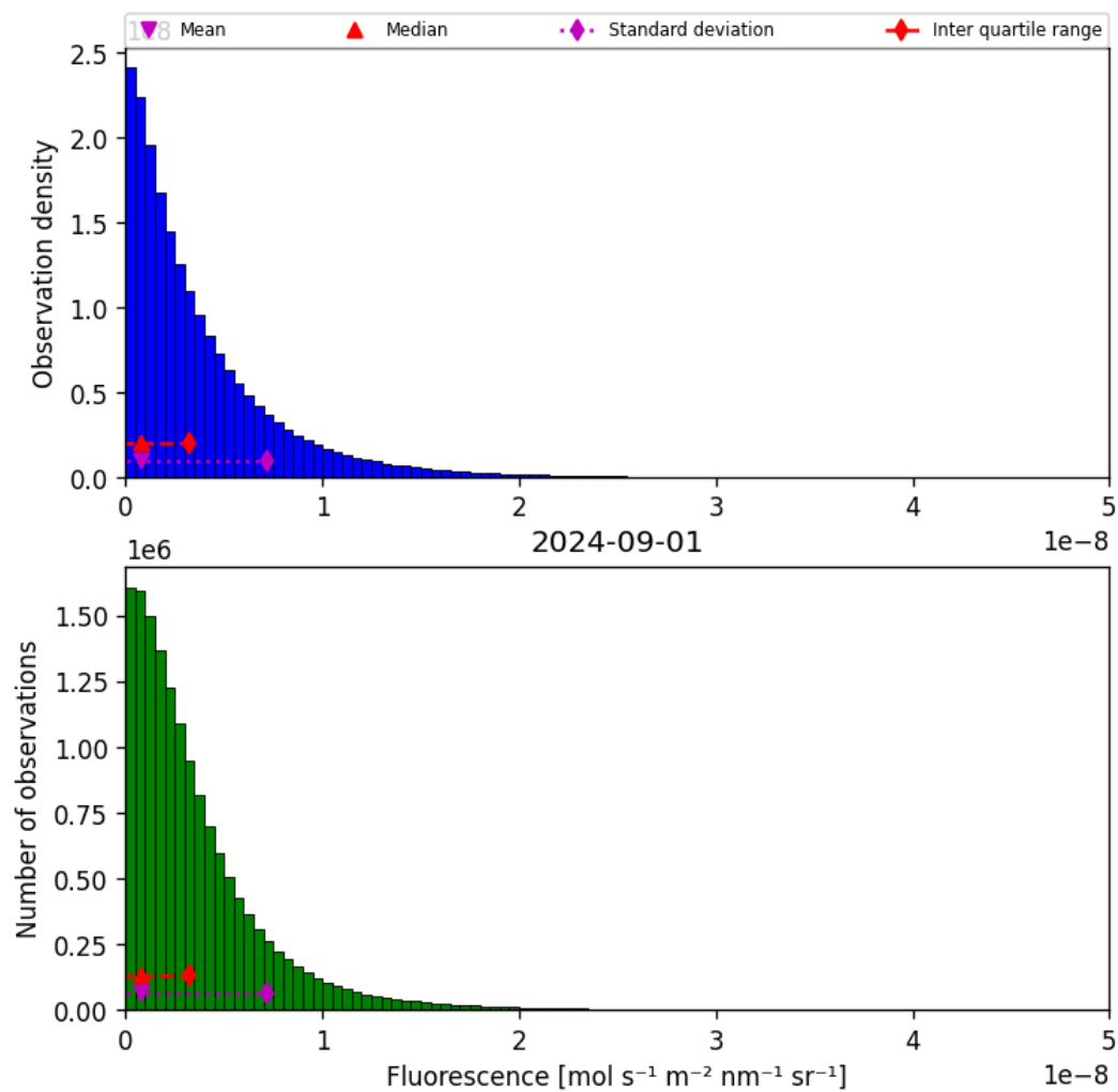
Figure 40: Histogram of “Fluorescence” for 2024-09-01 to 2024-09-02
