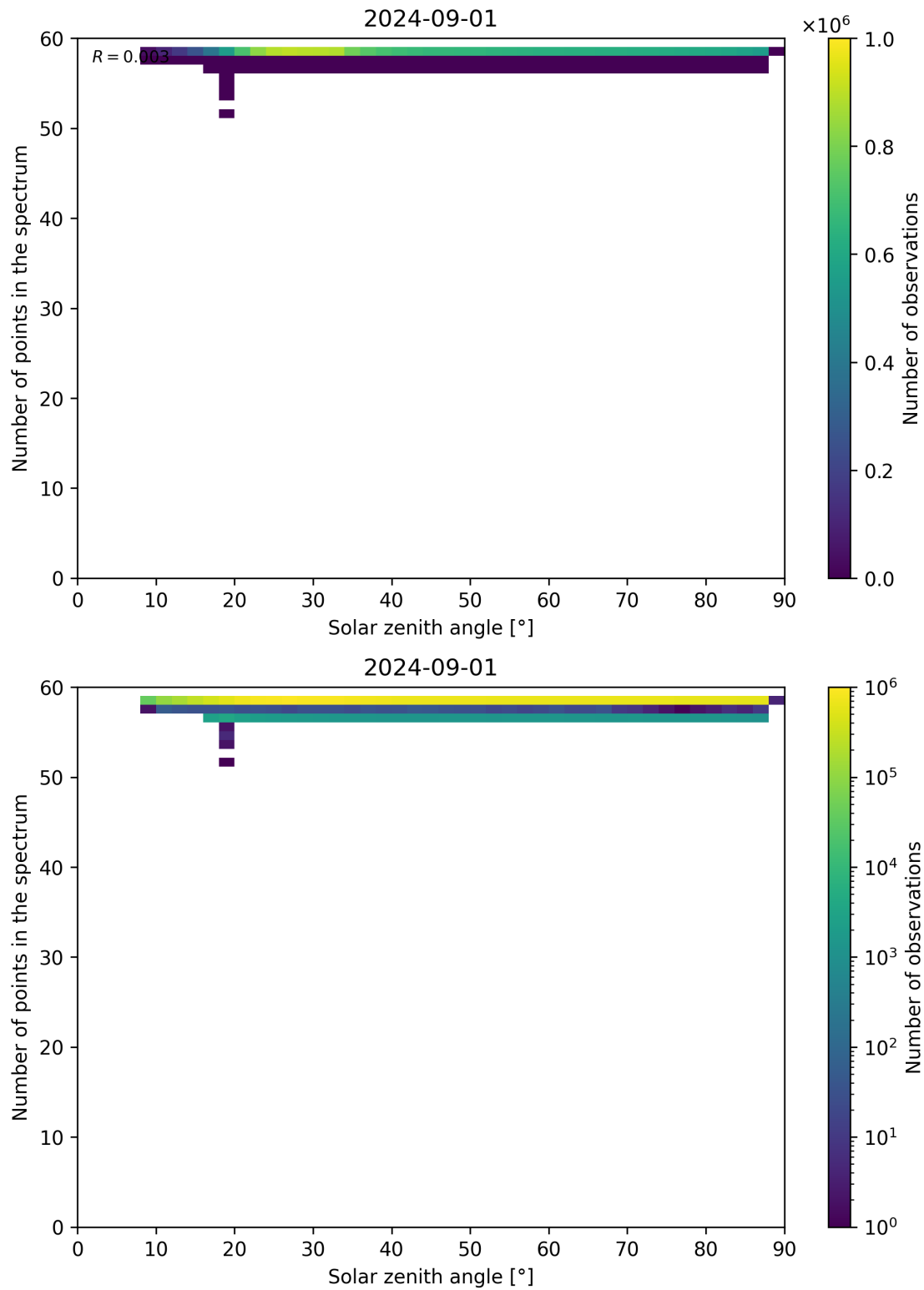
Figure 115: Scatter density plot of “Solar zenith angle” against “Number of points in the spectrum” for 2024-09-01 to 2024-09-02.
