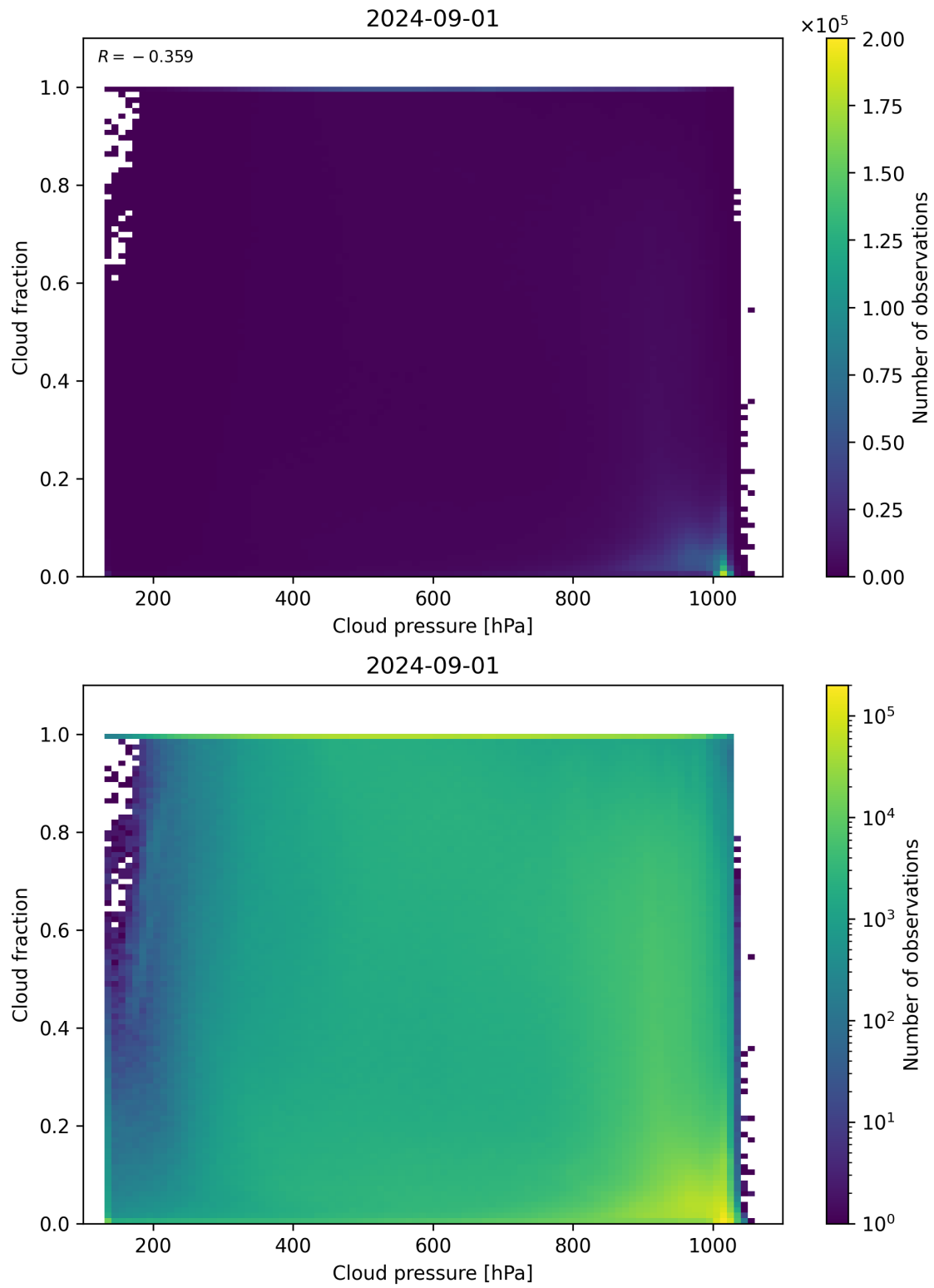
Figure 79: Scatter density plot of “Cloud pressure” against “Cloud fraction” for 2024-09-01 to 2024-09-02.
