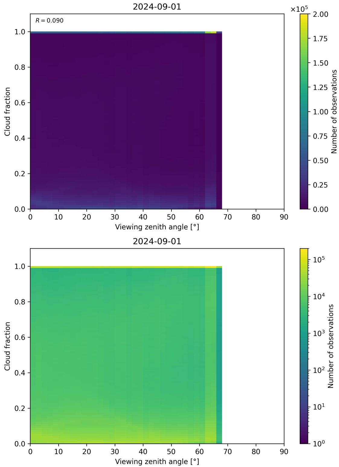
Figure 120: Scatter density plot of “Viewing zenith angle” against “Cloud fraction” for 2024-09-01 to 2024-09-02.
