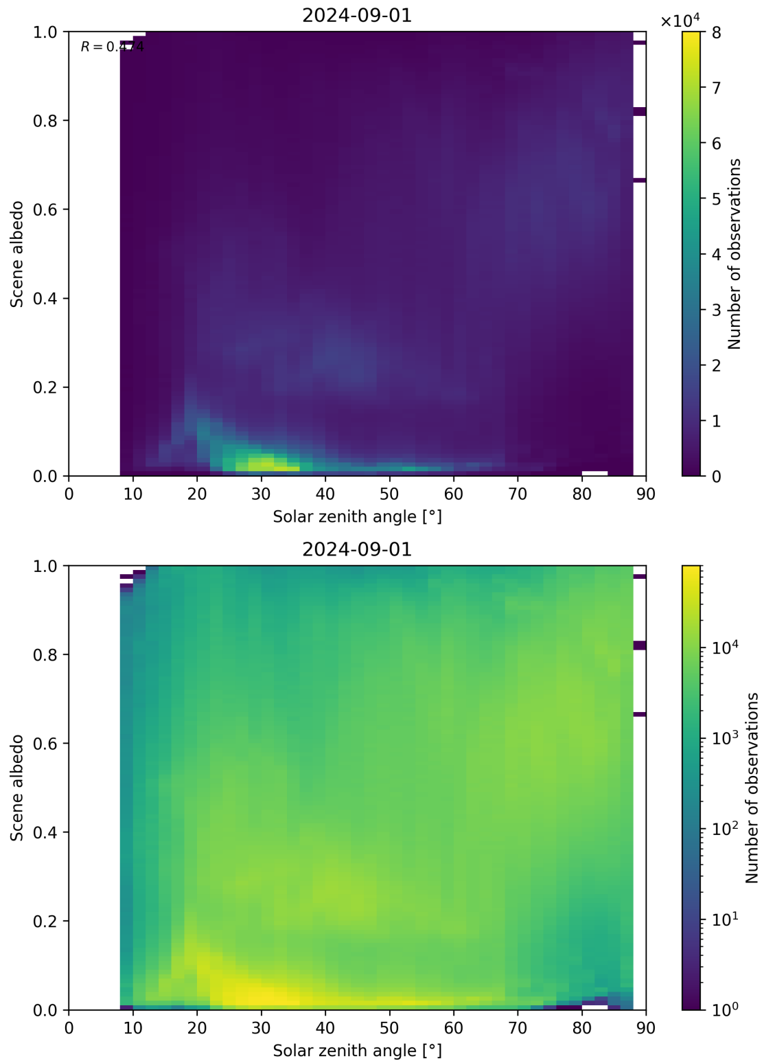
Figure 116: Scatter density plot of “Solar zenith angle” against “Scene albedo” for 2024-09-01 to 2024-09-02.
