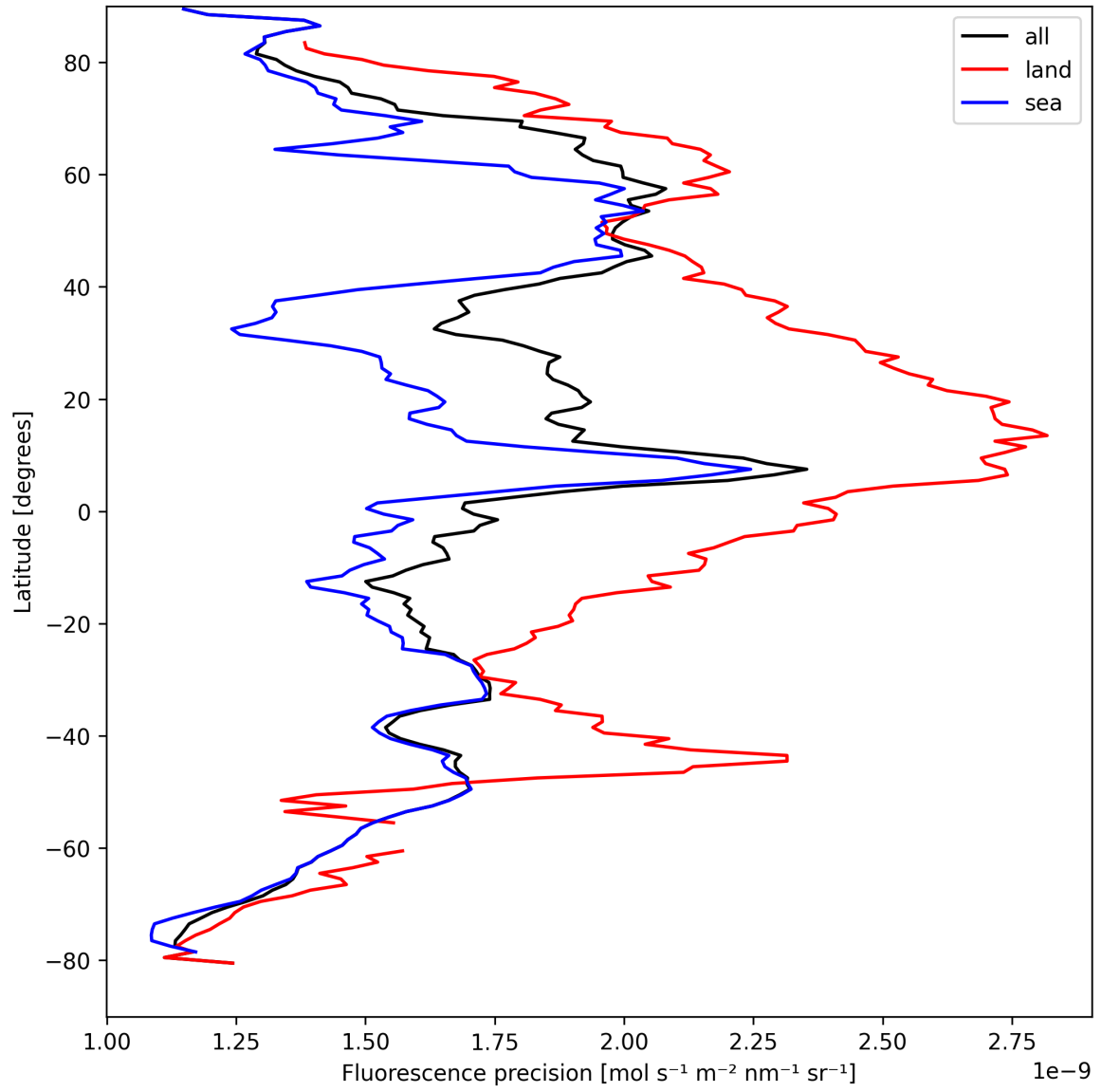
Figure 24: Zonal average of “Fluorescence precision” for 2024-09-01 to 2024-09-02.
