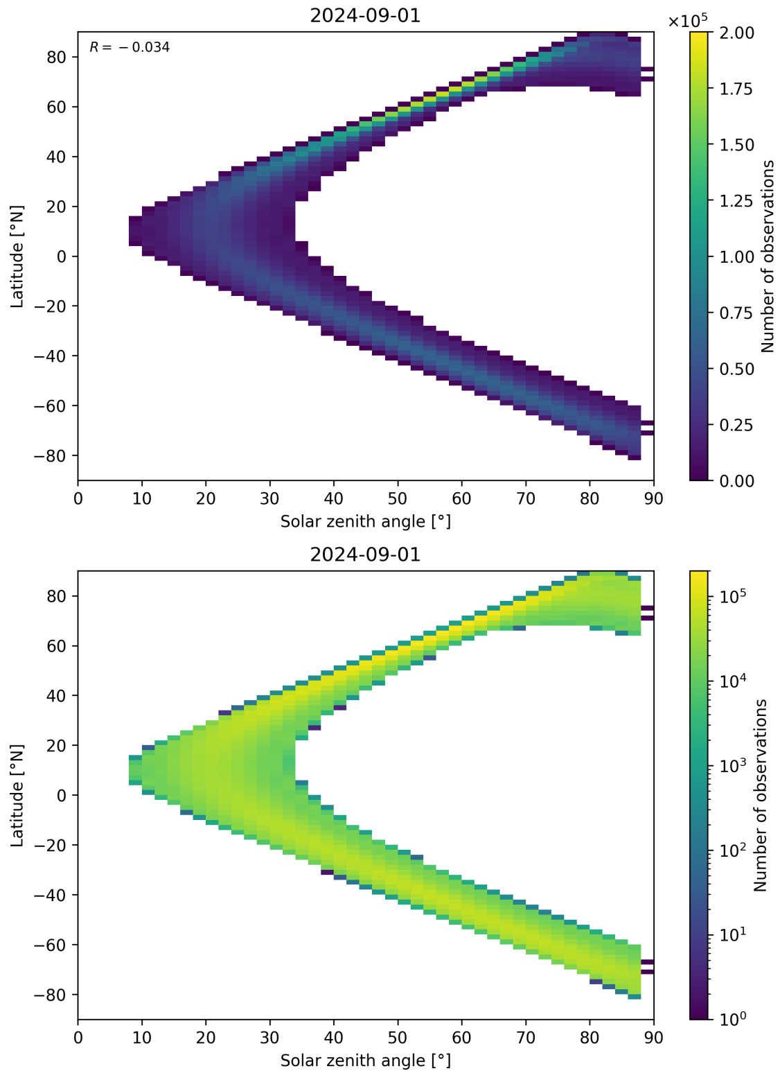
Figure 113: Scatter density plot of “Solar zenith angle” against “Latitude” for 2024-09-01 to 2024-09-02.
