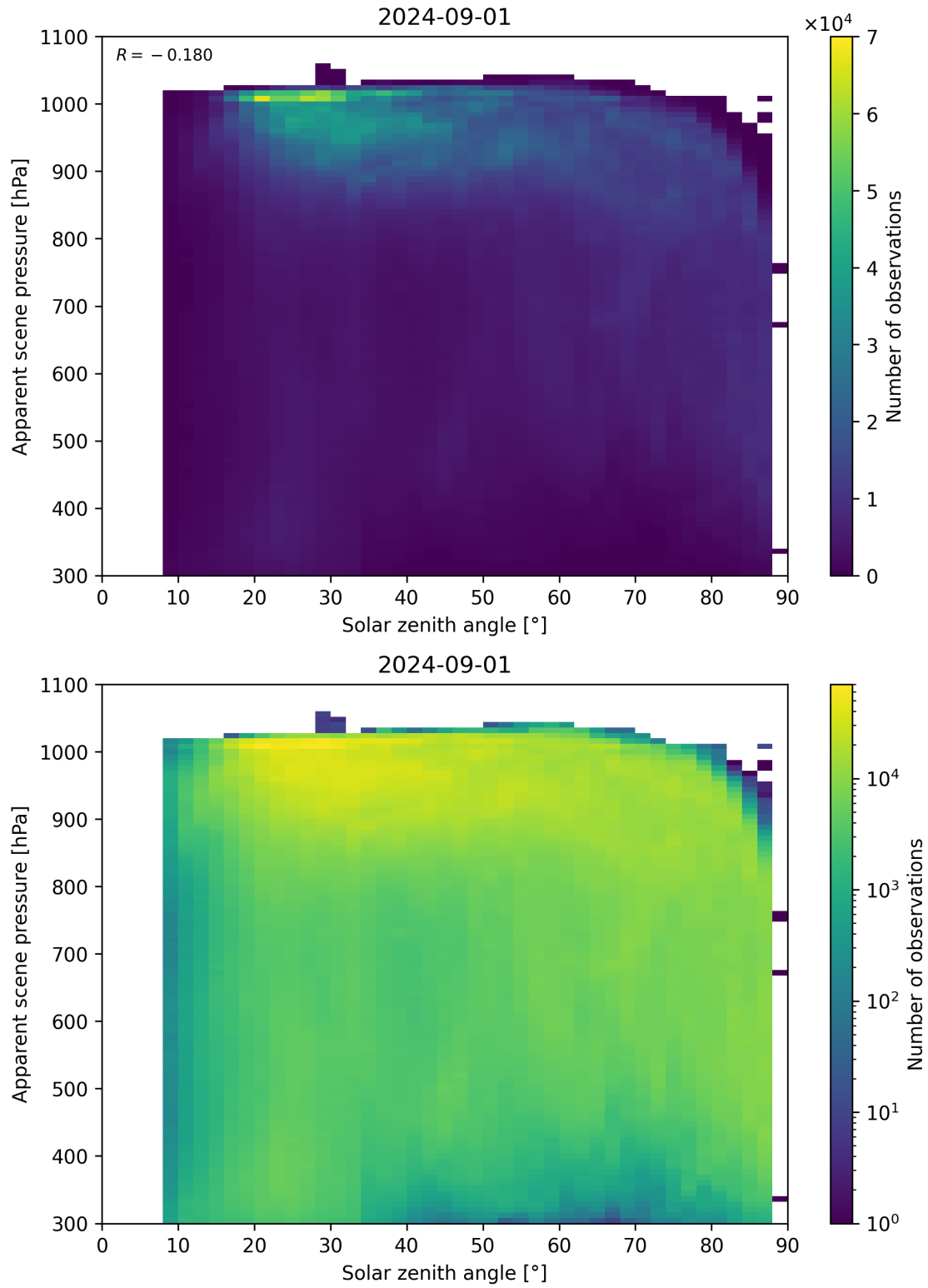
Figure 108: Scatter density plot of “Solar zenith angle” against “Apparent scene pressure” for 2024-09-01 to 2024-09-02.
