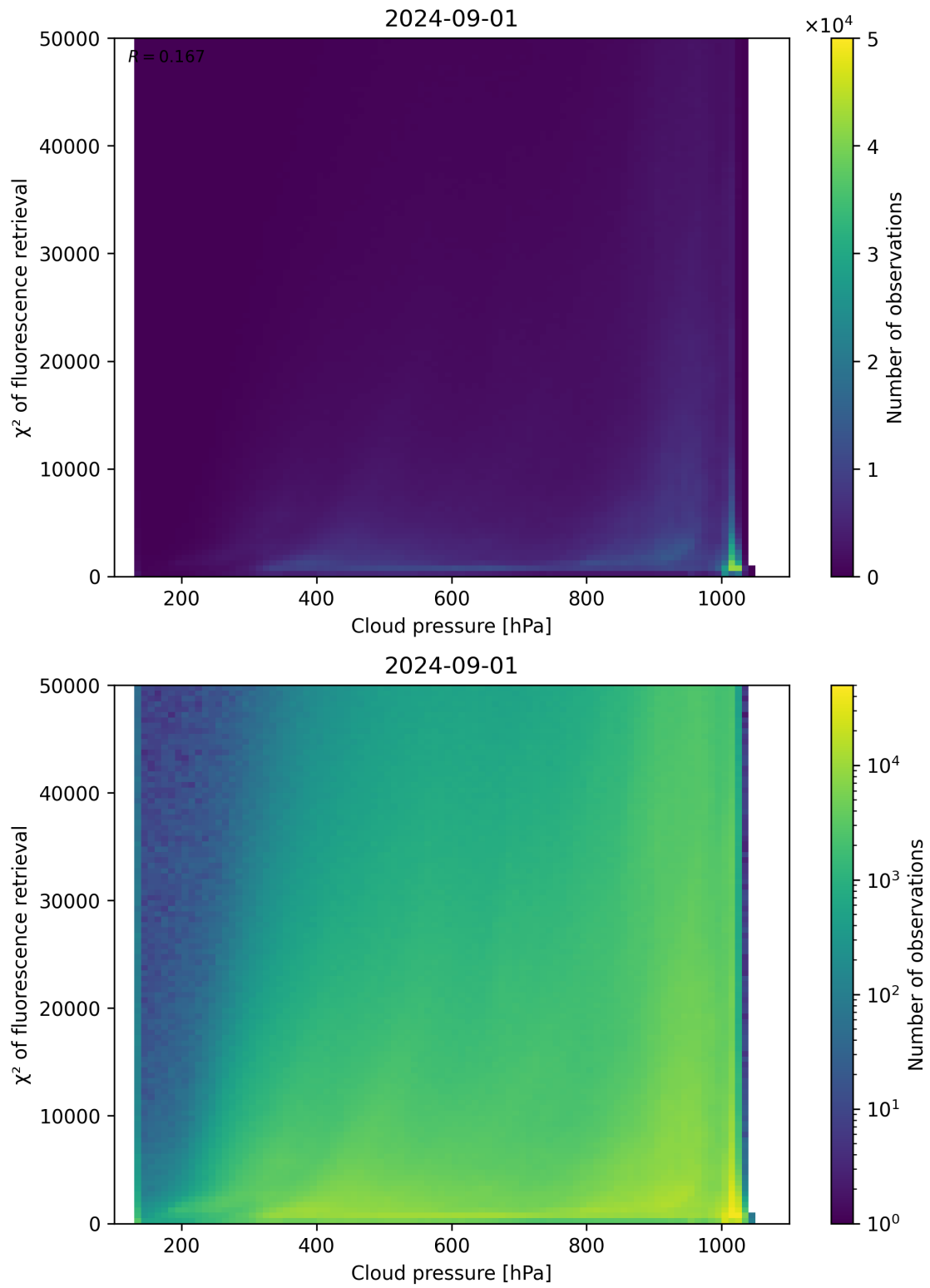
Figure 78: Scatter density plot of “Cloud pressure” against “ \chi^2 of fluorescence retrieval” for 2024-09-01 to 2024-09-02.
