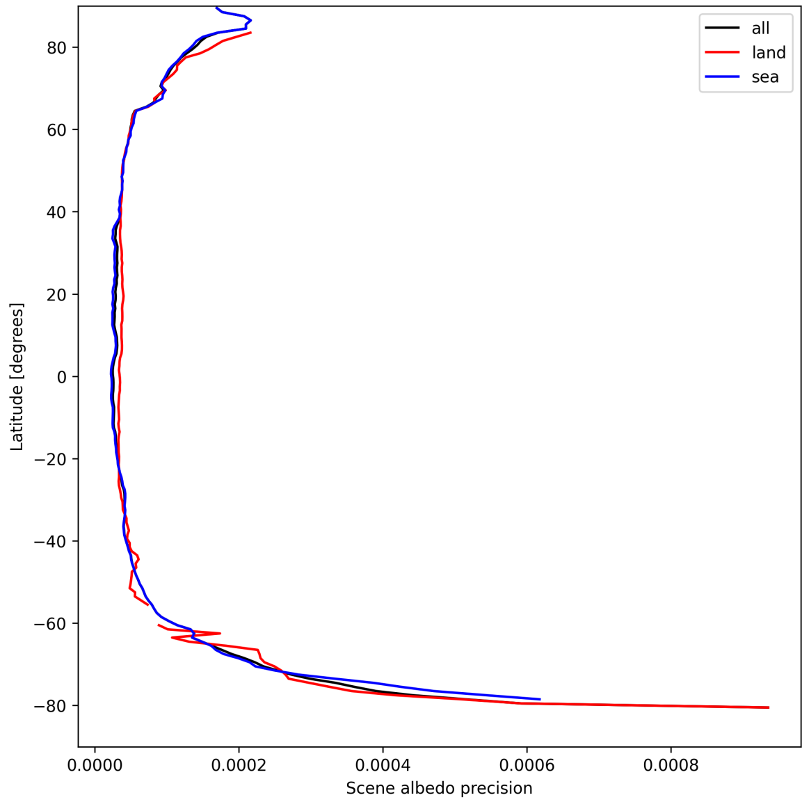
Figure 18: Zonal average of “Scene albedo precision” for 2024-09-01 to 2024-09-02.
