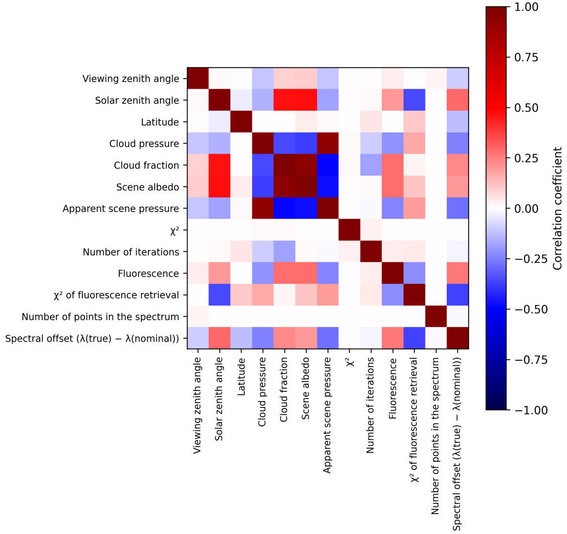
Figure 2: Map of correlation matrix for 2024-09-01 to 2024-09-02.
