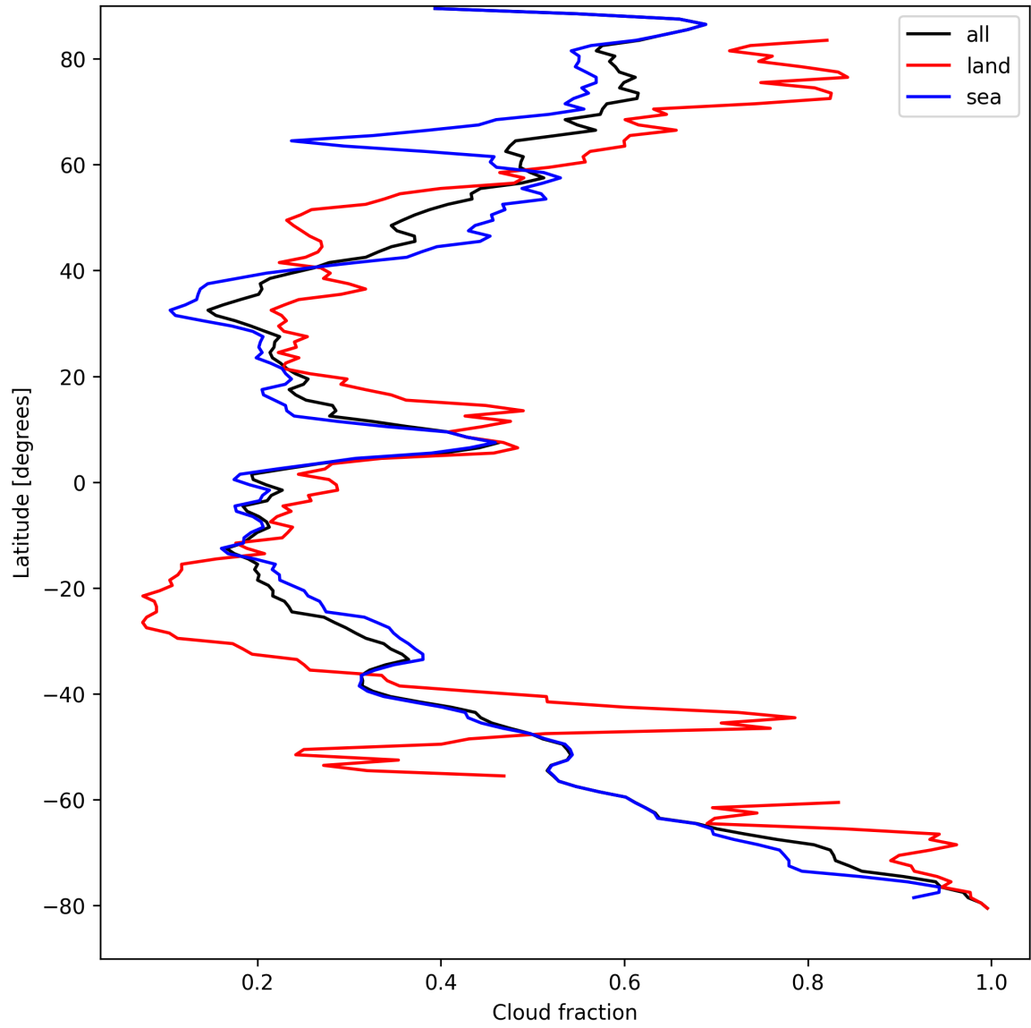
Figure 15: Zonal average of “Cloud fraction” for 2024-09-01 to 2024-09-02.
