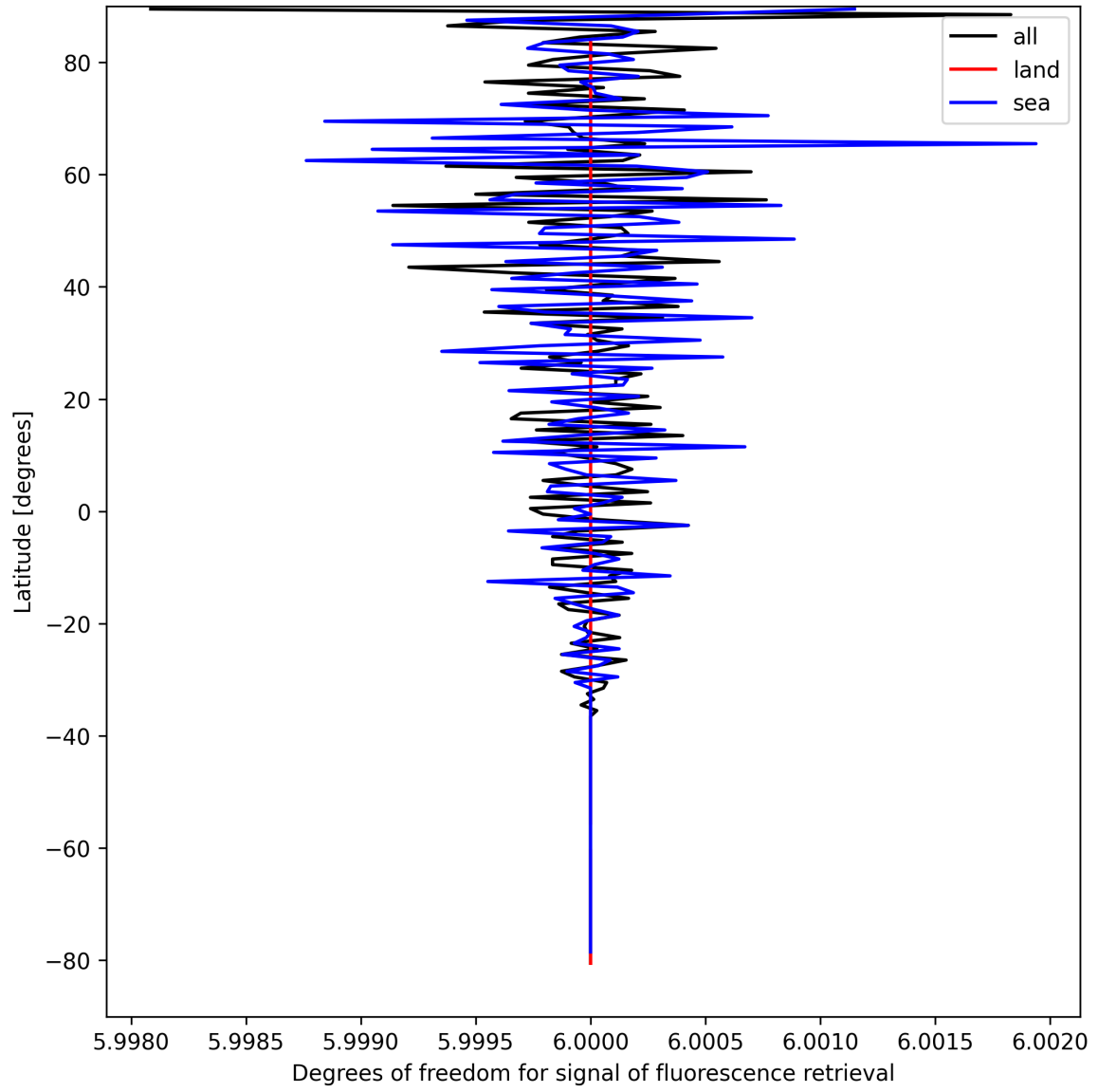
Figure 26: Zonal average of “Degrees of freedom for signal of fluorescence retrieval” for 2024-09-01 to 2024-09-02.
