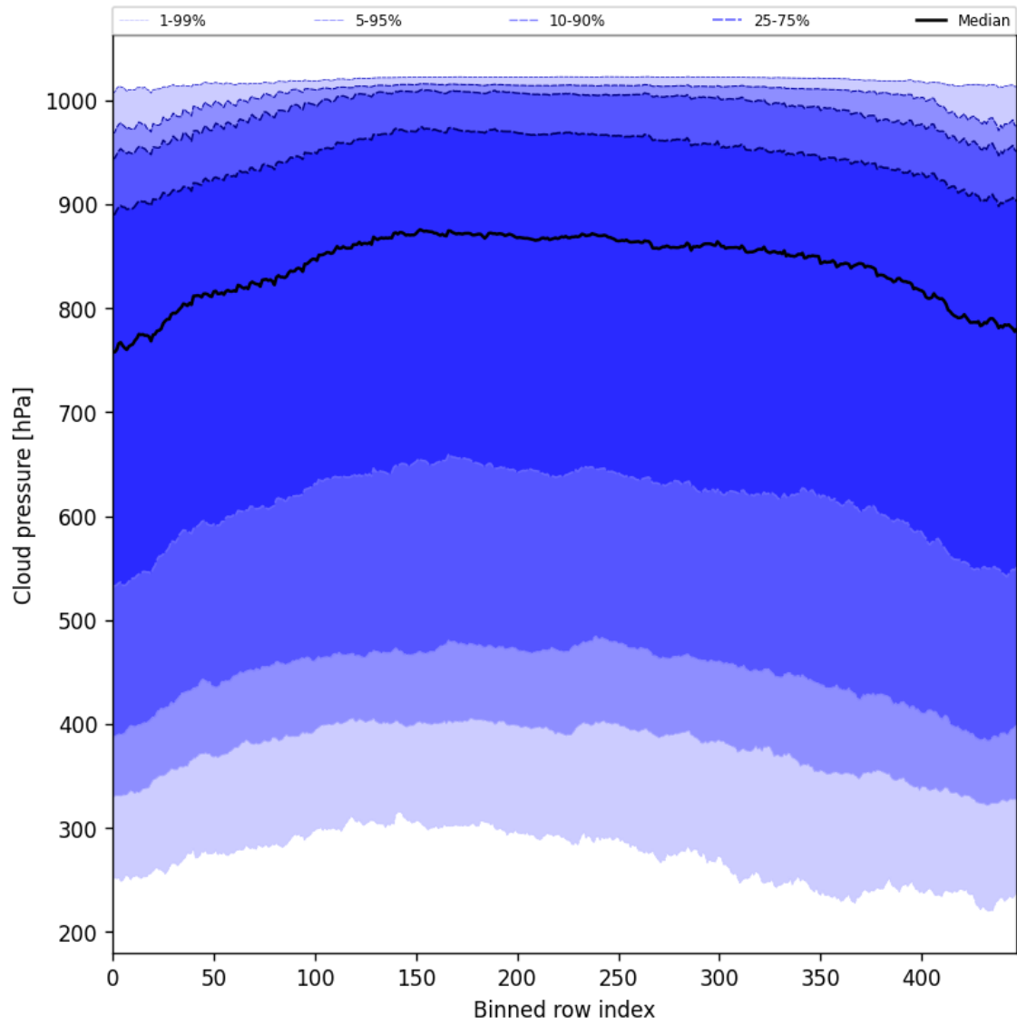
Figure 47: Along track statistics of “Cloud pressure” for 2024-09-01 to 2024-09-02
