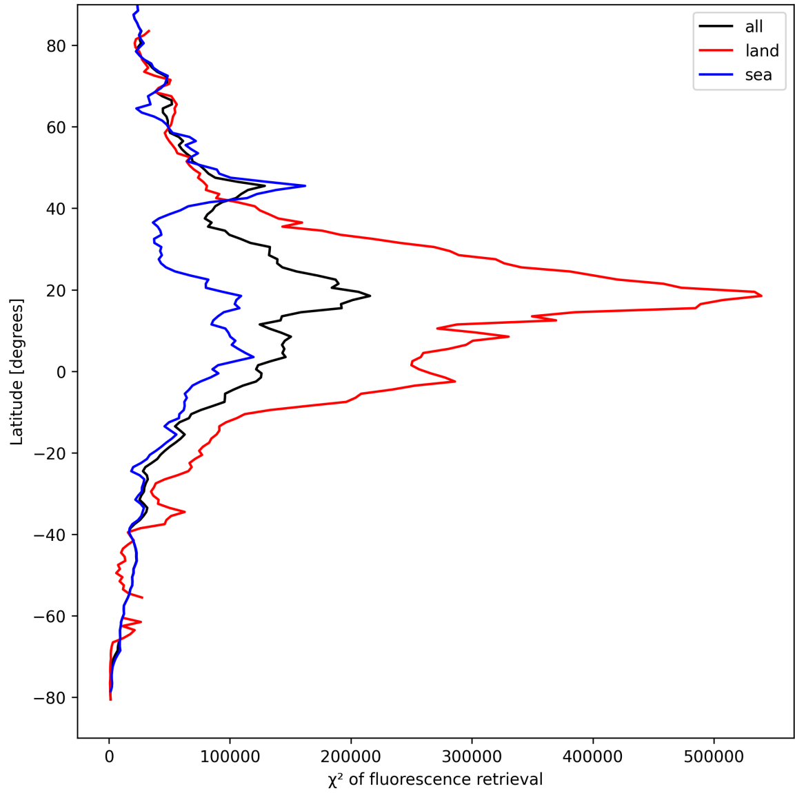
Figure 25: Zonal average of “ \chi^2 of fluorescence retrieval” for 2024-09-01 to 2024-09-02.
