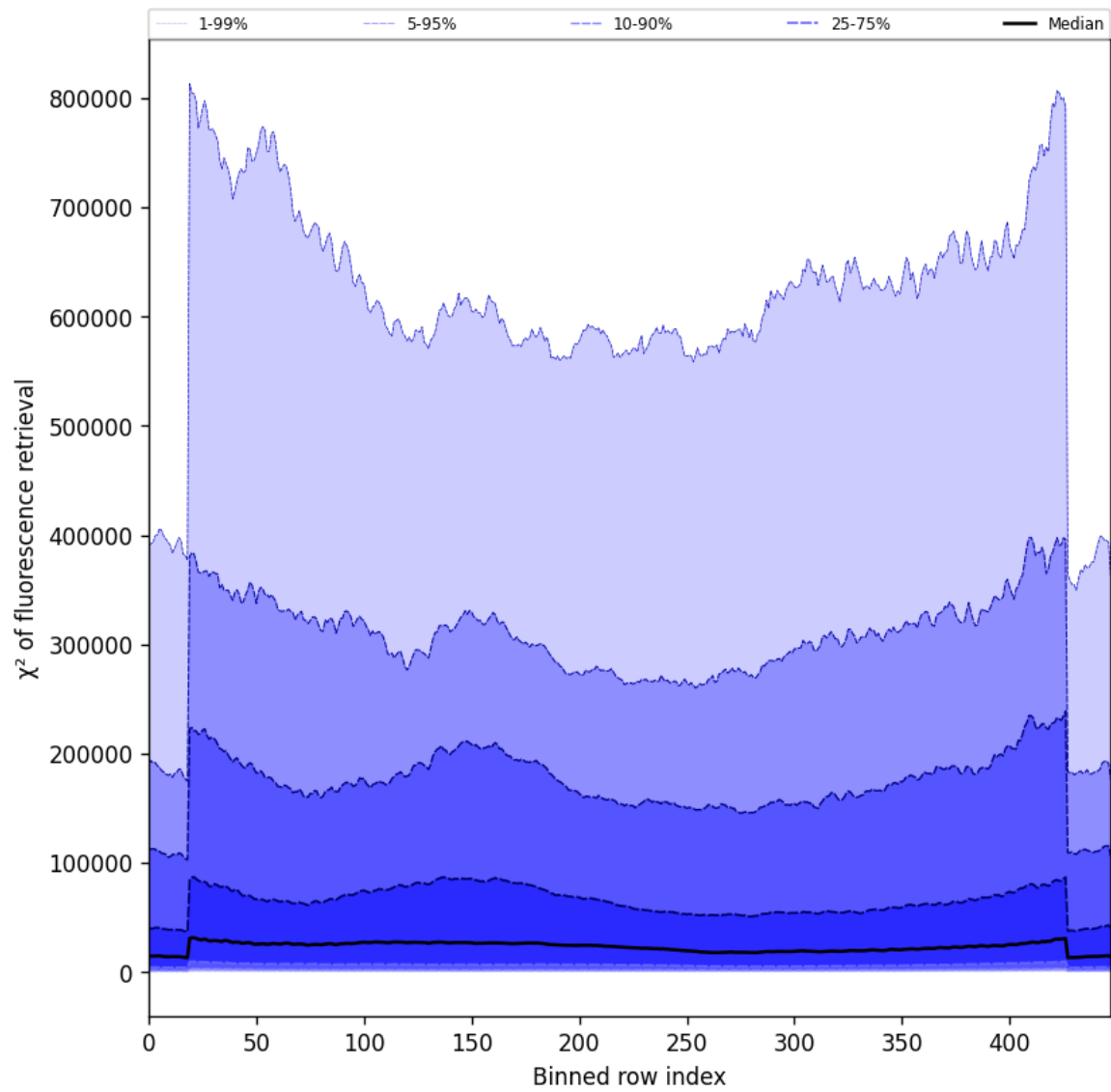
Figure 59: Along track statistics of “ \chi^2 of fluorescence retrieval” for 2024-09-01 to 2024-09-02
