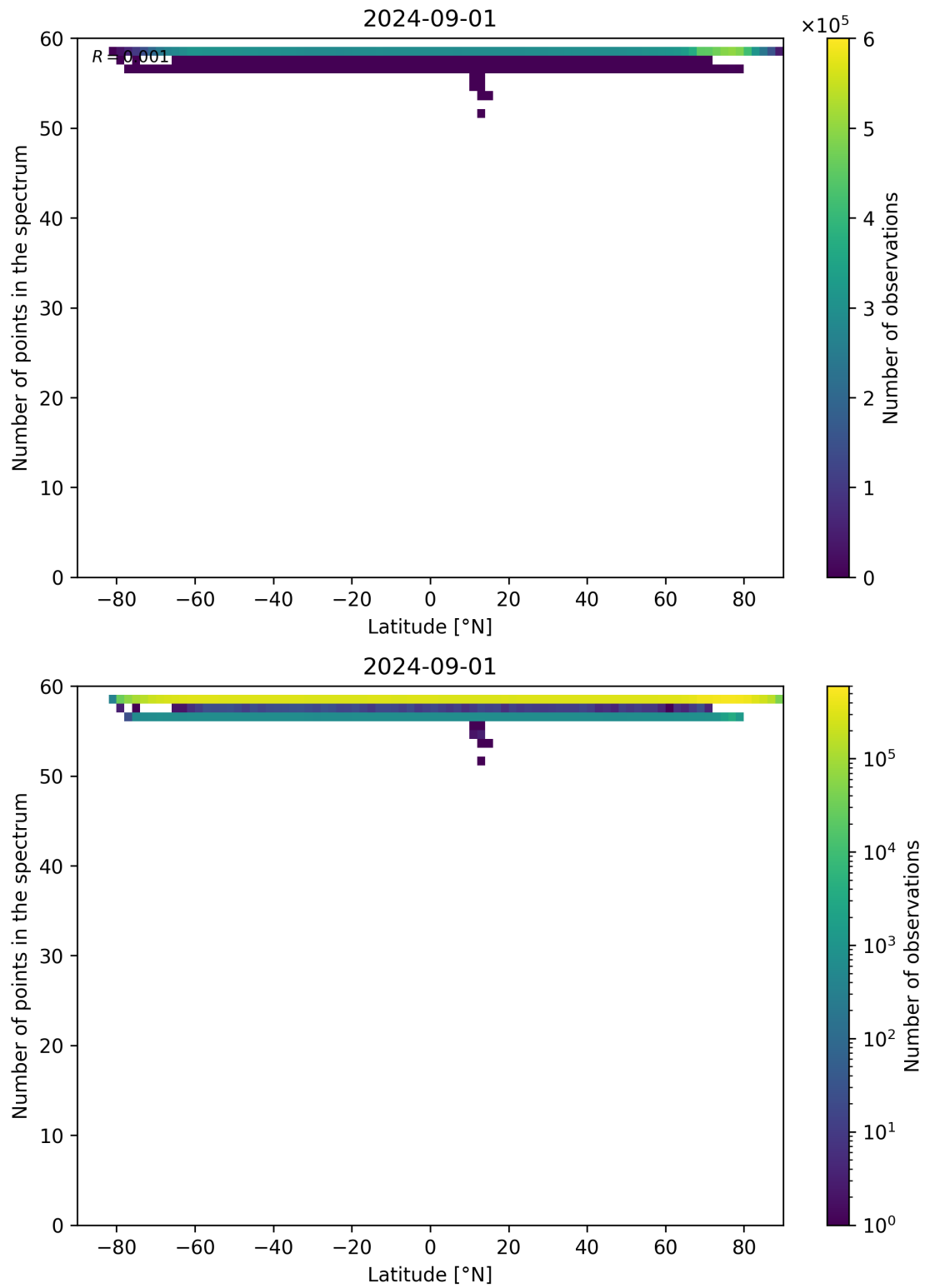
Figure 94: Scatter density plot of “Latitude” against “Number of points in the spectrum” for 2024-09-01 to 2024-09-02.
