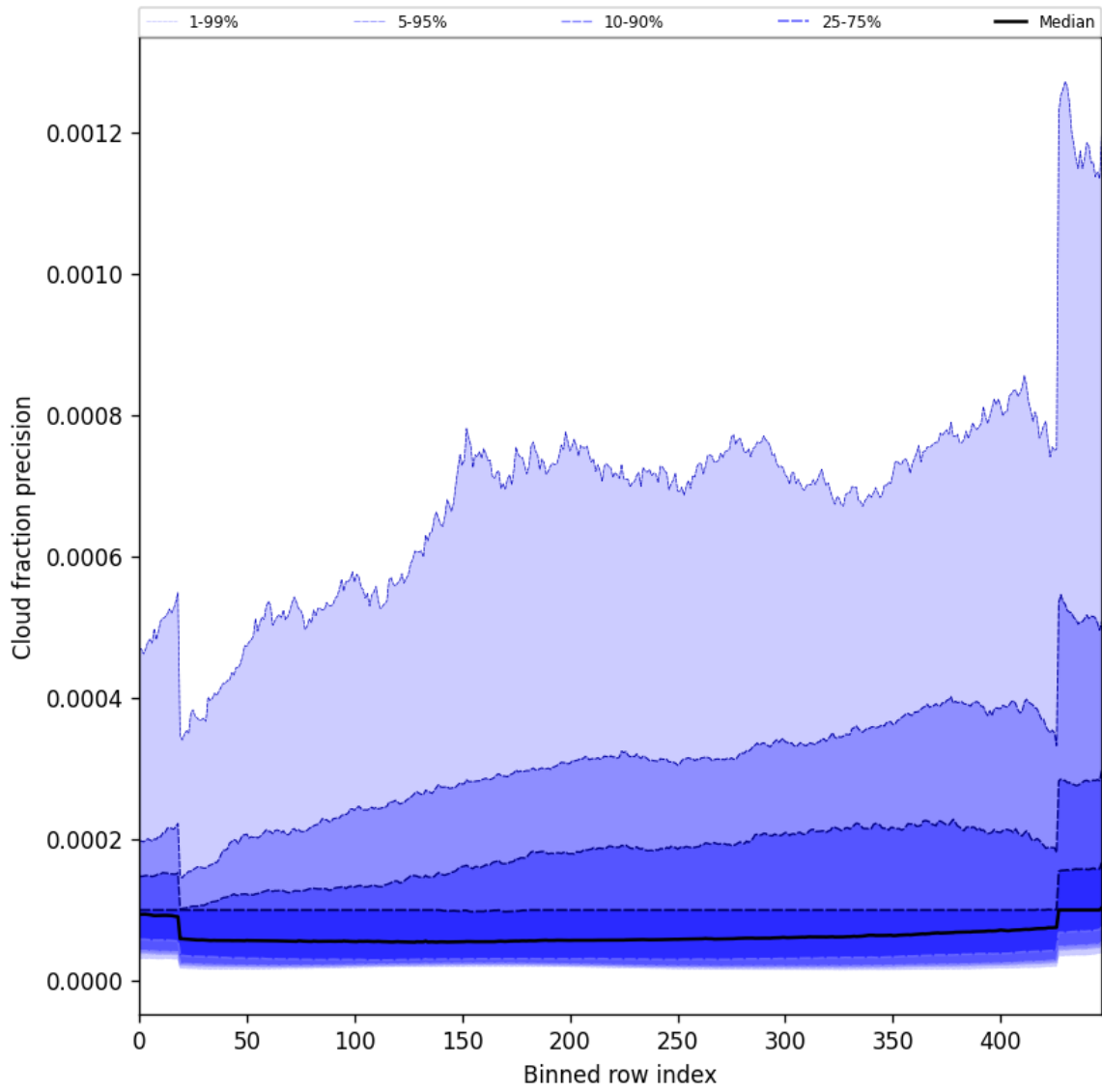
Figure 50: Along track statistics of “Cloud fraction precision” for 2024-09-01 to 2024-09-02
