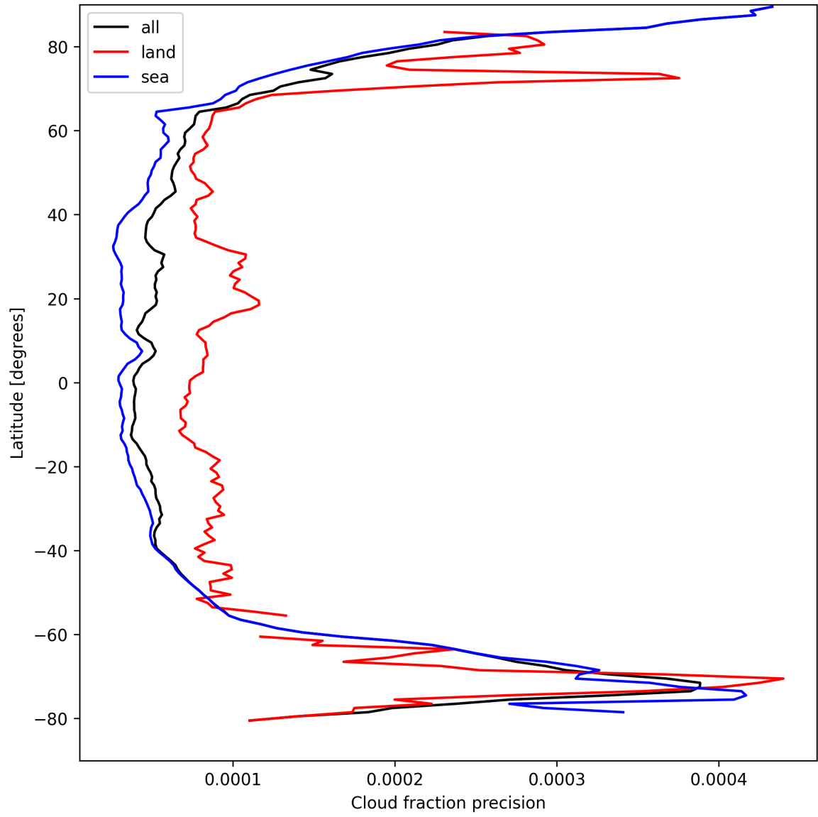
Figure 16: Zonal average of “Cloud fraction precision” for 2024-09-01 to 2024-09-02.
