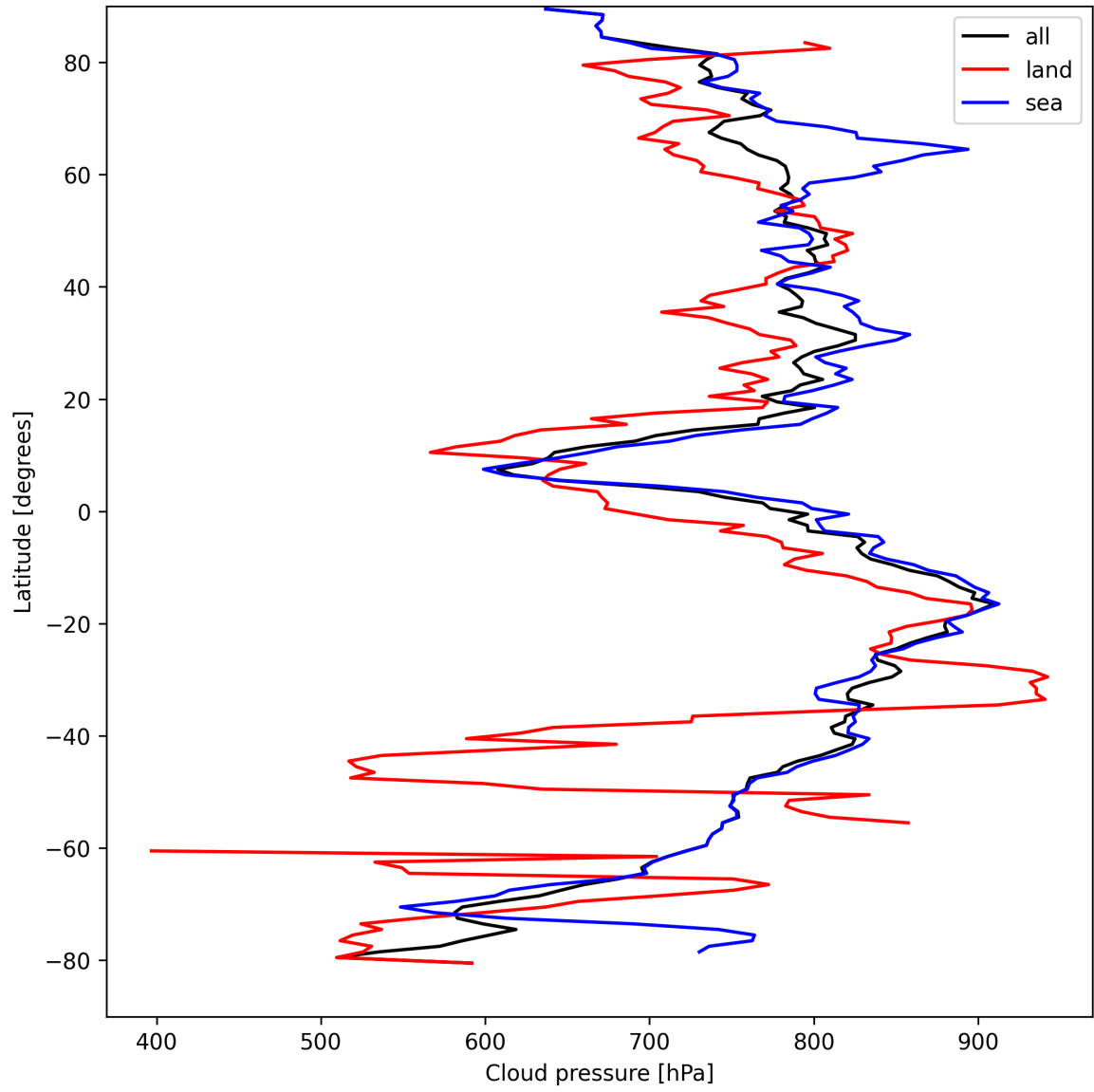
Figure 13: Zonal average of “Cloud pressure” for 2024-09-01 to 2024-09-02.
