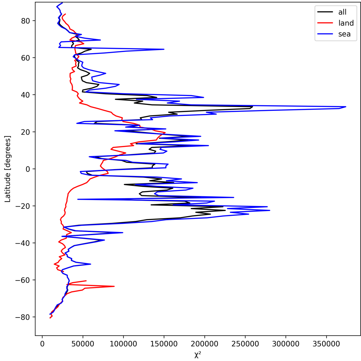
Figure 21: Zonal average of “ \chi^2 ” for 2024-09-01 to 2024-09-02.
