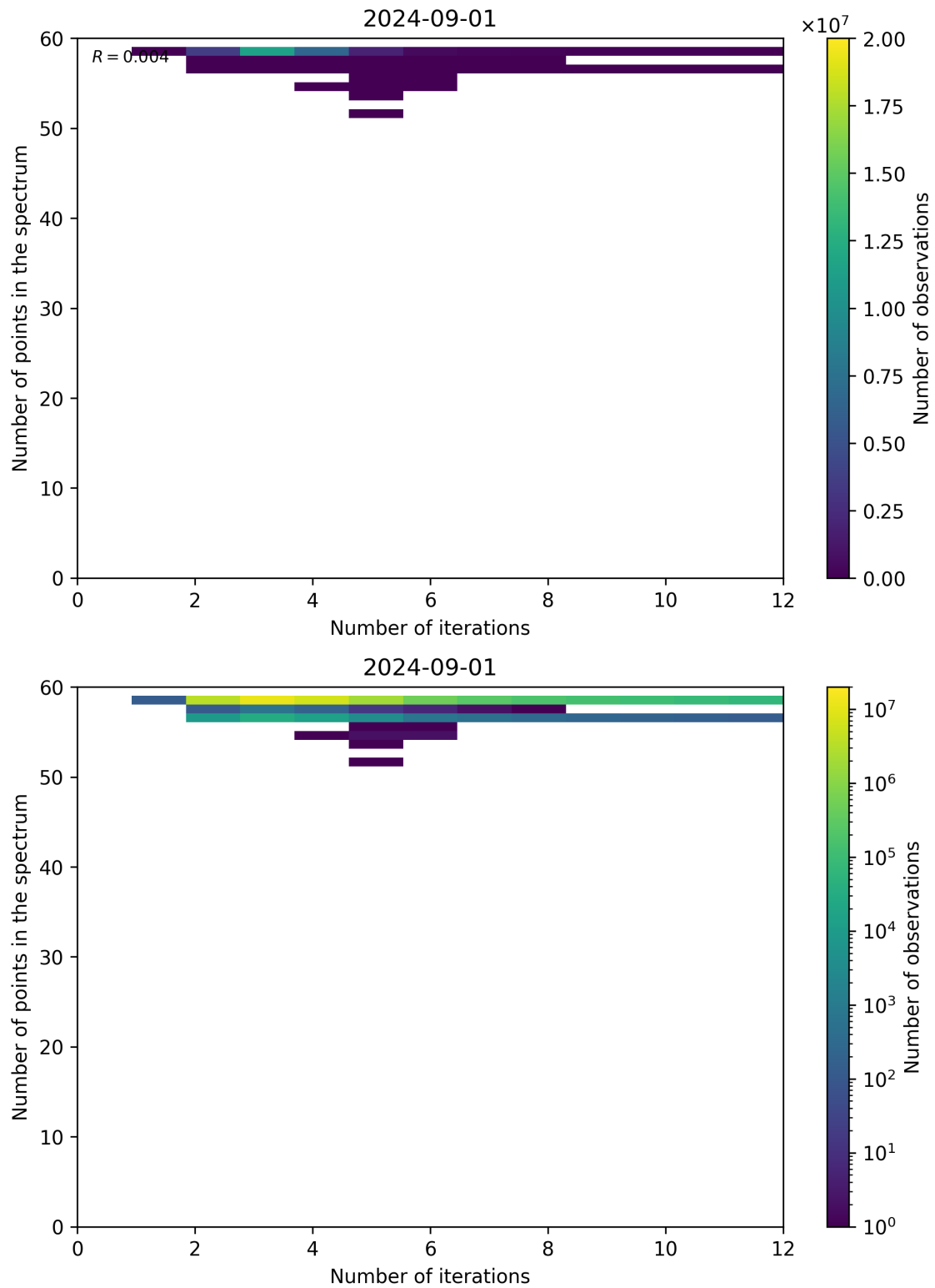
Figure 99: Scatter density plot of “Number of iterations” against “Number of points in the spectrum” for 2024-09-01 to 2024-09-02.
