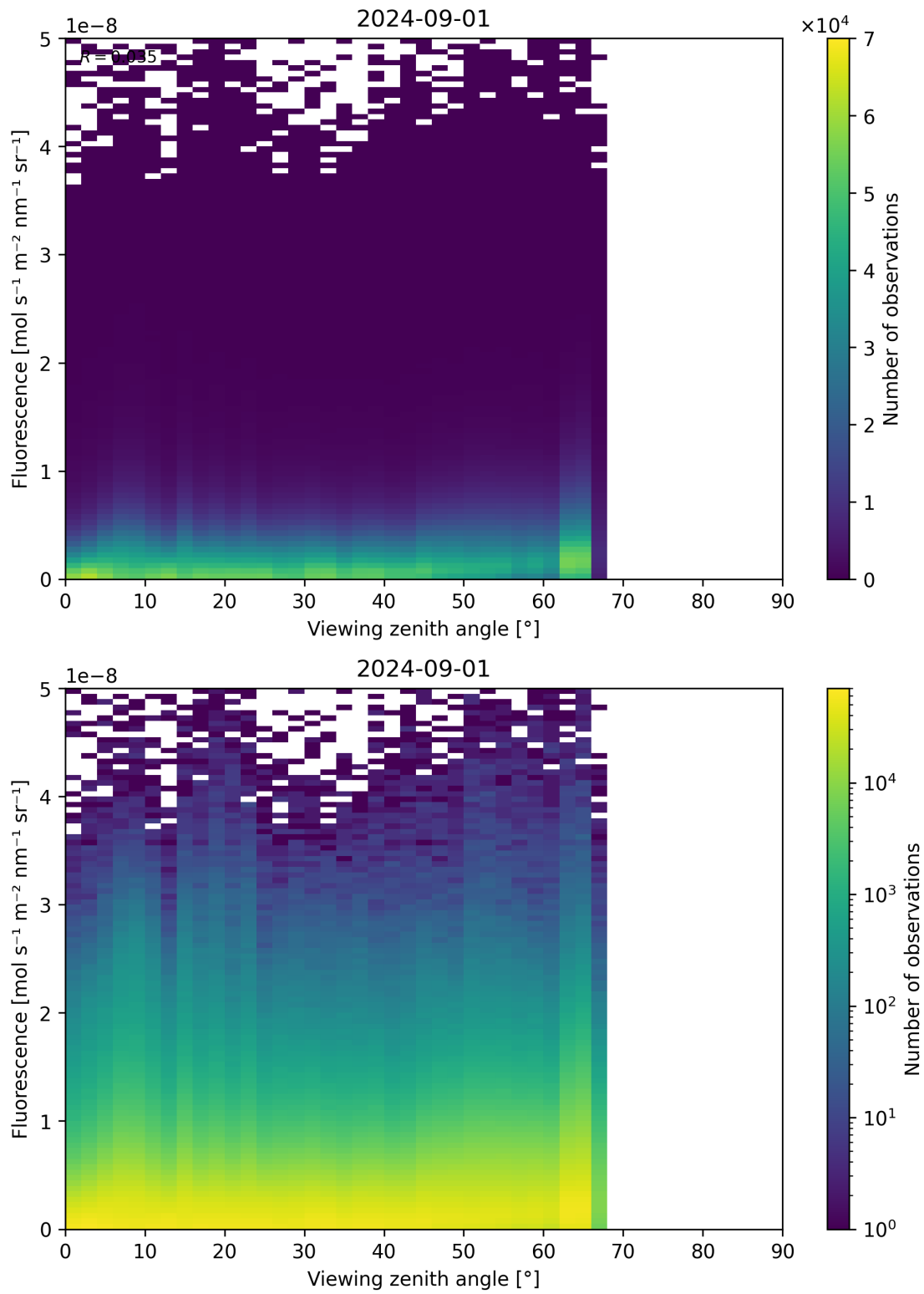
Figure 122: Scatter density plot of “Viewing zenith angle” against “Fluorescence” for 2024-09-01 to 2024-09-02.
