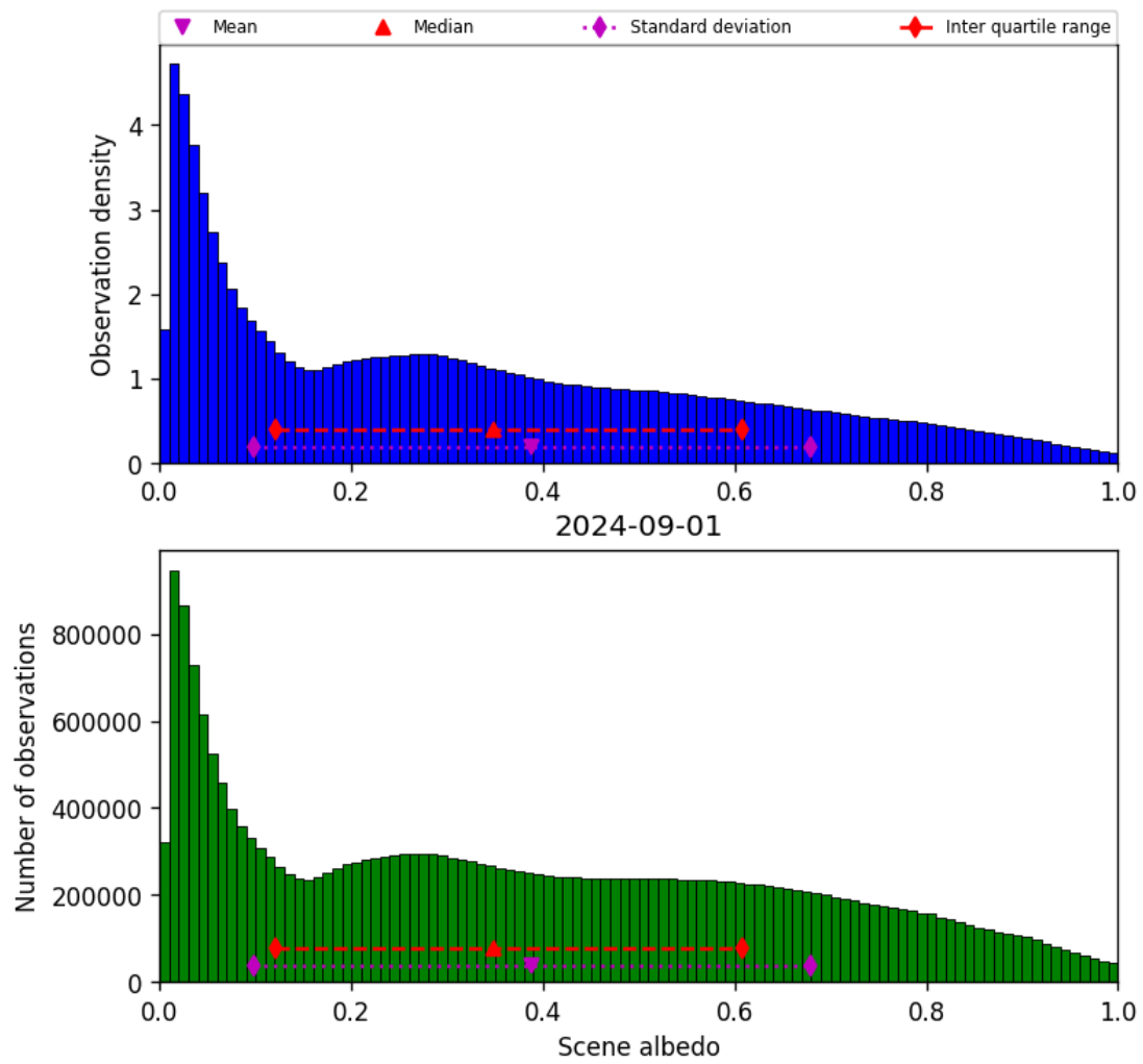
Figure 34: Histogram of “Scene albedo” for 2024-09-01 to 2024-09-02
