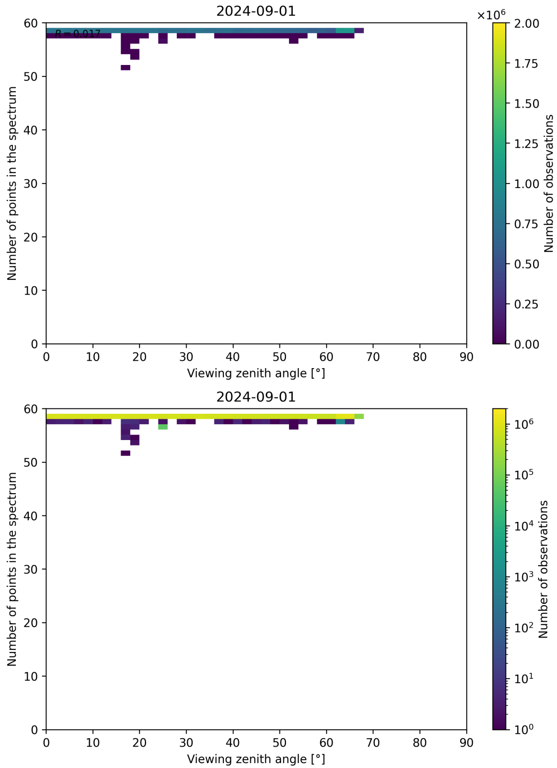
Figure 125: Scatter density plot of “Viewing zenith angle” against “Number of points in the spectrum” for 2024-09-01 to 2024-09-02.
