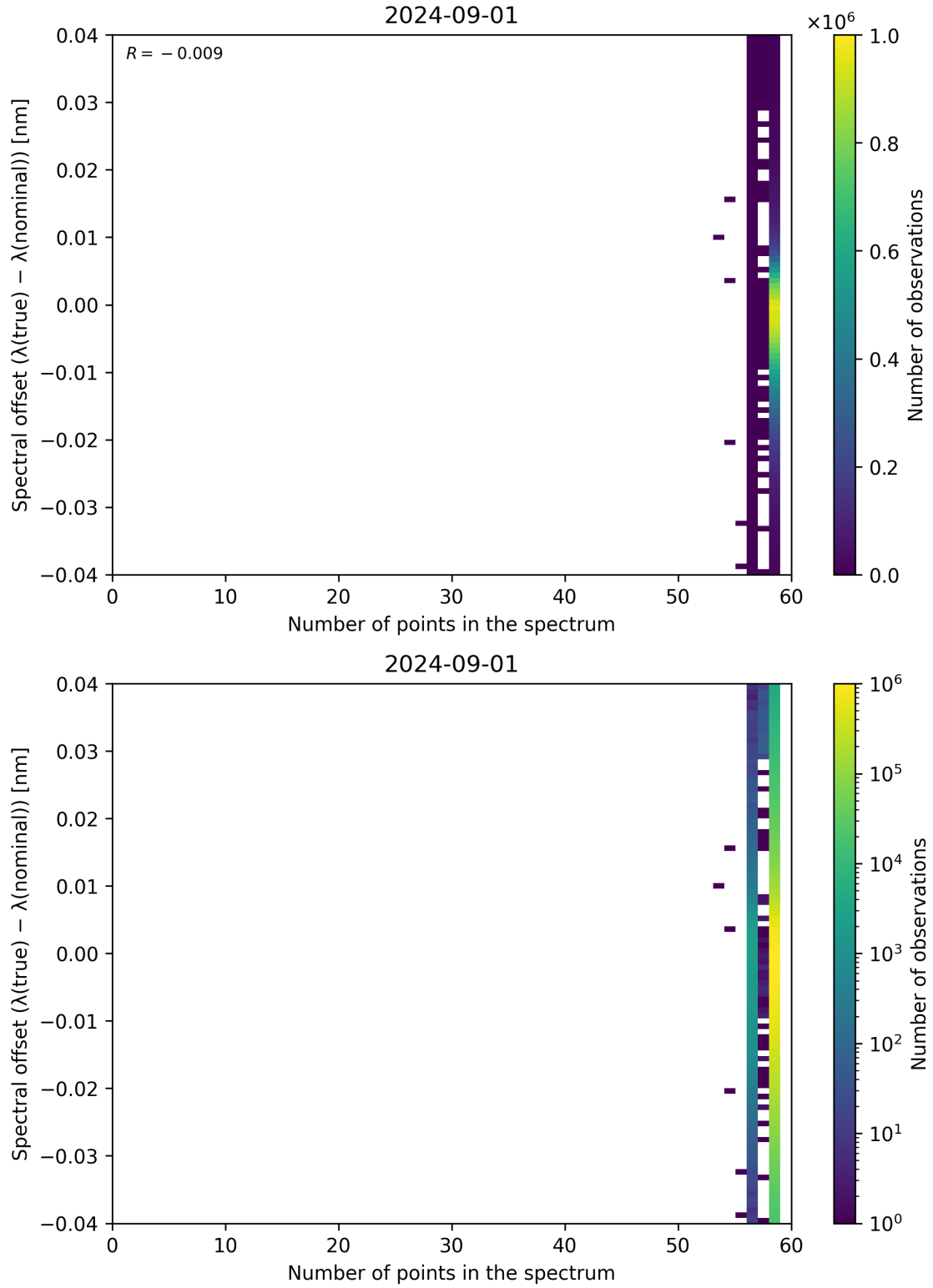
Figure 101: Scatter density plot of “Number of points in the spectrum” against “Spectral offset ( \lambda_{\text{true}} - \lambda_{\text{nominal}} )” for 2024-09-01 to 2024-09-02.
