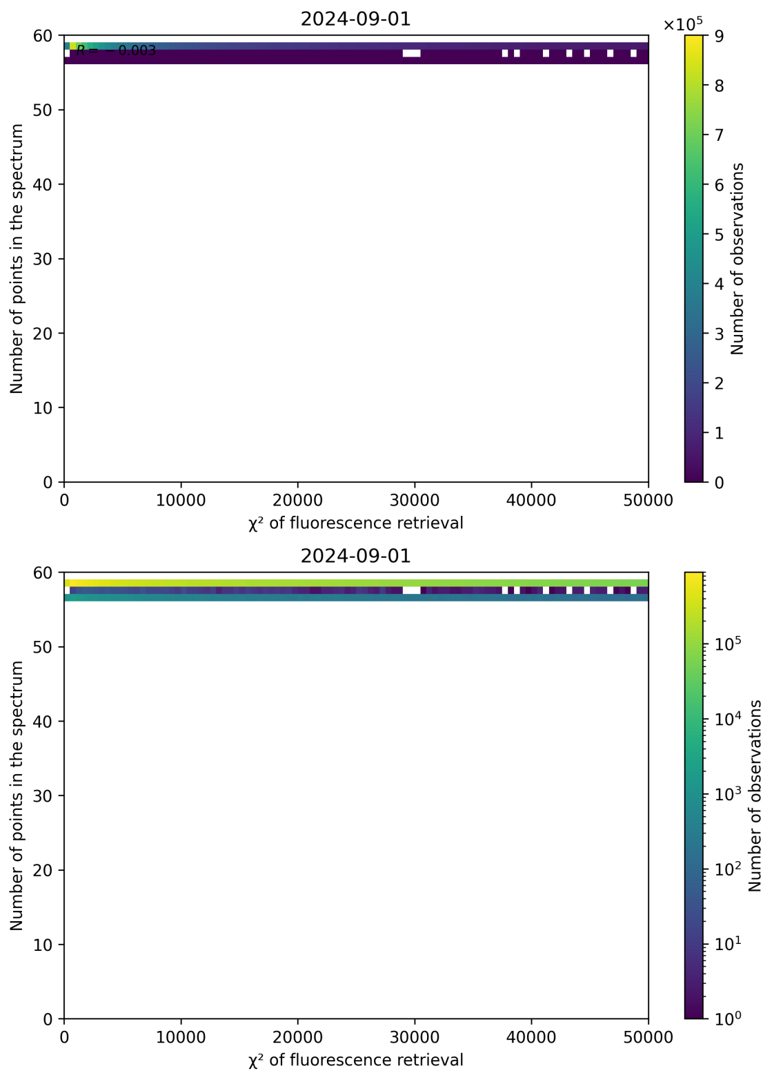
Figure 68: Scatter density plot of “ \chi^2 of fluorescence retrieval” against “Number of points in the spectrum” for 2024-09-01 to 2024-09-02.
