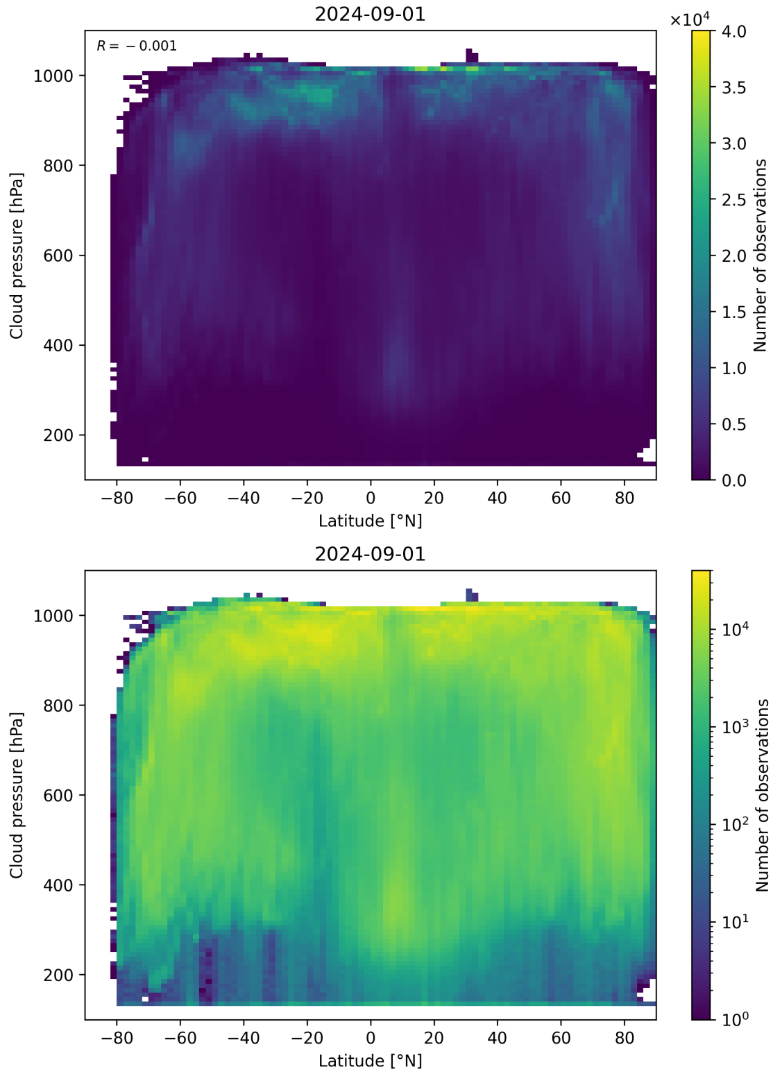
Figure 91: Scatter density plot of “Latitude” against “Cloud pressure” for 2024-09-01 to 2024-09-02.
