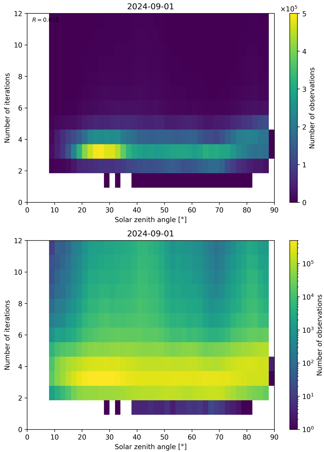
Figure 114: Scatter density plot of “Solar zenith angle” against “Number of iterations” for 2024-09-01 to 2024-09-02.
