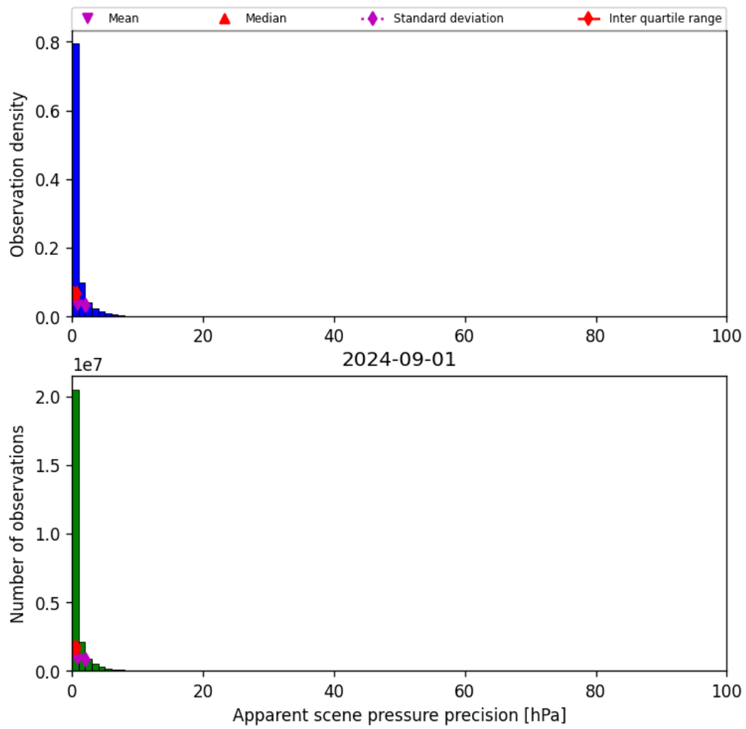
Figure 37: Histogram of “Apparent scene pressure precision” for 2024-09-01 to 2024-09-02
