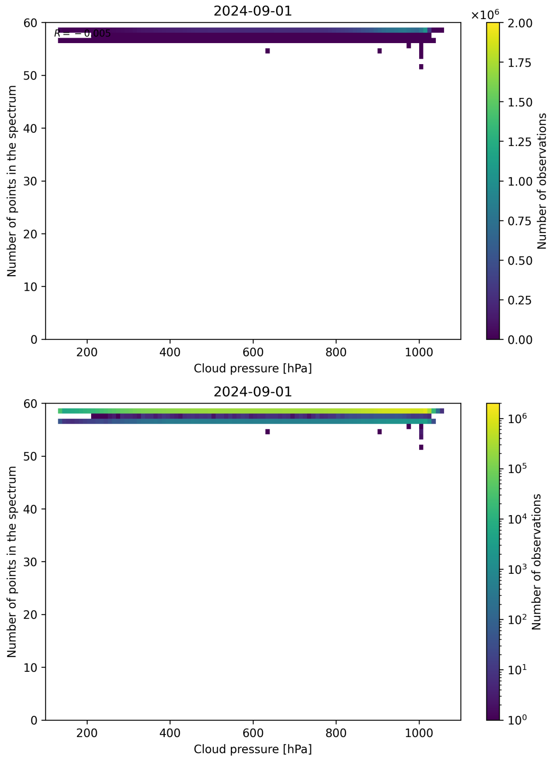
Figure 82: Scatter density plot of “Cloud pressure” against “Number of points in the spectrum” for 2024-09-01 to 2024-09-02.
