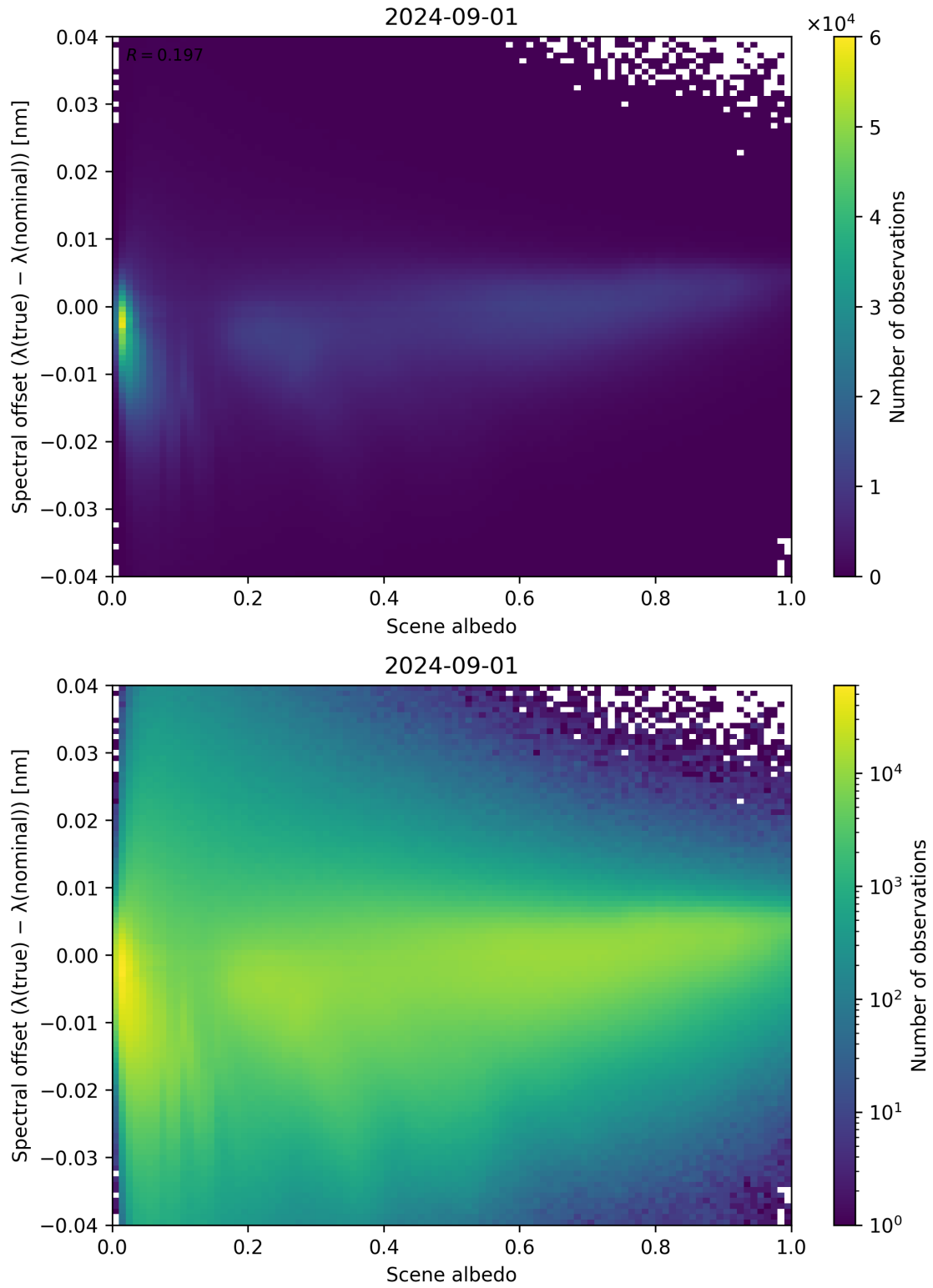
Figure 107: Scatter density plot of “Scene albedo” against “Spectral offset ( \lambda_{\text{true}} - \lambda_{\text{nominal}} )” for 2024-09-01 to 2024-09-02.
