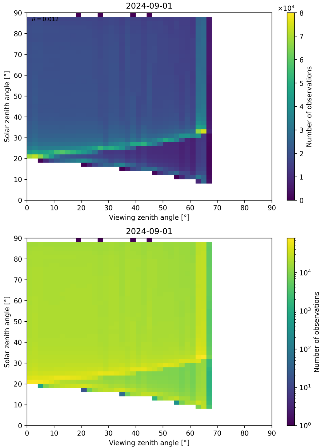
Figure 127: Scatter density plot of “Viewing zenith angle” against “Solar zenith angle” for 2024-09-01 to 2024-09-02.
