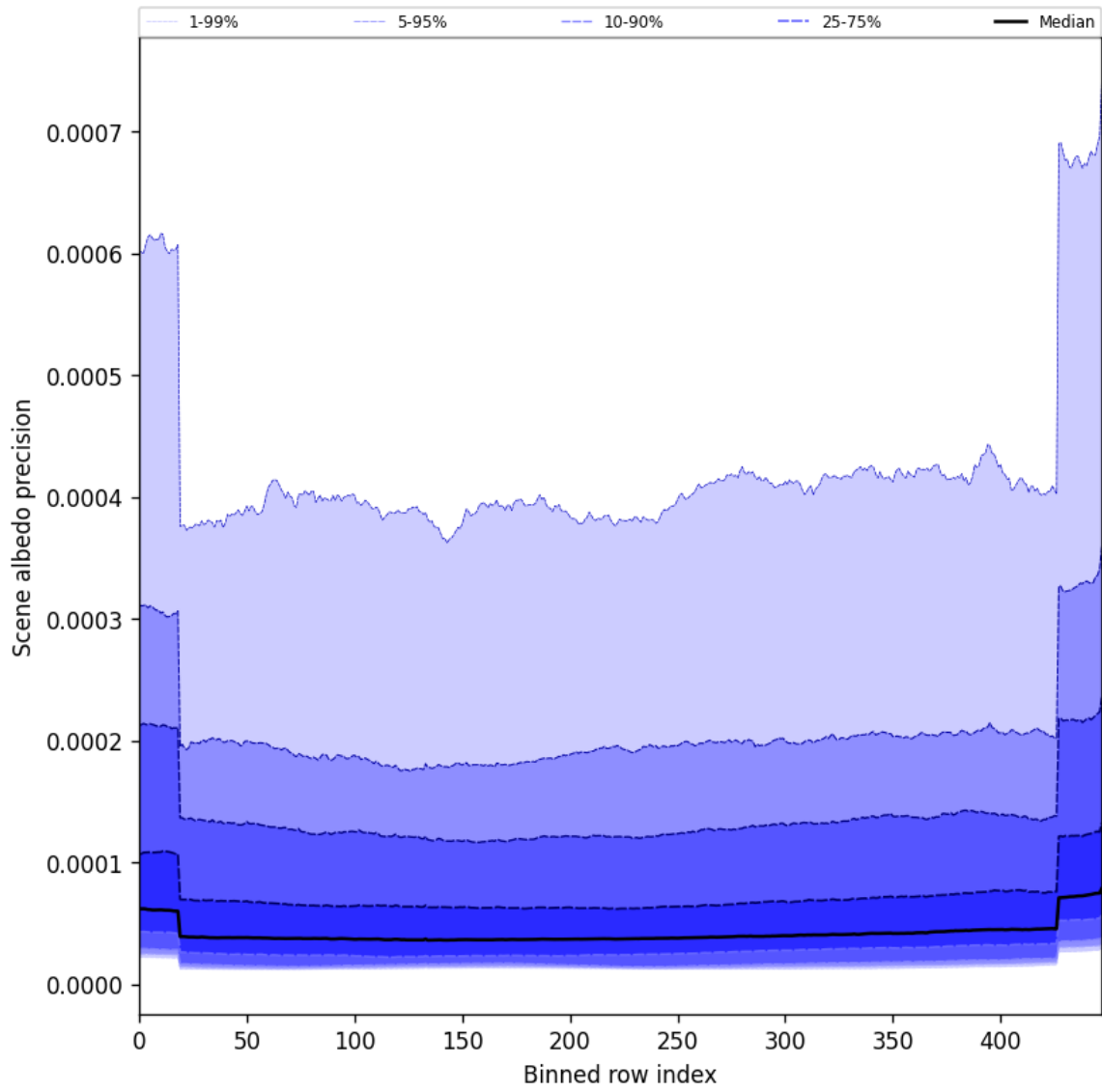
Figure 52: Along track statistics of “Scene albedo precision” for 2024-09-01 to 2024-09-02
