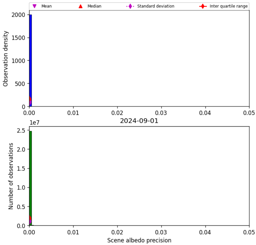
Figure 35: Histogram of “Scene albedo precision” for 2024-09-01 to 2024-09-02
