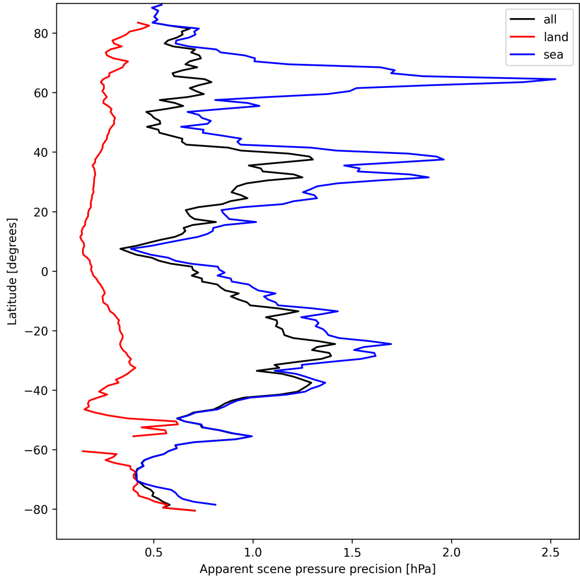
Figure 20: Zonal average of “Apparent scene pressure precision” for 2024-09-01 to 2024-09-02.
