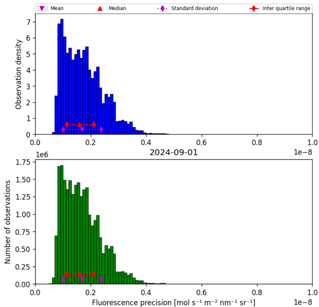
Figure 41: Histogram of “Fluorescence precision” for 2024-09-01 to 2024-09-02
