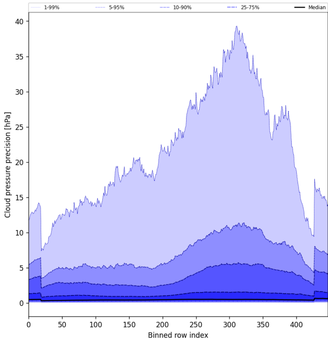
Figure 48: Along track statistics of “Cloud pressure precision” for 2024-09-01 to 2024-09-02
