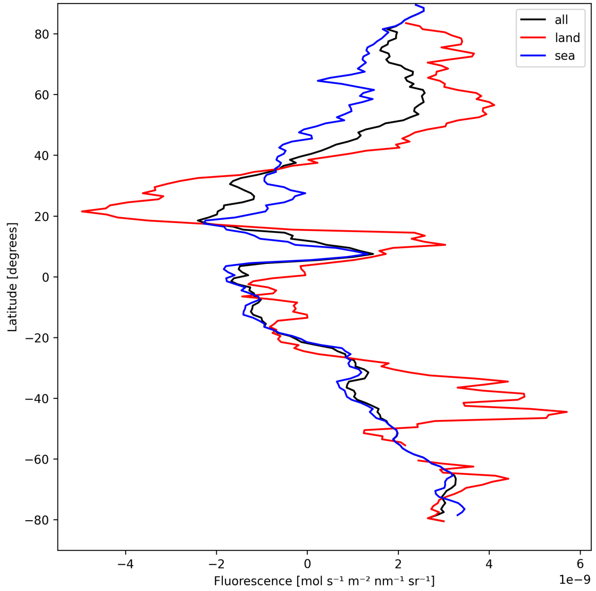
Figure 23: Zonal average of “Fluorescence” for 2024-09-01 to 2024-09-02.
