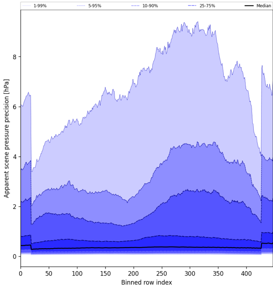
Figure 54: Along track statistics of “Apparent scene pressure precision” for 2024-09-01 to 2024-09-02
