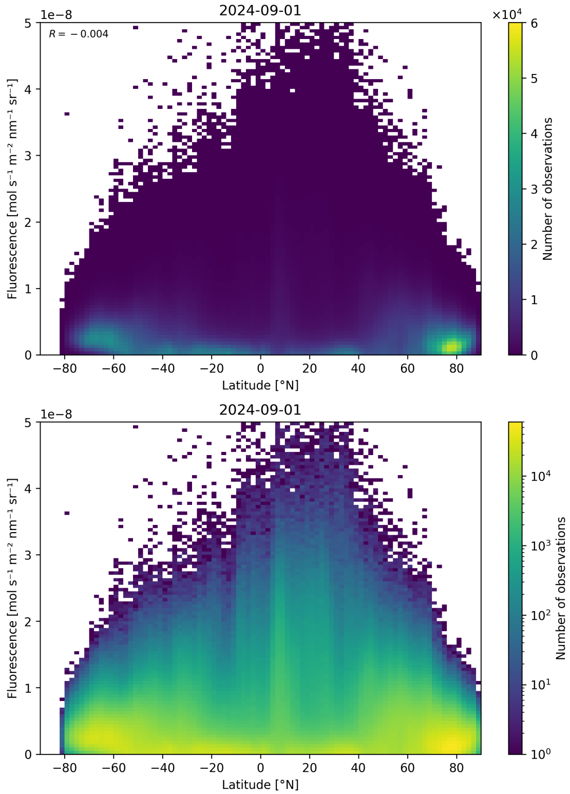
Figure 92: Scatter density plot of “Latitude” against “Fluorescence” for 2024-09-01 to 2024-09-02.
