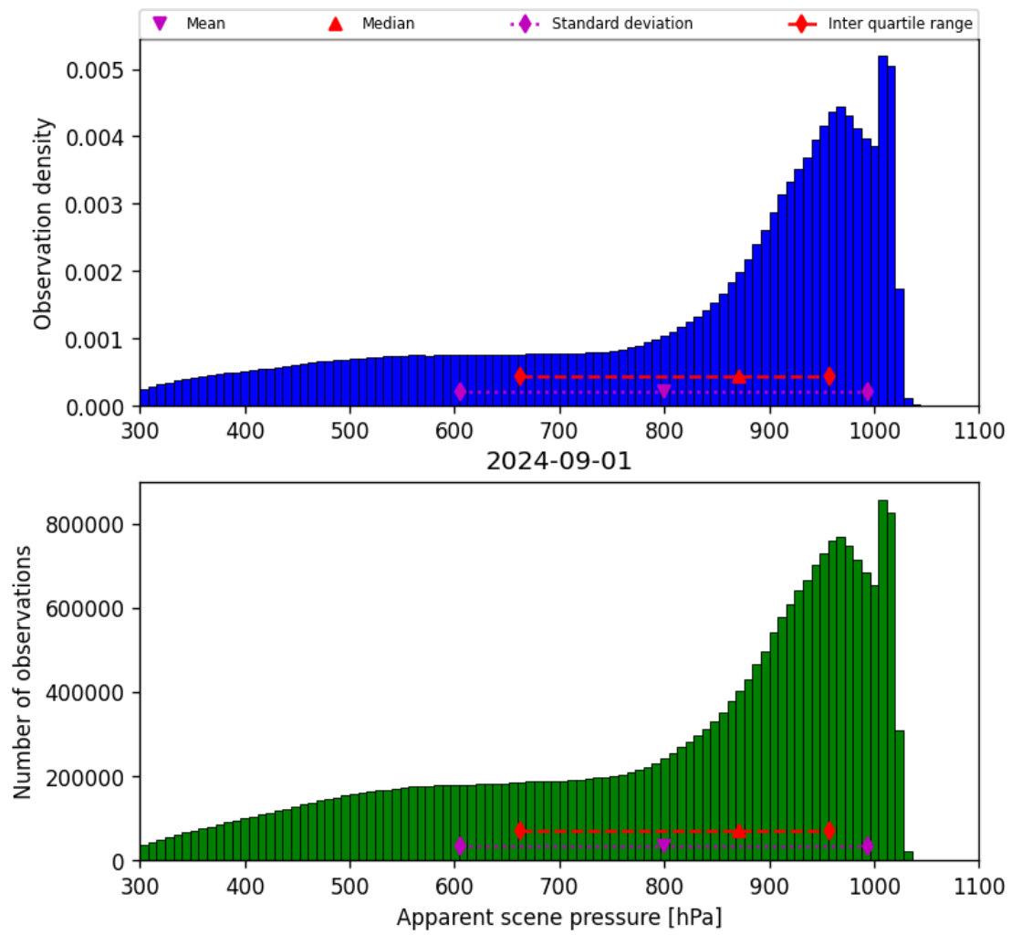
Figure 36: Histogram of “Apparent scene pressure” for 2024-09-01 to 2024-09-02
