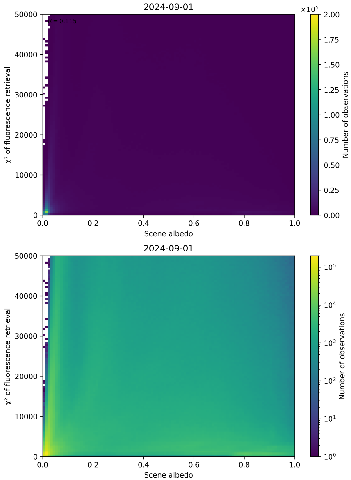
Figure 103: Scatter density plot of “Scene albedo” against “ \chi^2 of fluorescence retrieval” for 2024-09-01 to 2024-09-02.
