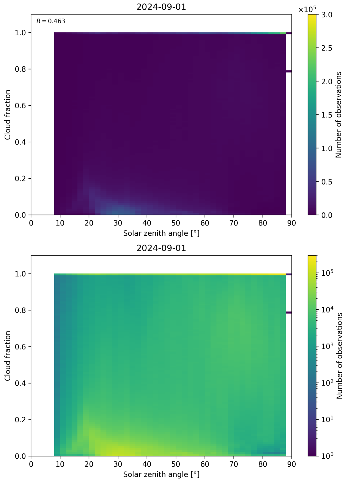
Figure 110: Scatter density plot of “Solar zenith angle” against “Cloud fraction” for 2024-09-01 to 2024-09-02.
