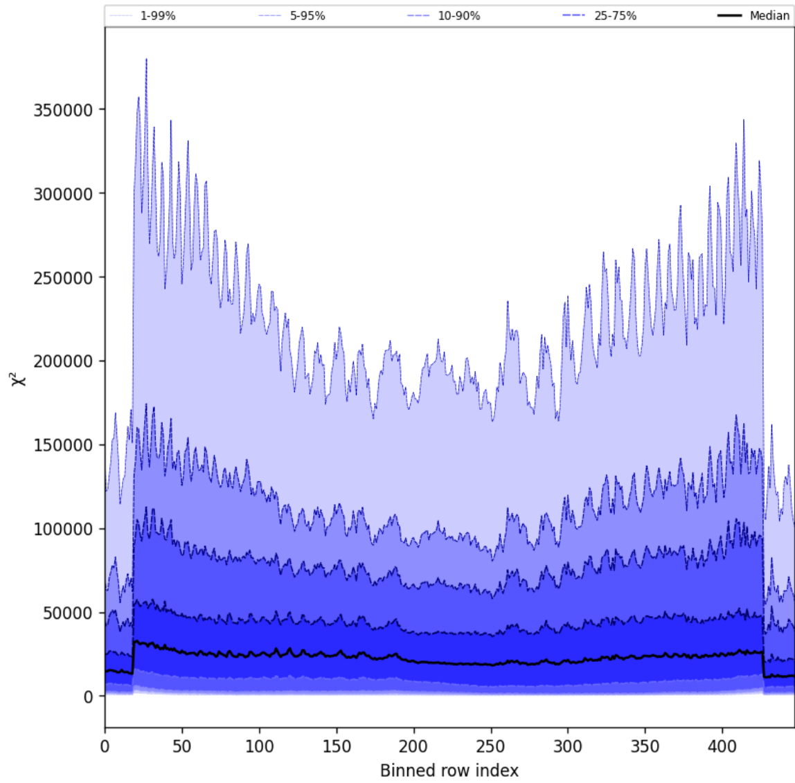
Figure 55: Along track statistics of “ \chi^2 ” for 2024-09-01 to 2024-09-02
