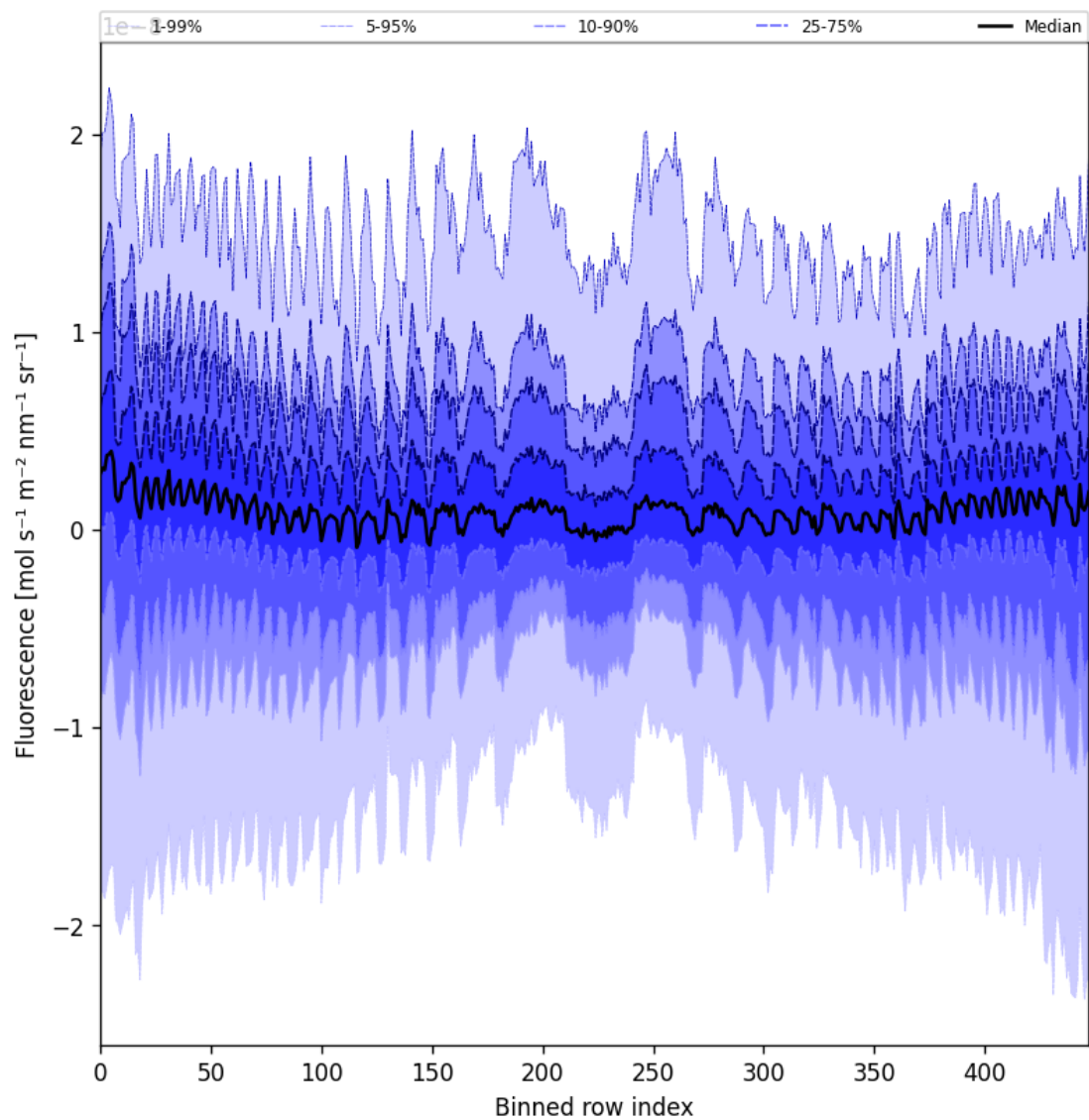
Figure 57: Along track statistics of “Fluorescence” for 2024-09-01 to 2024-09-02
