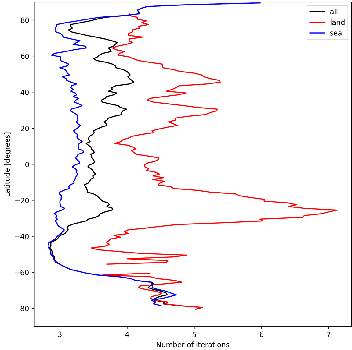
Figure 22: Zonal average of “Number of iterations” for 2024-09-01 to 2024-09-02.
