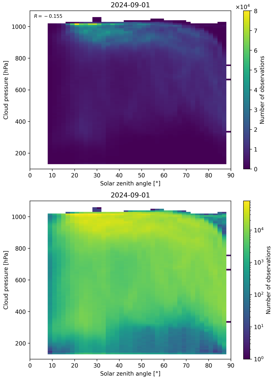
Figure 111: Scatter density plot of “Solar zenith angle” against “Cloud pressure” for 2024-09-01 to 2024-09-02.
