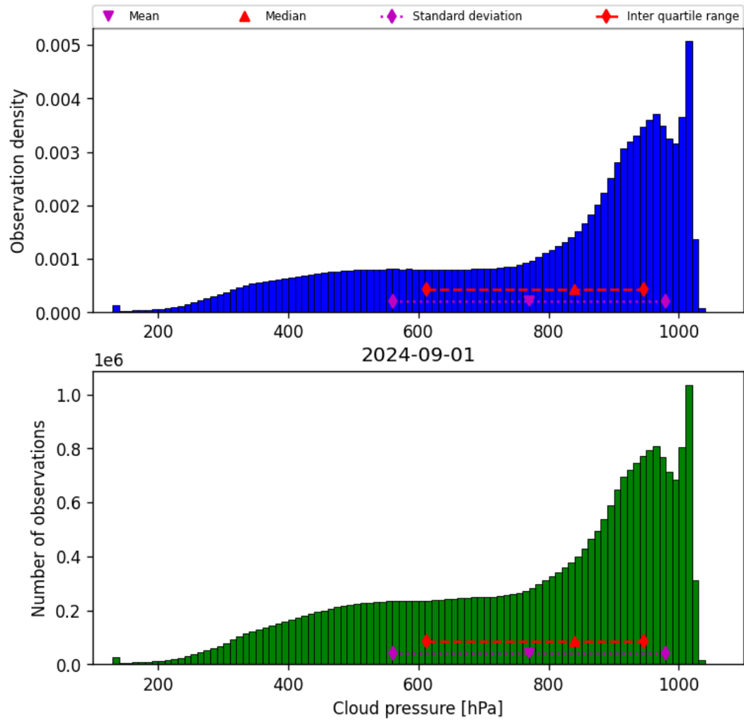
Figure 30: Histogram of “Cloud pressure” for 2024-09-01 to 2024-09-02
