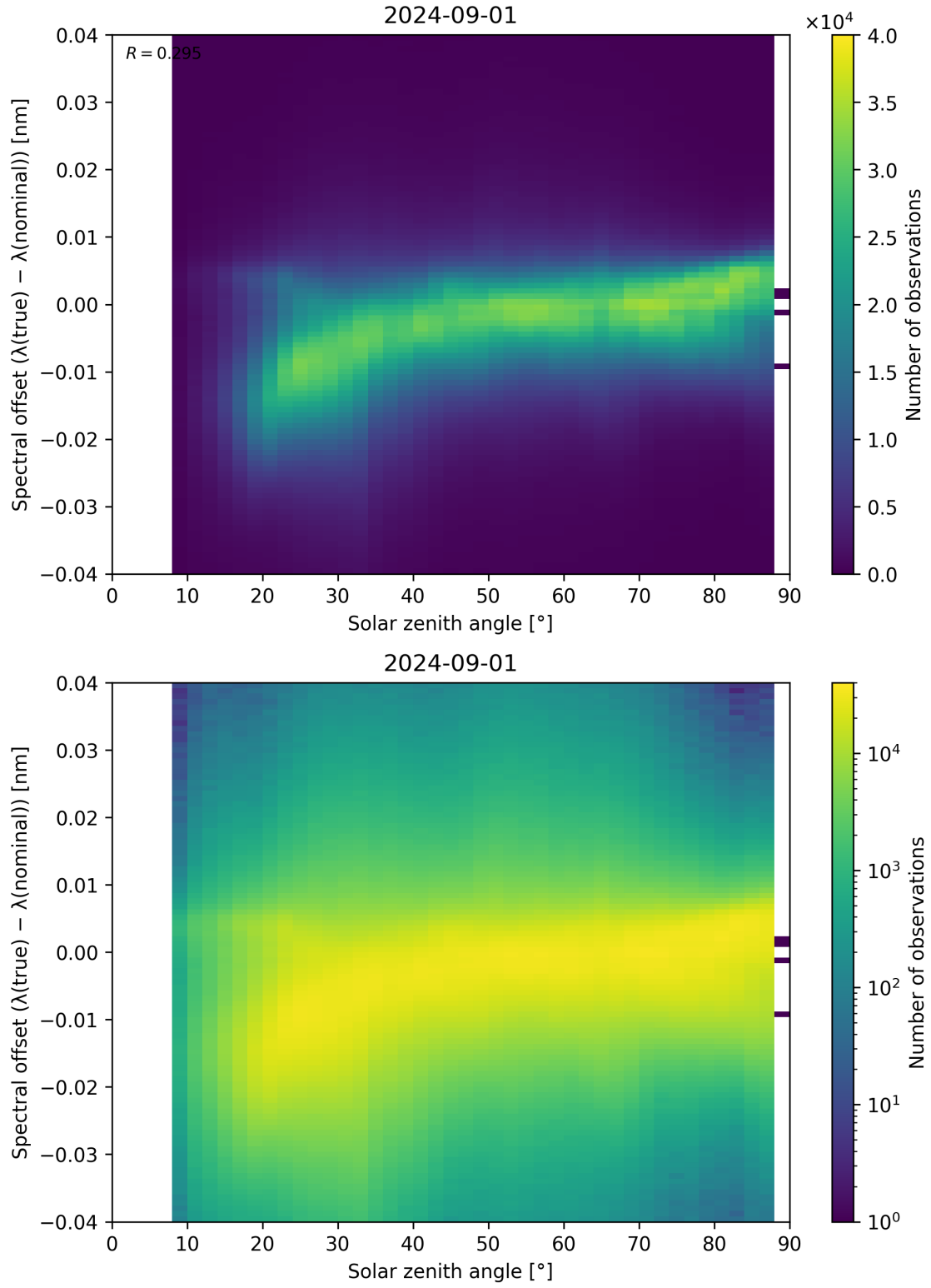
Figure 117: Scatter density plot of “Solar zenith angle” against “Spectral offset ( \lambda_{\text{true}} - \lambda_{\text{nominal}} )” for 2024-09-01 to 2024-09-02.
