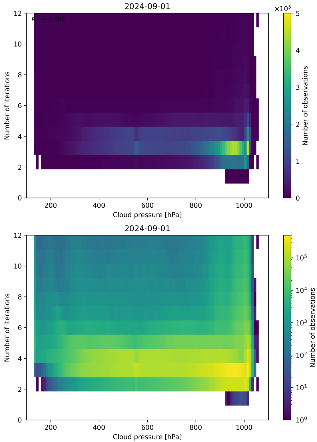
Figure 81: Scatter density plot of “Cloud pressure” against “Number of iterations” for 2024-09-01 to 2024-09-02.
