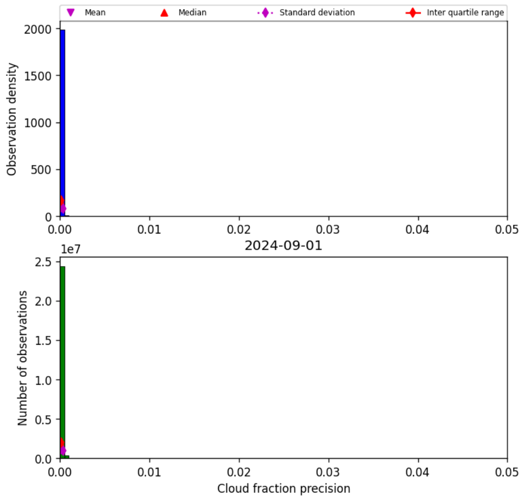
Figure 33: Histogram of “Cloud fraction precision” for 2024-09-01 to 2024-09-02
