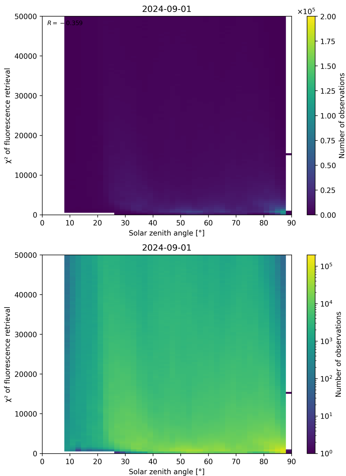
Figure 109: Scatter density plot of “Solar zenith angle” against “ \chi^2 of fluorescence retrieval” for 2024-09-01 to 2024-09-02.
