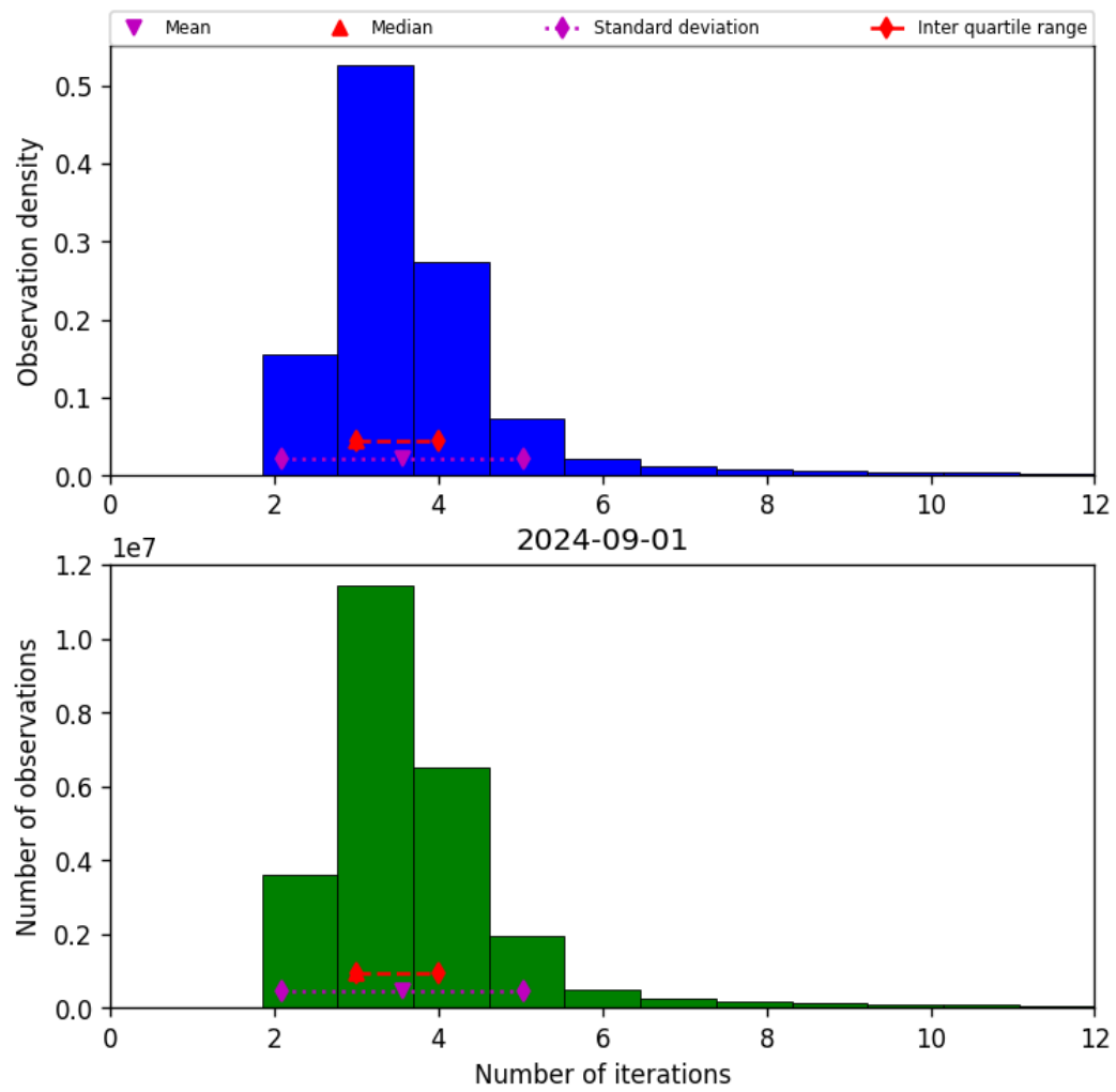
Figure 39: Histogram of “Number of iterations” for 2024-09-01 to 2024-09-02
