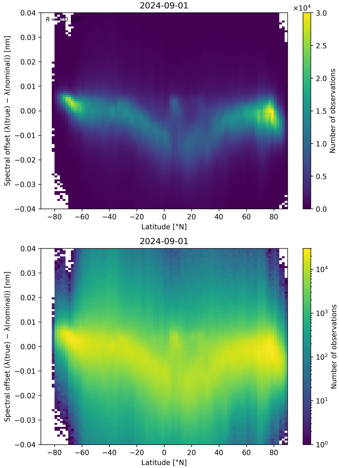
Figure 96: Scatter density plot of “Latitude” against “Spectral offset ( \lambda_{\text{true}} - \lambda_{\text{nominal}} )” for 2024-09-01 to 2024-09-02.
