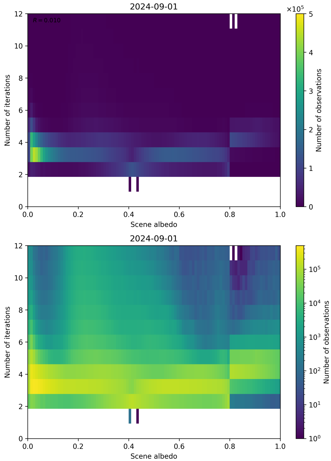
Figure 105: Scatter density plot of “Scene albedo” against “Number of iterations” for 2024-09-01 to 2024-09-02.
