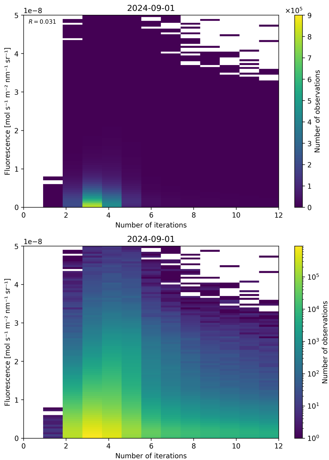
Figure 98: Scatter density plot of “Number of iterations” against “Fluorescence” for 2024-09-01 to 2024-09-02.
