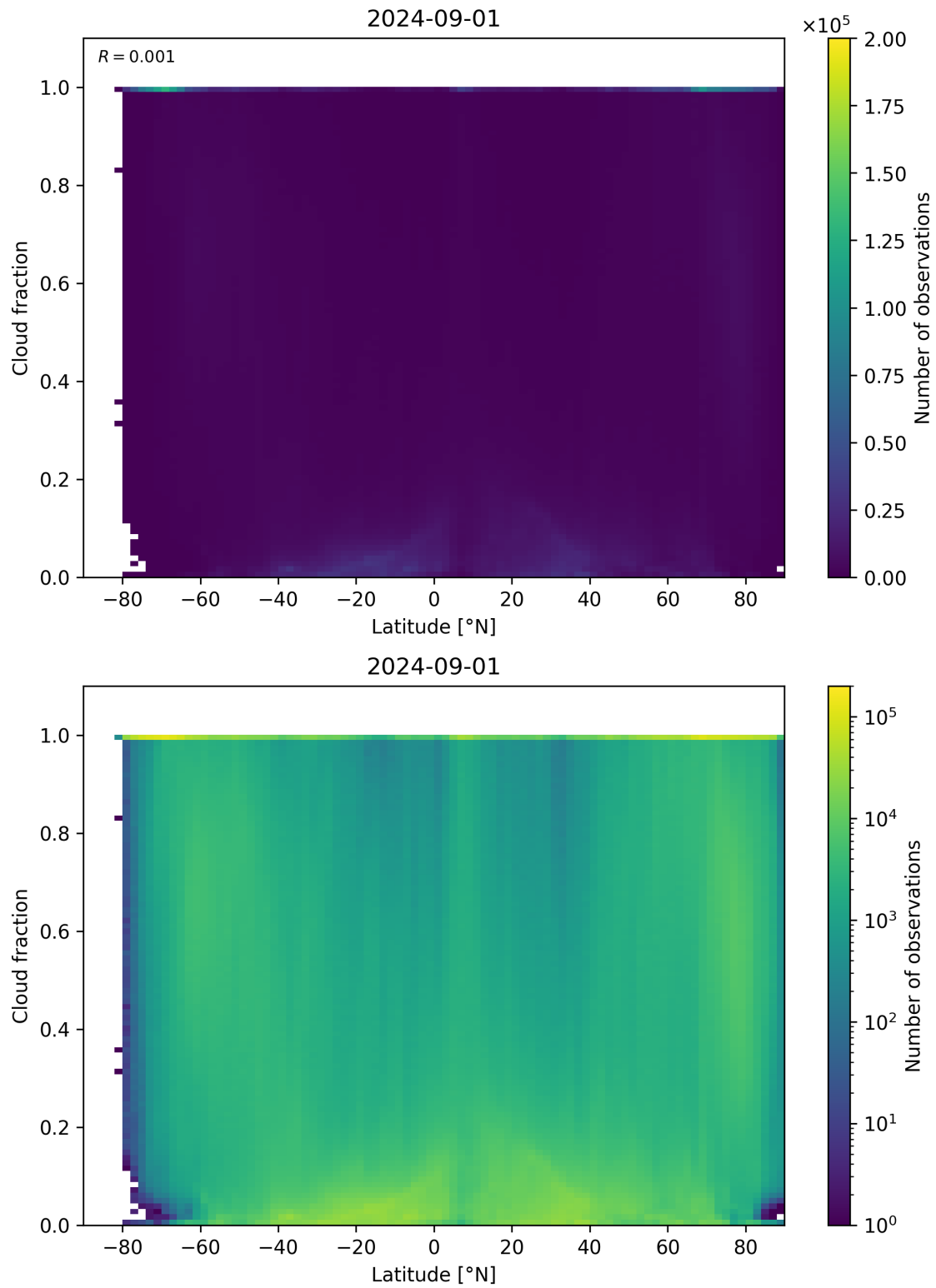
Figure 90: Scatter density plot of “Latitude” against “Cloud fraction” for 2024-09-01 to 2024-09-02.
