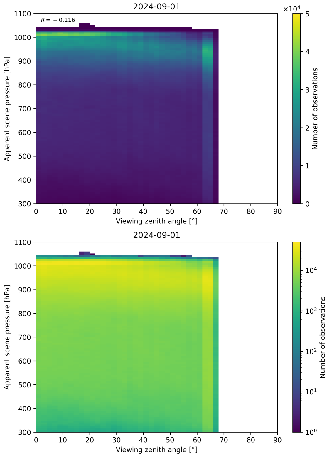
Figure 118: Scatter density plot of “Viewing zenith angle” against “Apparent scene pressure” for 2024-09-01 to 2024-09-02.
