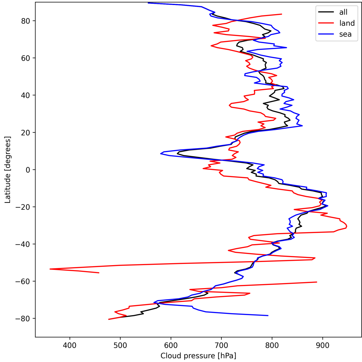
Figure 13: Zonal average of “Cloud pressure” for 2024-09-01 to 2024-09-03.
