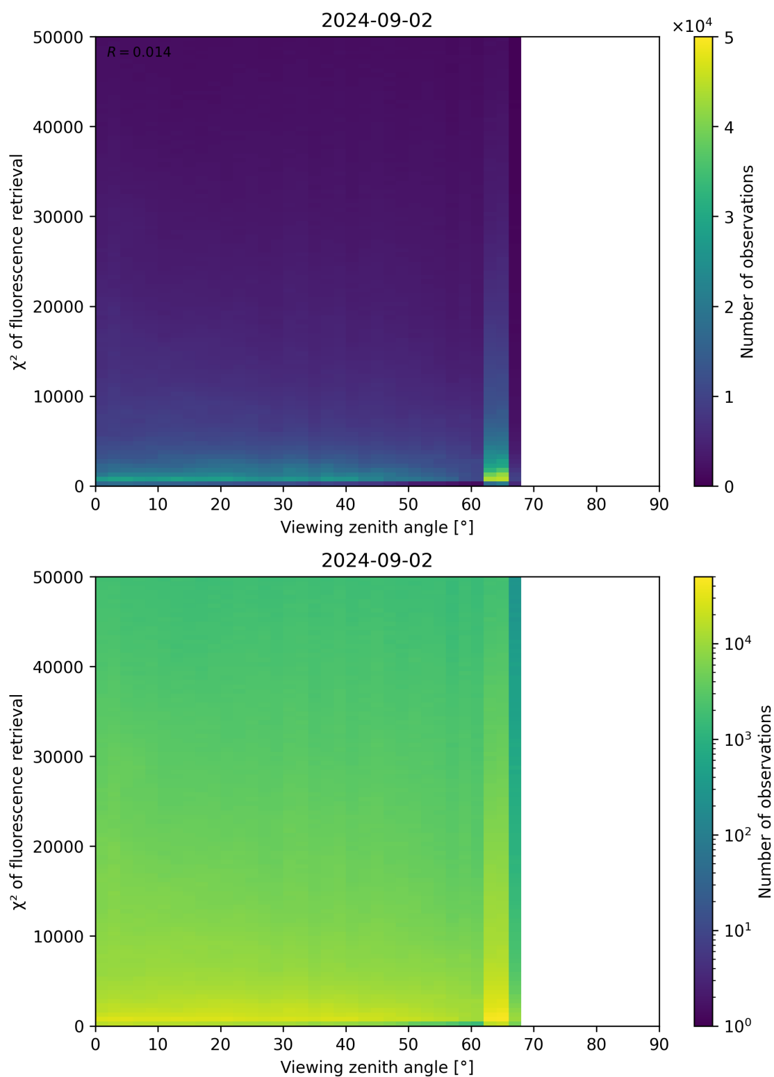
Figure 119: Scatter density plot of “Viewing zenith angle” against “ \chi^2 of fluorescence retrieval” for 2024-09-01 to 2024-09-03.
