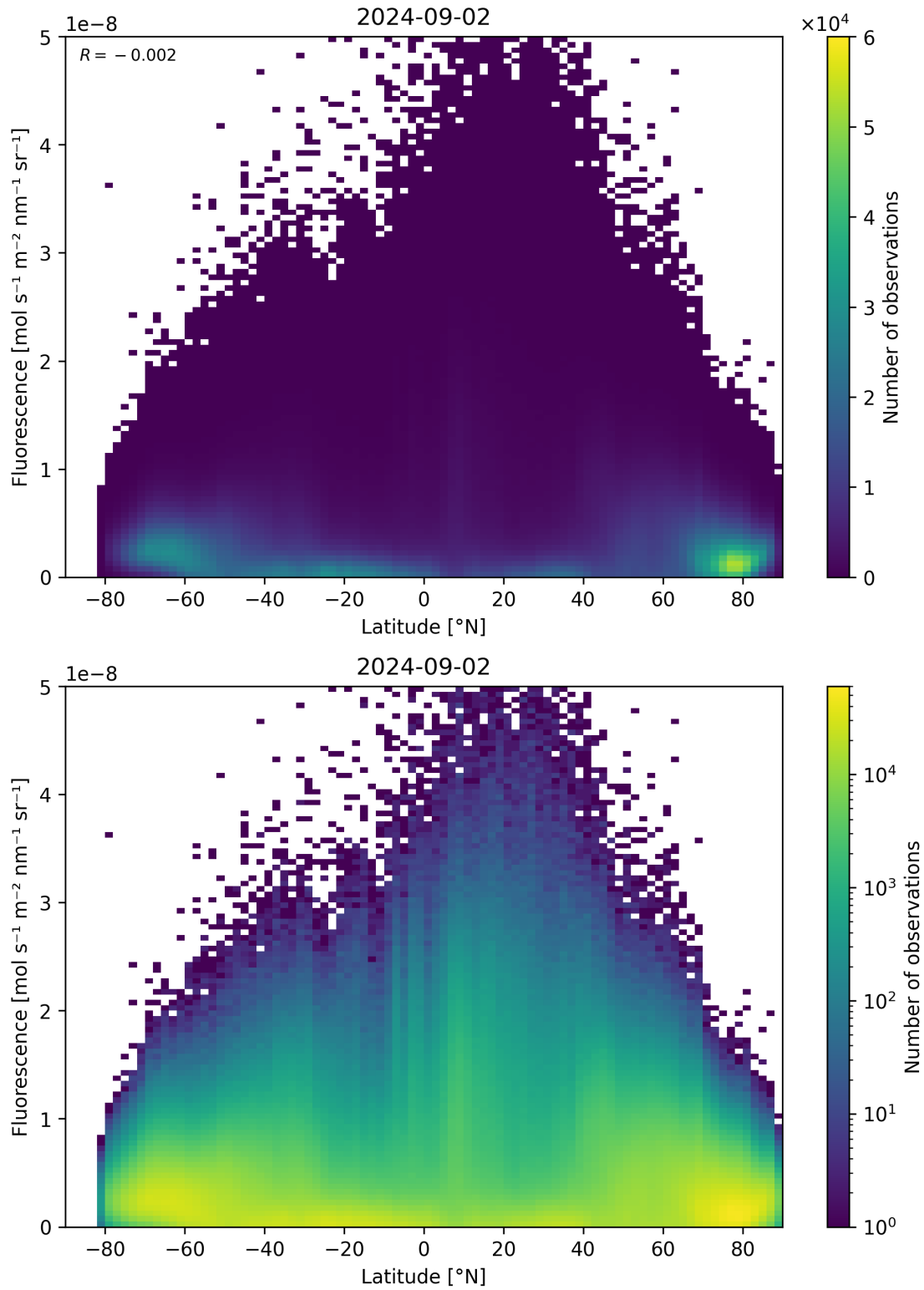
Figure 92: Scatter density plot of “Latitude” against “Fluorescence” for 2024-09-01 to 2024-09-03.
