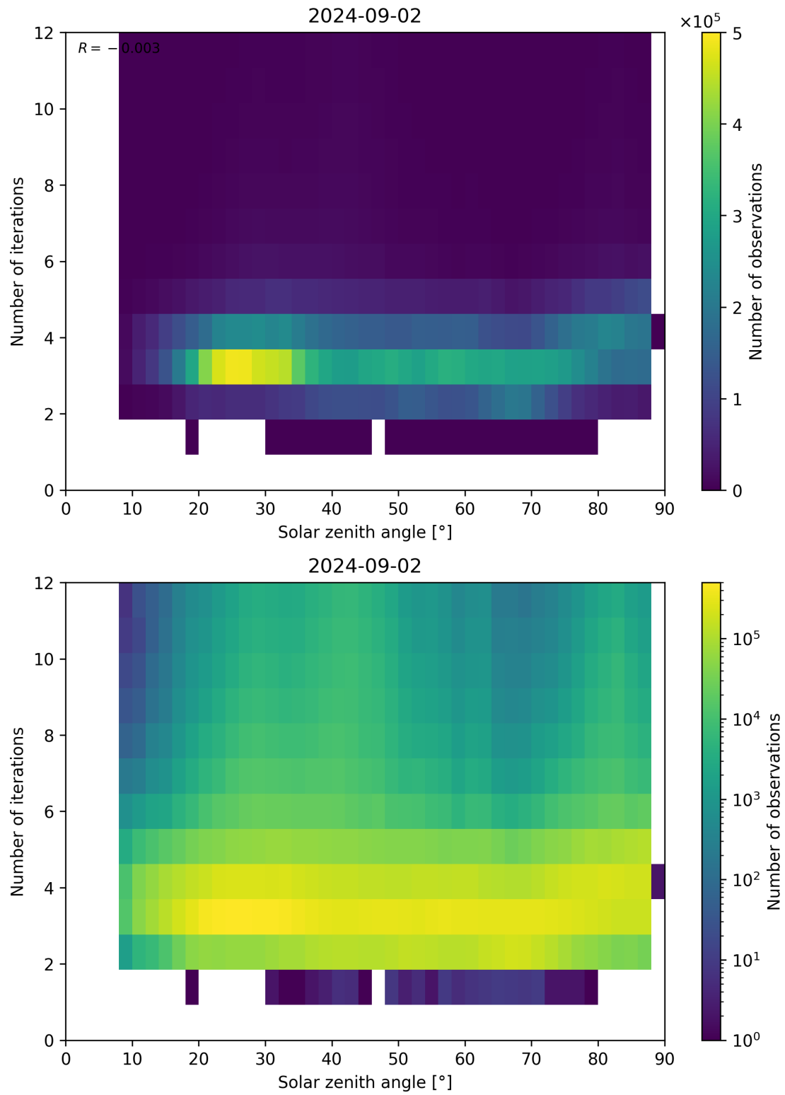
Figure 114: Scatter density plot of “Solar zenith angle” against “Number of iterations” for 2024-09-01 to 2024-09-03.
