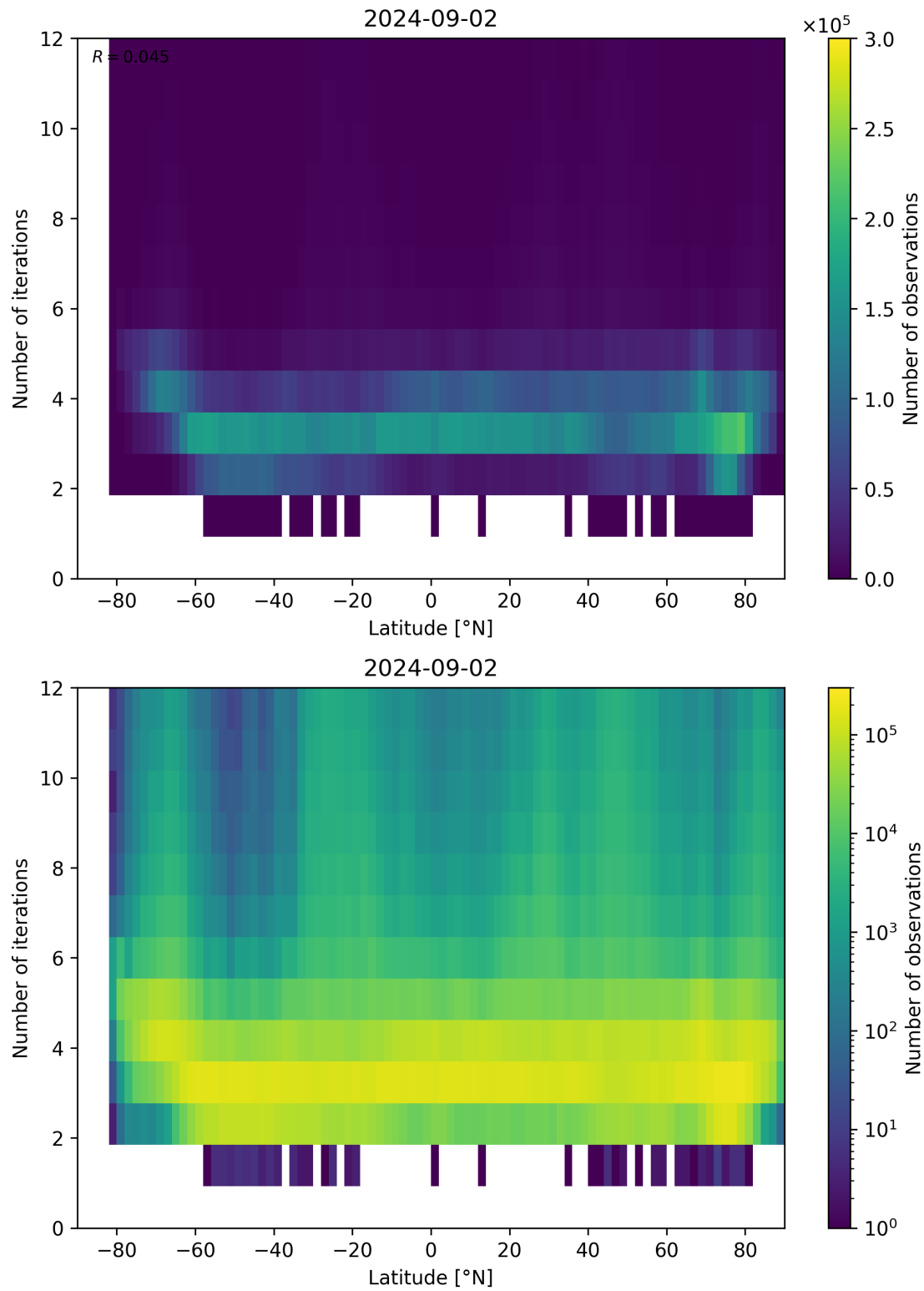
Figure 93: Scatter density plot of “Latitude” against “Number of iterations” for 2024-09-01 to 2024-09-03.
