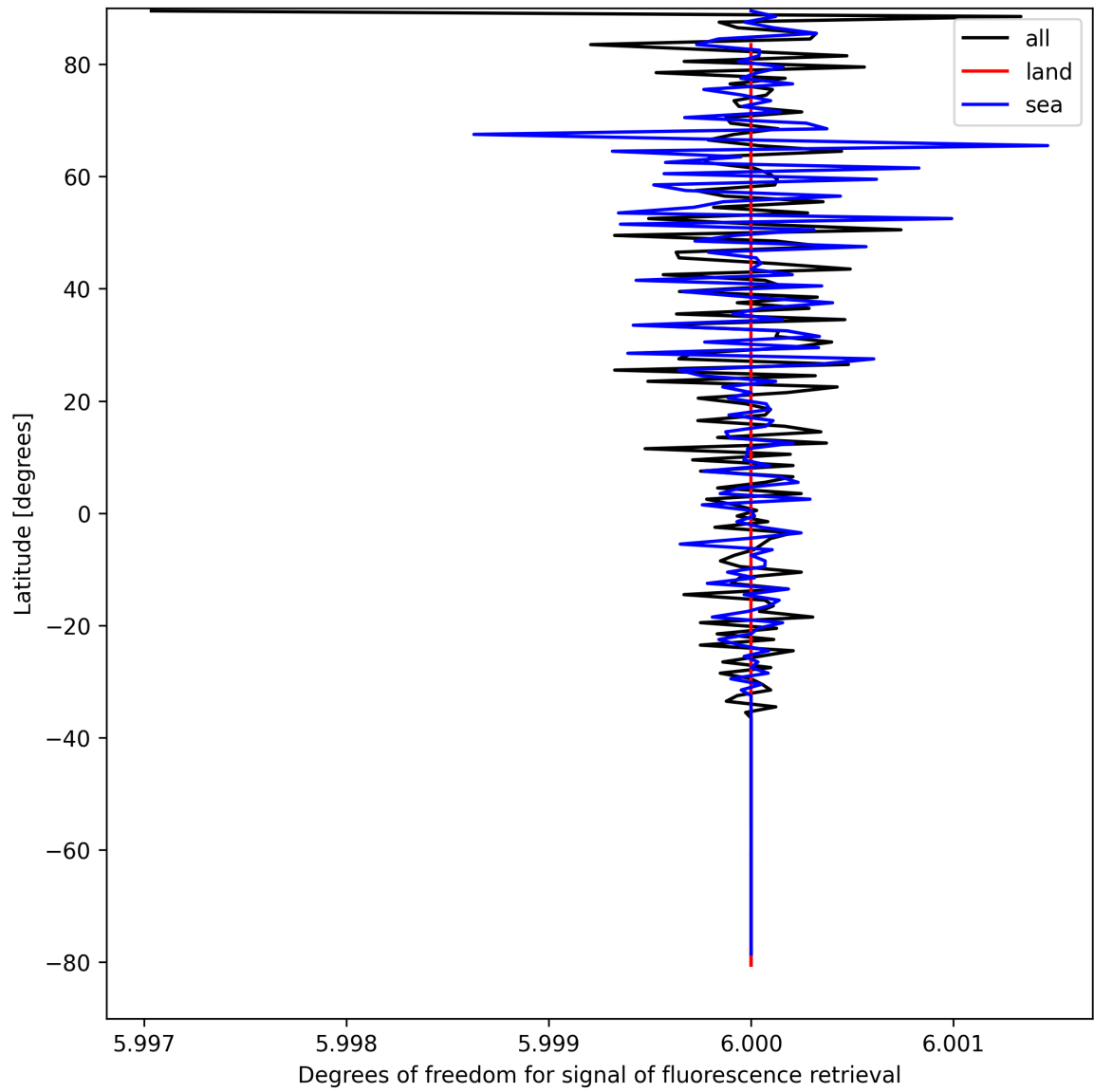
Figure 26: Zonal average of “Degrees of freedom for signal of fluorescence retrieval” for 2024-09-01 to 2024-09-03.
