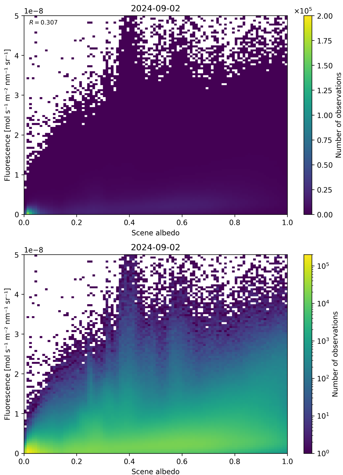
Figure 104: Scatter density plot of “Scene albedo” against “Fluorescence” for 2024-09-01 to 2024-09-03.
