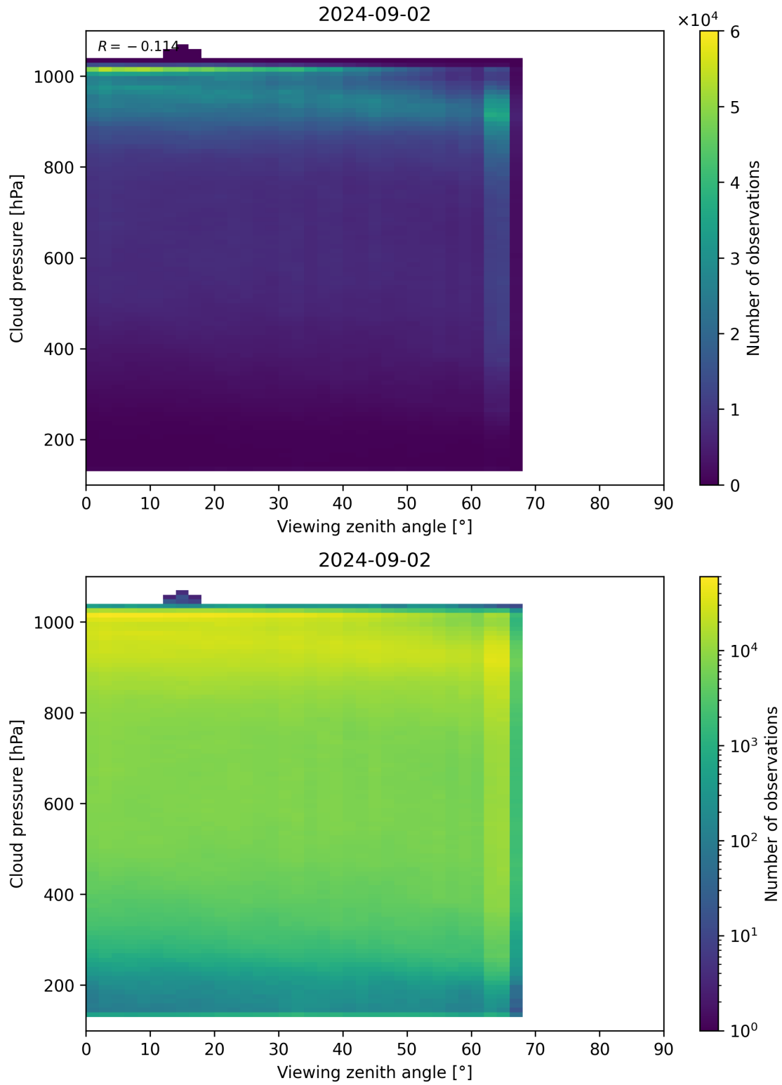
Figure 121: Scatter density plot of “Viewing zenith angle” against “Cloud pressure” for 2024-09-01 to 2024-09-03.
