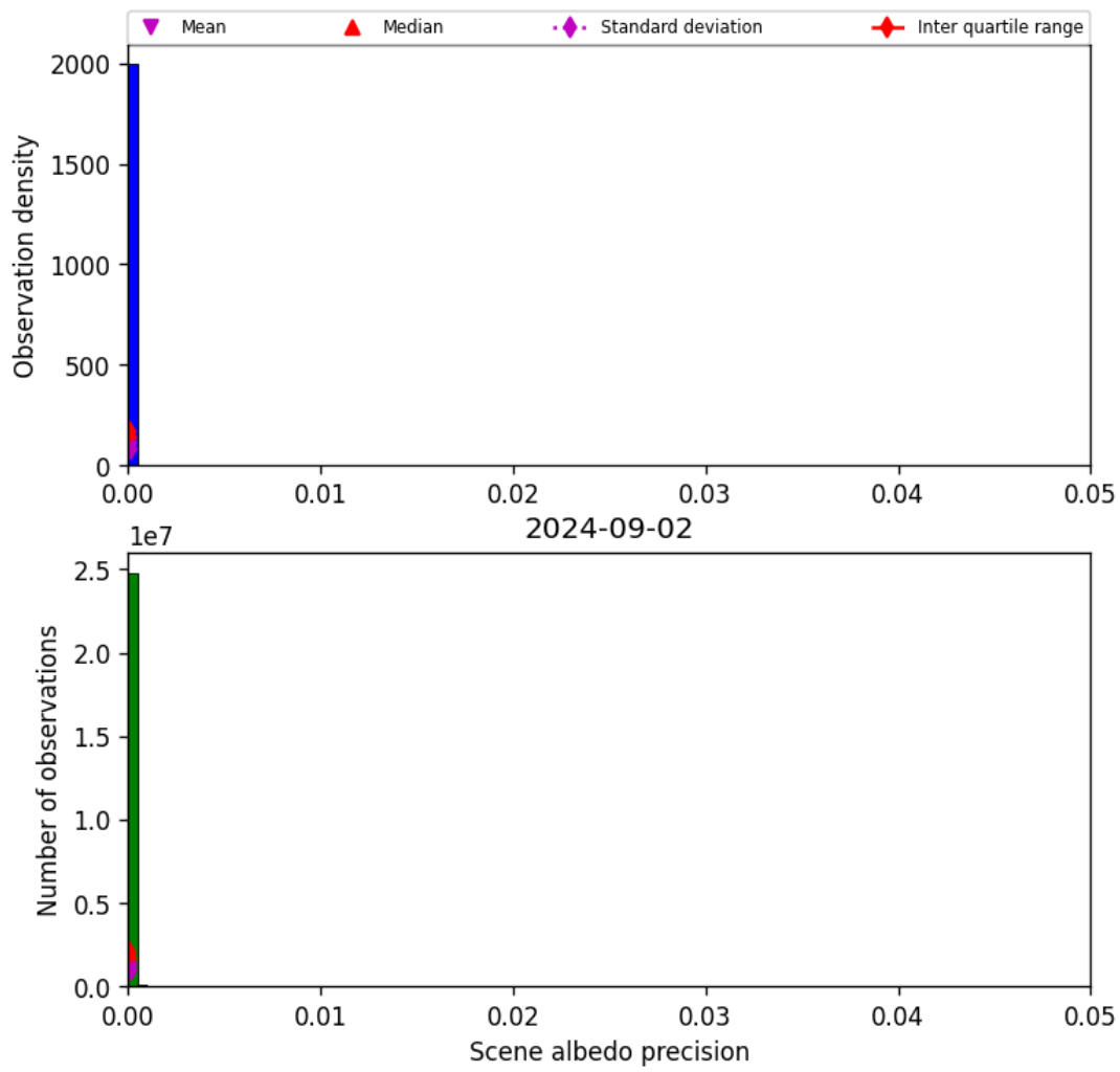
Figure 35: Histogram of “Scene albedo precision” for 2024-09-01 to 2024-09-03
