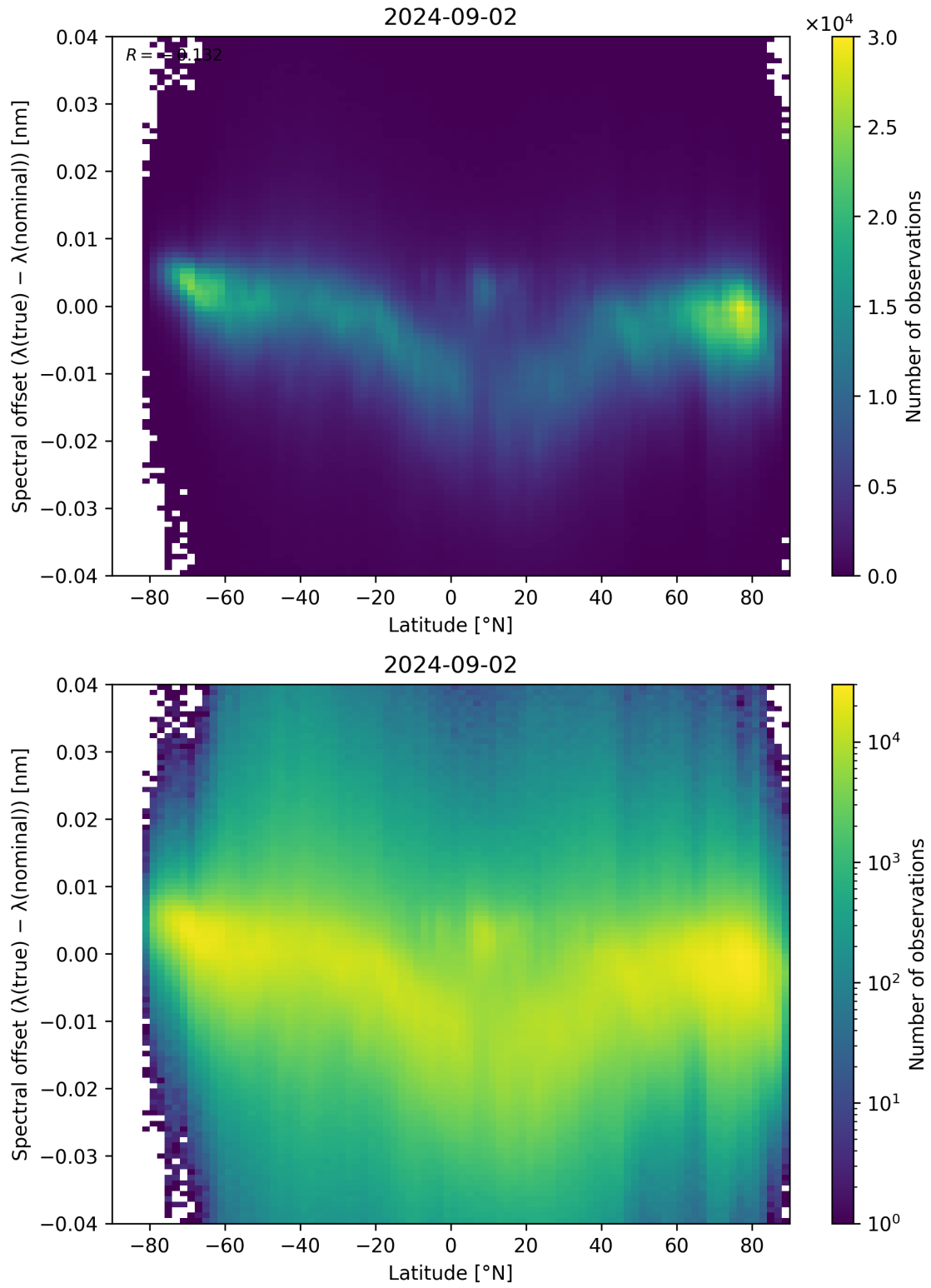
Figure 96: Scatter density plot of “Latitude” against “Spectral offset ( \lambda_{\text{true}} - \lambda_{\text{nominal}} )” for 2024-09-01 to 2024-09-03.
