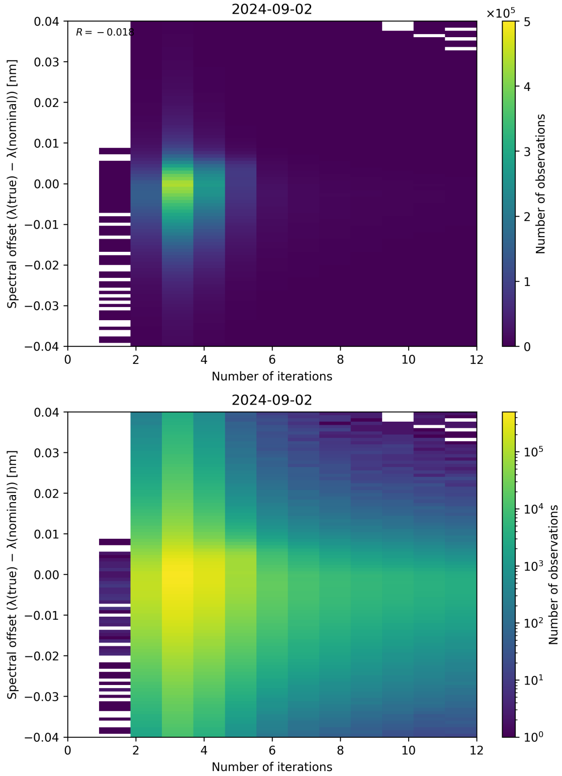
Figure 100: Scatter density plot of “Number of iterations” against “Spectral offset ( \lambda_{\text{true}} - \lambda_{\text{nominal}} )” for 2024-09-01 to 2024-09-03.
