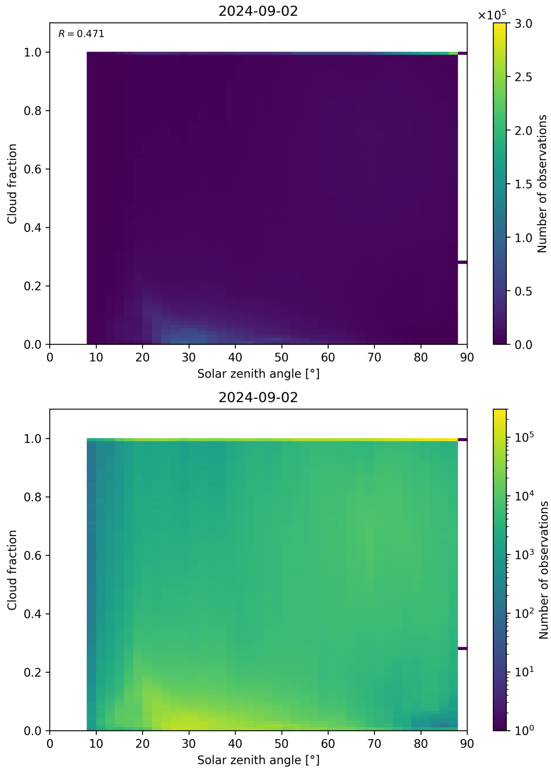
Figure 110: Scatter density plot of “Solar zenith angle” against “Cloud fraction” for 2024-09-01 to 2024-09-03.
