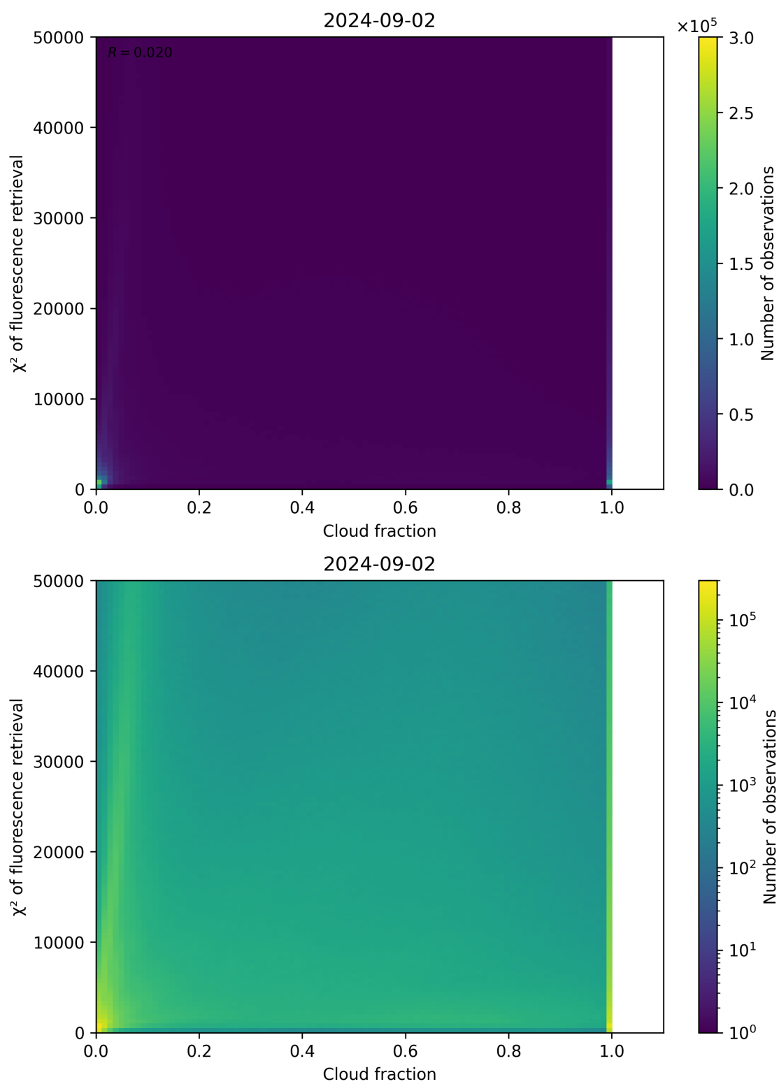
Figure 71: Scatter density plot of “Cloud fraction” against “ \chi^2 of fluorescence retrieval” for 2024-09-01 to 2024-09-03.
