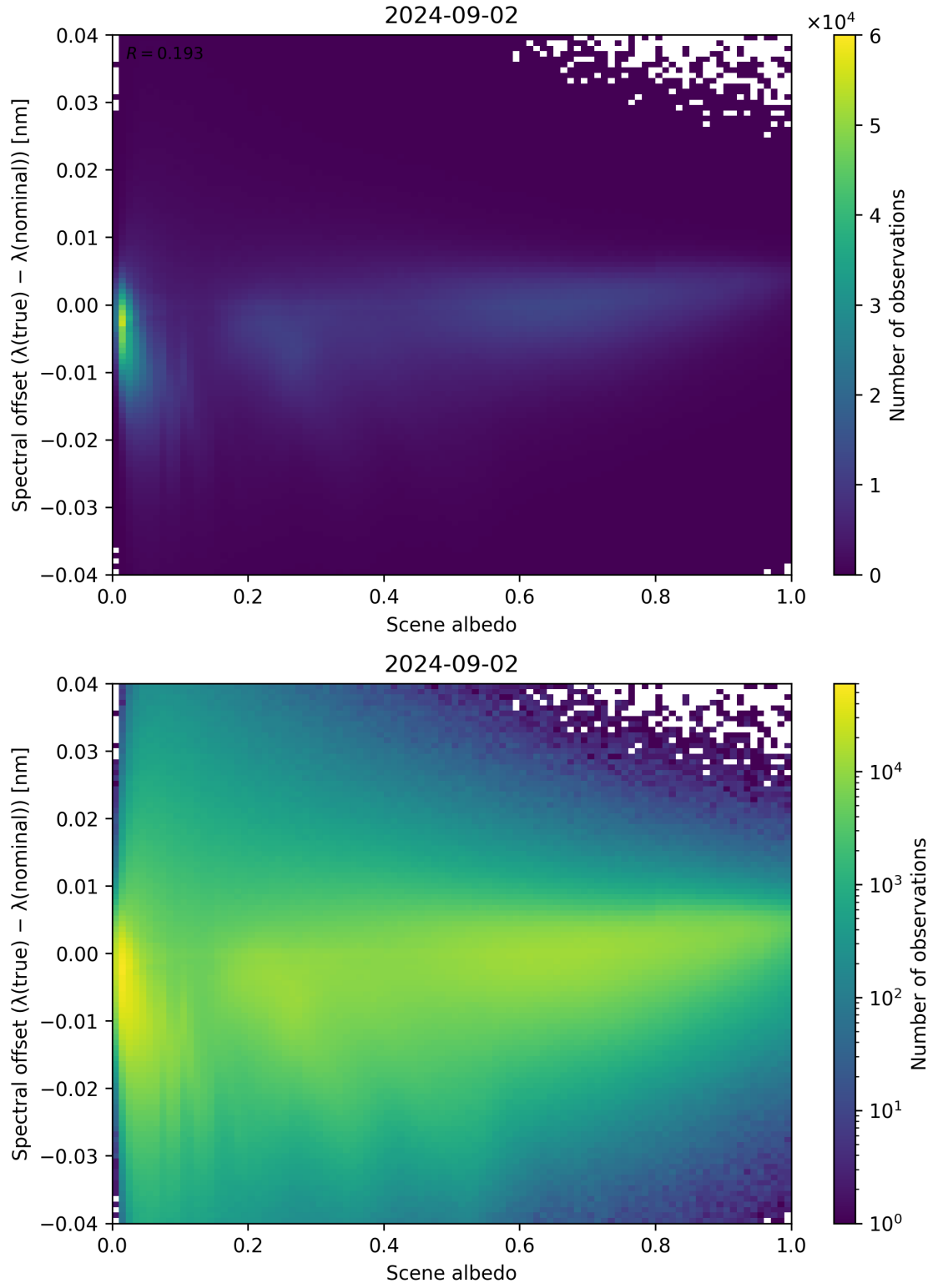
Figure 107: Scatter density plot of “Scene albedo” against “Spectral offset ( \lambda_{\text{true}} - \lambda_{\text{nominal}} )” for 2024-09-01 to 2024-09-03.
