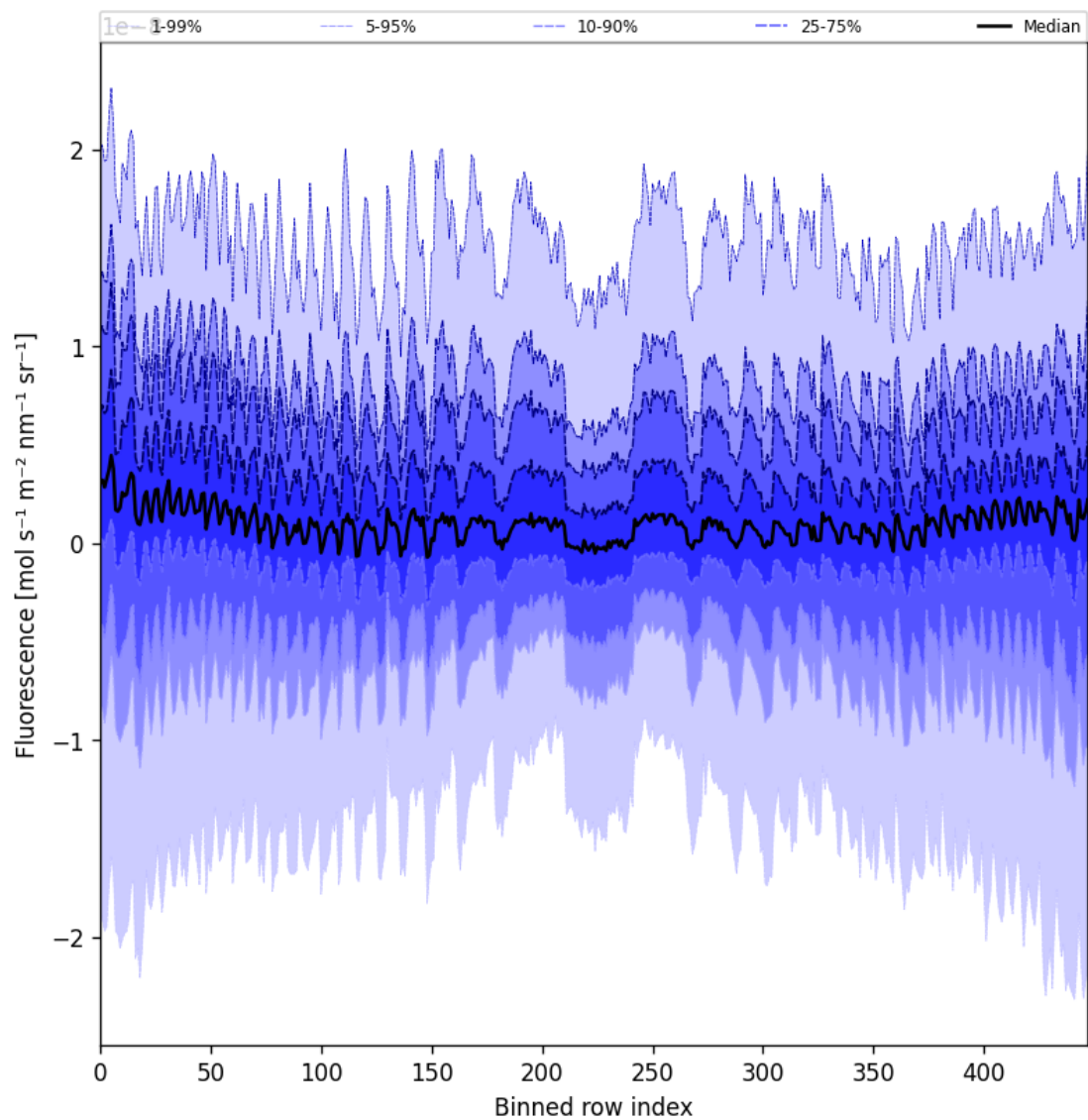
Figure 57: Along track statistics of “Fluorescence” for 2024-09-01 to 2024-09-03
