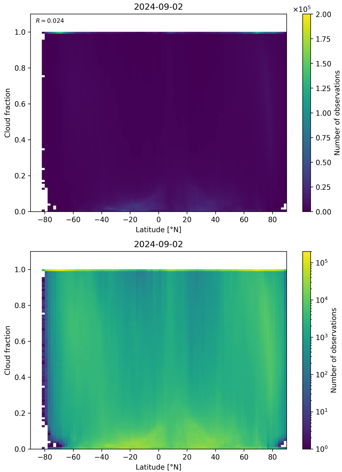
Figure 90: Scatter density plot of “Latitude” against “Cloud fraction” for 2024-09-01 to 2024-09-03.
