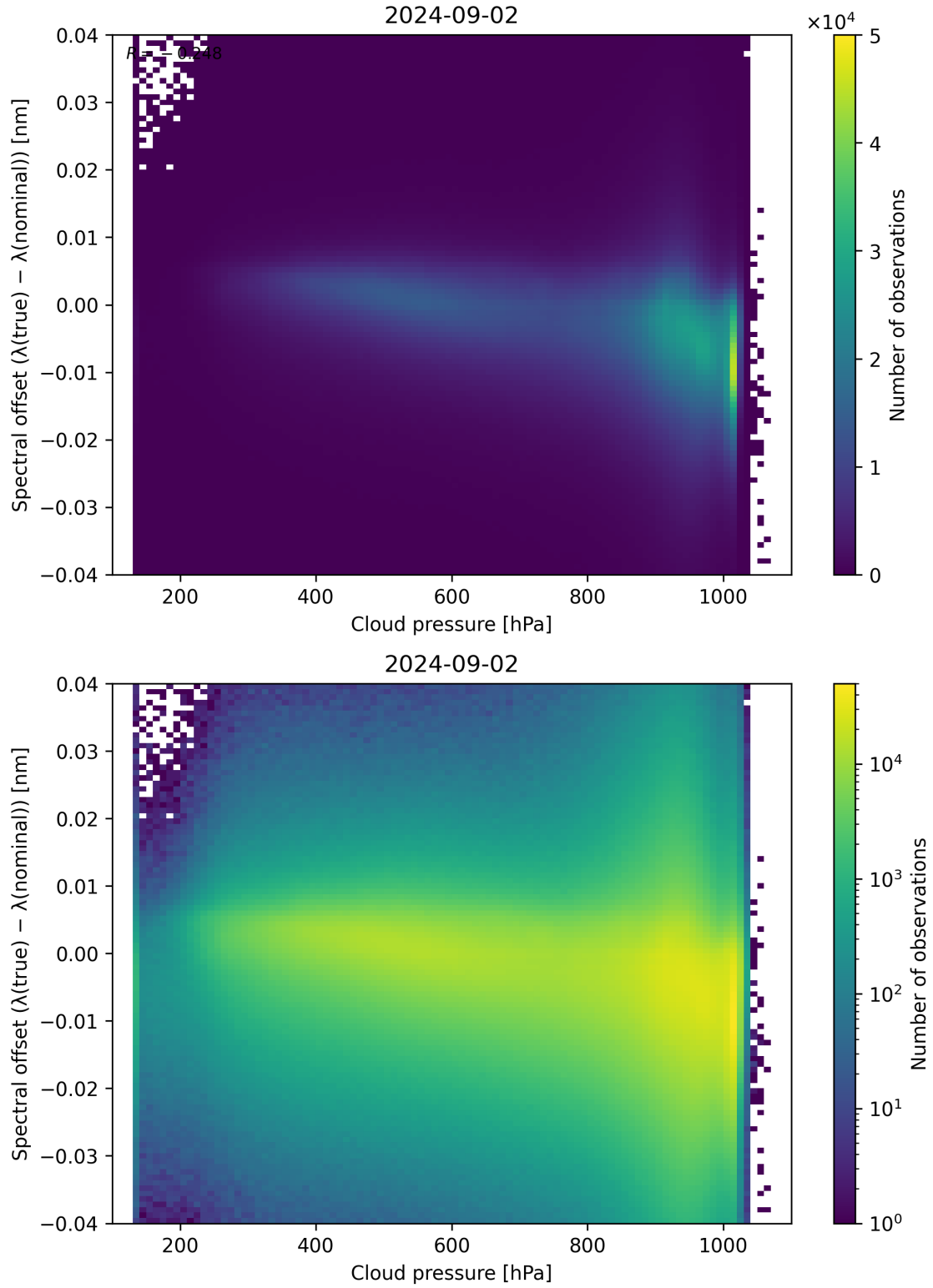
Figure 84: Scatter density plot of “Cloud pressure” against “Spectral offset ( \lambda_{\text{true}} - \lambda_{\text{nominal}} )” for 2024-09-01 to 2024-09-03.
