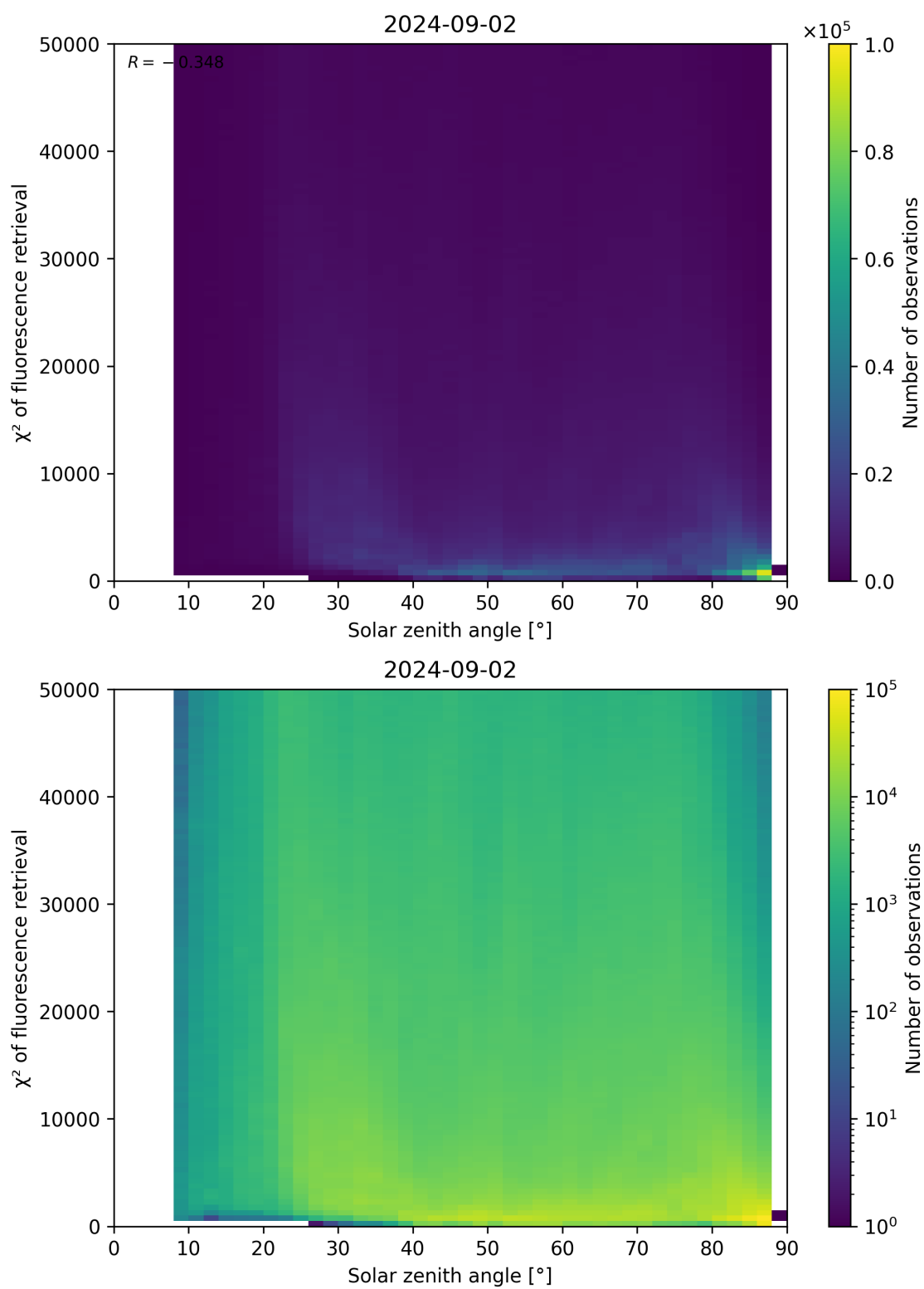
Figure 109: Scatter density plot of “Solar zenith angle” against “ \chi^2 of fluorescence retrieval” for 2024-09-01 to 2024-09-03.
