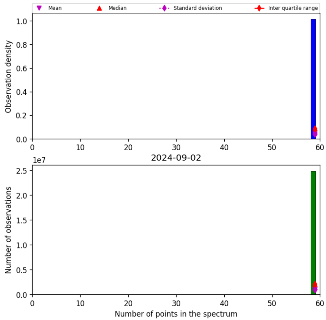
Figure 44: Histogram of "Number of points in the spectrum" for 2024-09-01 to 2024-09-03
