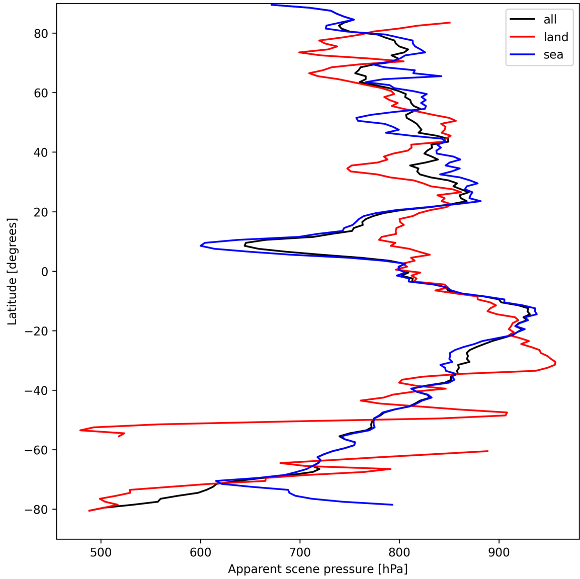
Figure 19: Zonal average of “Apparent scene pressure” for 2024-09-01 to 2024-09-03.
