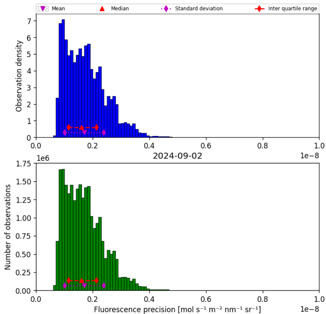
Figure 41: Histogram of “Fluorescence precision” for 2024-09-01 to 2024-09-03
