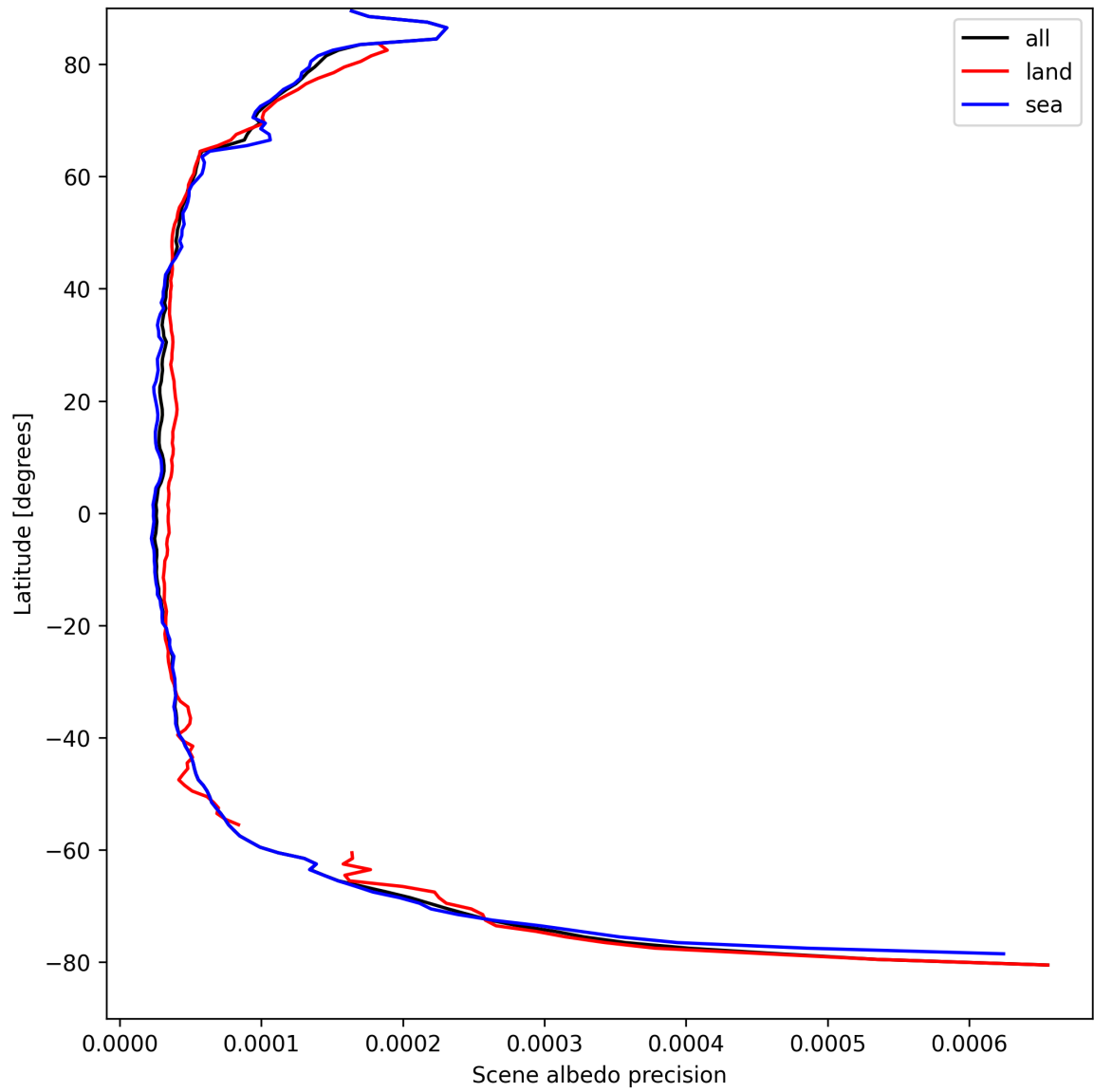
Figure 18: Zonal average of “Scene albedo precision” for 2024-09-01 to 2024-09-03.
