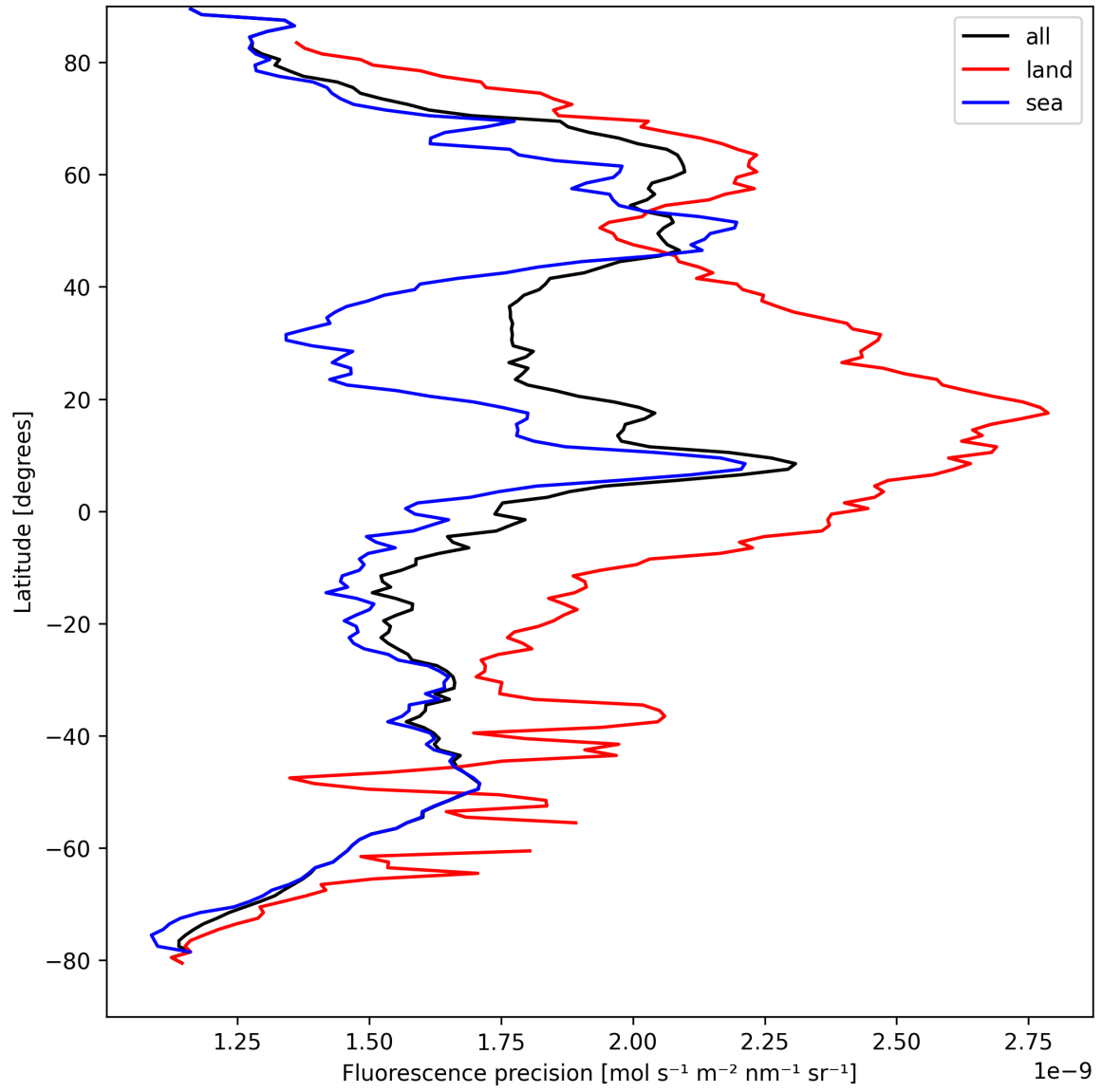
Figure 24: Zonal average of “Fluorescence precision” for 2024-09-01 to 2024-09-03.
