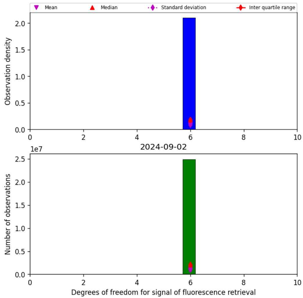
Figure 43: Histogram of "Degrees of freedom for signal of fluorescence retrieval" for 2024-09-01 to 2024-09-03
