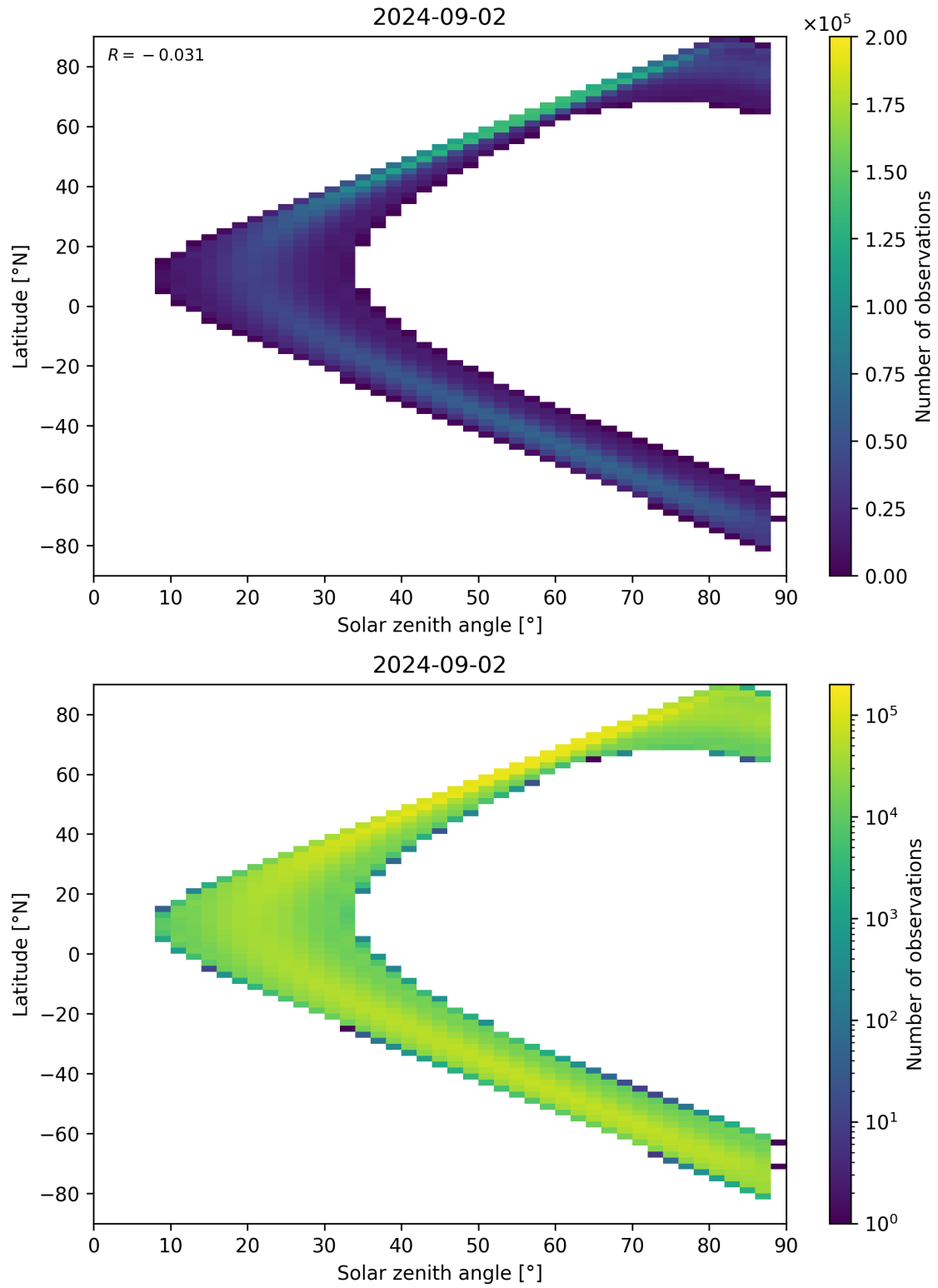
Figure 113: Scatter density plot of “Solar zenith angle” against “Latitude” for 2024-09-01 to 2024-09-03.
