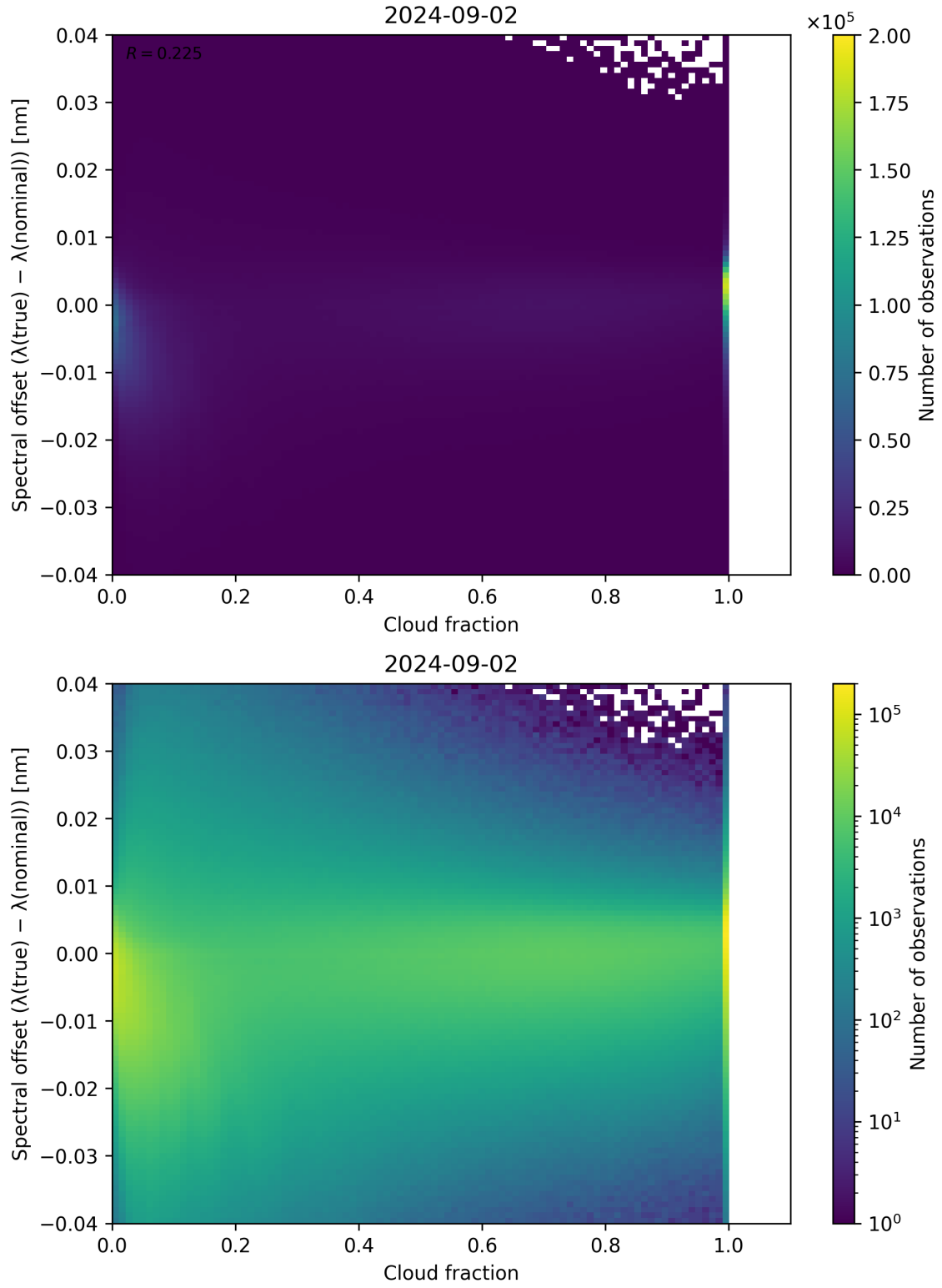
Figure 76: Scatter density plot of “Cloud fraction” against “Spectral offset ( \lambda_{\text{true}} - \lambda_{\text{nominal}} )” for 2024-09-01 to 2024-09-03.
