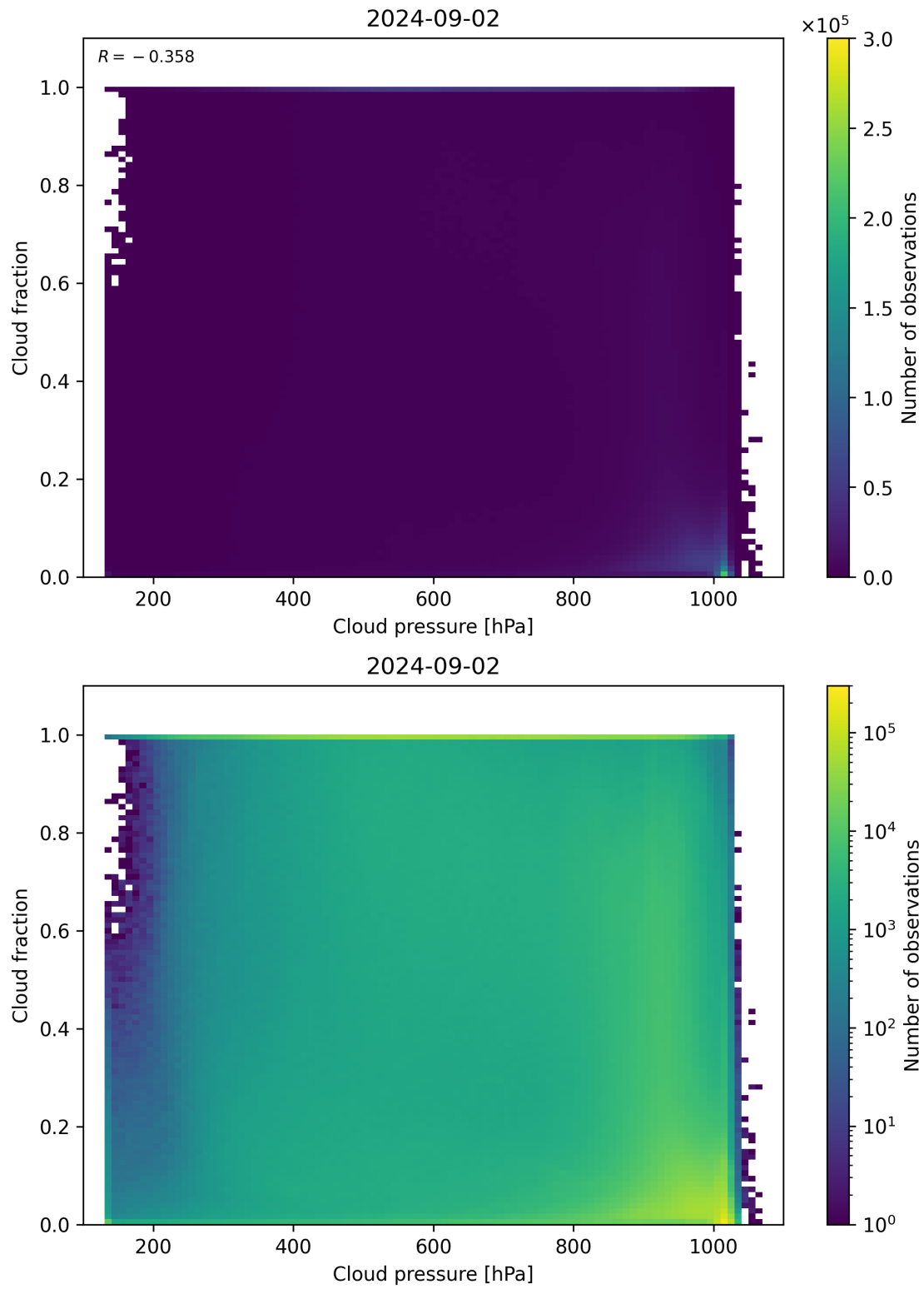
Figure 79: Scatter density plot of “Cloud pressure” against “Cloud fraction” for 2024-09-01 to 2024-09-03.
