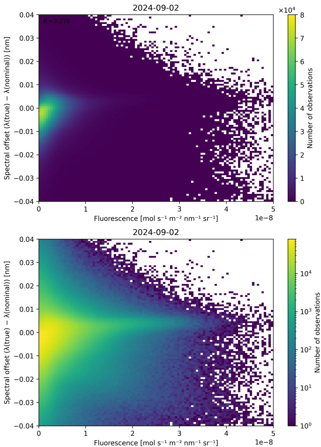
Figure 87: Scatter density plot of “Fluorescence” against “Spectral offset ( \lambda_{\text{true}} - \lambda_{\text{nominal}} )” for 2024-09-01 to 2024-09-03.
