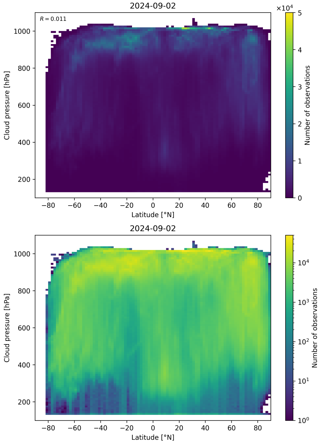
Figure 91: Scatter density plot of “Latitude” against “Cloud pressure” for 2024-09-01 to 2024-09-03.
