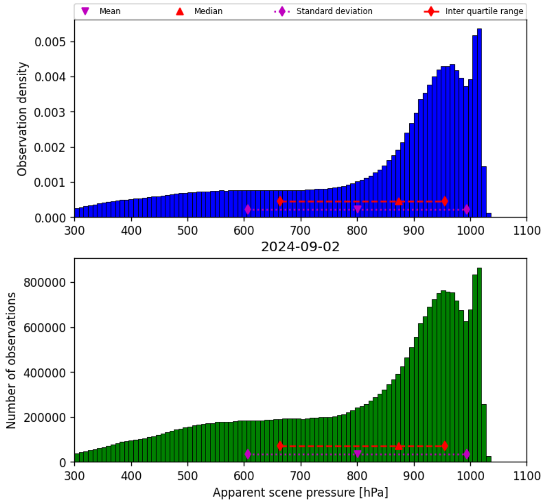
Figure 36: Histogram of “Apparent scene pressure” for 2024-09-01 to 2024-09-03
