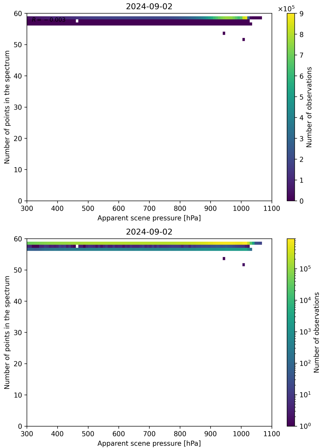
Figure 66: Scatter density plot of “Apparent scene pressure” against “Number of points in the spectrum” for 2024-09-01 to 2024-09-03.
