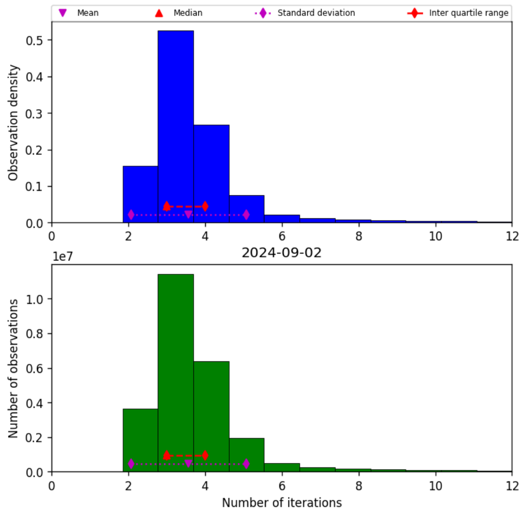
Figure 39: Histogram of “Number of iterations” for 2024-09-01 to 2024-09-03
