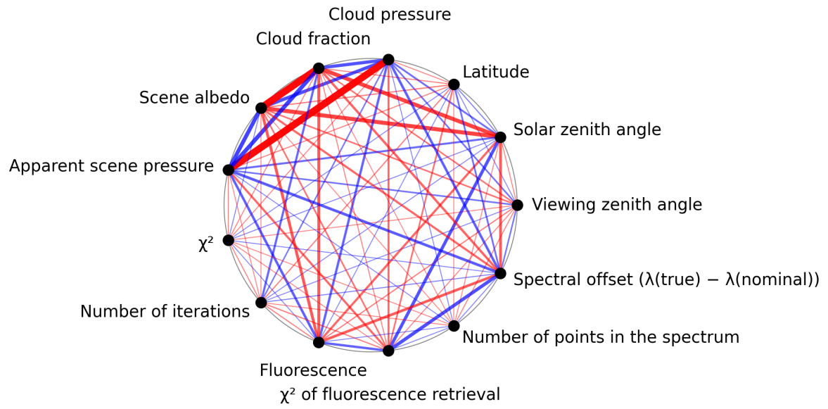
Figure 1: Map of correlation graph for 2024-09-01 to 2024-09-03.
