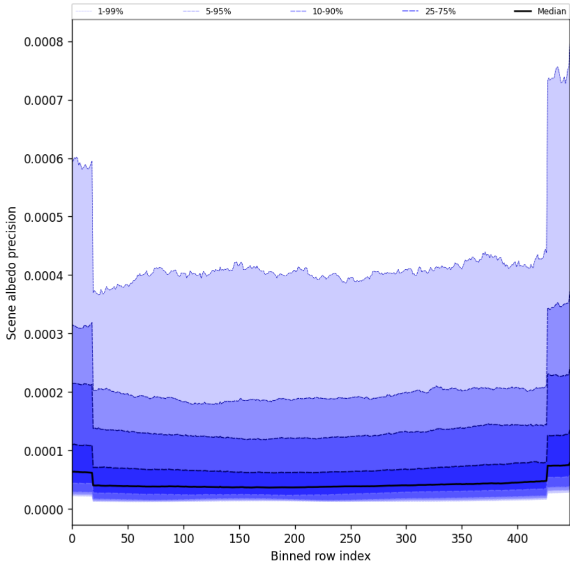
Figure 52: Along track statistics of “Scene albedo precision” for 2024-09-01 to 2024-09-03
