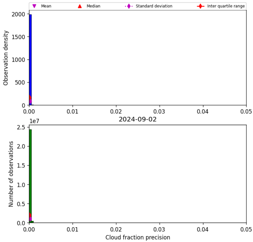
Figure 33: Histogram of “Cloud fraction precision” for 2024-09-01 to 2024-09-03
