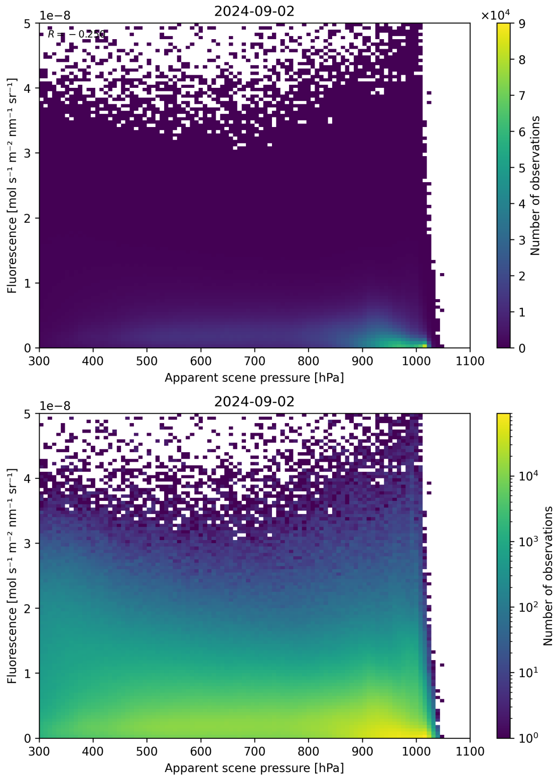
Figure 64: Scatter density plot of “Apparent scene pressure” against “Fluorescence” for 2024-09-01 to 2024-09-03.
