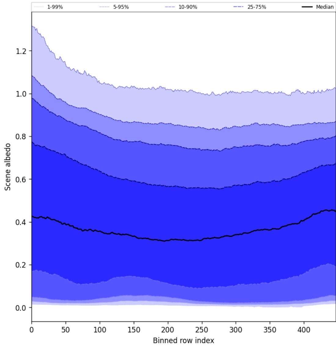
Figure 51: Along track statistics of “Scene albedo” for 2024-09-01 to 2024-09-03
