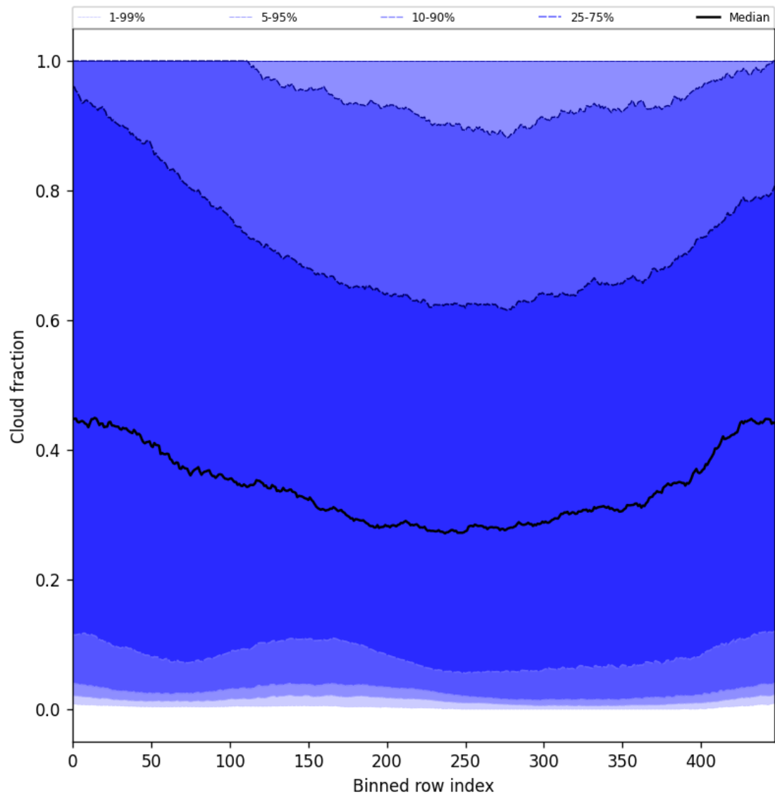
Figure 49: Along track statistics of “Cloud fraction” for 2024-09-01 to 2024-09-03
