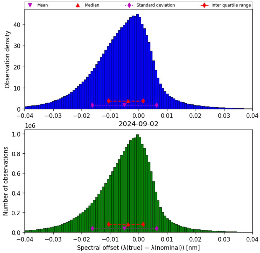
Figure 45: Histogram of “Spectral offset ( \lambda_{\text{true}} - \lambda_{\text{nominal}} )” for 2024-09-01 to 2024-09-03
