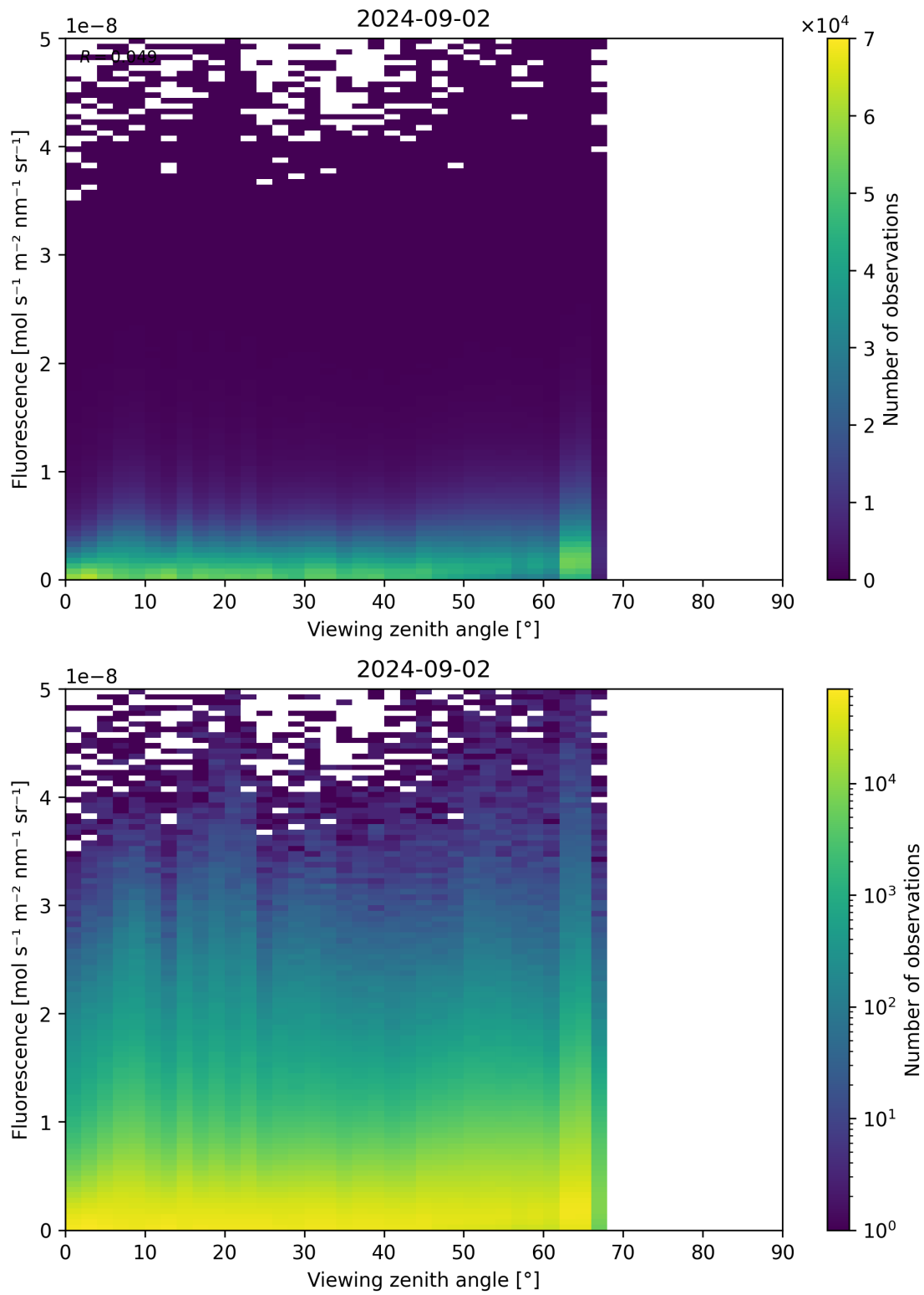
Figure 122: Scatter density plot of “Viewing zenith angle” against “Fluorescence” for 2024-09-01 to 2024-09-03.
