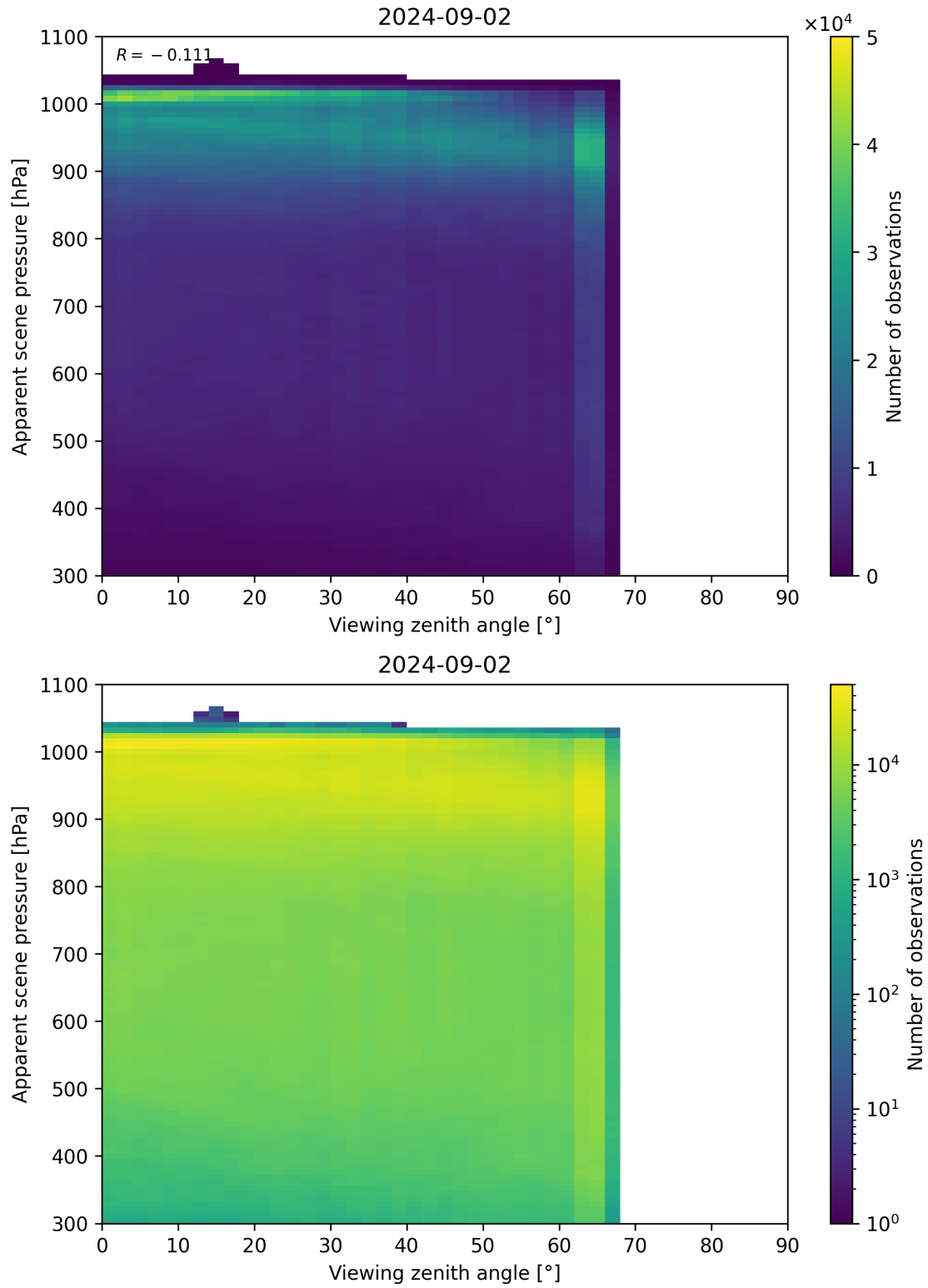
Figure 118: Scatter density plot of “Viewing zenith angle” against “Apparent scene pressure” for 2024-09-01 to 2024-09-03.
