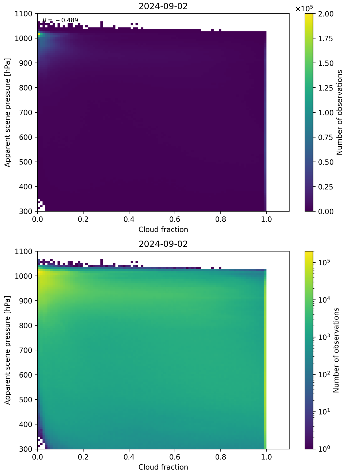
Figure 70: Scatter density plot of “Cloud fraction” against “Apparent scene pressure” for 2024-09-01 to 2024-09-03.
