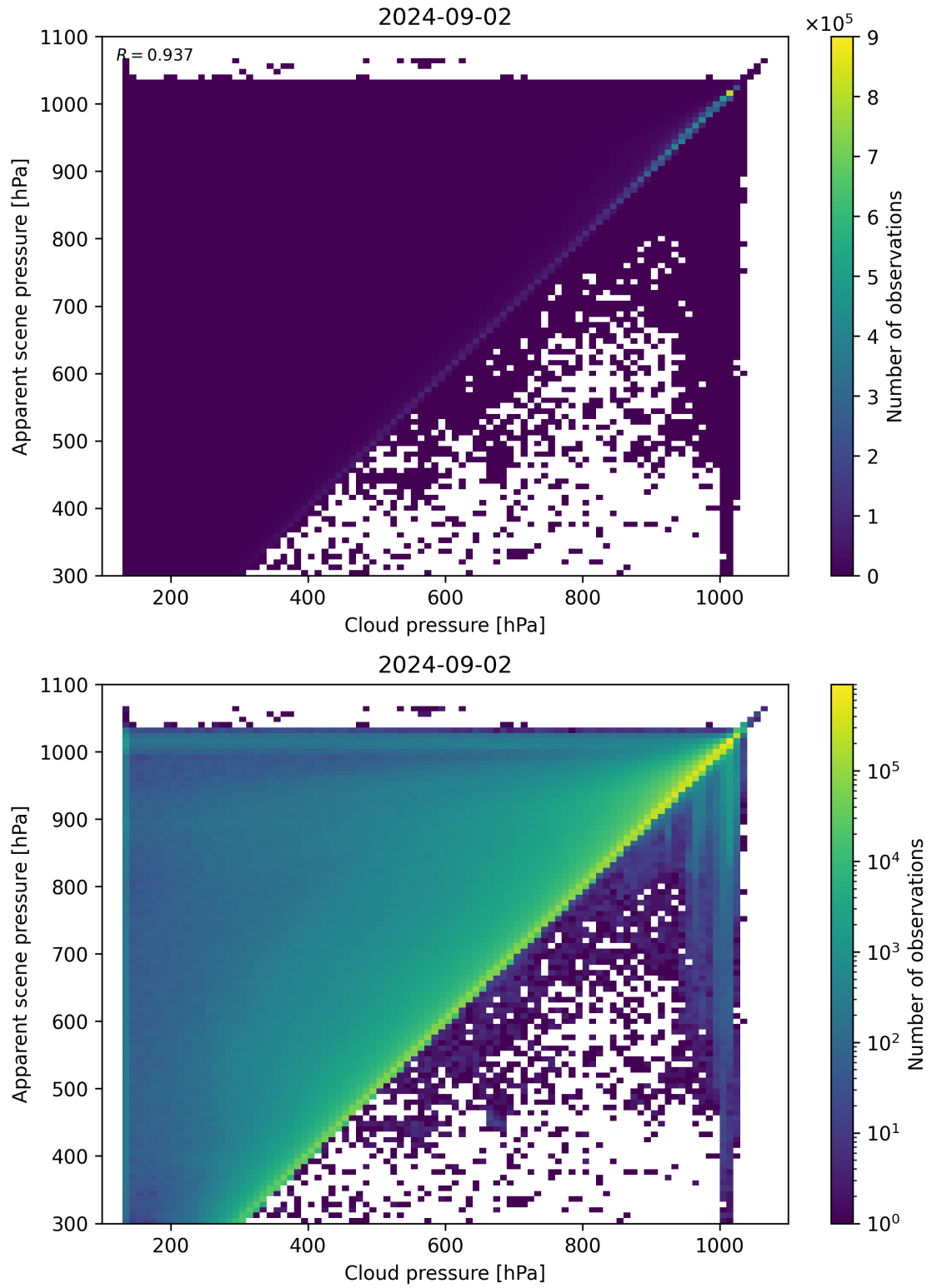
Figure 77: Scatter density plot of “Cloud pressure” against “Apparent scene pressure” for 2024-09-01 to 2024-09-03.
