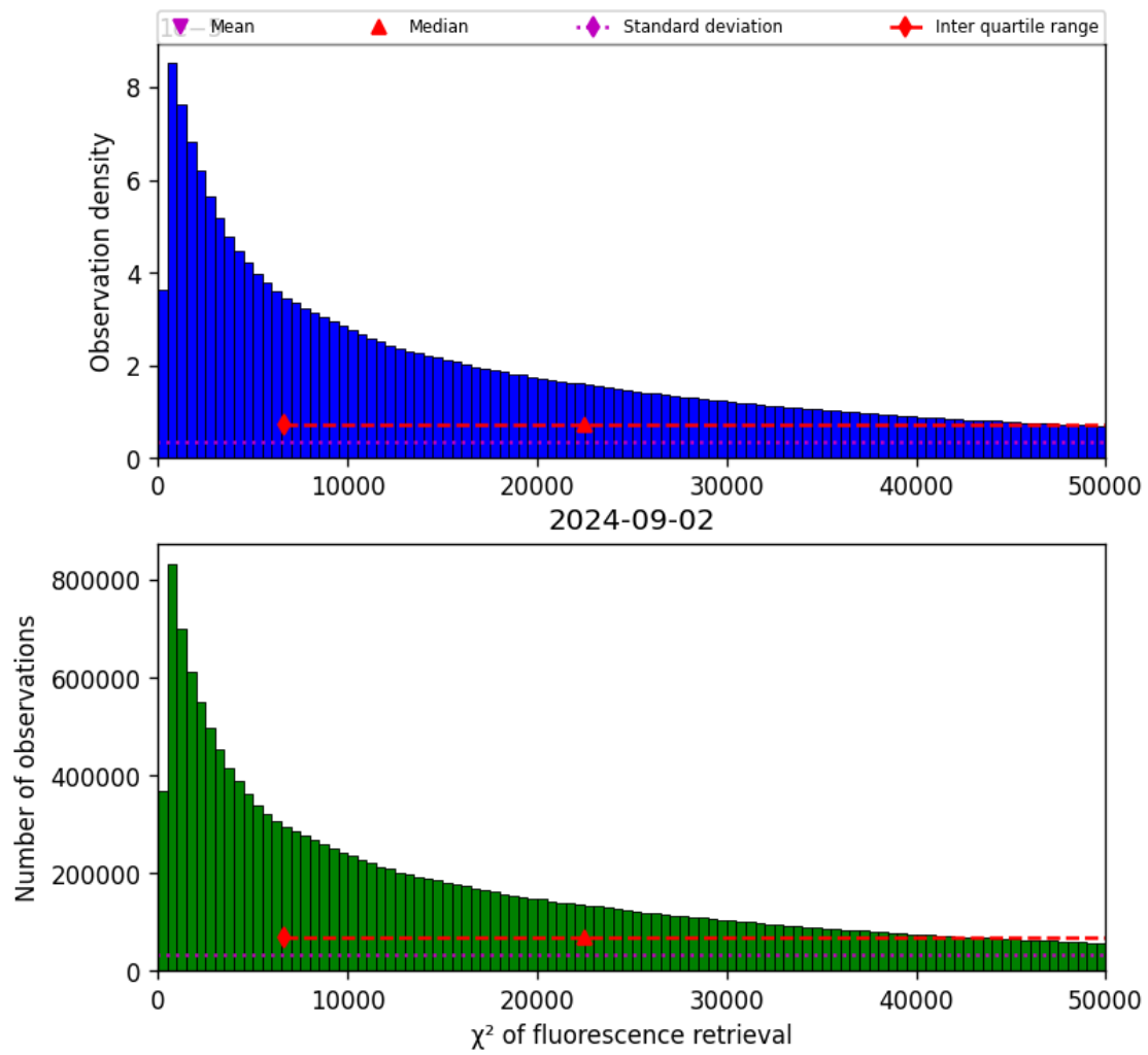
Figure 42: Histogram of “ \chi^2 of fluorescence retrieval” for 2024-09-01 to 2024-09-03
