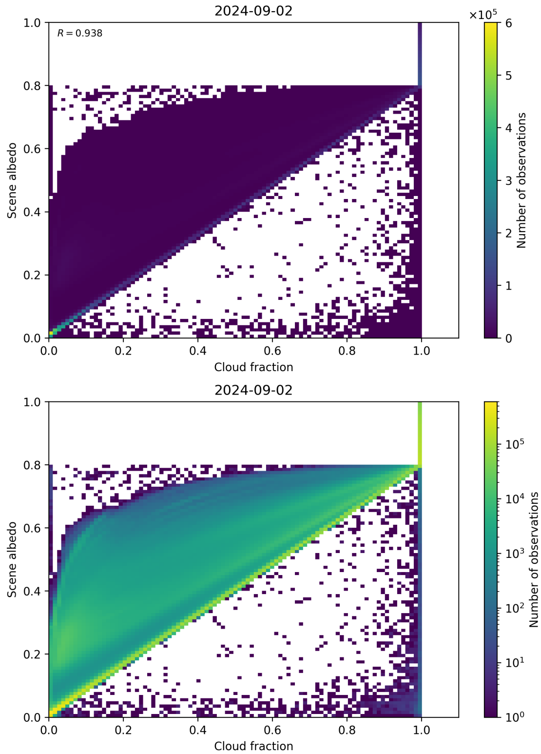
Figure 75: Scatter density plot of “Cloud fraction” against “Scene albedo” for 2024-09-01 to 2024-09-03.
