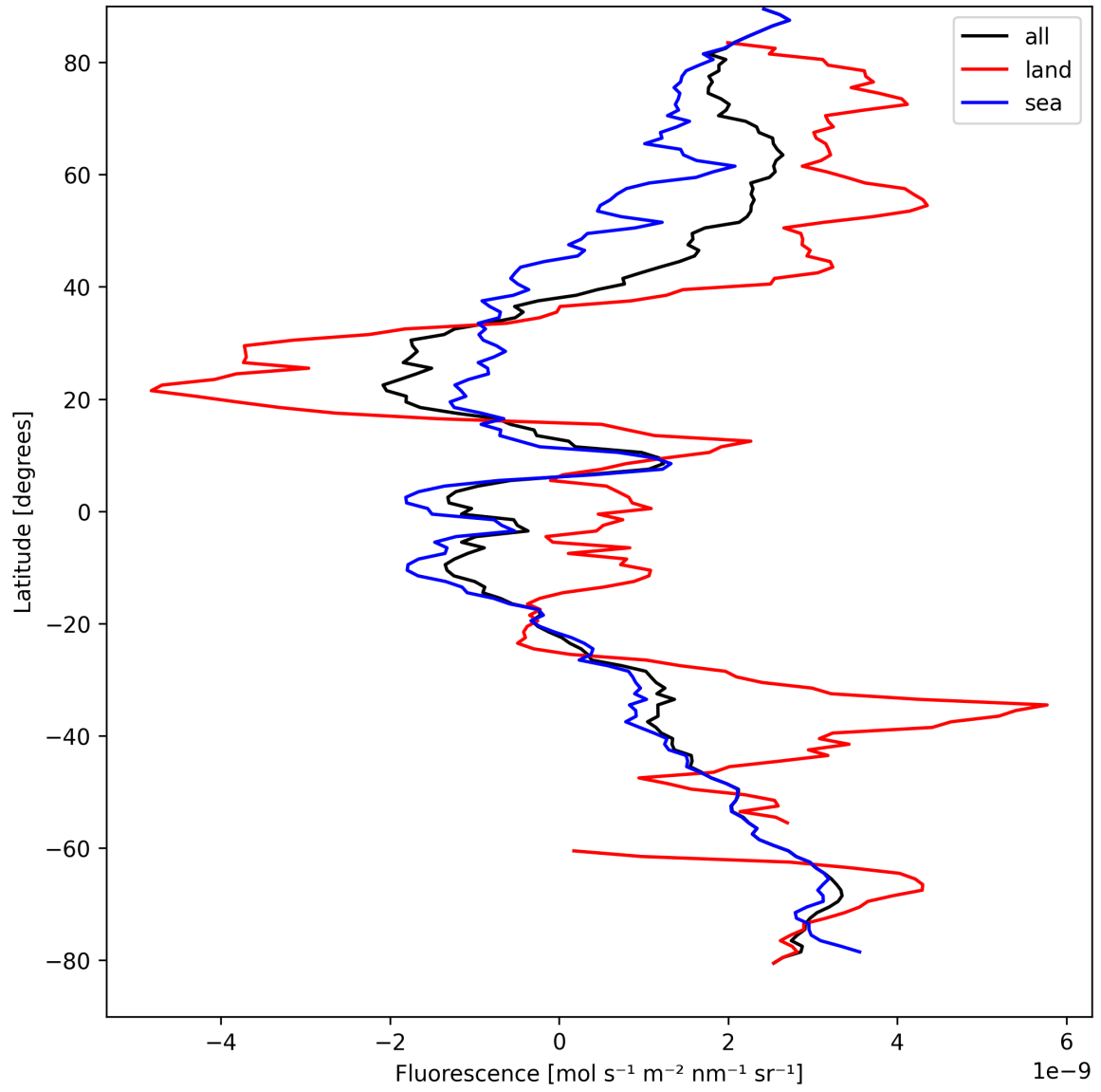
Figure 23: Zonal average of “Fluorescence” for 2024-09-01 to 2024-09-03.
