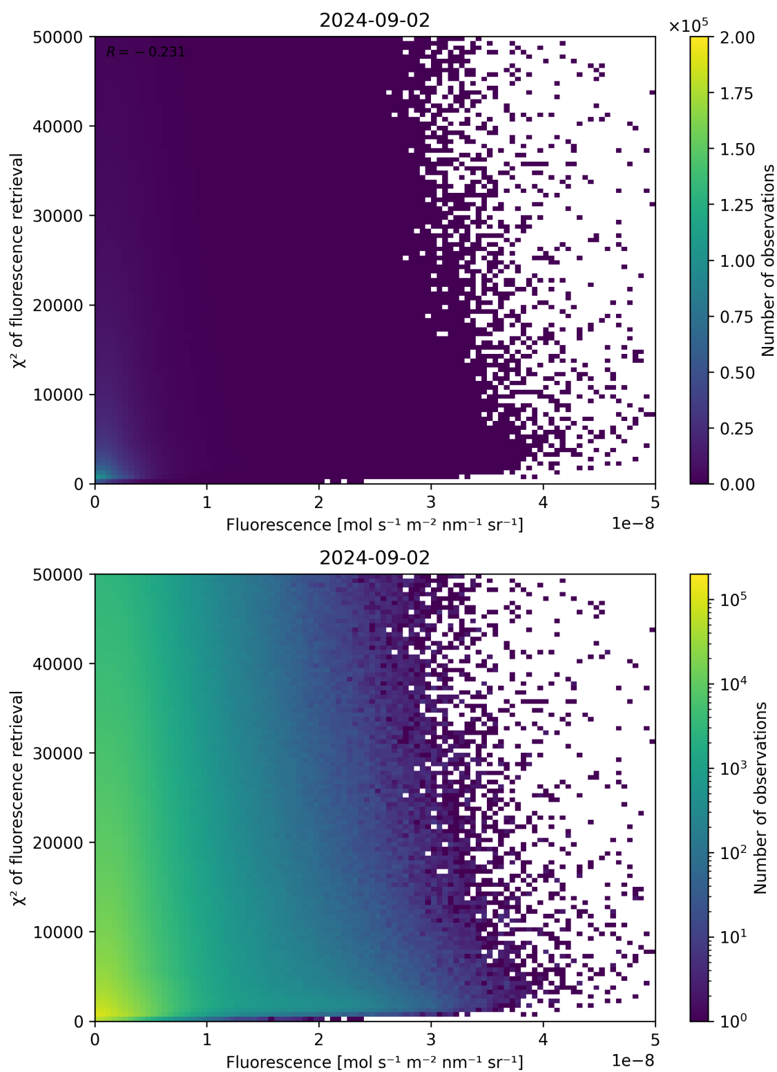
Figure 85: Scatter density plot of “Fluorescence” against “ \chi^2 of fluorescence retrieval” for 2024-09-01 to 2024-09-03.
