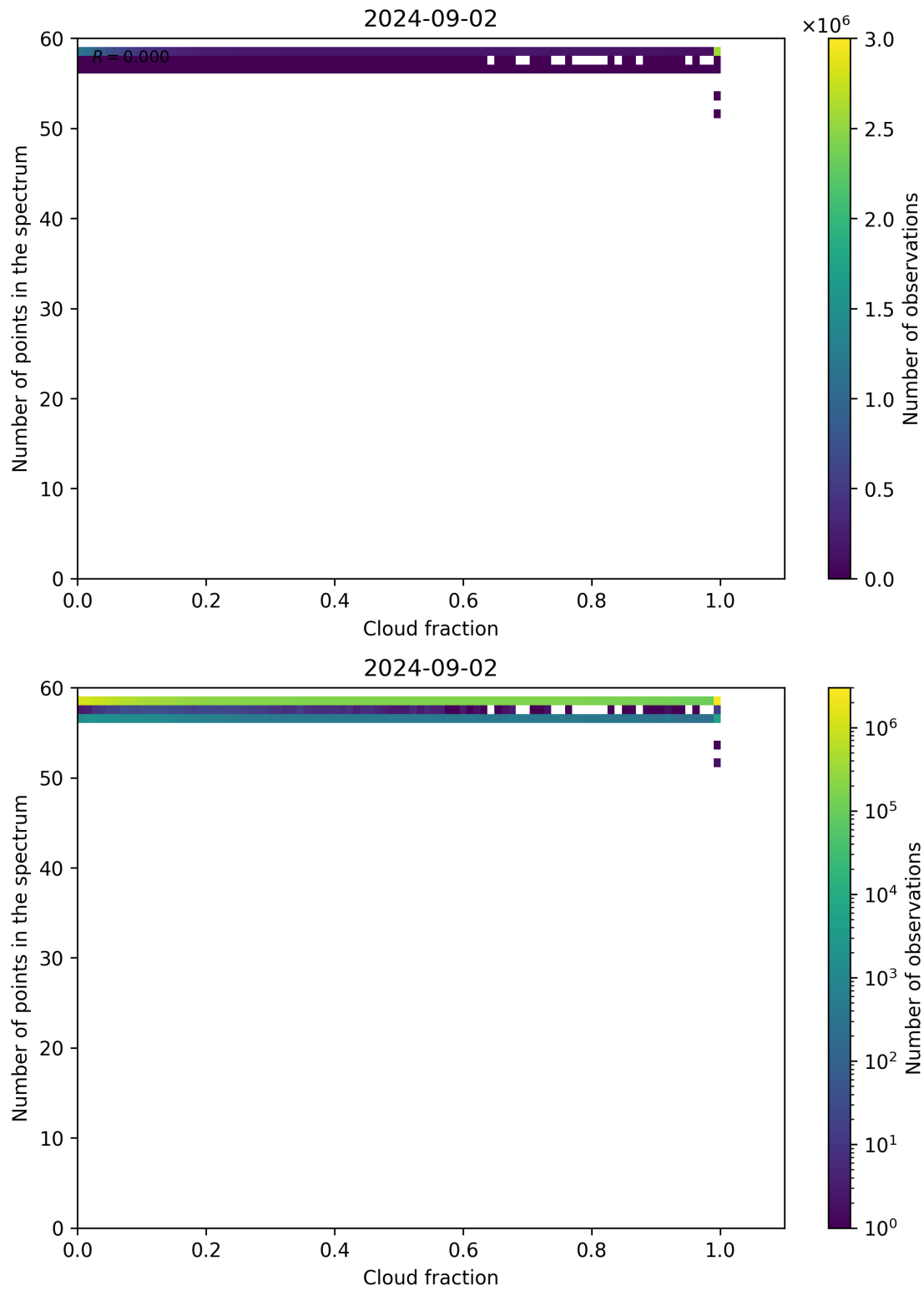
Figure 74: Scatter density plot of “Cloud fraction” against “Number of points in the spectrum” for 2024-09-01 to 2024-09-03.
