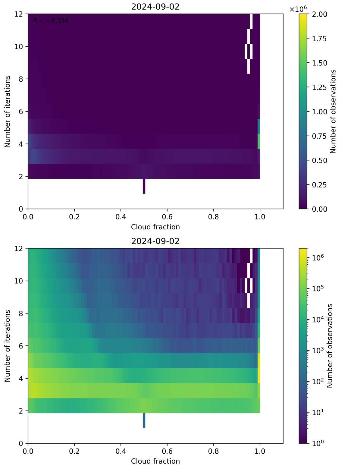
Figure 73: Scatter density plot of “Cloud fraction” against “Number of iterations” for 2024-09-01 to 2024-09-03.
