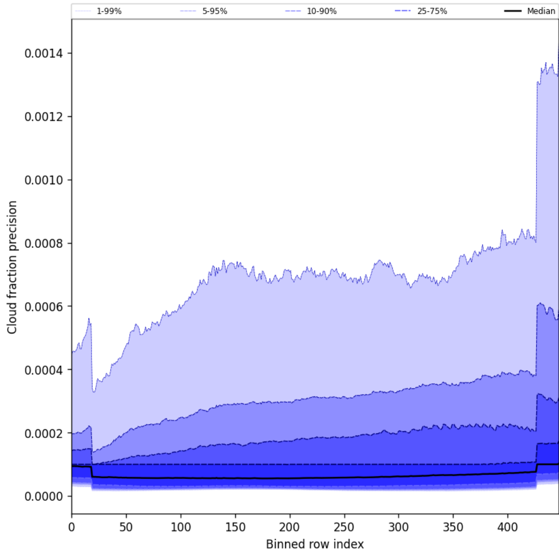
Figure 50: Along track statistics of “Cloud fraction precision” for 2024-09-01 to 2024-09-03
