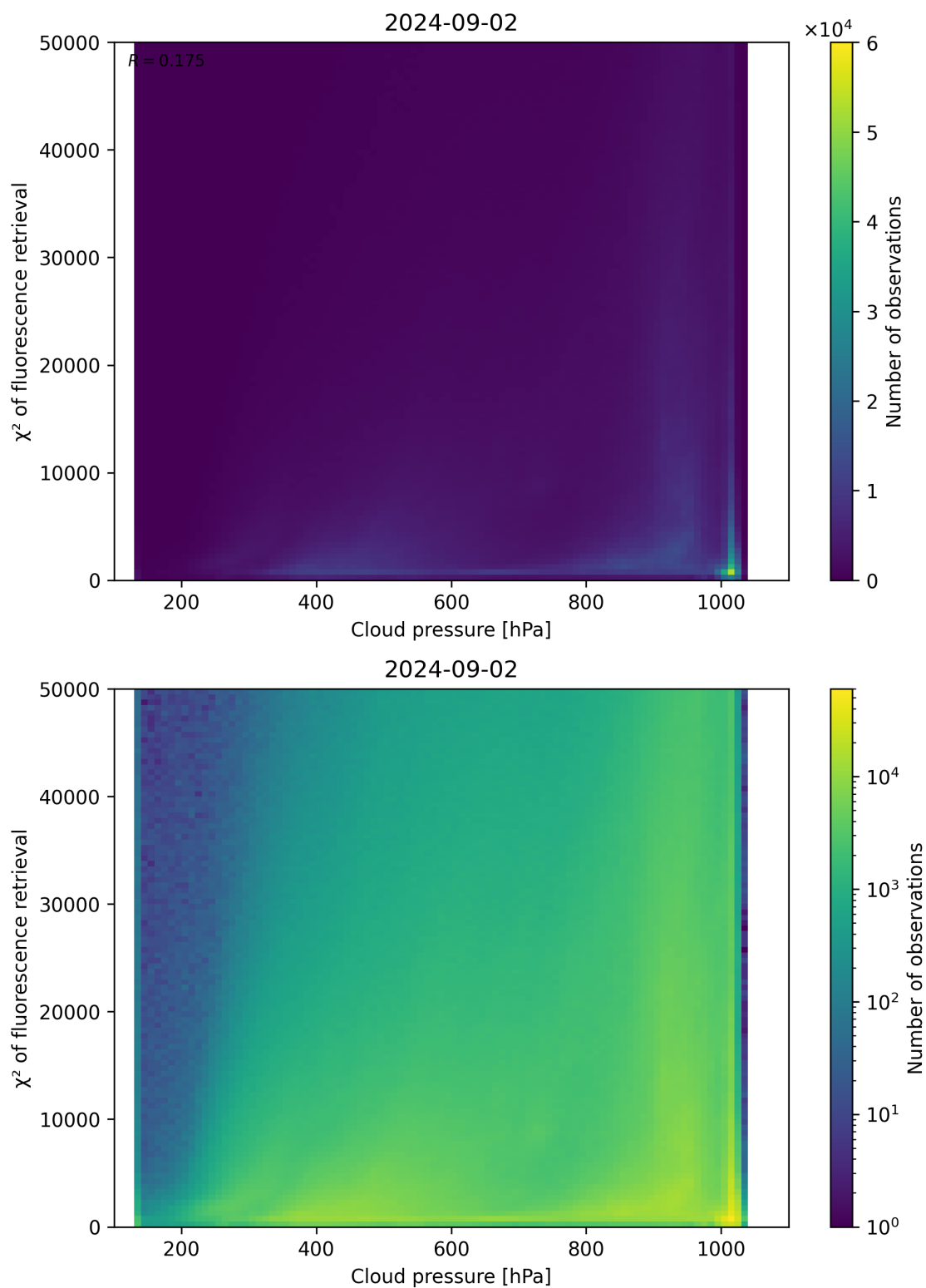
Figure 78: Scatter density plot of “Cloud pressure” against “ \chi^2 of fluorescence retrieval” for 2024-09-01 to 2024-09-03.
