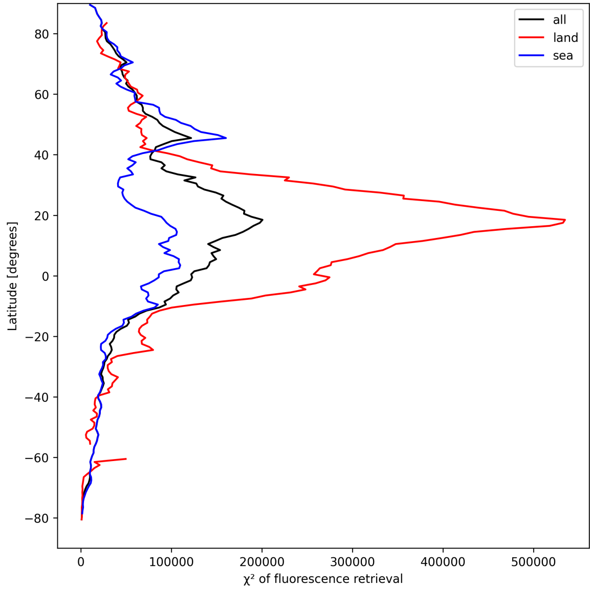
Figure 25: Zonal average of “ \chi^2 of fluorescence retrieval” for 2024-09-01 to 2024-09-03.
