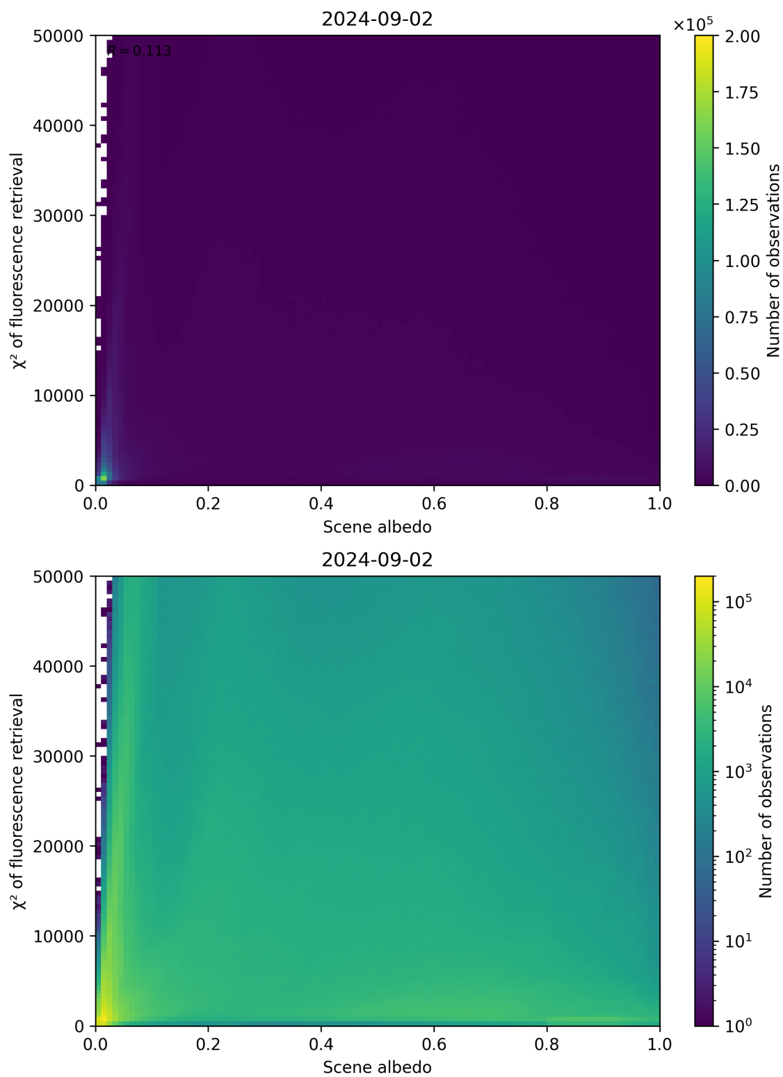
Figure 103: Scatter density plot of “Scene albedo” against “ \chi^2 of fluorescence retrieval” for 2024-09-01 to 2024-09-03.
