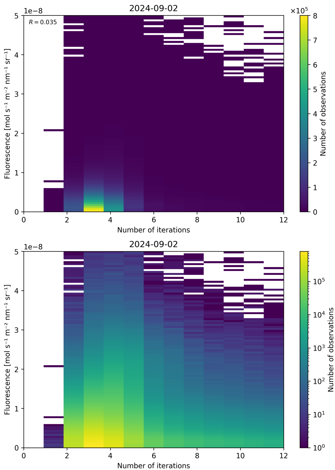
Figure 98: Scatter density plot of “Number of iterations” against “Fluorescence” for 2024-09-01 to 2024-09-03.
