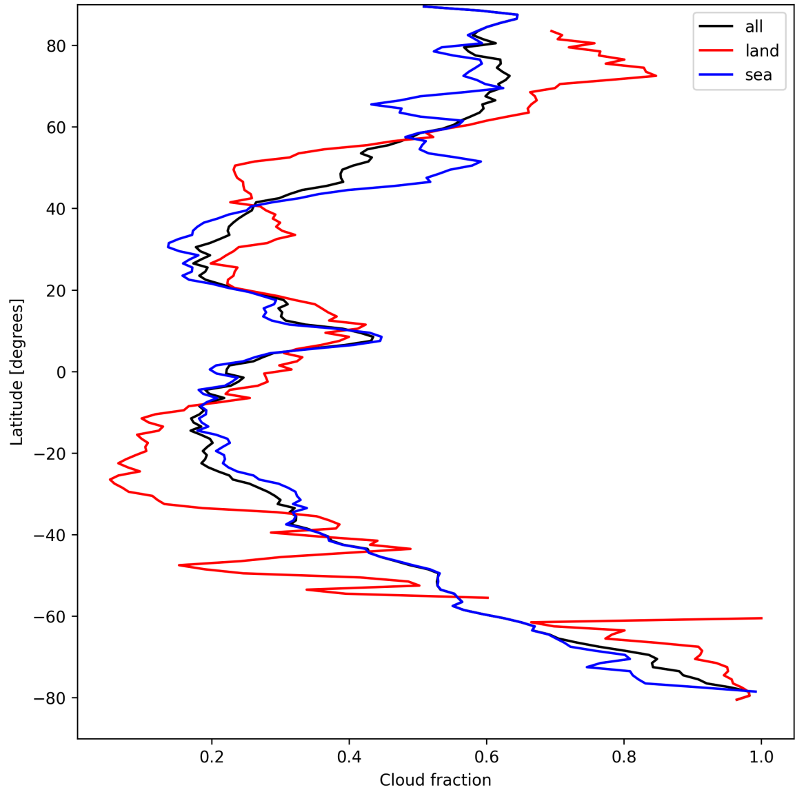
Figure 15: Zonal average of “Cloud fraction” for 2024-09-01 to 2024-09-03.
