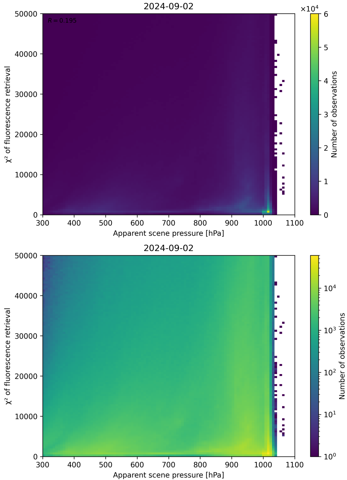
Figure 63: Scatter density plot of “Apparent scene pressure” against “ \chi^2 of fluorescence retrieval” for 2024-09-01 to 2024-09-03.
