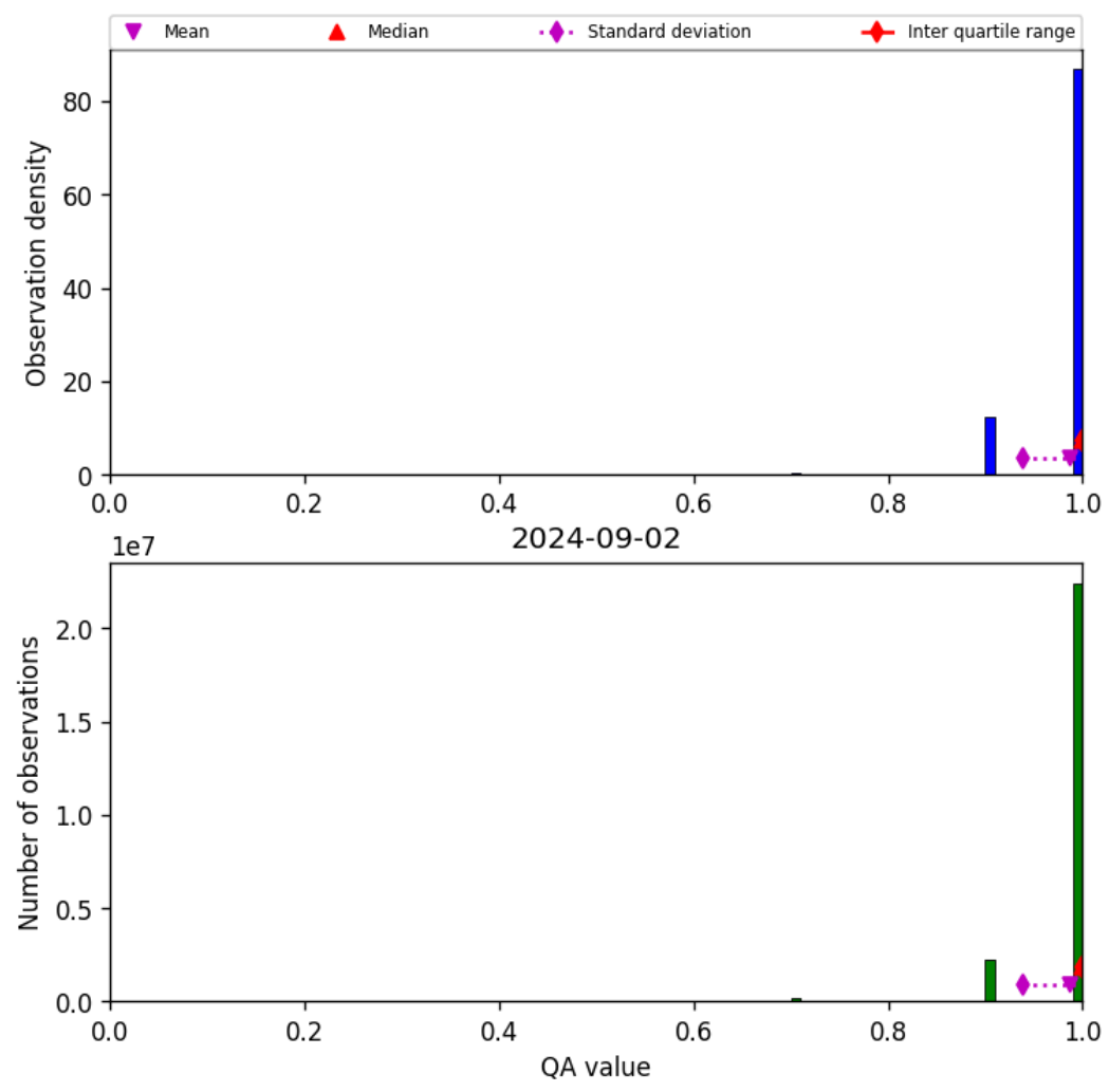
Figure 29: Histogram of “QA value” for 2024-09-01 to 2024-09-03
