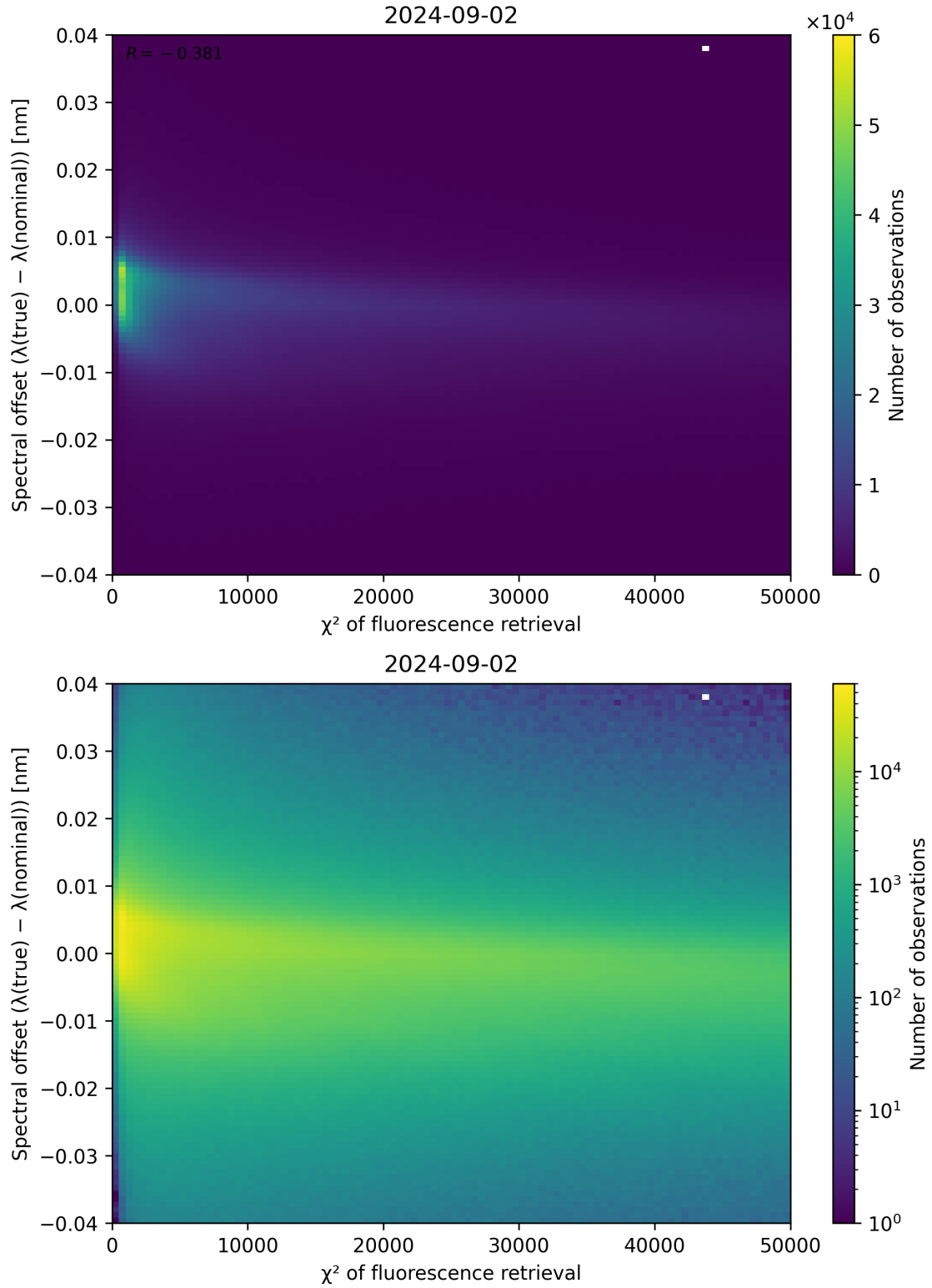
Figure 69: Scatter density plot of “ \chi^2 of fluorescence retrieval” against “Spectral offset ( \lambda_{\text{true}} - \lambda_{\text{nominal}} )” for 2024-09-01 to 2024-09-03.
