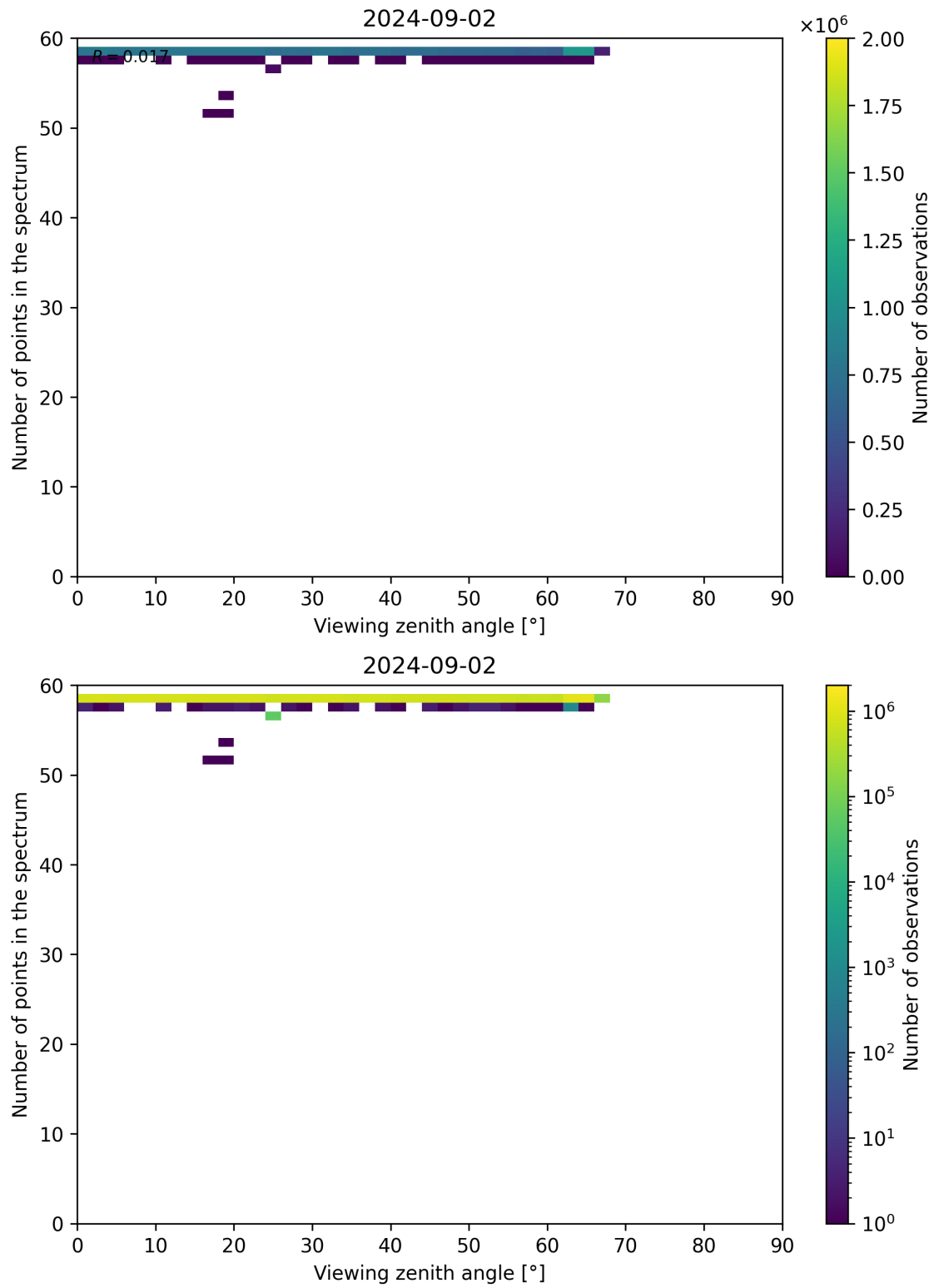
Figure 125: Scatter density plot of “Viewing zenith angle” against “Number of points in the spectrum” for 2024-09-01 to 2024-09-03.
