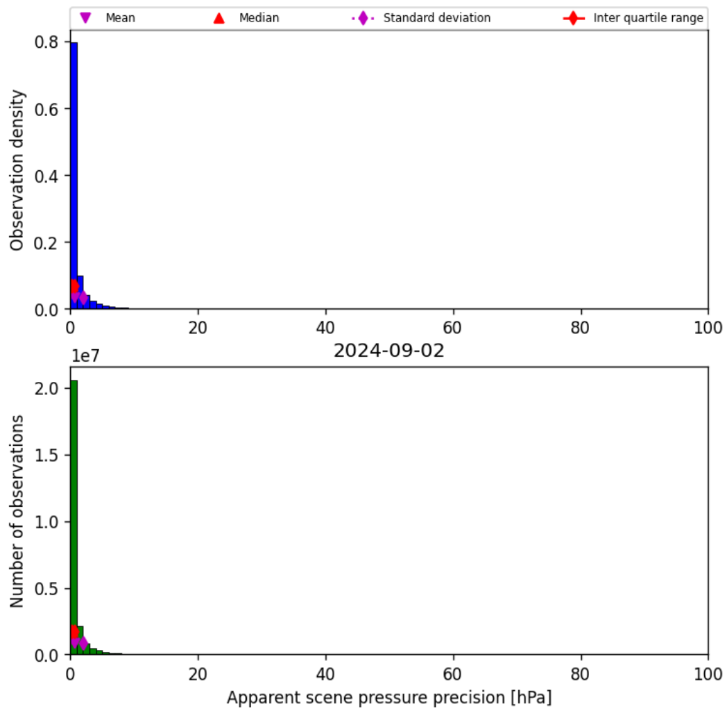
Figure 37: Histogram of “Apparent scene pressure precision” for 2024-09-01 to 2024-09-03
