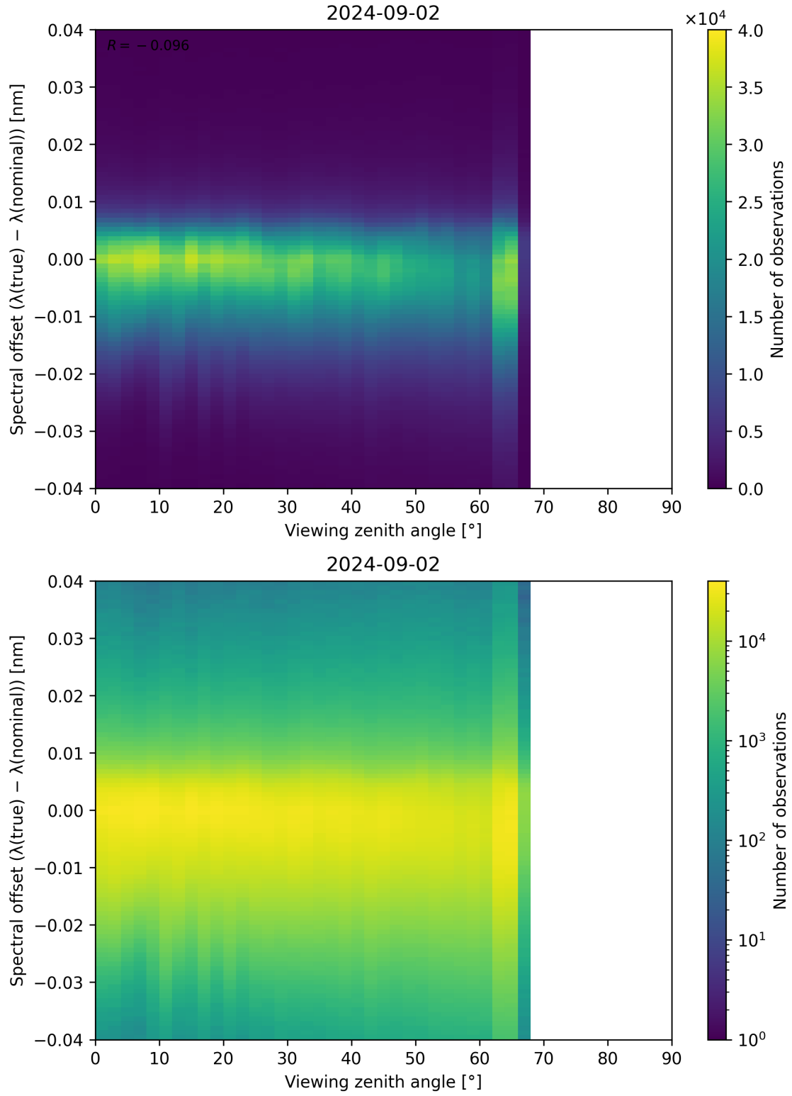
Figure 128: Scatter density plot of “Viewing zenith angle” against “Spectral offset ( \lambda_{\text{true}} - \lambda_{\text{nominal}} )” for 2024-09-01 to 2024-09-03.
