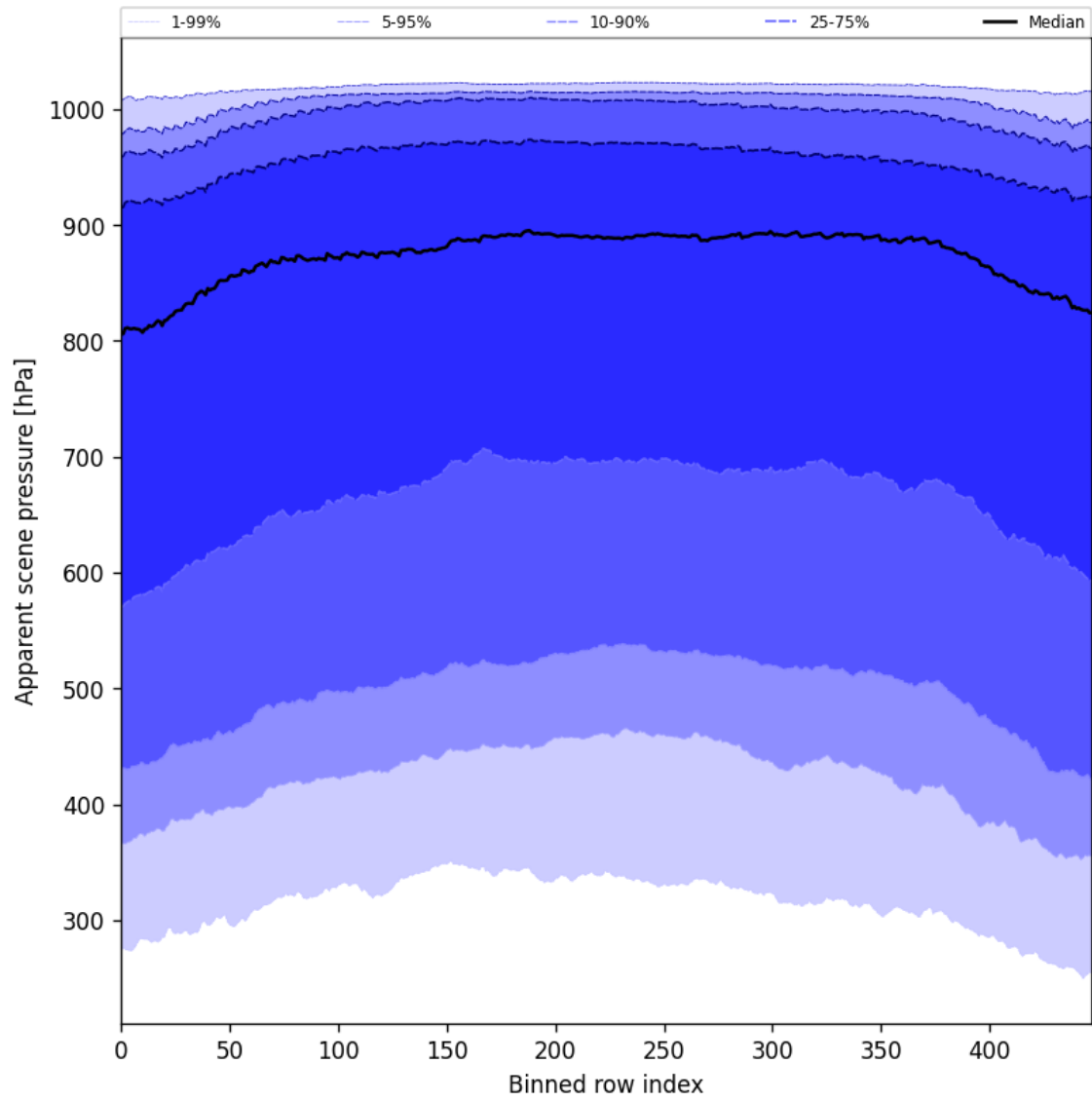
Figure 53: Along track statistics of “Apparent scene pressure” for 2024-09-01 to 2024-09-03
