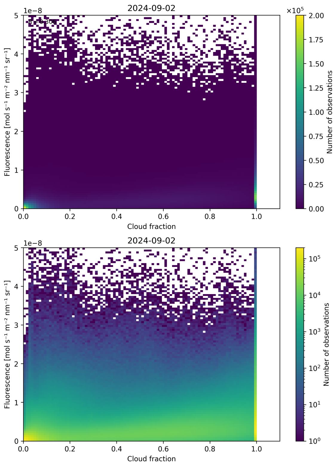
Figure 72: Scatter density plot of “Cloud fraction” against “Fluorescence” for 2024-09-01 to 2024-09-03.
