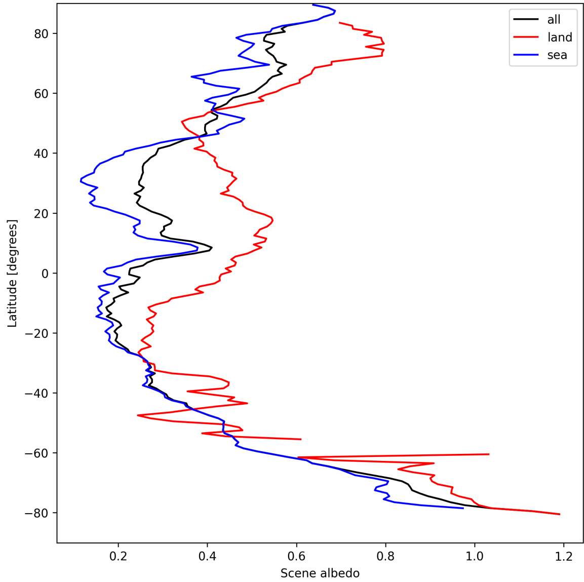
Figure 17: Zonal average of “Scene albedo” for 2024-09-01 to 2024-09-03.
