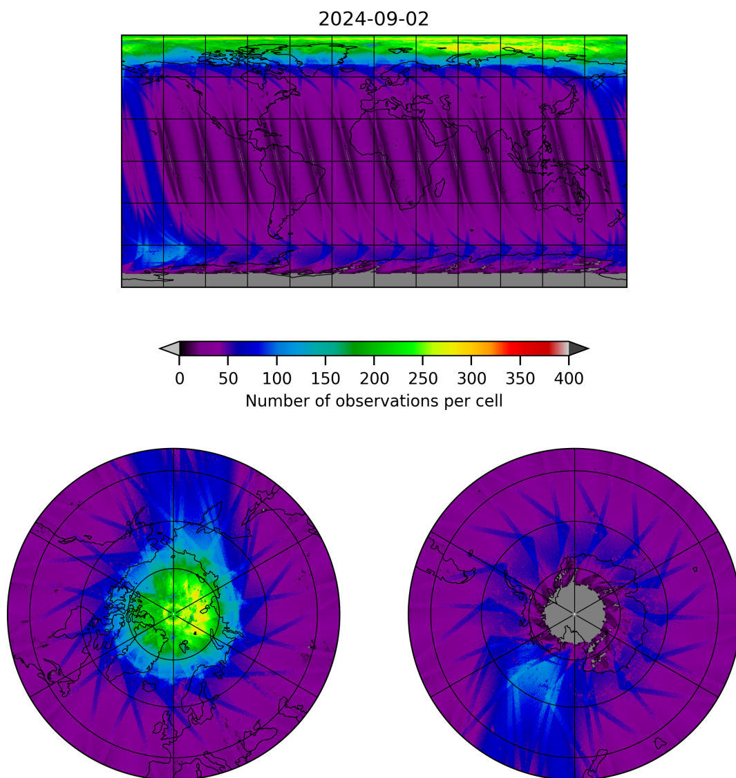
Figure 11: Map of the number of observations for 2024-09-01 to 2024-09-03
