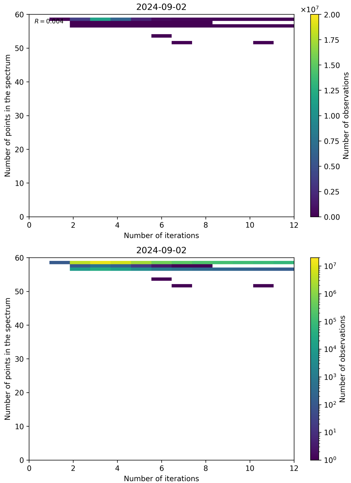
Figure 99: Scatter density plot of “Number of iterations” against “Number of points in the spectrum” for 2024-09-01 to 2024-09-03.
