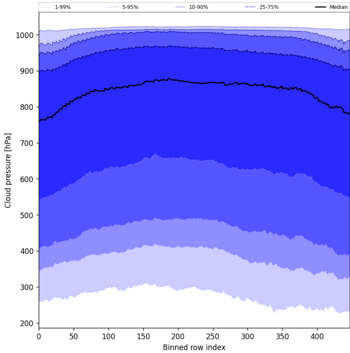
Figure 47: Along track statistics of “Cloud pressure” for 2024-09-01 to 2024-09-03
