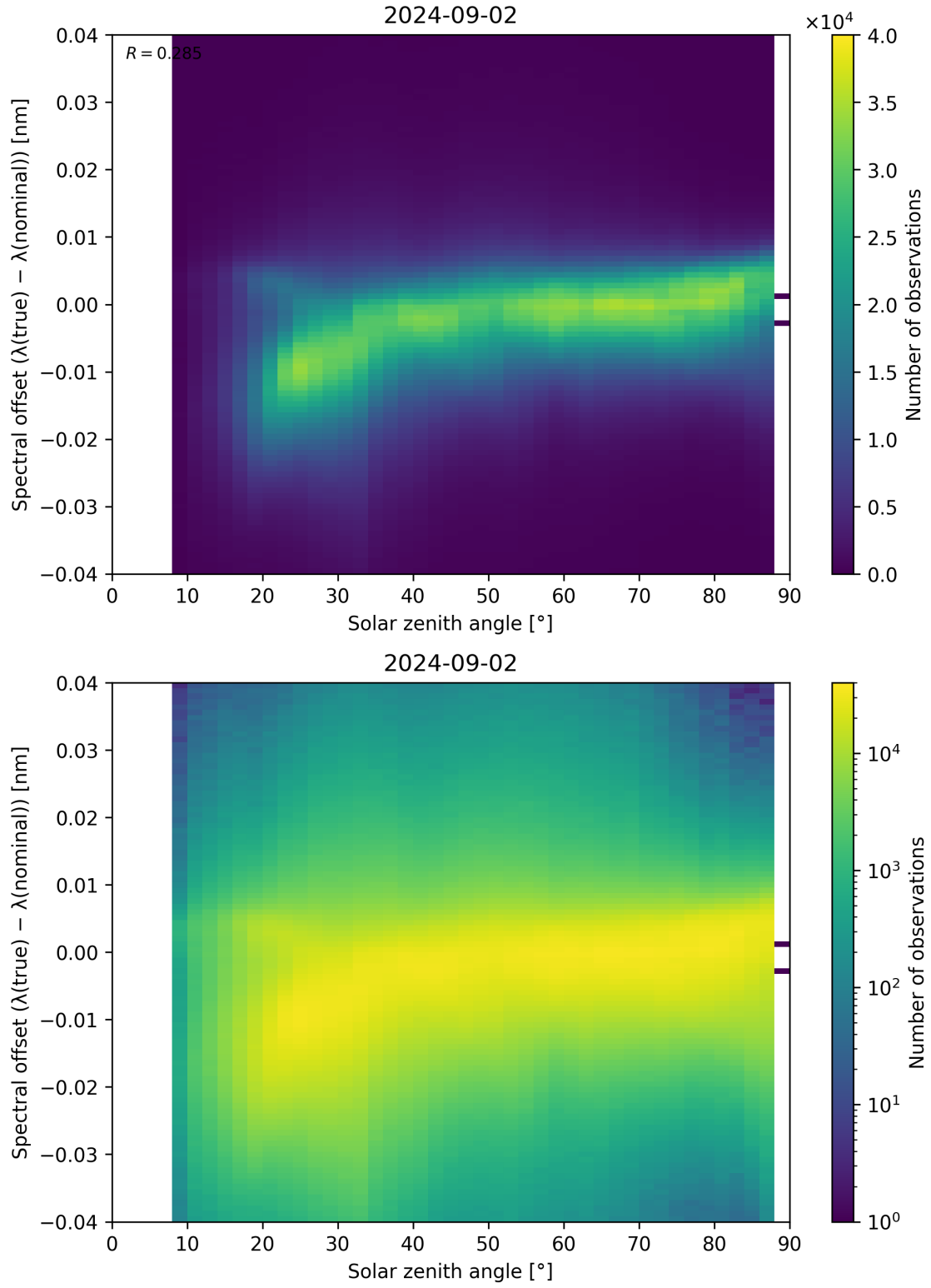
Figure 117: Scatter density plot of “Solar zenith angle” against “Spectral offset ( \lambda_{\text{true}} - \lambda_{\text{nominal}} )” for 2024-09-01 to 2024-09-03.
