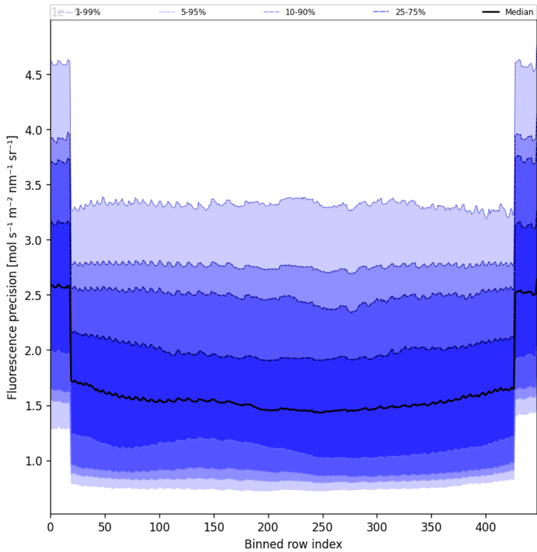
Figure 58: Along track statistics of “Fluorescence precision” for 2024-09-01 to 2024-09-03
