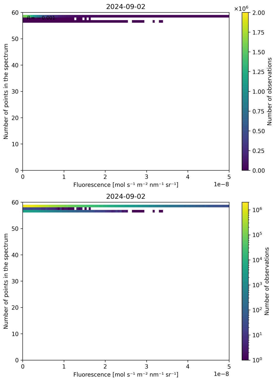
Figure 86: Scatter density plot of “Fluorescence” against “Number of points in the spectrum” for 2024-09-01 to 2024-09-03.
