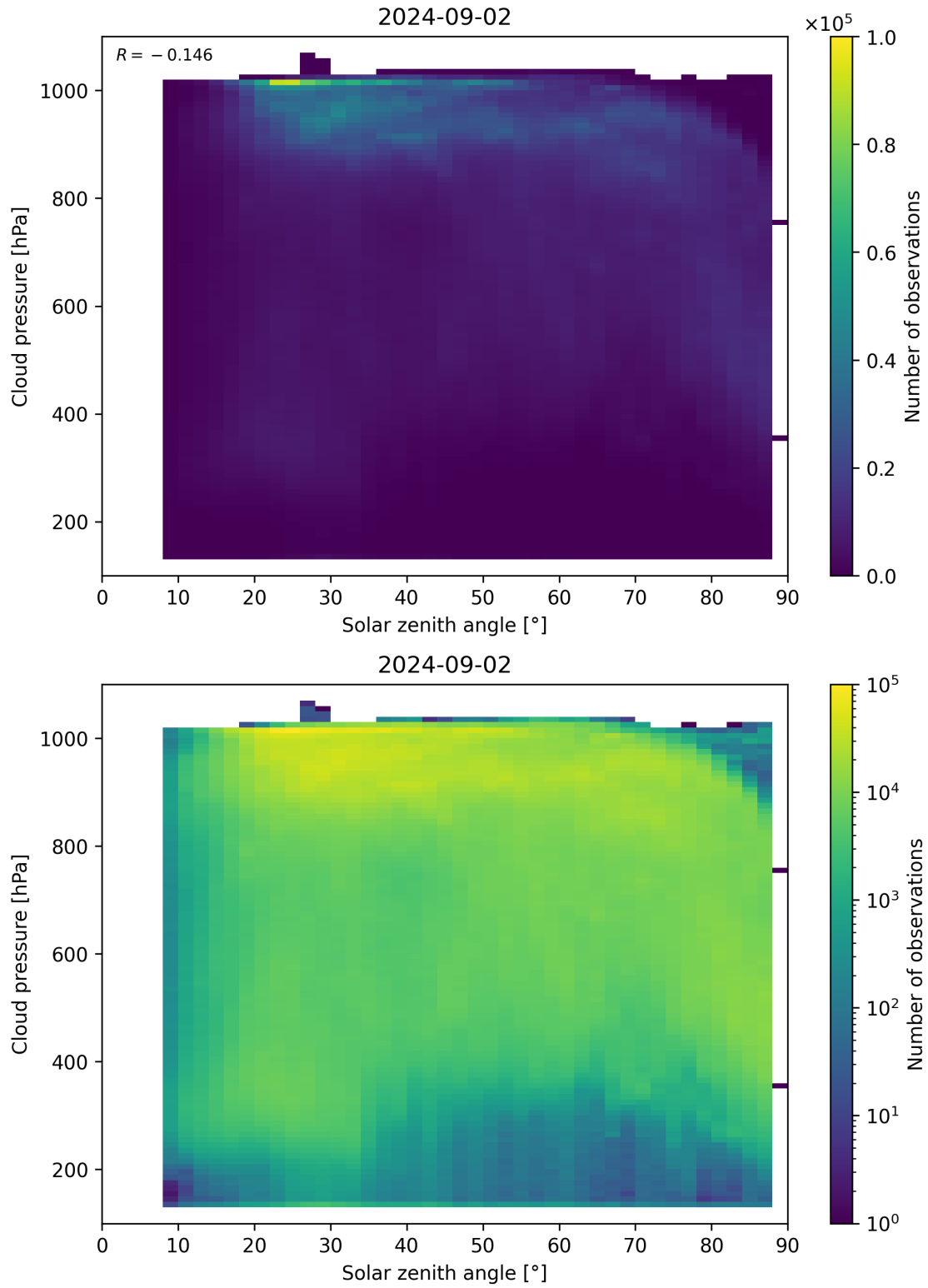
Figure 111: Scatter density plot of “Solar zenith angle” against “Cloud pressure” for 2024-09-01 to 2024-09-03.
