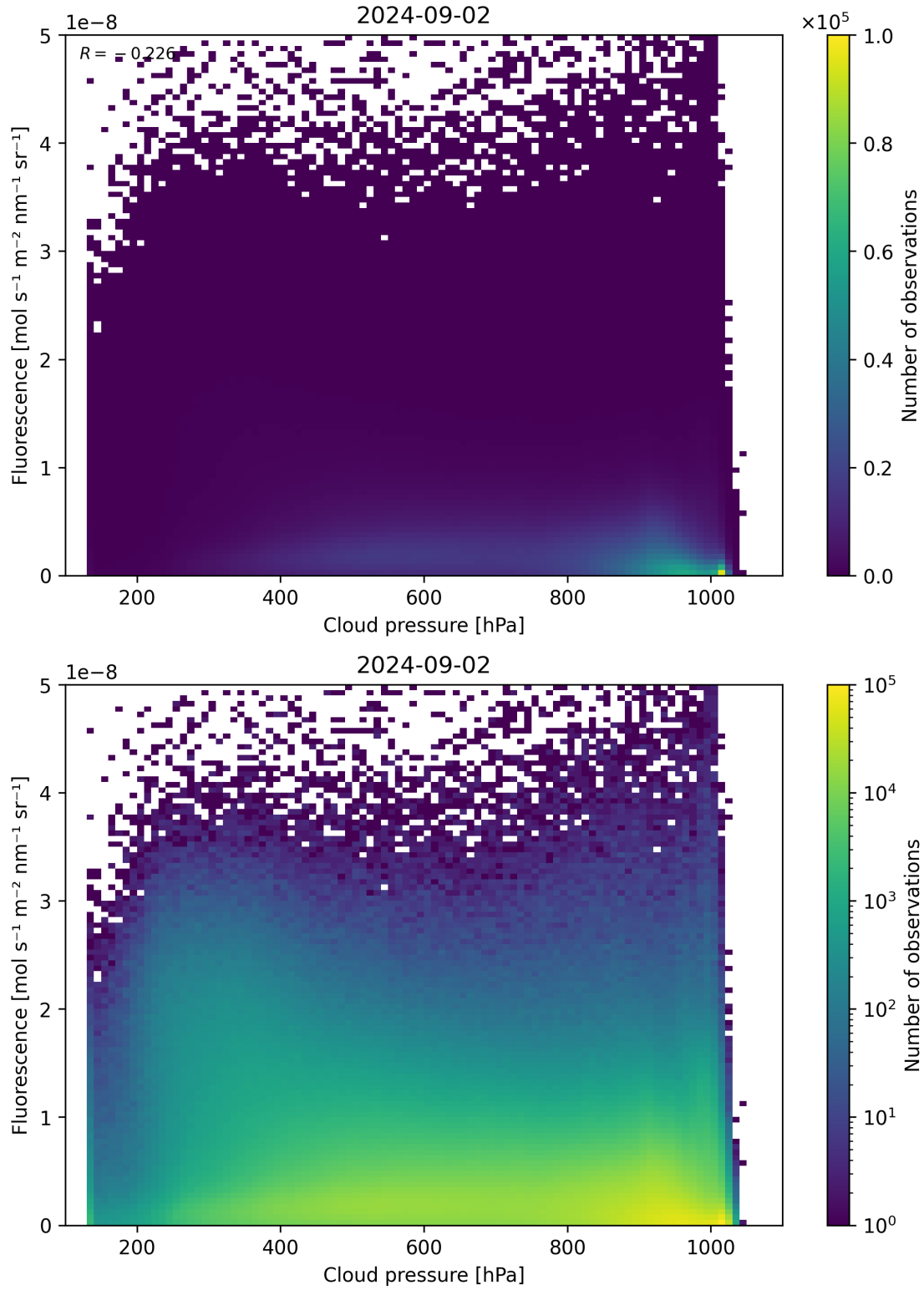
Figure 80: Scatter density plot of “Cloud pressure” against “Fluorescence” for 2024-09-01 to 2024-09-03.
