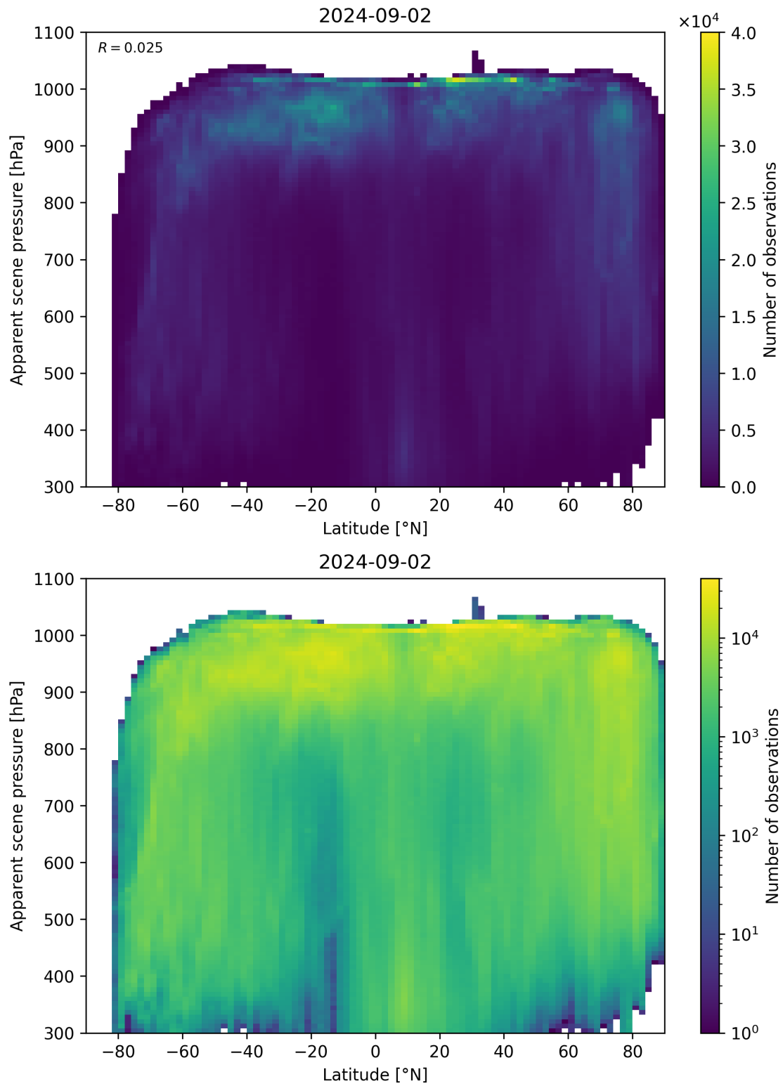
Figure 88: Scatter density plot of “Latitude” against “Apparent scene pressure” for 2024-09-01 to 2024-09-03.
