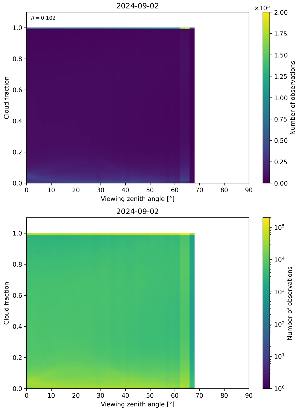
Figure 120: Scatter density plot of “Viewing zenith angle” against “Cloud fraction” for 2024-09-01 to 2024-09-03.
