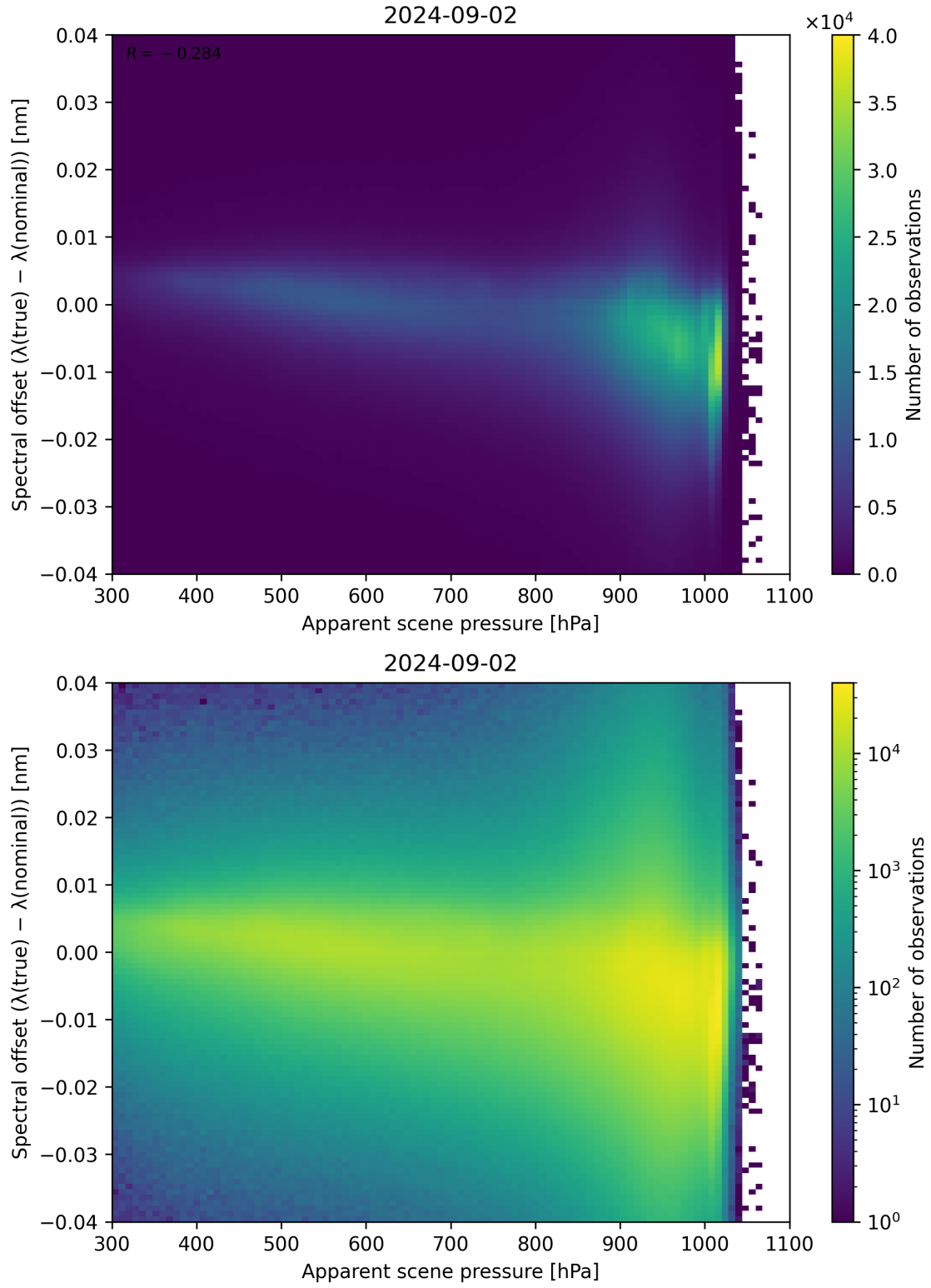
Figure 67: Scatter density plot of “Apparent scene pressure” against “Spectral offset ( \lambda_{\text{true}} - \lambda_{\text{nominal}} )” for 2024-09-01 to 2024-09-03.
