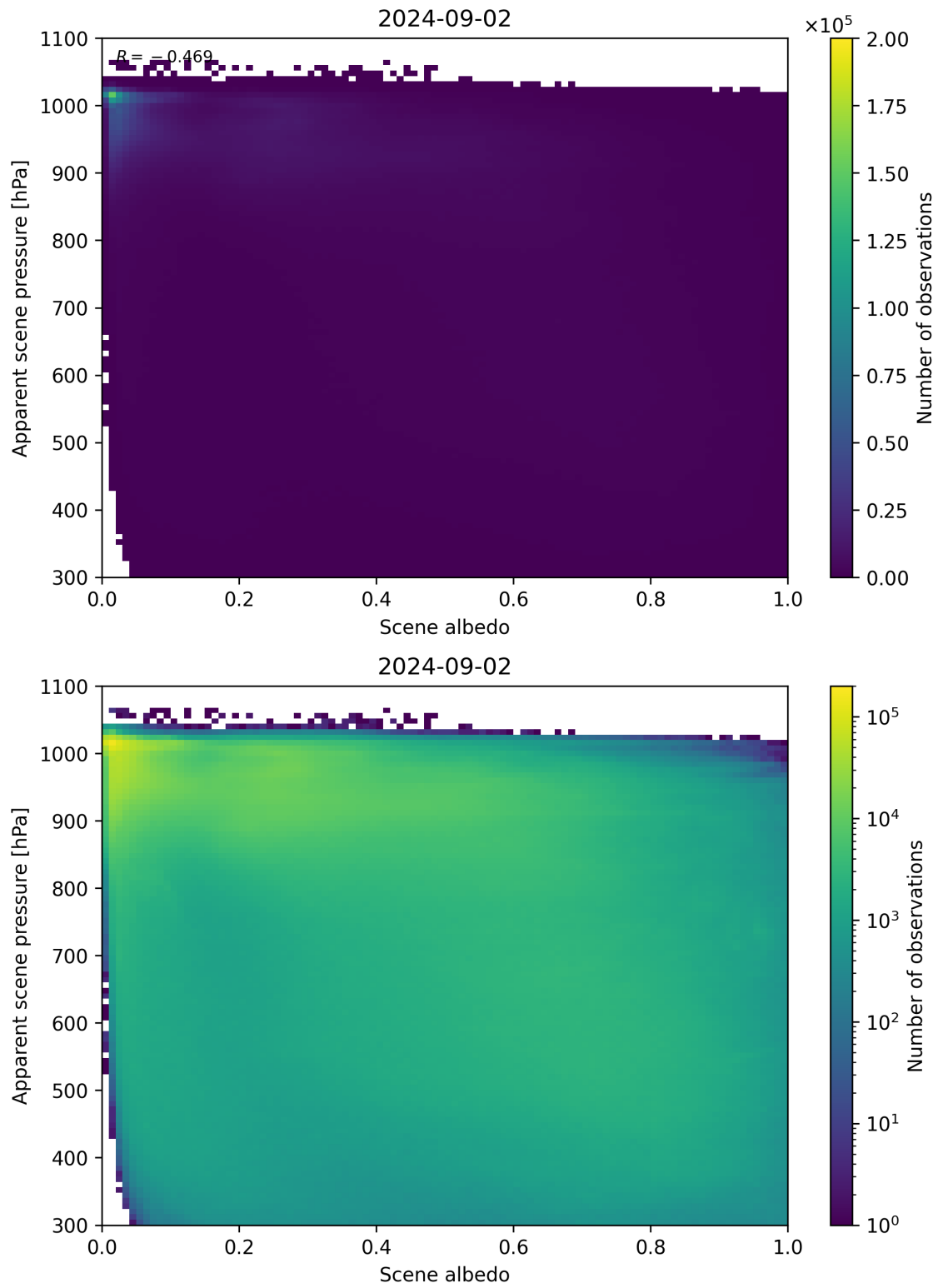
Figure 102: Scatter density plot of “Scene albedo” against “Apparent scene pressure” for 2024-09-01 to 2024-09-03.
