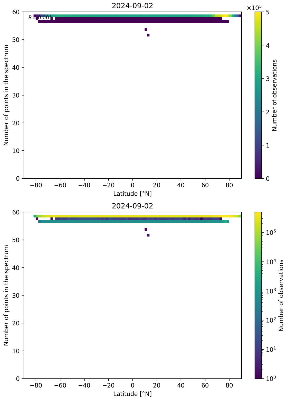
Figure 94: Scatter density plot of “Latitude” against “Number of points in the spectrum” for 2024-09-01 to 2024-09-03.
