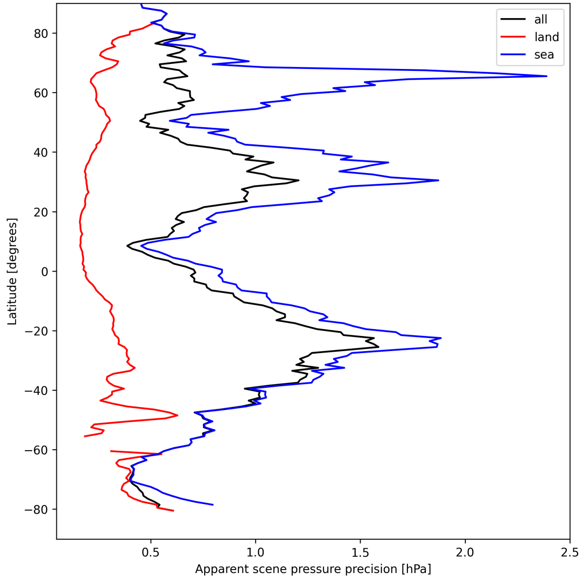
Figure 20: Zonal average of “Apparent scene pressure precision” for 2024-09-01 to 2024-09-03.
