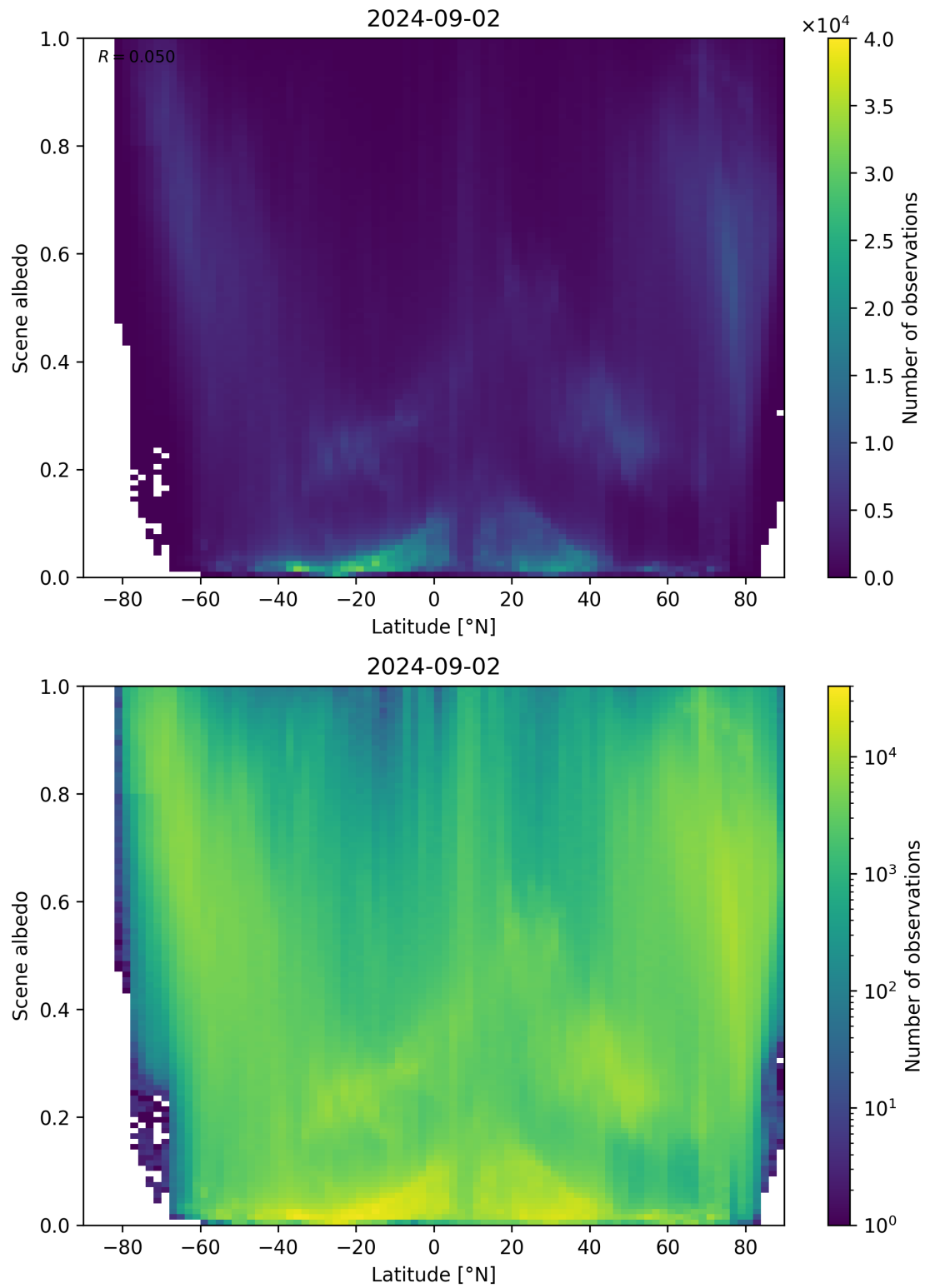
Figure 95: Scatter density plot of “Latitude” against “Scene albedo” for 2024-09-01 to 2024-09-03.
