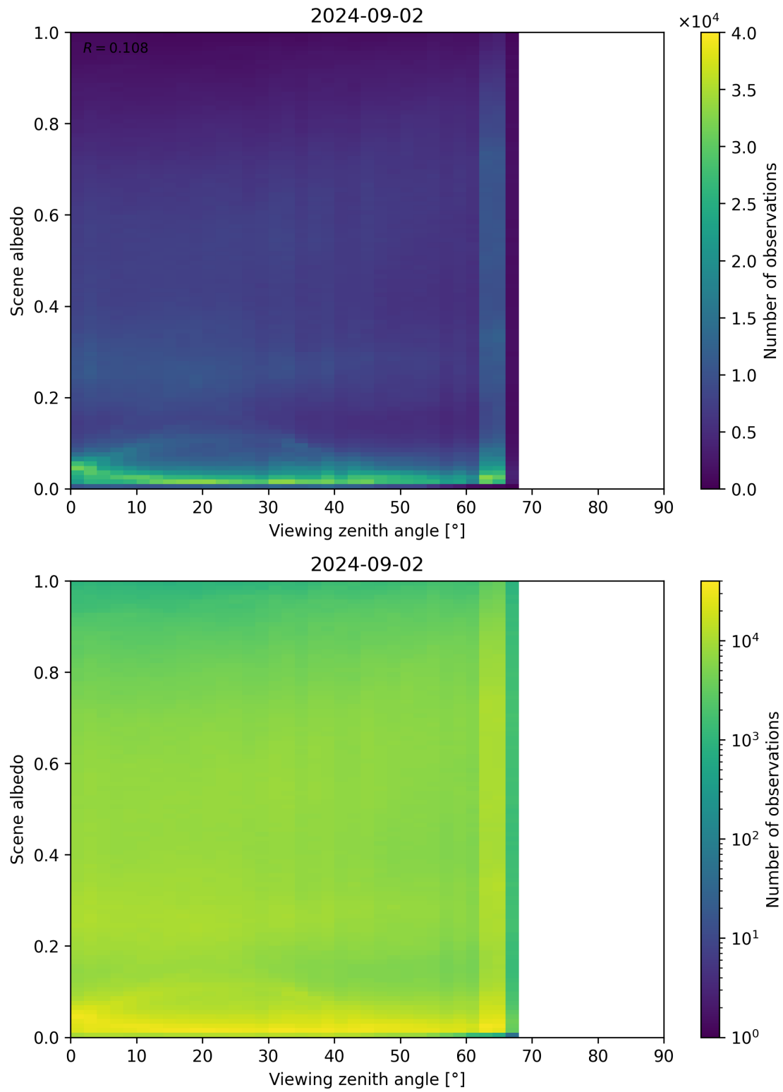
Figure 126: Scatter density plot of “Viewing zenith angle” against “Scene albedo” for 2024-09-01 to 2024-09-03.
