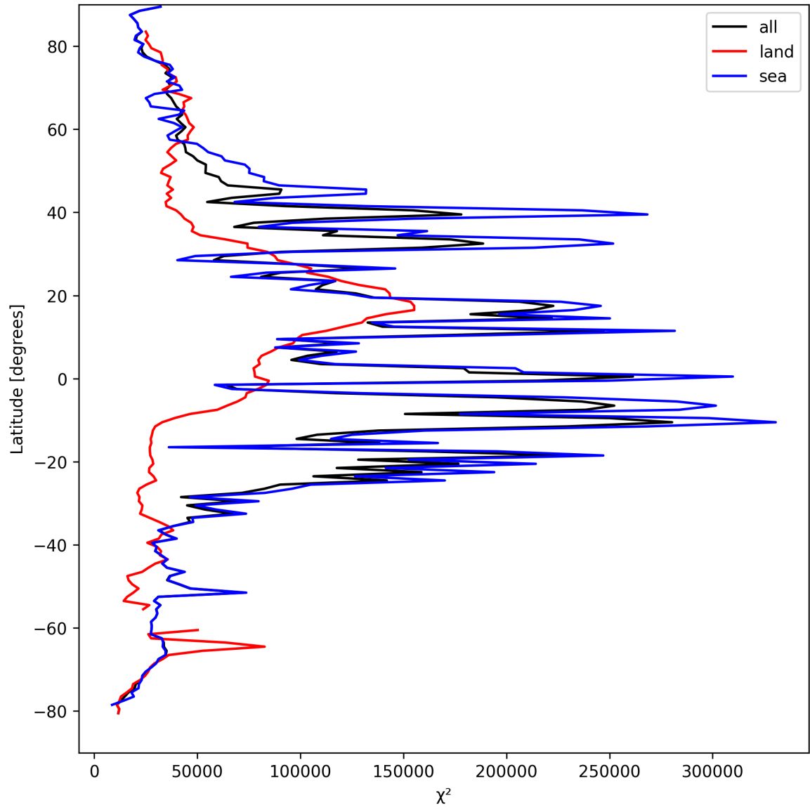
Figure 21: Zonal average of “ \chi^2 ” for 2024-09-01 to 2024-09-03.
