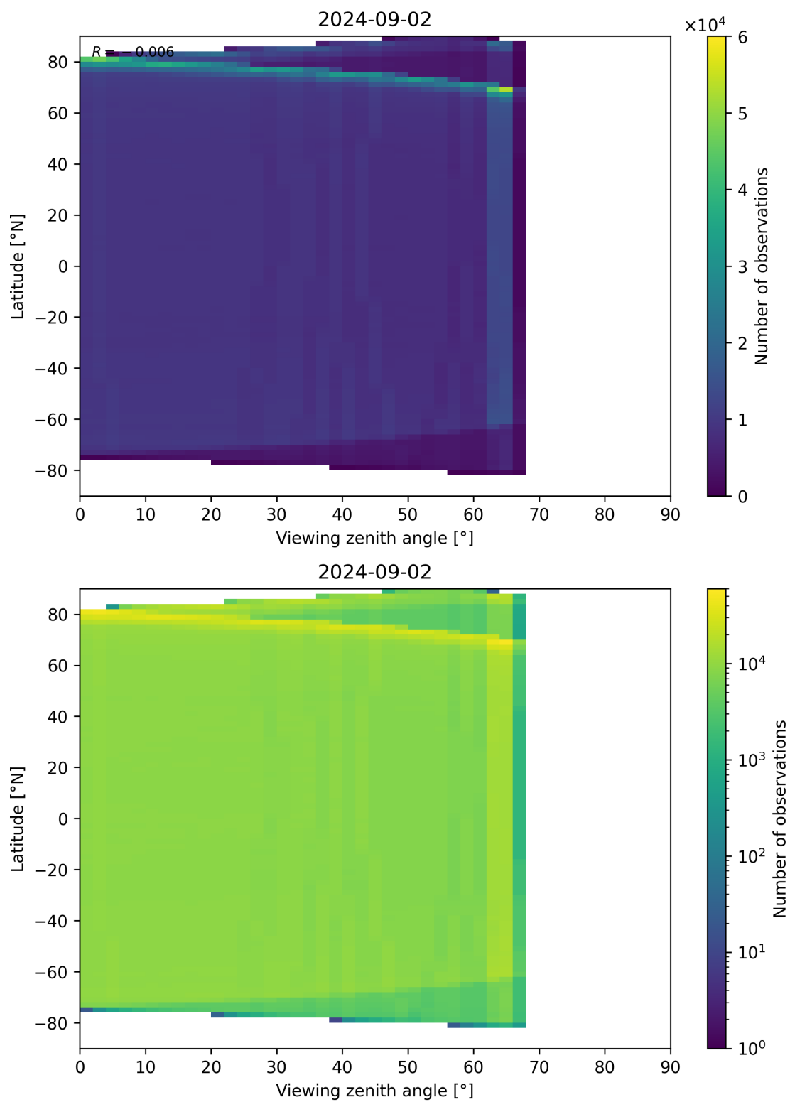
Figure 123: Scatter density plot of “Viewing zenith angle” against “Latitude” for 2024-09-01 to 2024-09-03.
