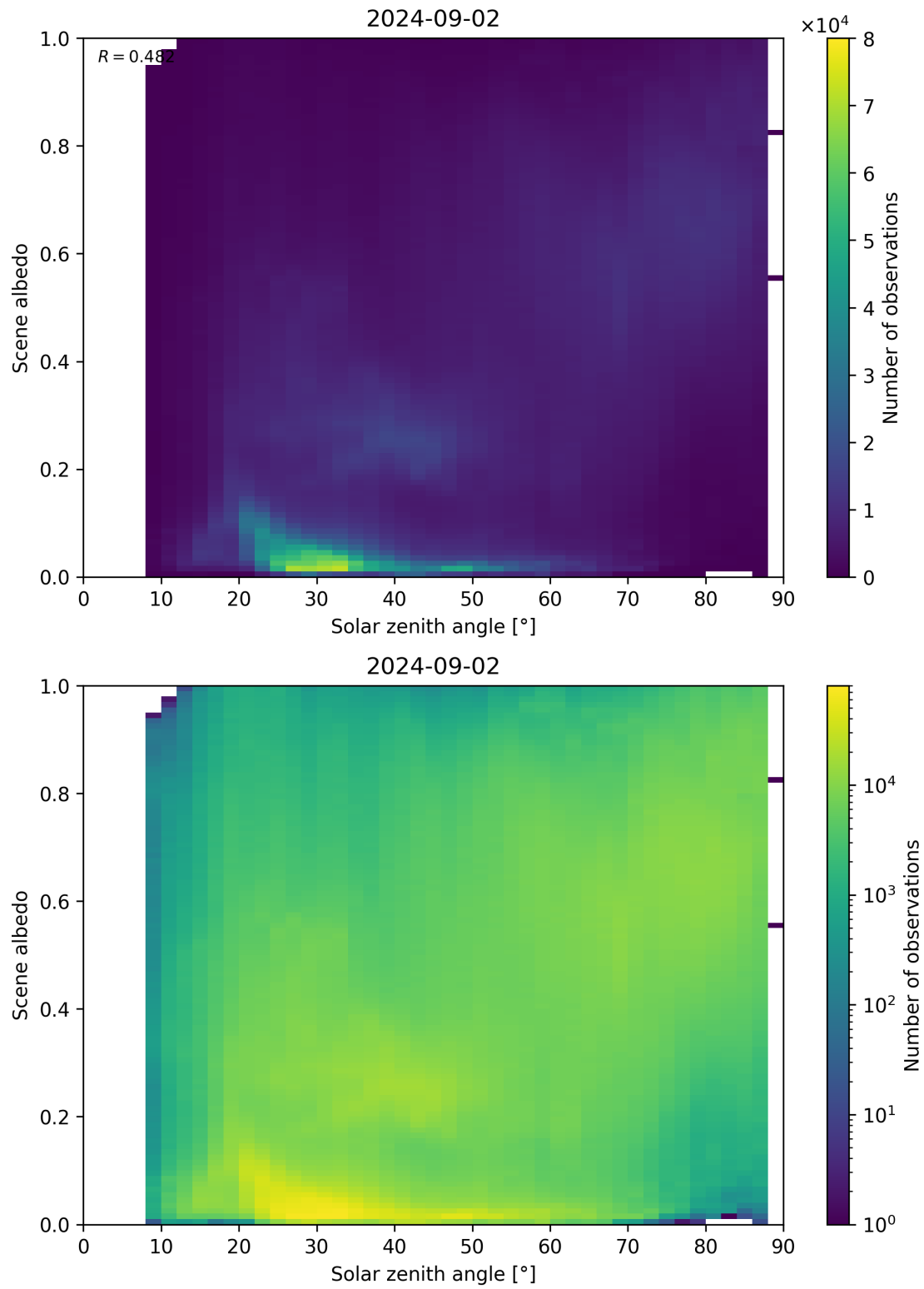
Figure 116: Scatter density plot of “Solar zenith angle” against “Scene albedo” for 2024-09-01 to 2024-09-03.
