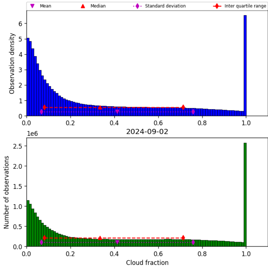
Figure 32: Histogram of “Cloud fraction” for 2024-09-01 to 2024-09-03
