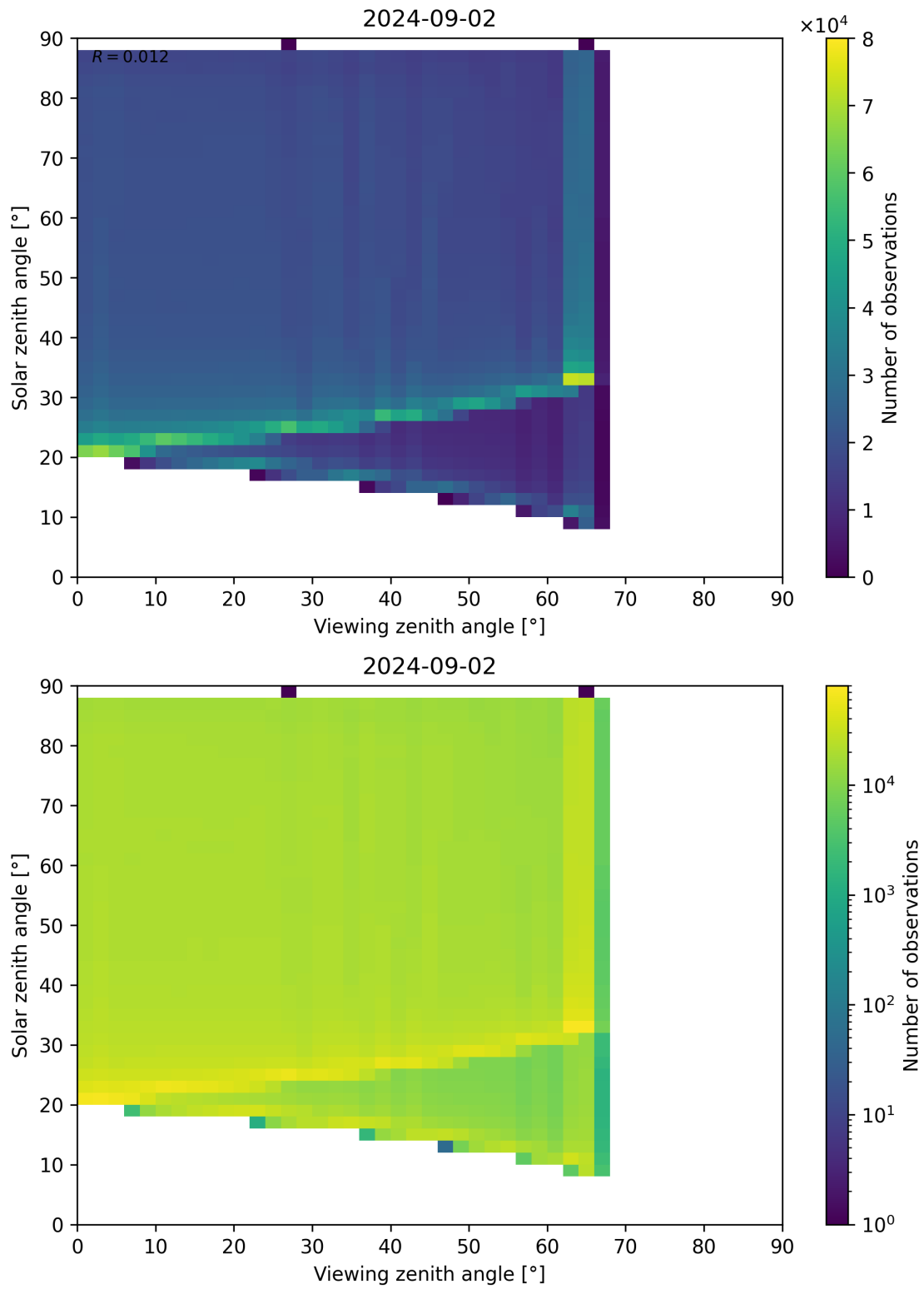
Figure 127: Scatter density plot of “Viewing zenith angle” against “Solar zenith angle” for 2024-09-01 to 2024-09-03.
