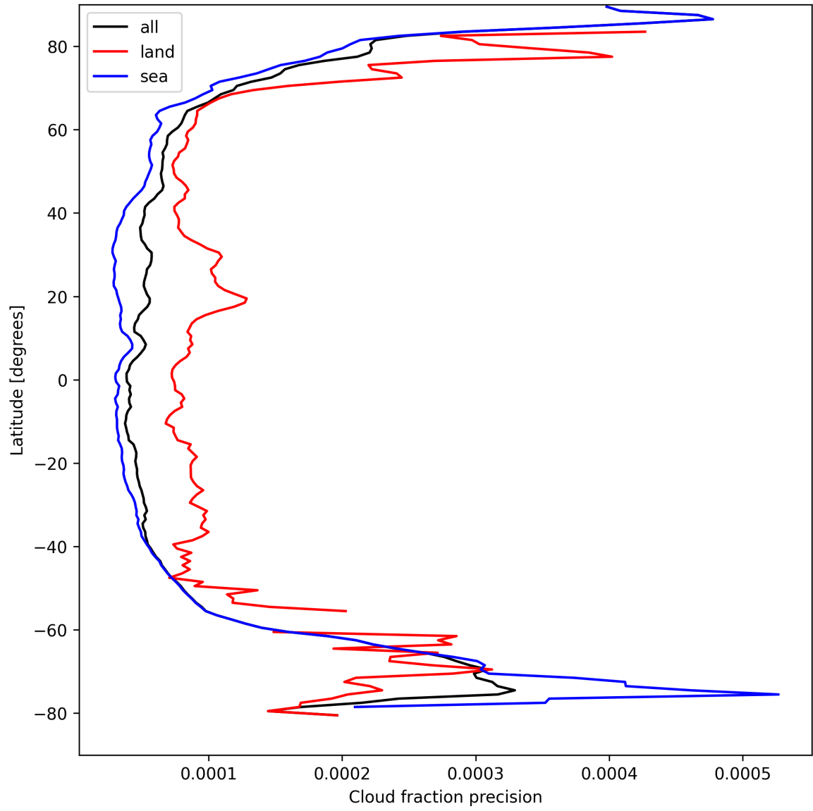
Figure 16: Zonal average of “Cloud fraction precision” for 2024-09-01 to 2024-09-03.
