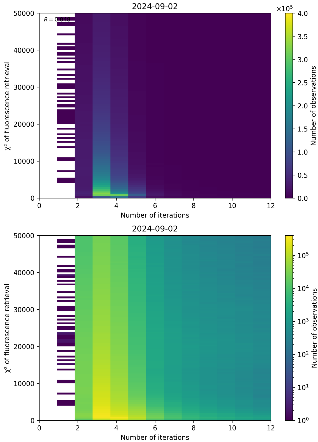
Figure 97: Scatter density plot of “Number of iterations” against “ \chi^2 of fluorescence retrieval” for 2024-09-01 to 2024-09-03.
