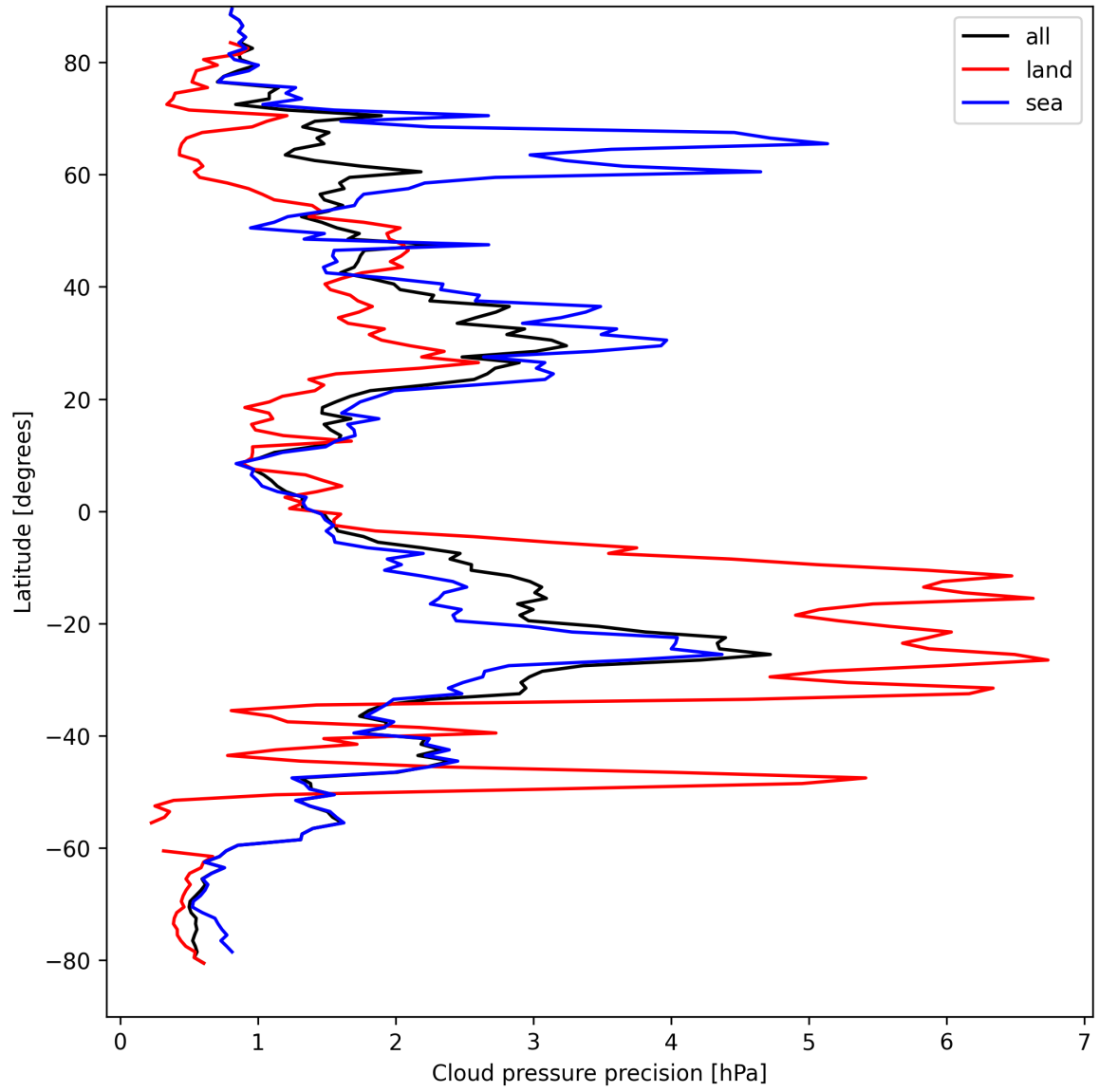
Figure 14: Zonal average of “Cloud pressure precision” for 2024-09-01 to 2024-09-03.
