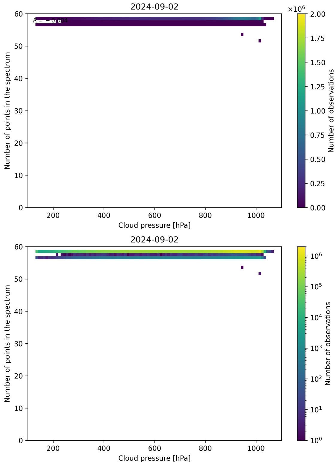
Figure 82: Scatter density plot of “Cloud pressure” against “Number of points in the spectrum” for 2024-09-01 to 2024-09-03.
