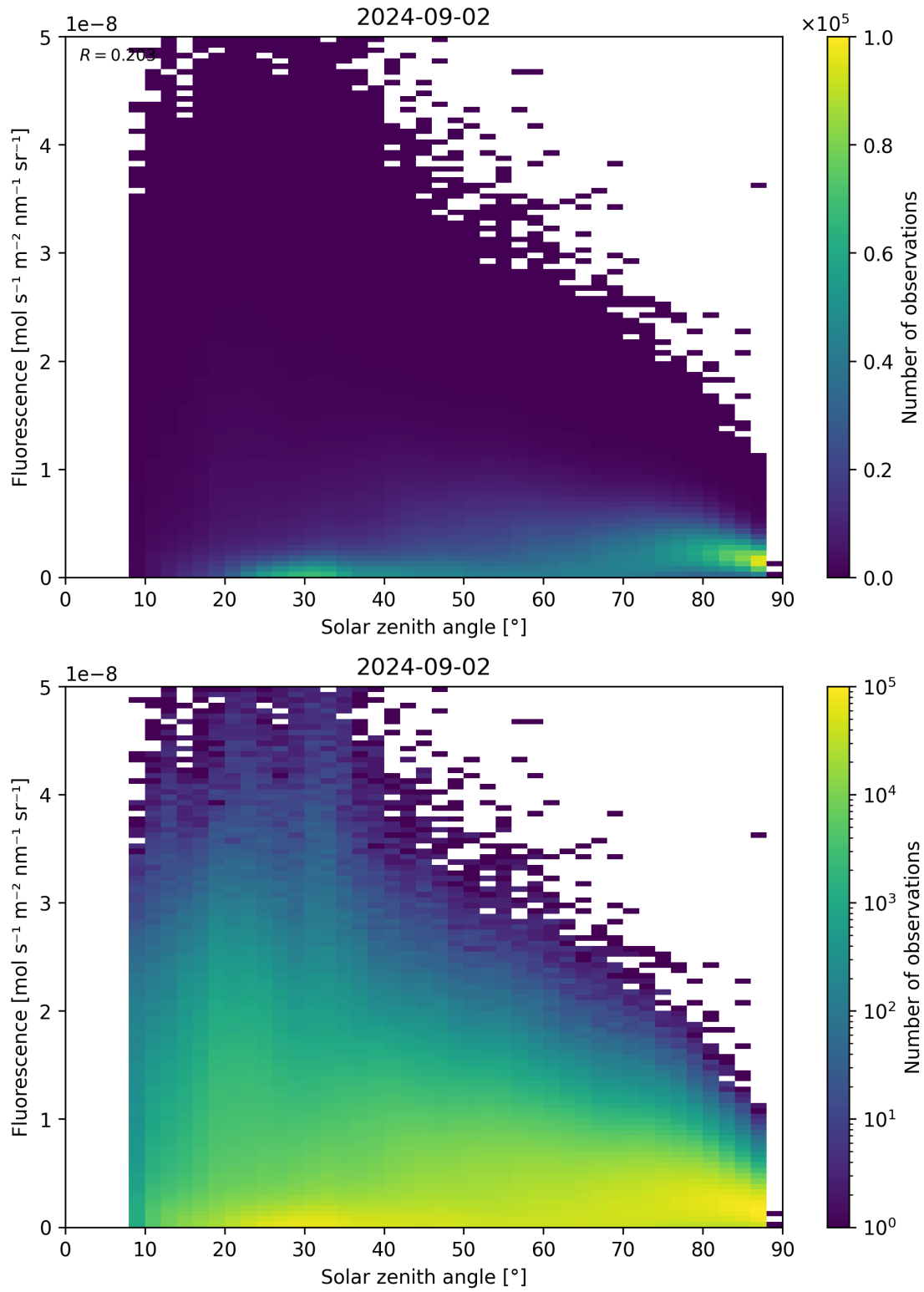
Figure 112: Scatter density plot of “Solar zenith angle” against “Fluorescence” for 2024-09-01 to 2024-09-03.
