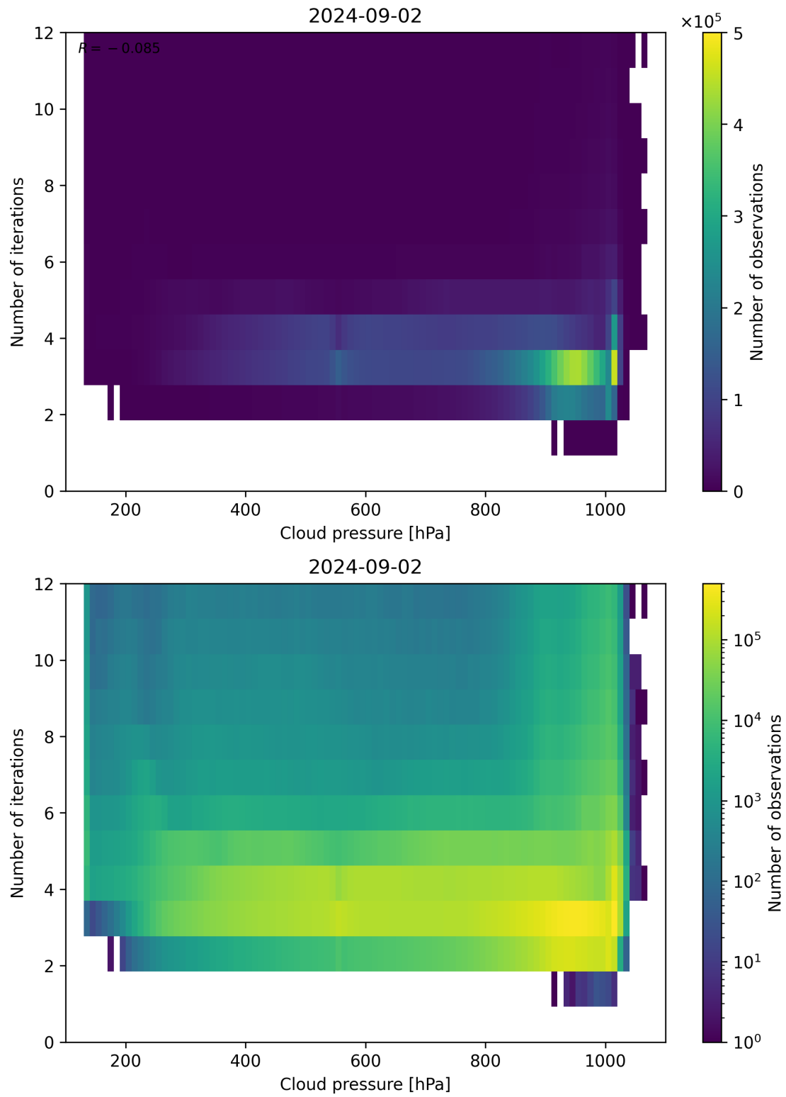
Figure 81: Scatter density plot of “Cloud pressure” against “Number of iterations” for 2024-09-01 to 2024-09-03.
