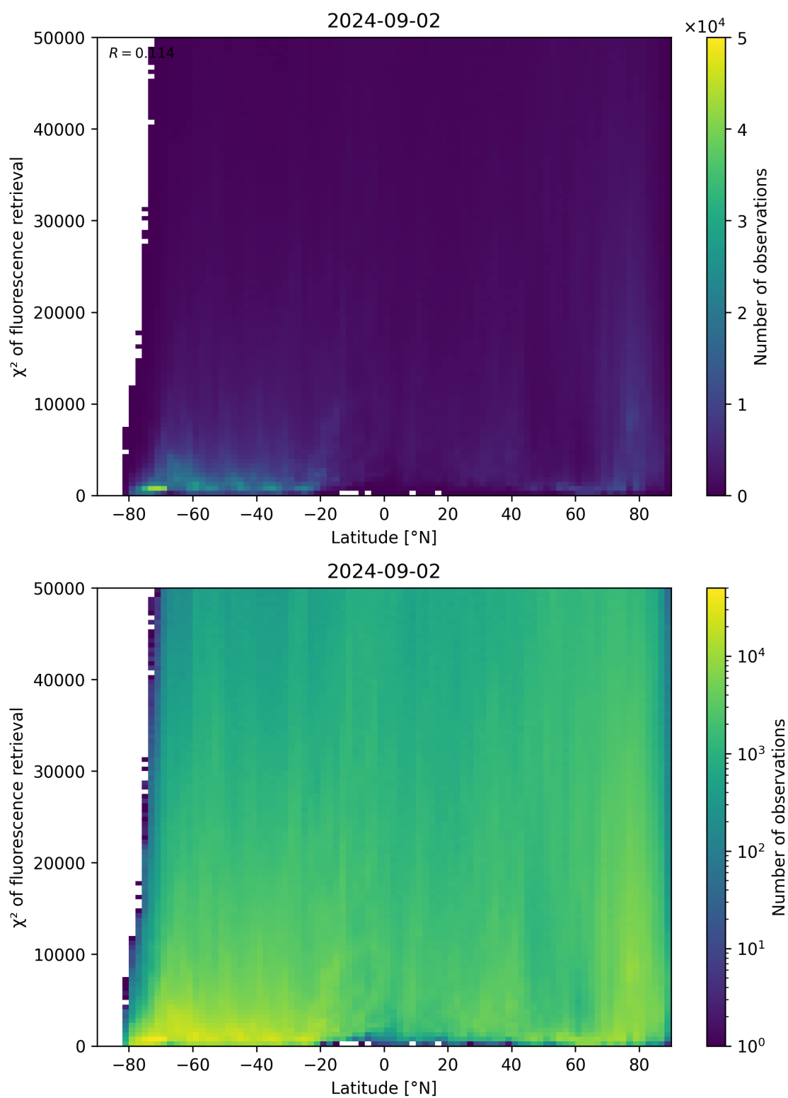
Figure 89: Scatter density plot of “Latitude” against “ \chi^2 of fluorescence retrieval” for 2024-09-01 to 2024-09-03.
