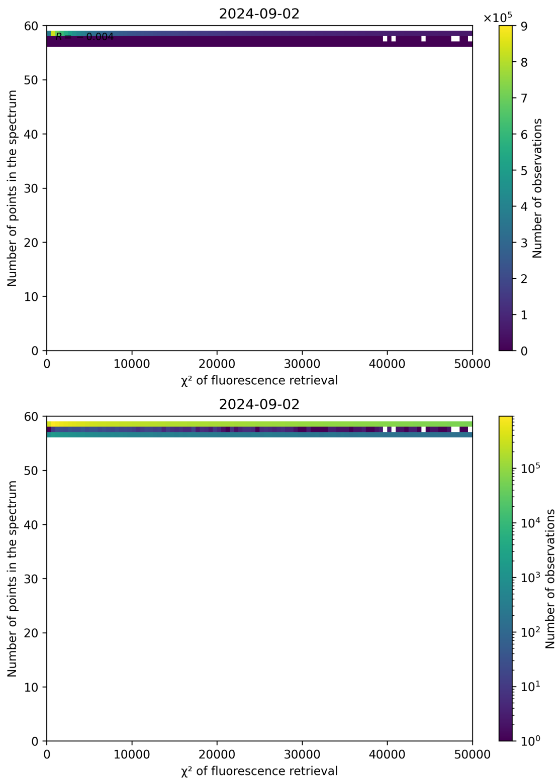
Figure 68: Scatter density plot of " \chi^2 of fluorescence retrieval" against "Number of points in the spectrum" for 2024-09-01 to 2024-09-03.
