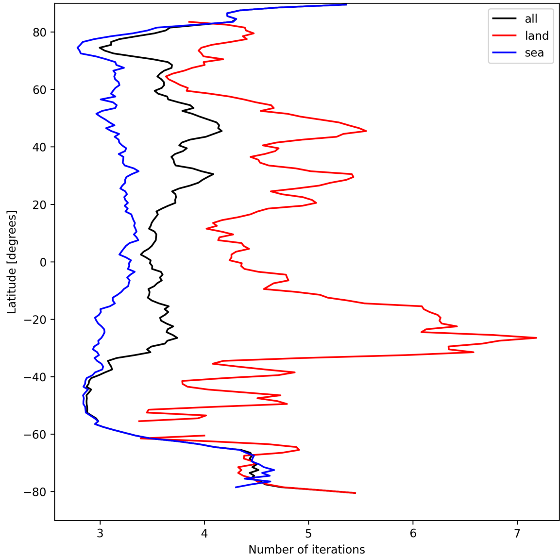
Figure 22: Zonal average of “Number of iterations” for 2024-09-01 to 2024-09-03.
