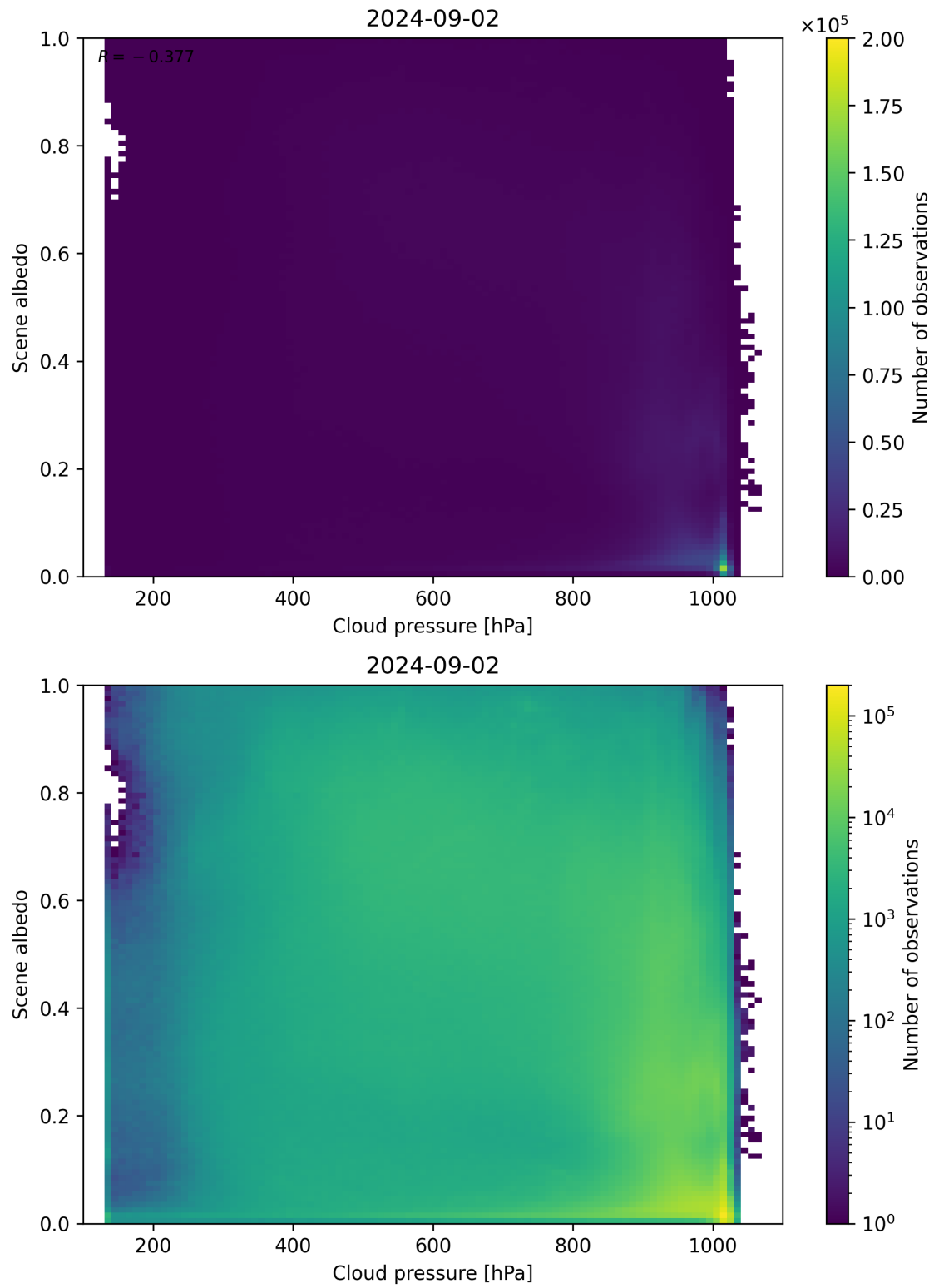
Figure 83: Scatter density plot of “Cloud pressure” against “Scene albedo” for 2024-09-01 to 2024-09-03.
