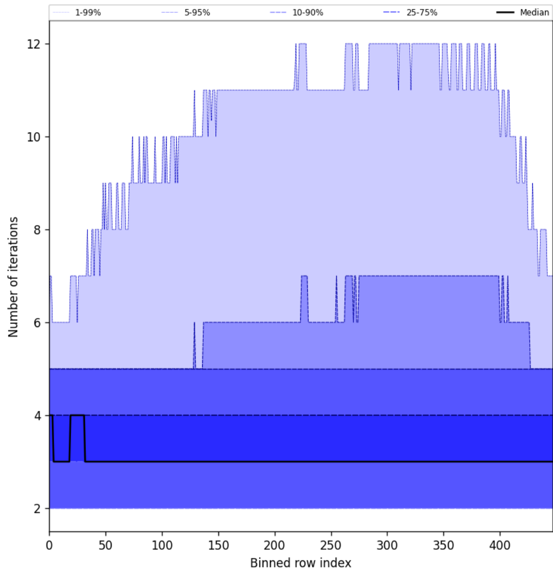
Figure 56: Along track statistics of “Number of iterations” for 2024-09-01 to 2024-09-03
