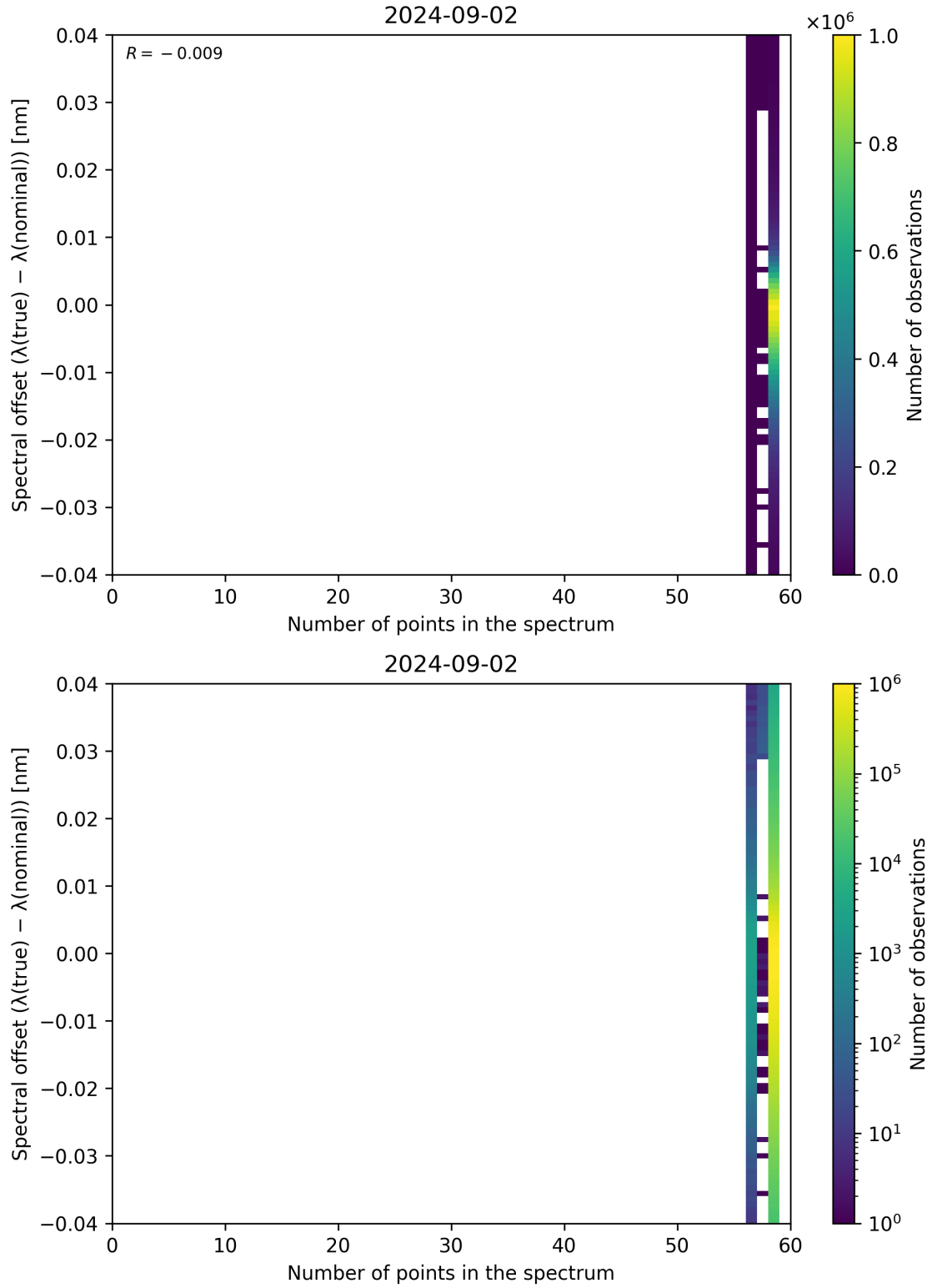
Figure 101: Scatter density plot of “Number of points in the spectrum” against “Spectral offset ( \lambda_{\text{true}} - \lambda_{\text{nominal}} )” for 2024-09-01 to 2024-09-03.
