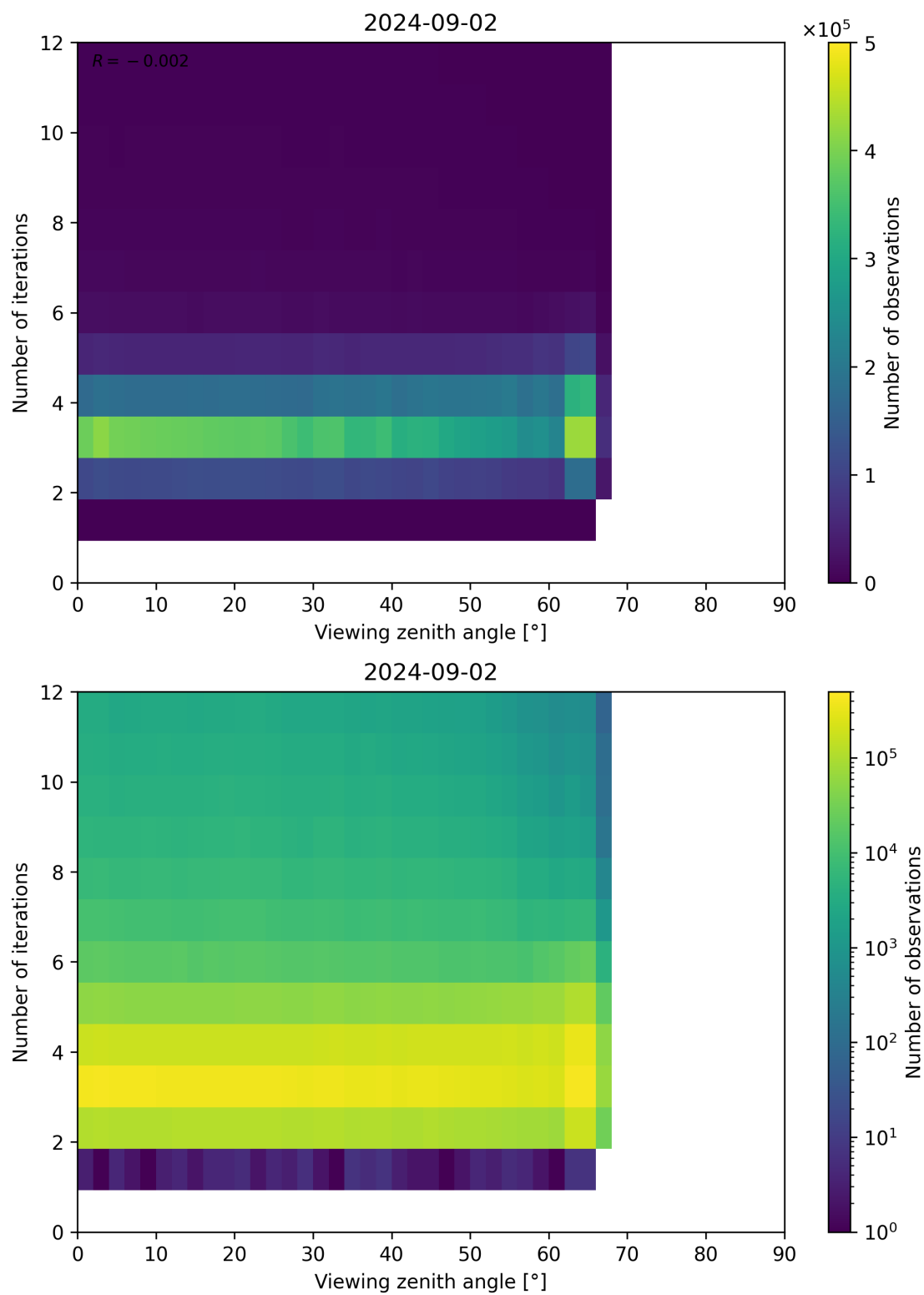
Figure 124: Scatter density plot of “Viewing zenith angle” against “Number of iterations” for 2024-09-01 to 2024-09-03.
