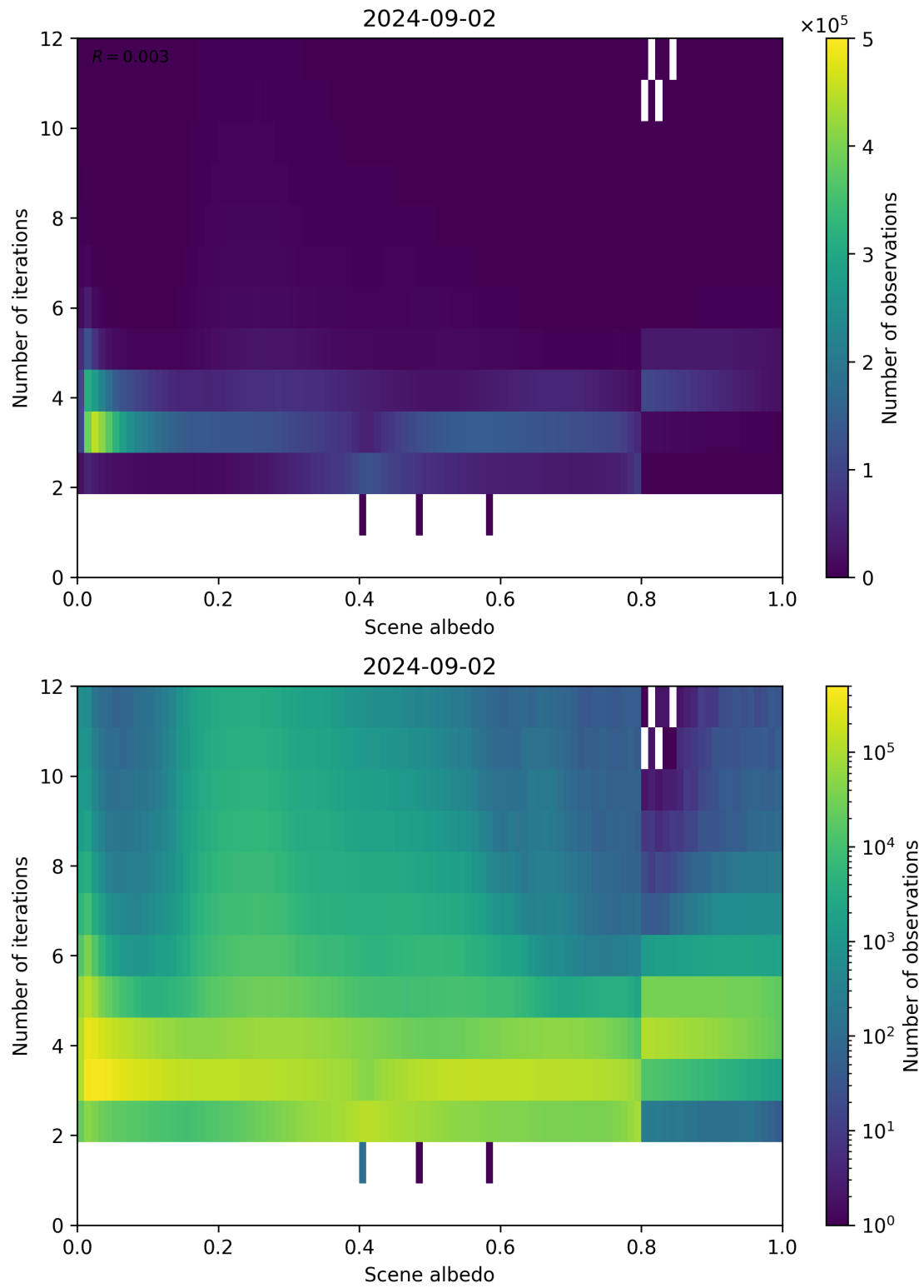
Figure 105: Scatter density plot of “Scene albedo” against “Number of iterations” for 2024-09-01 to 2024-09-03.
