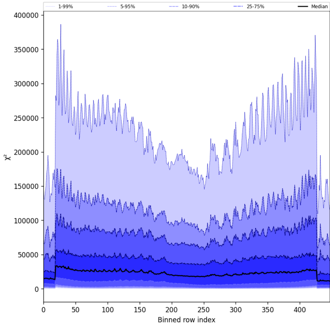
Figure 55: Along track statistics of “ \chi^2 ” for 2024-09-01 to 2024-09-03
