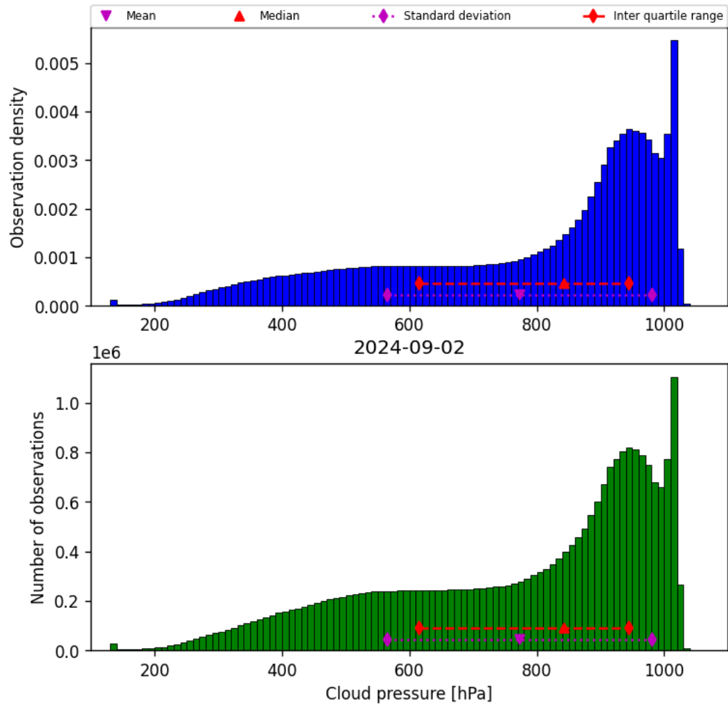
Figure 30: Histogram of “Cloud pressure” for 2024-09-01 to 2024-09-03
