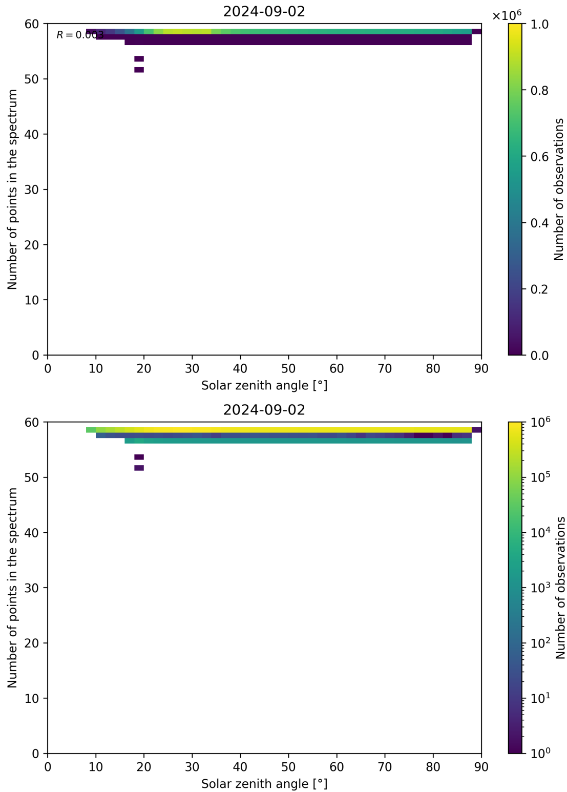
Figure 115: Scatter density plot of “Solar zenith angle” against “Number of points in the spectrum” for 2024-09-01 to 2024-09-03.
