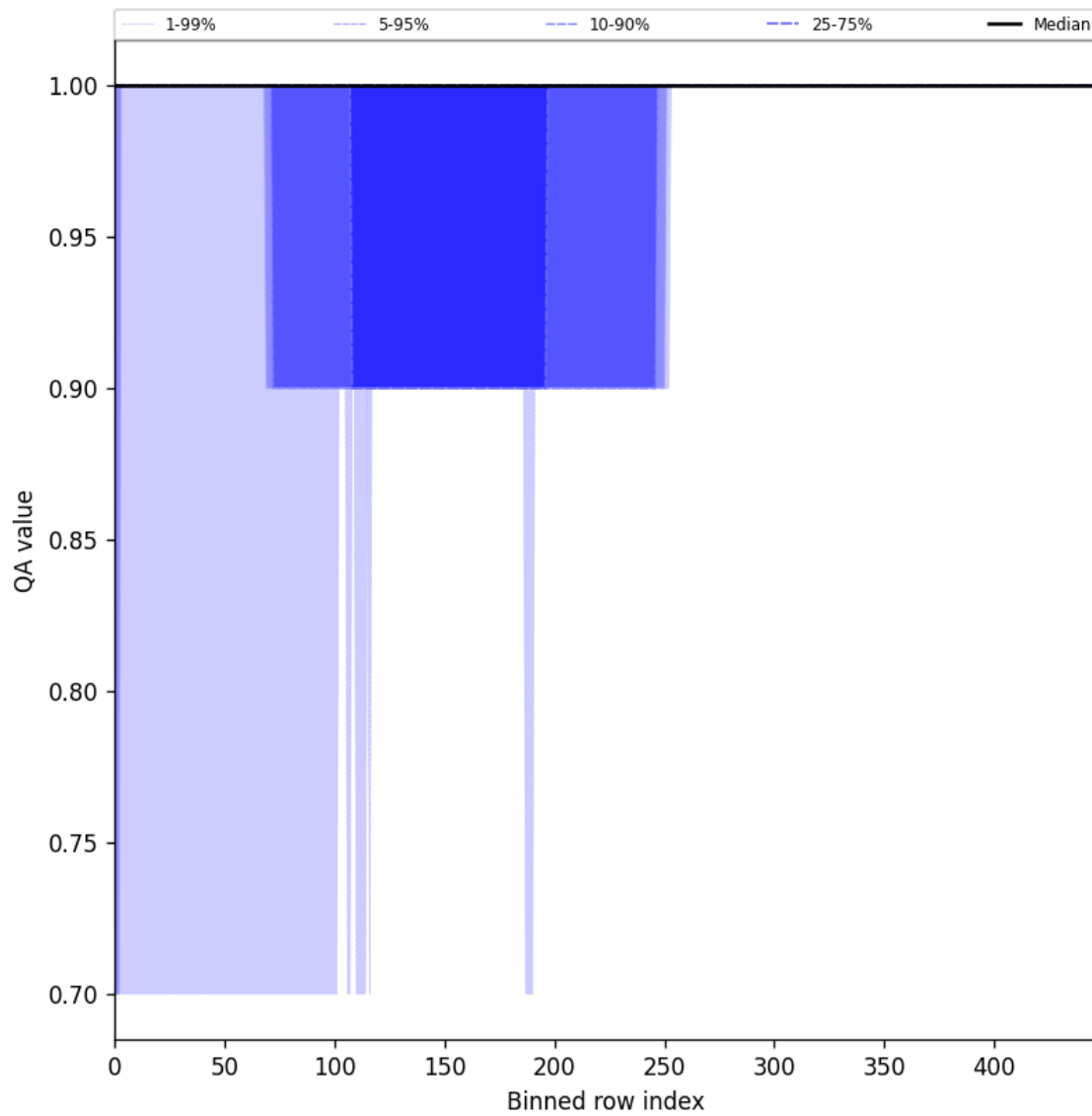
Figure 46: Along track statistics of “QA value” for 2024-09-01 to 2024-09-03
