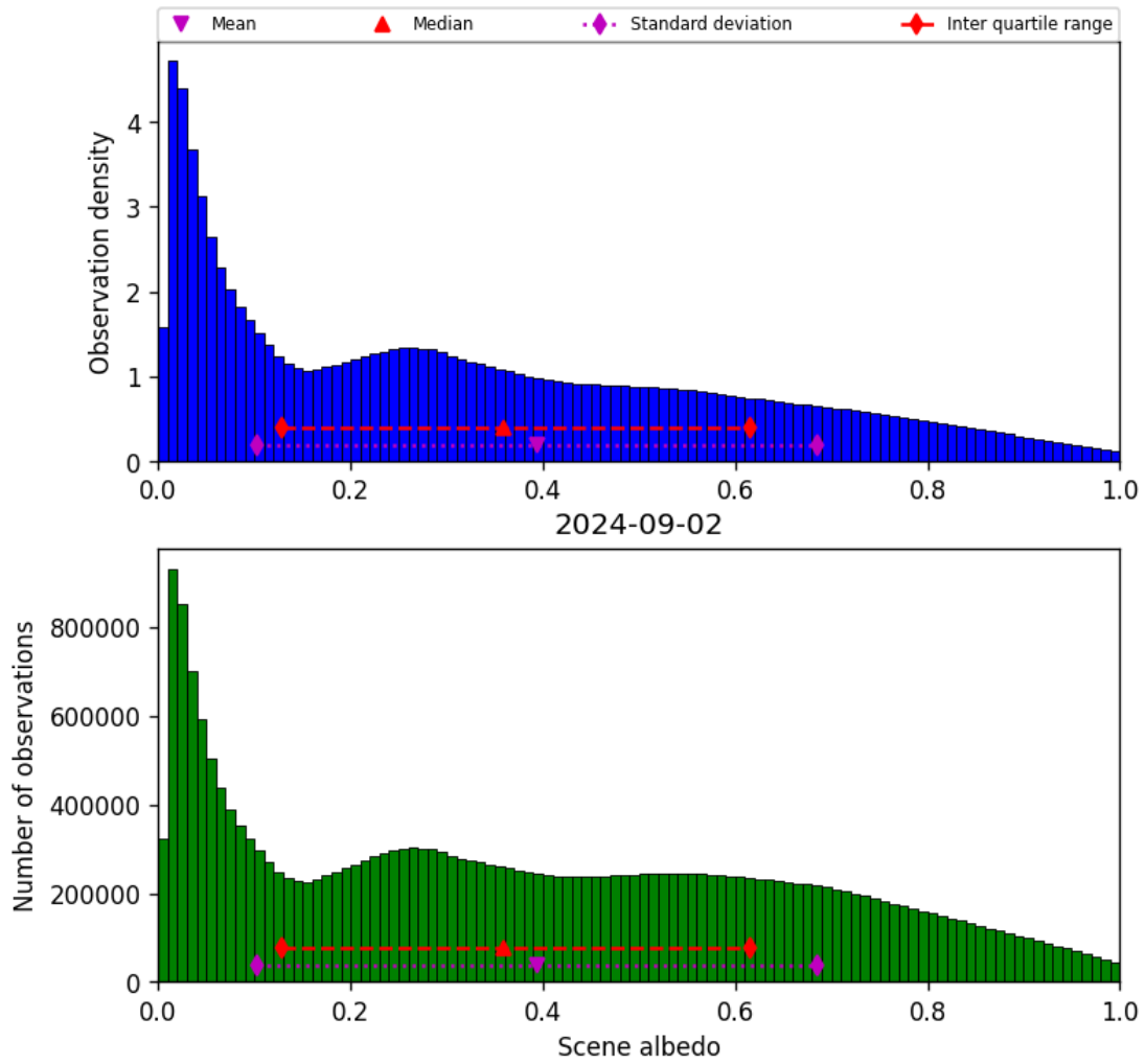
Figure 34: Histogram of “Scene albedo” for 2024-09-01 to 2024-09-03
