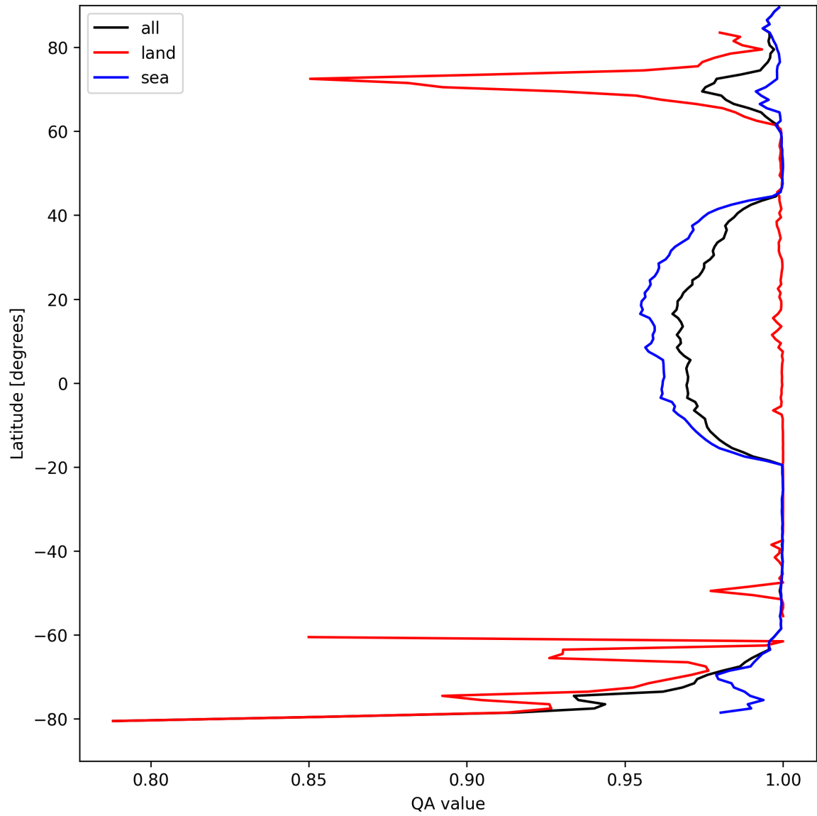
Figure 12: Zonal average of "QA value" for 2024-09-01 to 2024-09-03.
