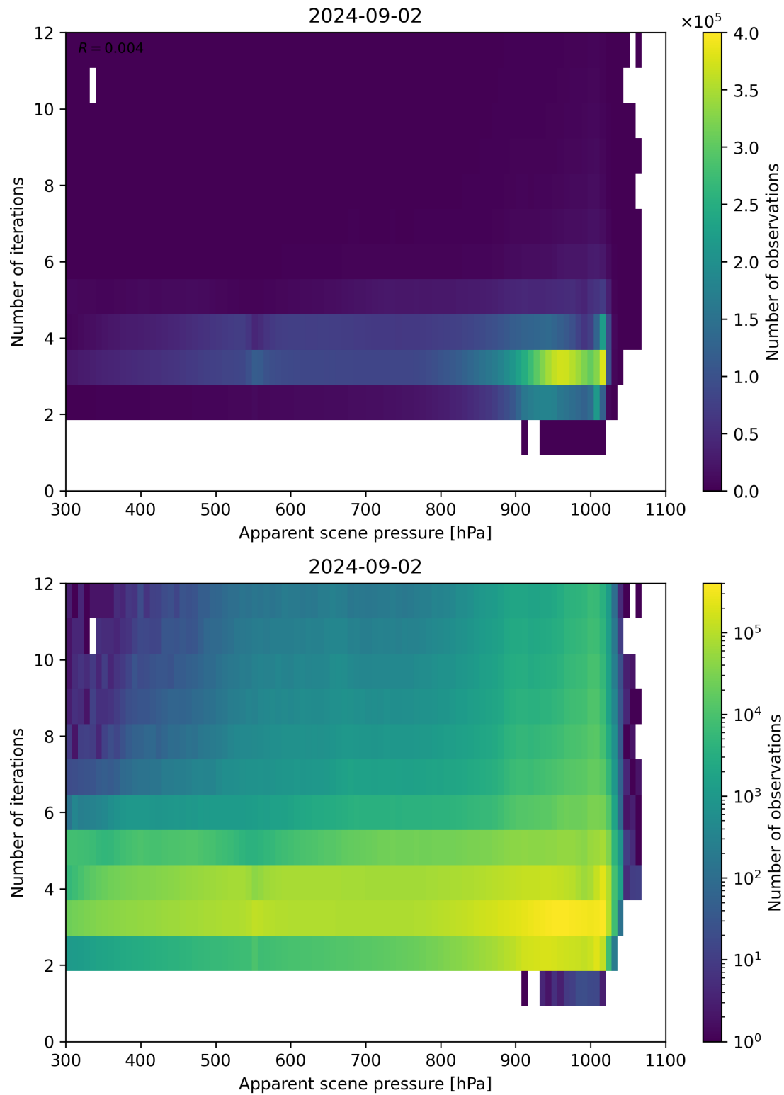
Figure 65: Scatter density plot of “Apparent scene pressure” against “Number of iterations” for 2024-09-01 to 2024-09-03.
