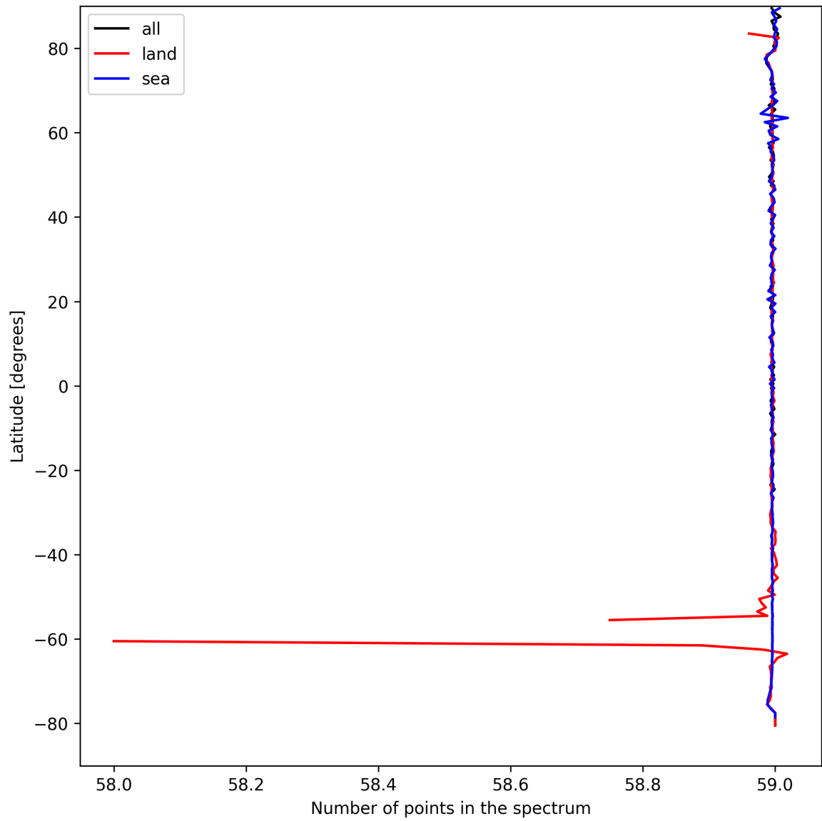
Figure 27: Zonal average of “Number of points in the spectrum” for 2024-09-01 to 2024-09-03.
