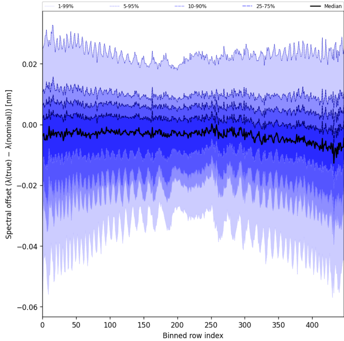
Figure 62: Along track statistics of “Spectral offset ( \lambda_{\text{true}} - \lambda_{\text{nominal}} )” for 2024-09-01 to 2024-09-03
