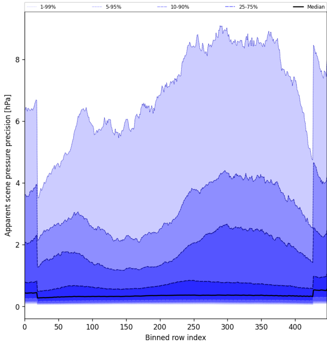
Figure 54: Along track statistics of “Apparent scene pressure precision” for 2024-09-01 to 2024-09-03
