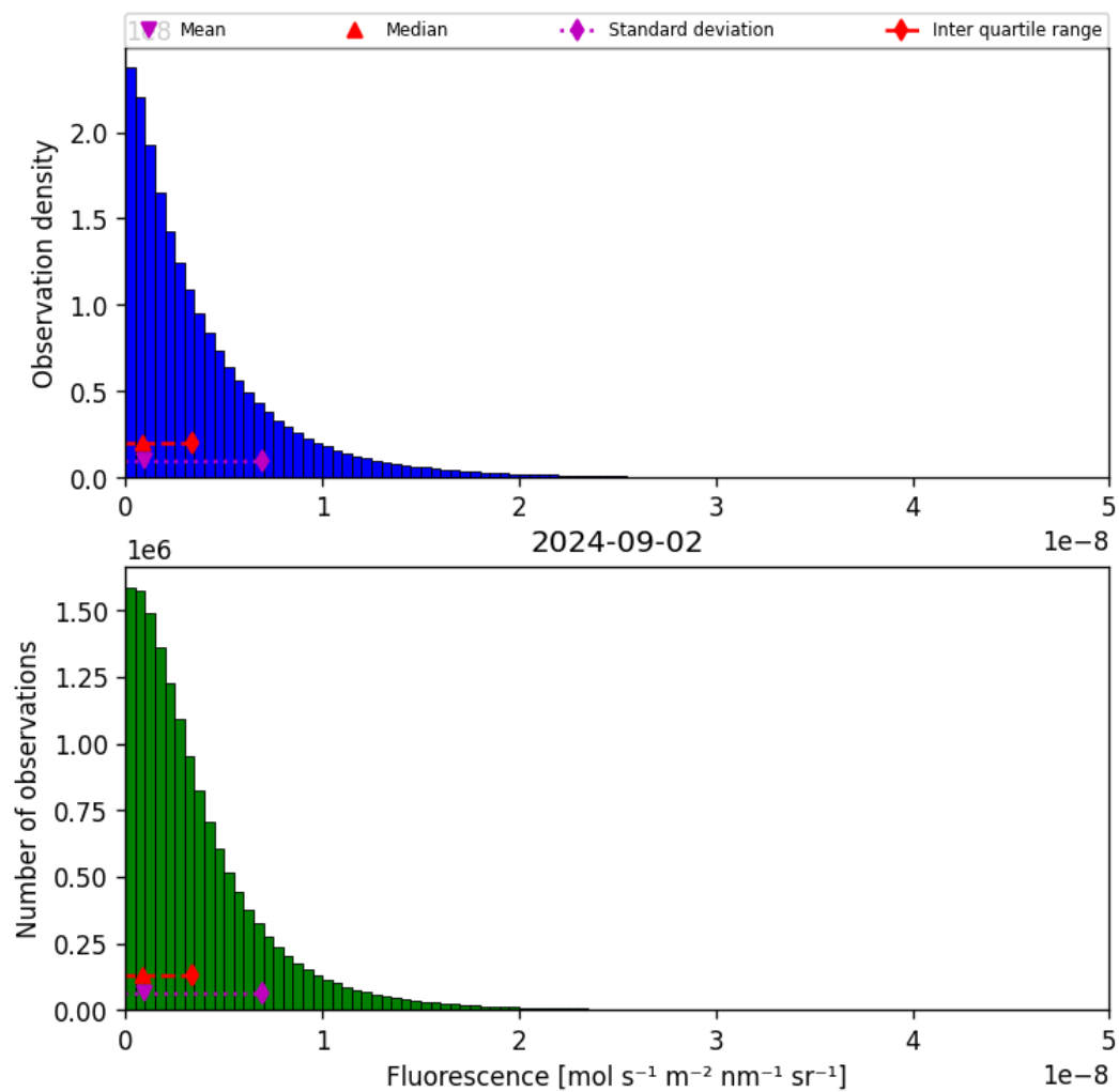
Figure 40: Histogram of “Fluorescence” for 2024-09-01 to 2024-09-03
