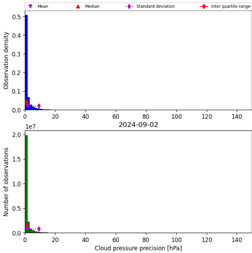
Figure 31: Histogram of “Cloud pressure precision” for 2024-09-01 to 2024-09-03
