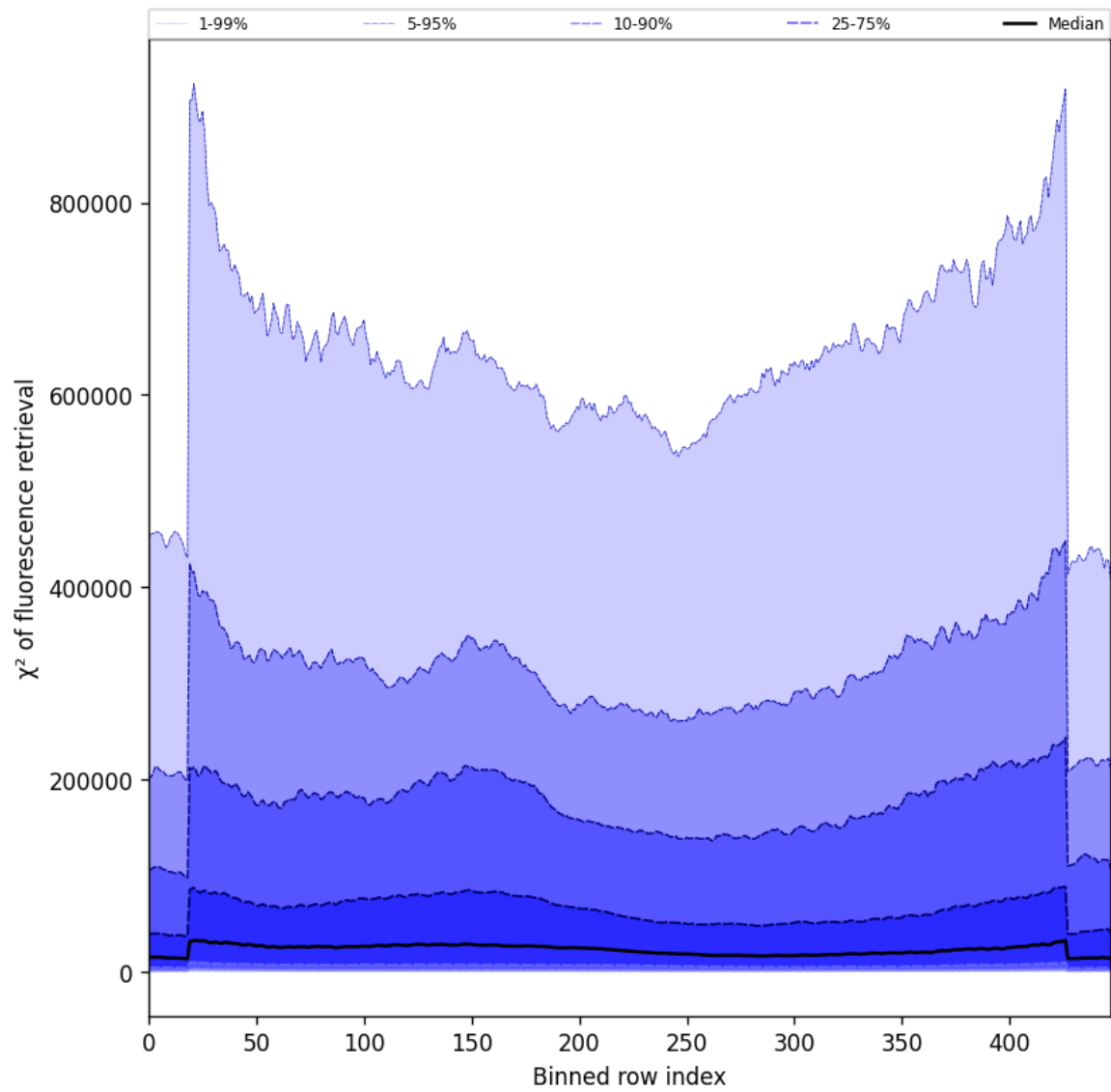
Figure 59: Along track statistics of “ \chi^2 of fluorescence retrieval” for 2024-09-01 to 2024-09-03
