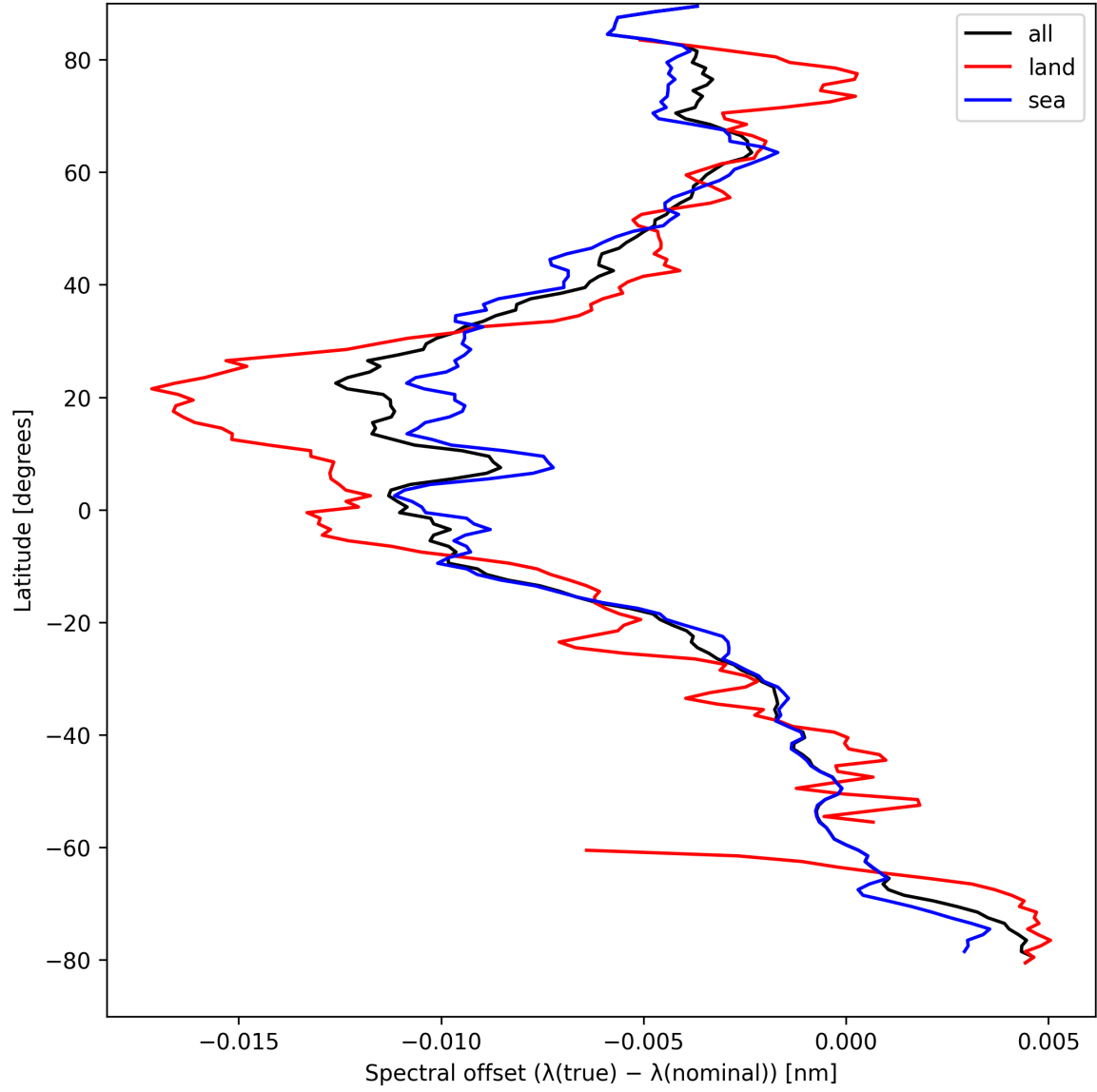
Figure 28: Zonal average of “Spectral offset ( \lambda_{\text{true}} - \lambda_{\text{nominal}} )” for 2024-09-01 to 2024-09-03.
