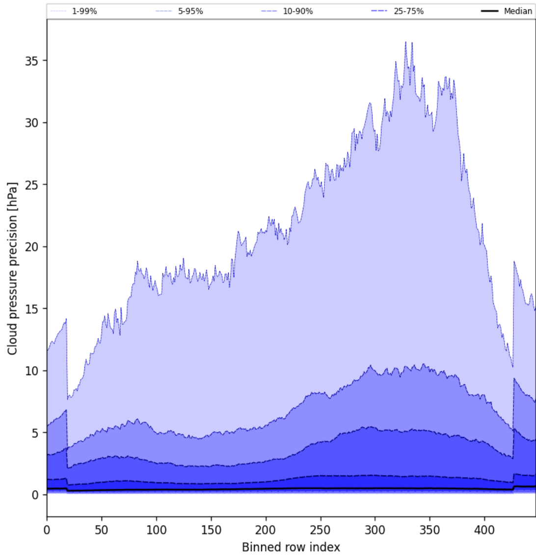
Figure 48: Along track statistics of “Cloud pressure precision” for 2024-09-01 to 2024-09-03
