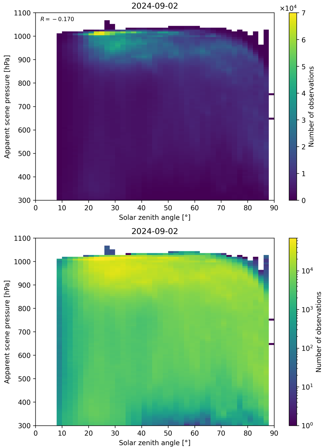
Figure 108: Scatter density plot of “Solar zenith angle” against “Apparent scene pressure” for 2024-09-01 to 2024-09-03.
