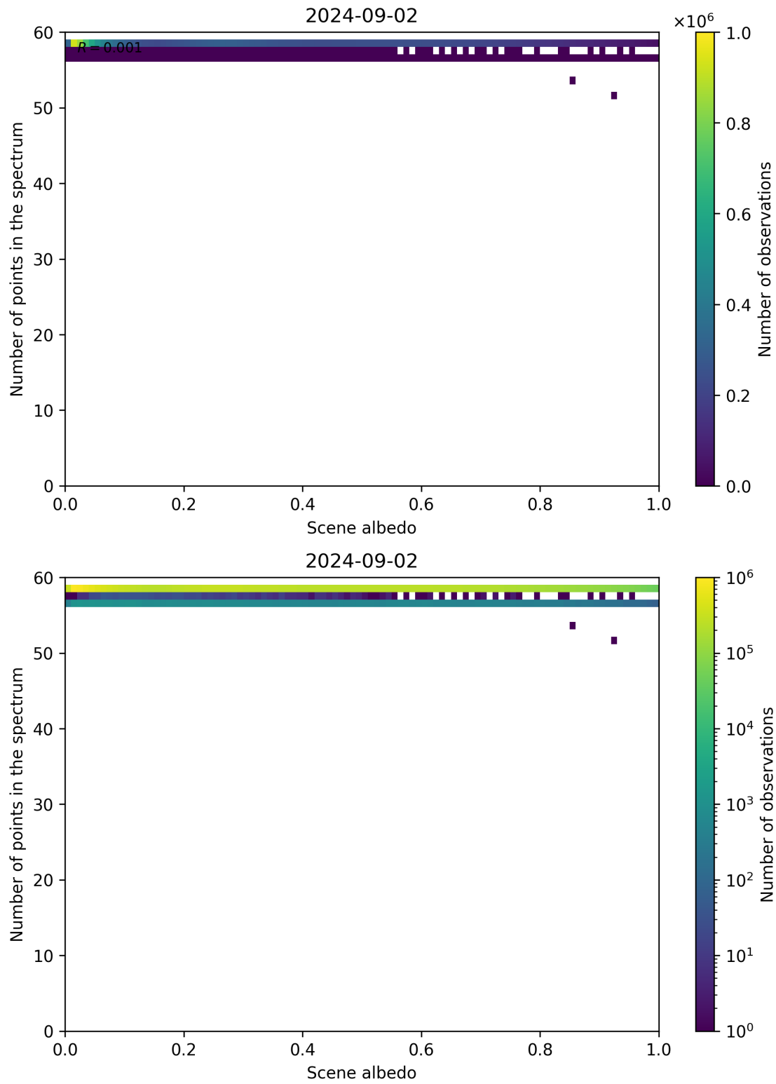
Figure 106: Scatter density plot of “Scene albedo” against “Number of points in the spectrum” for 2024-09-01 to 2024-09-03.
