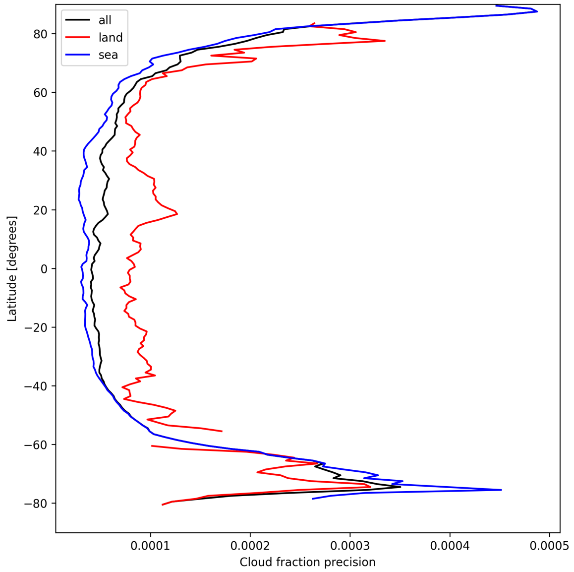
Figure 16: Zonal average of “Cloud fraction precision” for 2024-09-02 to 2024-09-04.
