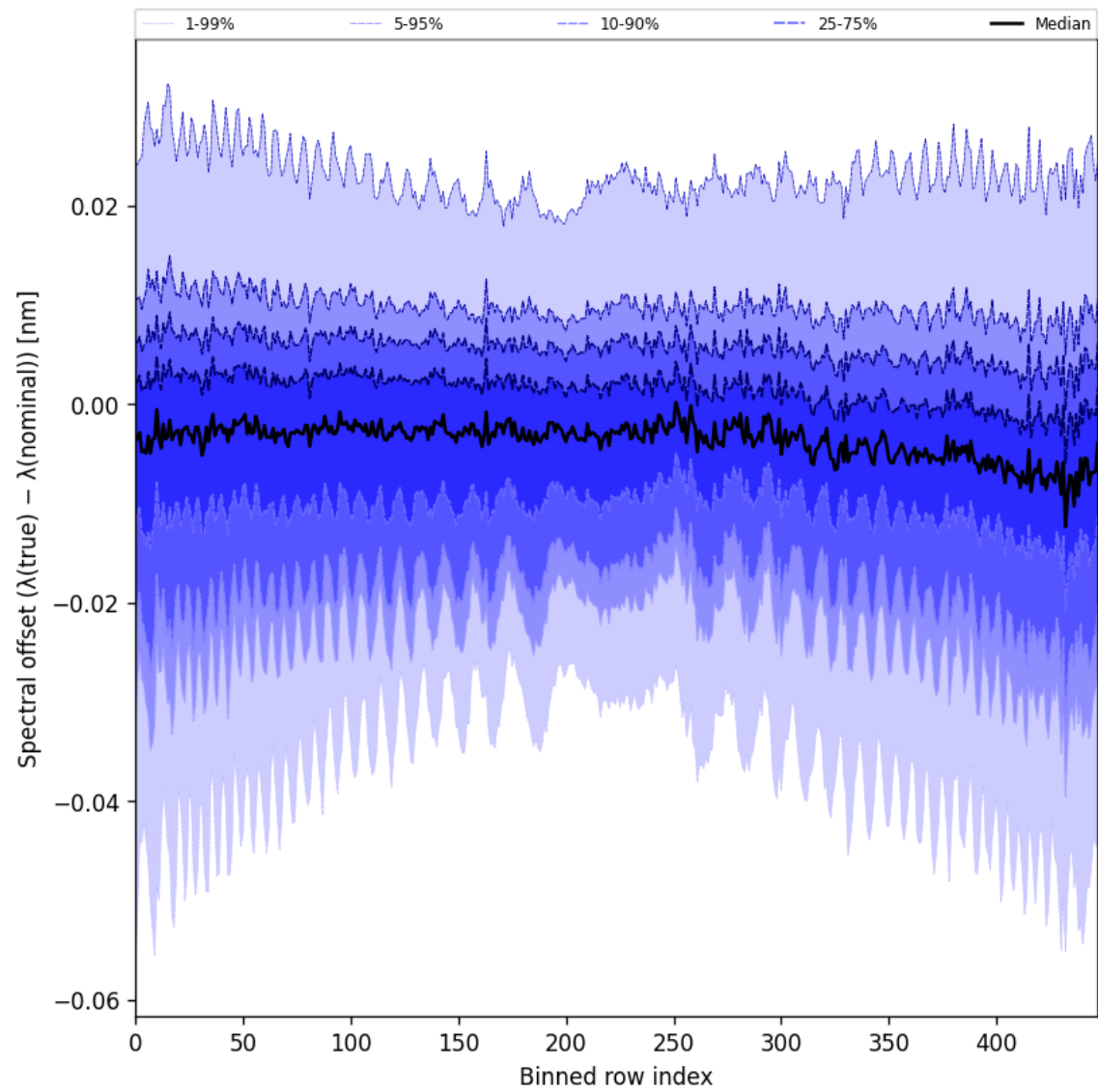
Figure 62: Along track statistics of “Spectral offset ( \lambda_{\text{true}} - \lambda_{\text{nominal}} )” for 2024-09-02 to 2024-09-04
