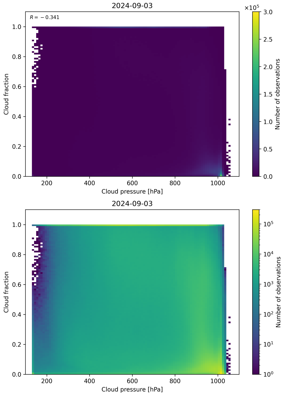
Figure 79: Scatter density plot of “Cloud pressure” against “Cloud fraction” for 2024-09-02 to 2024-09-04.
