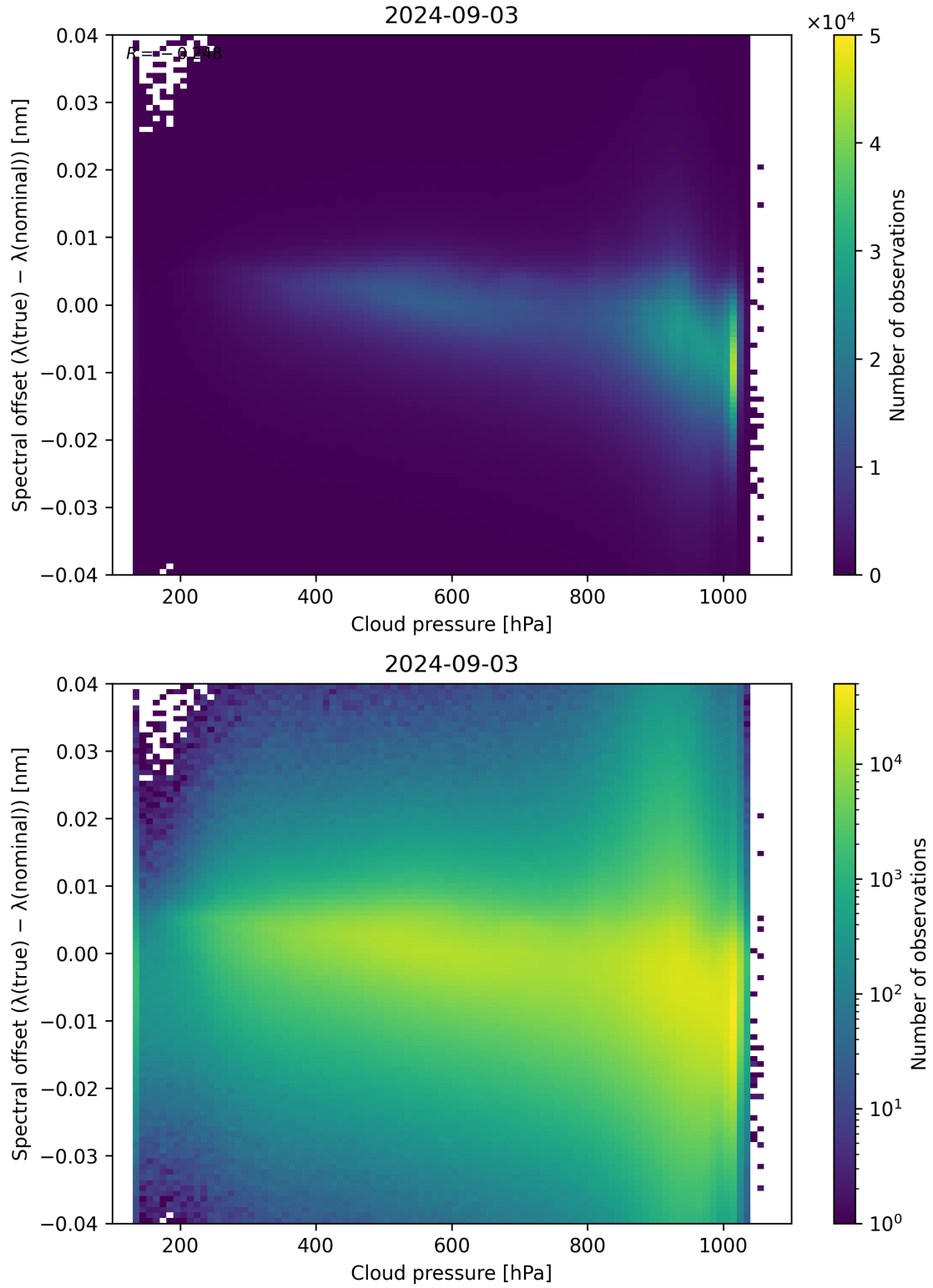
Figure 84: Scatter density plot of “Cloud pressure” against “Spectral offset ( \lambda_{\text{true}} - \lambda_{\text{nominal}} )” for 2024-09-02 to 2024-09-04.
