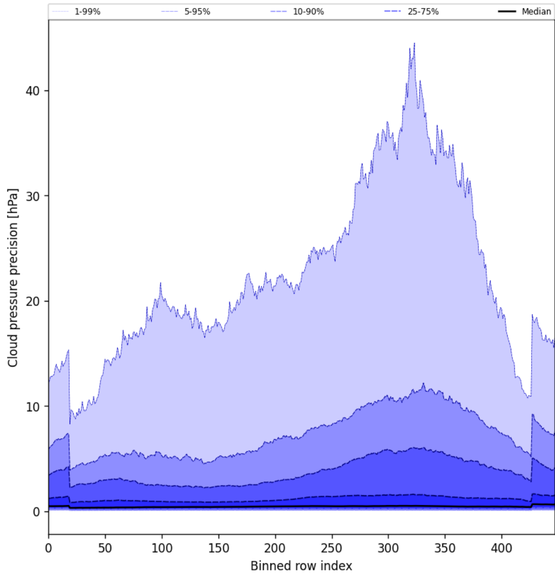
Figure 48: Along track statistics of “Cloud pressure precision” for 2024-09-02 to 2024-09-04
