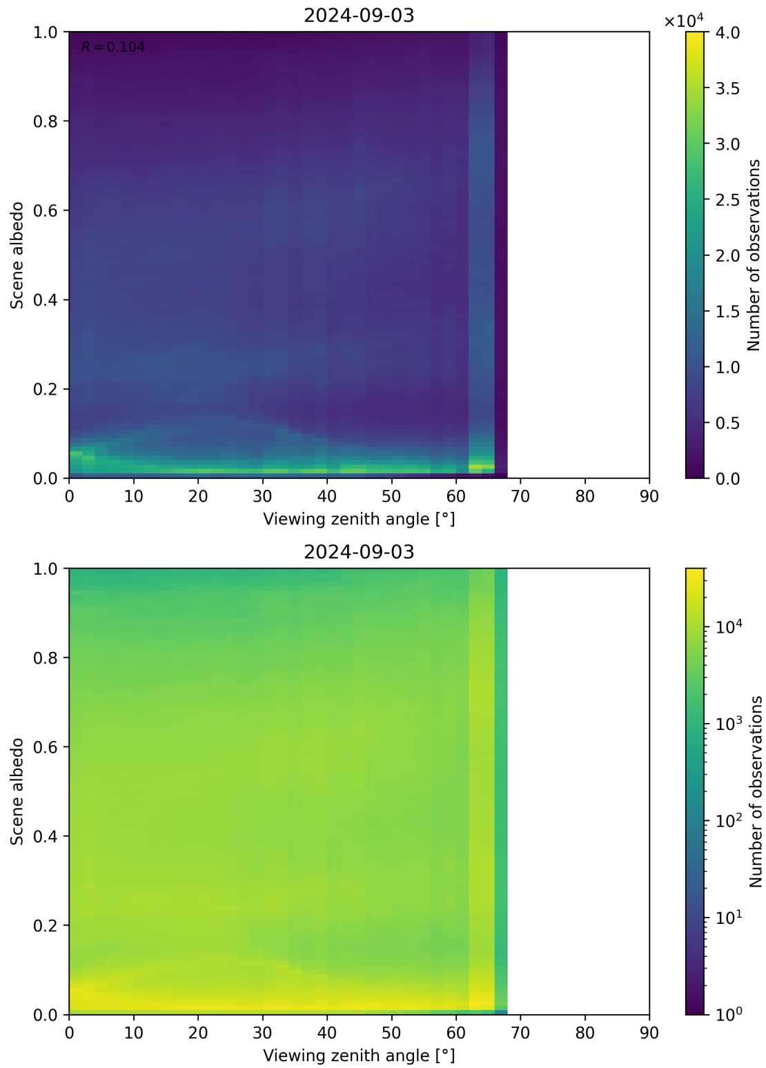
Figure 126: Scatter density plot of “Viewing zenith angle” against “Scene albedo” for 2024-09-02 to 2024-09-04.
