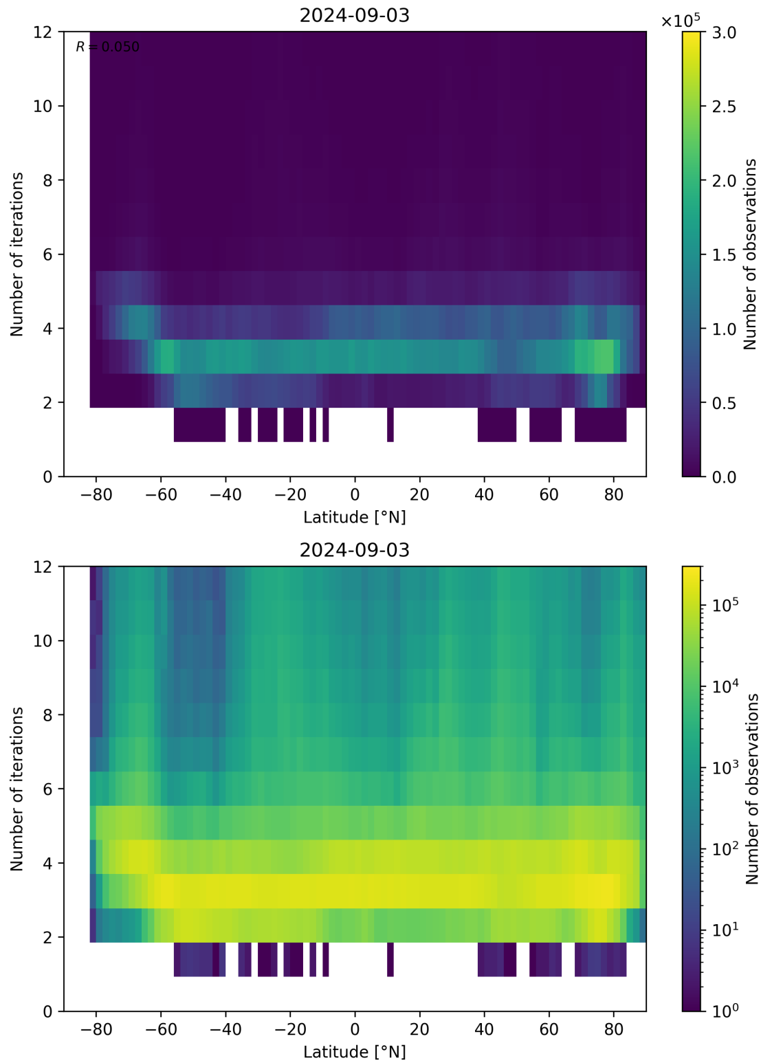
Figure 93: Scatter density plot of “Latitude” against “Number of iterations” for 2024-09-02 to 2024-09-04.
