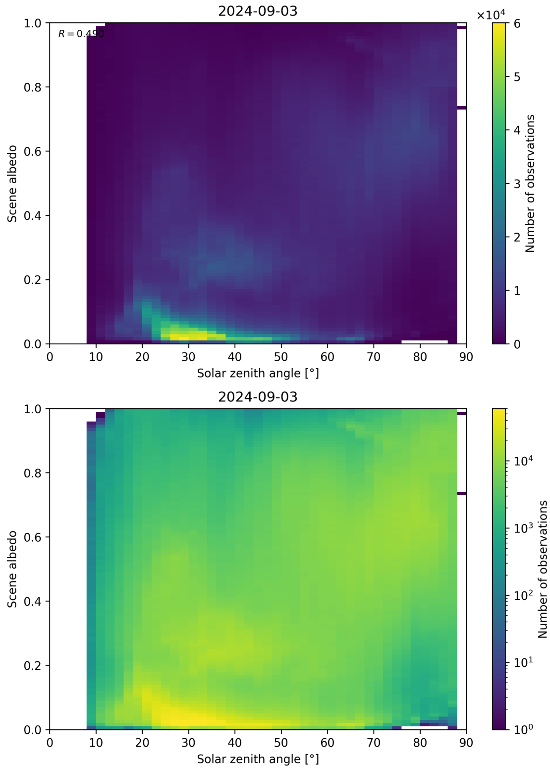
Figure 116: Scatter density plot of “Solar zenith angle” against “Scene albedo” for 2024-09-02 to 2024-09-04.
