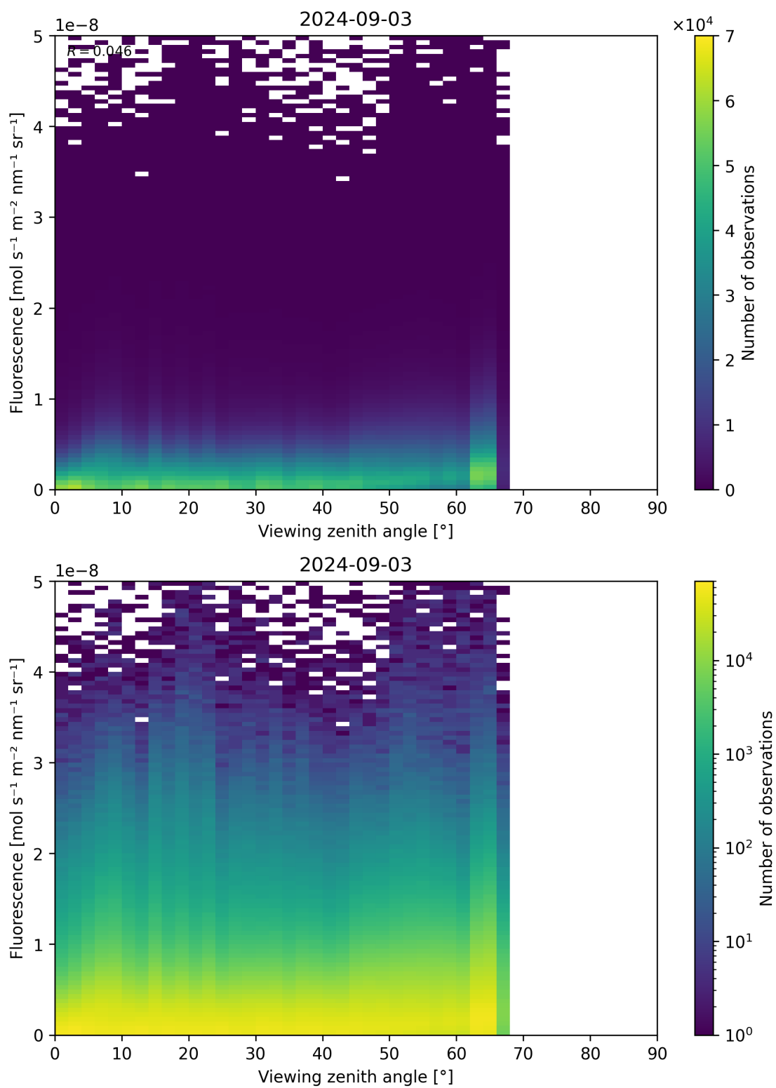
Figure 122: Scatter density plot of “Viewing zenith angle” against “Fluorescence” for 2024-09-02 to 2024-09-04.
