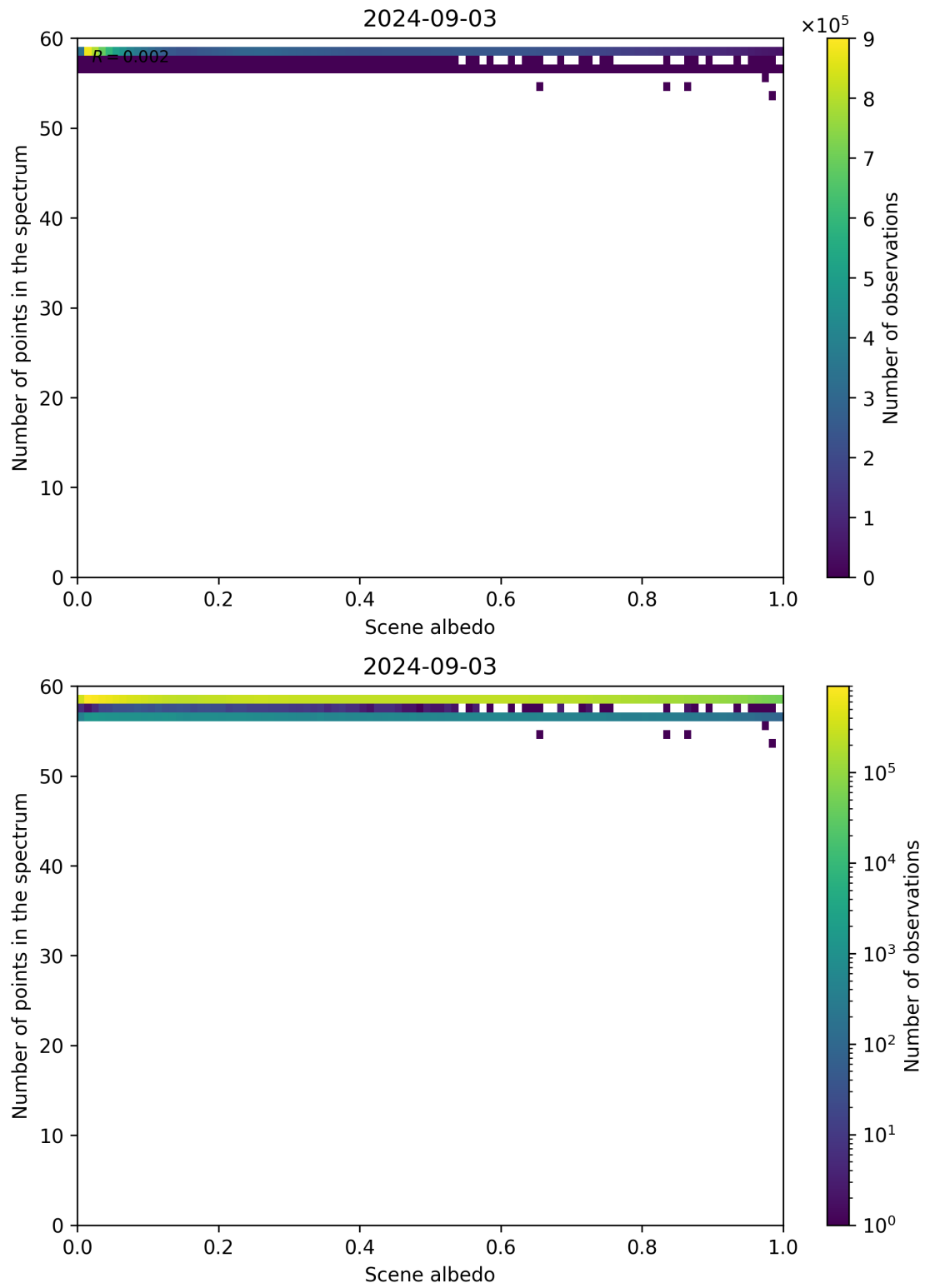
Figure 106: Scatter density plot of “Scene albedo” against “Number of points in the spectrum” for 2024-09-02 to 2024-09-04.
