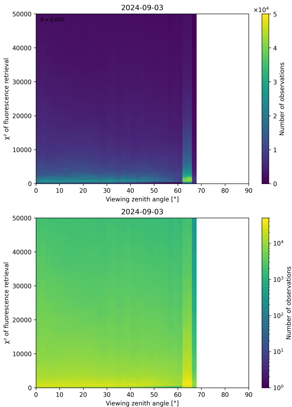
Figure 119: Scatter density plot of “Viewing zenith angle” against “ \chi^2 of fluorescence retrieval” for 2024-09-02 to 2024-09-04.
