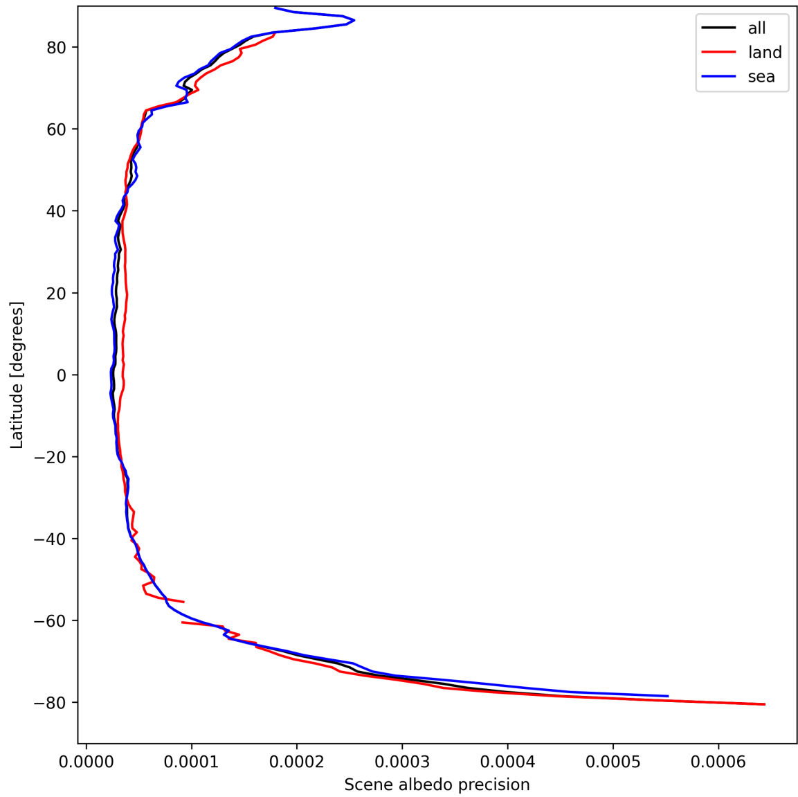
Figure 18: Zonal average of “Scene albedo precision” for 2024-09-02 to 2024-09-04.
