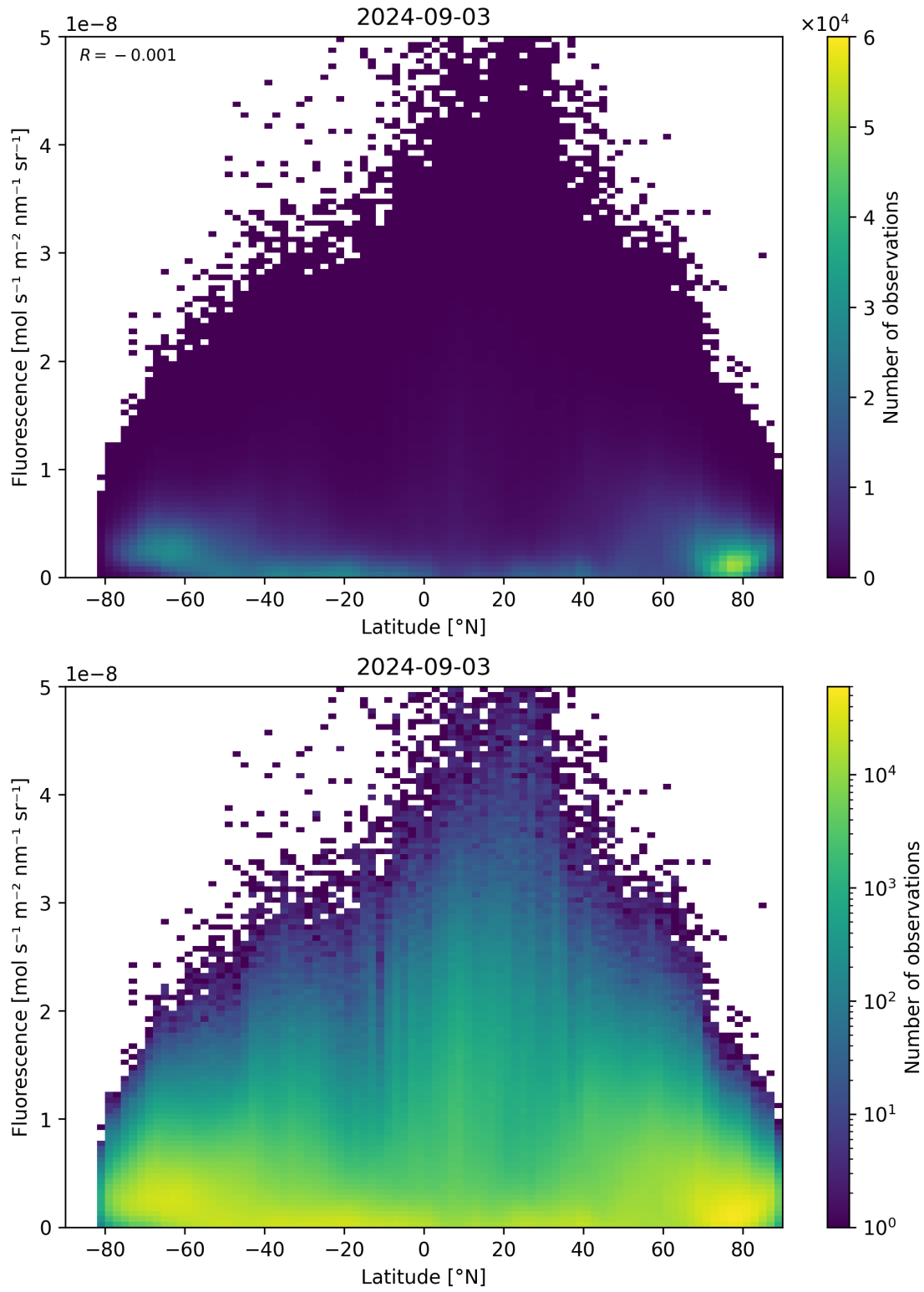
Figure 92: Scatter density plot of “Latitude” against “Fluorescence” for 2024-09-02 to 2024-09-04.
