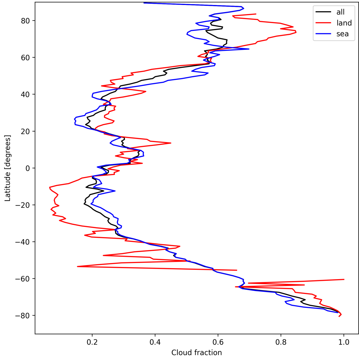
Figure 15: Zonal average of “Cloud fraction” for 2024-09-02 to 2024-09-04.
