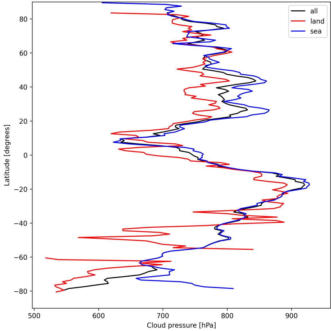
Figure 13: Zonal average of “Cloud pressure” for 2024-09-02 to 2024-09-04.
