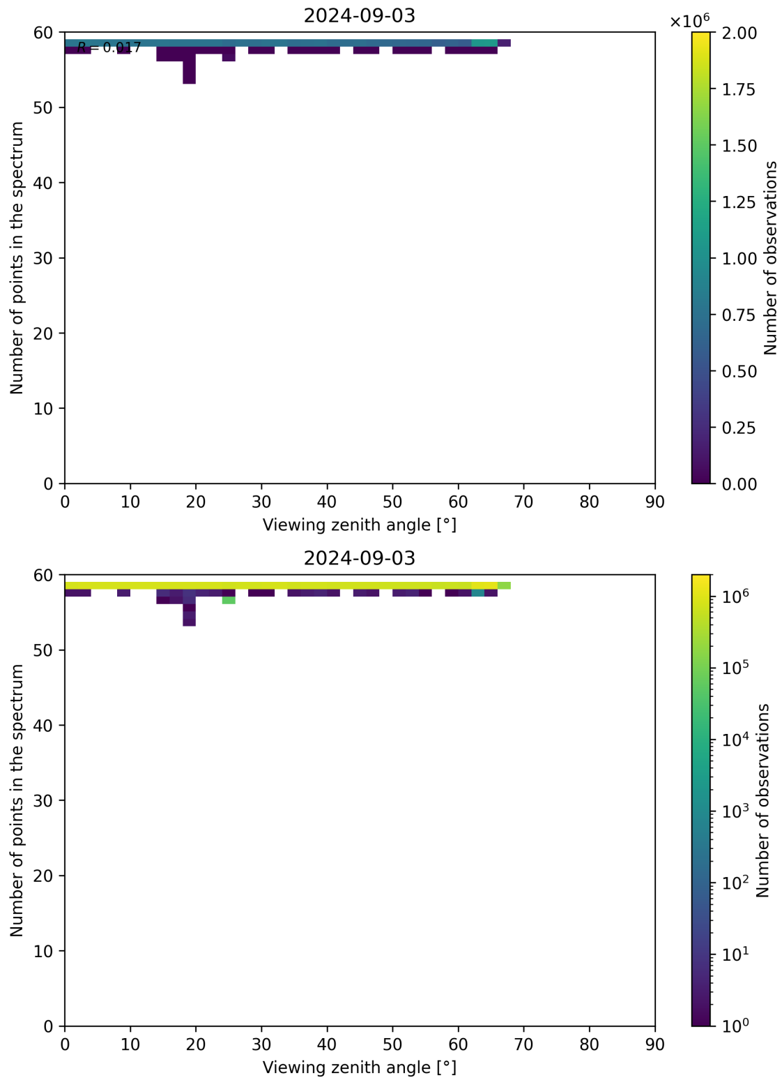
Figure 125: Scatter density plot of “Viewing zenith angle” against “Number of points in the spectrum” for 2024-09-02 to 2024-09-04.
