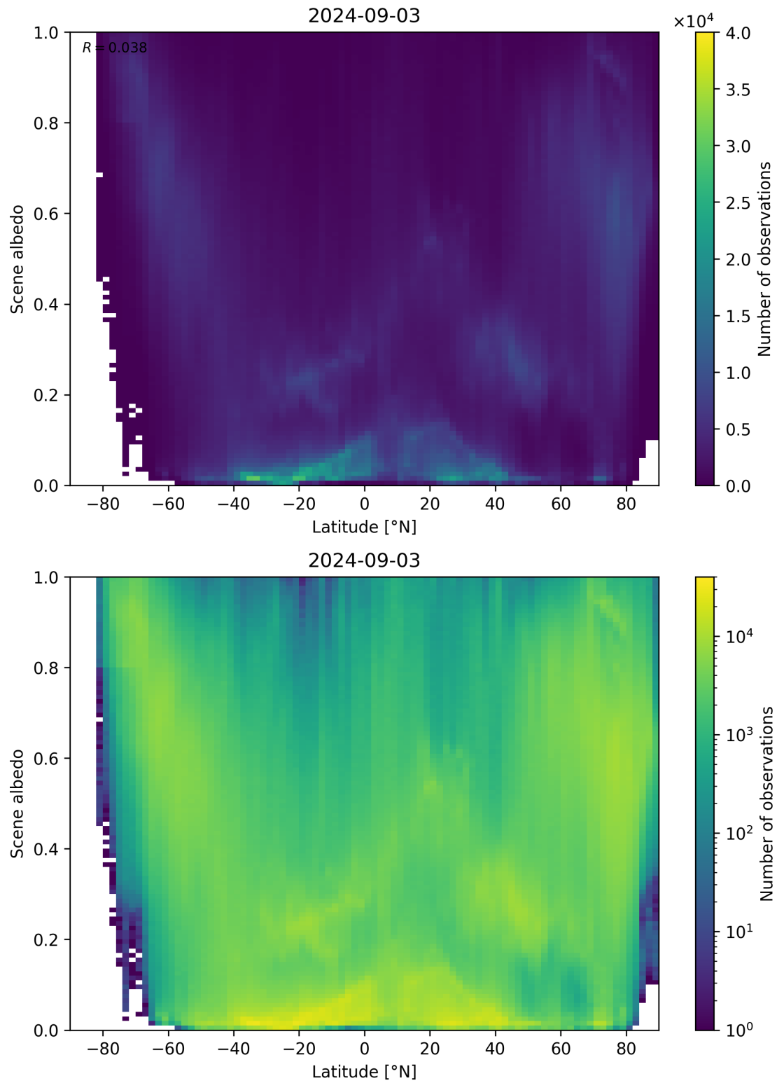
Figure 95: Scatter density plot of “Latitude” against “Scene albedo” for 2024-09-02 to 2024-09-04.
