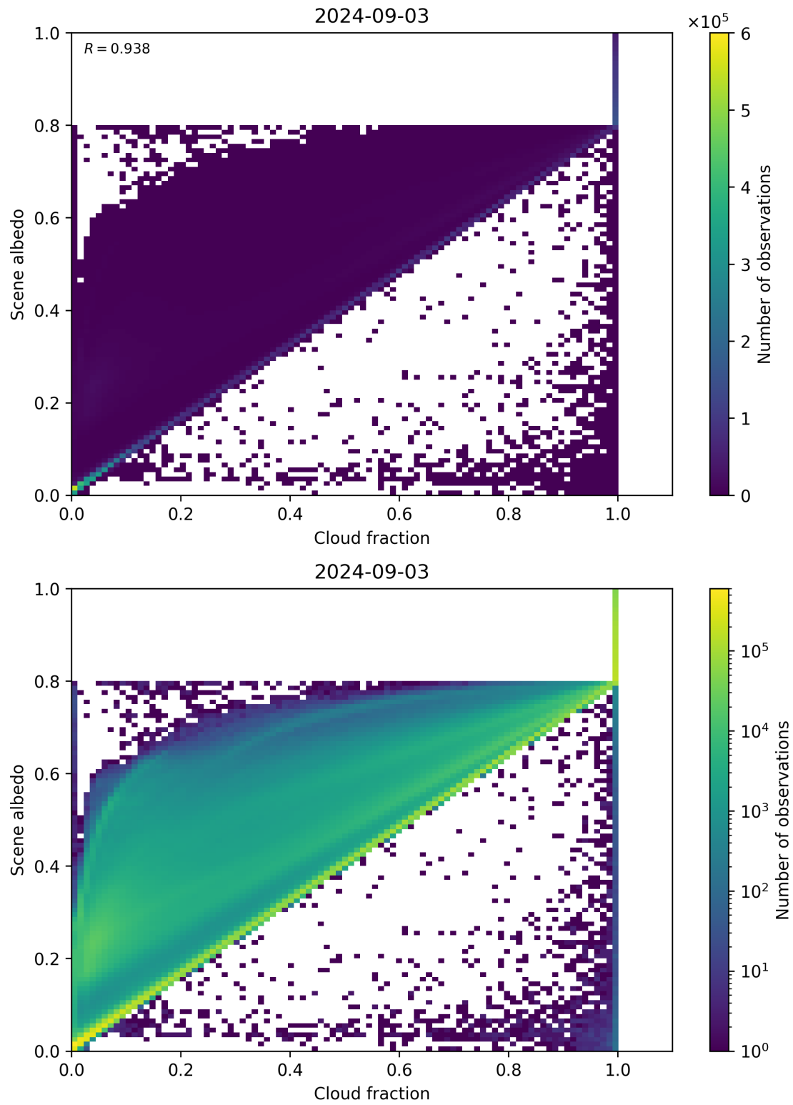
Figure 75: Scatter density plot of “Cloud fraction” against “Scene albedo” for 2024-09-02 to 2024-09-04.
