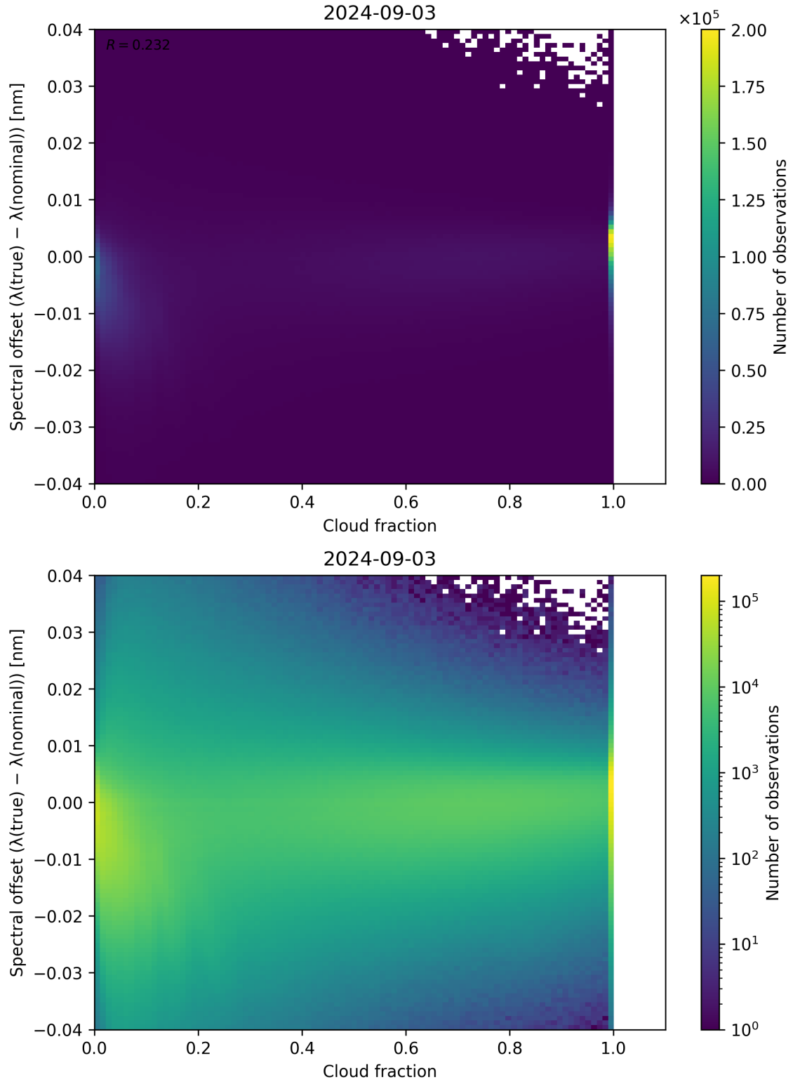
Figure 76: Scatter density plot of “Cloud fraction” against “Spectral offset ( \lambda_{\text{true}} - \lambda_{\text{nominal}} )” for 2024-09-02 to 2024-09-04.
