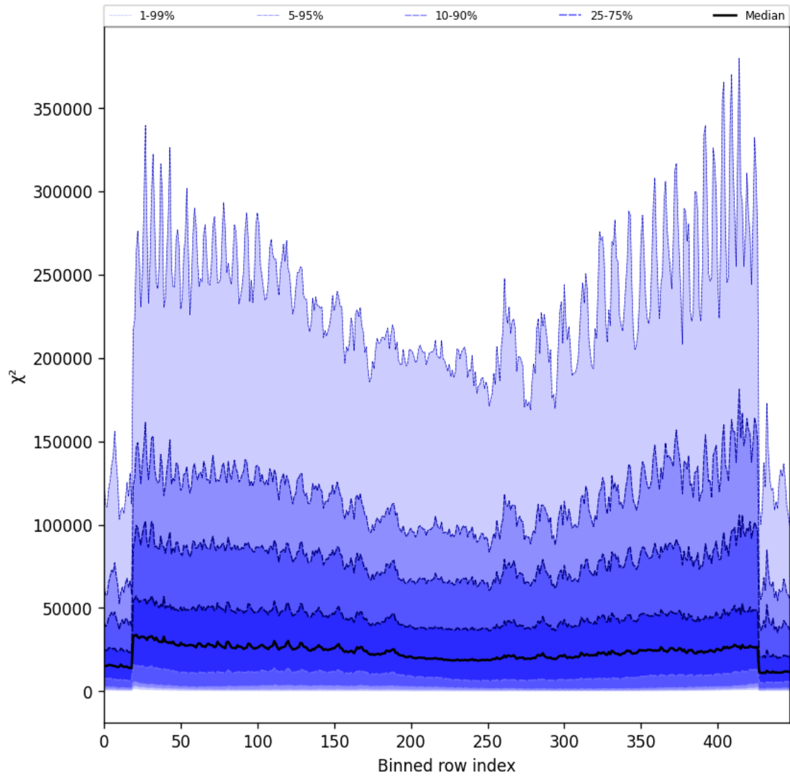
Figure 55: Along track statistics of “ \chi^2 ” for 2024-09-02 to 2024-09-04
