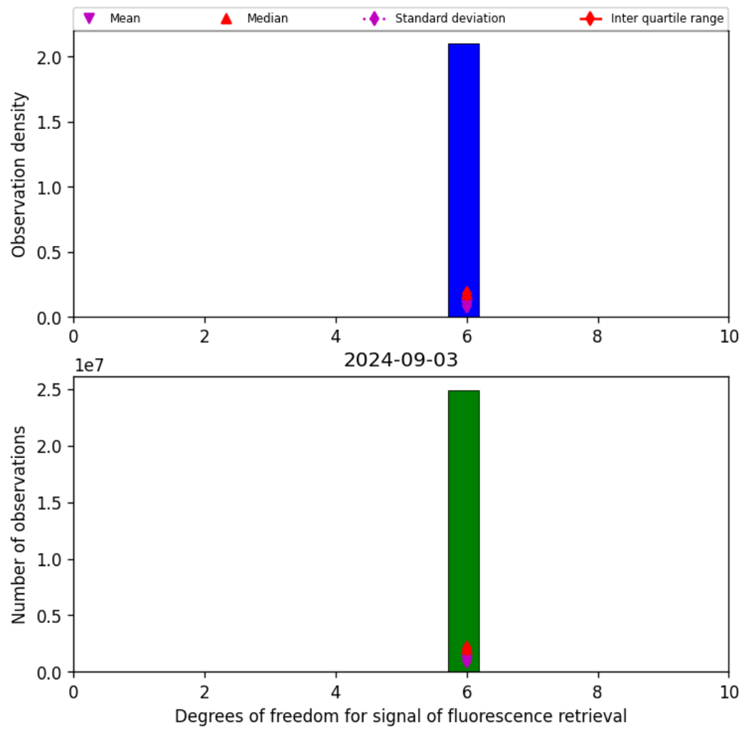
Figure 43: Histogram of “Degrees of freedom for signal of fluorescence retrieval” for 2024-09-02 to 2024-09-04
