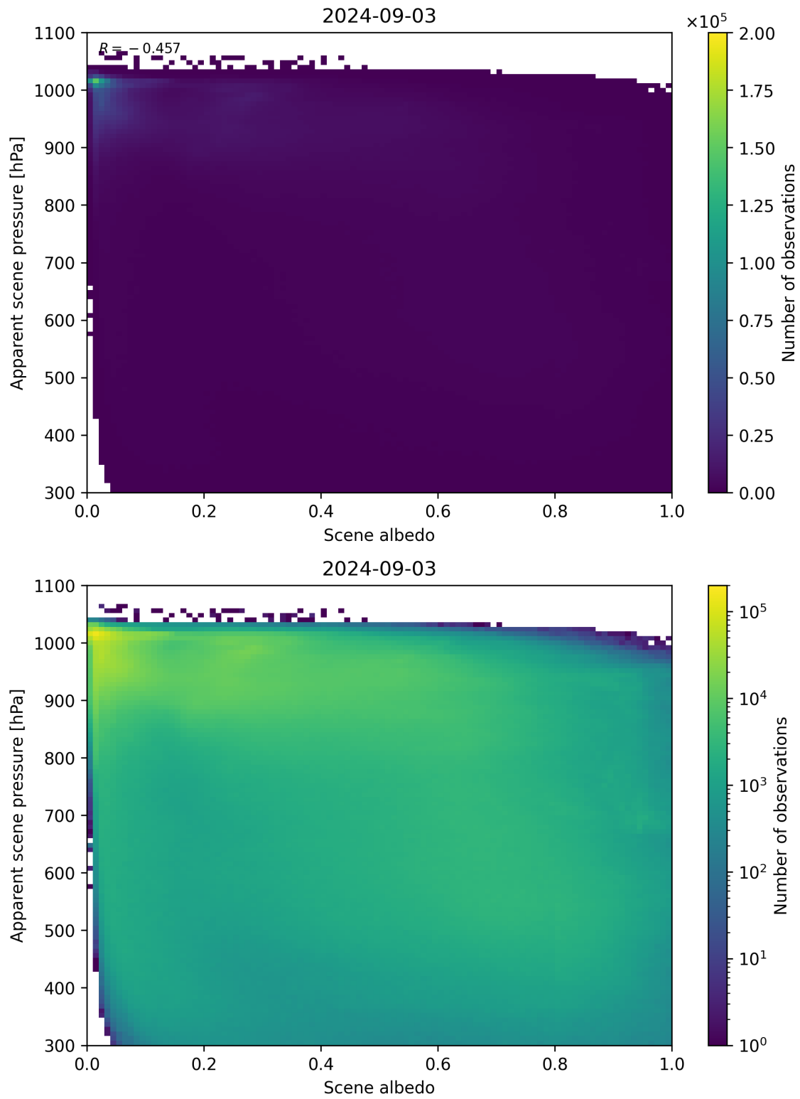
Figure 102: Scatter density plot of “Scene albedo” against “Apparent scene pressure” for 2024-09-02 to 2024-09-04.
