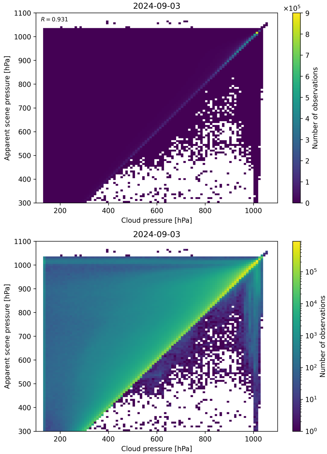
Figure 77: Scatter density plot of “Cloud pressure” against “Apparent scene pressure” for 2024-09-02 to 2024-09-04.
