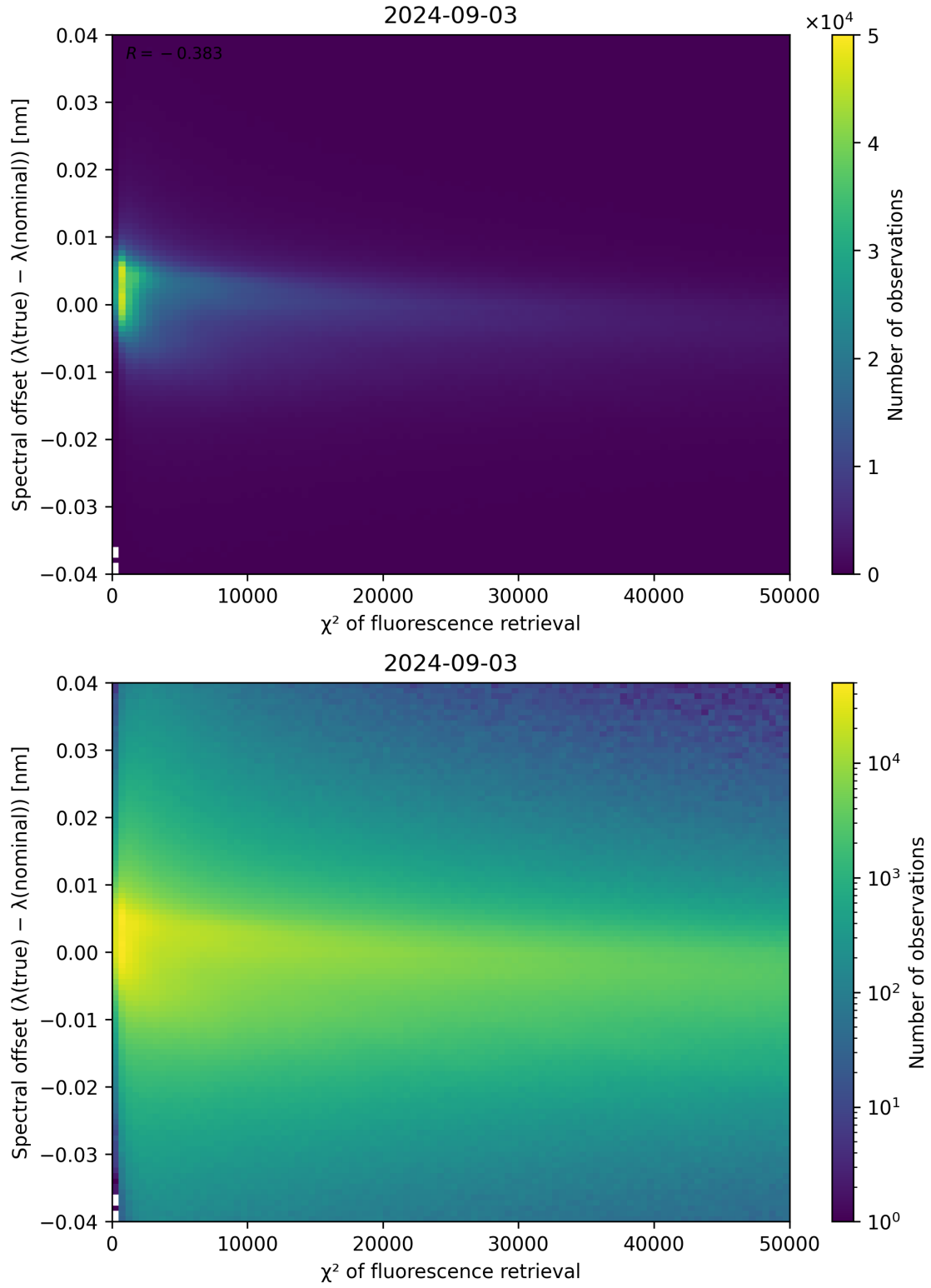
Figure 69: Scatter density plot of “ \chi^2 of fluorescence retrieval” against “Spectral offset ( \lambda_{\text{true}} - \lambda_{\text{nominal}} )” for 2024-09-02 to 2024-09-04.
