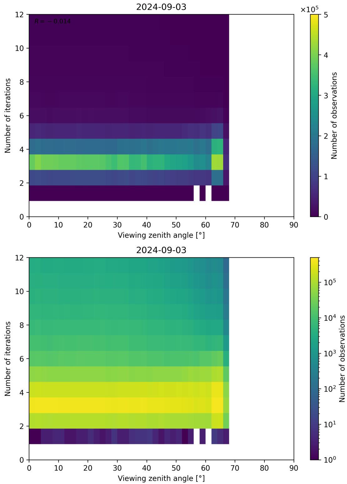
Figure 124: Scatter density plot of “Viewing zenith angle” against “Number of iterations” for 2024-09-02 to 2024-09-04.
