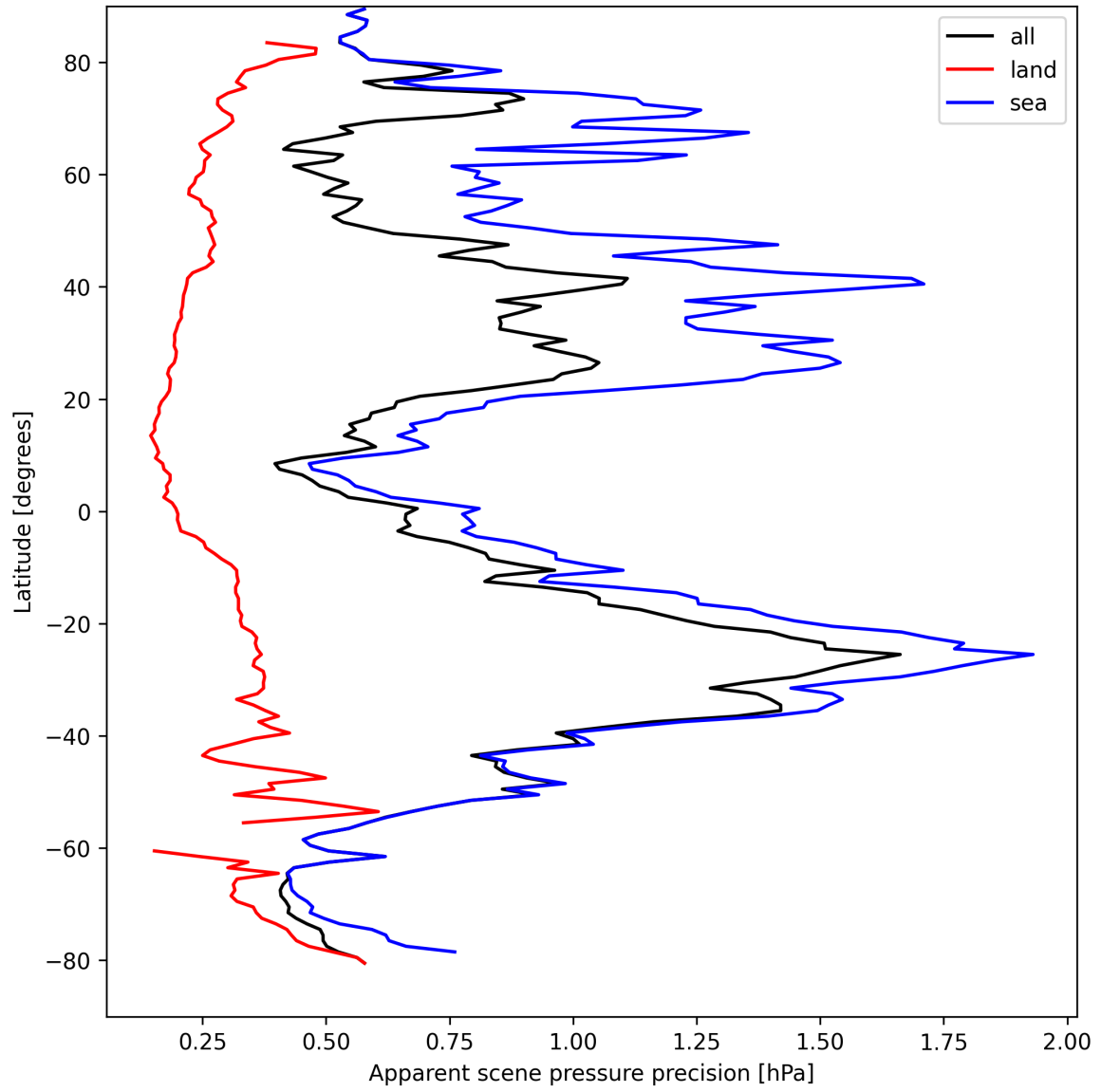
Figure 20: Zonal average of “Apparent scene pressure precision” for 2024-09-02 to 2024-09-04.
