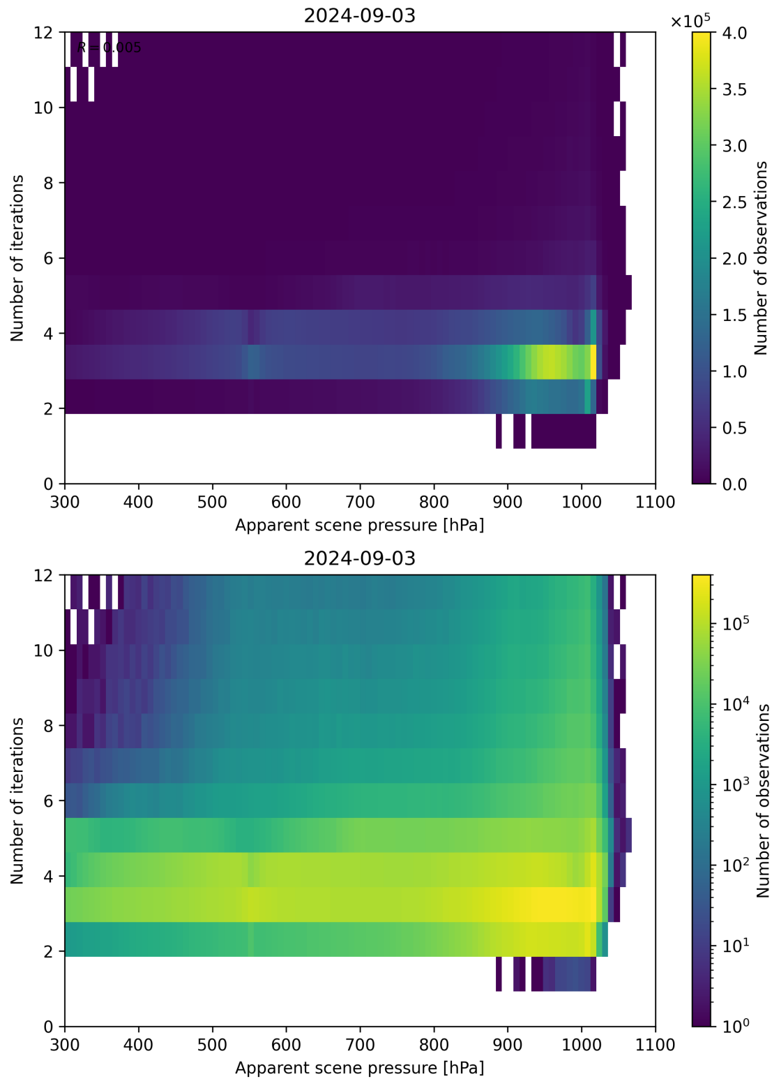
Figure 65: Scatter density plot of “Apparent scene pressure” against “Number of iterations” for 2024-09-02 to 2024-09-04.
