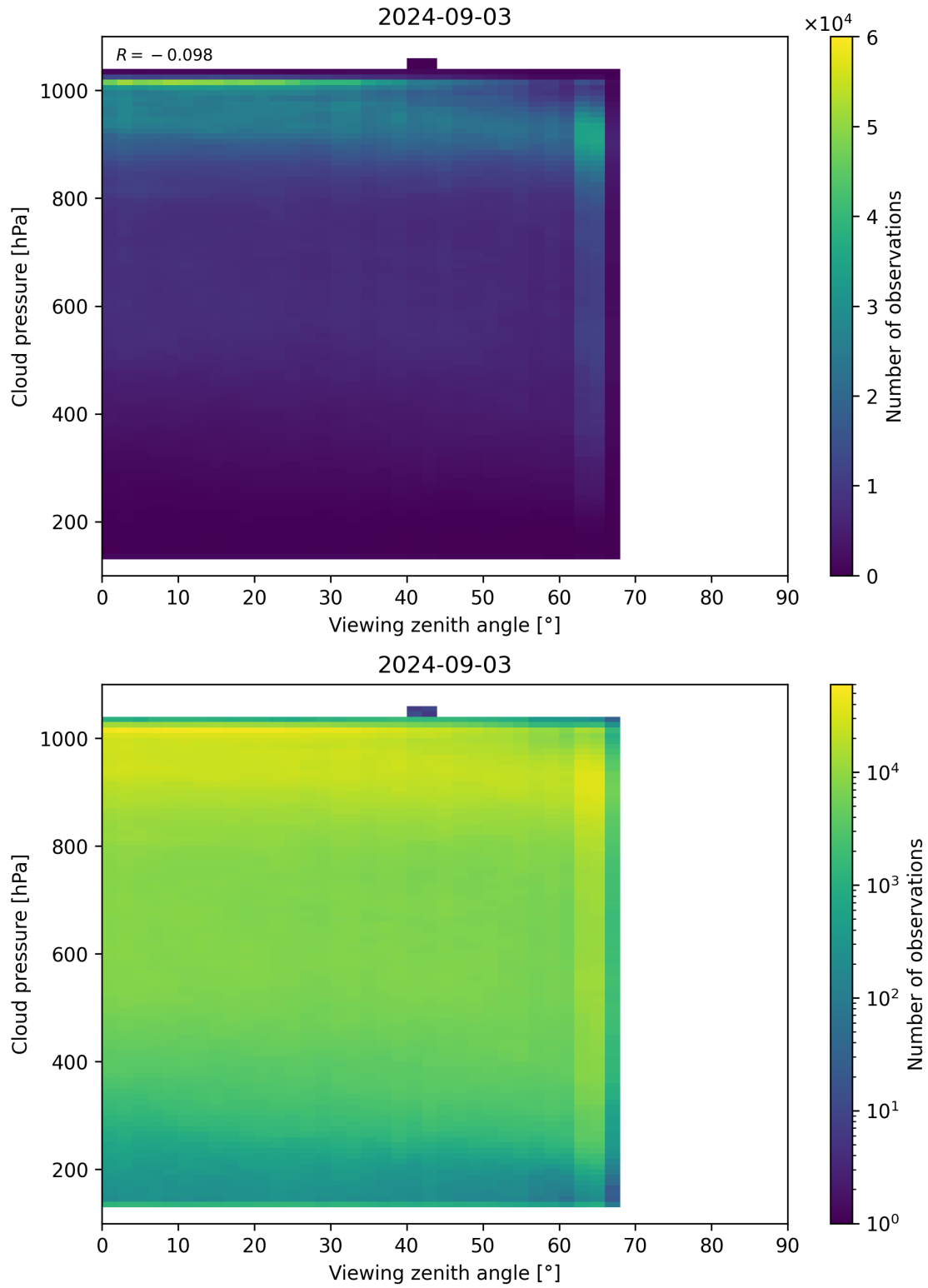
Figure 121: Scatter density plot of “Viewing zenith angle” against “Cloud pressure” for 2024-09-02 to 2024-09-04.
