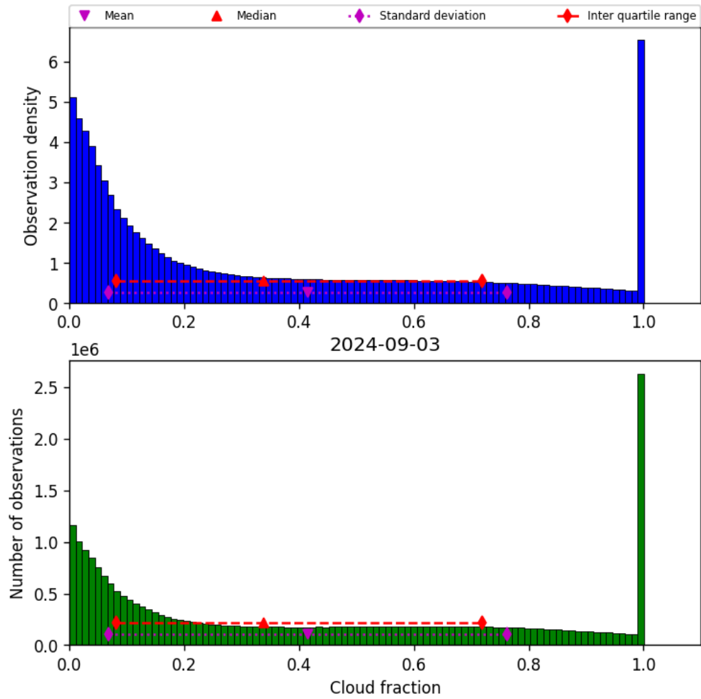
Figure 32: Histogram of “Cloud fraction” for 2024-09-02 to 2024-09-04
