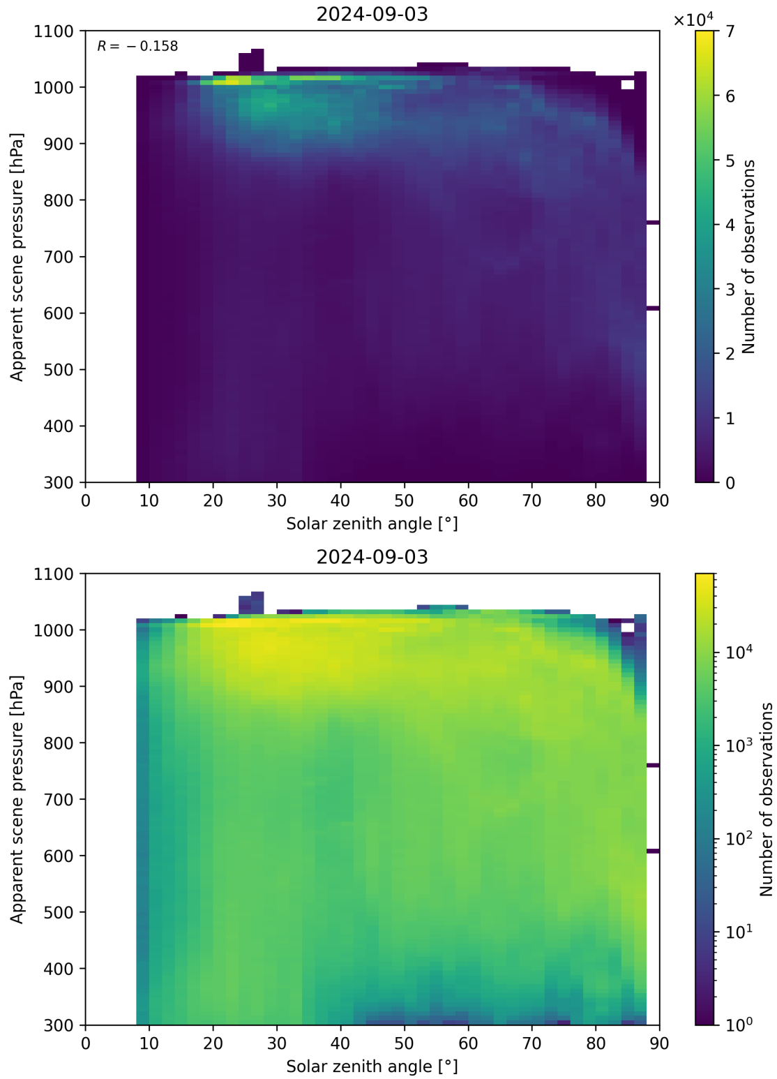
Figure 108: Scatter density plot of “Solar zenith angle” against “Apparent scene pressure” for 2024-09-02 to 2024-09-04.
