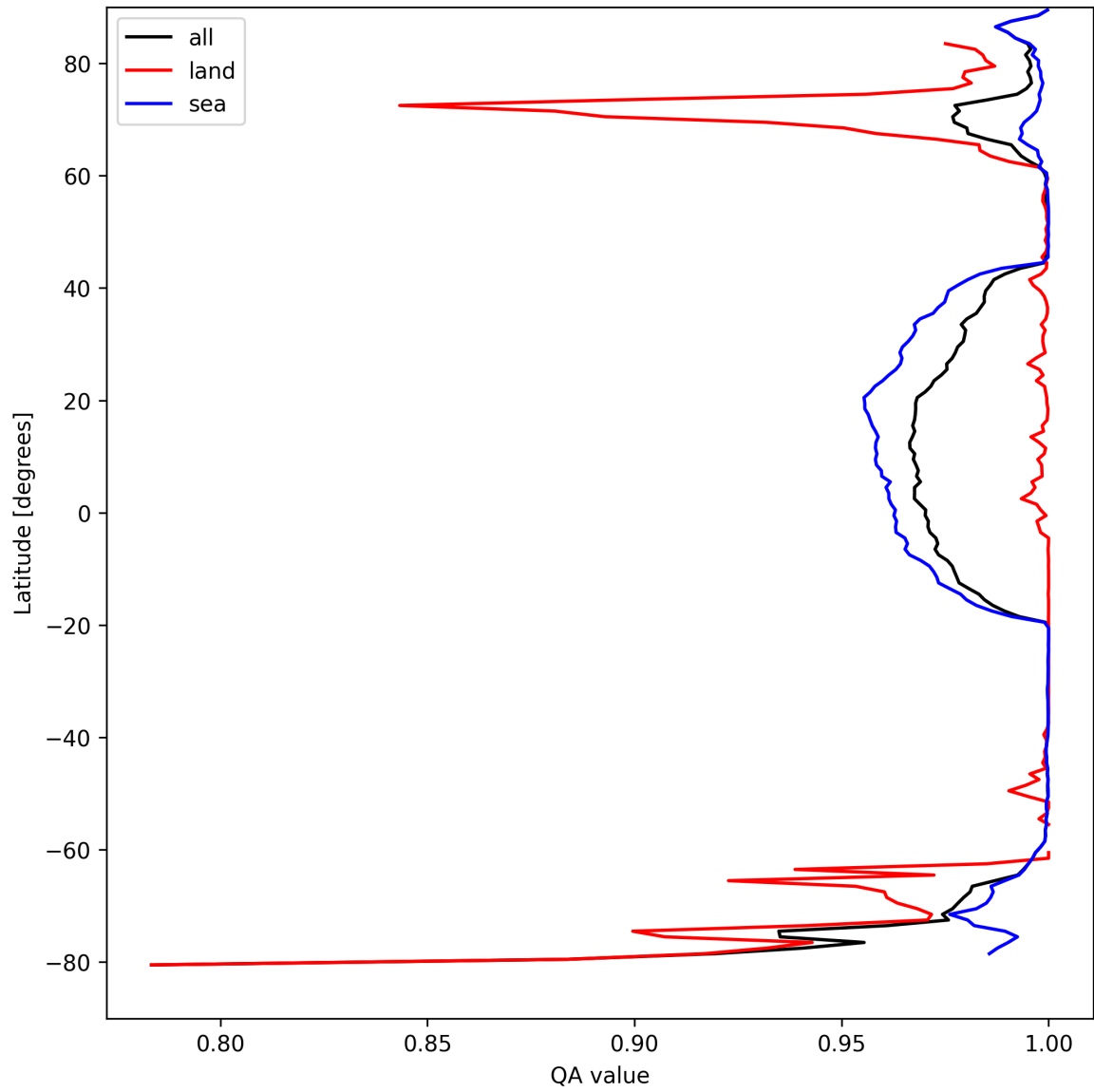
Figure 12: Zonal average of “QA value” for 2024-09-02 to 2024-09-04.
