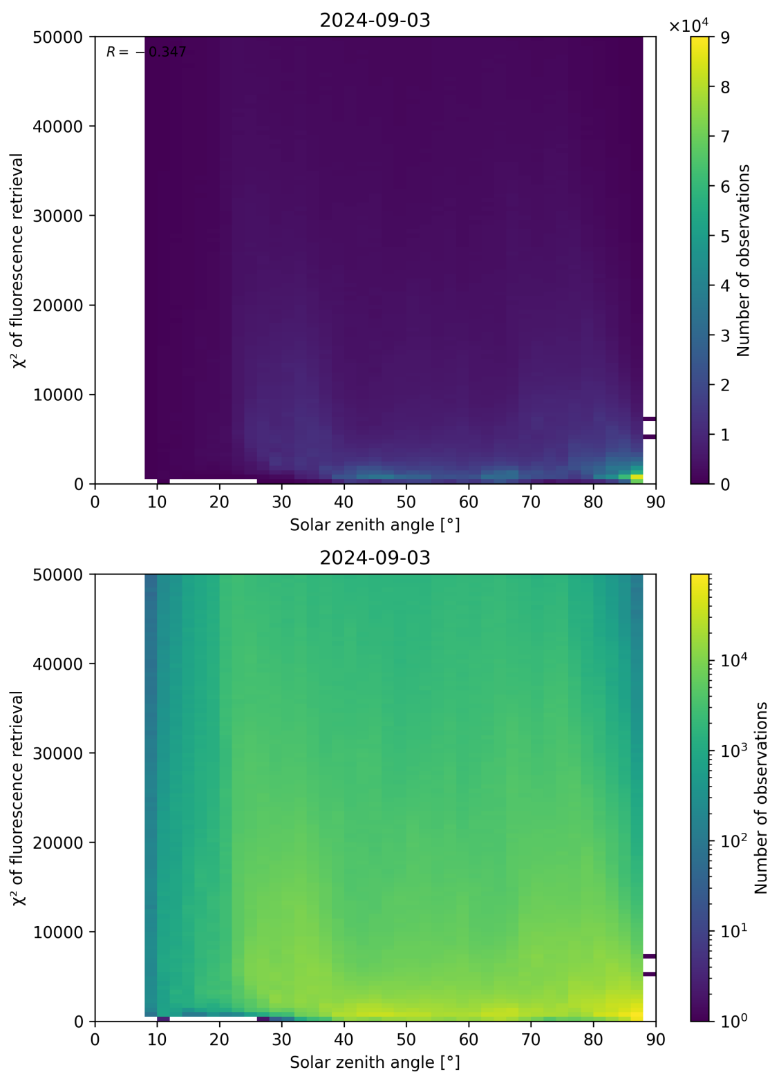
Figure 109: Scatter density plot of “Solar zenith angle” against “ \chi^2 of fluorescence retrieval” for 2024-09-02 to 2024-09-04.
