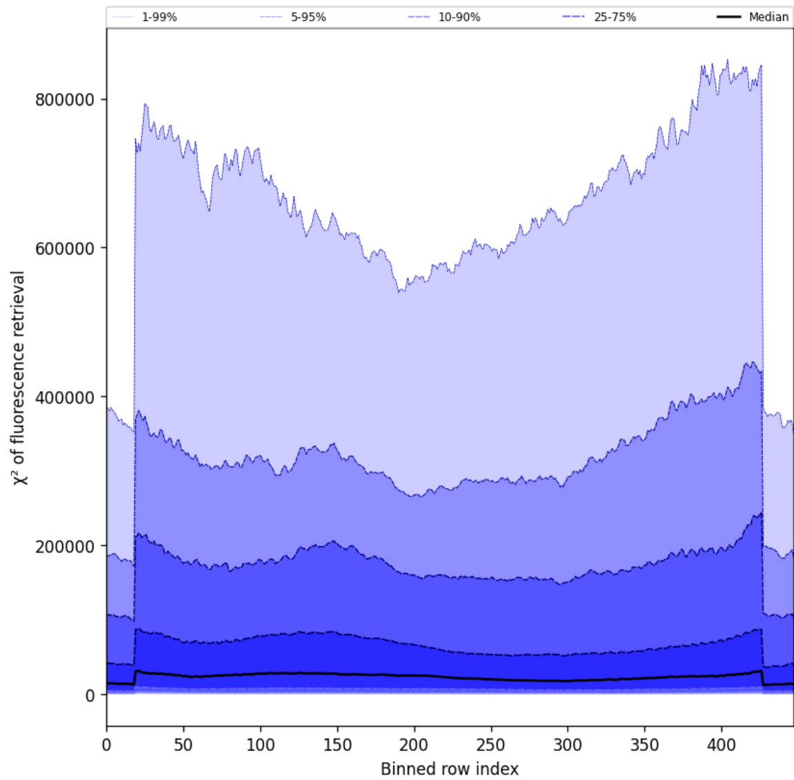
Figure 59: Along track statistics of “ \chi^2 of fluorescence retrieval” for 2024-09-02 to 2024-09-04
