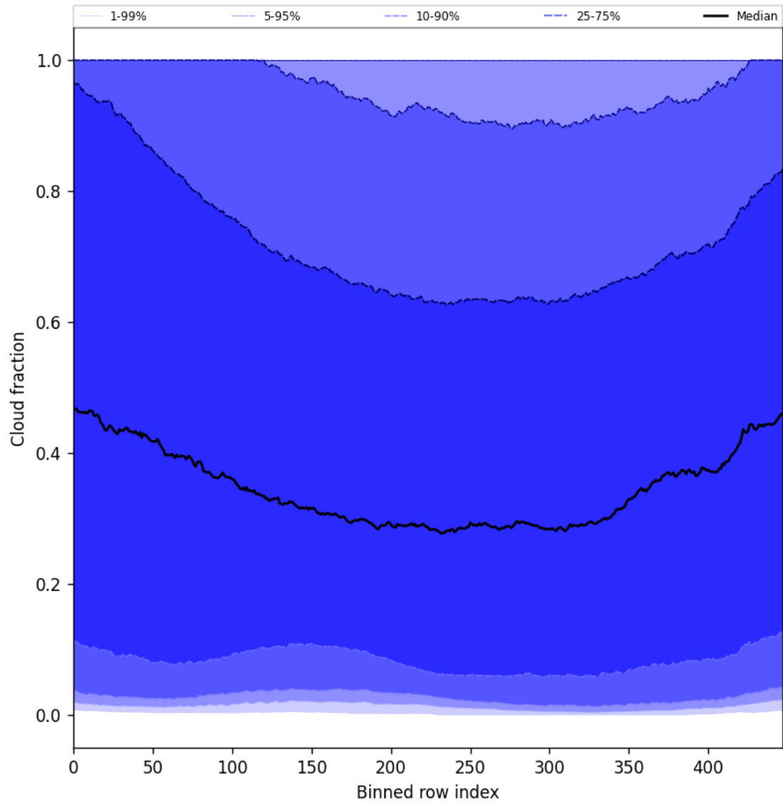
Figure 49: Along track statistics of “Cloud fraction” for 2024-09-02 to 2024-09-04
