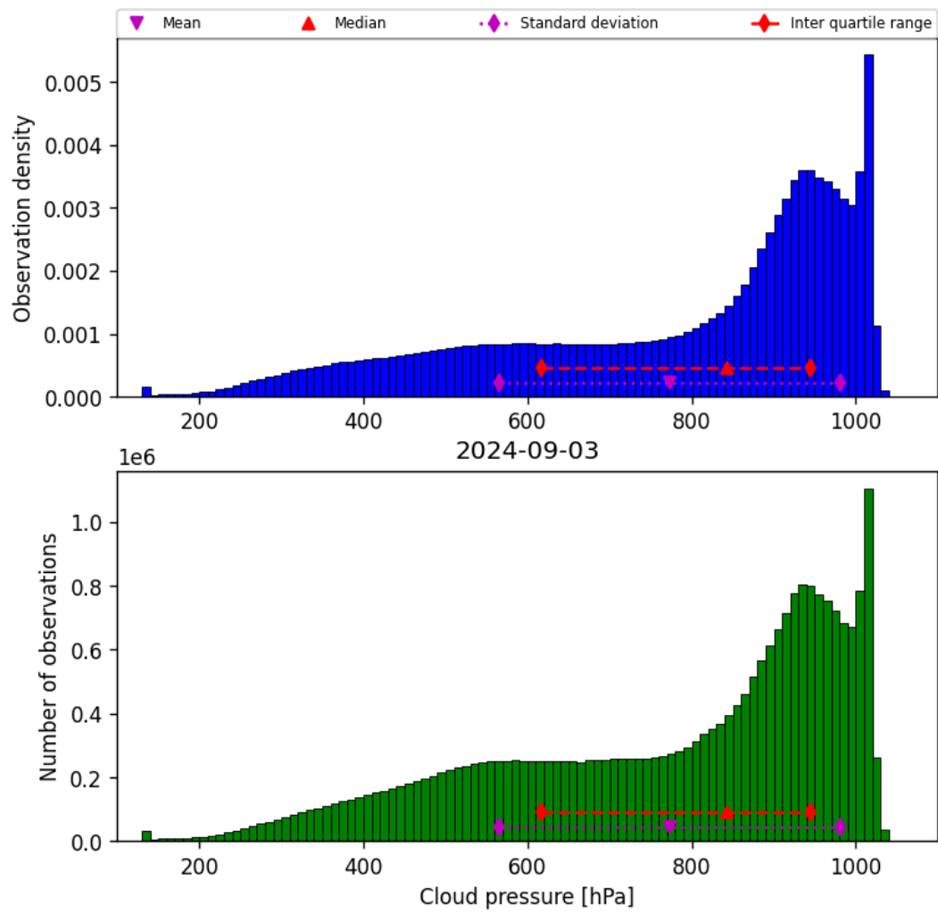
Figure 30: Histogram of “Cloud pressure” for 2024-09-02 to 2024-09-04
