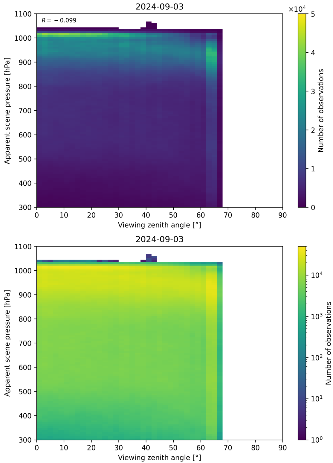
Figure 118: Scatter density plot of “Viewing zenith angle” against “Apparent scene pressure” for 2024-09-02 to 2024-09-04.
