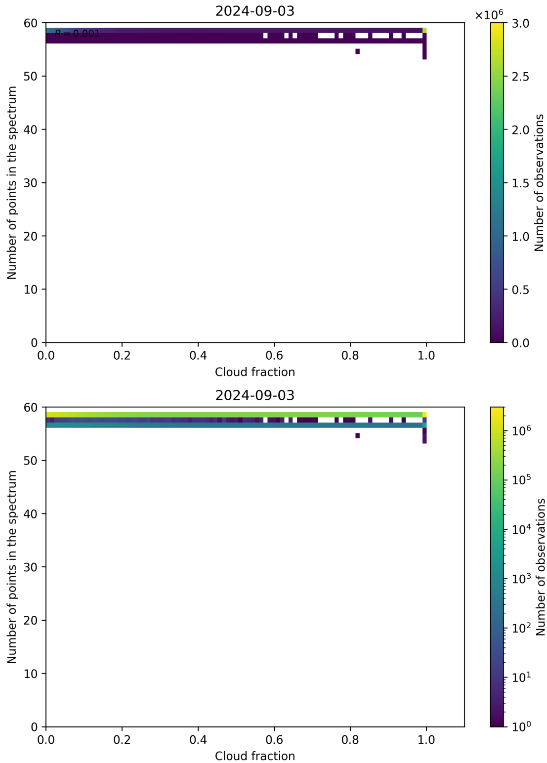
Figure 74: Scatter density plot of “Cloud fraction” against “Number of points in the spectrum” for 2024-09-02 to 2024-09-04.
