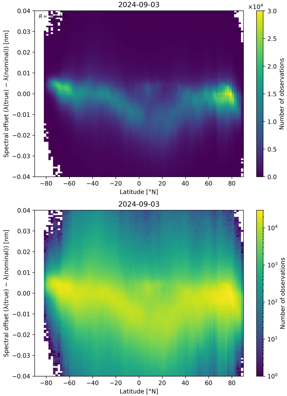
Figure 96: Scatter density plot of “Latitude” against “Spectral offset ( \lambda_{\text{true}} - \lambda_{\text{nominal}} )” for 2024-09-02 to 2024-09-04.
