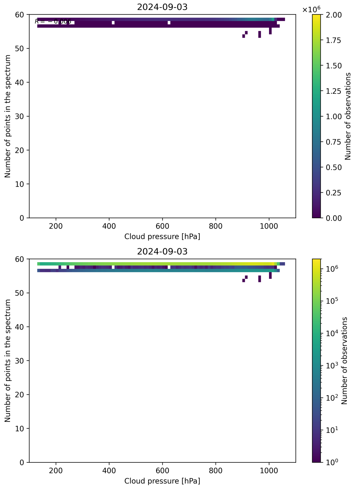
Figure 82: Scatter density plot of “Cloud pressure” against “Number of points in the spectrum” for 2024-09-02 to 2024-09-04.
