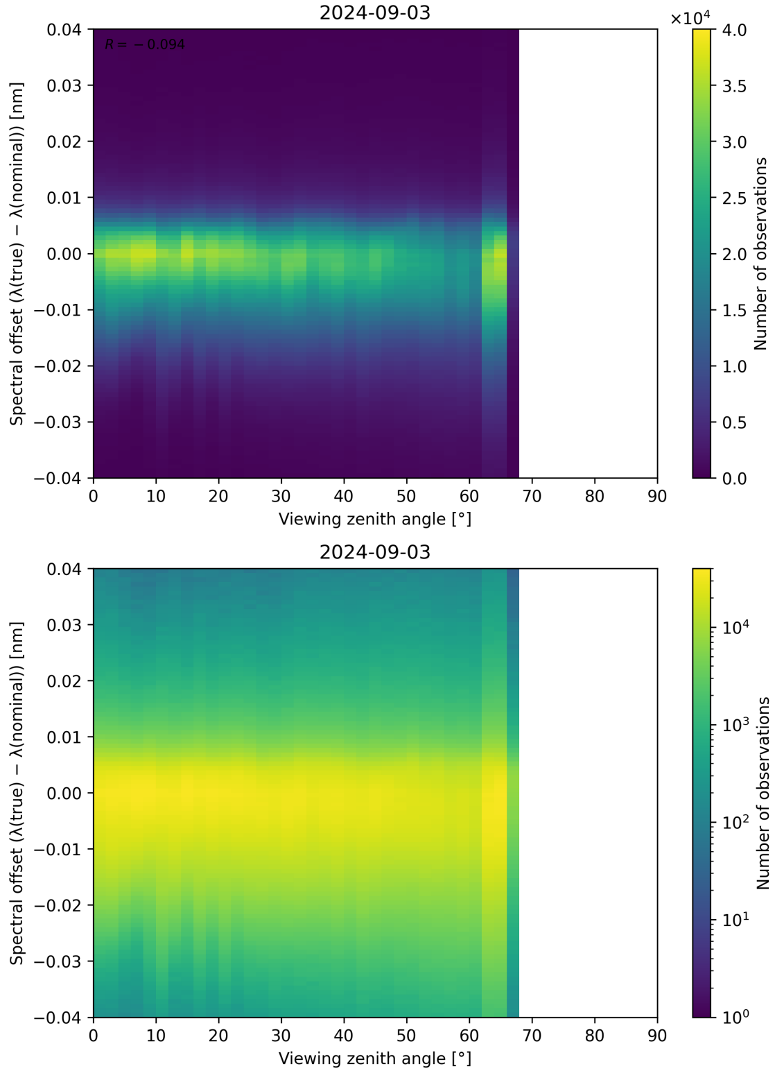
Figure 128: Scatter density plot of “Viewing zenith angle” against “Spectral offset ( \lambda_{\text{true}} - \lambda_{\text{nominal}} )” for 2024-09-02 to 2024-09-04.
