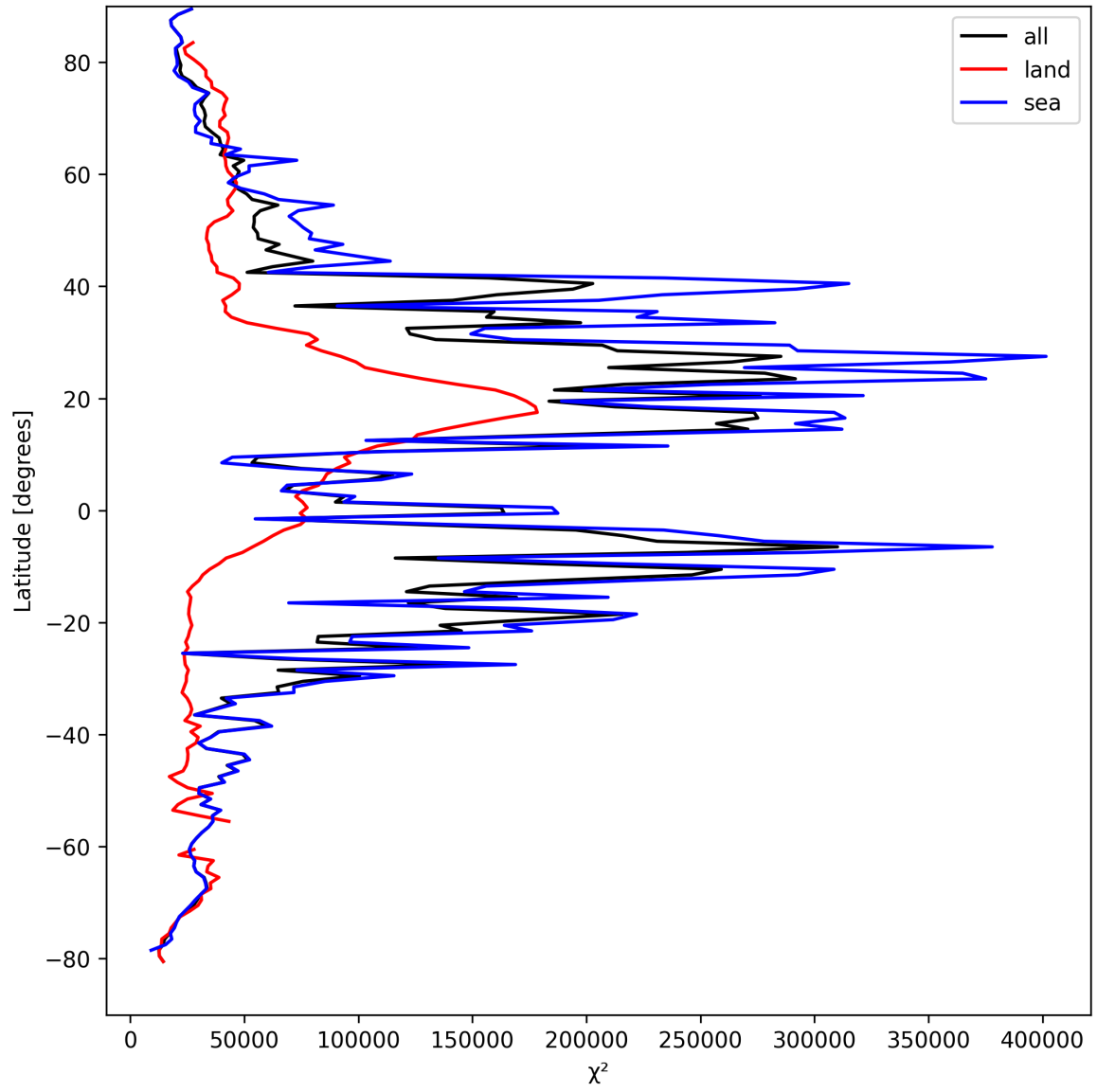
Figure 21: Zonal average of “ \chi^2 ” for 2024-09-02 to 2024-09-04.
