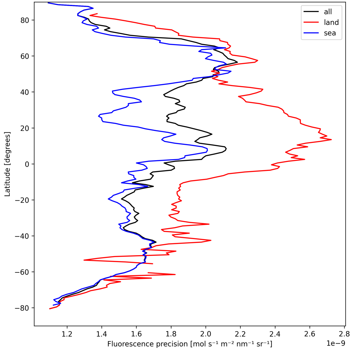
Figure 24: Zonal average of “Fluorescence precision” for 2024-09-02 to 2024-09-04.
