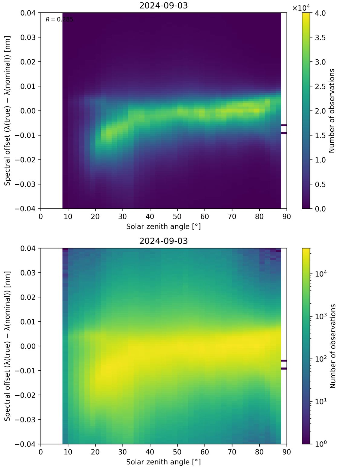
Figure 117: Scatter density plot of “Solar zenith angle” against “Spectral offset ( \lambda_{\text{true}} - \lambda_{\text{nominal}} )” for 2024-09-02 to 2024-09-04.
