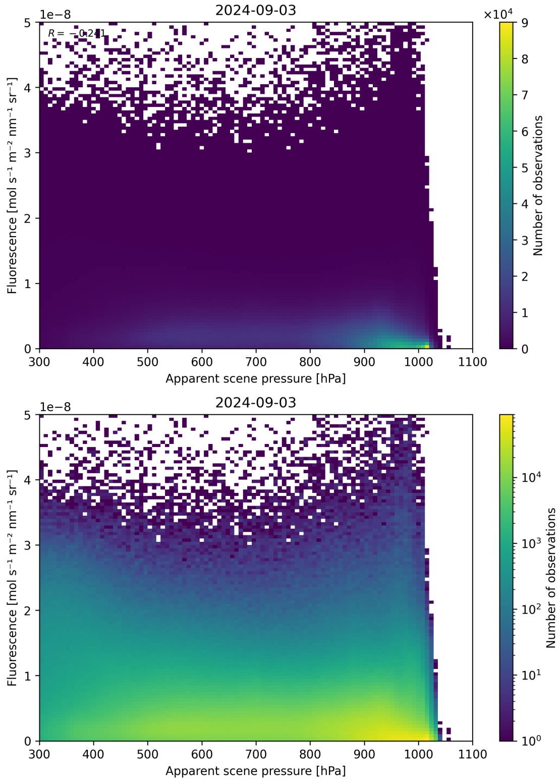
Figure 64: Scatter density plot of “Apparent scene pressure” against “Fluorescence” for 2024-09-02 to 2024-09-04.
