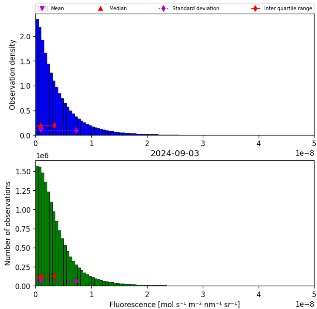
Figure 40: Histogram of “Fluorescence” for 2024-09-02 to 2024-09-04
