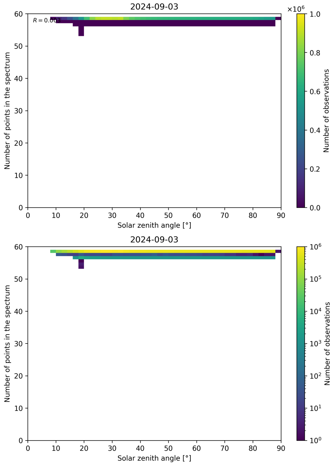
Figure 115: Scatter density plot of “Solar zenith angle” against “Number of points in the spectrum” for 2024-09-02 to 2024-09-04.
