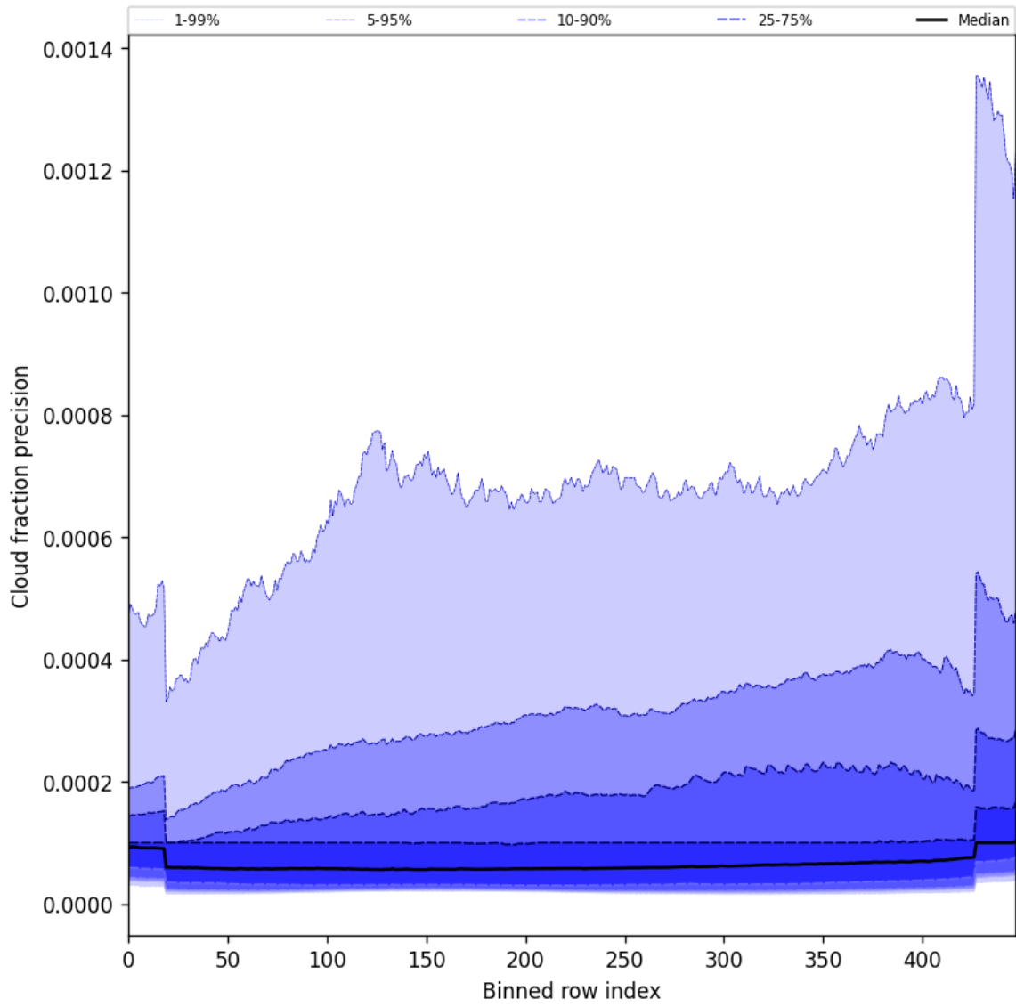
Figure 50: Along track statistics of “Cloud fraction precision” for 2024-09-02 to 2024-09-04
