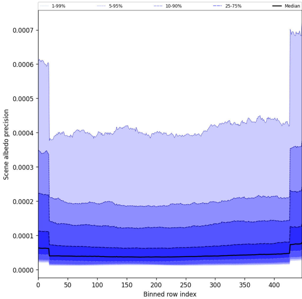
Figure 52: Along track statistics of “Scene albedo precision” for 2024-09-02 to 2024-09-04
