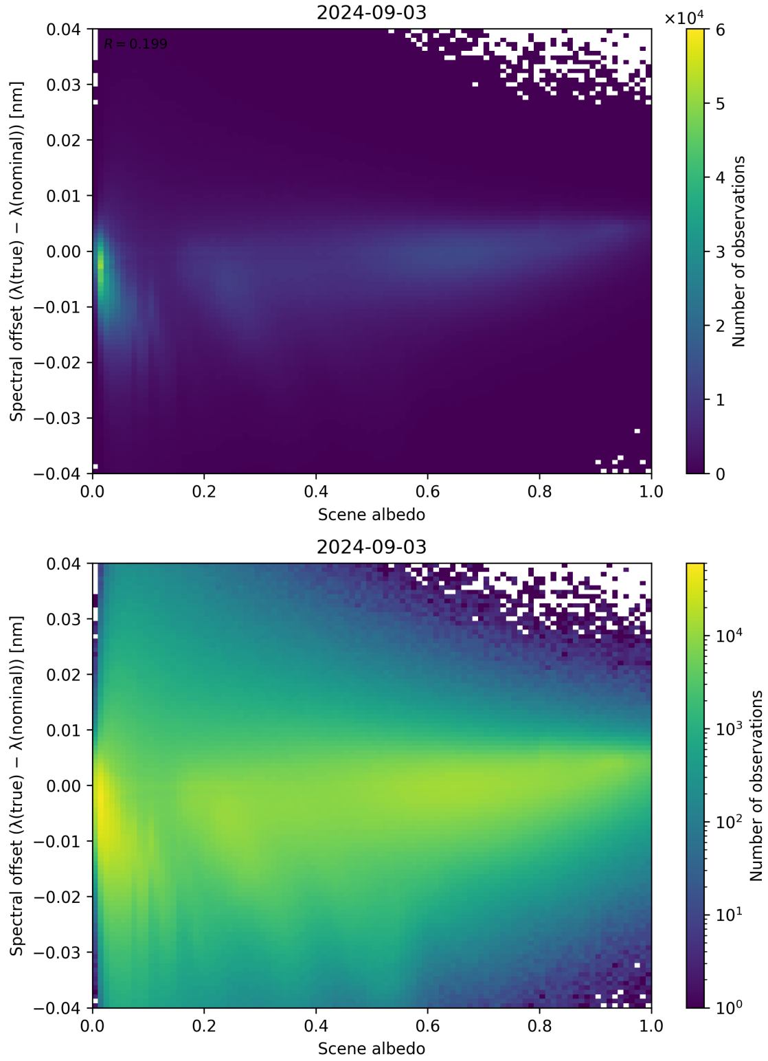
Figure 107: Scatter density plot of “Scene albedo” against “Spectral offset ( \lambda_{\text{true}} - \lambda_{\text{nominal}} )” for 2024-09-02 to 2024-09-04.
