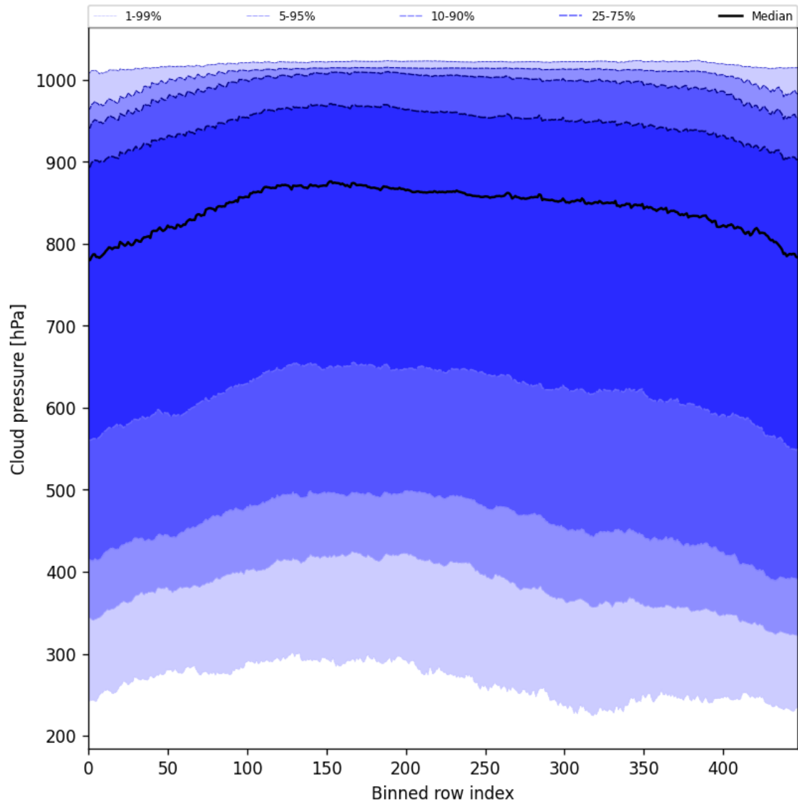
Figure 47: Along track statistics of “Cloud pressure” for 2024-09-02 to 2024-09-04
