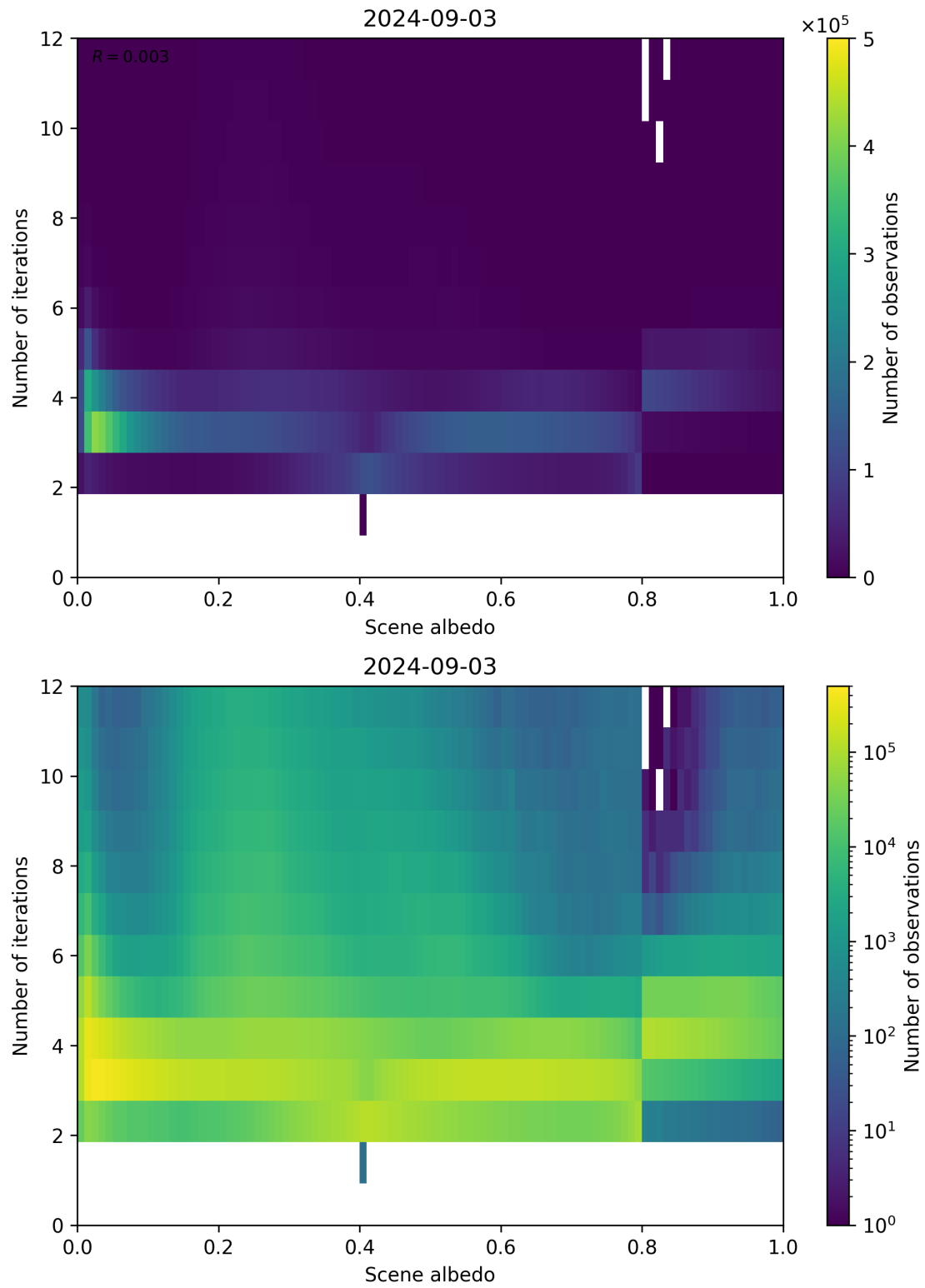
Figure 105: Scatter density plot of “Scene albedo” against “Number of iterations” for 2024-09-02 to 2024-09-04.
