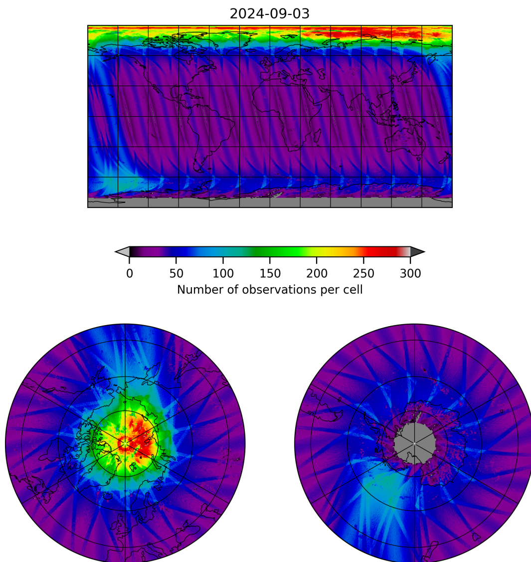
Figure 11: Map of the number of observations for 2024-09-02 to 2024-09-04
