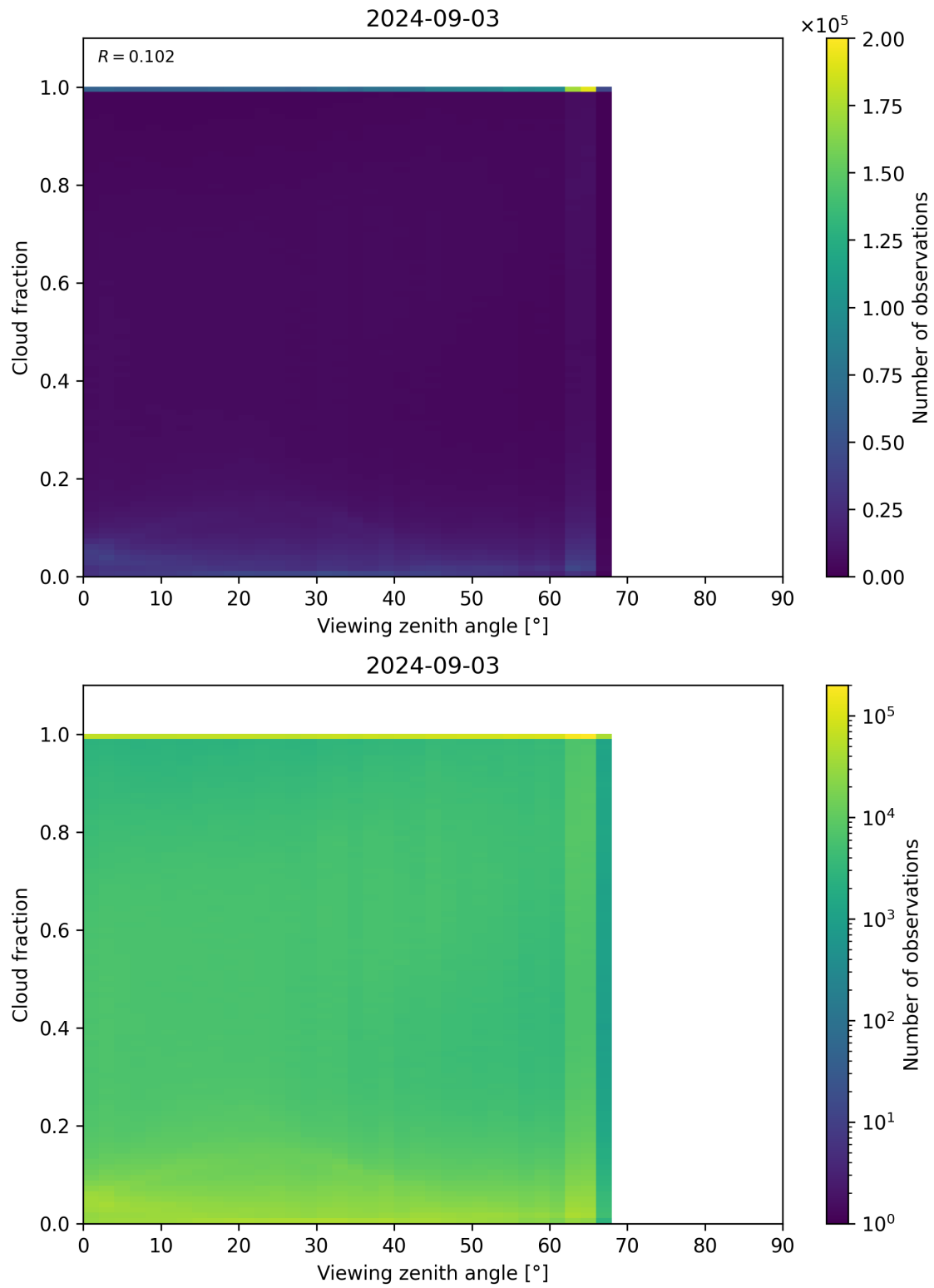
Figure 120: Scatter density plot of “Viewing zenith angle” against “Cloud fraction” for 2024-09-02 to 2024-09-04.
