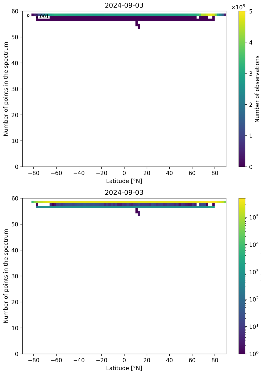
Figure 94: Scatter density plot of “Latitude” against “Number of points in the spectrum” for 2024-09-02 to 2024-09-04.
