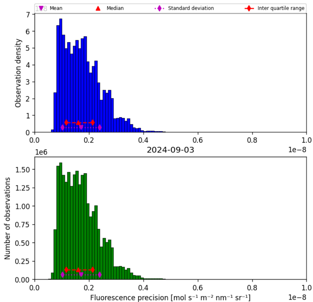
Figure 41: Histogram of “Fluorescence precision” for 2024-09-02 to 2024-09-04
