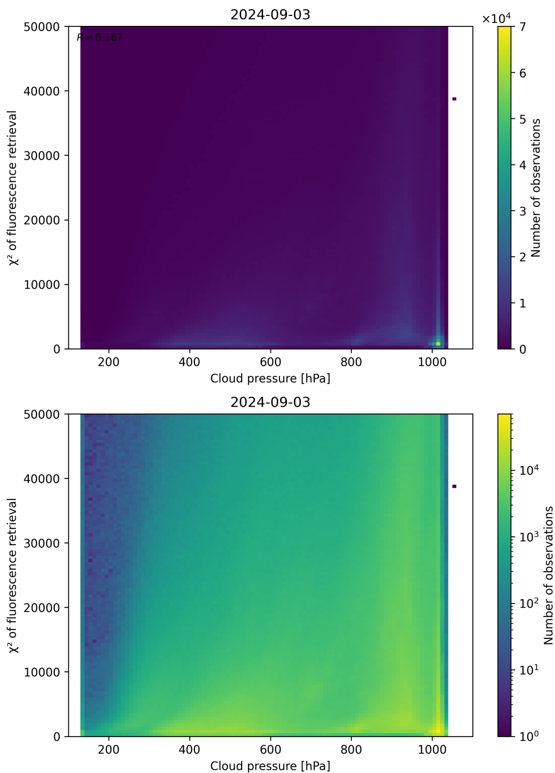
Figure 78: Scatter density plot of “Cloud pressure” against “ \chi^2 of fluorescence retrieval” for 2024-09-02 to 2024-09-04.
