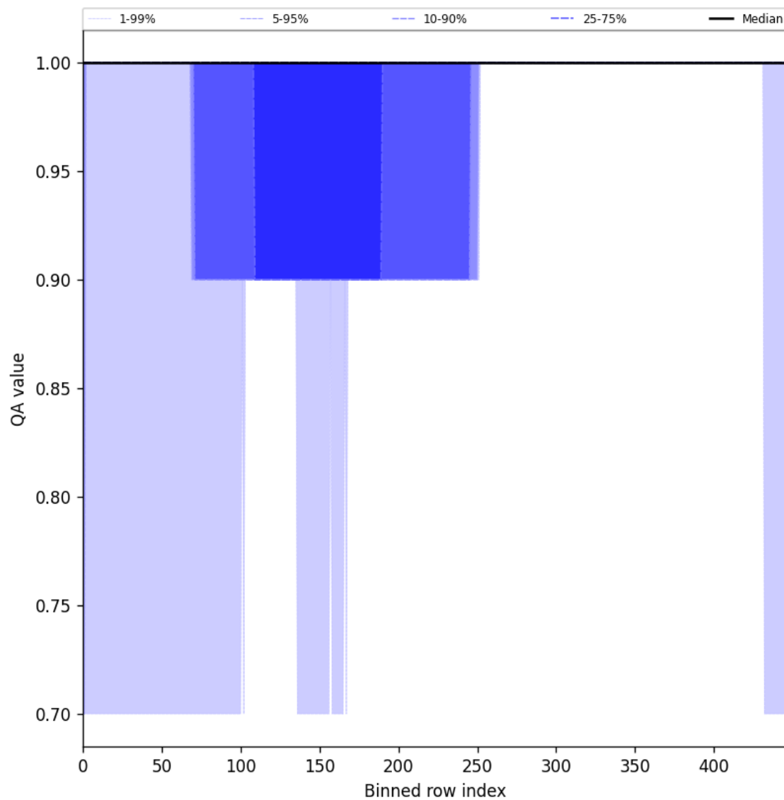
Figure 46: Along track statistics of “QA value” for 2024-09-02 to 2024-09-04
