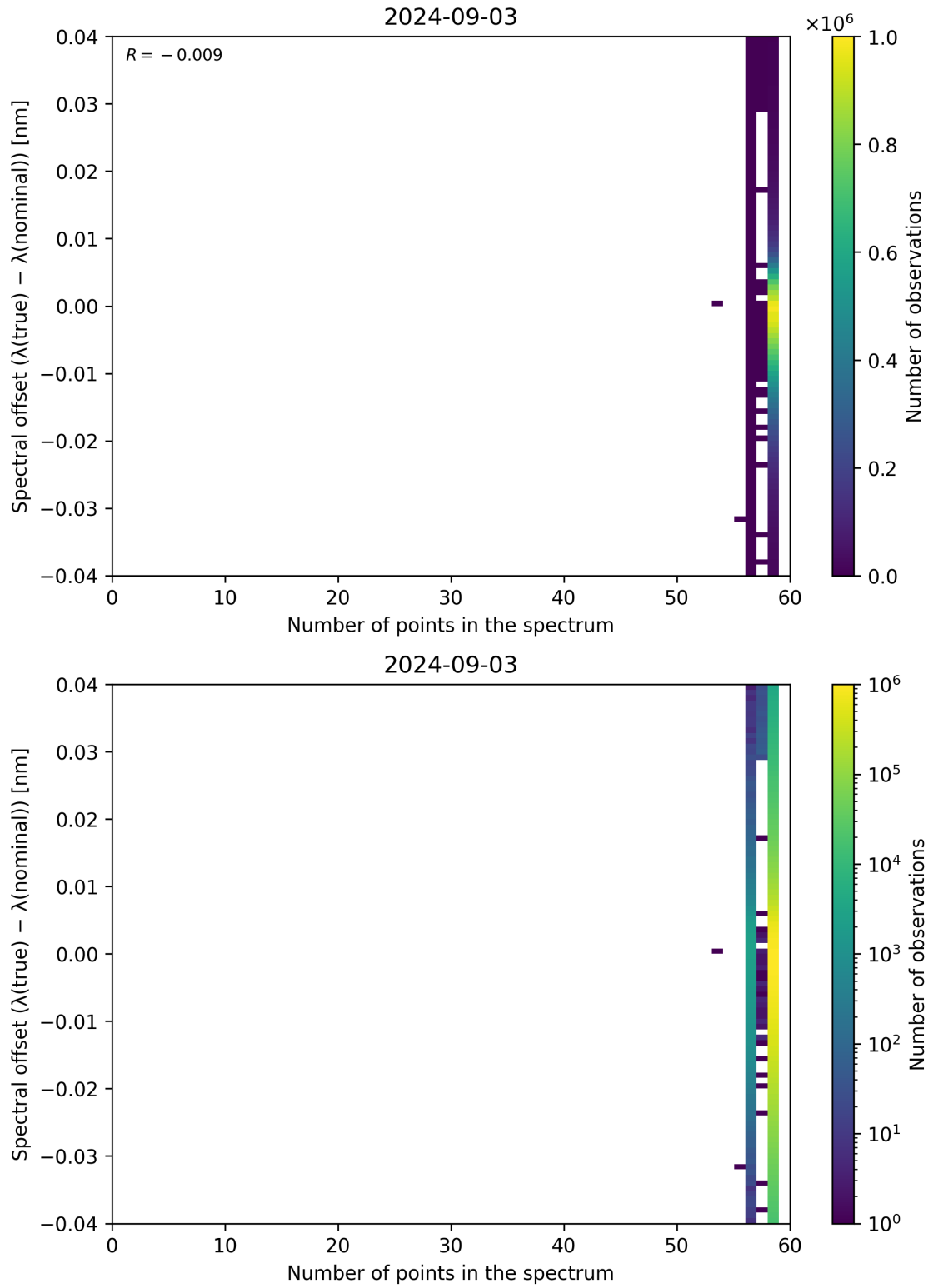
Figure 101: Scatter density plot of “Number of points in the spectrum” against “Spectral offset ( \lambda_{\text{true}} - \lambda_{\text{nominal}} )” for 2024-09-02 to 2024-09-04.
