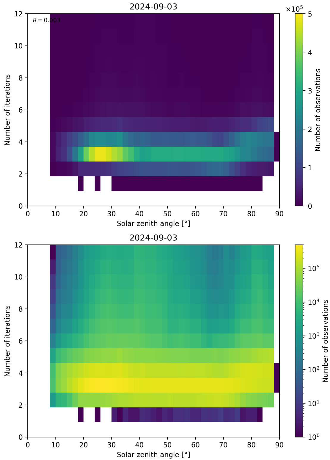
Figure 114: Scatter density plot of “Solar zenith angle” against “Number of iterations” for 2024-09-02 to 2024-09-04.
