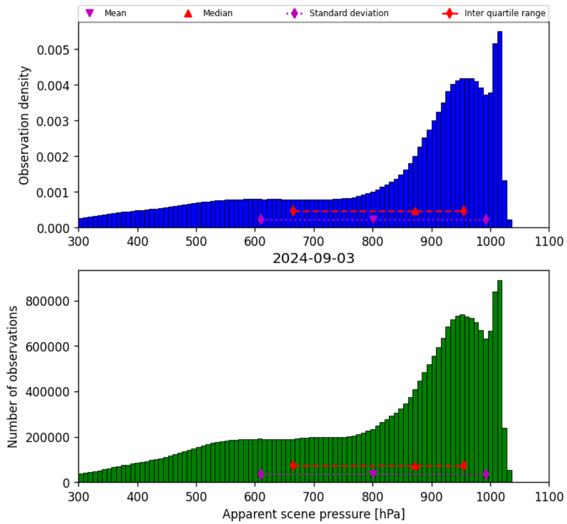
Figure 36: Histogram of “Apparent scene pressure” for 2024-09-02 to 2024-09-04
