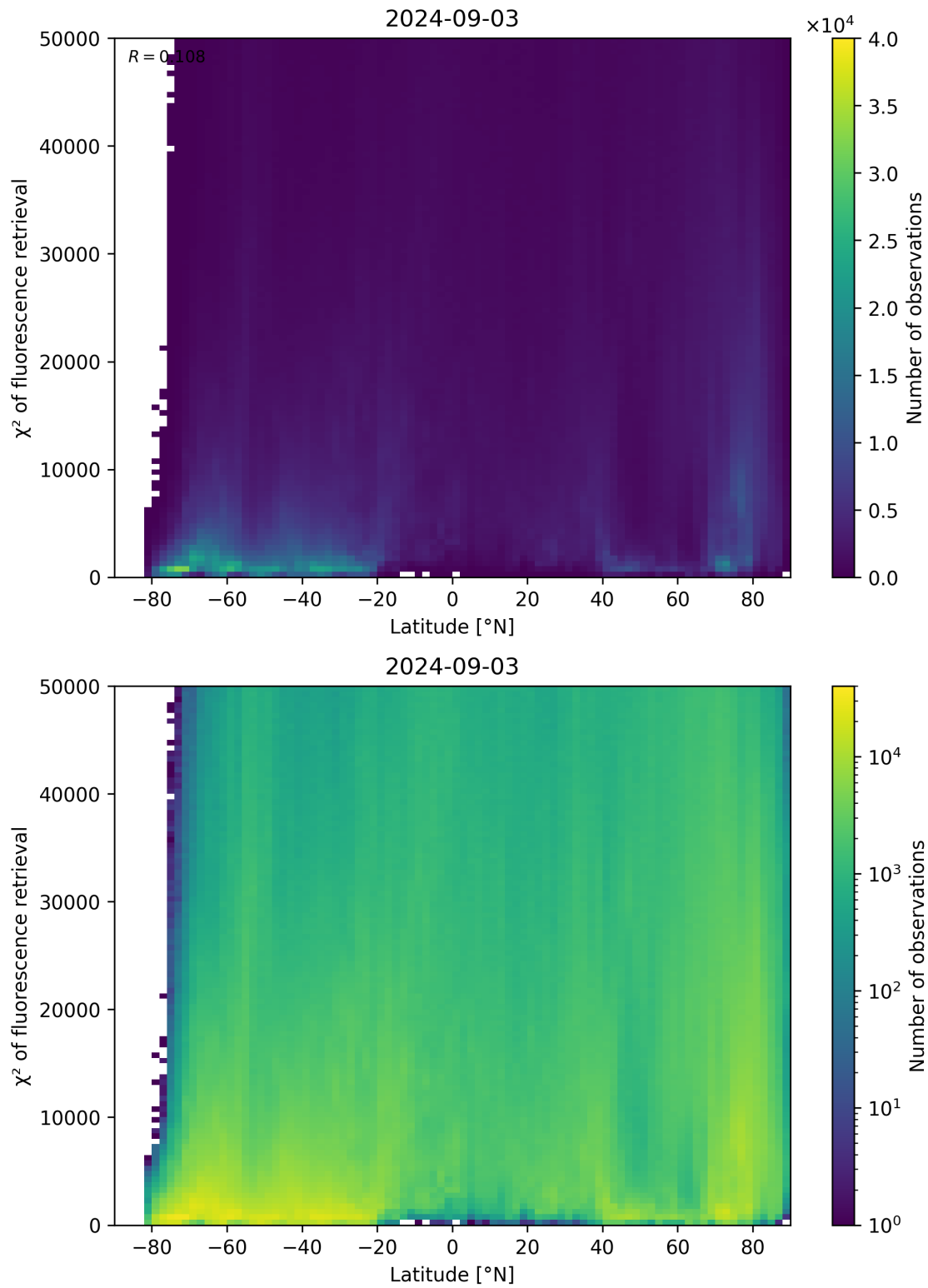
Figure 89: Scatter density plot of “Latitude” against “ \chi^2 of fluorescence retrieval” for 2024-09-02 to 2024-09-04.
