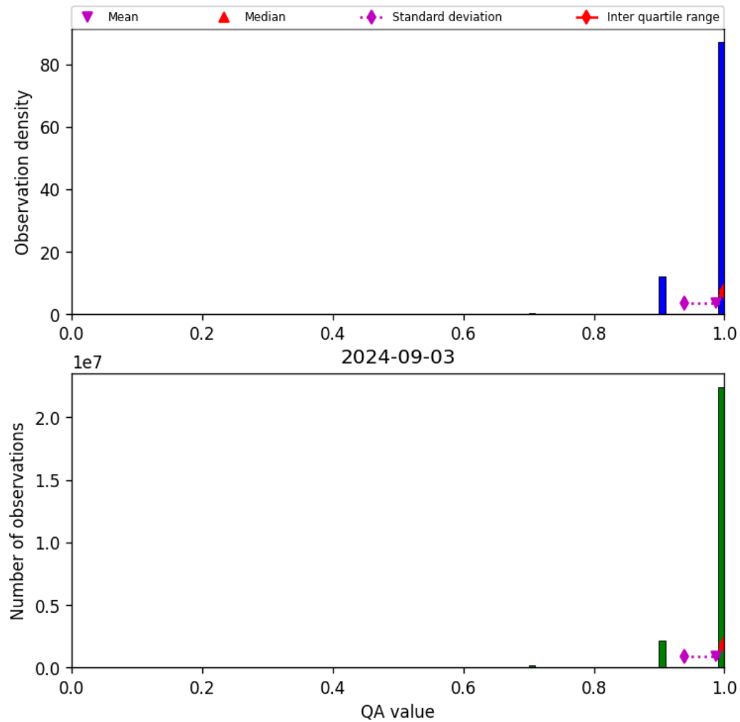
Figure 29: Histogram of “QA value” for 2024-09-02 to 2024-09-04
