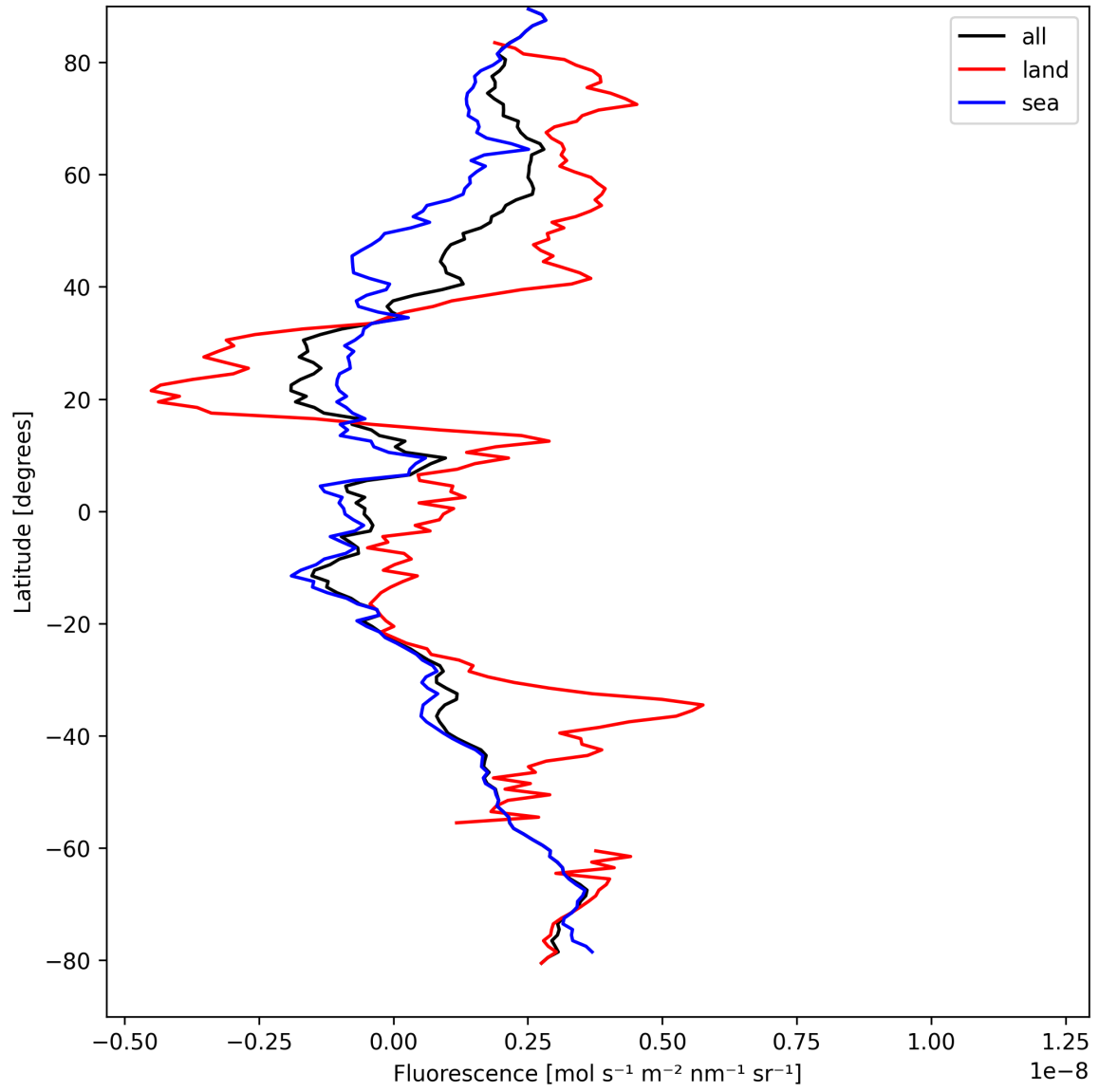
Figure 23: Zonal average of “Fluorescence” for 2024-09-02 to 2024-09-04.
