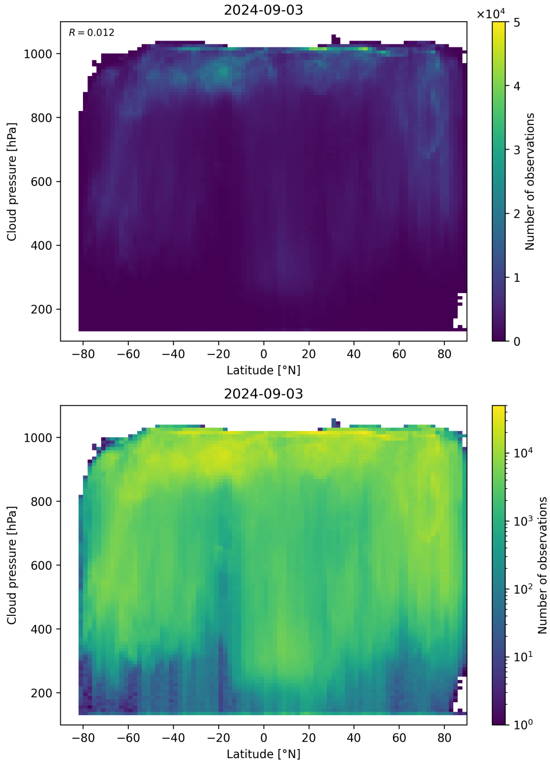
Figure 91: Scatter density plot of “Latitude” against “Cloud pressure” for 2024-09-02 to 2024-09-04.
