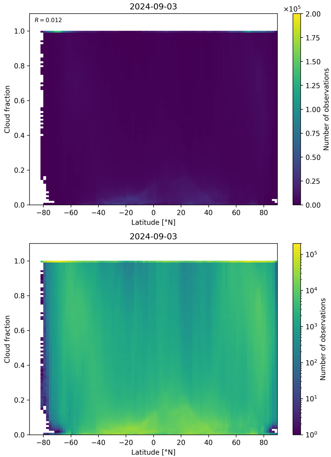
Figure 90: Scatter density plot of “Latitude” against “Cloud fraction” for 2024-09-02 to 2024-09-04.
