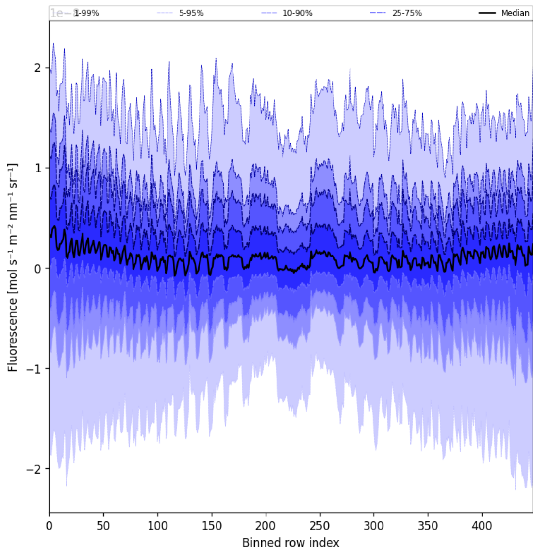
Figure 57: Along track statistics of “Fluorescence” for 2024-09-02 to 2024-09-04
