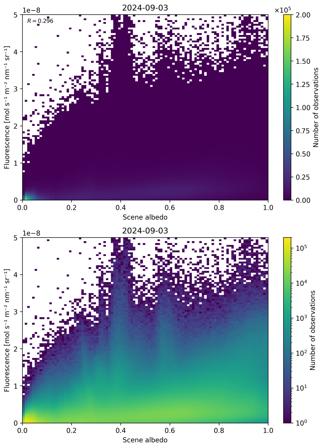
Figure 104: Scatter density plot of “Scene albedo” against “Fluorescence” for 2024-09-02 to 2024-09-04.
