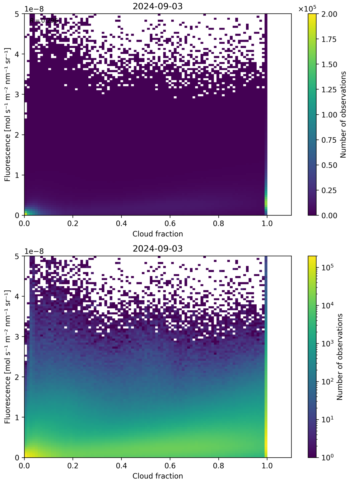
Figure 72: Scatter density plot of “Cloud fraction” against “Fluorescence” for 2024-09-02 to 2024-09-04.
