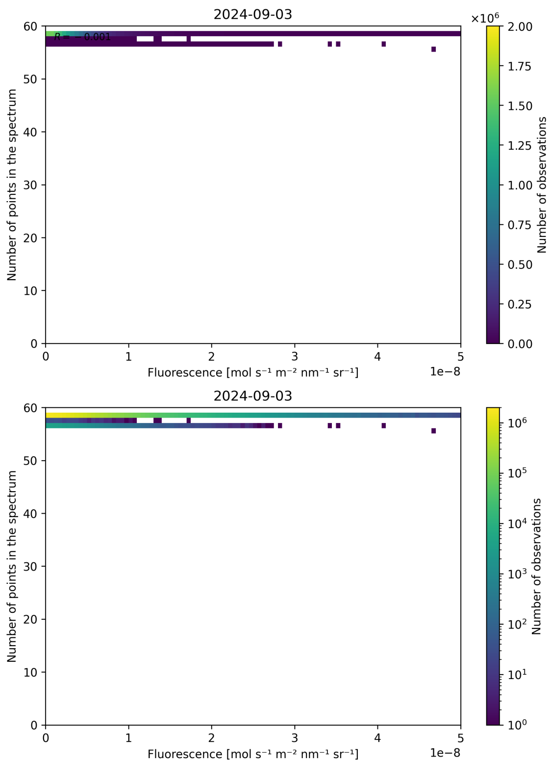
Figure 86: Scatter density plot of “Fluorescence” against “Number of points in the spectrum” for 2024-09-02 to 2024-09-04.
