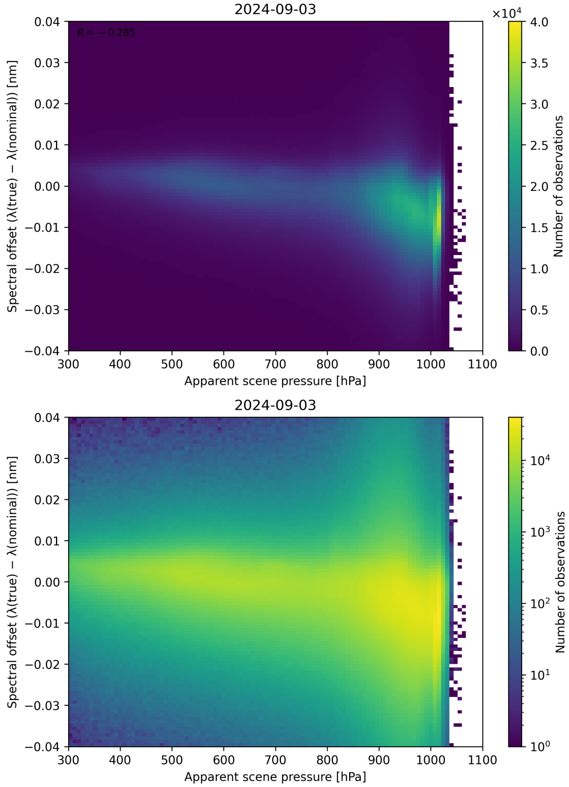
Figure 67: Scatter density plot of “Apparent scene pressure” against “Spectral offset ( \lambda_{\text{true}} - \lambda_{\text{nominal}} )” for 2024-09-02 to 2024-09-04.
