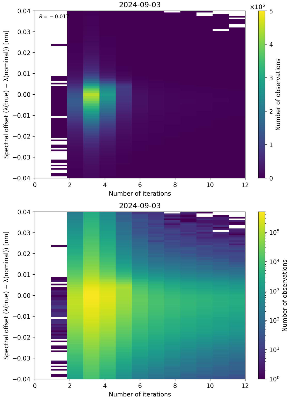
Figure 100: Scatter density plot of “Number of iterations” against “Spectral offset ( \lambda_{\text{true}} - \lambda_{\text{nominal}} )” for 2024-09-02 to 2024-09-04.
