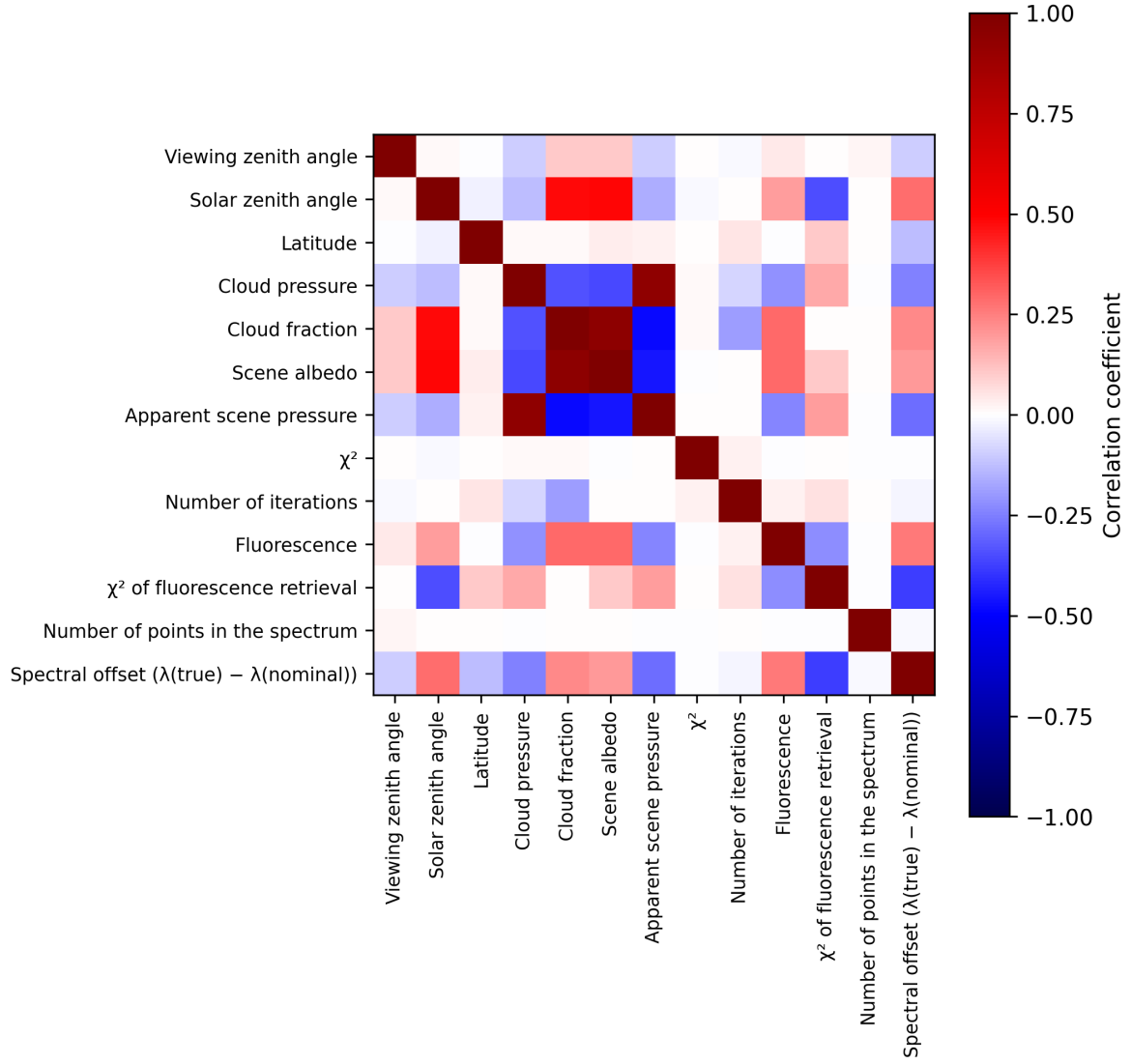
Figure 2: Map of correlation matrix for 2024-09-02 to 2024-09-04.
