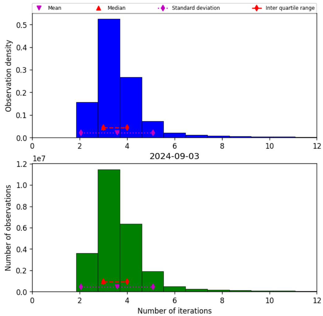
Figure 39: Histogram of “Number of iterations” for 2024-09-02 to 2024-09-04
