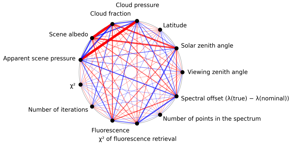
Figure 1: Map of correlation graph for 2024-09-02 to 2024-09-04.
