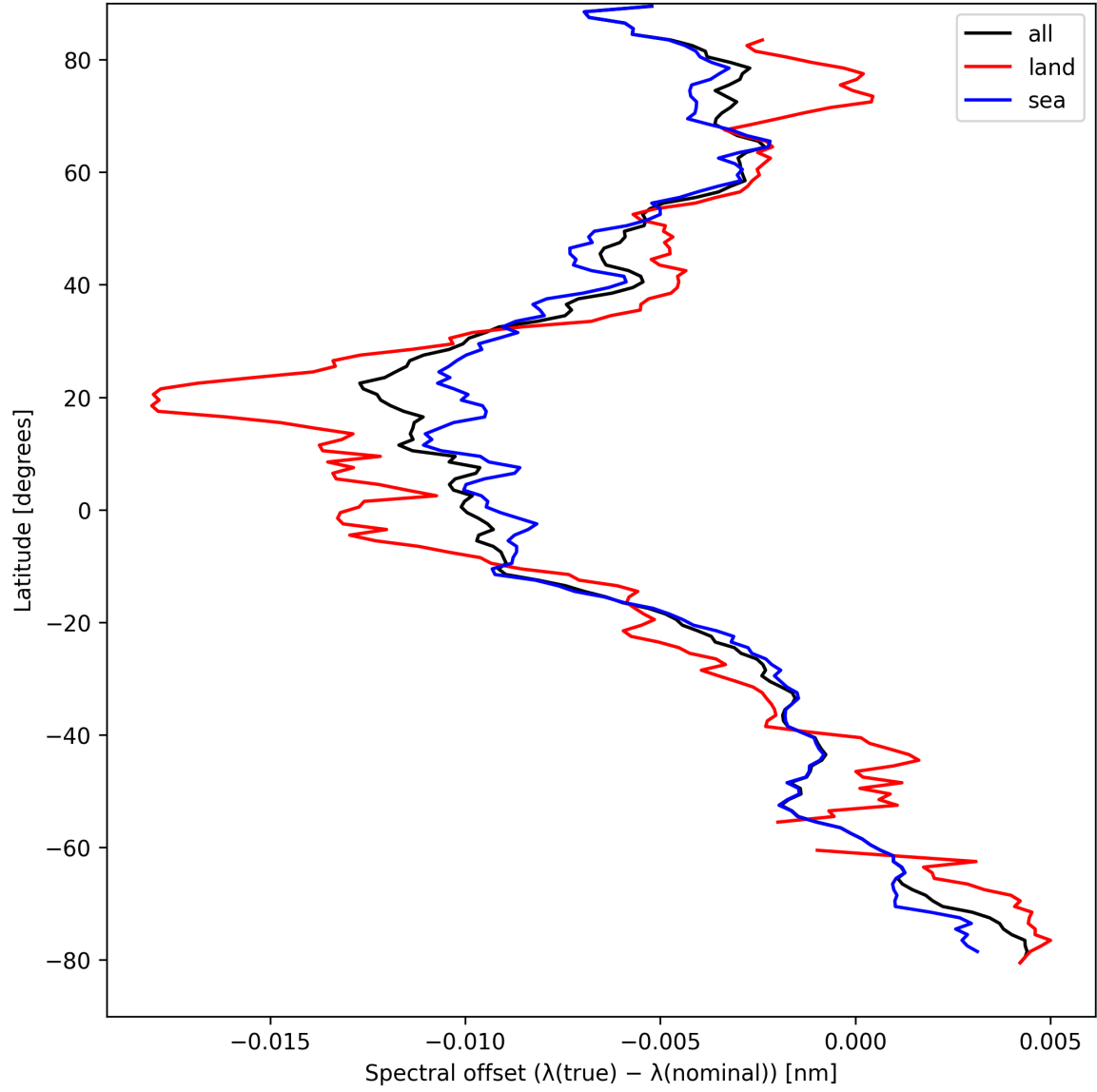
Figure 28: Zonal average of “Spectral offset ( \lambda_{\text{true}} - \lambda_{\text{nominal}} )” for 2024-09-02 to 2024-09-04.
