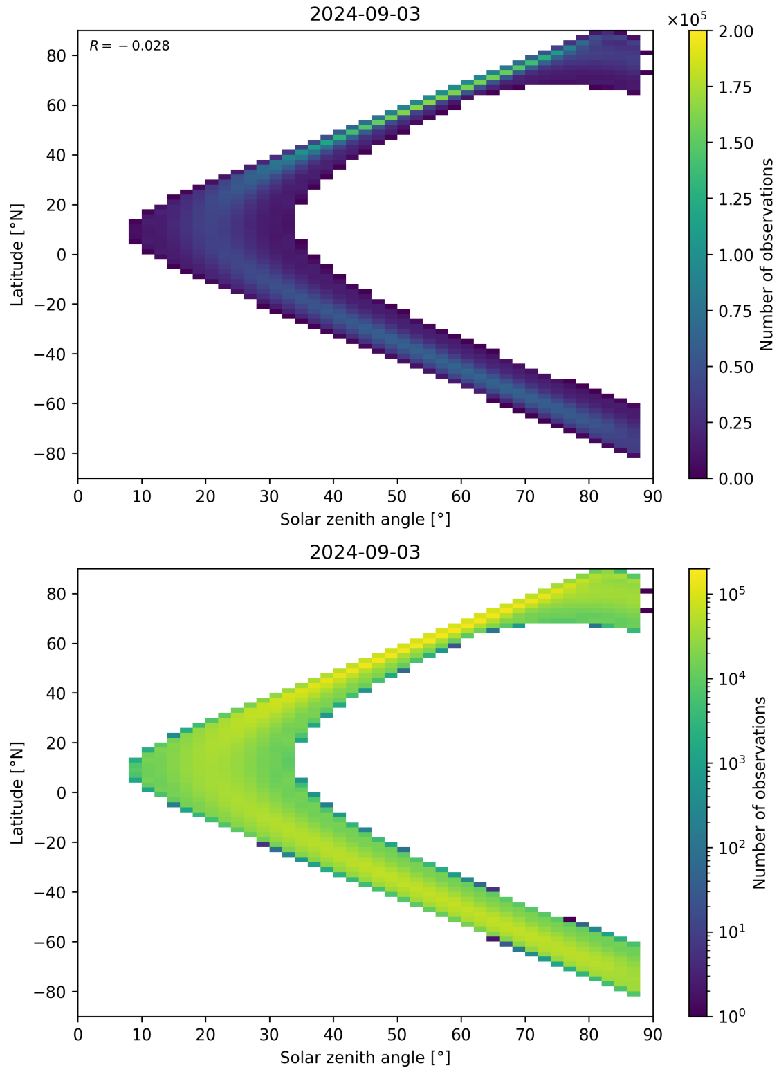
Figure 113: Scatter density plot of “Solar zenith angle” against “Latitude” for 2024-09-02 to 2024-09-04.
