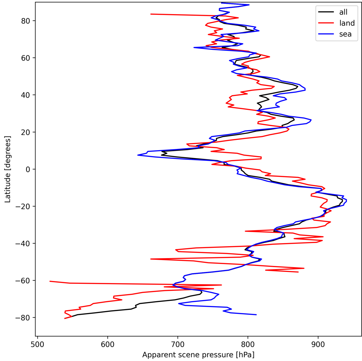
Figure 19: Zonal average of “Apparent scene pressure” for 2024-09-02 to 2024-09-04.
