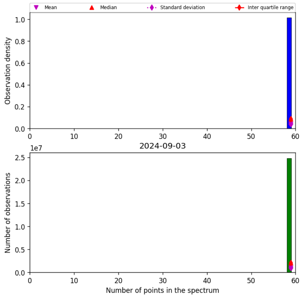
Figure 44: Histogram of “Number of points in the spectrum” for 2024-09-02 to 2024-09-04
