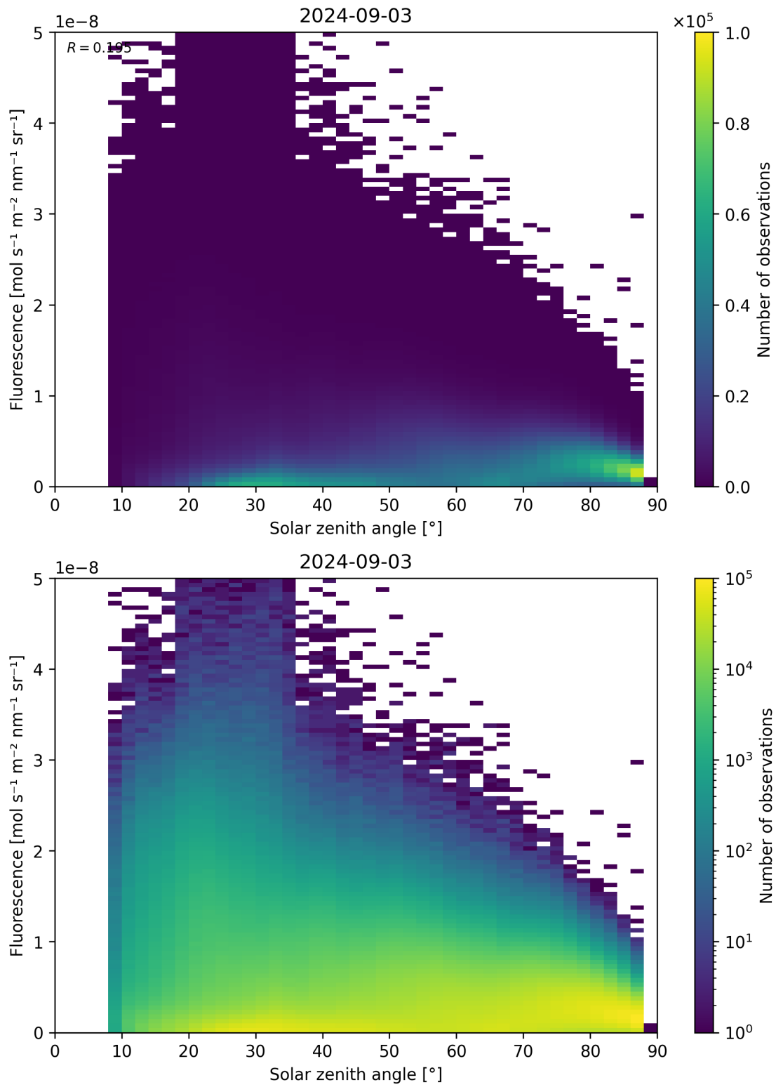
Figure 112: Scatter density plot of “Solar zenith angle” against “Fluorescence” for 2024-09-02 to 2024-09-04.
