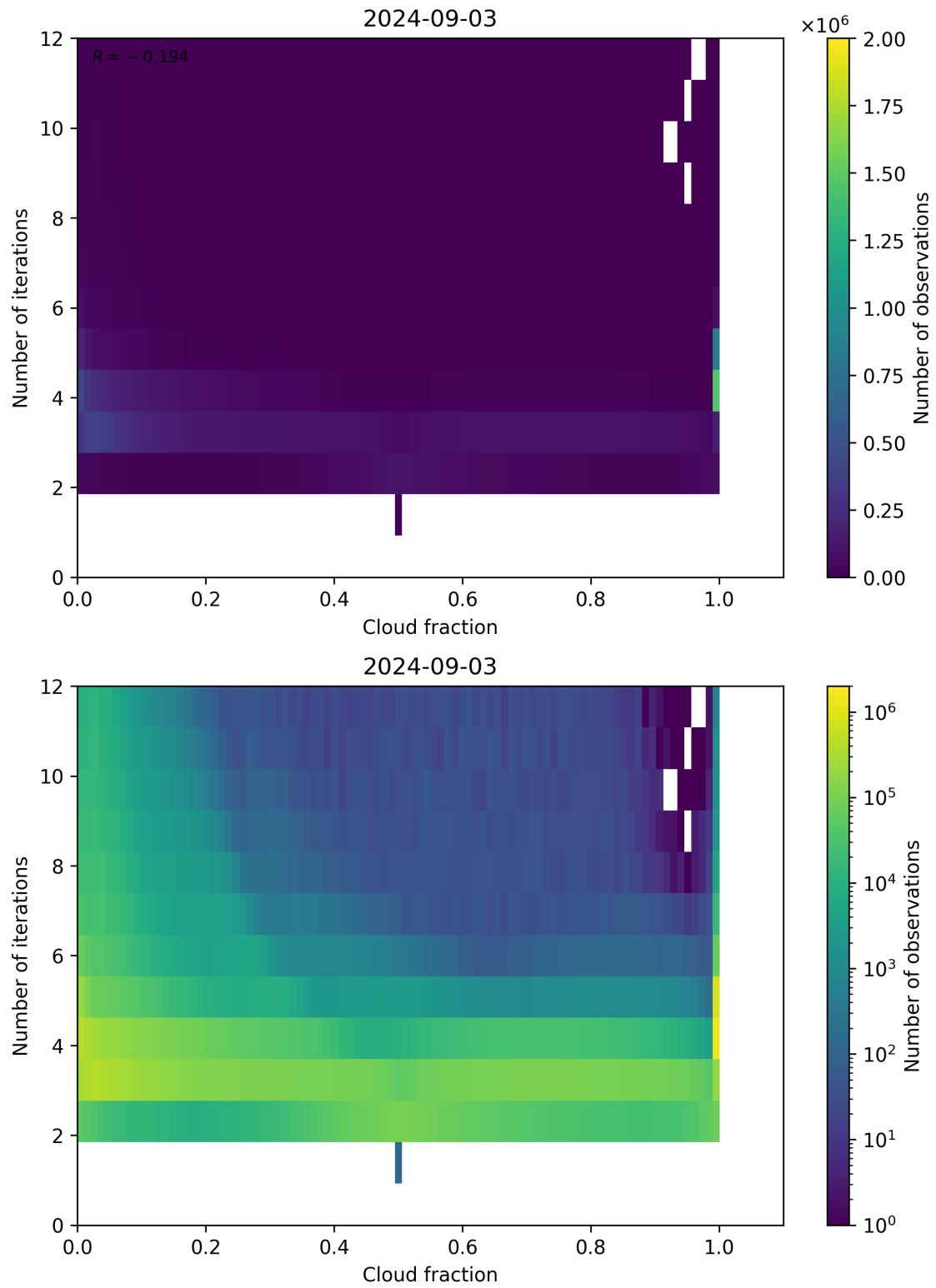
Figure 73: Scatter density plot of “Cloud fraction” against “Number of iterations” for 2024-09-02 to 2024-09-04.
