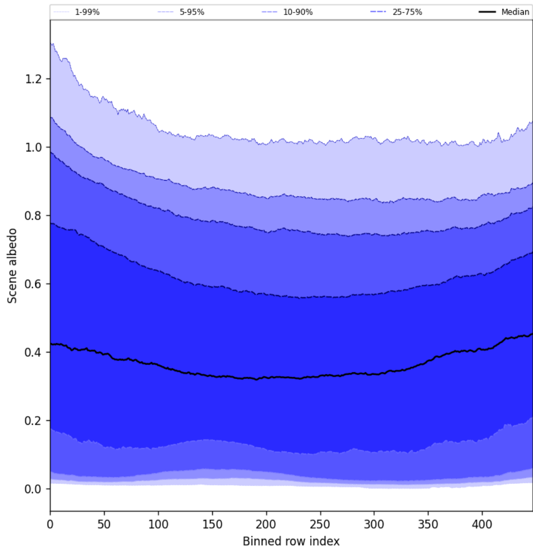
Figure 51: Along track statistics of “Scene albedo” for 2024-09-02 to 2024-09-04
