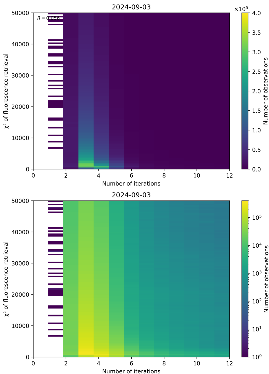
Figure 97: Scatter density plot of “Number of iterations” against “ \chi^2 of fluorescence retrieval” for 2024-09-02 to 2024-09-04.
