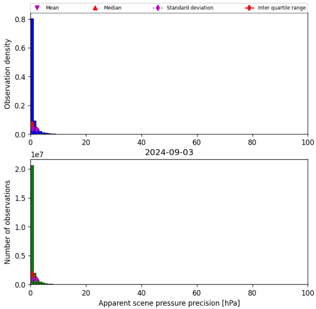
Figure 37: Histogram of “Apparent scene pressure precision” for 2024-09-02 to 2024-09-04
