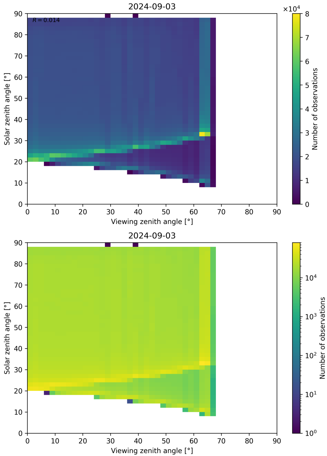
Figure 127: Scatter density plot of “Viewing zenith angle” against “Solar zenith angle” for 2024-09-02 to 2024-09-04.
