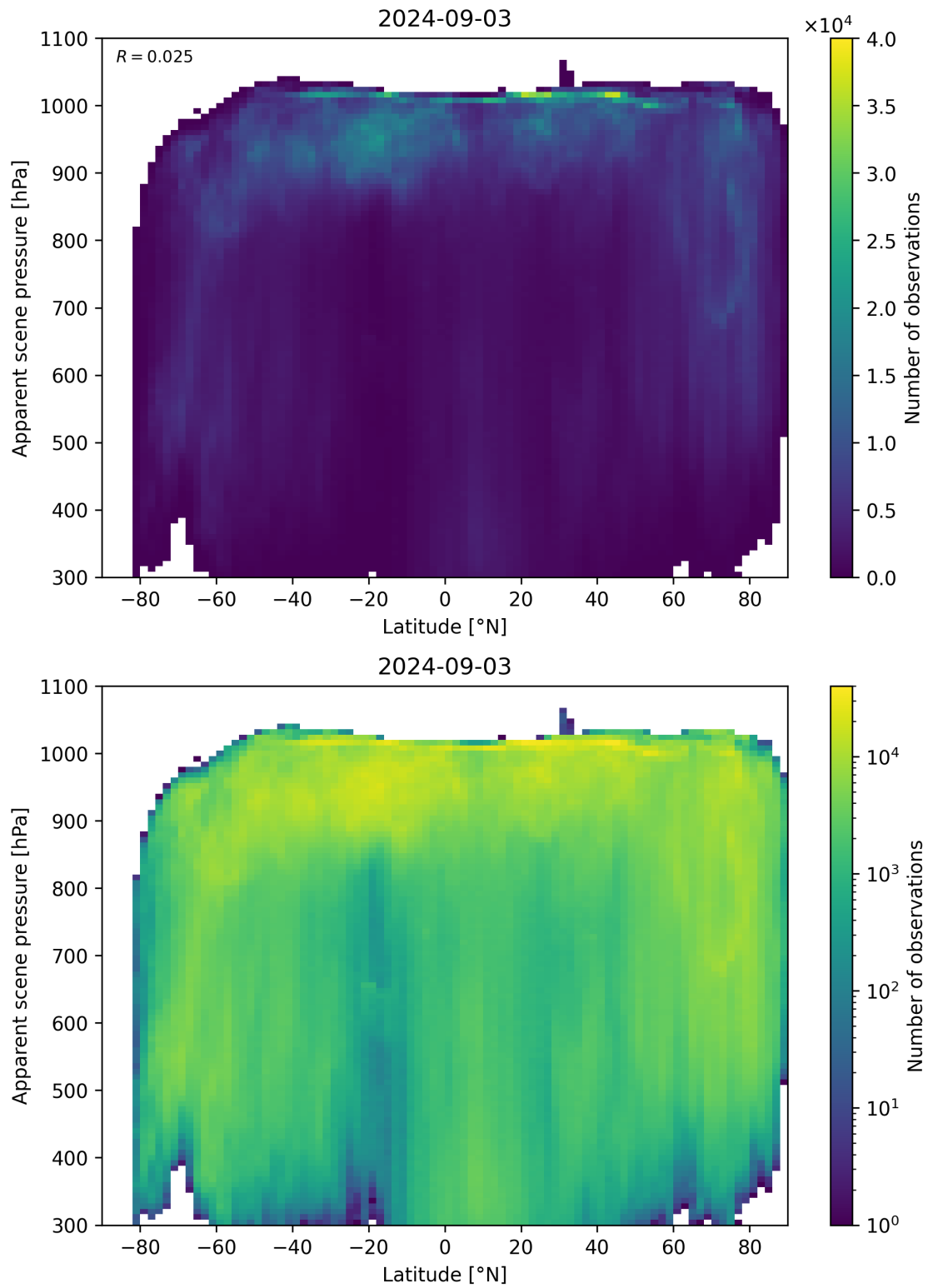
Figure 88: Scatter density plot of “Latitude” against “Apparent scene pressure” for 2024-09-02 to 2024-09-04.
