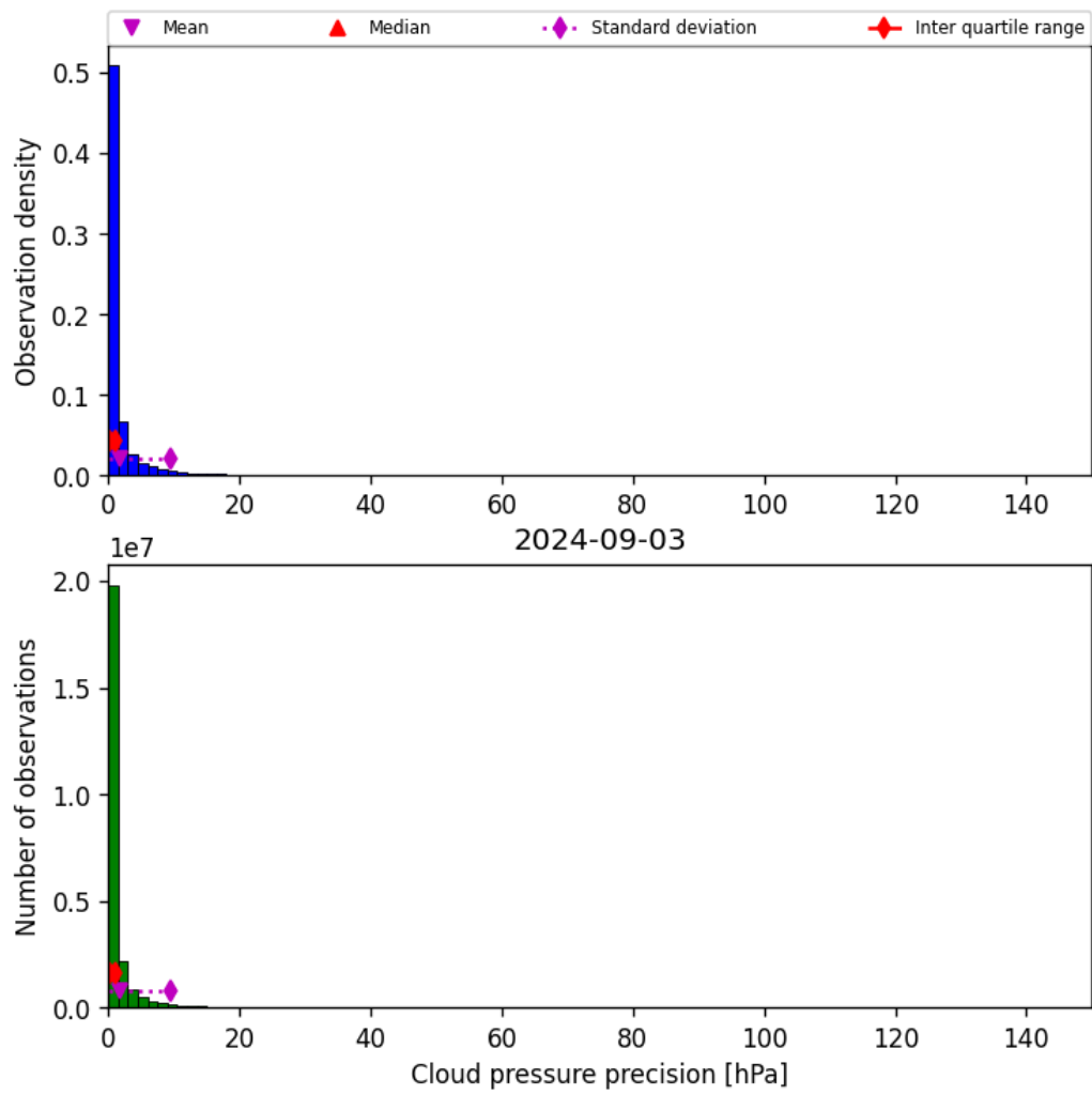
Figure 31: Histogram of “Cloud pressure precision” for 2024-09-02 to 2024-09-04
