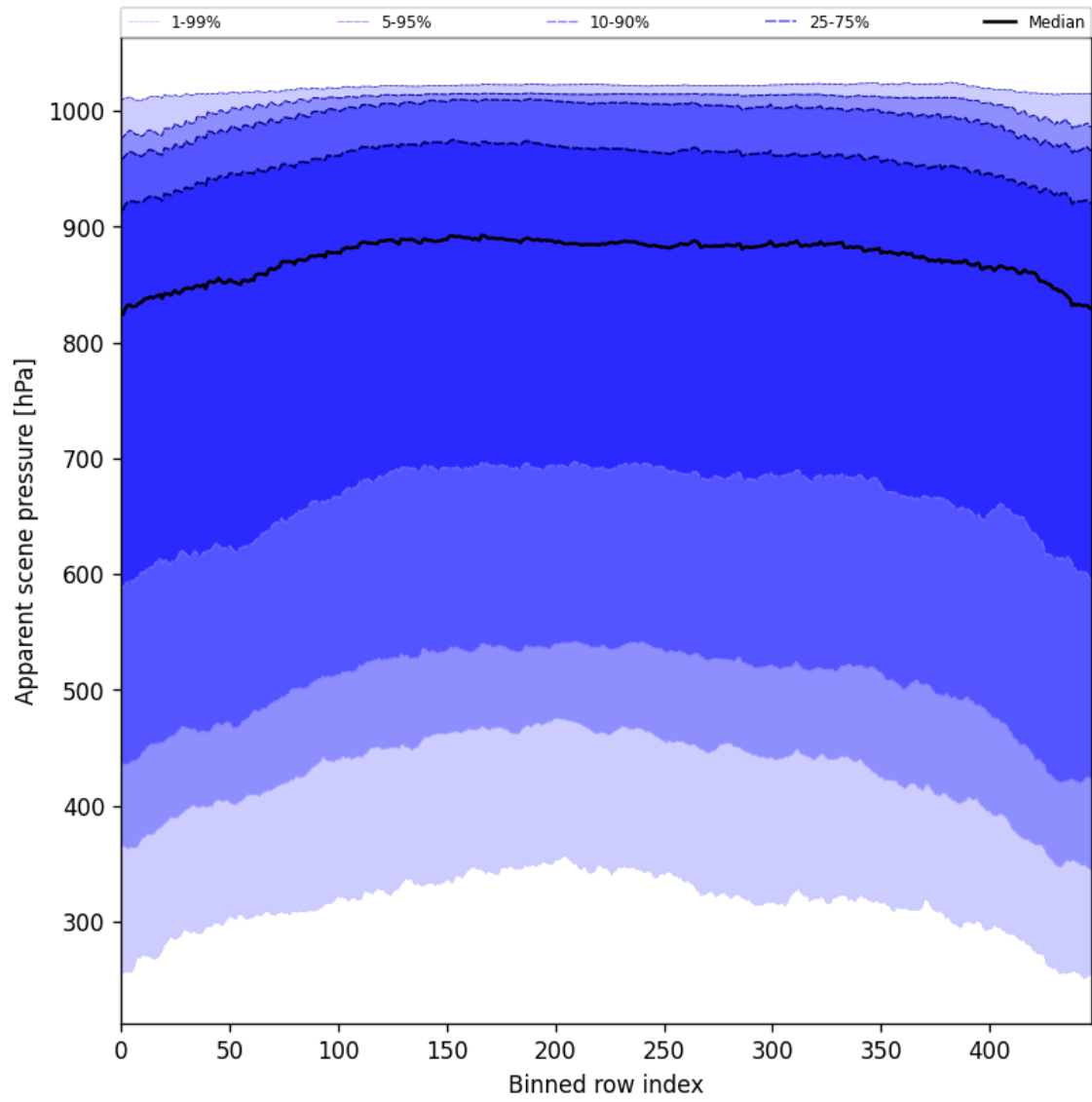
Figure 53: Along track statistics of “Apparent scene pressure” for 2024-09-02 to 2024-09-04
