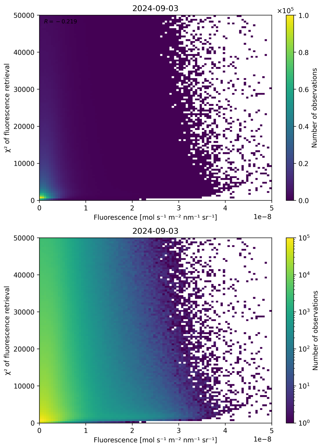
Figure 85: Scatter density plot of “Fluorescence” against “ \chi^2 of fluorescence retrieval” for 2024-09-02 to 2024-09-04.
