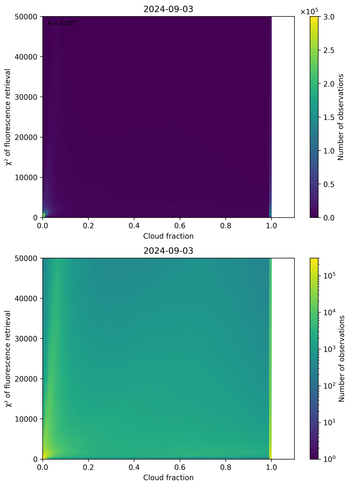
Figure 71: Scatter density plot of “Cloud fraction” against “ \chi^2 of fluorescence retrieval” for 2024-09-02 to 2024-09-04.
