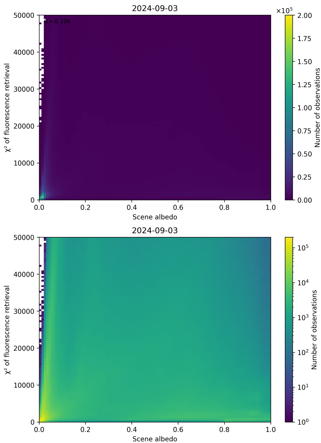
Figure 103: Scatter density plot of “Scene albedo” against “ \chi^2 of fluorescence retrieval” for 2024-09-02 to 2024-09-04.
