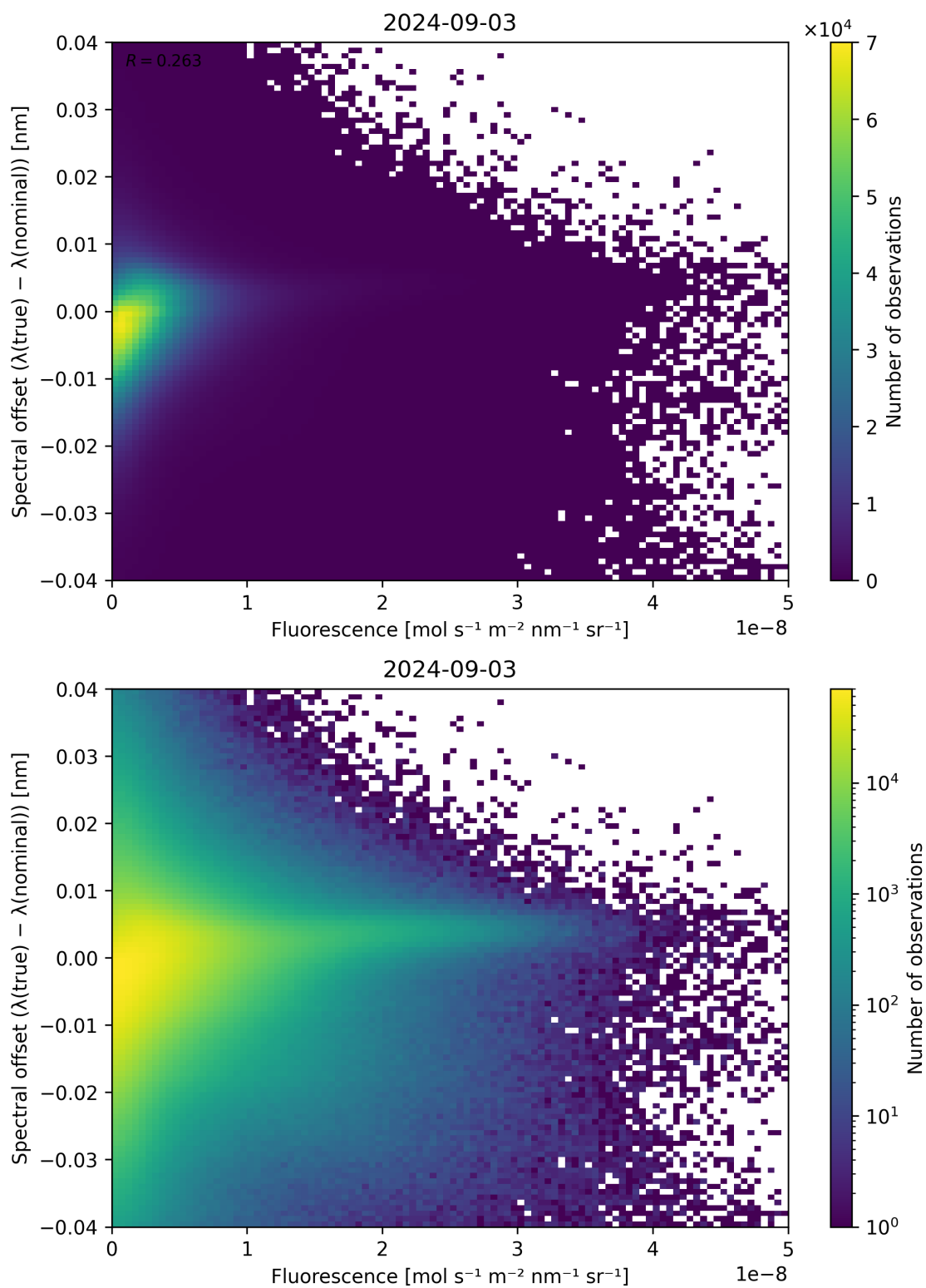
Figure 87: Scatter density plot of “Fluorescence” against “Spectral offset ( \lambda_{\text{true}} - \lambda_{\text{nominal}} )” for 2024-09-02 to 2024-09-04.
