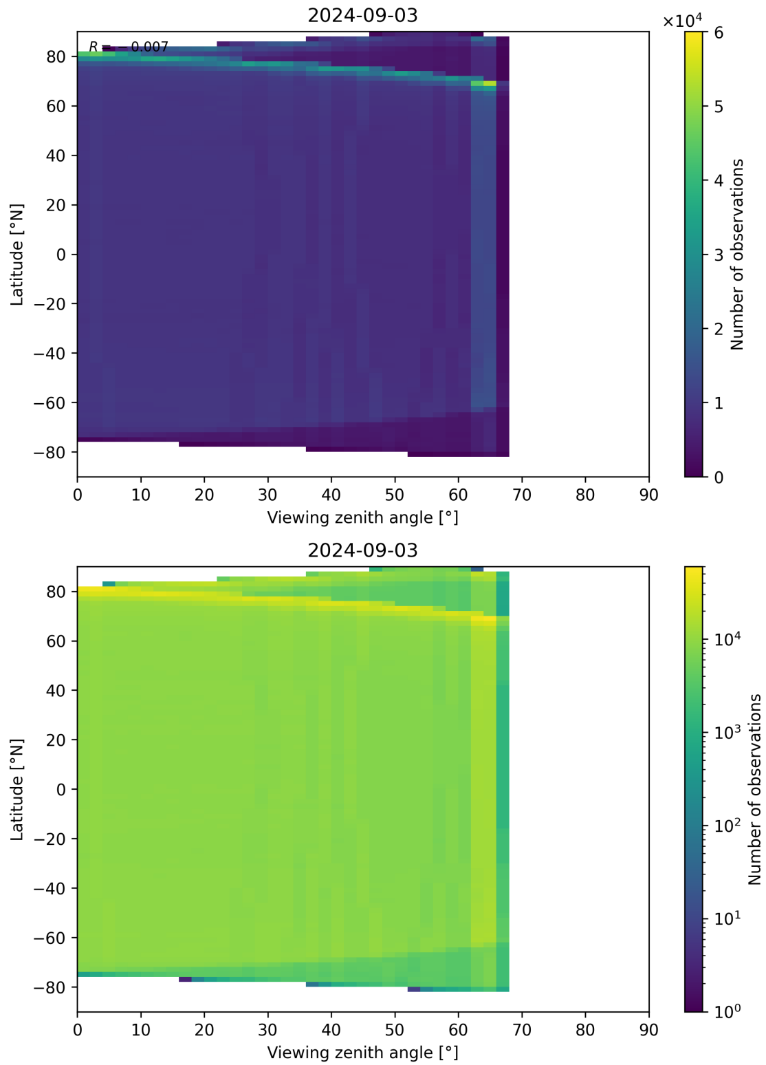
Figure 123: Scatter density plot of “Viewing zenith angle” against “Latitude” for 2024-09-02 to 2024-09-04.
