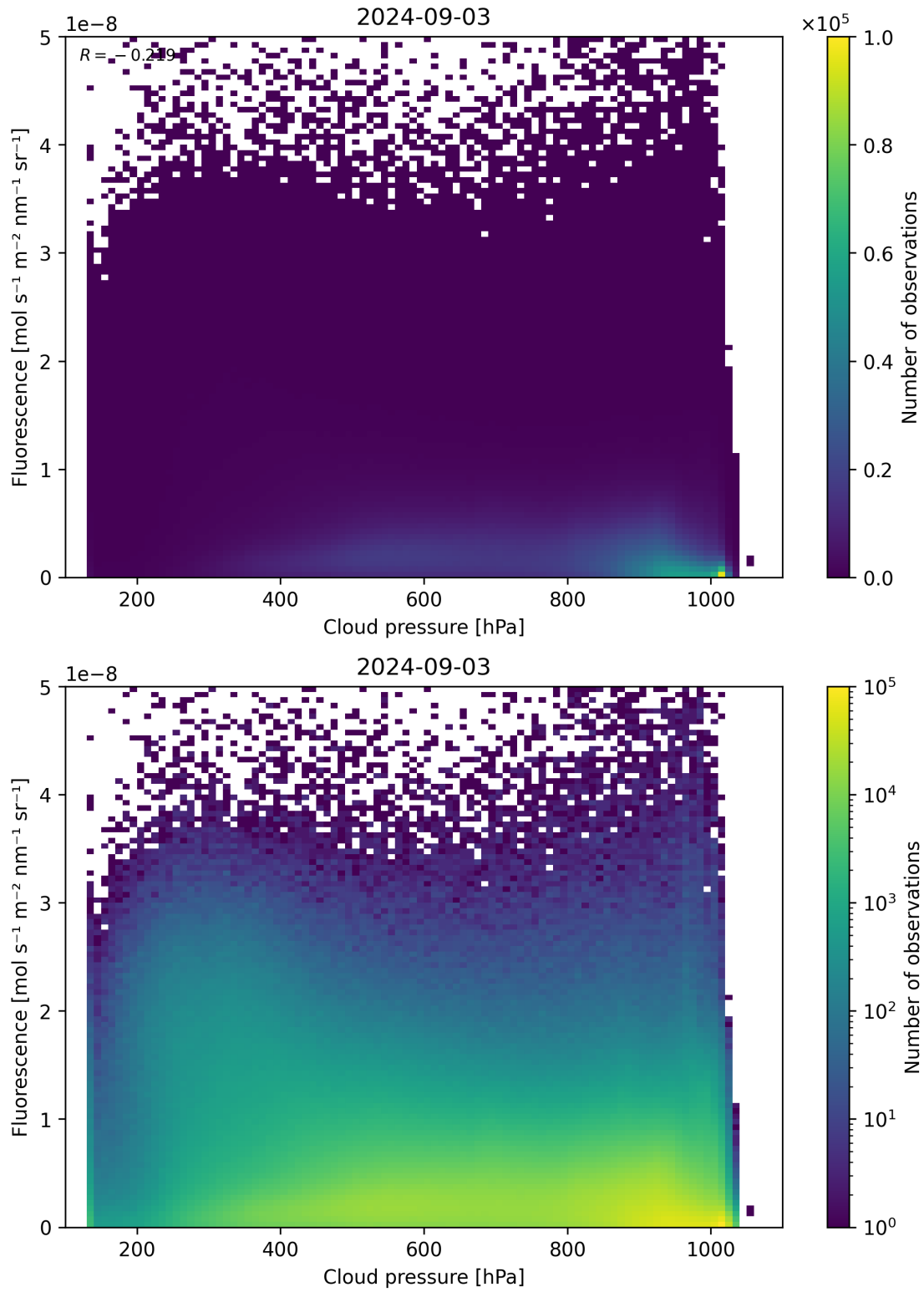
Figure 80: Scatter density plot of “Cloud pressure” against “Fluorescence” for 2024-09-02 to 2024-09-04.
