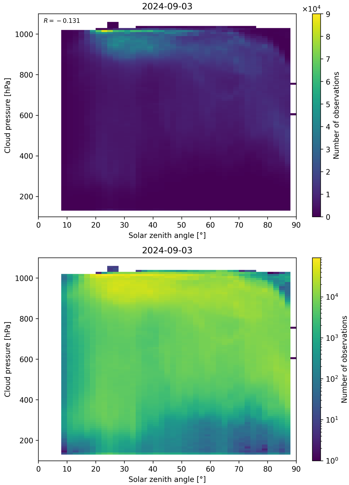
Figure 111: Scatter density plot of “Solar zenith angle” against “Cloud pressure” for 2024-09-02 to 2024-09-04.
