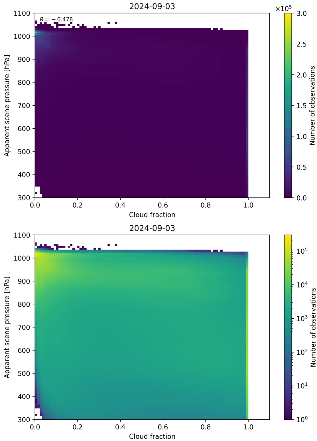
Figure 70: Scatter density plot of “Cloud fraction” against “Apparent scene pressure” for 2024-09-02 to 2024-09-04.
