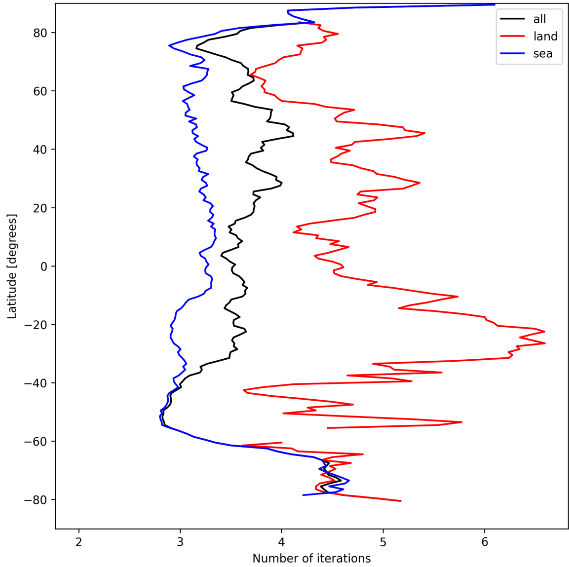
Figure 22: Zonal average of “Number of iterations” for 2024-09-02 to 2024-09-04.
