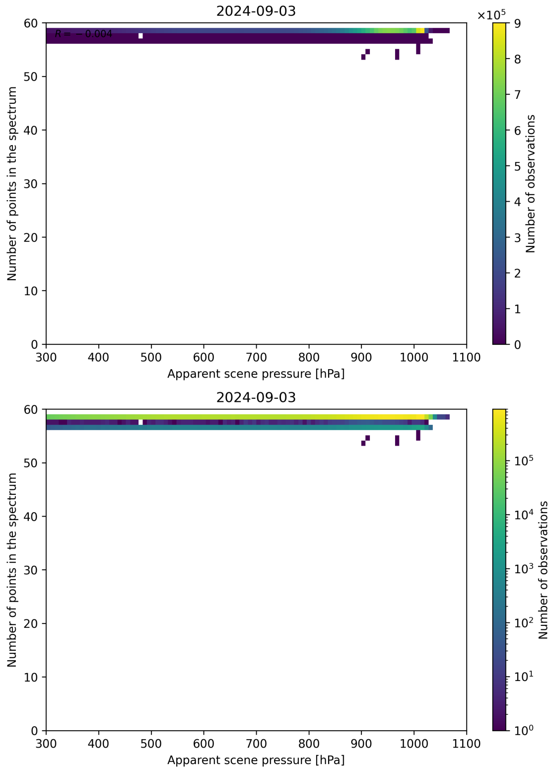
Figure 66: Scatter density plot of “Apparent scene pressure” against “Number of points in the spectrum” for 2024-09-02 to 2024-09-04.
