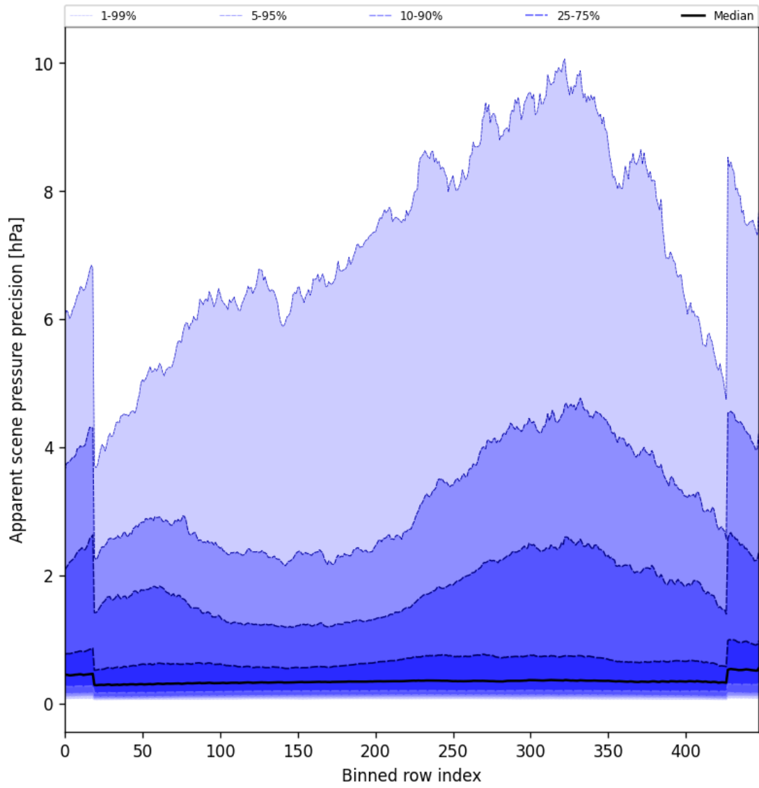
Figure 54: Along track statistics of “Apparent scene pressure precision” for 2024-09-02 to 2024-09-04
