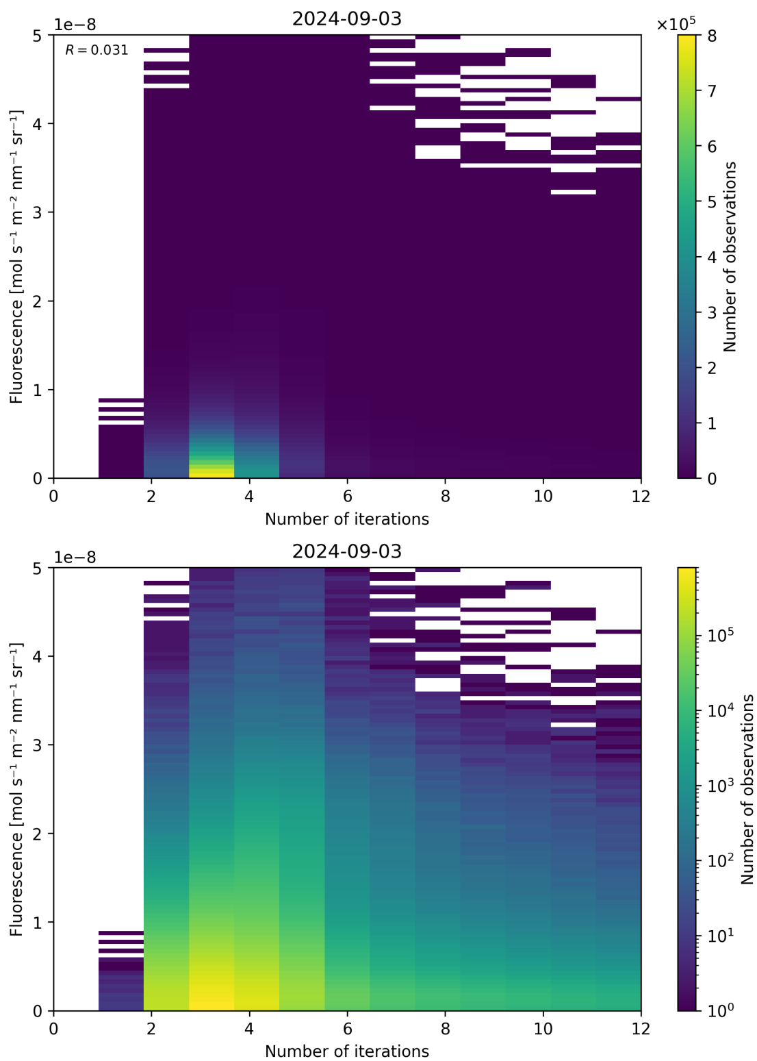
Figure 98: Scatter density plot of “Number of iterations” against “Fluorescence” for 2024-09-02 to 2024-09-04.
