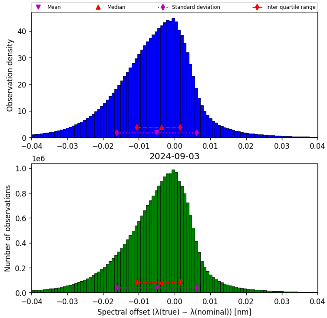
Figure 45: Histogram of “Spectral offset ( \lambda_{\text{true}} - \lambda_{\text{nominal}} )” for 2024-09-02 to 2024-09-04
