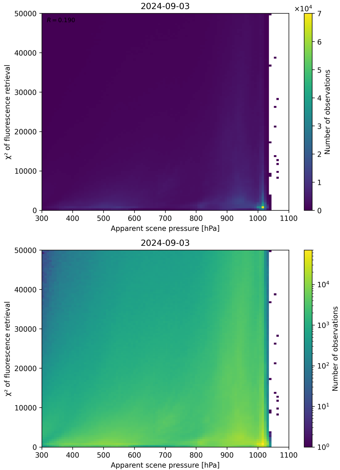
Figure 63: Scatter density plot of “Apparent scene pressure” against “ \chi^2 of fluorescence retrieval” for 2024-09-02 to 2024-09-04.
