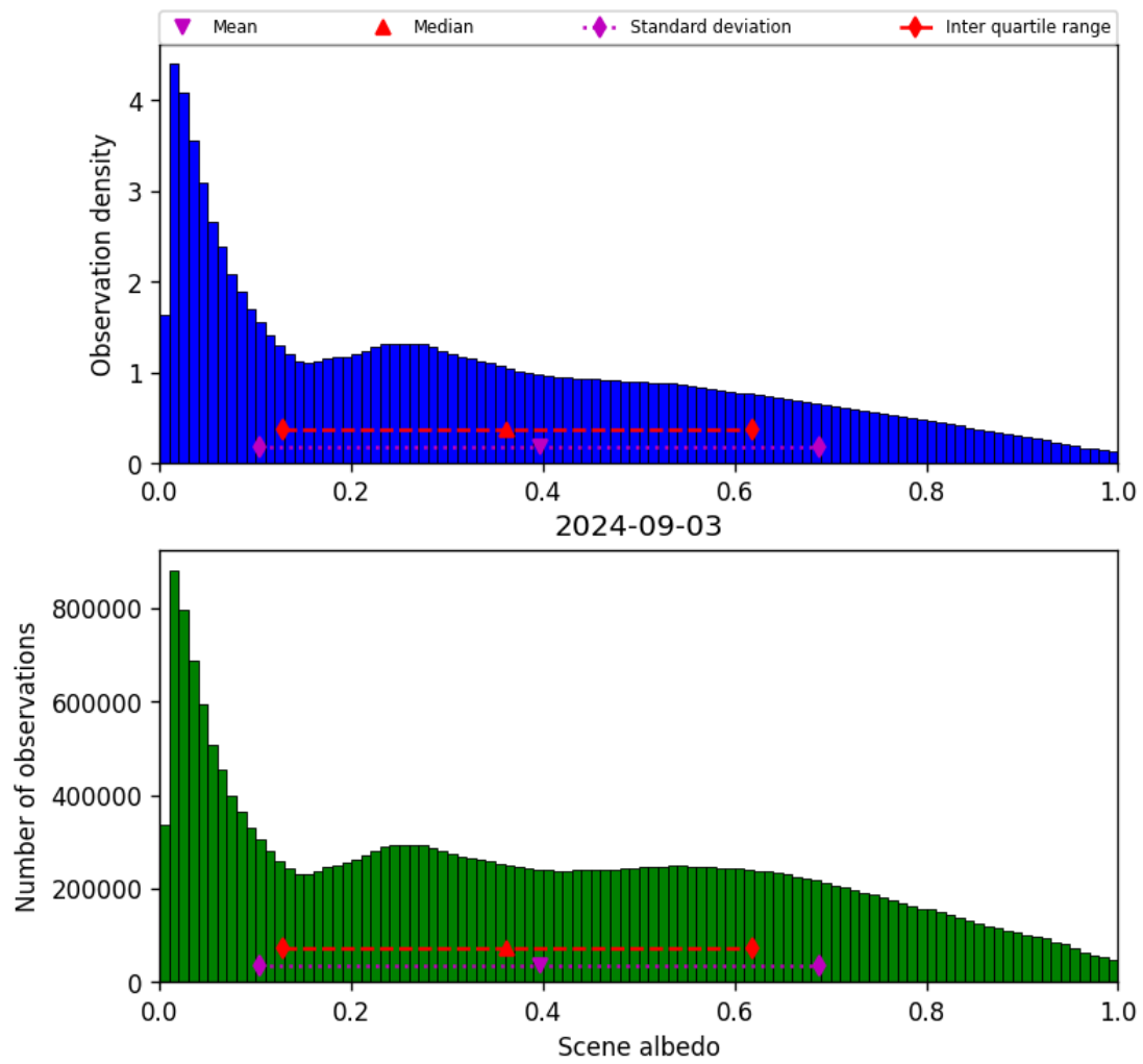
Figure 34: Histogram of “Scene albedo” for 2024-09-02 to 2024-09-04
