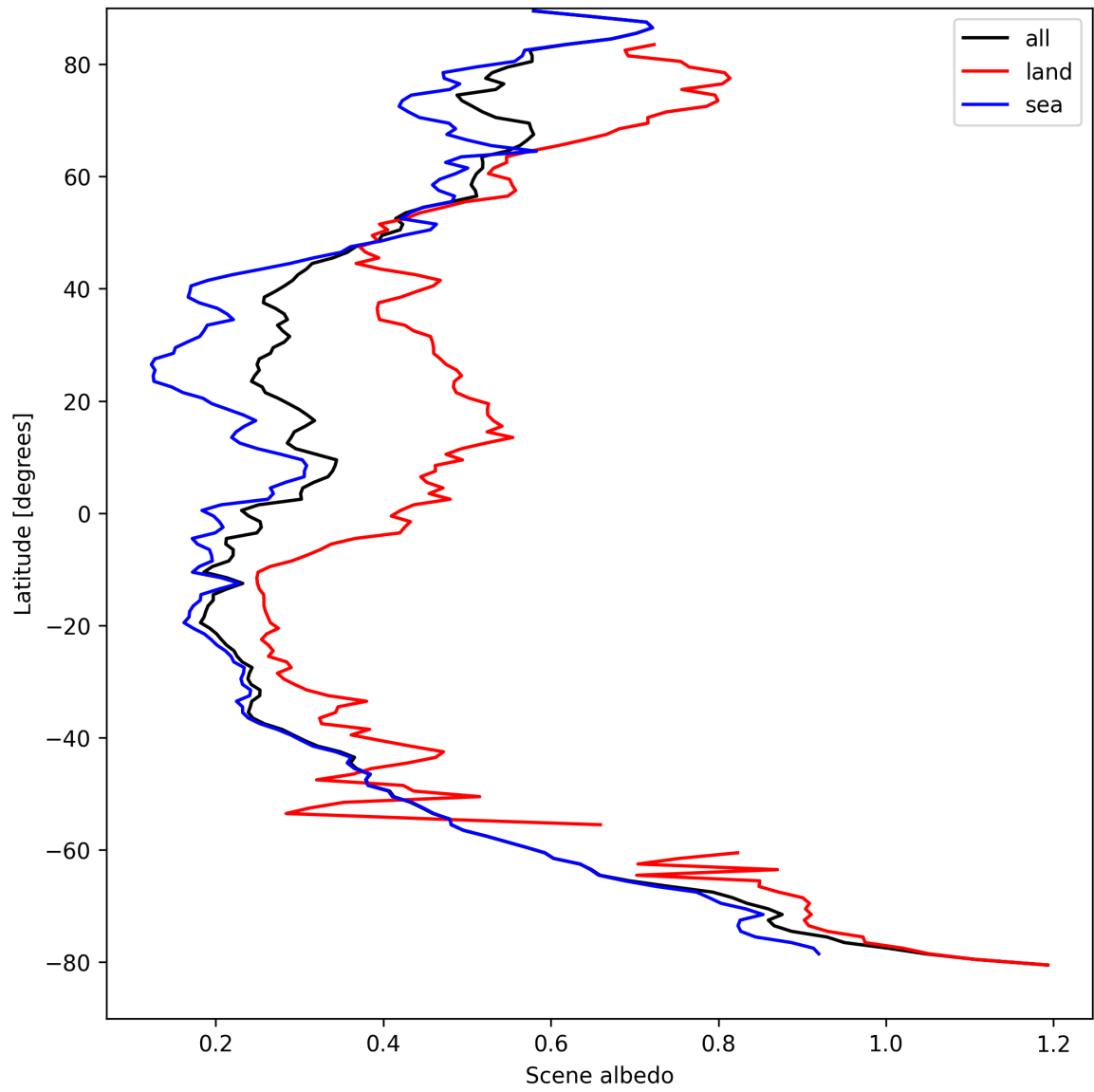
Figure 17: Zonal average of “Scene albedo” for 2024-09-02 to 2024-09-04.
