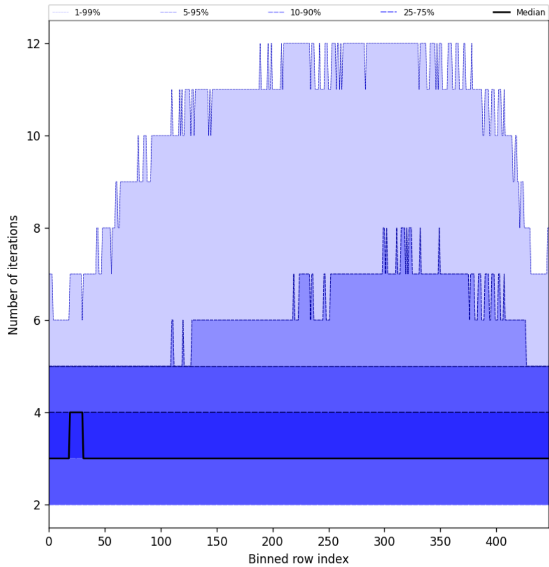
Figure 56: Along track statistics of “Number of iterations” for 2024-09-02 to 2024-09-04
