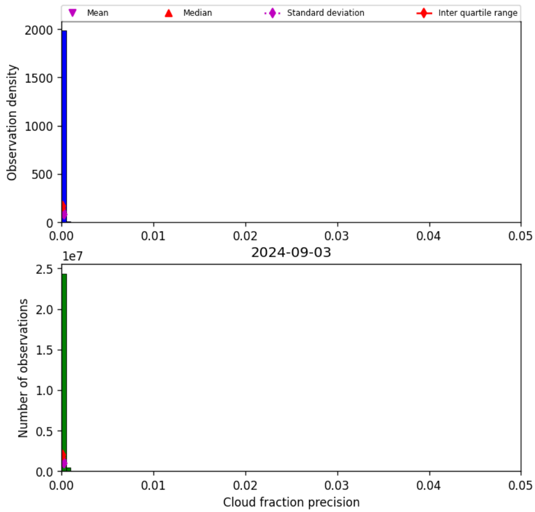
Figure 33: Histogram of “Cloud fraction precision” for 2024-09-02 to 2024-09-04
