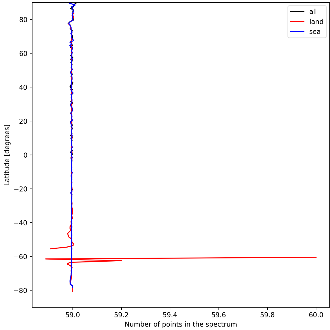
Figure 27: Zonal average of “Number of points in the spectrum” for 2024-09-02 to 2024-09-04.
