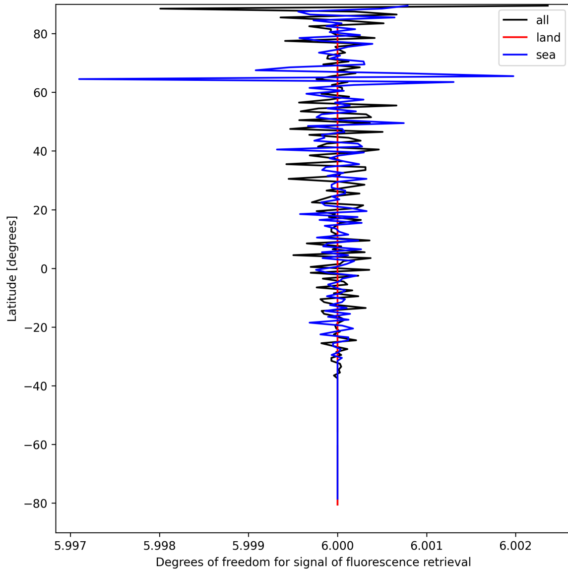
Figure 26: Zonal average of “Degrees of freedom for signal of fluorescence retrieval” for 2024-09-02 to 2024-09-04.
