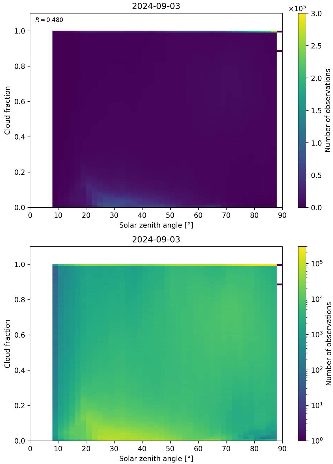
Figure 110: Scatter density plot of “Solar zenith angle” against “Cloud fraction” for 2024-09-02 to 2024-09-04.
