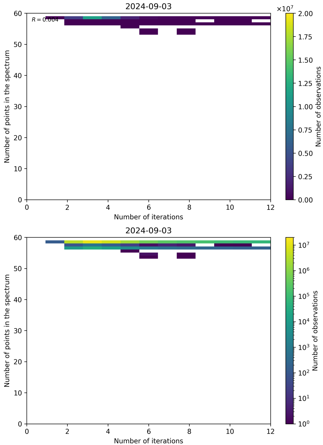
Figure 99: Scatter density plot of “Number of iterations” against “Number of points in the spectrum” for 2024-09-02 to 2024-09-04.
