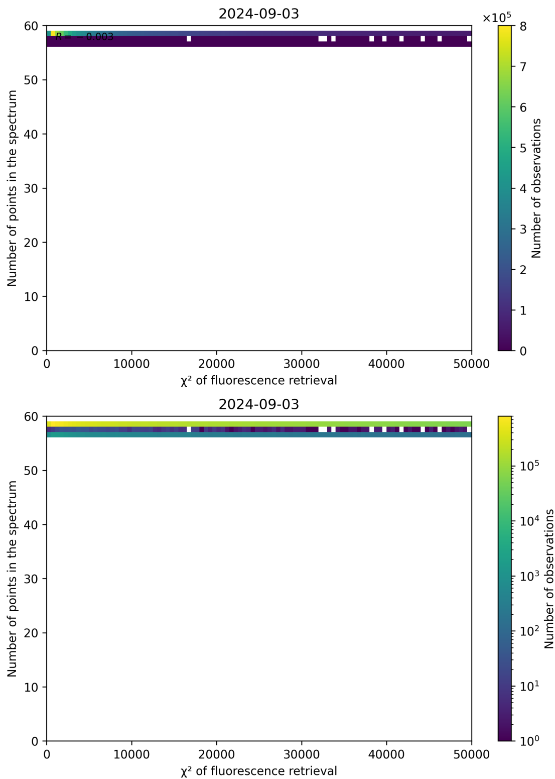
Figure 68: Scatter density plot of " \chi^2 of fluorescence retrieval" against "Number of points in the spectrum" for 2024-09-02 to 2024-09-04.
