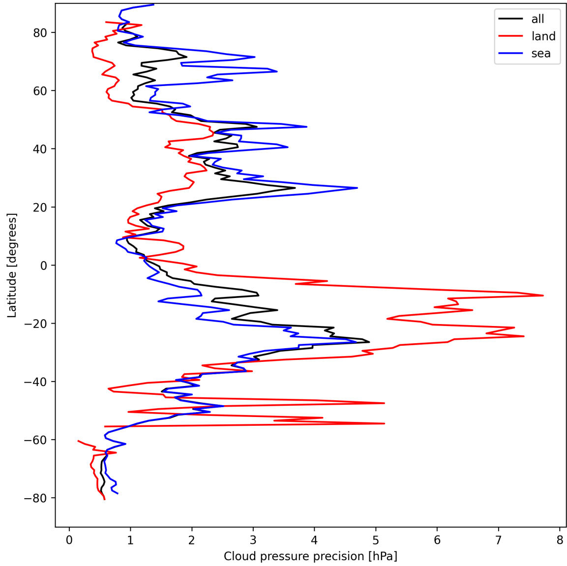
Figure 14: Zonal average of “Cloud pressure precision” for 2024-09-02 to 2024-09-04.
