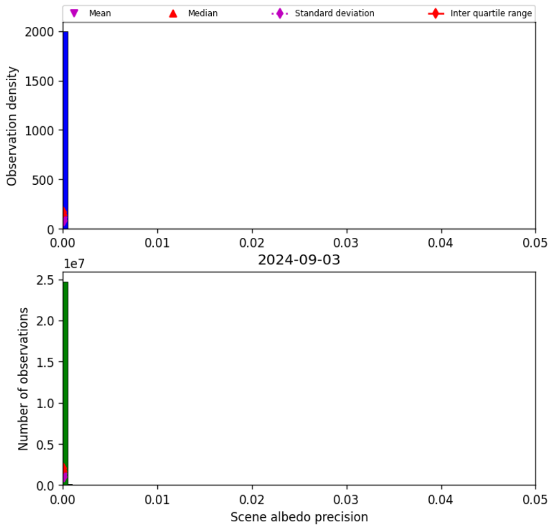
Figure 35: Histogram of “Scene albedo precision” for 2024-09-02 to 2024-09-04
