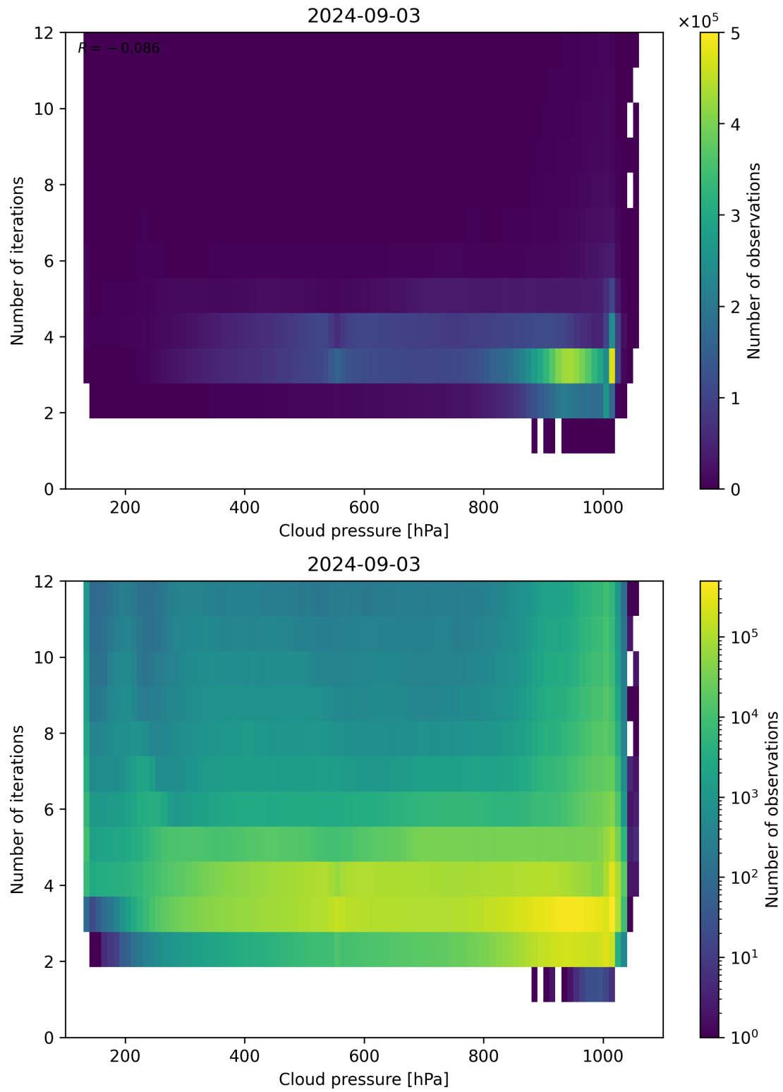
Figure 81: Scatter density plot of “Cloud pressure” against “Number of iterations” for 2024-09-02 to 2024-09-04.
