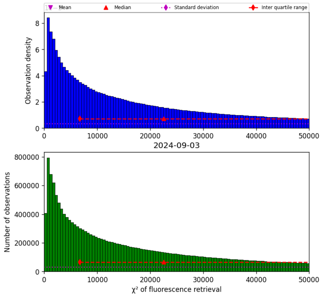
Figure 42: Histogram of “ \chi^2 of fluorescence retrieval” for 2024-09-02 to 2024-09-04
