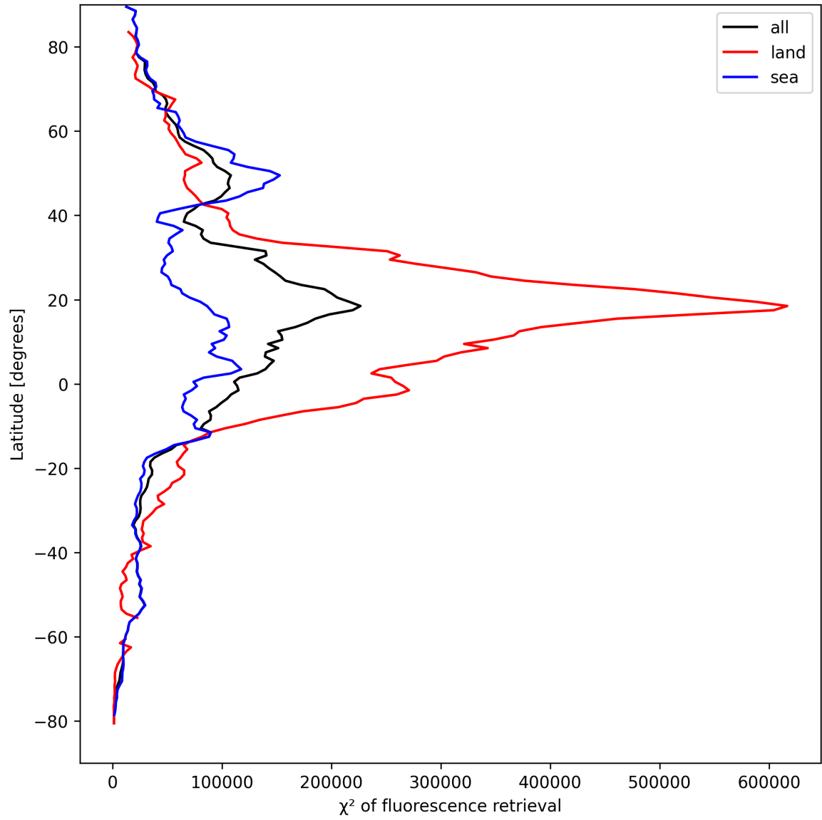
Figure 25: Zonal average of “ \chi^2 of fluorescence retrieval” for 2024-09-02 to 2024-09-04.
