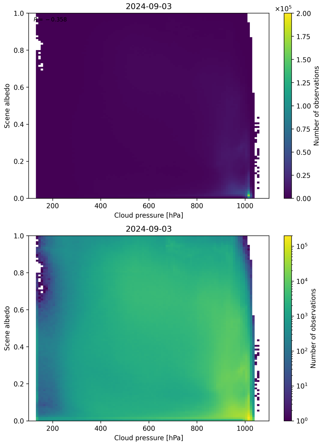
Figure 83: Scatter density plot of “Cloud pressure” against “Scene albedo” for 2024-09-02 to 2024-09-04.
