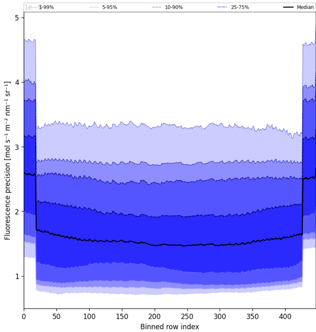
Figure 58: Along track statistics of “Fluorescence precision” for 2024-09-02 to 2024-09-04
