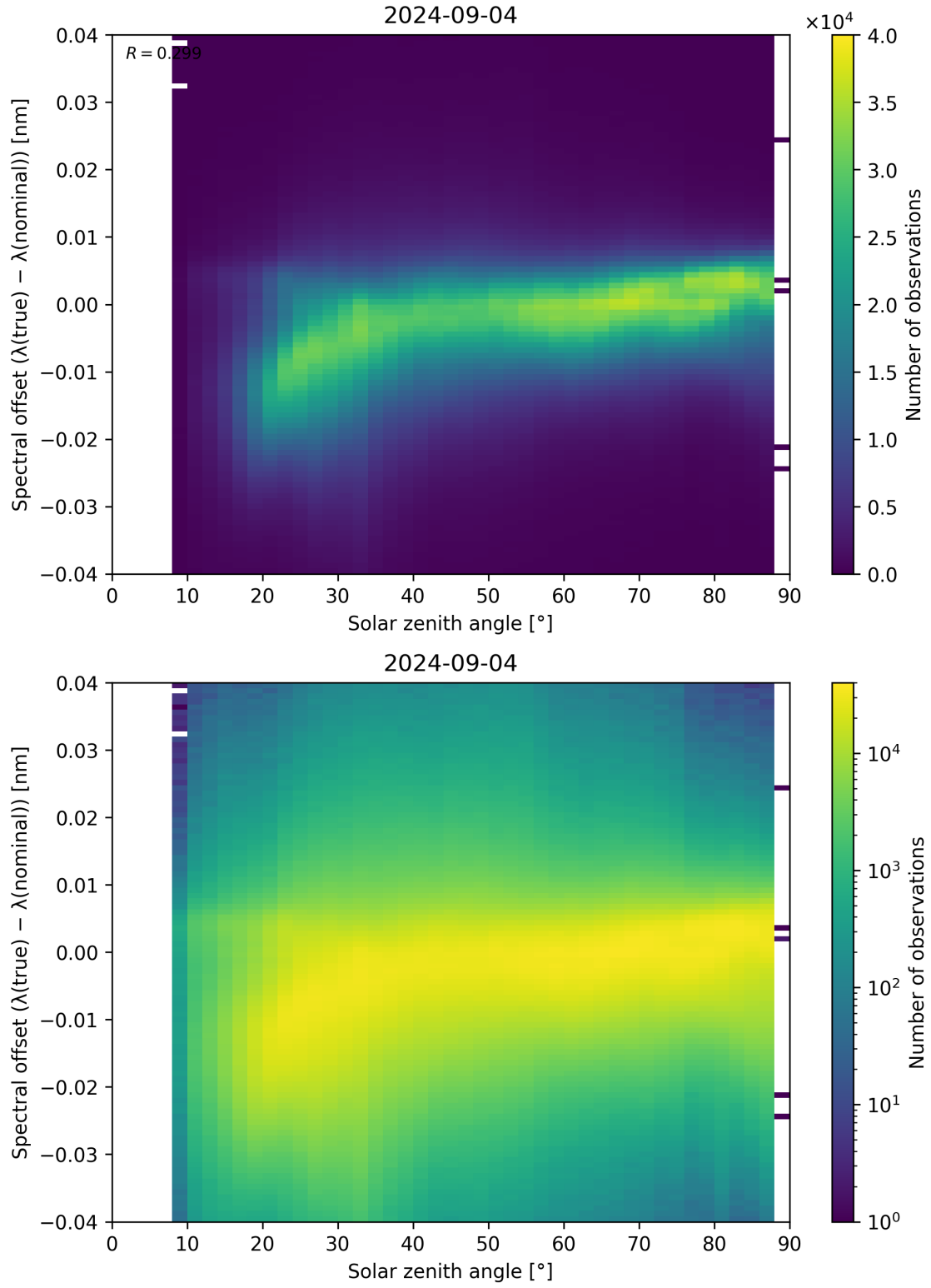
Figure 117: Scatter density plot of “Solar zenith angle” against “Spectral offset ( \lambda_{\text{true}} - \lambda_{\text{nominal}} )” for 2024-09-03 to 2024-09-05.
