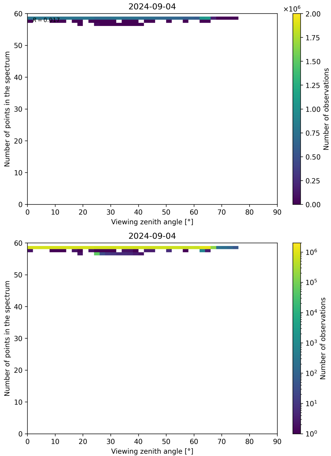
Figure 125: Scatter density plot of “Viewing zenith angle” against “Number of points in the spectrum” for 2024-09-03 to 2024-09-05.
