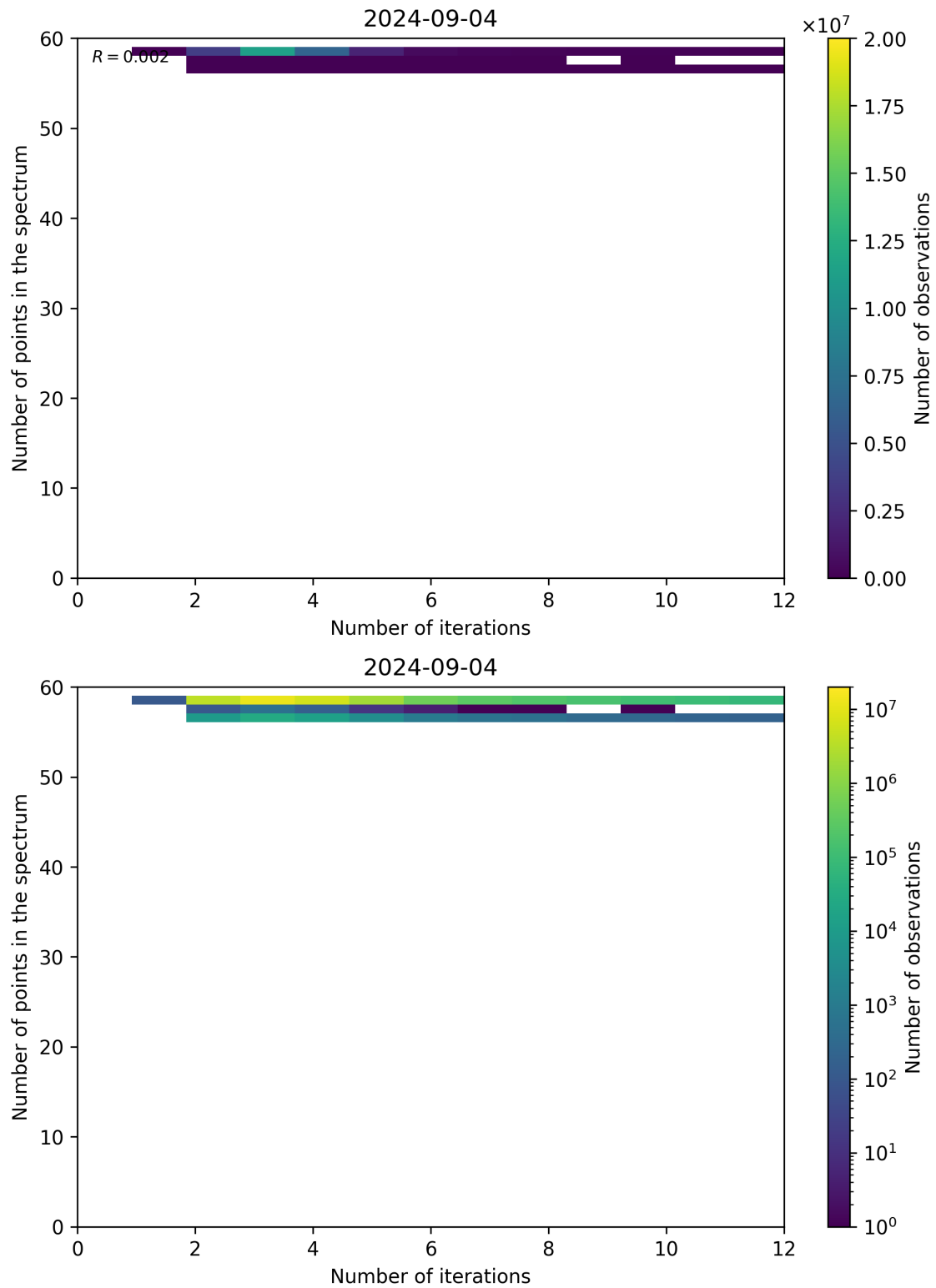
Figure 99: Scatter density plot of “Number of iterations” against “Number of points in the spectrum” for 2024-09-03 to 2024-09-05.
