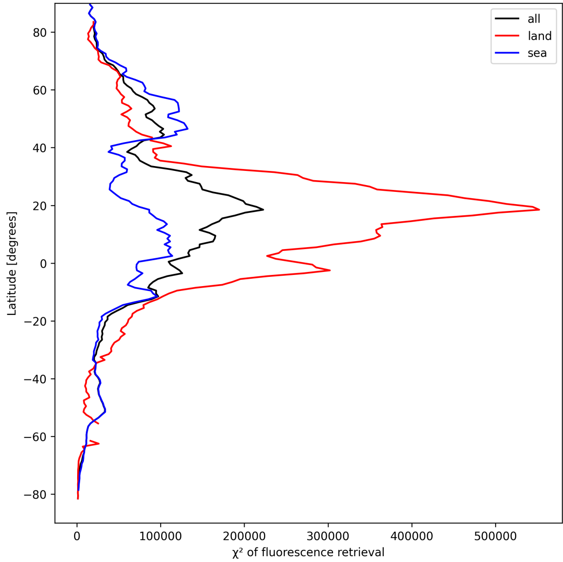
Figure 25: Zonal average of “ \chi^2 of fluorescence retrieval” for 2024-09-03 to 2024-09-05.
