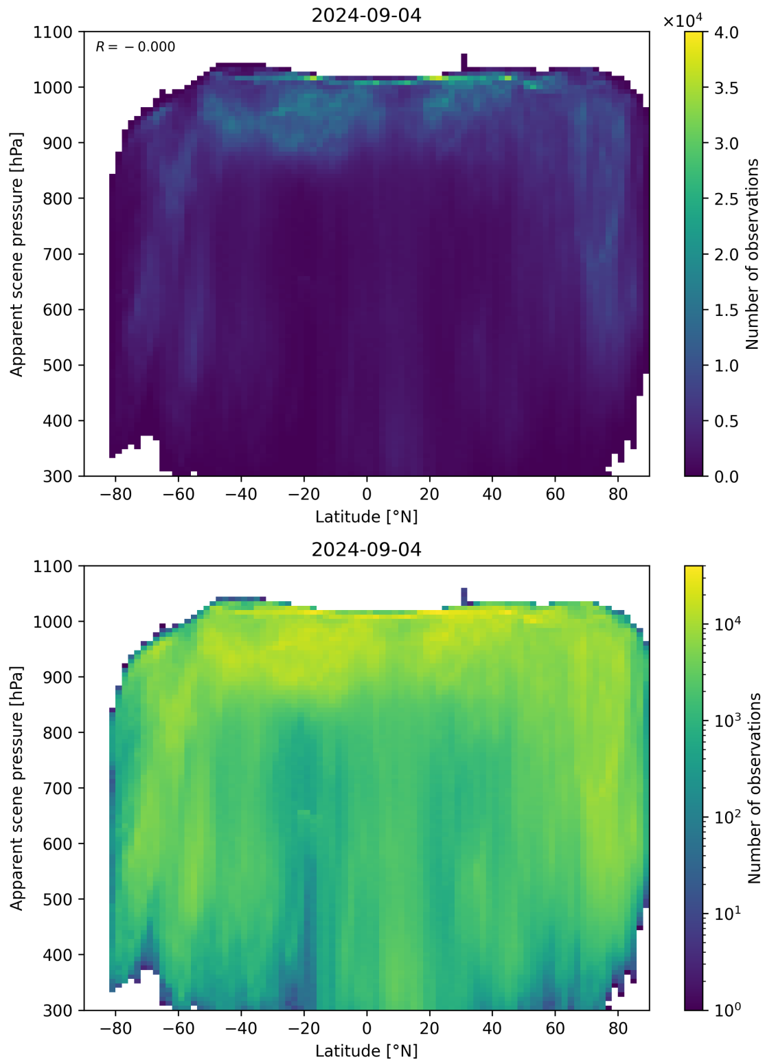
Figure 88: Scatter density plot of “Latitude” against “Apparent scene pressure” for 2024-09-03 to 2024-09-05.
