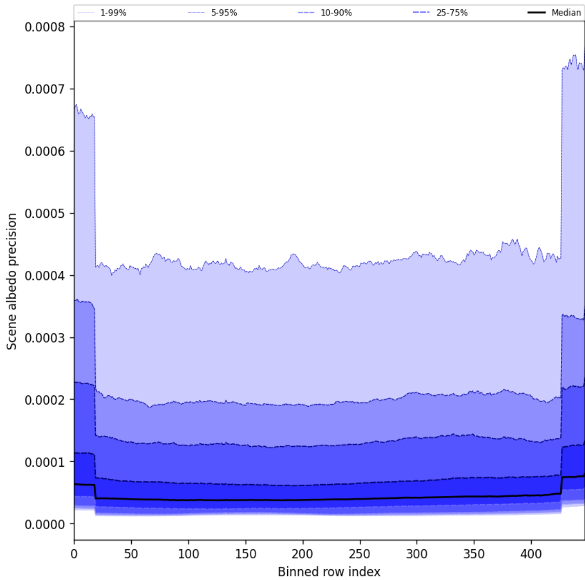
Figure 52: Along track statistics of “Scene albedo precision” for 2024-09-03 to 2024-09-05
