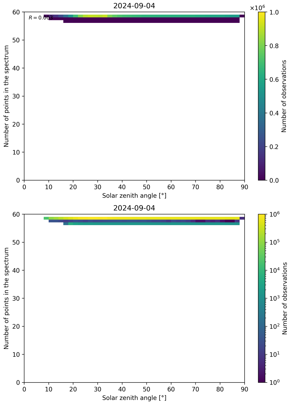
Figure 115: Scatter density plot of “Solar zenith angle” against “Number of points in the spectrum” for 2024-09-03 to 2024-09-05.
