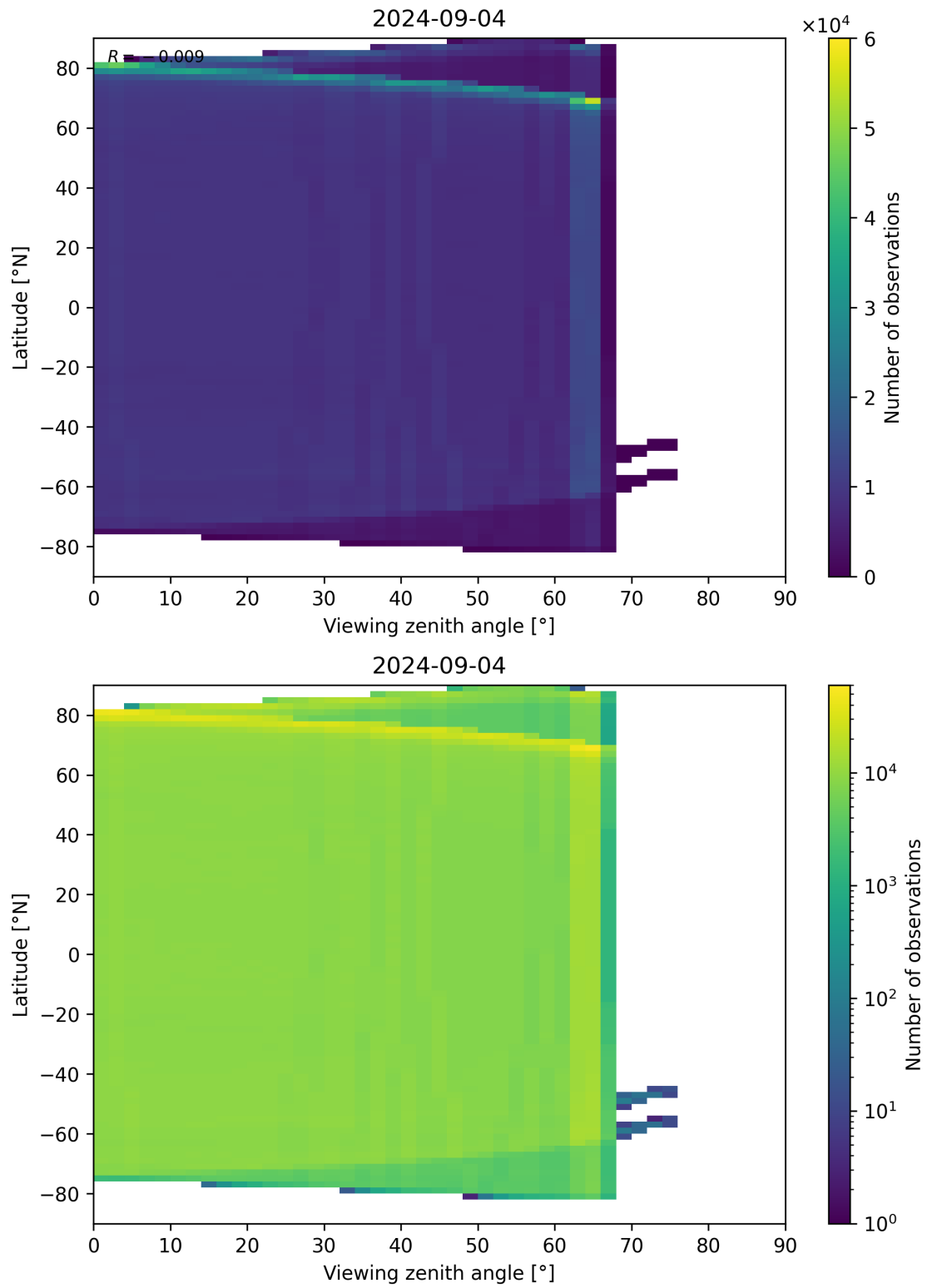
Figure 123: Scatter density plot of “Viewing zenith angle” against “Latitude” for 2024-09-03 to 2024-09-05.
