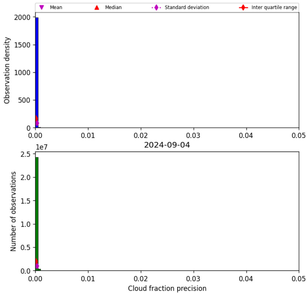
Figure 33: Histogram of “Cloud fraction precision” for 2024-09-03 to 2024-09-05
