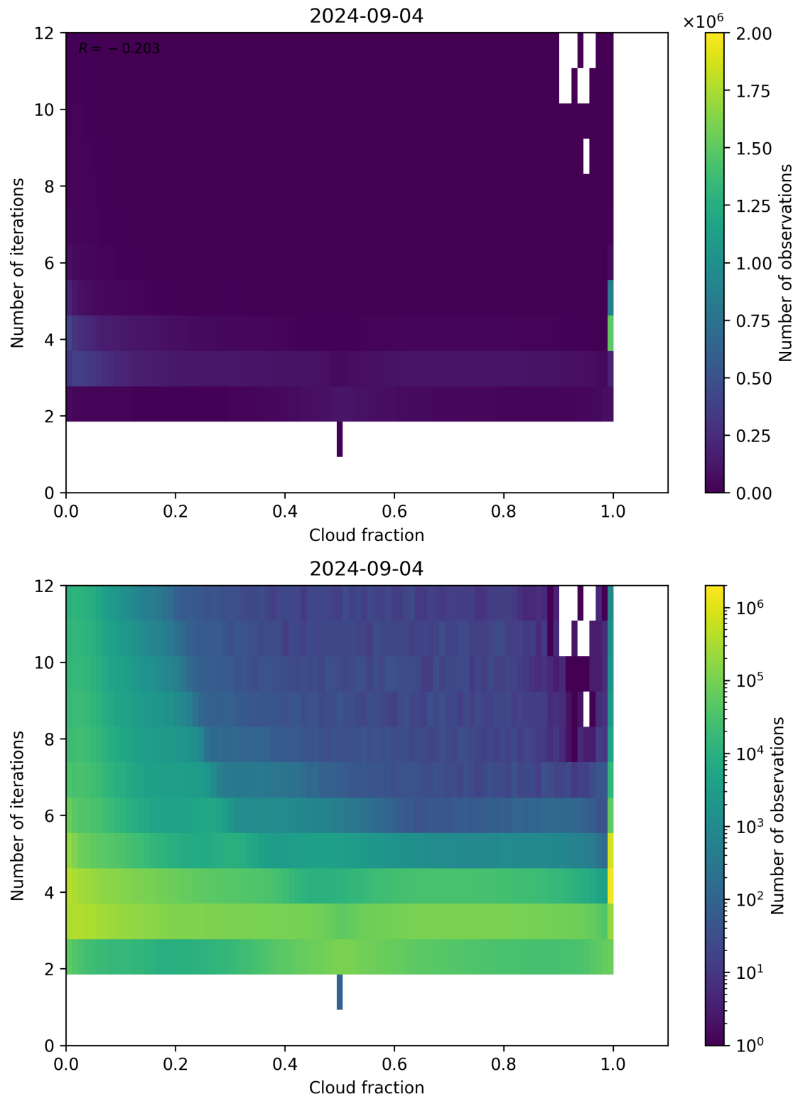
Figure 73: Scatter density plot of “Cloud fraction” against “Number of iterations” for 2024-09-03 to 2024-09-05.
