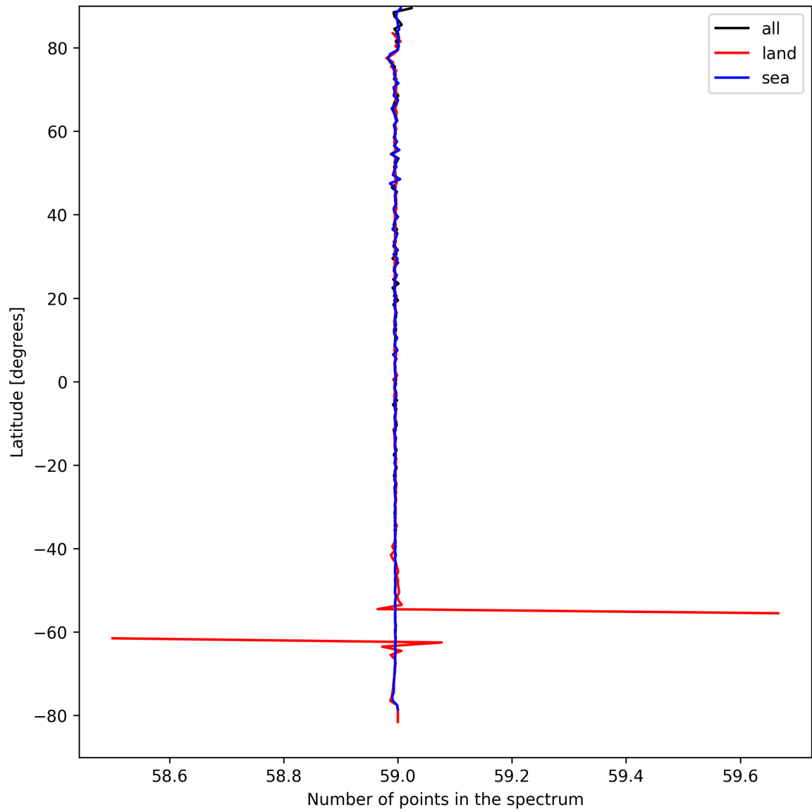
Figure 27: Zonal average of “Number of points in the spectrum” for 2024-09-03 to 2024-09-05.
