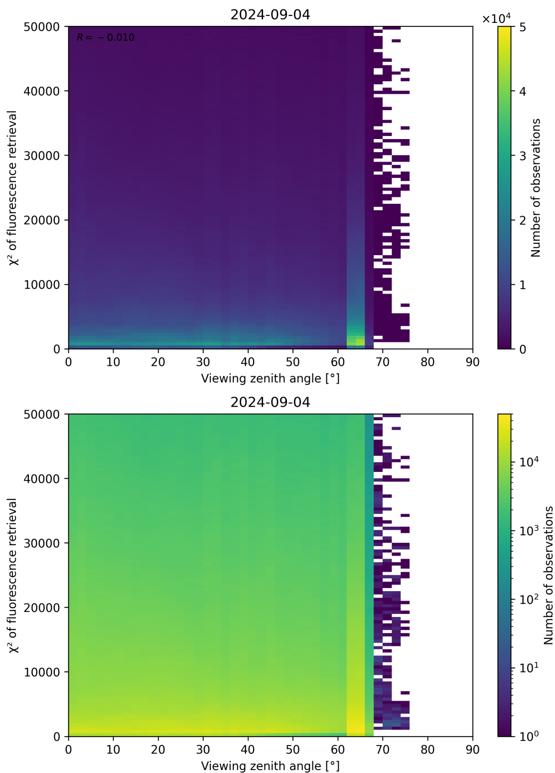
Figure 119: Scatter density plot of “Viewing zenith angle” against “ \chi^2 of fluorescence retrieval” for 2024-09-03 to 2024-09-05.
