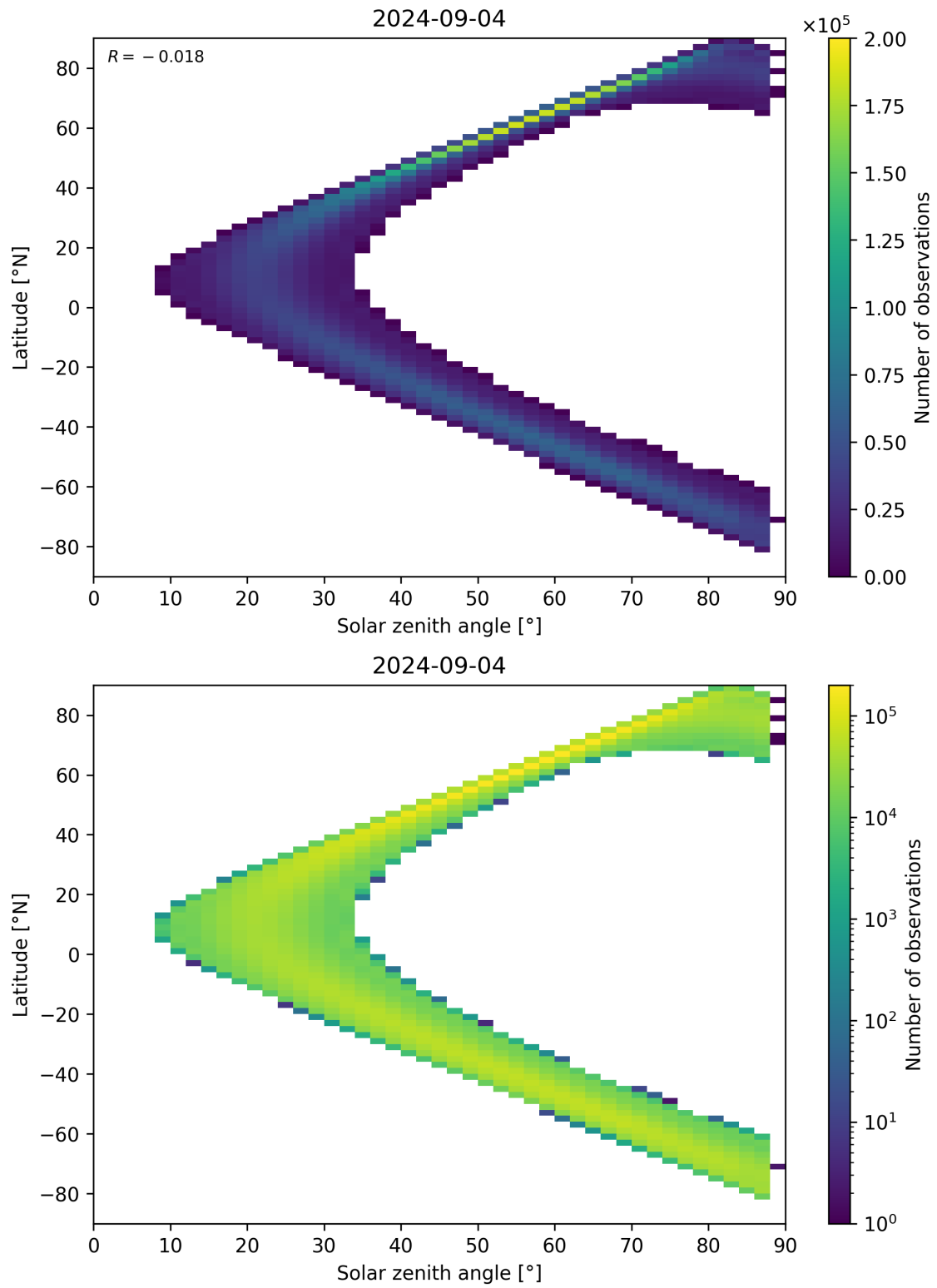
Figure 113: Scatter density plot of “Solar zenith angle” against “Latitude” for 2024-09-03 to 2024-09-05.
