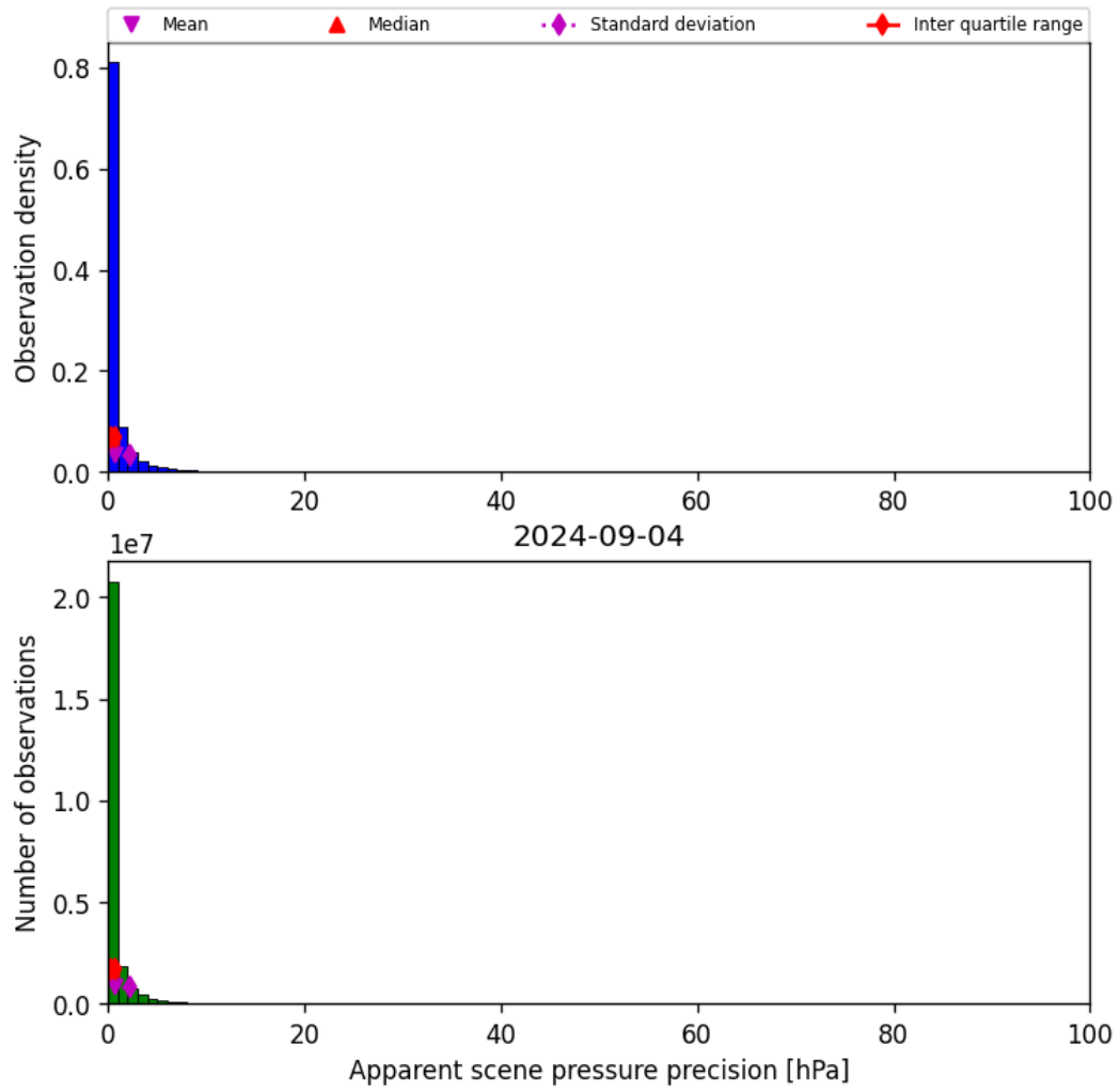
Figure 37: Histogram of “Apparent scene pressure precision” for 2024-09-03 to 2024-09-05
