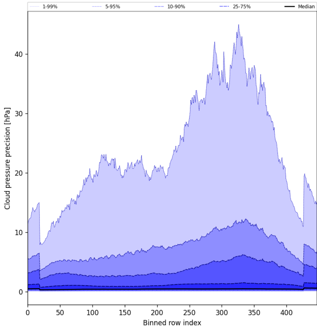
Figure 48: Along track statistics of “Cloud pressure precision” for 2024-09-03 to 2024-09-05
