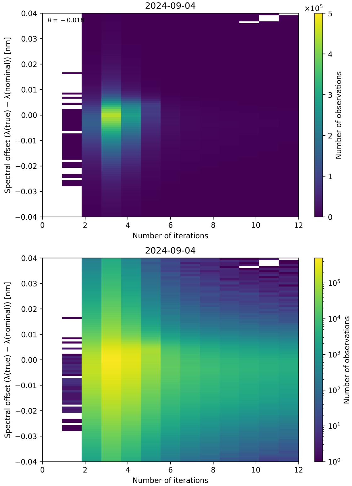
Figure 100: Scatter density plot of “Number of iterations” against “Spectral offset ( \lambda_{\text{true}} - \lambda_{\text{nominal}} )” for 2024-09-03 to 2024-09-05.
