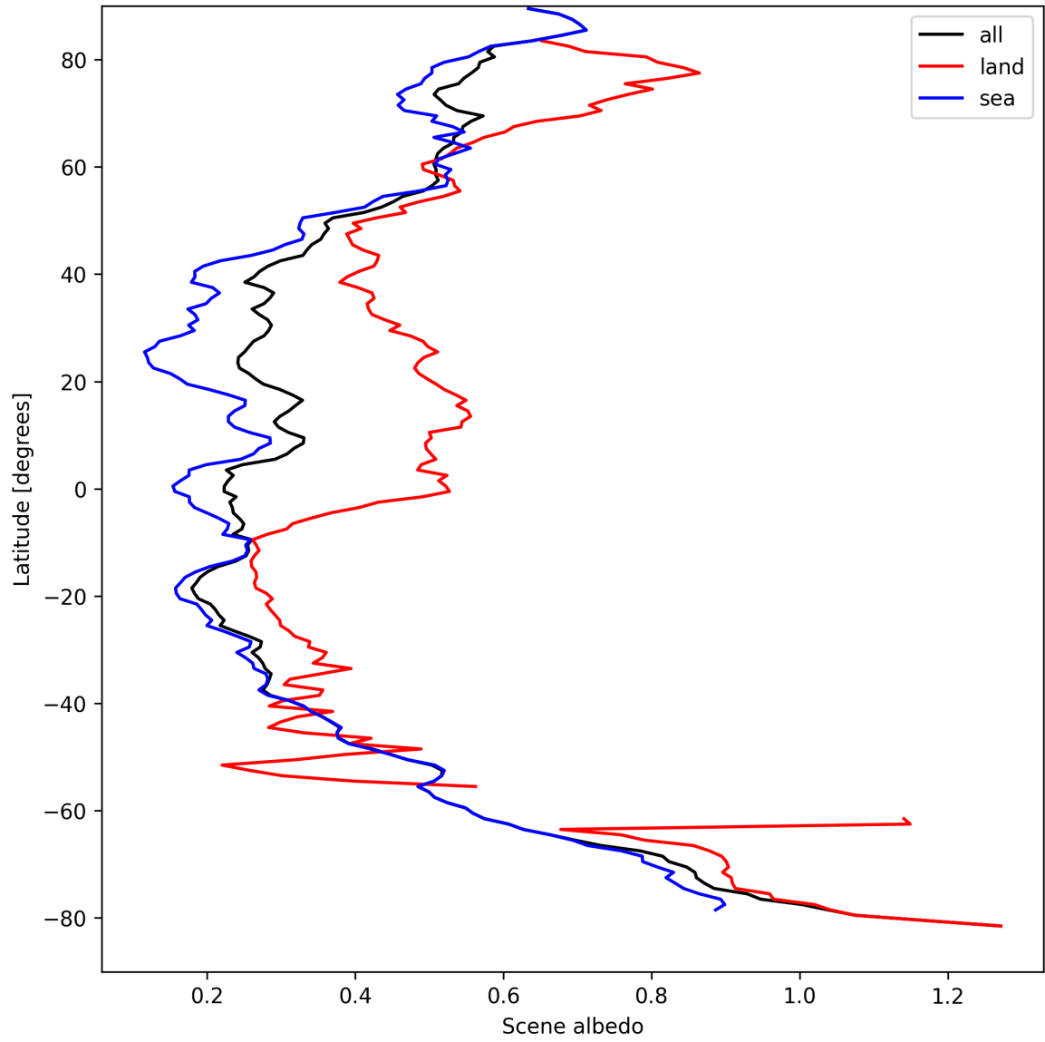
Figure 17: Zonal average of “Scene albedo” for 2024-09-03 to 2024-09-05.
