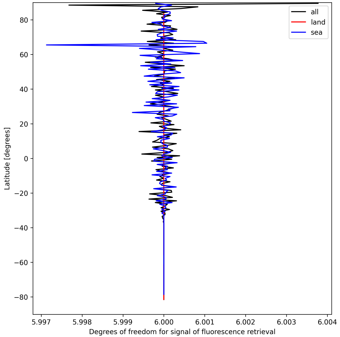
Figure 26: Zonal average of “Degrees of freedom for signal of fluorescence retrieval” for 2024-09-03 to 2024-09-05.
