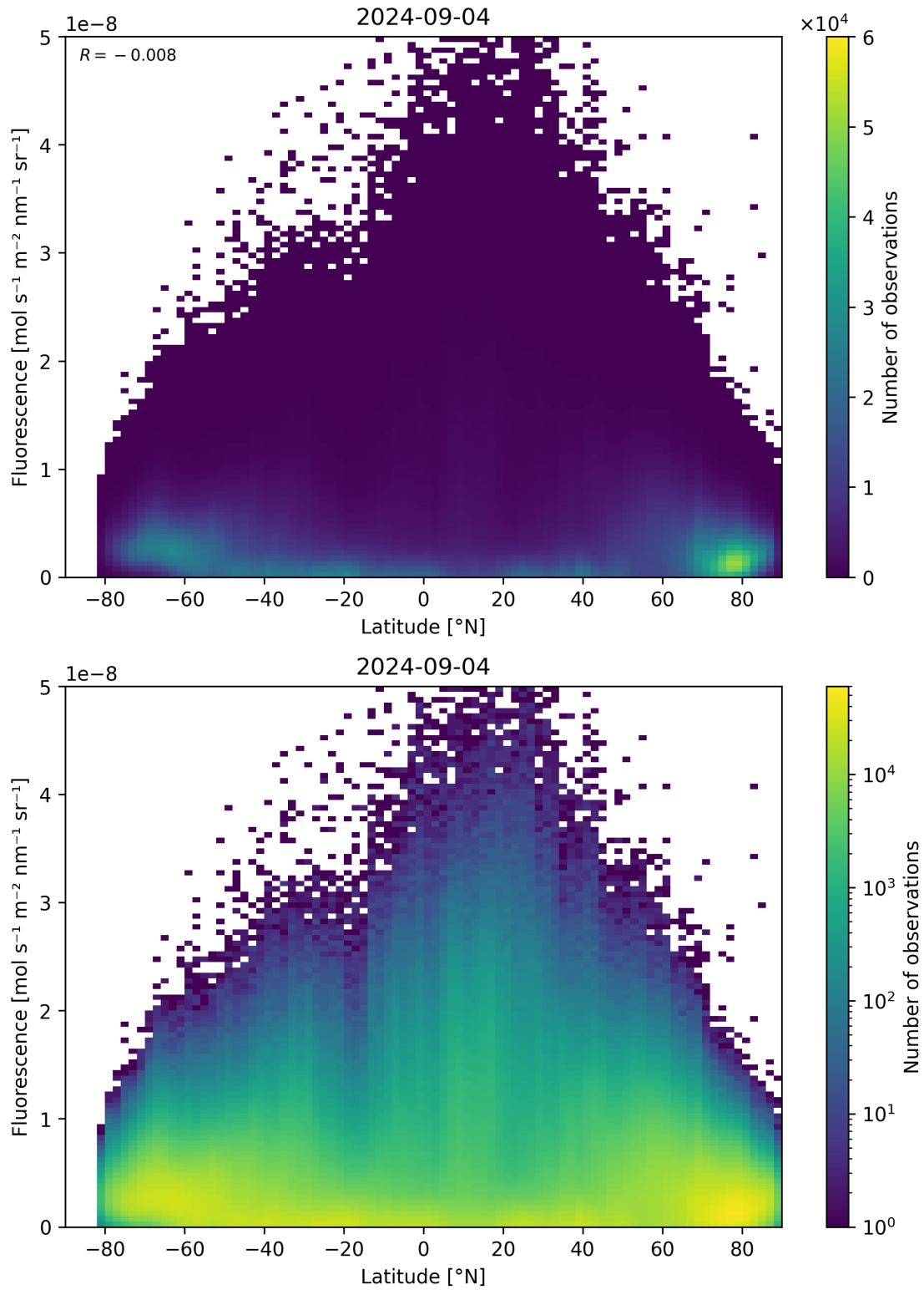
Figure 92: Scatter density plot of “Latitude” against “Fluorescence” for 2024-09-03 to 2024-09-05.
