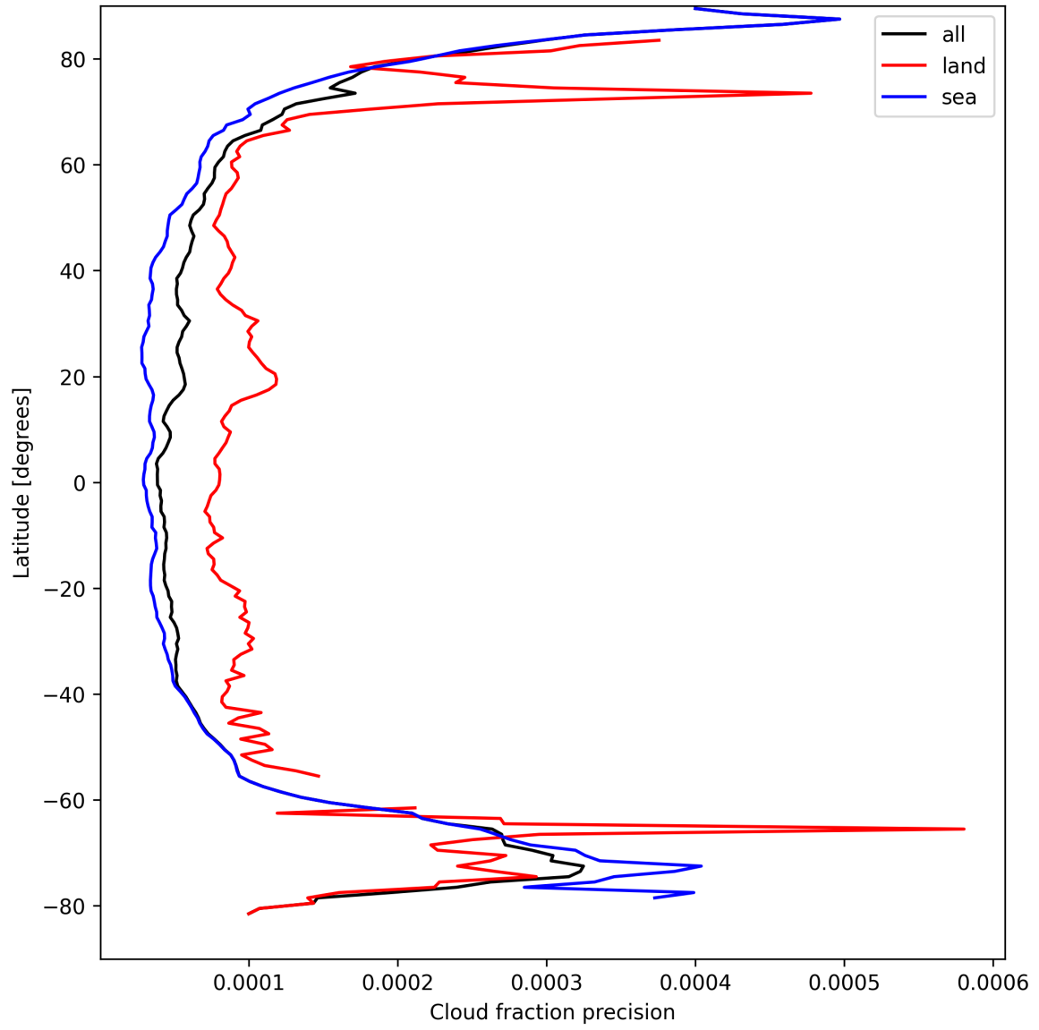
Figure 16: Zonal average of “Cloud fraction precision” for 2024-09-03 to 2024-09-05.
