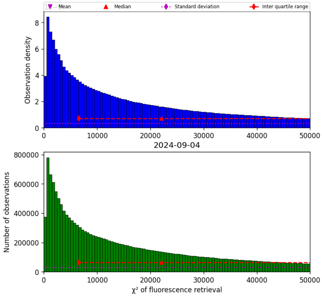
Figure 42: Histogram of “ \chi^2 of fluorescence retrieval” for 2024-09-03 to 2024-09-05
