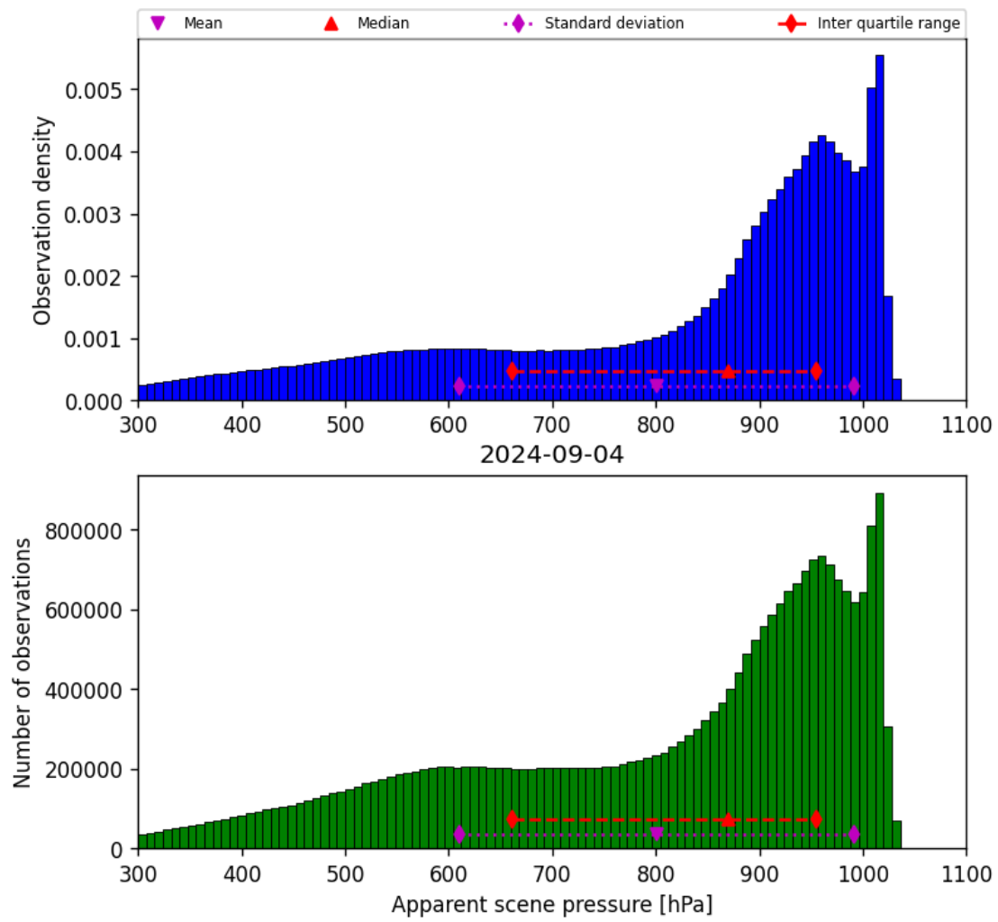
Figure 36: Histogram of “Apparent scene pressure” for 2024-09-03 to 2024-09-05
