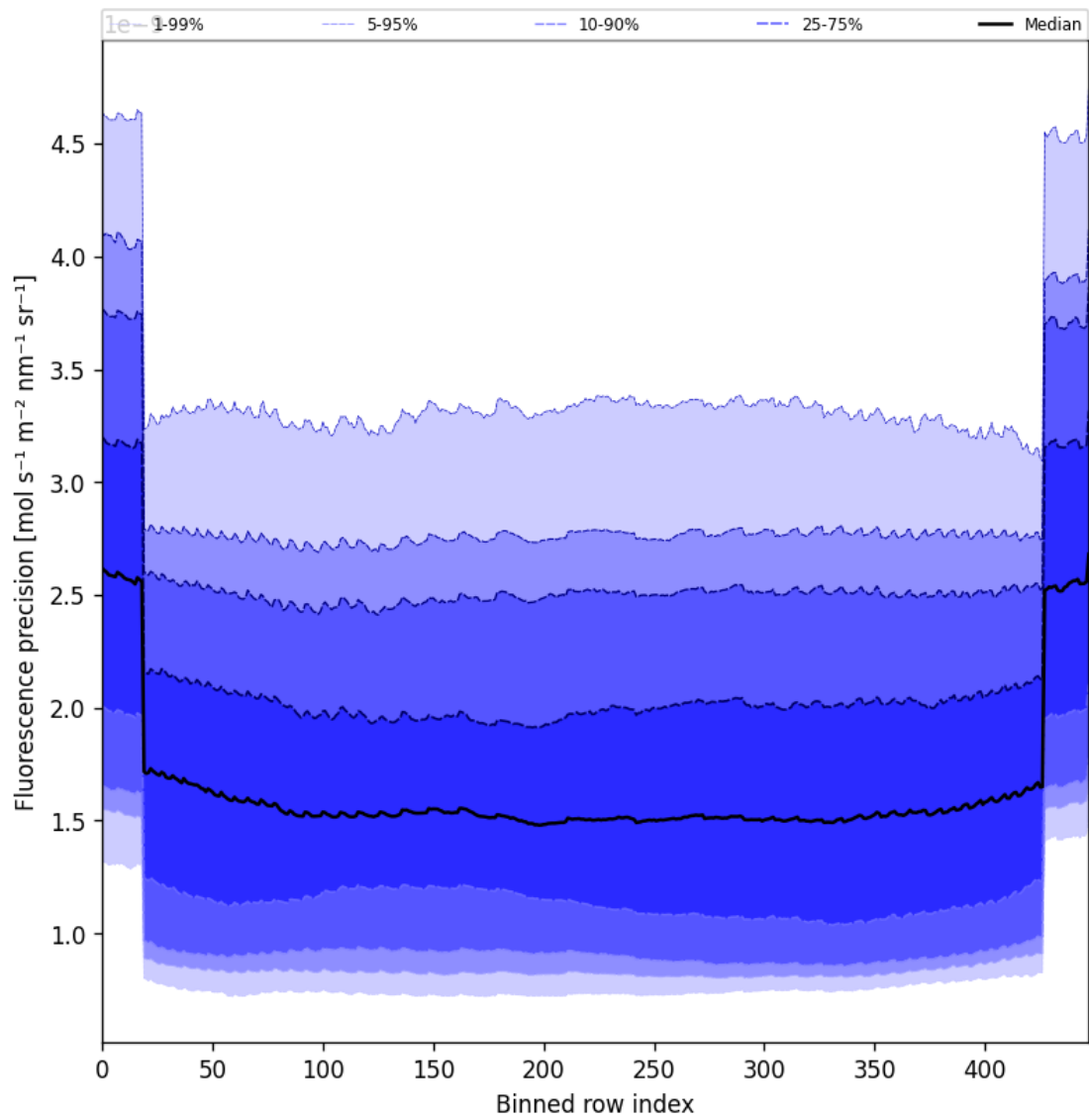
Figure 58: Along track statistics of “Fluorescence precision” for 2024-09-03 to 2024-09-05
