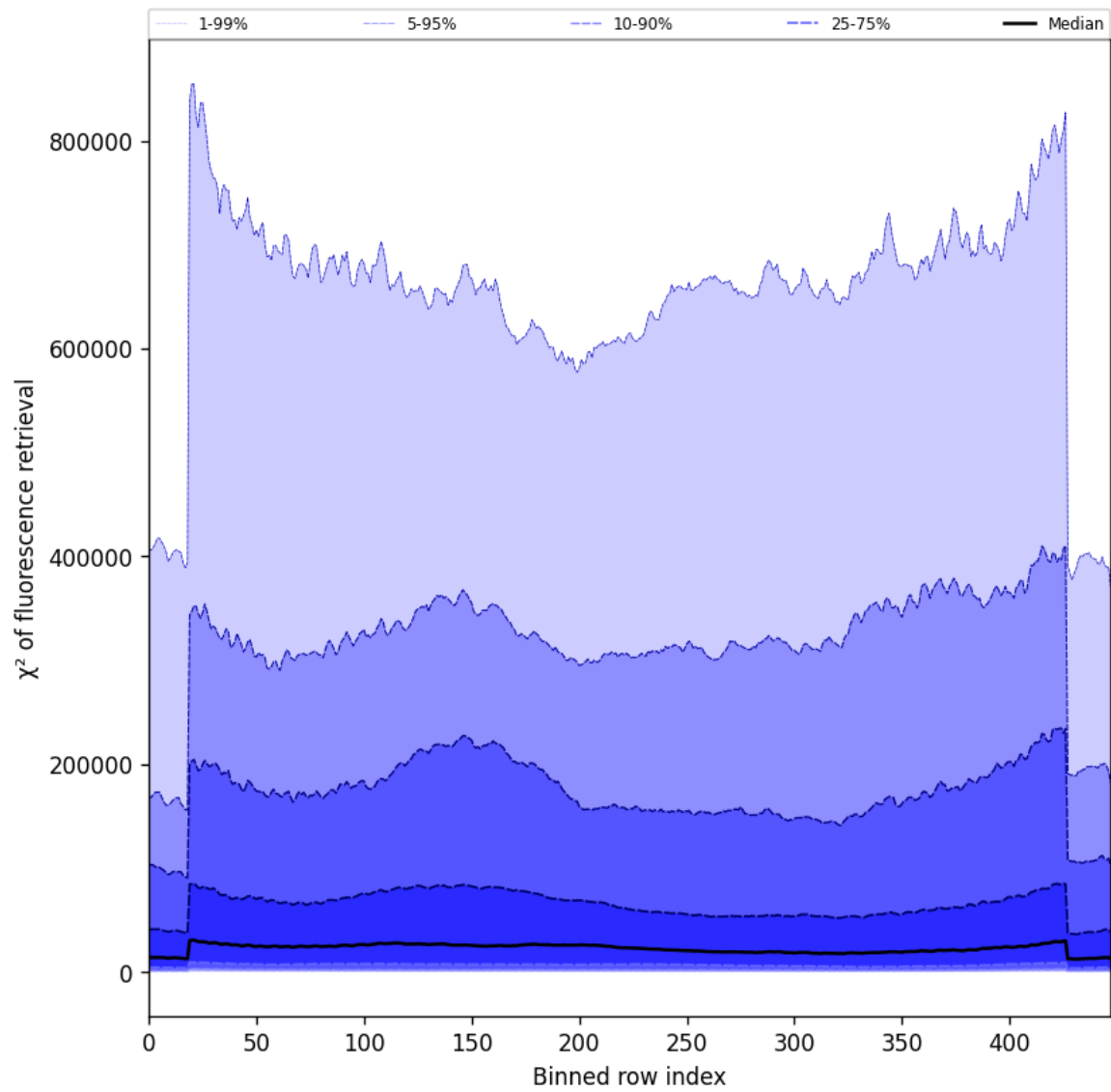
Figure 59: Along track statistics of “ \chi^2 of fluorescence retrieval” for 2024-09-03 to 2024-09-05
