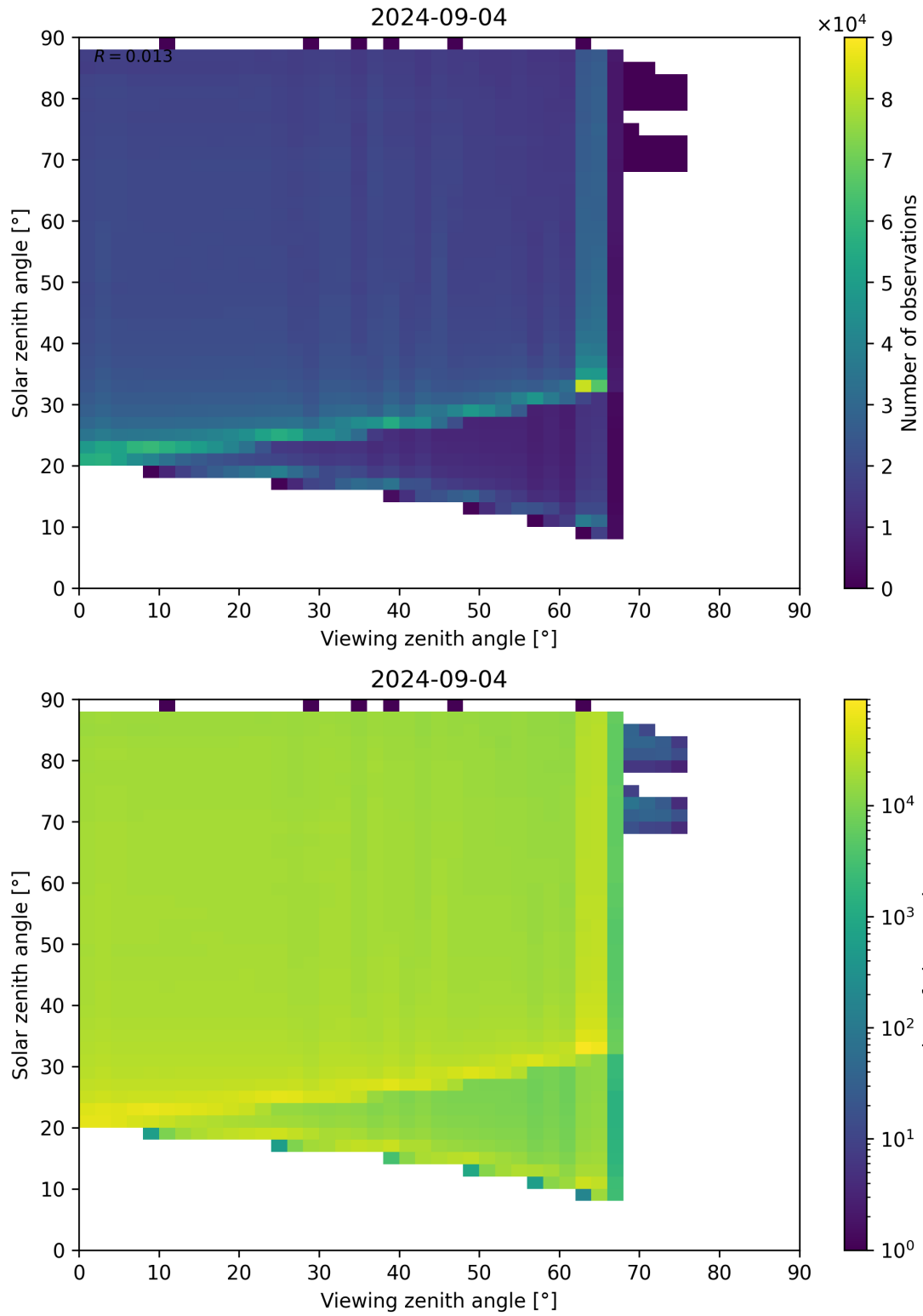
Figure 127: Scatter density plot of “Viewing zenith angle” against “Solar zenith angle” for 2024-09-03 to 2024-09-05.
