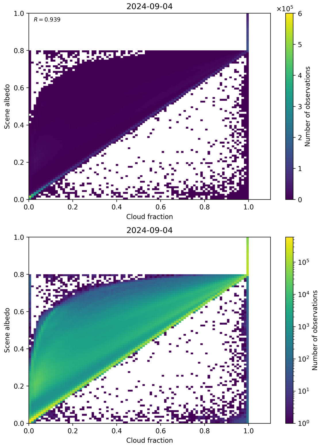
Figure 75: Scatter density plot of “Cloud fraction” against “Scene albedo” for 2024-09-03 to 2024-09-05.
