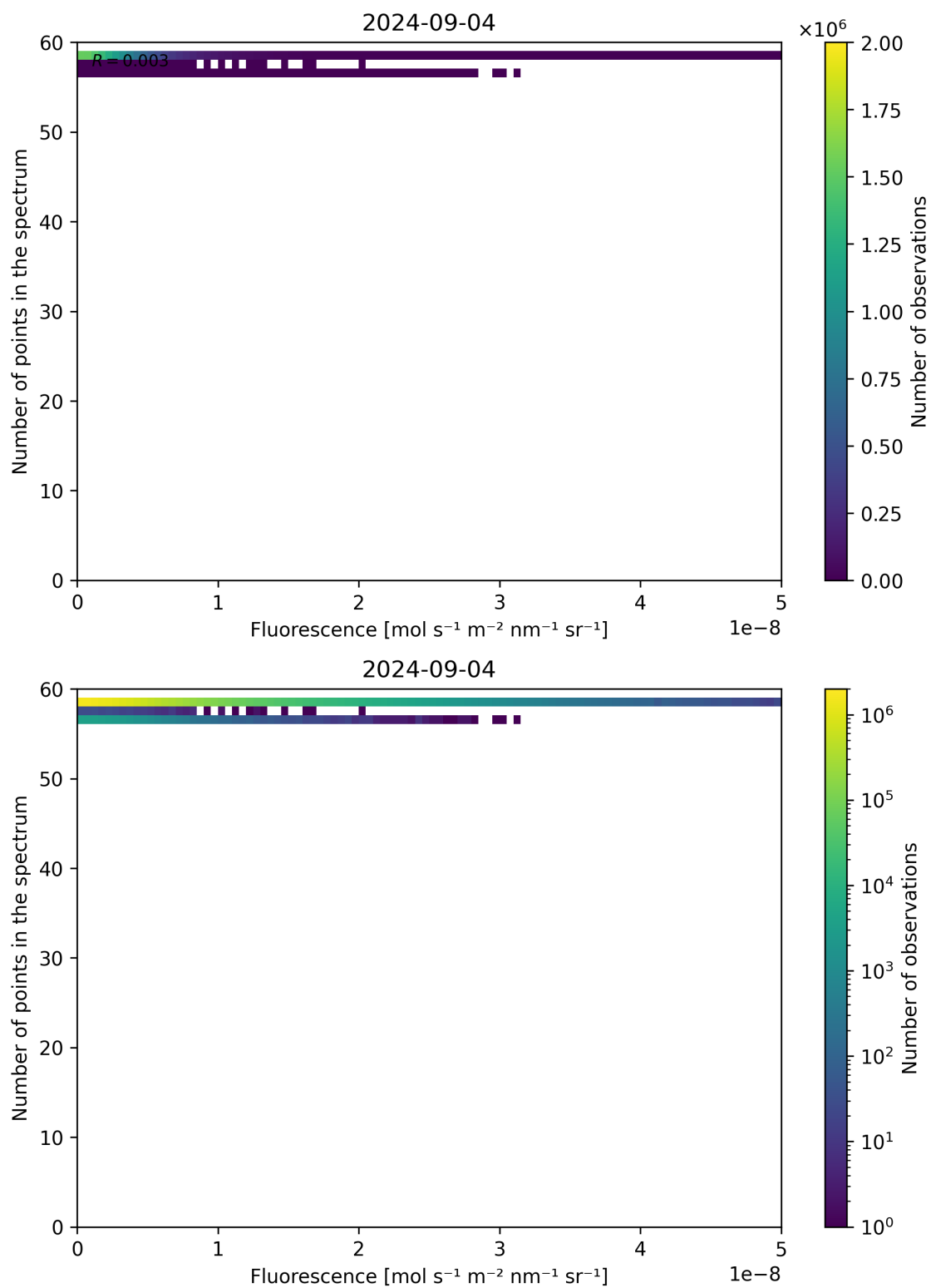
Figure 86: Scatter density plot of “Fluorescence” against “Number of points in the spectrum” for 2024-09-03 to 2024-09-05.
