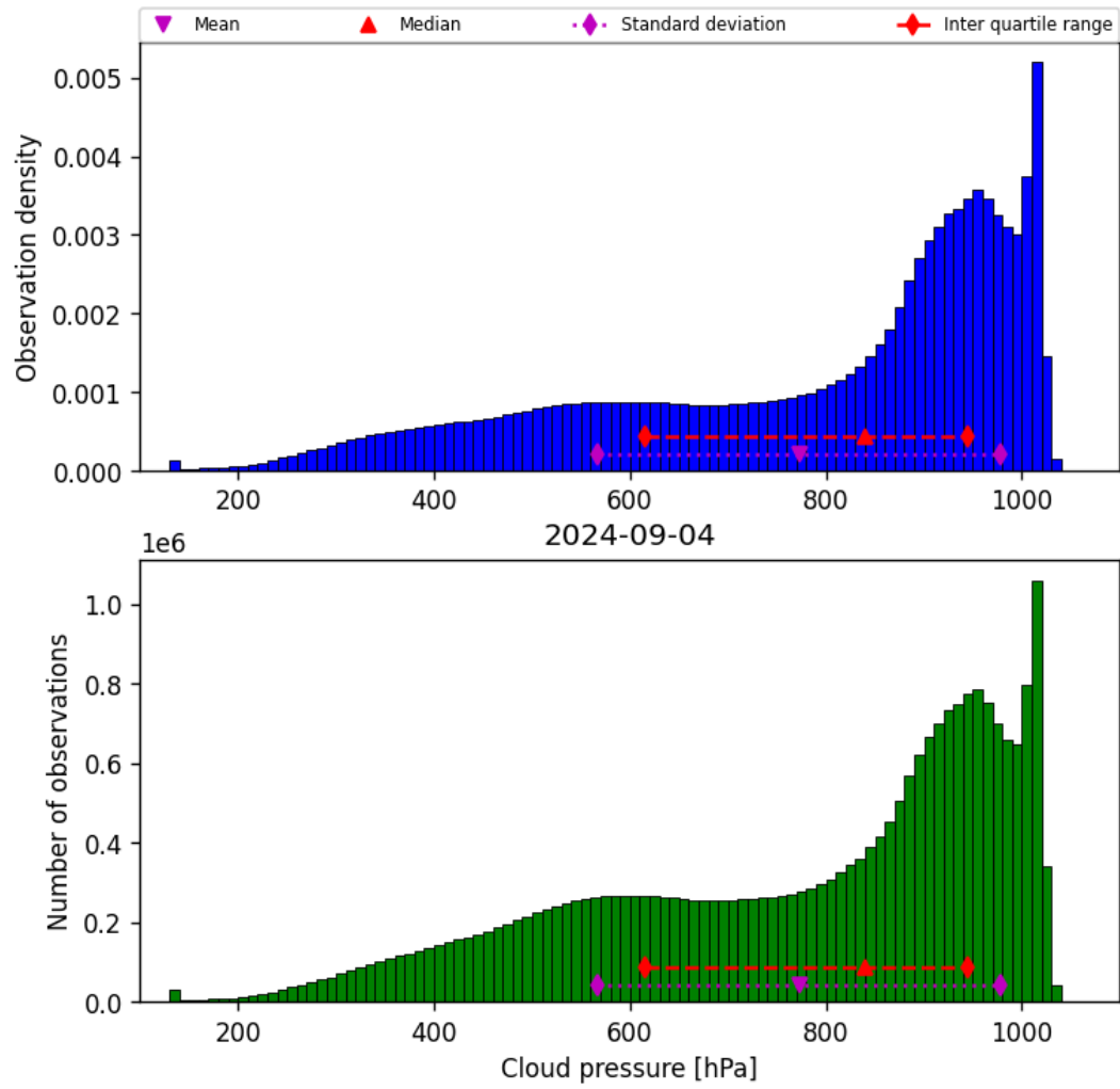
Figure 30: Histogram of “Cloud pressure” for 2024-09-03 to 2024-09-05
