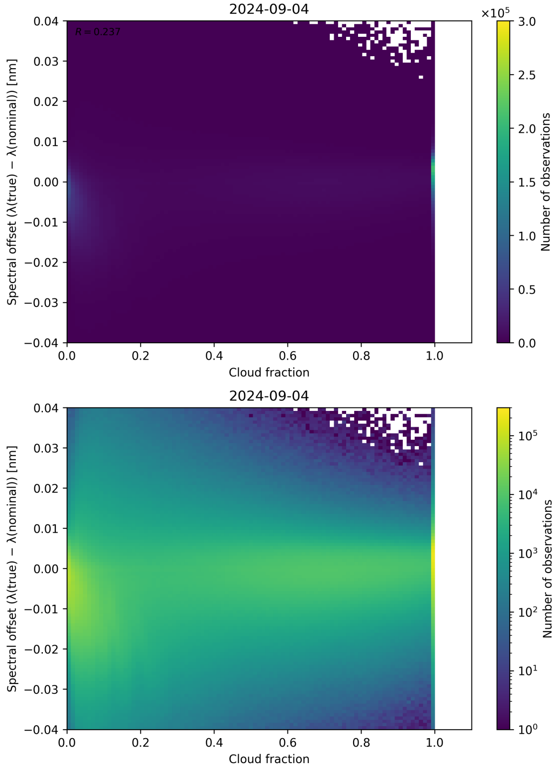
Figure 76: Scatter density plot of “Cloud fraction” against “Spectral offset ( \lambda_{\text{true}} - \lambda_{\text{nominal}} )” for 2024-09-03 to 2024-09-05.
