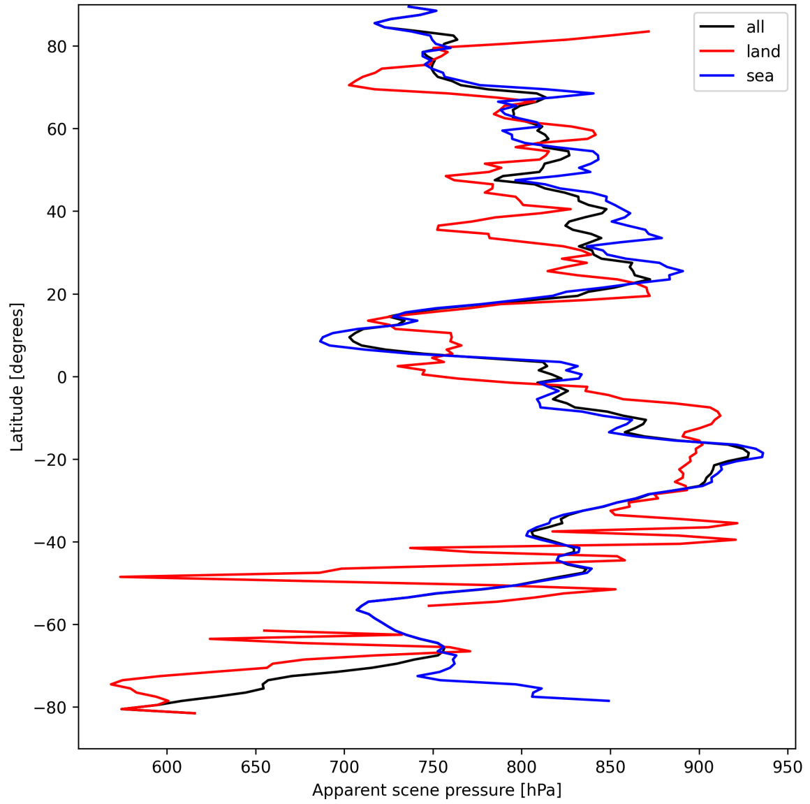
Figure 19: Zonal average of “Apparent scene pressure” for 2024-09-03 to 2024-09-05.
