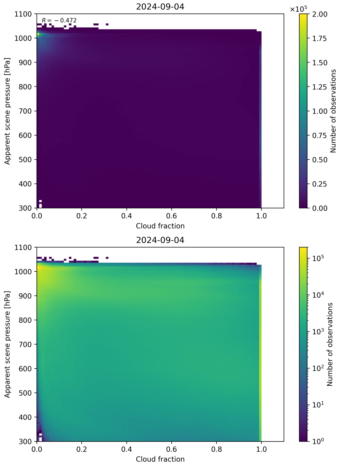
Figure 70: Scatter density plot of “Cloud fraction” against “Apparent scene pressure” for 2024-09-03 to 2024-09-05.
