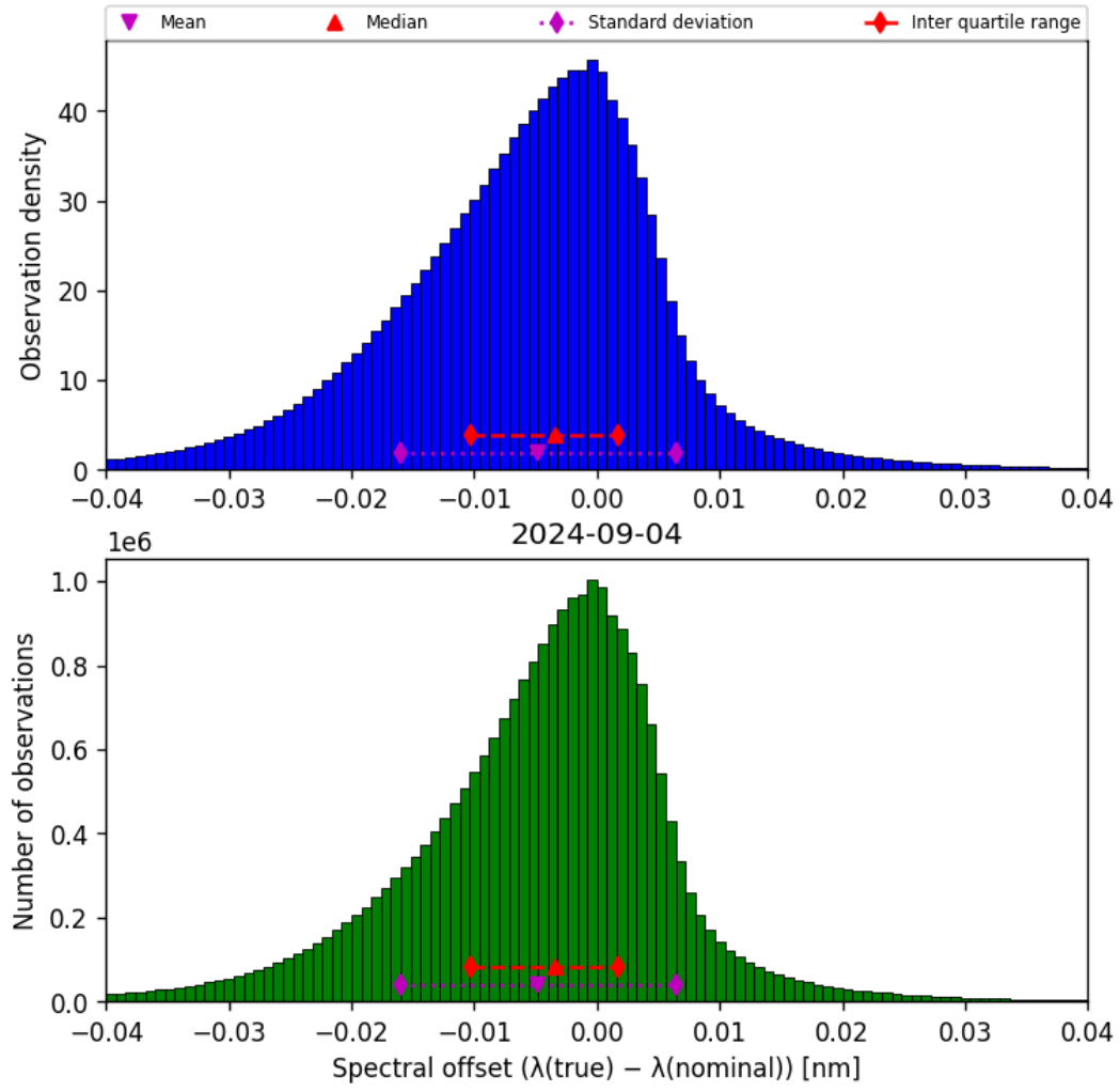
Figure 45: Histogram of “Spectral offset ( \lambda_{\text{true}} - \lambda_{\text{nominal}} )” for 2024-09-03 to 2024-09-05
