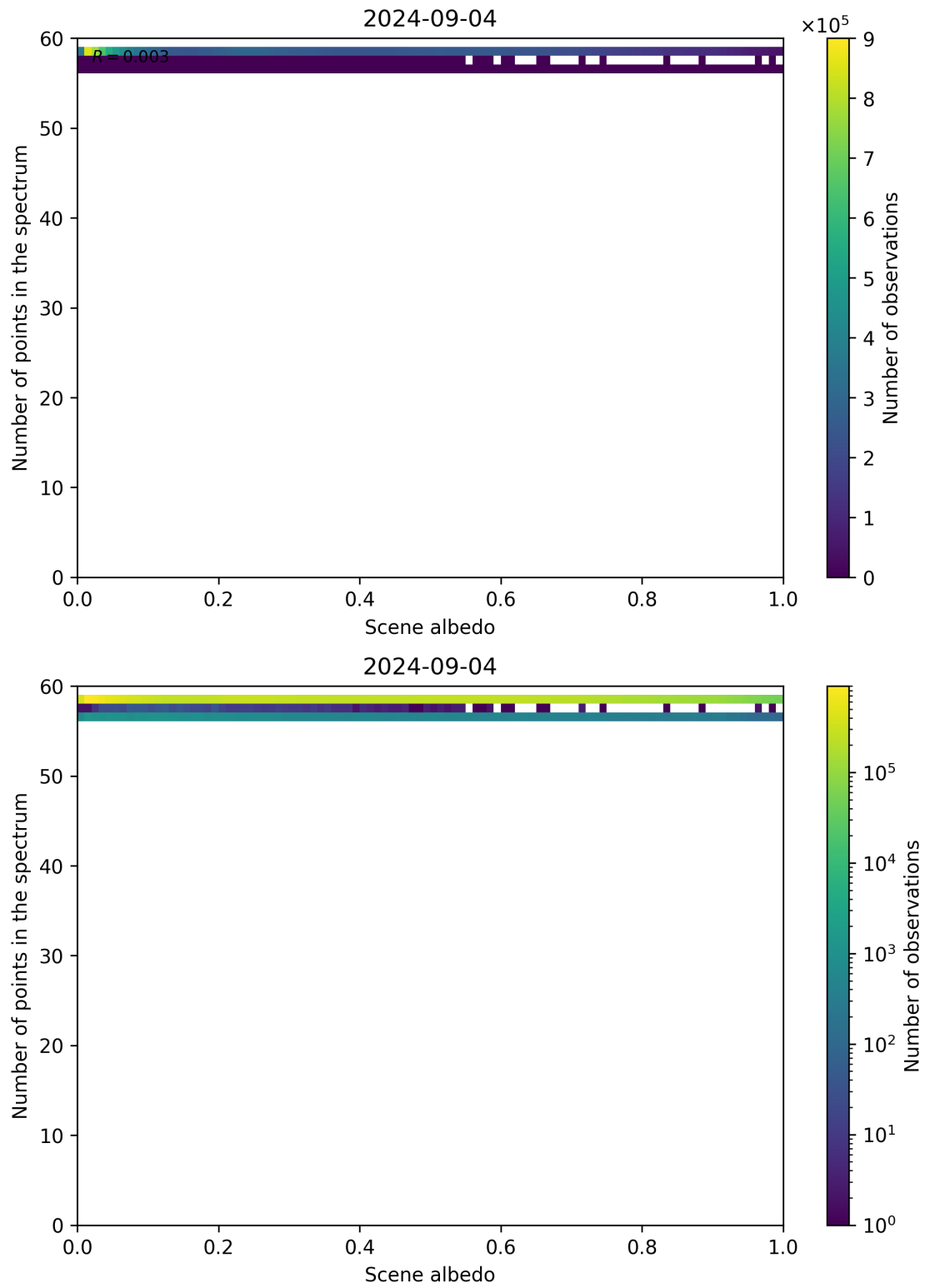
Figure 106: Scatter density plot of “Scene albedo” against “Number of points in the spectrum” for 2024-09-03 to 2024-09-05.
