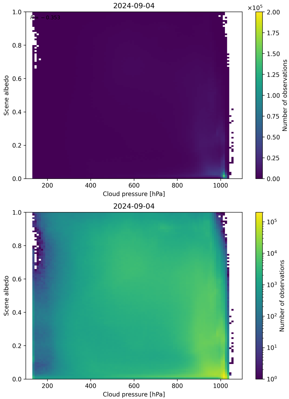
Figure 83: Scatter density plot of “Cloud pressure” against “Scene albedo” for 2024-09-03 to 2024-09-05.
