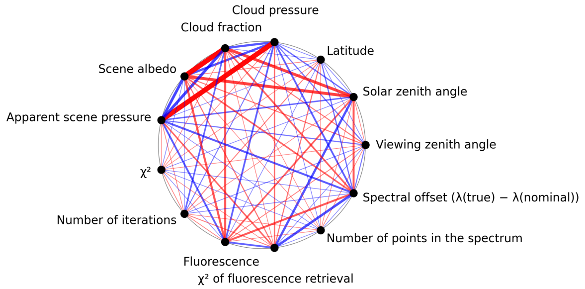
Figure 1: Map of correlation graph for 2024-09-03 to 2024-09-05.
