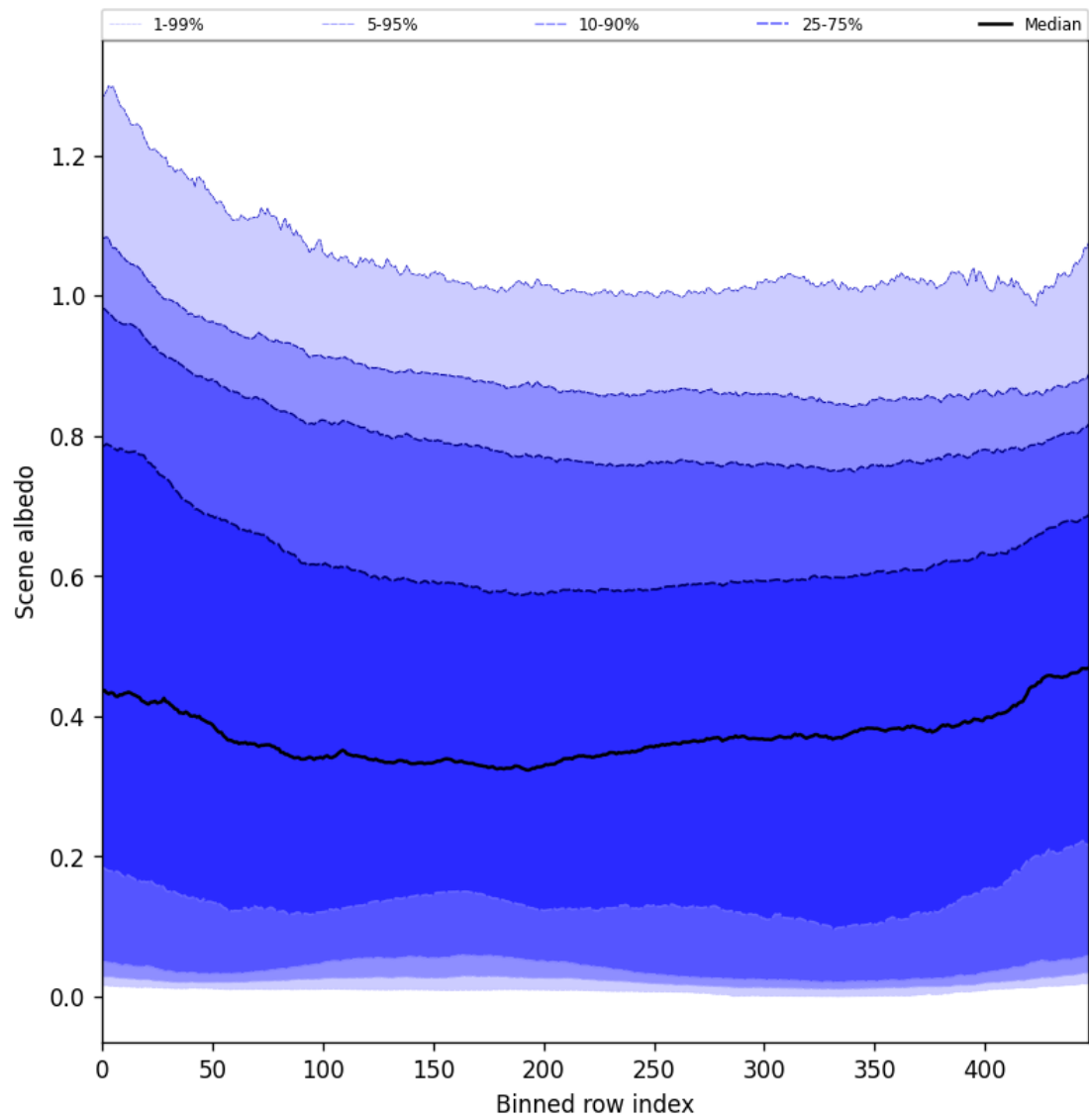
Figure 51: Along track statistics of “Scene albedo” for 2024-09-03 to 2024-09-05
