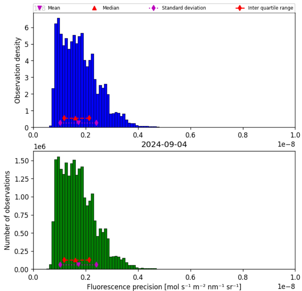
Figure 41: Histogram of “Fluorescence precision” for 2024-09-03 to 2024-09-05
