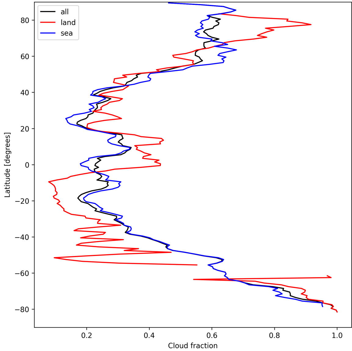
Figure 15: Zonal average of “Cloud fraction” for 2024-09-03 to 2024-09-05.
