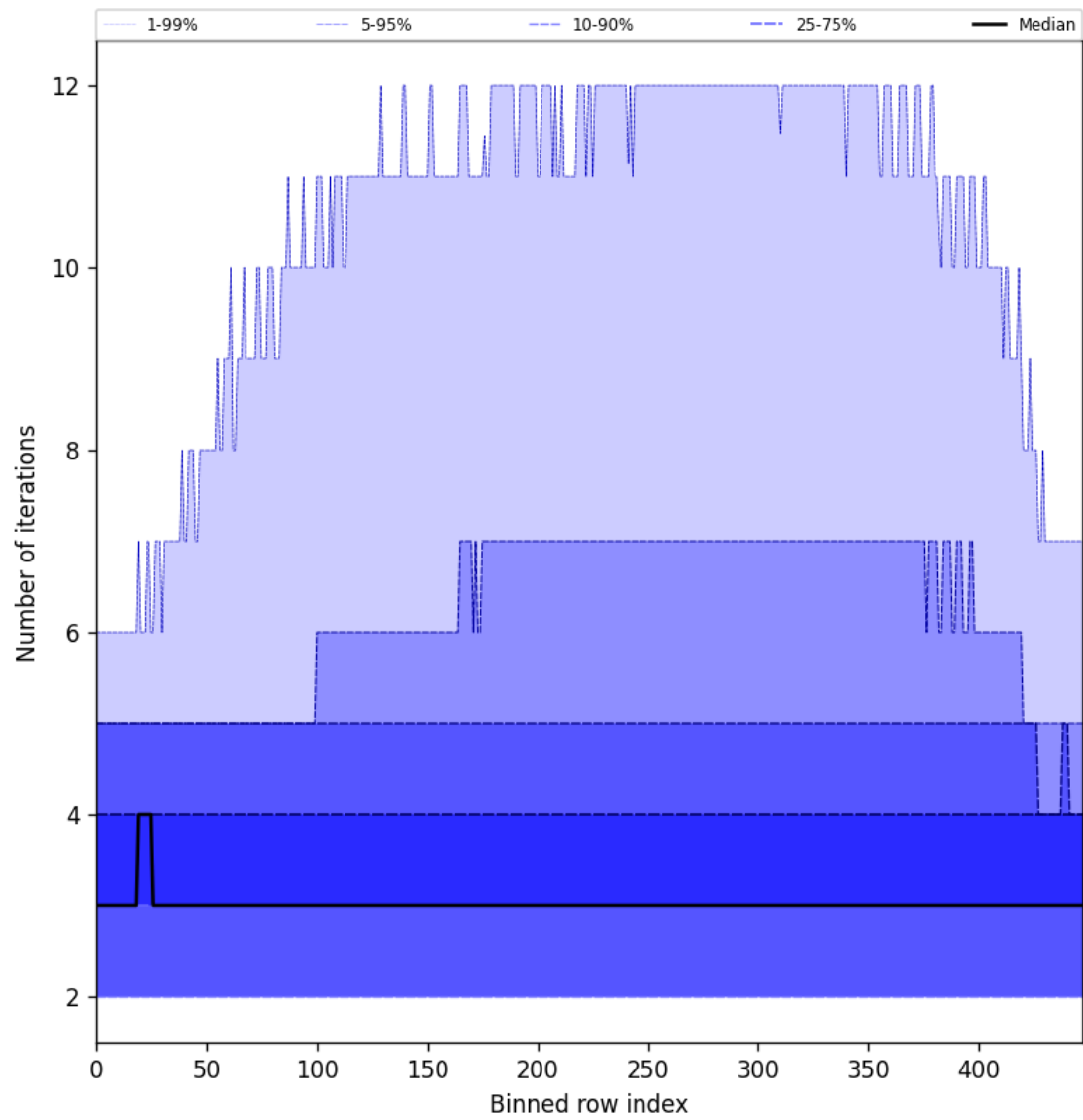
Figure 56: Along track statistics of “Number of iterations” for 2024-09-03 to 2024-09-05
