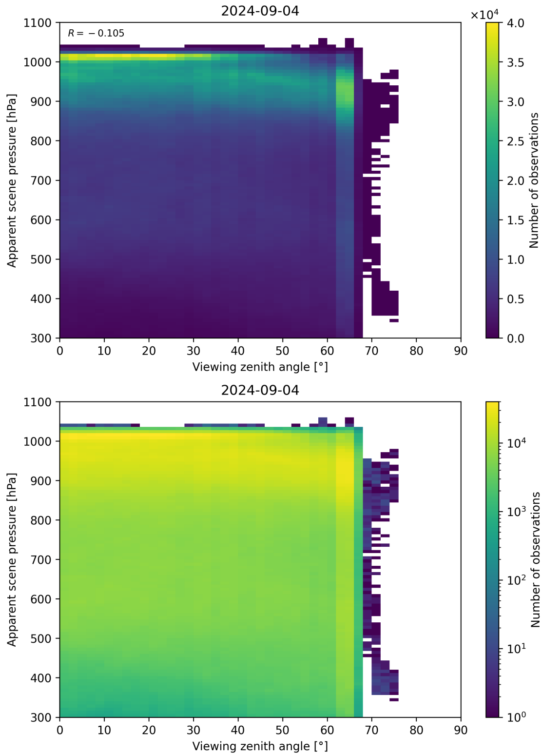
Figure 118: Scatter density plot of “Viewing zenith angle” against “Apparent scene pressure” for 2024-09-03 to 2024-09-05.
