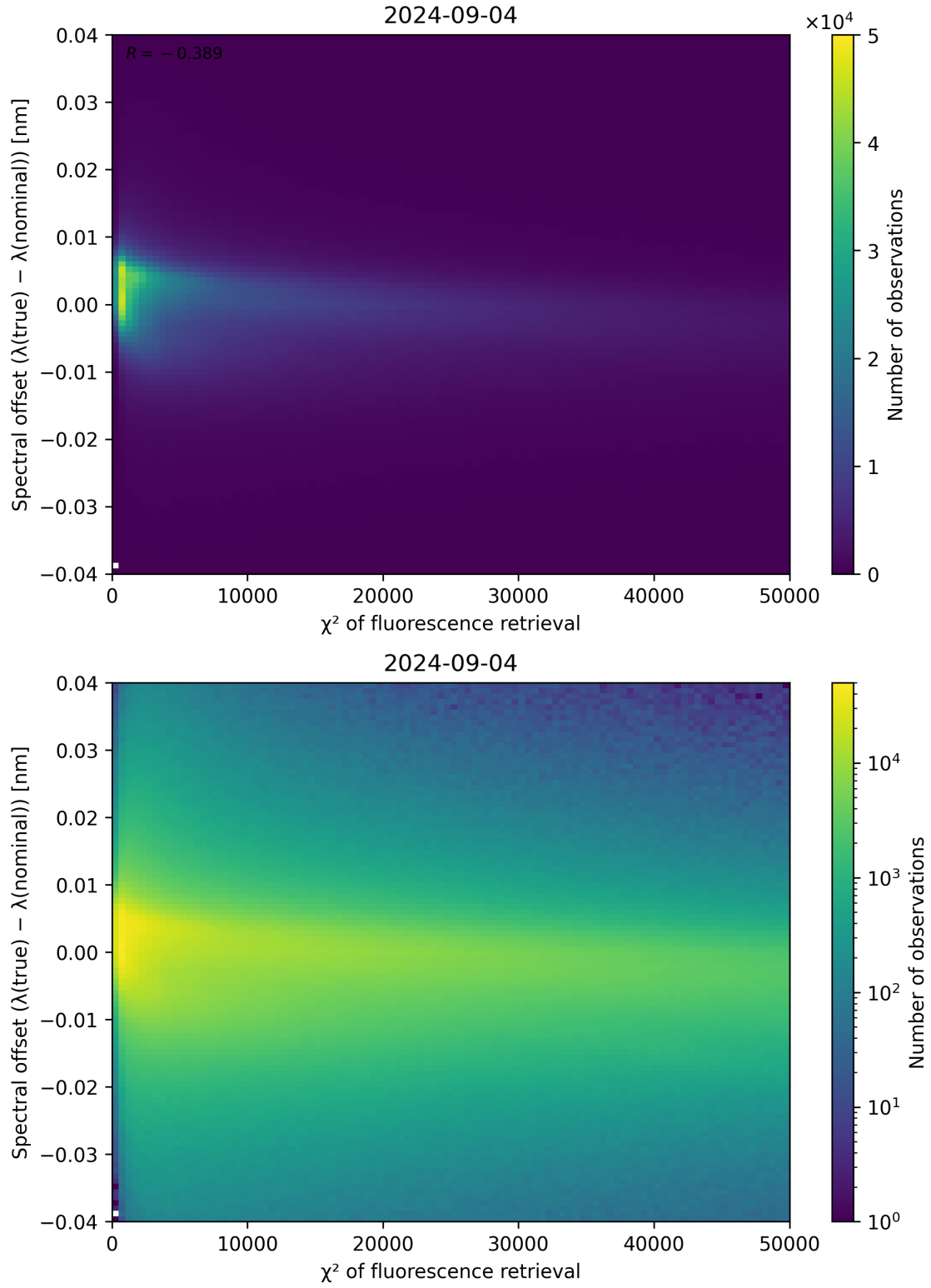
Figure 69: Scatter density plot of “ \chi^2 of fluorescence retrieval” against “Spectral offset ( \lambda_{\text{true}} - \lambda_{\text{nominal}} )” for 2024-09-03 to 2024-09-05.
