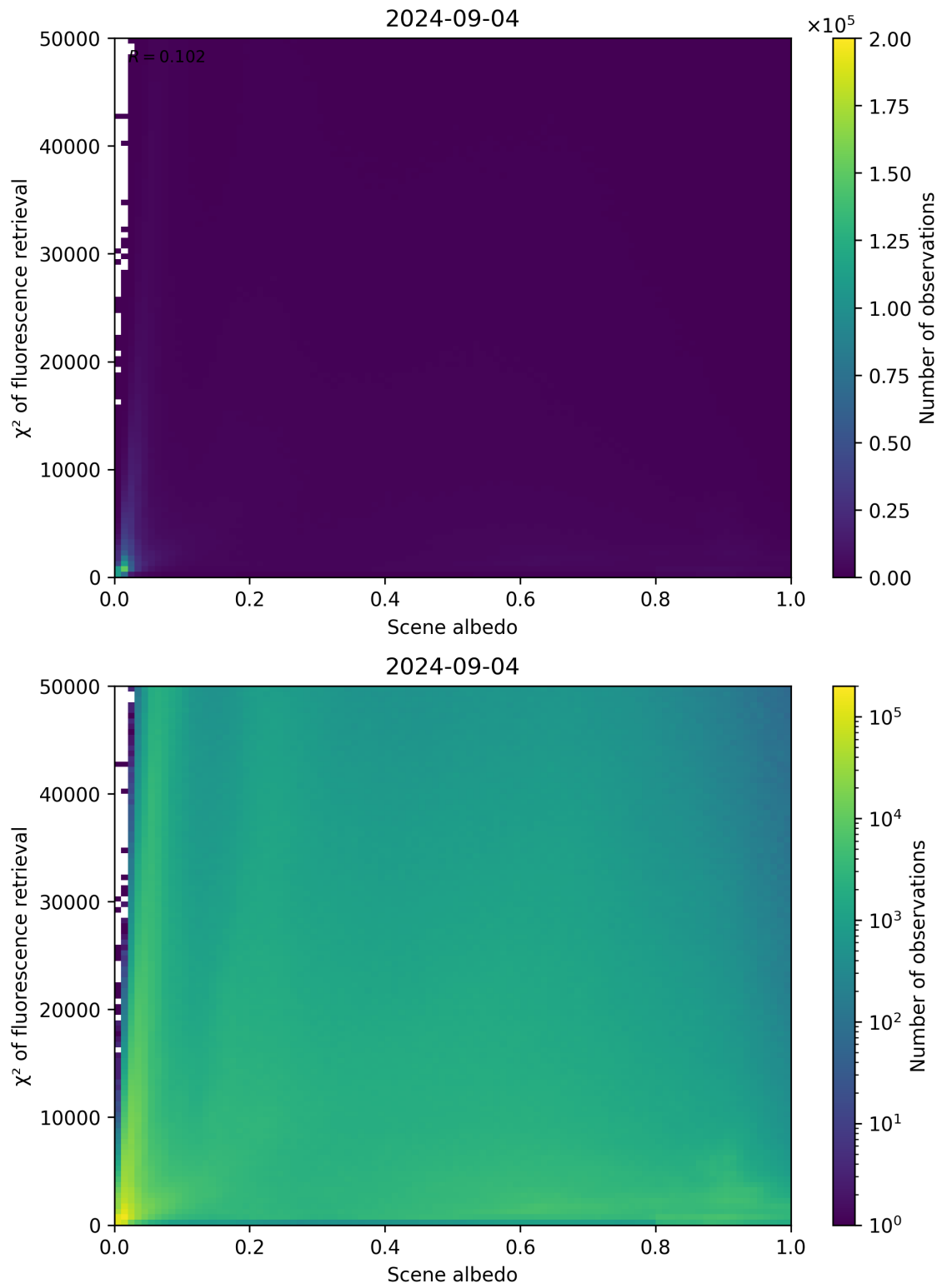
Figure 103: Scatter density plot of “Scene albedo” against “ \chi^2 of fluorescence retrieval” for 2024-09-03 to 2024-09-05.
