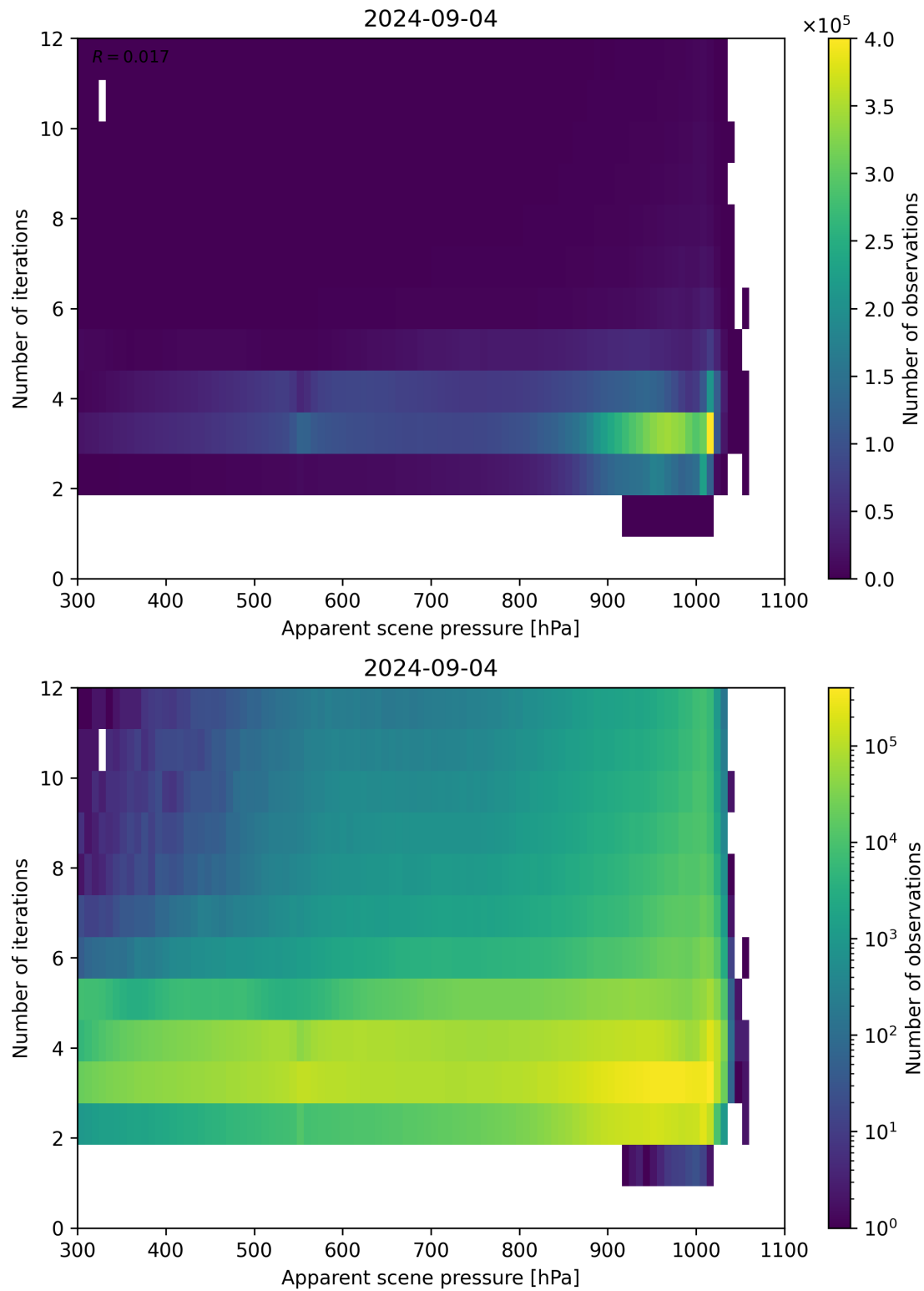
Figure 65: Scatter density plot of “Apparent scene pressure” against “Number of iterations” for 2024-09-03 to 2024-09-05.
