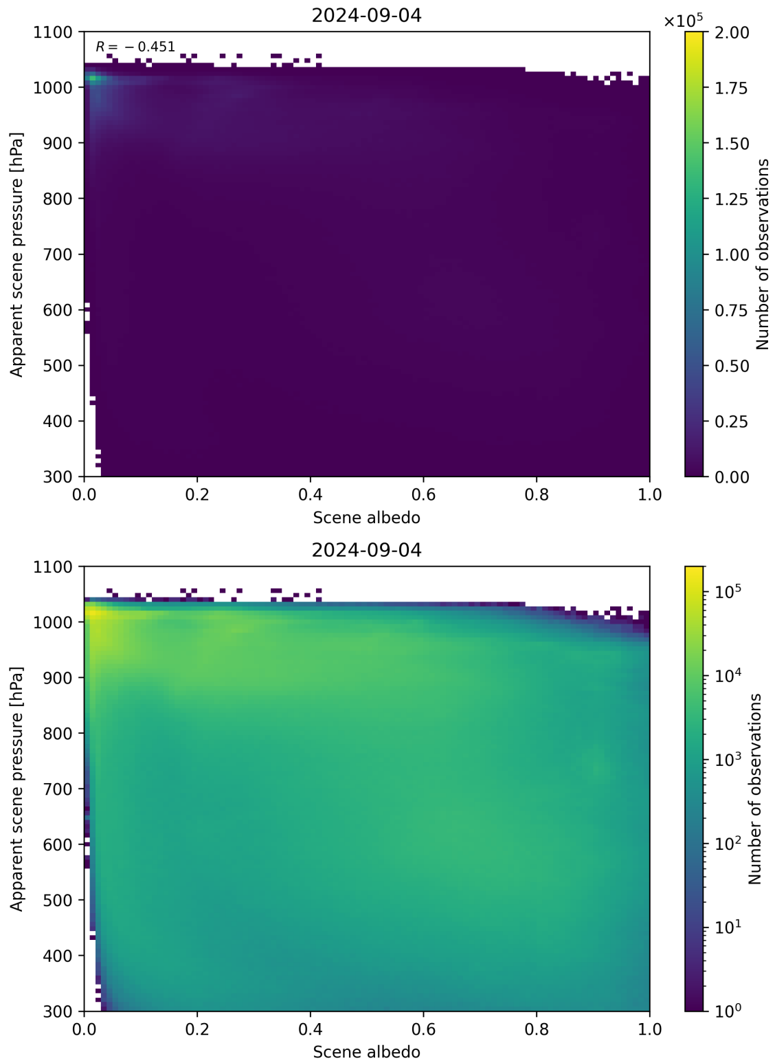
Figure 102: Scatter density plot of “Scene albedo” against “Apparent scene pressure” for 2024-09-03 to 2024-09-05.
