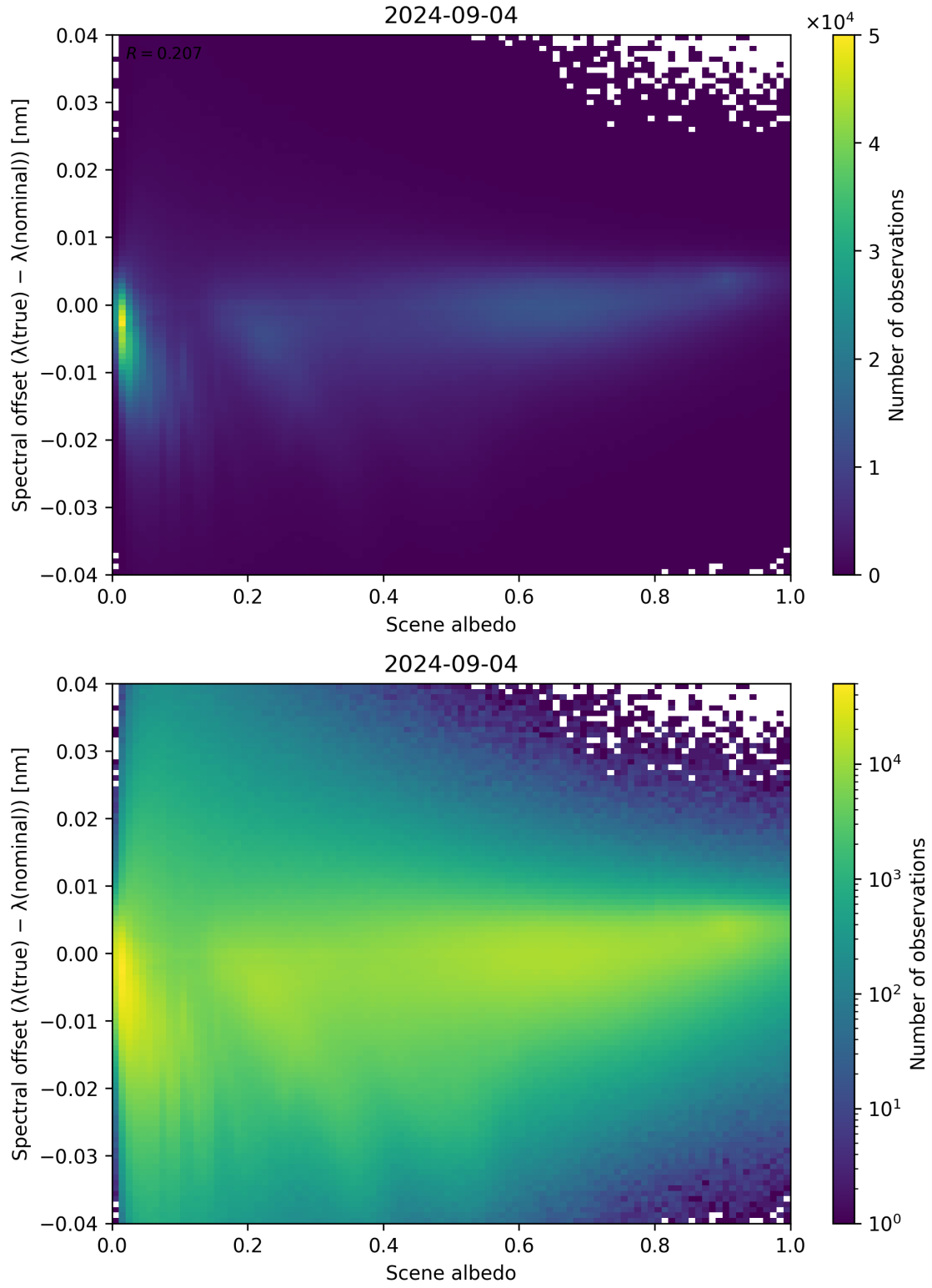
Figure 107: Scatter density plot of “Scene albedo” against “Spectral offset ( \lambda_{\text{true}} - \lambda_{\text{nominal}} )” for 2024-09-03 to 2024-09-05.
