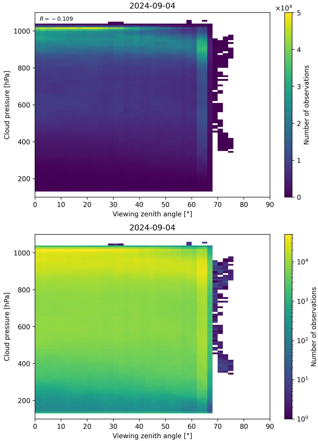
Figure 121: Scatter density plot of “Viewing zenith angle” against “Cloud pressure” for 2024-09-03 to 2024-09-05.
