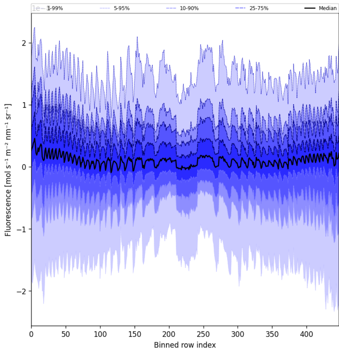
Figure 57: Along track statistics of “Fluorescence” for 2024-09-03 to 2024-09-05
