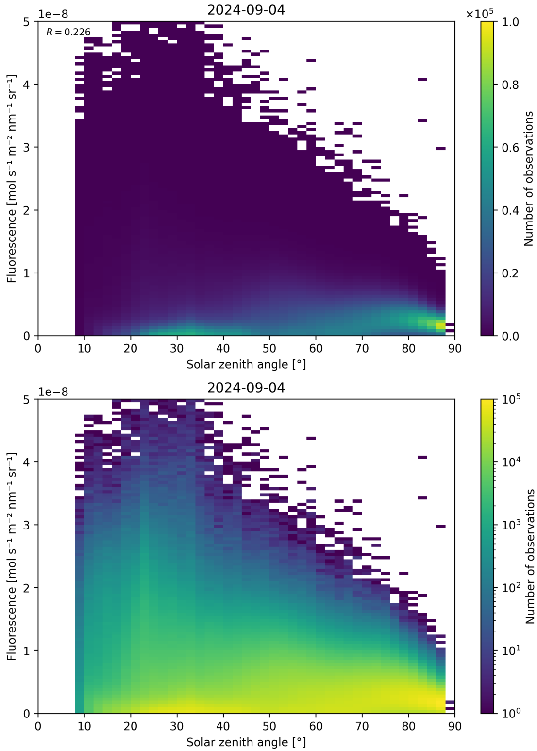
Figure 112: Scatter density plot of “Solar zenith angle” against “Fluorescence” for 2024-09-03 to 2024-09-05.
