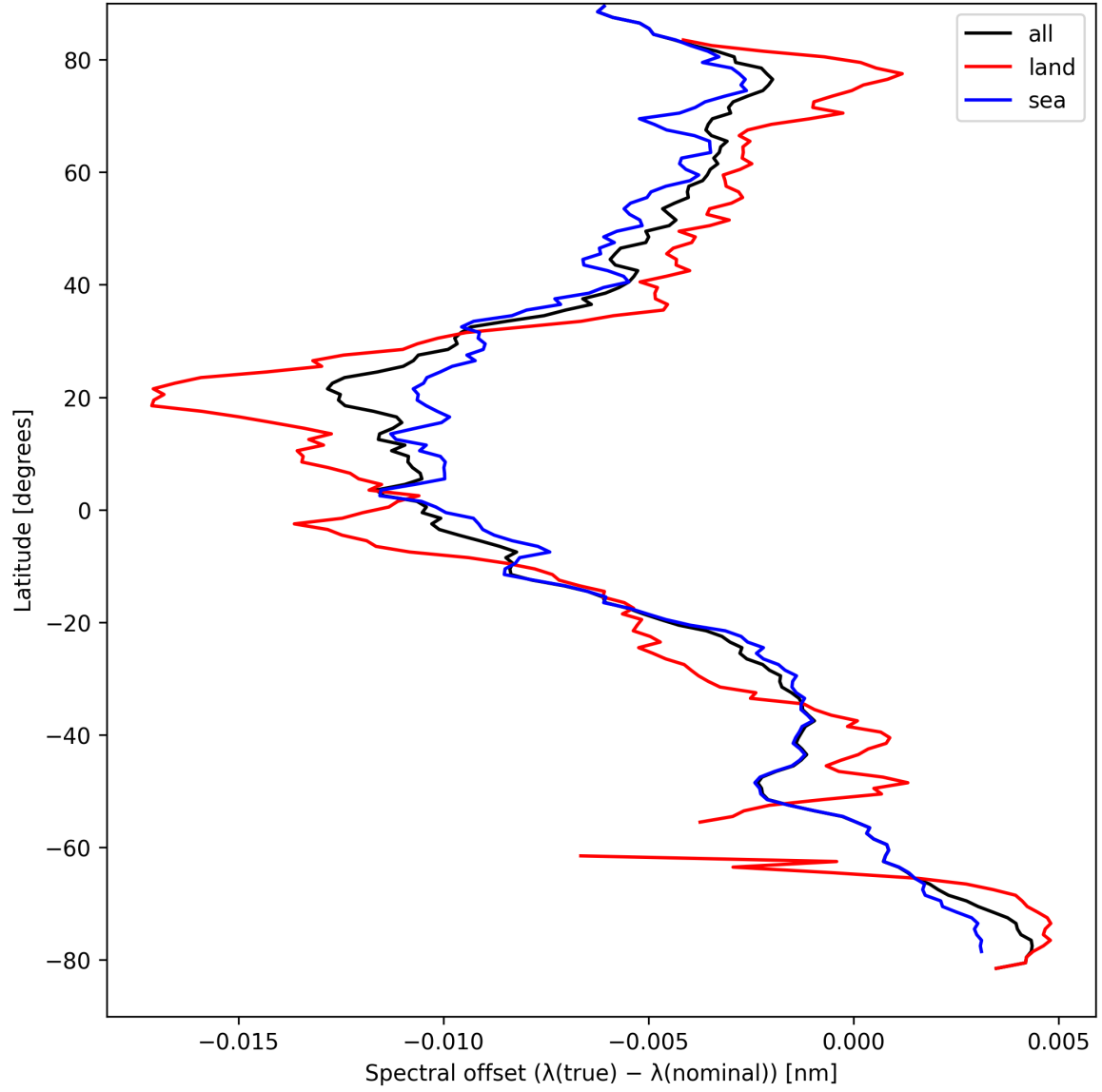
Figure 28: Zonal average of “Spectral offset ( \lambda_{\text{true}} - \lambda_{\text{nominal}} )” for 2024-09-03 to 2024-09-05.
