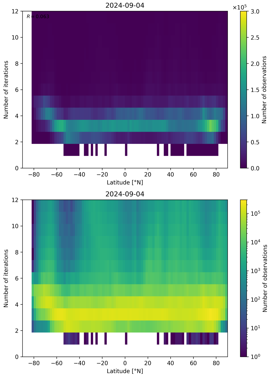
Figure 93: Scatter density plot of “Latitude” against “Number of iterations” for 2024-09-03 to 2024-09-05.
