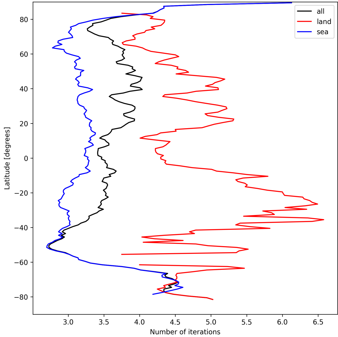
Figure 22: Zonal average of “Number of iterations” for 2024-09-03 to 2024-09-05.
