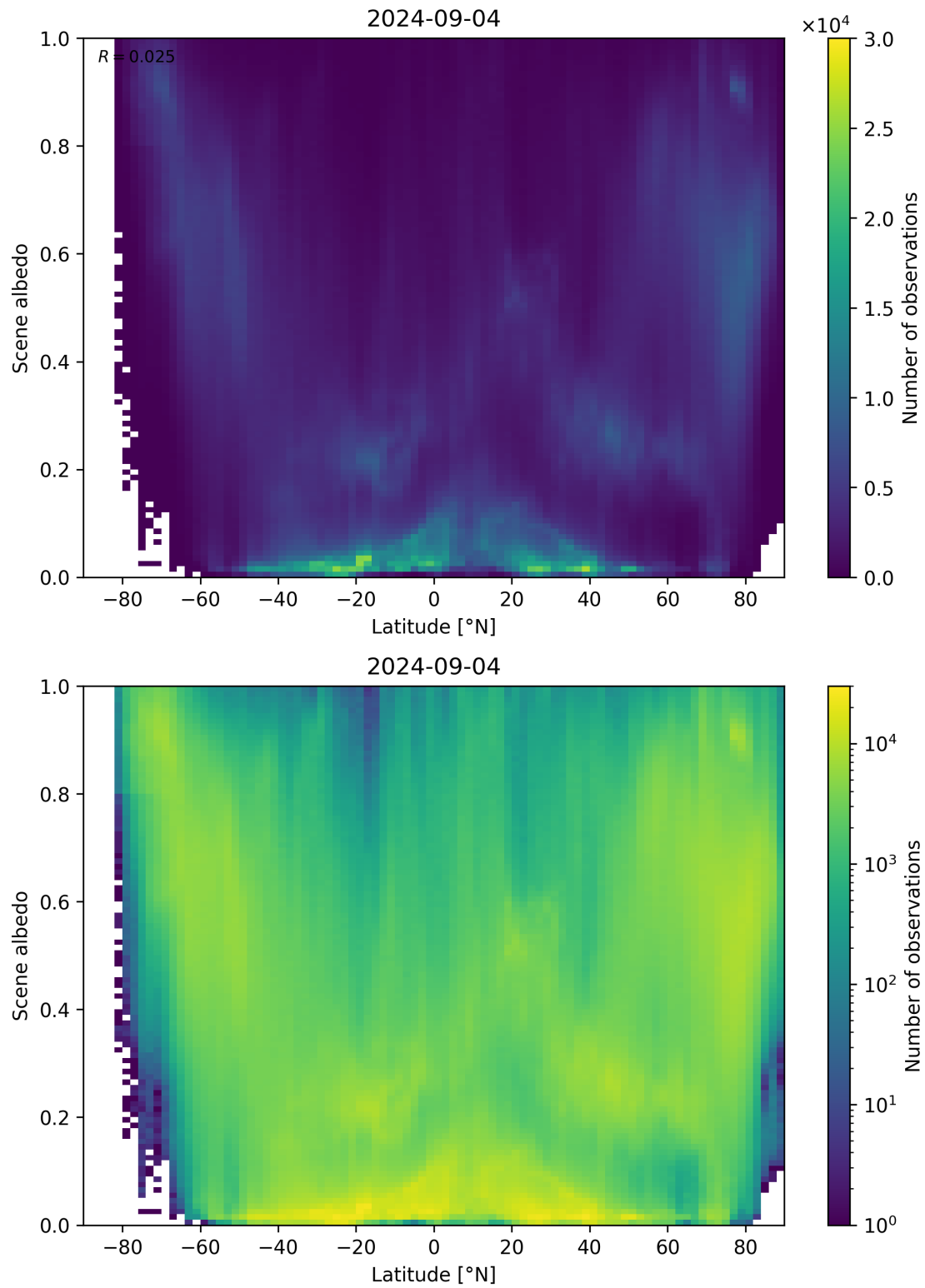
Figure 95: Scatter density plot of “Latitude” against “Scene albedo” for 2024-09-03 to 2024-09-05.
