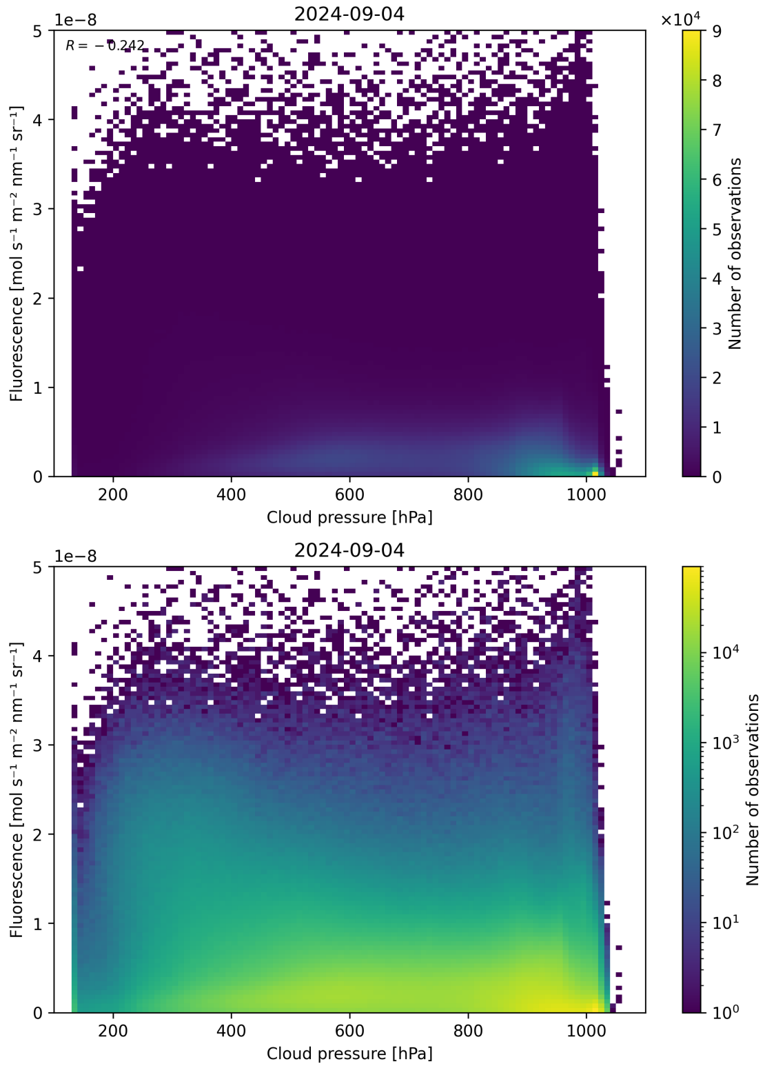
Figure 80: Scatter density plot of “Cloud pressure” against “Fluorescence” for 2024-09-03 to 2024-09-05.
