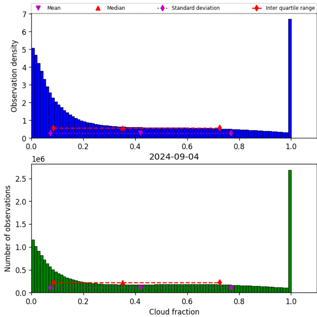
Figure 32: Histogram of “Cloud fraction” for 2024-09-03 to 2024-09-05
