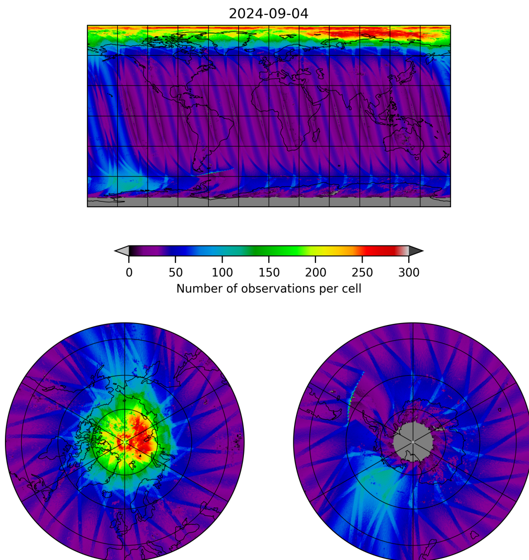
Figure 11: Map of the number of observations for 2024-09-03 to 2024-09-05
