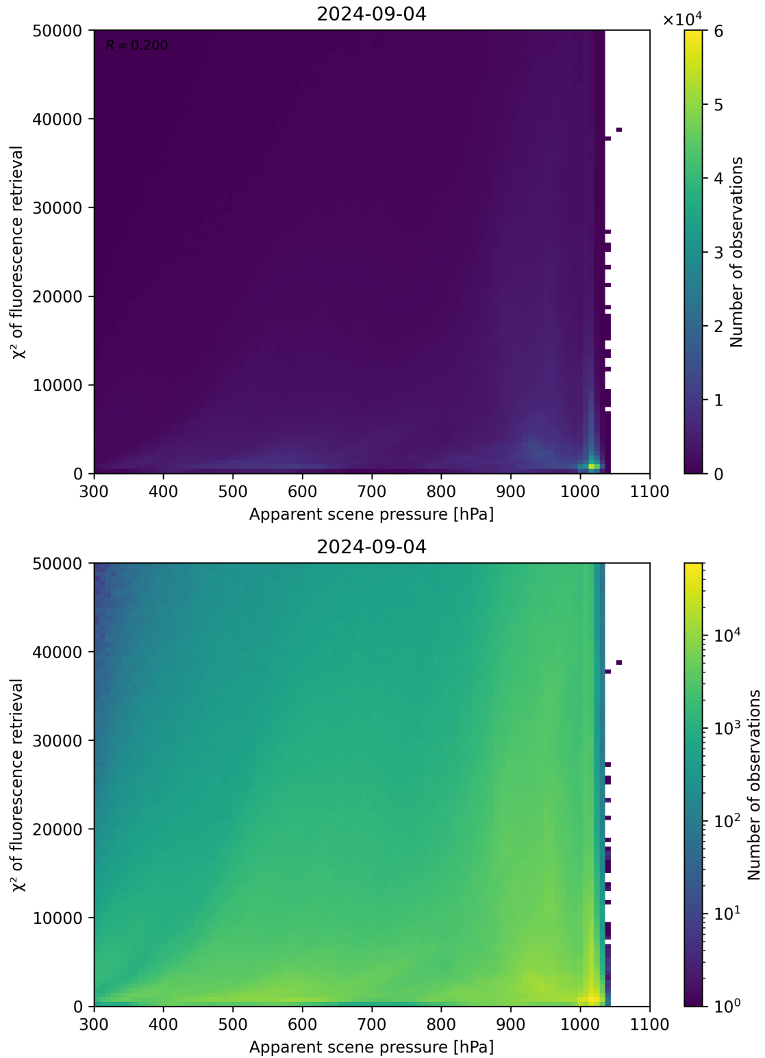
Figure 63: Scatter density plot of “Apparent scene pressure” against “ \chi^2 of fluorescence retrieval” for 2024-09-03 to 2024-09-05.
