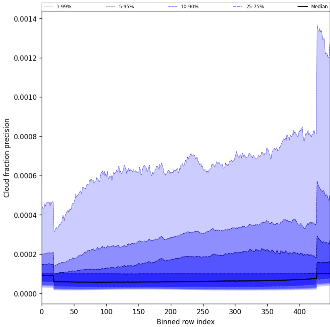
Figure 50: Along track statistics of “Cloud fraction precision” for 2024-09-03 to 2024-09-05
