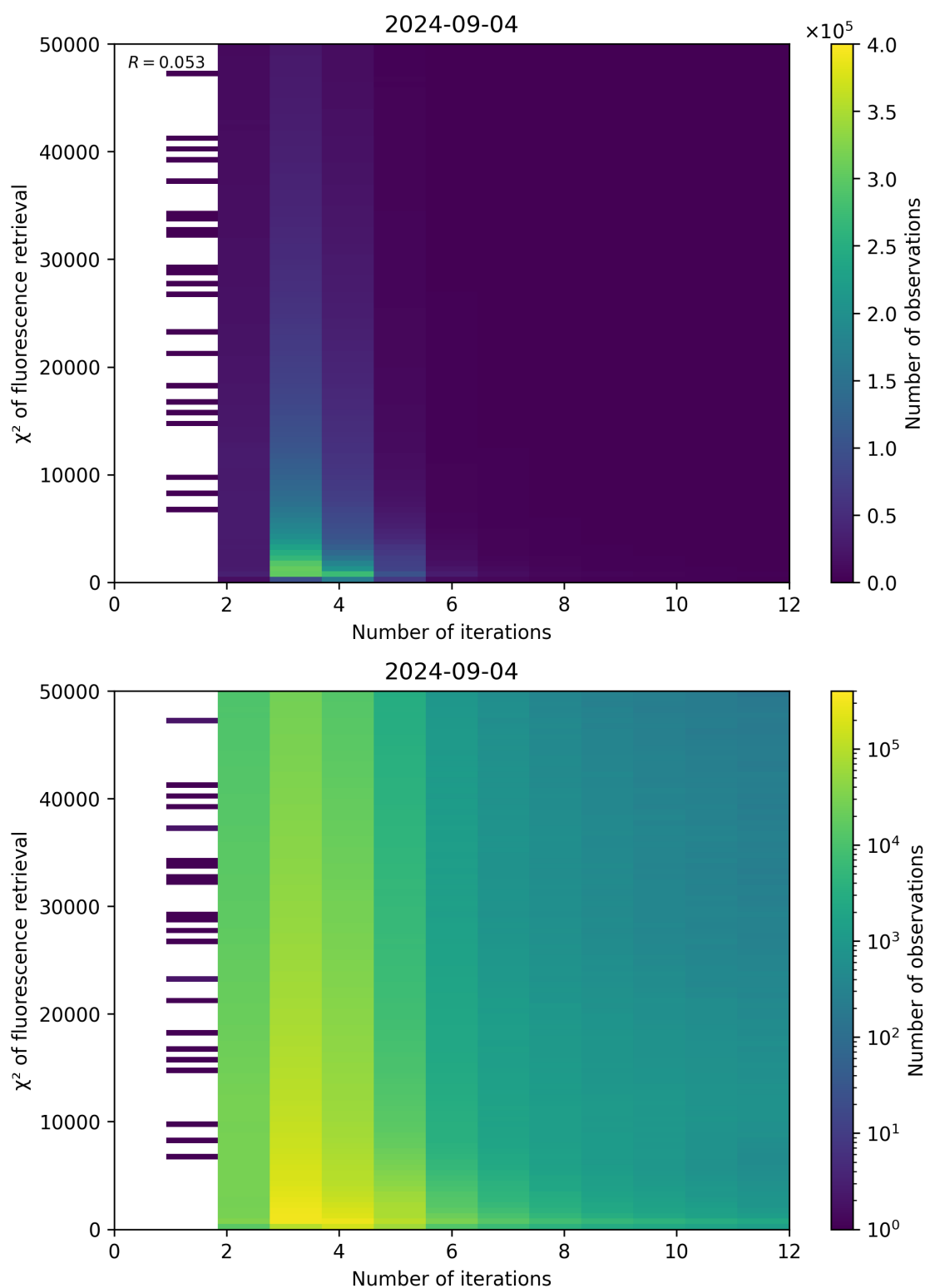
Figure 97: Scatter density plot of “Number of iterations” against “ \chi^2 of fluorescence retrieval” for 2024-09-03 to 2024-09-05.
