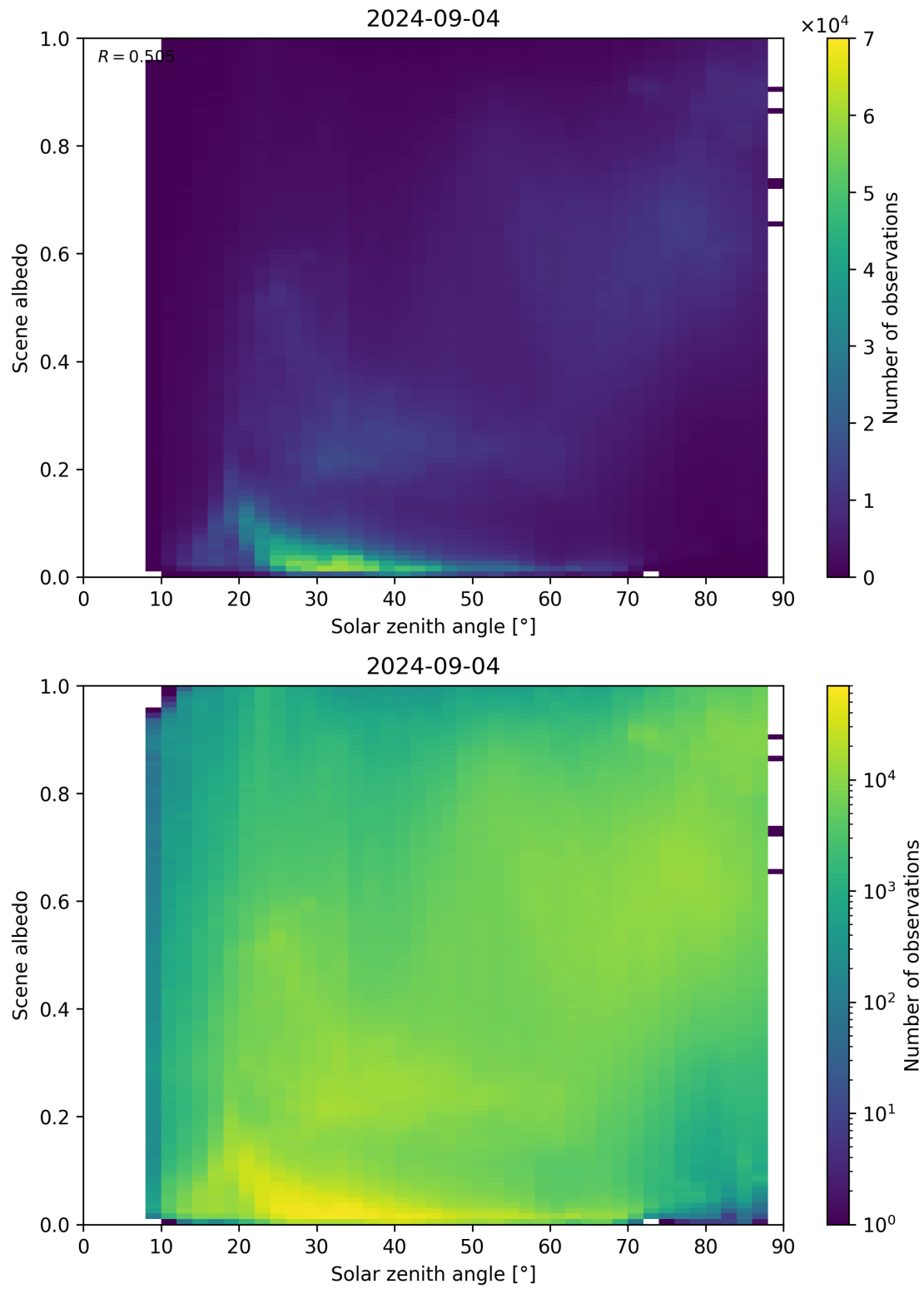
Figure 116: Scatter density plot of “Solar zenith angle” against “Scene albedo” for 2024-09-03 to 2024-09-05.
