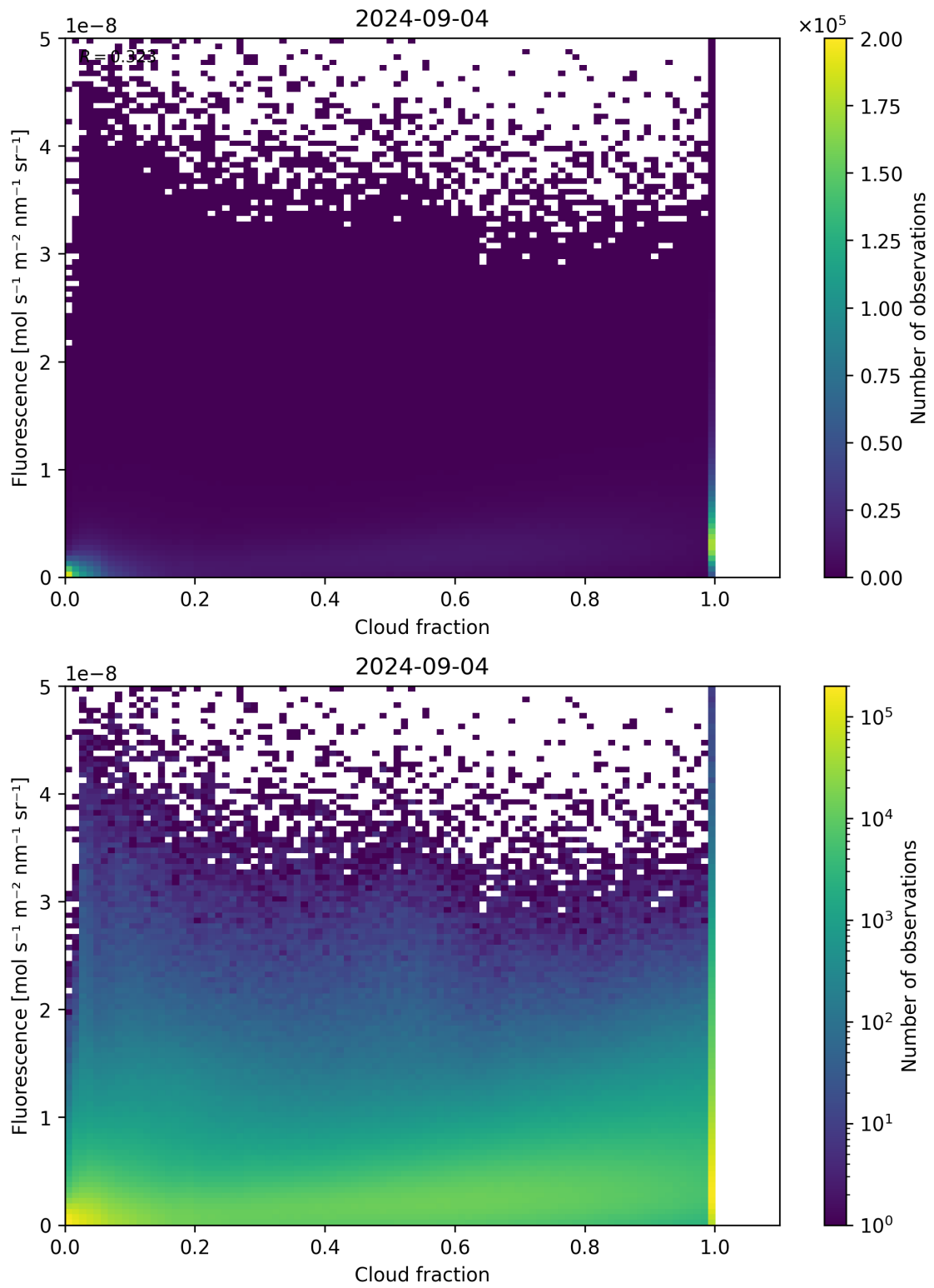
Figure 72: Scatter density plot of “Cloud fraction” against “Fluorescence” for 2024-09-03 to 2024-09-05.
