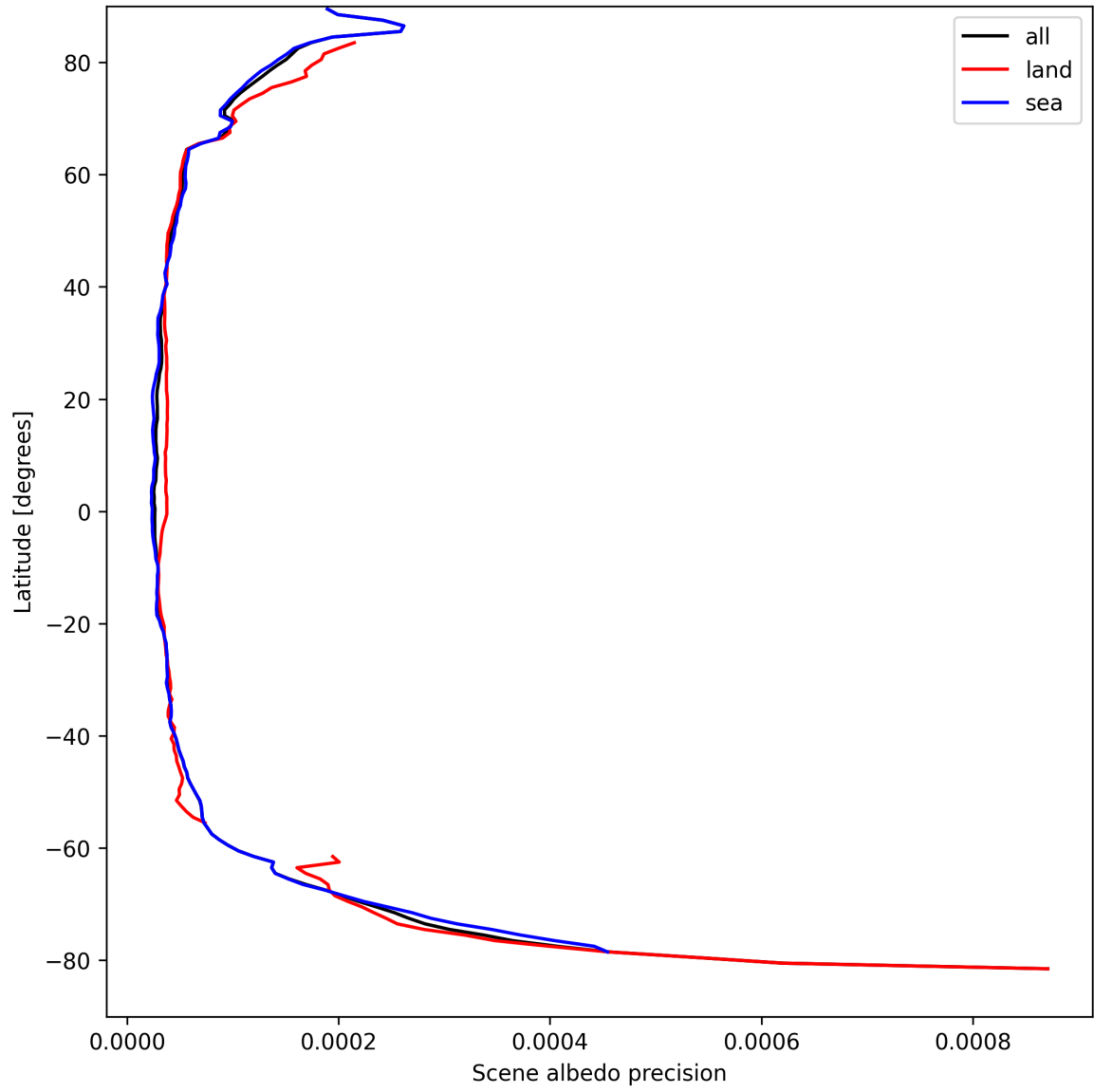
Figure 18: Zonal average of “Scene albedo precision” for 2024-09-03 to 2024-09-05.
