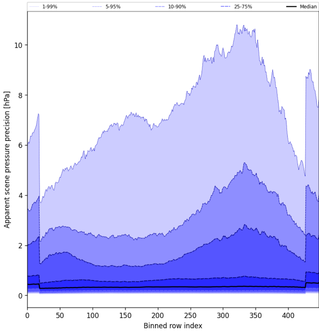
Figure 54: Along track statistics of “Apparent scene pressure precision” for 2024-09-03 to 2024-09-05
