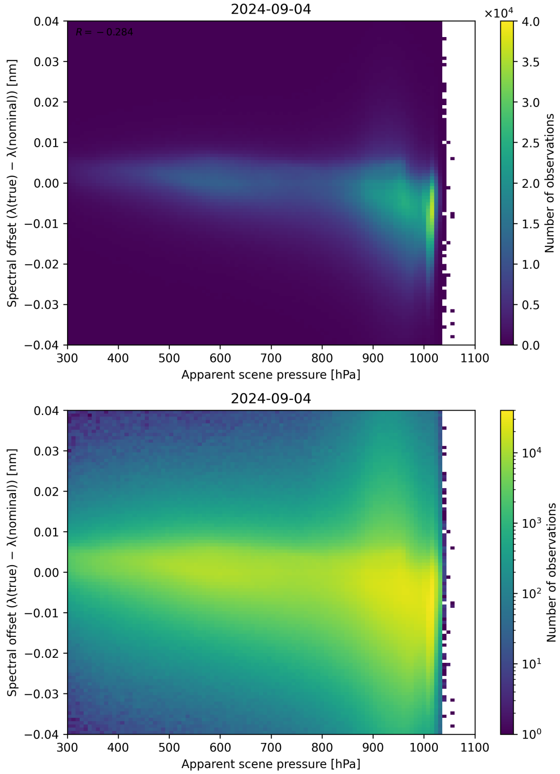
Figure 67: Scatter density plot of “Apparent scene pressure” against “Spectral offset ( \lambda_{\text{true}} - \lambda_{\text{nominal}} )” for 2024-09-03 to 2024-09-05.
