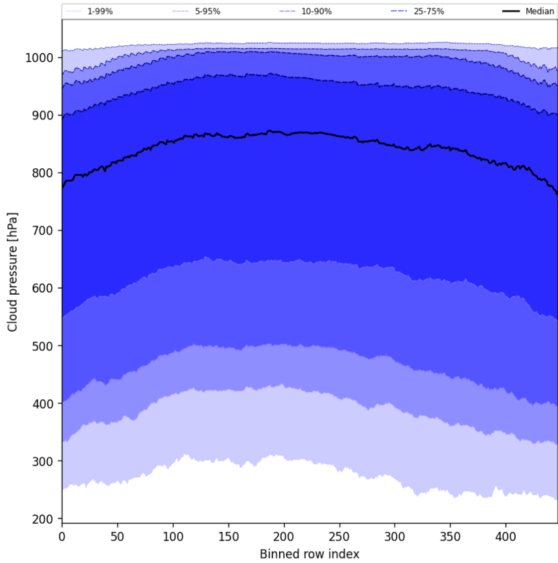
Figure 47: Along track statistics of “Cloud pressure” for 2024-09-03 to 2024-09-05
