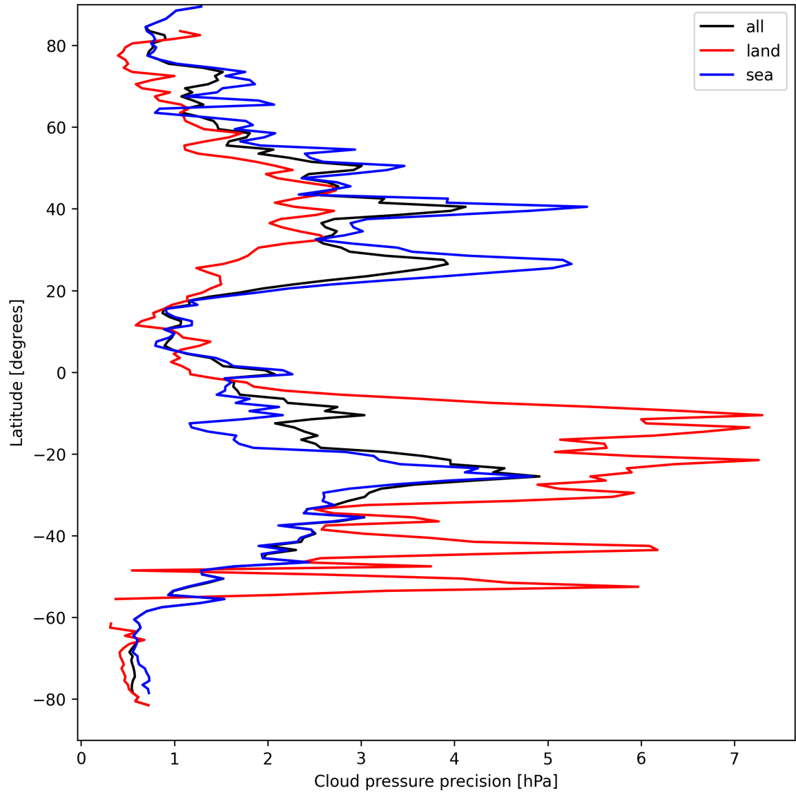
Figure 14: Zonal average of “Cloud pressure precision” for 2024-09-03 to 2024-09-05.
