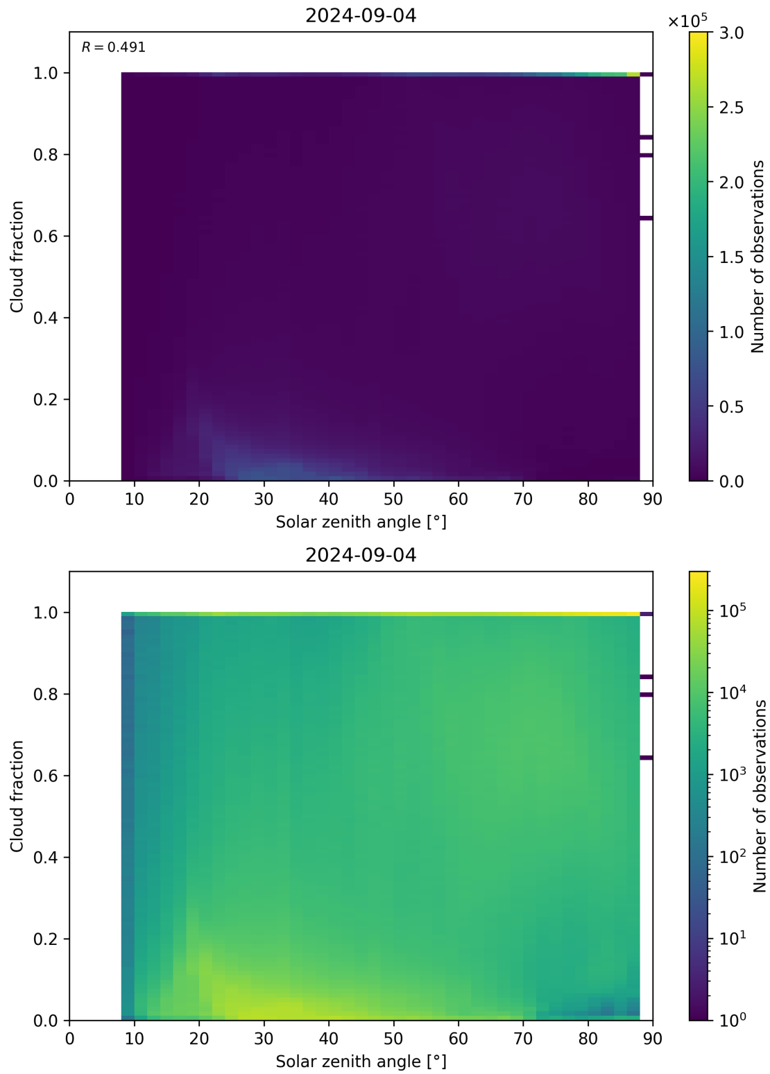
Figure 110: Scatter density plot of “Solar zenith angle” against “Cloud fraction” for 2024-09-03 to 2024-09-05.
