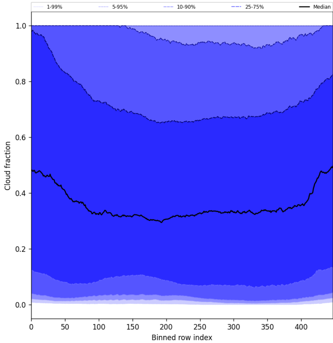
Figure 49: Along track statistics of “Cloud fraction” for 2024-09-03 to 2024-09-05
