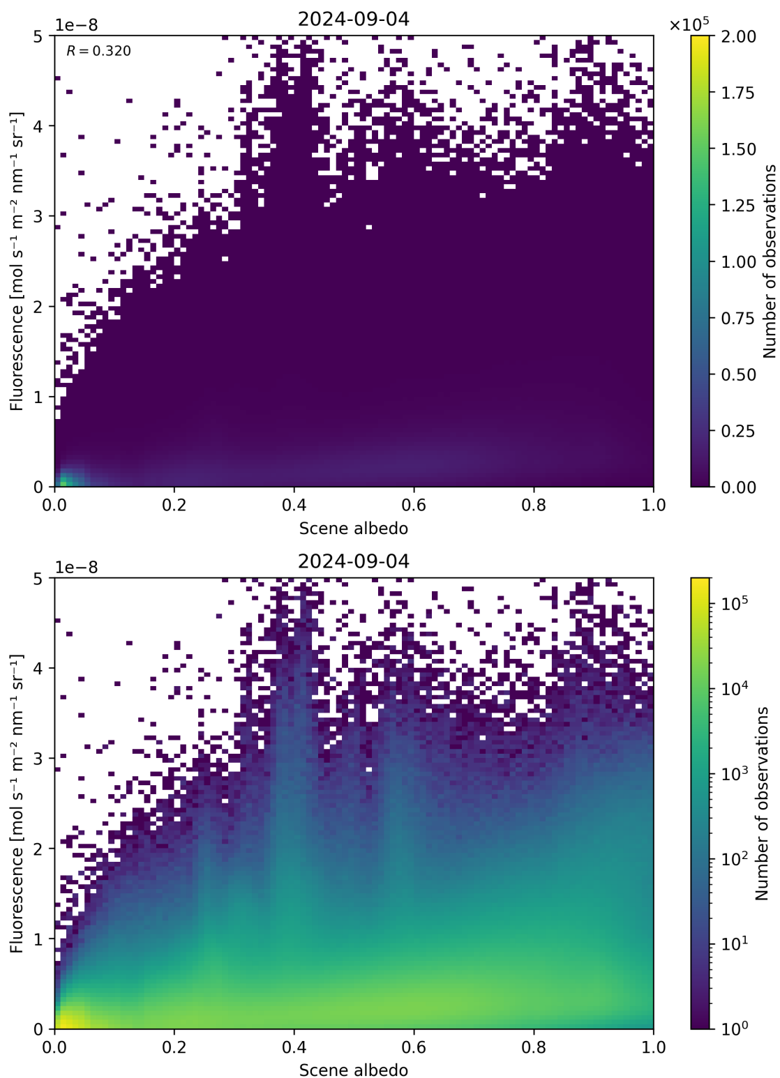
Figure 104: Scatter density plot of “Scene albedo” against “Fluorescence” for 2024-09-03 to 2024-09-05.
