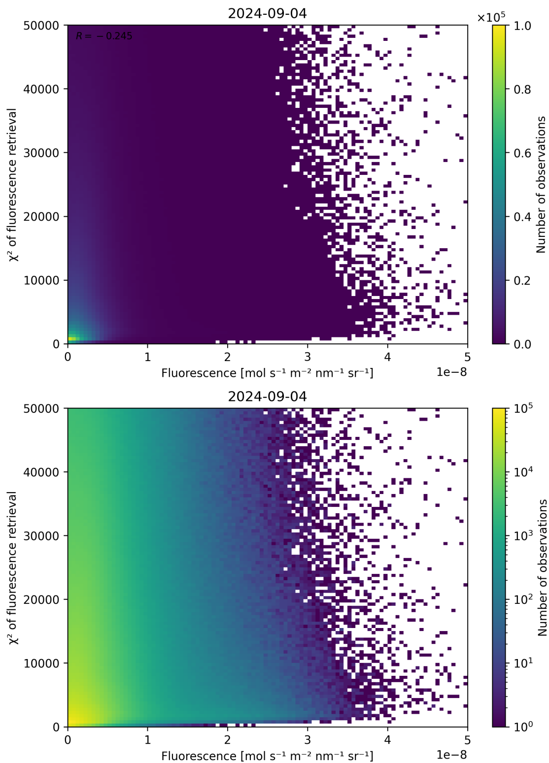
Figure 85: Scatter density plot of “Fluorescence” against “ \chi^2 of fluorescence retrieval” for 2024-09-03 to 2024-09-05.
