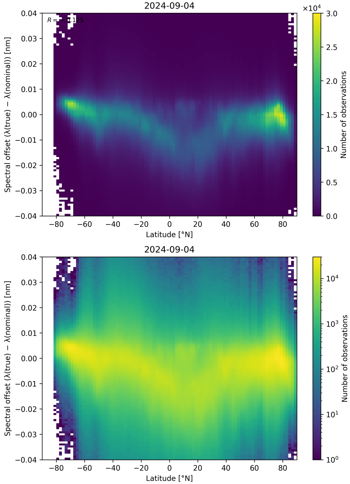
Figure 96: Scatter density plot of “Latitude” against “Spectral offset ( \lambda_{\text{true}} - \lambda_{\text{nominal}} )” for 2024-09-03 to 2024-09-05.
