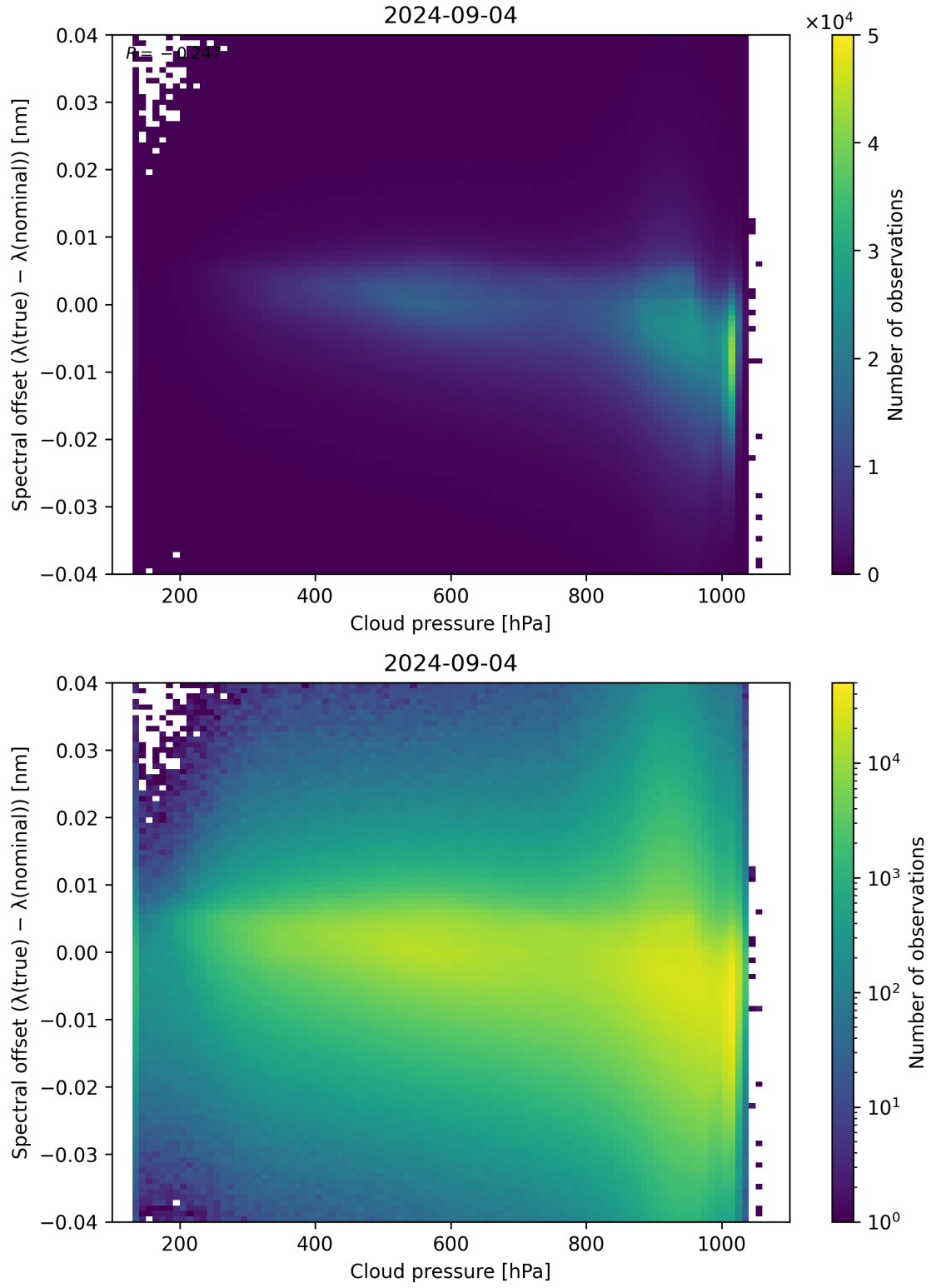
Figure 84: Scatter density plot of “Cloud pressure” against “Spectral offset ( \lambda_{\text{true}} - \lambda_{\text{nominal}} )” for 2024-09-03 to 2024-09-05.
