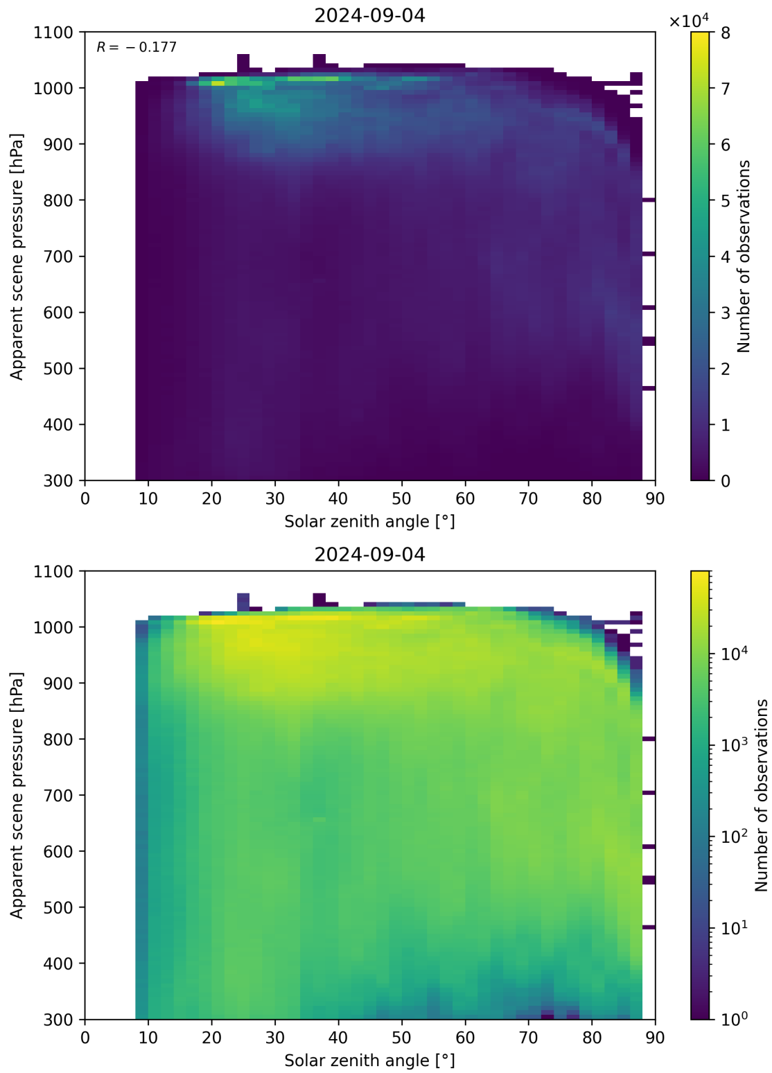
Figure 108: Scatter density plot of “Solar zenith angle” against “Apparent scene pressure” for 2024-09-03 to 2024-09-05.
