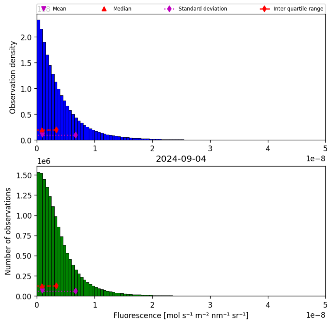
Figure 40: Histogram of “Fluorescence” for 2024-09-03 to 2024-09-05
