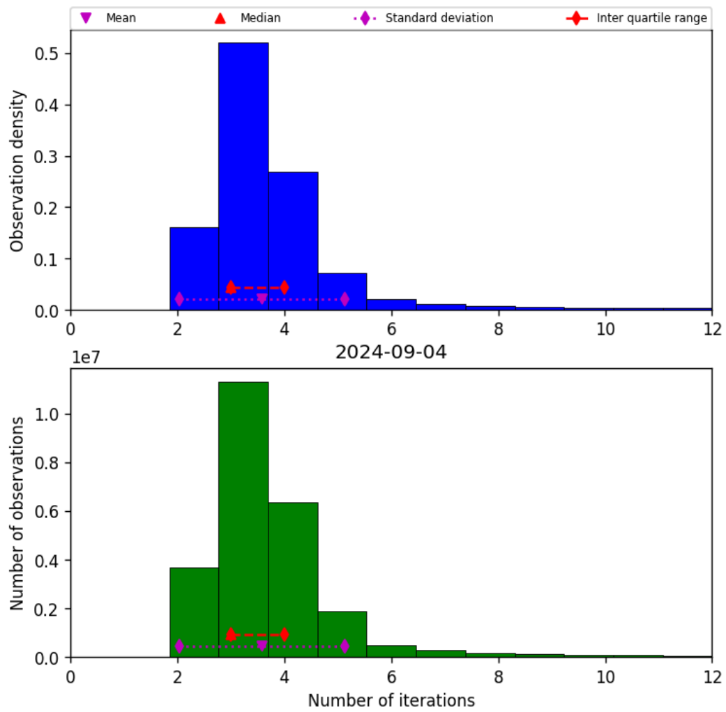
Figure 39: Histogram of “Number of iterations” for 2024-09-03 to 2024-09-05
