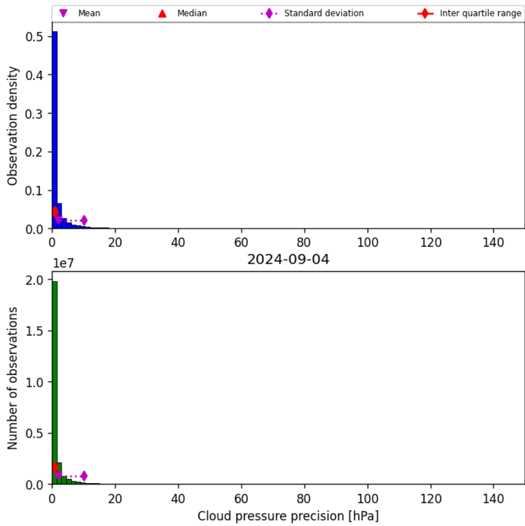
Figure 31: Histogram of “Cloud pressure precision” for 2024-09-03 to 2024-09-05
