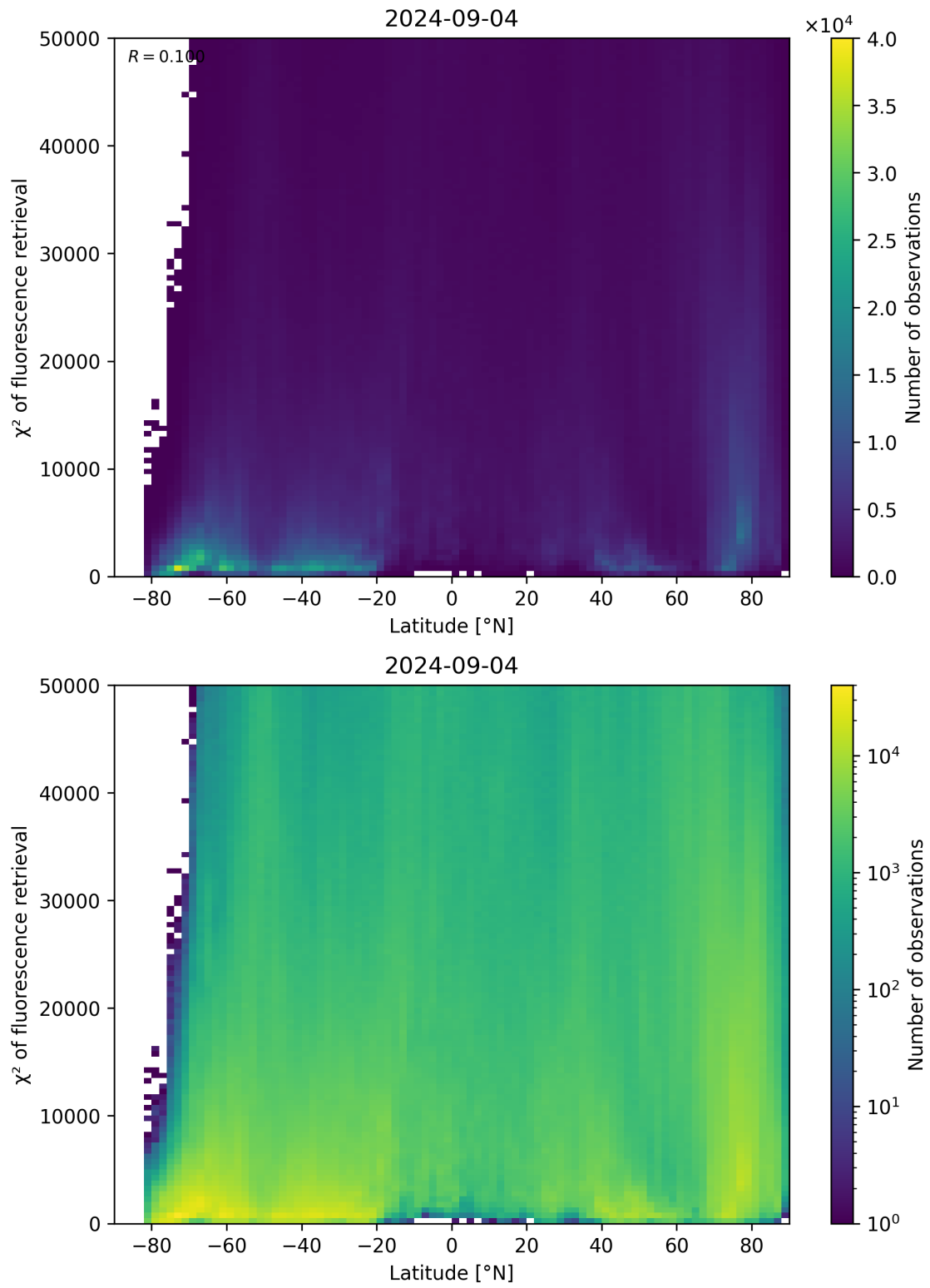
Figure 89: Scatter density plot of “Latitude” against “ \chi^2 of fluorescence retrieval” for 2024-09-03 to 2024-09-05.
