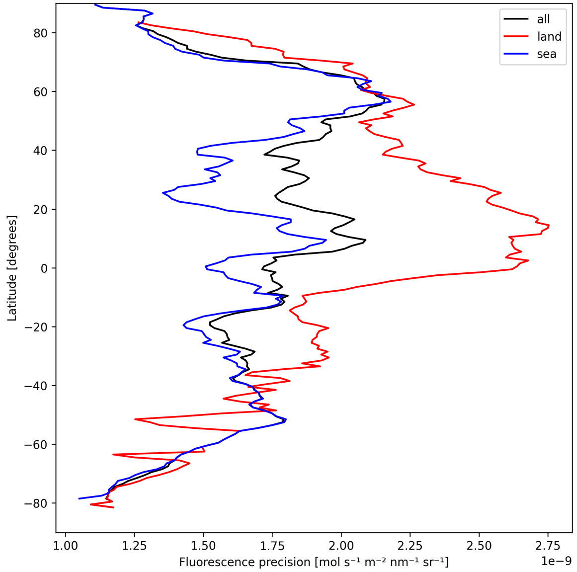
Figure 24: Zonal average of “Fluorescence precision” for 2024-09-03 to 2024-09-05.
