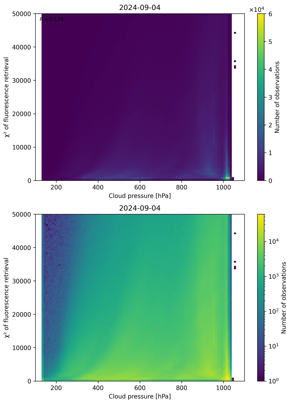
Figure 78: Scatter density plot of “Cloud pressure” against “ \chi^2 of fluorescence retrieval” for 2024-09-03 to 2024-09-05.
