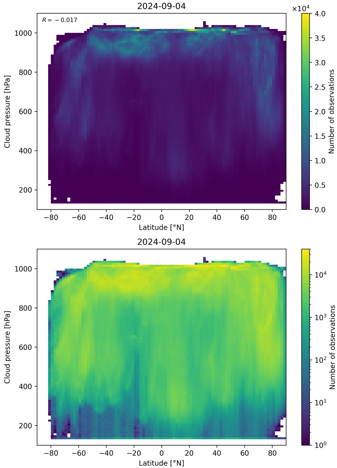
Figure 91: Scatter density plot of “Latitude” against “Cloud pressure” for 2024-09-03 to 2024-09-05.
