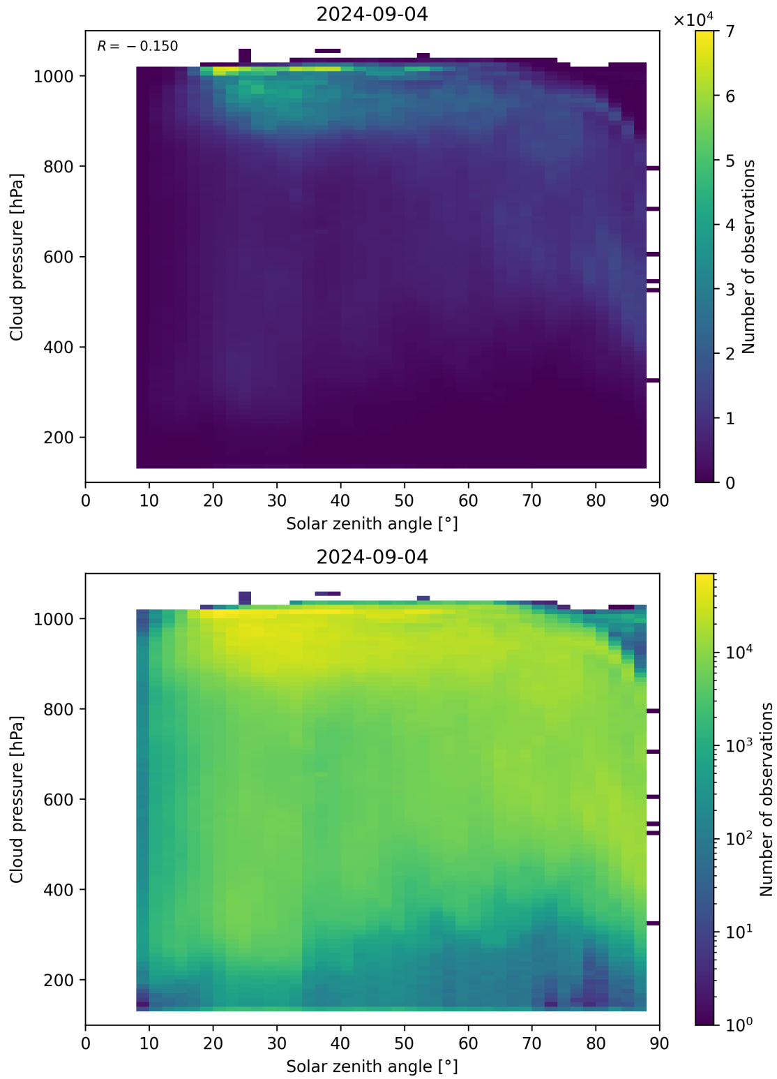
Figure 111: Scatter density plot of “Solar zenith angle” against “Cloud pressure” for 2024-09-03 to 2024-09-05.
