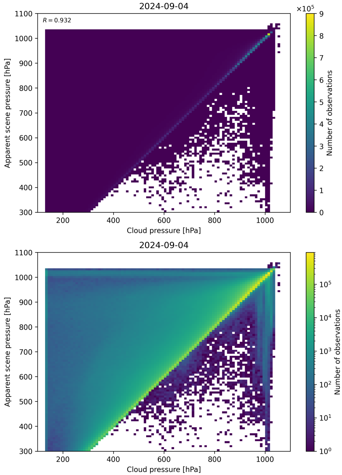
Figure 77: Scatter density plot of “Cloud pressure” against “Apparent scene pressure” for 2024-09-03 to 2024-09-05.
