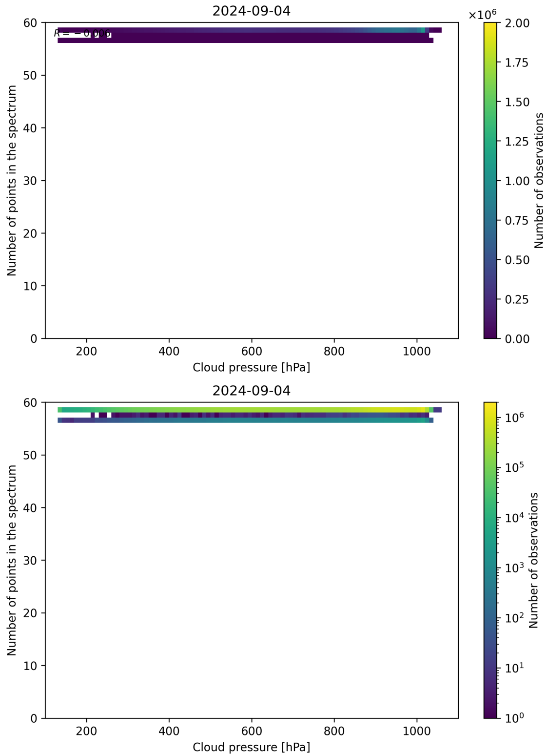
Figure 82: Scatter density plot of “Cloud pressure” against “Number of points in the spectrum” for 2024-09-03 to 2024-09-05.
