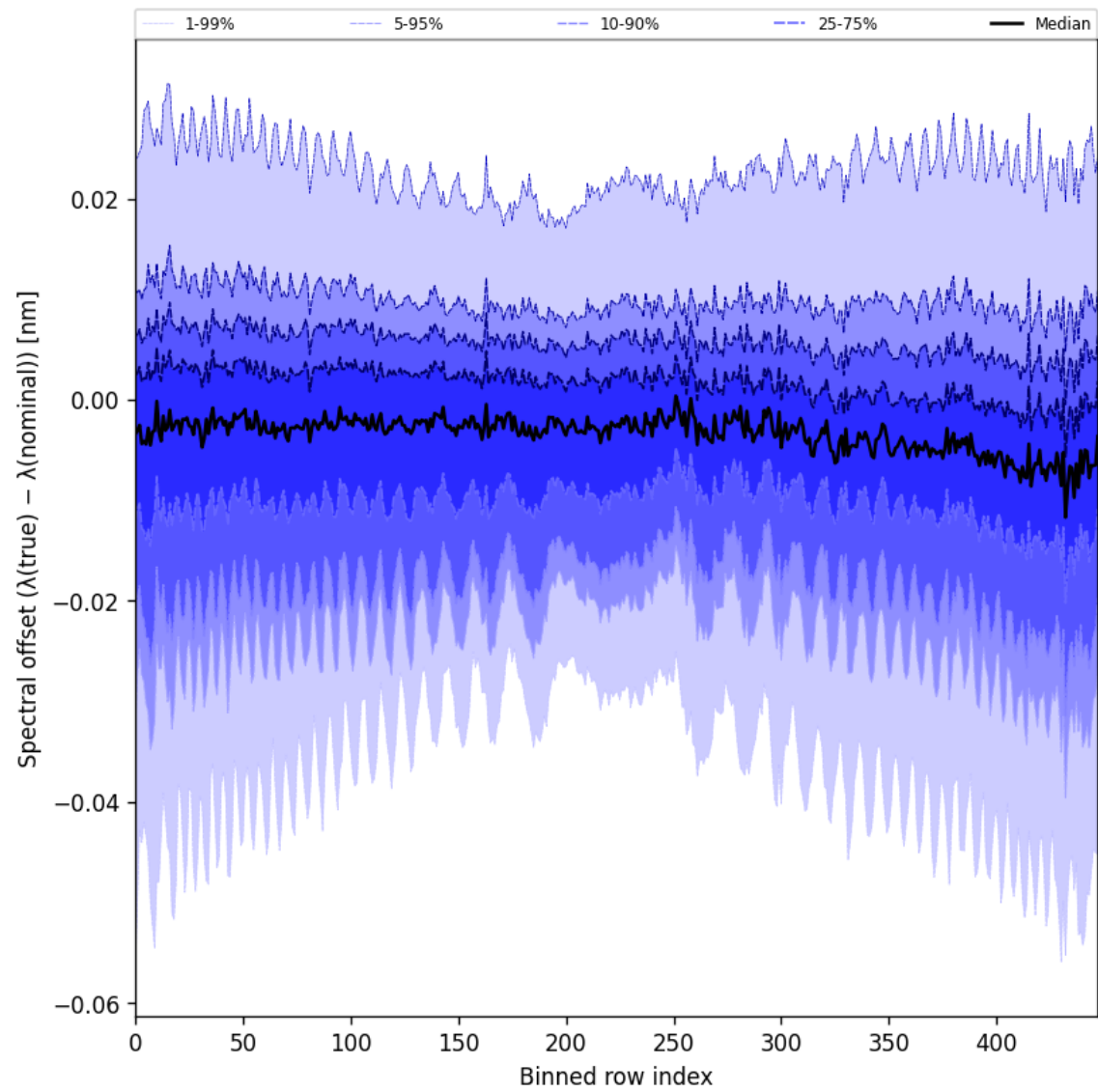
Figure 62: Along track statistics of “Spectral offset ( \lambda_{\text{true}} - \lambda_{\text{nominal}} )” for 2024-09-03 to 2024-09-05
