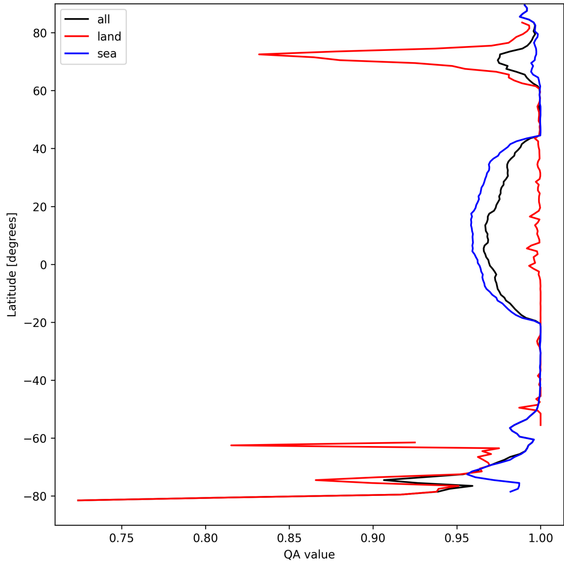
Figure 12: Zonal average of "QA value" for 2024-09-03 to 2024-09-05.
