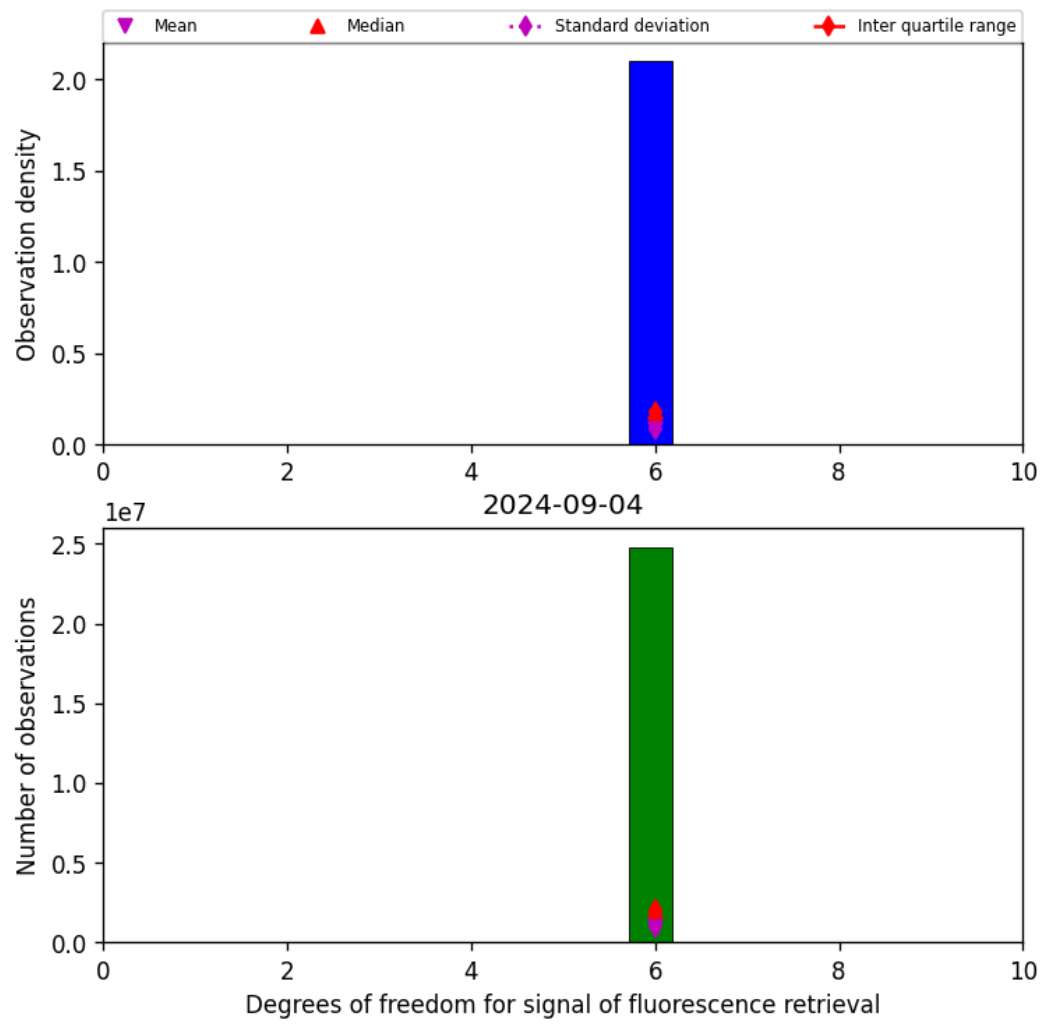
Figure 43: Histogram of “Degrees of freedom for signal of fluorescence retrieval” for 2024-09-03 to 2024-09-05
