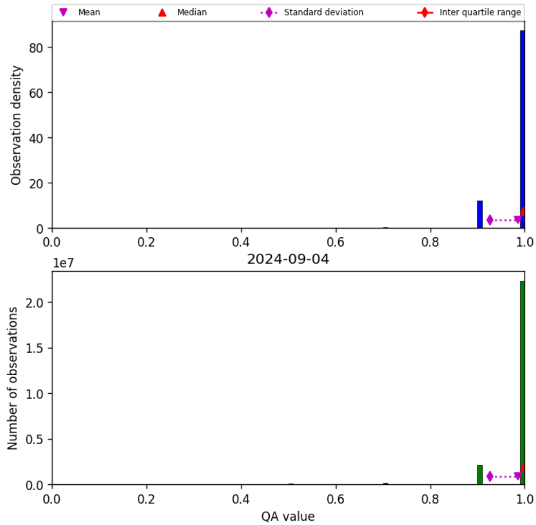
Figure 29: Histogram of “QA value” for 2024-09-03 to 2024-09-05
