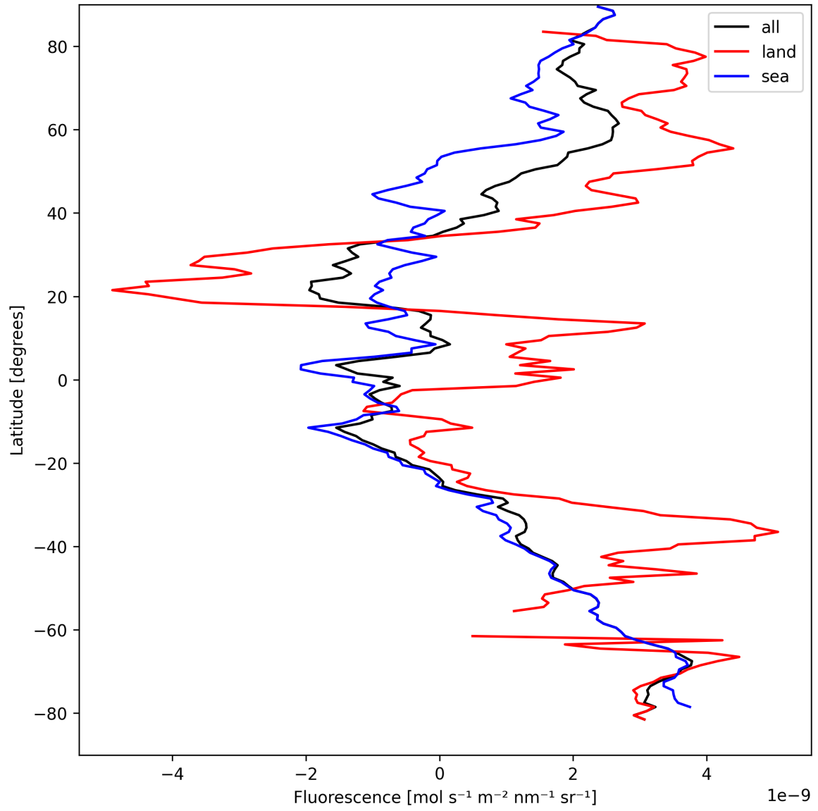
Figure 23: Zonal average of “Fluorescence” for 2024-09-03 to 2024-09-05.
