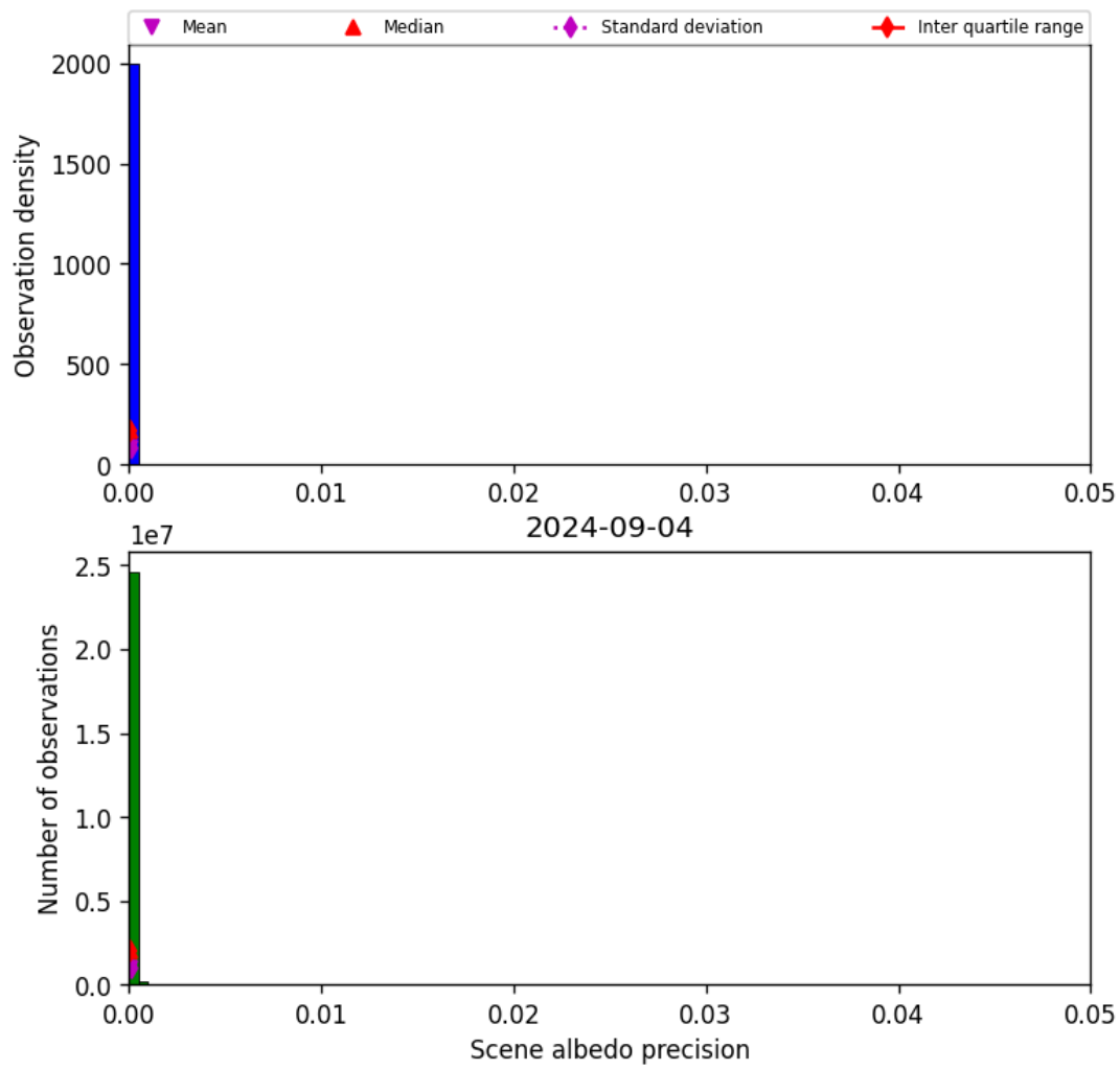
Figure 35: Histogram of “Scene albedo precision” for 2024-09-03 to 2024-09-05
