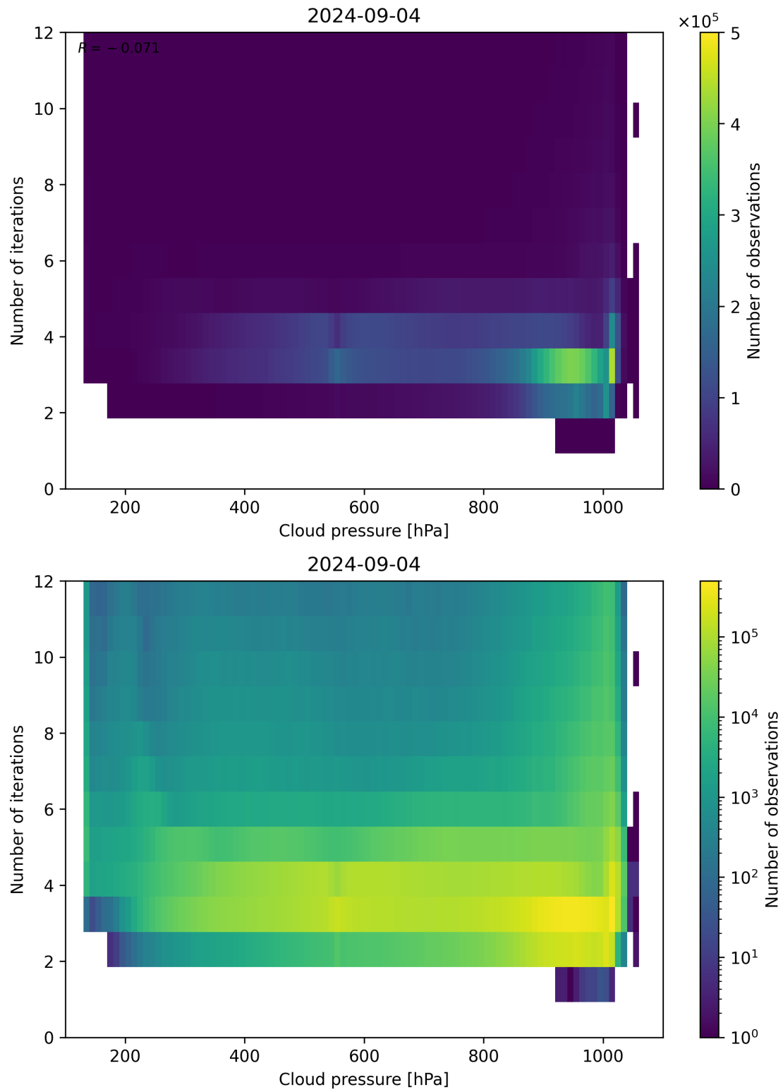
Figure 81: Scatter density plot of “Cloud pressure” against “Number of iterations” for 2024-09-03 to 2024-09-05.
