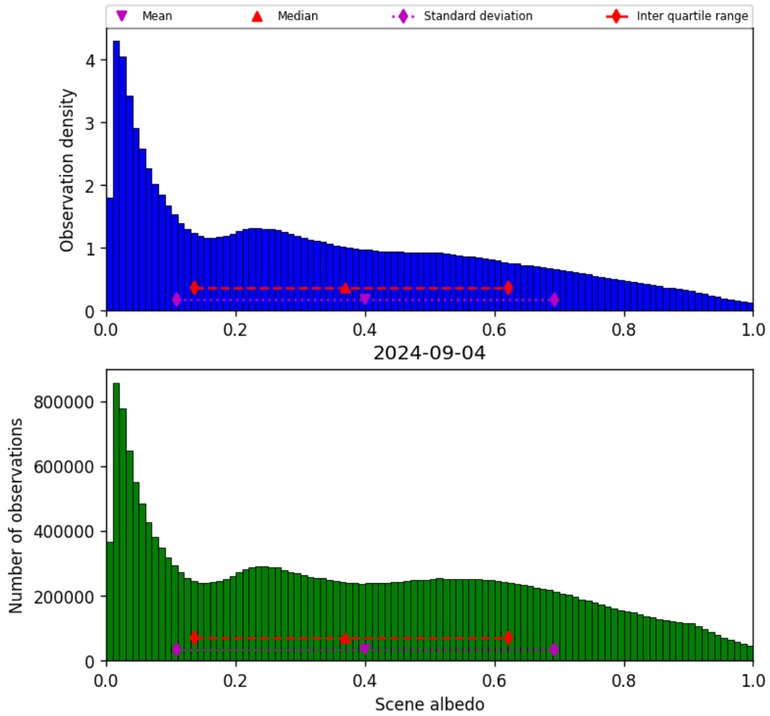
Figure 34: Histogram of “Scene albedo” for 2024-09-03 to 2024-09-05
