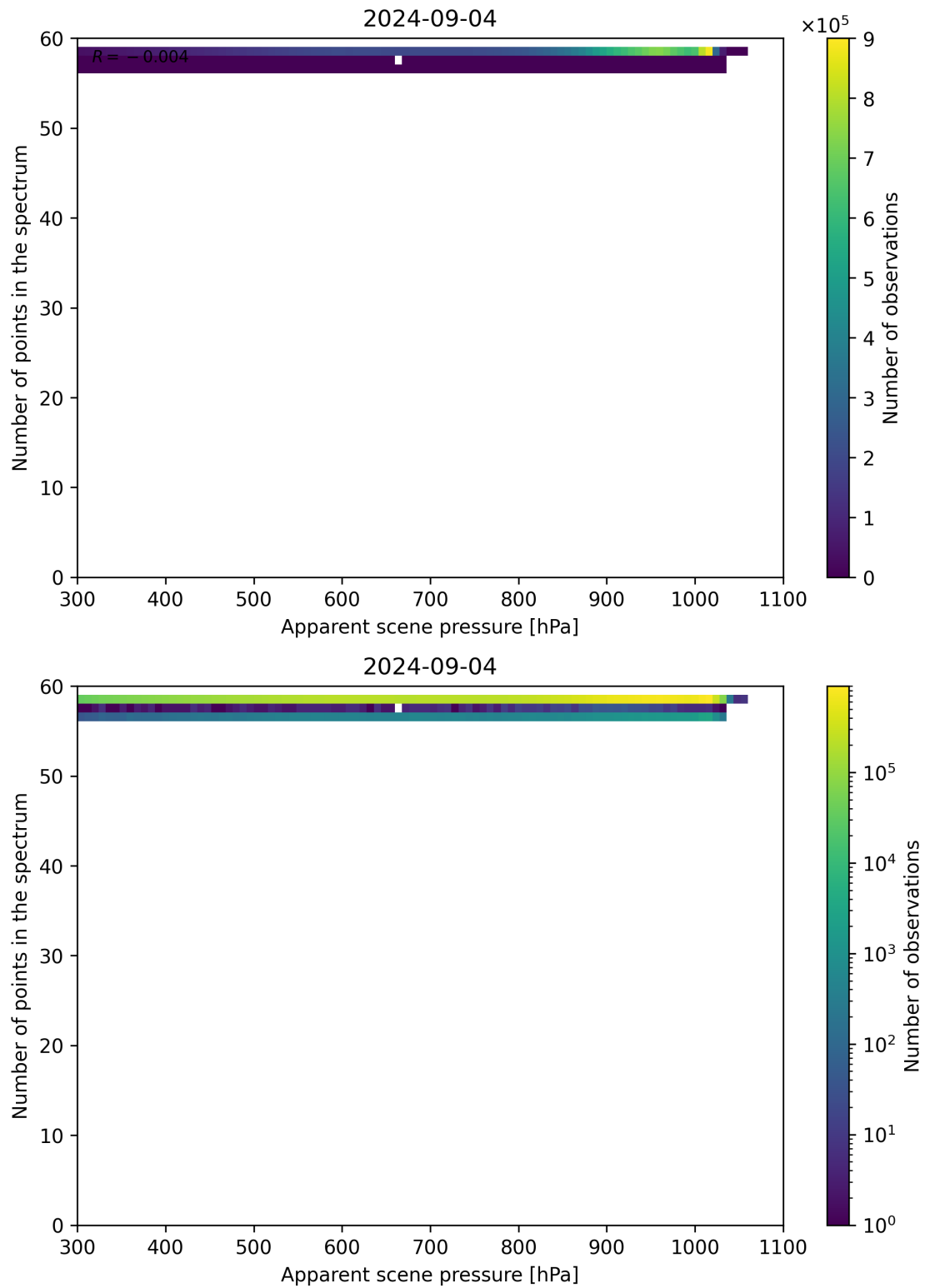
Figure 66: Scatter density plot of “Apparent scene pressure” against “Number of points in the spectrum” for 2024-09-03 to 2024-09-05.
