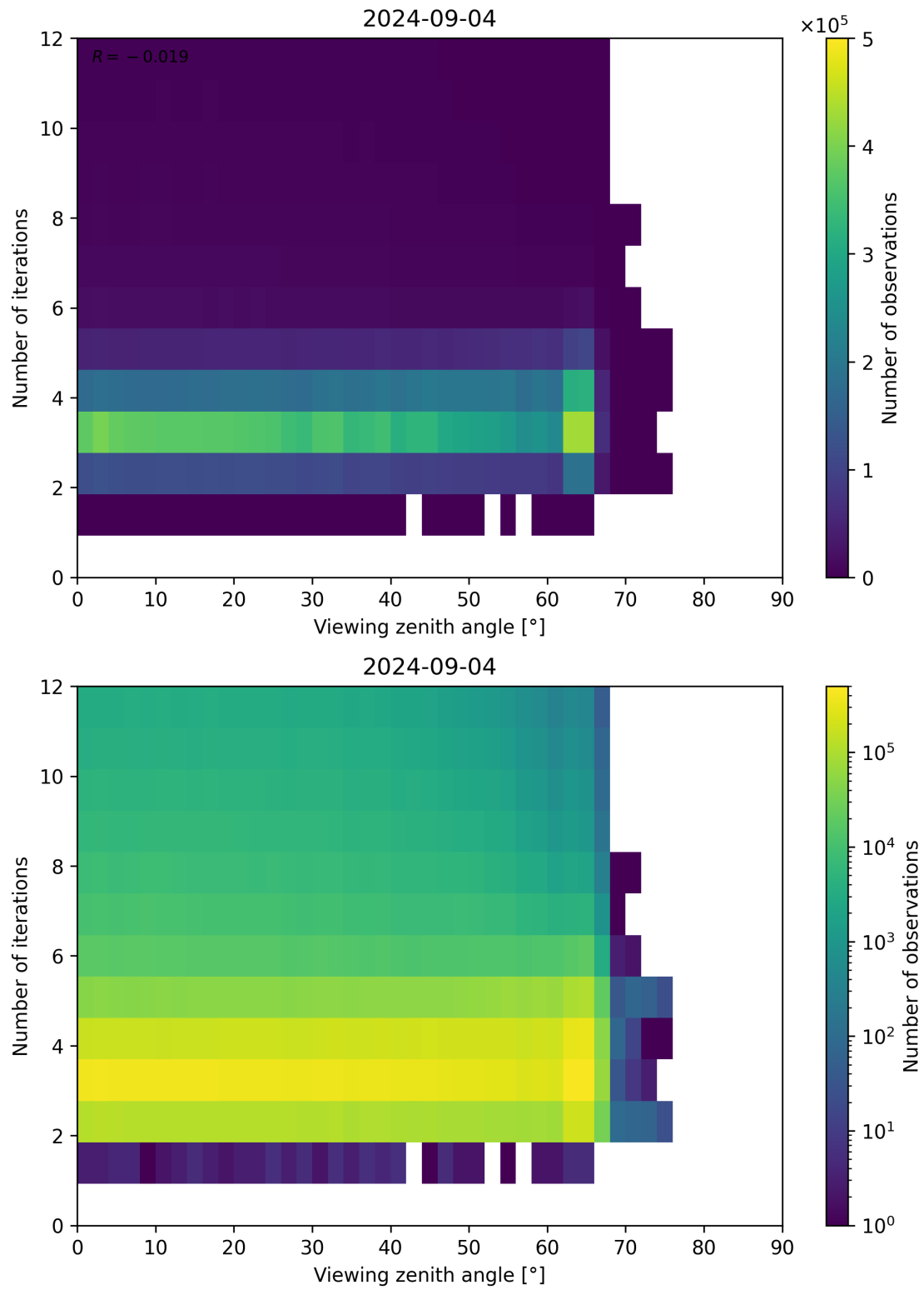
Figure 124: Scatter density plot of “Viewing zenith angle” against “Number of iterations” for 2024-09-03 to 2024-09-05.
