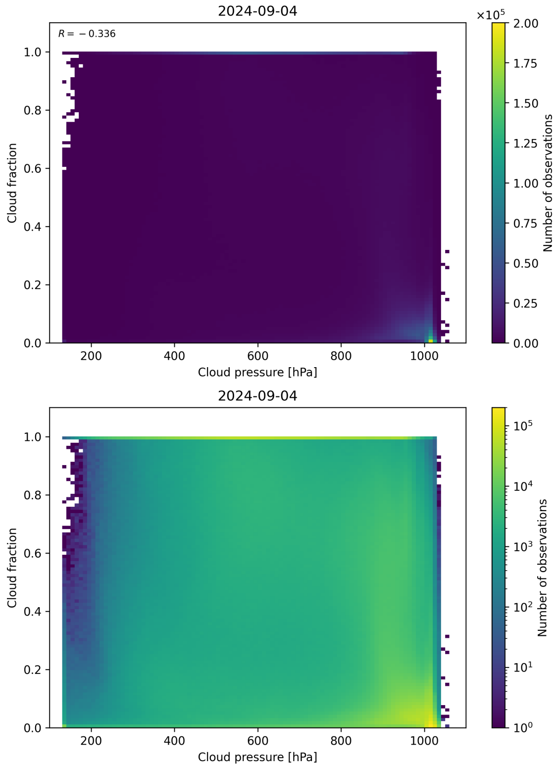
Figure 79: Scatter density plot of “Cloud pressure” against “Cloud fraction” for 2024-09-03 to 2024-09-05.
