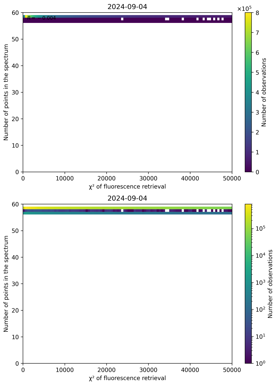
Figure 68: Scatter density plot of " \chi^2 of fluorescence retrieval" against "Number of points in the spectrum" for 2024-09-03 to 2024-09-05.
