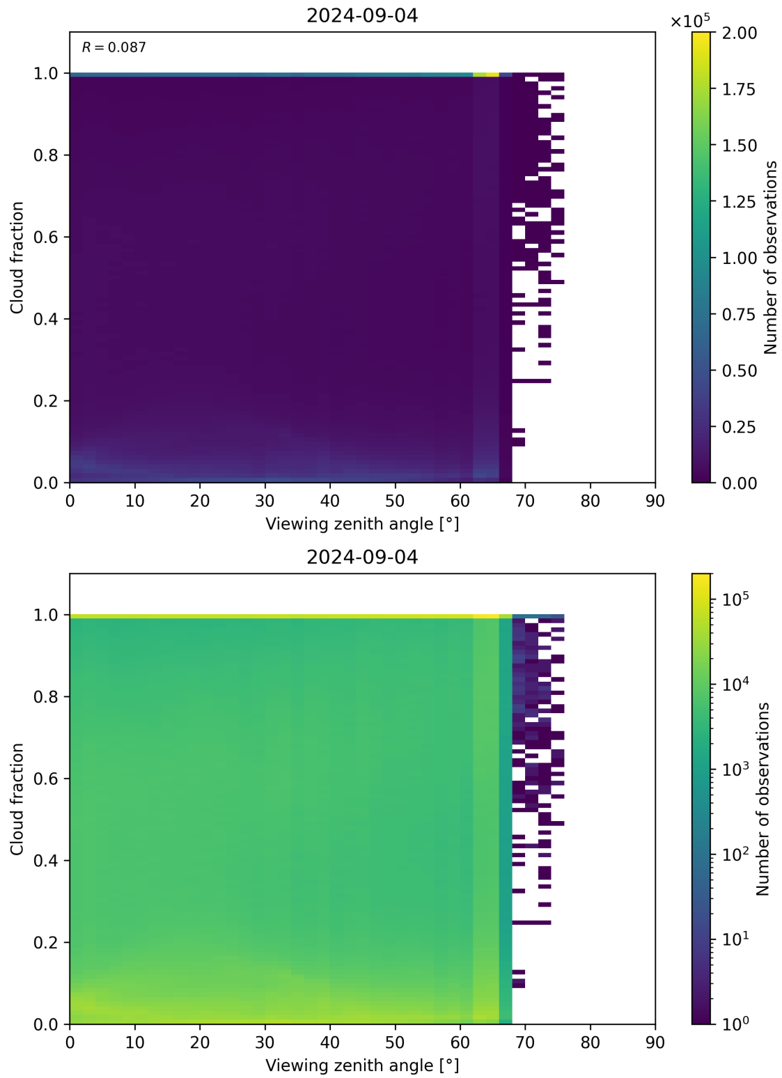
Figure 120: Scatter density plot of “Viewing zenith angle” against “Cloud fraction” for 2024-09-03 to 2024-09-05.
