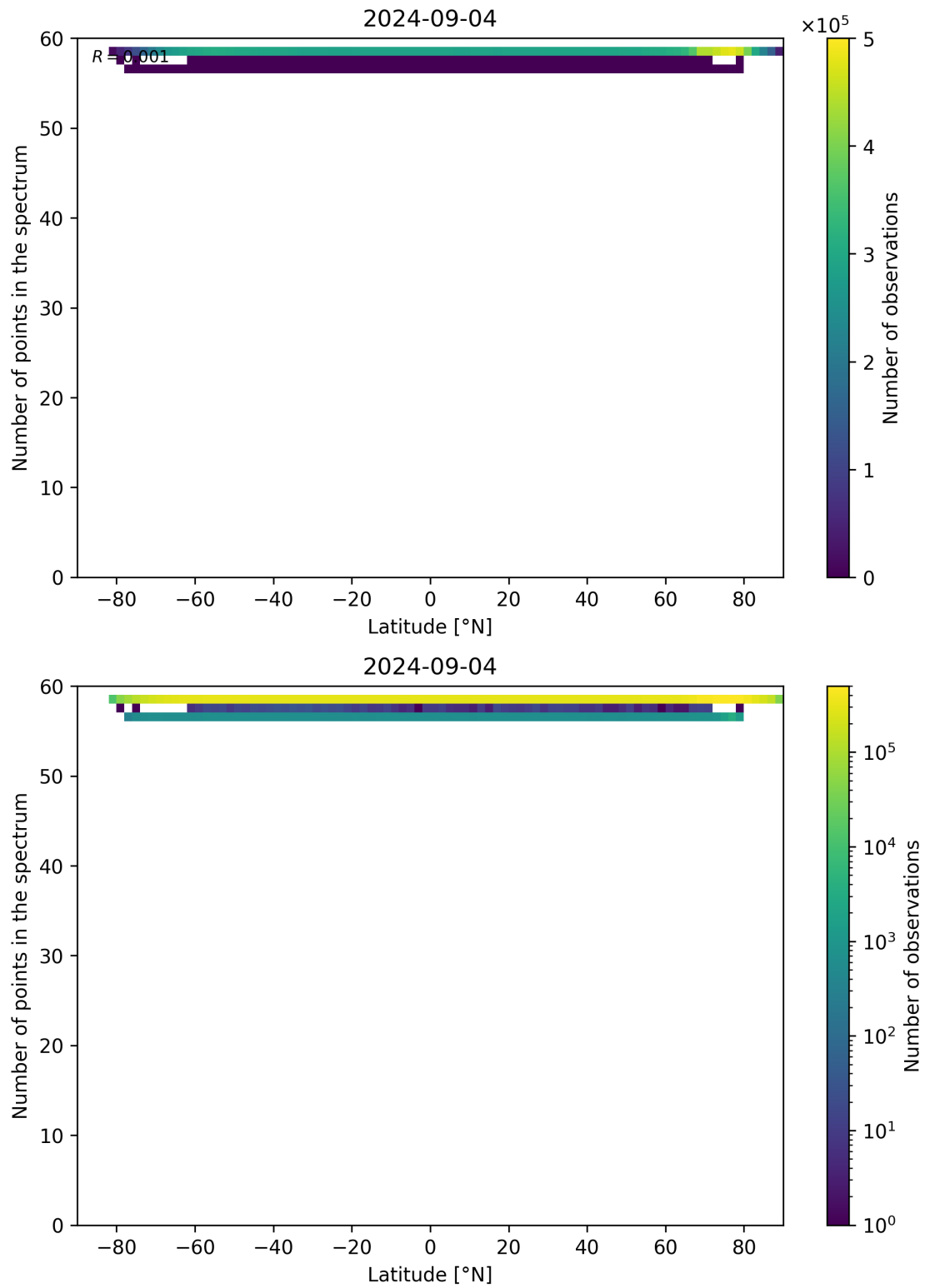
Figure 94: Scatter density plot of “Latitude” against “Number of points in the spectrum” for 2024-09-03 to 2024-09-05.
