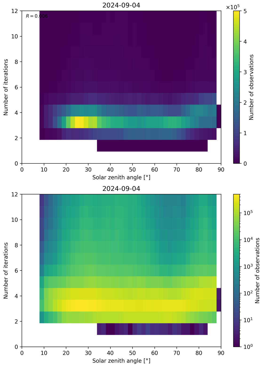
Figure 114: Scatter density plot of “Solar zenith angle” against “Number of iterations” for 2024-09-03 to 2024-09-05.
