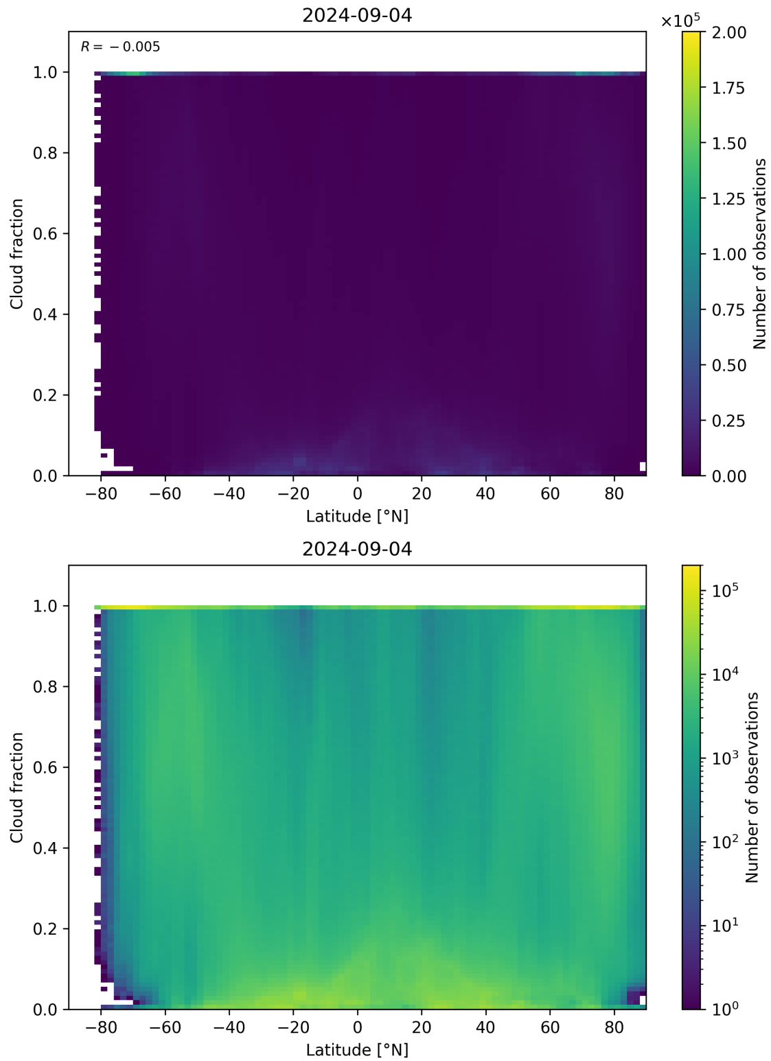
Figure 90: Scatter density plot of “Latitude” against “Cloud fraction” for 2024-09-03 to 2024-09-05.
