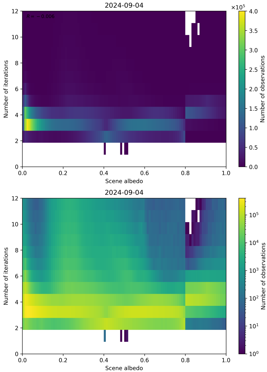
Figure 105: Scatter density plot of “Scene albedo” against “Number of iterations” for 2024-09-03 to 2024-09-05.
