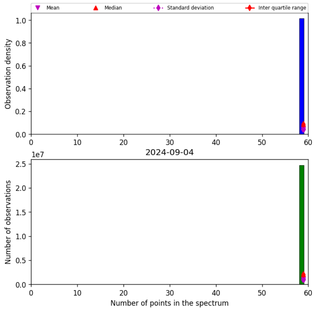
Figure 44: Histogram of “Number of points in the spectrum” for 2024-09-03 to 2024-09-05
