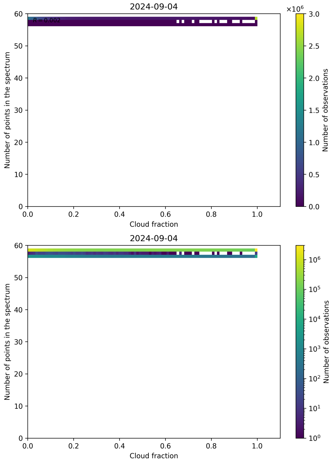
Figure 74: Scatter density plot of “Cloud fraction” against “Number of points in the spectrum” for 2024-09-03 to 2024-09-05.
