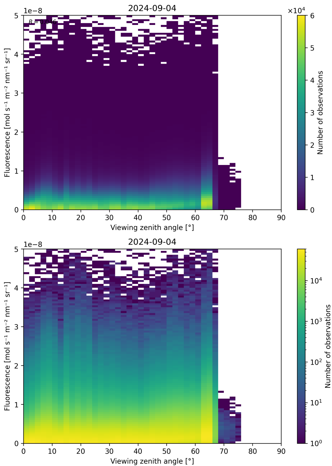
Figure 122: Scatter density plot of “Viewing zenith angle” against “Fluorescence” for 2024-09-03 to 2024-09-05.
