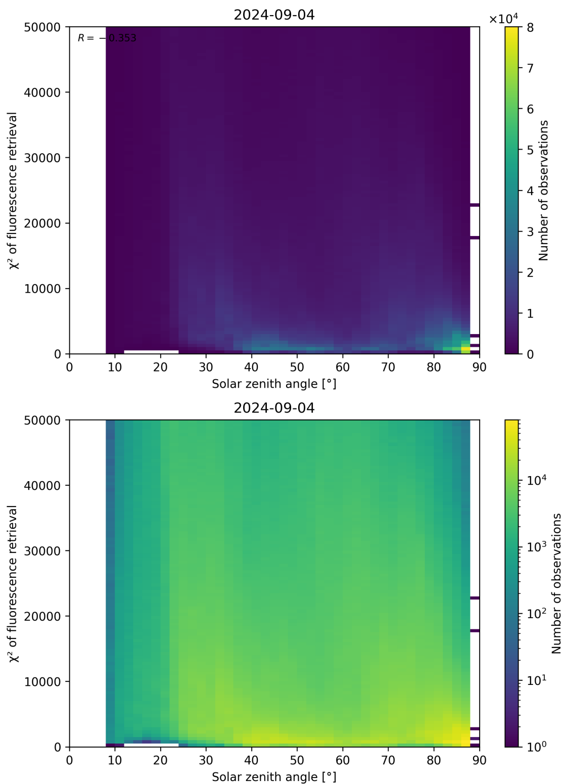
Figure 109: Scatter density plot of “Solar zenith angle” against “ \chi^2 of fluorescence retrieval” for 2024-09-03 to 2024-09-05.
