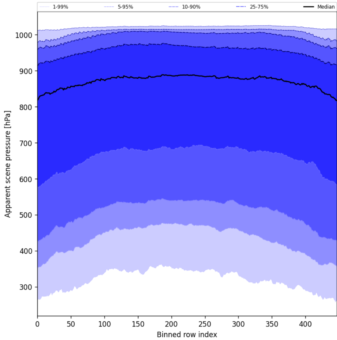
Figure 53: Along track statistics of “Apparent scene pressure” for 2024-09-03 to 2024-09-05
