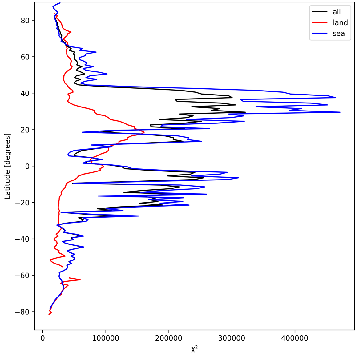
Figure 21: Zonal average of “ \chi^2 ” for 2024-09-03 to 2024-09-05.
