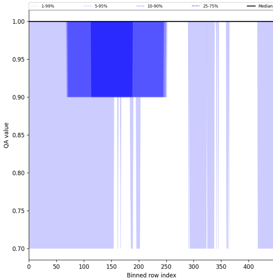
Figure 46: Along track statistics of “QA value” for 2024-09-03 to 2024-09-05
