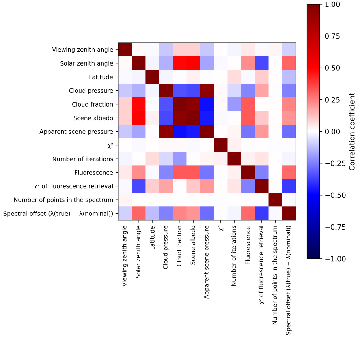
Figure 2: Map of correlation matrix for 2024-09-03 to 2024-09-05.
