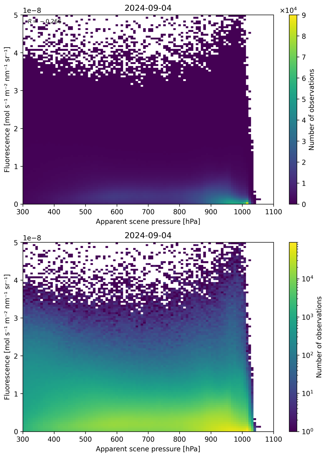
Figure 64: Scatter density plot of “Apparent scene pressure” against “Fluorescence” for 2024-09-03 to 2024-09-05.
