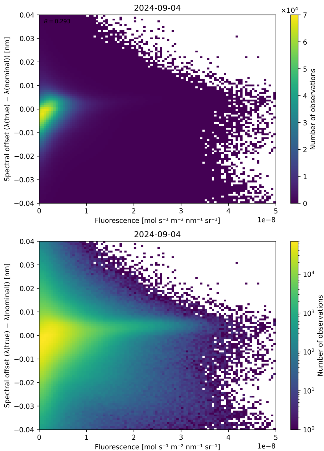
Figure 87: Scatter density plot of “Fluorescence” against “Spectral offset ( \lambda_{\text{true}} - \lambda_{\text{nominal}} )” for 2024-09-03 to 2024-09-05.
