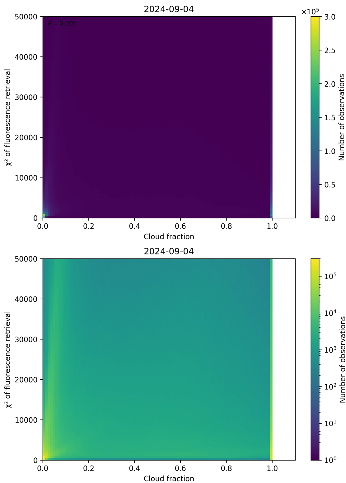
Figure 71: Scatter density plot of “Cloud fraction” against “ \chi^2 of fluorescence retrieval” for 2024-09-03 to 2024-09-05.
