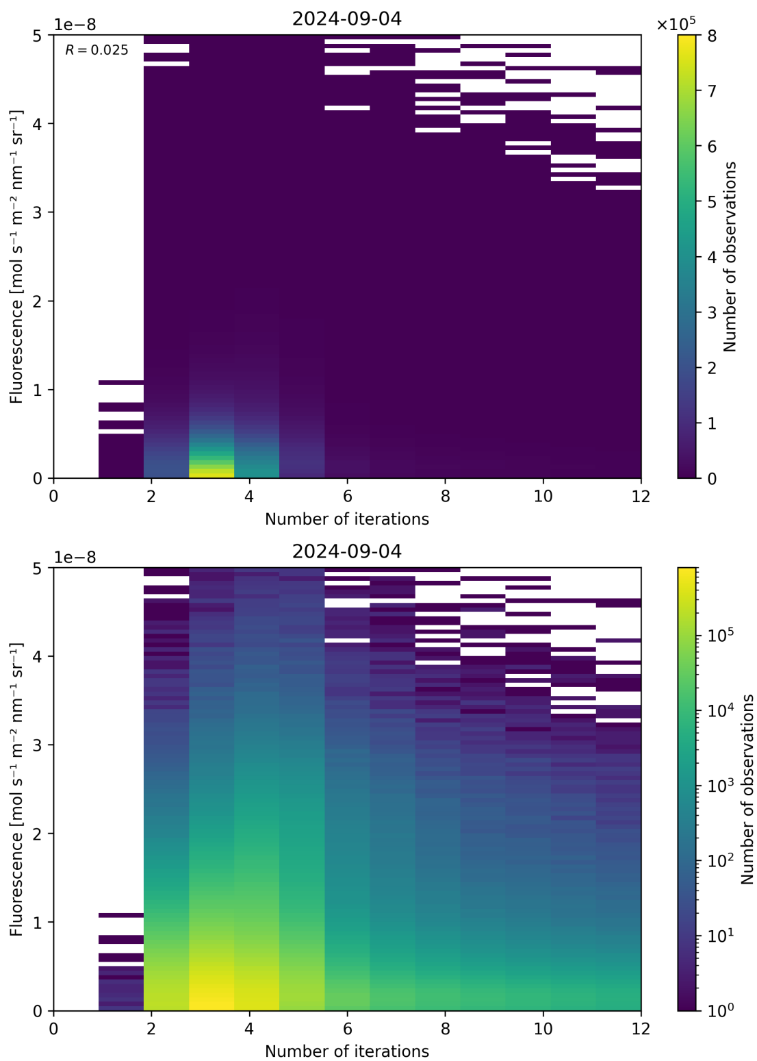
Figure 98: Scatter density plot of “Number of iterations” against “Fluorescence” for 2024-09-03 to 2024-09-05.
