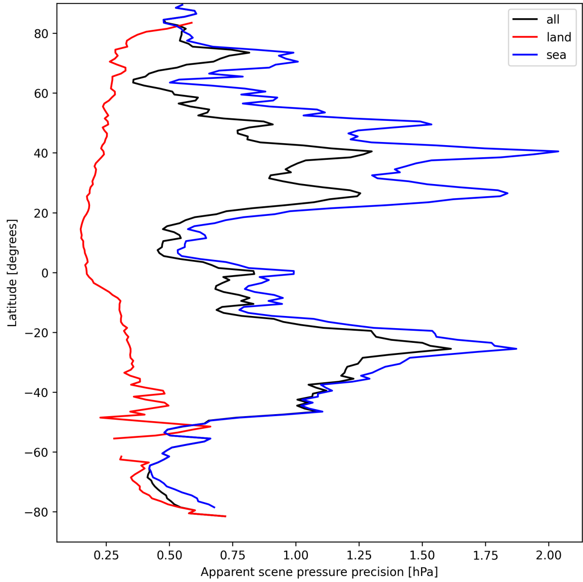
Figure 20: Zonal average of “Apparent scene pressure precision” for 2024-09-03 to 2024-09-05.
