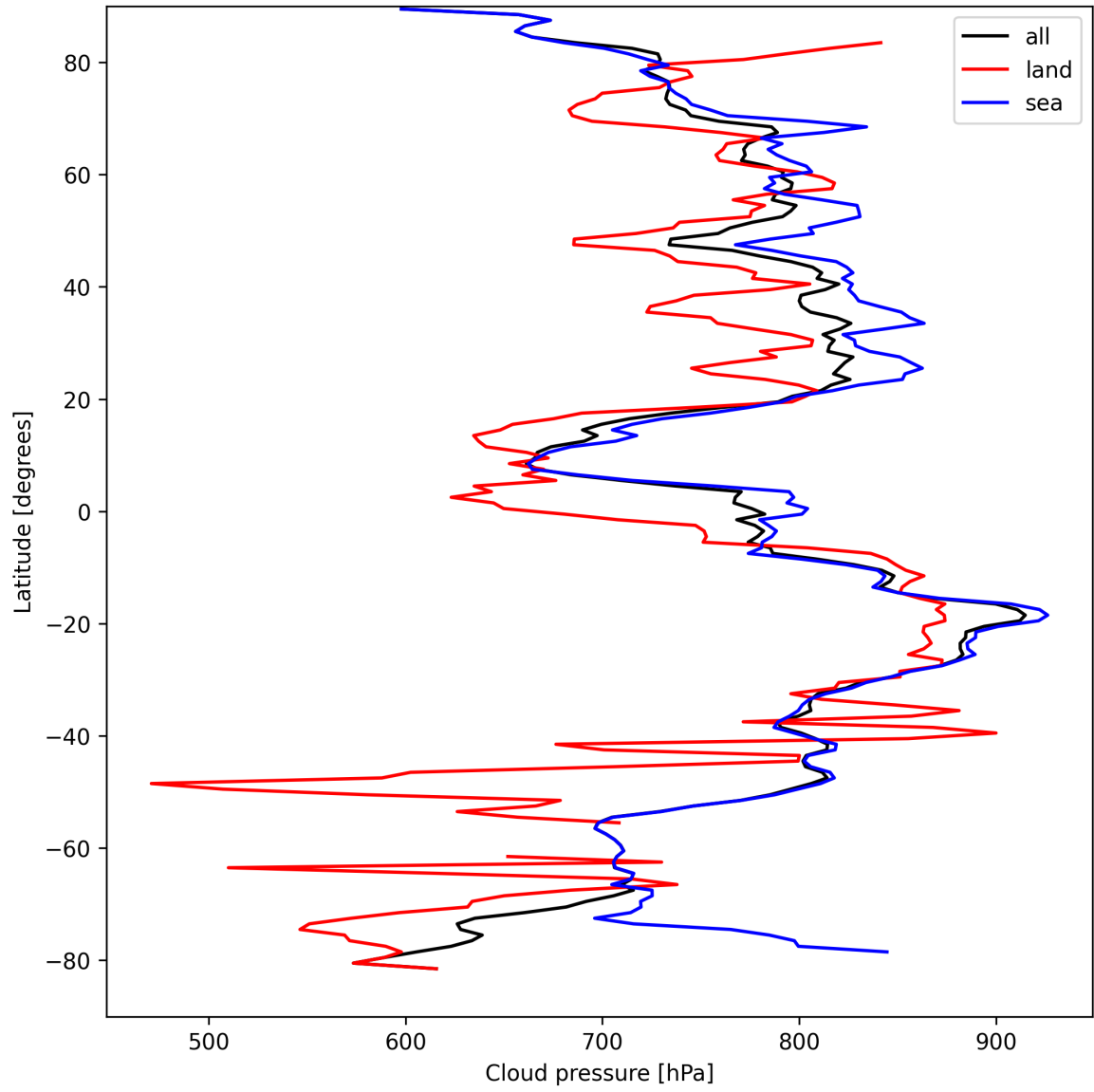
Figure 13: Zonal average of “Cloud pressure” for 2024-09-03 to 2024-09-05.
