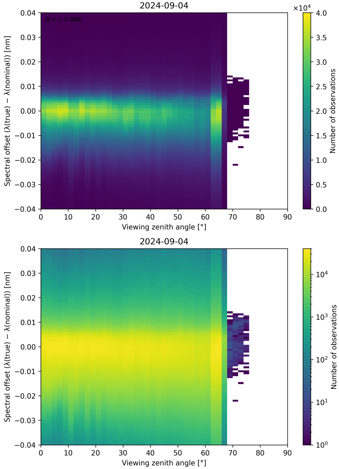
Figure 128: Scatter density plot of “Viewing zenith angle” against “Spectral offset ( \lambda_{\text{true}} - \lambda_{\text{nominal}} )” for 2024-09-03 to 2024-09-05.
