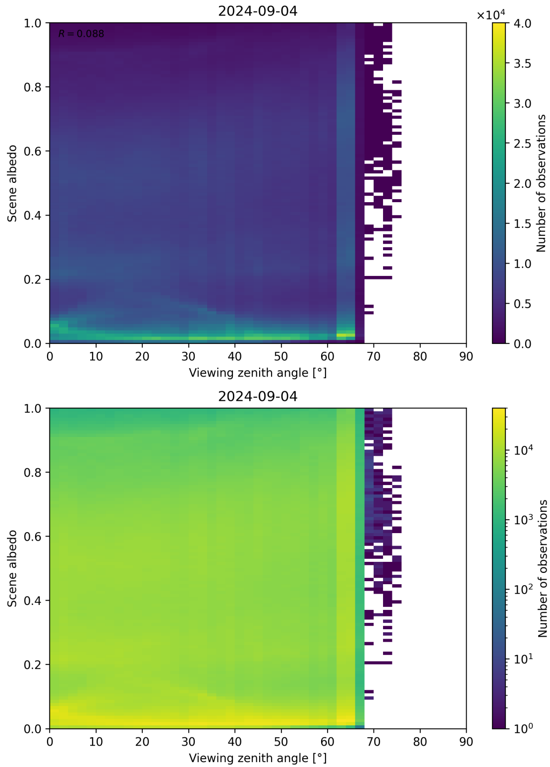
Figure 126: Scatter density plot of “Viewing zenith angle” against “Scene albedo” for 2024-09-03 to 2024-09-05.
