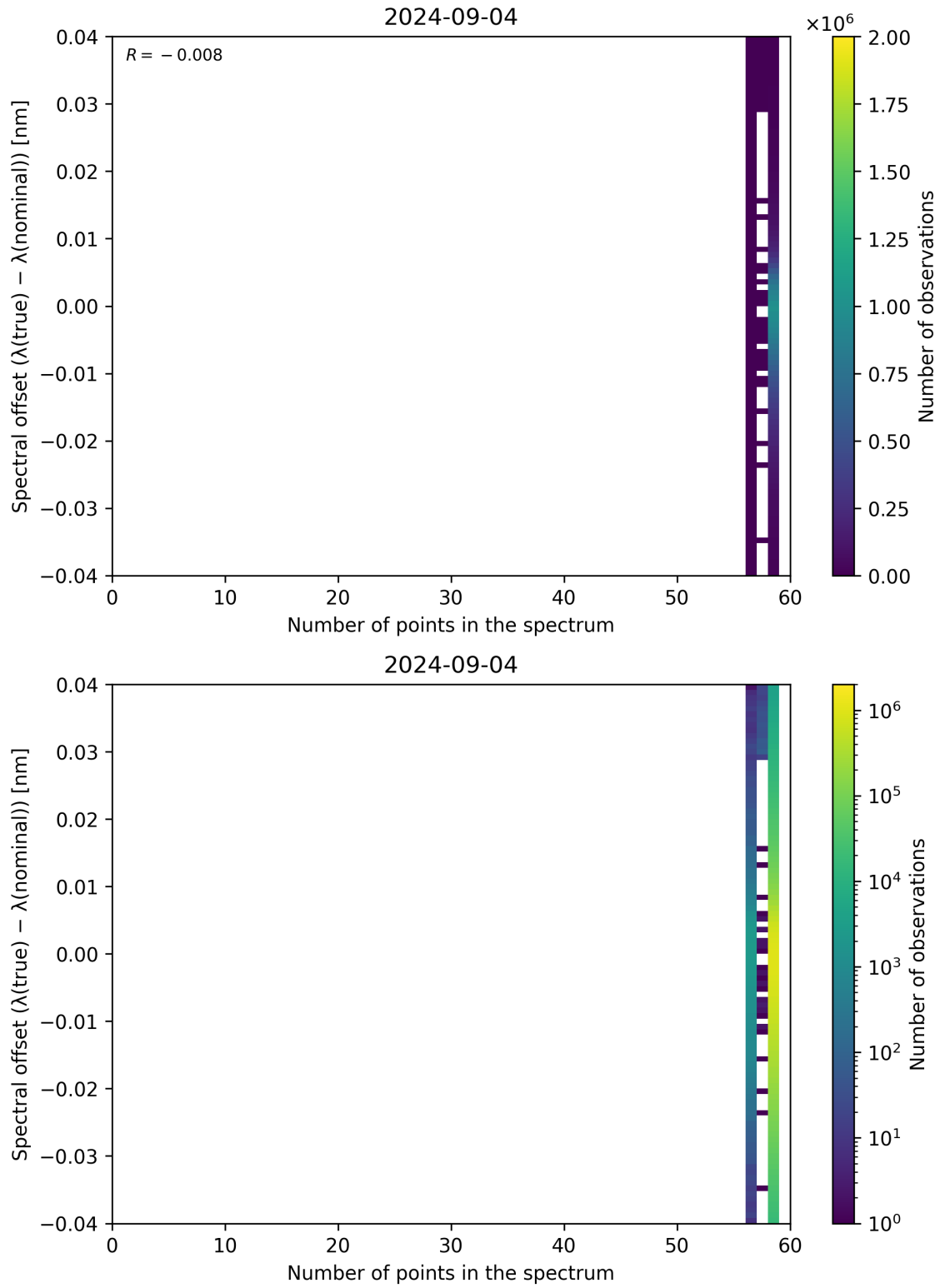
Figure 101: Scatter density plot of “Number of points in the spectrum” against “Spectral offset ( \lambda_{\text{true}} - \lambda_{\text{nominal}} )” for 2024-09-03 to 2024-09-05.
