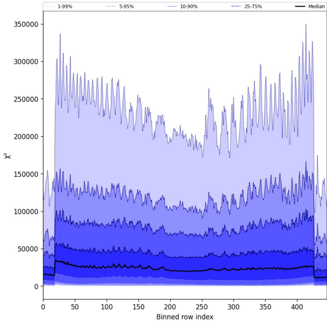
Figure 55: Along track statistics of “ \chi^2 ” for 2024-09-03 to 2024-09-05
