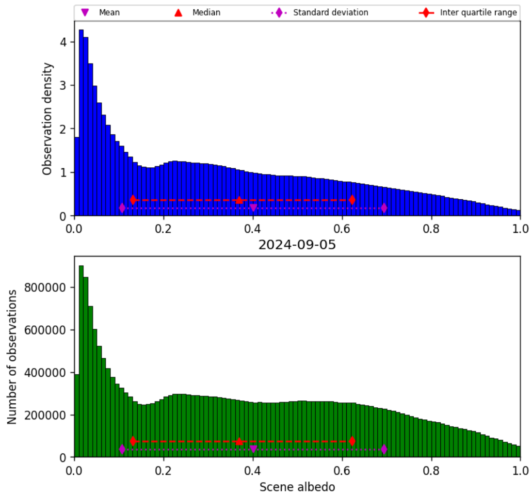
Figure 34: Histogram of “Scene albedo” for 2024-09-04 to 2024-09-06
