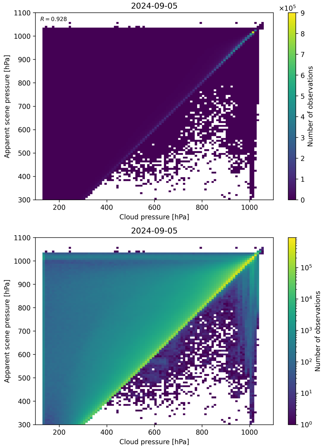
Figure 77: Scatter density plot of “Cloud pressure” against “Apparent scene pressure” for 2024-09-04 to 2024-09-06.
