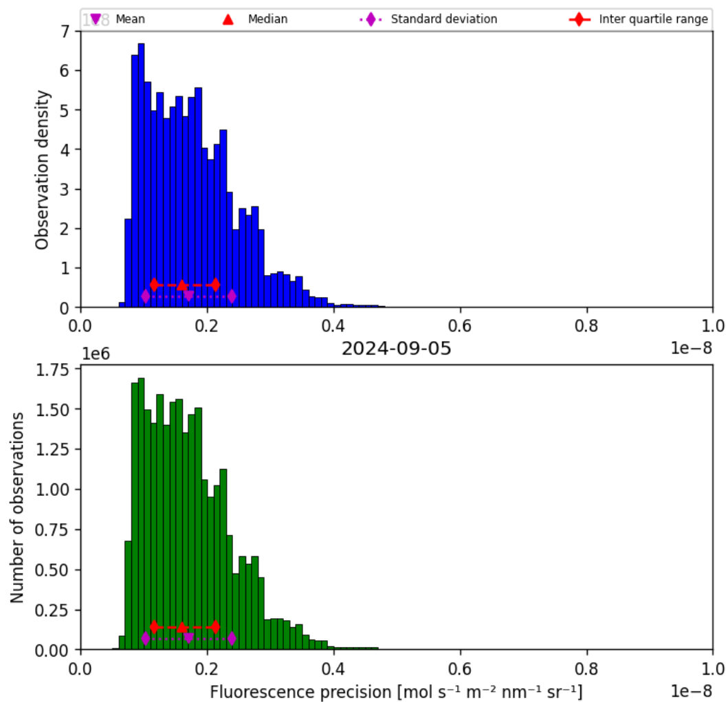
Figure 41: Histogram of “Fluorescence precision” for 2024-09-04 to 2024-09-06
