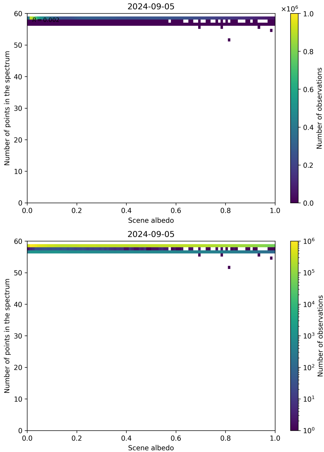
Figure 106: Scatter density plot of “Scene albedo” against “Number of points in the spectrum” for 2024-09-04 to 2024-09-06.
