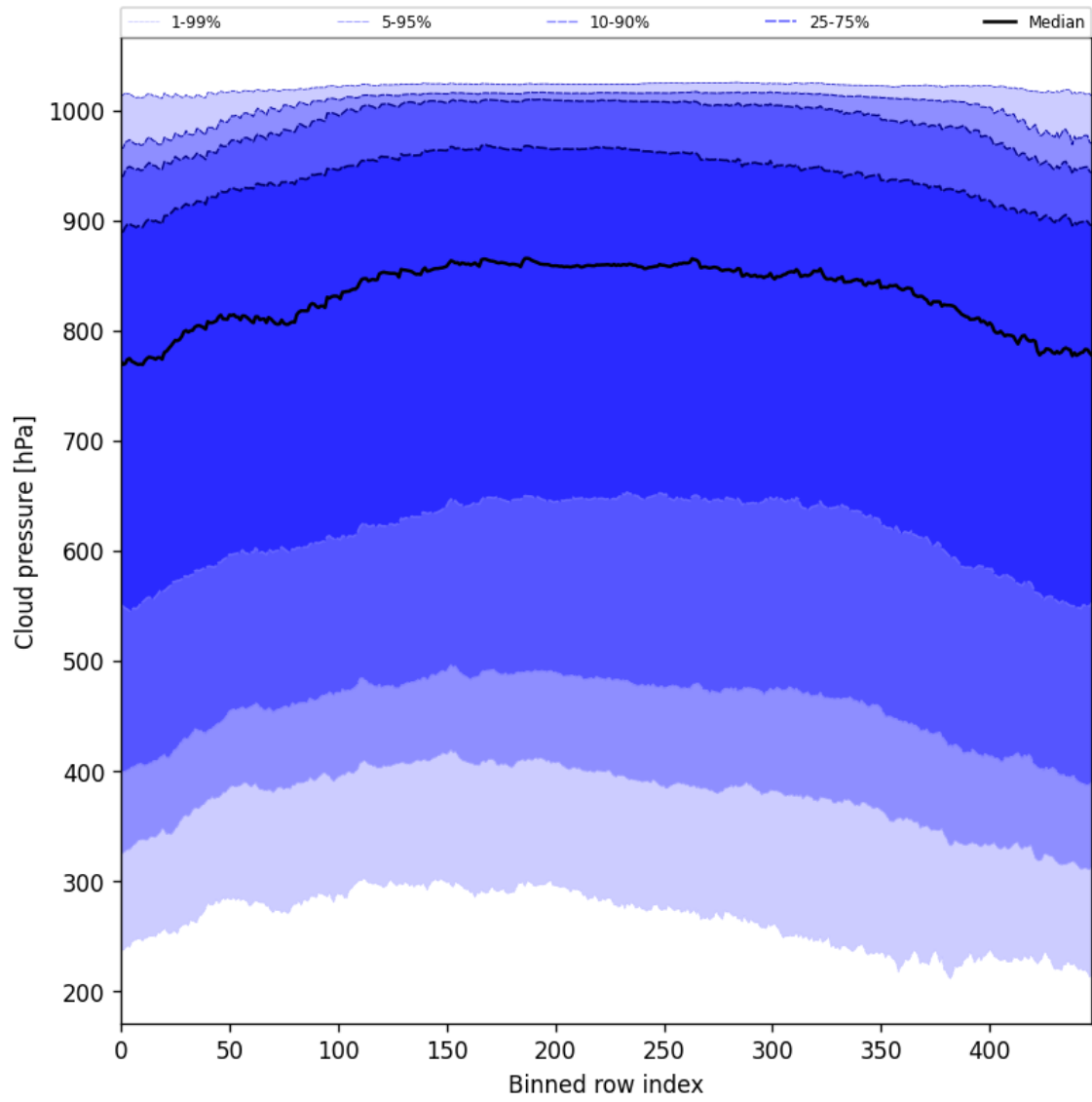
Figure 47: Along track statistics of “Cloud pressure” for 2024-09-04 to 2024-09-06
