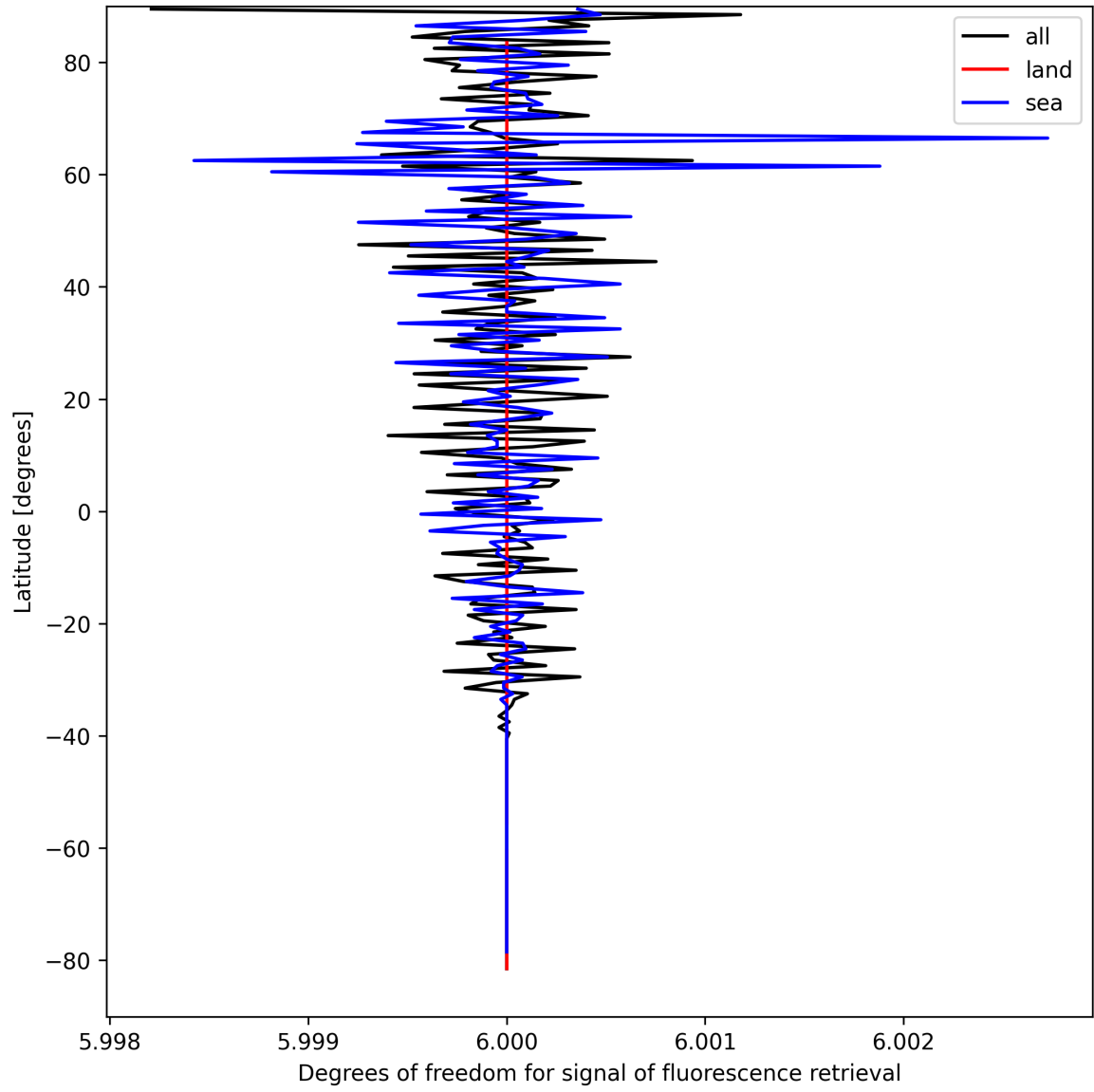
Figure 26: Zonal average of “Degrees of freedom for signal of fluorescence retrieval” for 2024-09-04 to 2024-09-06.
