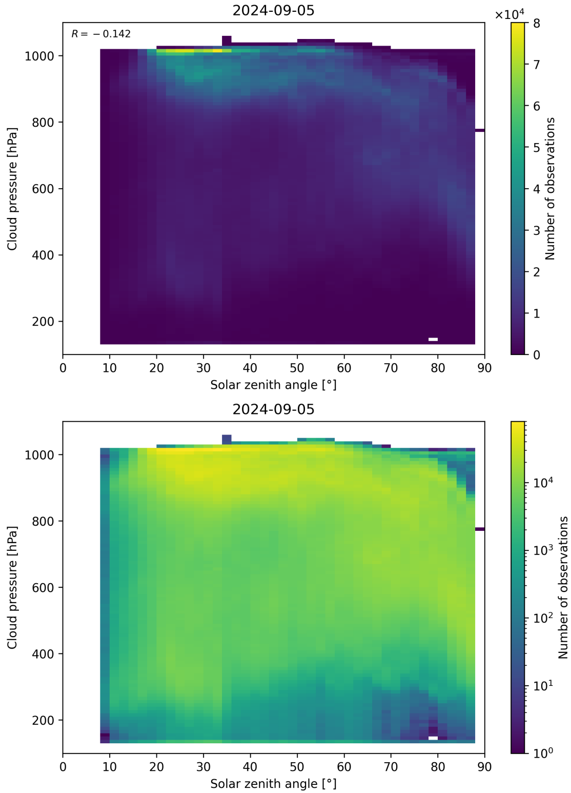
Figure 111: Scatter density plot of “Solar zenith angle” against “Cloud pressure” for 2024-09-04 to 2024-09-06.
