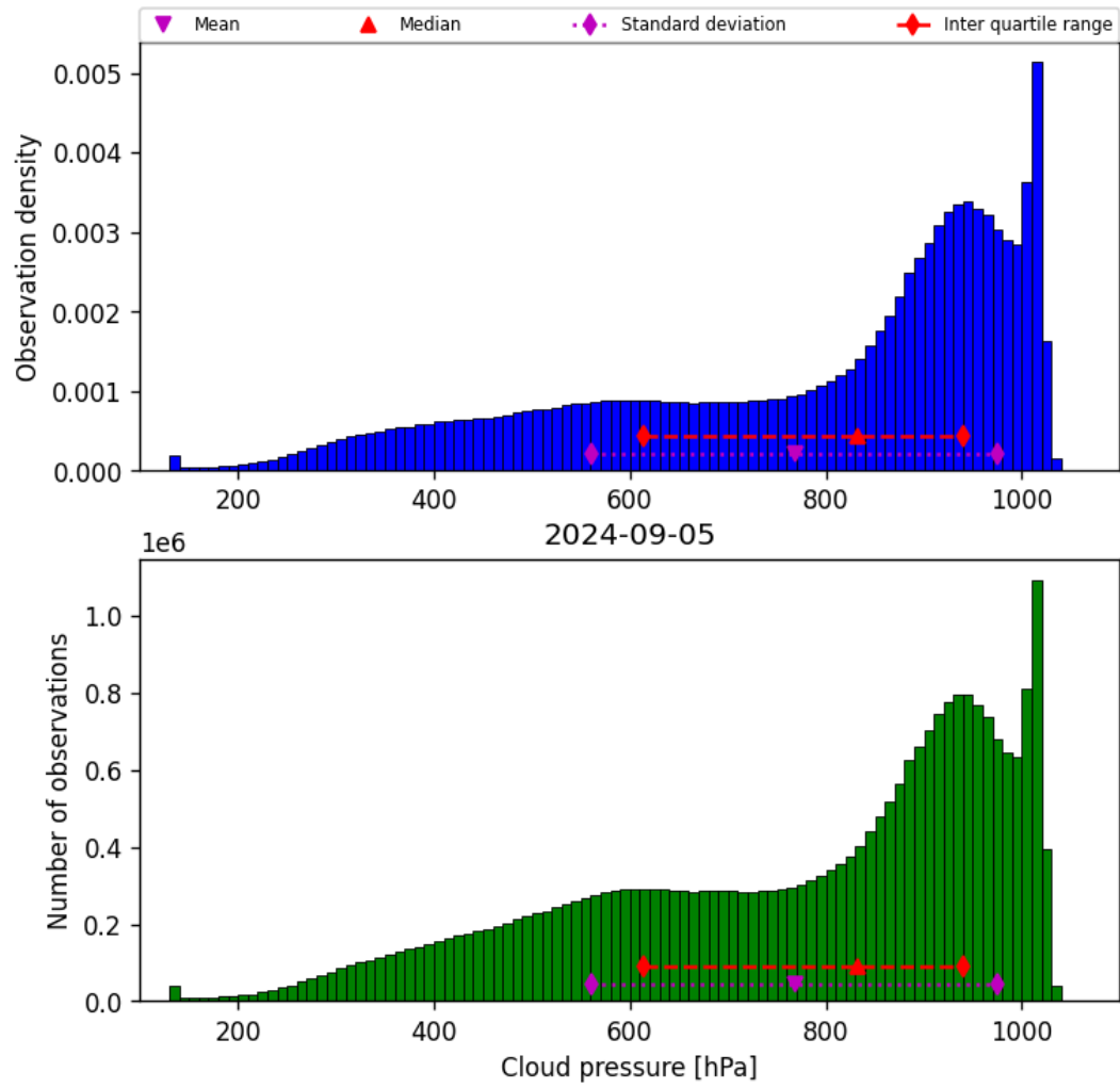
Figure 30: Histogram of “Cloud pressure” for 2024-09-04 to 2024-09-06
