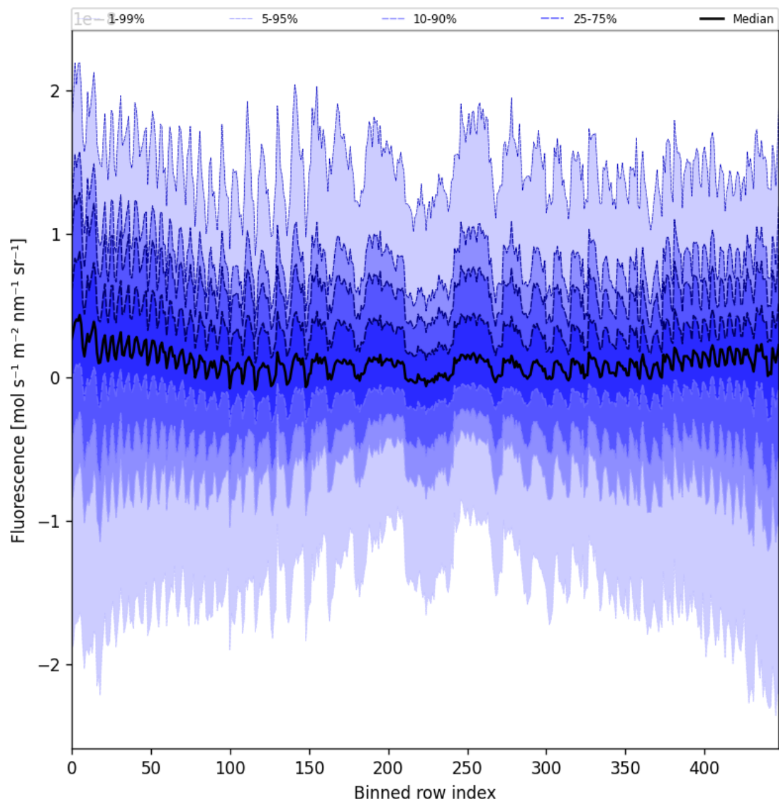
Figure 57: Along track statistics of “Fluorescence” for 2024-09-04 to 2024-09-06
