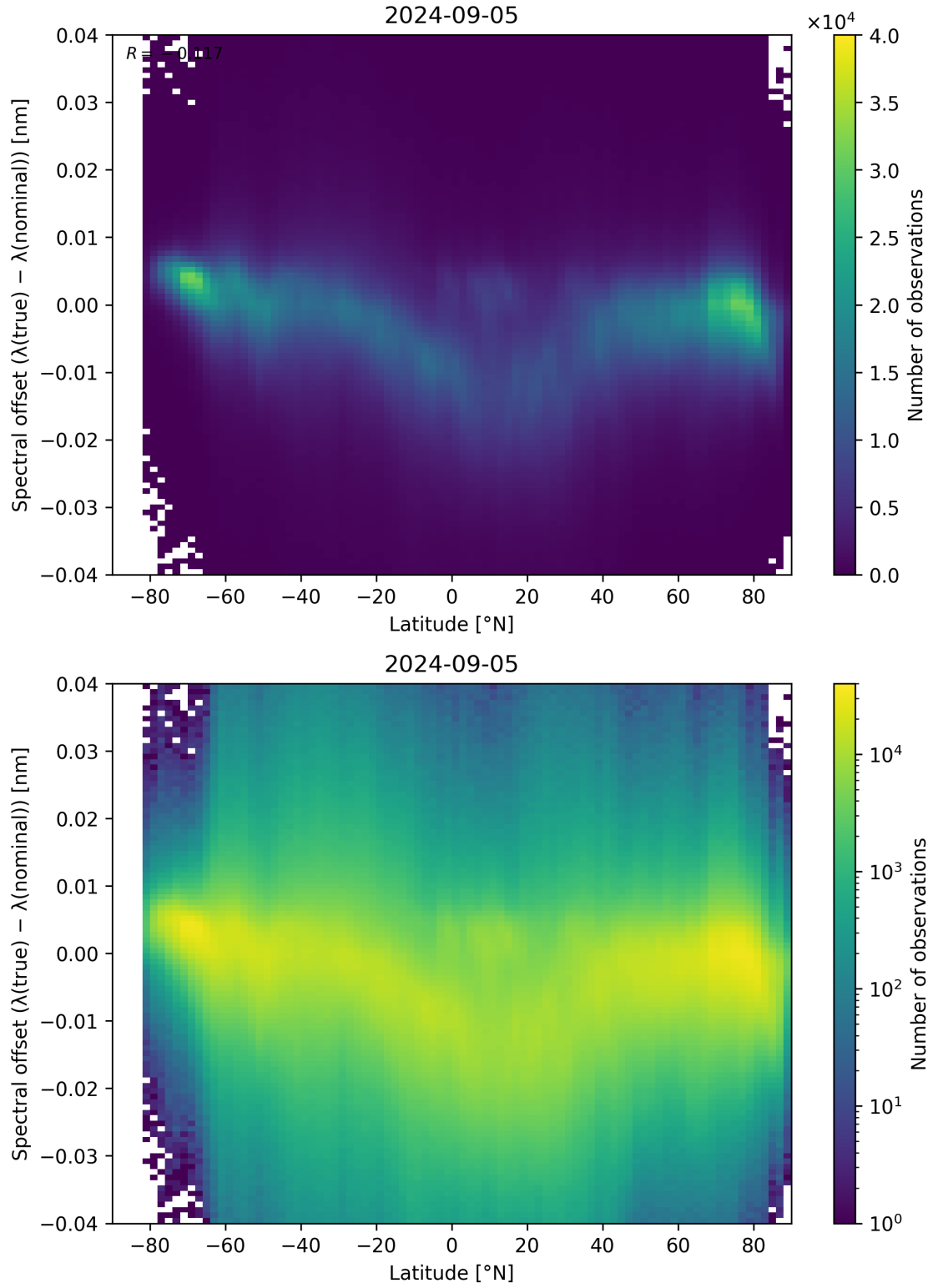
Figure 96: Scatter density plot of “Latitude” against “Spectral offset ( \lambda_{\text{true}} - \lambda_{\text{nominal}} )” for 2024-09-04 to 2024-09-06.
