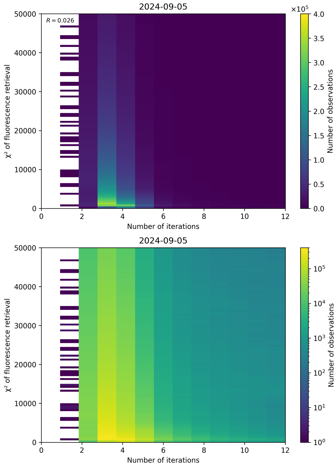
Figure 97: Scatter density plot of “Number of iterations” against “ \chi^2 of fluorescence retrieval” for 2024-09-04 to 2024-09-06.
