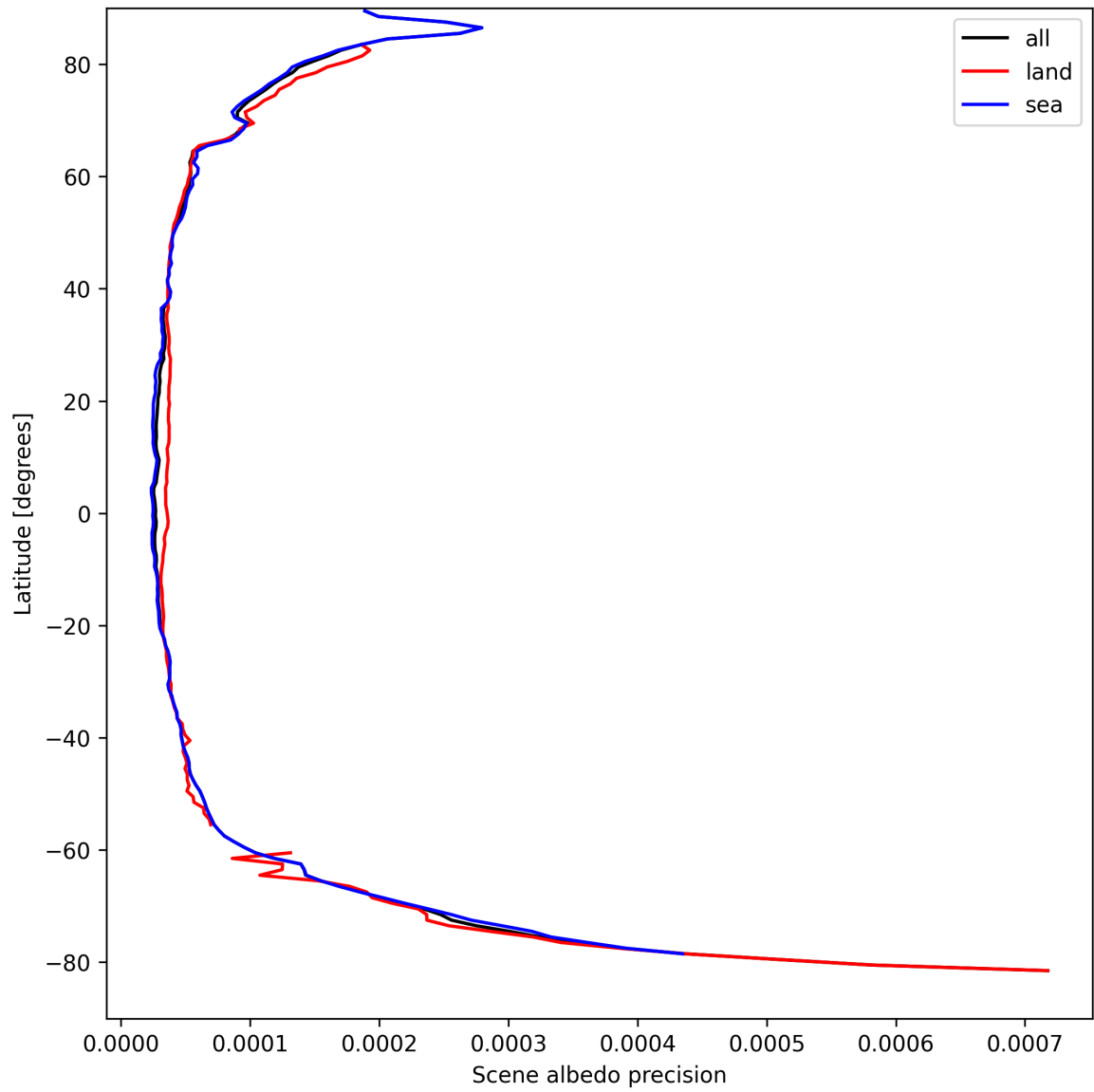
Figure 18: Zonal average of “Scene albedo precision” for 2024-09-04 to 2024-09-06.
