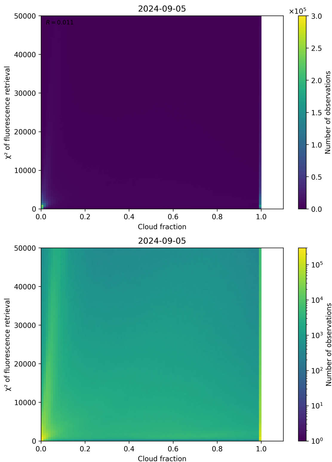
Figure 71: Scatter density plot of “Cloud fraction” against “ \chi^2 of fluorescence retrieval” for 2024-09-04 to 2024-09-06.
