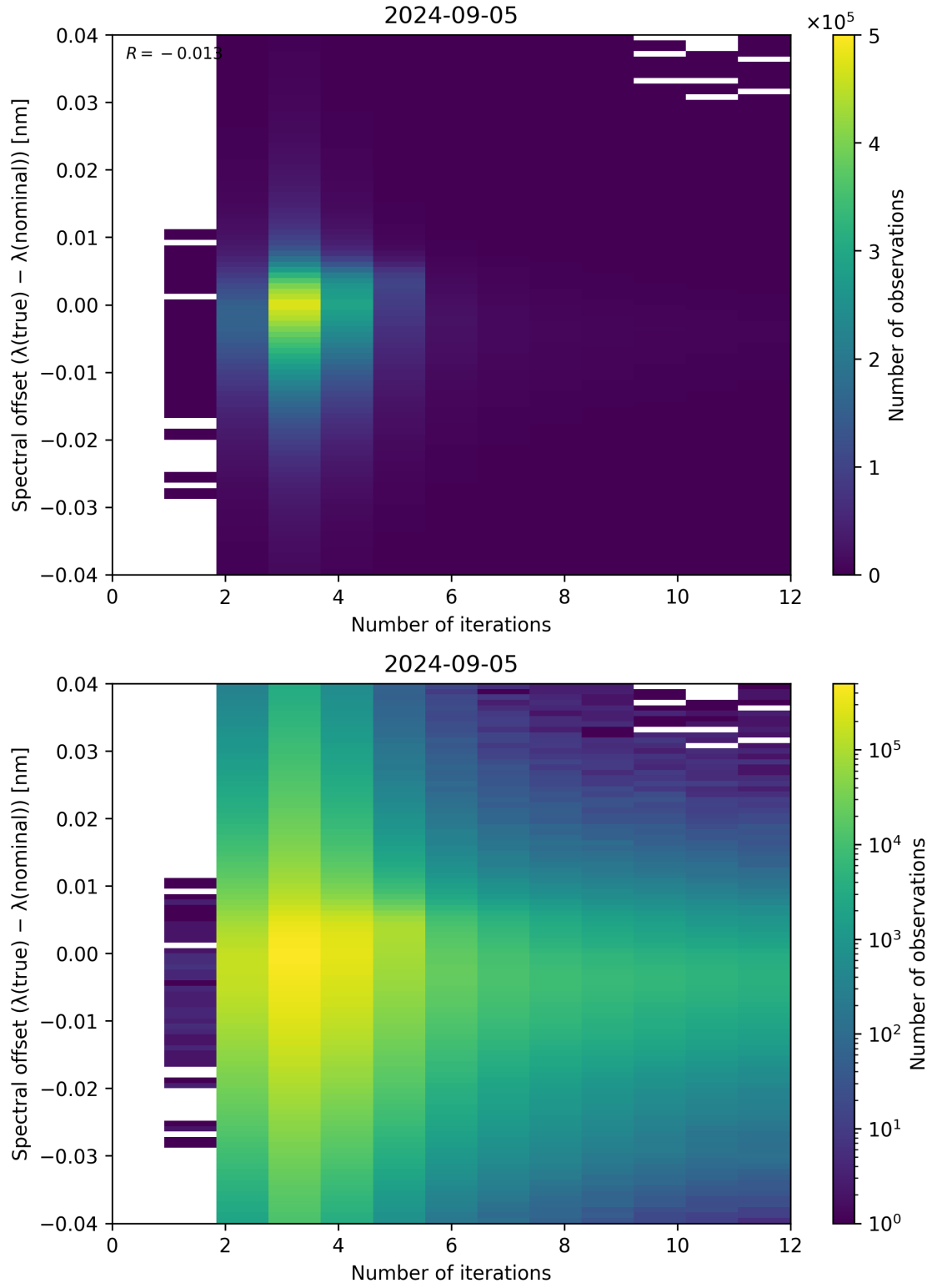
Figure 100: Scatter density plot of “Number of iterations” against “Spectral offset ( \lambda_{\text{true}} - \lambda_{\text{nominal}} )” for 2024-09-04 to 2024-09-06.
