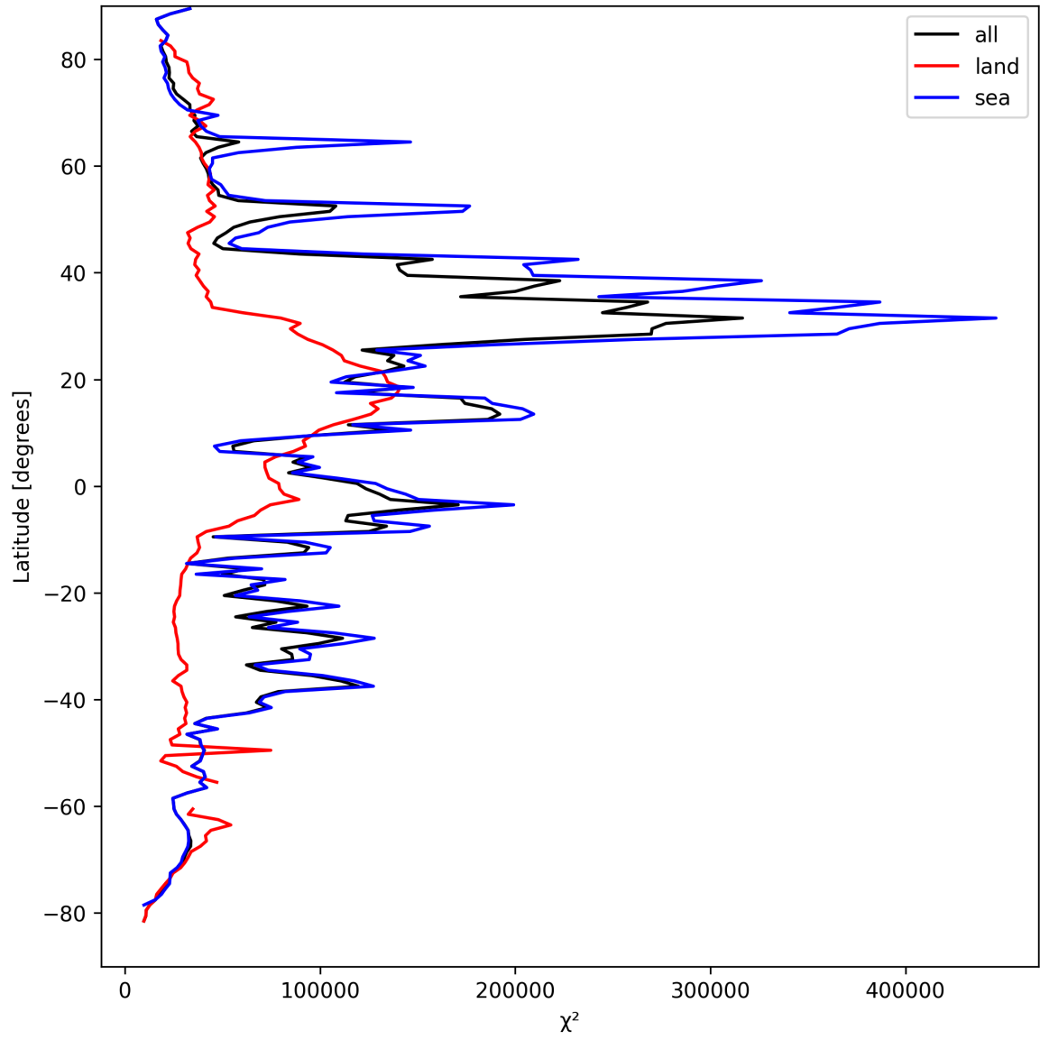
Figure 21: Zonal average of “ \chi^2 ” for 2024-09-04 to 2024-09-06.
