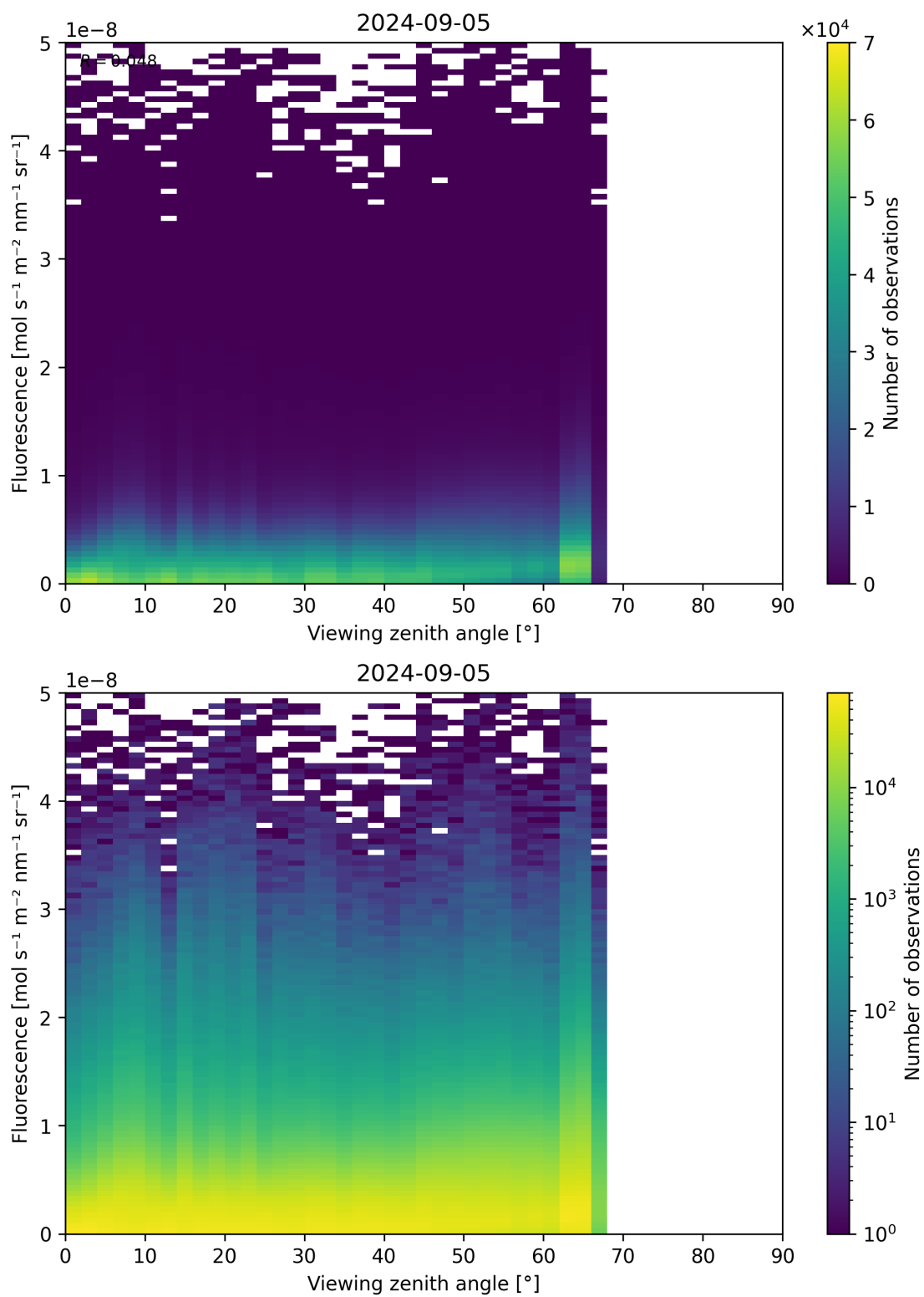
Figure 122: Scatter density plot of “Viewing zenith angle” against “Fluorescence” for 2024-09-04 to 2024-09-06.
