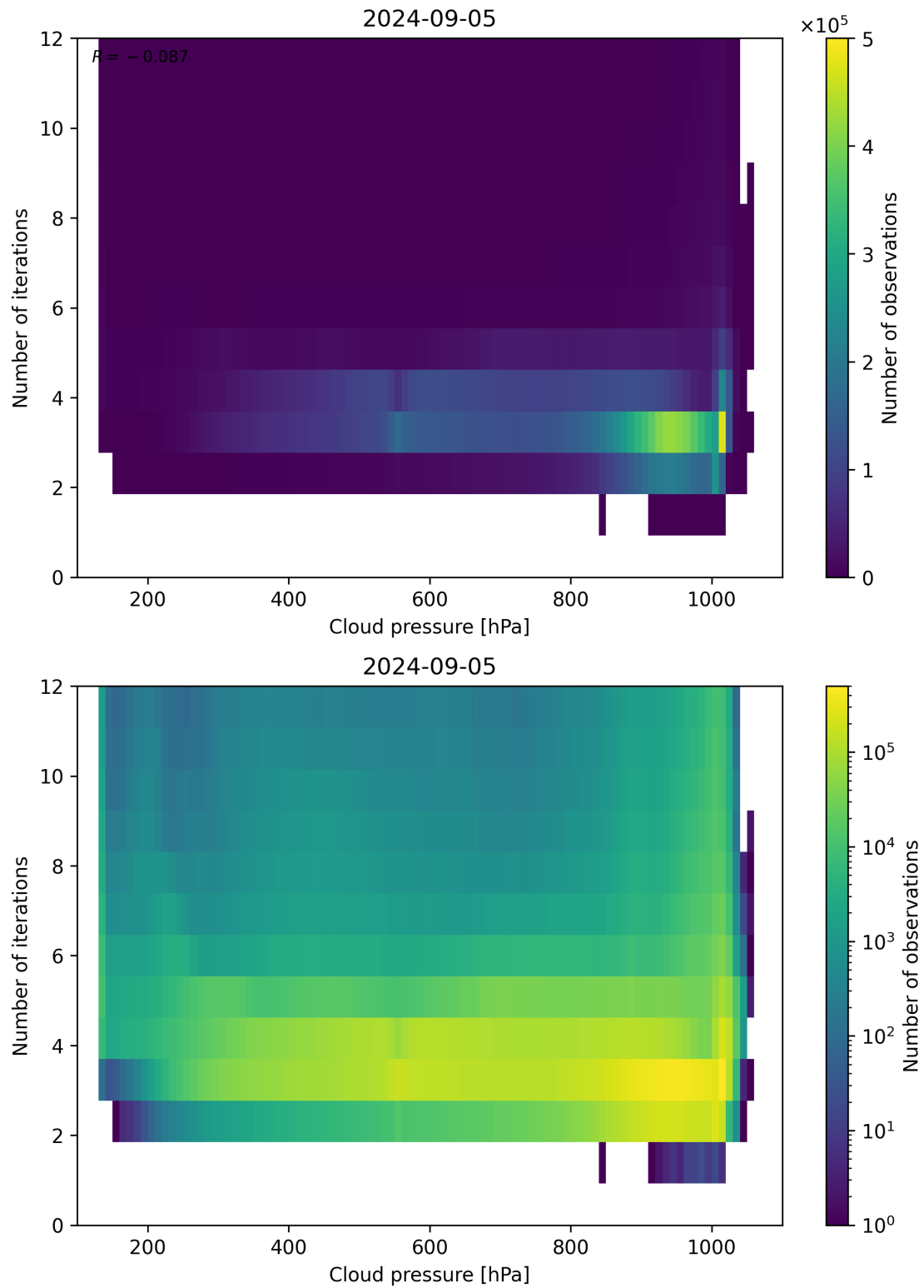
Figure 81: Scatter density plot of “Cloud pressure” against “Number of iterations” for 2024-09-04 to 2024-09-06.
