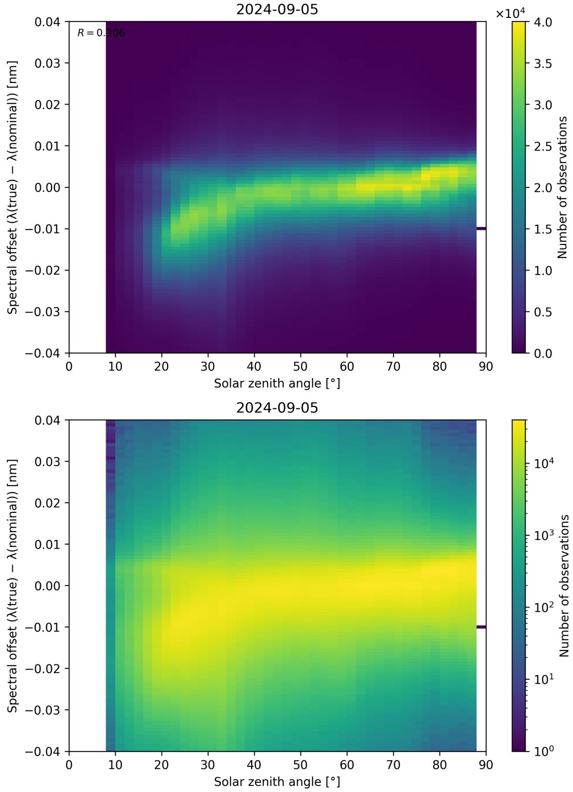
Figure 117: Scatter density plot of “Solar zenith angle” against “Spectral offset ( \lambda_{\text{true}} - \lambda_{\text{nominal}} )” for 2024-09-04 to 2024-09-06.
