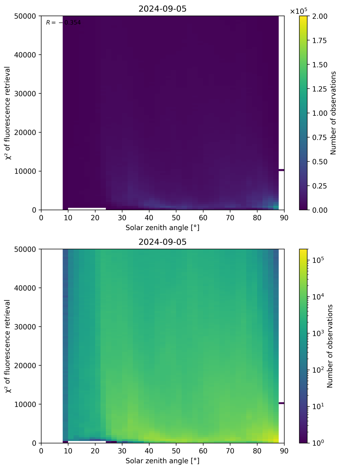
Figure 109: Scatter density plot of “Solar zenith angle” against “ \chi^2 of fluorescence retrieval” for 2024-09-04 to 2024-09-06.
