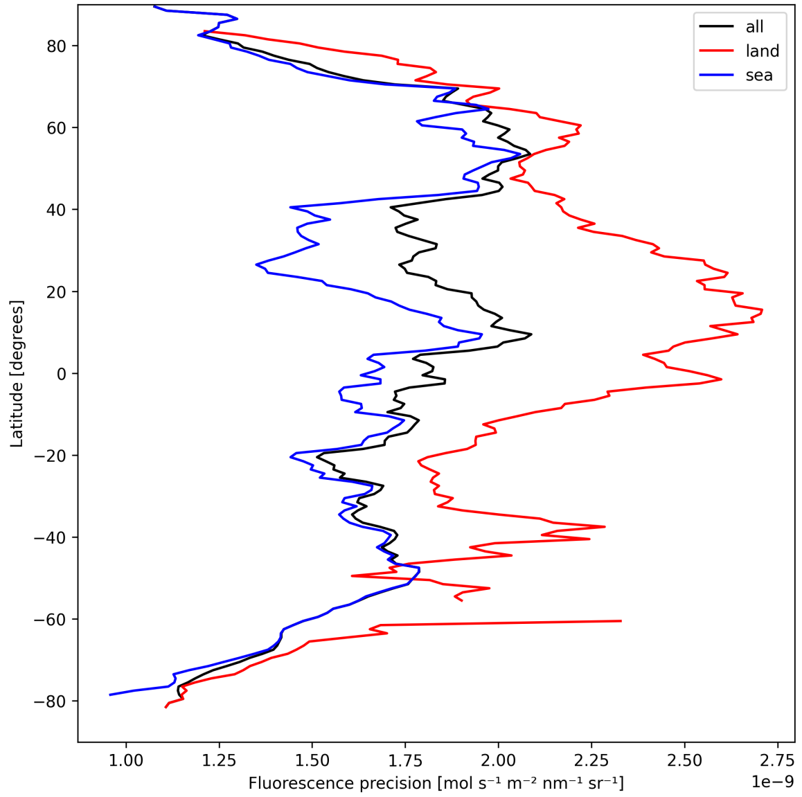
Figure 24: Zonal average of “Fluorescence precision” for 2024-09-04 to 2024-09-06.
