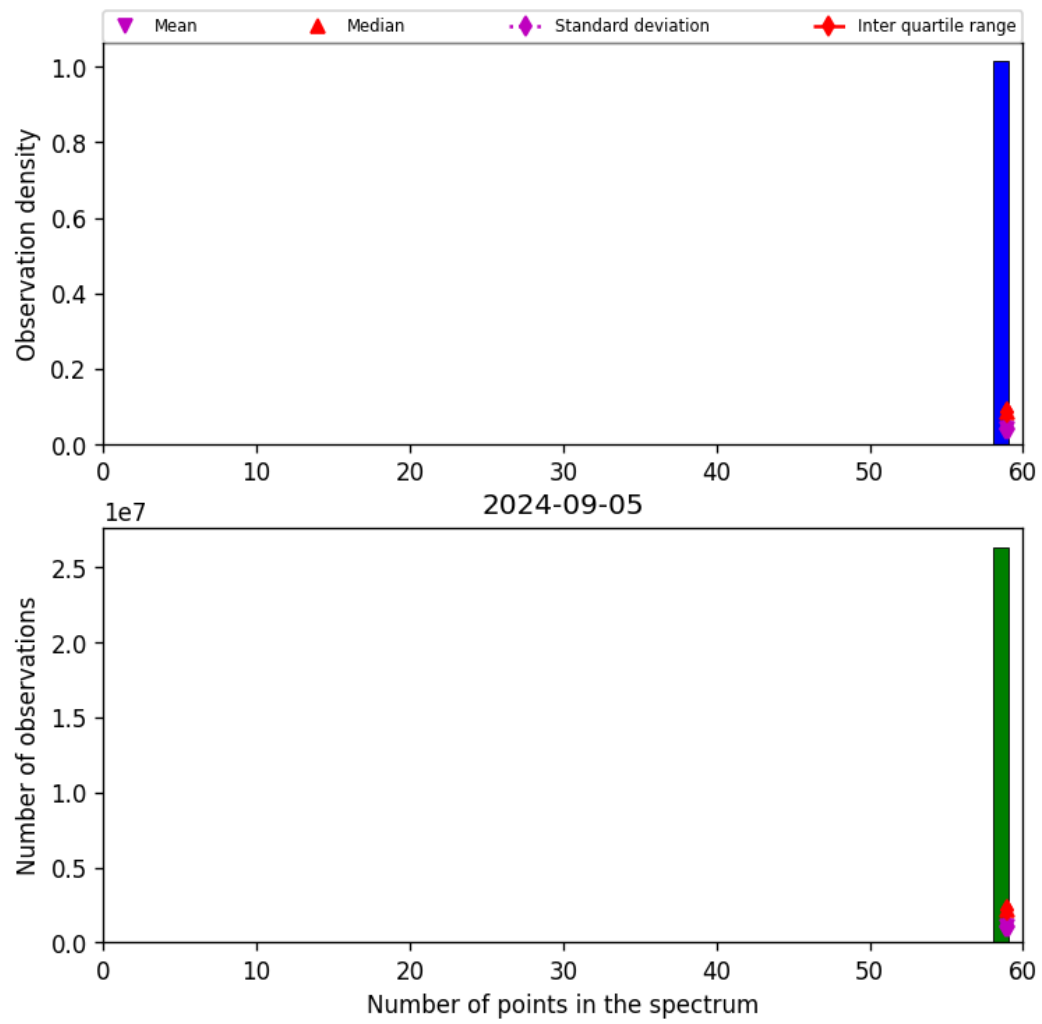
Figure 44: Histogram of “Number of points in the spectrum” for 2024-09-04 to 2024-09-06
