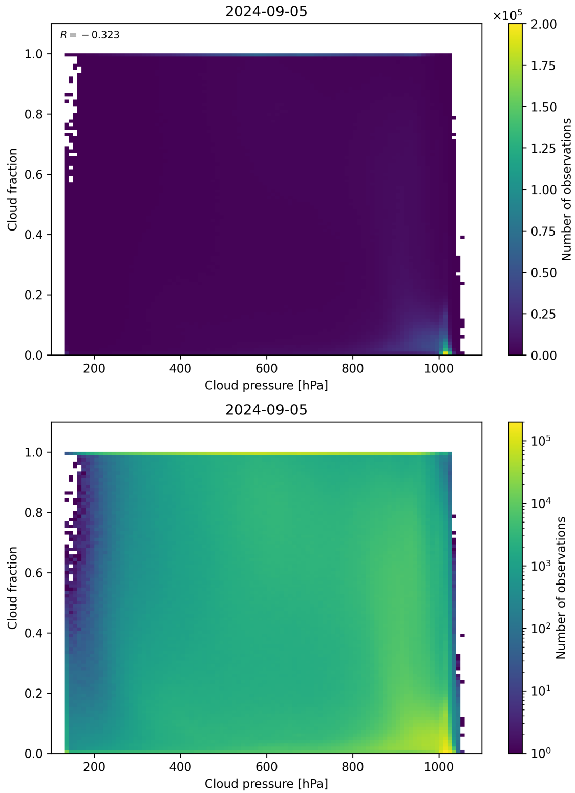
Figure 79: Scatter density plot of “Cloud pressure” against “Cloud fraction” for 2024-09-04 to 2024-09-06.
