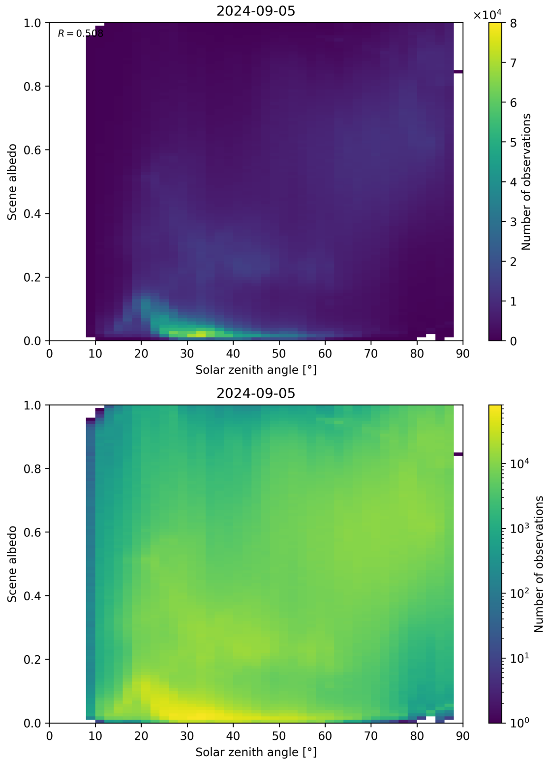
Figure 116: Scatter density plot of “Solar zenith angle” against “Scene albedo” for 2024-09-04 to 2024-09-06.
