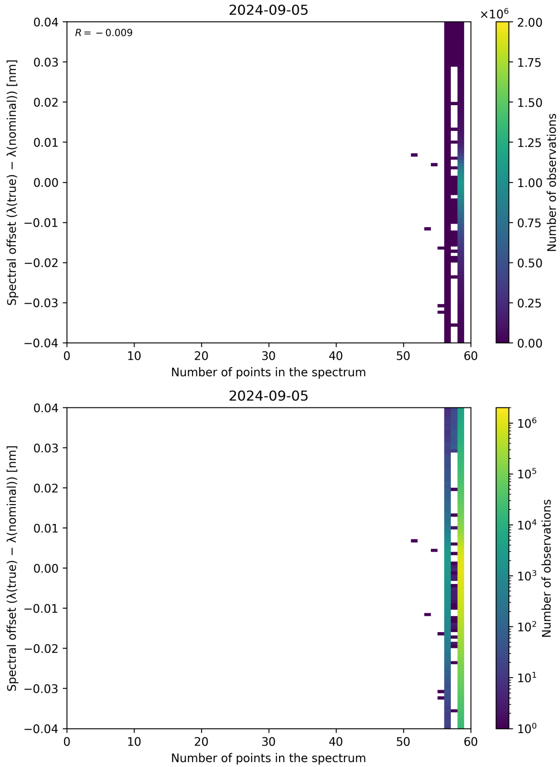
Figure 101: Scatter density plot of “Number of points in the spectrum” against “Spectral offset ( \lambda_{\text{true}} - \lambda_{\text{nominal}} )” for 2024-09-04 to 2024-09-06.
