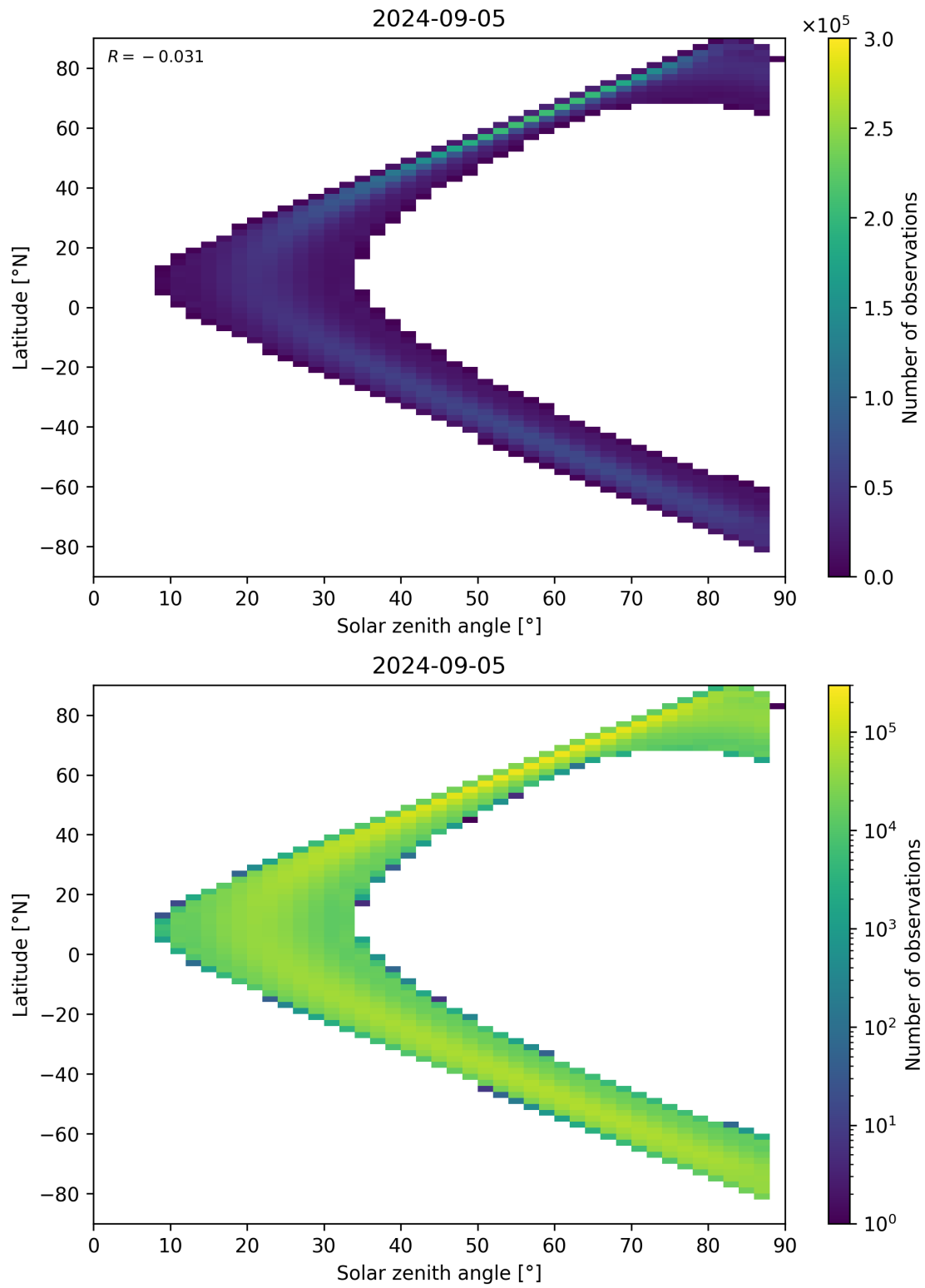
Figure 113: Scatter density plot of “Solar zenith angle” against “Latitude” for 2024-09-04 to 2024-09-06.
