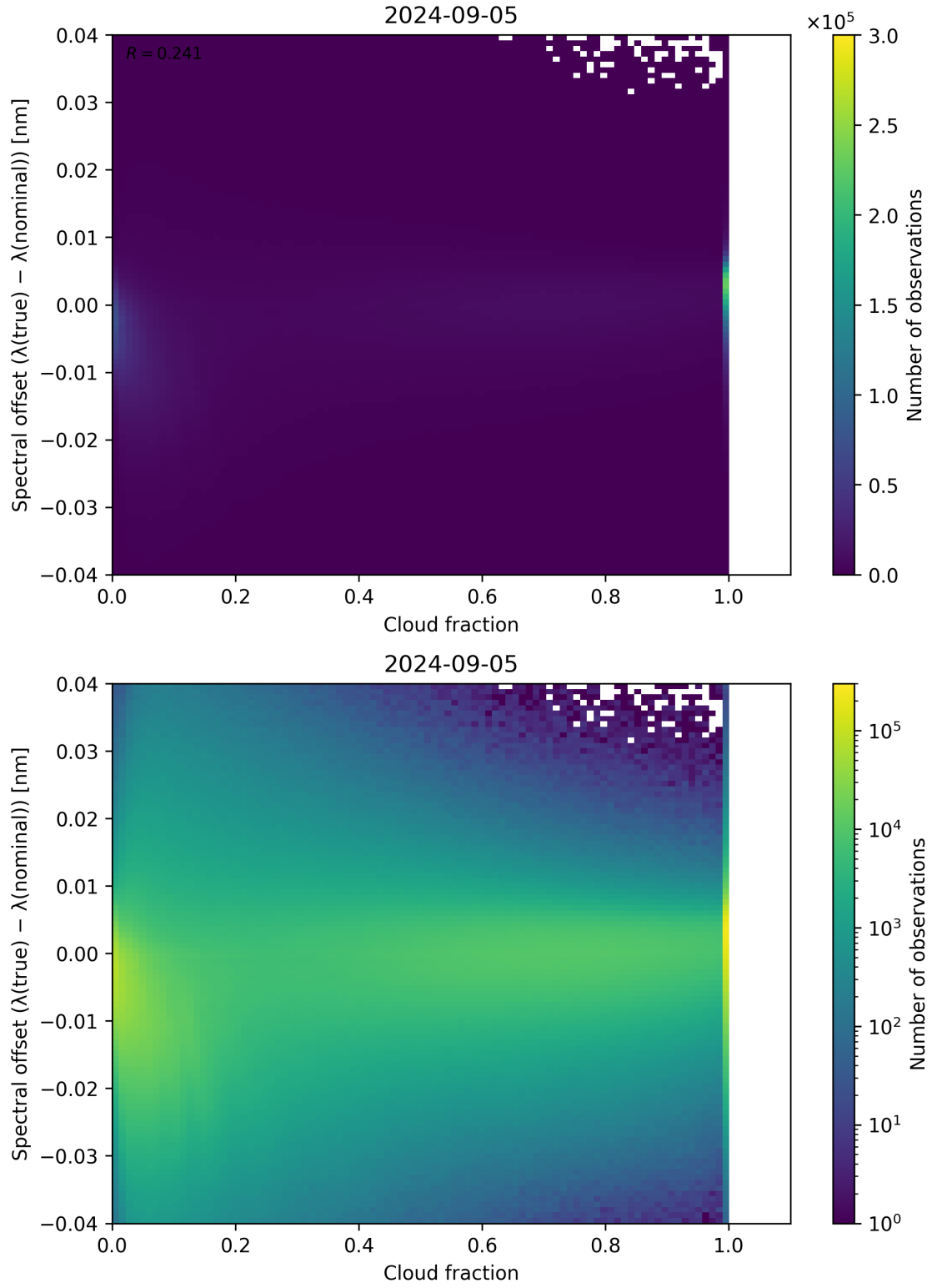
Figure 76: Scatter density plot of “Cloud fraction” against “Spectral offset ( \lambda_{\text{true}} - \lambda_{\text{nominal}} )” for 2024-09-04 to 2024-09-06.
