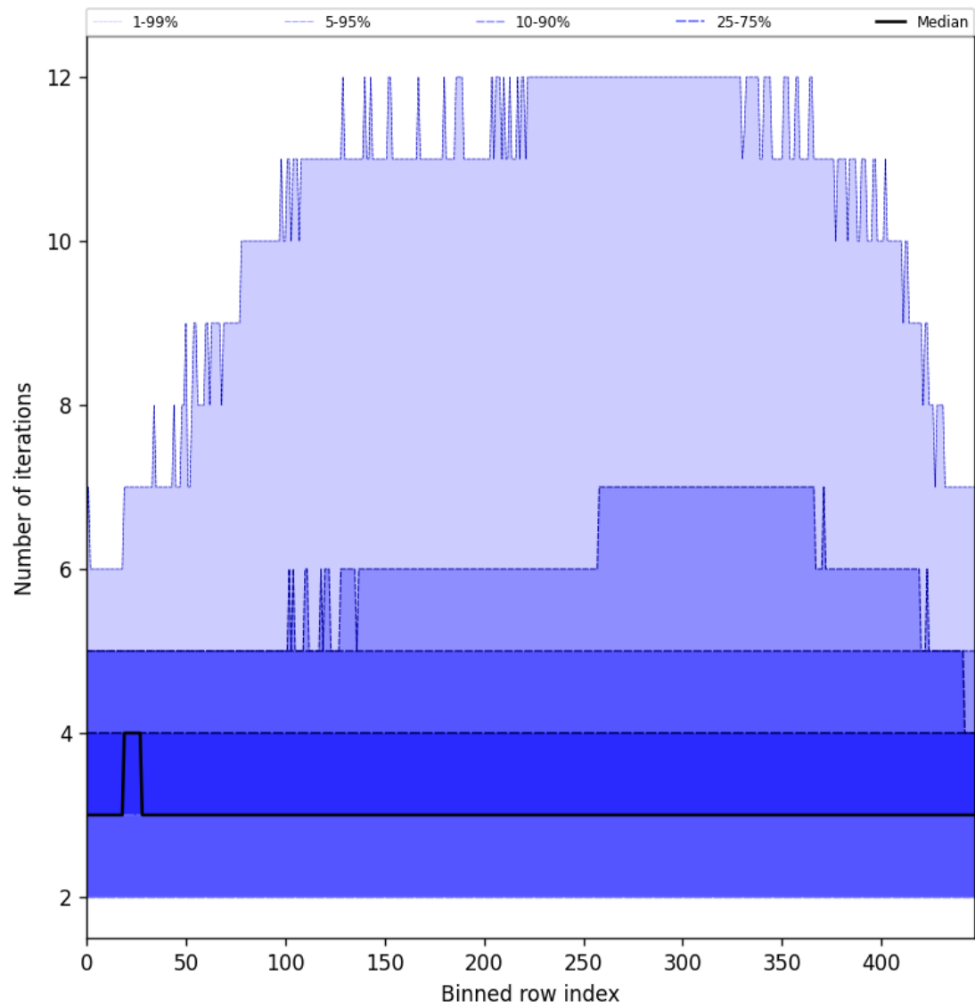
Figure 56: Along track statistics of “Number of iterations” for 2024-09-04 to 2024-09-06
