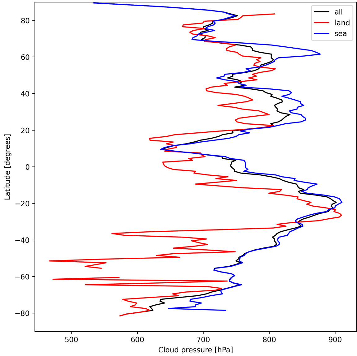
Figure 13: Zonal average of “Cloud pressure” for 2024-09-04 to 2024-09-06.
