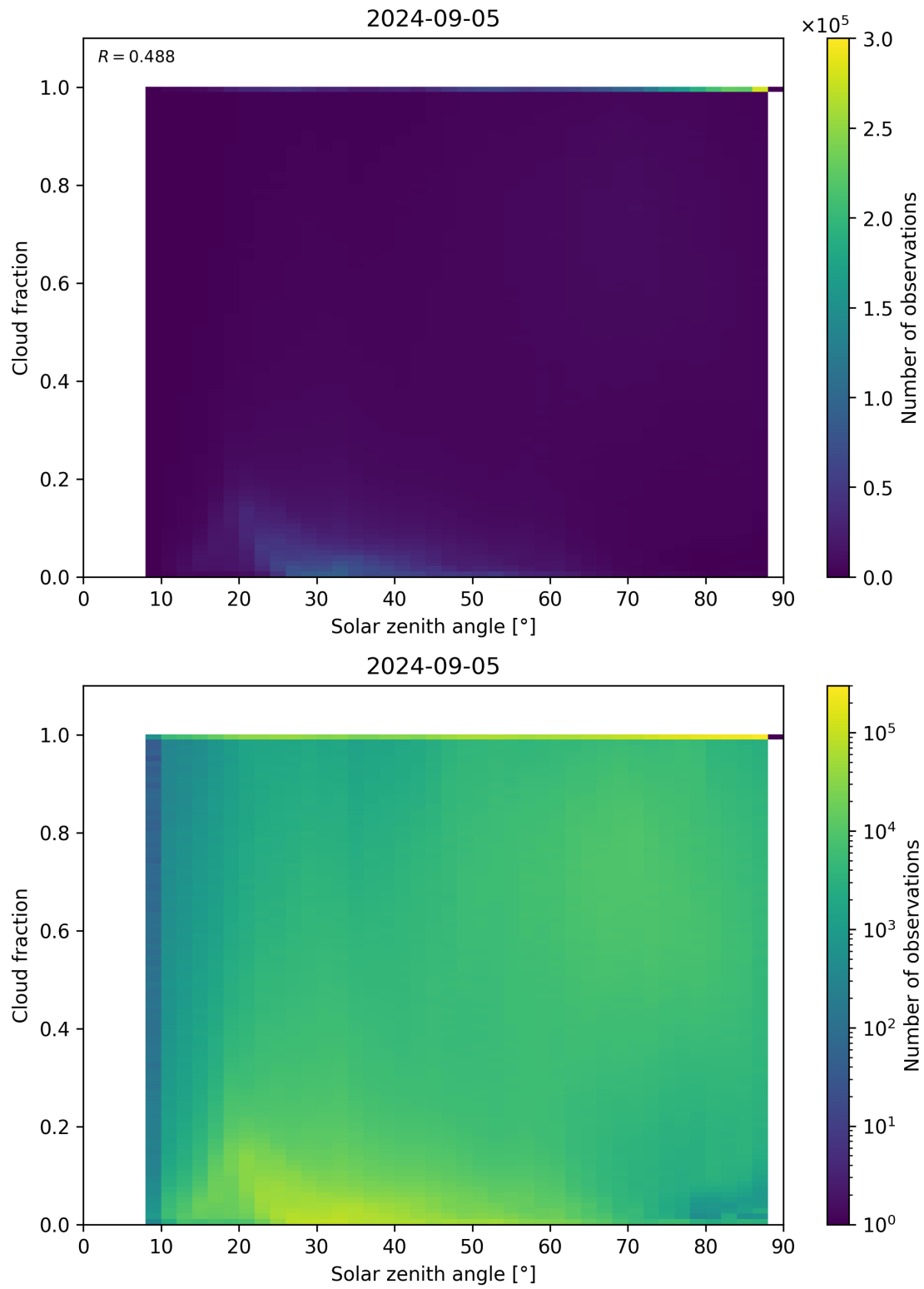
Figure 110: Scatter density plot of “Solar zenith angle” against “Cloud fraction” for 2024-09-04 to 2024-09-06.
