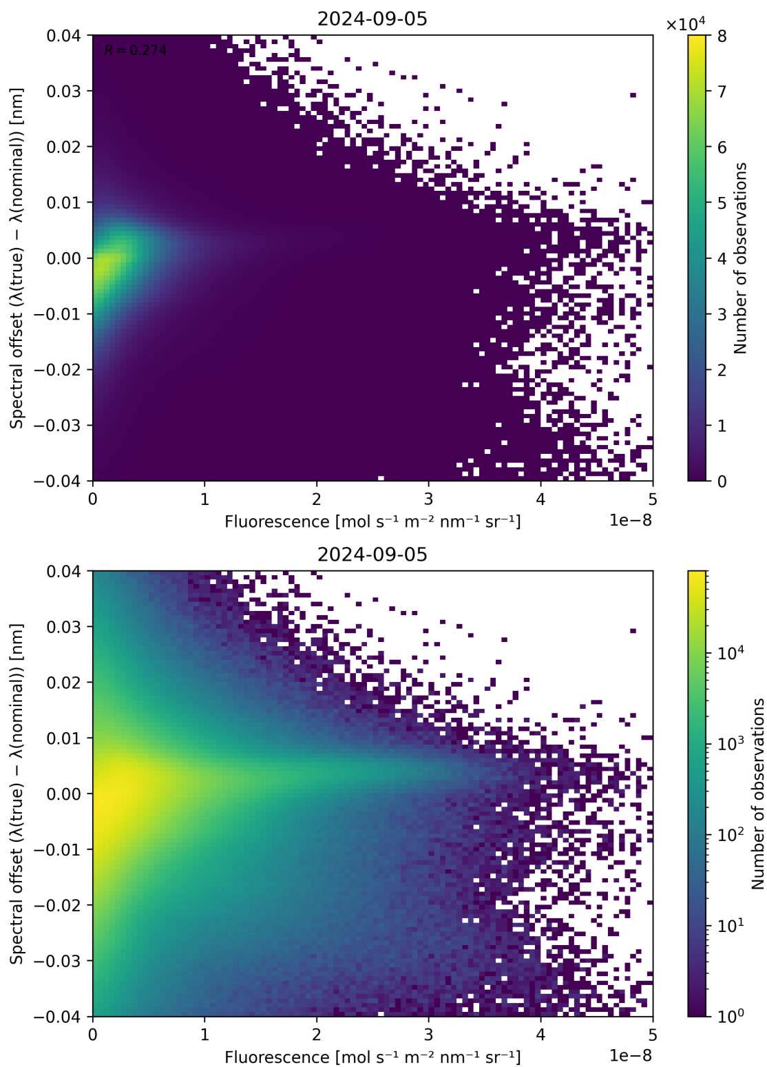
Figure 87: Scatter density plot of “Fluorescence” against “Spectral offset ( \lambda_{\text{true}} - \lambda_{\text{nominal}} )” for 2024-09-04 to 2024-09-06.
