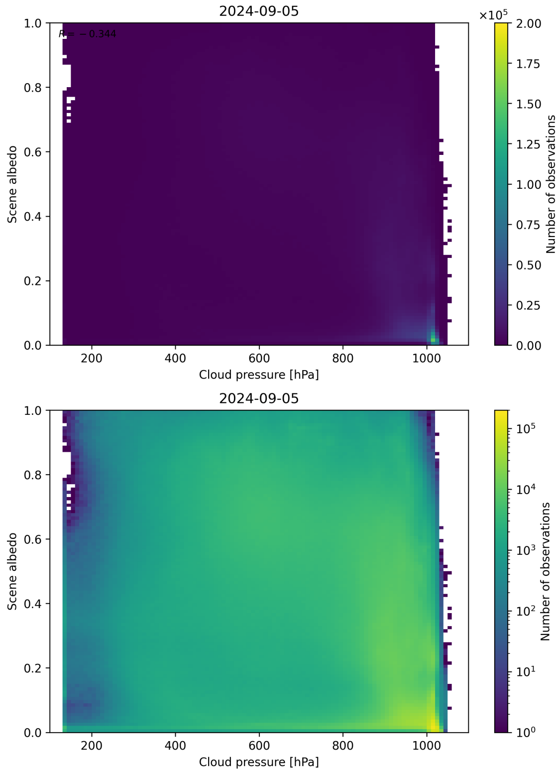
Figure 83: Scatter density plot of “Cloud pressure” against “Scene albedo” for 2024-09-04 to 2024-09-06.
