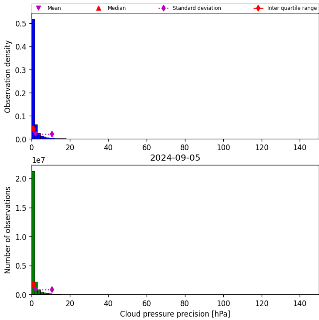
Figure 31: Histogram of “Cloud pressure precision” for 2024-09-04 to 2024-09-06
