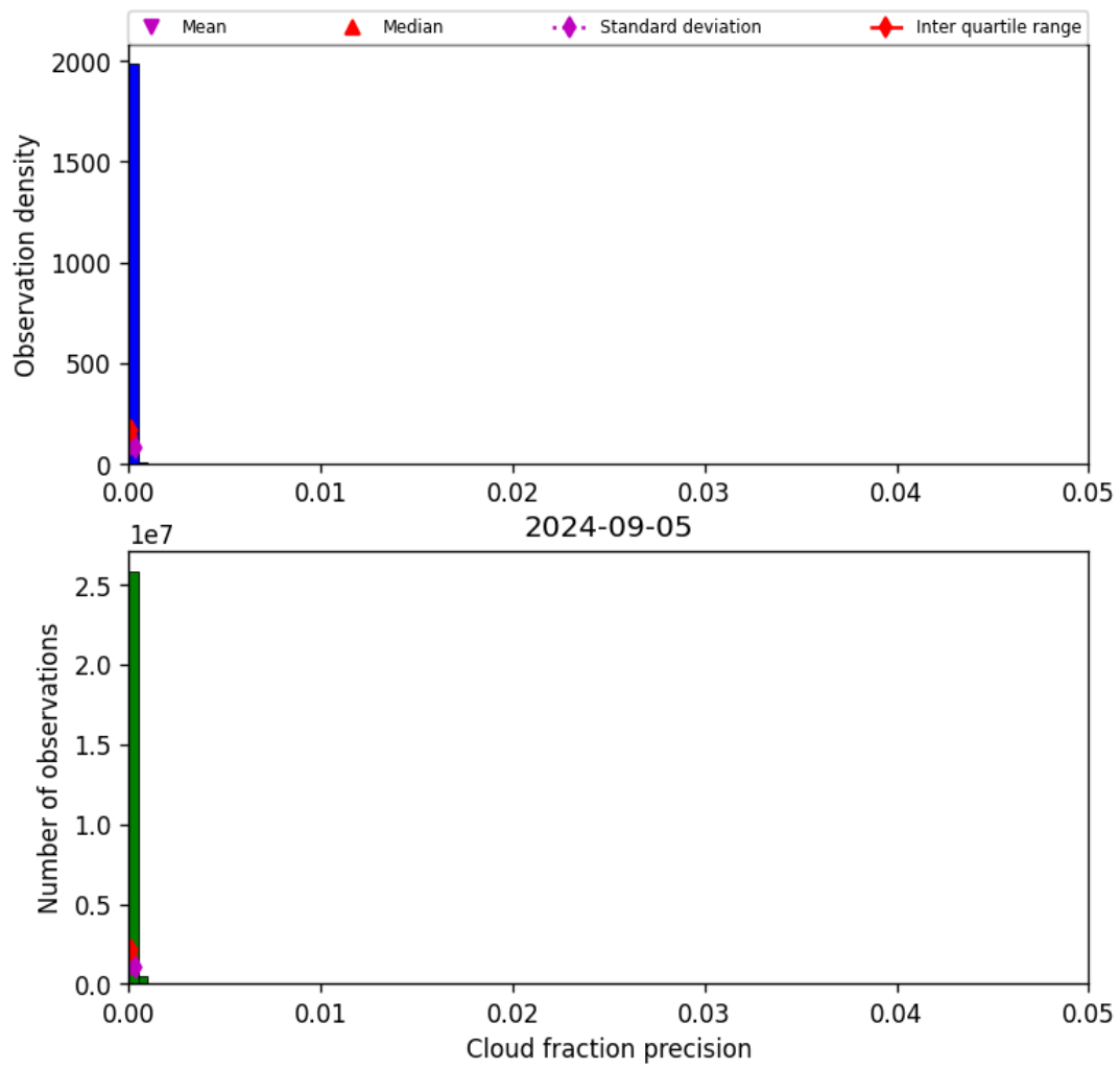
Figure 33: Histogram of “Cloud fraction precision” for 2024-09-04 to 2024-09-06
