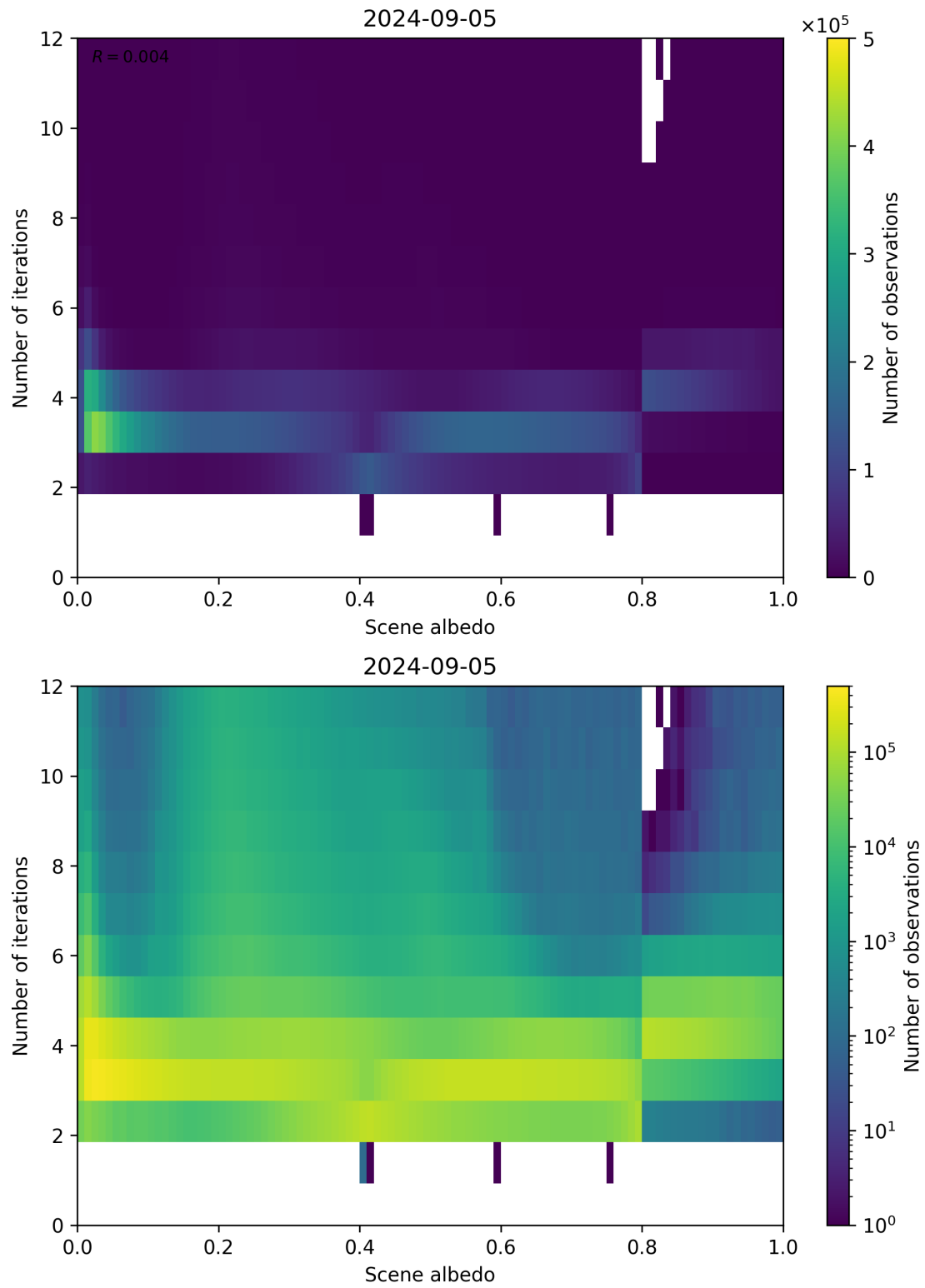
Figure 105: Scatter density plot of “Scene albedo” against “Number of iterations” for 2024-09-04 to 2024-09-06.
