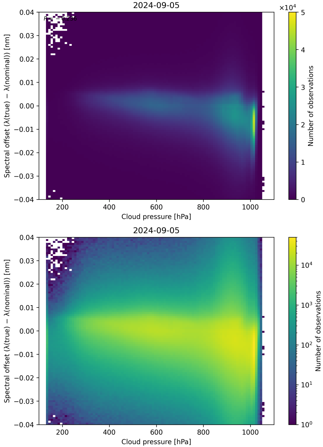
Figure 84: Scatter density plot of “Cloud pressure” against “Spectral offset ( \lambda_{\text{true}} - \lambda_{\text{nominal}} )” for 2024-09-04 to 2024-09-06.
