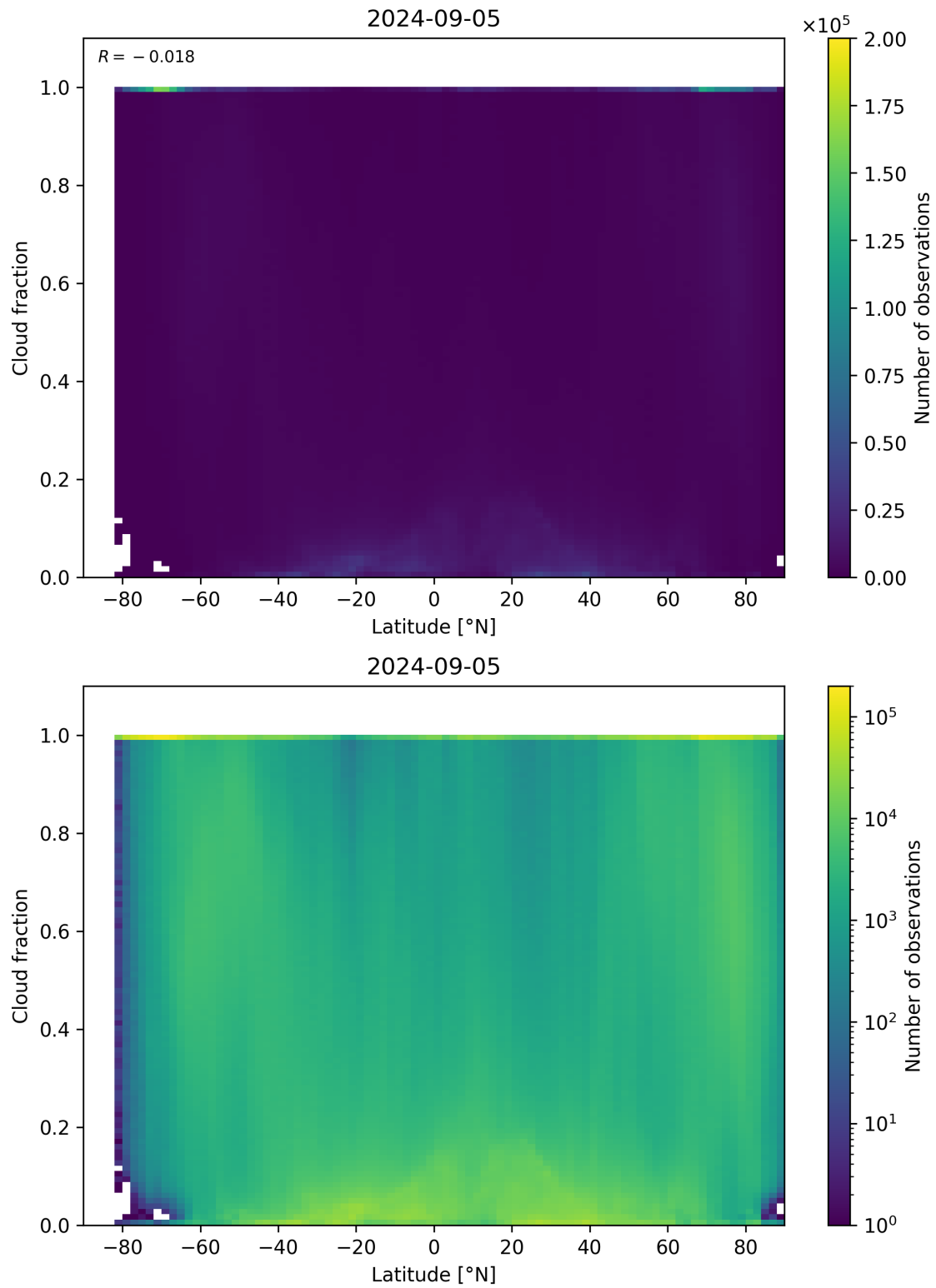
Figure 90: Scatter density plot of “Latitude” against “Cloud fraction” for 2024-09-04 to 2024-09-06.
