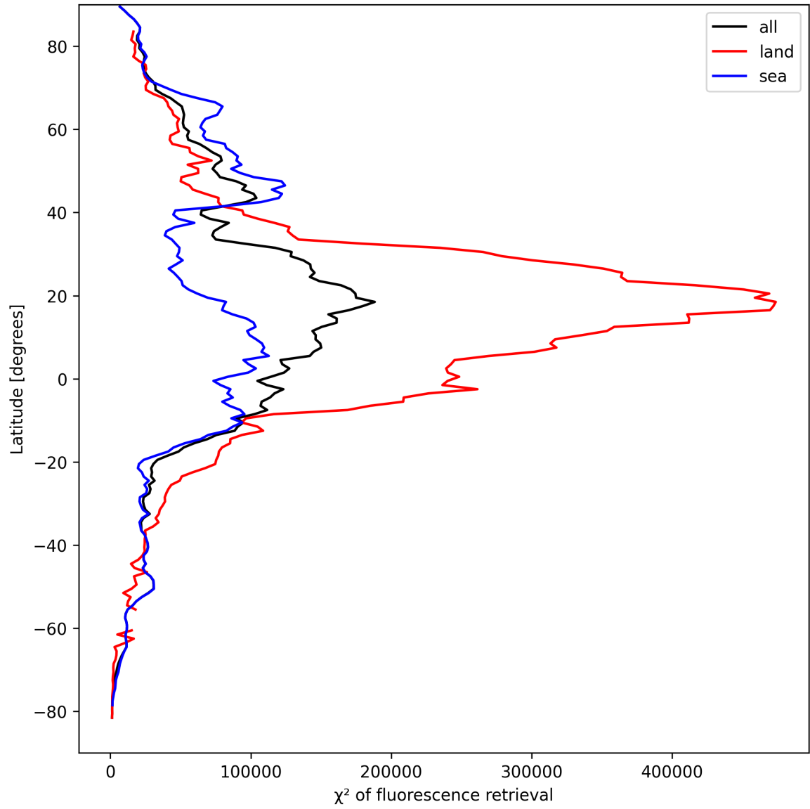
Figure 25: Zonal average of “ \chi^2 of fluorescence retrieval” for 2024-09-04 to 2024-09-06.
