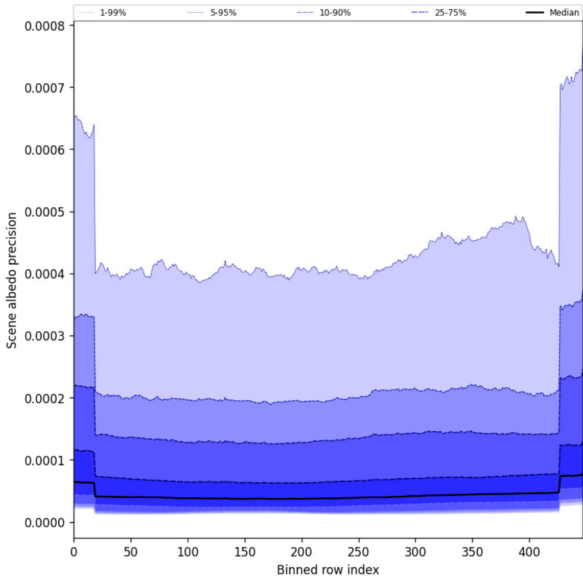
Figure 52: Along track statistics of “Scene albedo precision” for 2024-09-04 to 2024-09-06
