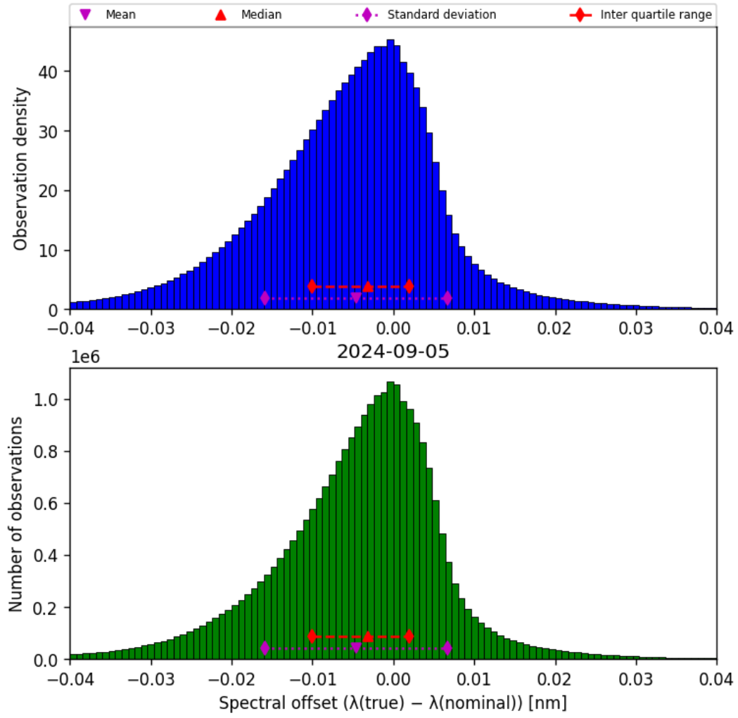
Figure 45: Histogram of “Spectral offset ( \lambda_{\text{true}} - \lambda_{\text{nominal}} )” for 2024-09-04 to 2024-09-06
