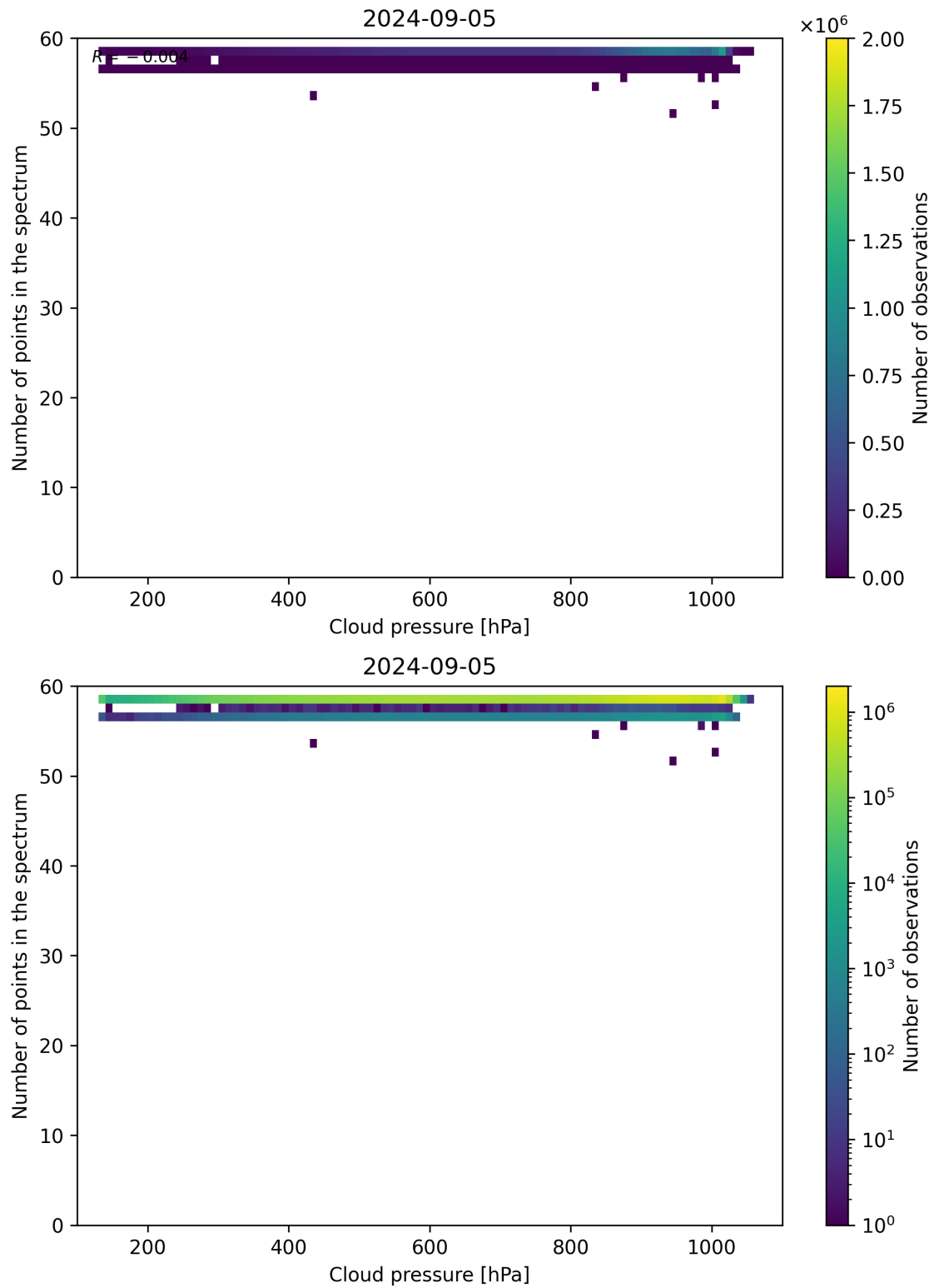
Figure 82: Scatter density plot of “Cloud pressure” against “Number of points in the spectrum” for 2024-09-04 to 2024-09-06.
