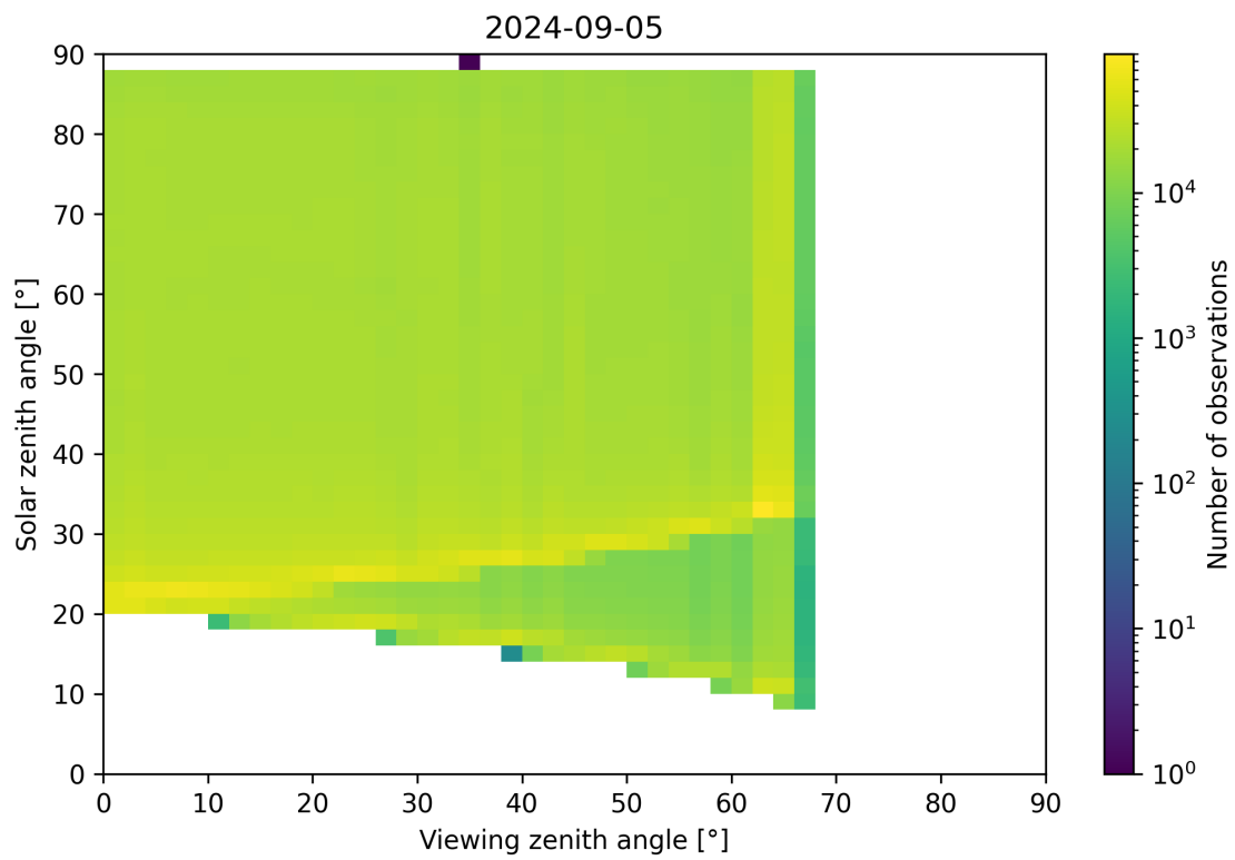
Figure 127: Scatter density plot of “Viewing zenith angle” against “Solar zenith angle” for 2024-09-04 to 2024-09-06.
