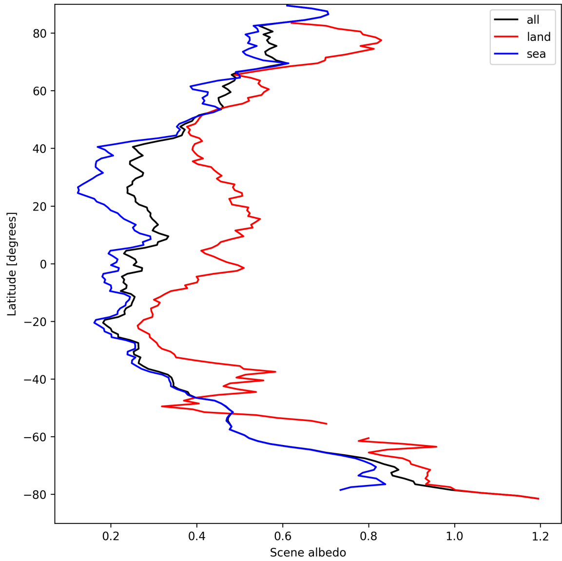
Figure 17: Zonal average of “Scene albedo” for 2024-09-04 to 2024-09-06.
