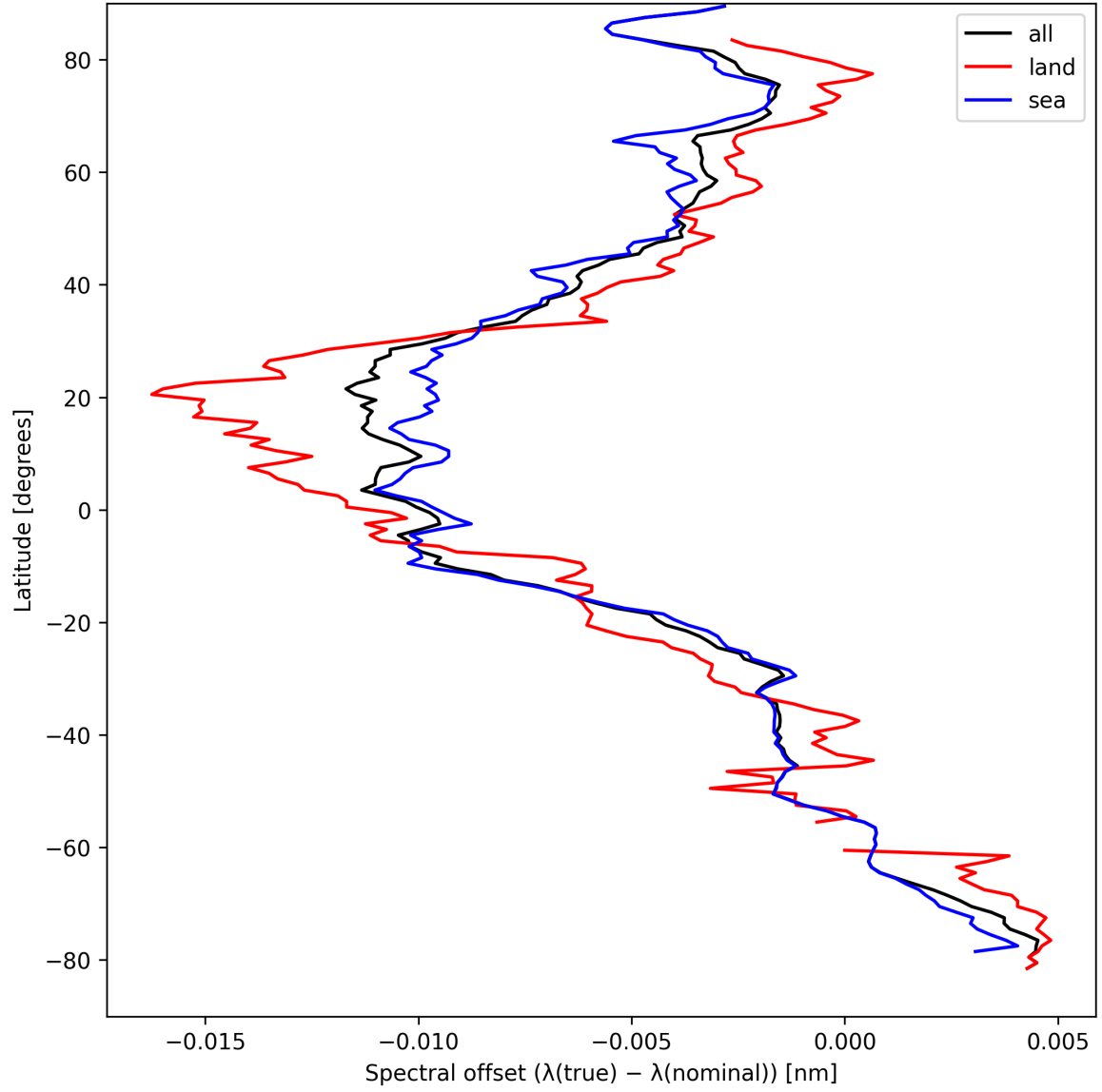
Figure 28: Zonal average of “Spectral offset ( \lambda_{\text{true}} - \lambda_{\text{nominal}} )” for 2024-09-04 to 2024-09-06.
