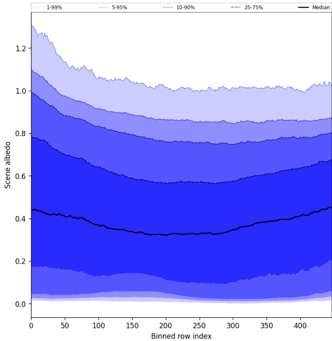
Figure 51: Along track statistics of “Scene albedo” for 2024-09-04 to 2024-09-06
