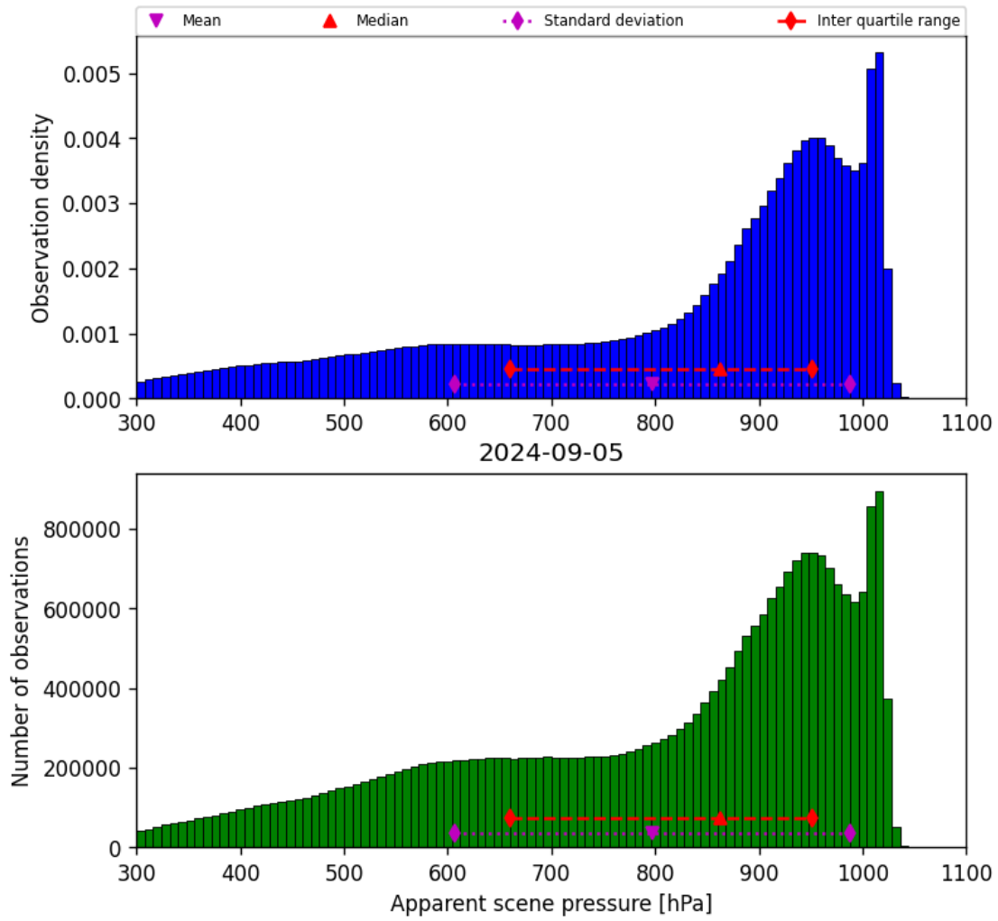
Figure 36: Histogram of “Apparent scene pressure” for 2024-09-04 to 2024-09-06
