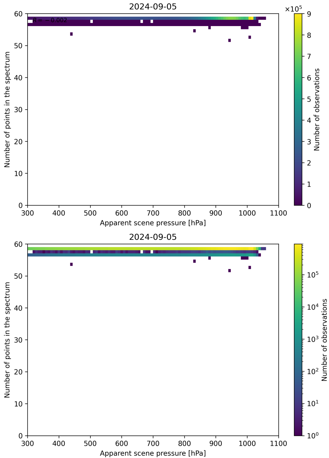
Figure 66: Scatter density plot of “Apparent scene pressure” against “Number of points in the spectrum” for 2024-09-04 to 2024-09-06.
