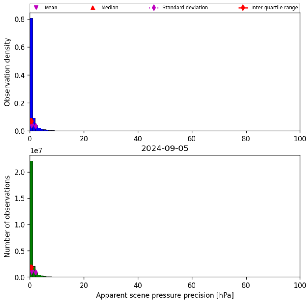
Figure 37: Histogram of “Apparent scene pressure precision” for 2024-09-04 to 2024-09-06
