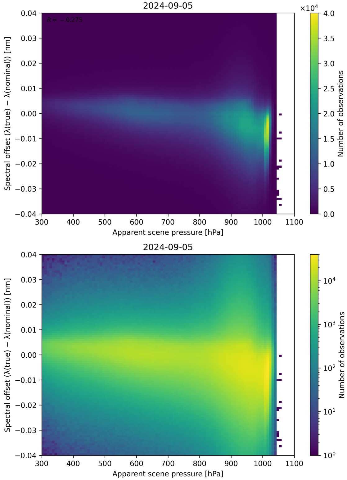
Figure 67: Scatter density plot of “Apparent scene pressure” against “Spectral offset ( \lambda_{\text{true}} - \lambda_{\text{nominal}} )” for 2024-09-04 to 2024-09-06.
