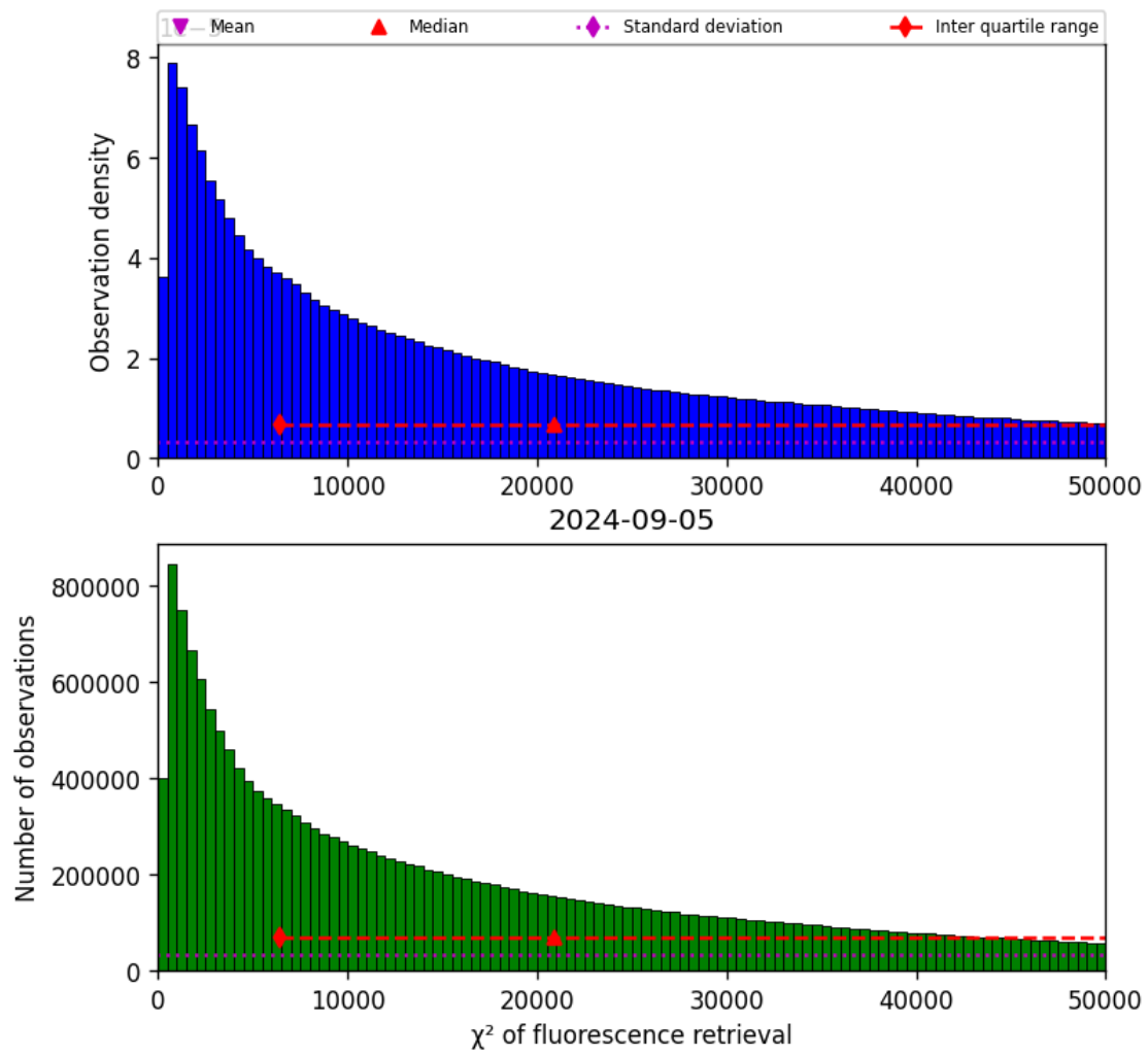
Figure 42: Histogram of “ \chi^2 of fluorescence retrieval” for 2024-09-04 to 2024-09-06
