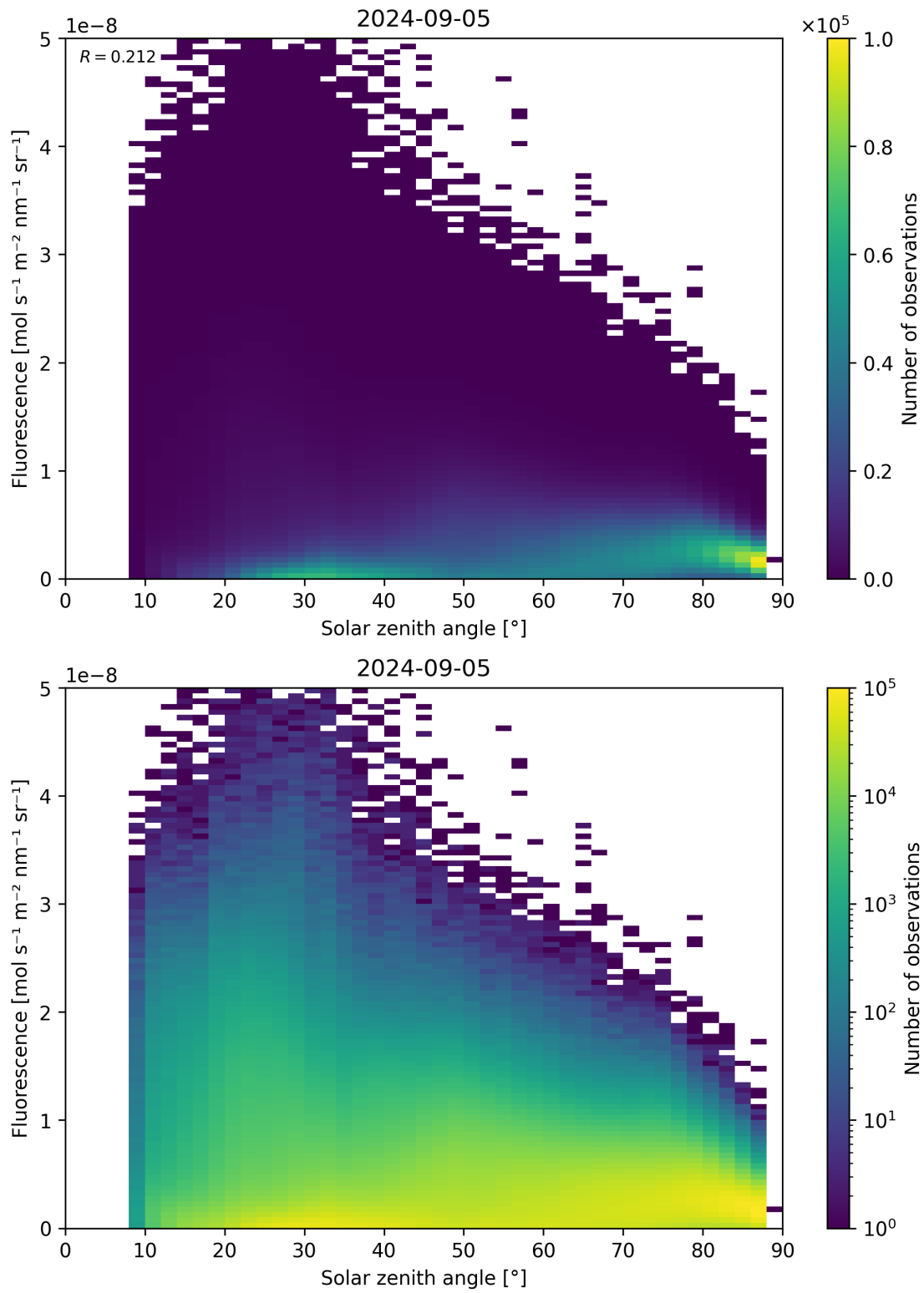
Figure 112: Scatter density plot of “Solar zenith angle” against “Fluorescence” for 2024-09-04 to 2024-09-06.
