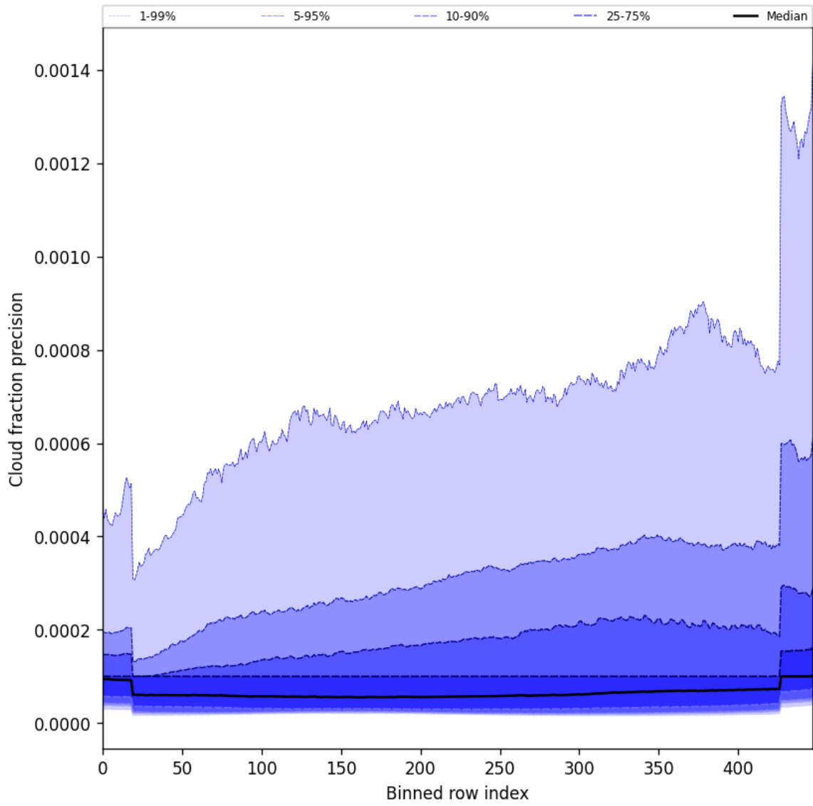
Figure 50: Along track statistics of “Cloud fraction precision” for 2024-09-04 to 2024-09-06
