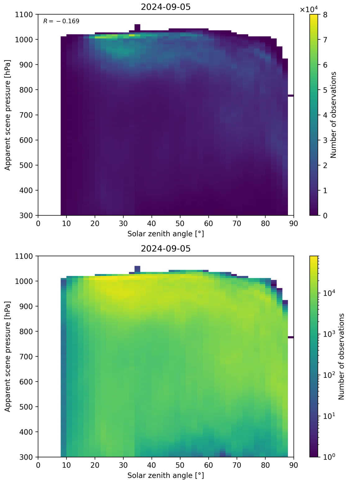
Figure 108: Scatter density plot of “Solar zenith angle” against “Apparent scene pressure” for 2024-09-04 to 2024-09-06.
