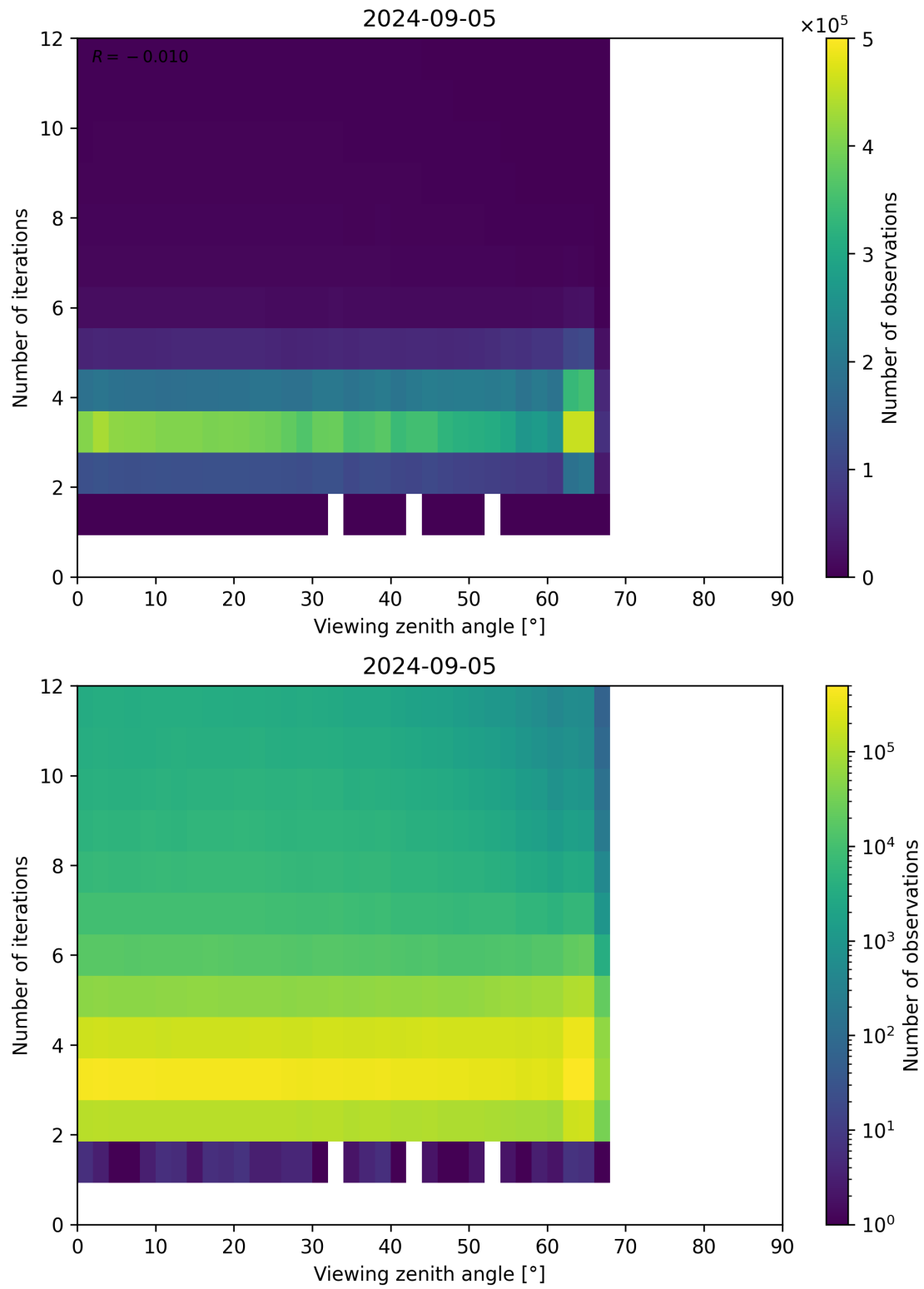
Figure 124: Scatter density plot of “Viewing zenith angle” against “Number of iterations” for 2024-09-04 to 2024-09-06.
