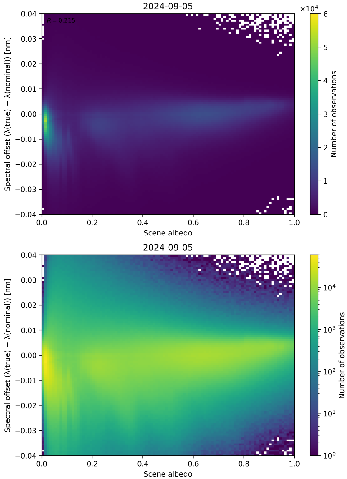
Figure 107: Scatter density plot of “Scene albedo” against “Spectral offset ( \lambda_{\text{true}} - \lambda_{\text{nominal}} )” for 2024-09-04 to 2024-09-06.
