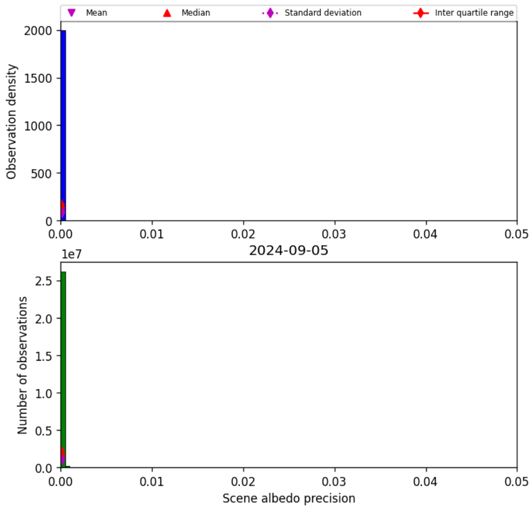
Figure 35: Histogram of “Scene albedo precision” for 2024-09-04 to 2024-09-06
