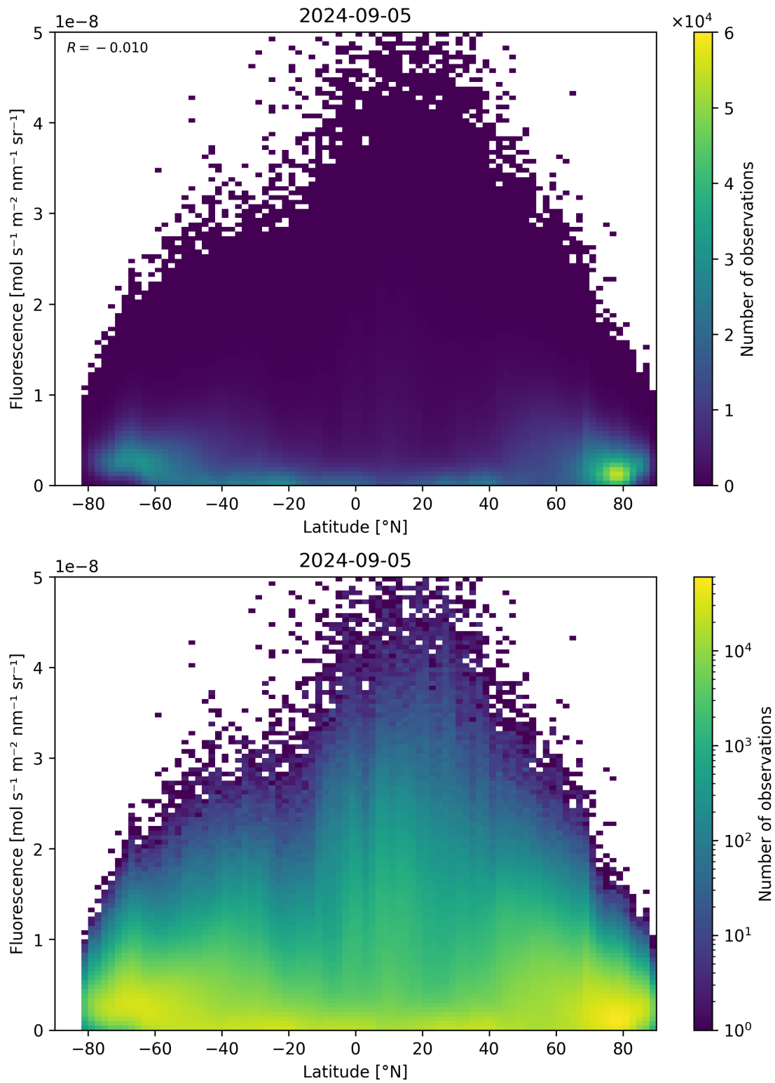
Figure 92: Scatter density plot of “Latitude” against “Fluorescence” for 2024-09-04 to 2024-09-06.
