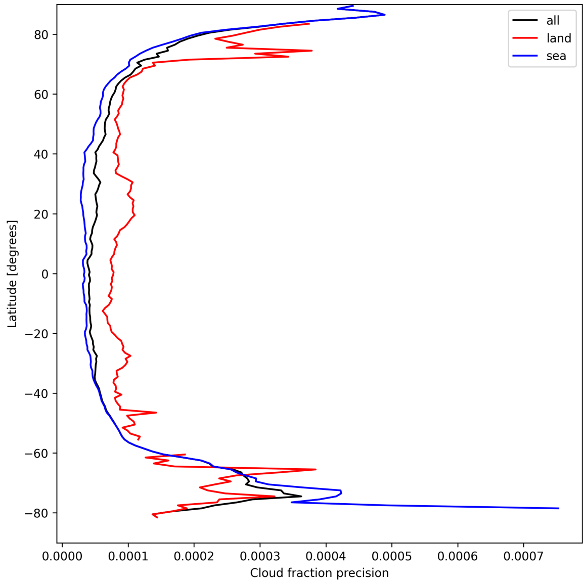
Figure 16: Zonal average of “Cloud fraction precision” for 2024-09-04 to 2024-09-06.
