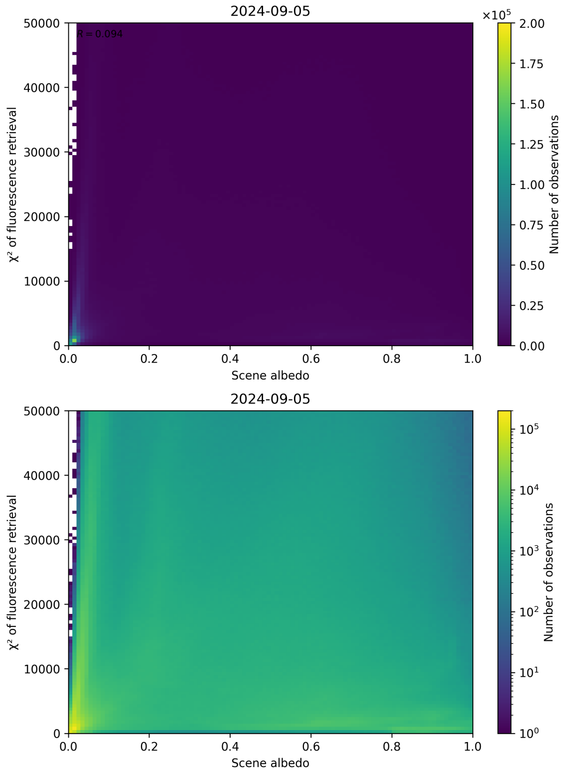
Figure 103: Scatter density plot of “Scene albedo” against “ \chi^2 of fluorescence retrieval” for 2024-09-04 to 2024-09-06.
