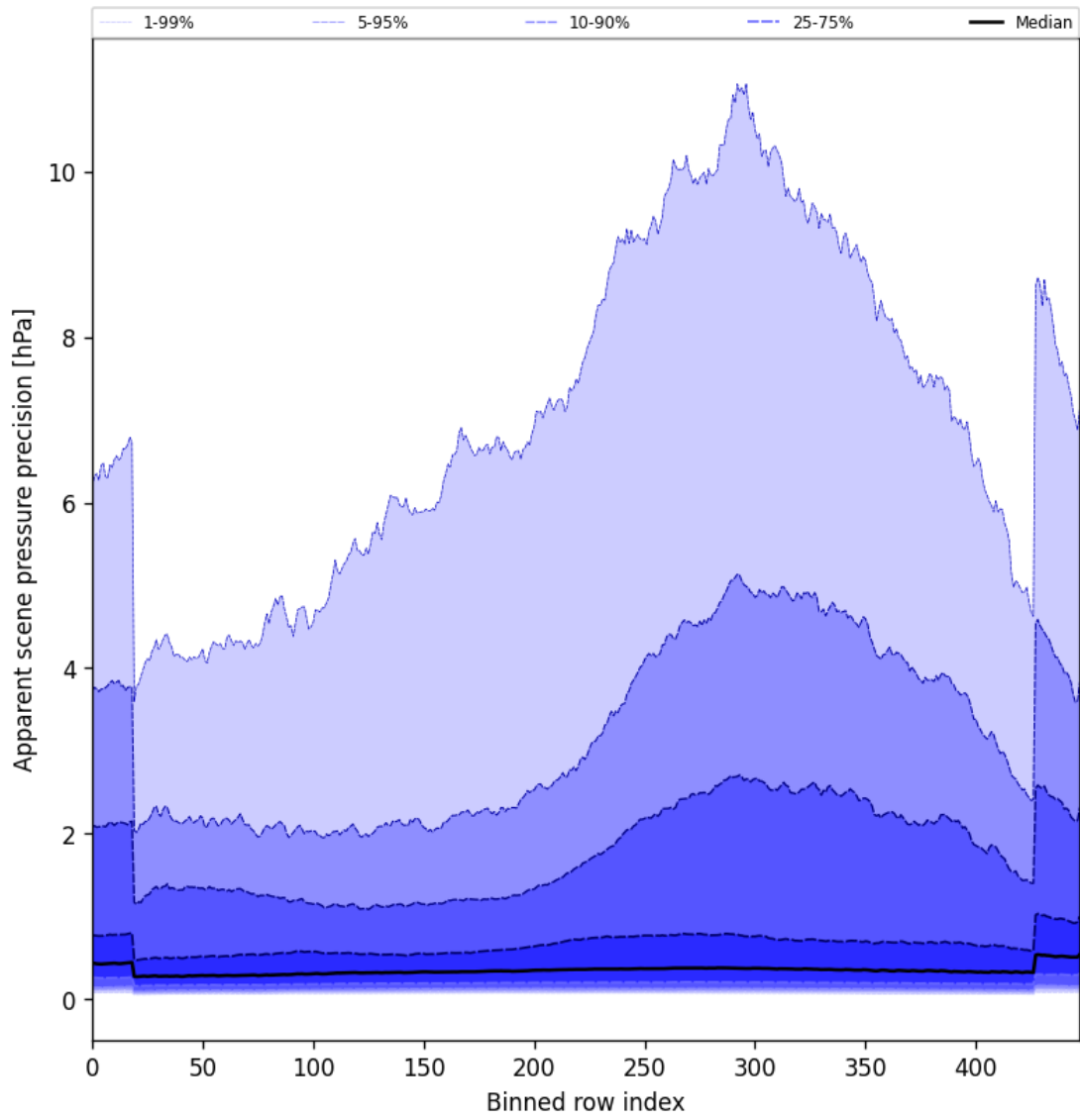
Figure 54: Along track statistics of “Apparent scene pressure precision” for 2024-09-04 to 2024-09-06
