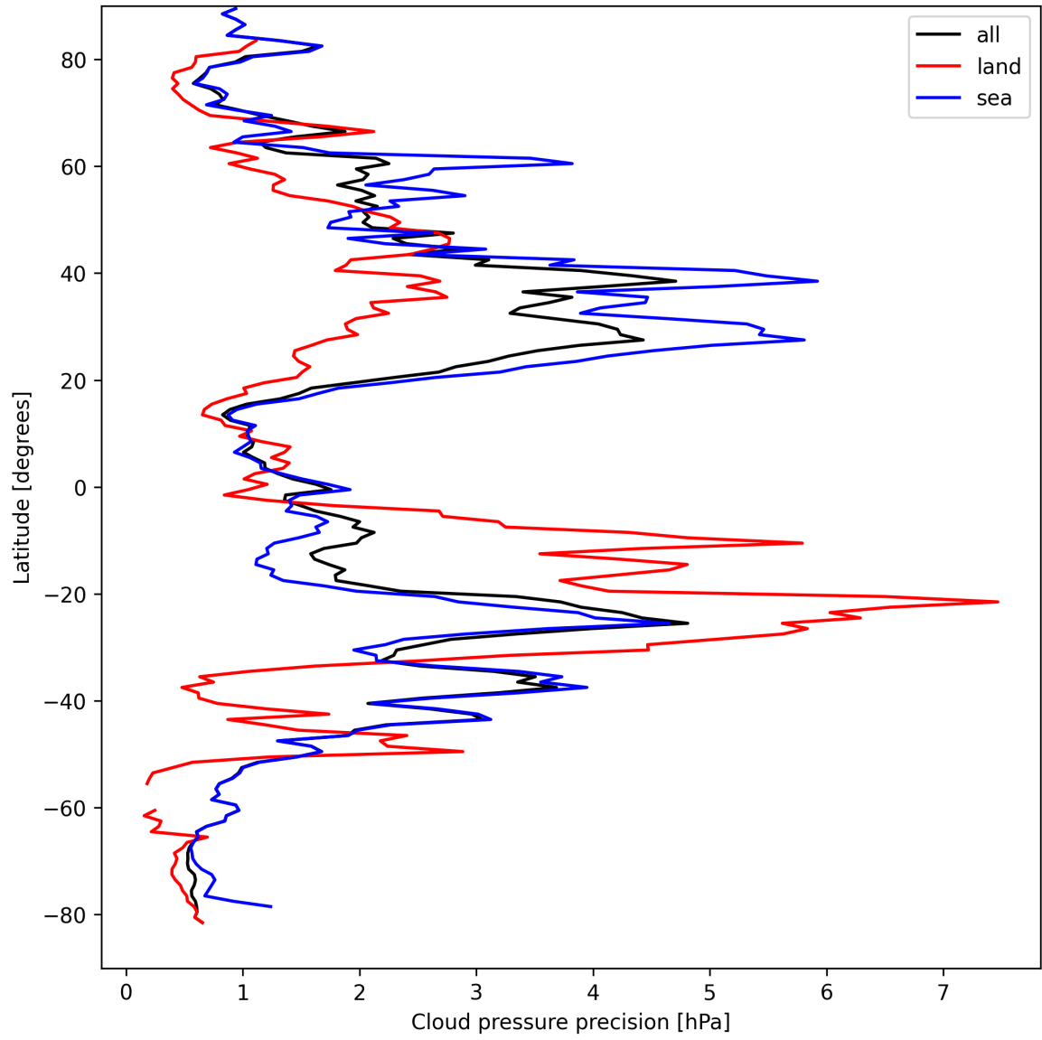
Figure 14: Zonal average of “Cloud pressure precision” for 2024-09-04 to 2024-09-06.
