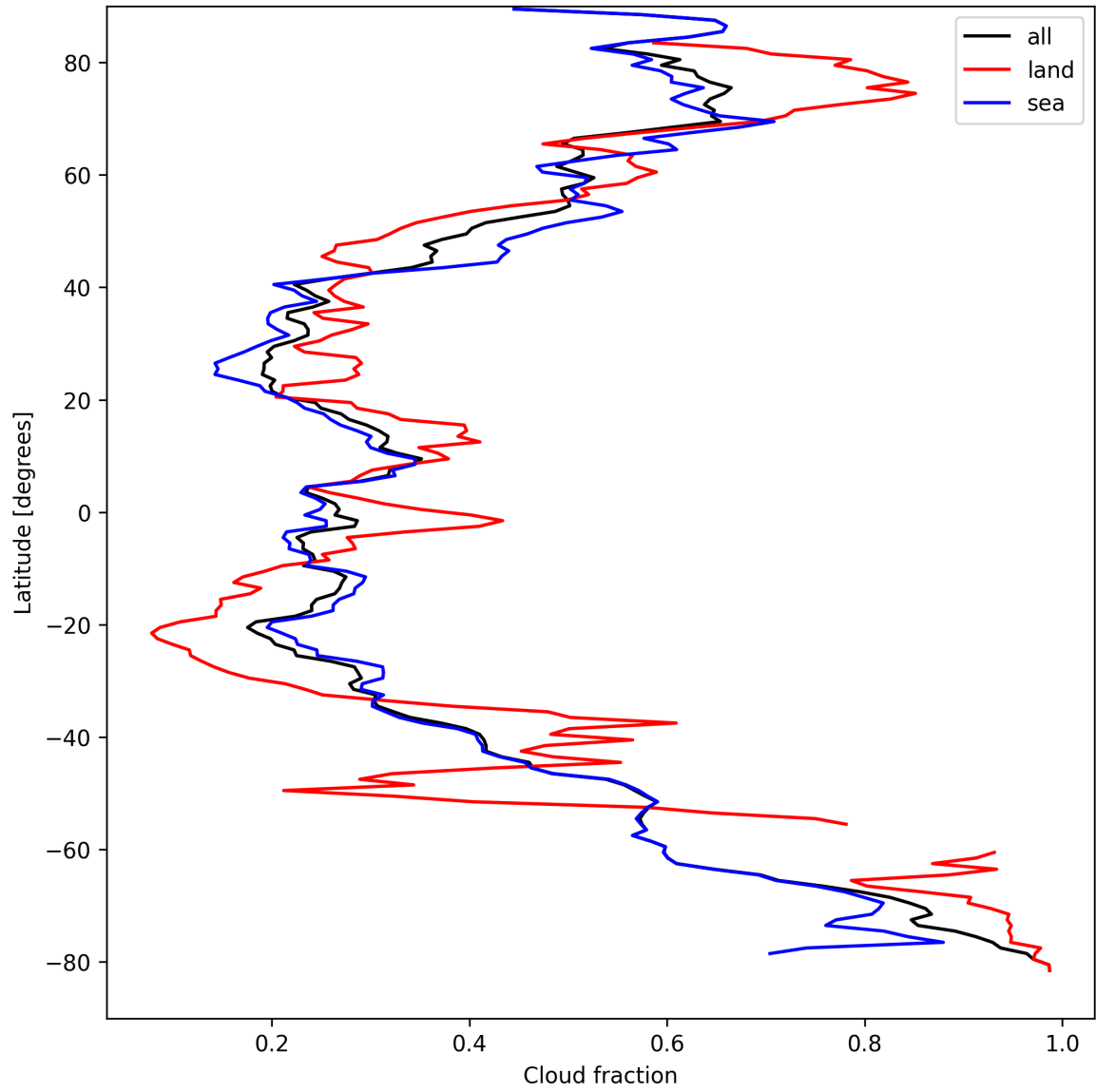
Figure 15: Zonal average of “Cloud fraction” for 2024-09-04 to 2024-09-06.
