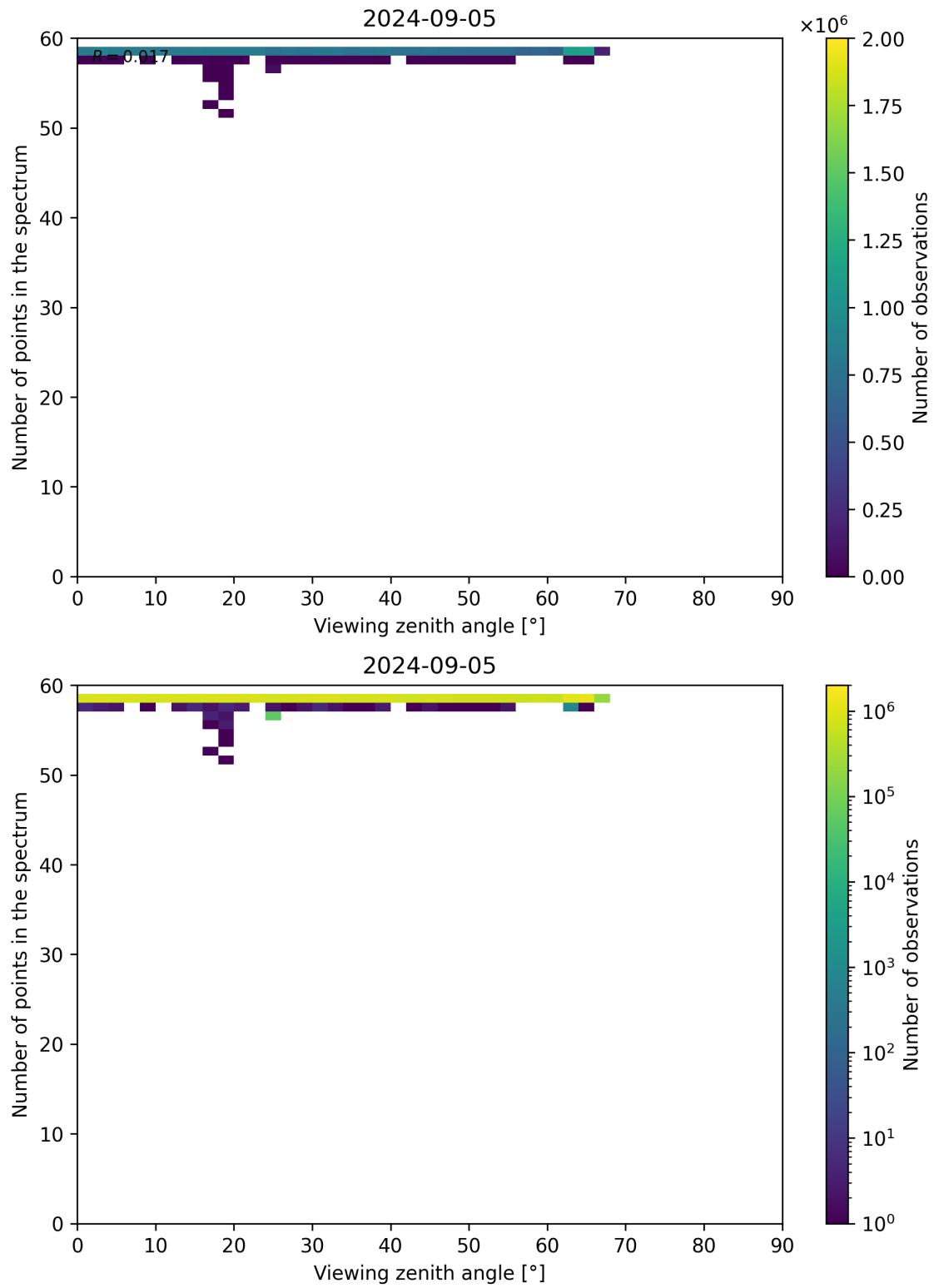
Figure 125: Scatter density plot of “Viewing zenith angle” against “Number of points in the spectrum” for 2024-09-04 to 2024-09-06.
