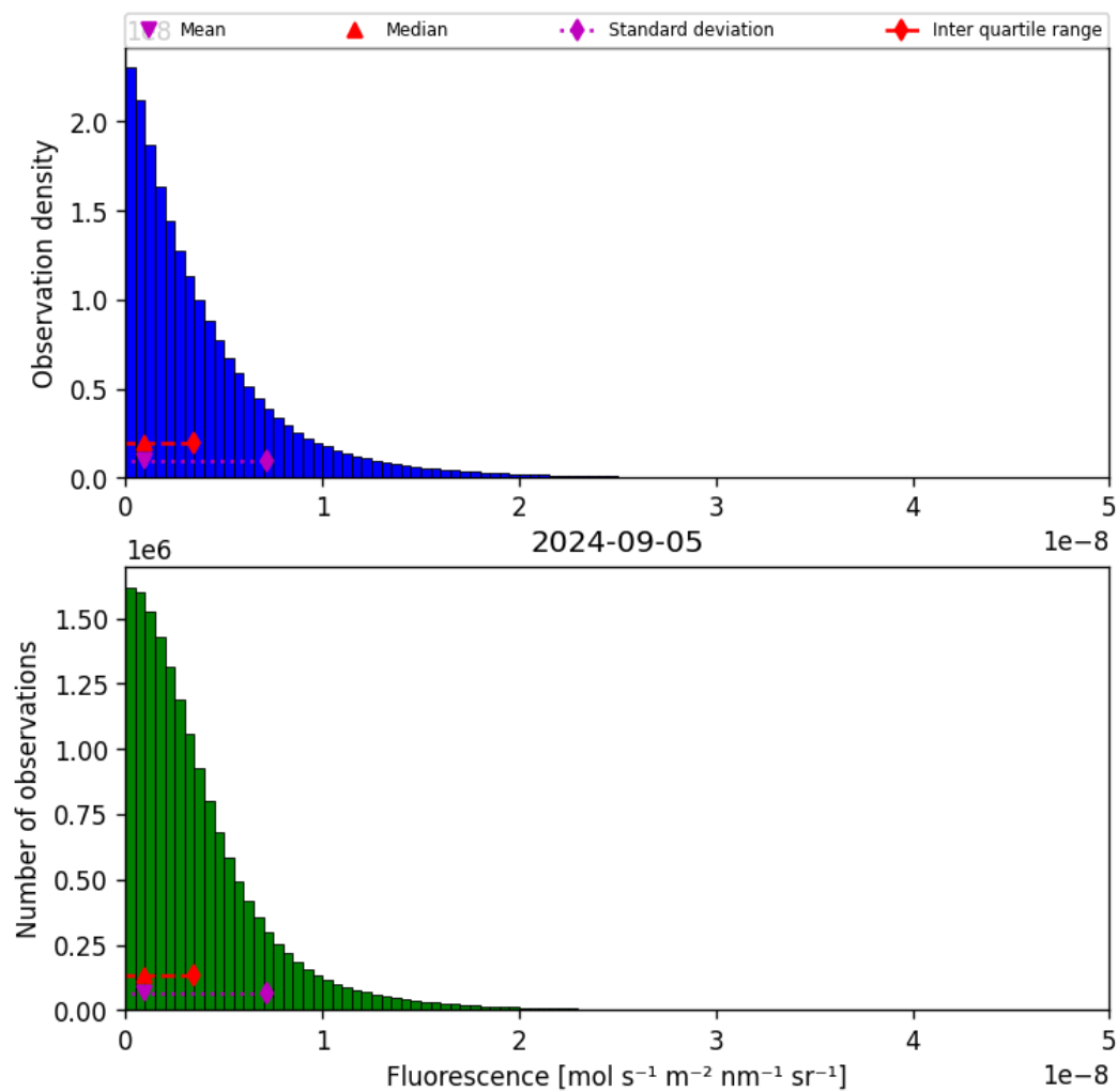
Figure 40: Histogram of “Fluorescence” for 2024-09-04 to 2024-09-06
