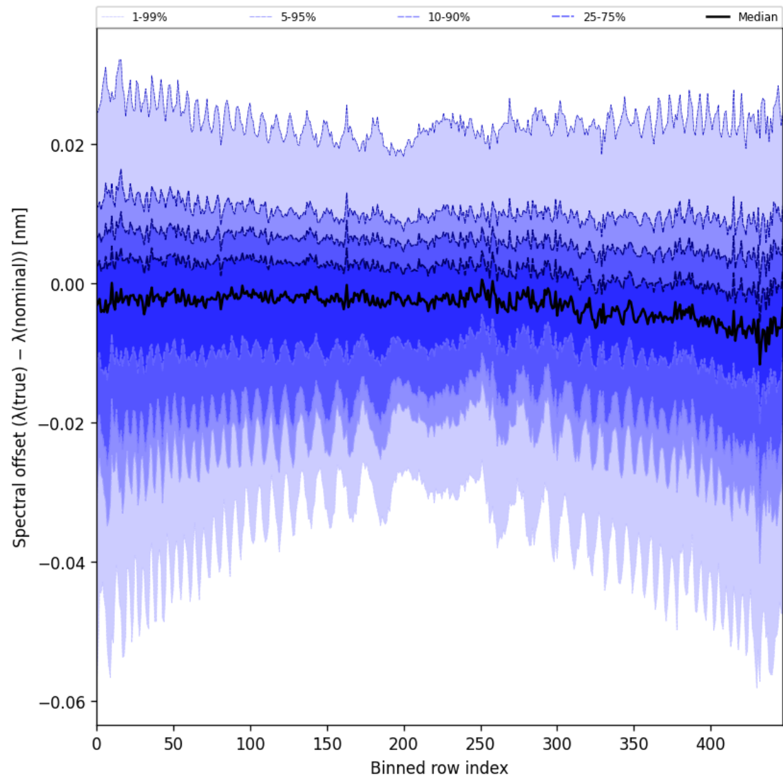
Figure 62: Along track statistics of “Spectral offset ( \lambda_{\text{true}} - \lambda_{\text{nominal}} )” for 2024-09-04 to 2024-09-06
