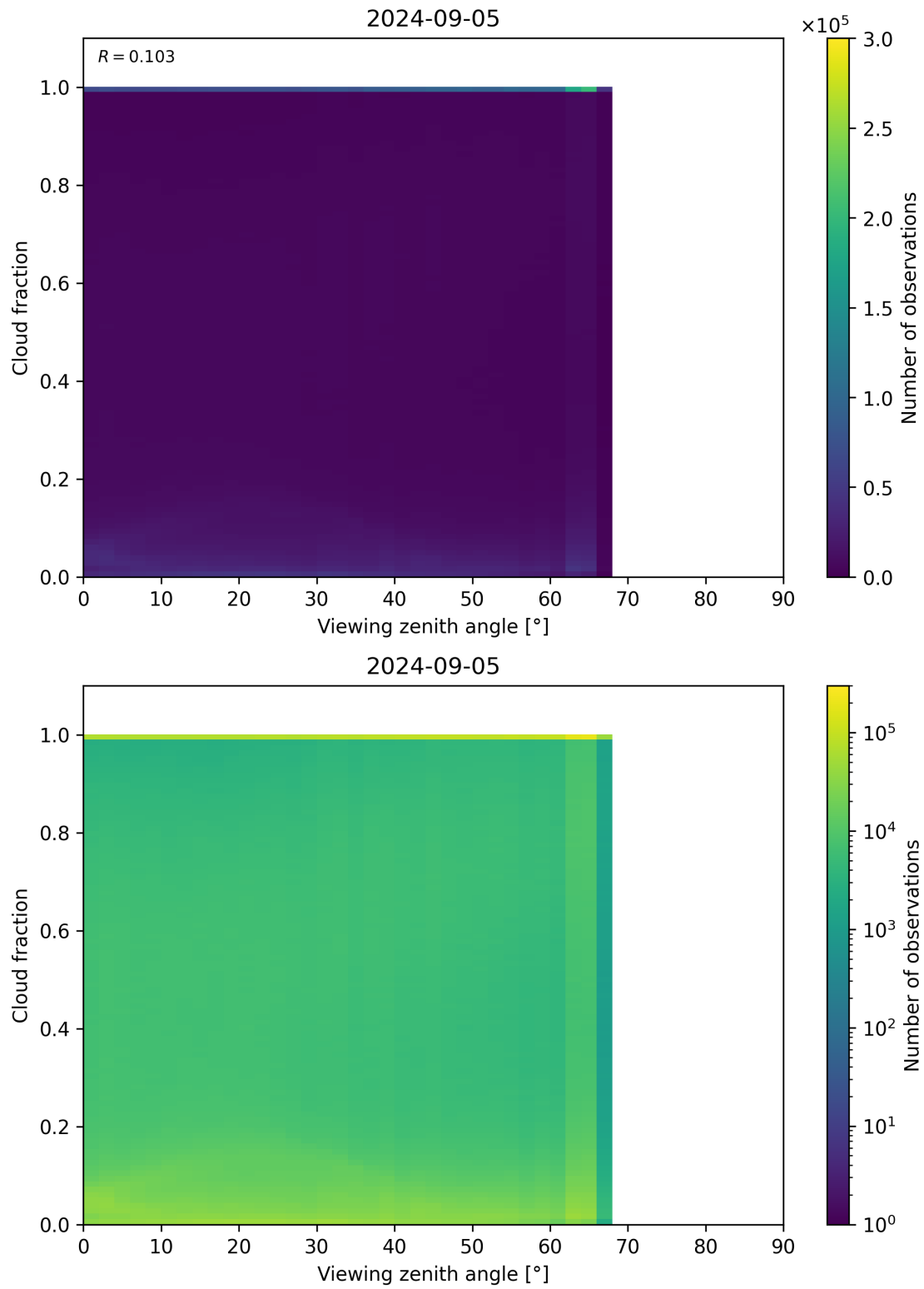
Figure 120: Scatter density plot of “Viewing zenith angle” against “Cloud fraction” for 2024-09-04 to 2024-09-06.
