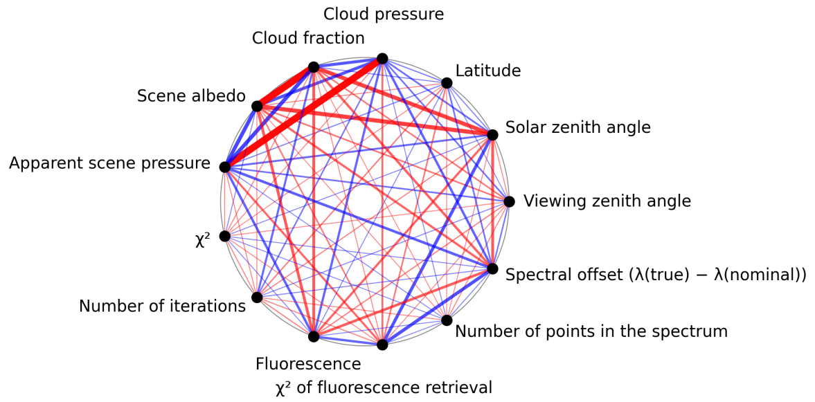
Figure 1: Map of correlation graph for 2024-09-04 to 2024-09-06.
