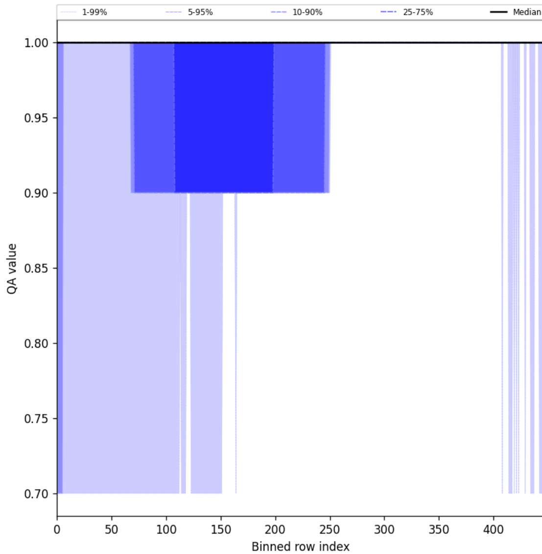
Figure 46: Along track statistics of “QA value” for 2024-09-04 to 2024-09-06
