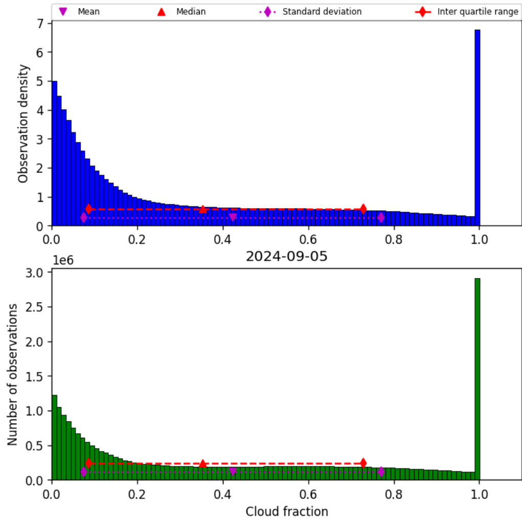
Figure 32: Histogram of “Cloud fraction” for 2024-09-04 to 2024-09-06
