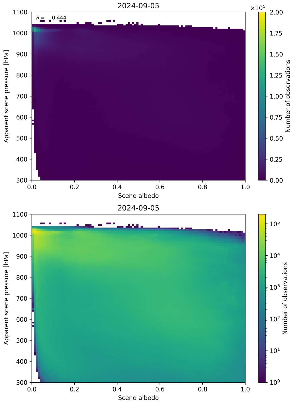
Figure 102: Scatter density plot of “Scene albedo” against “Apparent scene pressure” for 2024-09-04 to 2024-09-06.
