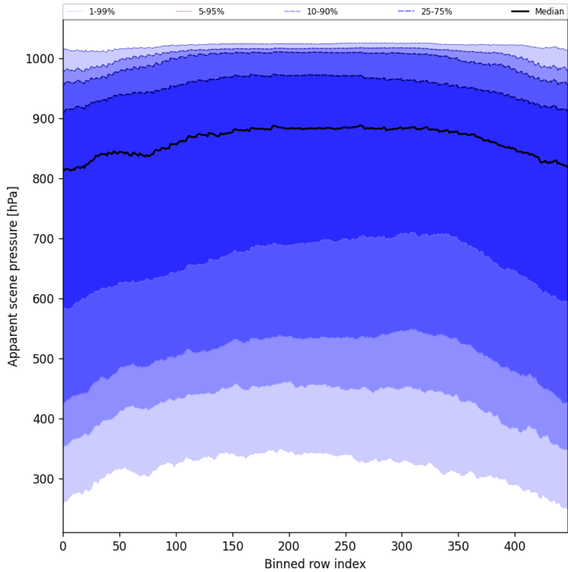
Figure 53: Along track statistics of “Apparent scene pressure” for 2024-09-04 to 2024-09-06
