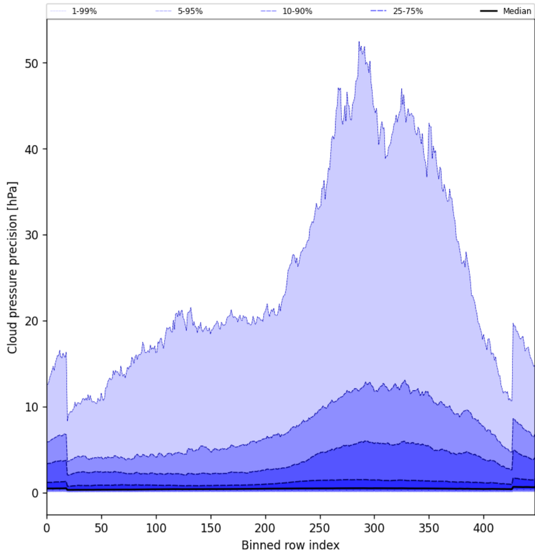
Figure 48: Along track statistics of “Cloud pressure precision” for 2024-09-04 to 2024-09-06
