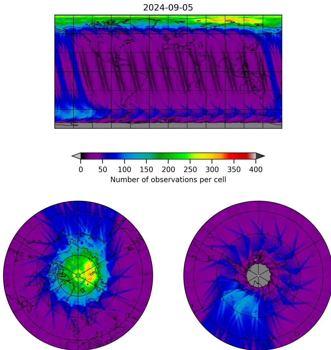
Figure 11: Map of the number of observations for 2024-09-04 to 2024-09-06
