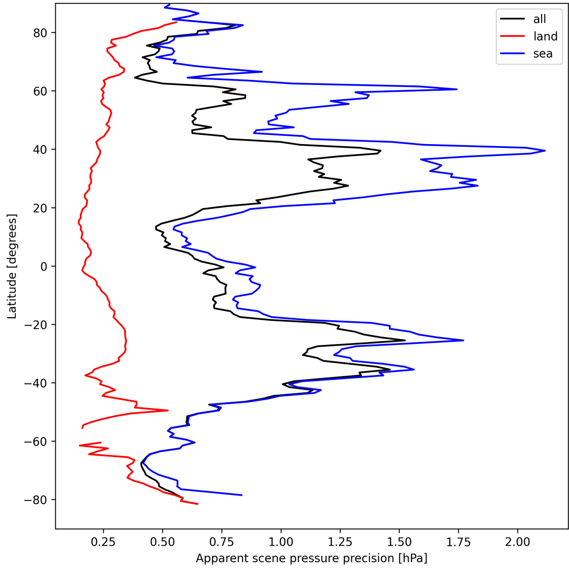
Figure 20: Zonal average of “Apparent scene pressure precision” for 2024-09-04 to 2024-09-06.
