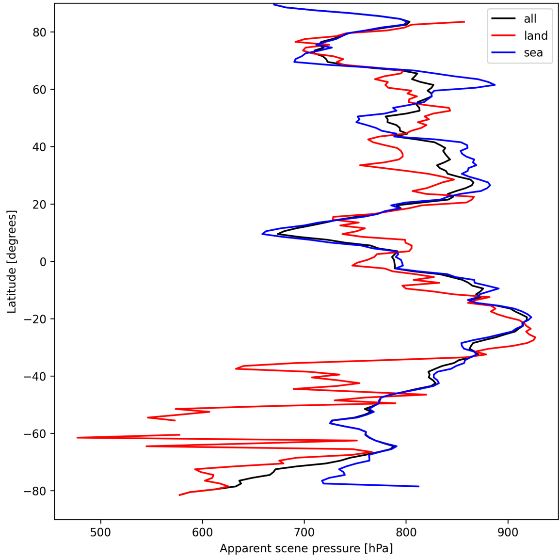
Figure 19: Zonal average of “Apparent scene pressure” for 2024-09-04 to 2024-09-06.
