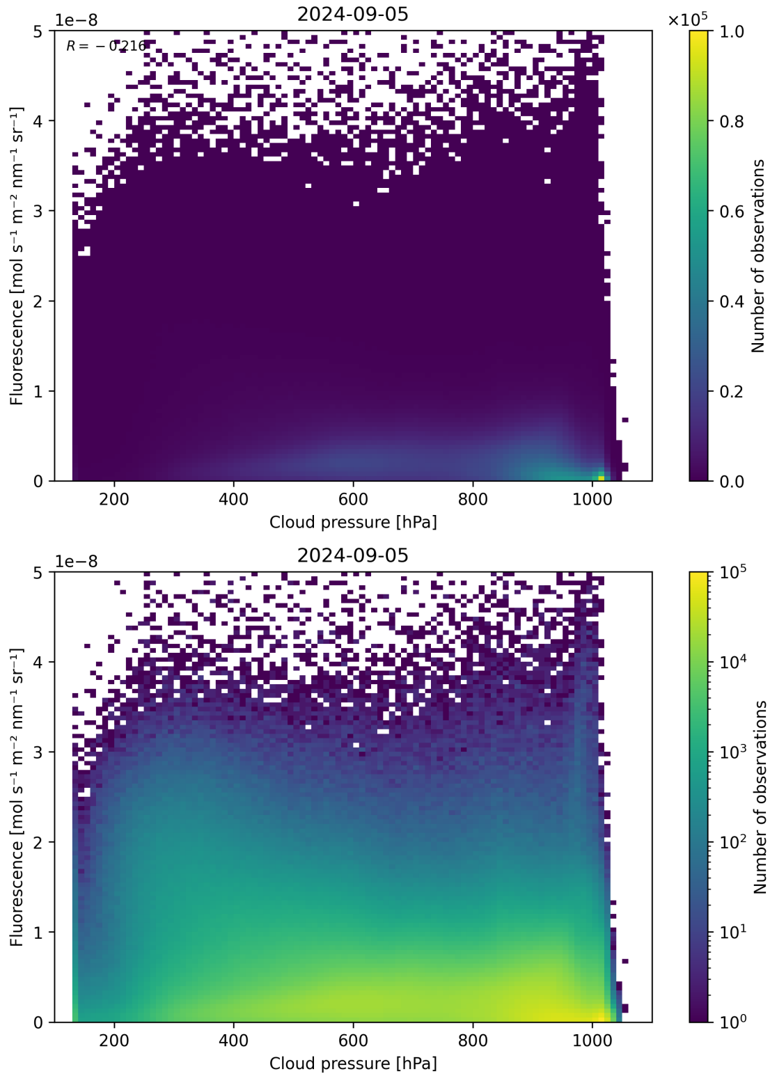
Figure 80: Scatter density plot of “Cloud pressure” against “Fluorescence” for 2024-09-04 to 2024-09-06.
