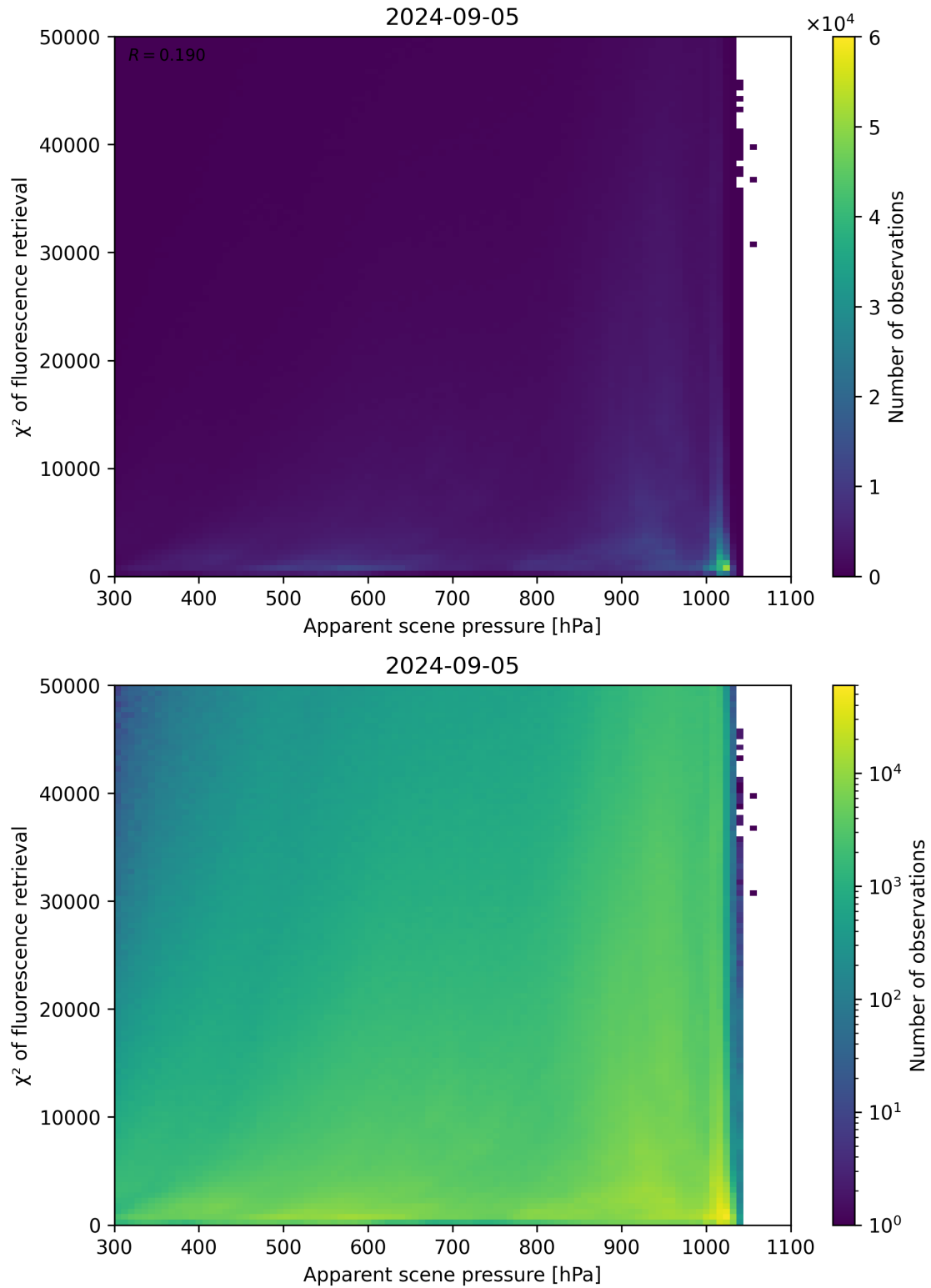
Figure 63: Scatter density plot of “Apparent scene pressure” against “ \chi^2 of fluorescence retrieval” for 2024-09-04 to 2024-09-06.
