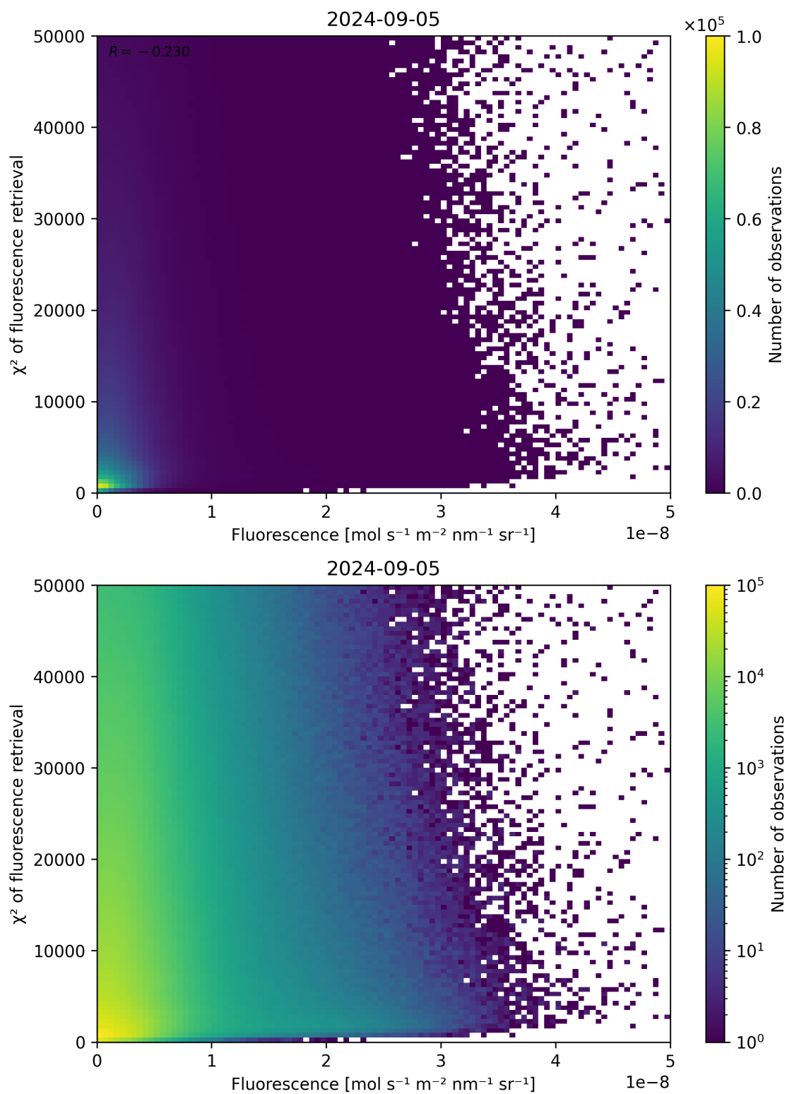
Figure 85: Scatter density plot of “Fluorescence” against “ \chi^2 of fluorescence retrieval” for 2024-09-04 to 2024-09-06.
