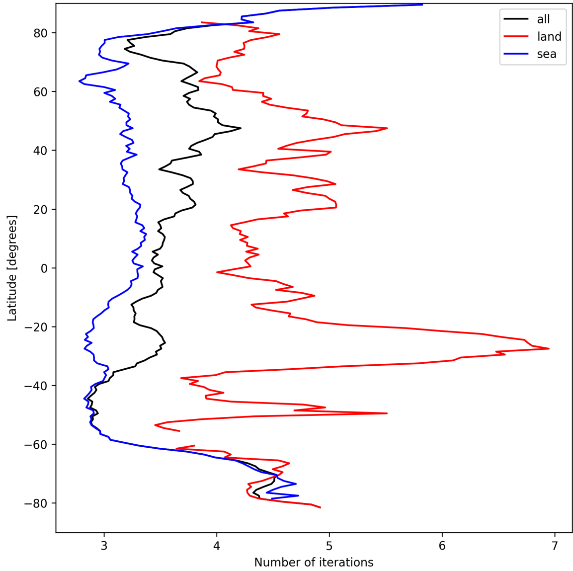
Figure 22: Zonal average of “Number of iterations” for 2024-09-04 to 2024-09-06.
