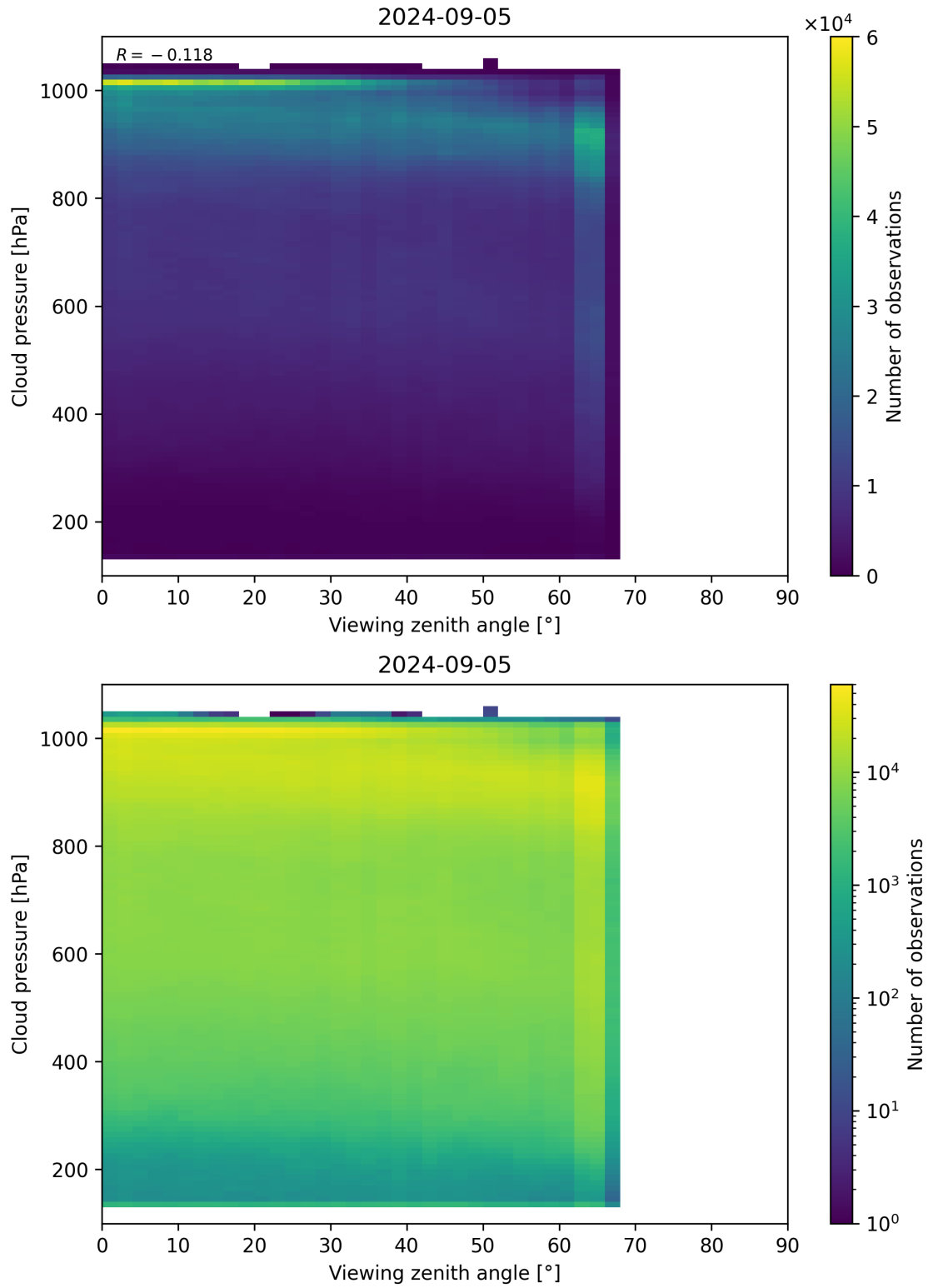
Figure 121: Scatter density plot of “Viewing zenith angle” against “Cloud pressure” for 2024-09-04 to 2024-09-06.
