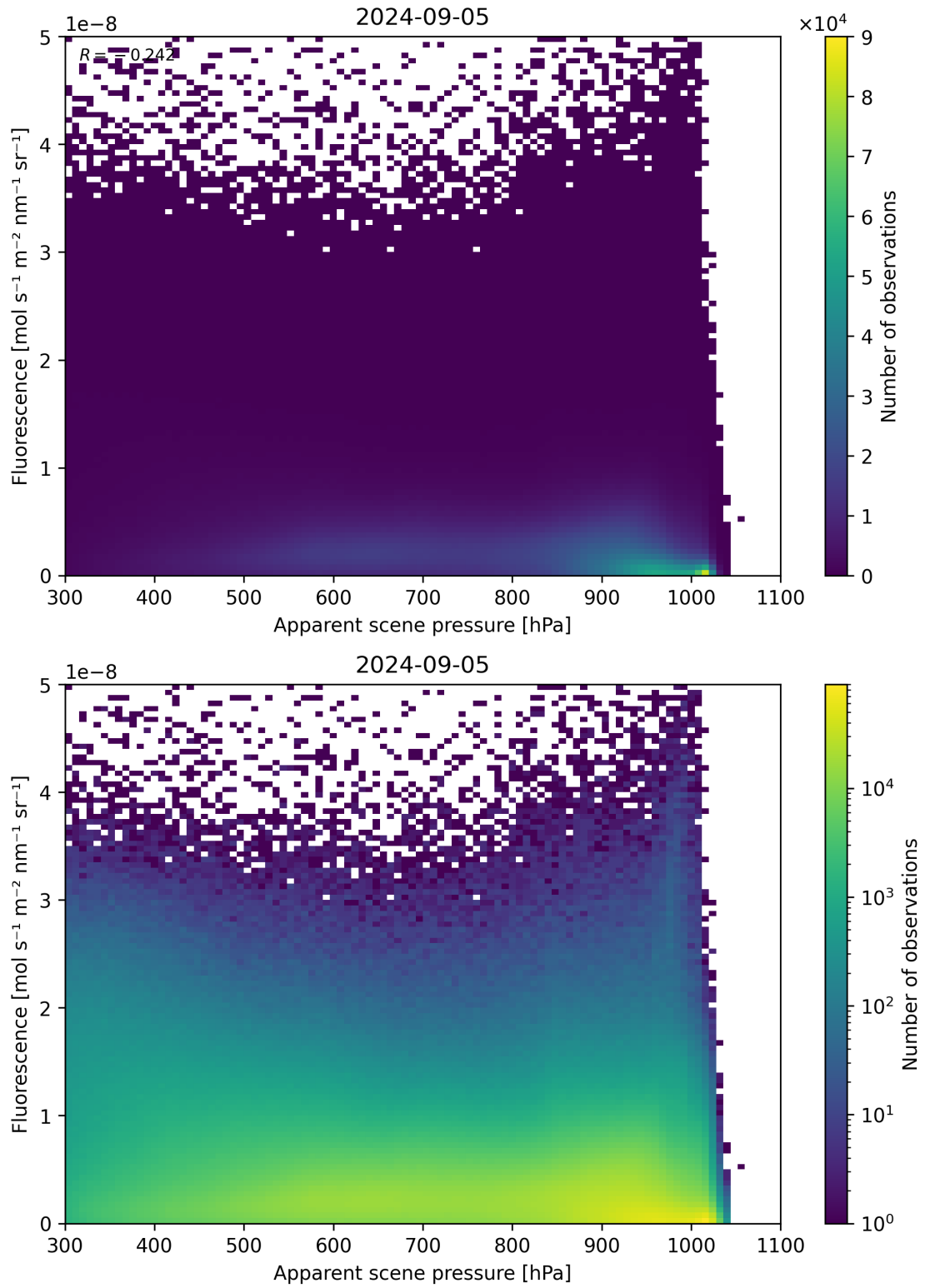
Figure 64: Scatter density plot of “Apparent scene pressure” against “Fluorescence” for 2024-09-04 to 2024-09-06.
