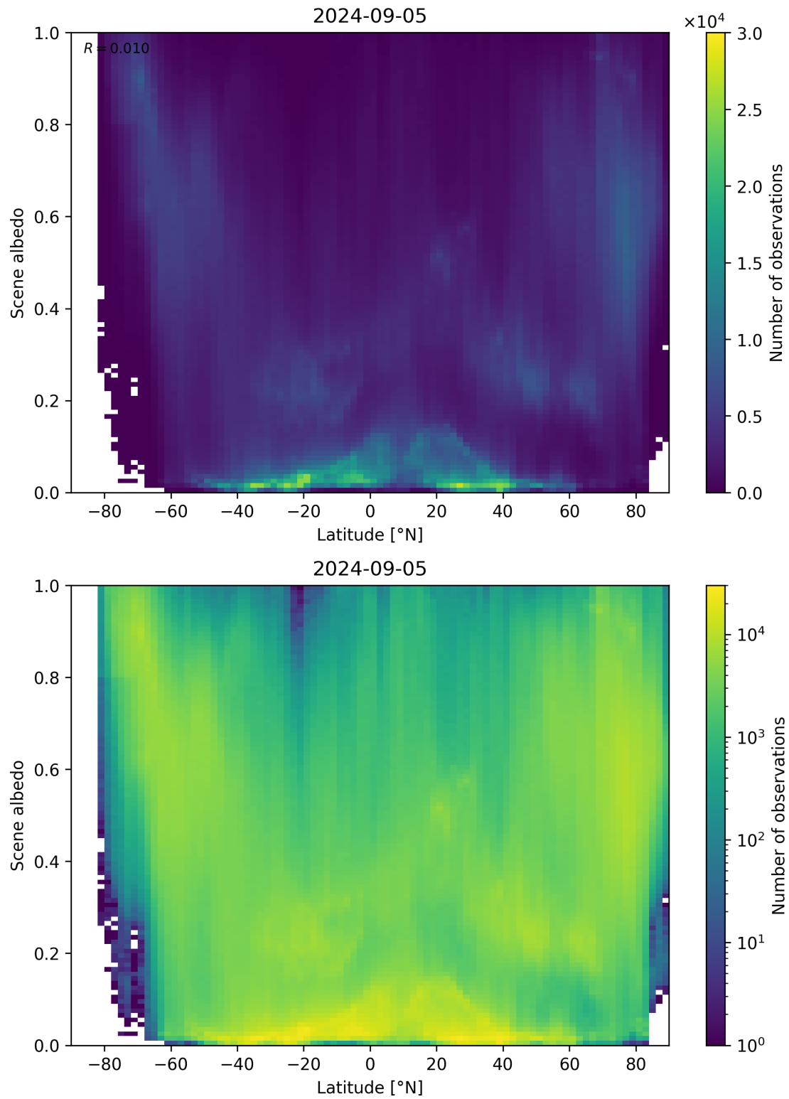
Figure 95: Scatter density plot of “Latitude” against “Scene albedo” for 2024-09-04 to 2024-09-06.
