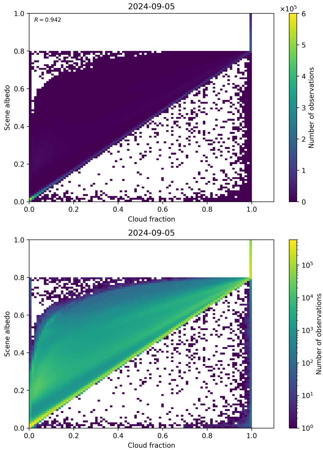
Figure 75: Scatter density plot of “Cloud fraction” against “Scene albedo” for 2024-09-04 to 2024-09-06.
