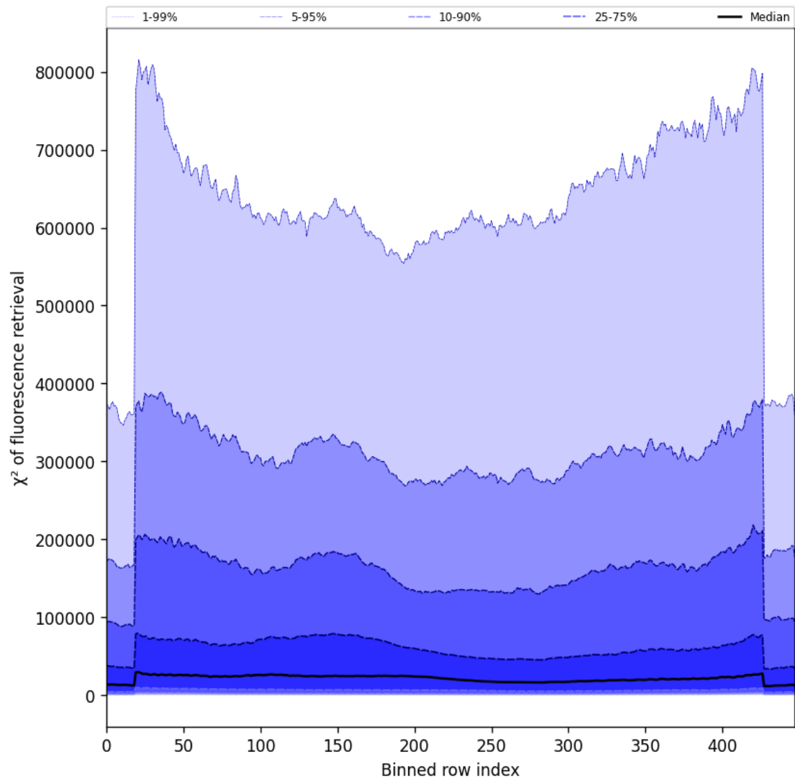
Figure 59: Along track statistics of “ \chi^2 of fluorescence retrieval” for 2024-09-04 to 2024-09-06
