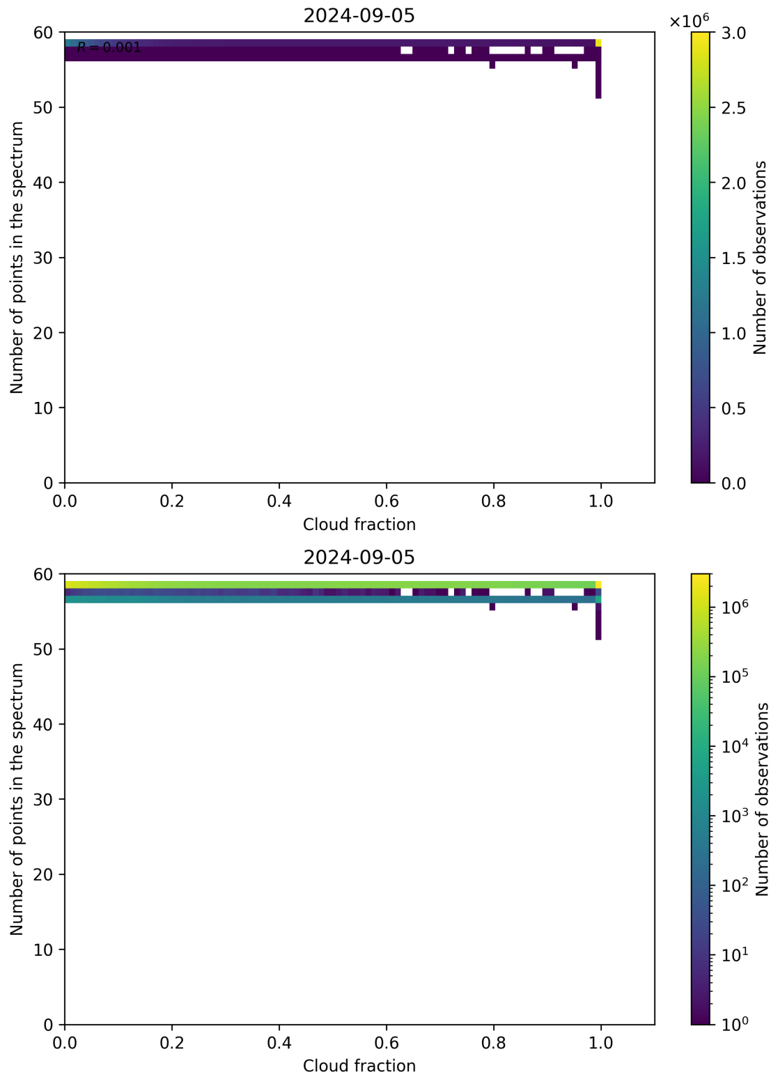
Figure 74: Scatter density plot of “Cloud fraction” against “Number of points in the spectrum” for 2024-09-04 to 2024-09-06.
