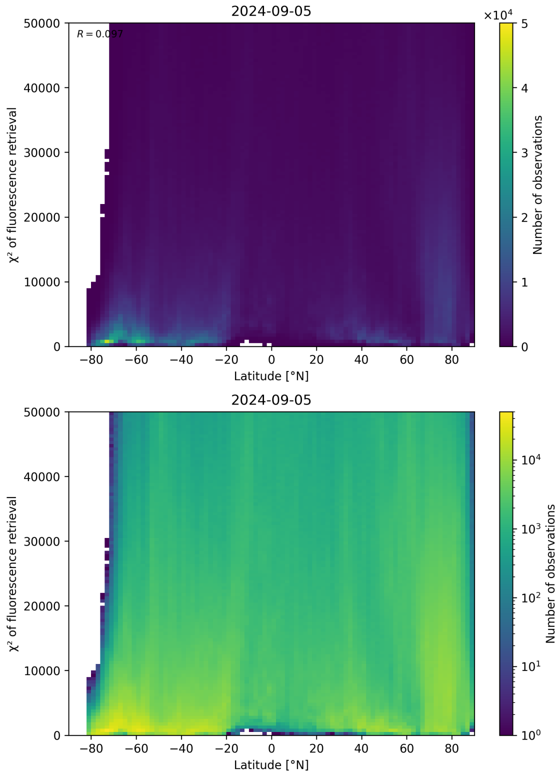
Figure 89: Scatter density plot of “Latitude” against “ \chi^2 of fluorescence retrieval” for 2024-09-04 to 2024-09-06.
