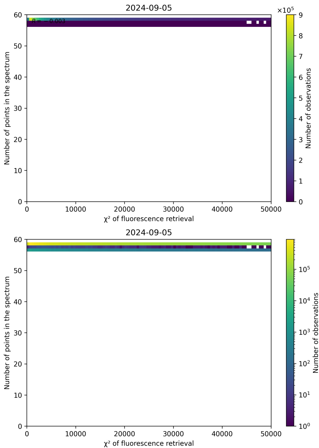
Figure 68: Scatter density plot of " \chi^2 of fluorescence retrieval" against "Number of points in the spectrum" for 2024-09-04 to 2024-09-06.
