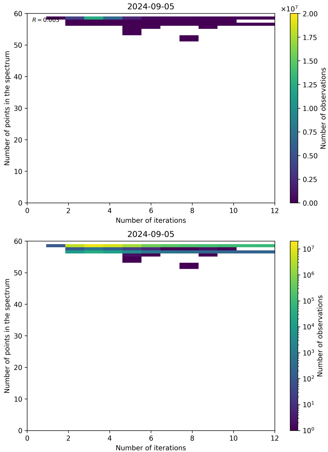
Figure 99: Scatter density plot of “Number of iterations” against “Number of points in the spectrum” for 2024-09-04 to 2024-09-06.
