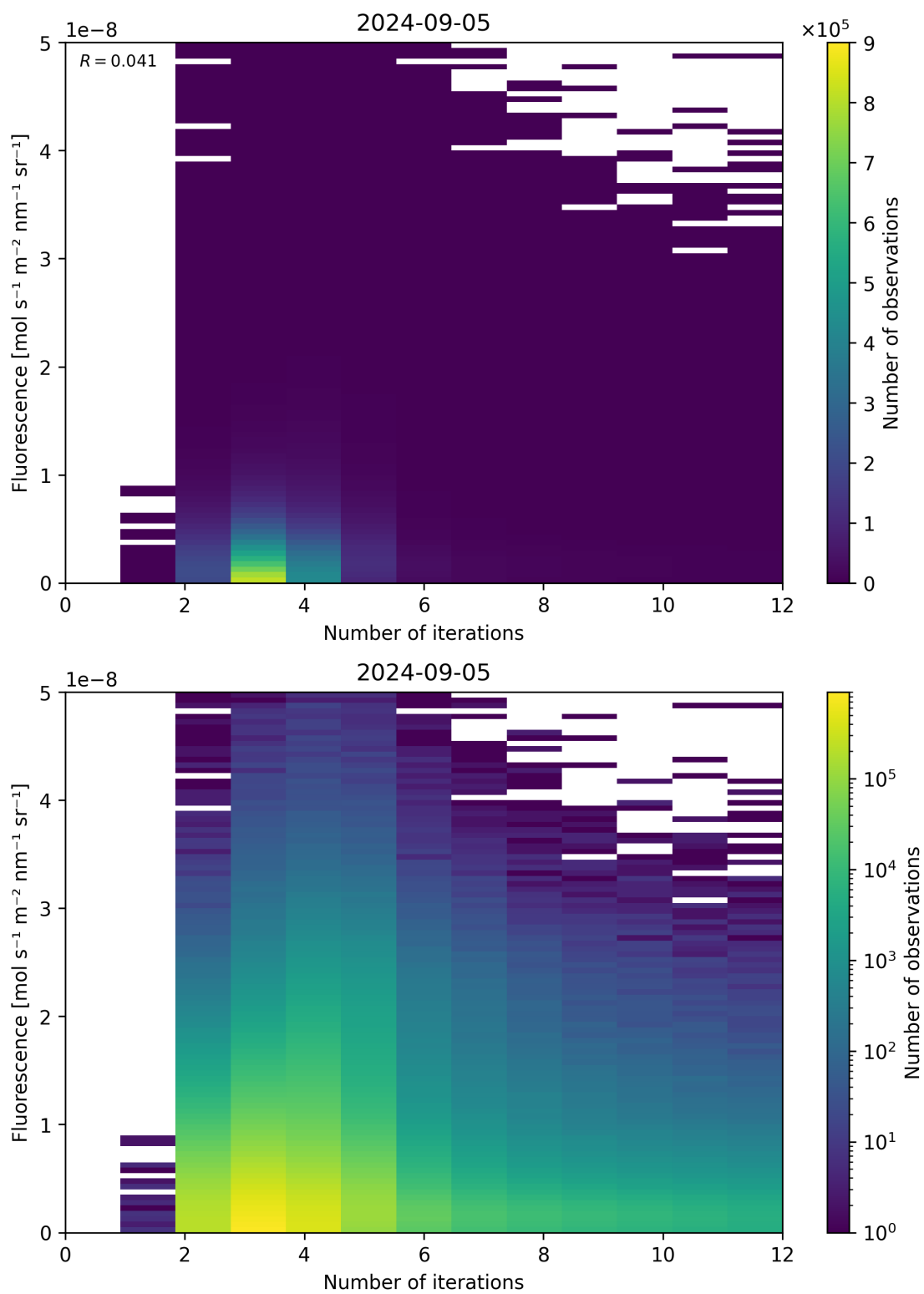
Figure 98: Scatter density plot of “Number of iterations” against “Fluorescence” for 2024-09-04 to 2024-09-06.
