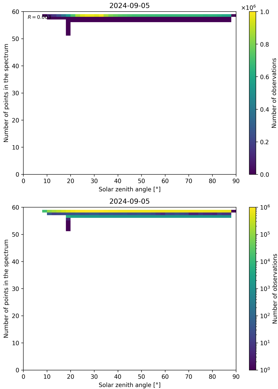
Figure 115: Scatter density plot of “Solar zenith angle” against “Number of points in the spectrum” for 2024-09-04 to 2024-09-06.
