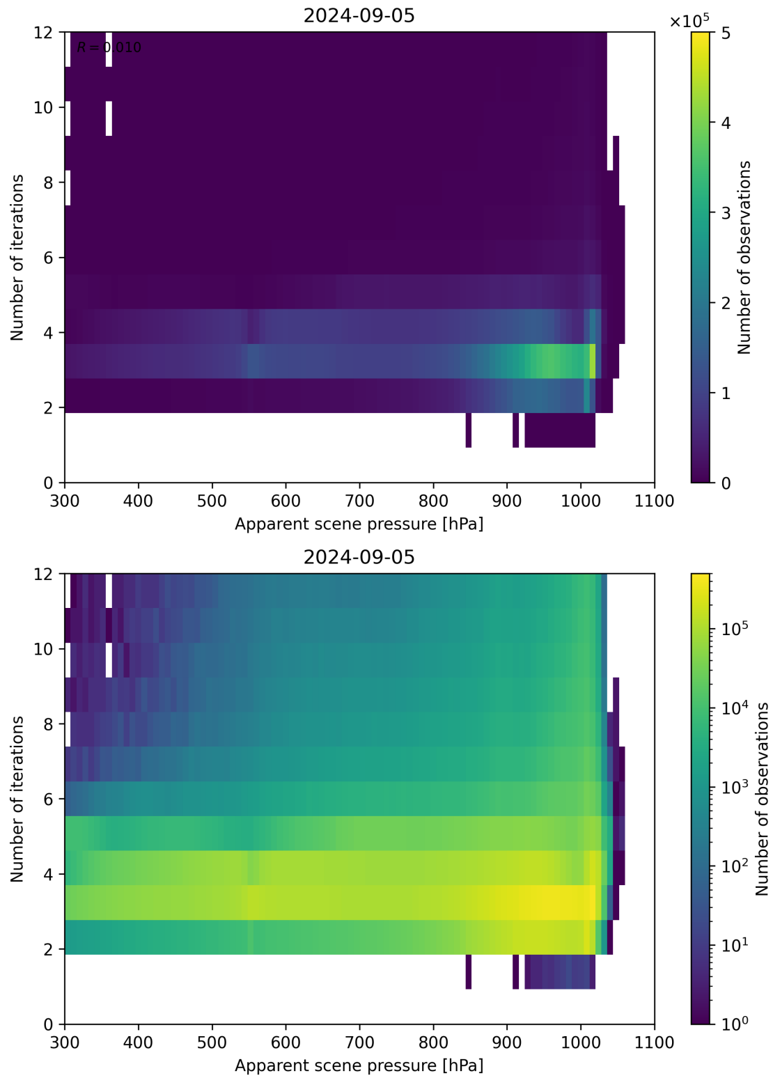
Figure 65: Scatter density plot of “Apparent scene pressure” against “Number of iterations” for 2024-09-04 to 2024-09-06.
