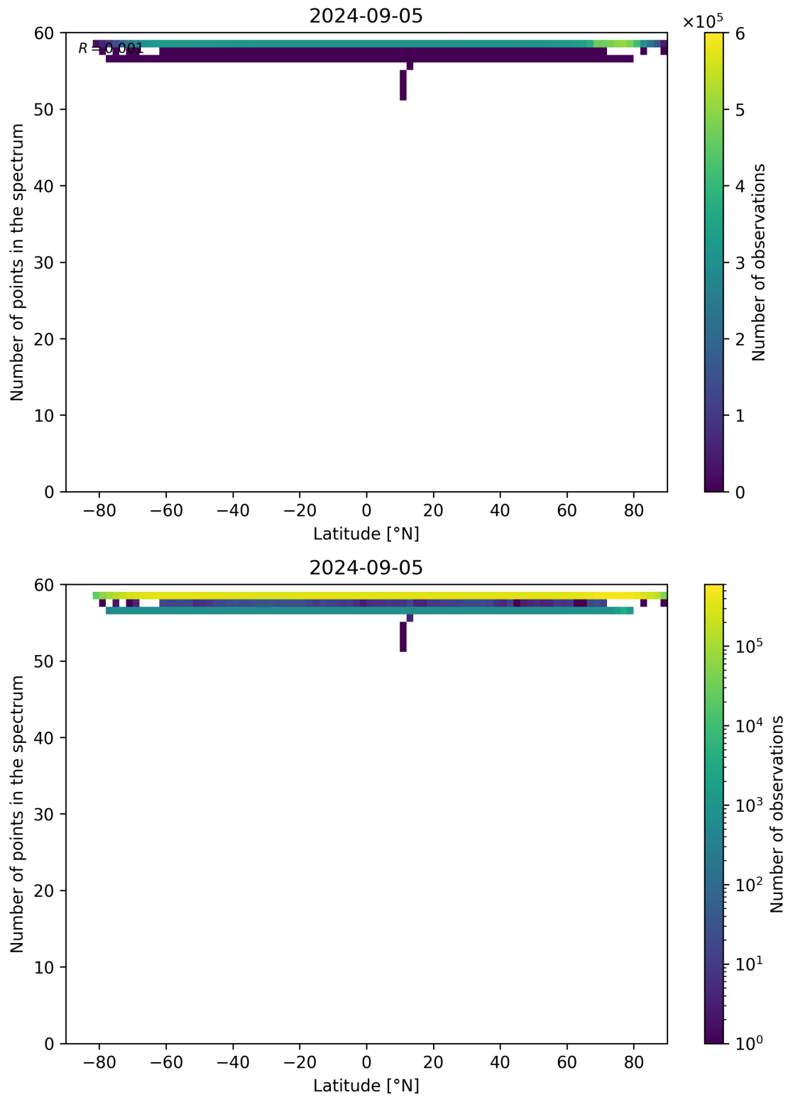
Figure 94: Scatter density plot of “Latitude” against “Number of points in the spectrum” for 2024-09-04 to 2024-09-06.
