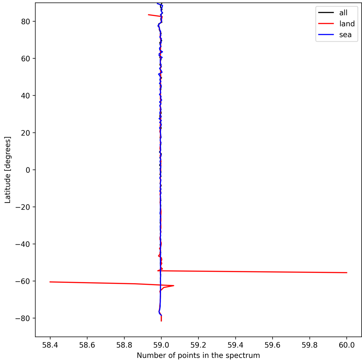
Figure 27: Zonal average of “Number of points in the spectrum” for 2024-09-04 to 2024-09-06.
