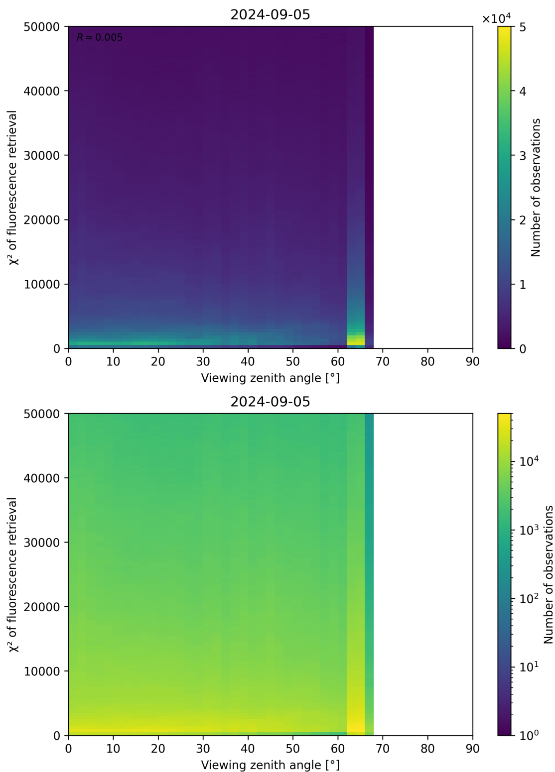
Figure 119: Scatter density plot of “Viewing zenith angle” against “ \chi^2 of fluorescence retrieval” for 2024-09-04 to 2024-09-06.
