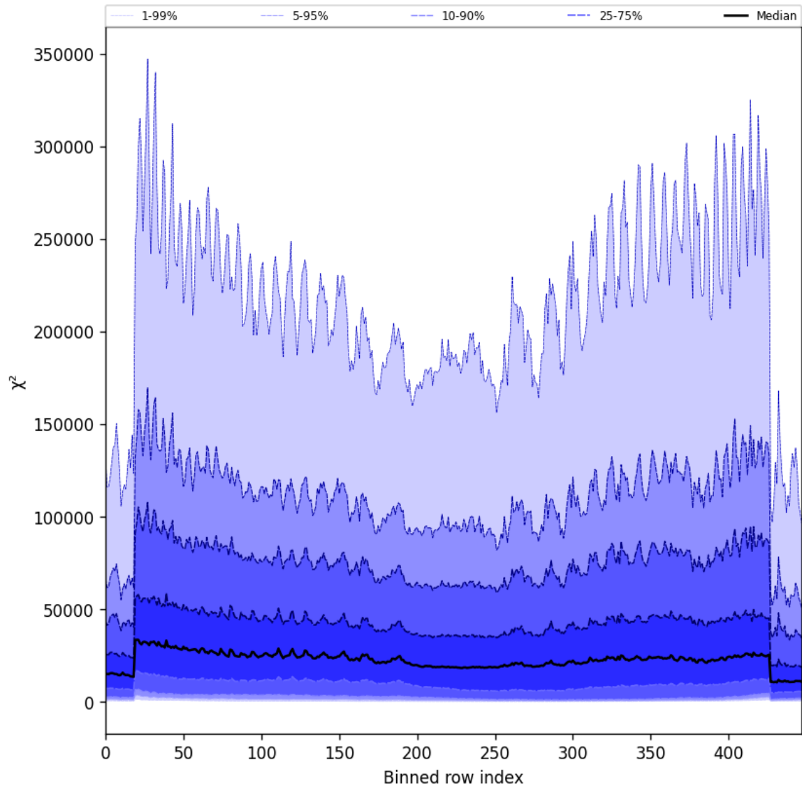
Figure 55: Along track statistics of “ \chi^2 ” for 2024-09-04 to 2024-09-06
