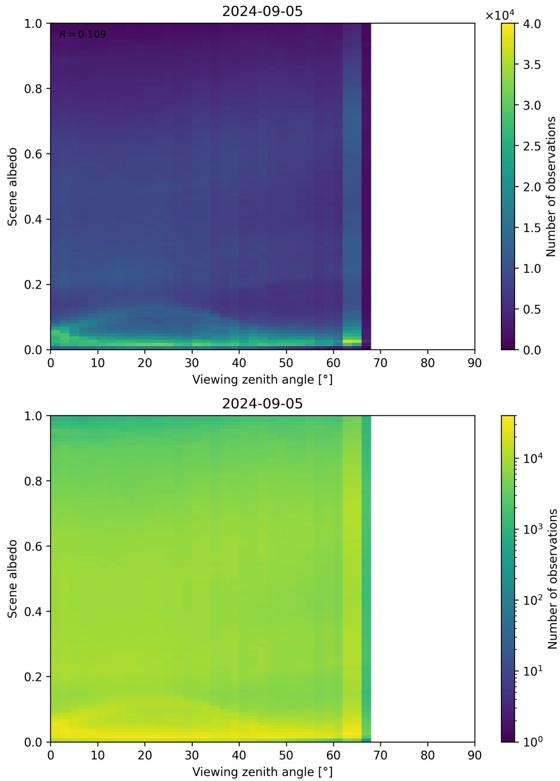
Figure 126: Scatter density plot of “Viewing zenith angle” against “Scene albedo” for 2024-09-04 to 2024-09-06.
