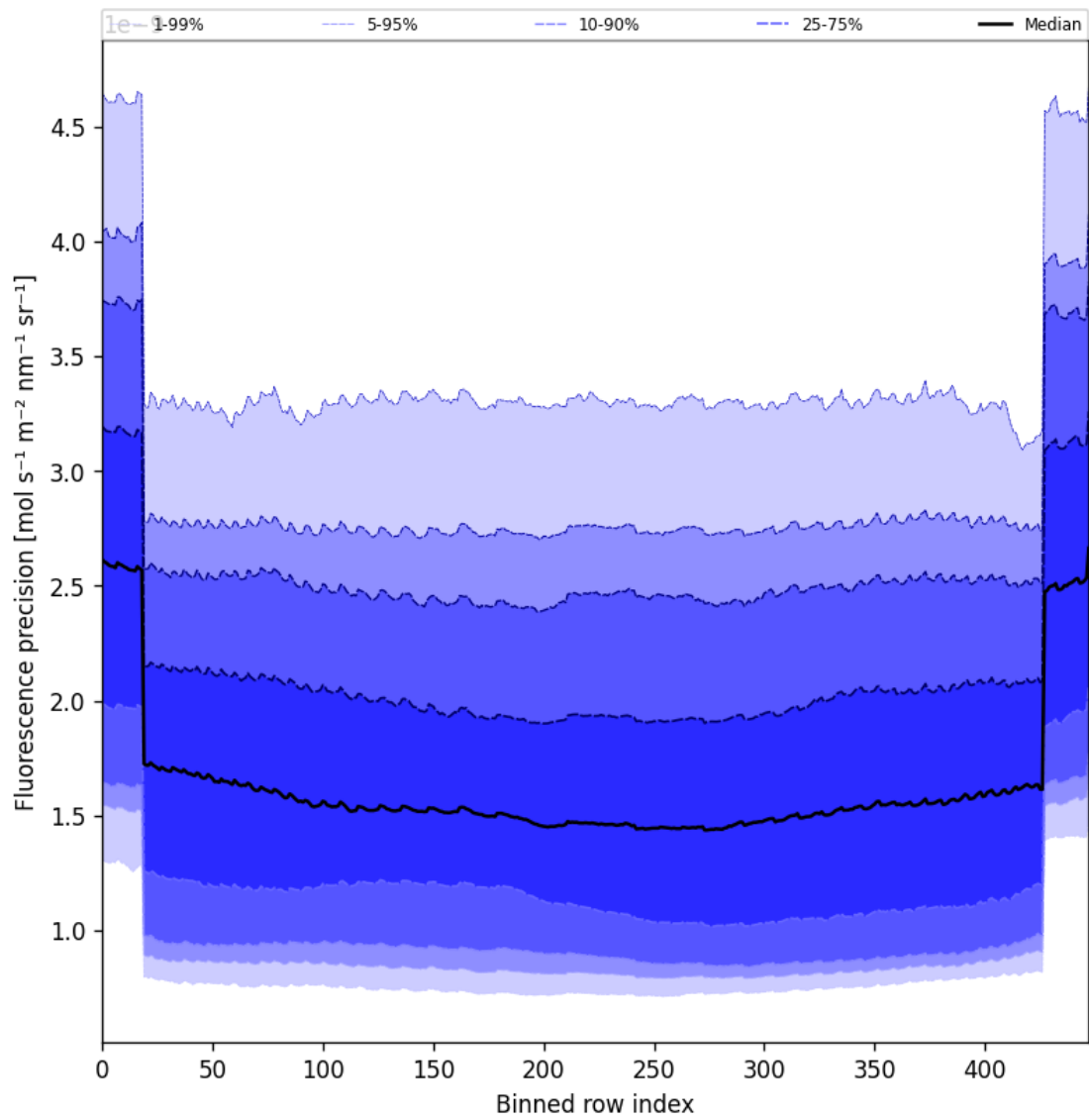
Figure 58: Along track statistics of “Fluorescence precision” for 2024-09-04 to 2024-09-06
