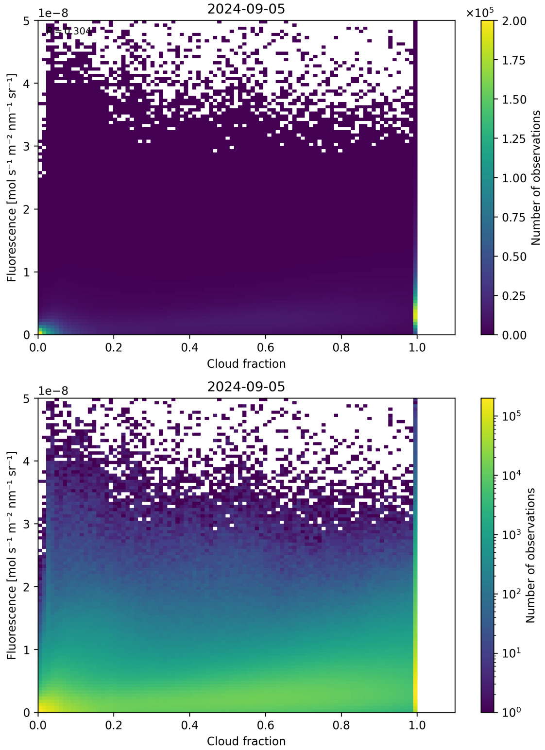
Figure 72: Scatter density plot of “Cloud fraction” against “Fluorescence” for 2024-09-04 to 2024-09-06.
