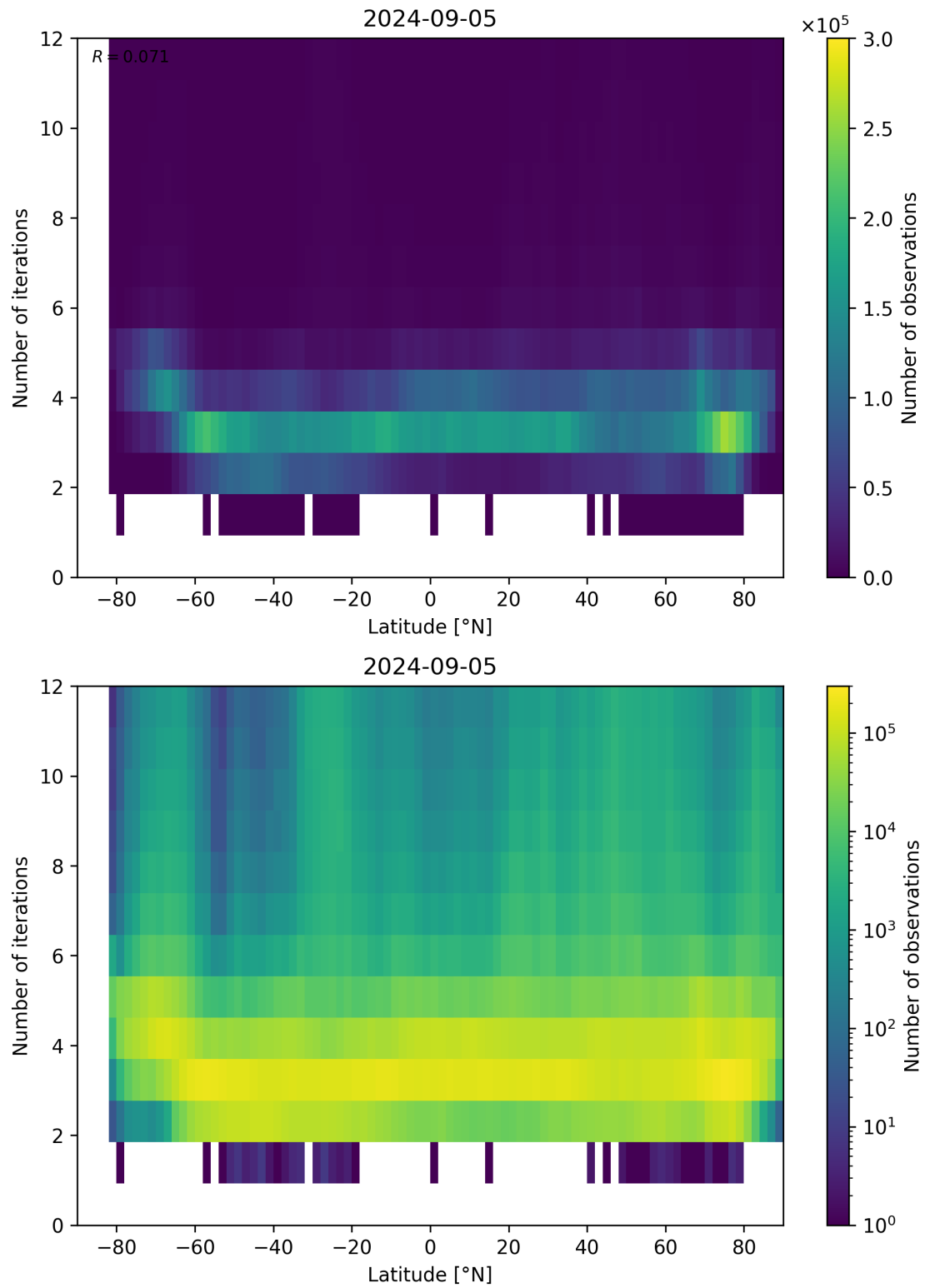
Figure 93: Scatter density plot of “Latitude” against “Number of iterations” for 2024-09-04 to 2024-09-06.
