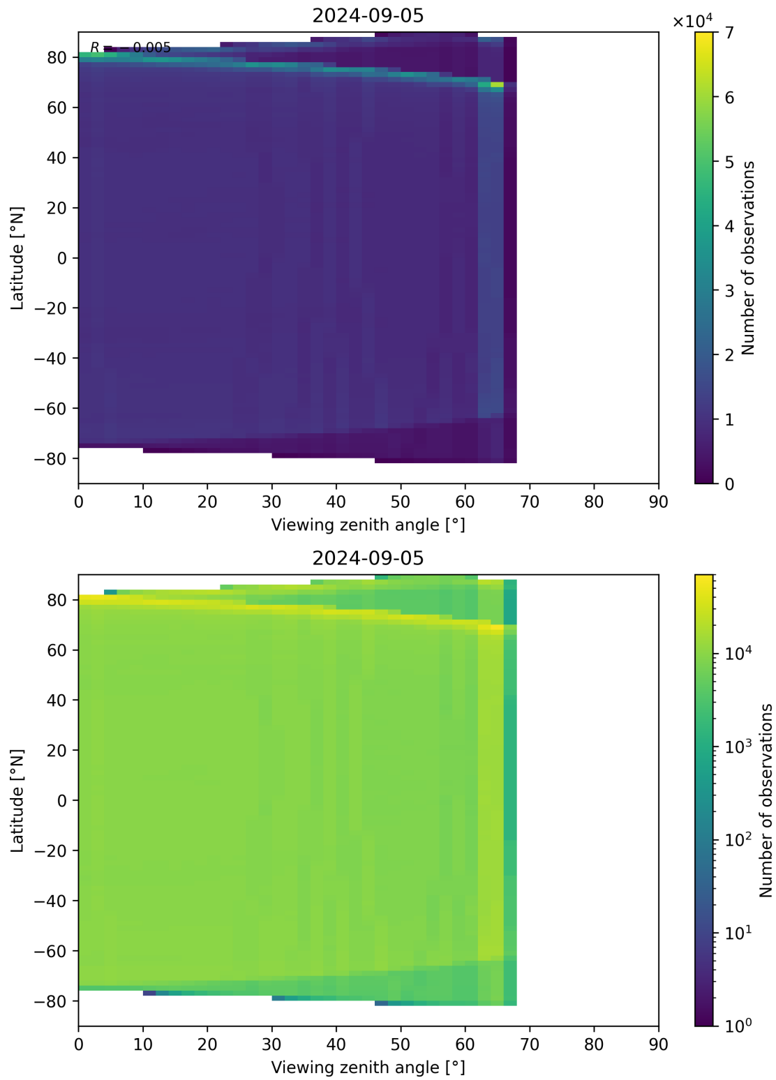
Figure 123: Scatter density plot of “Viewing zenith angle” against “Latitude” for 2024-09-04 to 2024-09-06.
