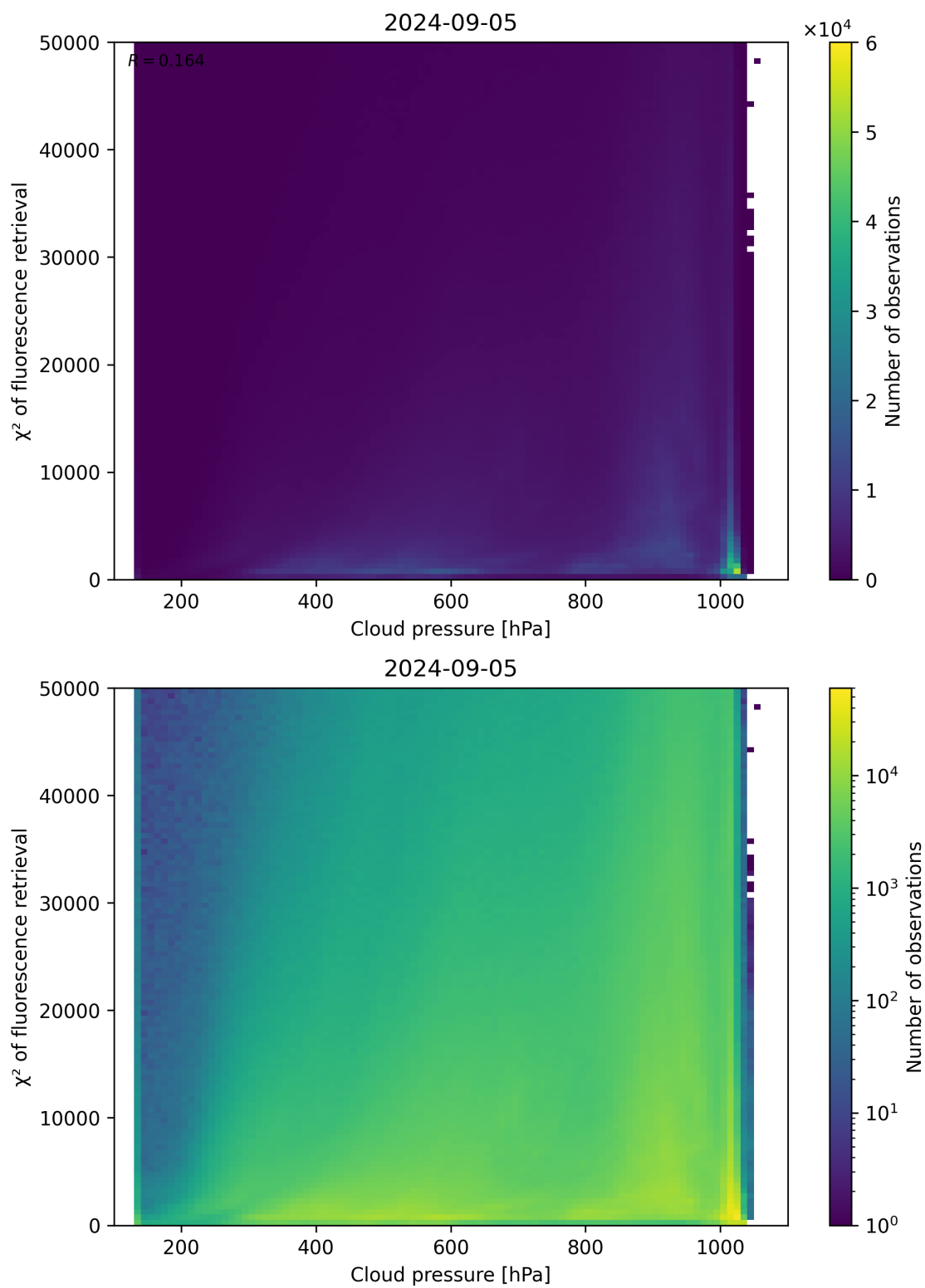
Figure 78: Scatter density plot of “Cloud pressure” against “ \chi^2 of fluorescence retrieval” for 2024-09-04 to 2024-09-06.
