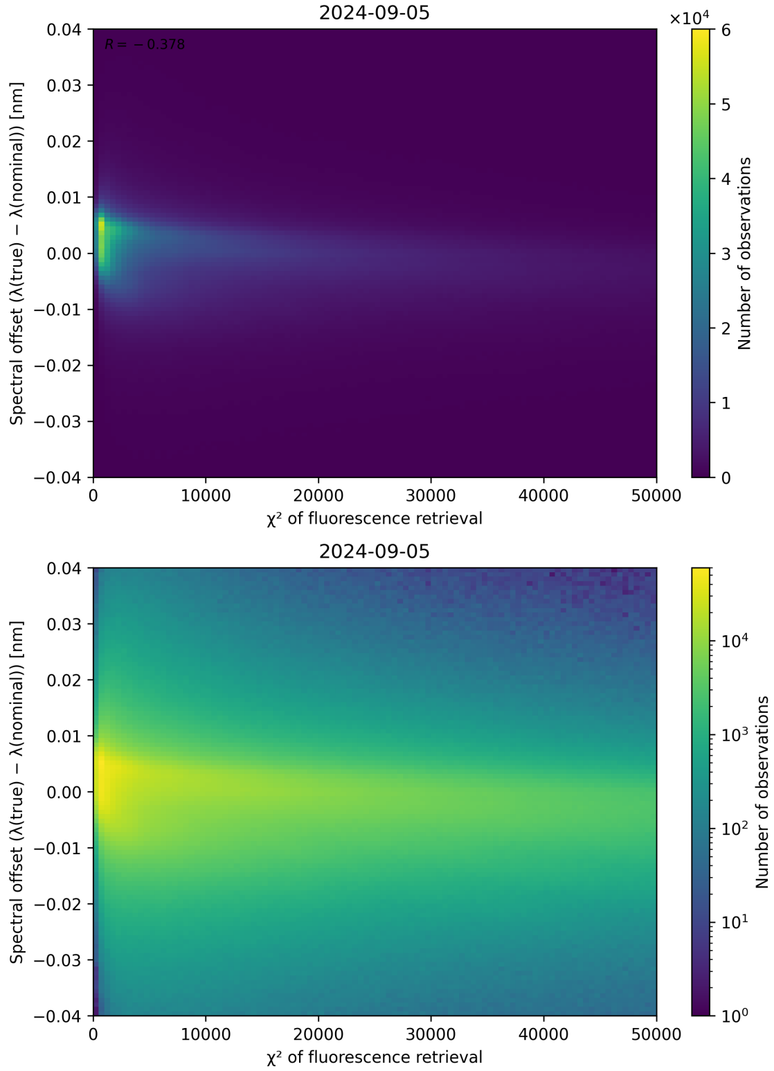
Figure 69: Scatter density plot of “ \chi^2 of fluorescence retrieval” against “Spectral offset ( \lambda_{\text{true}} - \lambda_{\text{nominal}} )” for 2024-09-04 to 2024-09-06.
