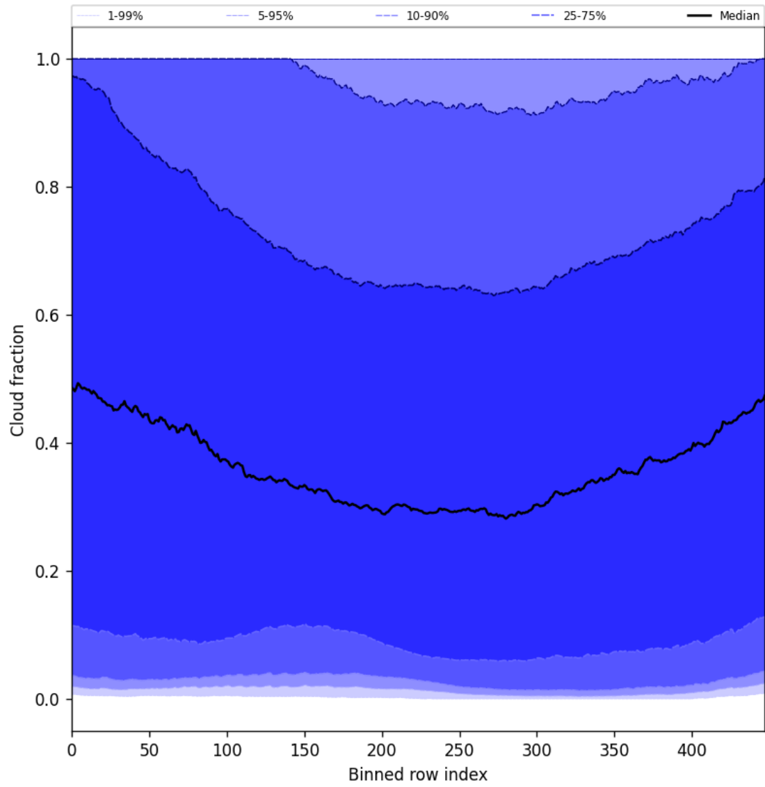
Figure 49: Along track statistics of “Cloud fraction” for 2024-09-04 to 2024-09-06
