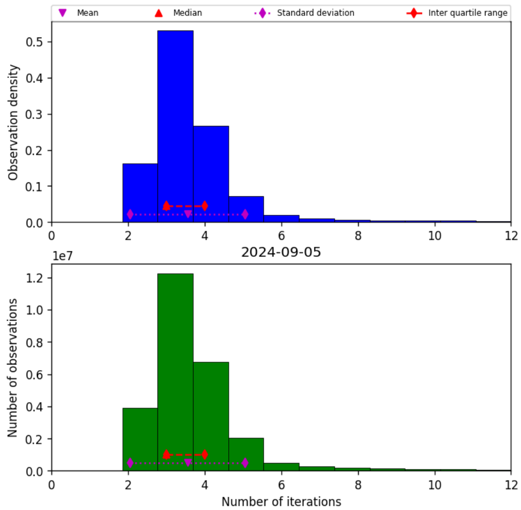
Figure 39: Histogram of “Number of iterations” for 2024-09-04 to 2024-09-06
