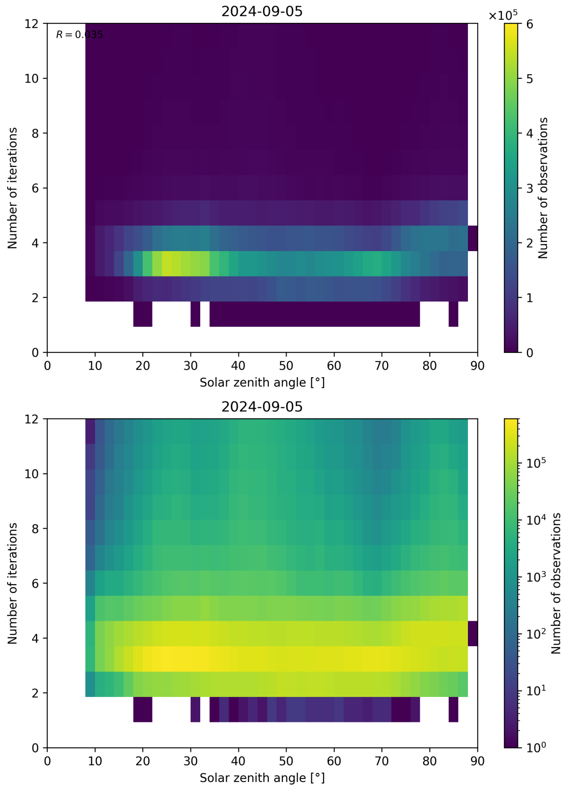
Figure 114: Scatter density plot of “Solar zenith angle” against “Number of iterations” for 2024-09-04 to 2024-09-06.
