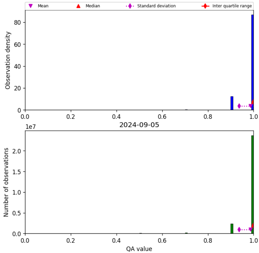
Figure 29: Histogram of “QA value” for 2024-09-04 to 2024-09-06
