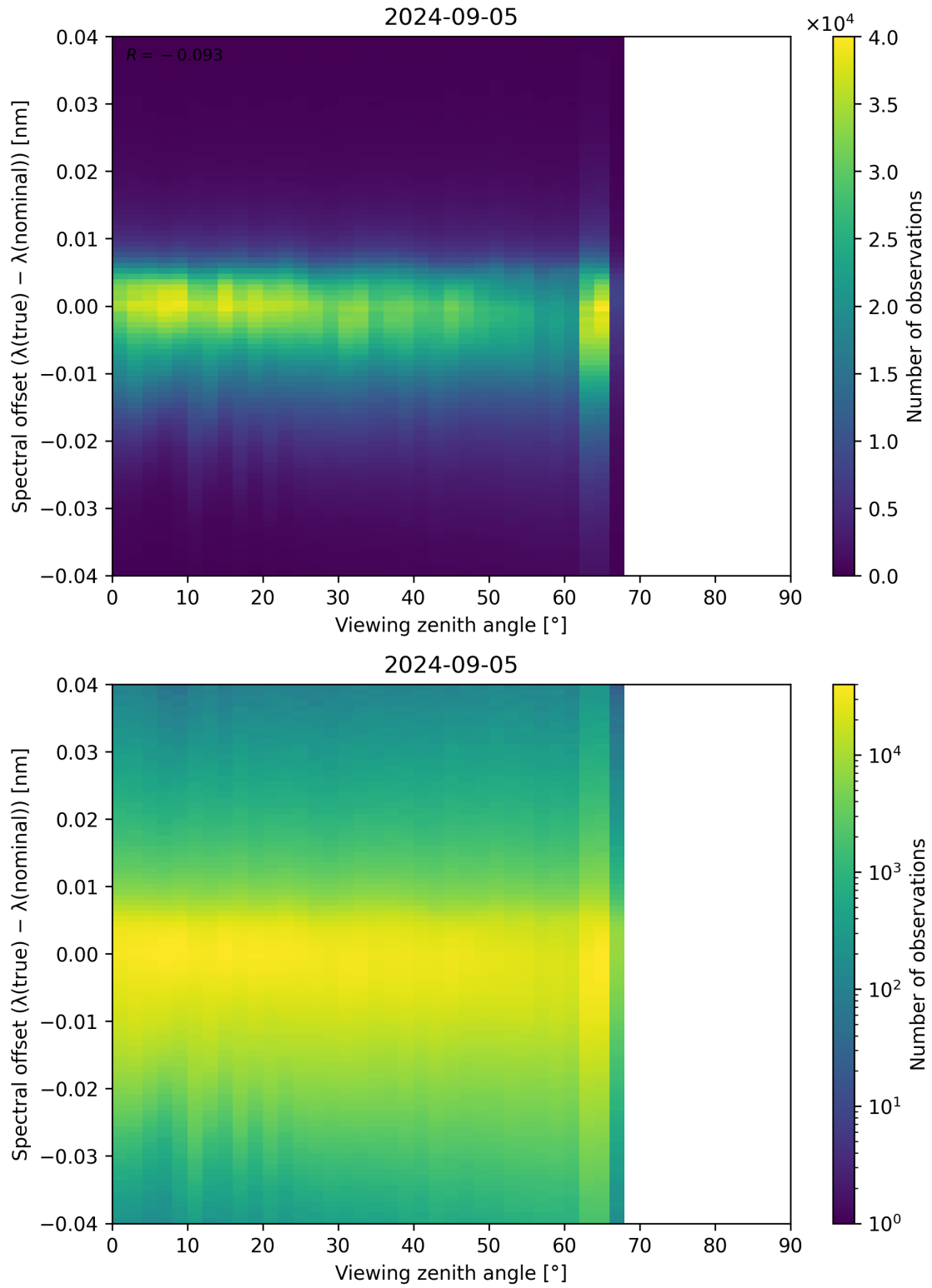
Figure 128: Scatter density plot of “Viewing zenith angle” against “Spectral offset ( \lambda_{\text{true}} - \lambda_{\text{nominal}} )” for 2024-09-04 to 2024-09-06.
