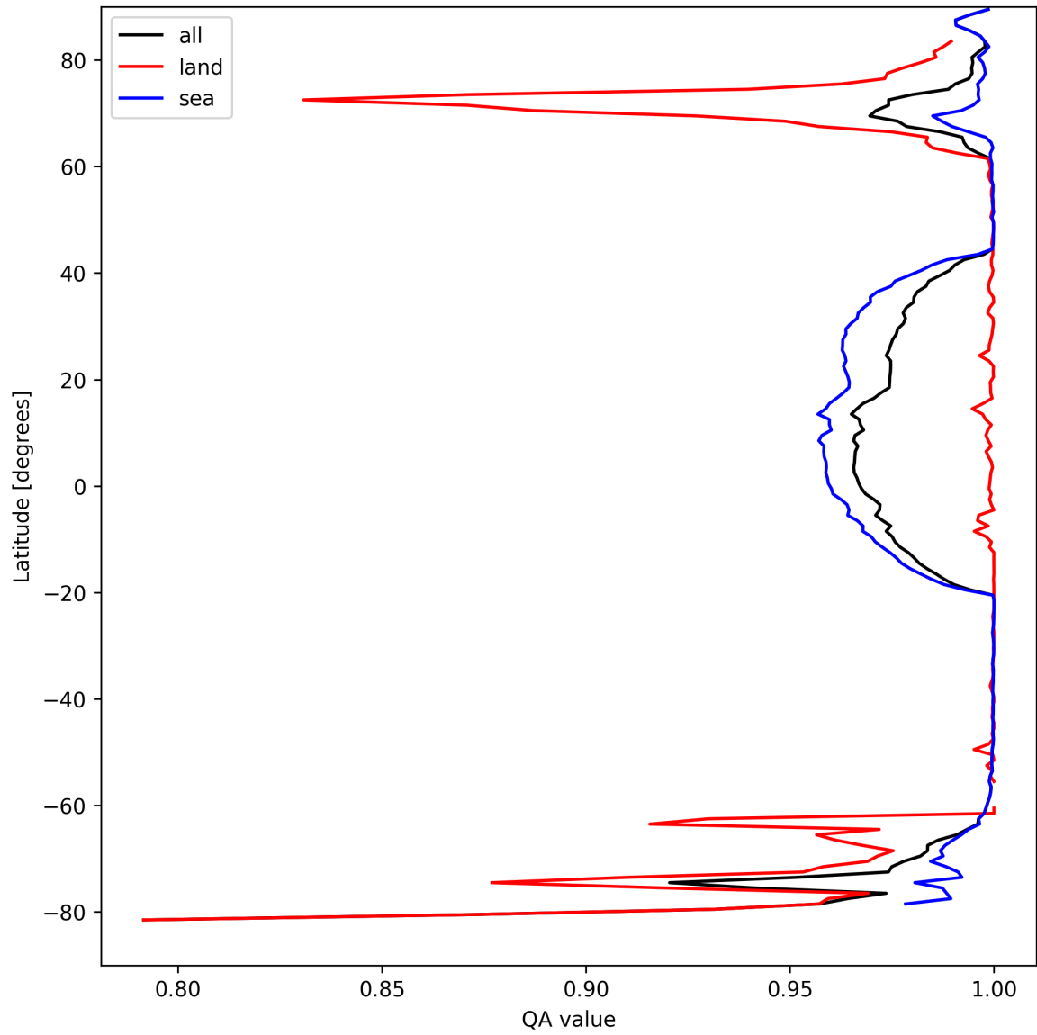
Figure 12: Zonal average of “QA value” for 2024-09-04 to 2024-09-06.
