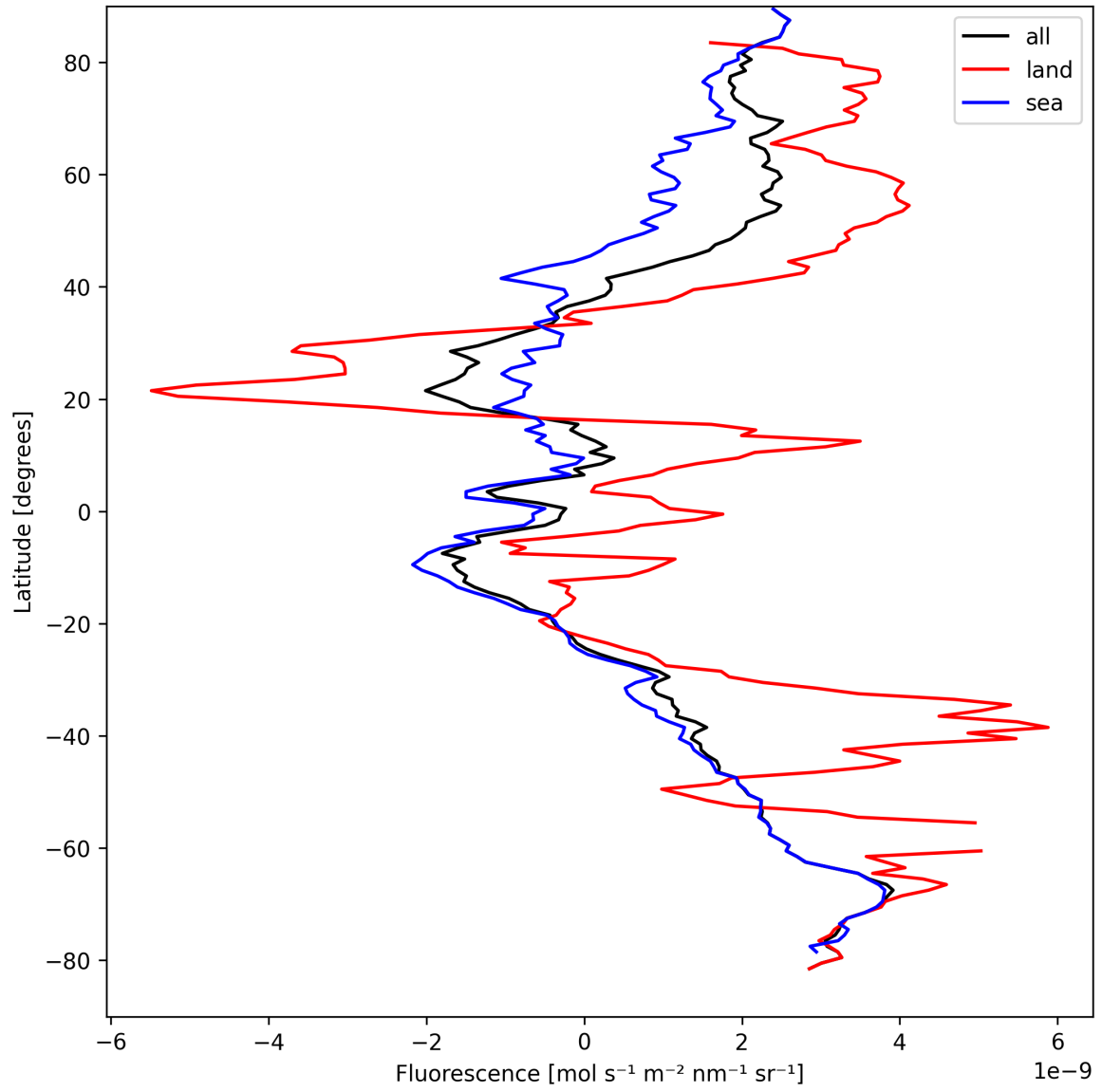
Figure 23: Zonal average of “Fluorescence” for 2024-09-04 to 2024-09-06.
