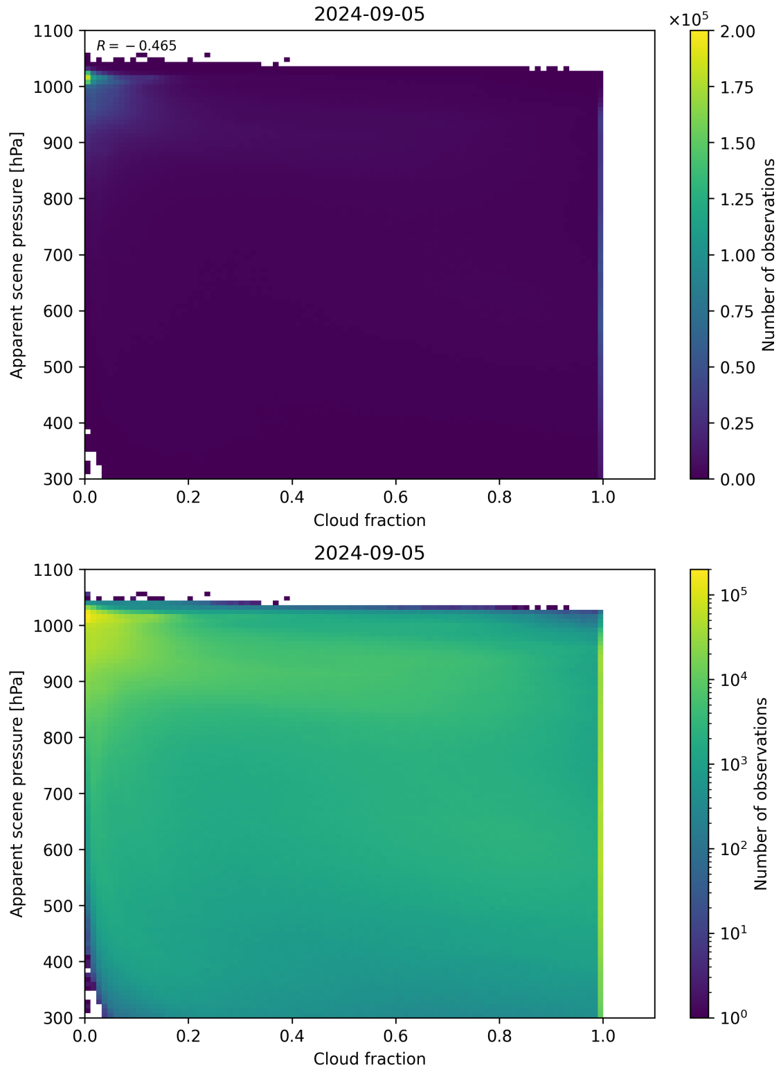
Figure 70: Scatter density plot of “Cloud fraction” against “Apparent scene pressure” for 2024-09-04 to 2024-09-06.
