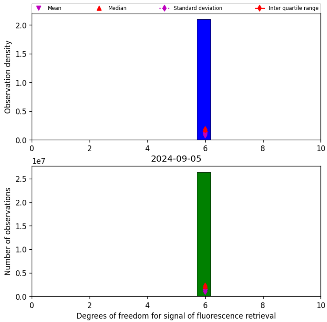
Figure 43: Histogram of "Degrees of freedom for signal of fluorescence retrieval" for 2024-09-04 to 2024-09-06
