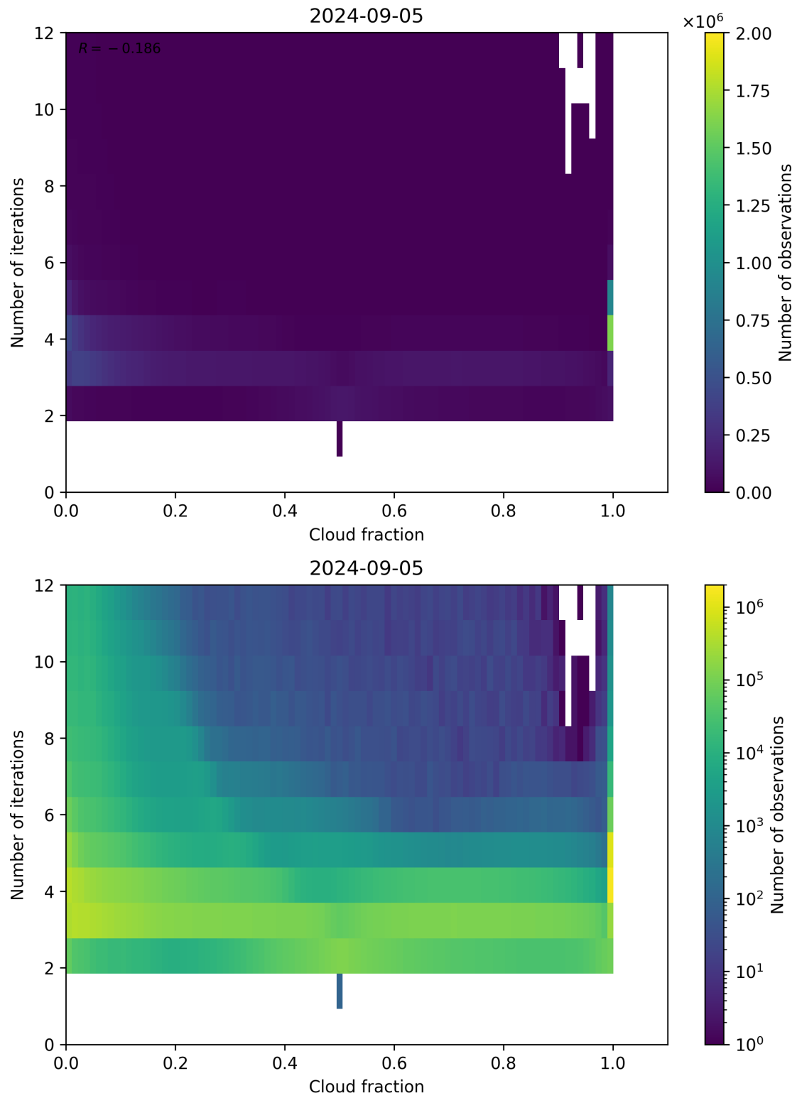
Figure 73: Scatter density plot of “Cloud fraction” against “Number of iterations” for 2024-09-04 to 2024-09-06.
