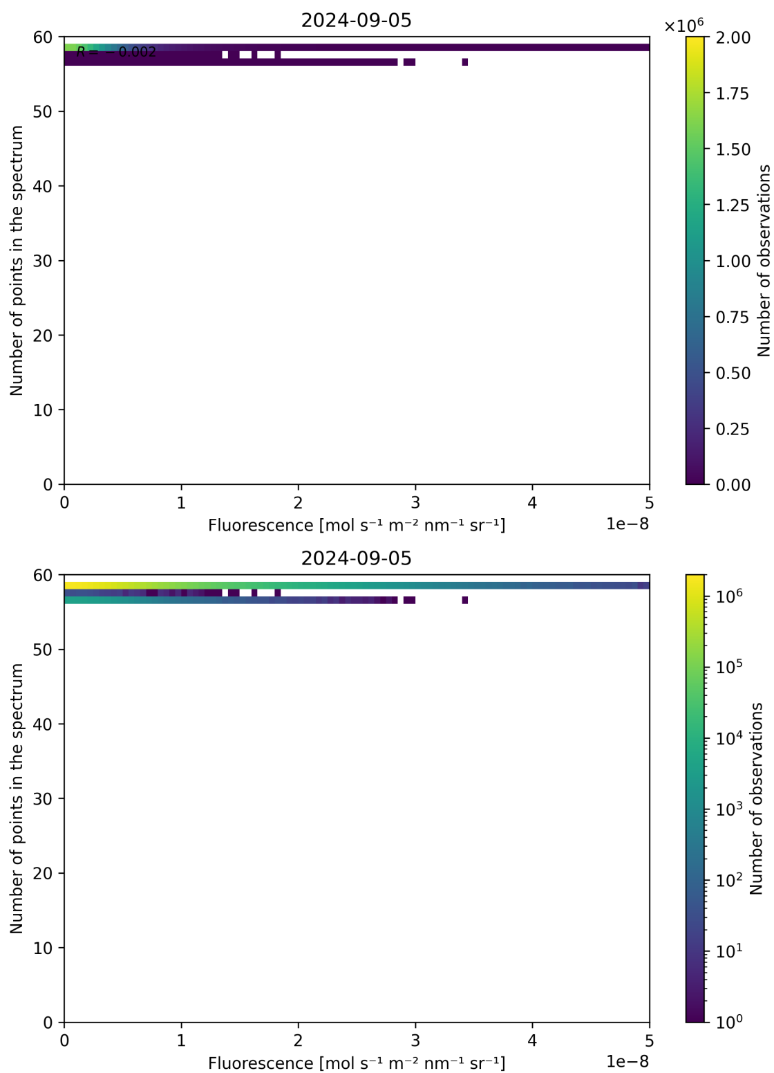
Figure 86: Scatter density plot of “Fluorescence” against “Number of points in the spectrum” for 2024-09-04 to 2024-09-06.
