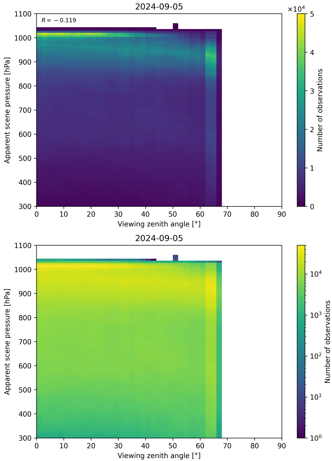
Figure 118: Scatter density plot of “Viewing zenith angle” against “Apparent scene pressure” for 2024-09-04 to 2024-09-06.
