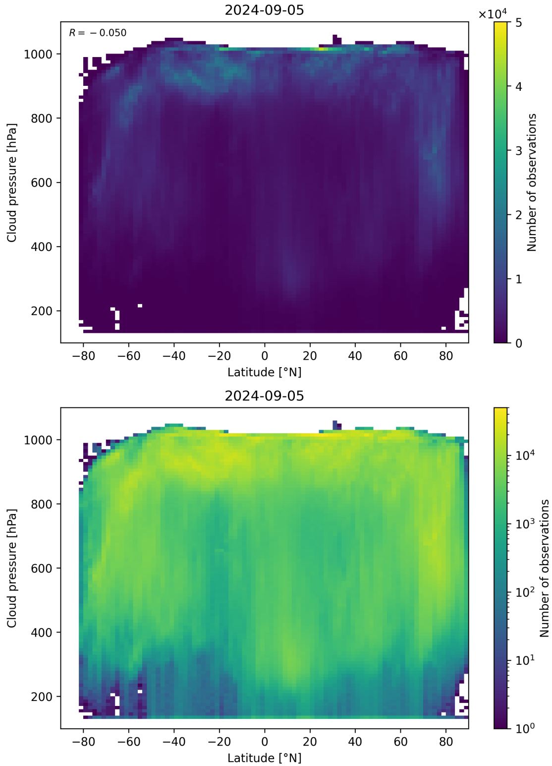
Figure 91: Scatter density plot of “Latitude” against “Cloud pressure” for 2024-09-04 to 2024-09-06.
