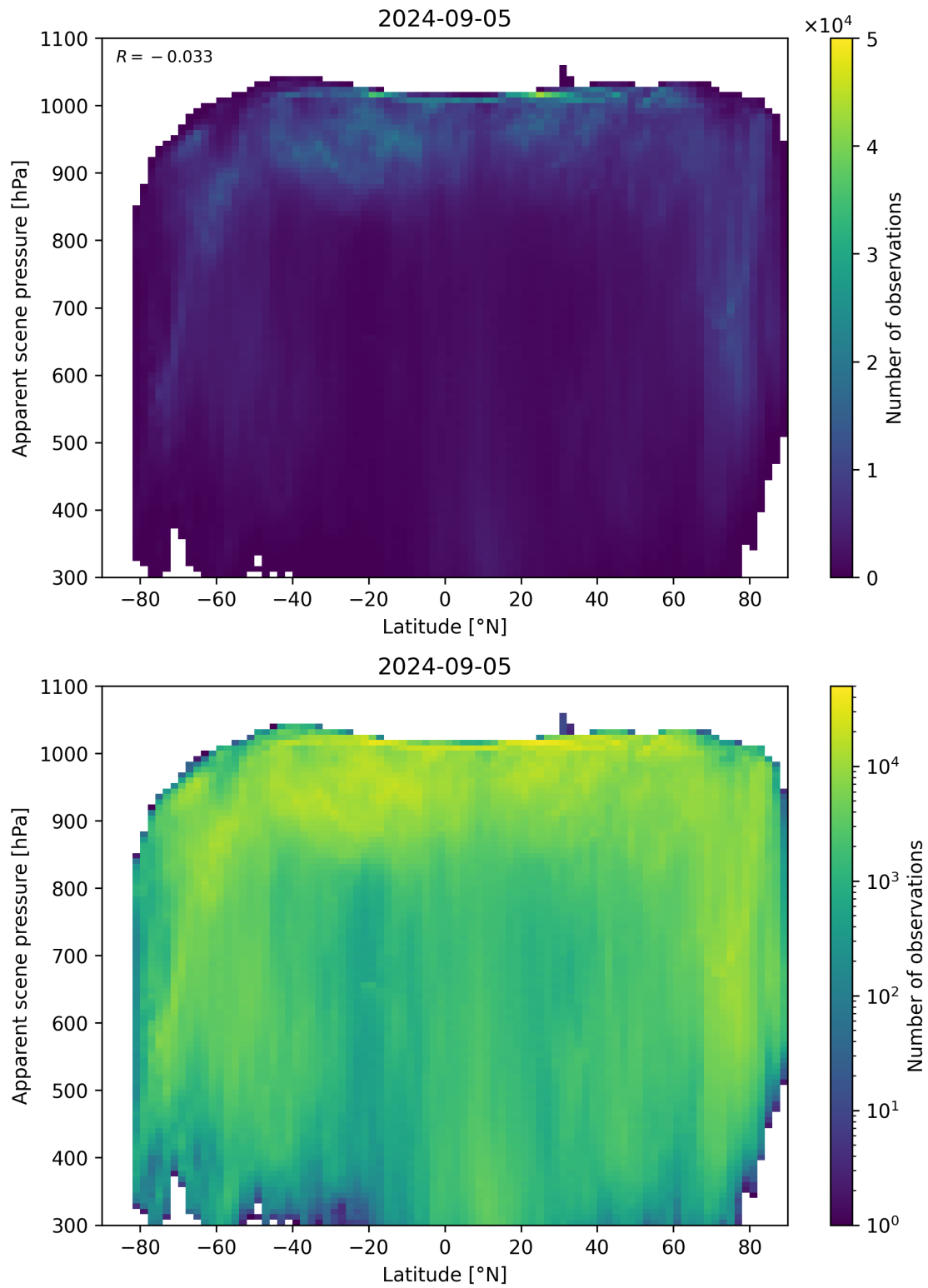
Figure 88: Scatter density plot of “Latitude” against “Apparent scene pressure” for 2024-09-04 to 2024-09-06.
