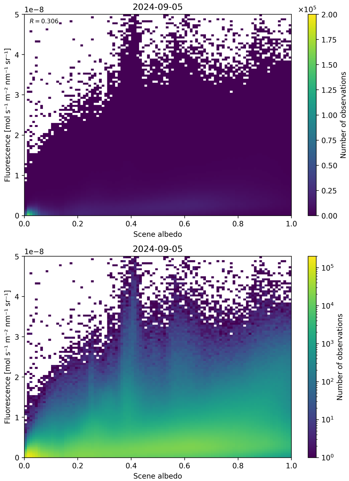
Figure 104: Scatter density plot of “Scene albedo” against “Fluorescence” for 2024-09-04 to 2024-09-06.
